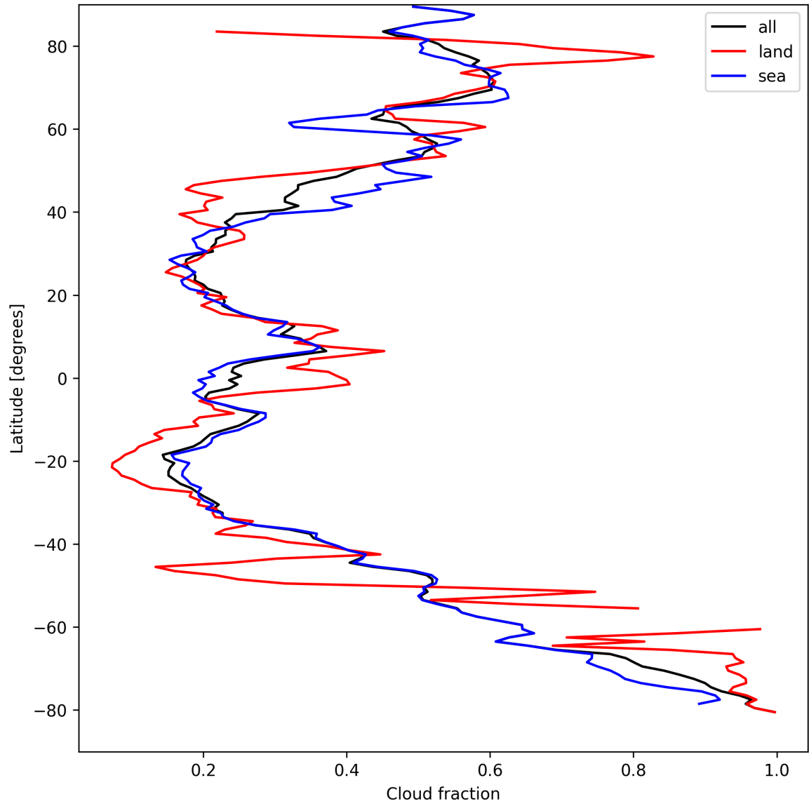
Figure 13: Zonal average of “Cloud fraction” for 2025-09-03 to 2025-09-04.
