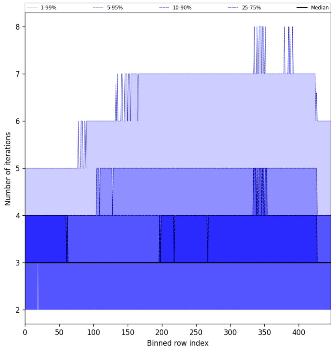
Figure 54: Along track statistics of “Number of iterations” for 2025-09-03 to 2025-09-04
