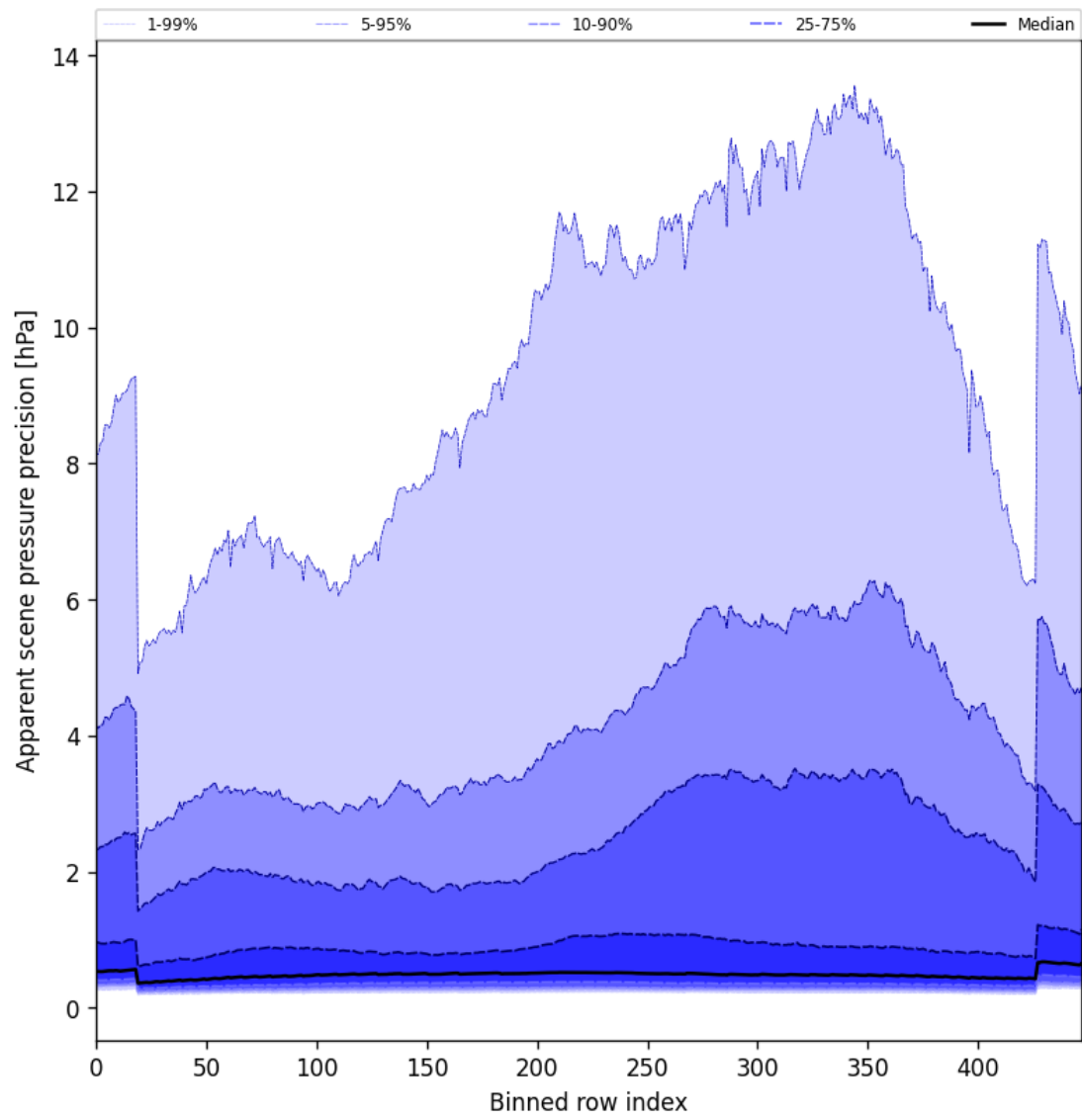
Figure 52: Along track statistics of “Apparent scene pressure precision” for 2025-09-03 to 2025-09-04
