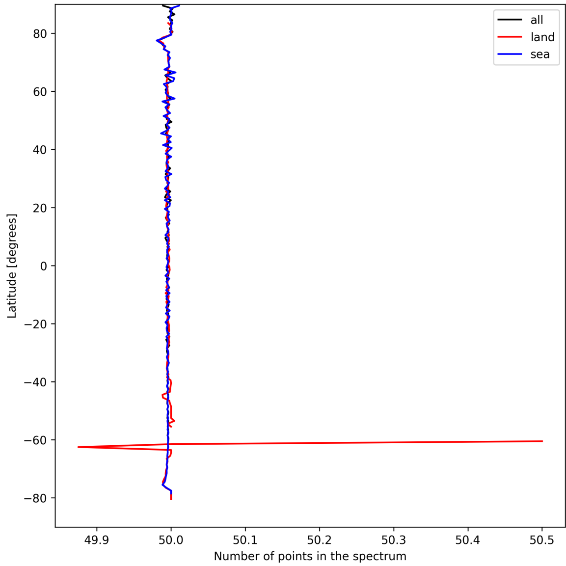
Figure 25: Zonal average of “Number of points in the spectrum” for 2025-09-03 to 2025-09-04.
