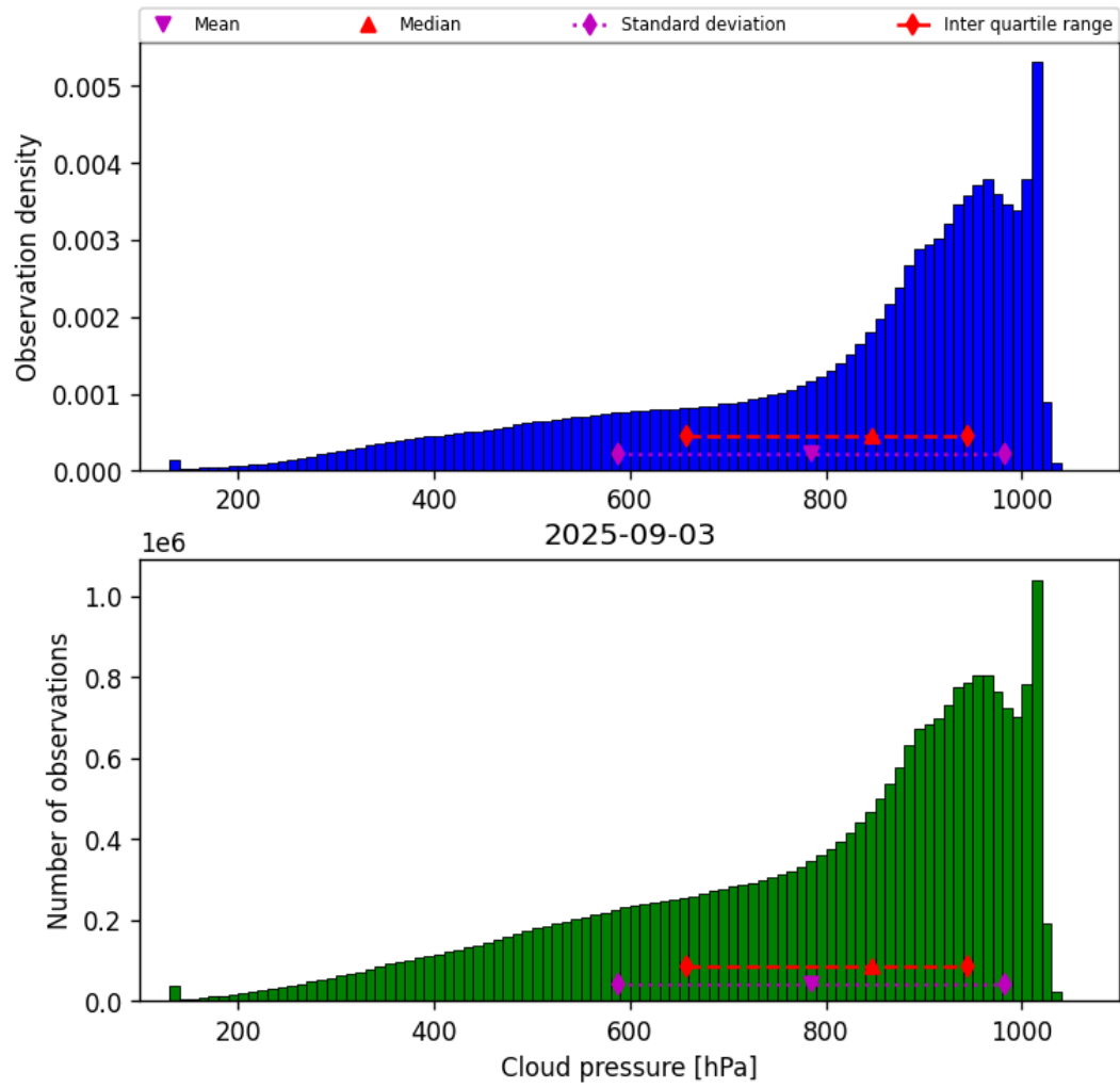
Figure 28: Histogram of “Cloud pressure” for 2025-09-03 to 2025-09-04
