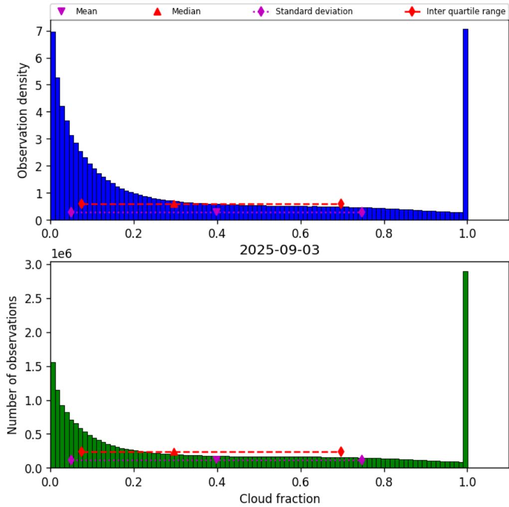
Figure 30: Histogram of “Cloud fraction” for 2025-09-03 to 2025-09-04
