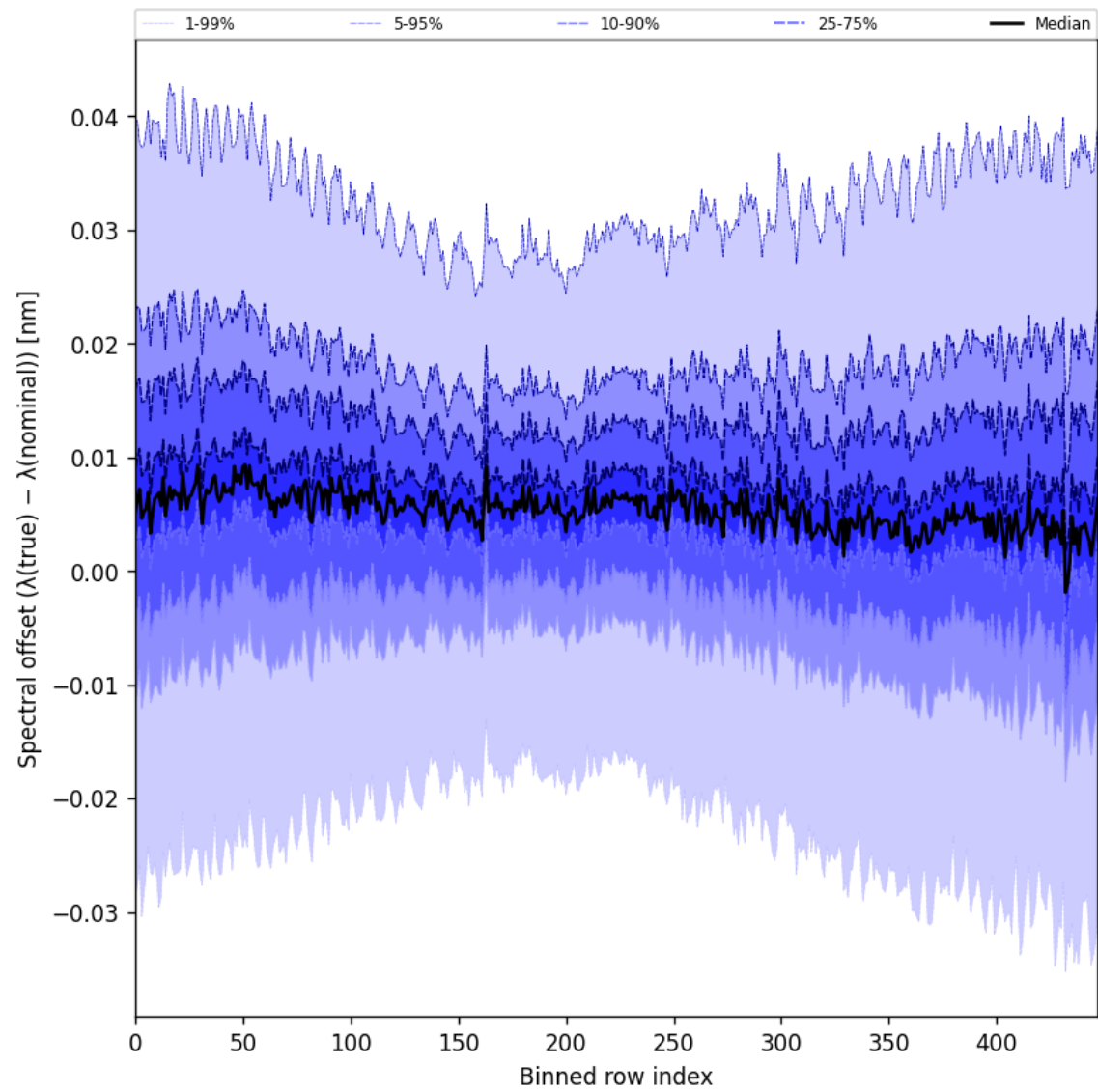
Figure 60: Along track statistics of “Spectral offset ( \lambda_{\text{true}} - \lambda_{\text{nominal}} )” for 2025-09-03 to 2025-09-04
