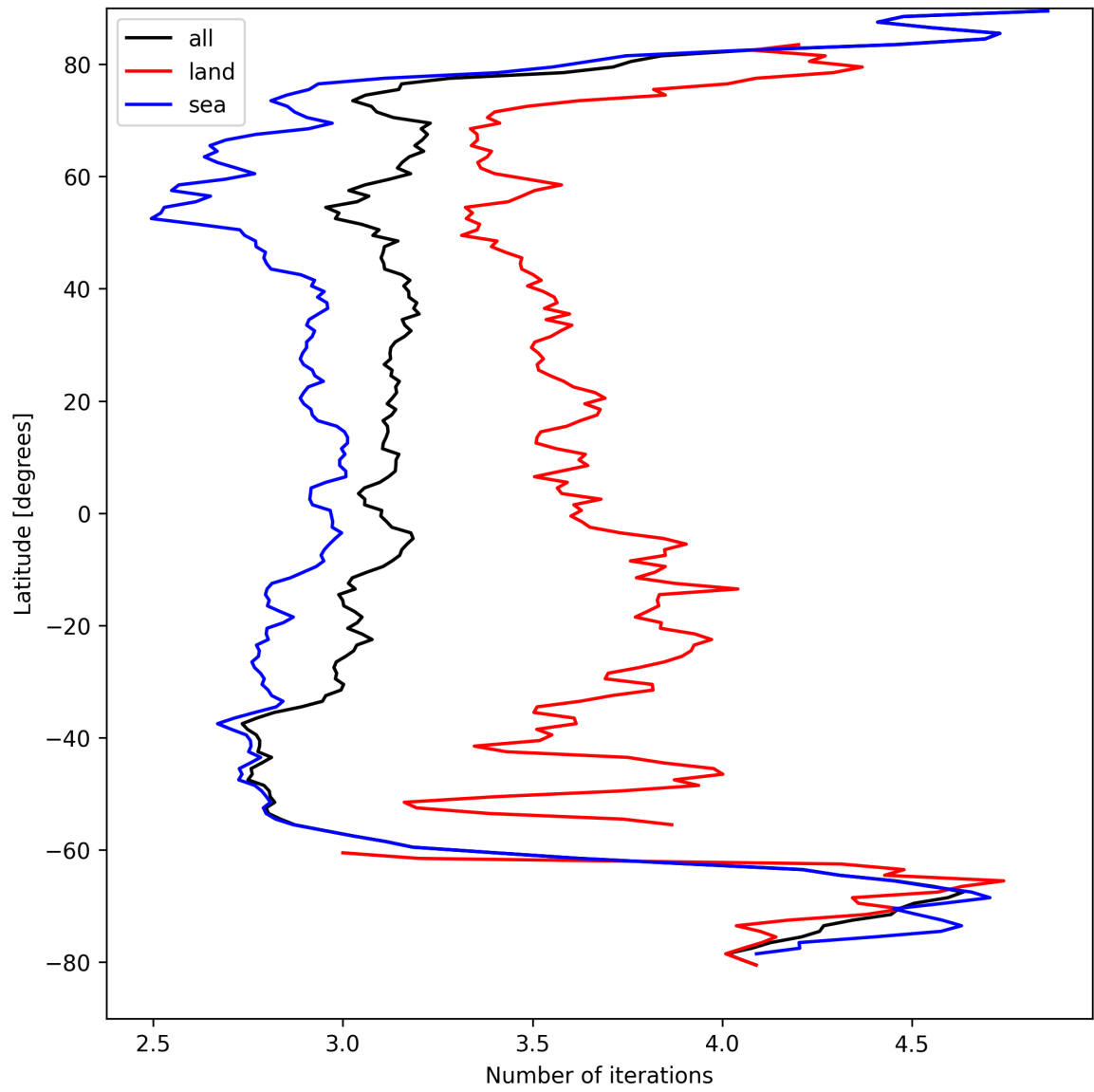
Figure 20: Zonal average of “Number of iterations” for 2025-09-03 to 2025-09-04.
