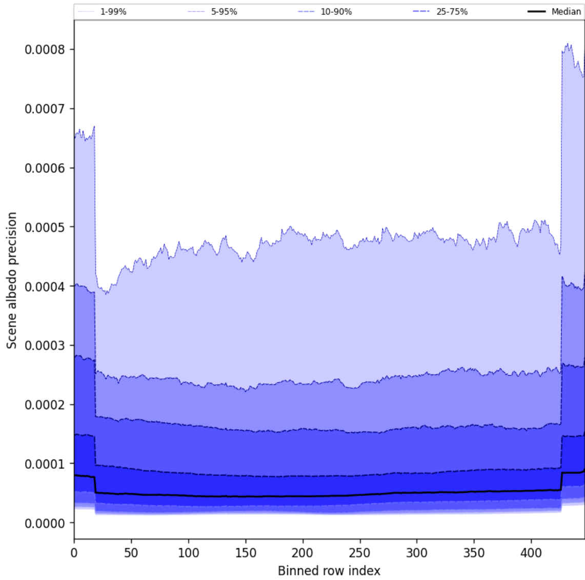
Figure 50: Along track statistics of “Scene albedo precision” for 2025-09-03 to 2025-09-04
