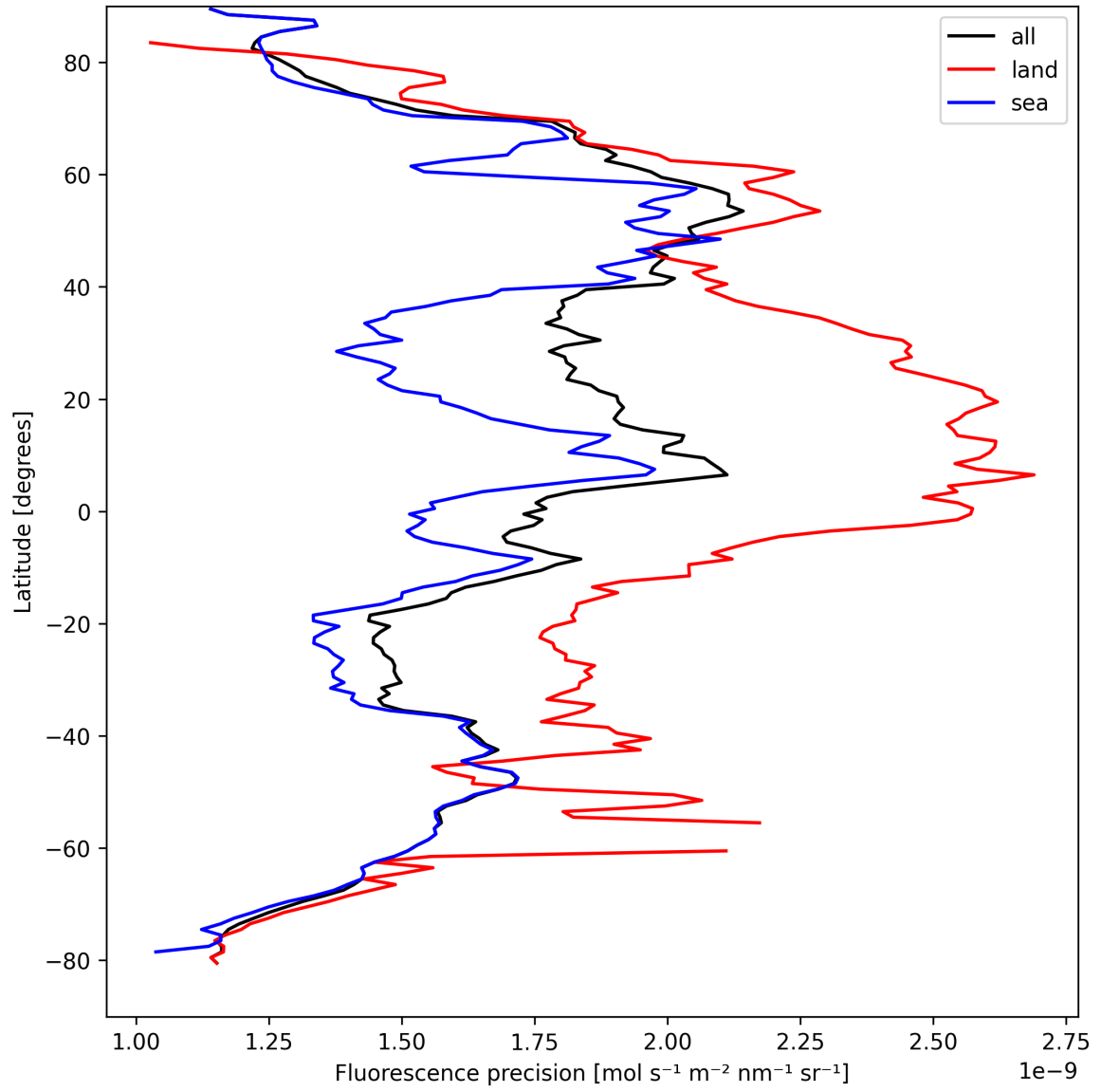
Figure 22: Zonal average of “Fluorescence precision” for 2025-09-03 to 2025-09-04.
