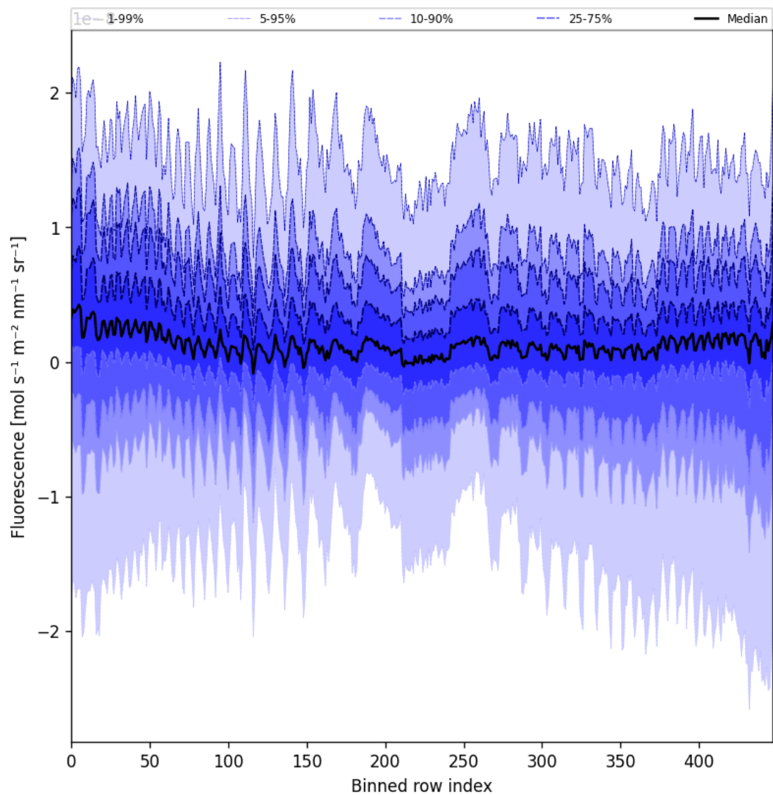
Figure 55: Along track statistics of "Fluorescence" for 2025-09-03 to 2025-09-04
