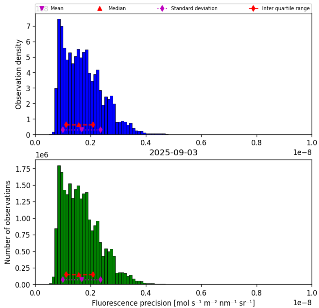
Figure 39: Histogram of “Fluorescence precision” for 2025-09-03 to 2025-09-04
