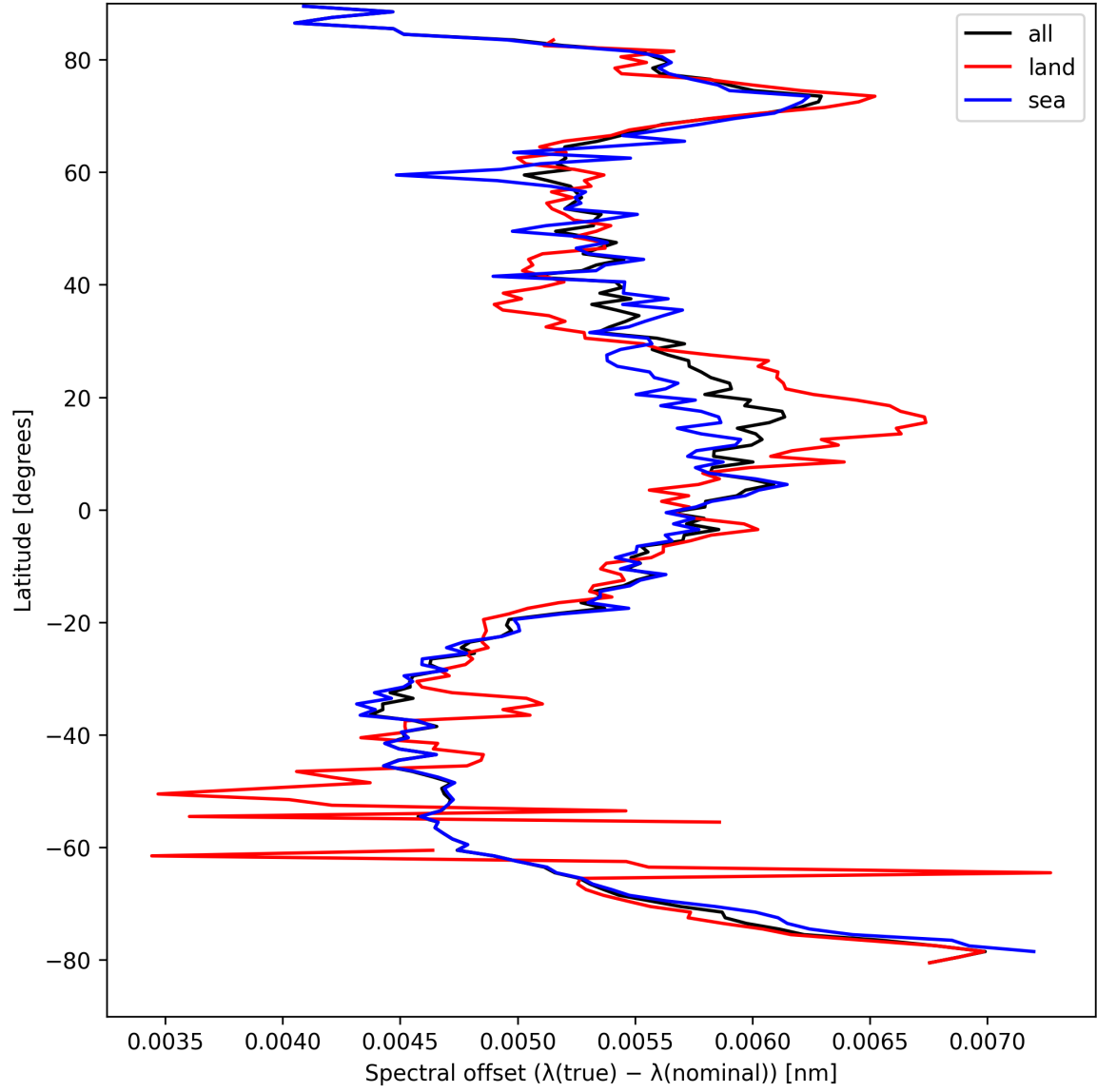
Figure 26: Zonal average of “Spectral offset ( \lambda_{\text{true}} - \lambda_{\text{nominal}} )” for 2025-09-03 to 2025-09-04.
