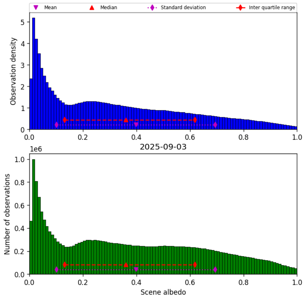
Figure 32: Histogram of “Scene albedo” for 2025-09-03 to 2025-09-04
