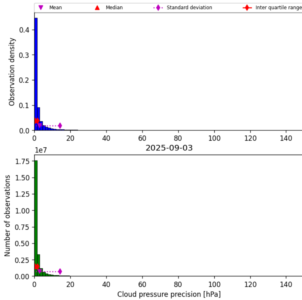
Figure 29: Histogram of “Cloud pressure precision” for 2025-09-03 to 2025-09-04
