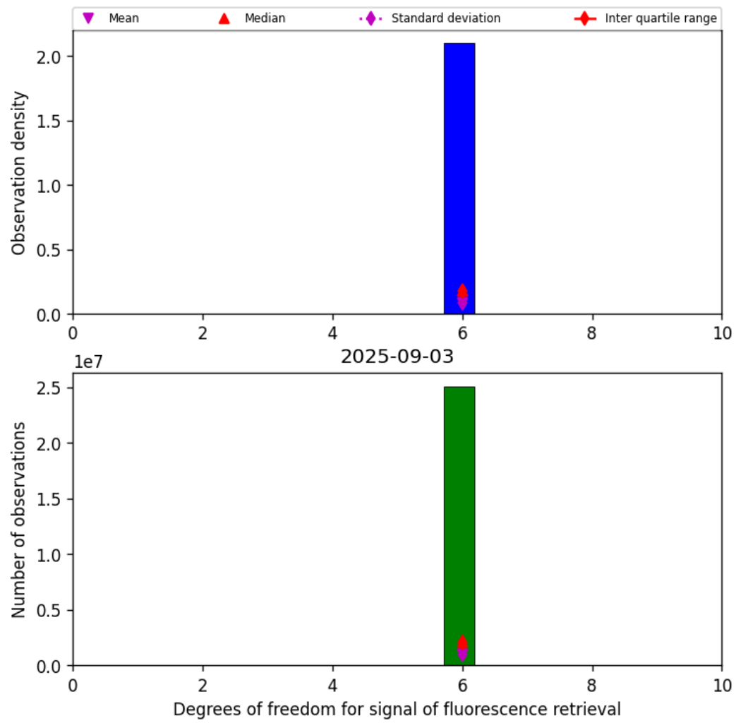
Figure 41: Histogram of “Degrees of freedom for signal of fluorescence retrieval” for 2025-09-03 to 2025-09-04
