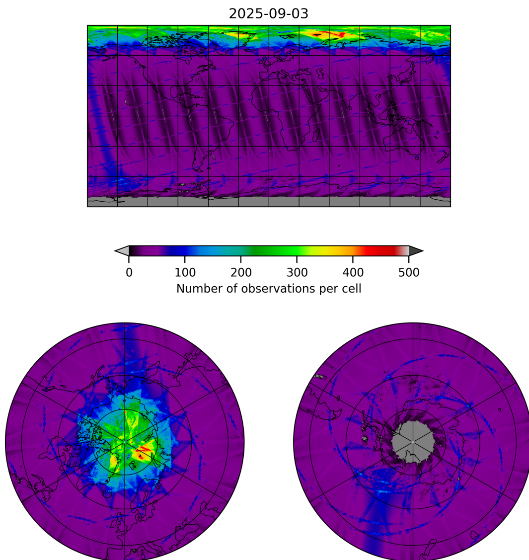
Figure 9: Map of the number of observations for 2025-09-03 to 2025-09-04
