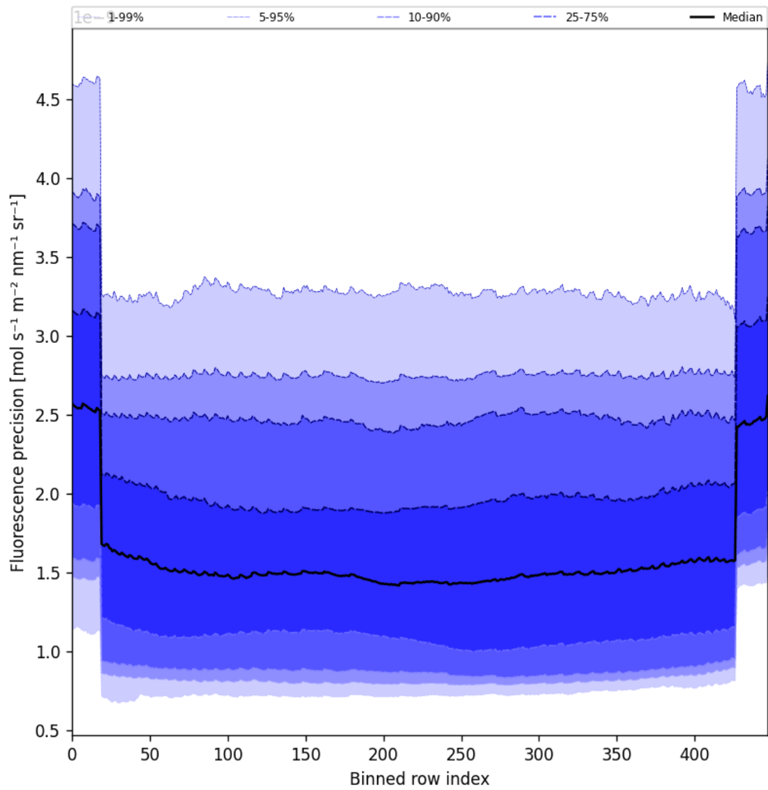
Figure 56: Along track statistics of “Fluorescence precision” for 2025-09-03 to 2025-09-04
