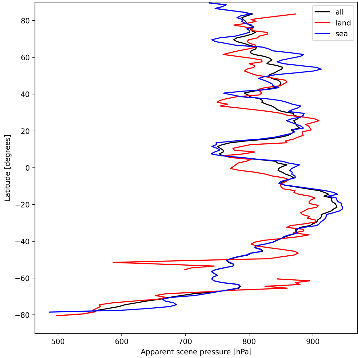
Figure 17: Zonal average of “Apparent scene pressure” for 2025-09-03 to 2025-09-04.
