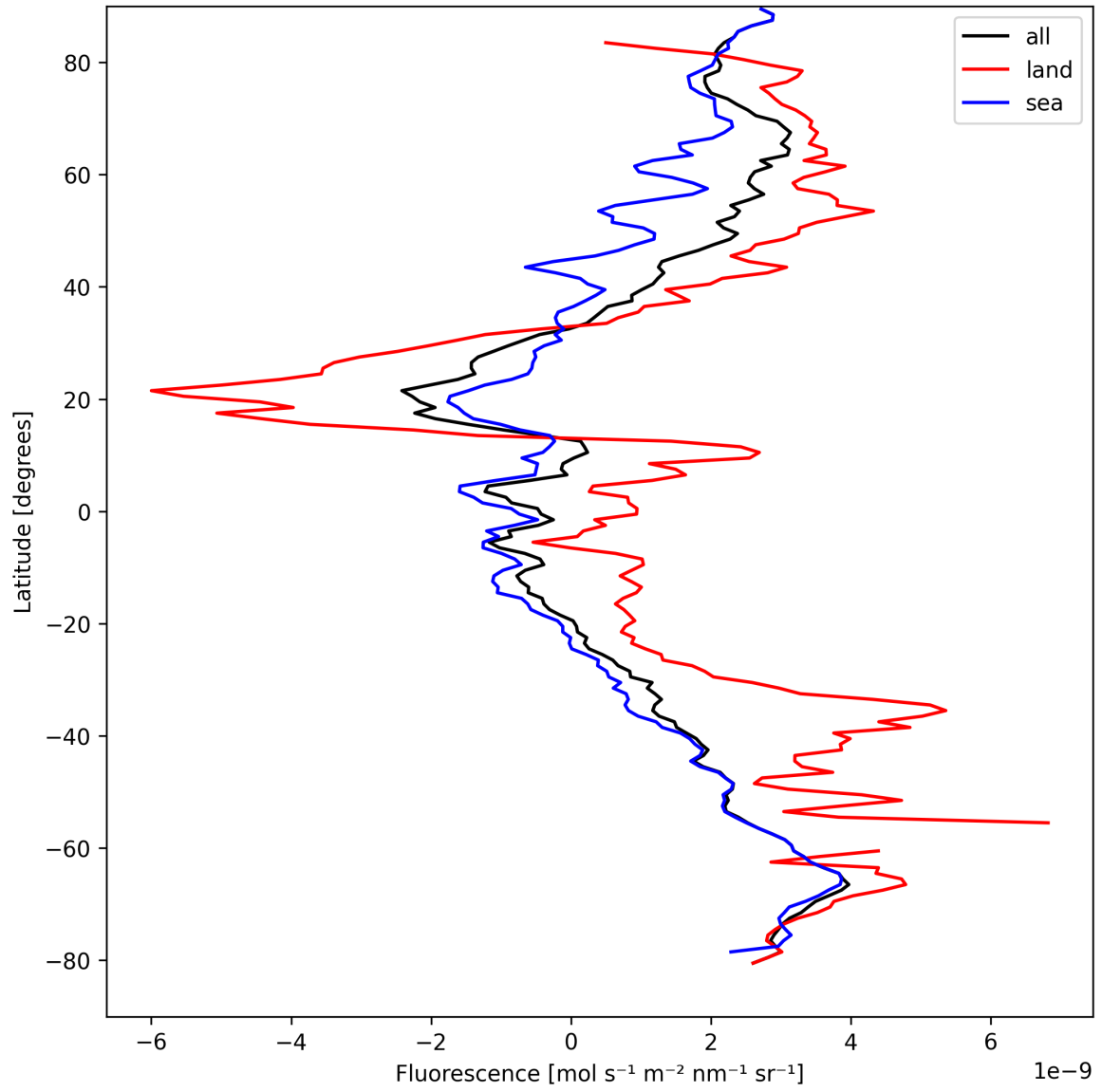
Figure 21: Zonal average of “Fluorescence” for 2025-09-03 to 2025-09-04.
