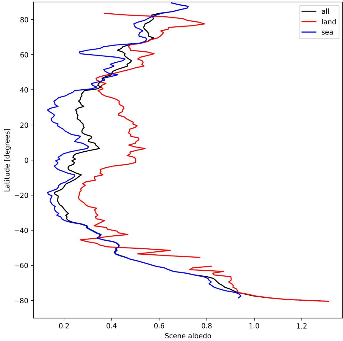
Figure 15: Zonal average of “Scene albedo” for 2025-09-03 to 2025-09-04.
