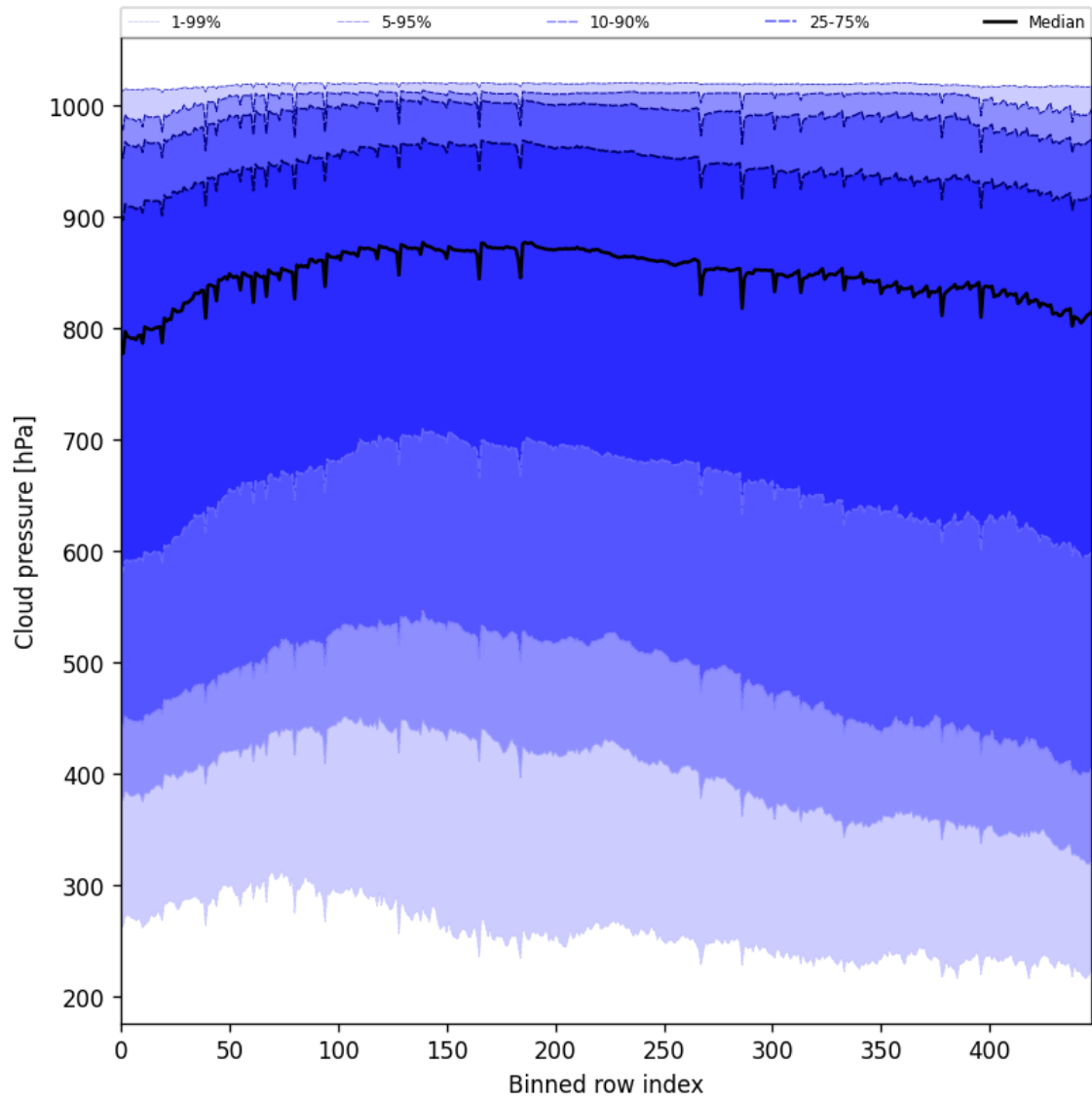
Figure 45: Along track statistics of “Cloud pressure” for 2025-09-03 to 2025-09-04
