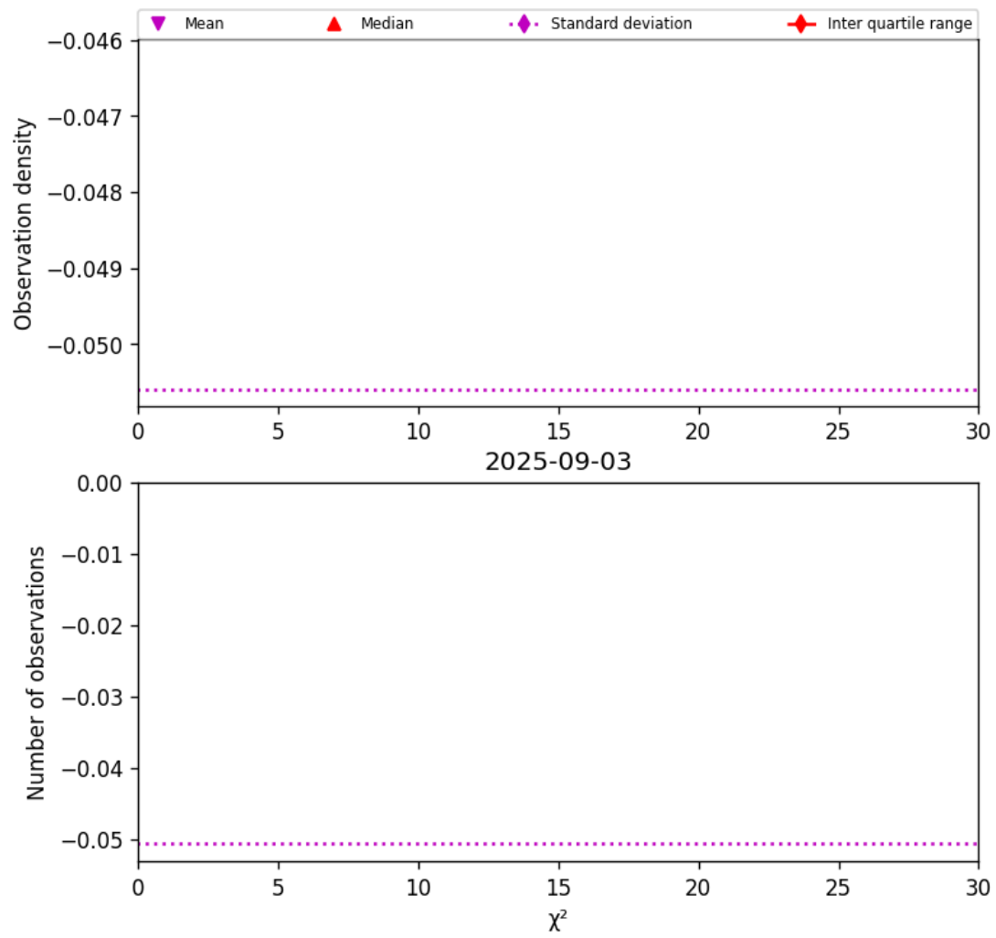
Figure 36: Histogram of " \chi^2 " for 2025-09-03 to 2025-09-04
