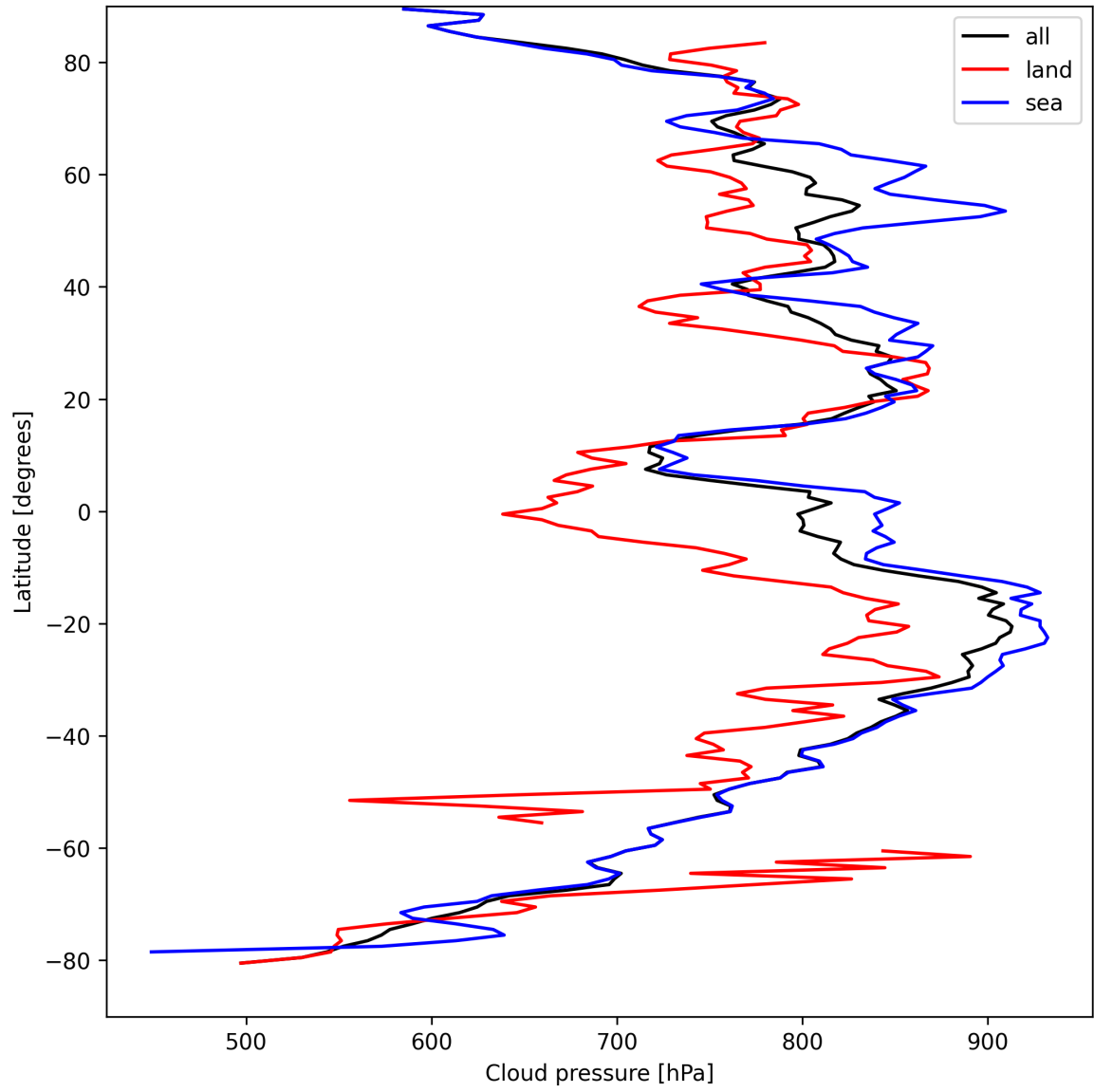
Figure 11: Zonal average of “Cloud pressure” for 2025-09-03 to 2025-09-04.
