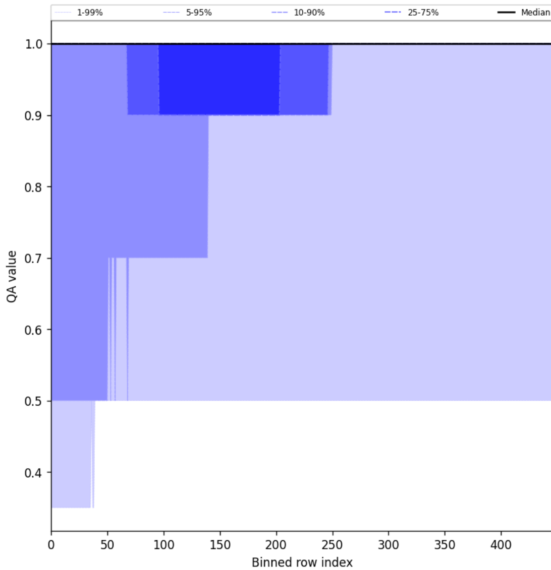
Figure 44: Along track statistics of “QA value” for 2025-09-03 to 2025-09-04
