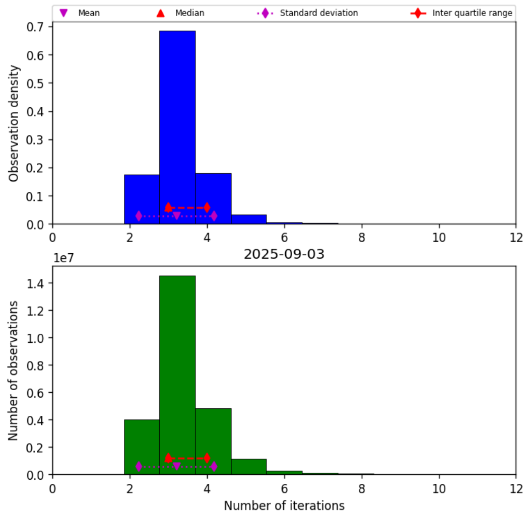
Figure 37: Histogram of “Number of iterations” for 2025-09-03 to 2025-09-04
