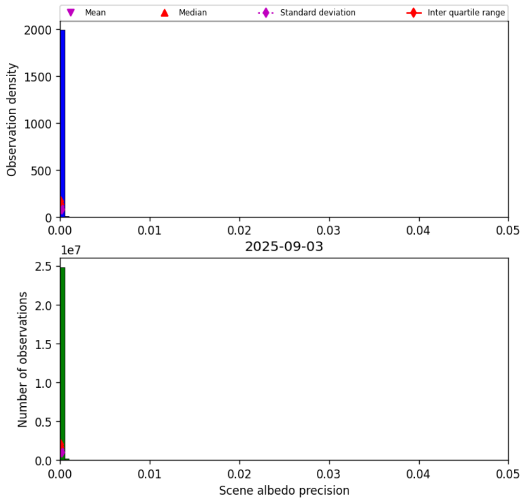
Figure 33: Histogram of “Scene albedo precision” for 2025-09-03 to 2025-09-04
