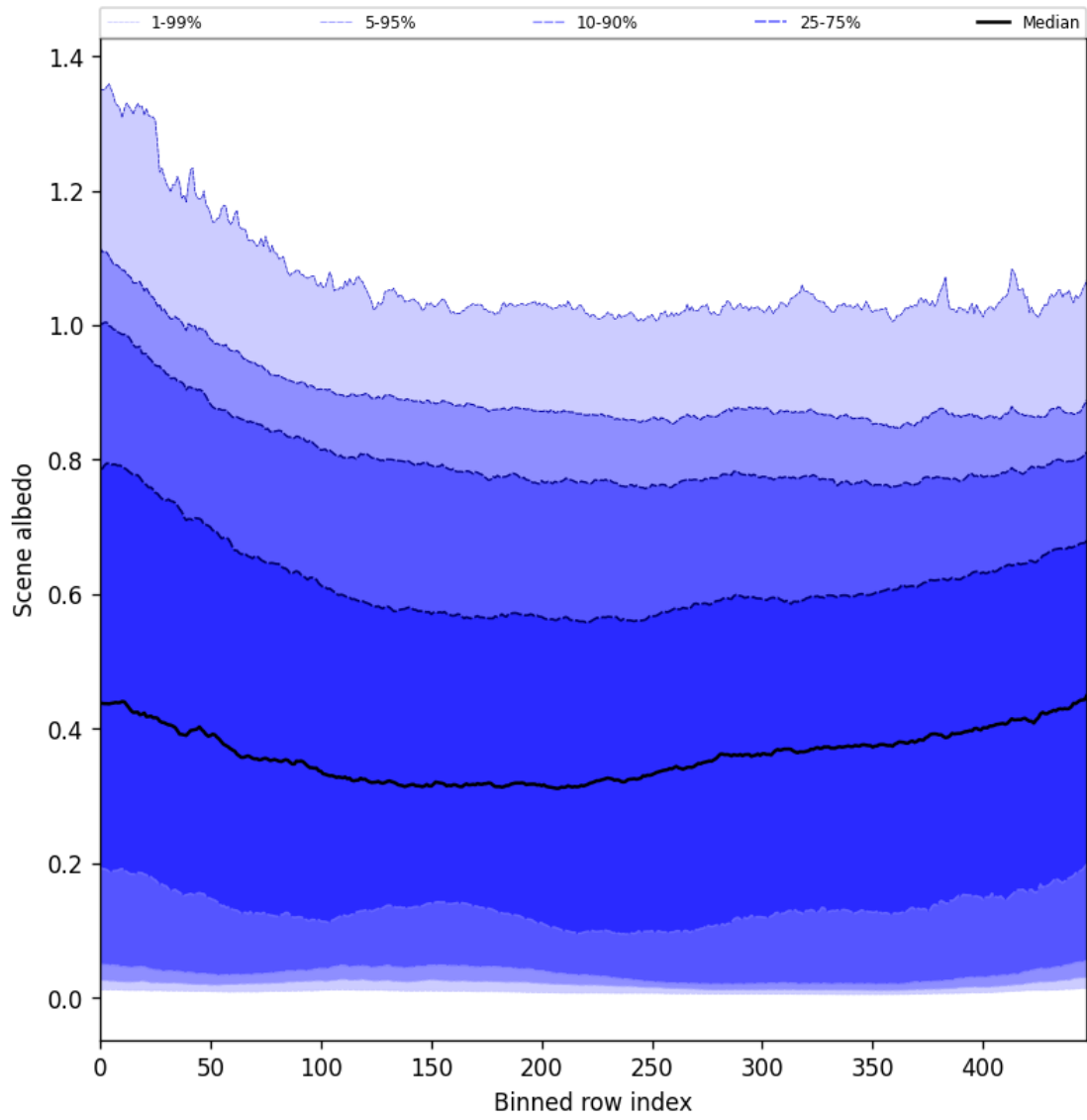
Figure 49: Along track statistics of "Scene albedo" for 2025-09-03 to 2025-09-04
