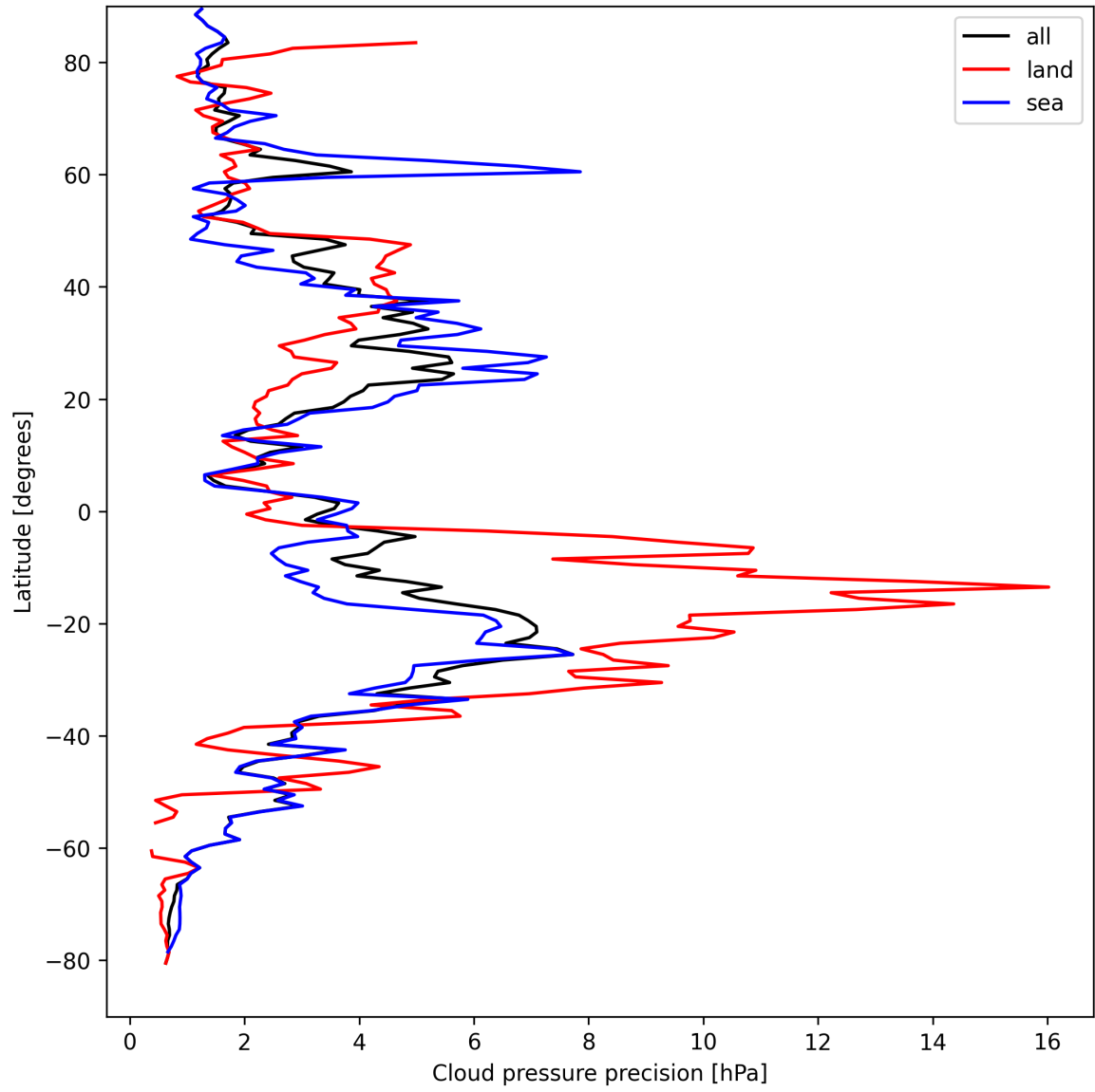
Figure 12: Zonal average of “Cloud pressure precision” for 2025-09-03 to 2025-09-04.
