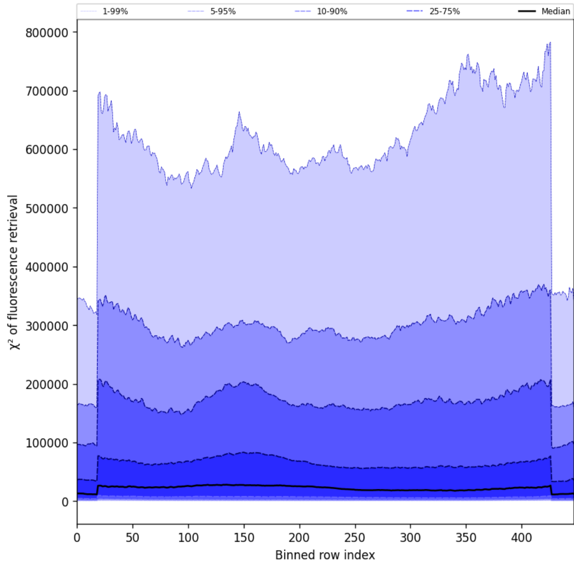
Figure 57: Along track statistics of “ \chi^2 of fluorescence retrieval” for 2025-09-03 to 2025-09-04
