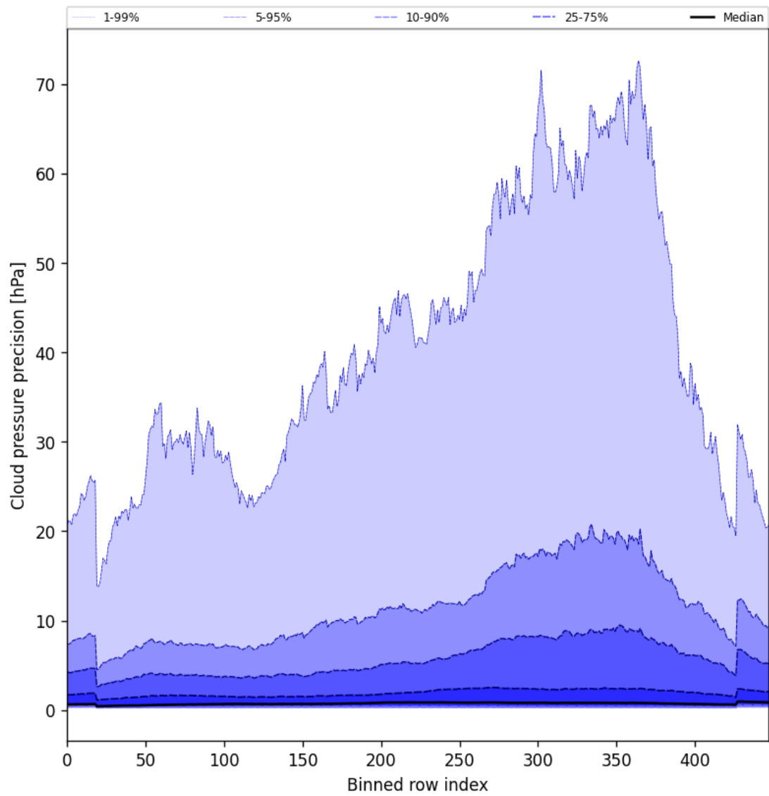
Figure 46: Along track statistics of “Cloud pressure precision” for 2025-09-03 to 2025-09-04
