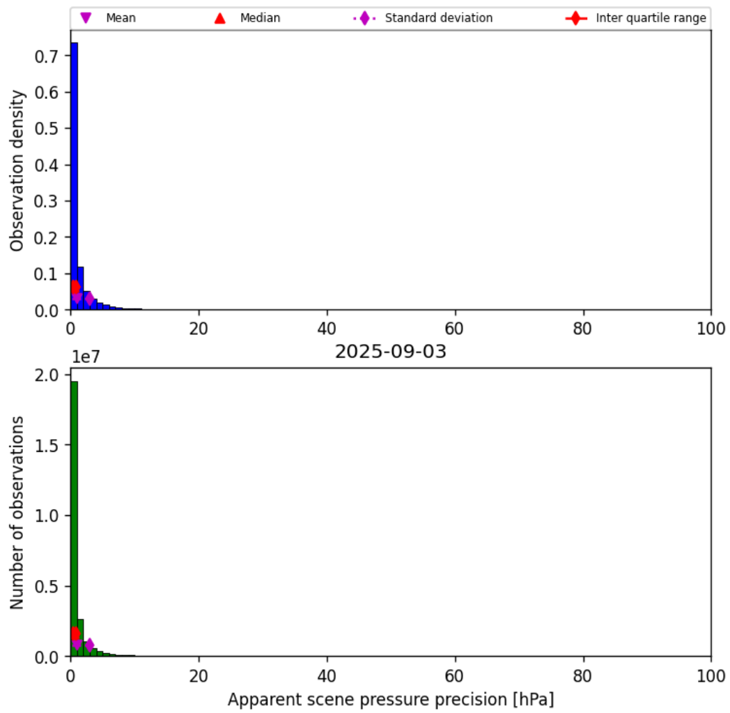
Figure 35: Histogram of “Apparent scene pressure precision” for 2025-09-03 to 2025-09-04
