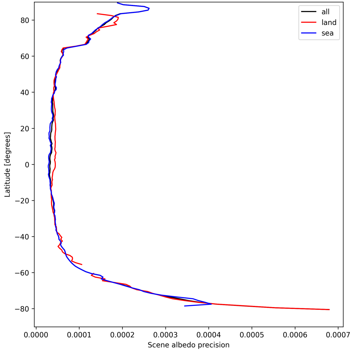
Figure 16: Zonal average of “Scene albedo precision” for 2025-09-03 to 2025-09-04.
