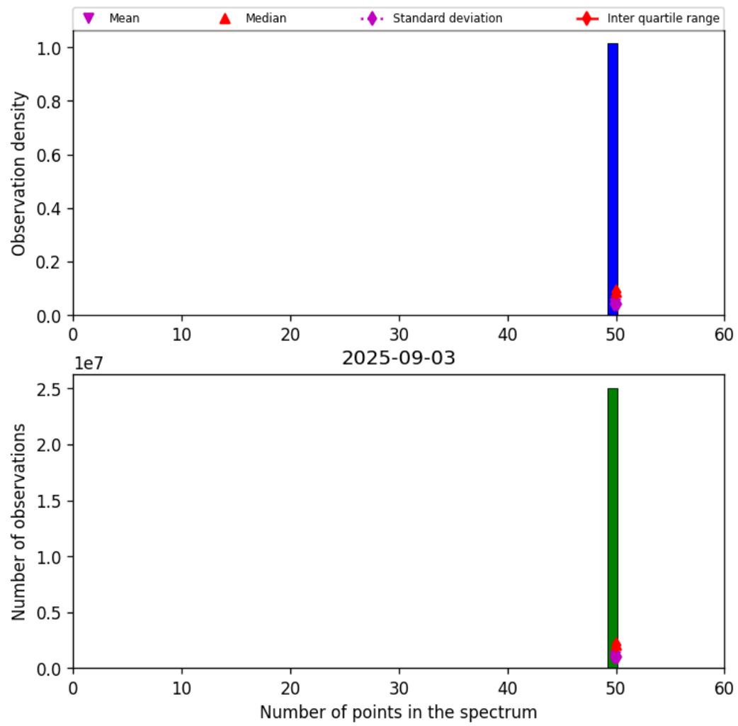
Figure 42: Histogram of “Number of points in the spectrum” for 2025-09-03 to 2025-09-04
