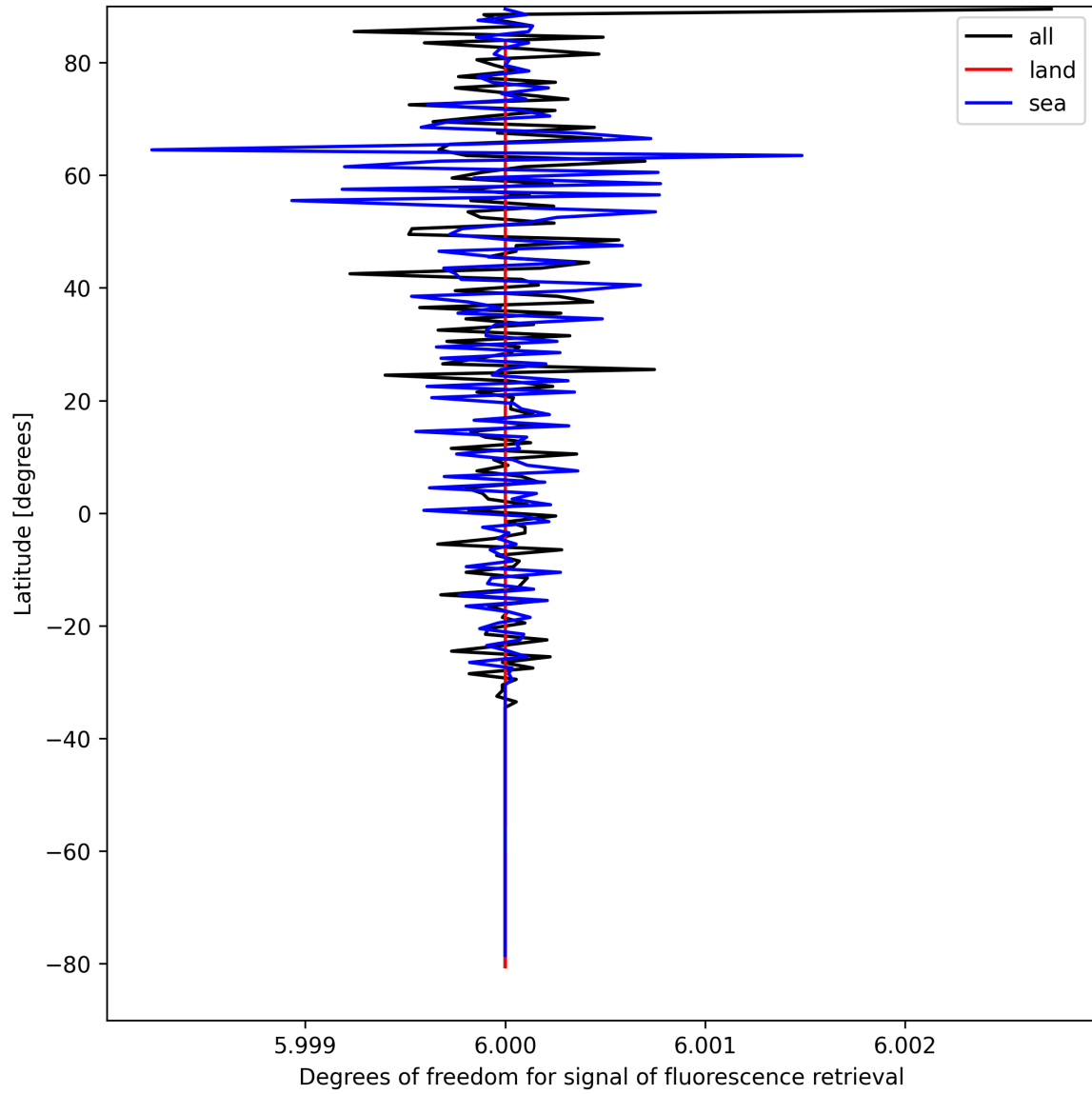
Figure 24: Zonal average of “Degrees of freedom for signal of fluorescence retrieval” for 2025-09-03 to 2025-09-04.
