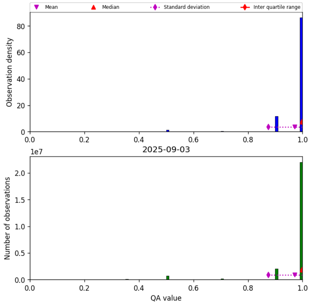
Figure 27: Histogram of “QA value” for 2025-09-03 to 2025-09-04
