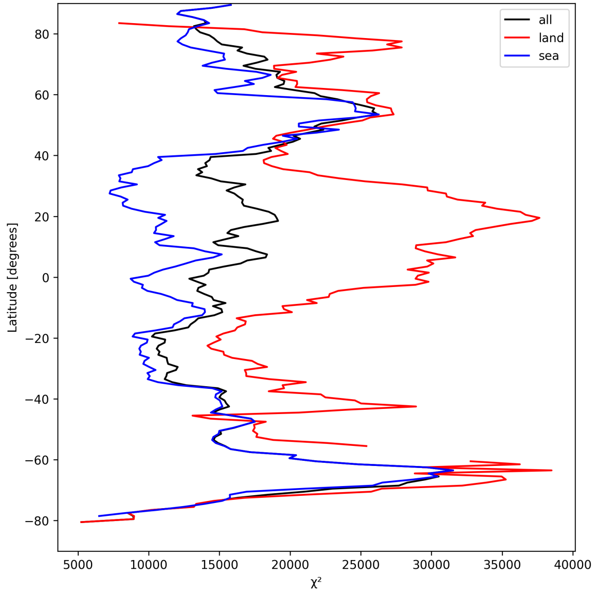
Figure 19: Zonal average of “ \chi^2 ” for 2025-09-03 to 2025-09-04.
