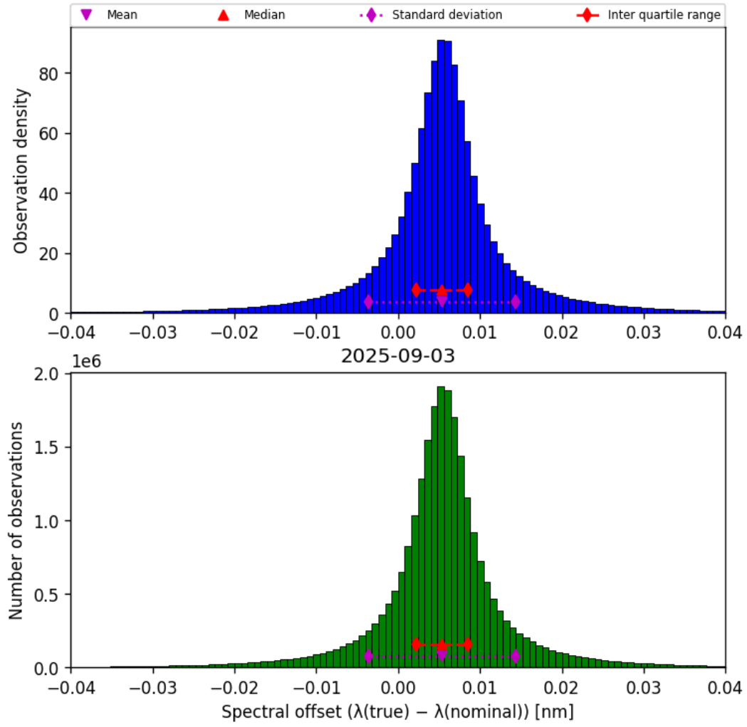
Figure 43: Histogram of “Spectral offset ( \lambda_{\text{true}} - \lambda_{\text{nominal}} )” for 2025-09-03 to 2025-09-04
