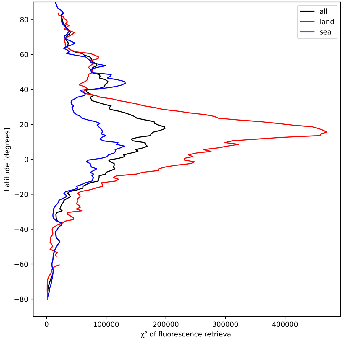
Figure 23: Zonal average of “ \chi^2 of fluorescence retrieval” for 2025-09-03 to 2025-09-04.
