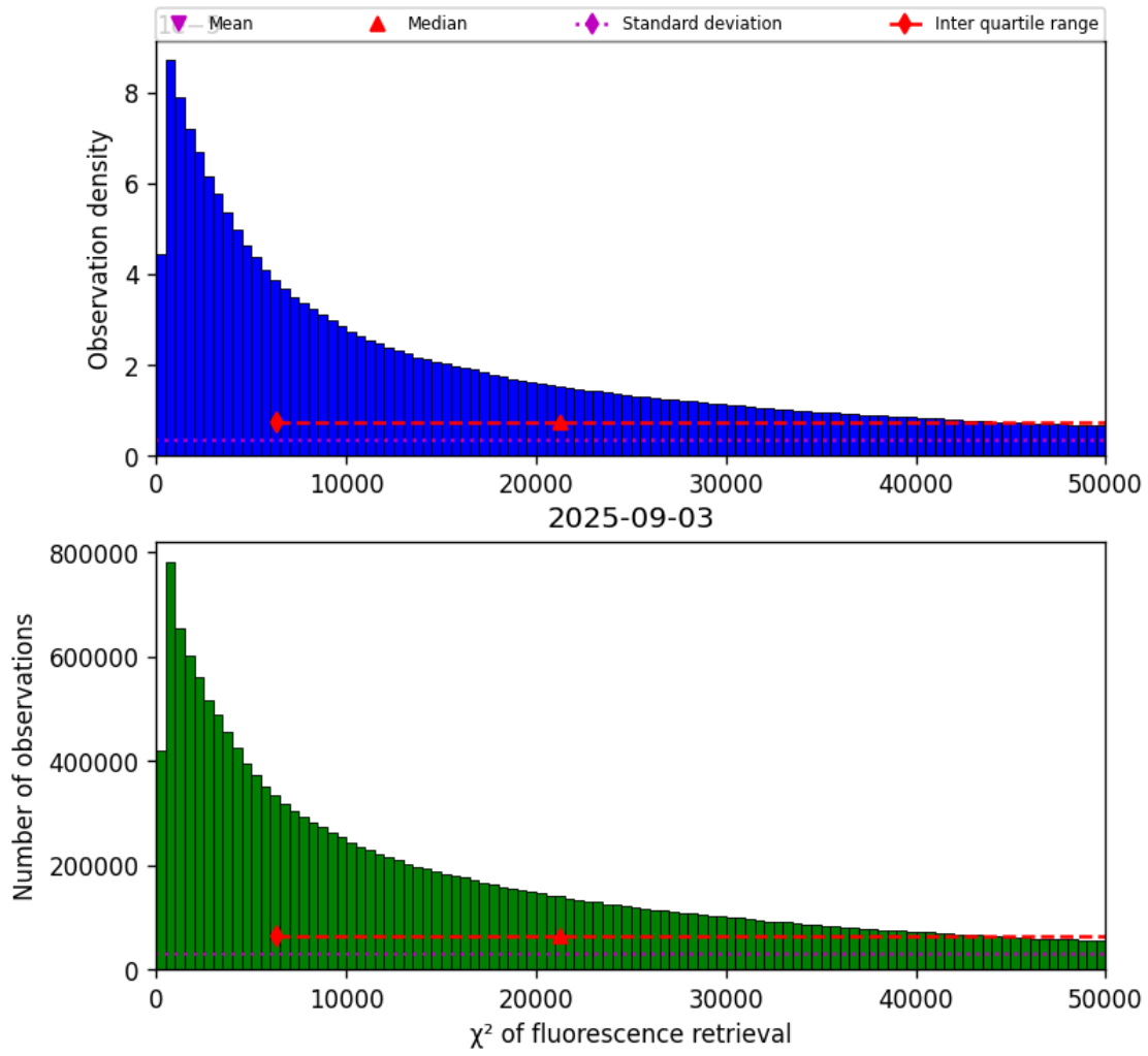
Figure 40: Histogram of “ \chi^2 of fluorescence retrieval” for 2025-09-03 to 2025-09-04
