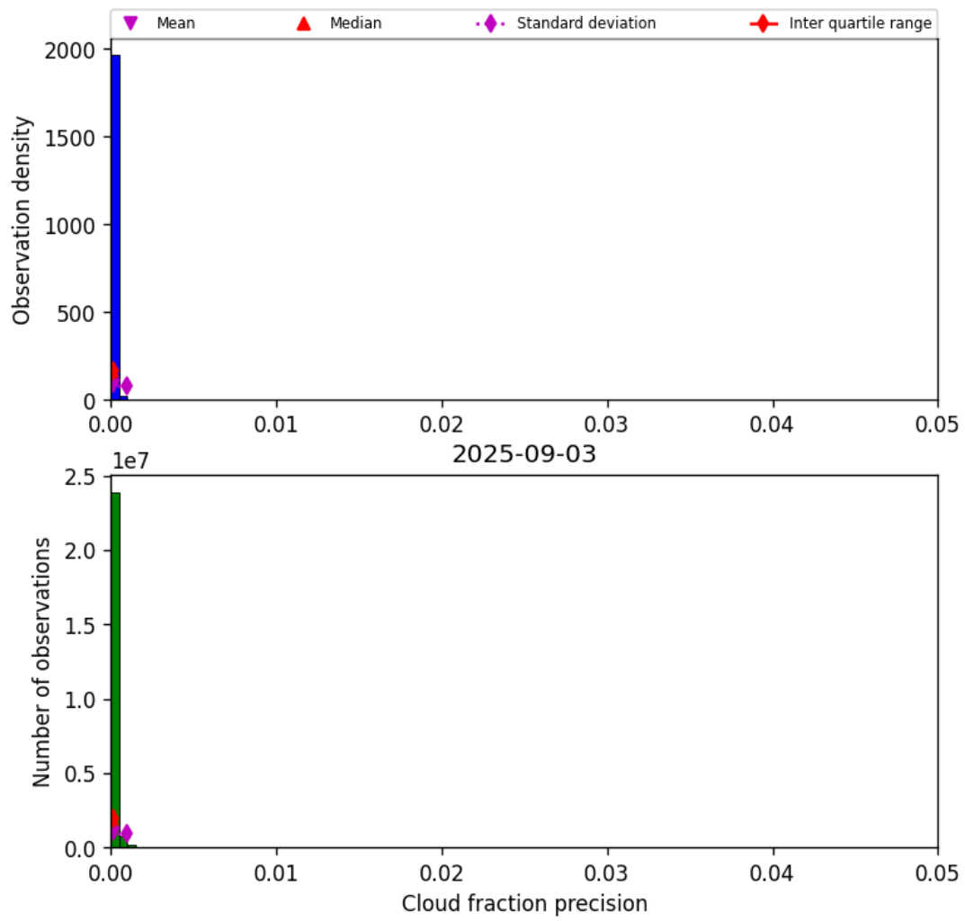
Figure 31: Histogram of “Cloud fraction precision” for 2025-09-03 to 2025-09-04
