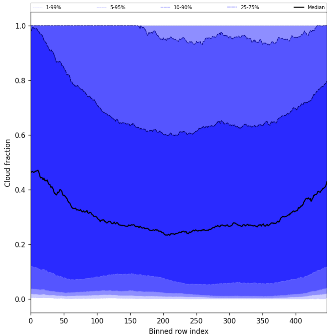
Figure 47: Along track statistics of “Cloud fraction” for 2025-09-03 to 2025-09-04
