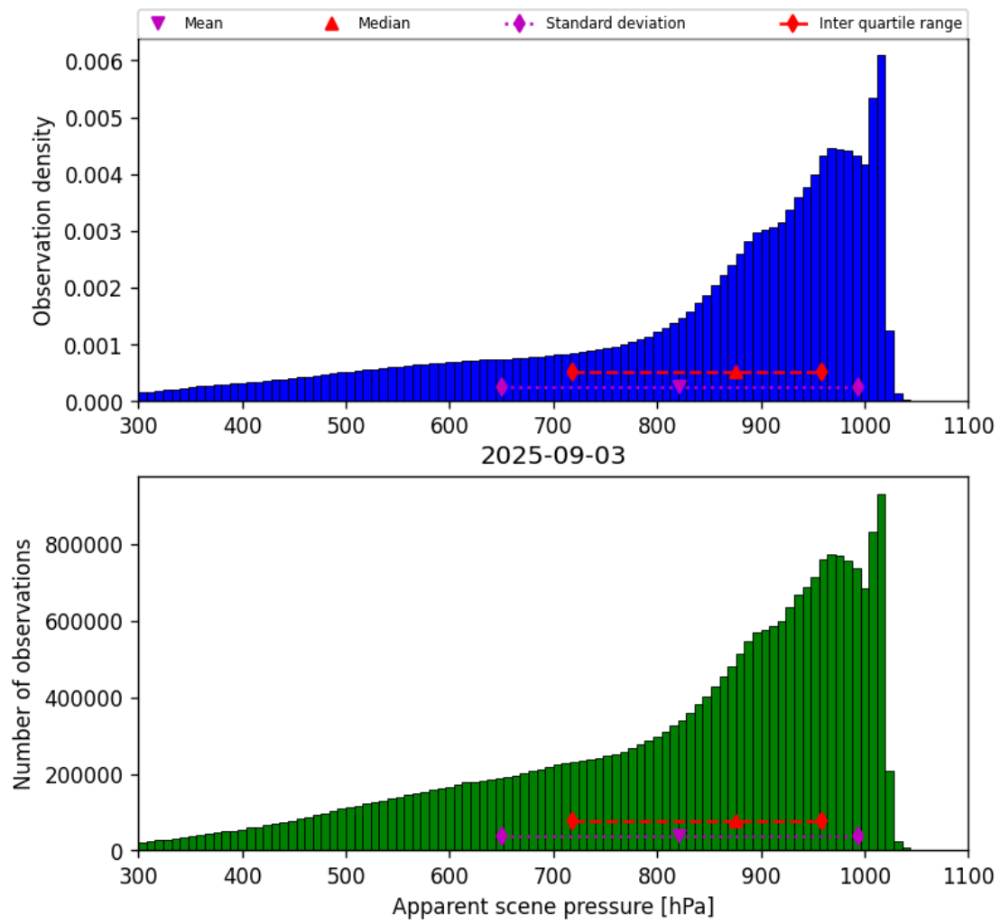
Figure 34: Histogram of “Apparent scene pressure” for 2025-09-03 to 2025-09-04
