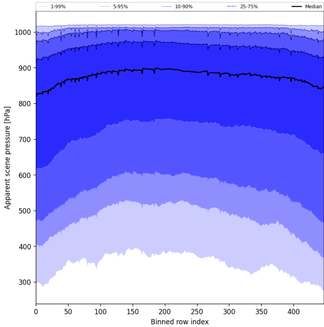
Figure 51: Along track statistics of “Apparent scene pressure” for 2025-09-03 to 2025-09-04
