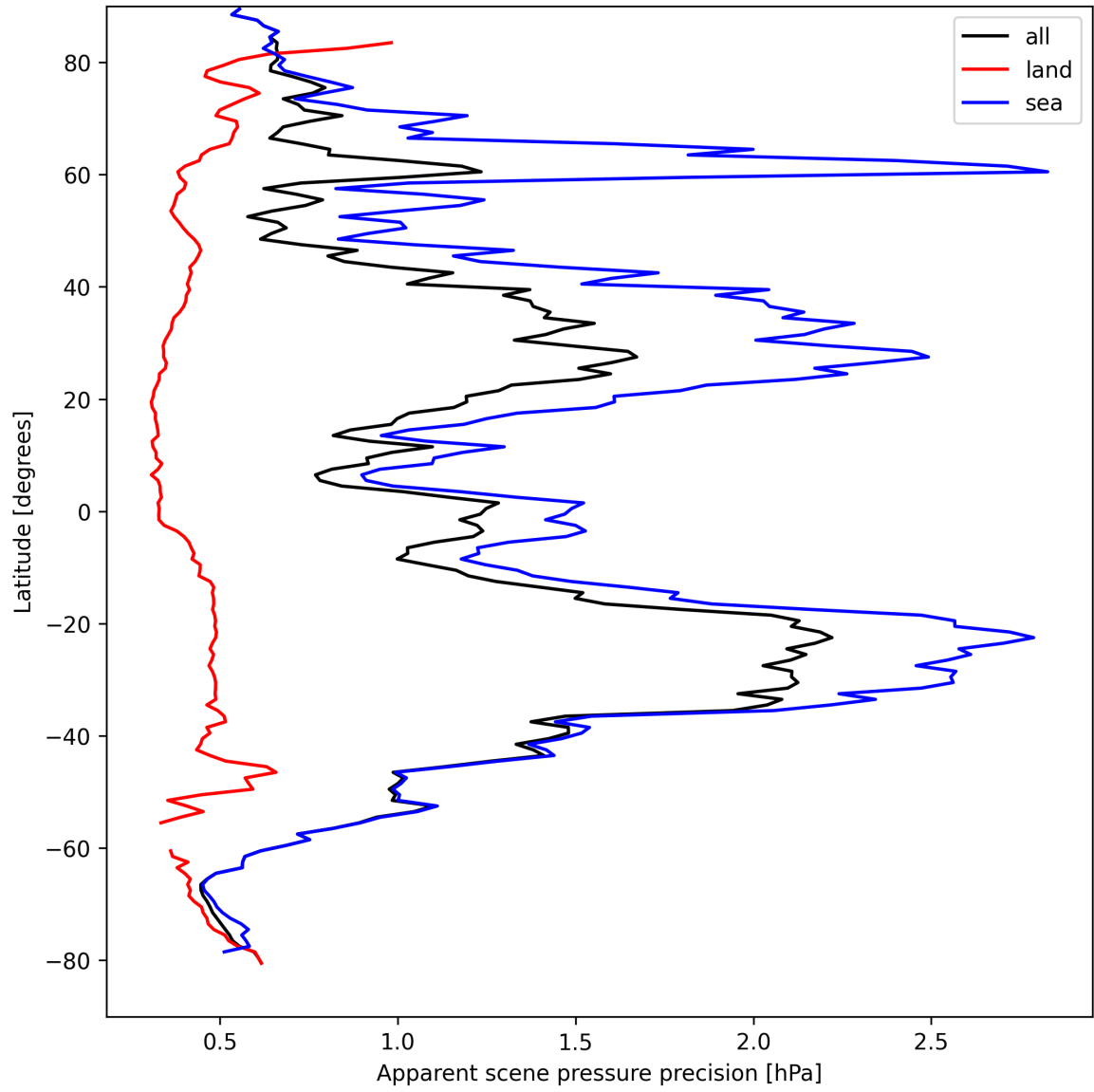
Figure 18: Zonal average of “Apparent scene pressure precision” for 2025-09-03 to 2025-09-04.
