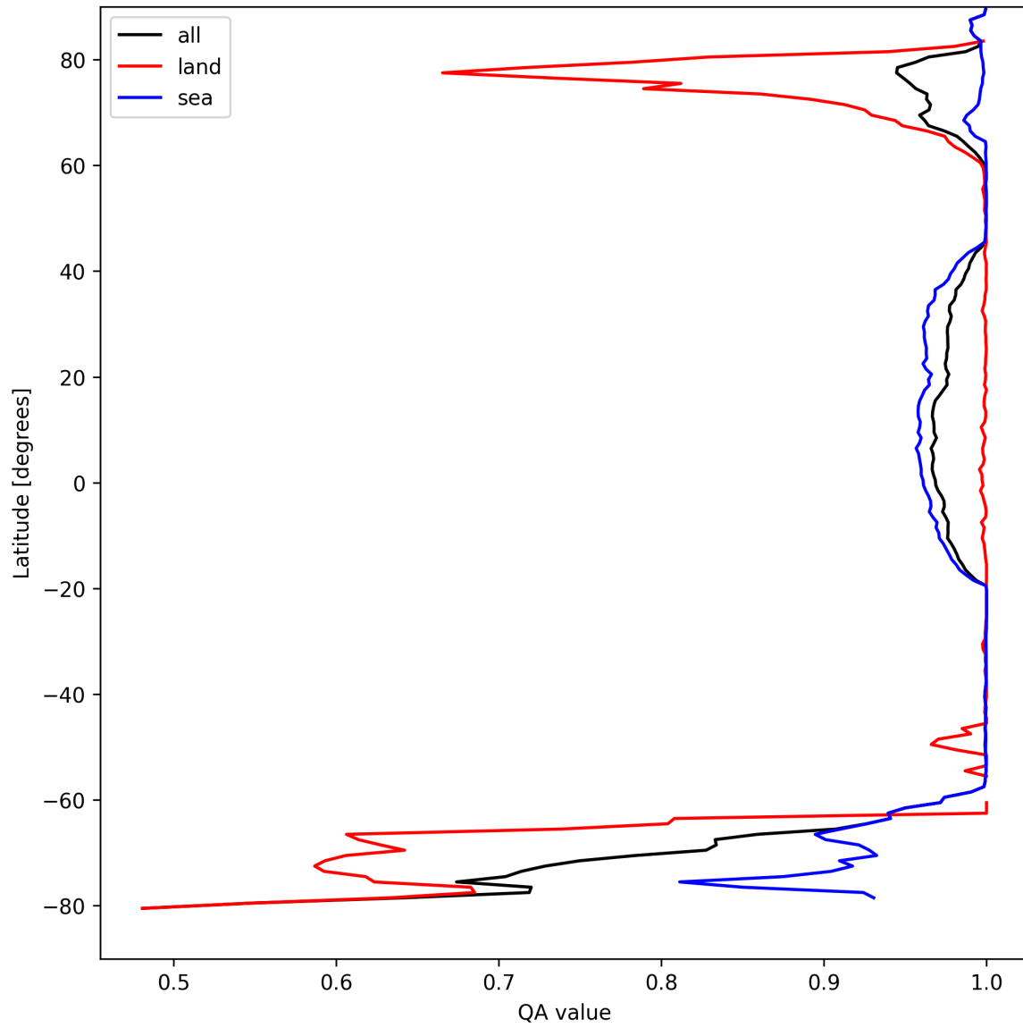
Figure 10: Zonal average of "QA value" for 2025-09-03 to 2025-09-04.
