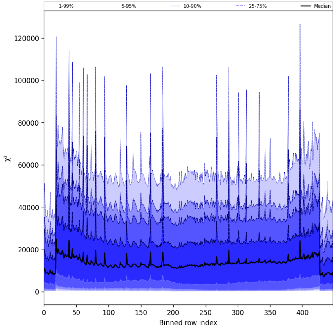
Figure 53: Along track statistics of “ \chi^2 ” for 2025-09-03 to 2025-09-04
