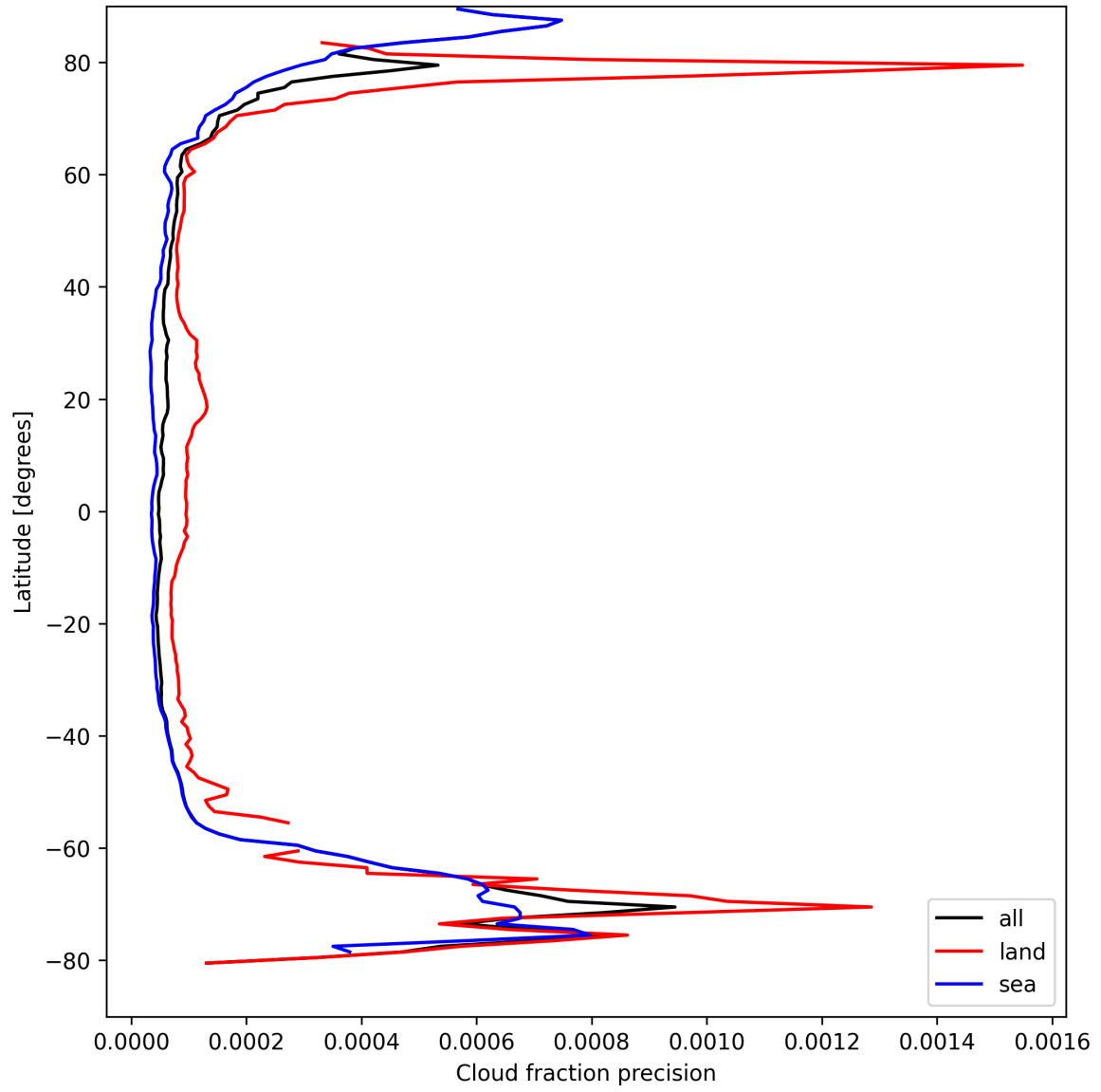
Figure 14: Zonal average of “Cloud fraction precision” for 2025-09-03 to 2025-09-04.
