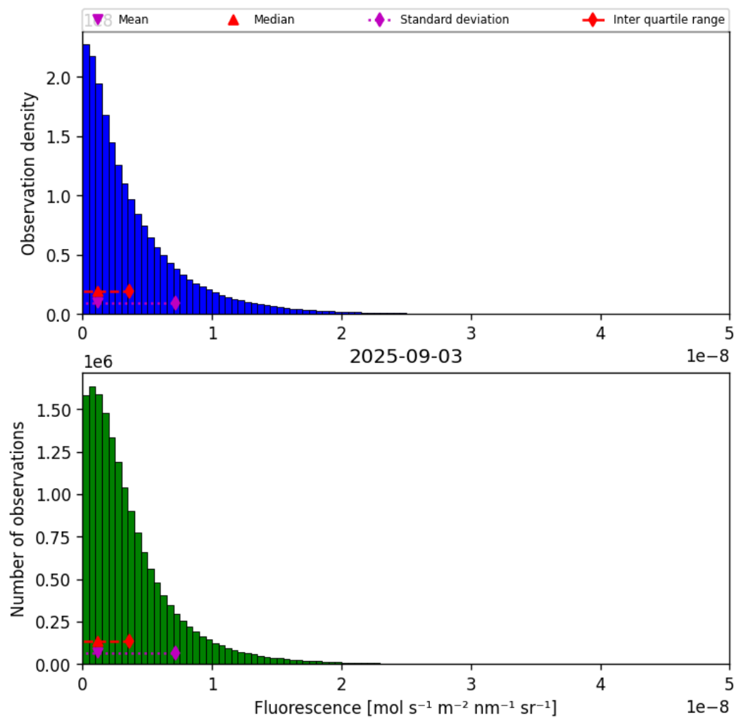
Figure 38: Histogram of “Fluorescence” for 2025-09-03 to 2025-09-04
