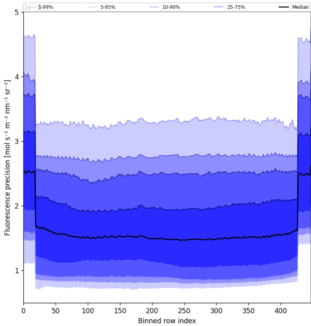
Figure 56: Along track statistics of “Fluorescence precision” for 2025-09-04 to 2025-09-05
