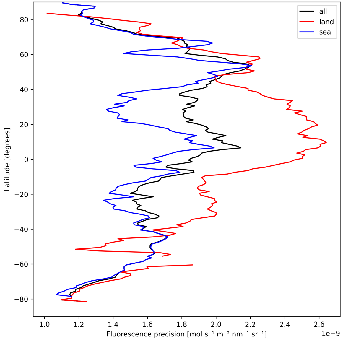
Figure 22: Zonal average of “Fluorescence precision” for 2025-09-04 to 2025-09-05.
