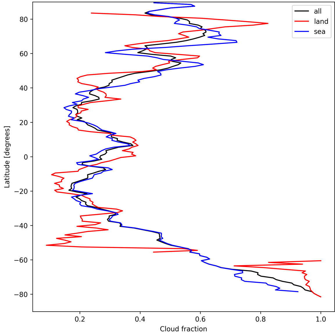
Figure 13: Zonal average of “Cloud fraction” for 2025-09-04 to 2025-09-05.
