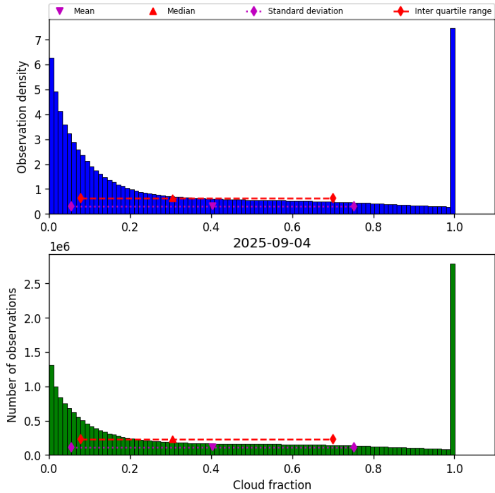
Figure 30: Histogram of “Cloud fraction” for 2025-09-04 to 2025-09-05
