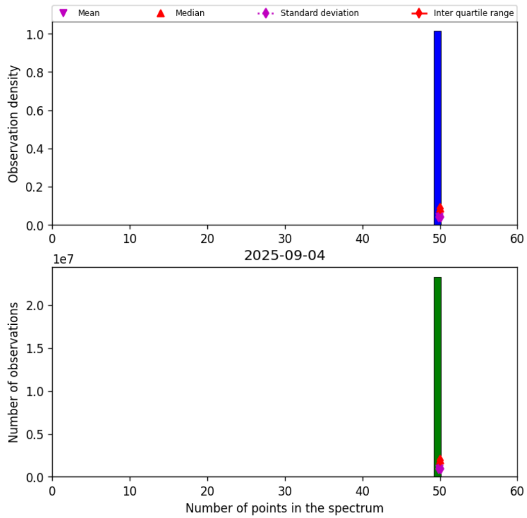
Figure 42: Histogram of “Number of points in the spectrum” for 2025-09-04 to 2025-09-05
