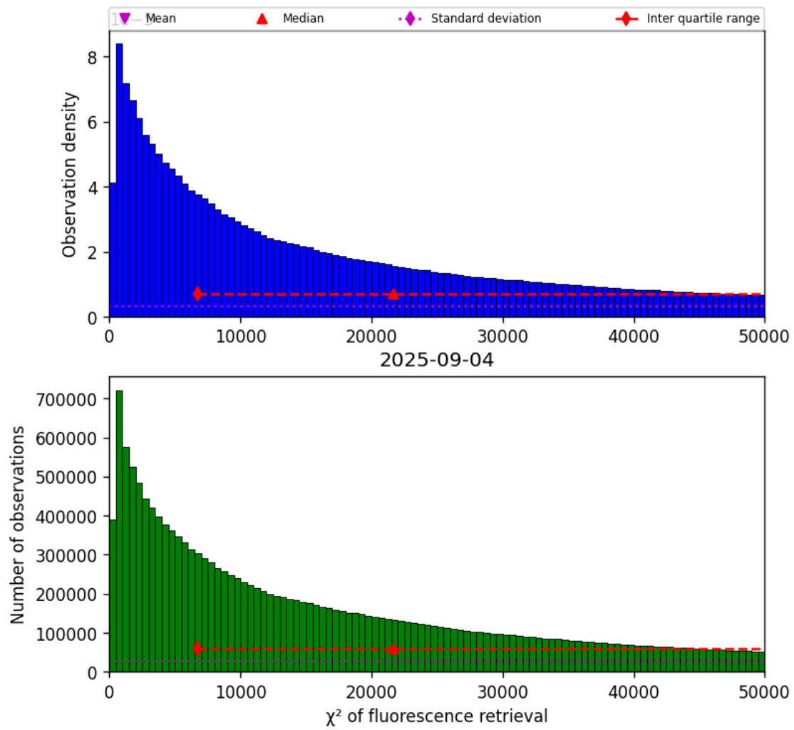
Figure 40: Histogram of “ \chi^2 of fluorescence retrieval” for 2025-09-04 to 2025-09-05
