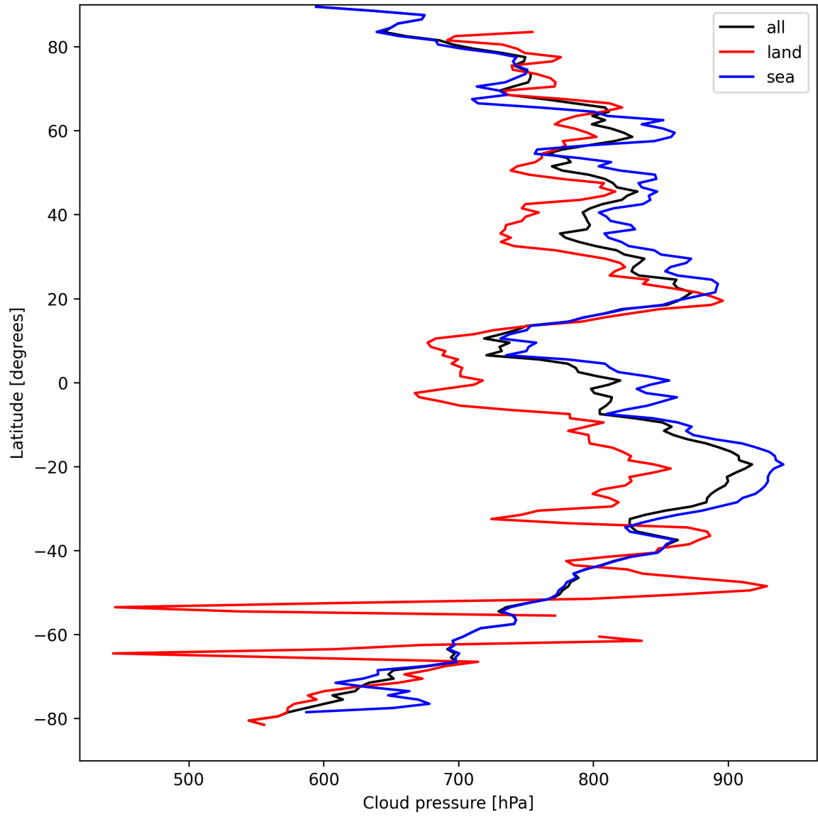
Figure 11: Zonal average of “Cloud pressure” for 2025-09-04 to 2025-09-05.
