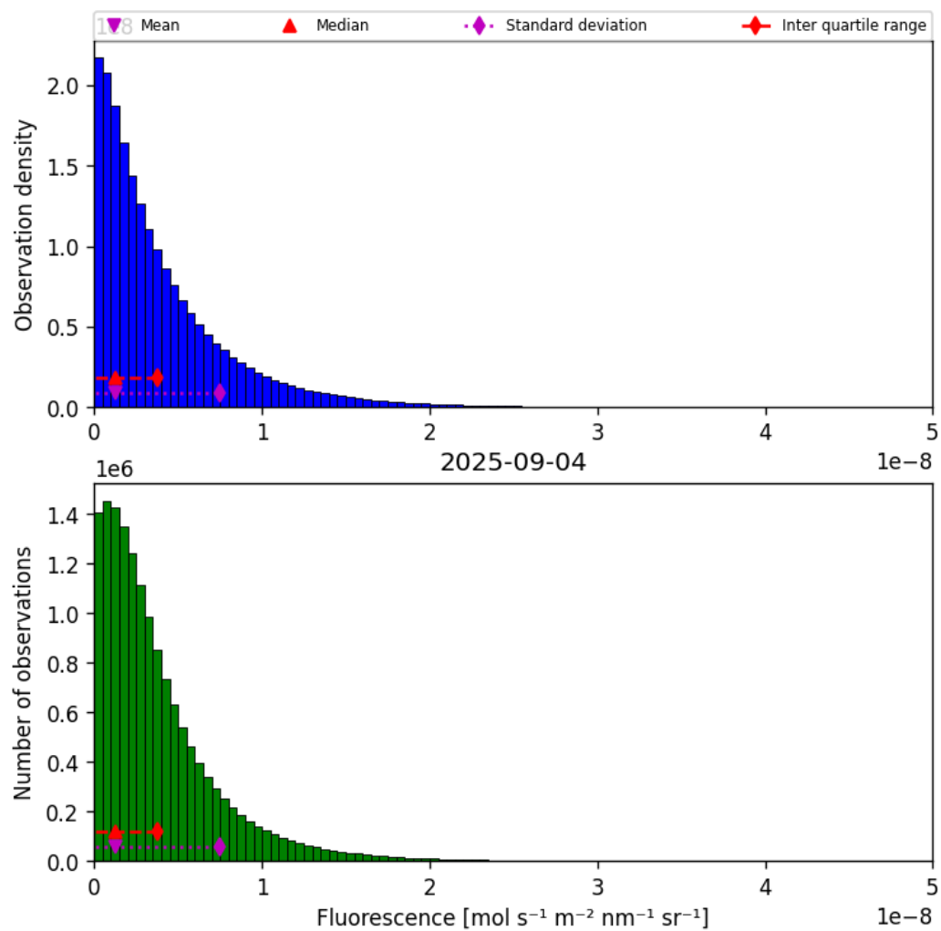
Figure 38: Histogram of “Fluorescence” for 2025-09-04 to 2025-09-05
