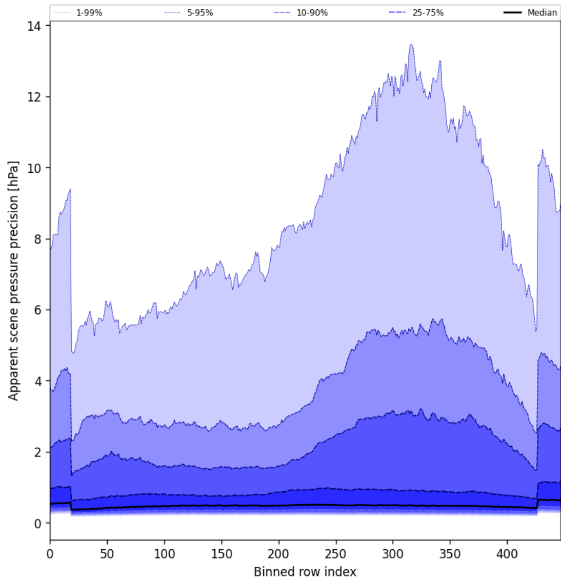
Figure 52: Along track statistics of “Apparent scene pressure precision” for 2025-09-04 to 2025-09-05
