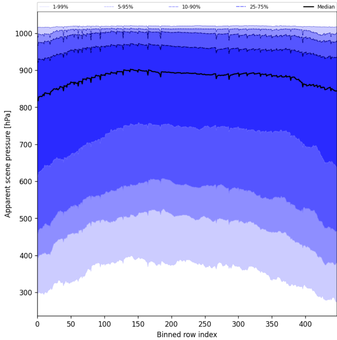
Figure 51: Along track statistics of “Apparent scene pressure” for 2025-09-04 to 2025-09-05
