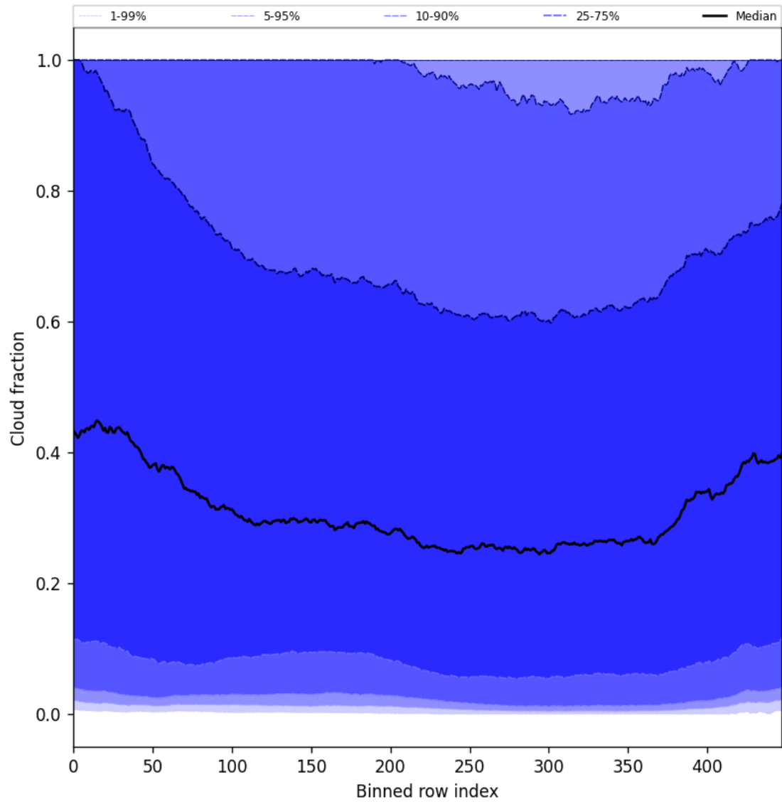
Figure 47: Along track statistics of “Cloud fraction” for 2025-09-04 to 2025-09-05
