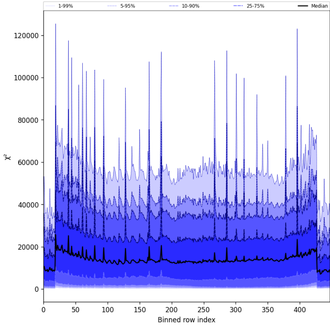
Figure 53: Along track statistics of “ \chi^2 ” for 2025-09-04 to 2025-09-05
