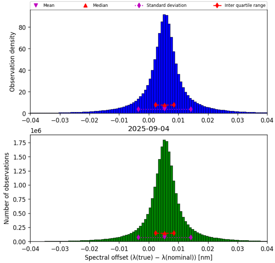
Figure 43: Histogram of “Spectral offset ( \lambda_{\text{true}} - \lambda_{\text{nominal}} )” for 2025-09-04 to 2025-09-05
