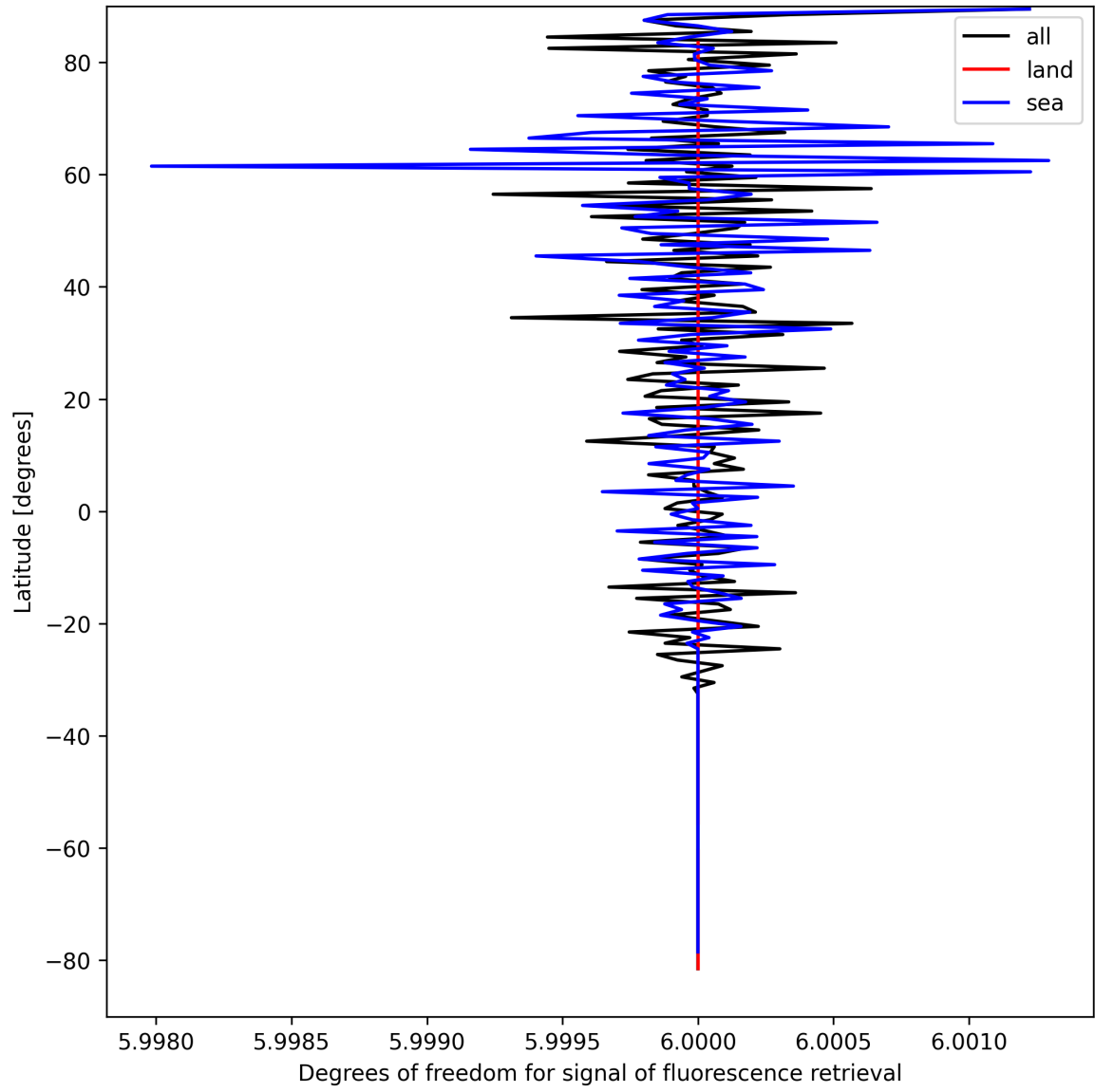
Figure 24: Zonal average of “Degrees of freedom for signal of fluorescence retrieval” for 2025-09-04 to 2025-09-05.
