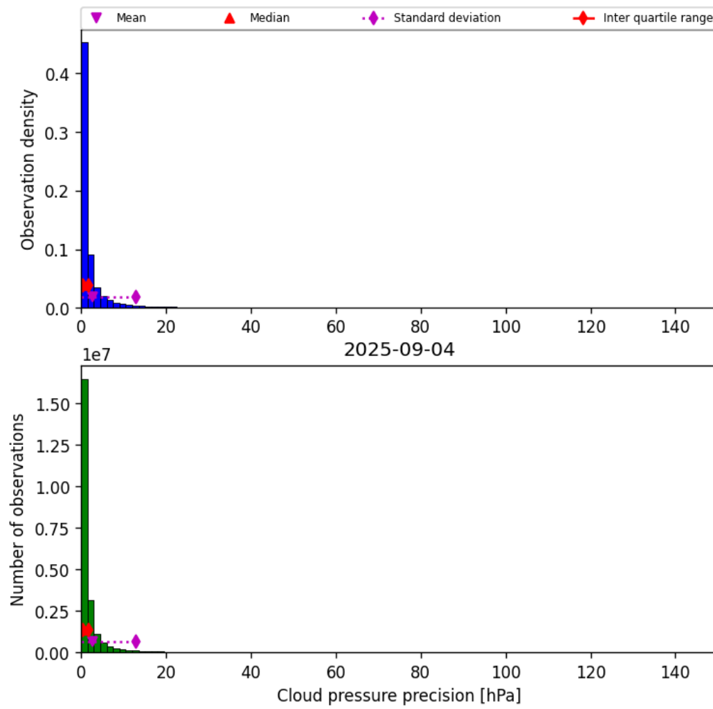
Figure 29: Histogram of “Cloud pressure precision” for 2025-09-04 to 2025-09-05
