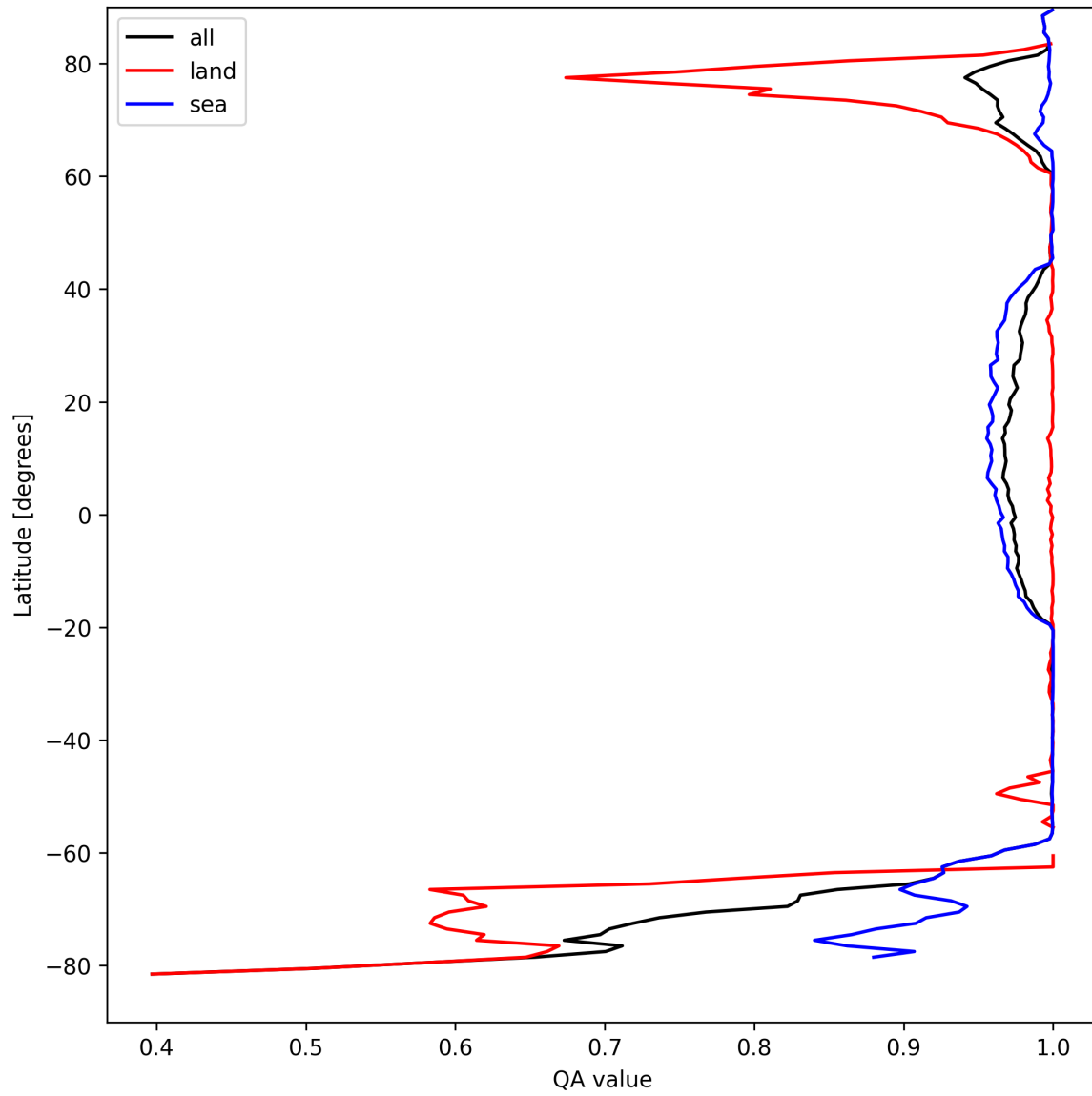
Figure 10: Zonal average of “QA value” for 2025-09-04 to 2025-09-05.
