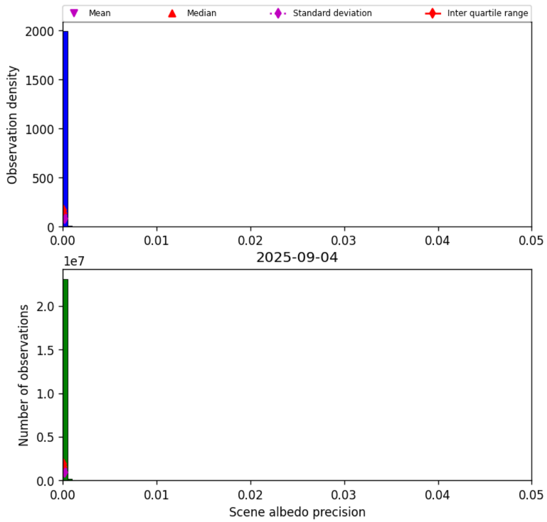
Figure 33: Histogram of “Scene albedo precision” for 2025-09-04 to 2025-09-05
