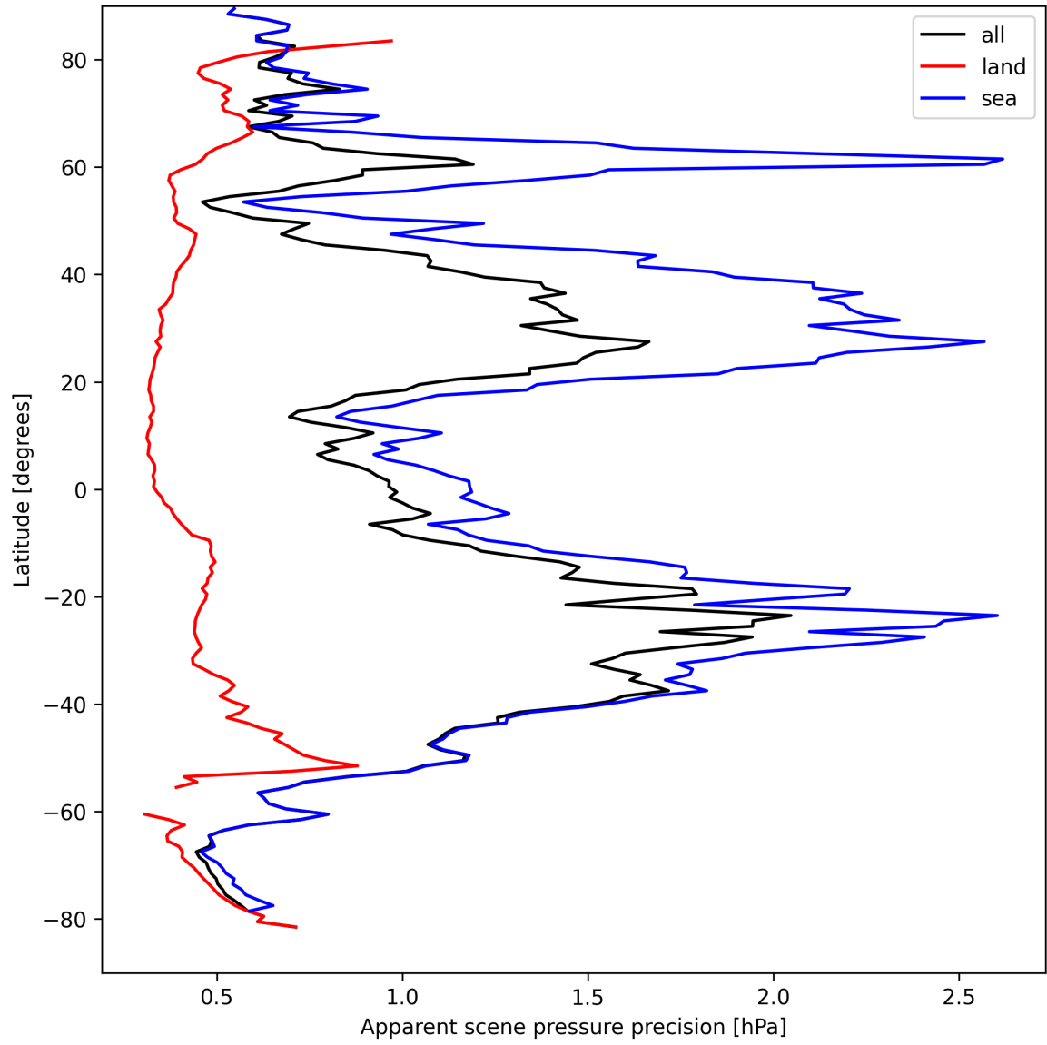
Figure 18: Zonal average of “Apparent scene pressure precision” for 2025-09-04 to 2025-09-05.
