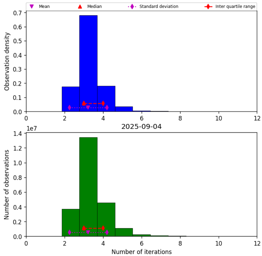
Figure 37: Histogram of “Number of iterations” for 2025-09-04 to 2025-09-05
