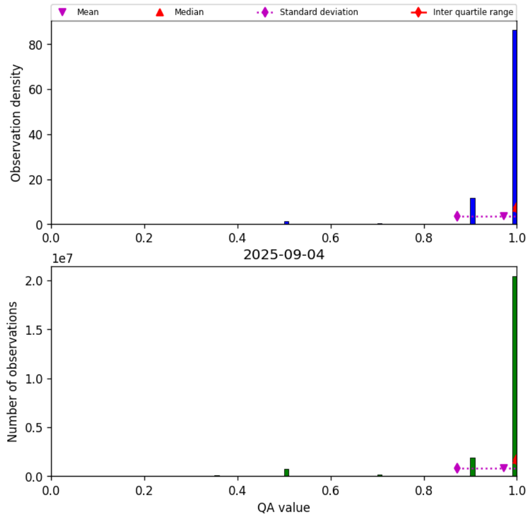
Figure 27: Histogram of “QA value” for 2025-09-04 to 2025-09-05
