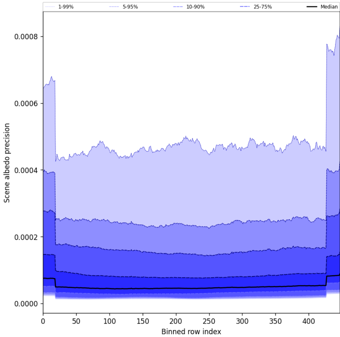
Figure 50: Along track statistics of “Scene albedo precision” for 2025-09-04 to 2025-09-05
