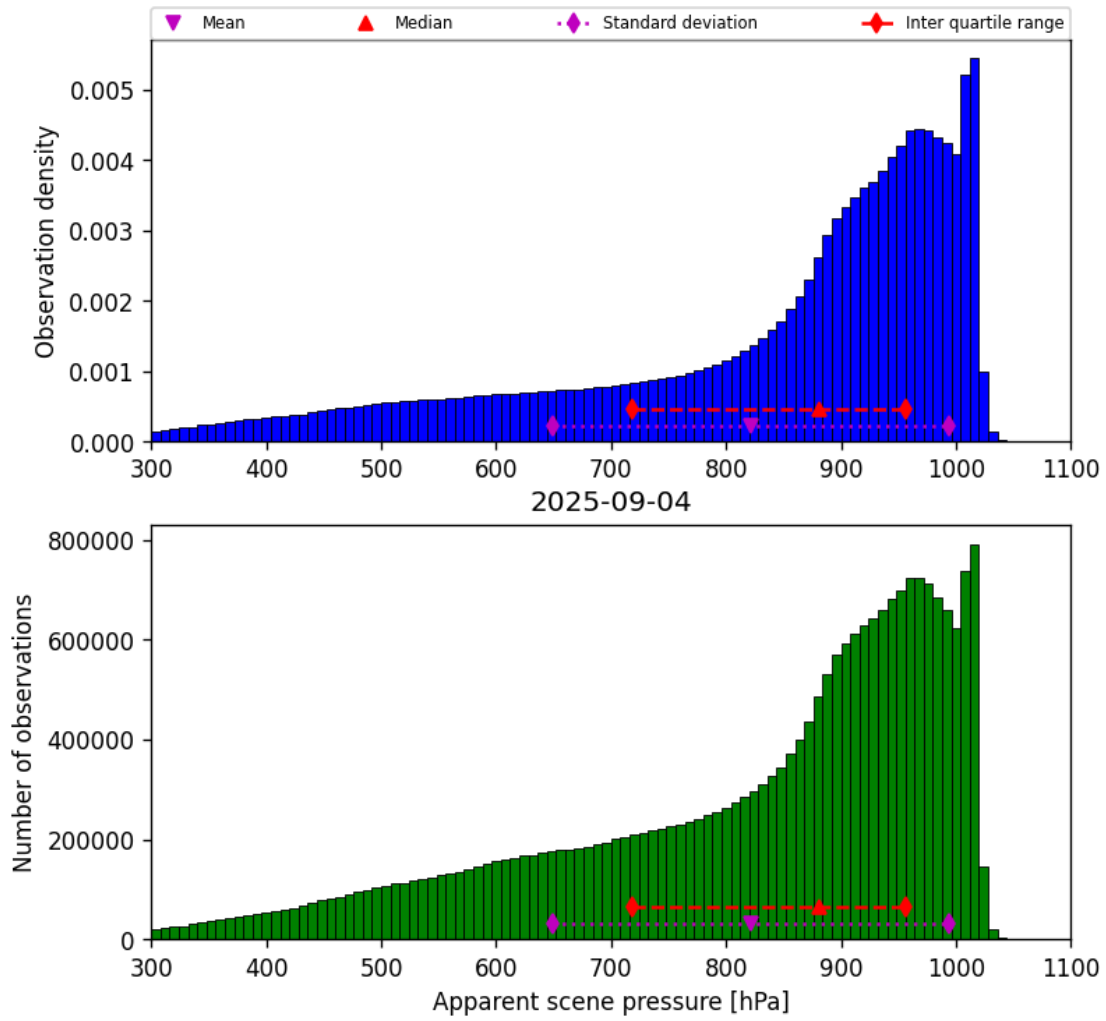
Figure 34: Histogram of “Apparent scene pressure” for 2025-09-04 to 2025-09-05
