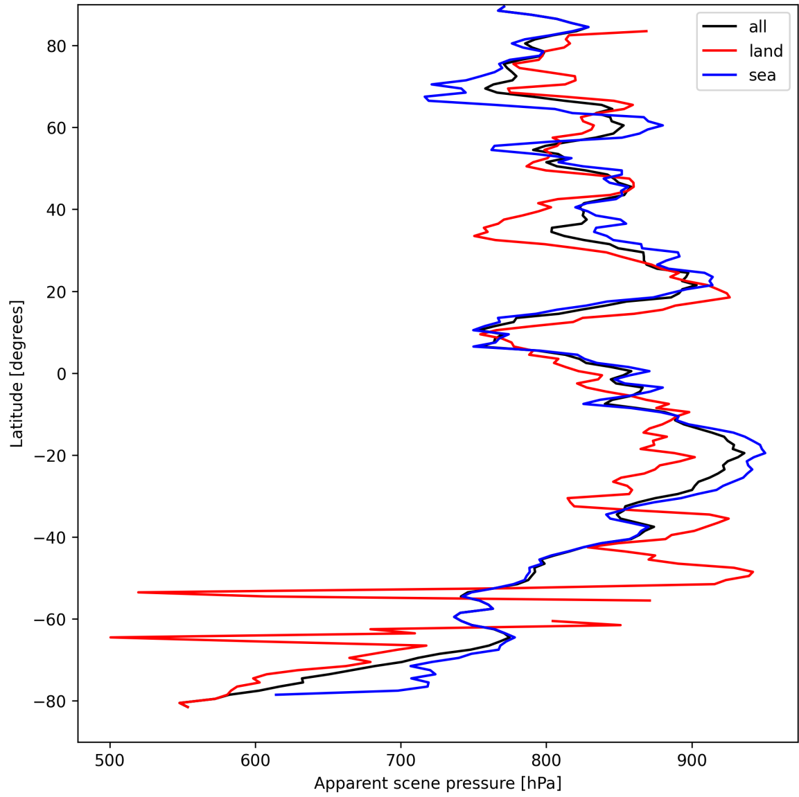
Figure 17: Zonal average of “Apparent scene pressure” for 2025-09-04 to 2025-09-05.
