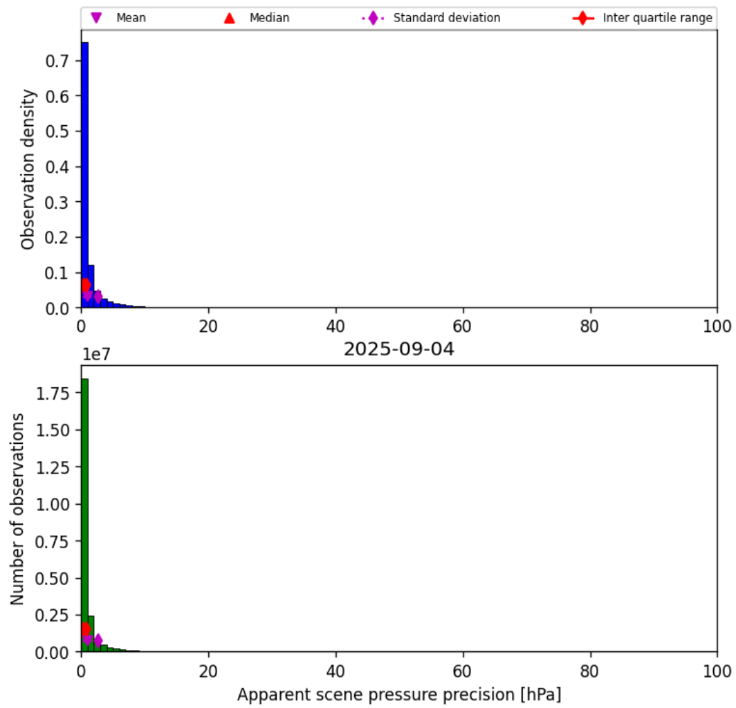
Figure 35: Histogram of “Apparent scene pressure precision” for 2025-09-04 to 2025-09-05
