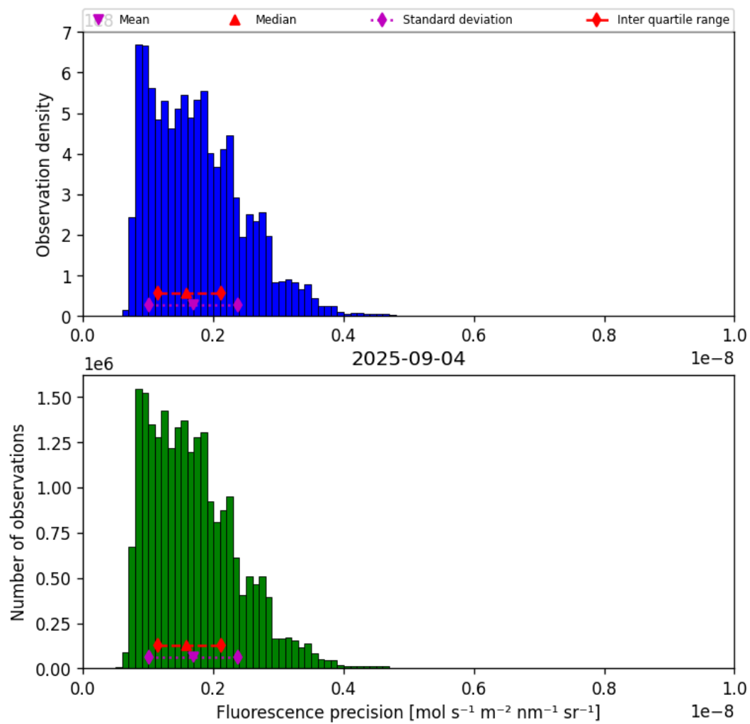
Figure 39: Histogram of “Fluorescence precision” for 2025-09-04 to 2025-09-05
