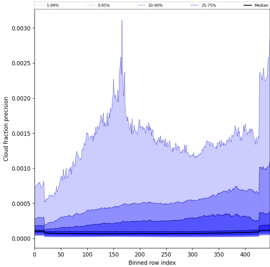
Figure 48: Along track statistics of “Cloud fraction precision” for 2025-09-04 to 2025-09-05
