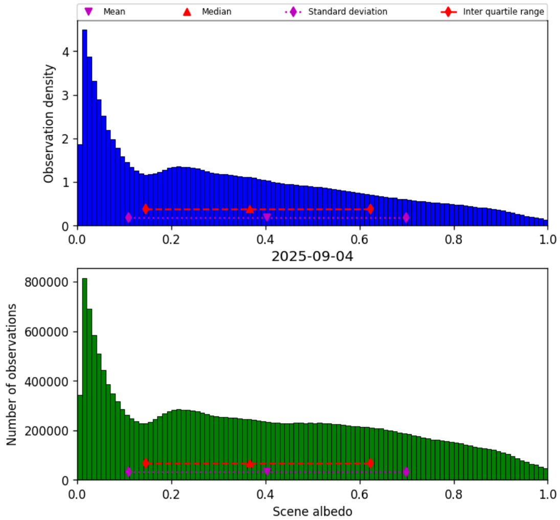
Figure 32: Histogram of “Scene albedo” for 2025-09-04 to 2025-09-05
