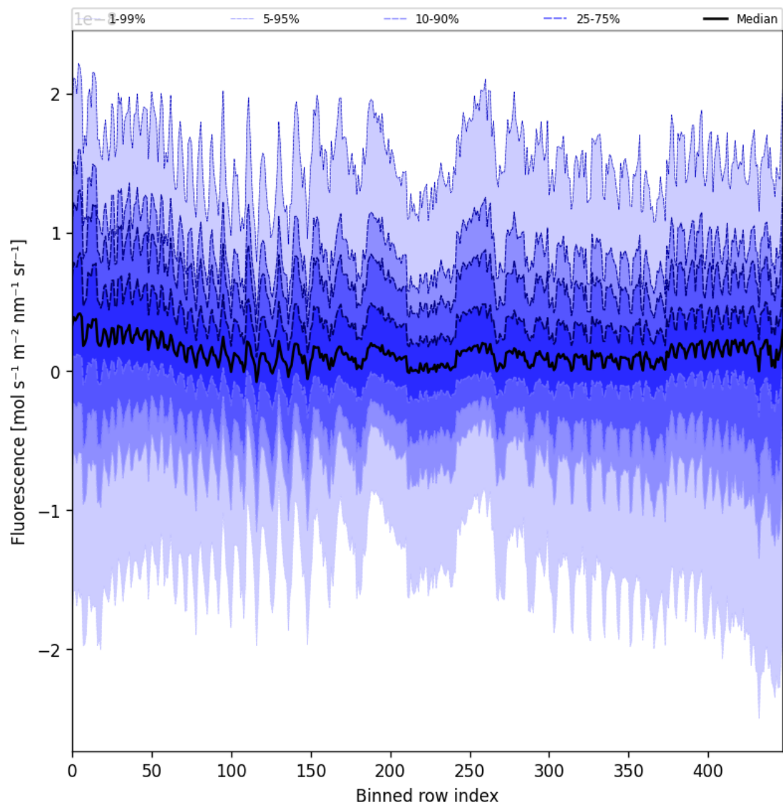
Figure 55: Along track statistics of “Fluorescence” for 2025-09-04 to 2025-09-05
