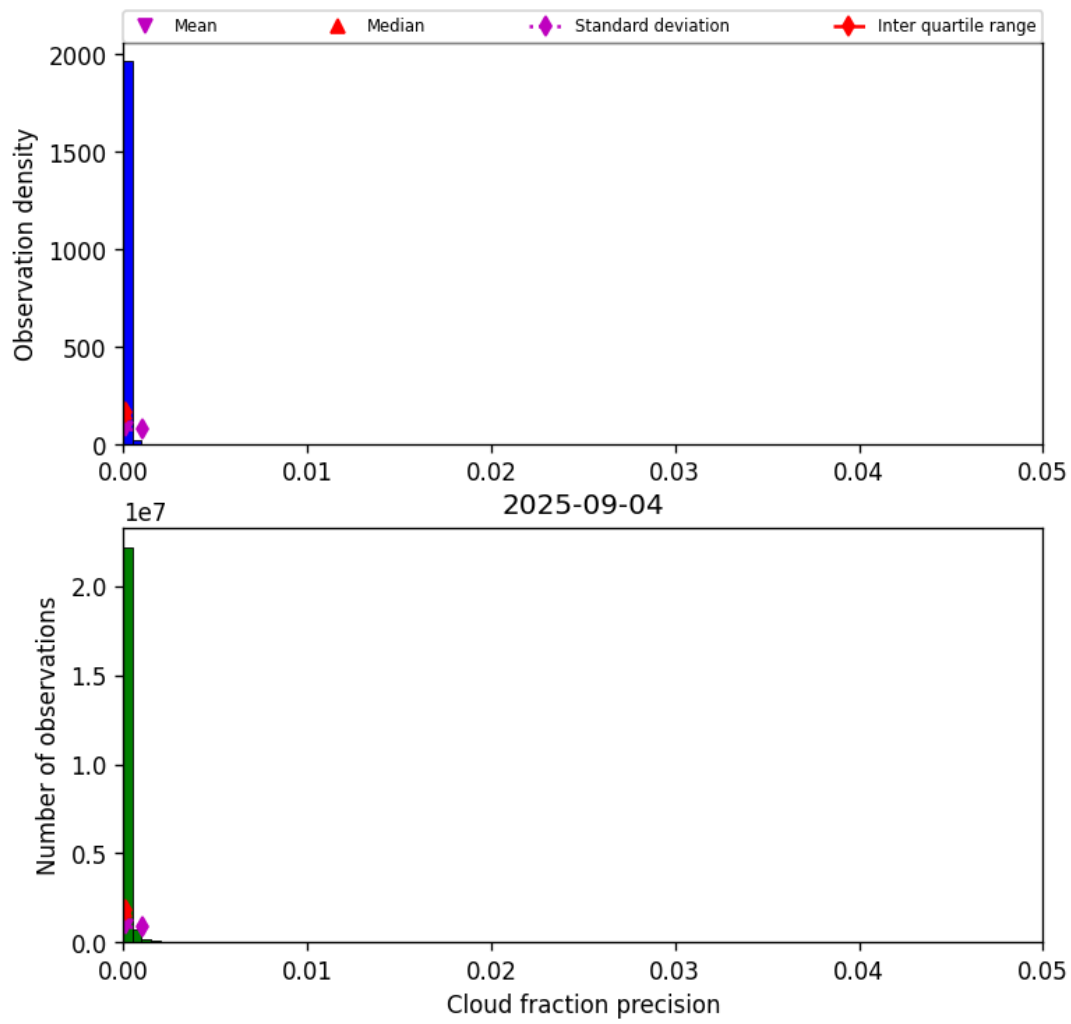
Figure 31: Histogram of “Cloud fraction precision” for 2025-09-04 to 2025-09-05
