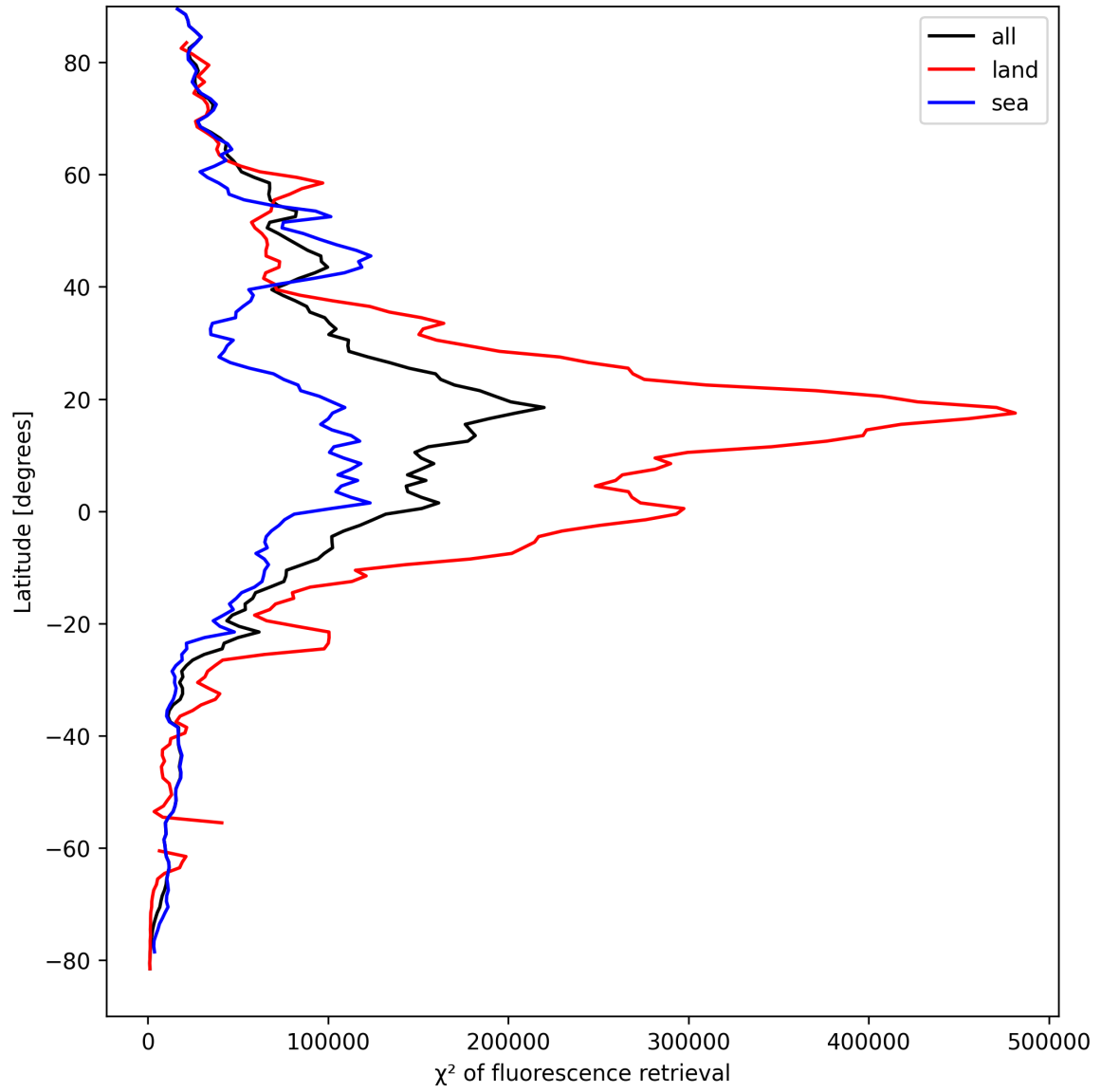
Figure 23: Zonal average of “ \chi^2 of fluorescence retrieval” for 2025-09-04 to 2025-09-05.
