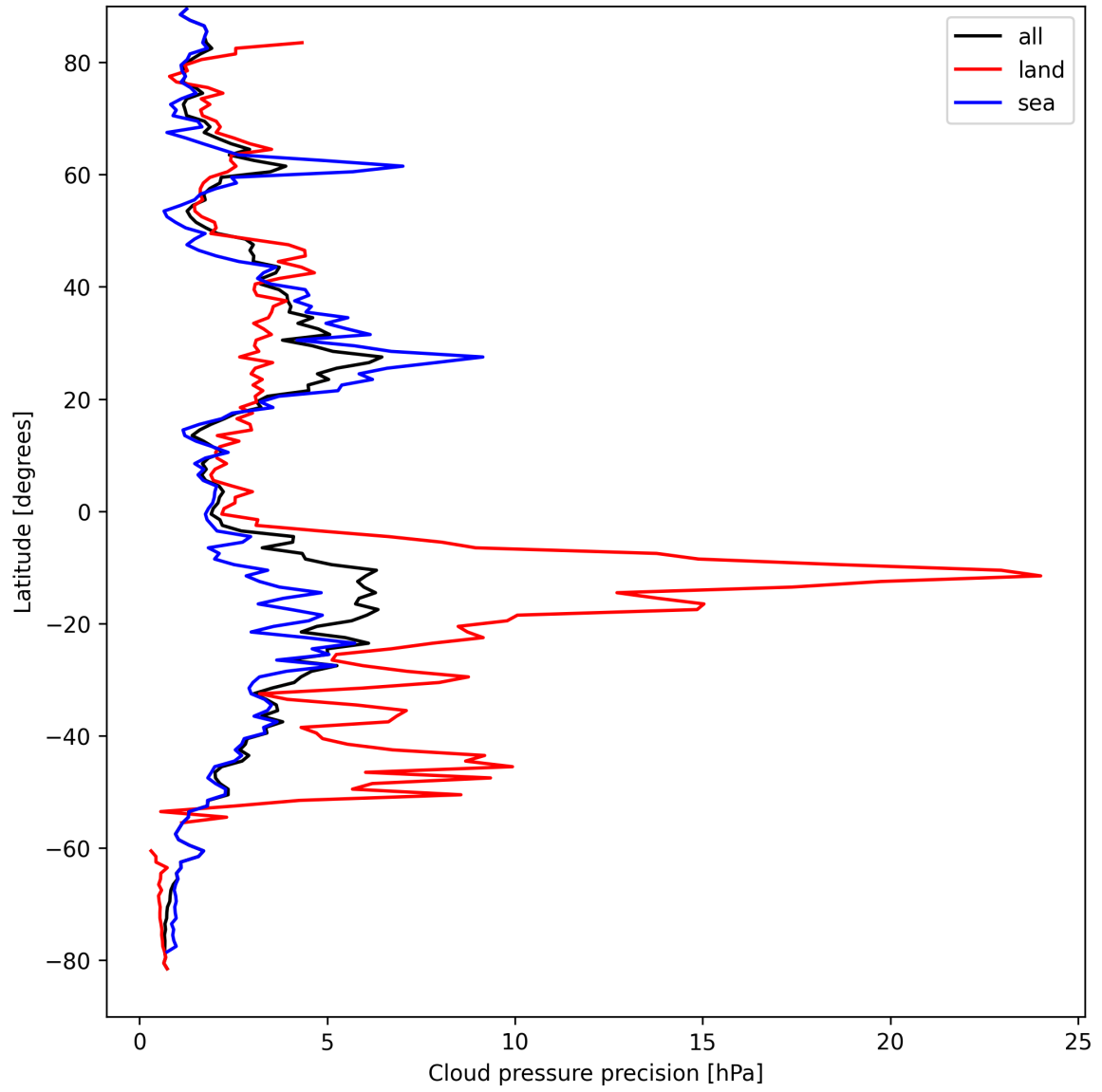
Figure 12: Zonal average of "Cloud pressure precision" for 2025-09-04 to 2025-09-05.
