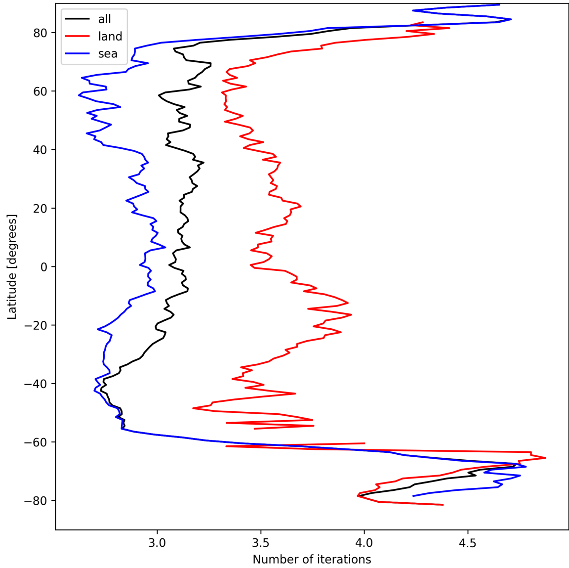
Figure 20: Zonal average of “Number of iterations” for 2025-09-04 to 2025-09-05.
