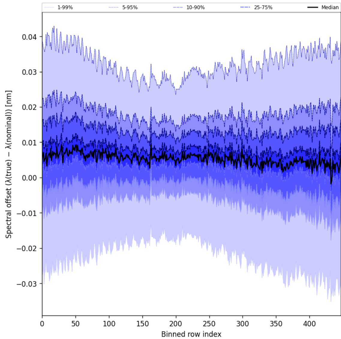
Figure 60: Along track statistics of “Spectral offset ( \lambda_{\text{true}} - \lambda_{\text{nominal}} )” for 2025-09-04 to 2025-09-05
