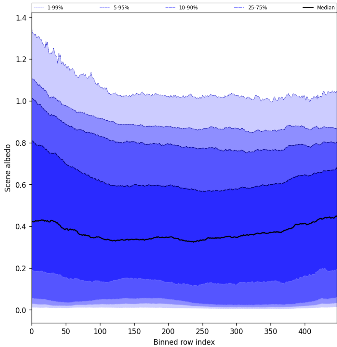
Figure 49: Along track statistics of "Scene albedo" for 2025-09-04 to 2025-09-05
