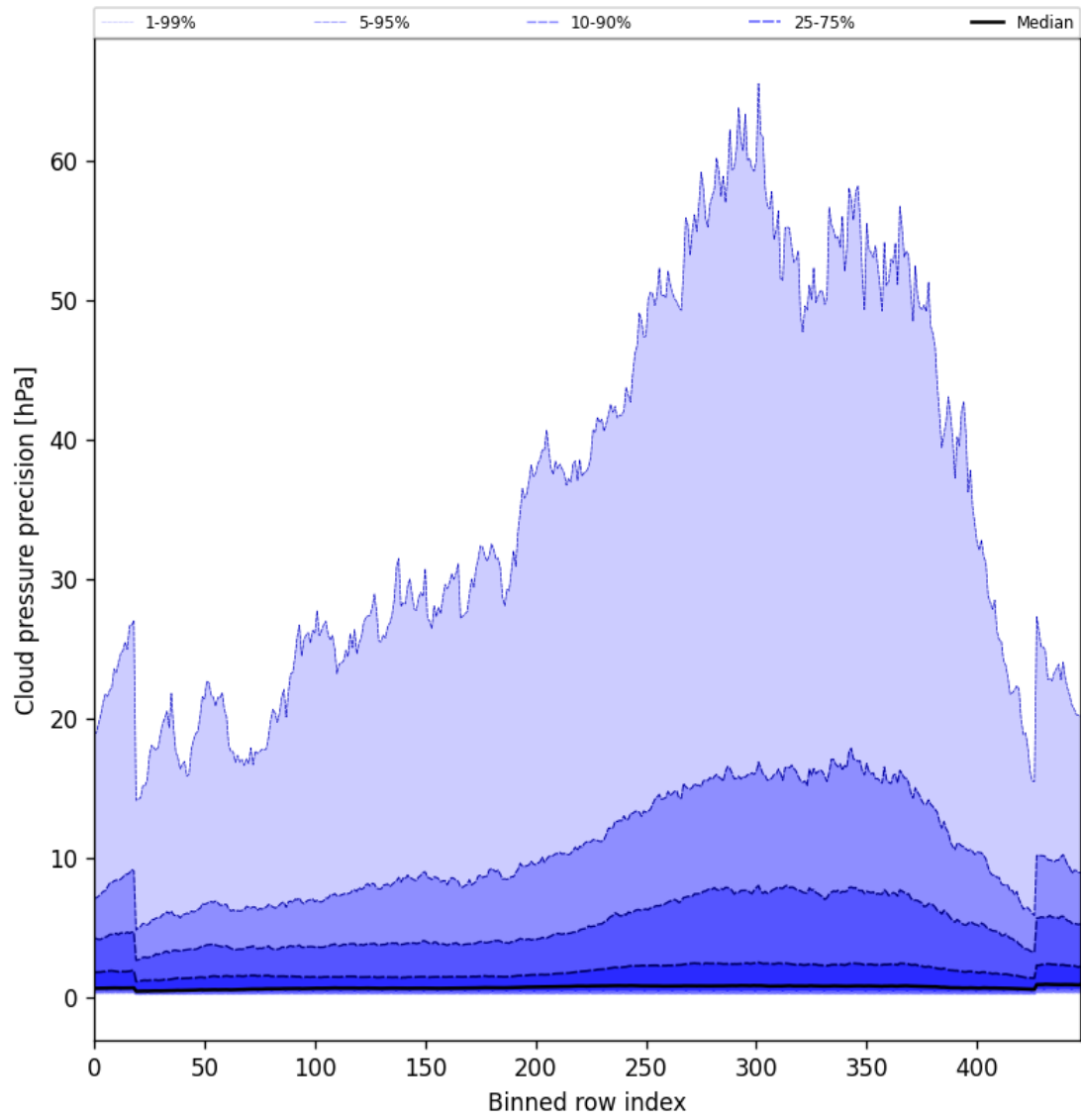
Figure 46: Along track statistics of “Cloud pressure precision” for 2025-09-04 to 2025-09-05
