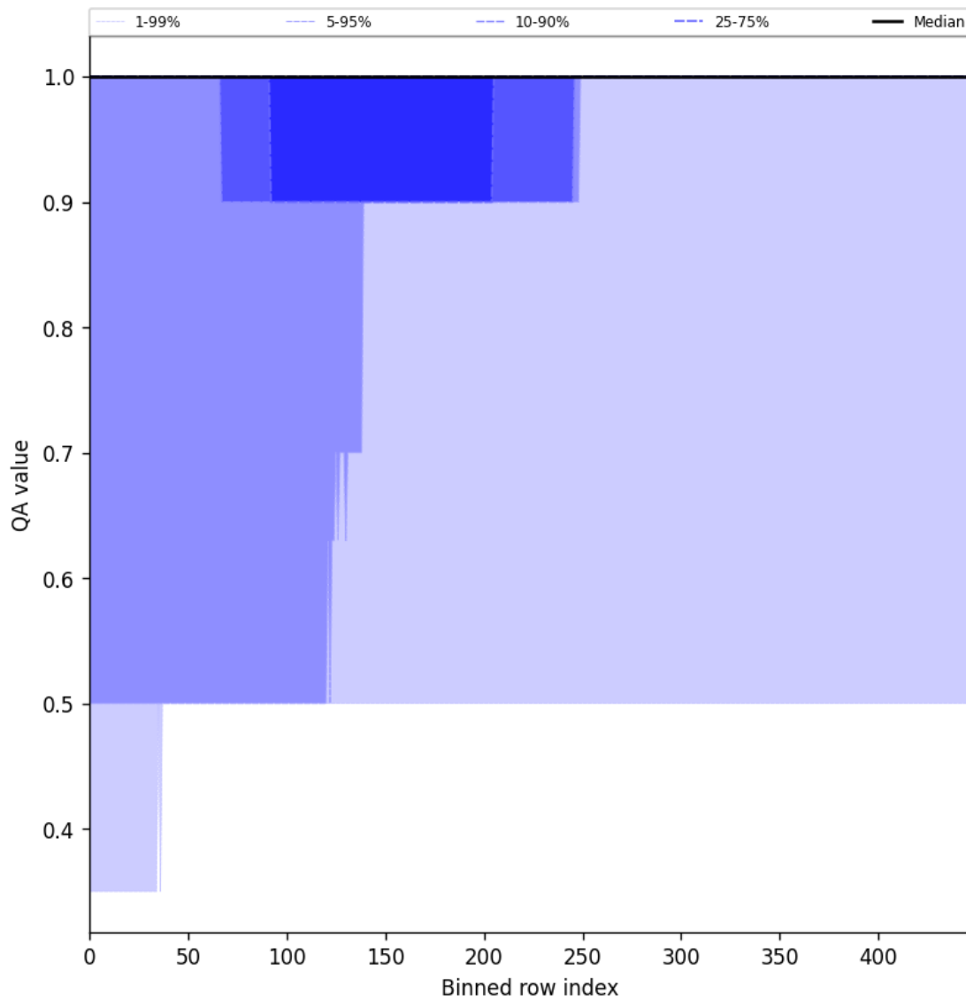
Figure 44: Along track statistics of “QA value” for 2025-09-04 to 2025-09-05
