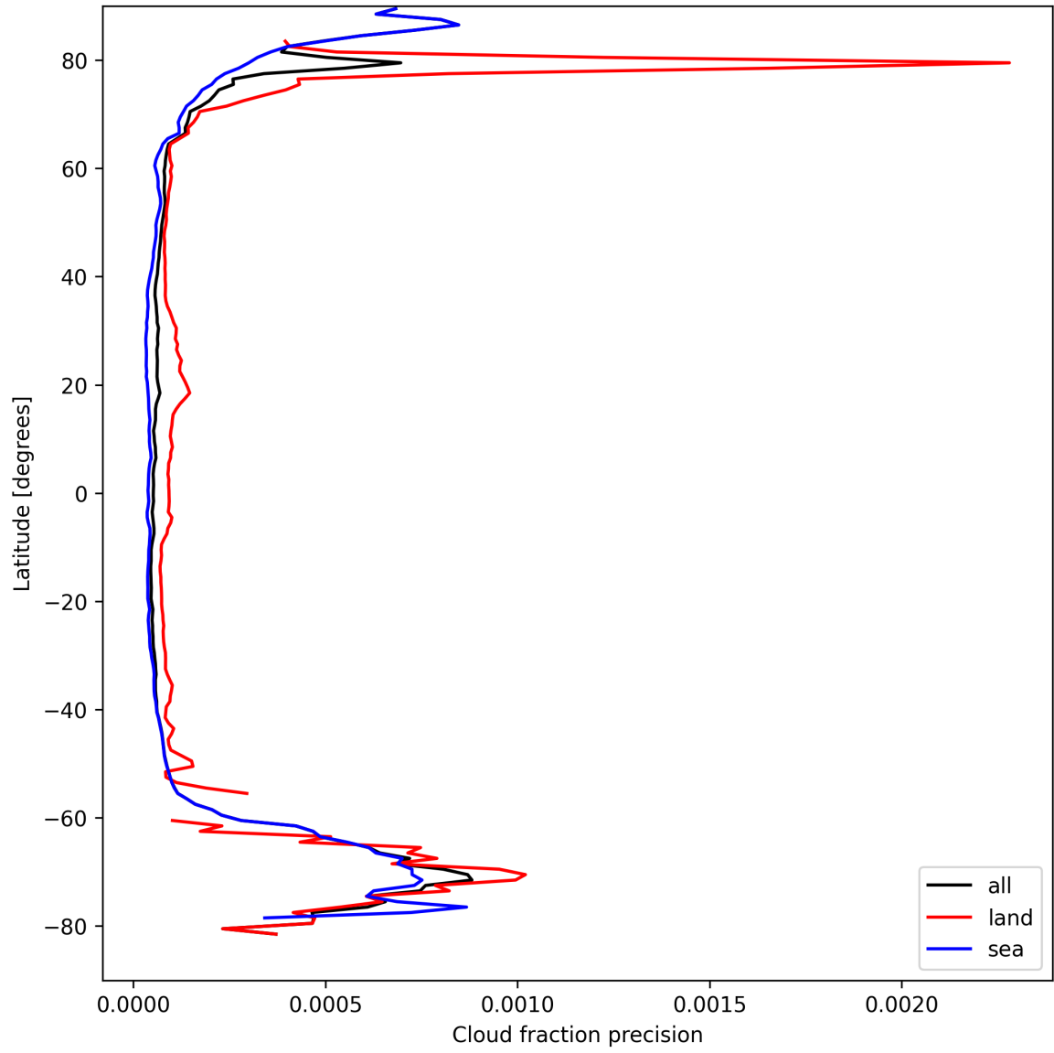
Figure 14: Zonal average of “Cloud fraction precision” for 2025-09-04 to 2025-09-05.
