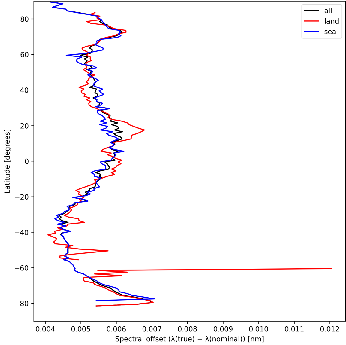
Figure 26: Zonal average of “Spectral offset ( \lambda_{\text{true}} - \lambda_{\text{nominal}} )” for 2025-09-04 to 2025-09-05.
