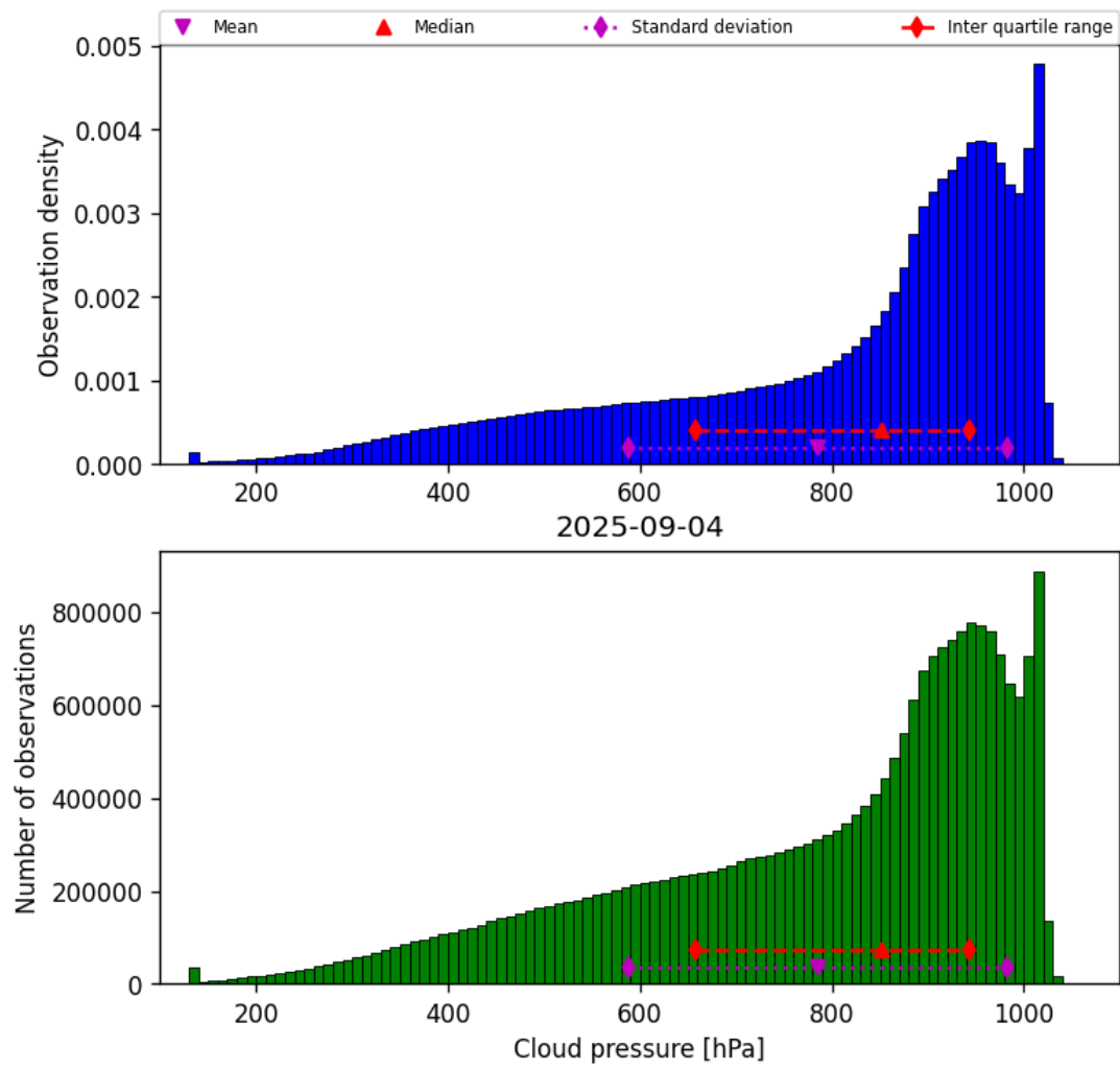
Figure 28: Histogram of “Cloud pressure” for 2025-09-04 to 2025-09-05
