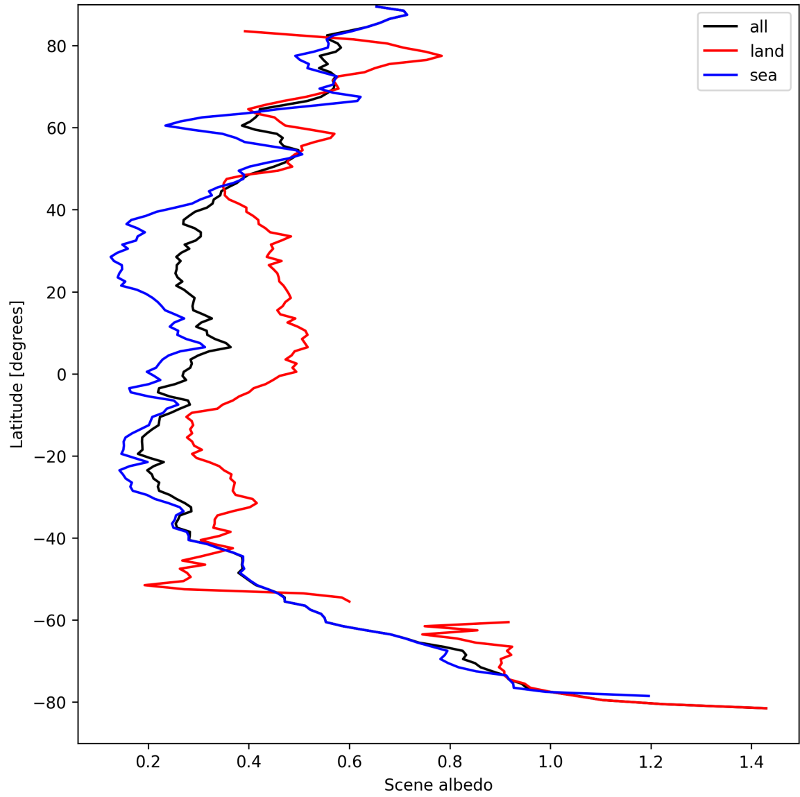
Figure 15: Zonal average of “Scene albedo” for 2025-09-04 to 2025-09-05.
