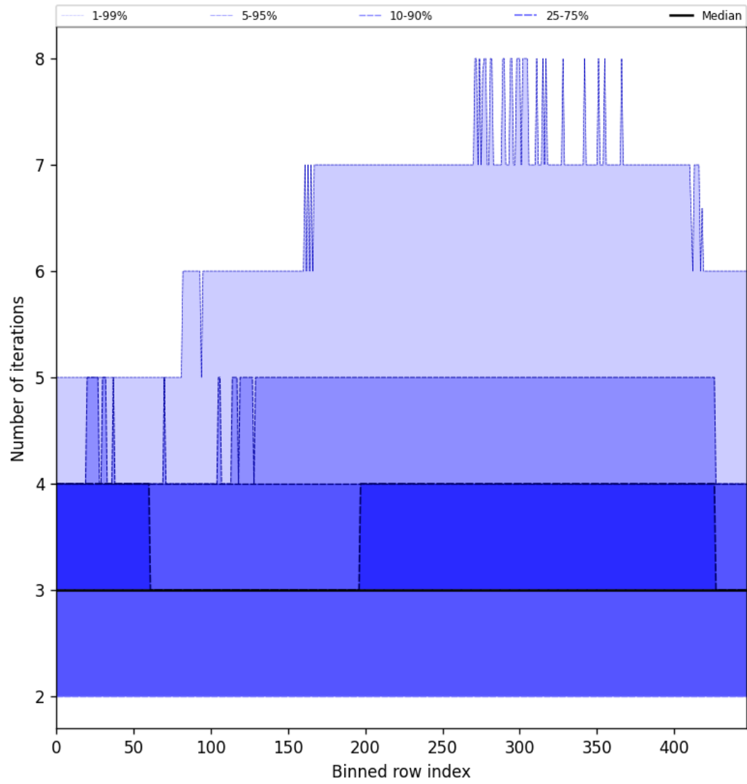
Figure 54: Along track statistics of “Number of iterations” for 2025-09-04 to 2025-09-05
