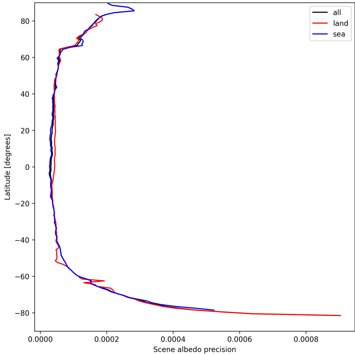
Figure 16: Zonal average of “Scene albedo precision” for 2025-09-04 to 2025-09-05.
