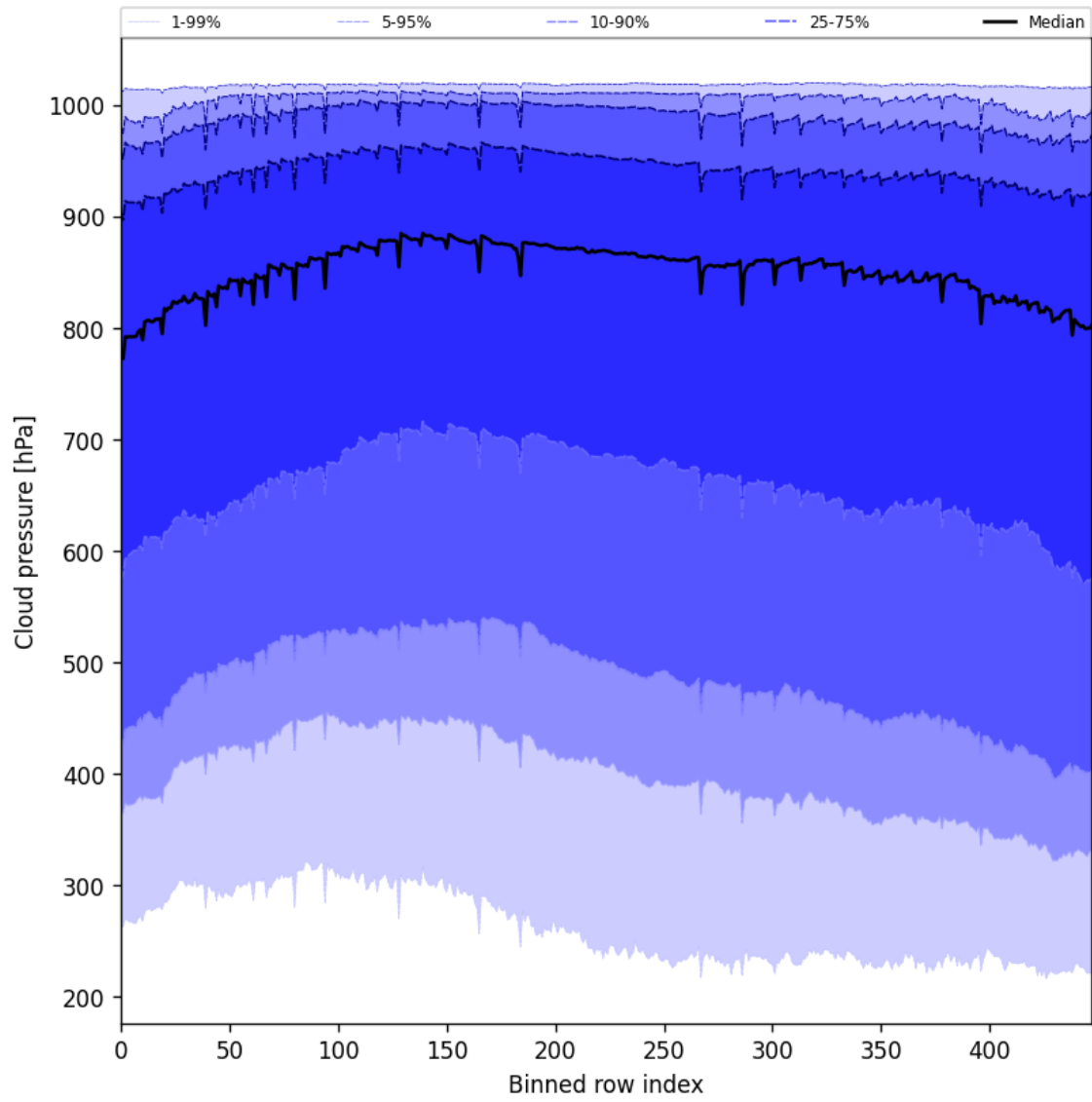
Figure 45: Along track statistics of “Cloud pressure” for 2025-09-04 to 2025-09-05
