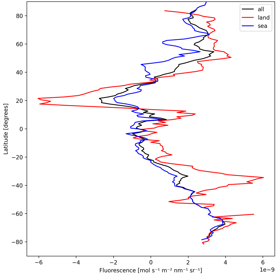
Figure 21: Zonal average of “Fluorescence” for 2025-09-04 to 2025-09-05.
