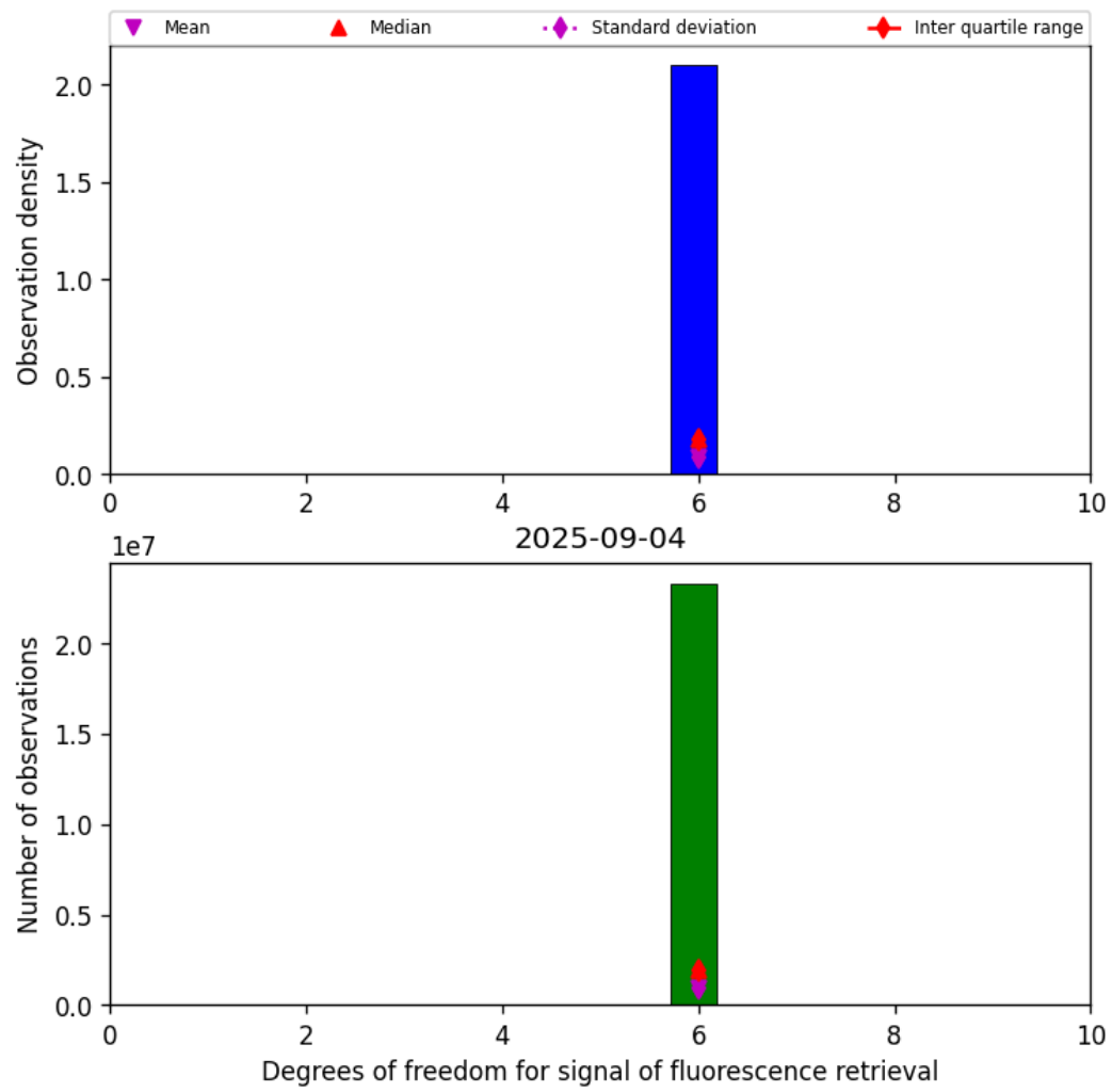
Figure 41: Histogram of “Degrees of freedom for signal of fluorescence retrieval” for 2025-09-04 to 2025-09-05
