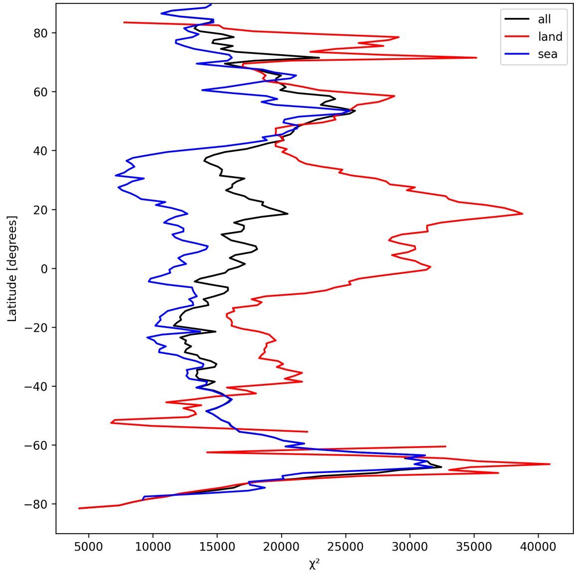
Figure 19: Zonal average of “ \chi^2 ” for 2025-09-04 to 2025-09-05.
