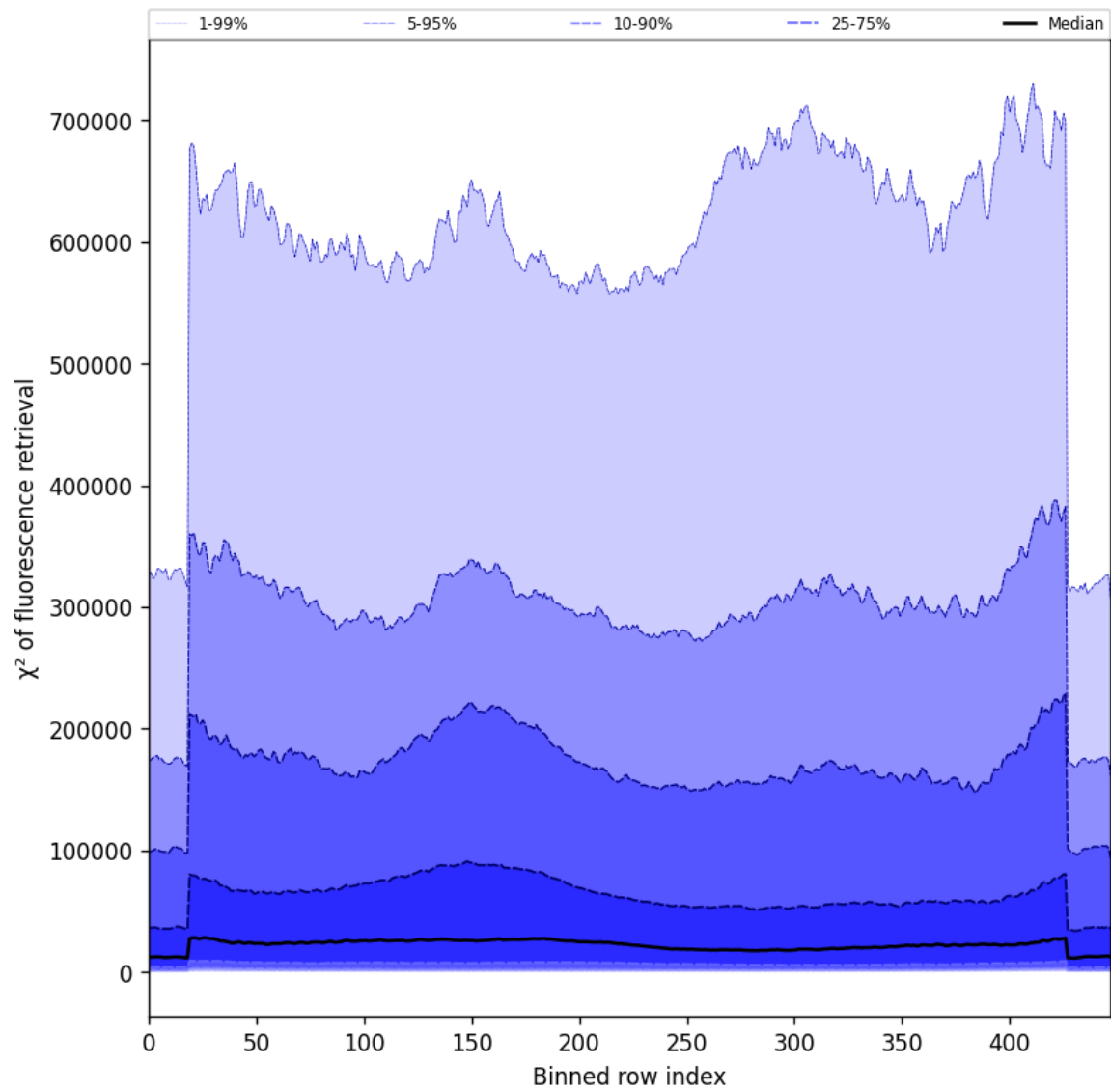
Figure 57: Along track statistics of “ \chi^2 of fluorescence retrieval” for 2025-09-04 to 2025-09-05
