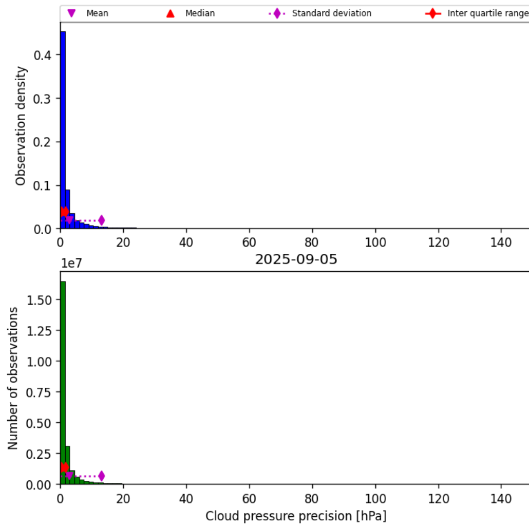
Figure 29: Histogram of “Cloud pressure precision” for 2025-09-05 to 2025-09-06
