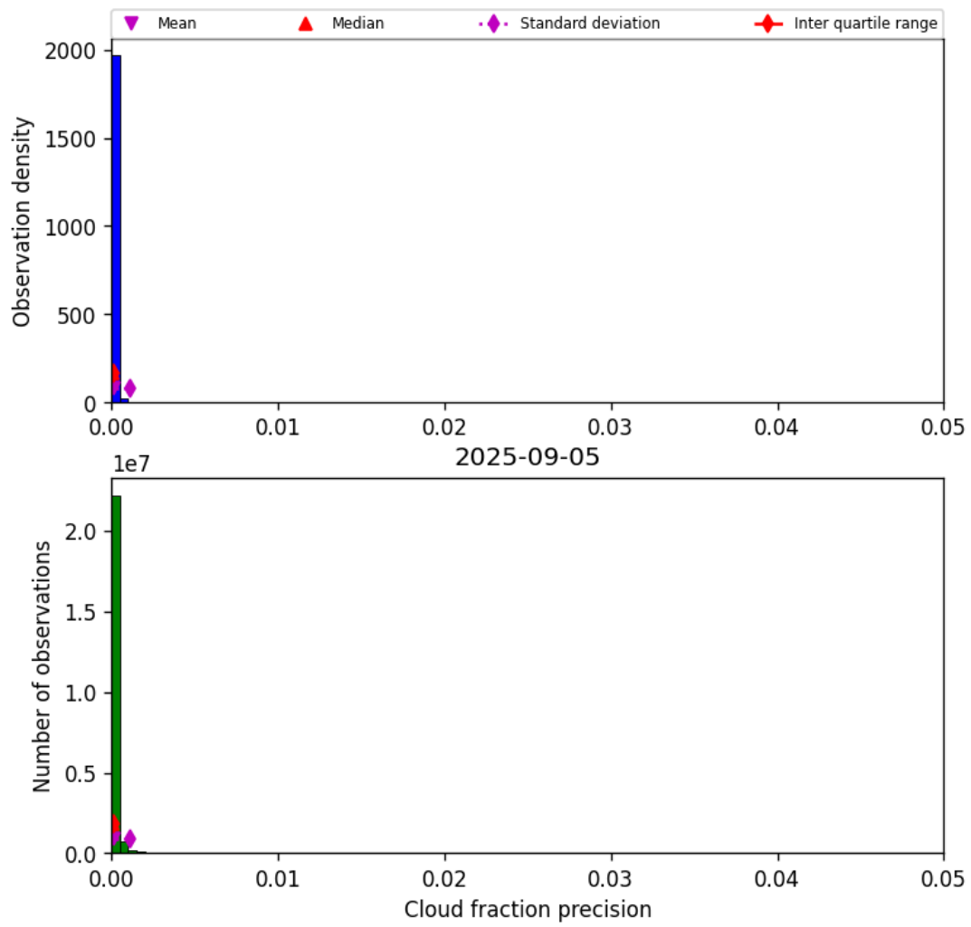
Figure 31: Histogram of “Cloud fraction precision” for 2025-09-05 to 2025-09-06
