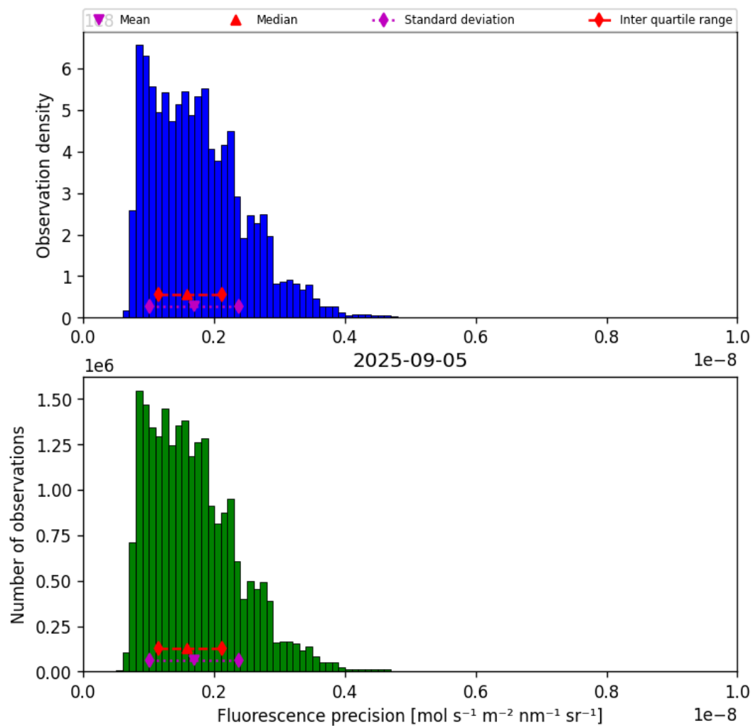
Figure 39: Histogram of “Fluorescence precision” for 2025-09-05 to 2025-09-06
