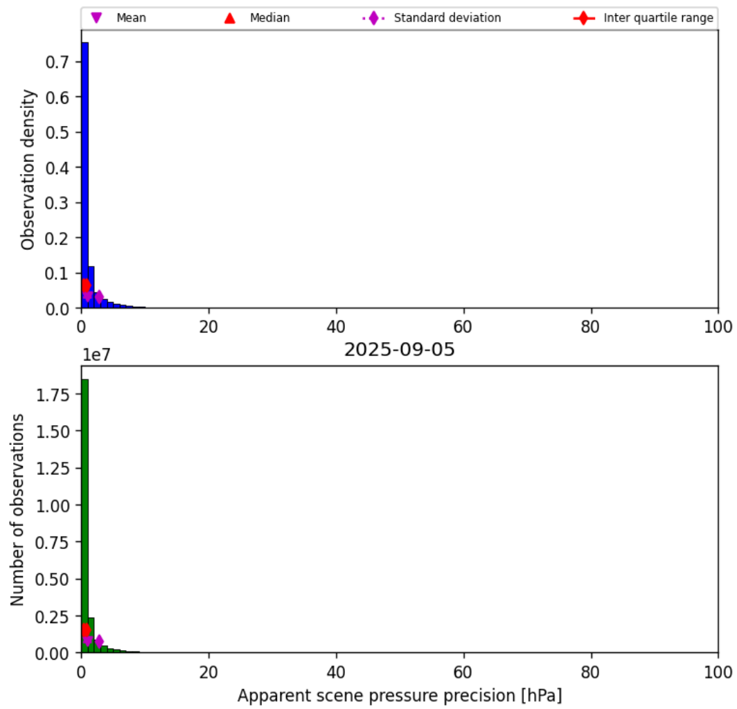
Figure 35: Histogram of “Apparent scene pressure precision” for 2025-09-05 to 2025-09-06
