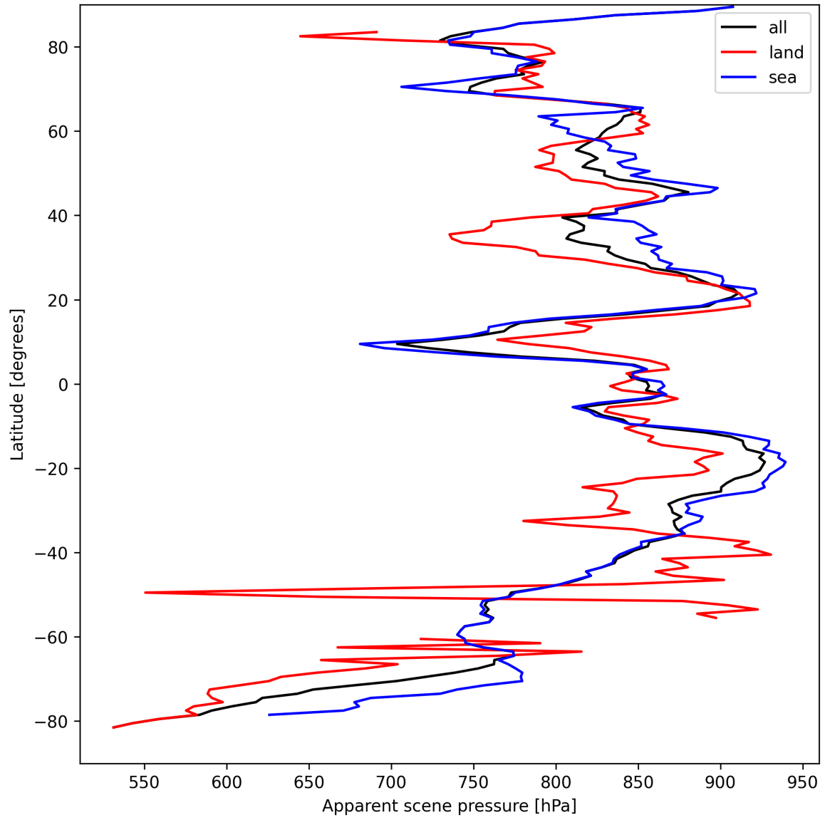
Figure 17: Zonal average of “Apparent scene pressure” for 2025-09-05 to 2025-09-06.
