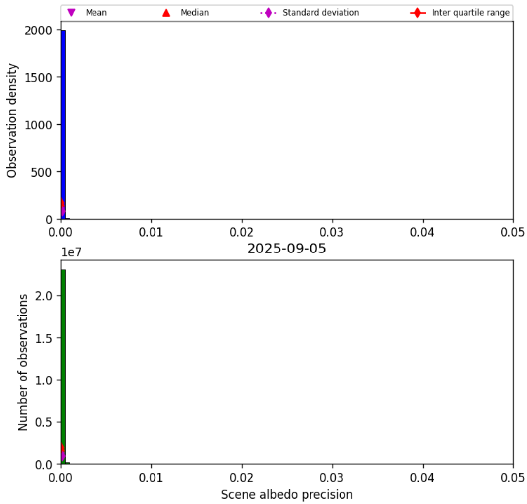
Figure 33: Histogram of “Scene albedo precision” for 2025-09-05 to 2025-09-06
