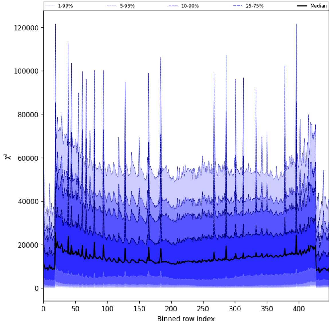
Figure 53: Along track statistics of “ \chi^2 ” for 2025-09-05 to 2025-09-06
