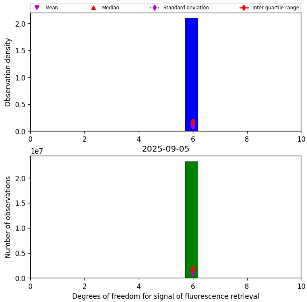
Figure 41: Histogram of “Degrees of freedom for signal of fluorescence retrieval” for 2025-09-05 to 2025-09-06
