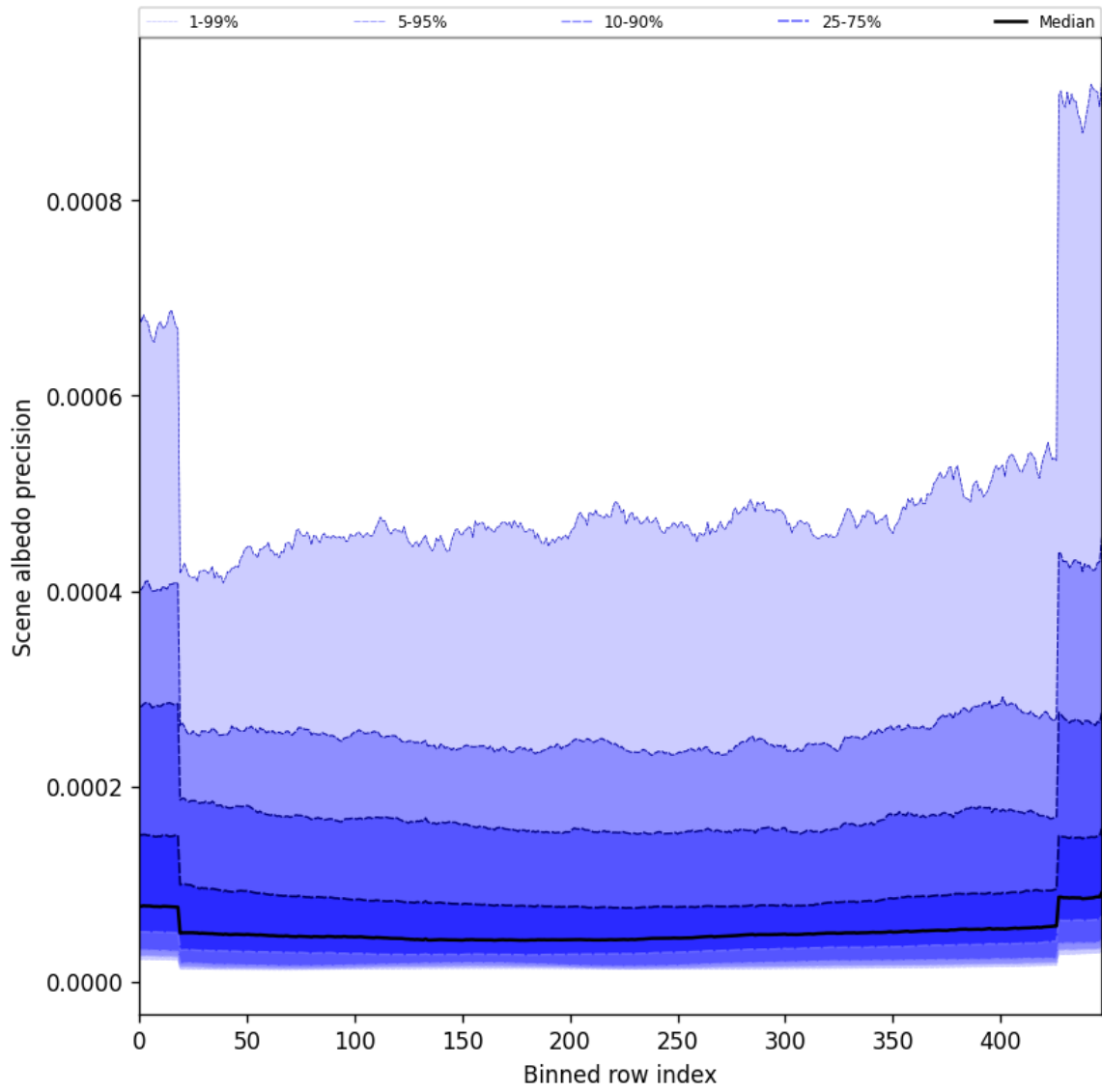
Figure 50: Along track statistics of “Scene albedo precision” for 2025-09-05 to 2025-09-06
