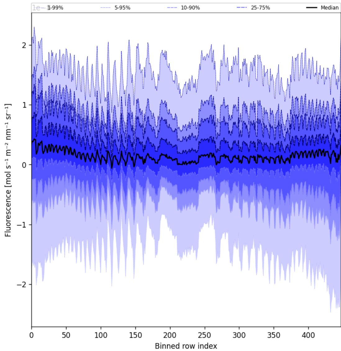
Figure 55: Along track statistics of “Fluorescence” for 2025-09-05 to 2025-09-06
