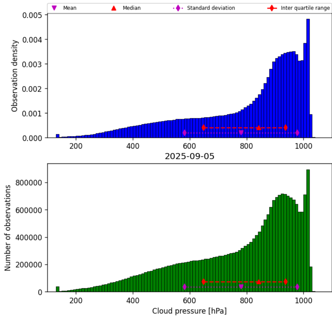
Figure 28: Histogram of “Cloud pressure” for 2025-09-05 to 2025-09-06
