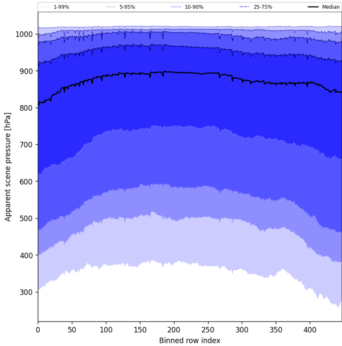
Figure 51: Along track statistics of “Apparent scene pressure” for 2025-09-05 to 2025-09-06
