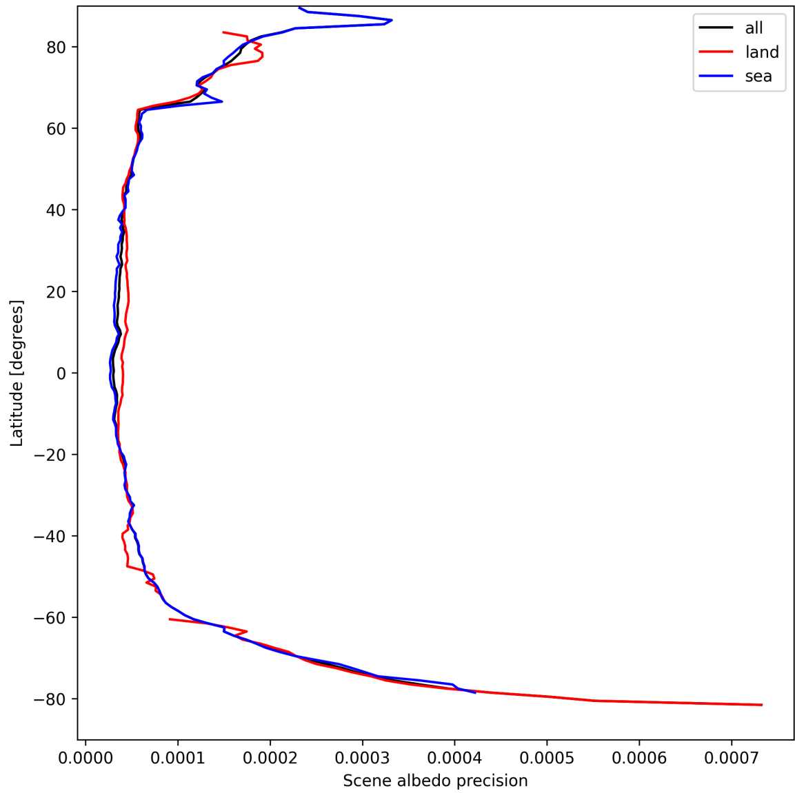
Figure 16: Zonal average of “Scene albedo precision” for 2025-09-05 to 2025-09-06.
