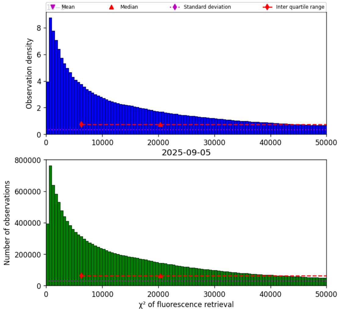
Figure 40: Histogram of “ \chi^2 of fluorescence retrieval” for 2025-09-05 to 2025-09-06
