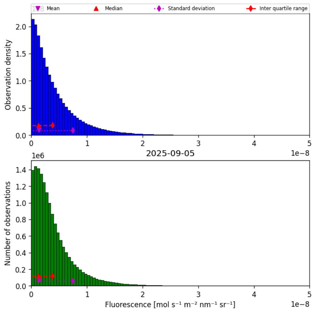
Figure 38: Histogram of “Fluorescence” for 2025-09-05 to 2025-09-06
