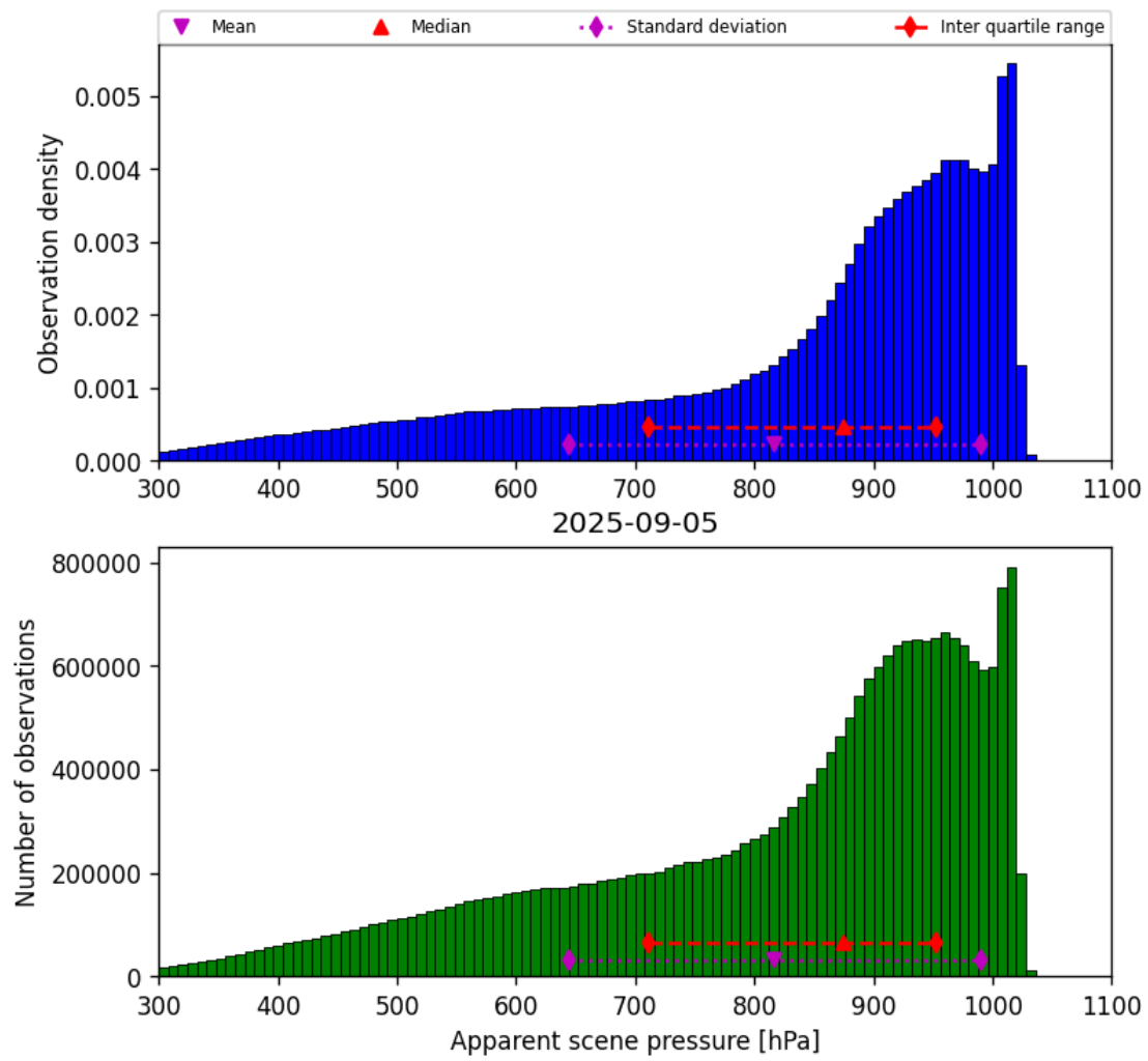
Figure 34: Histogram of “Apparent scene pressure” for 2025-09-05 to 2025-09-06
