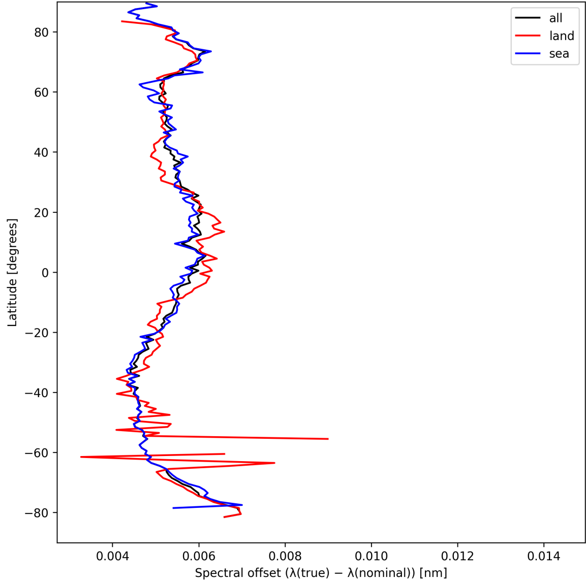
Figure 26: Zonal average of “Spectral offset ( \lambda_{\text{true}} - \lambda_{\text{nominal}} )” for 2025-09-05 to 2025-09-06.
