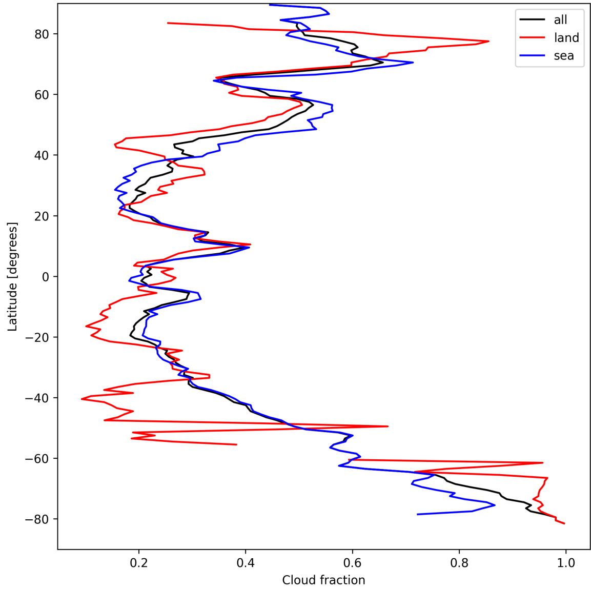
Figure 13: Zonal average of “Cloud fraction” for 2025-09-05 to 2025-09-06.
