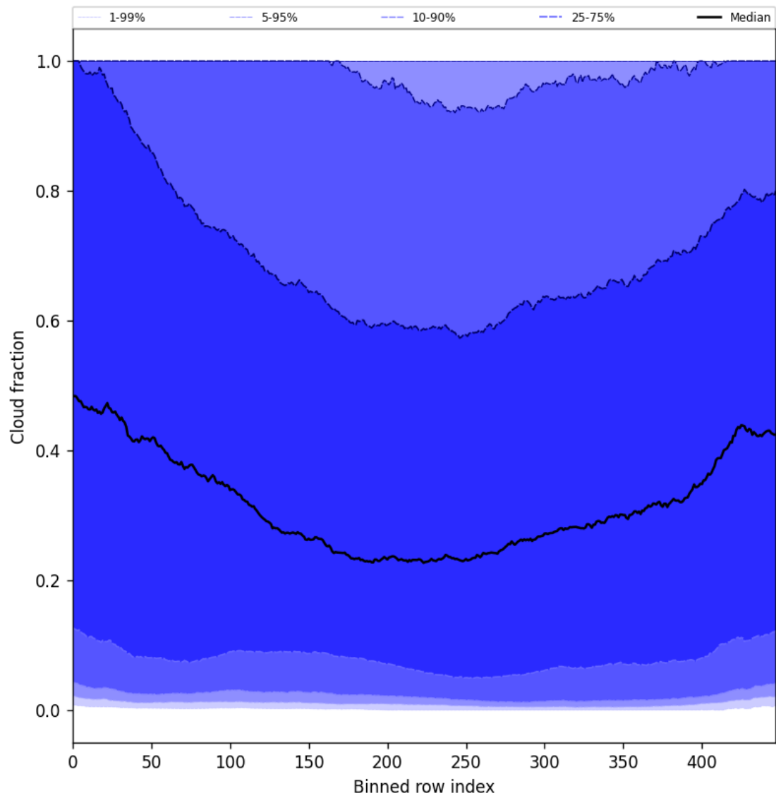
Figure 47: Along track statistics of “Cloud fraction” for 2025-09-05 to 2025-09-06
