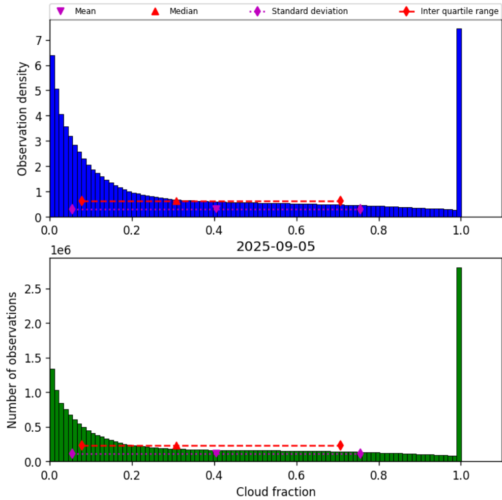
Figure 30: Histogram of “Cloud fraction” for 2025-09-05 to 2025-09-06
