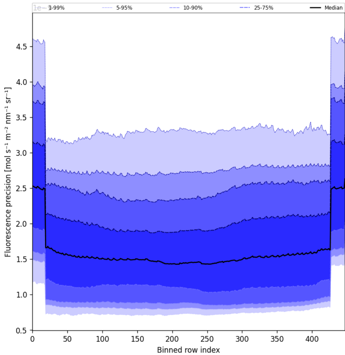
Figure 56: Along track statistics of “Fluorescence precision” for 2025-09-05 to 2025-09-06
