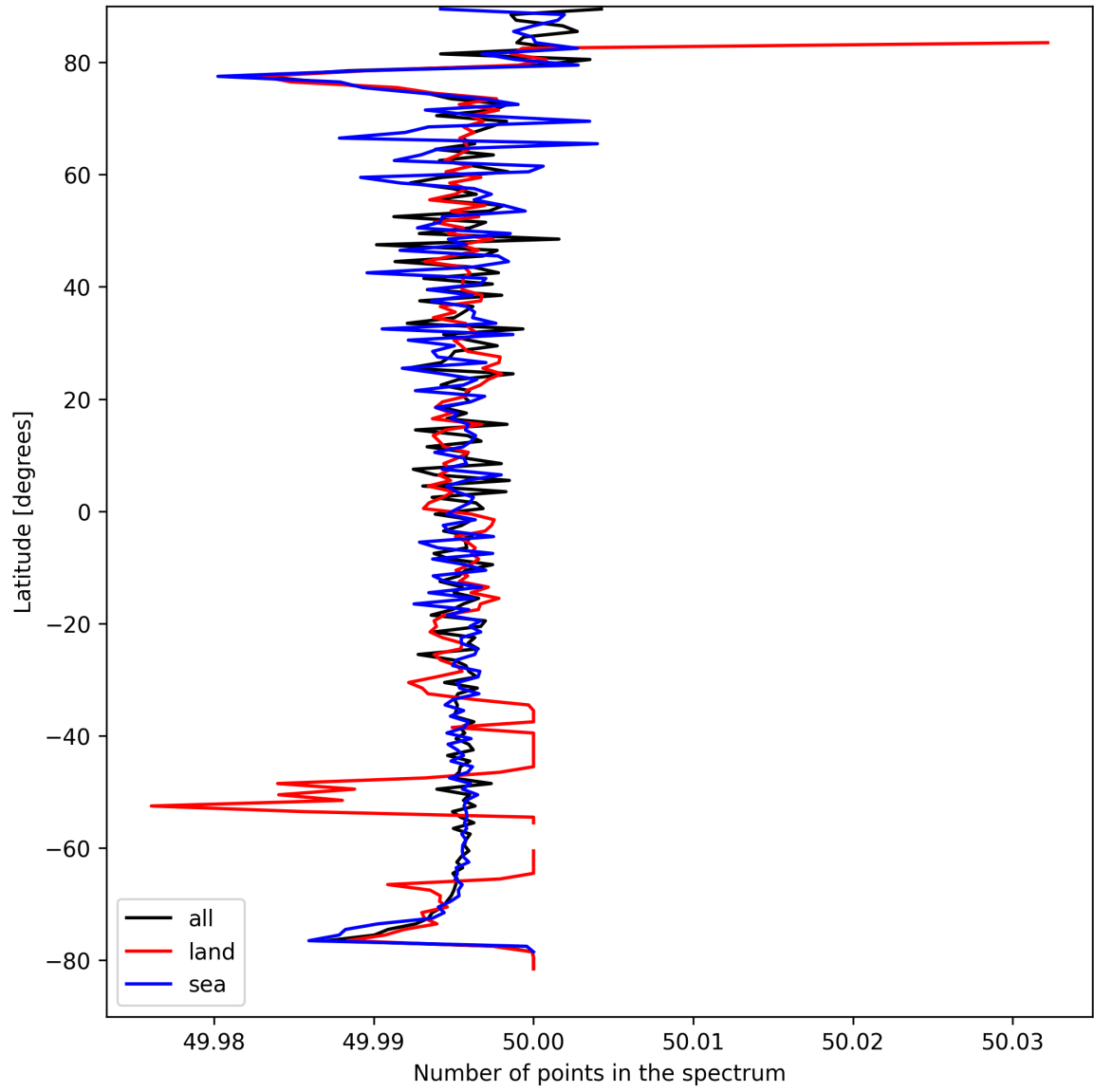
Figure 25: Zonal average of “Number of points in the spectrum” for 2025-09-05 to 2025-09-06.
