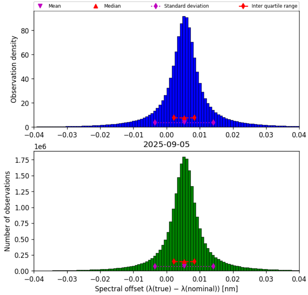
Figure 43: Histogram of “Spectral offset ( \lambda_{\text{true}} - \lambda_{\text{nominal}} )” for 2025-09-05 to 2025-09-06
