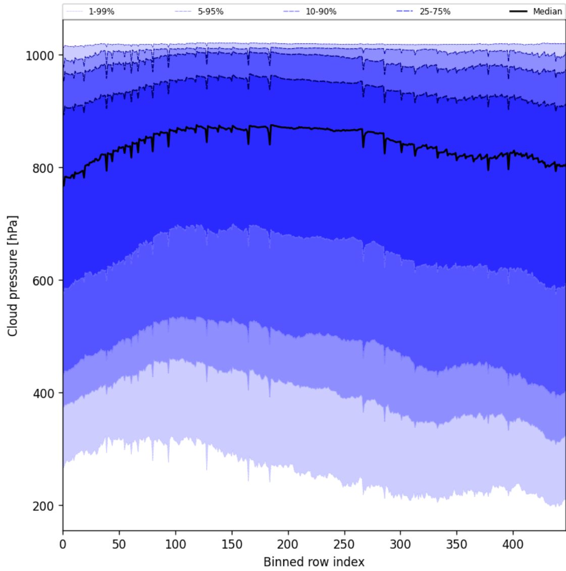
Figure 45: Along track statistics of “Cloud pressure” for 2025-09-05 to 2025-09-06
