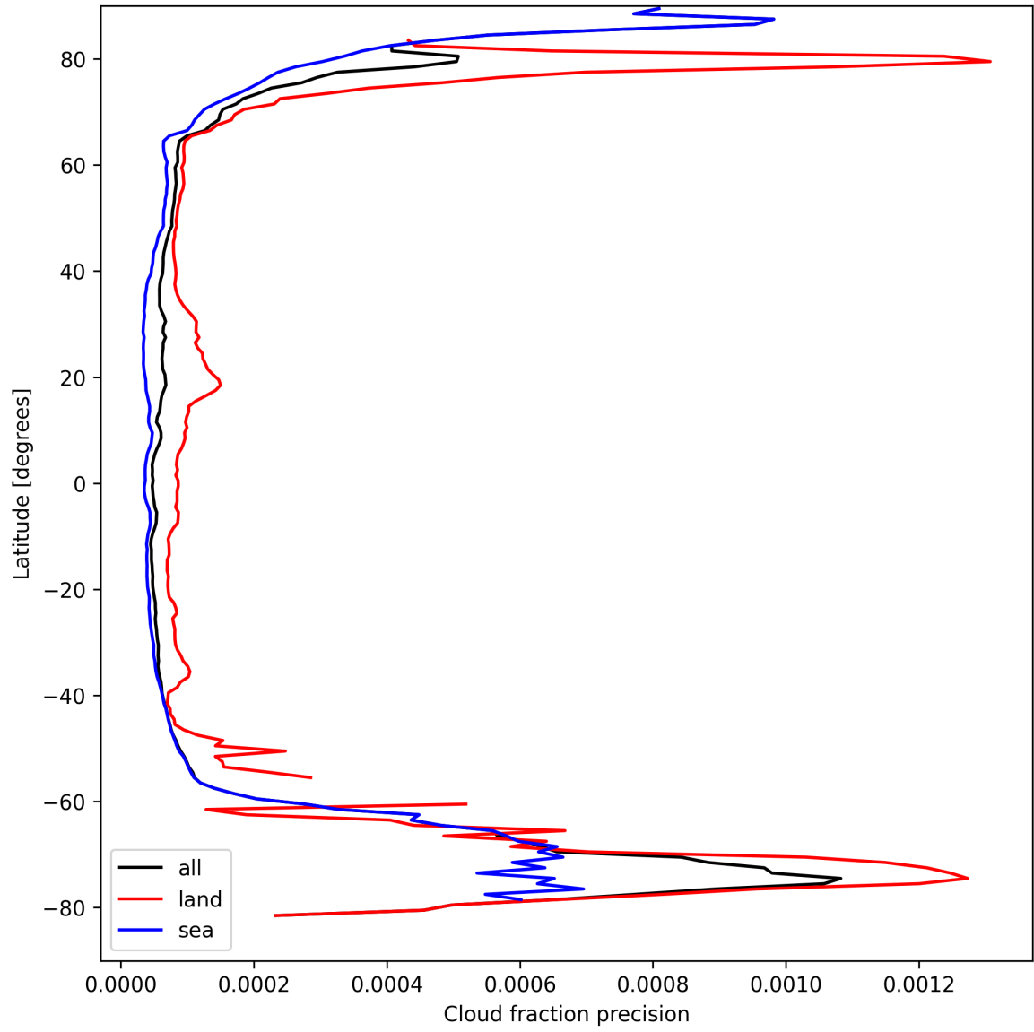
Figure 14: Zonal average of “Cloud fraction precision” for 2025-09-05 to 2025-09-06.
