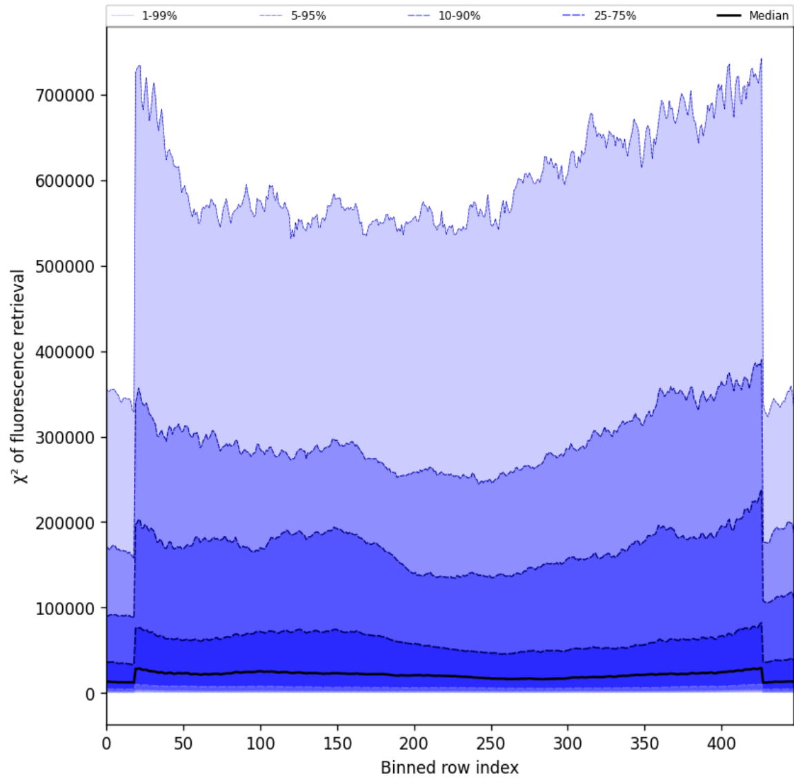
Figure 57: Along track statistics of “ \chi^2 of fluorescence retrieval” for 2025-09-05 to 2025-09-06
