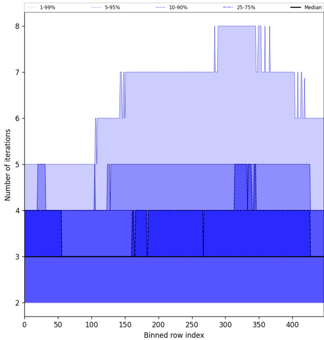
Figure 54: Along track statistics of “Number of iterations” for 2025-09-05 to 2025-09-06
