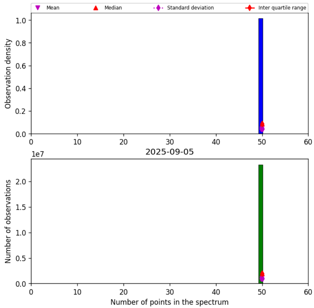
Figure 42: Histogram of “Number of points in the spectrum” for 2025-09-05 to 2025-09-06
