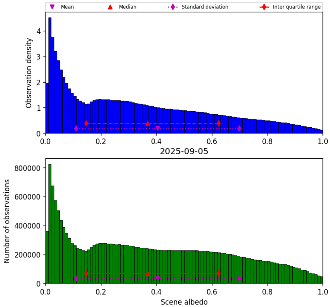
Figure 32: Histogram of “Scene albedo” for 2025-09-05 to 2025-09-06
