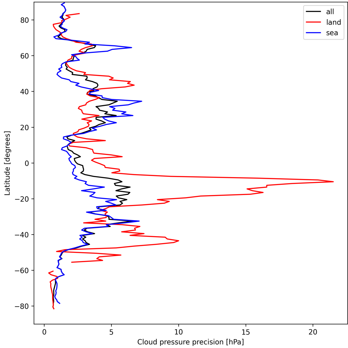
Figure 12: Zonal average of “Cloud pressure precision” for 2025-09-05 to 2025-09-06.
