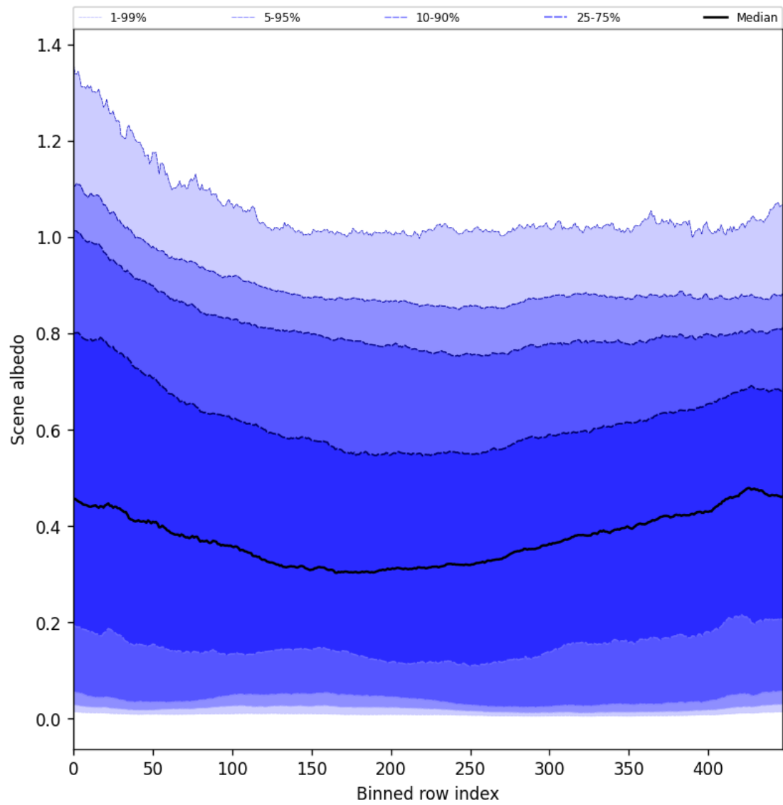
Figure 49: Along track statistics of “Scene albedo” for 2025-09-05 to 2025-09-06
