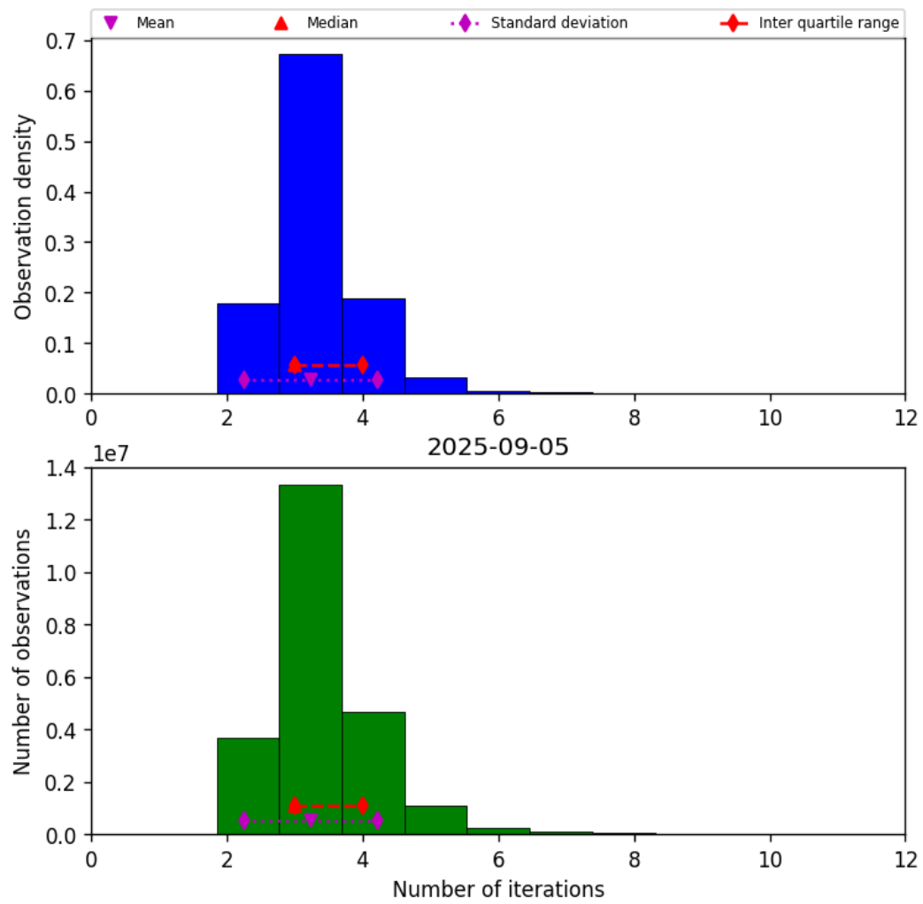
Figure 37: Histogram of “Number of iterations” for 2025-09-05 to 2025-09-06
