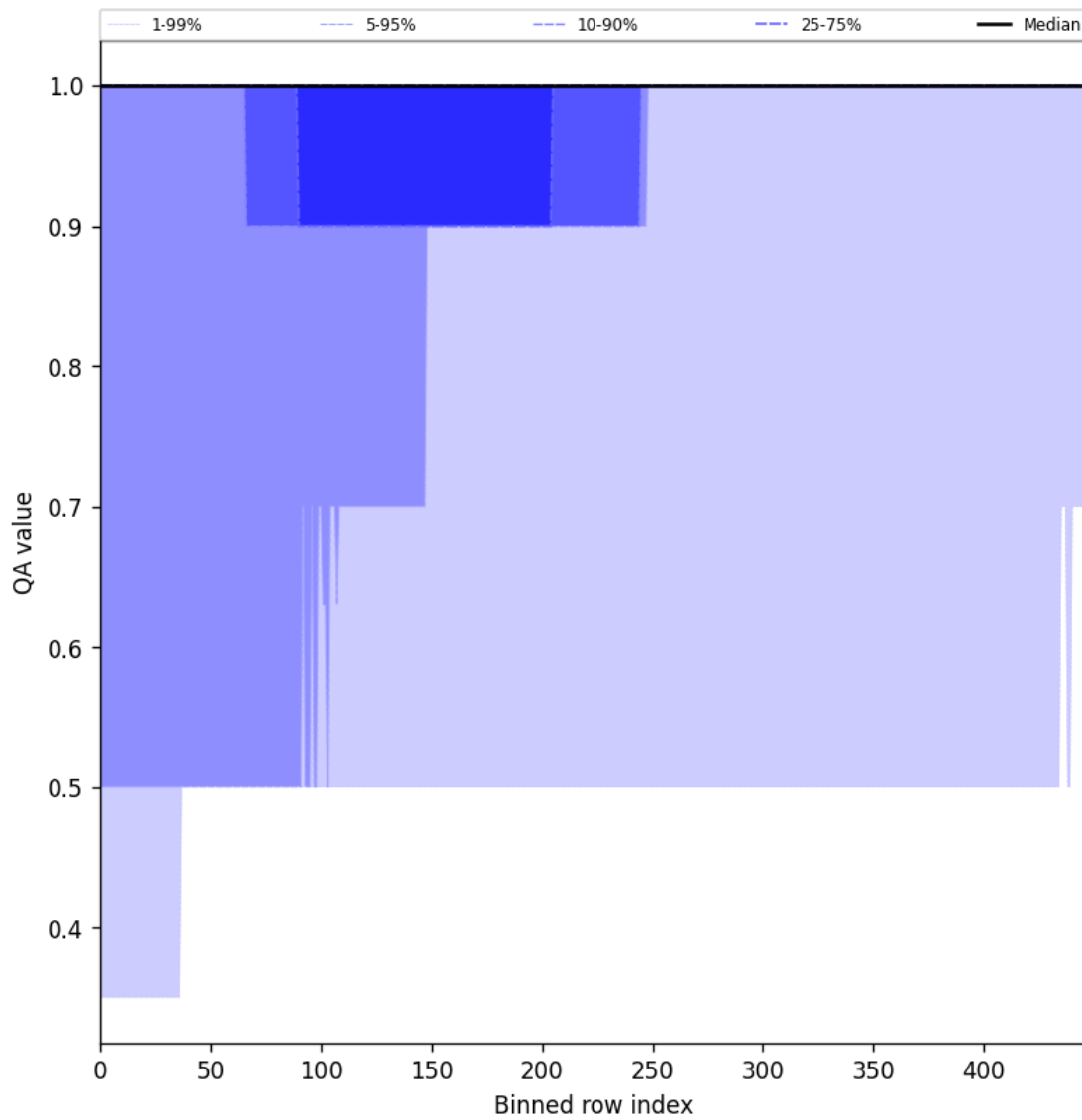
Figure 44: Along track statistics of “QA value” for 2025-09-05 to 2025-09-06
