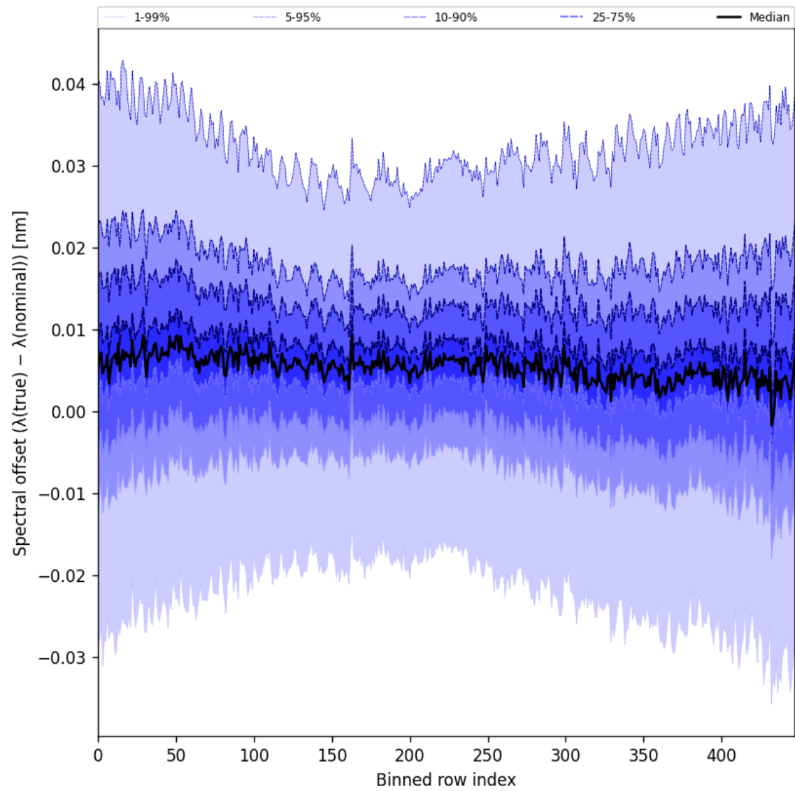
Figure 60: Along track statistics of “Spectral offset ( \lambda_{\text{true}} - \lambda_{\text{nominal}} )” for 2025-09-05 to 2025-09-06
