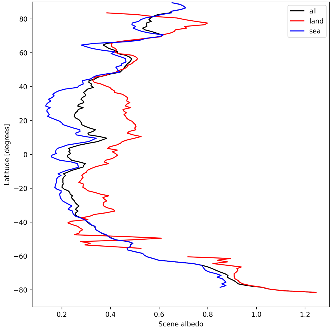
Figure 15: Zonal average of “Scene albedo” for 2025-09-05 to 2025-09-06.
