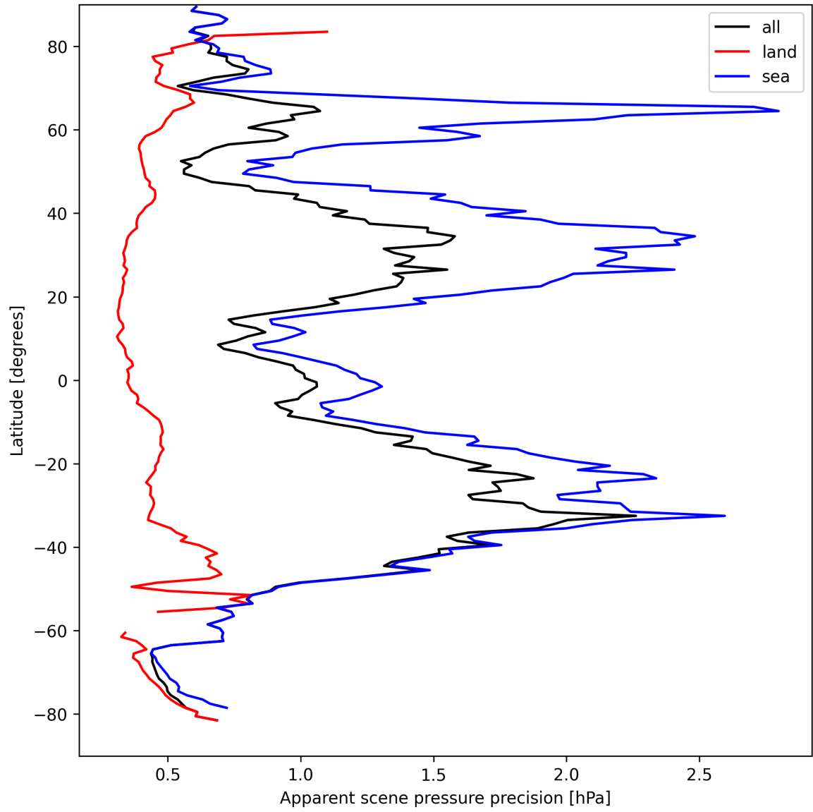
Figure 18: Zonal average of “Apparent scene pressure precision” for 2025-09-05 to 2025-09-06.
