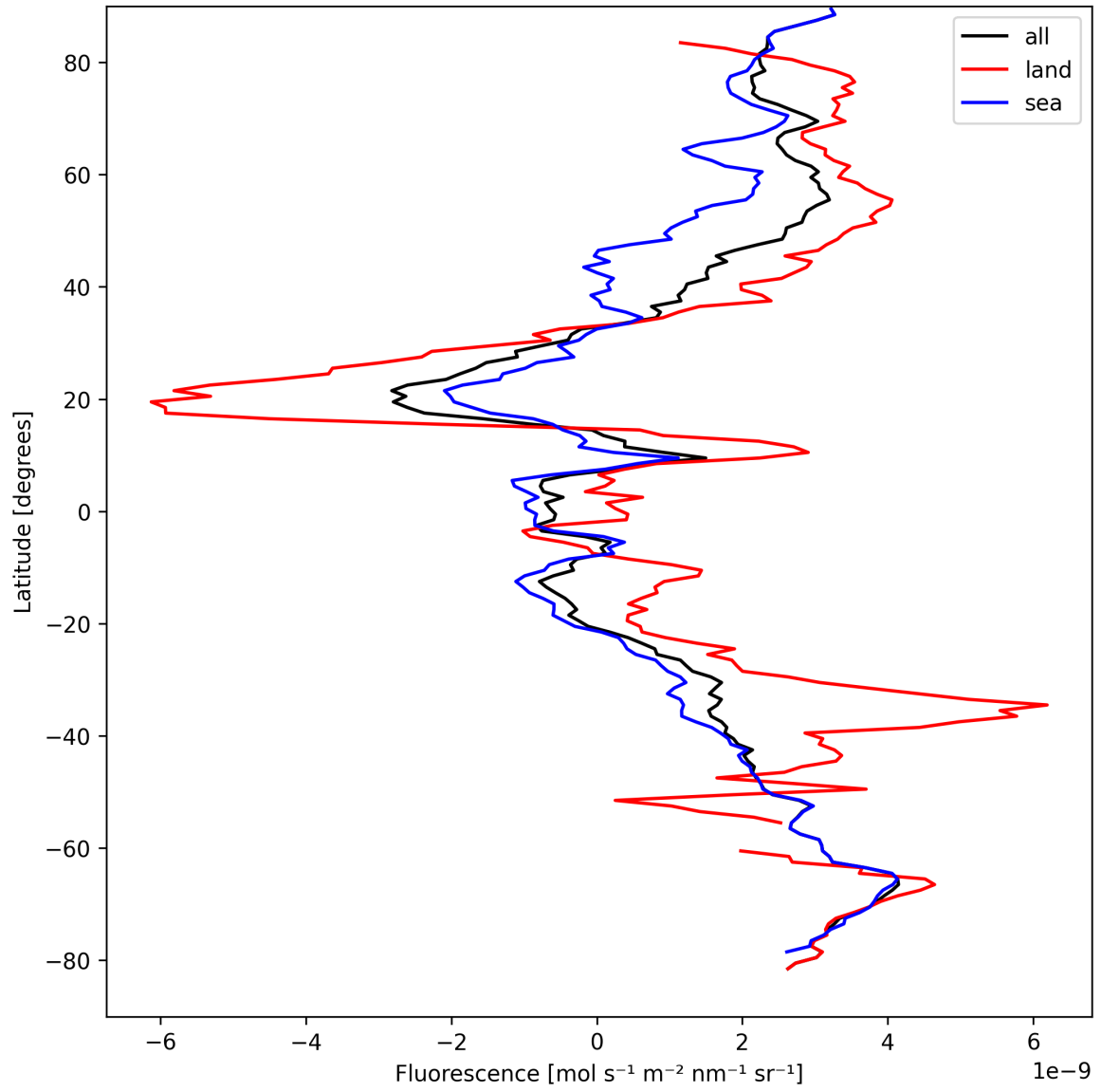
Figure 21: Zonal average of “Fluorescence” for 2025-09-05 to 2025-09-06.
