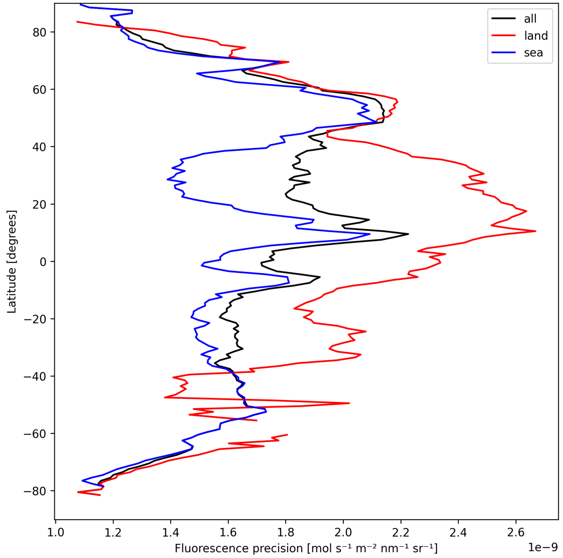
Figure 22: Zonal average of “Fluorescence precision” for 2025-09-05 to 2025-09-06.
