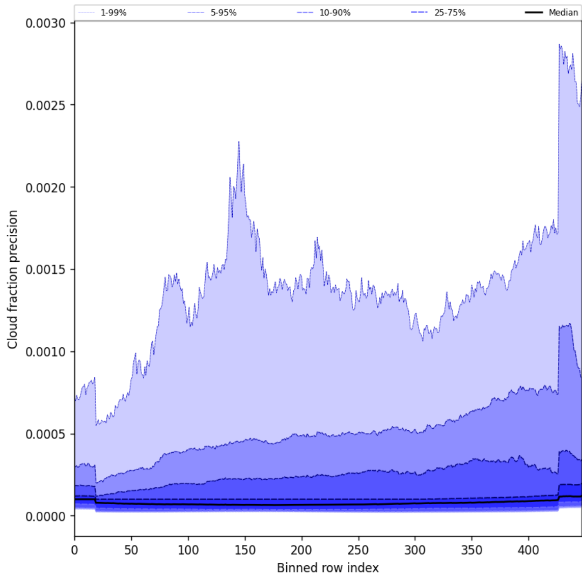
Figure 48: Along track statistics of “Cloud fraction precision” for 2025-09-05 to 2025-09-06
