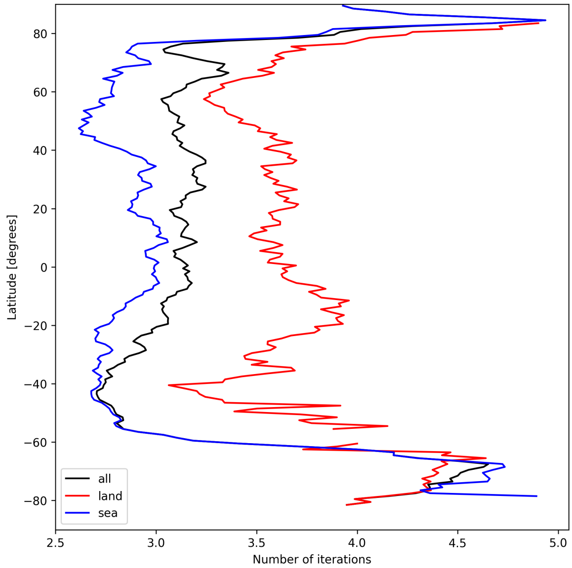
Figure 20: Zonal average of “Number of iterations” for 2025-09-05 to 2025-09-06.
