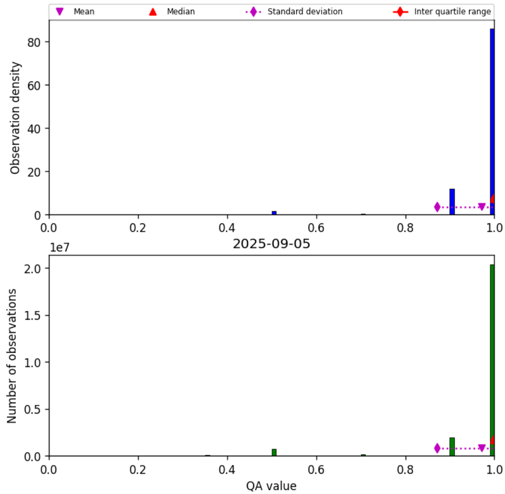
Figure 27: Histogram of “QA value” for 2025-09-05 to 2025-09-06
