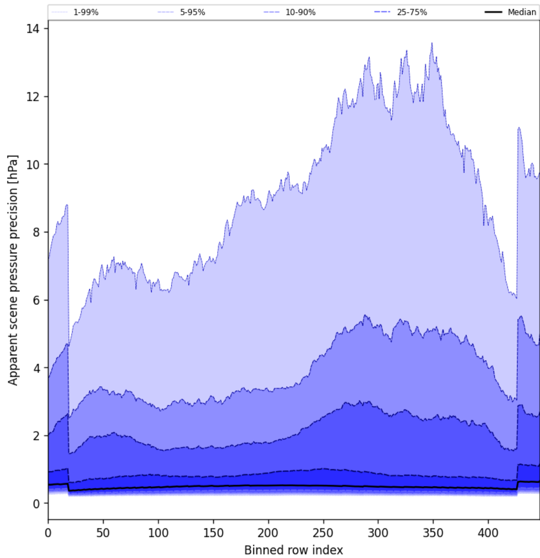
Figure 52: Along track statistics of “Apparent scene pressure precision” for 2025-09-05 to 2025-09-06
