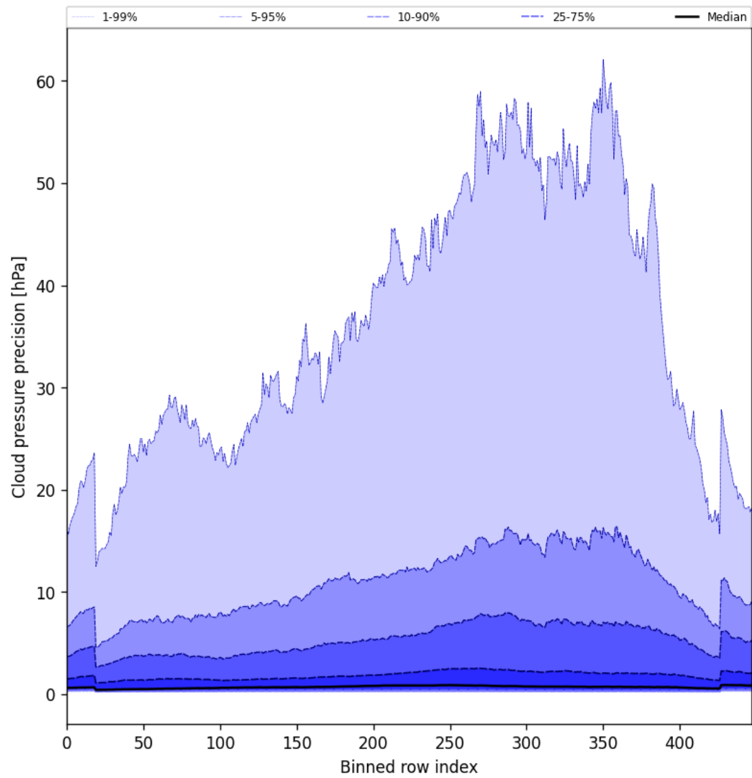
Figure 46: Along track statistics of “Cloud pressure precision” for 2025-09-05 to 2025-09-06
