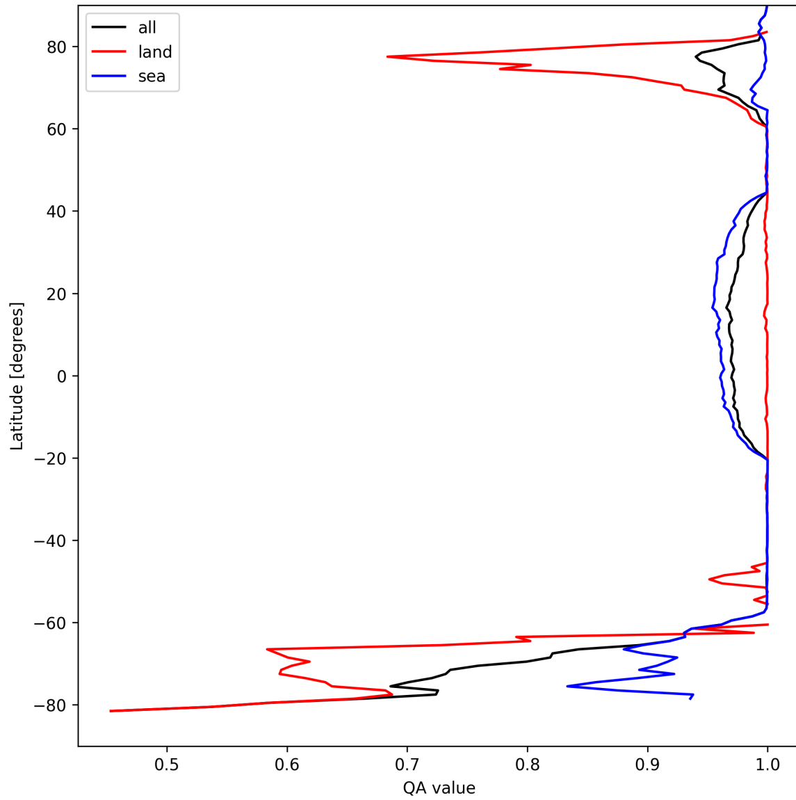
Figure 10: Zonal average of “QA value” for 2025-09-05 to 2025-09-06.
