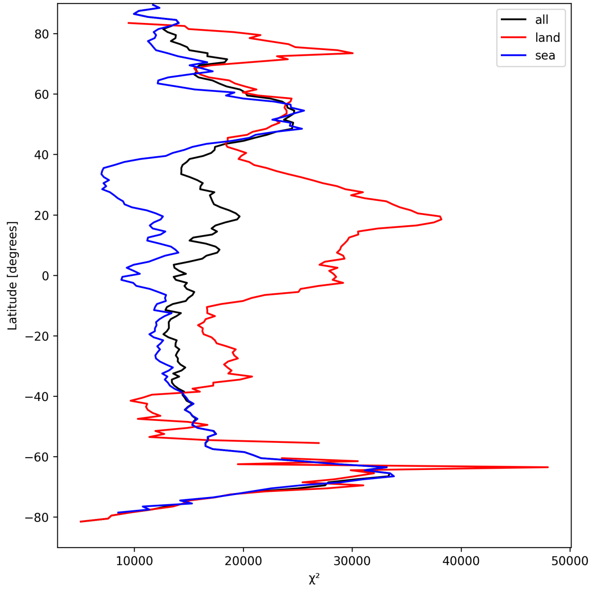
Figure 19: Zonal average of “ \chi^2 ” for 2025-09-05 to 2025-09-06.
