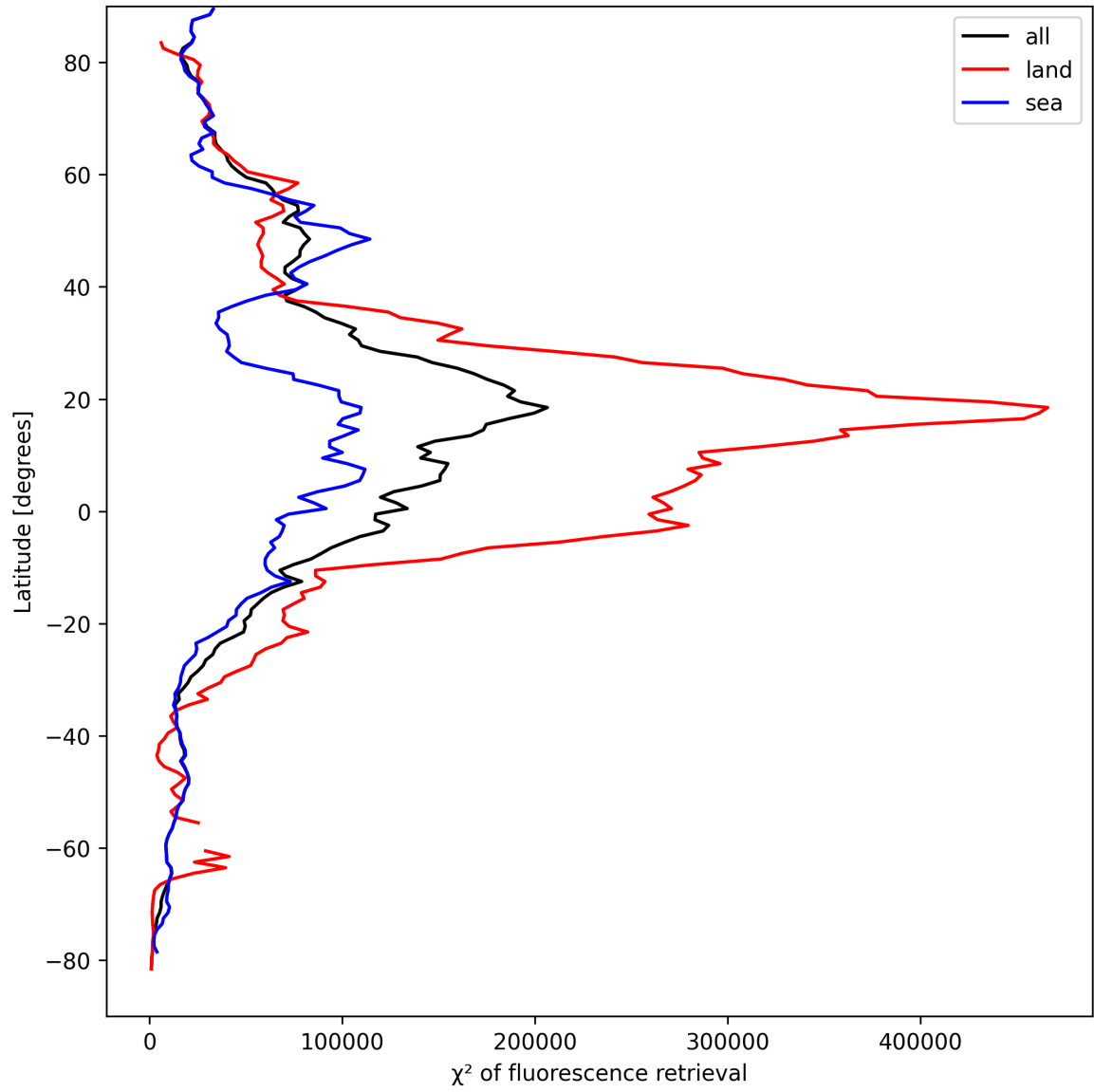
Figure 23: Zonal average of “ \chi^2 of fluorescence retrieval” for 2025-09-05 to 2025-09-06.
