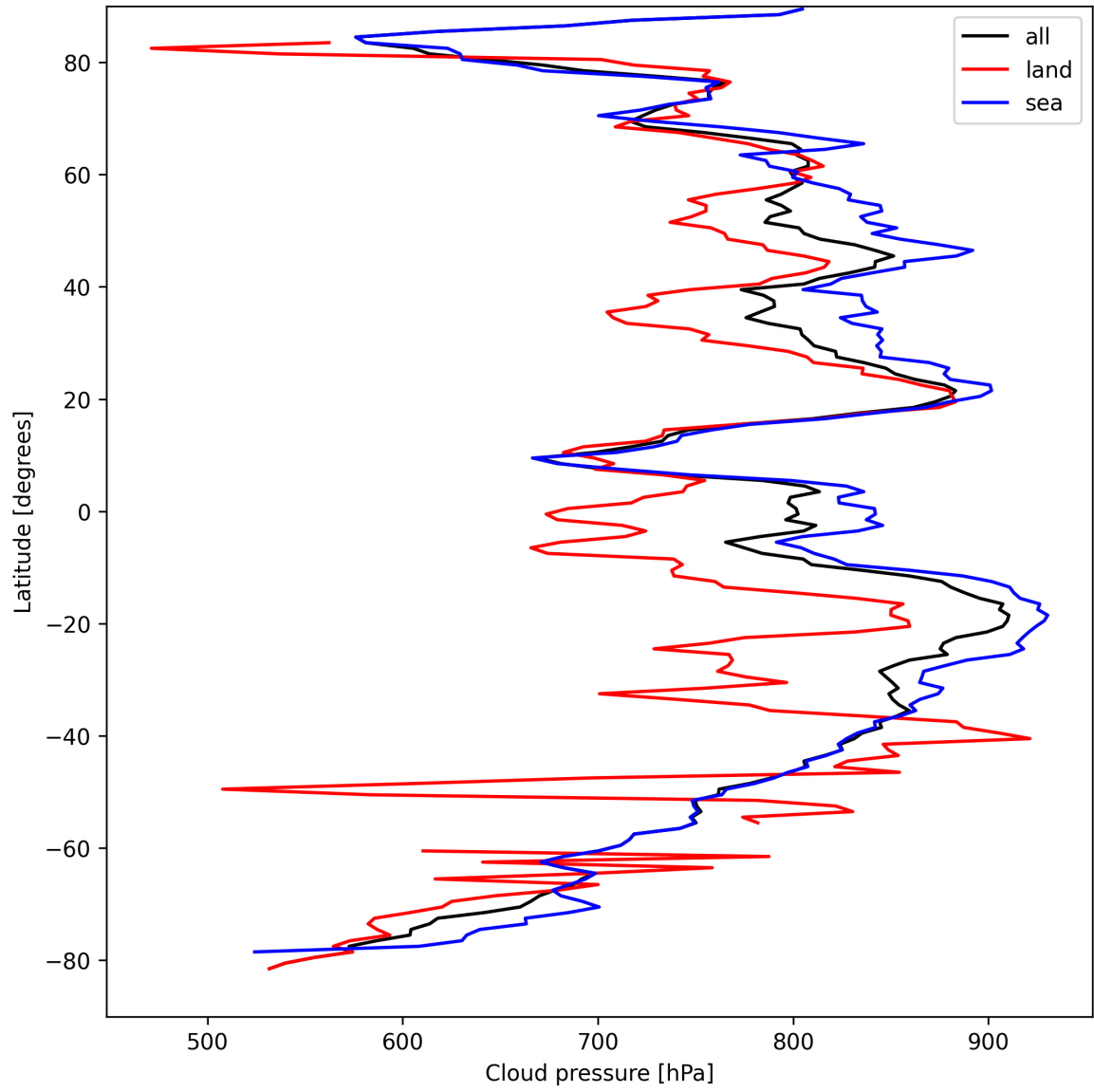
Figure 11: Zonal average of “Cloud pressure” for 2025-09-05 to 2025-09-06.
