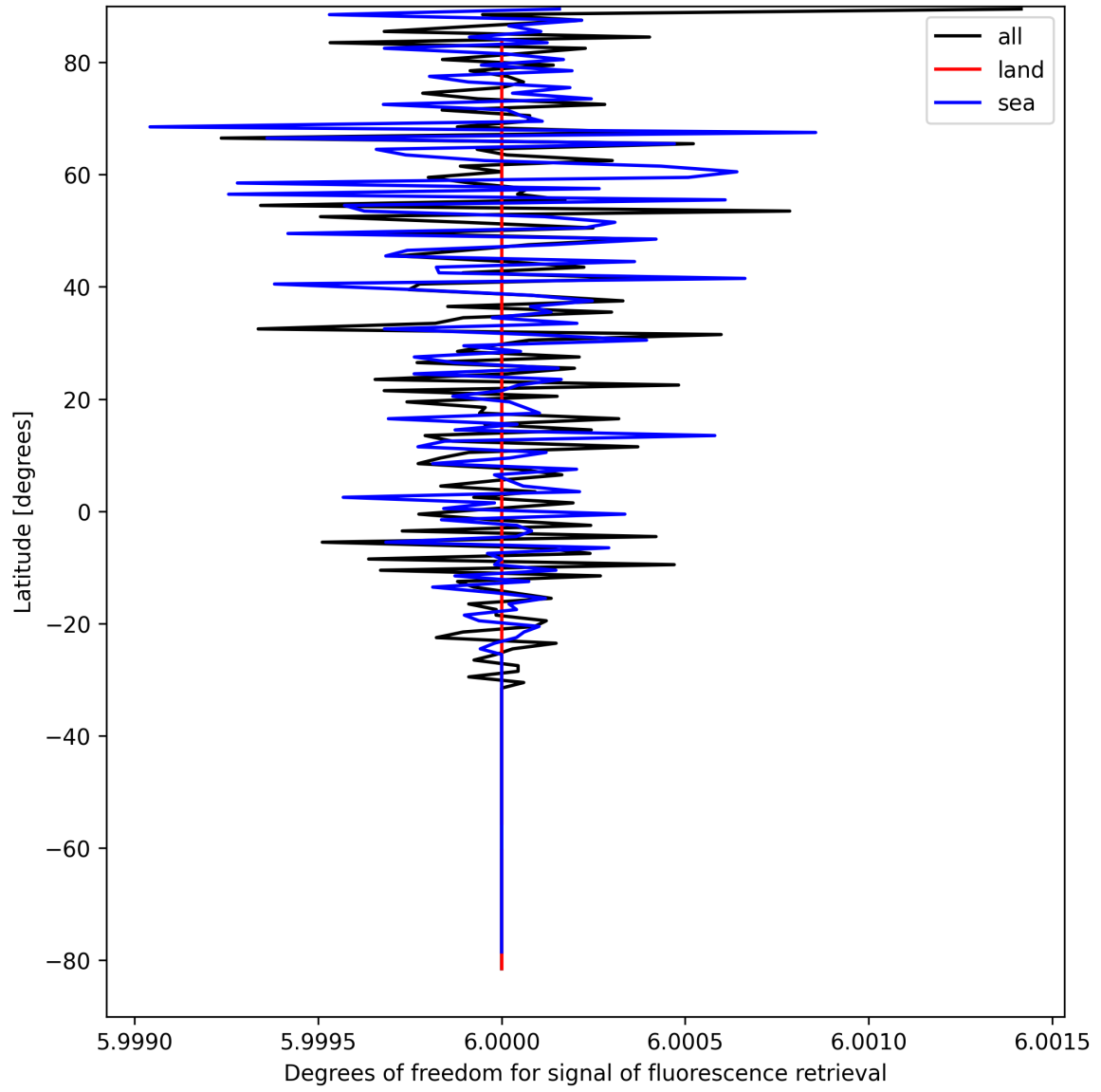
Figure 24: Zonal average of “Degrees of freedom for signal of fluorescence retrieval” for 2025-09-05 to 2025-09-06.
