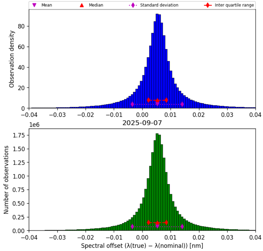
Figure 43: Histogram of “Spectral offset ( \lambda_{\text{true}} - \lambda_{\text{nominal}} )” for 2025-09-07 to 2025-09-07
