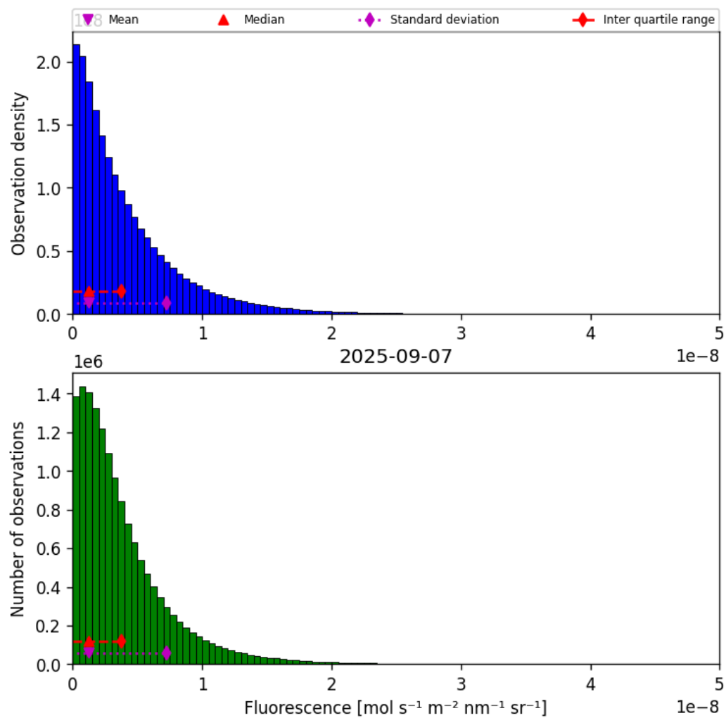
Figure 38: Histogram of “Fluorescence” for 2025-09-07 to 2025-09-07
