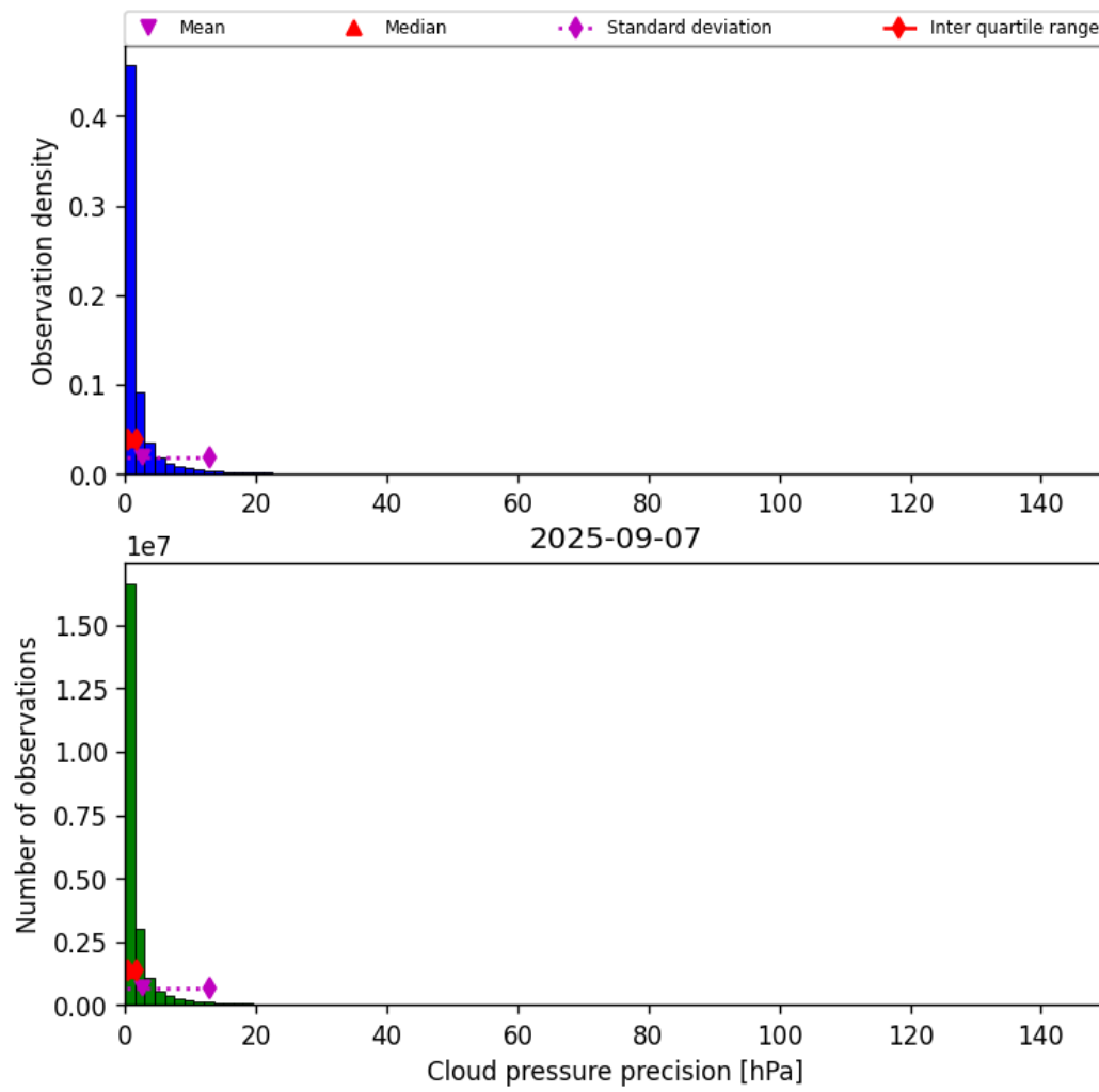
Figure 29: Histogram of “Cloud pressure precision” for 2025-09-07 to 2025-09-07
