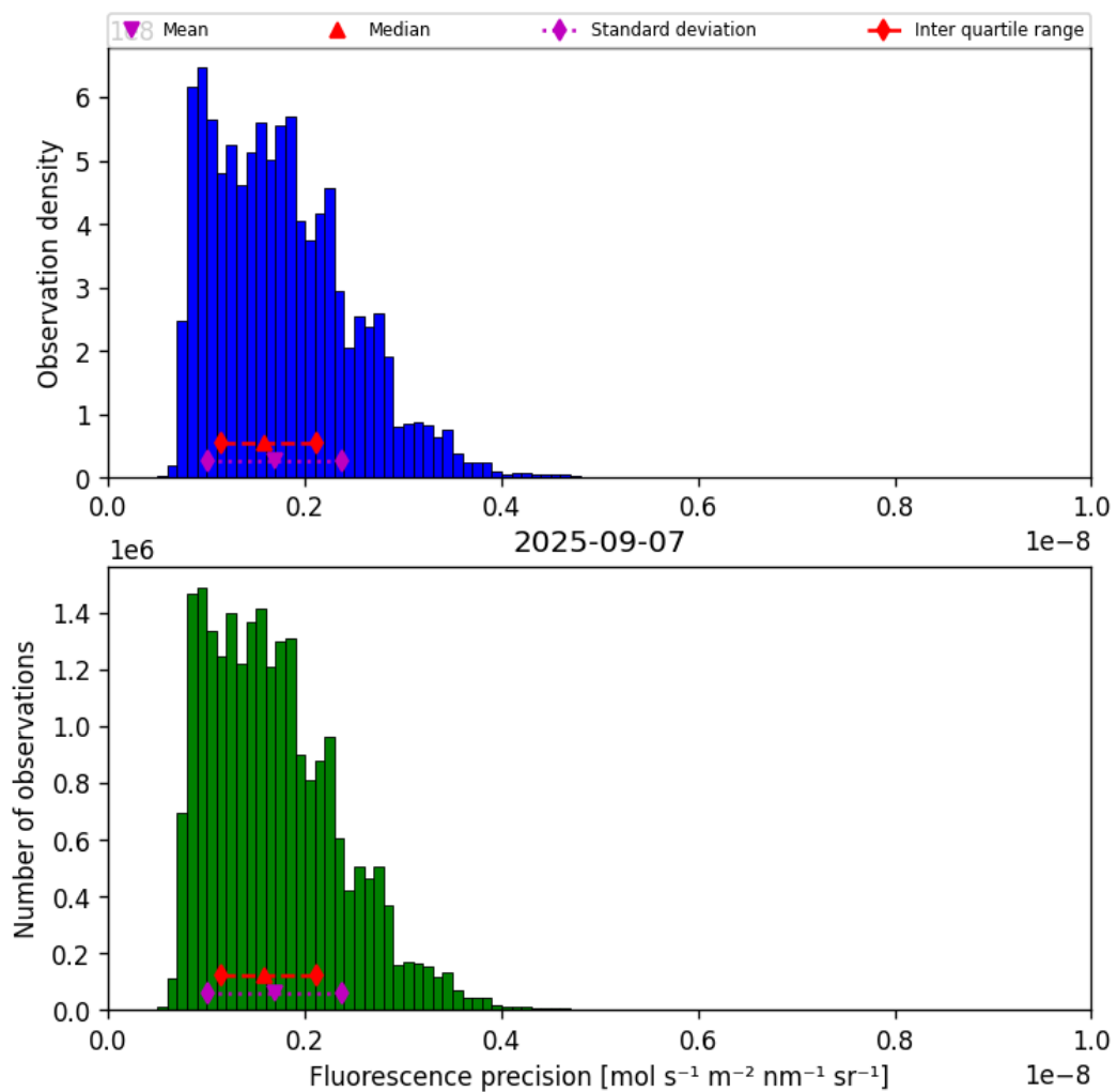
Figure 39: Histogram of “Fluorescence precision” for 2025-09-07 to 2025-09-07
