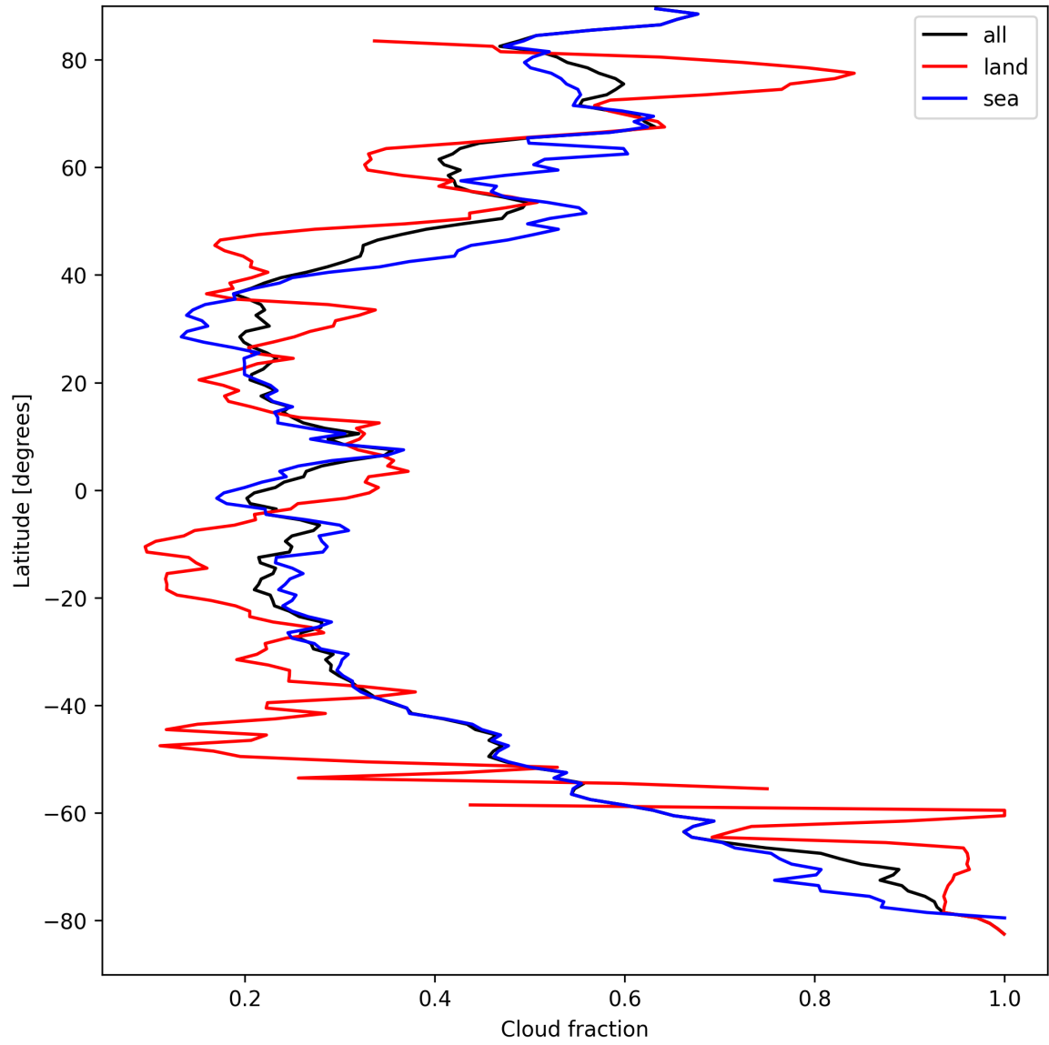
Figure 13: Zonal average of “Cloud fraction” for 2025-09-07 to 2025-09-07.
