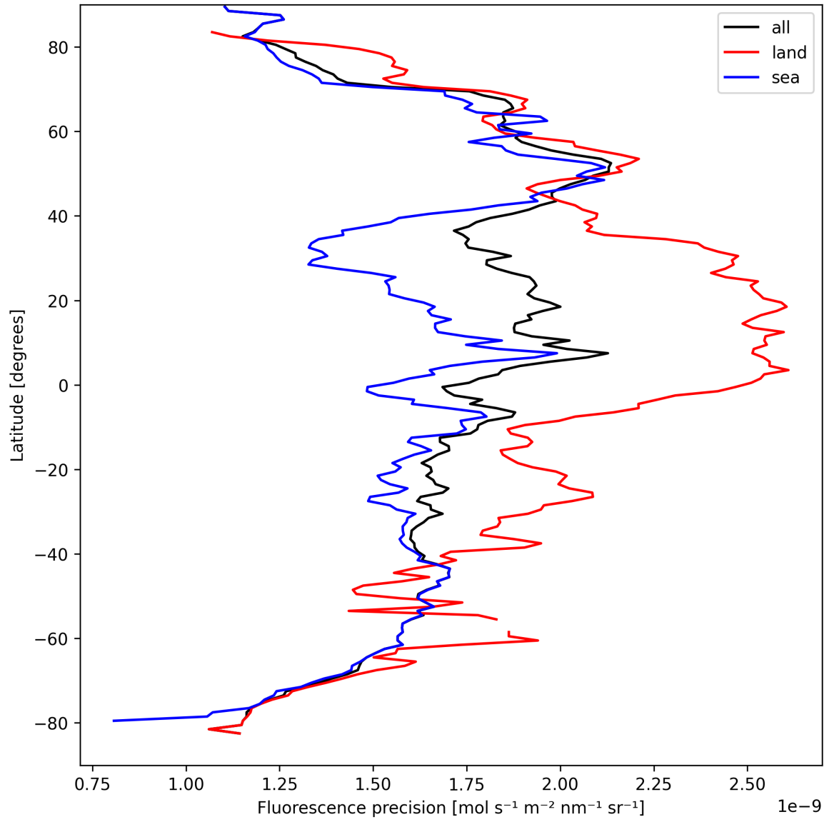
Figure 22: Zonal average of “Fluorescence precision” for 2025-09-07 to 2025-09-07.
