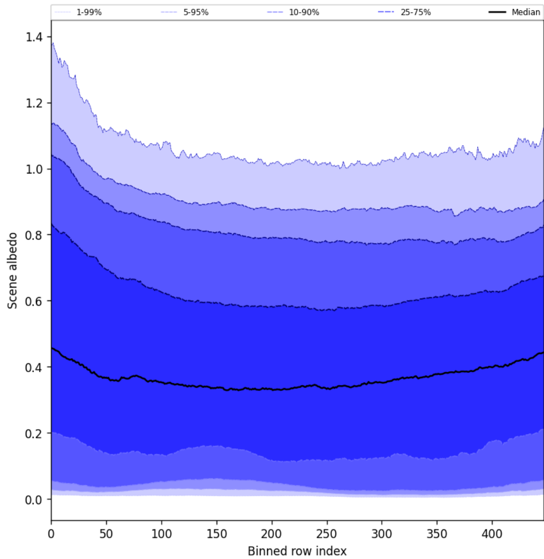
Figure 49: Along track statistics of “Scene albedo” for 2025-09-07 to 2025-09-07
