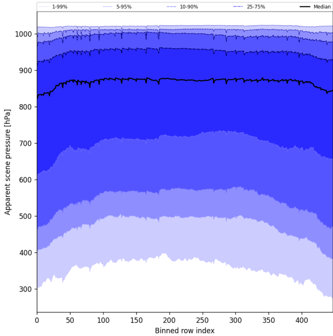
Figure 51: Along track statistics of “Apparent scene pressure” for 2025-09-07 to 2025-09-07
