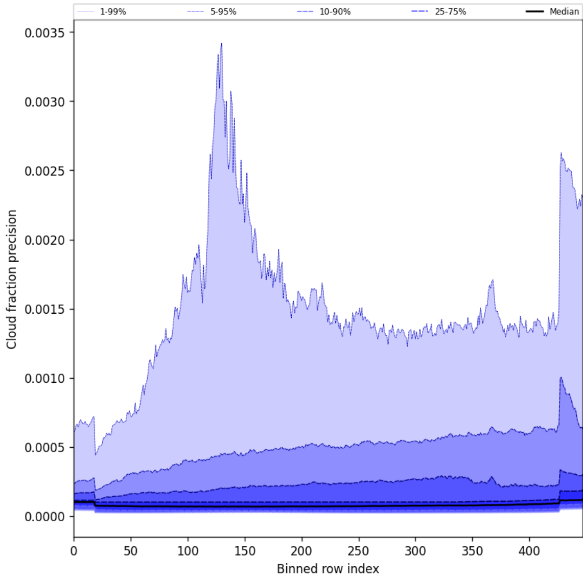
Figure 48: Along track statistics of “Cloud fraction precision” for 2025-09-07 to 2025-09-07
