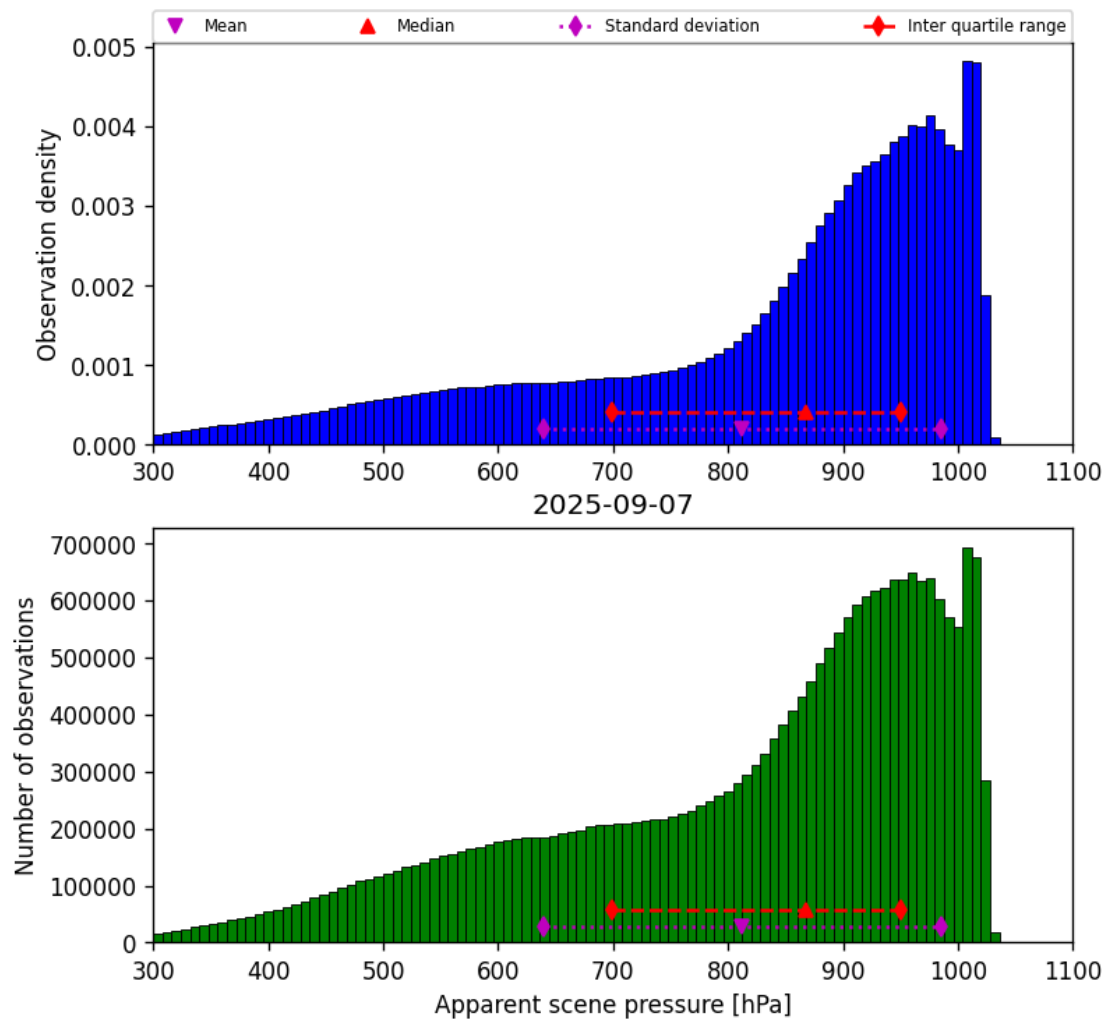
Figure 34: Histogram of “Apparent scene pressure” for 2025-09-07 to 2025-09-07
