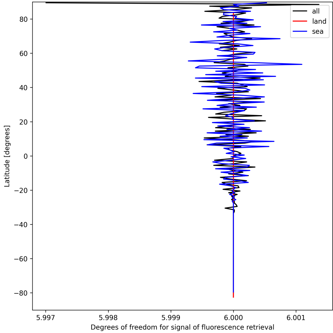
Figure 24: Zonal average of “Degrees of freedom for signal of fluorescence retrieval” for 2025-09-07 to 2025-09-07.
