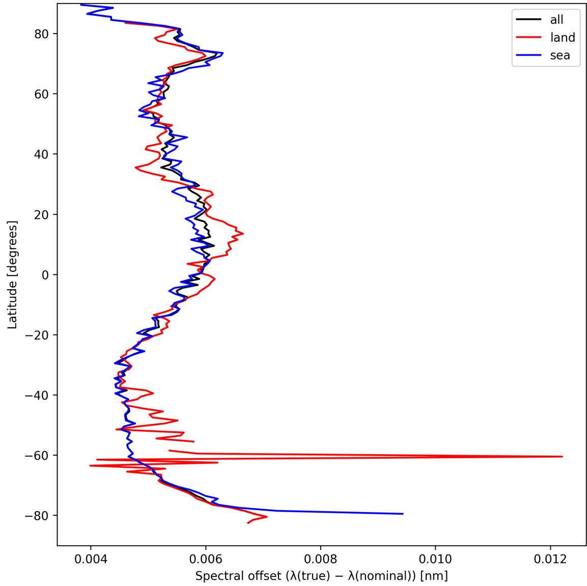
Figure 26: Zonal average of “Spectral offset ( \lambda_{\text{true}} - \lambda_{\text{nominal}} )” for 2025-09-07 to 2025-09-07.
