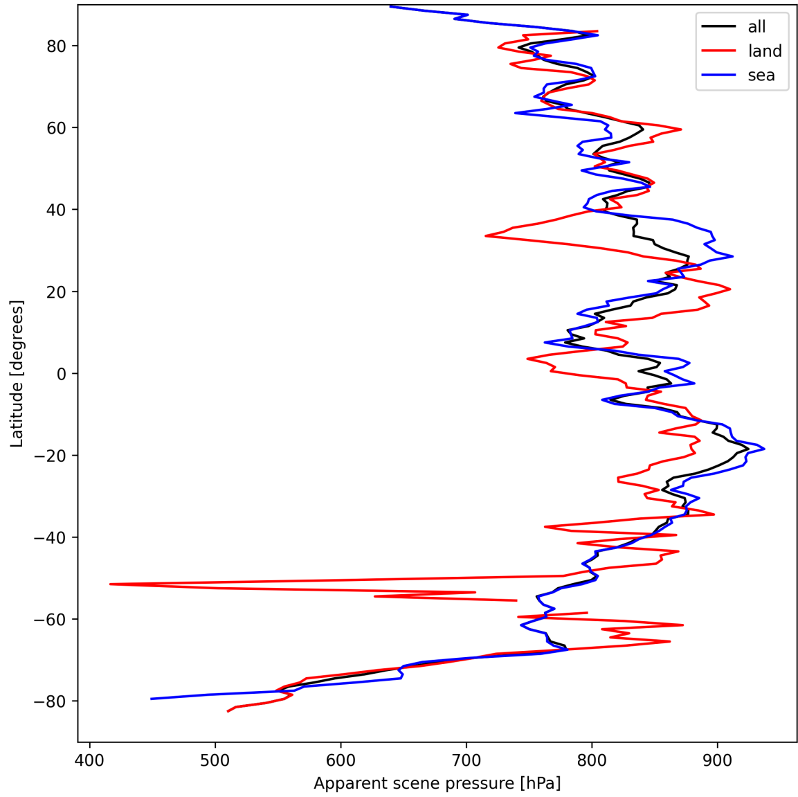
Figure 17: Zonal average of “Apparent scene pressure” for 2025-09-07 to 2025-09-07.
