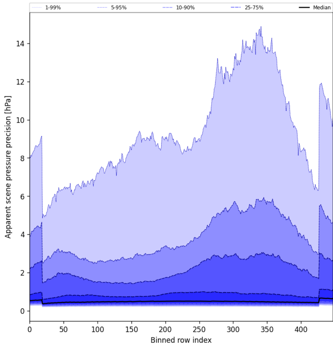
Figure 52: Along track statistics of “Apparent scene pressure precision” for 2025-09-07 to 2025-09-07
