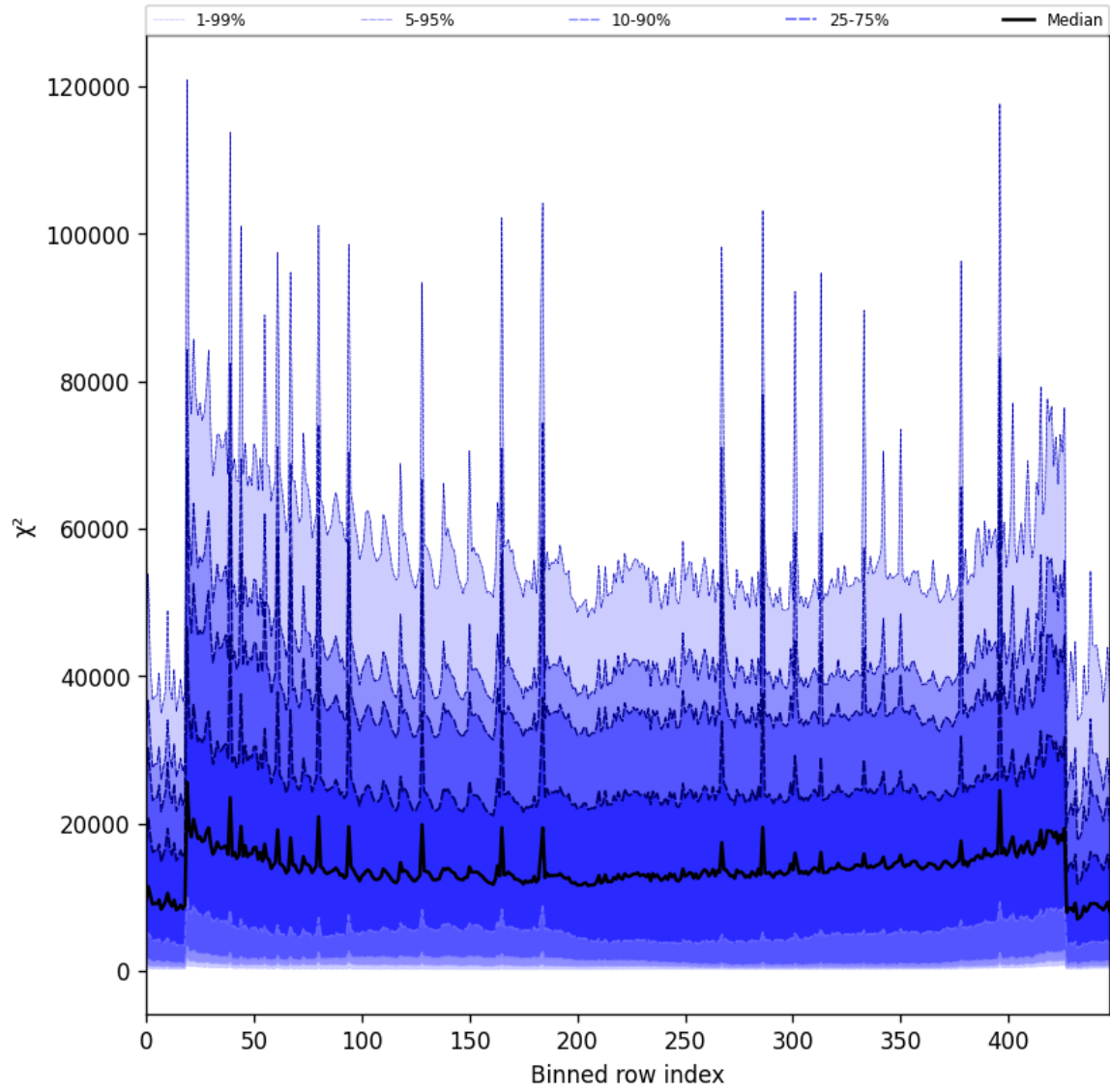
Figure 53: Along track statistics of “ \chi^2 ” for 2025-09-07 to 2025-09-07
