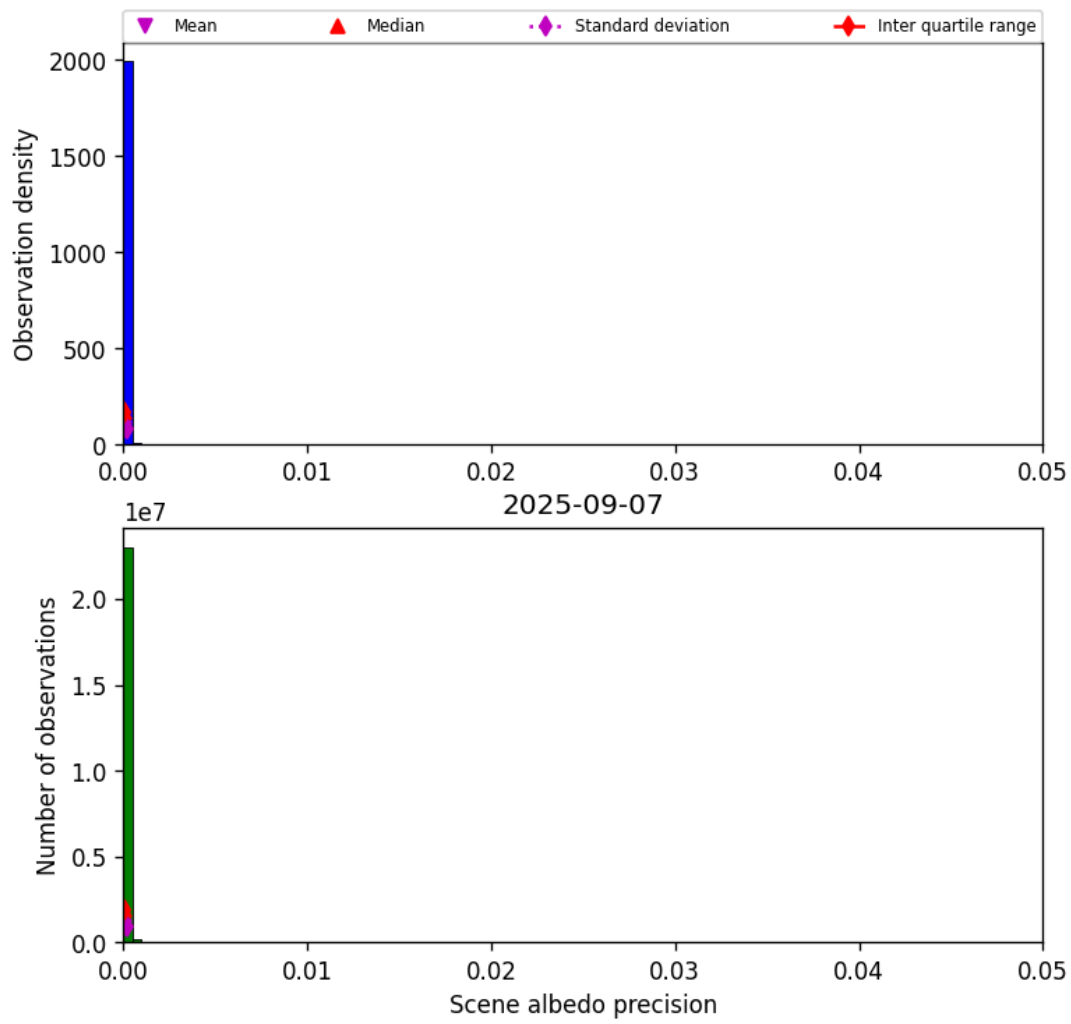
Figure 33: Histogram of “Scene albedo precision” for 2025-09-07 to 2025-09-07
