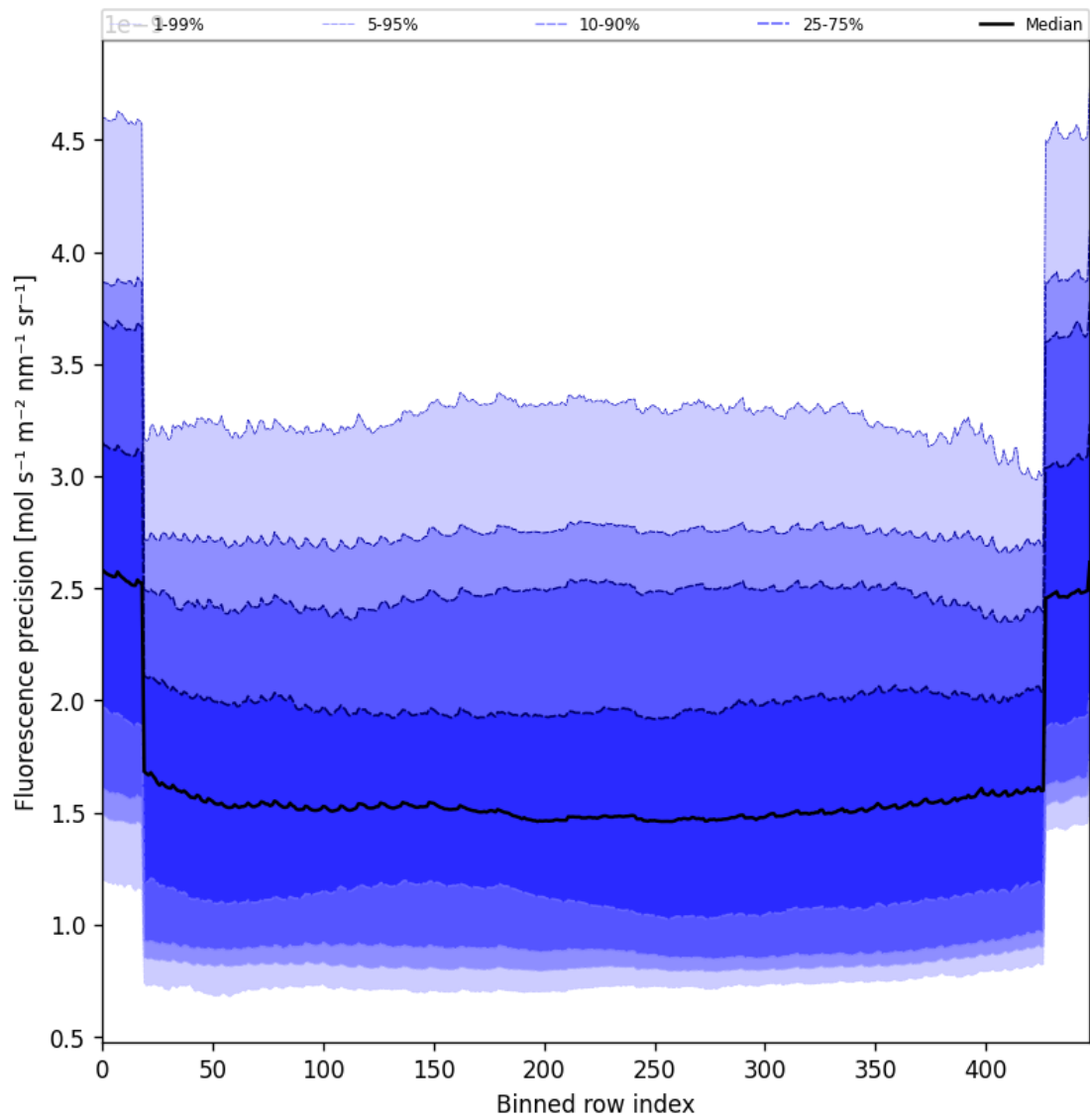
Figure 56: Along track statistics of “Fluorescence precision” for 2025-09-07 to 2025-09-07
