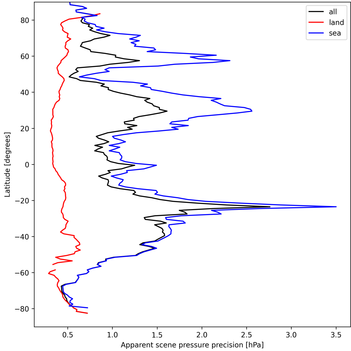
Figure 18: Zonal average of “Apparent scene pressure precision” for 2025-09-07 to 2025-09-07.
