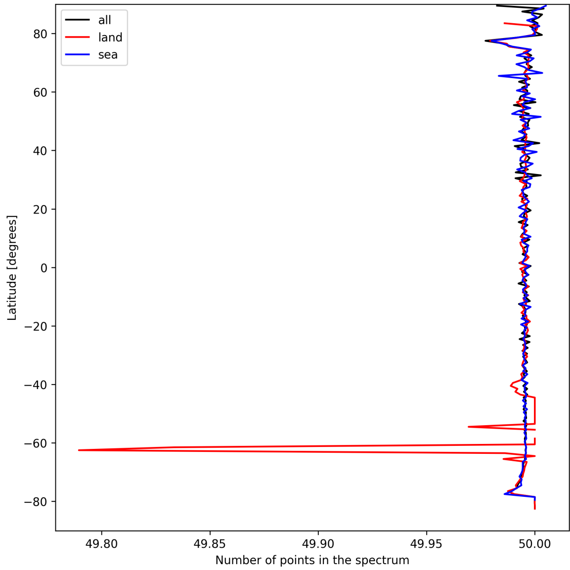
Figure 25: Zonal average of “Number of points in the spectrum” for 2025-09-07 to 2025-09-07.
