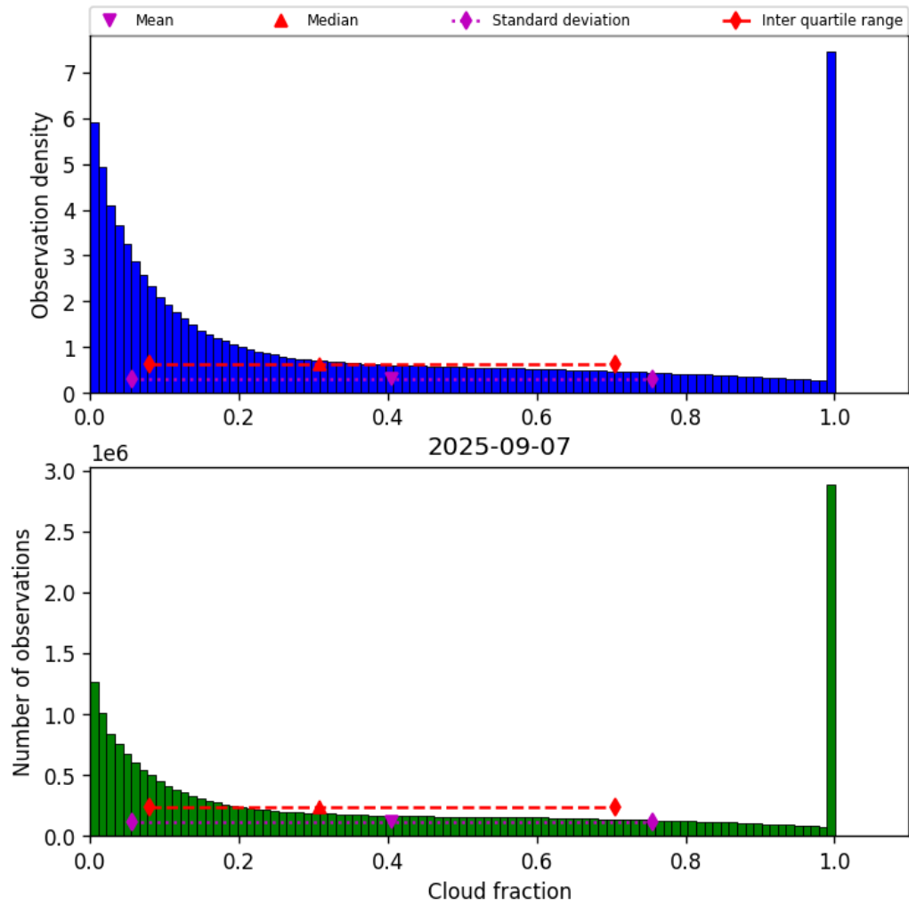
Figure 30: Histogram of “Cloud fraction” for 2025-09-07 to 2025-09-07
