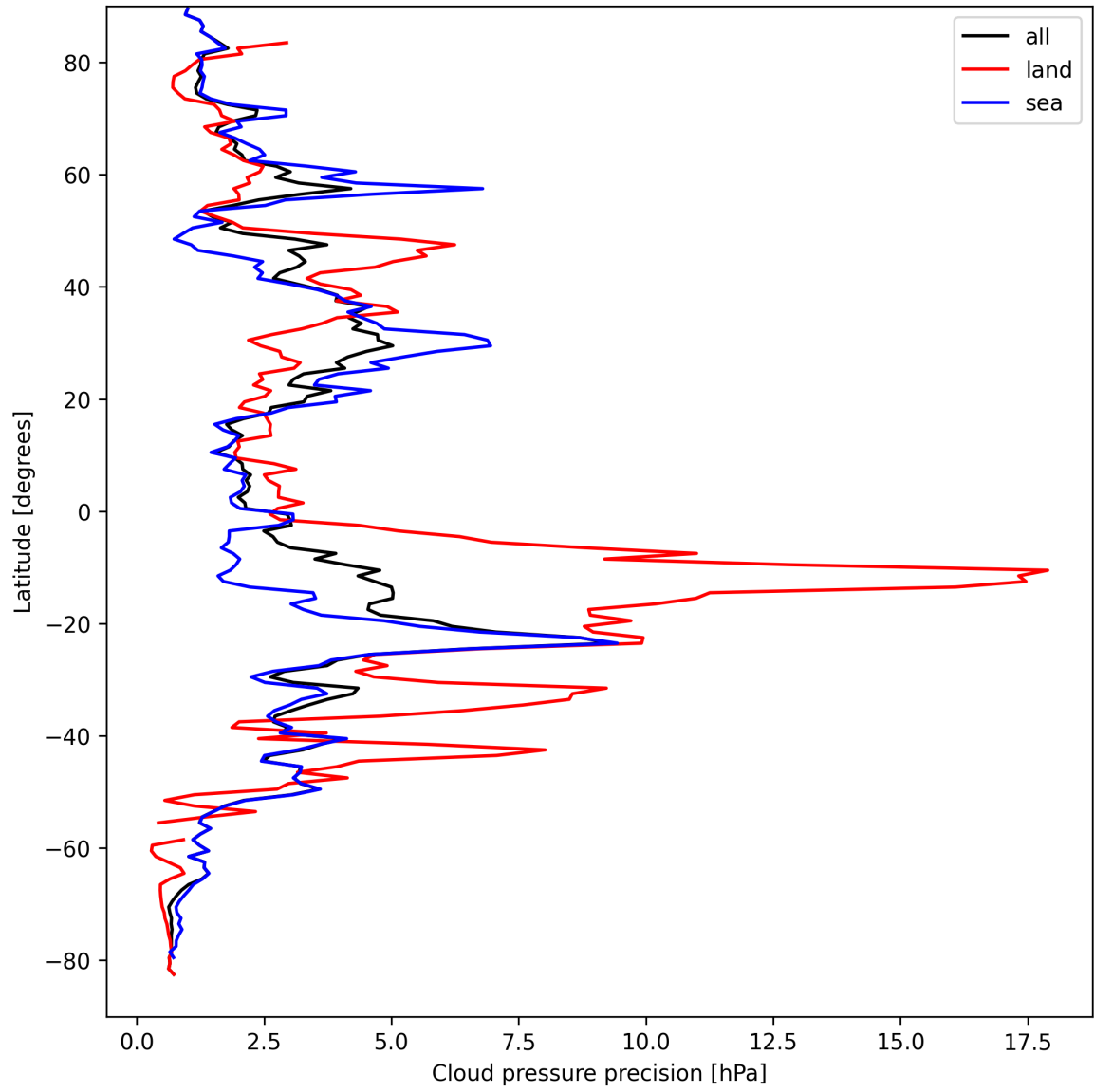
Figure 12: Zonal average of “Cloud pressure precision” for 2025-09-07 to 2025-09-07.
