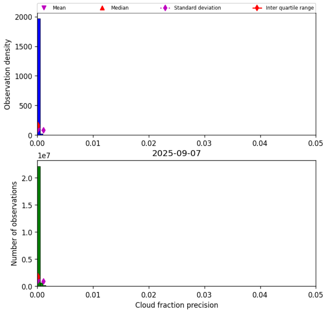
Figure 31: Histogram of “Cloud fraction precision” for 2025-09-07 to 2025-09-07
