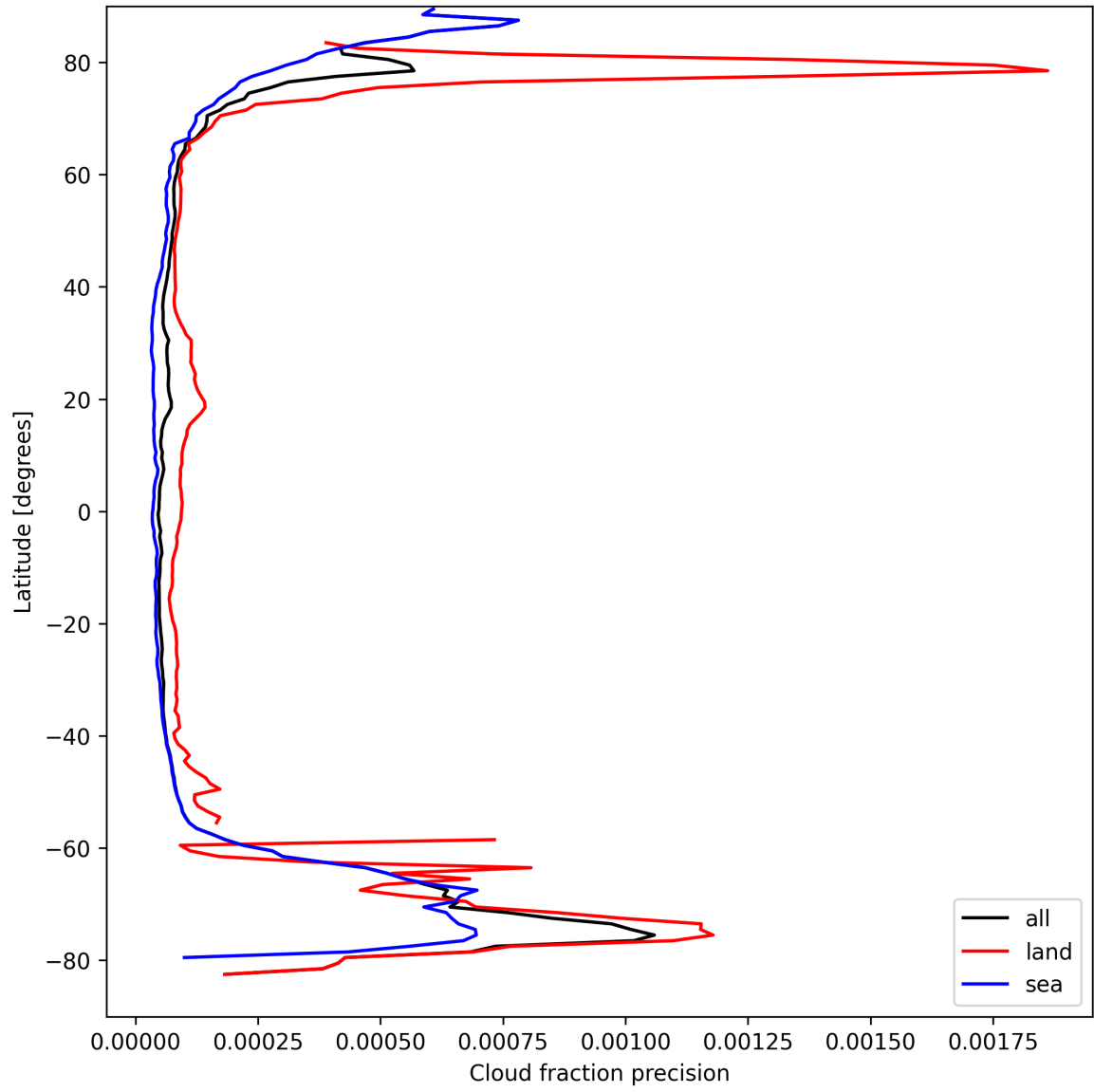
Figure 14: Zonal average of “Cloud fraction precision” for 2025-09-07 to 2025-09-07.
