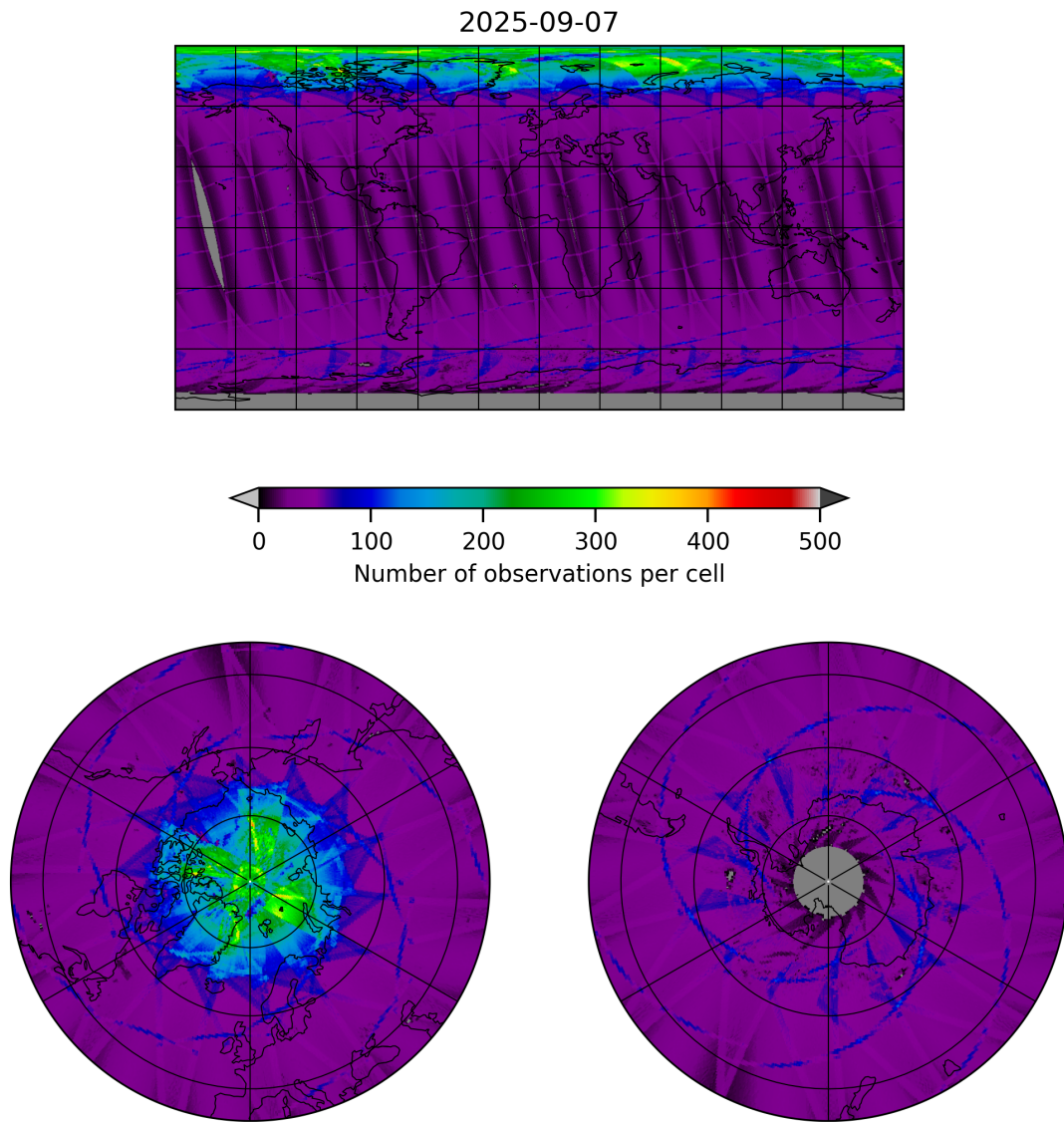
Figure 9: Map of the number of observations for 2025-09-07 to 2025-09-07
