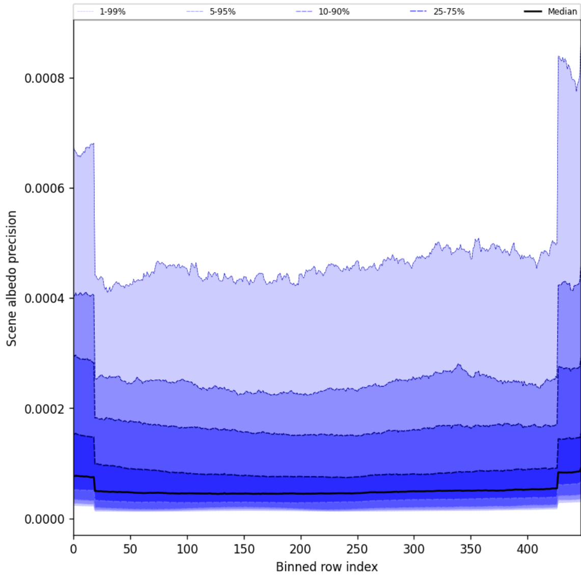
Figure 50: Along track statistics of “Scene albedo precision” for 2025-09-07 to 2025-09-07
