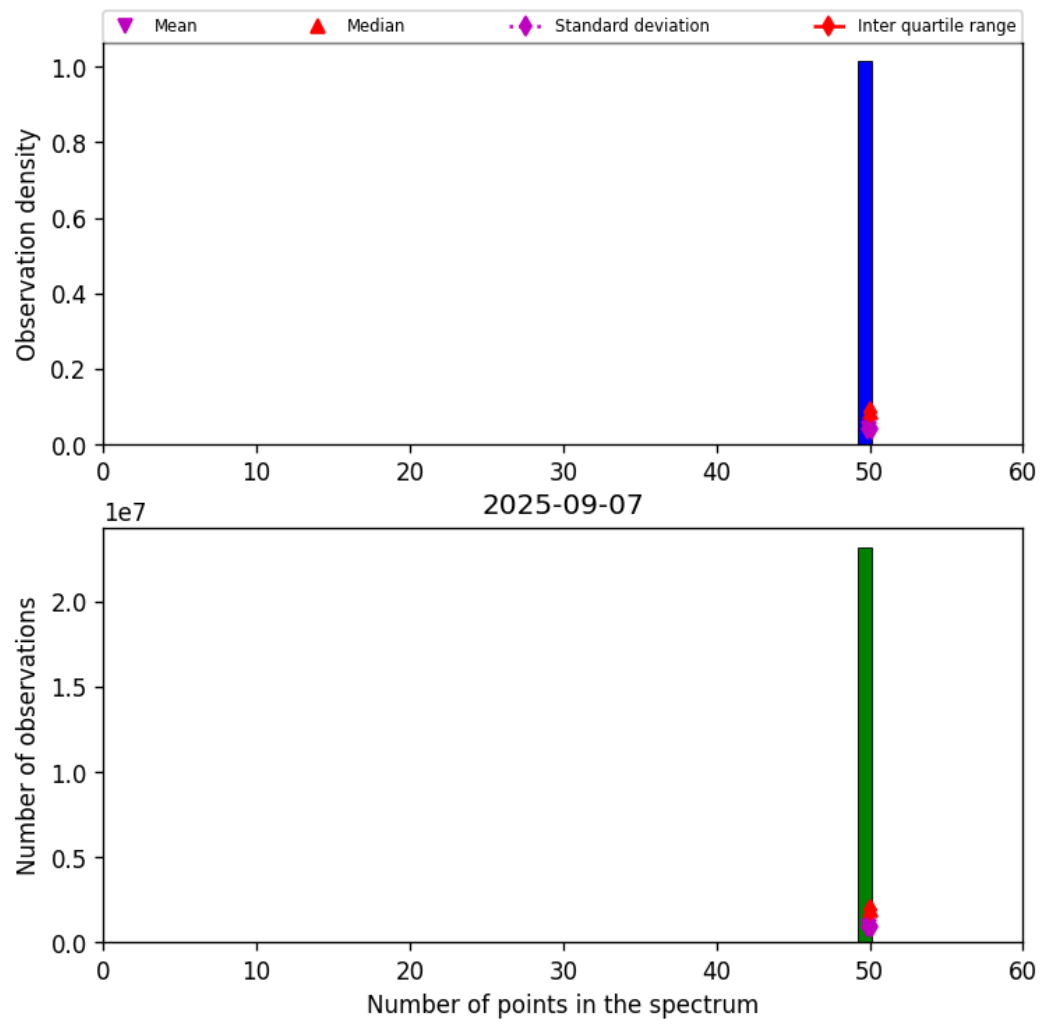
Figure 42: Histogram of "Number of points in the spectrum" for 2025-09-07 to 2025-09-07
