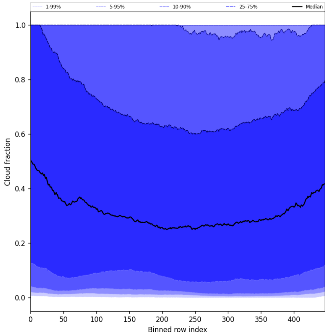
Figure 47: Along track statistics of “Cloud fraction” for 2025-09-07 to 2025-09-07
