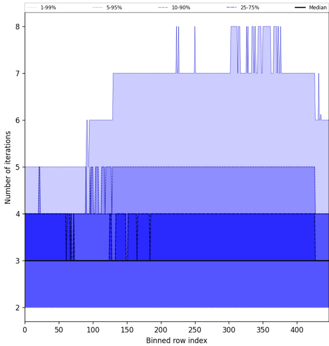
Figure 54: Along track statistics of “Number of iterations” for 2025-09-07 to 2025-09-07
