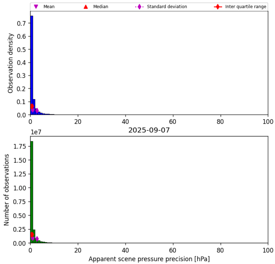
Figure 35: Histogram of “Apparent scene pressure precision” for 2025-09-07 to 2025-09-07
