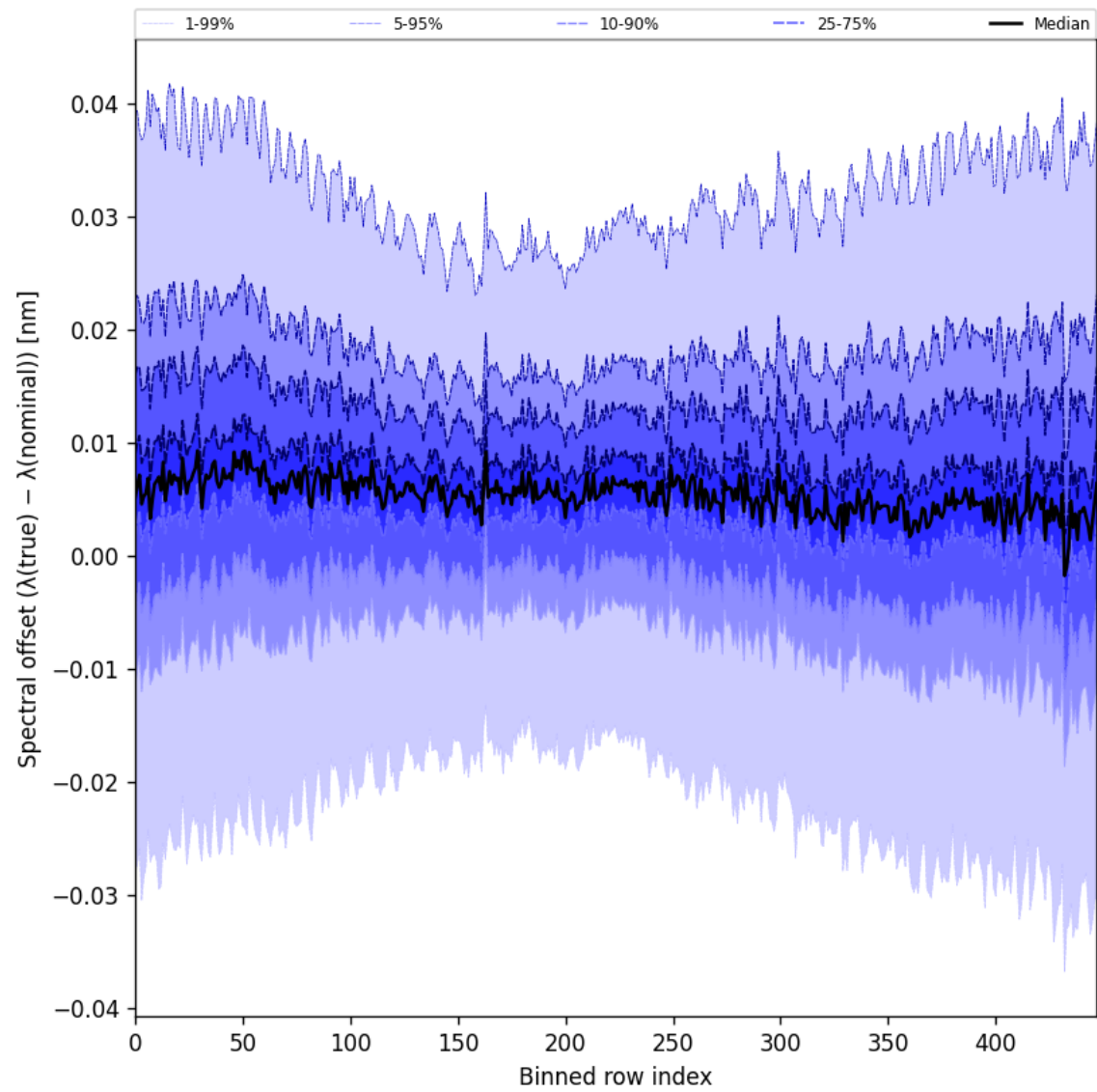
Figure 60: Along track statistics of “Spectral offset ( \lambda_{\text{true}} - \lambda_{\text{nominal}} )” for 2025-09-07 to 2025-09-07
