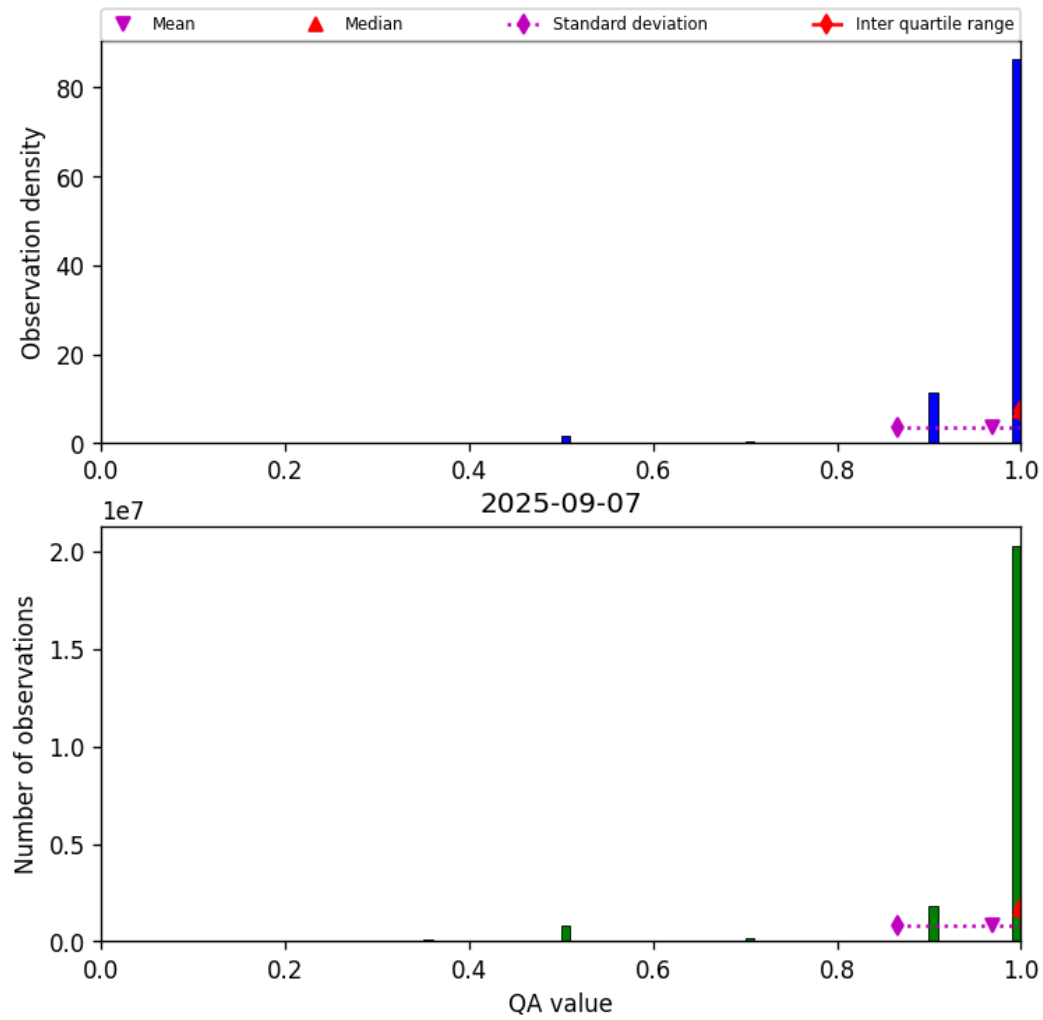
Figure 27: Histogram of “QA value” for 2025-09-07 to 2025-09-07
