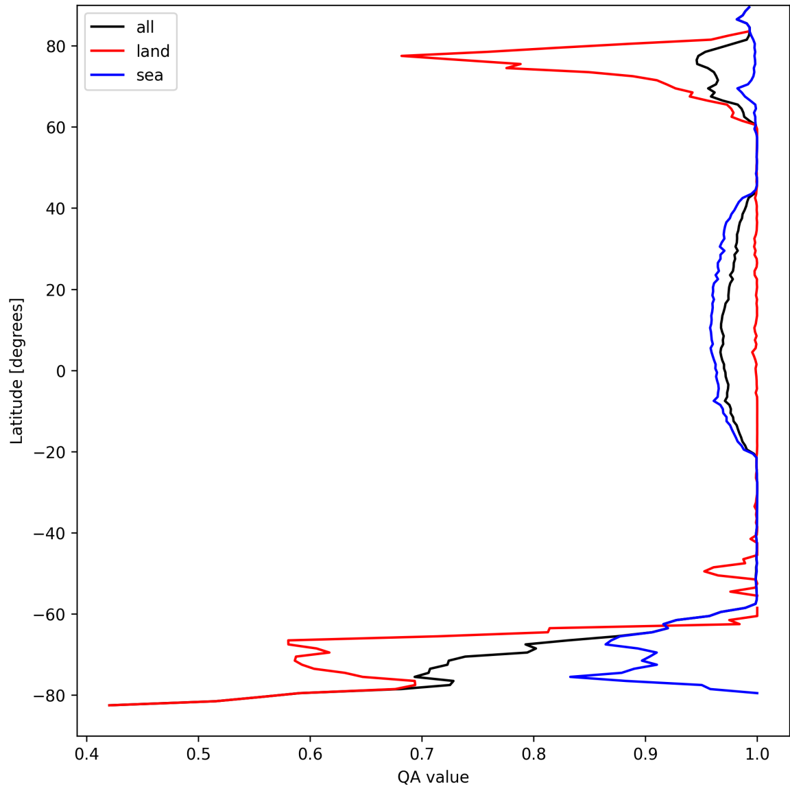
Figure 10: Zonal average of “QA value” for 2025-09-07 to 2025-09-07.
