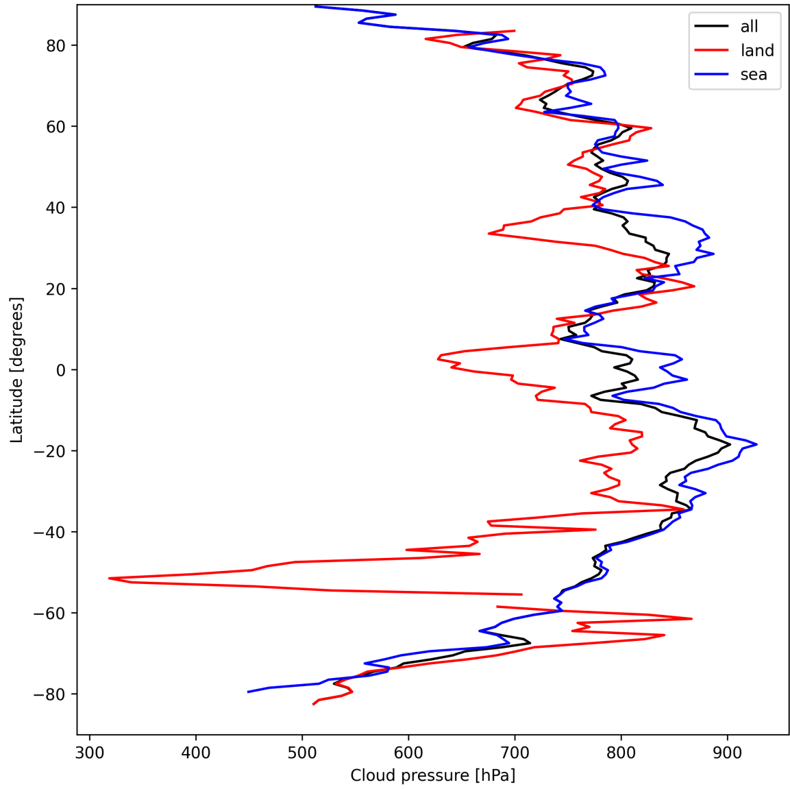
Figure 11: Zonal average of “Cloud pressure” for 2025-09-07 to 2025-09-07.
