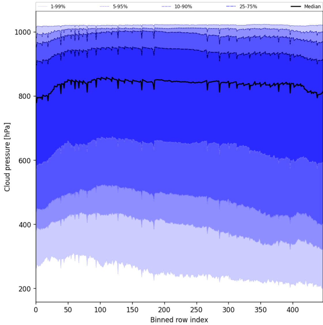
Figure 45: Along track statistics of “Cloud pressure” for 2025-09-07 to 2025-09-07
