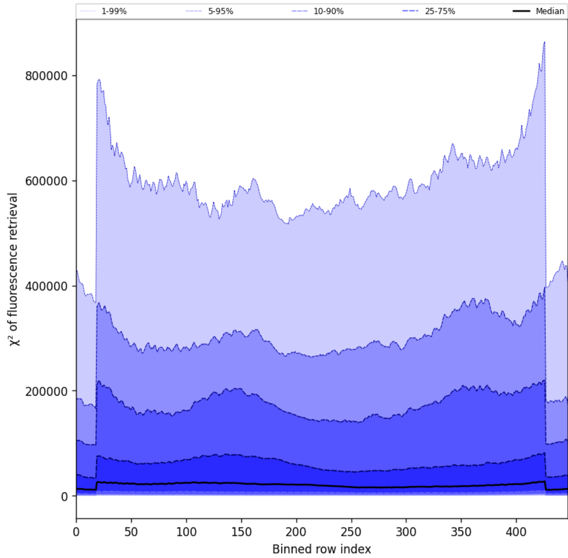
Figure 57: Along track statistics of “ \chi^2 of fluorescence retrieval” for 2025-09-07 to 2025-09-07
