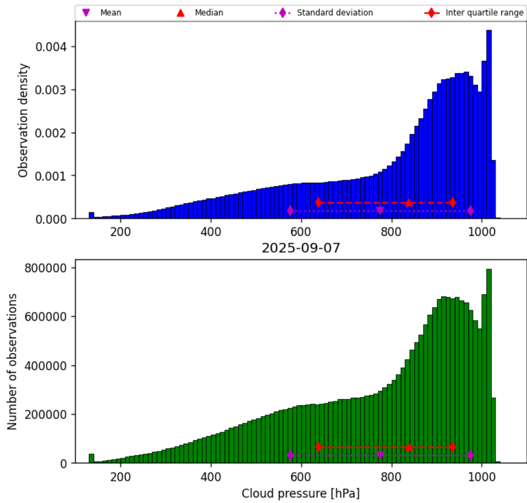
Figure 28: Histogram of “Cloud pressure” for 2025-09-07 to 2025-09-07
