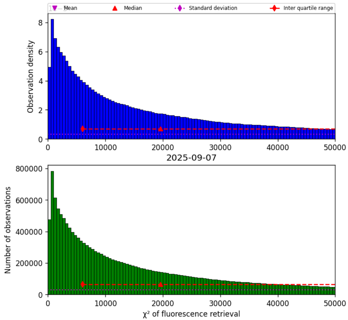
Figure 40: Histogram of “ \chi^2 of fluorescence retrieval” for 2025-09-07 to 2025-09-07
