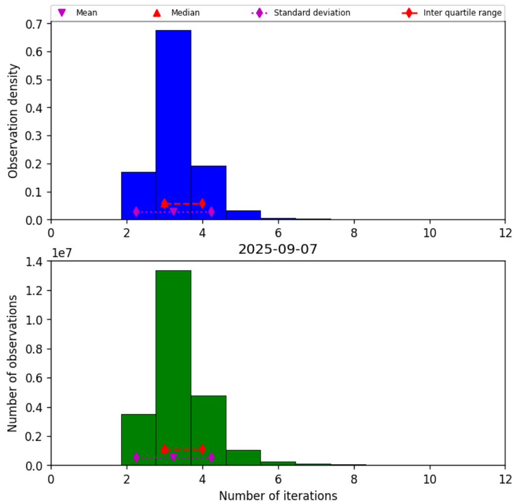
Figure 37: Histogram of “Number of iterations” for 2025-09-07 to 2025-09-07
