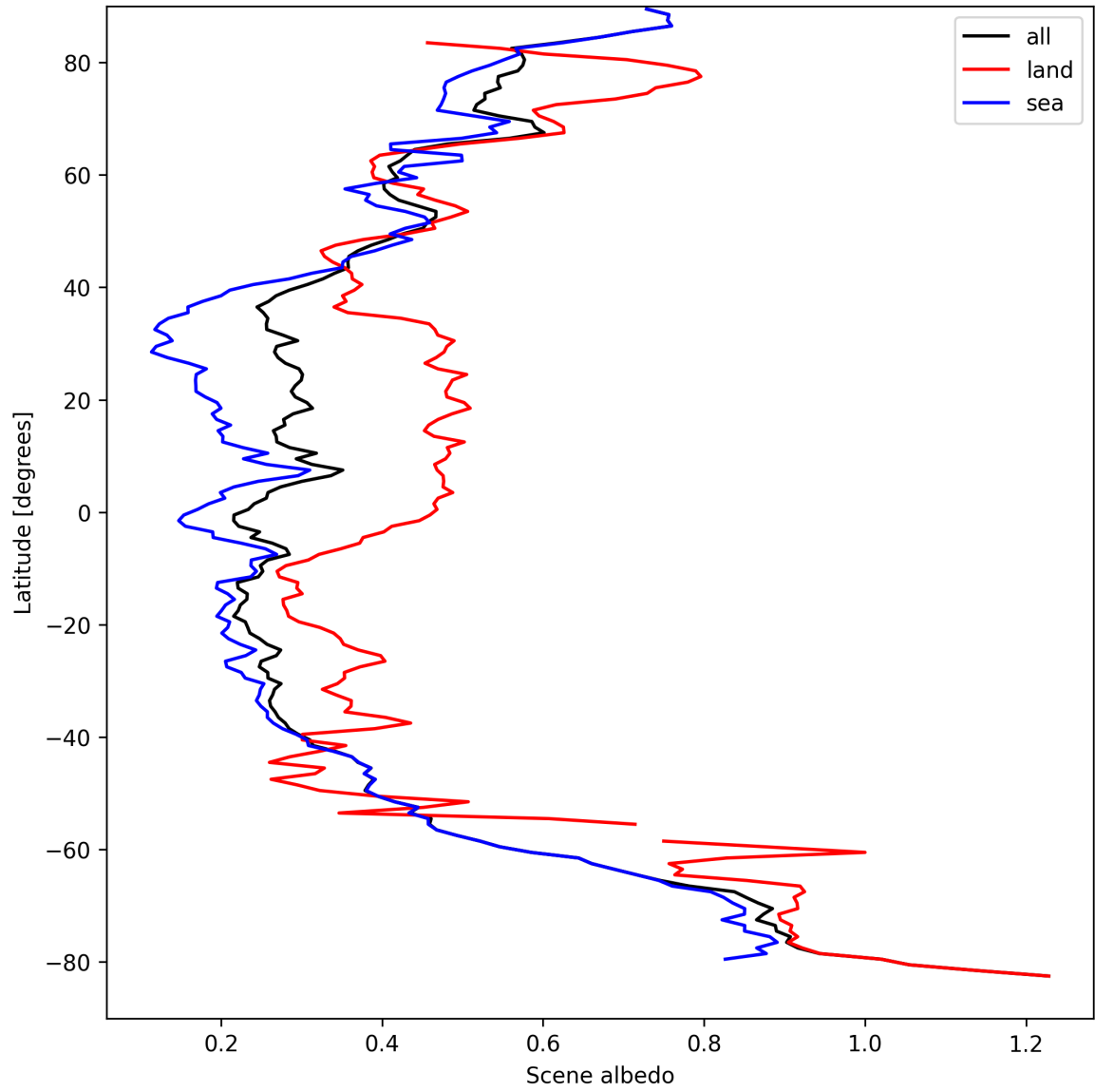
Figure 15: Zonal average of “Scene albedo” for 2025-09-07 to 2025-09-07.
