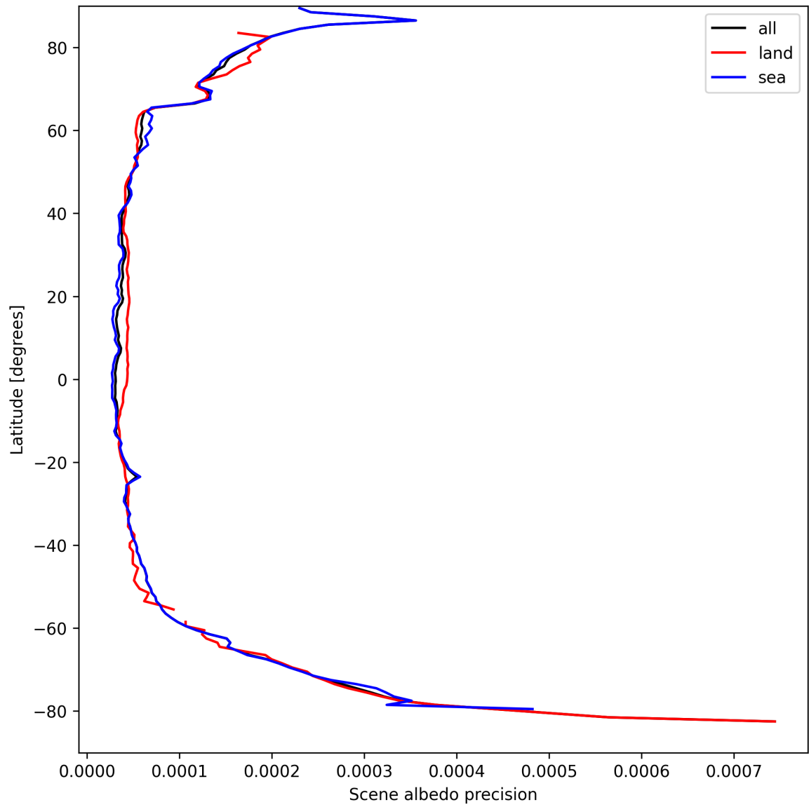
Figure 16: Zonal average of “Scene albedo precision” for 2025-09-07 to 2025-09-07.
