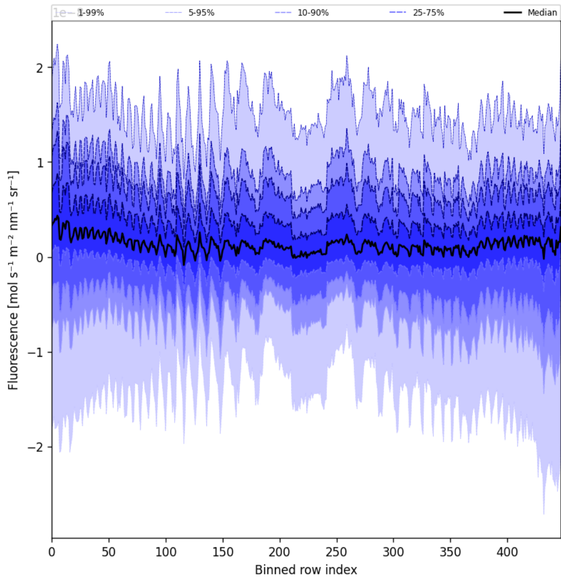
Figure 55: Along track statistics of "Fluorescence" for 2025-09-07 to 2025-09-07
