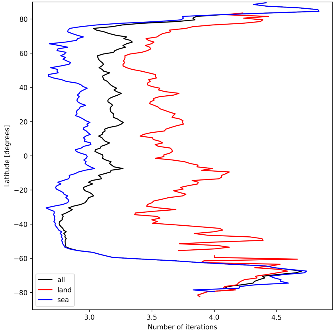
Figure 20: Zonal average of “Number of iterations” for 2025-09-07 to 2025-09-07.
