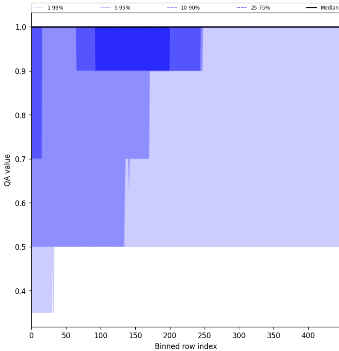
Figure 44: Along track statistics of “QA value” for 2025-09-07 to 2025-09-07
