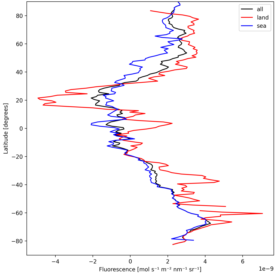
Figure 21: Zonal average of “Fluorescence” for 2025-09-07 to 2025-09-07.
