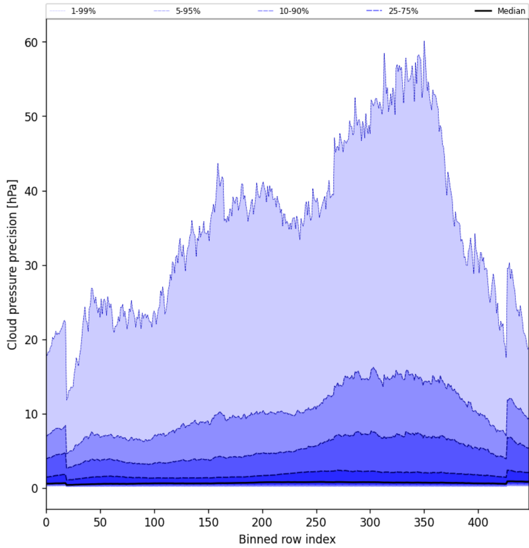
Figure 46: Along track statistics of “Cloud pressure precision” for 2025-09-07 to 2025-09-07
