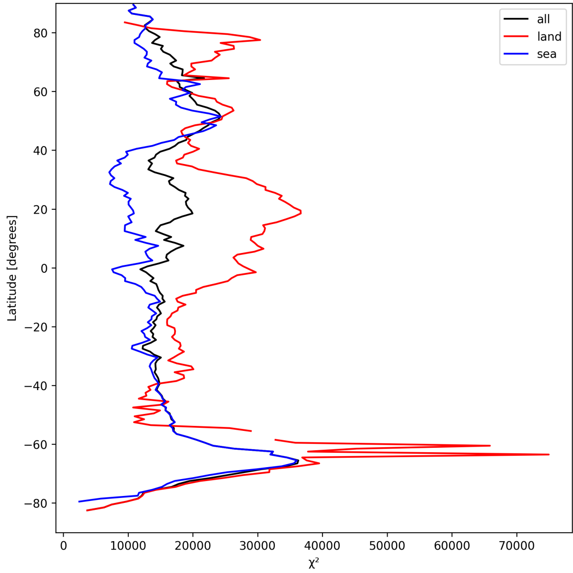
Figure 19: Zonal average of “ \chi^2 ” for 2025-09-07 to 2025-09-07.
