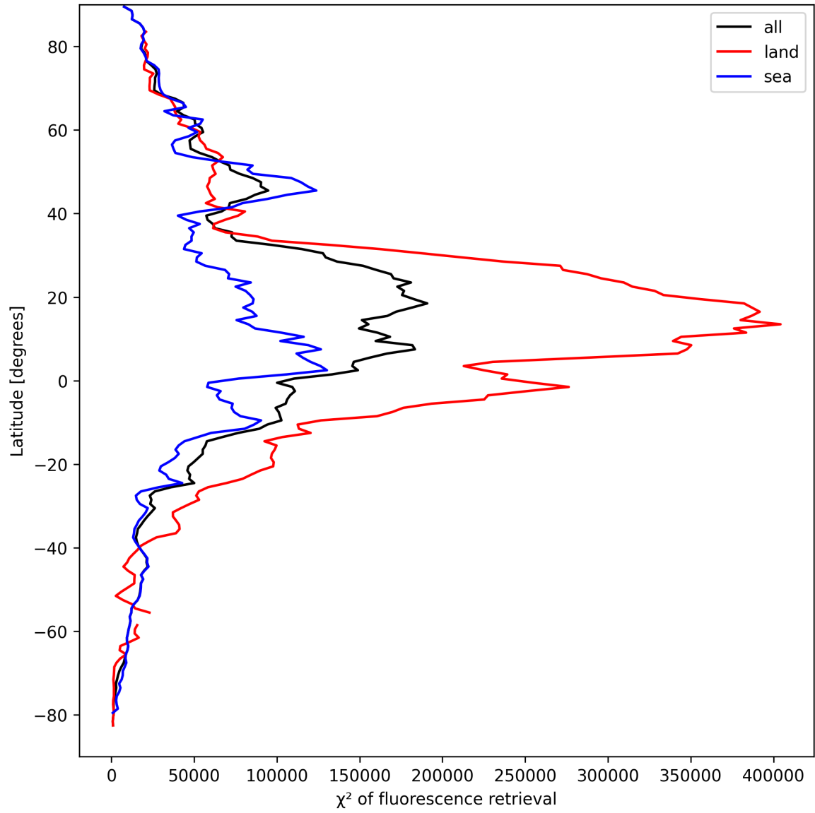
Figure 23: Zonal average of “ \chi^2 of fluorescence retrieval” for 2025-09-07 to 2025-09-07.
