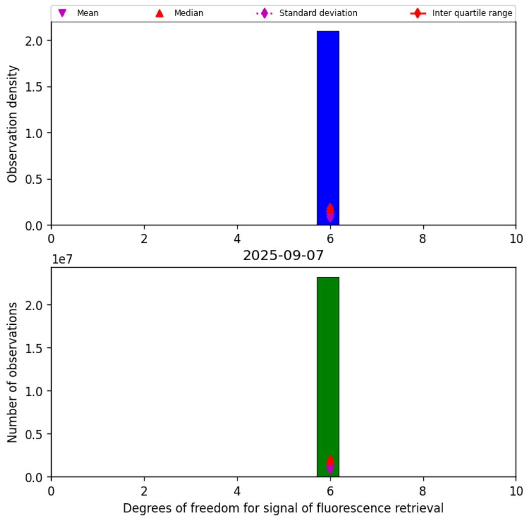
Figure 41: Histogram of “Degrees of freedom for signal of fluorescence retrieval” for 2025-09-07 to 2025-09-07
