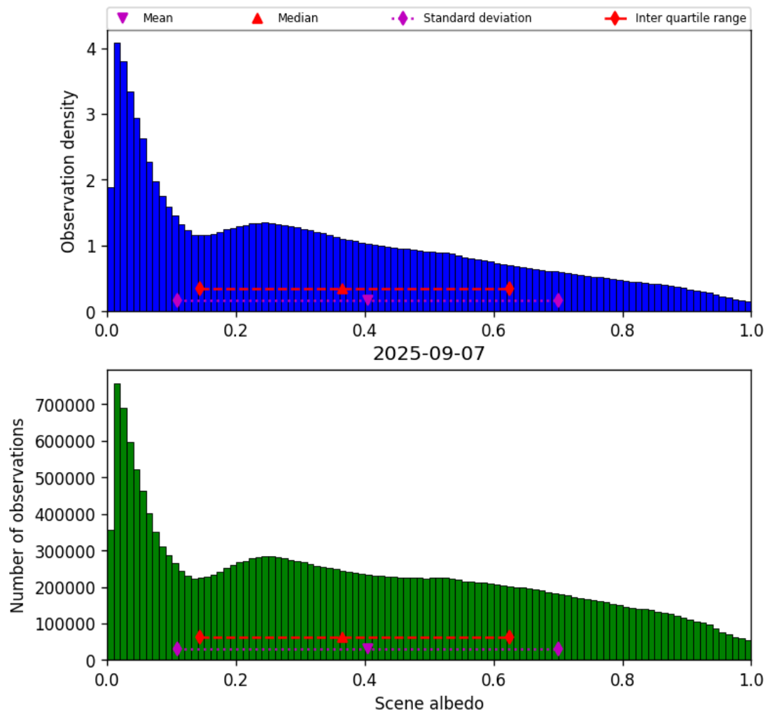
Figure 32: Histogram of “Scene albedo” for 2025-09-07 to 2025-09-07
