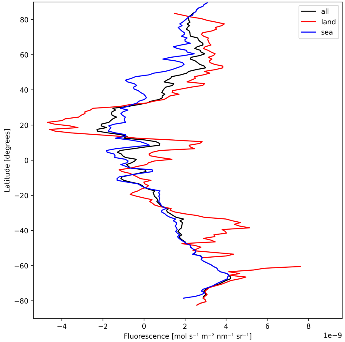
Figure 21: Zonal average of “Fluorescence” for 2025-09-08 to 2025-09-08.
