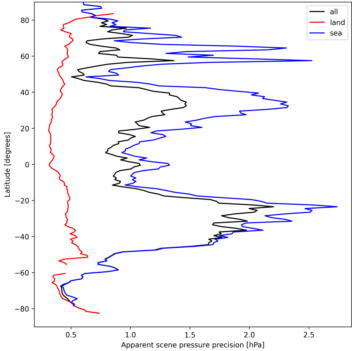
Figure 18: Zonal average of “Apparent scene pressure precision” for 2025-09-08 to 2025-09-08.
