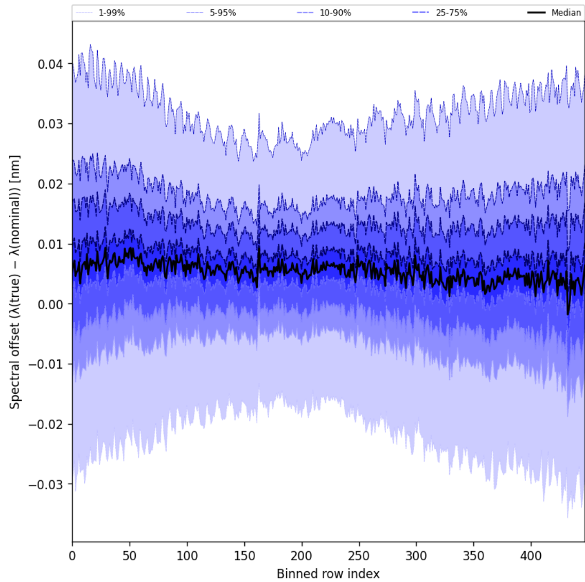
Figure 60: Along track statistics of “Spectral offset ( \lambda_{\text{true}} - \lambda_{\text{nominal}} )” for 2025-09-08 to 2025-09-08
