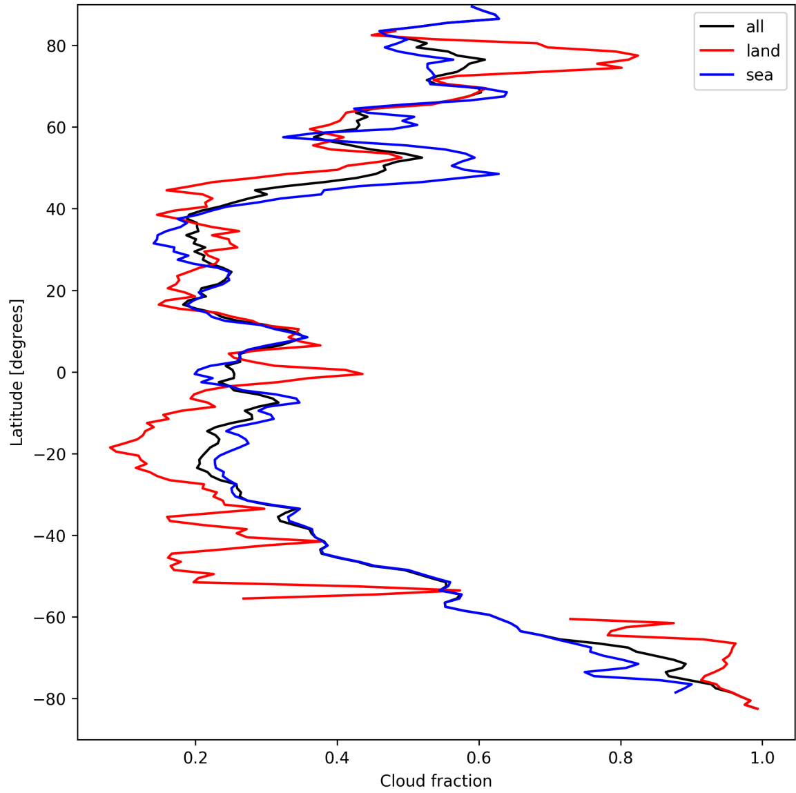
Figure 13: Zonal average of “Cloud fraction” for 2025-09-08 to 2025-09-08.
