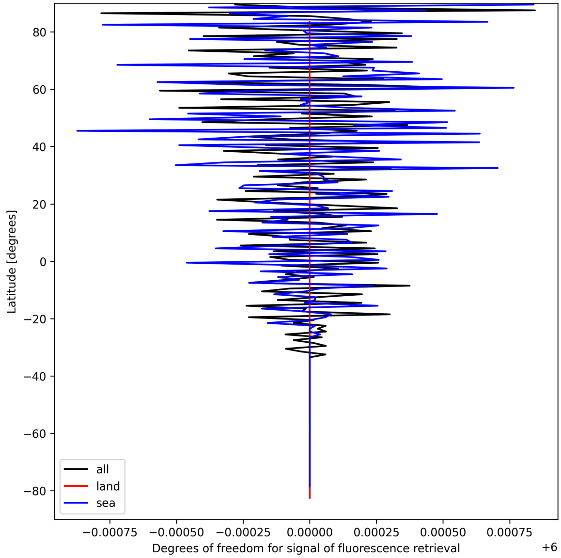
Figure 24: Zonal average of “Degrees of freedom for signal of fluorescence retrieval” for 2025-09-08 to 2025-09-08.
