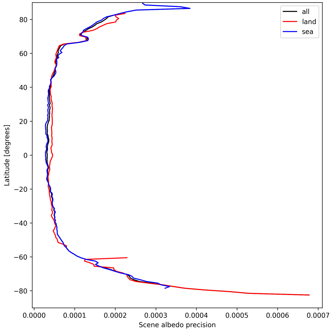
Figure 16: Zonal average of “Scene albedo precision” for 2025-09-08 to 2025-09-08.
