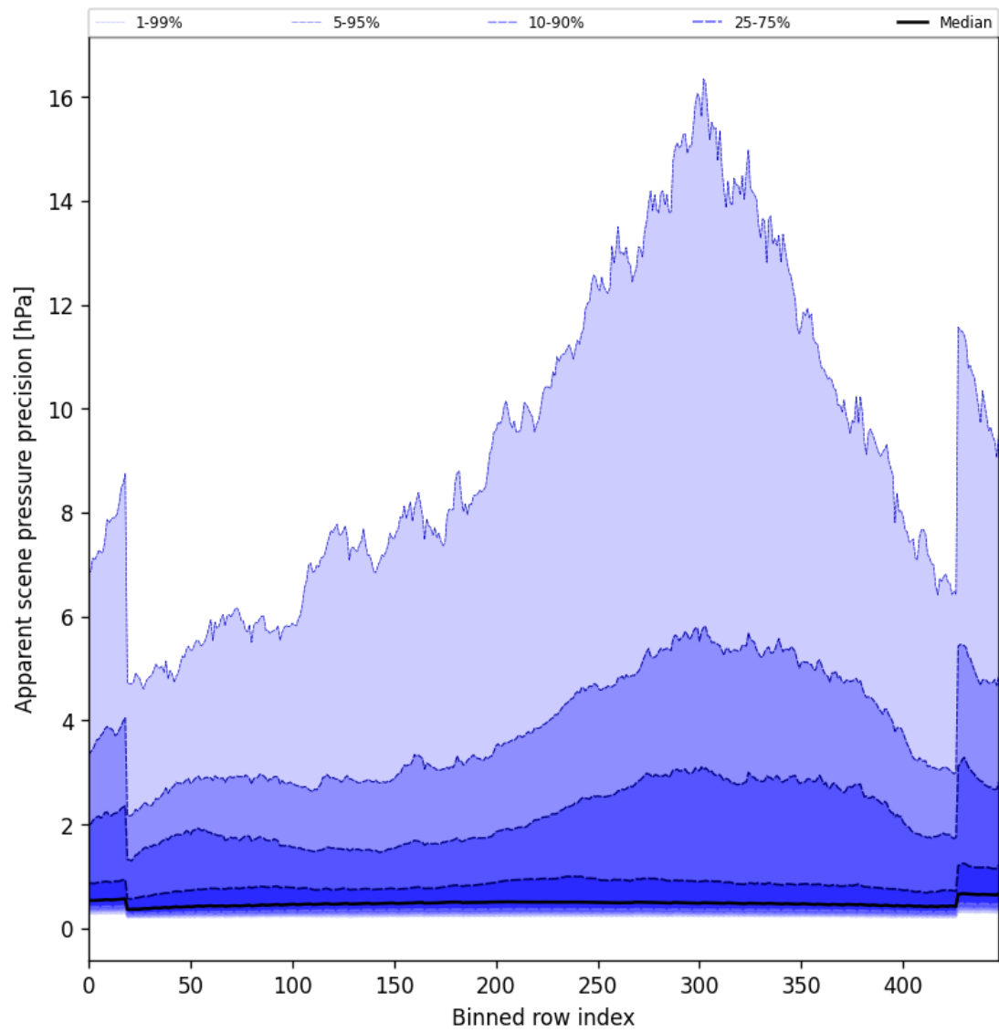
Figure 52: Along track statistics of “Apparent scene pressure precision” for 2025-09-08 to 2025-09-08
