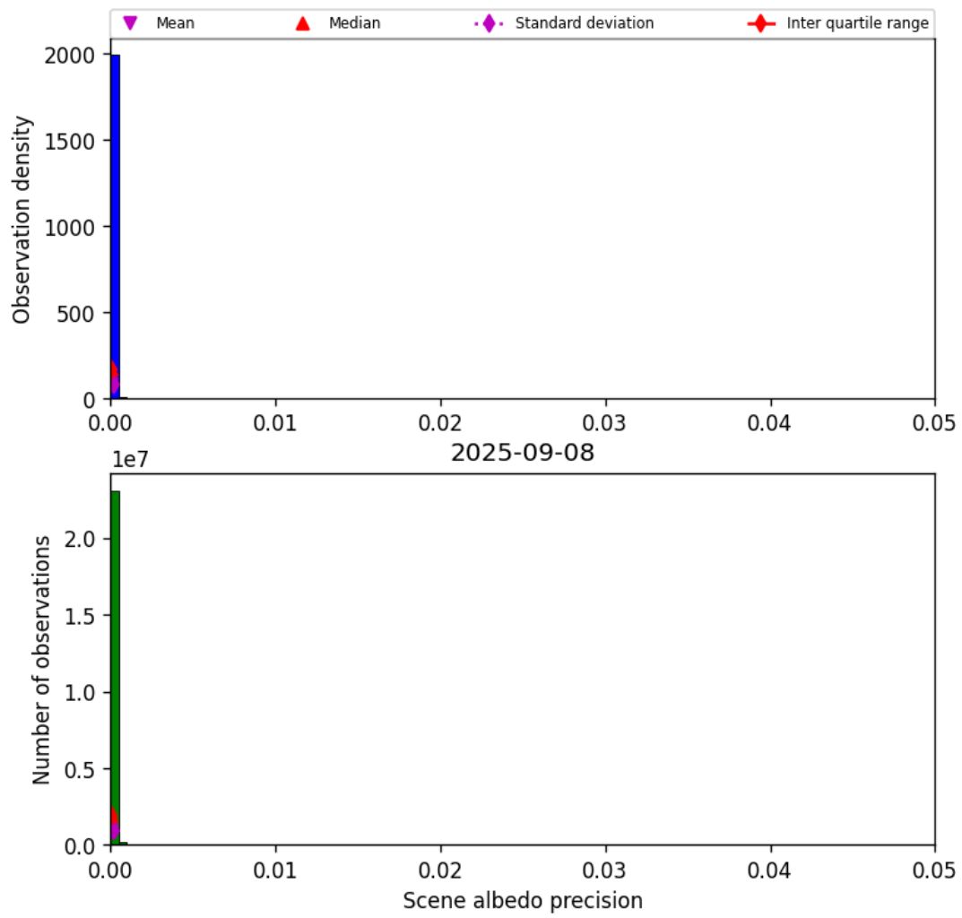
Figure 33: Histogram of “Scene albedo precision” for 2025-09-08 to 2025-09-08
