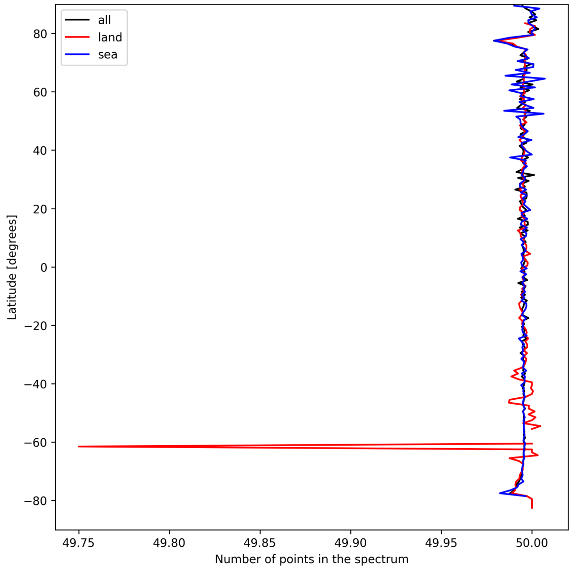
Figure 25: Zonal average of “Number of points in the spectrum” for 2025-09-08 to 2025-09-08.
