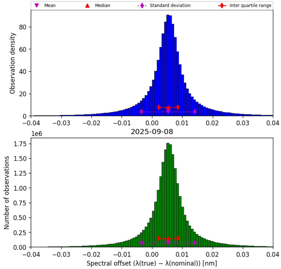
Figure 43: Histogram of “Spectral offset ( \lambda_{\text{true}} - \lambda_{\text{nominal}} )” for 2025-09-08 to 2025-09-08
