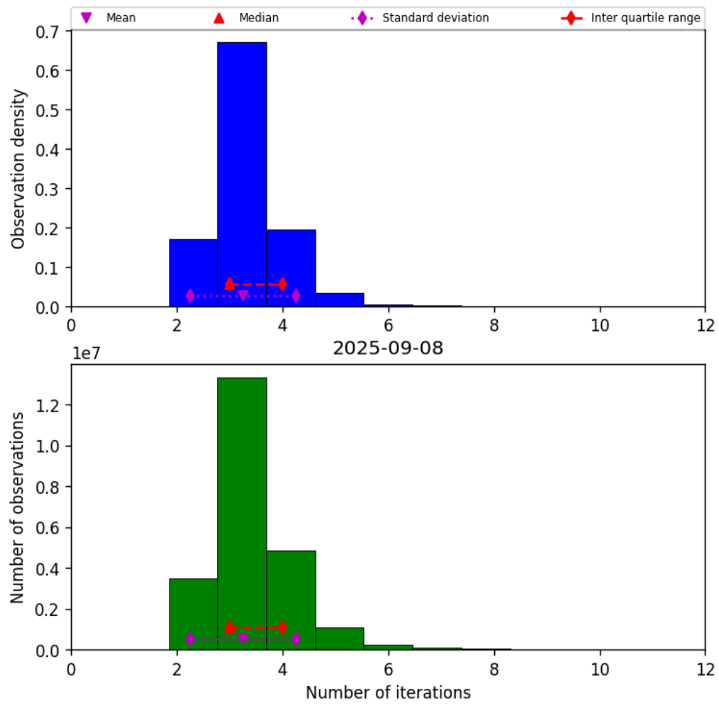
Figure 37: Histogram of “Number of iterations” for 2025-09-08 to 2025-09-08
