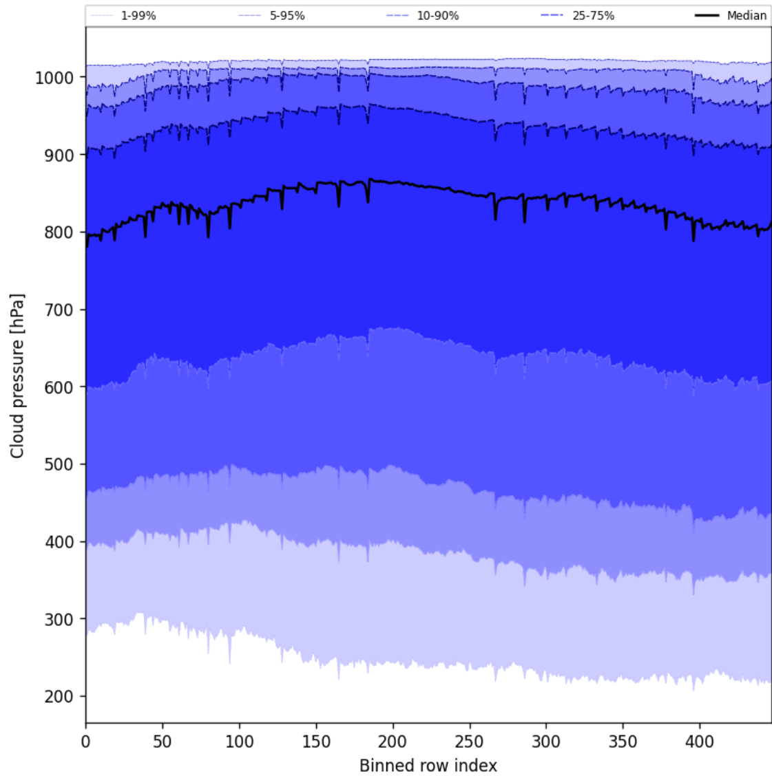
Figure 45: Along track statistics of “Cloud pressure” for 2025-09-08 to 2025-09-08
