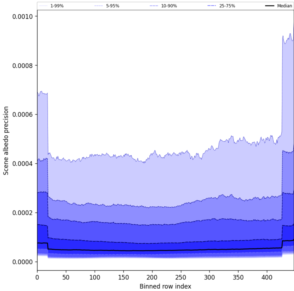
Figure 50: Along track statistics of “Scene albedo precision” for 2025-09-08 to 2025-09-08
