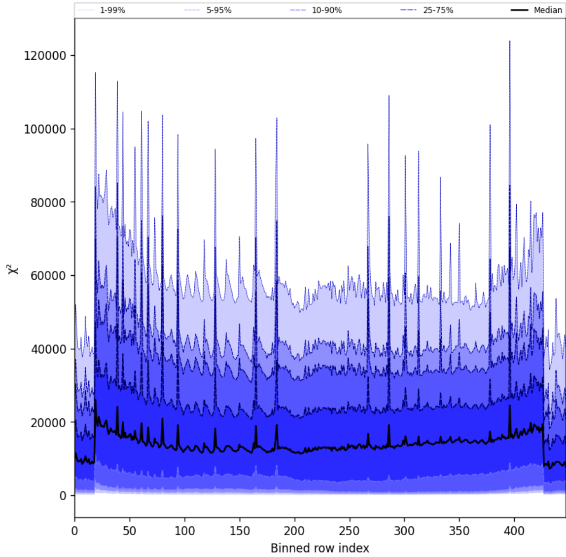
Figure 53: Along track statistics of “ \chi^2 ” for 2025-09-08 to 2025-09-08
