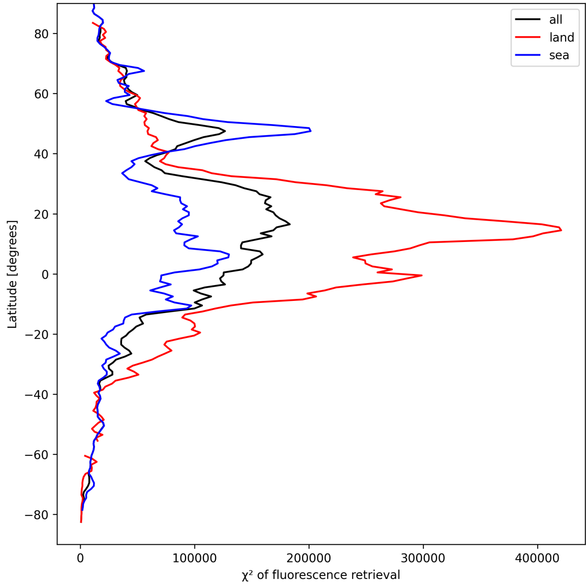
Figure 23: Zonal average of “ \chi^2 of fluorescence retrieval” for 2025-09-08 to 2025-09-08.
