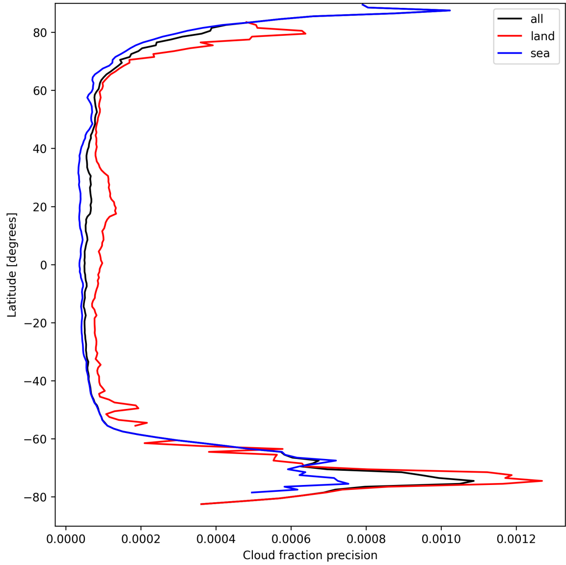
Figure 14: Zonal average of “Cloud fraction precision” for 2025-09-08 to 2025-09-08.
