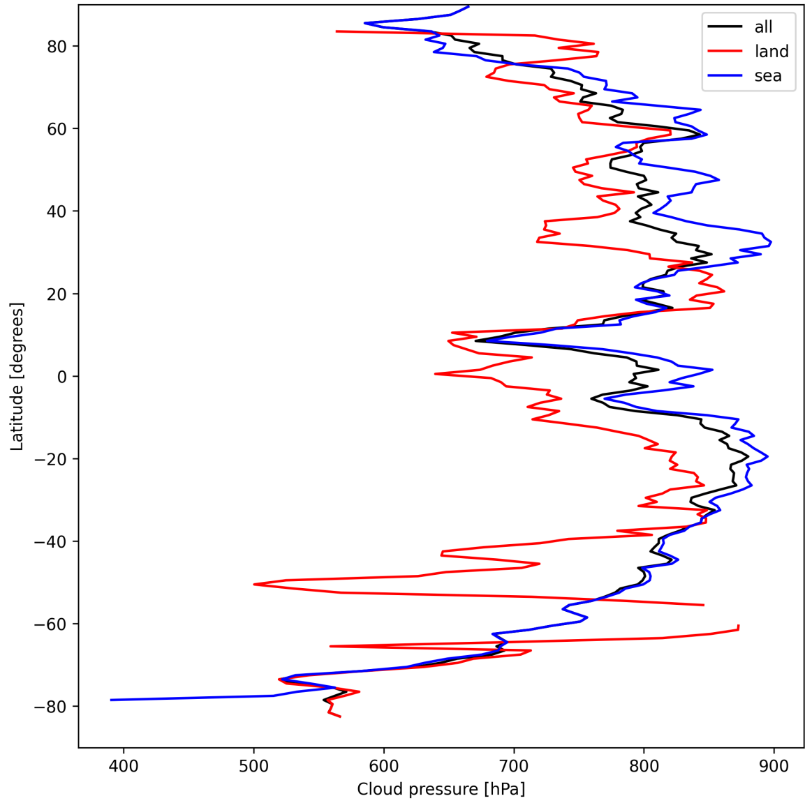
Figure 11: Zonal average of “Cloud pressure” for 2025-09-08 to 2025-09-08.
