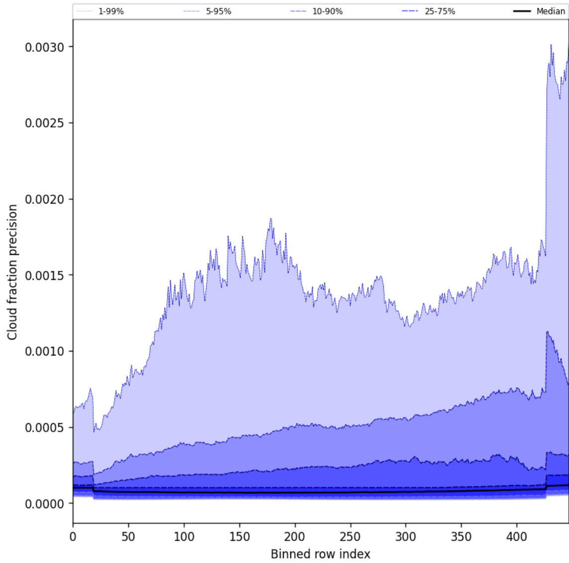
Figure 48: Along track statistics of “Cloud fraction precision” for 2025-09-08 to 2025-09-08
