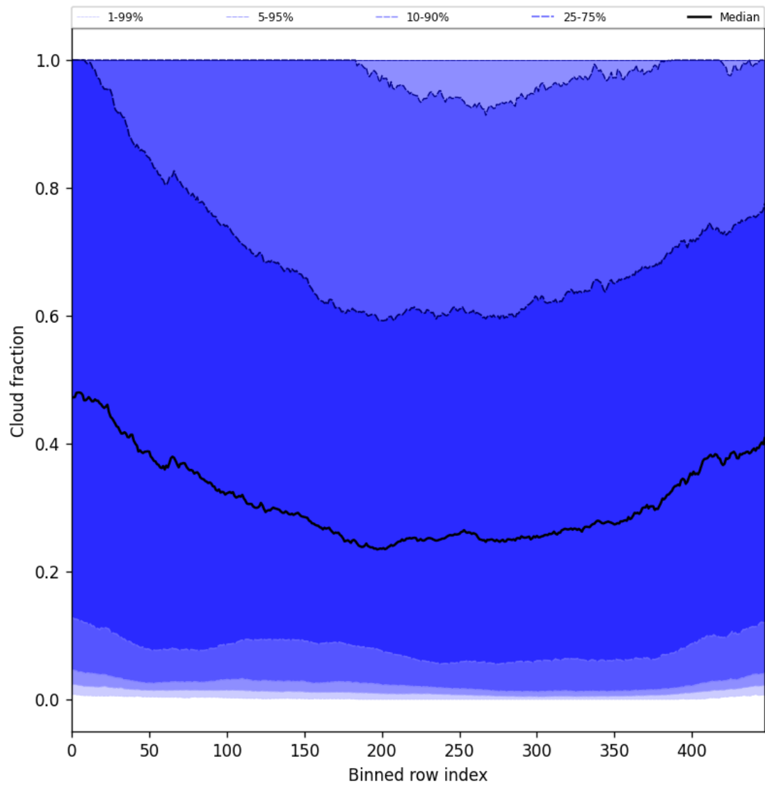
Figure 47: Along track statistics of “Cloud fraction” for 2025-09-08 to 2025-09-08
