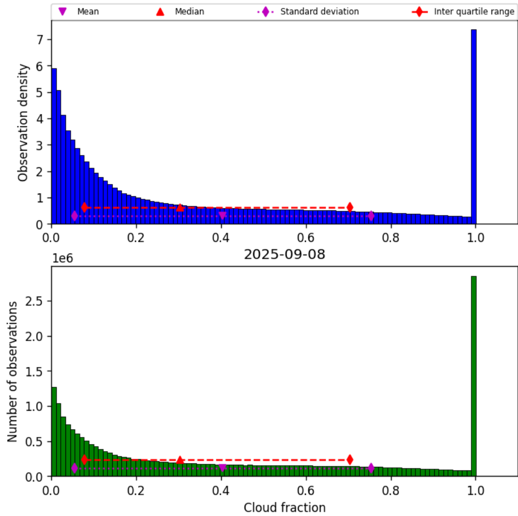
Figure 30: Histogram of “Cloud fraction” for 2025-09-08 to 2025-09-08
