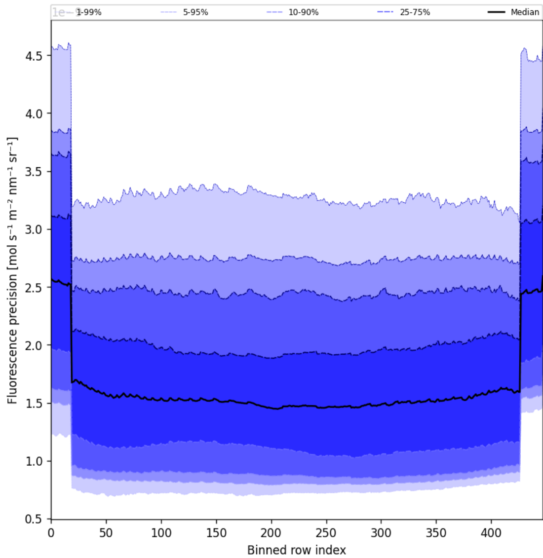
Figure 56: Along track statistics of “Fluorescence precision” for 2025-09-08 to 2025-09-08
