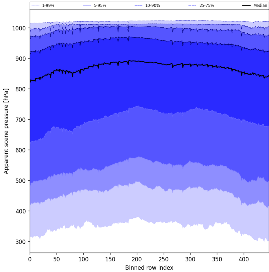
Figure 51: Along track statistics of “Apparent scene pressure” for 2025-09-08 to 2025-09-08
