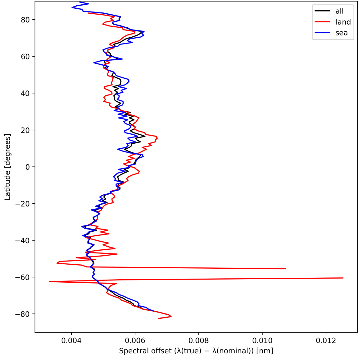
Figure 26: Zonal average of “Spectral offset ( \lambda_{\text{true}} - \lambda_{\text{nominal}} )” for 2025-09-08 to 2025-09-08.
