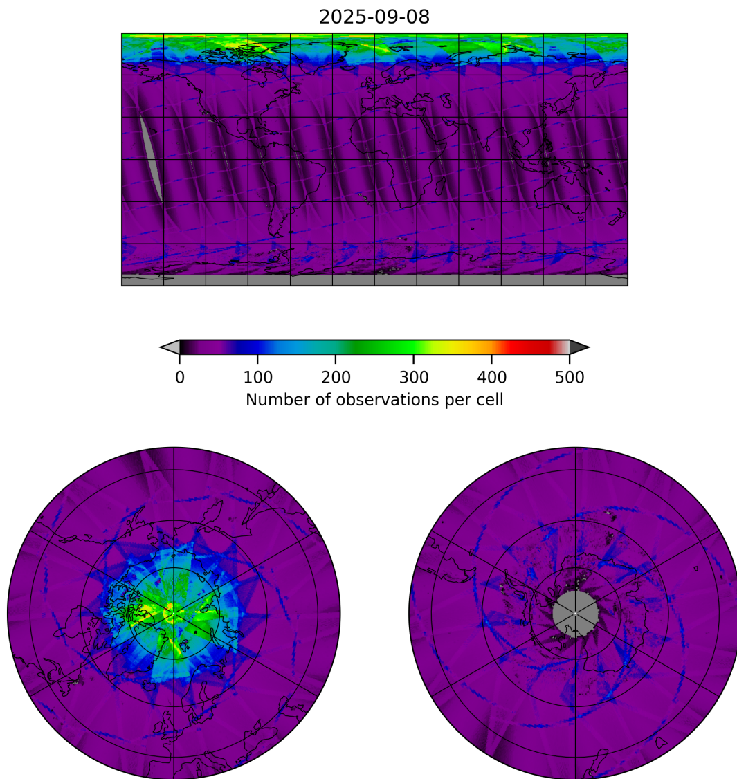
Figure 9: Map of the number of observations for 2025-09-08 to 2025-09-08
