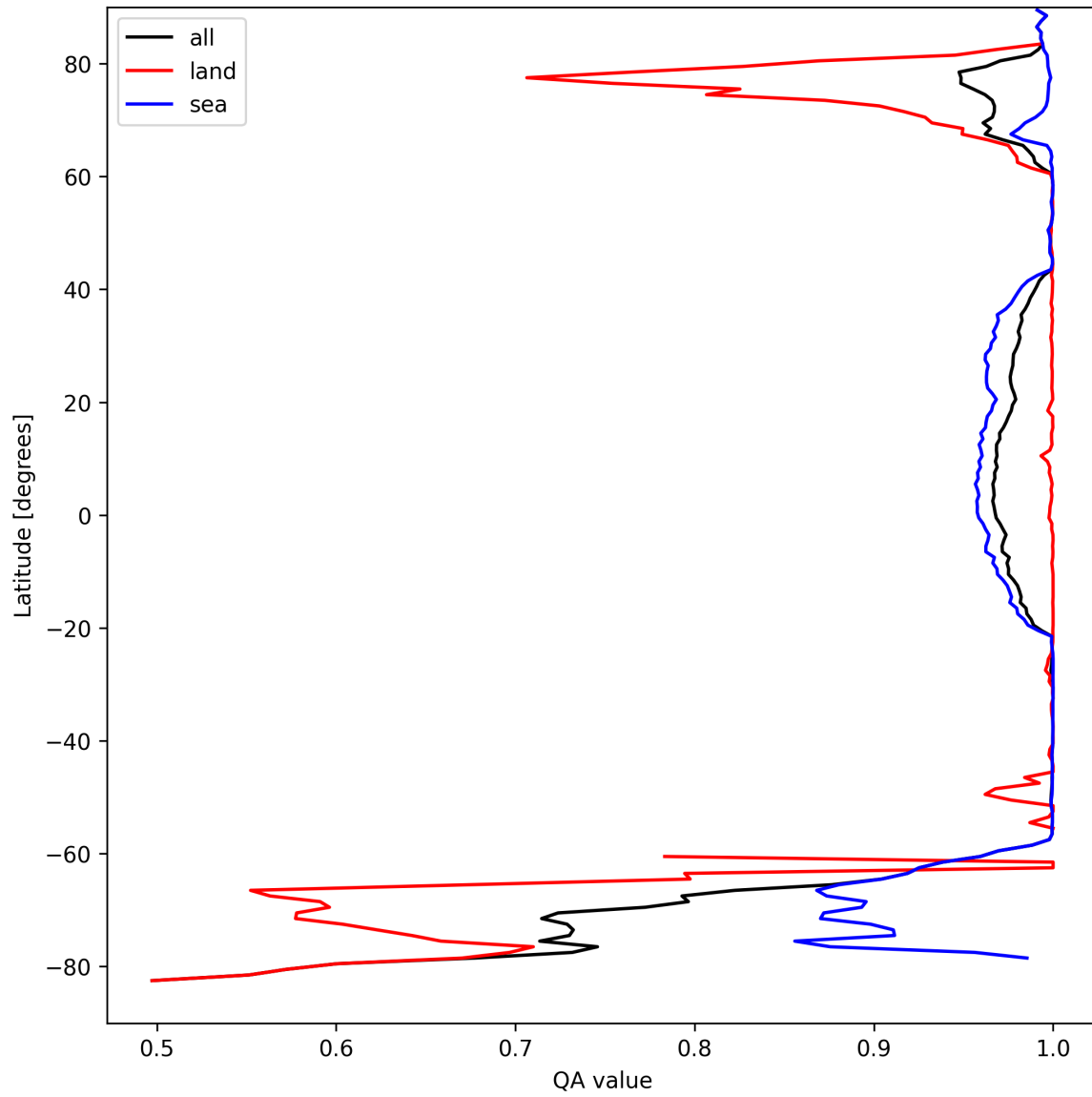
Figure 10: Zonal average of "QA value" for 2025-09-08 to 2025-09-08.
