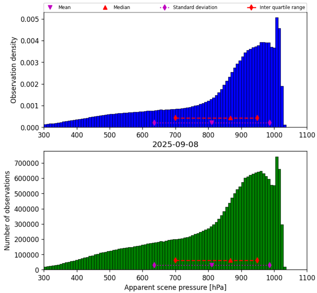
Figure 34: Histogram of “Apparent scene pressure” for 2025-09-08 to 2025-09-08
