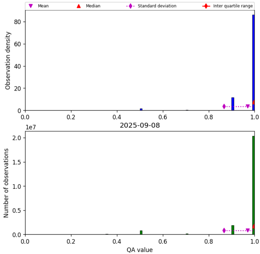
Figure 27: Histogram of “QA value” for 2025-09-08 to 2025-09-08
