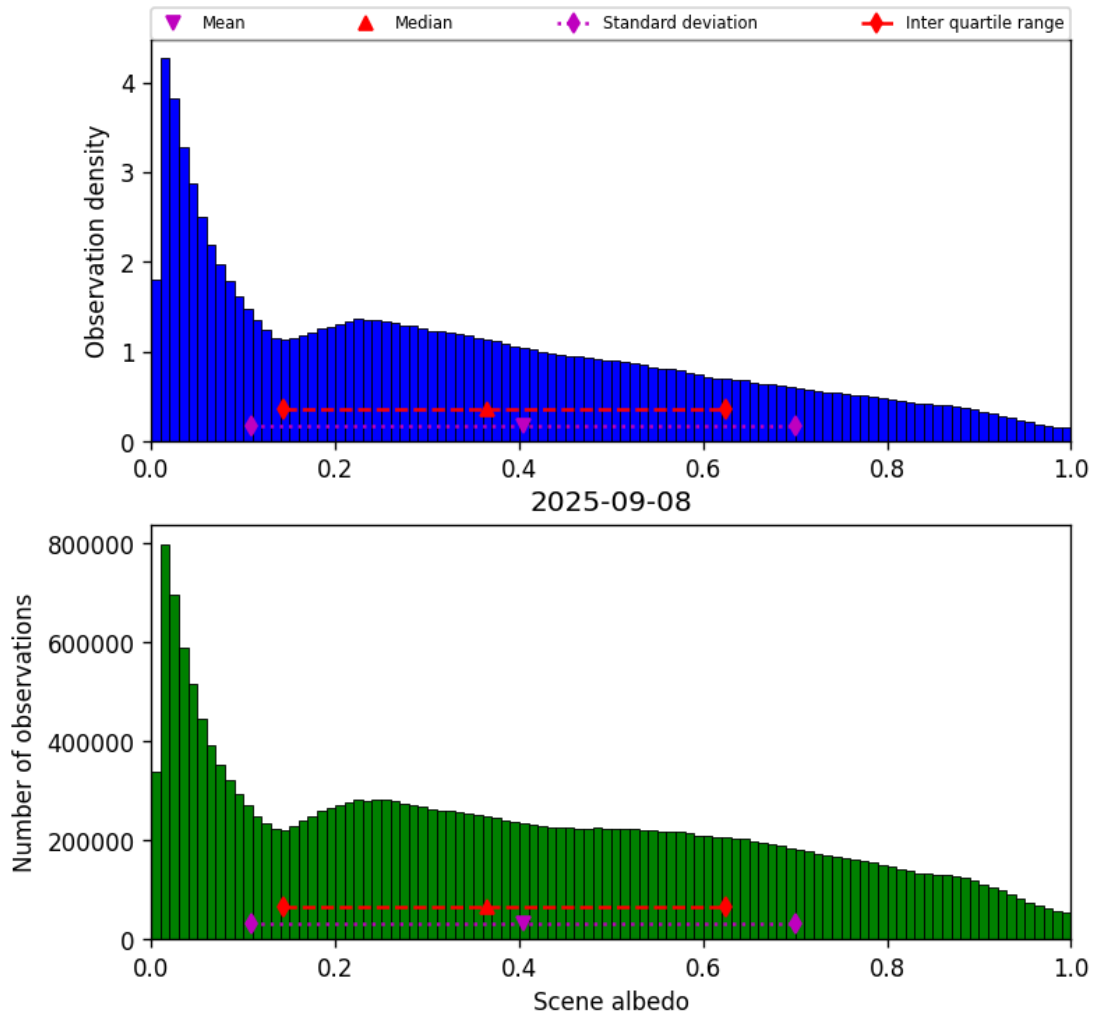
Figure 32: Histogram of “Scene albedo” for 2025-09-08 to 2025-09-08
