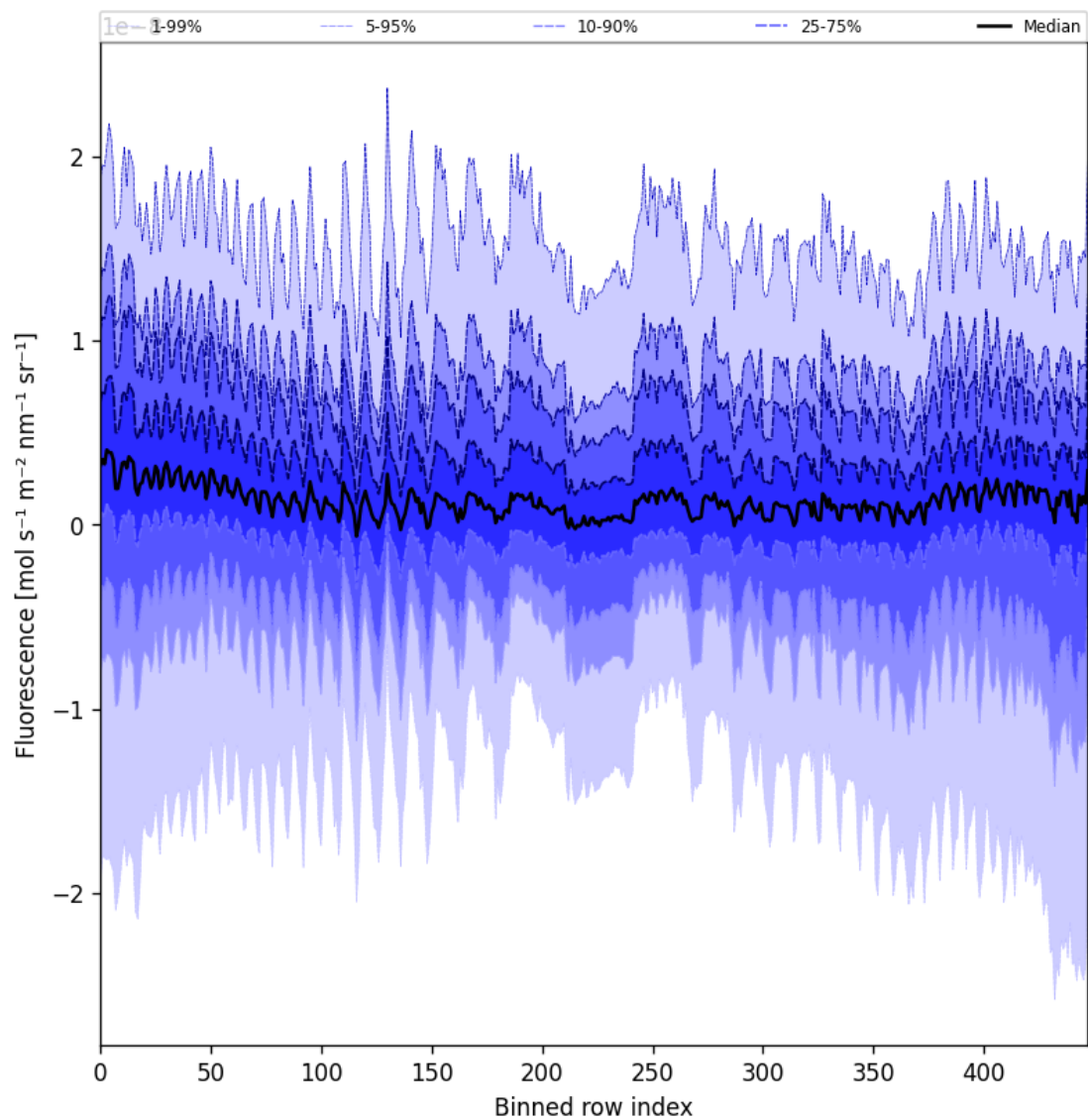
Figure 55: Along track statistics of “Fluorescence” for 2025-09-08 to 2025-09-08
