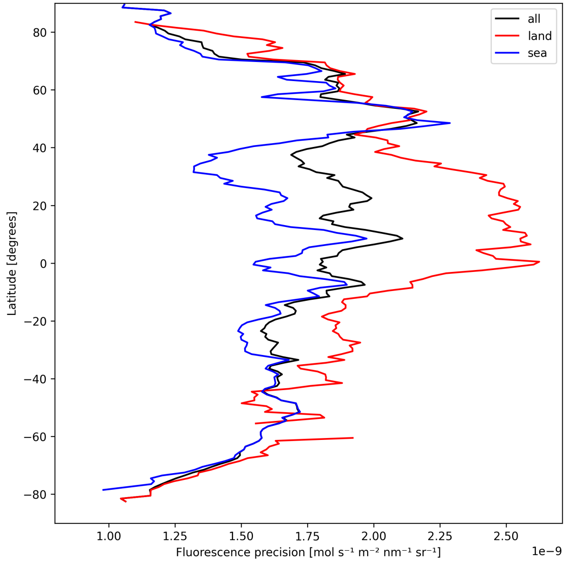
Figure 22: Zonal average of “Fluorescence precision” for 2025-09-08 to 2025-09-08.
