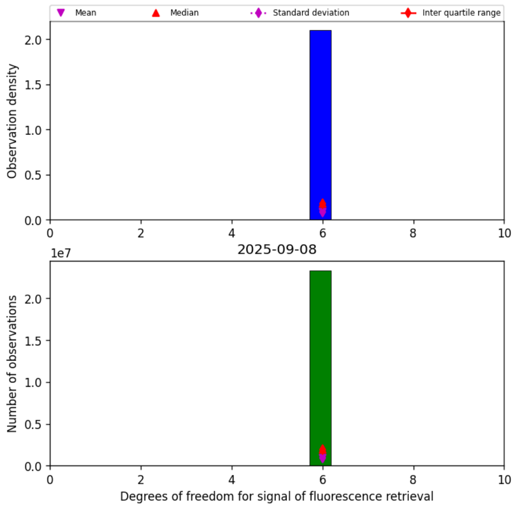
Figure 41: Histogram of “Degrees of freedom for signal of fluorescence retrieval” for 2025-09-08 to 2025-09-08
