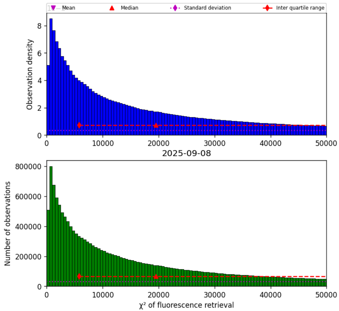
Figure 40: Histogram of “ \chi^2 of fluorescence retrieval” for 2025-09-08 to 2025-09-08
