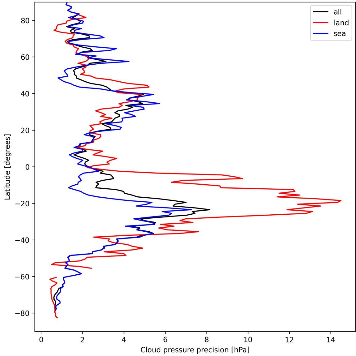
Figure 12: Zonal average of “Cloud pressure precision” for 2025-09-08 to 2025-09-08.
