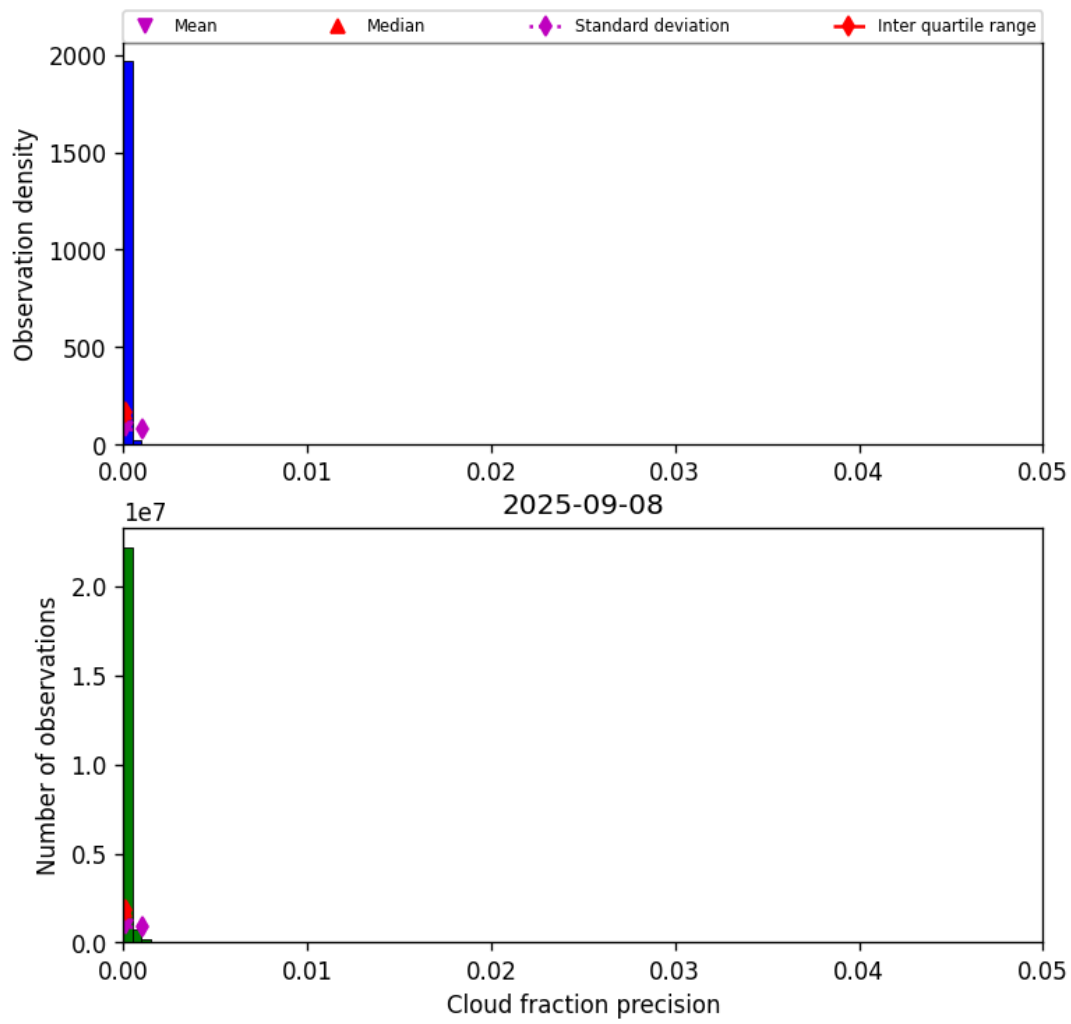
Figure 31: Histogram of “Cloud fraction precision” for 2025-09-08 to 2025-09-08
