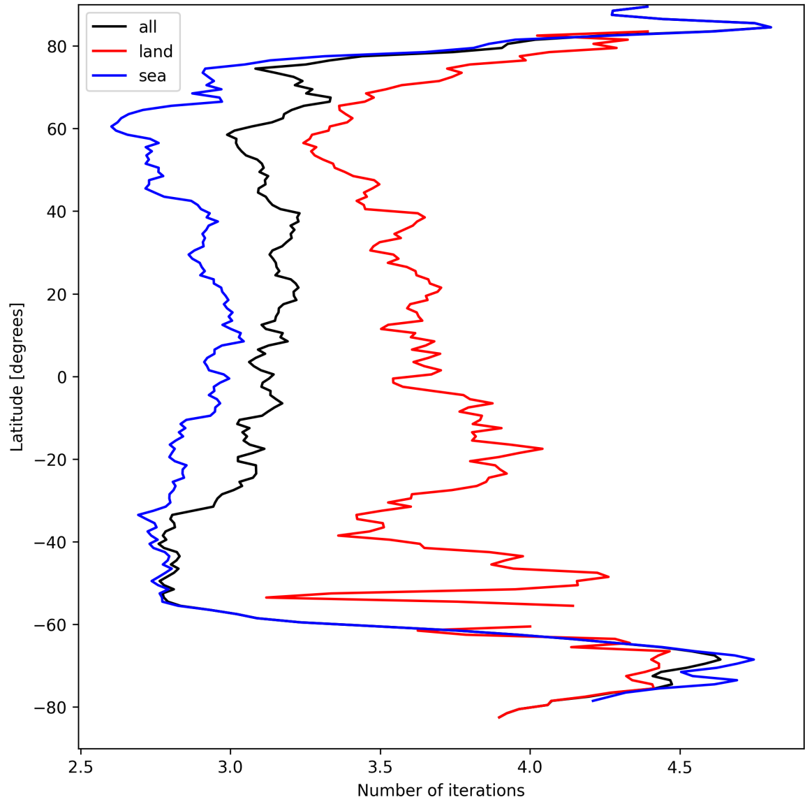
Figure 20: Zonal average of “Number of iterations” for 2025-09-08 to 2025-09-08.
