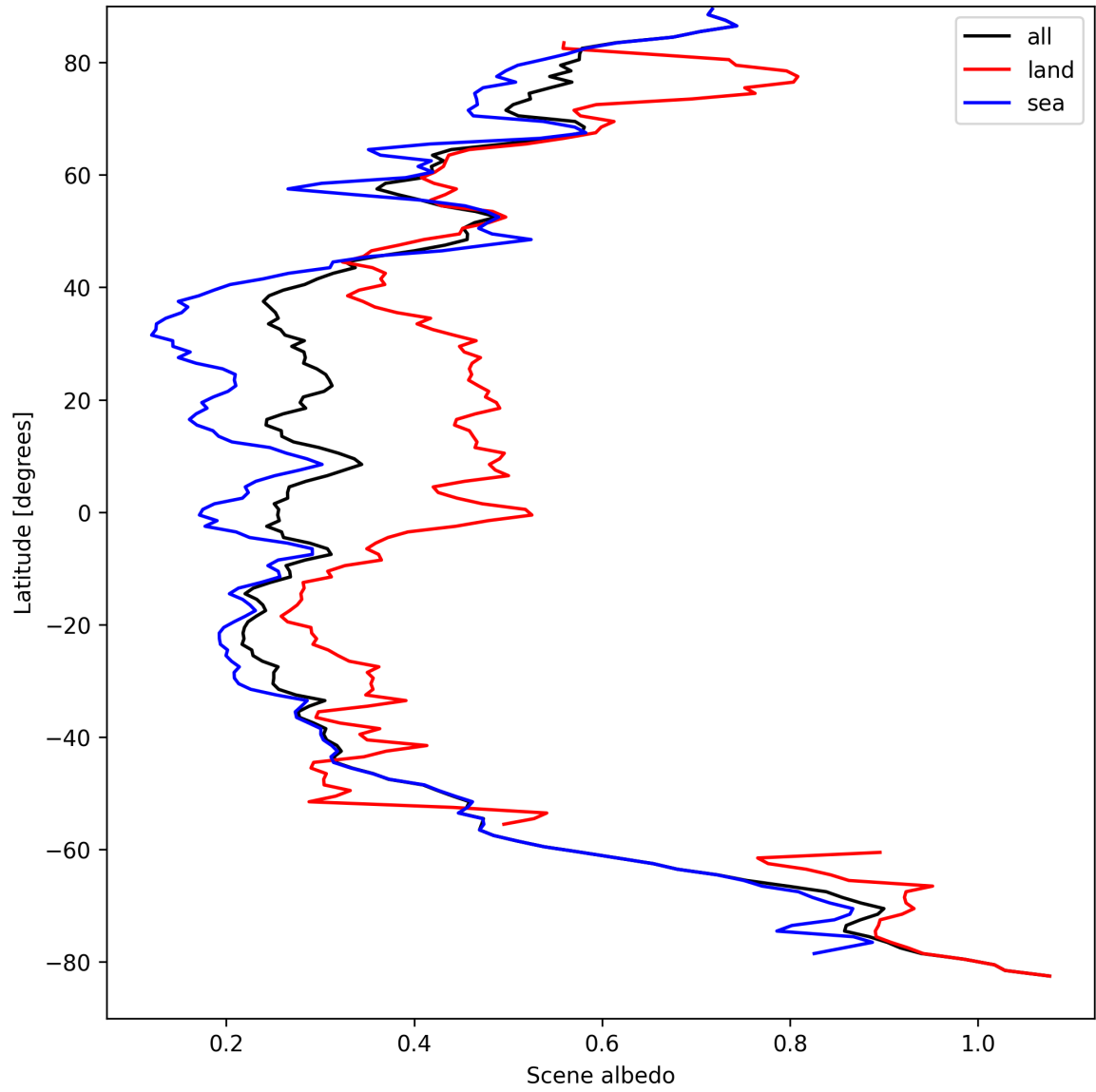
Figure 15: Zonal average of “Scene albedo” for 2025-09-08 to 2025-09-08.
