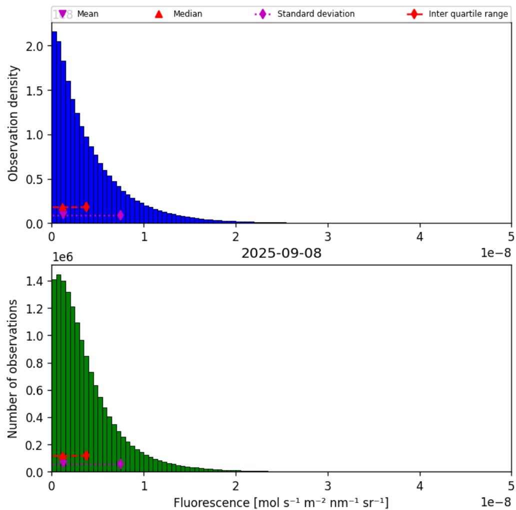
Figure 38: Histogram of “Fluorescence” for 2025-09-08 to 2025-09-08
