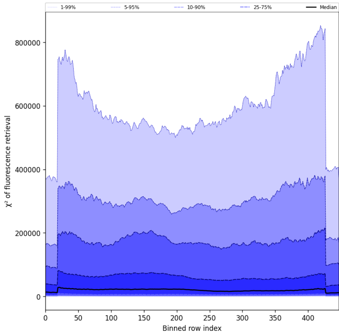
Figure 57: Along track statistics of “ \chi^2 of fluorescence retrieval” for 2025-09-08 to 2025-09-08
