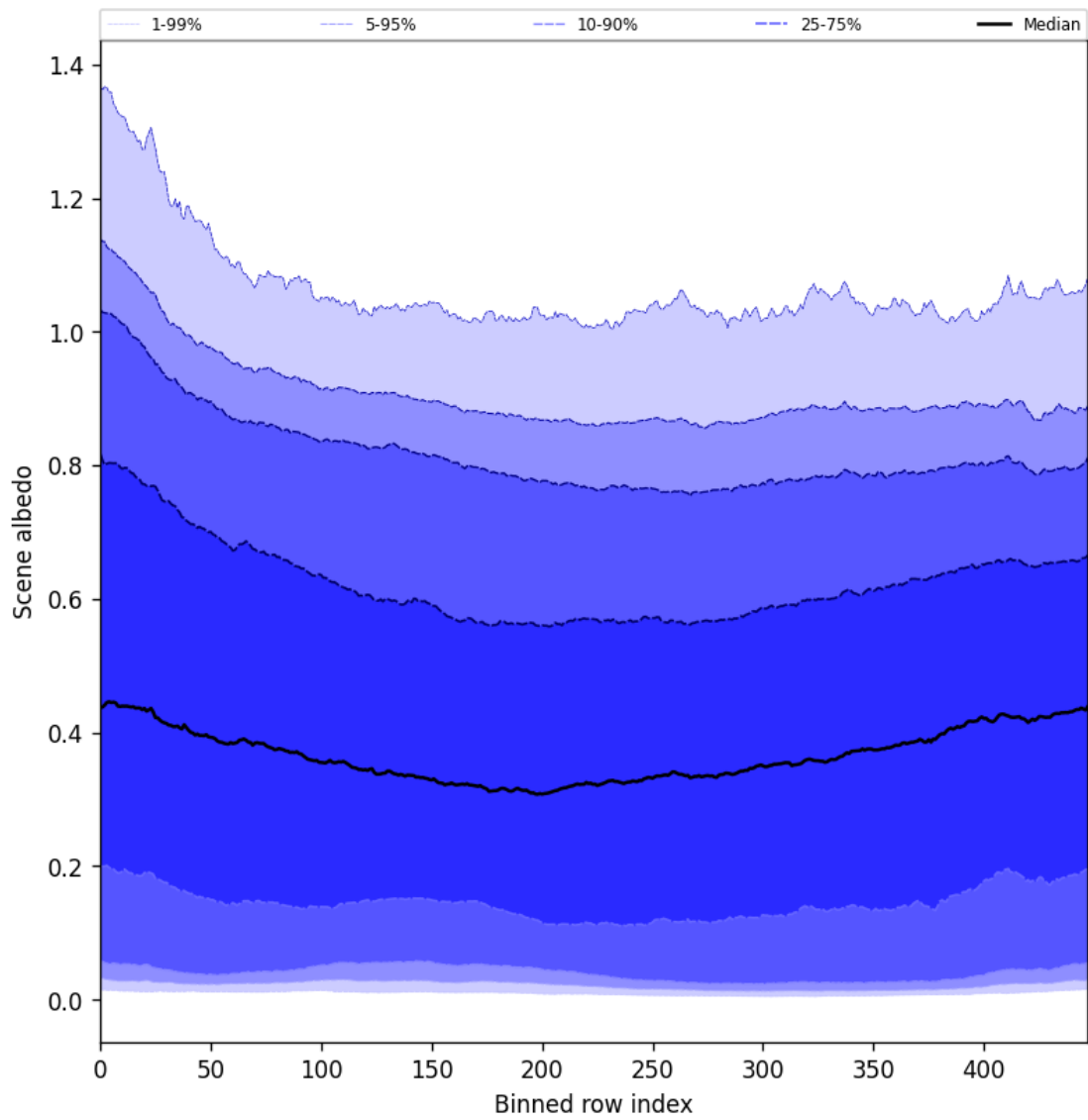
Figure 49: Along track statistics of “Scene albedo” for 2025-09-08 to 2025-09-08
