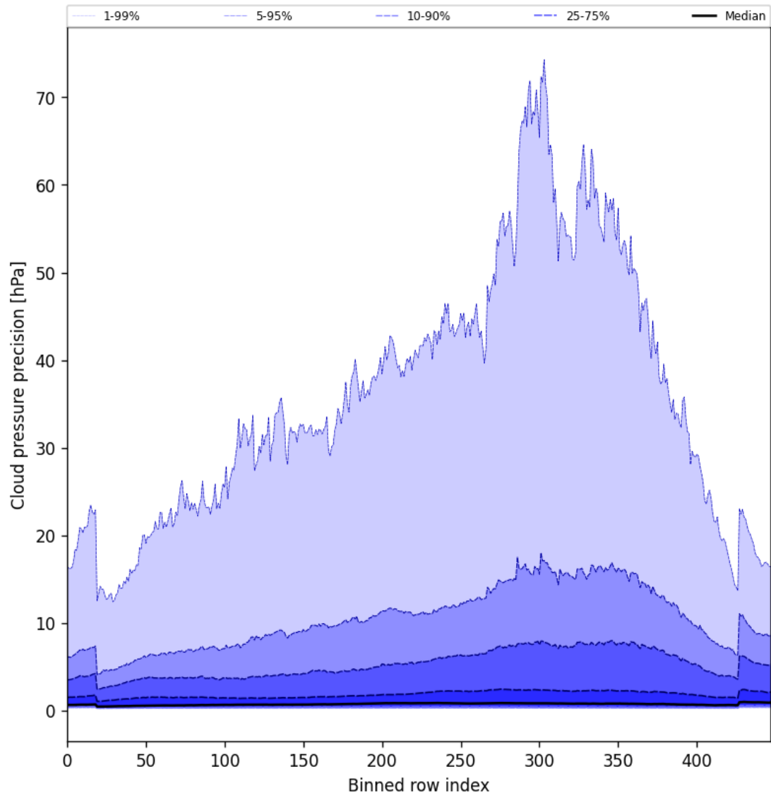
Figure 46: Along track statistics of “Cloud pressure precision” for 2025-09-08 to 2025-09-08
