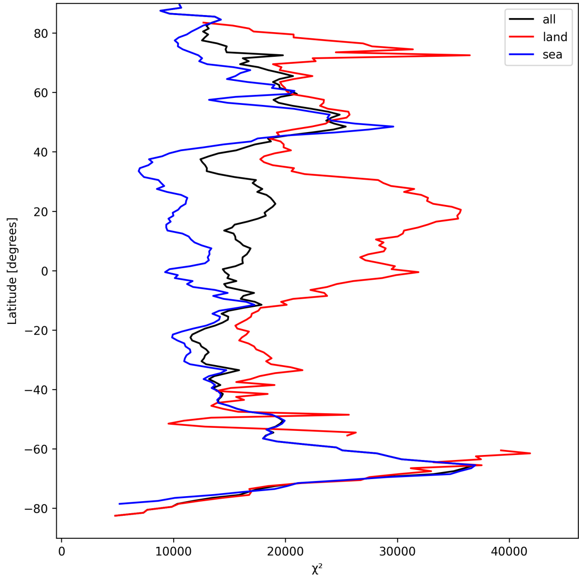
Figure 19: Zonal average of “ \chi^2 ” for 2025-09-08 to 2025-09-08.
