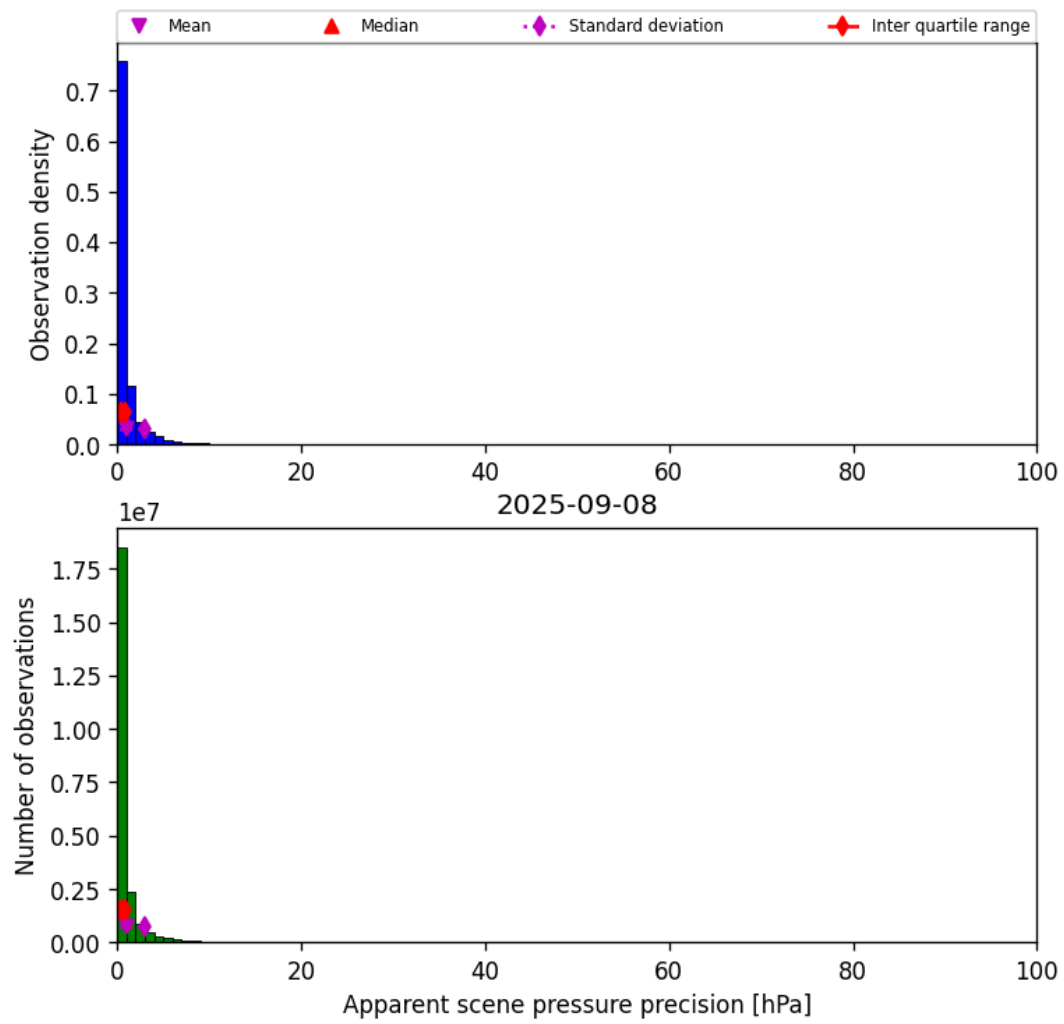
Figure 35: Histogram of “Apparent scene pressure precision” for 2025-09-08 to 2025-09-08
