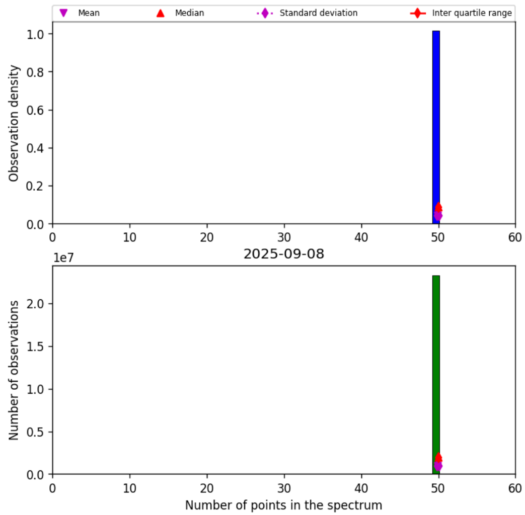
Figure 42: Histogram of “Number of points in the spectrum” for 2025-09-08 to 2025-09-08
