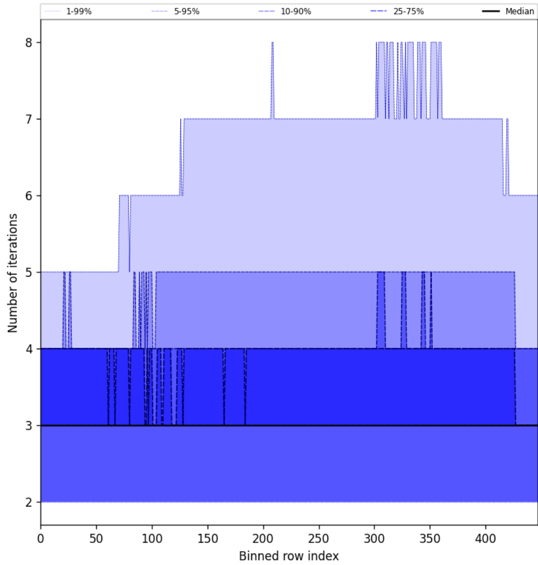
Figure 54: Along track statistics of “Number of iterations” for 2025-09-08 to 2025-09-08
