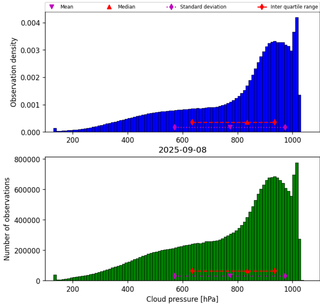
Figure 28: Histogram of “Cloud pressure” for 2025-09-08 to 2025-09-08
