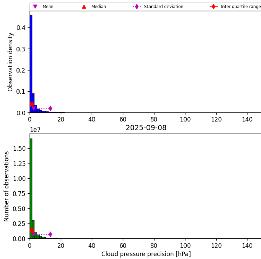
Figure 29: Histogram of “Cloud pressure precision” for 2025-09-08 to 2025-09-08
