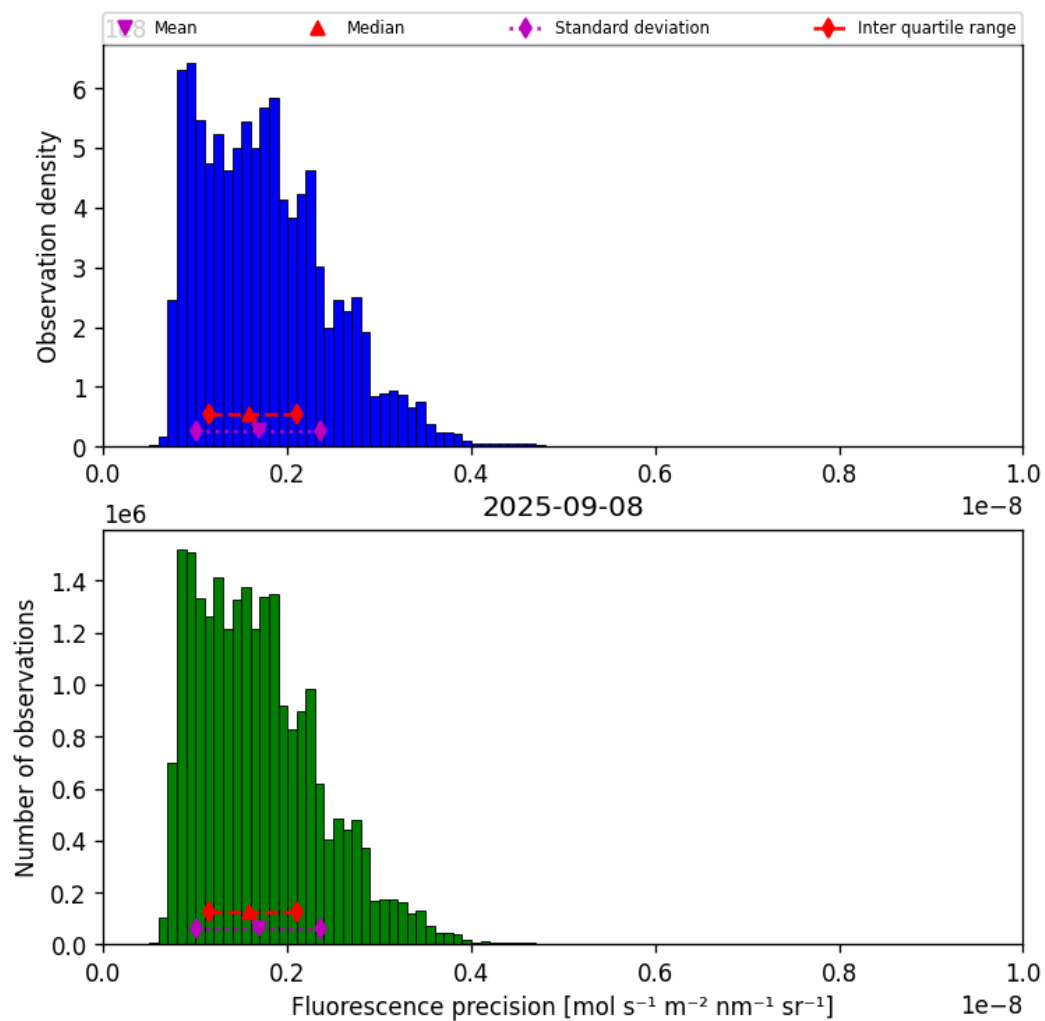
Figure 39: Histogram of “Fluorescence precision” for 2025-09-08 to 2025-09-08
