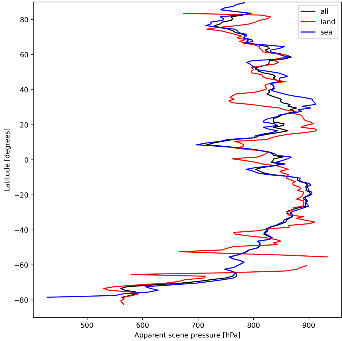
Figure 17: Zonal average of “Apparent scene pressure” for 2025-09-08 to 2025-09-08.
