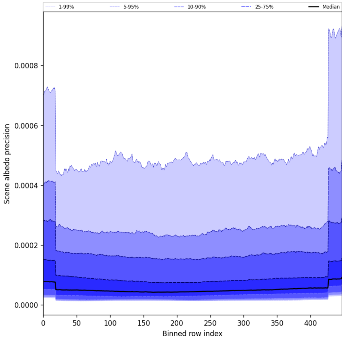
Figure 50: Along track statistics of “Scene albedo precision” for 2025-09-11 to 2025-09-12
