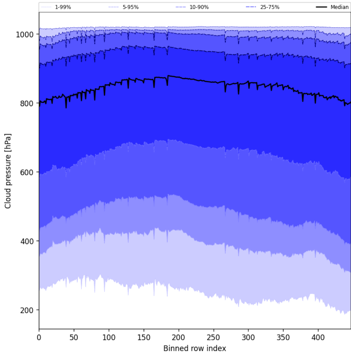
Figure 45: Along track statistics of “Cloud pressure” for 2025-09-11 to 2025-09-12
