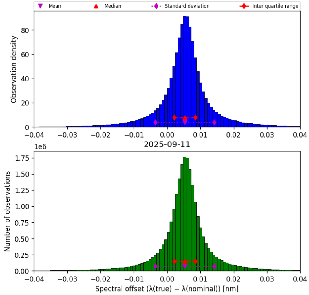
Figure 43: Histogram of “Spectral offset ( \lambda_{\text{true}} - \lambda_{\text{nominal}} )” for 2025-09-11 to 2025-09-12
