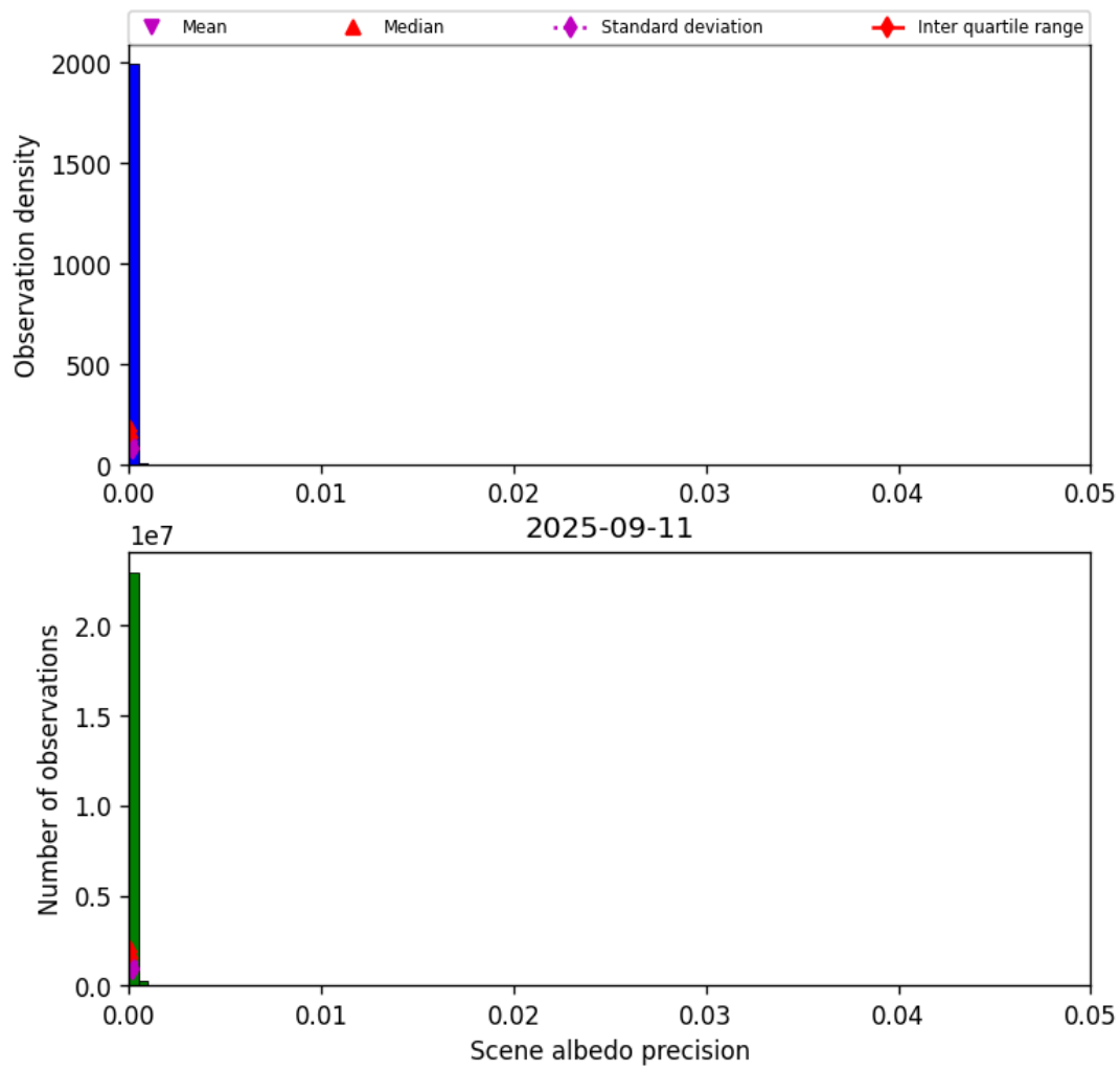
Figure 33: Histogram of “Scene albedo precision” for 2025-09-11 to 2025-09-12
