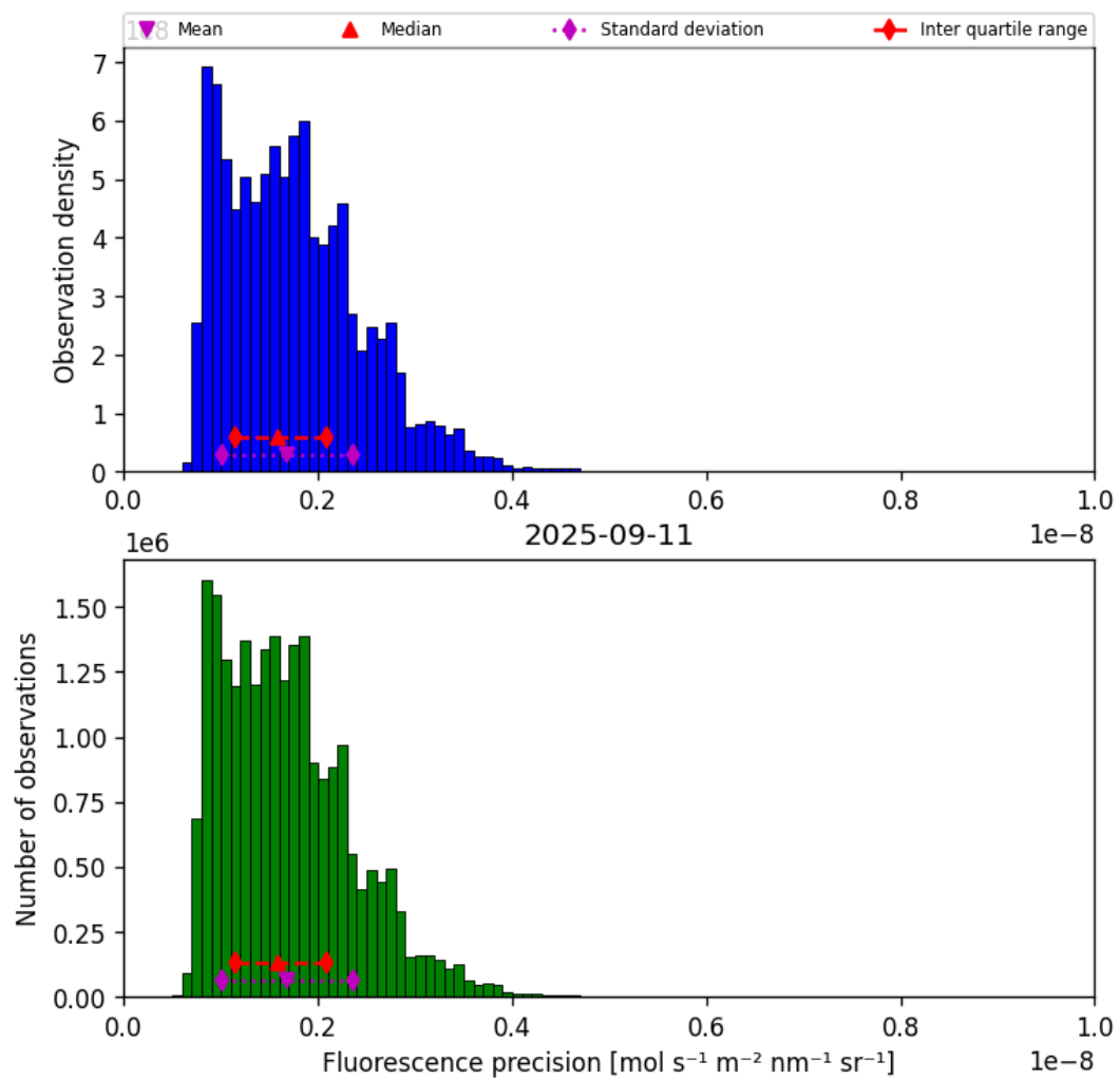
Figure 39: Histogram of “Fluorescence precision” for 2025-09-11 to 2025-09-12
