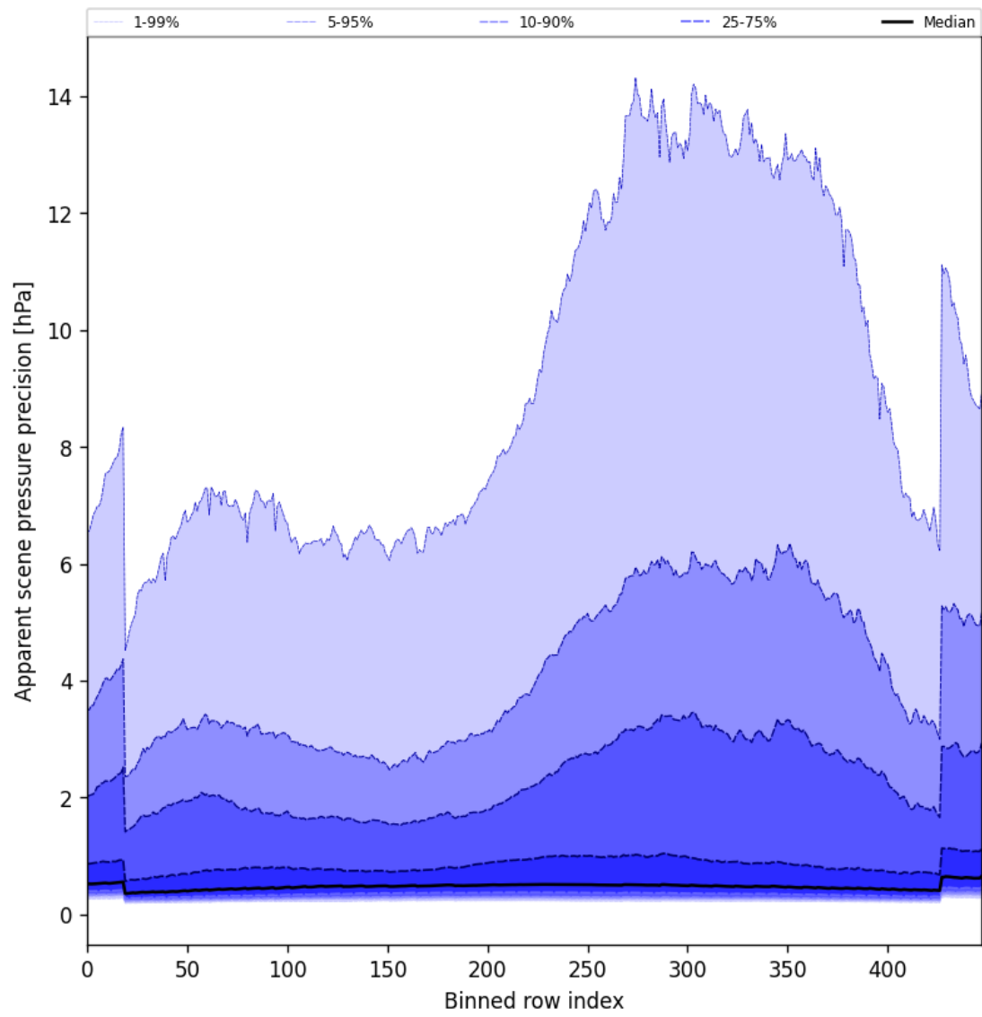
Figure 52: Along track statistics of “Apparent scene pressure precision” for 2025-09-11 to 2025-09-12
