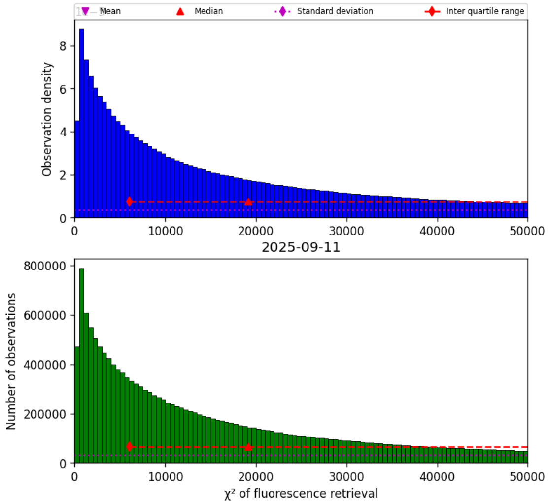
Figure 40: Histogram of “ \chi^2 of fluorescence retrieval” for 2025-09-11 to 2025-09-12
