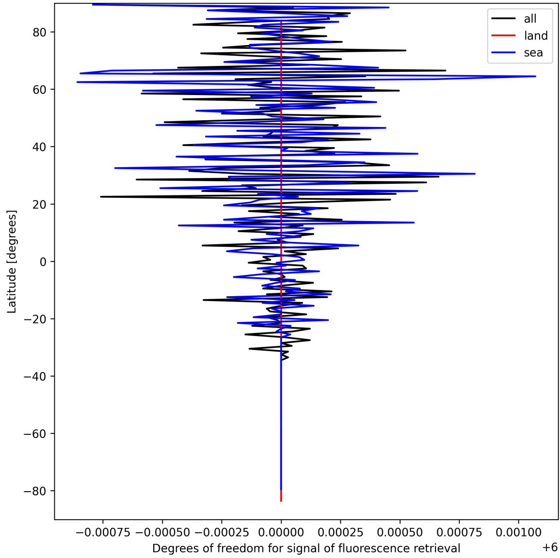
Figure 24: Zonal average of “Degrees of freedom for signal of fluorescence retrieval” for 2025-09-11 to 2025-09-12.
