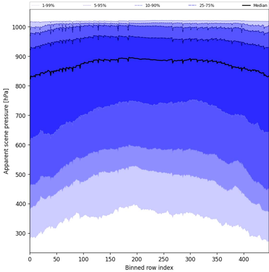
Figure 51: Along track statistics of “Apparent scene pressure” for 2025-09-11 to 2025-09-12
