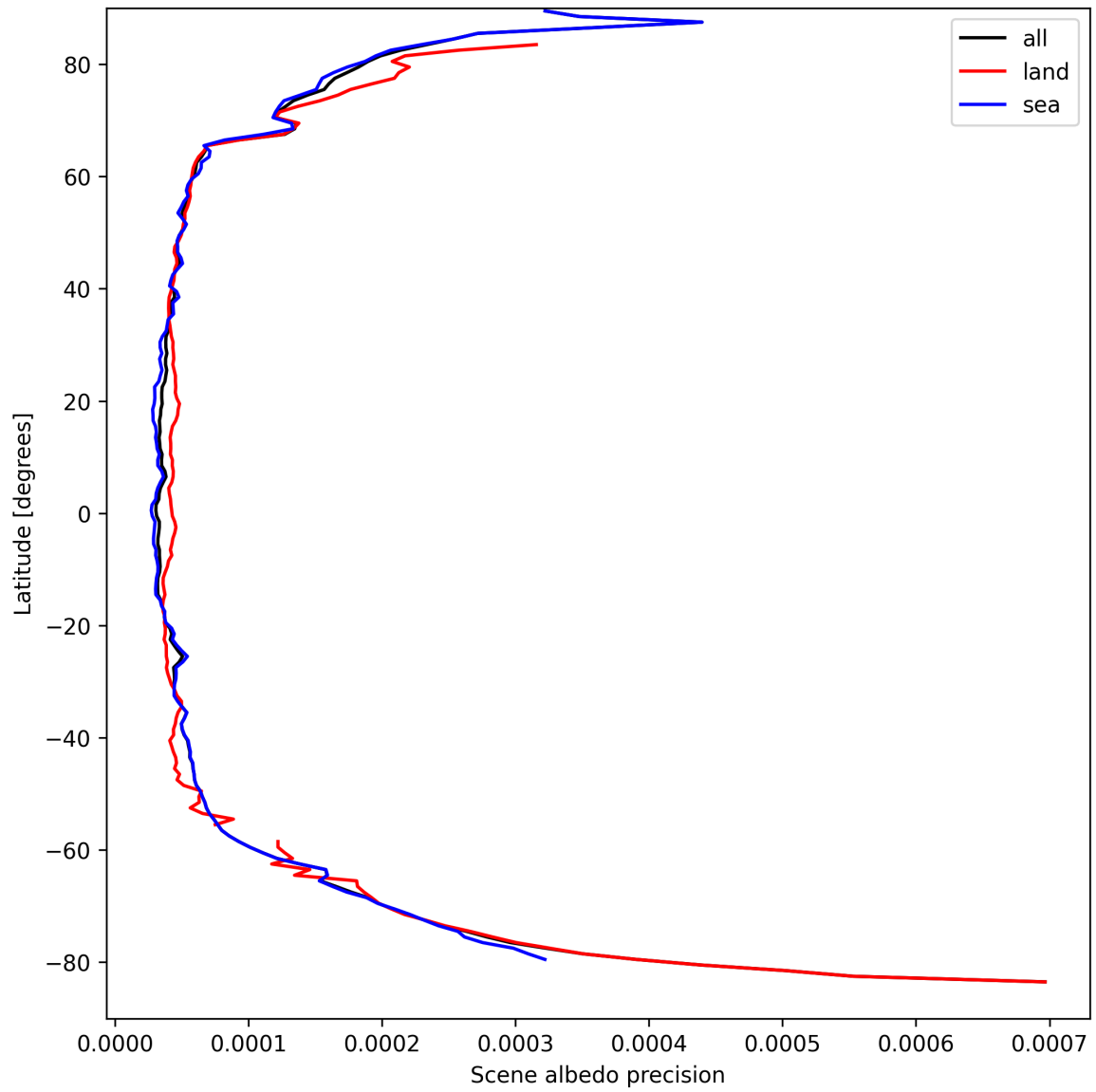
Figure 16: Zonal average of “Scene albedo precision” for 2025-09-11 to 2025-09-12.
