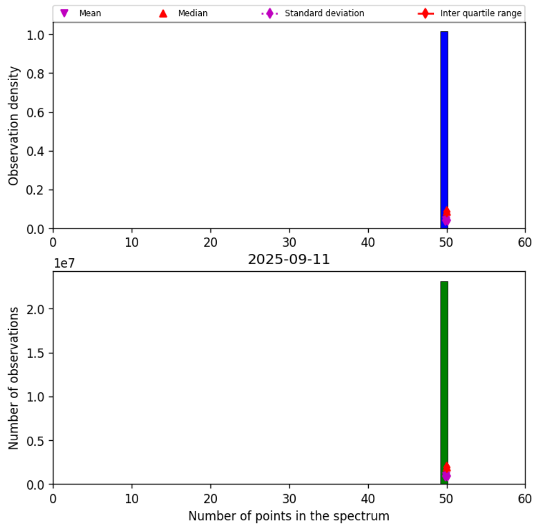
Figure 42: Histogram of “Number of points in the spectrum” for 2025-09-11 to 2025-09-12
