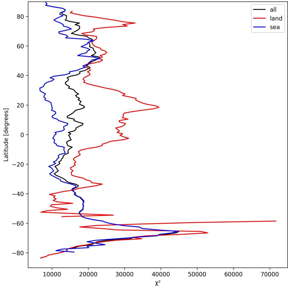
Figure 19: Zonal average of “ \chi^2 ” for 2025-09-11 to 2025-09-12.
