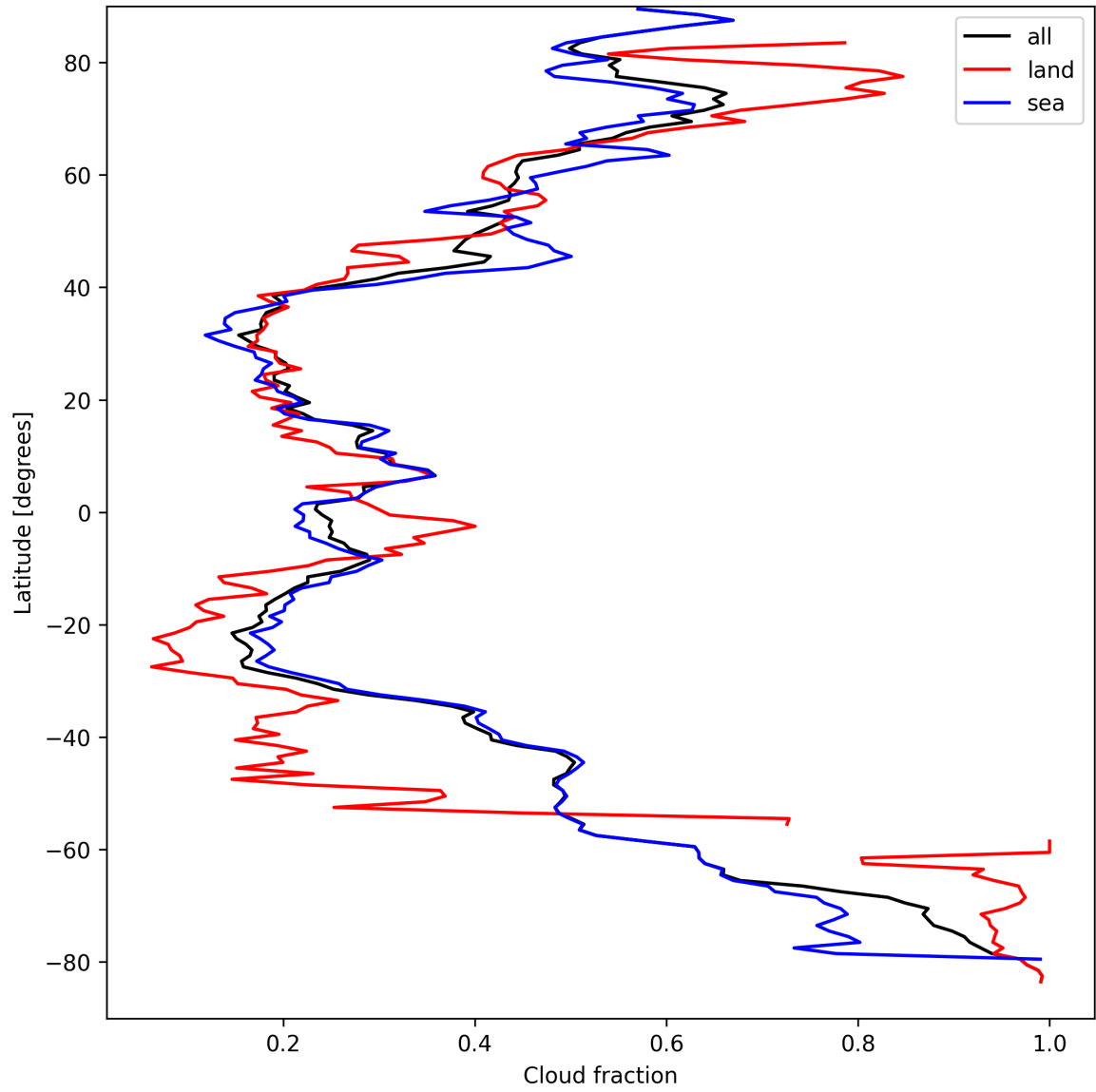
Figure 13: Zonal average of “Cloud fraction” for 2025-09-11 to 2025-09-12.
