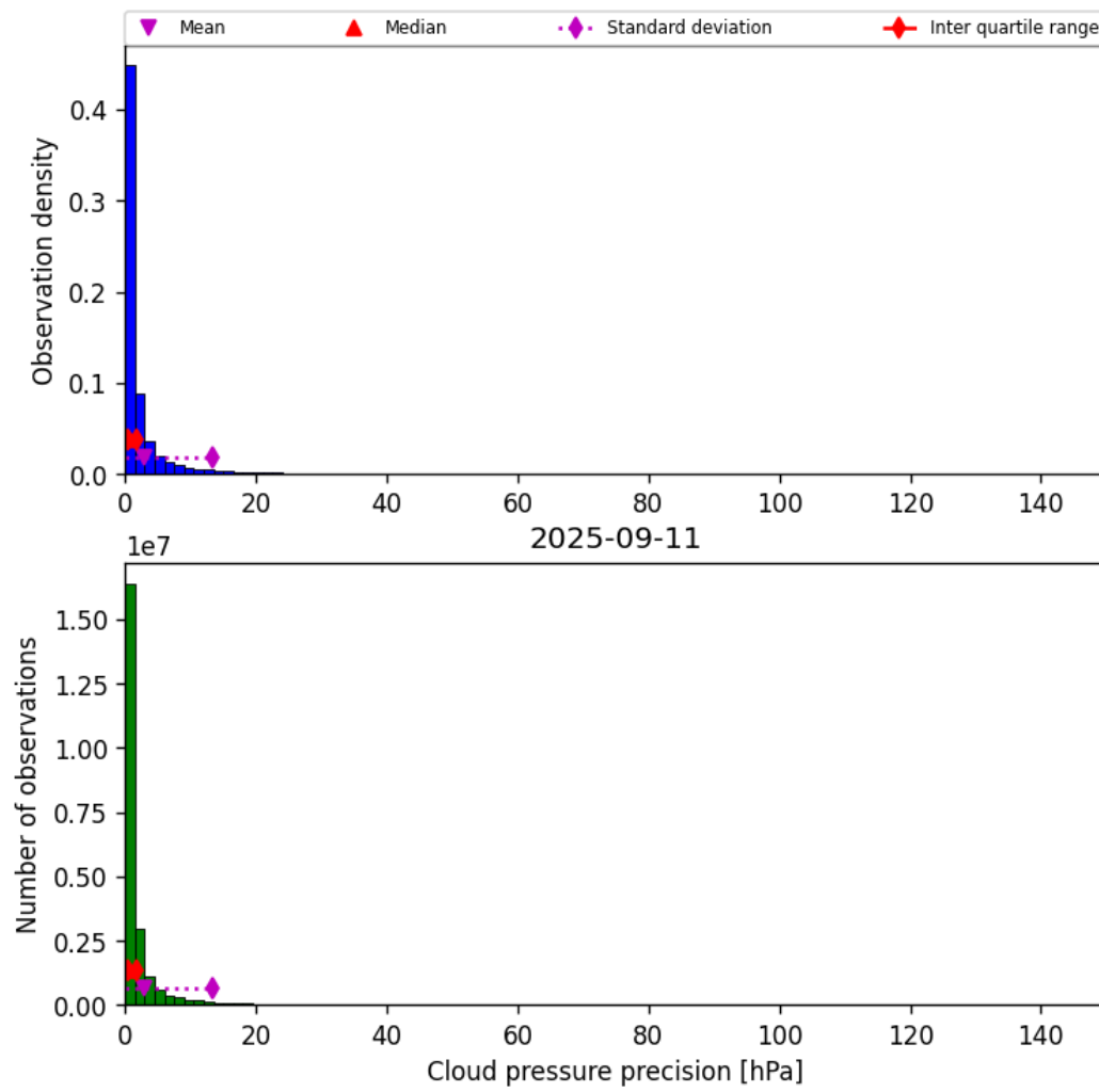
Figure 29: Histogram of “Cloud pressure precision” for 2025-09-11 to 2025-09-12
