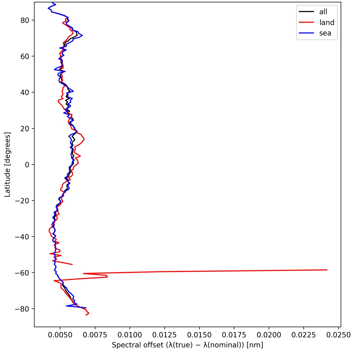
Figure 26: Zonal average of “Spectral offset ( \lambda_{\text{true}} - \lambda_{\text{nominal}} )” for 2025-09-11 to 2025-09-12.
