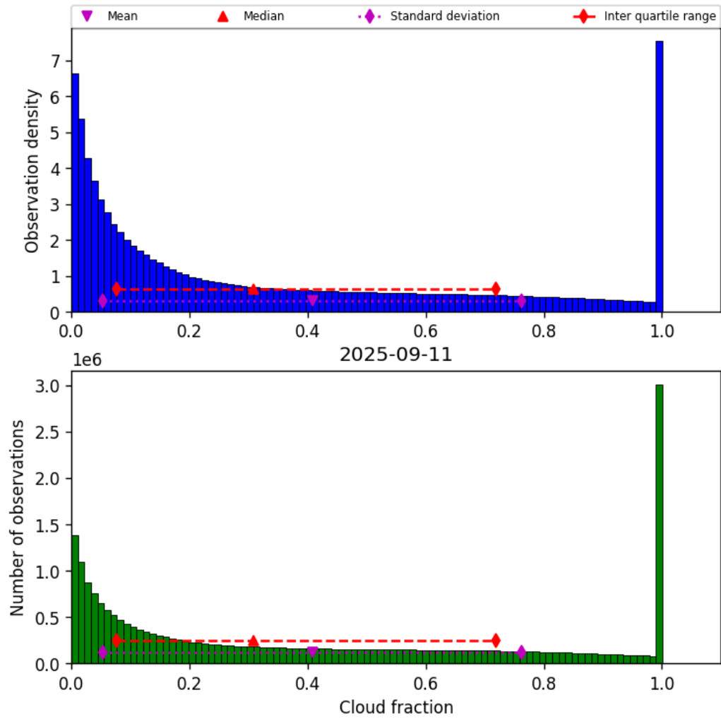
Figure 30: Histogram of “Cloud fraction” for 2025-09-11 to 2025-09-12
