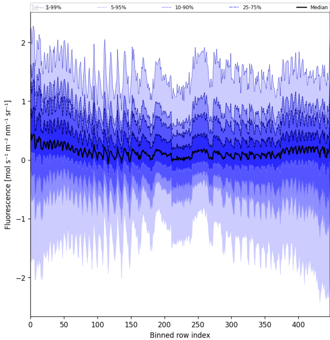
Figure 55: Along track statistics of “Fluorescence” for 2025-09-11 to 2025-09-12
