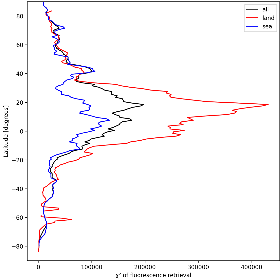
Figure 23: Zonal average of “ \chi^2 of fluorescence retrieval” for 2025-09-11 to 2025-09-12.
