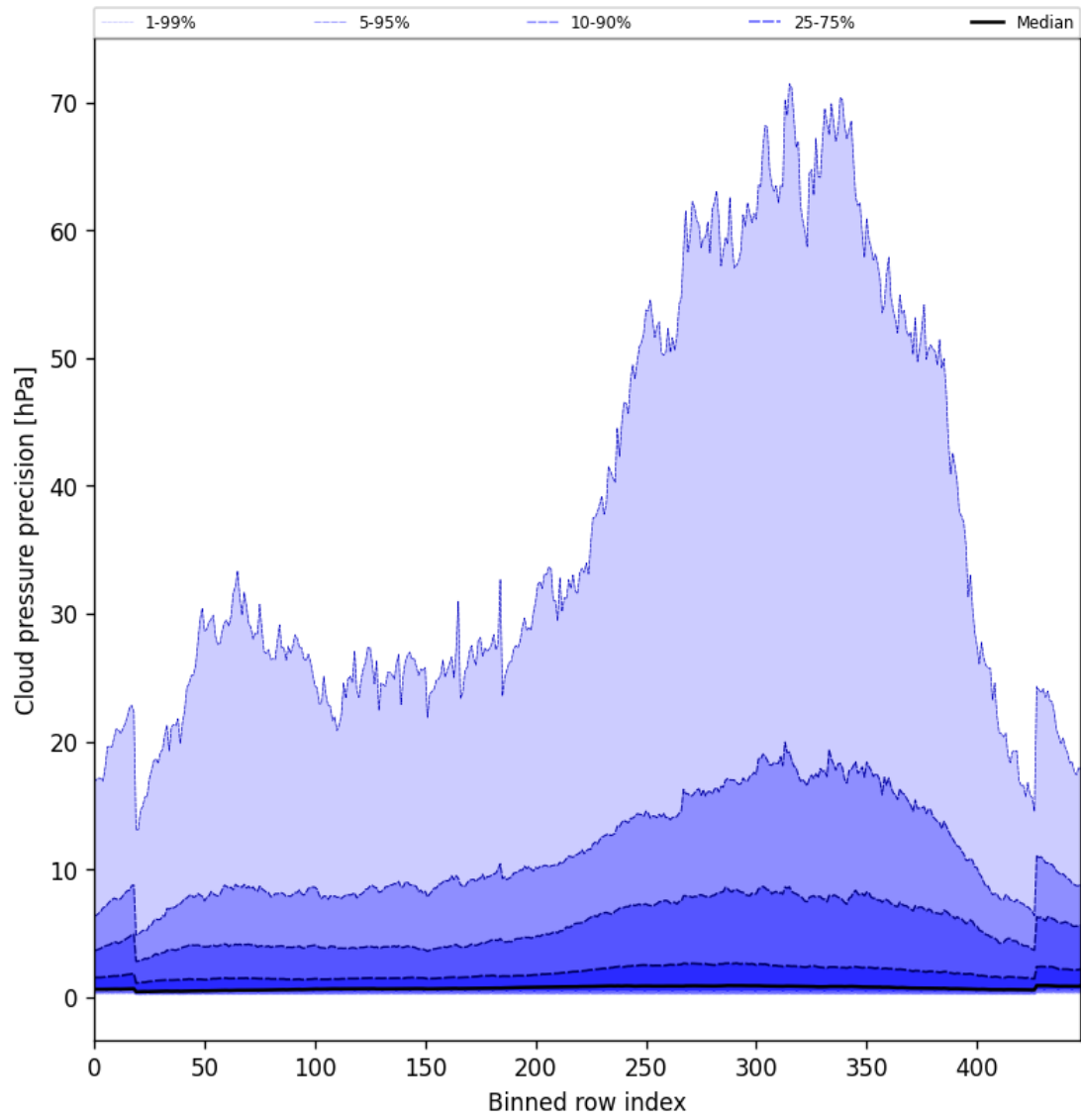
Figure 46: Along track statistics of “Cloud pressure precision” for 2025-09-11 to 2025-09-12
