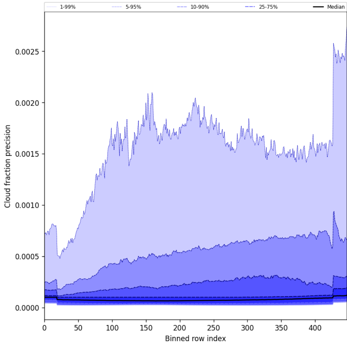
Figure 48: Along track statistics of “Cloud fraction precision” for 2025-09-11 to 2025-09-12
