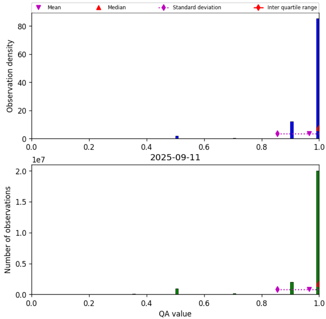
Figure 27: Histogram of “QA value” for 2025-09-11 to 2025-09-12
