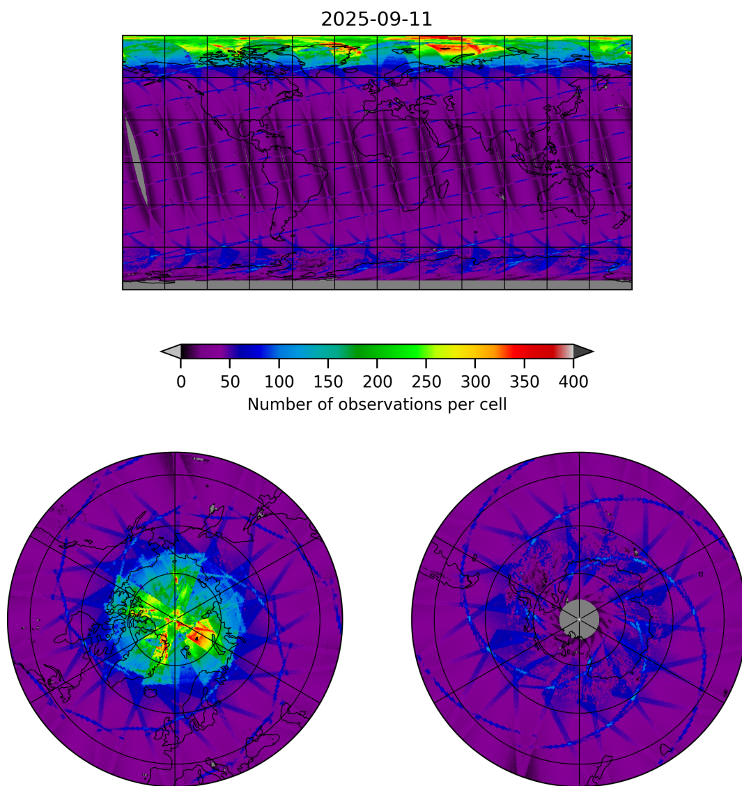
Figure 9: Map of the number of observations for 2025-09-11 to 2025-09-12
