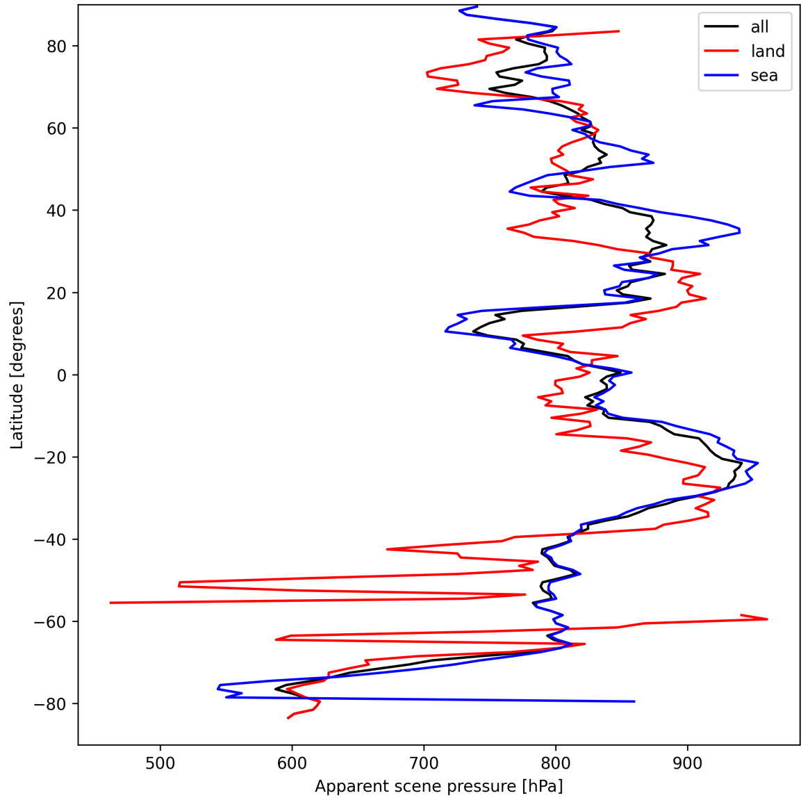
Figure 17: Zonal average of “Apparent scene pressure” for 2025-09-11 to 2025-09-12.
