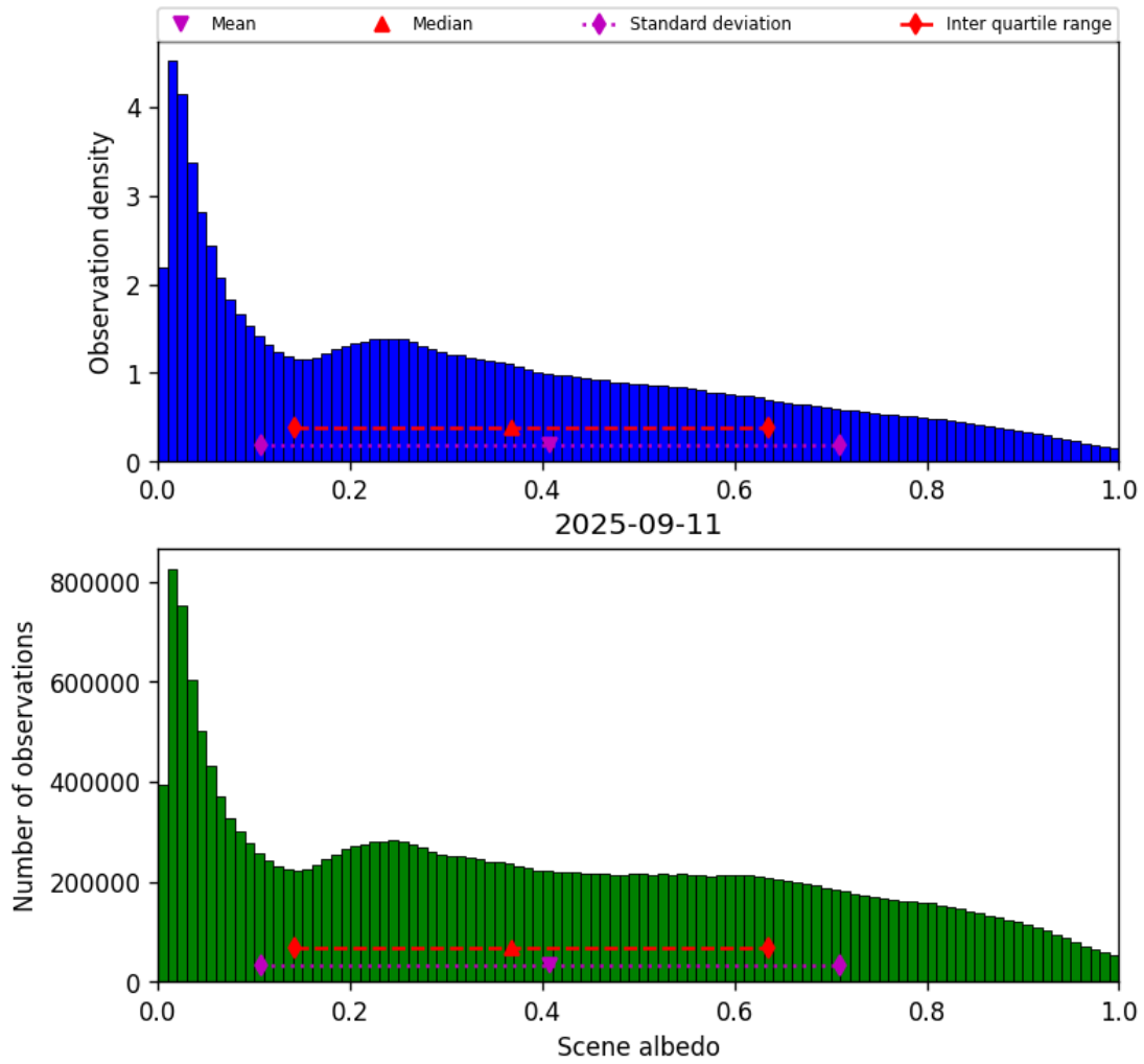
Figure 32: Histogram of “Scene albedo” for 2025-09-11 to 2025-09-12
