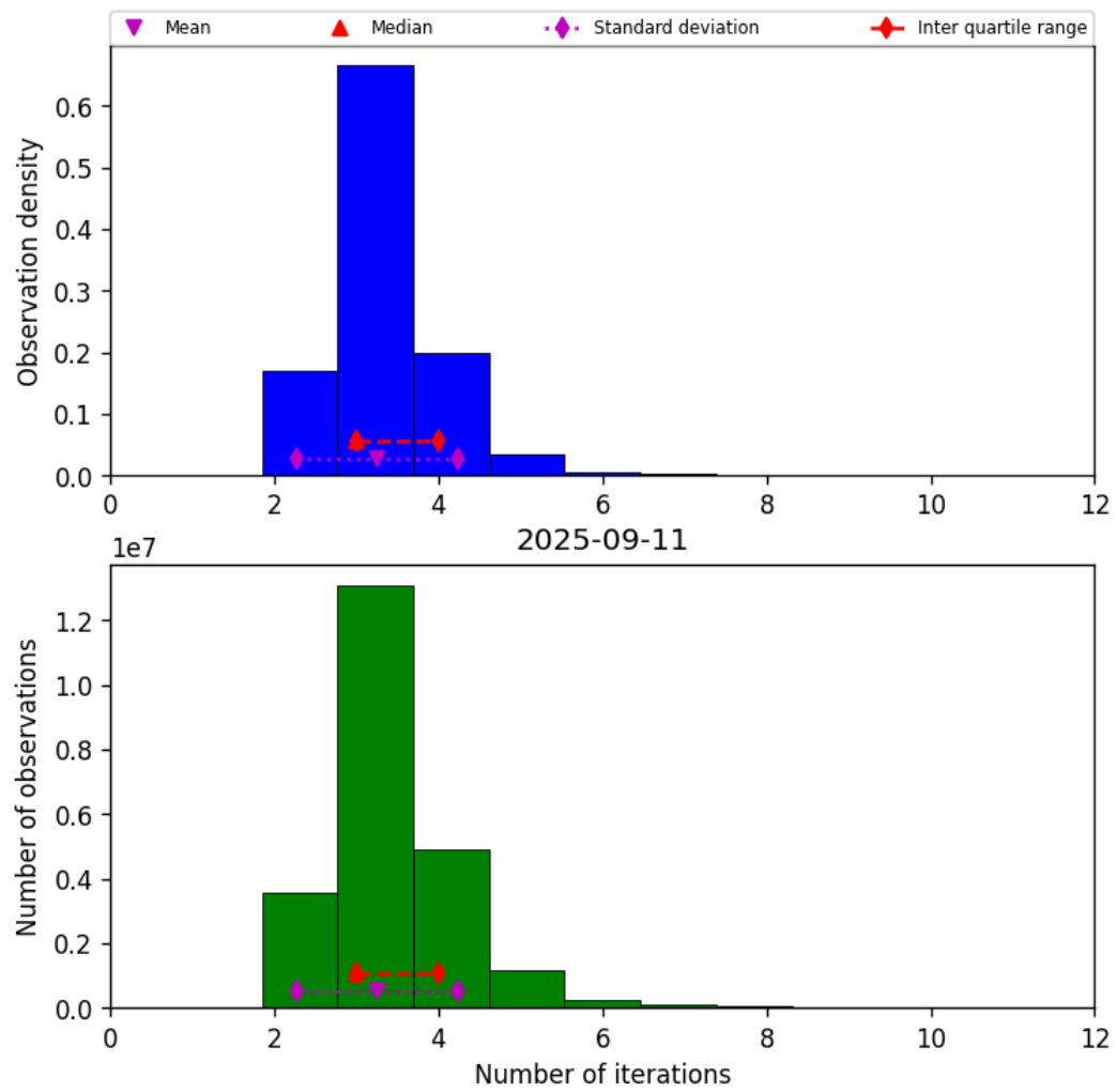
Figure 37: Histogram of “Number of iterations” for 2025-09-11 to 2025-09-12
