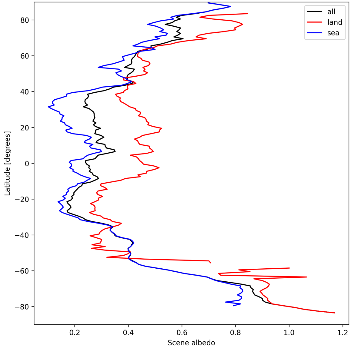
Figure 15: Zonal average of “Scene albedo” for 2025-09-11 to 2025-09-12.
