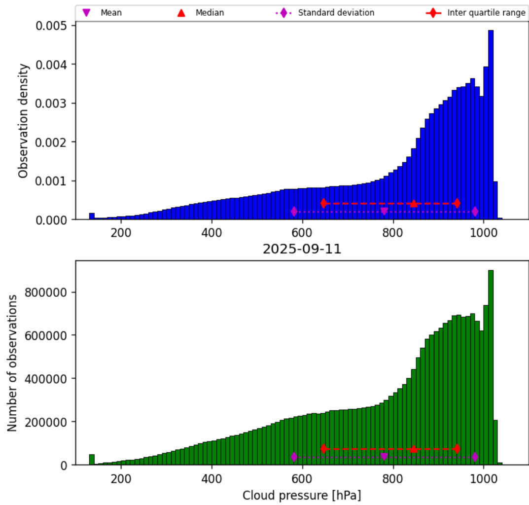
Figure 28: Histogram of “Cloud pressure” for 2025-09-11 to 2025-09-12
