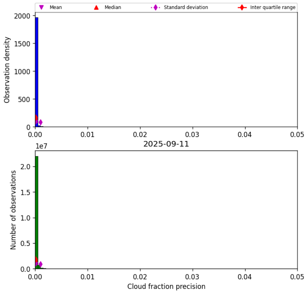
Figure 31: Histogram of “Cloud fraction precision” for 2025-09-11 to 2025-09-12
