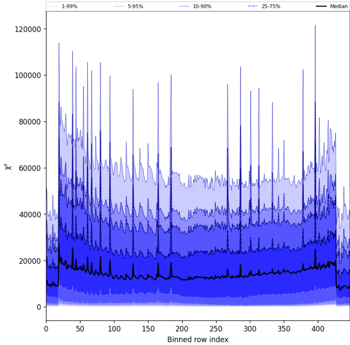
Figure 53: Along track statistics of “ \chi^2 ” for 2025-09-11 to 2025-09-12
