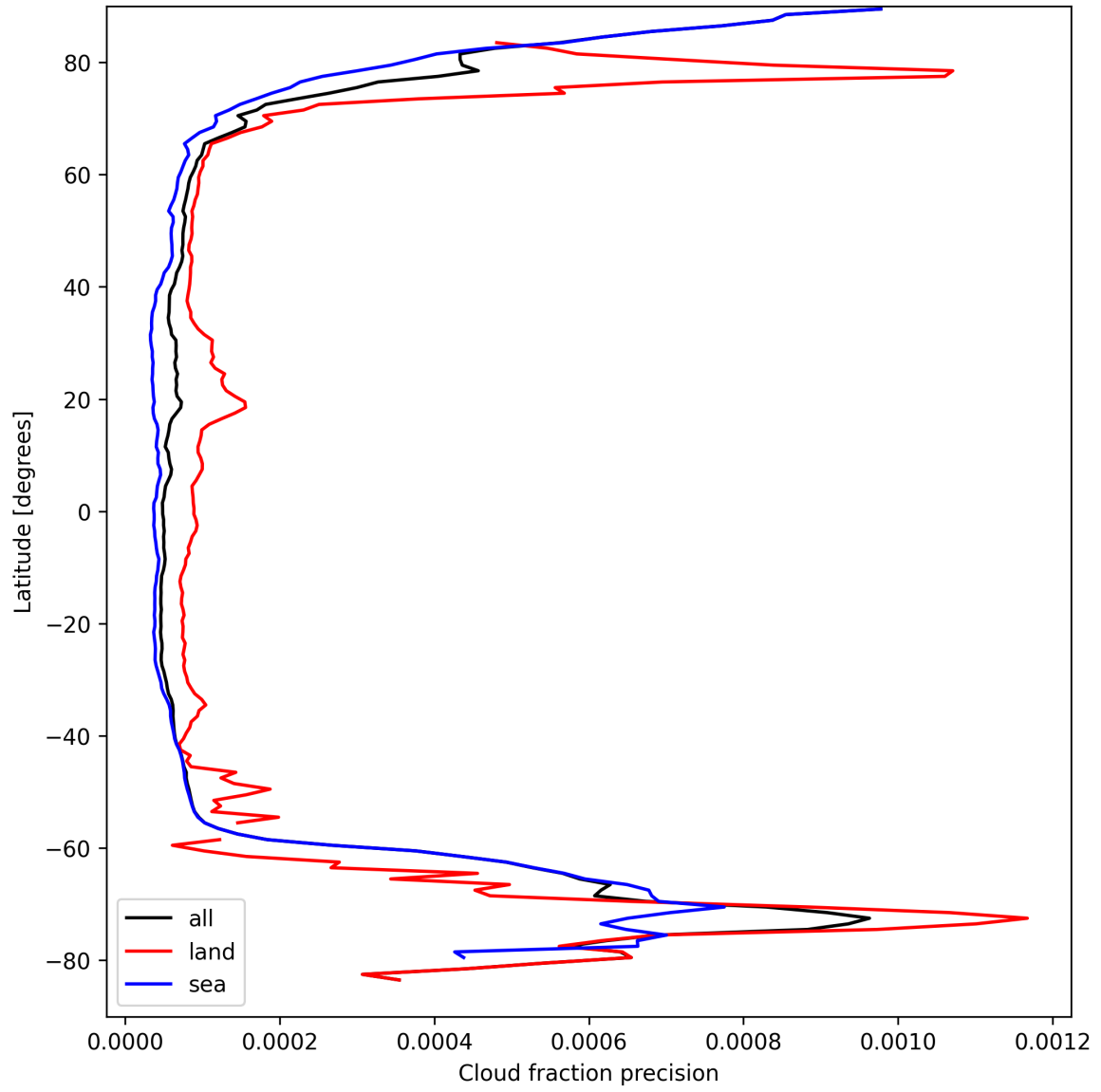
Figure 14: Zonal average of “Cloud fraction precision” for 2025-09-11 to 2025-09-12.
