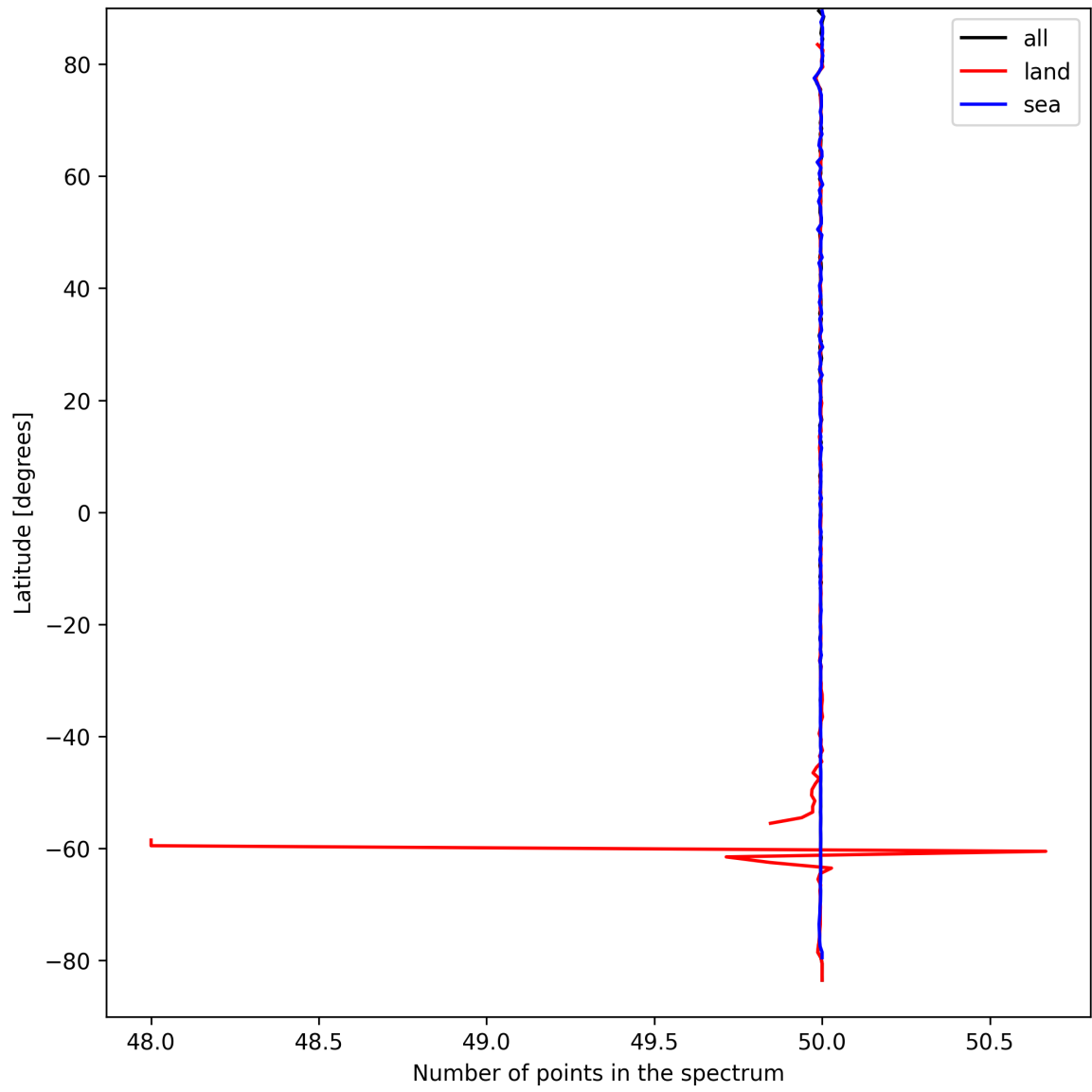
Figure 25: Zonal average of “Number of points in the spectrum” for 2025-09-11 to 2025-09-12.
