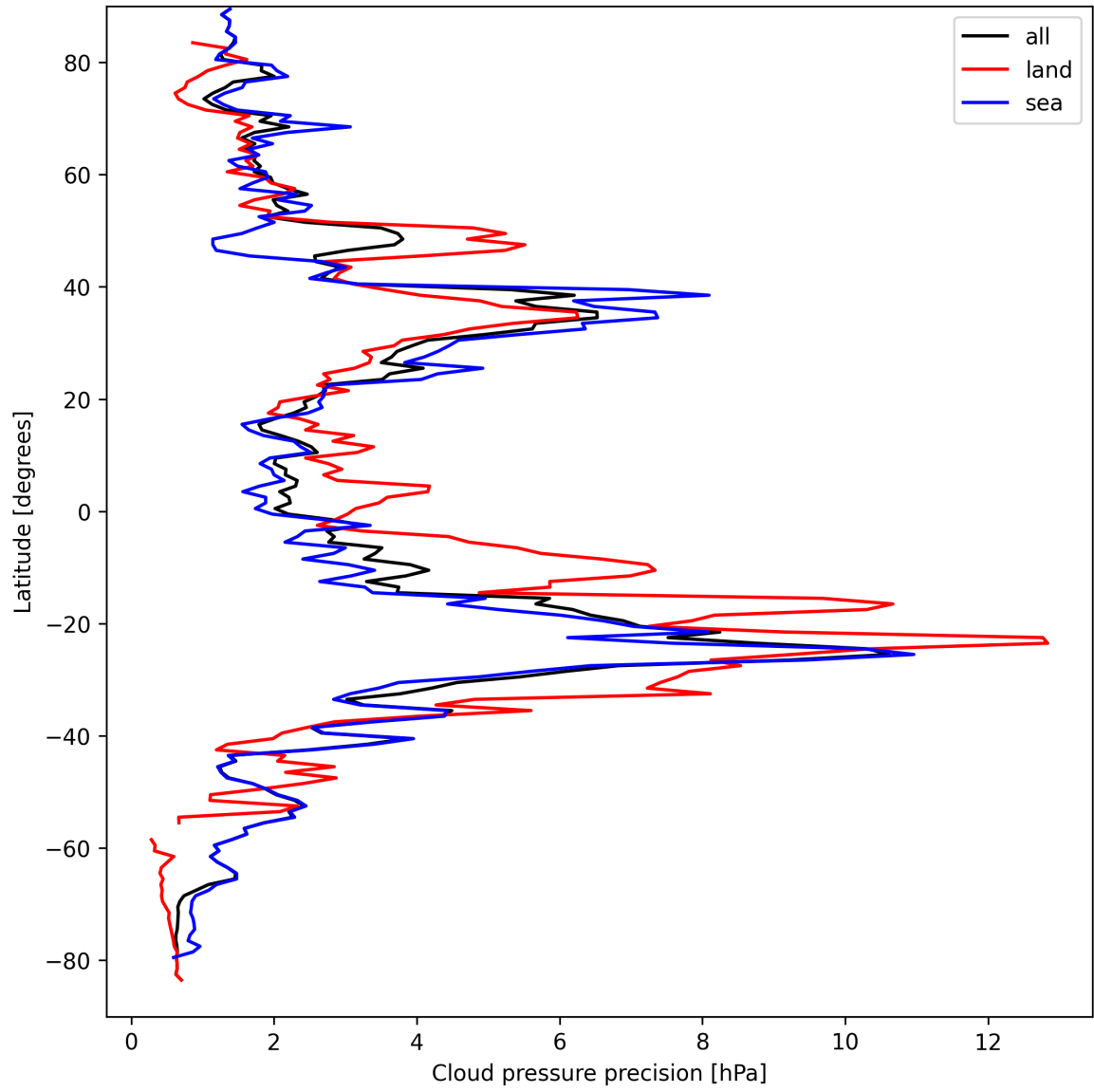
Figure 12: Zonal average of “Cloud pressure precision” for 2025-09-11 to 2025-09-12.
