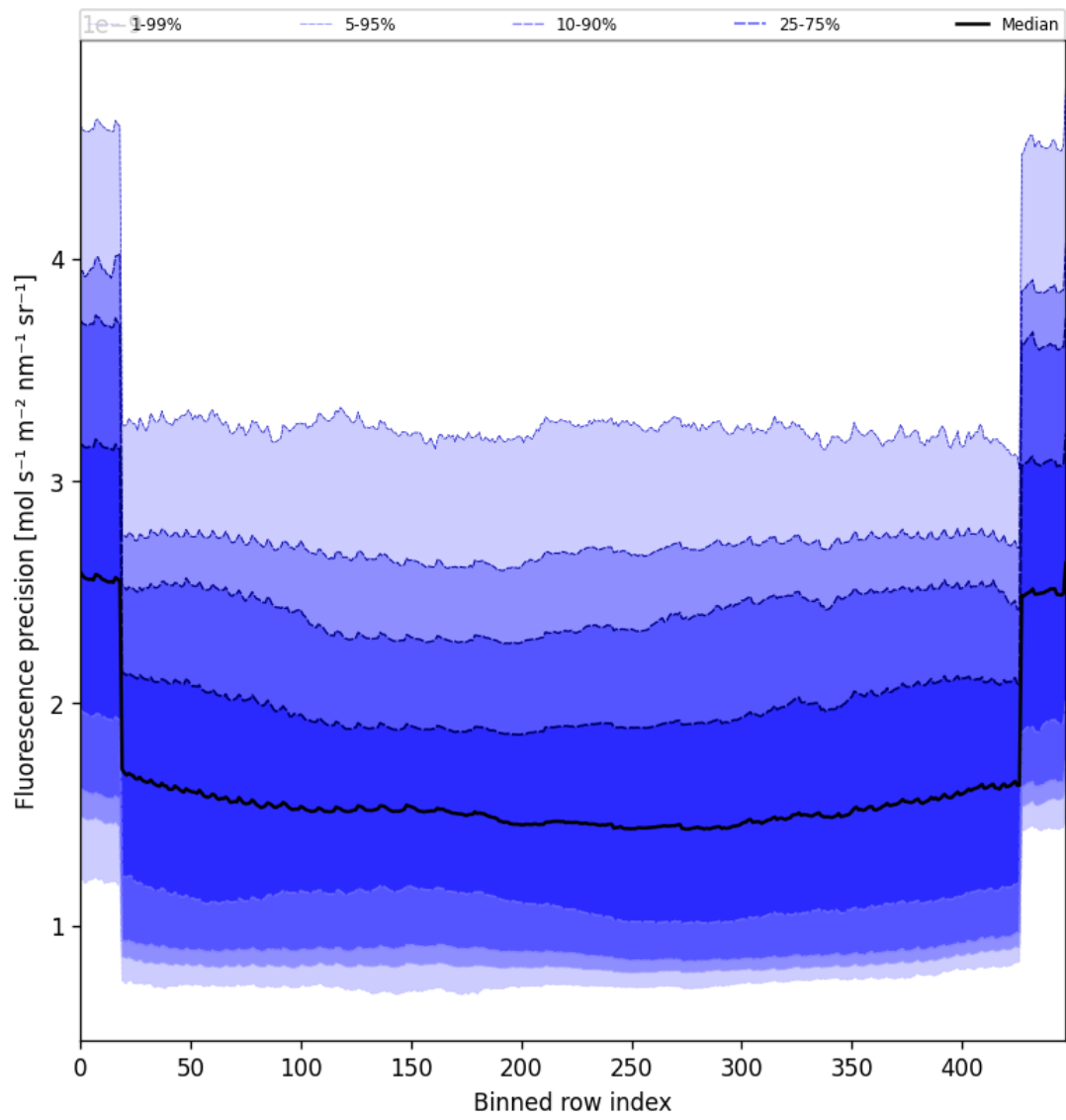
Figure 56: Along track statistics of “Fluorescence precision” for 2025-09-11 to 2025-09-12
