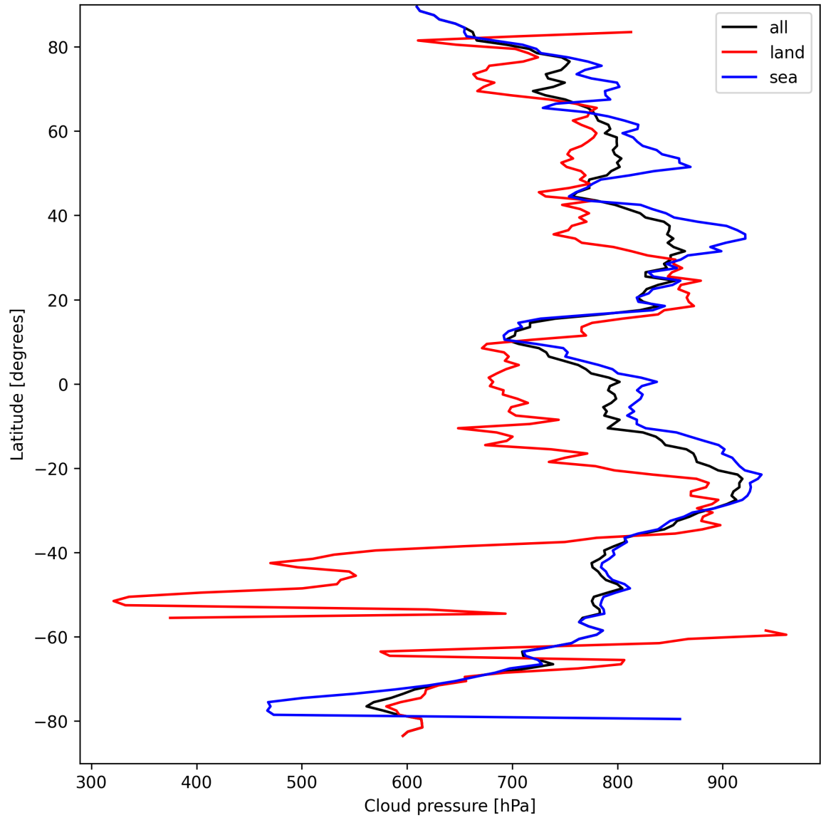
Figure 11: Zonal average of “Cloud pressure” for 2025-09-11 to 2025-09-12.
