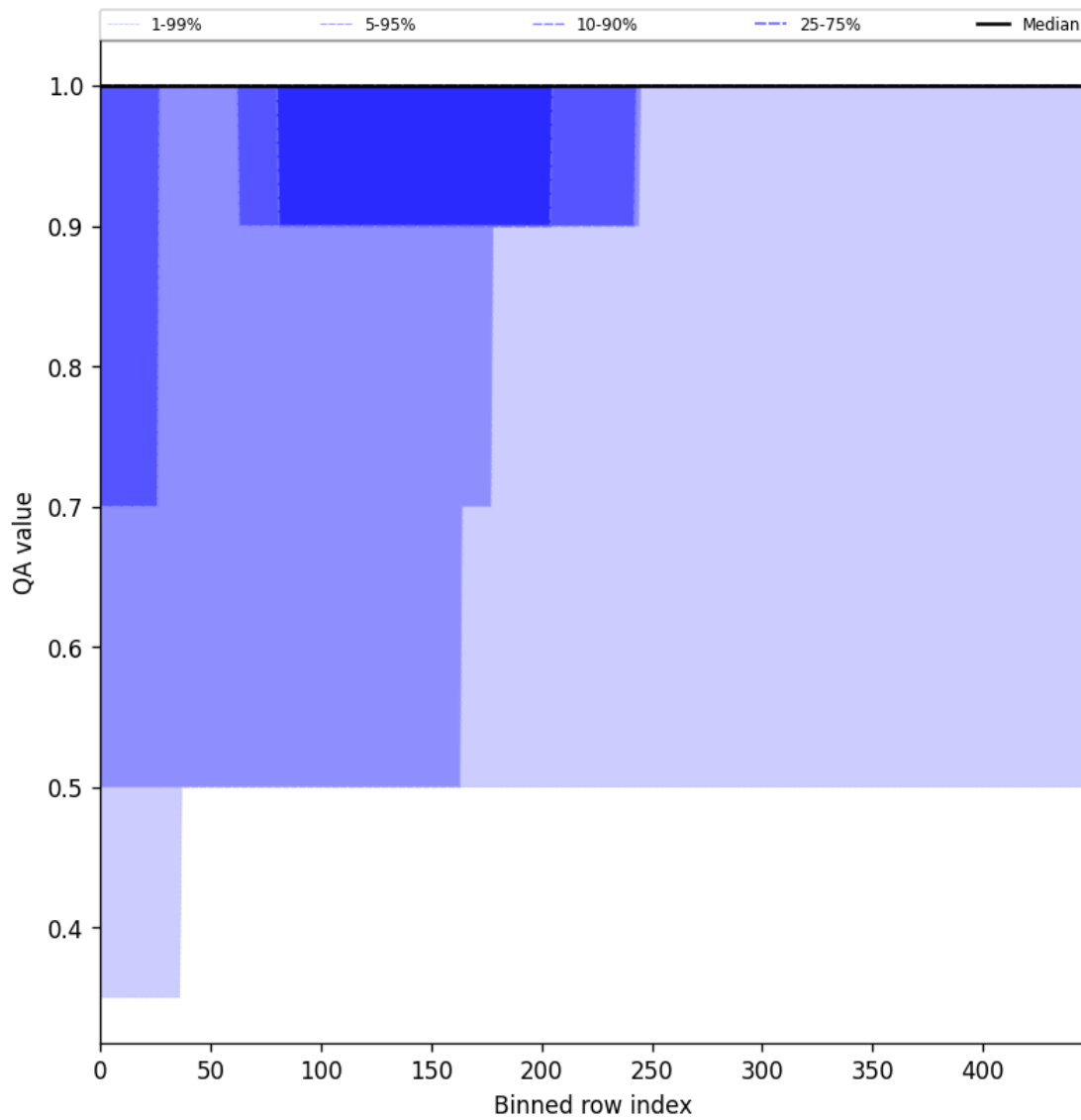
Figure 44: Along track statistics of “QA value” for 2025-09-11 to 2025-09-12
