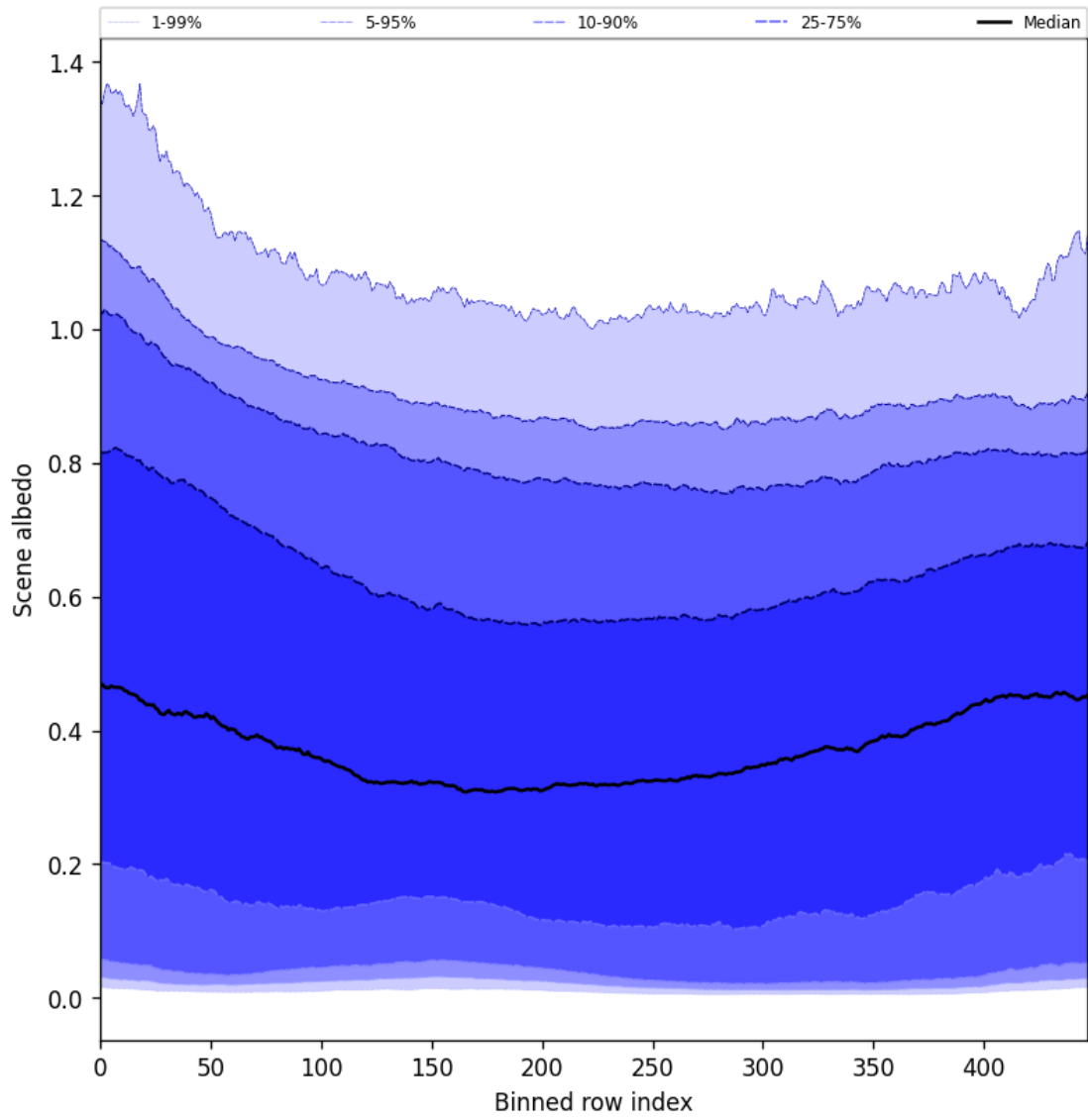
Figure 49: Along track statistics of “Scene albedo” for 2025-09-11 to 2025-09-12
