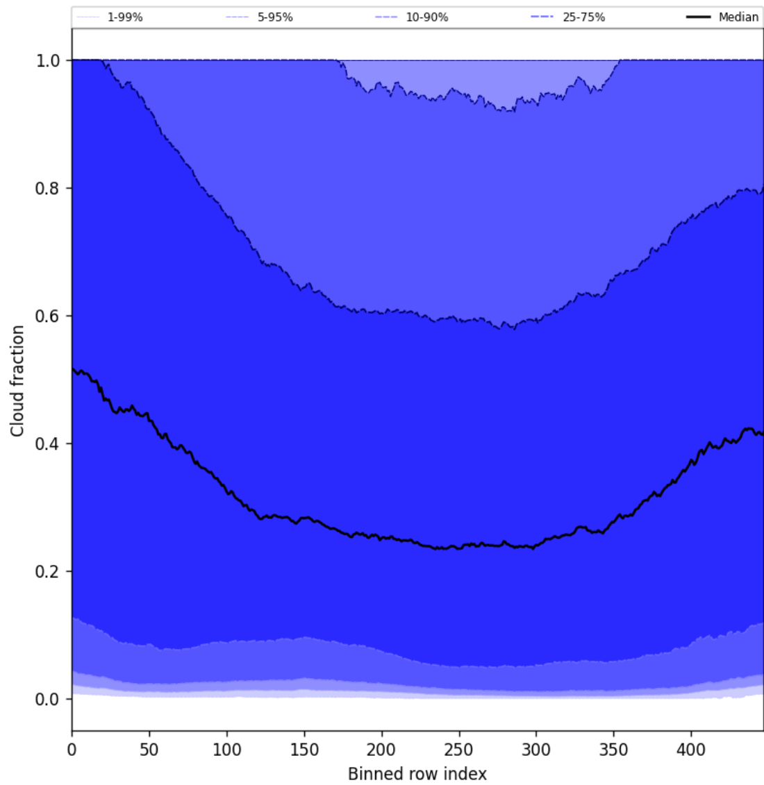
Figure 47: Along track statistics of “Cloud fraction” for 2025-09-11 to 2025-09-12
