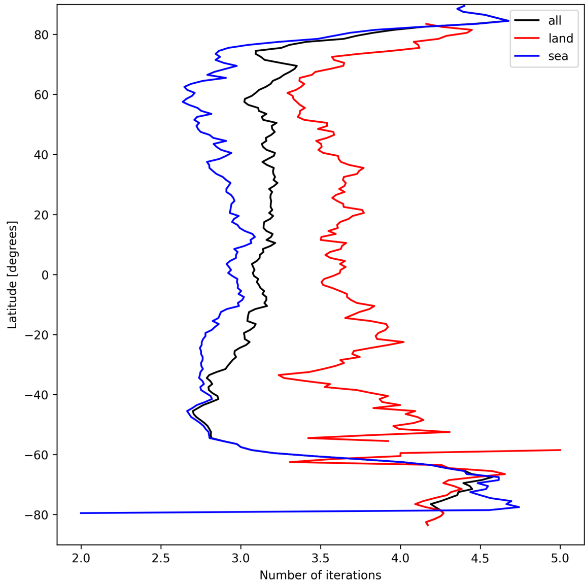
Figure 20: Zonal average of “Number of iterations” for 2025-09-11 to 2025-09-12.
