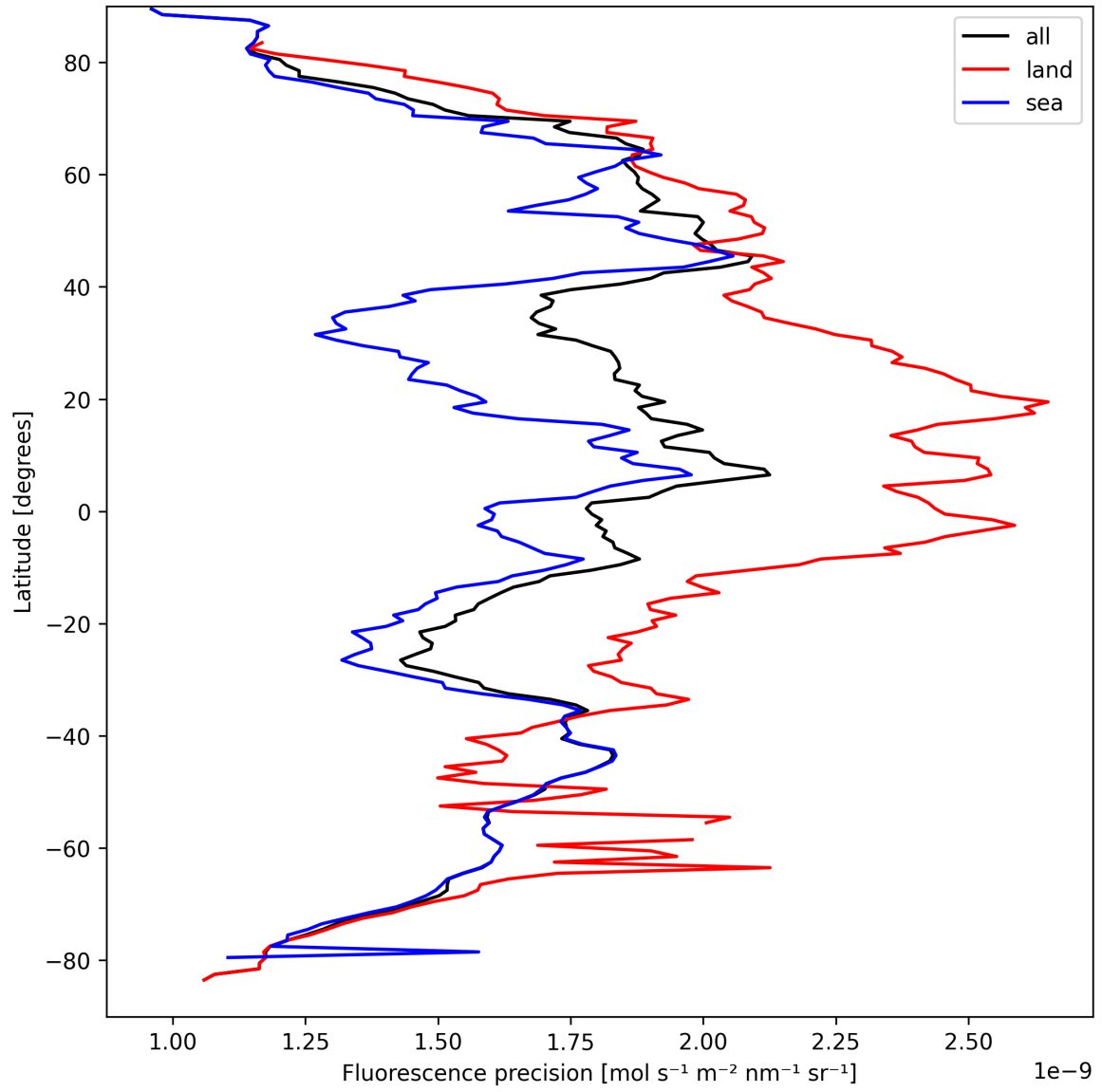
Figure 22: Zonal average of “Fluorescence precision” for 2025-09-11 to 2025-09-12.
