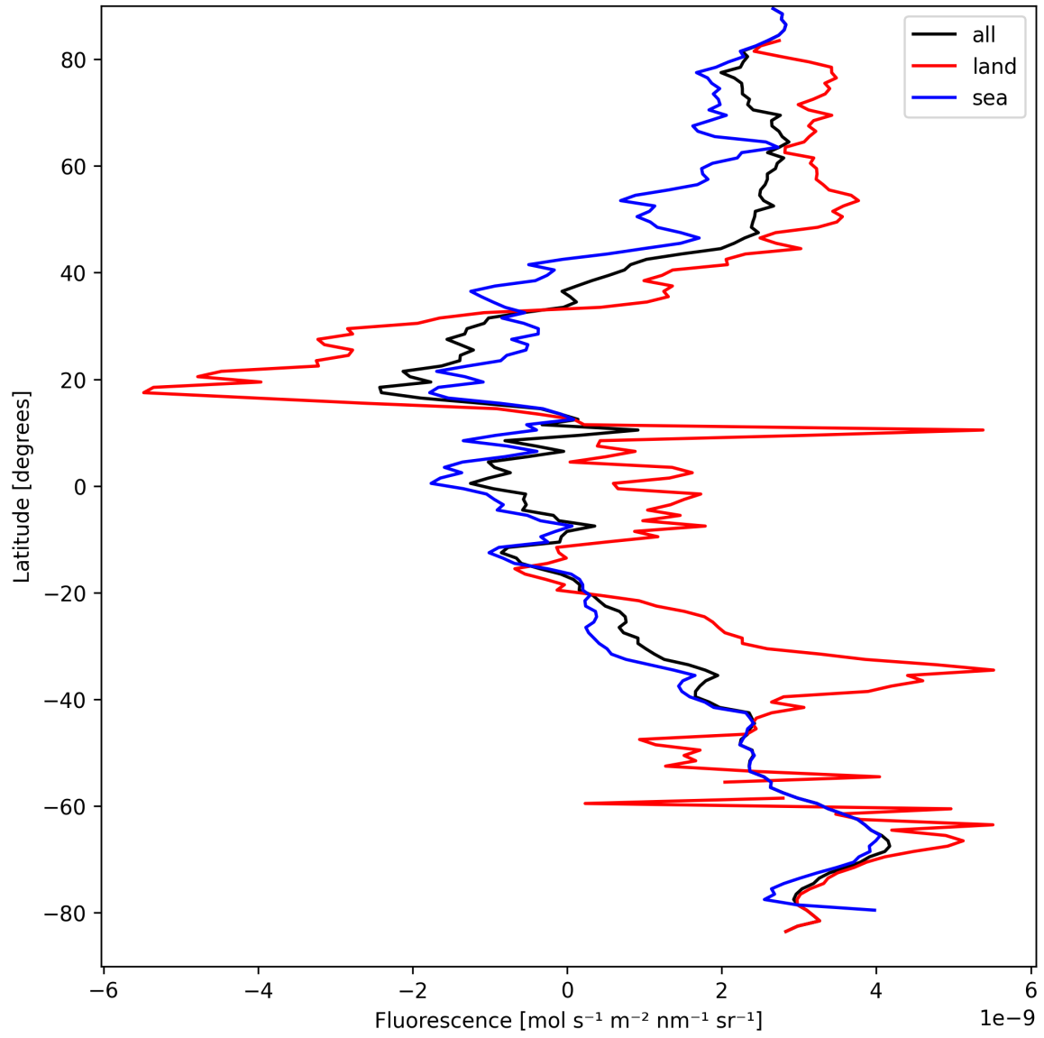
Figure 21: Zonal average of “Fluorescence” for 2025-09-11 to 2025-09-12.
