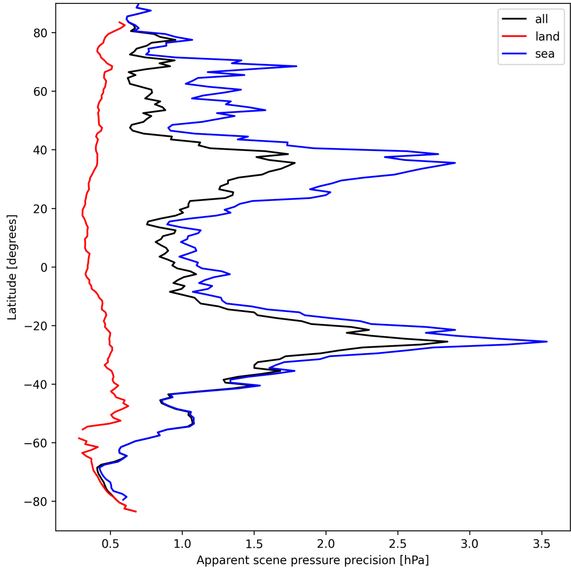
Figure 18: Zonal average of “Apparent scene pressure precision” for 2025-09-11 to 2025-09-12.
