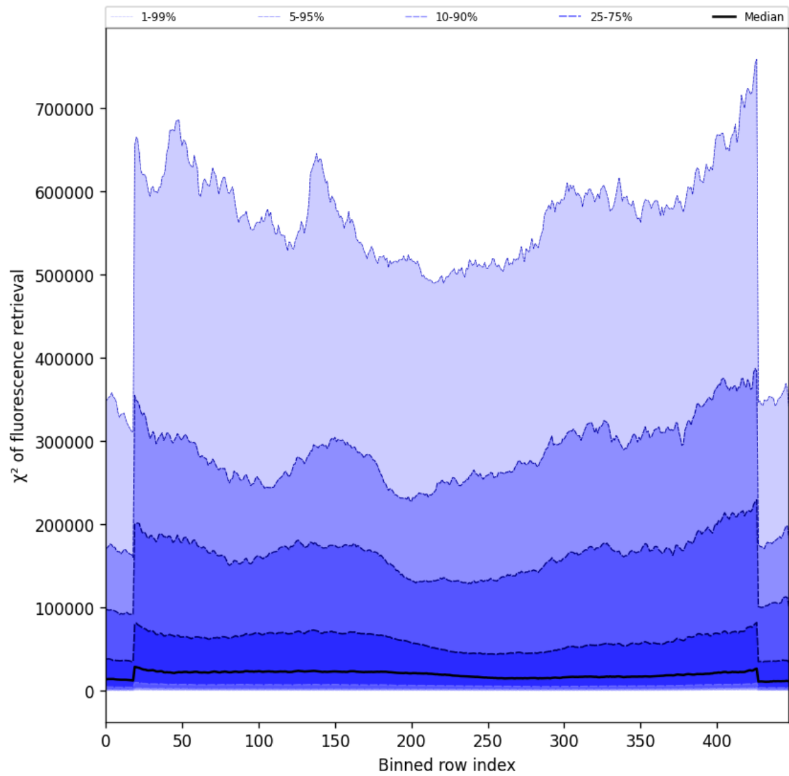
Figure 57: Along track statistics of “ \chi^2 of fluorescence retrieval” for 2025-09-11 to 2025-09-12
