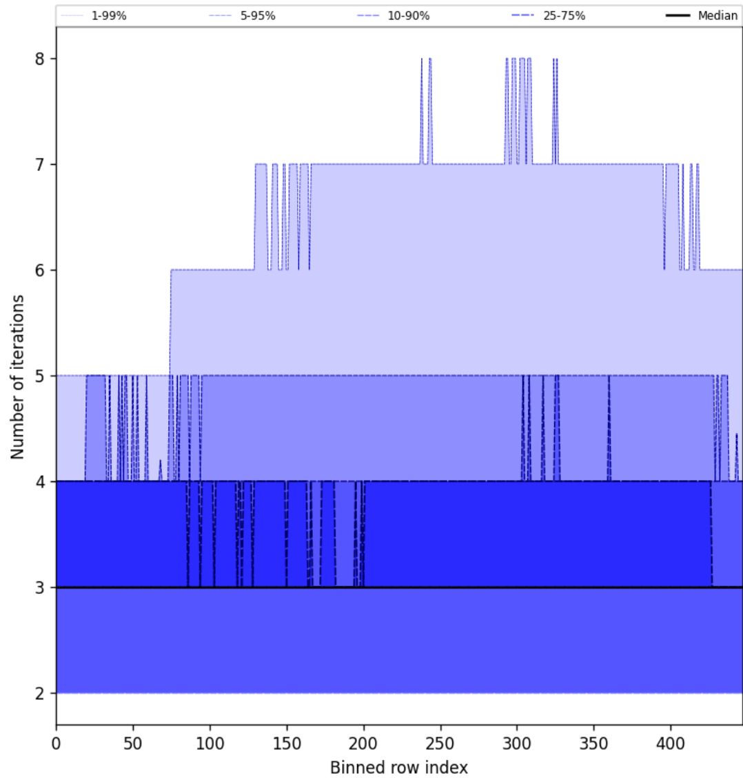
Figure 54: Along track statistics of “Number of iterations” for 2025-09-11 to 2025-09-12
