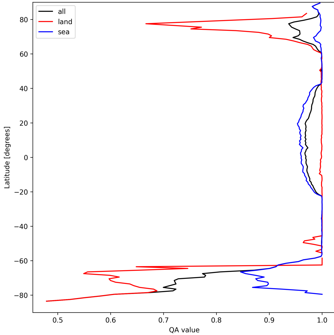
Figure 10: Zonal average of “QA value” for 2025-09-11 to 2025-09-12.
