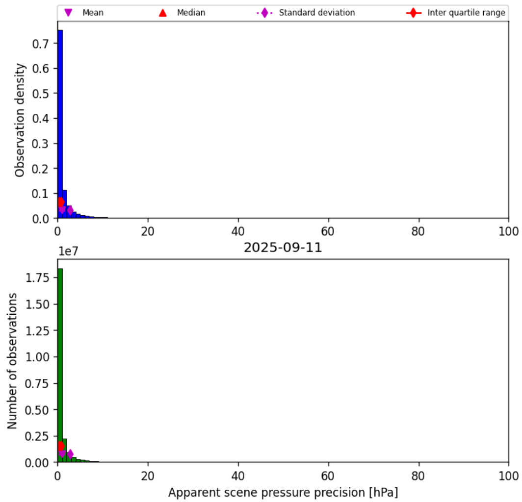
Figure 35: Histogram of “Apparent scene pressure precision” for 2025-09-11 to 2025-09-12
