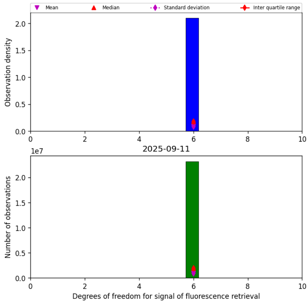
Figure 41: Histogram of “Degrees of freedom for signal of fluorescence retrieval” for 2025-09-11 to 2025-09-12
