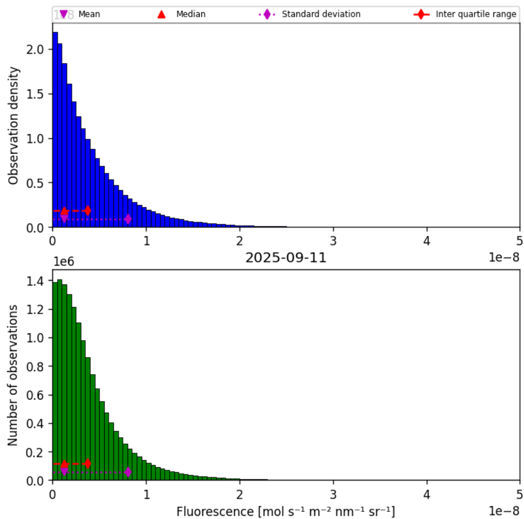
Figure 38: Histogram of “Fluorescence” for 2025-09-11 to 2025-09-12
