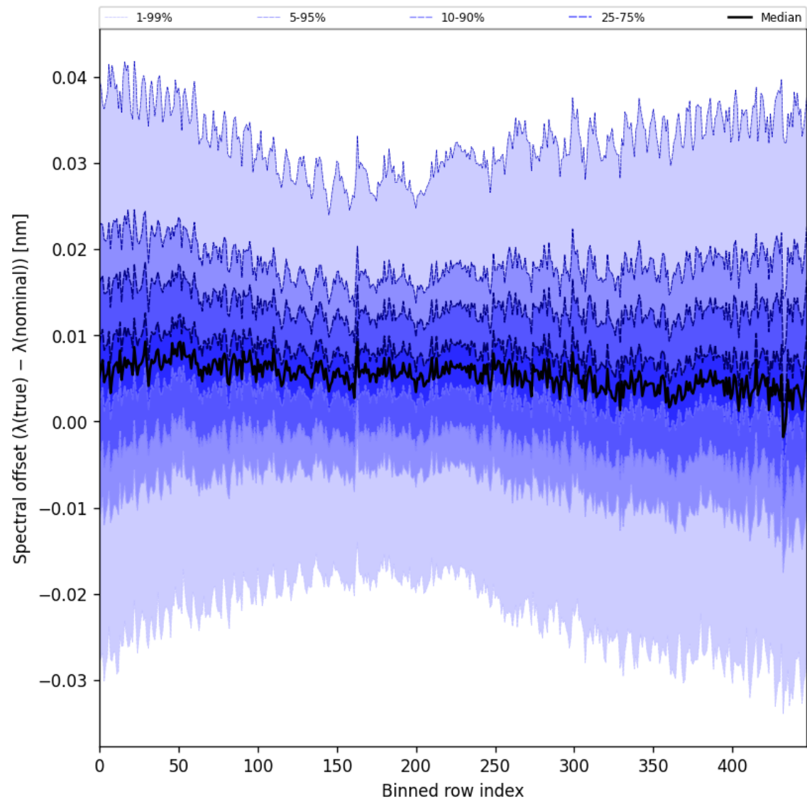
Figure 60: Along track statistics of “Spectral offset ( \lambda_{\text{true}} - \lambda_{\text{nominal}} )” for 2025-09-11 to 2025-09-12
