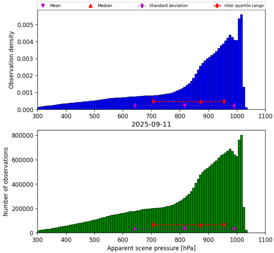
Figure 34: Histogram of “Apparent scene pressure” for 2025-09-11 to 2025-09-12
