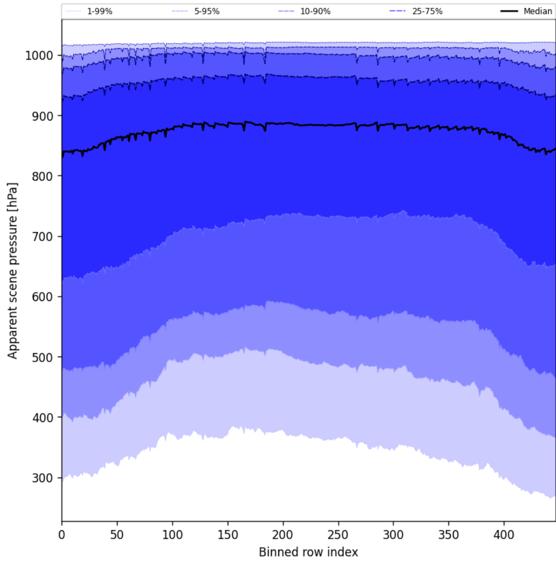
Figure 51: Along track statistics of “Apparent scene pressure” for 2025-09-12 to 2025-09-13
