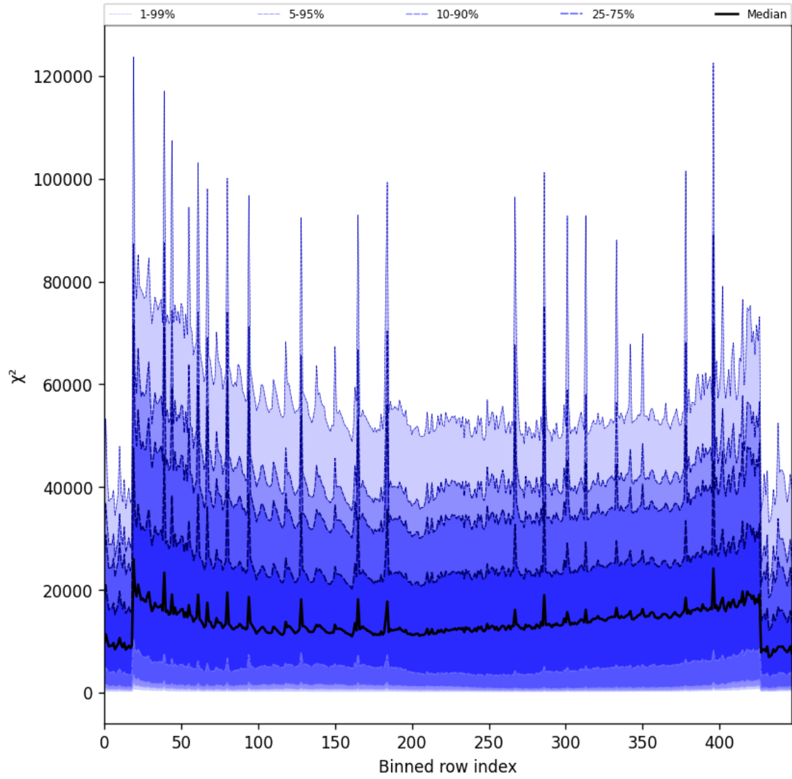
Figure 53: Along track statistics of “ \chi^2 ” for 2025-09-12 to 2025-09-13
