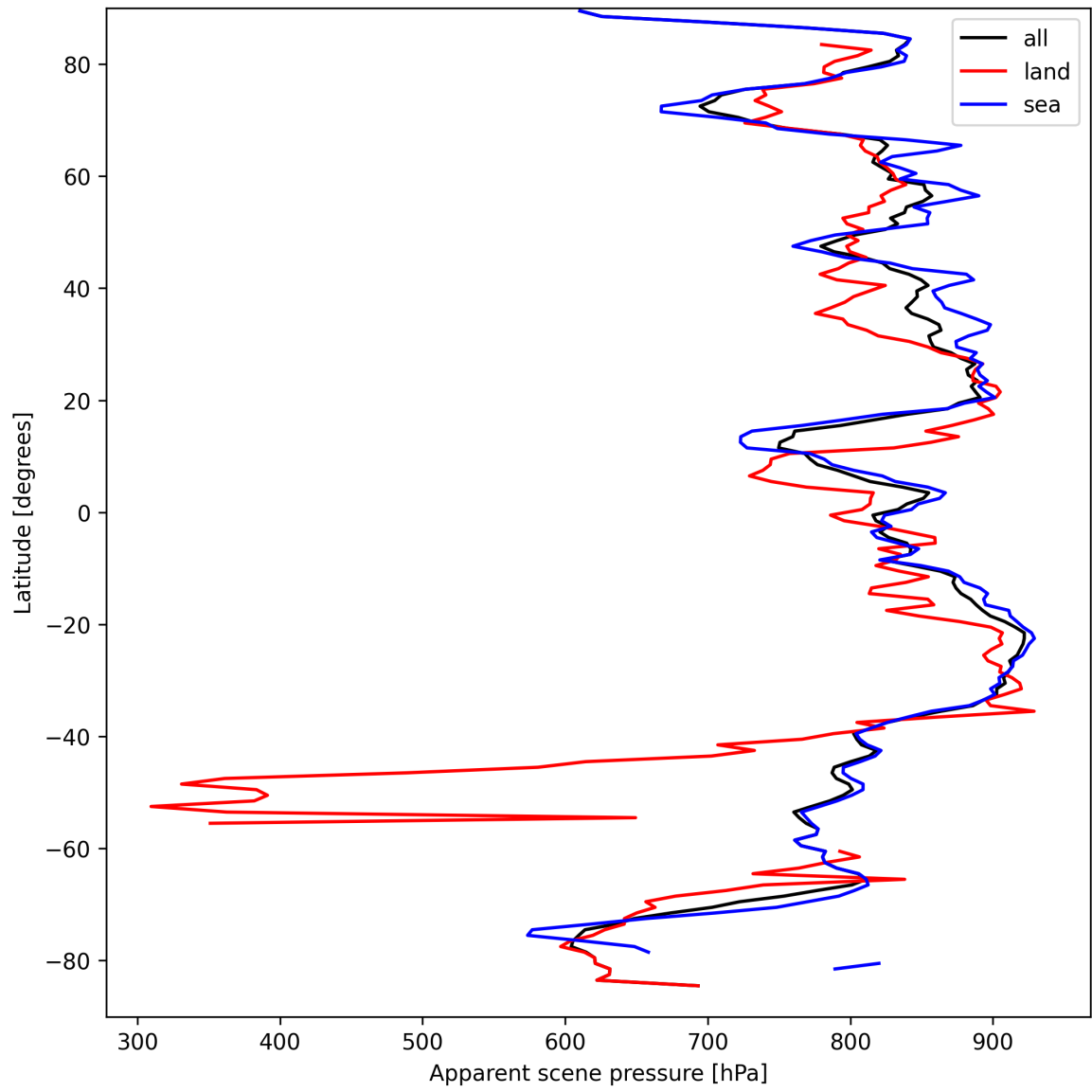
Figure 17: Zonal average of “Apparent scene pressure” for 2025-09-12 to 2025-09-13.
