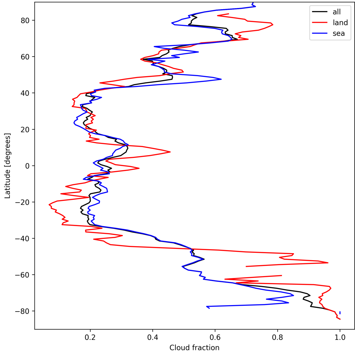
Figure 13: Zonal average of “Cloud fraction” for 2025-09-12 to 2025-09-13.
