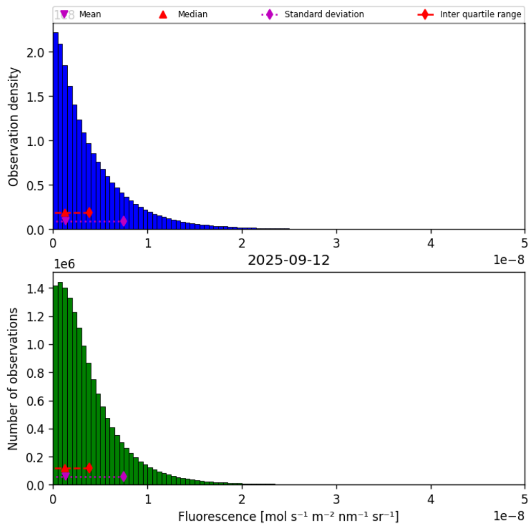
Figure 38: Histogram of “Fluorescence” for 2025-09-12 to 2025-09-13
