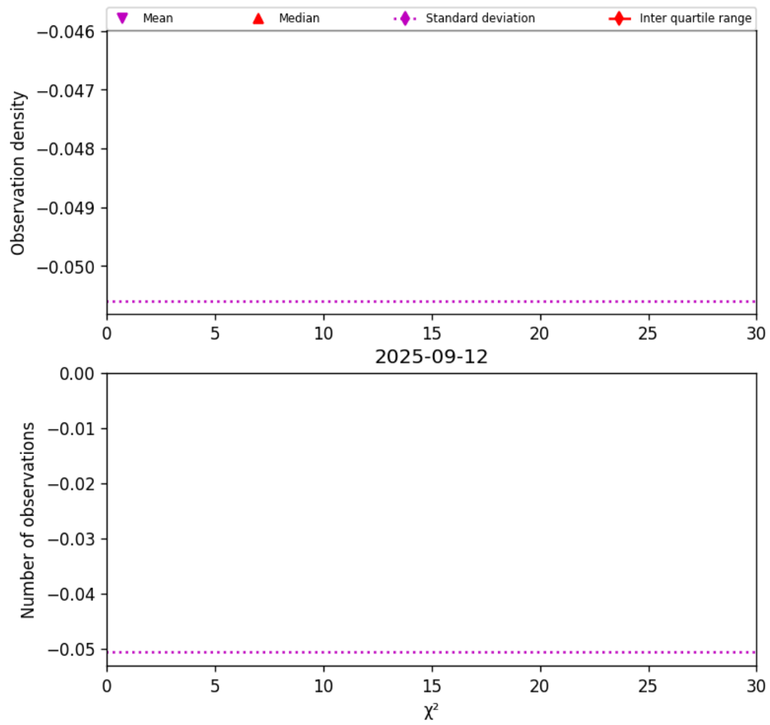
Figure 36: Histogram of “ \chi^2 ” for 2025-09-12 to 2025-09-13
