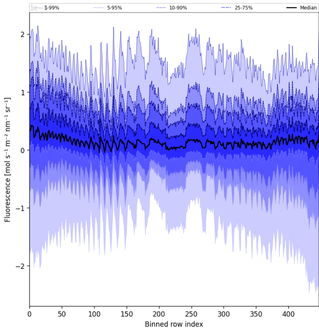
Figure 55: Along track statistics of “Fluorescence” for 2025-09-12 to 2025-09-13
