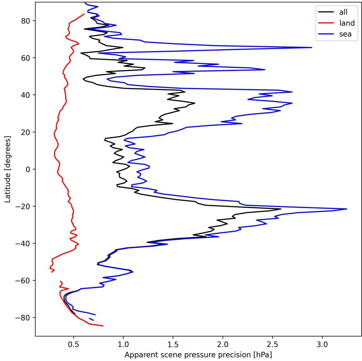
Figure 18: Zonal average of “Apparent scene pressure precision” for 2025-09-12 to 2025-09-13.
