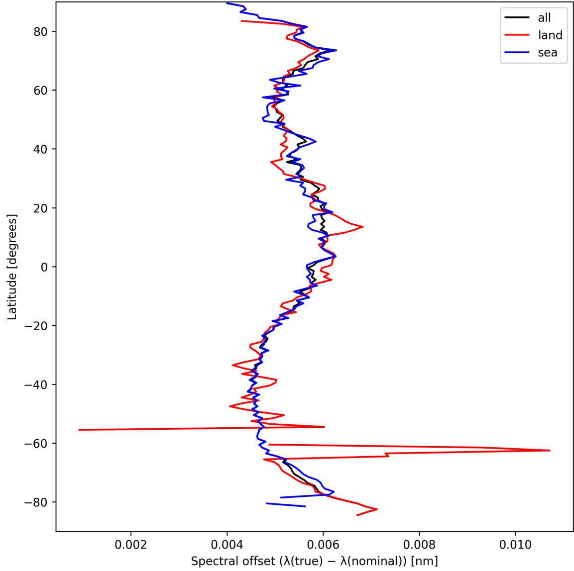
Figure 26: Zonal average of “Spectral offset ( \lambda_{\text{true}} - \lambda_{\text{nominal}} )” for 2025-09-12 to 2025-09-13.
