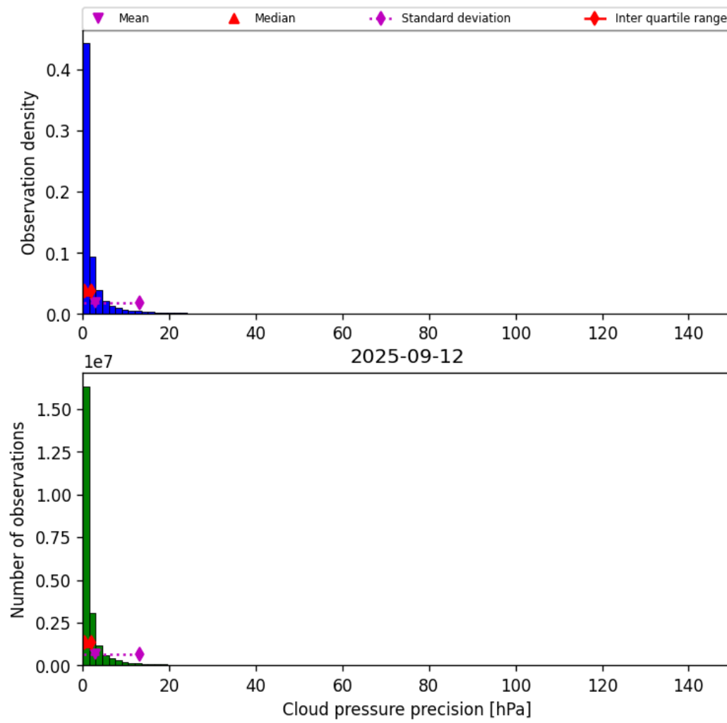
Figure 29: Histogram of “Cloud pressure precision” for 2025-09-12 to 2025-09-13
