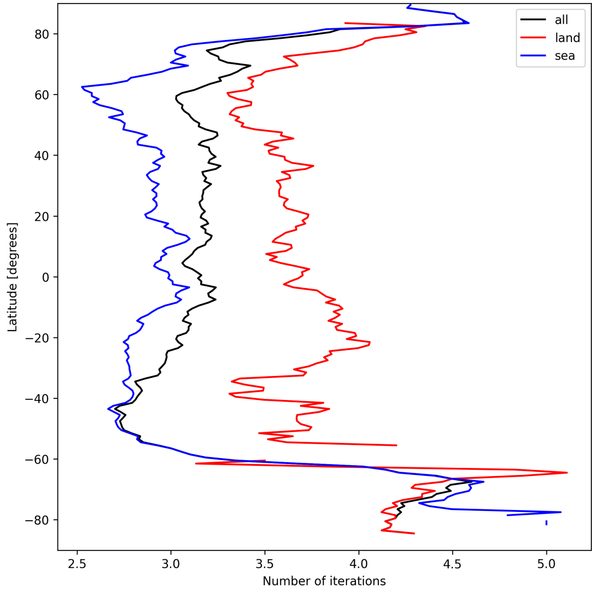
Figure 20: Zonal average of “Number of iterations” for 2025-09-12 to 2025-09-13.
