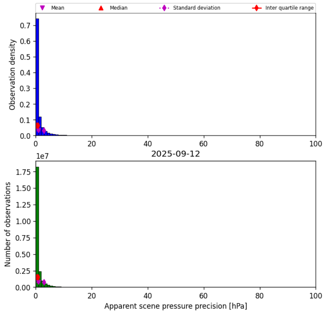
Figure 35: Histogram of “Apparent scene pressure precision” for 2025-09-12 to 2025-09-13
