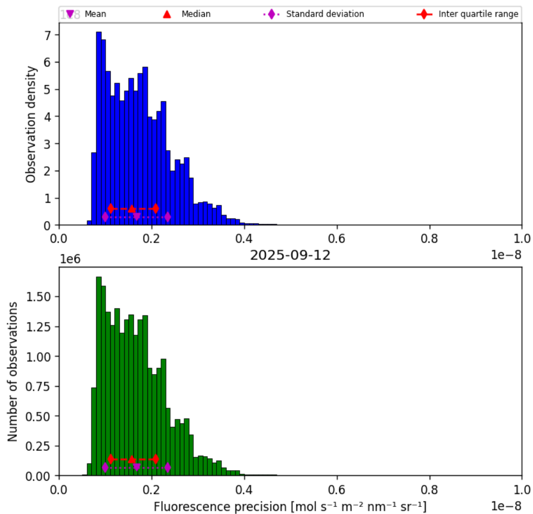
Figure 39: Histogram of “Fluorescence precision” for 2025-09-12 to 2025-09-13
