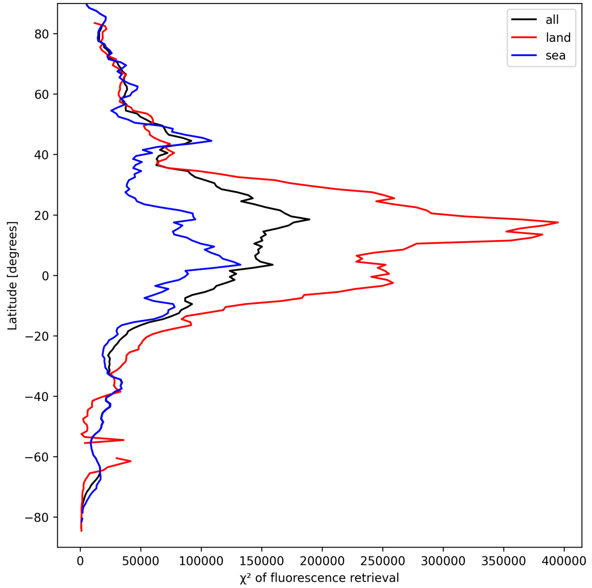
Figure 23: Zonal average of “ \chi^2 of fluorescence retrieval” for 2025-09-12 to 2025-09-13.
