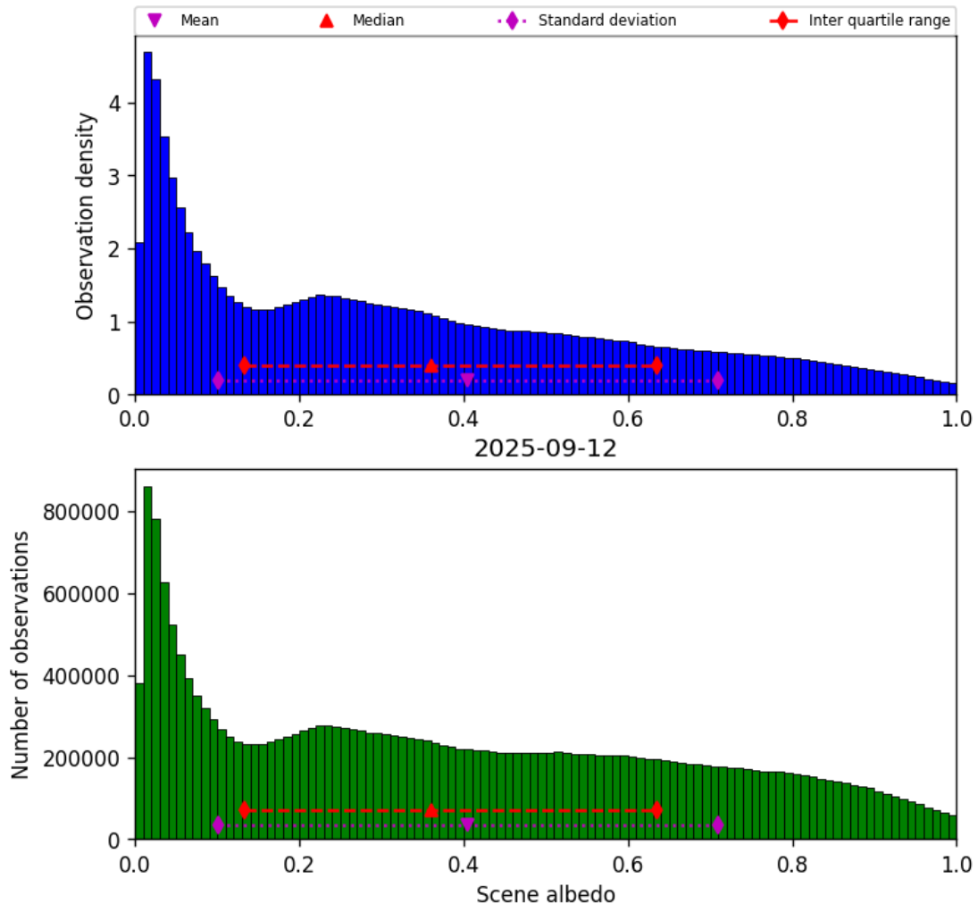
Figure 32: Histogram of “Scene albedo” for 2025-09-12 to 2025-09-13
