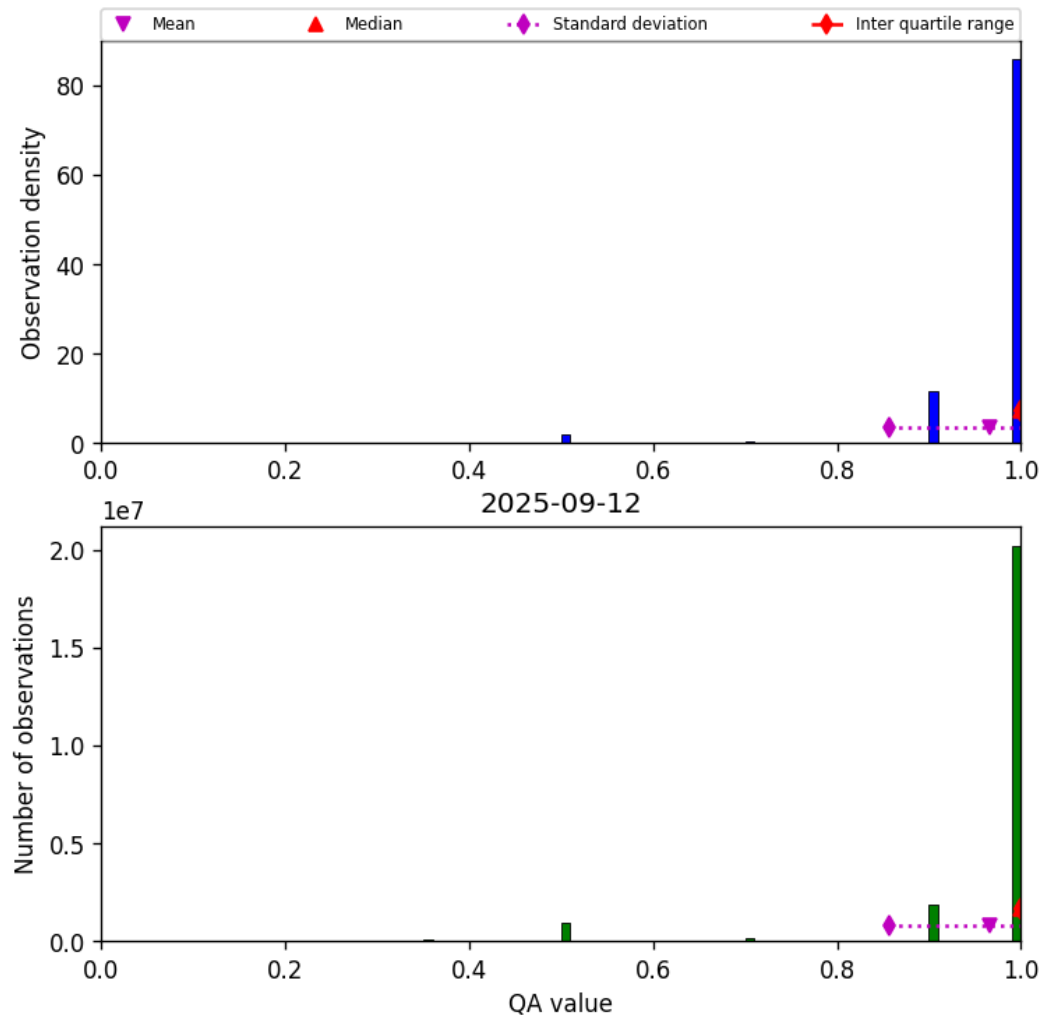
Figure 27: Histogram of “QA value” for 2025-09-12 to 2025-09-13
