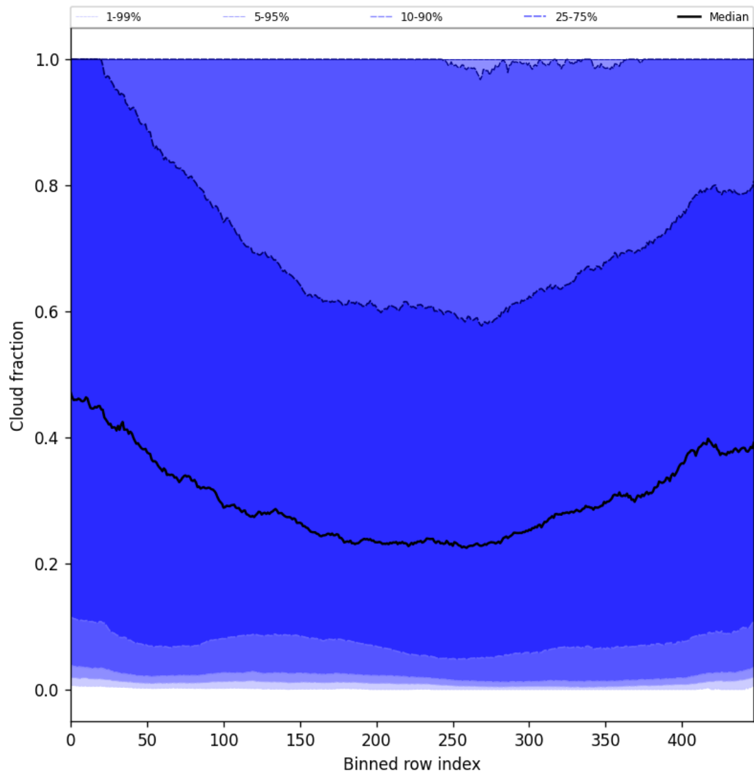
Figure 47: Along track statistics of “Cloud fraction” for 2025-09-12 to 2025-09-13
