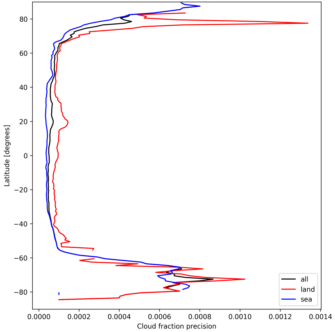
Figure 14: Zonal average of “Cloud fraction precision” for 2025-09-12 to 2025-09-13.
