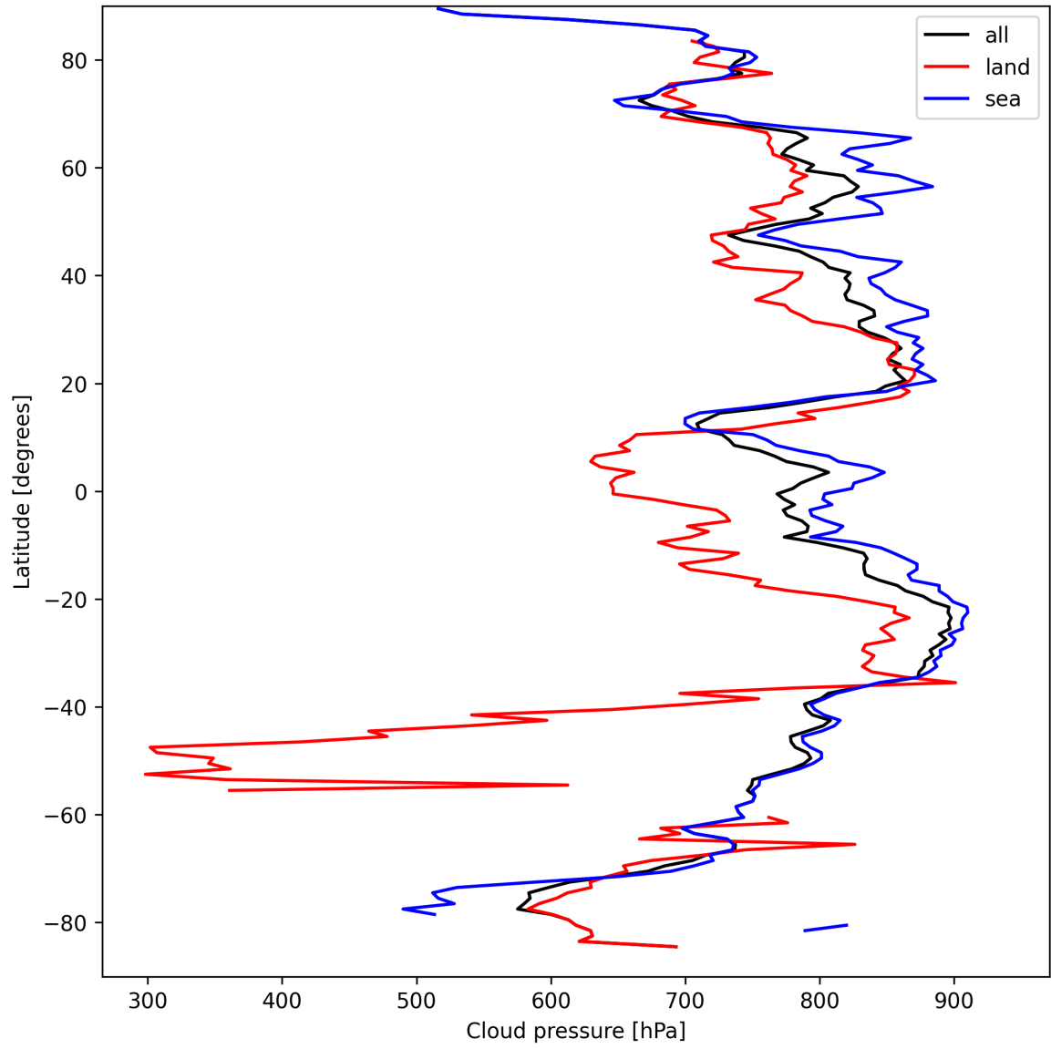
Figure 11: Zonal average of “Cloud pressure” for 2025-09-12 to 2025-09-13.
