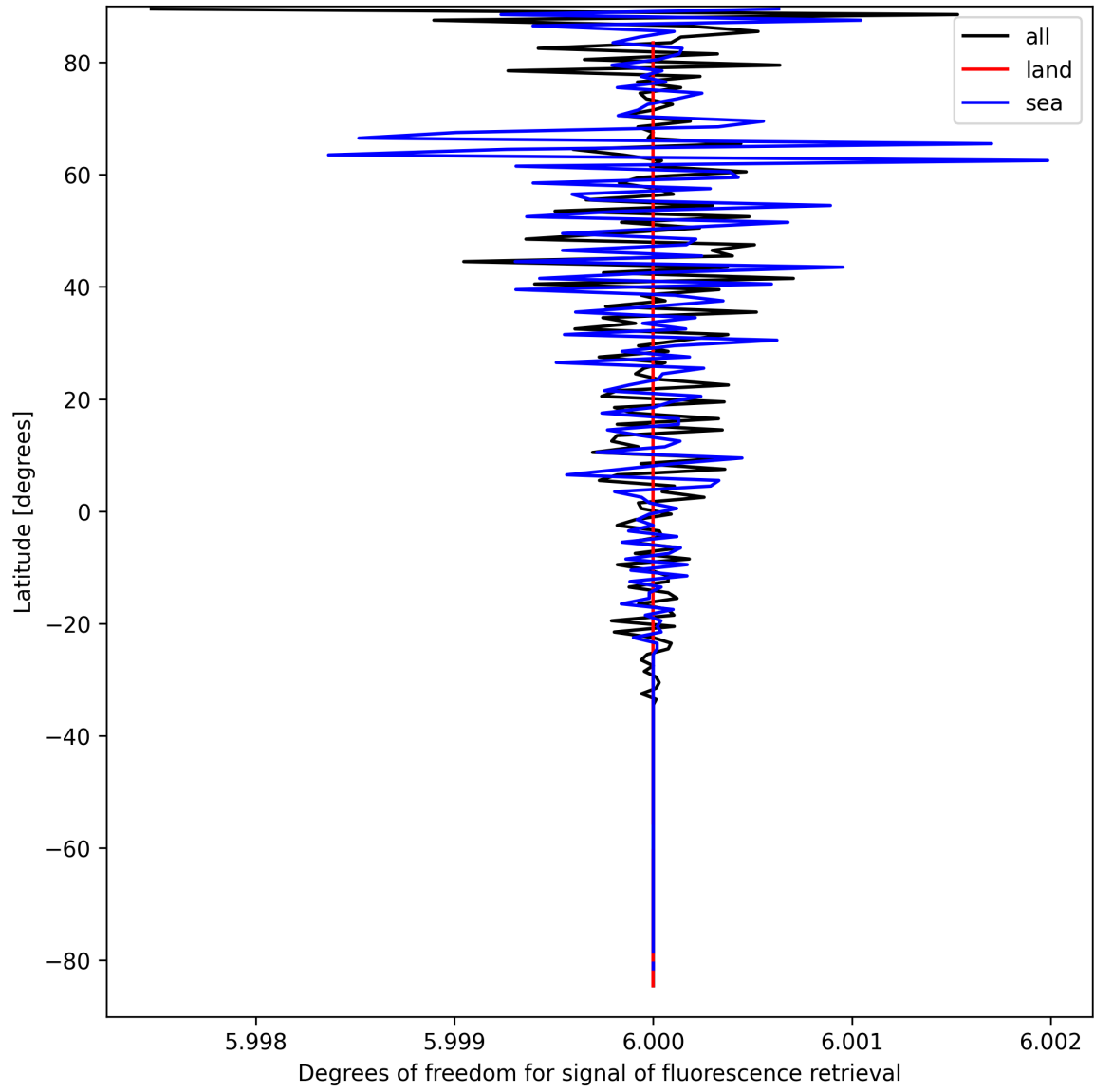
Figure 24: Zonal average of “Degrees of freedom for signal of fluorescence retrieval” for 2025-09-12 to 2025-09-13.
