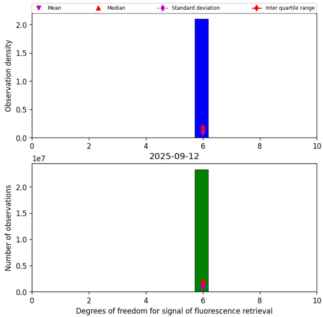
Figure 41: Histogram of “Degrees of freedom for signal of fluorescence retrieval” for 2025-09-12 to 2025-09-13
