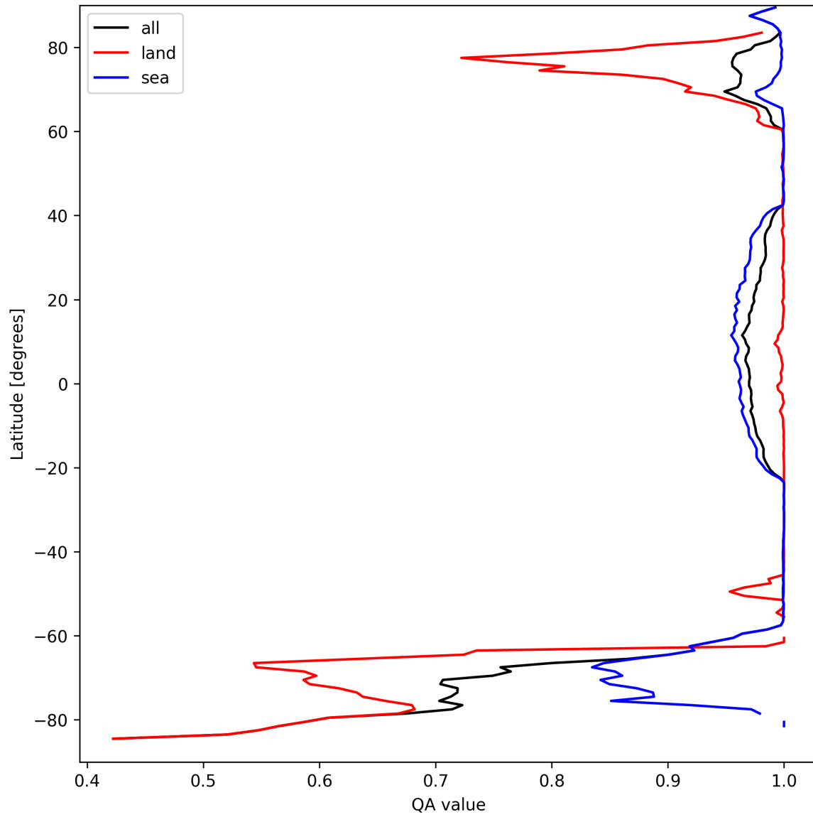
Figure 10: Zonal average of “QA value” for 2025-09-12 to 2025-09-13.
