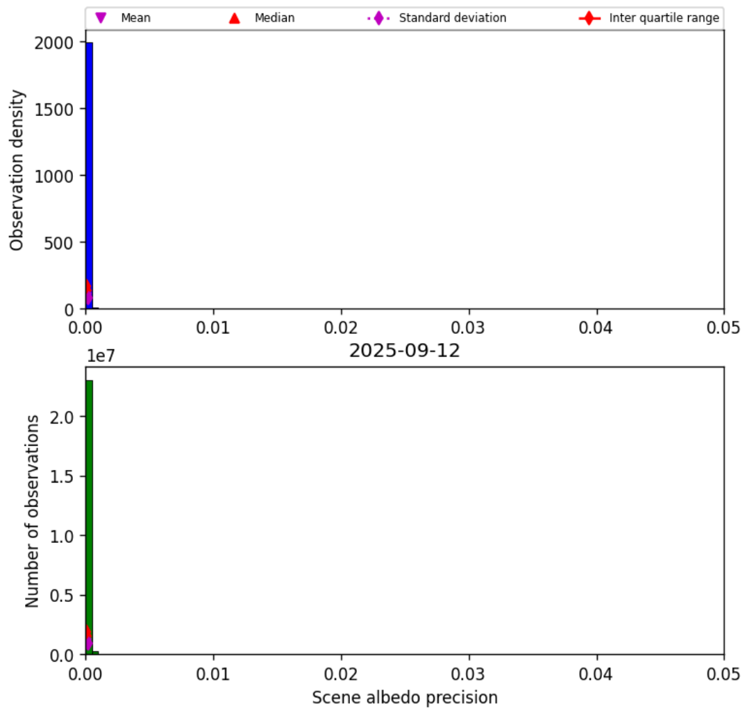
Figure 33: Histogram of “Scene albedo precision” for 2025-09-12 to 2025-09-13
