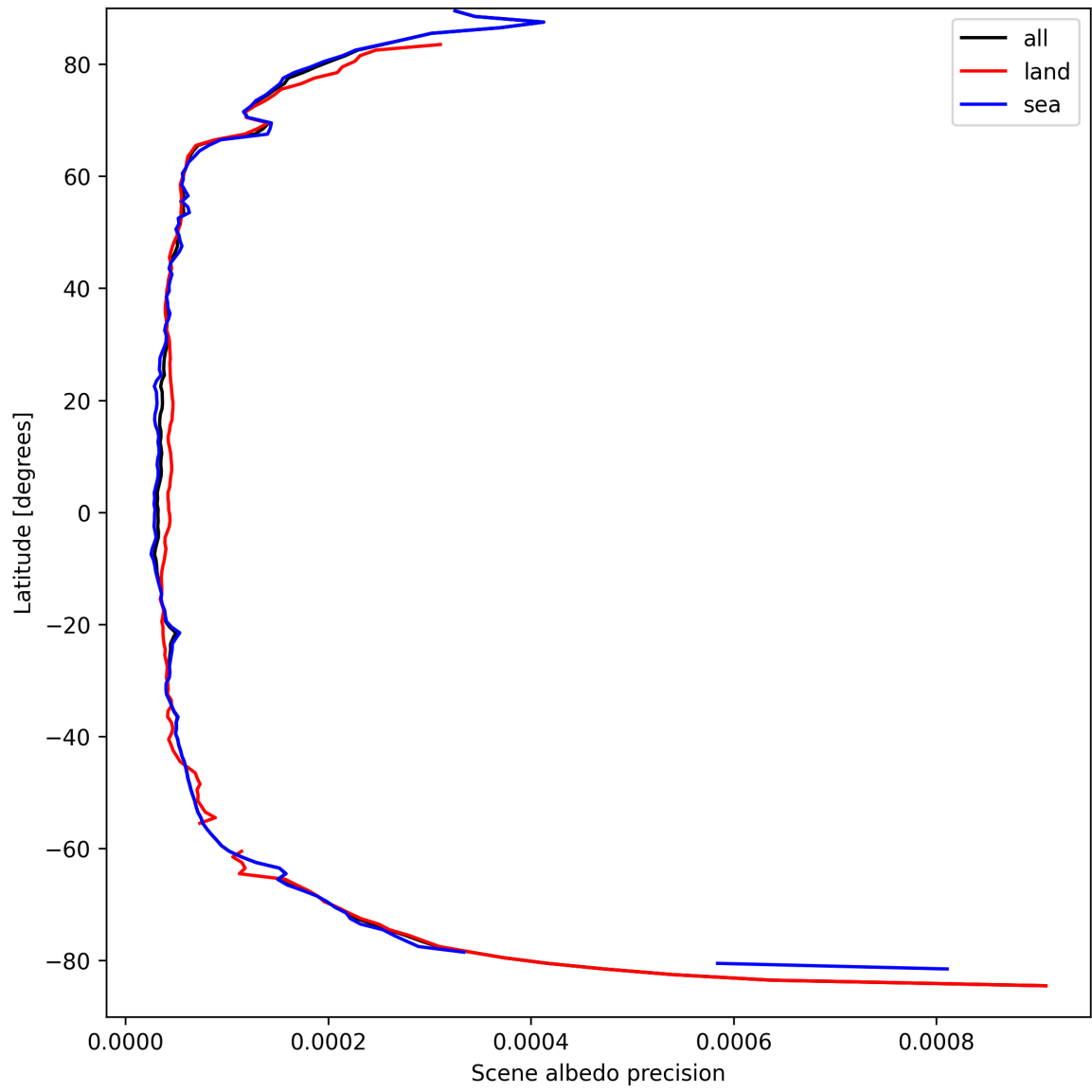
Figure 16: Zonal average of “Scene albedo precision” for 2025-09-12 to 2025-09-13.
