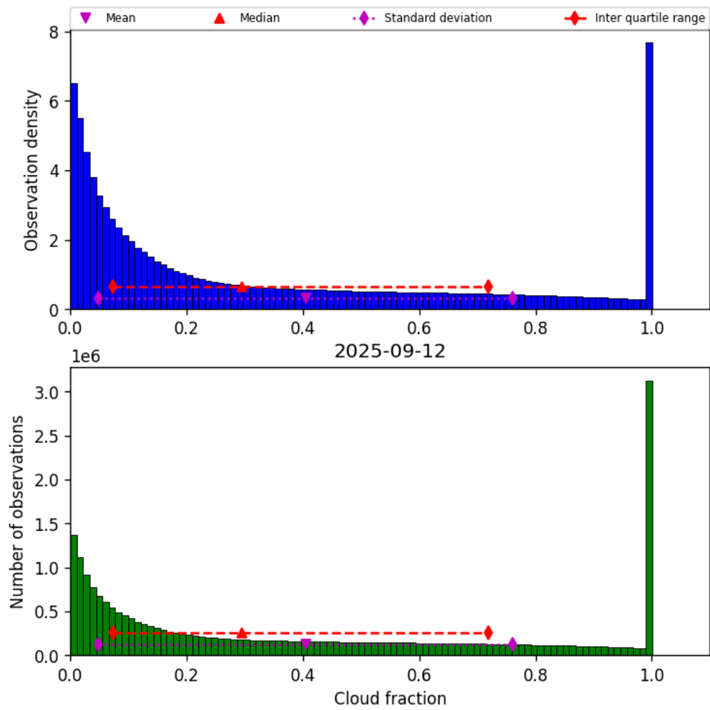
Figure 30: Histogram of “Cloud fraction” for 2025-09-12 to 2025-09-13
