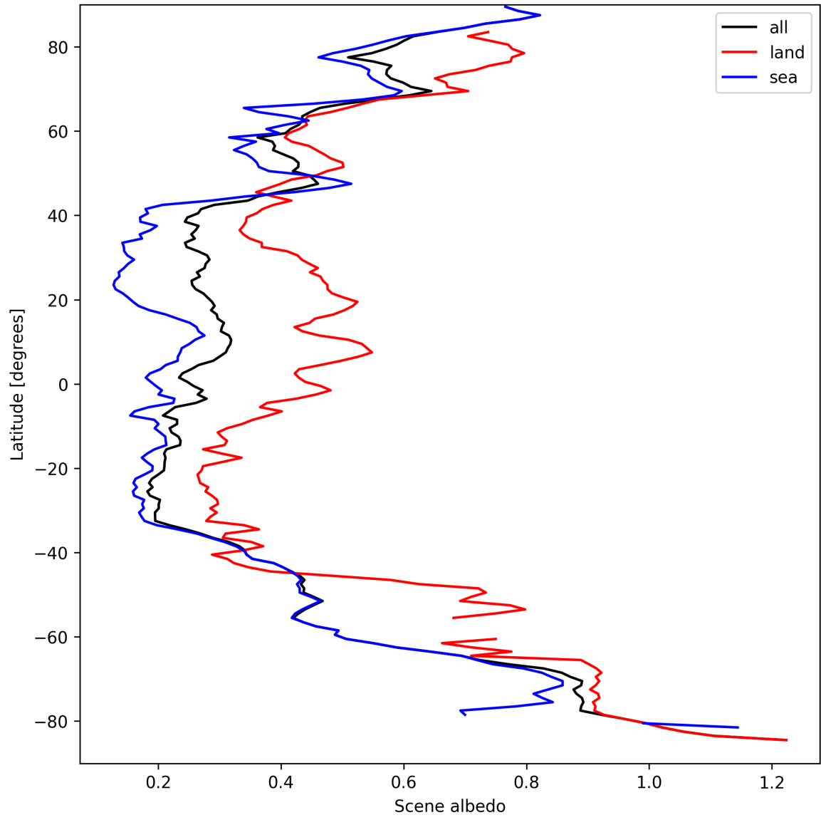
Figure 15: Zonal average of “Scene albedo” for 2025-09-12 to 2025-09-13.
