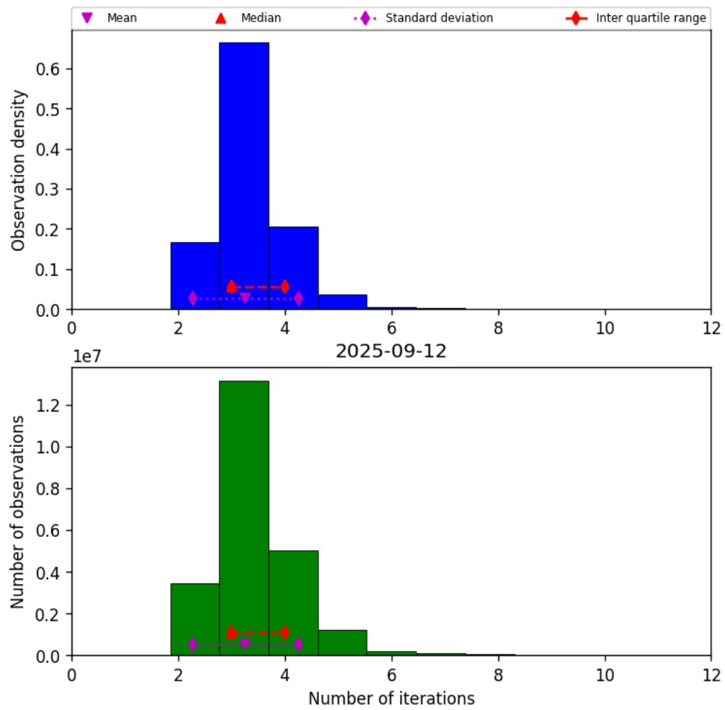
Figure 37: Histogram of “Number of iterations” for 2025-09-12 to 2025-09-13
