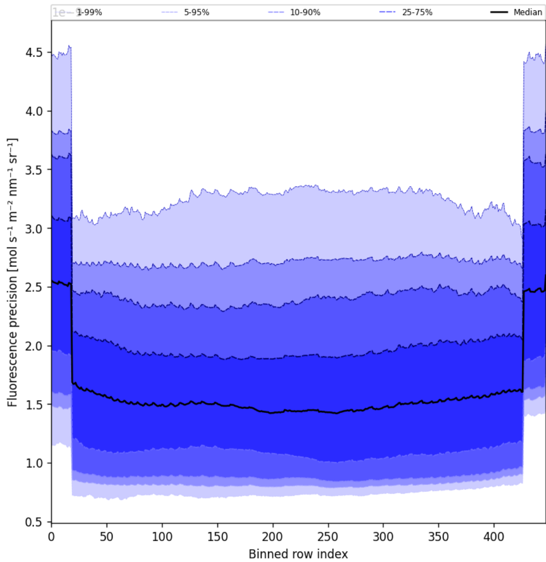
Figure 56: Along track statistics of “Fluorescence precision” for 2025-09-12 to 2025-09-13
