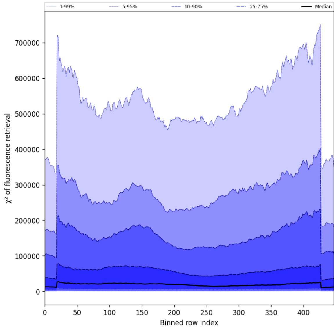
Figure 57: Along track statistics of “ \chi^2 of fluorescence retrieval” for 2025-09-12 to 2025-09-13
