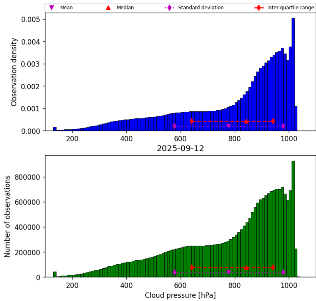
Figure 28: Histogram of “Cloud pressure” for 2025-09-12 to 2025-09-13
