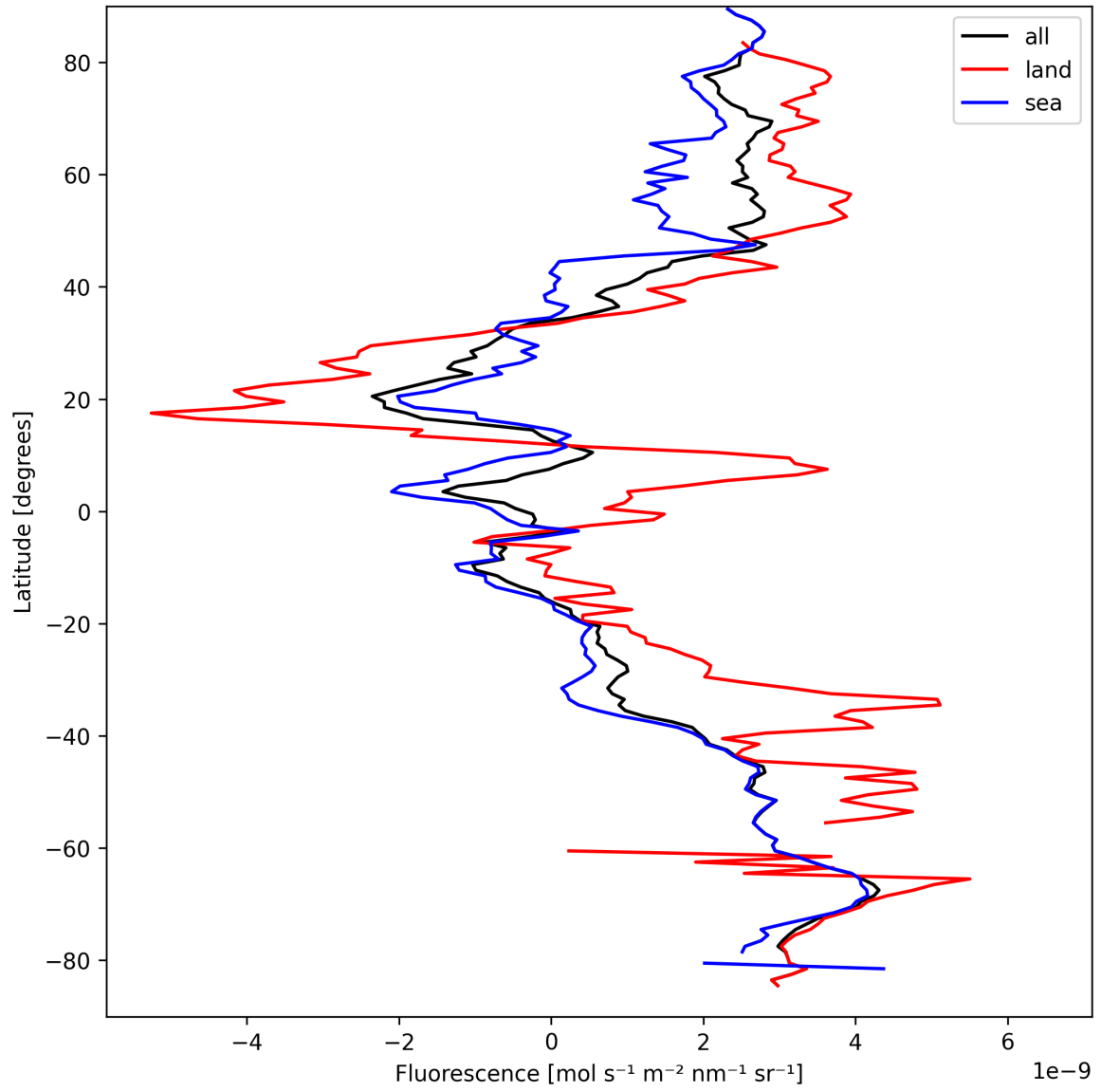
Figure 21: Zonal average of “Fluorescence” for 2025-09-12 to 2025-09-13.
