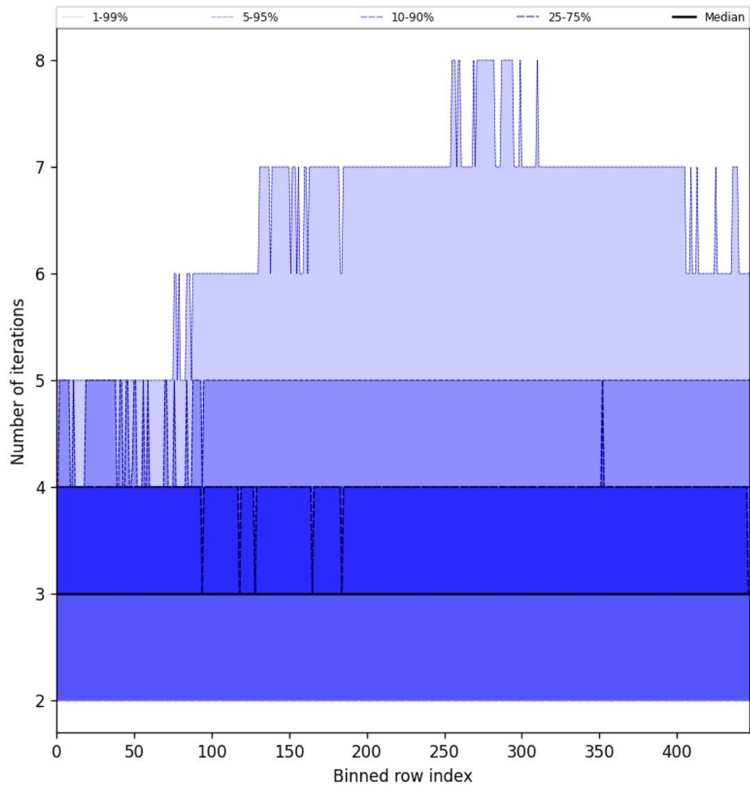
Figure 54: Along track statistics of “Number of iterations” for 2025-09-12 to 2025-09-13
