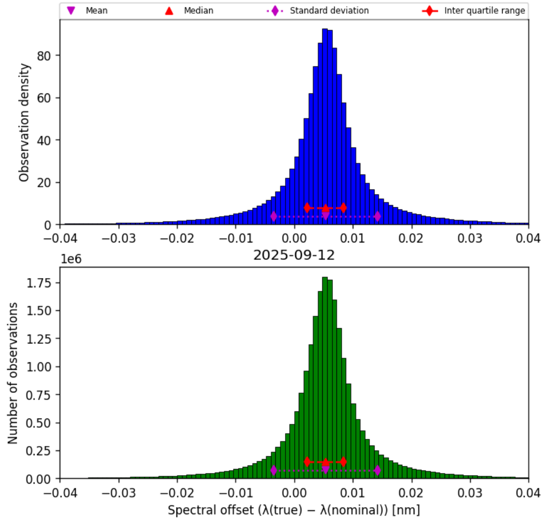
Figure 43: Histogram of “Spectral offset ( \lambda_{\text{true}} - \lambda_{\text{nominal}} )” for 2025-09-12 to 2025-09-13
