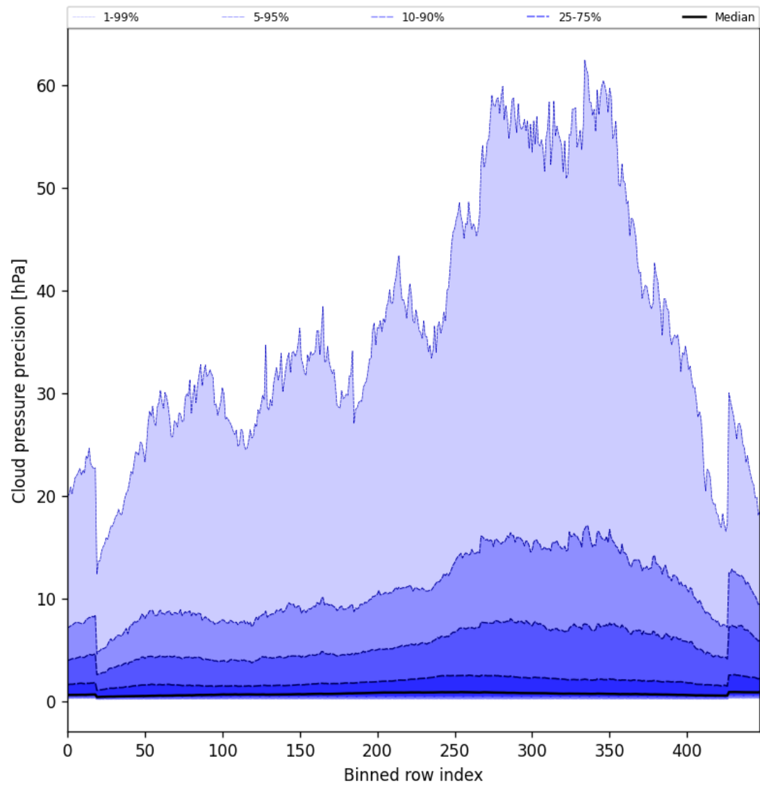
Figure 46: Along track statistics of “Cloud pressure precision” for 2025-09-12 to 2025-09-13
