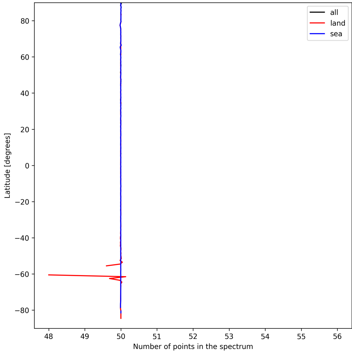
Figure 25: Zonal average of “Number of points in the spectrum” for 2025-09-12 to 2025-09-13.
