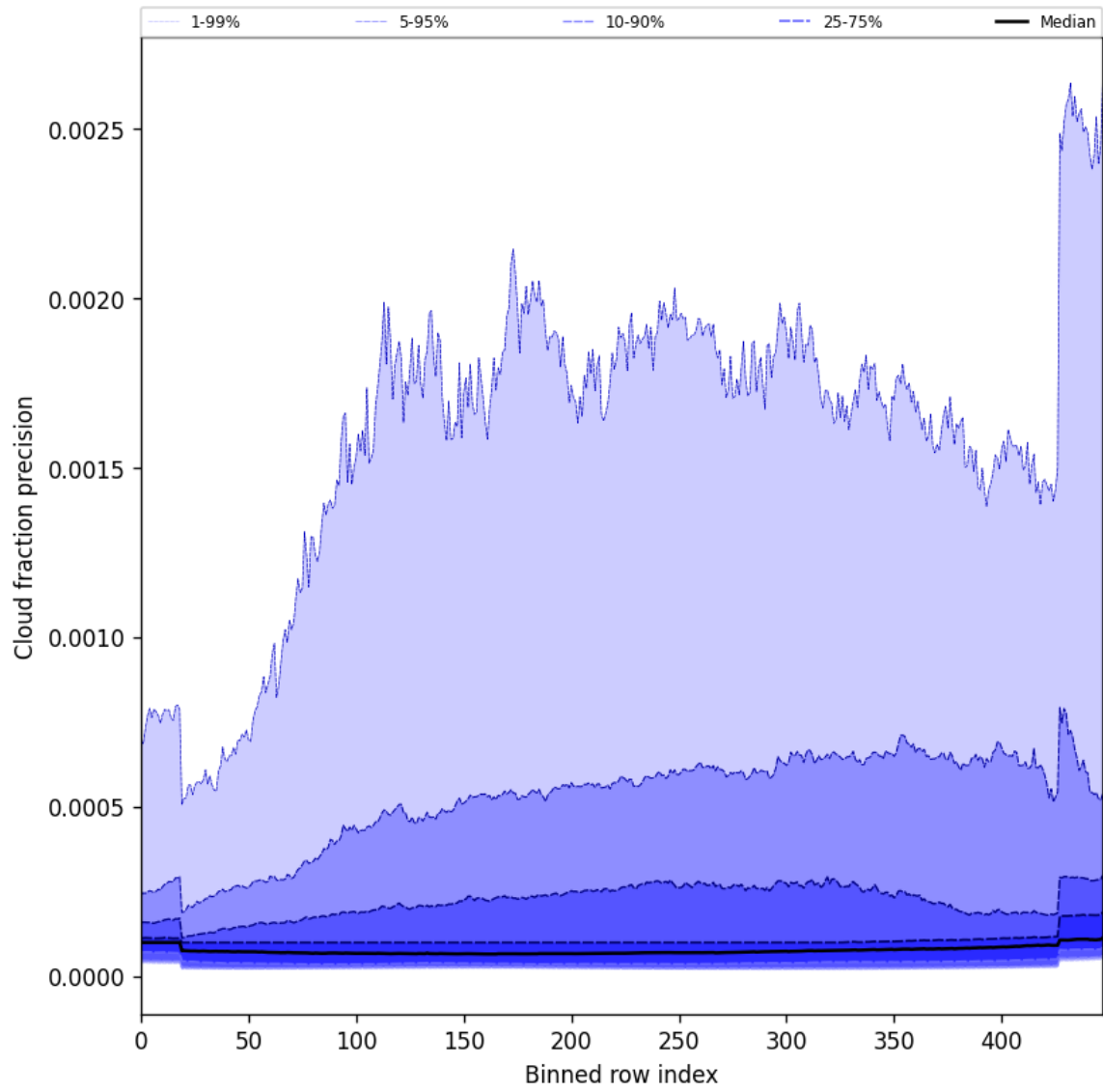
Figure 48: Along track statistics of “Cloud fraction precision” for 2025-09-12 to 2025-09-13
