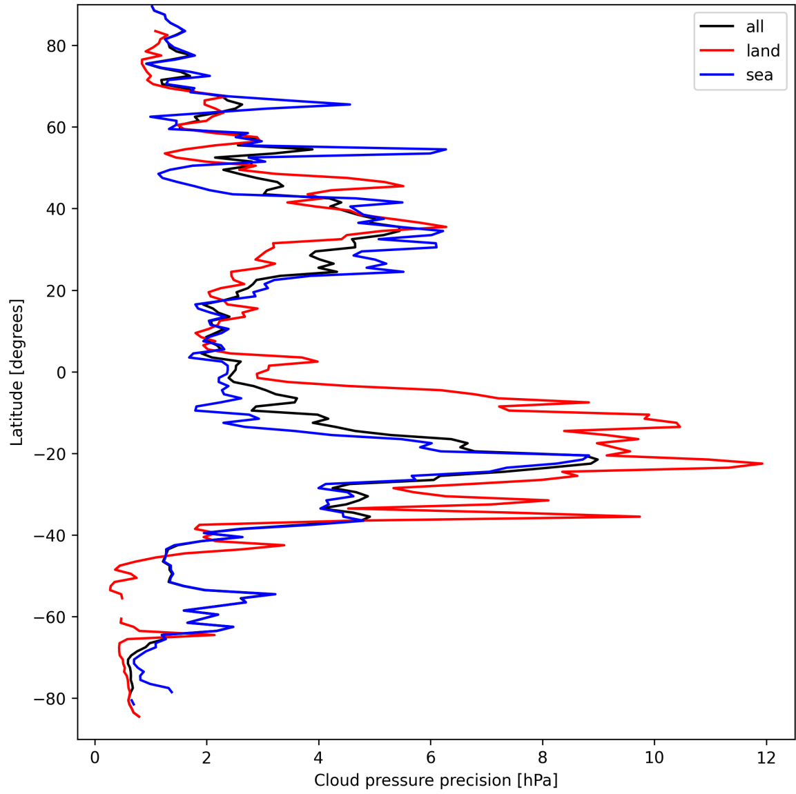
Figure 12: Zonal average of “Cloud pressure precision” for 2025-09-12 to 2025-09-13.
