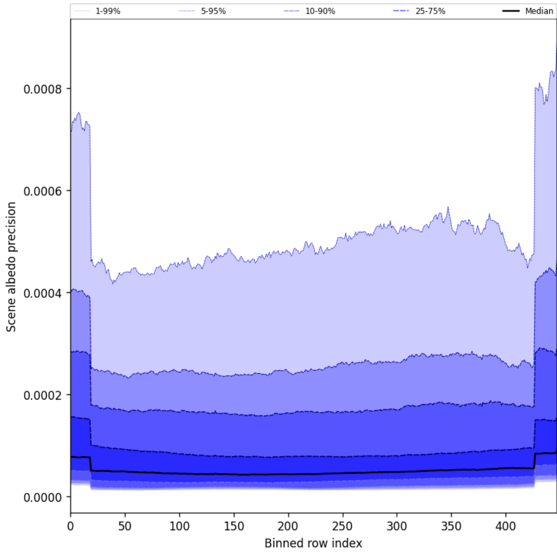
Figure 50: Along track statistics of “Scene albedo precision” for 2025-09-12 to 2025-09-13
