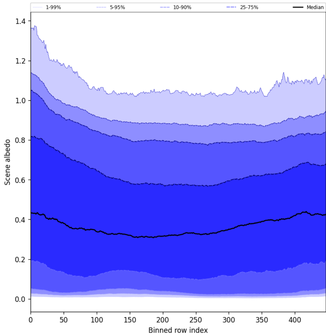
Figure 49: Along track statistics of “Scene albedo” for 2025-09-12 to 2025-09-13
