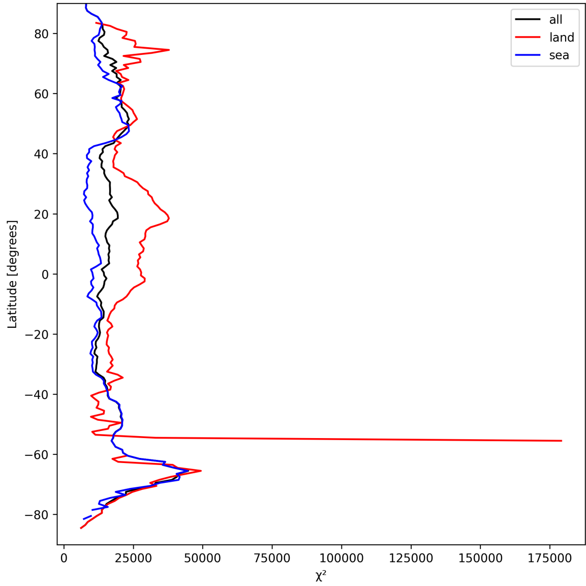
Figure 19: Zonal average of “ \chi^2 ” for 2025-09-12 to 2025-09-13.
