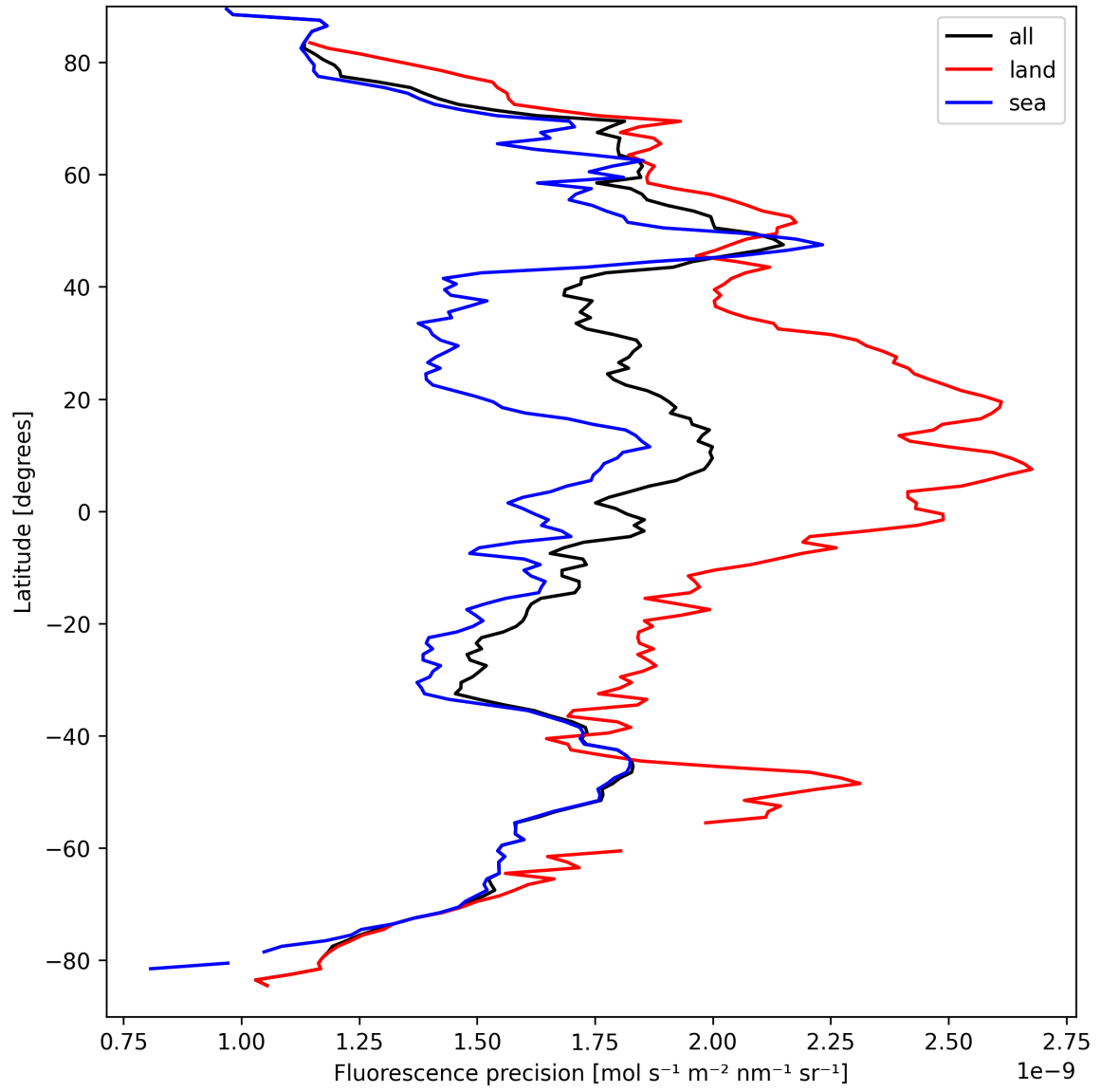
Figure 22: Zonal average of “Fluorescence precision” for 2025-09-12 to 2025-09-13.
