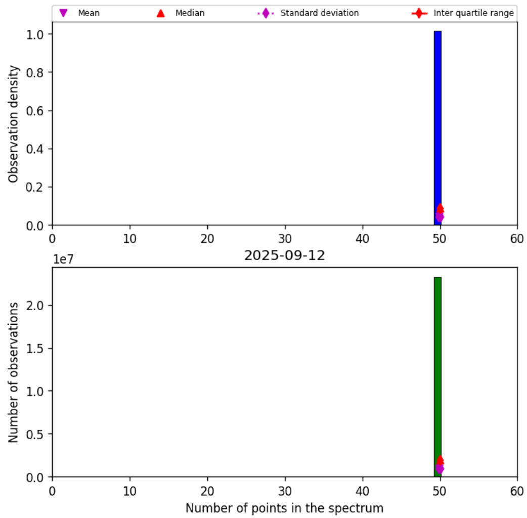
Figure 42: Histogram of “Number of points in the spectrum” for 2025-09-12 to 2025-09-13
