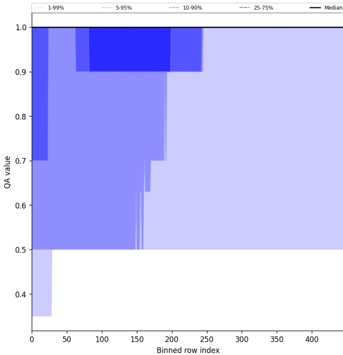
Figure 44: Along track statistics of “QA value” for 2025-09-12 to 2025-09-13
