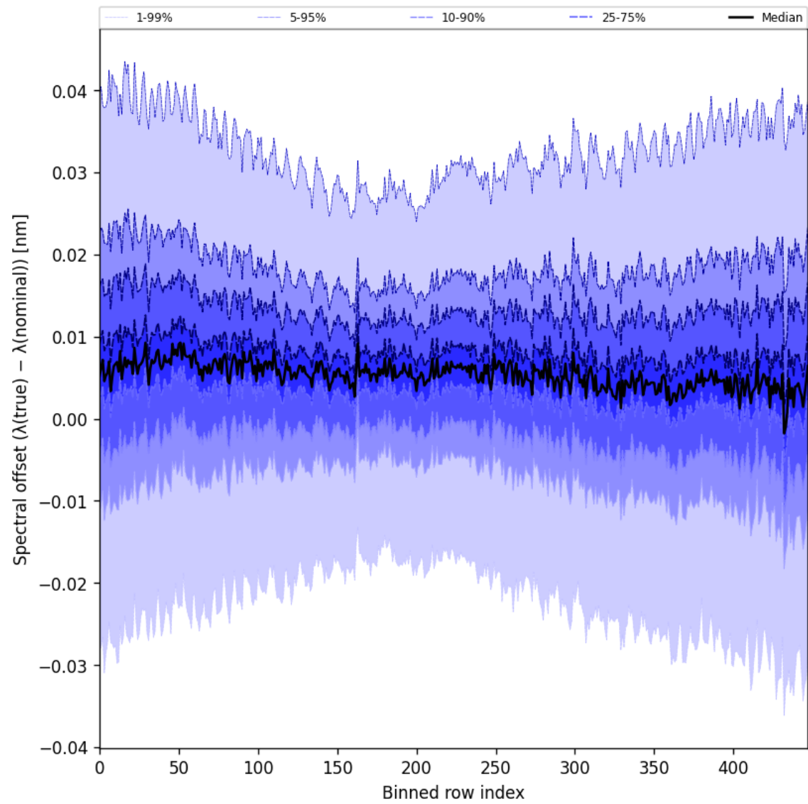
Figure 60: Along track statistics of “Spectral offset ( \lambda_{\text{true}} - \lambda_{\text{nominal}} )” for 2025-09-12 to 2025-09-13
