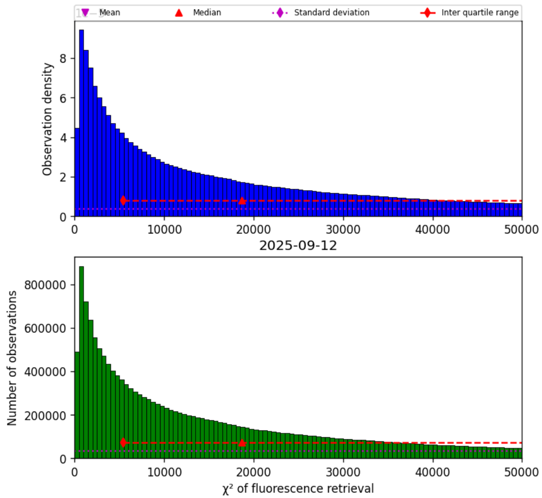
Figure 40: Histogram of “ \chi^2 of fluorescence retrieval” for 2025-09-12 to 2025-09-13
