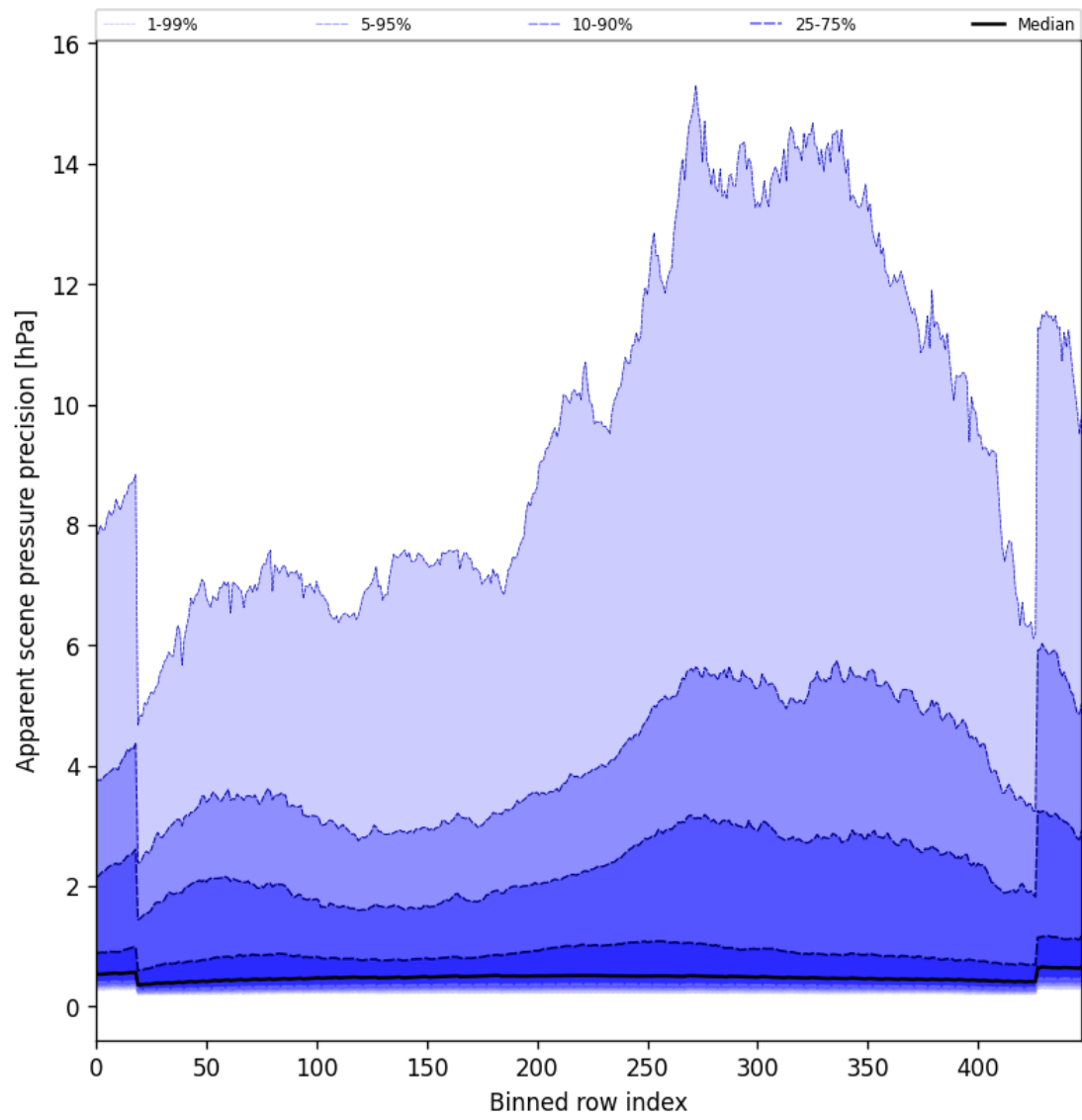
Figure 52: Along track statistics of “Apparent scene pressure precision” for 2025-09-12 to 2025-09-13
