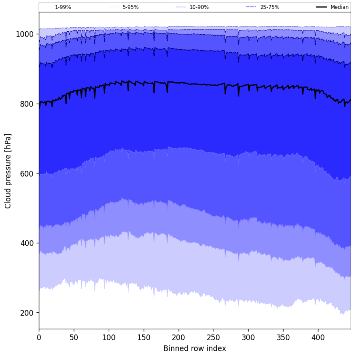
Figure 45: Along track statistics of “Cloud pressure” for 2025-09-12 to 2025-09-13
