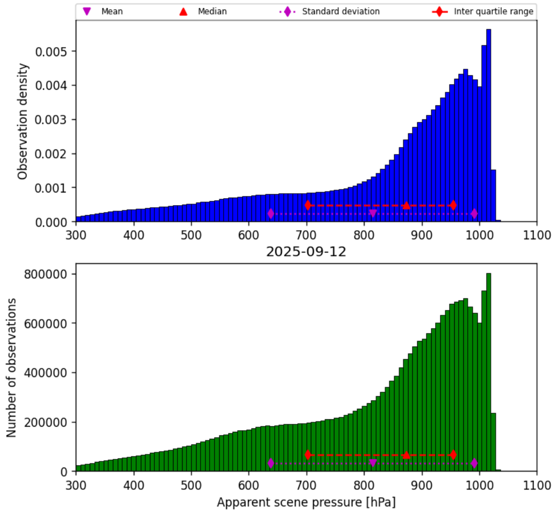
Figure 34: Histogram of “Apparent scene pressure” for 2025-09-12 to 2025-09-13
