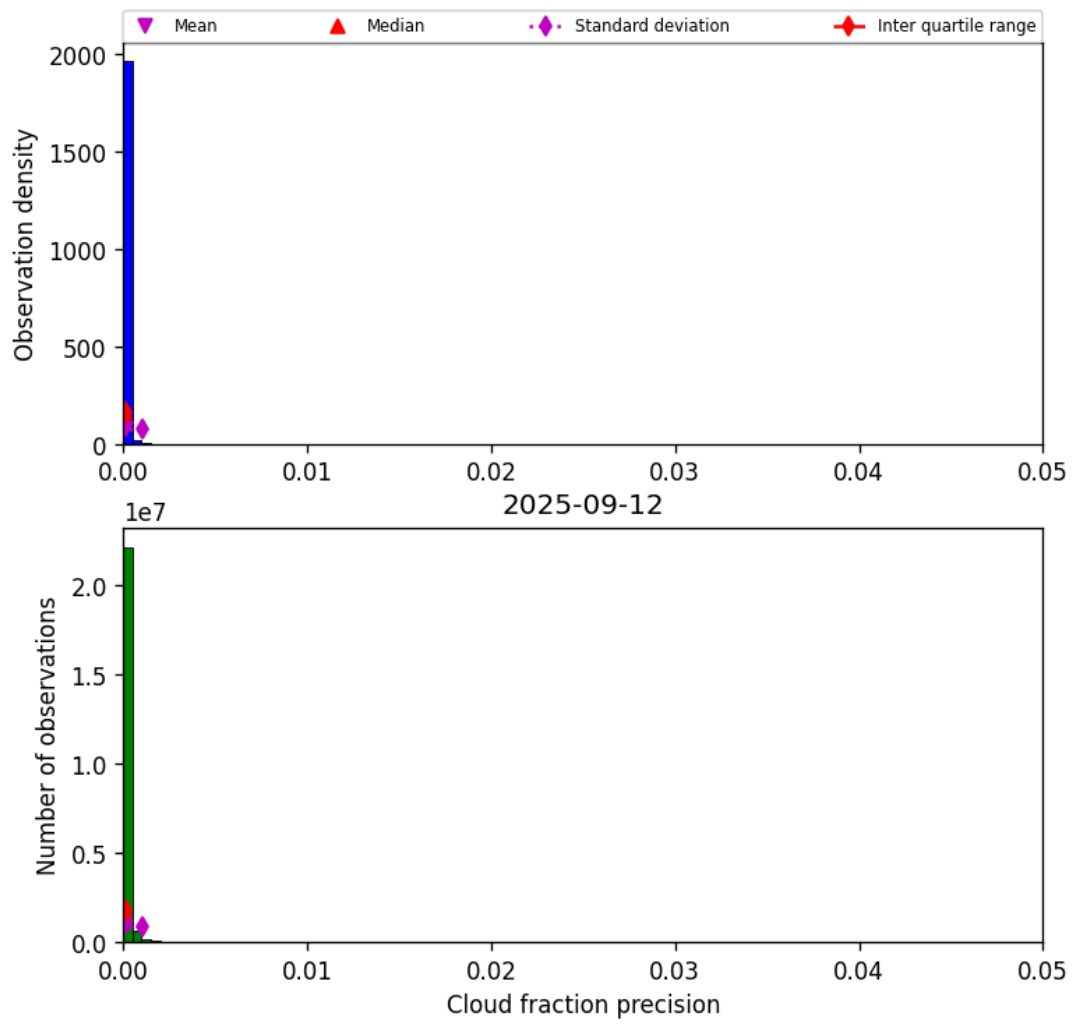
Figure 31: Histogram of “Cloud fraction precision” for 2025-09-12 to 2025-09-13
