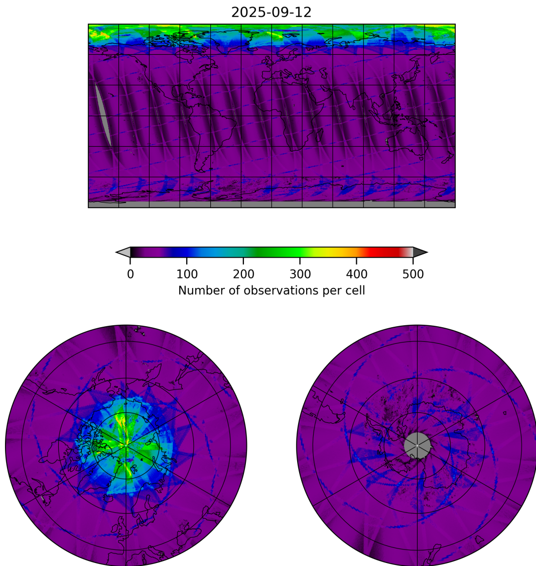
Figure 9: Map of the number of observations for 2025-09-12 to 2025-09-13
