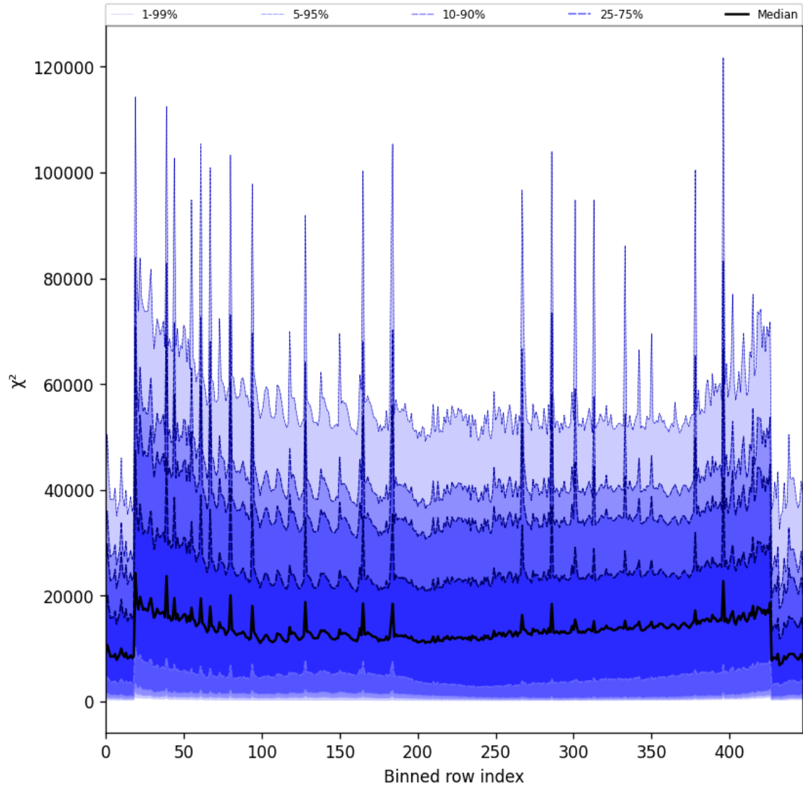
Figure 53: Along track statistics of “ \chi^2 ” for 2025-09-14 to 2025-09-15
