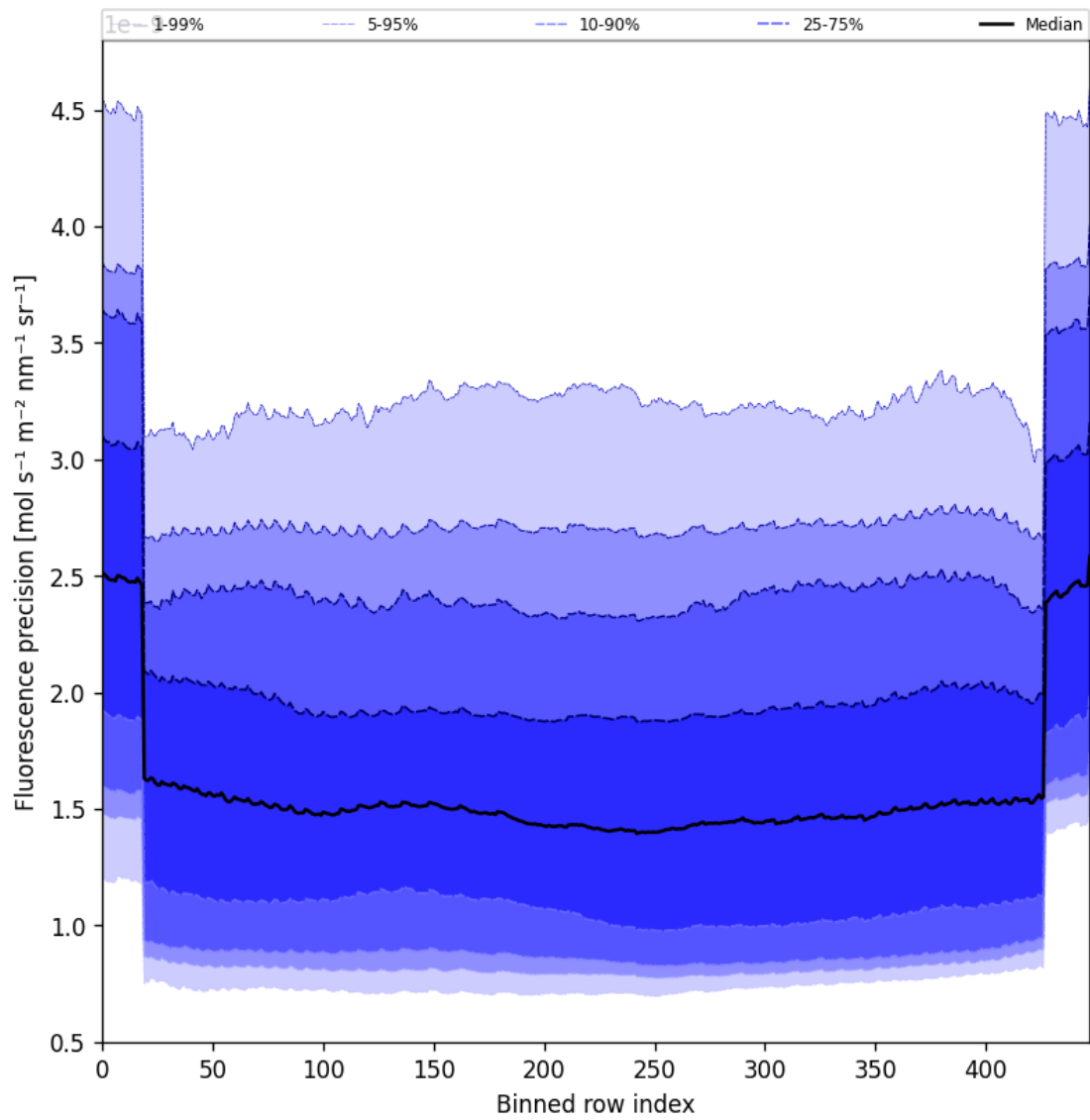
Figure 56: Along track statistics of “Fluorescence precision” for 2025-09-14 to 2025-09-15
