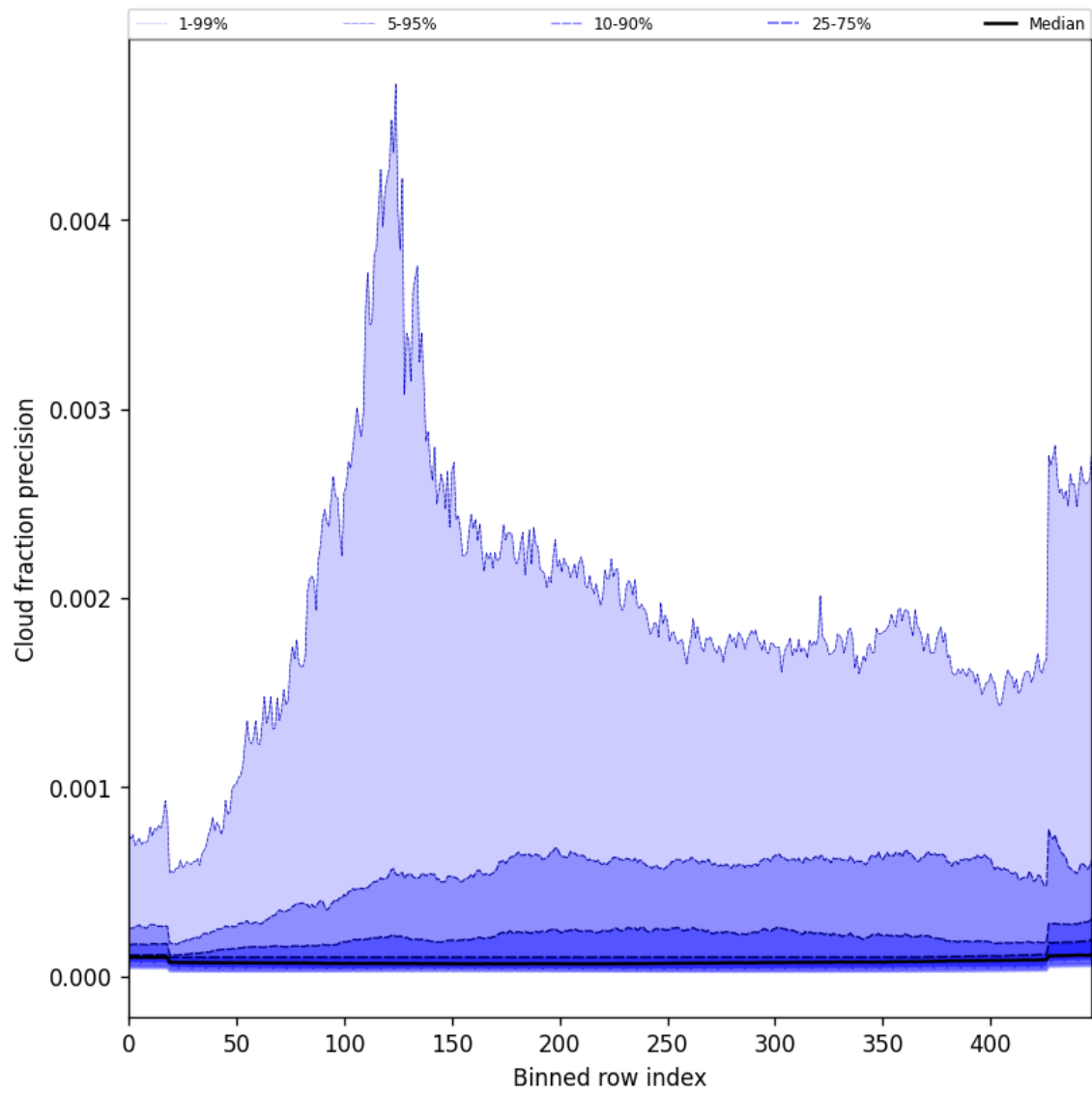
Figure 48: Along track statistics of “Cloud fraction precision” for 2025-09-14 to 2025-09-15
