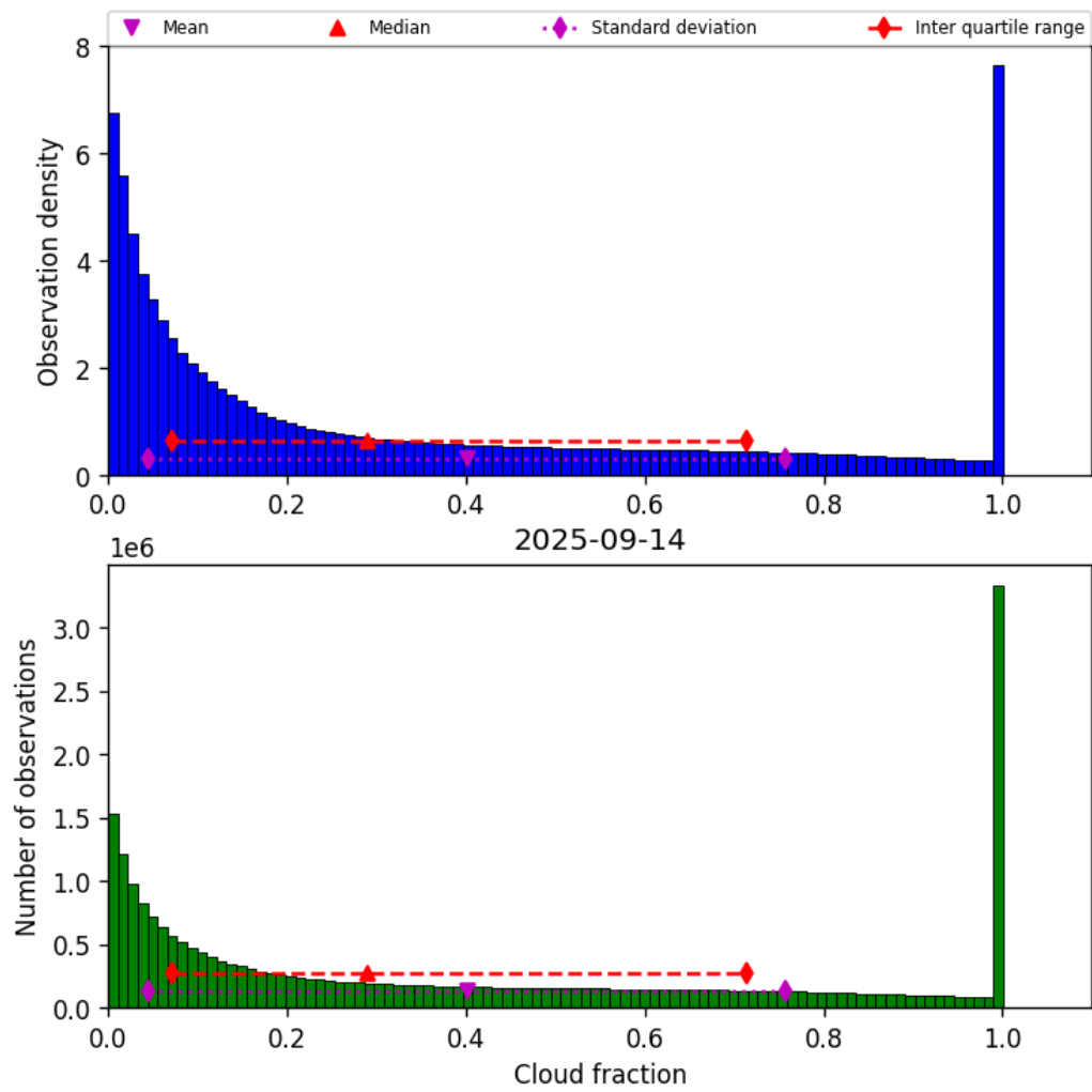
Figure 30: Histogram of “Cloud fraction” for 2025-09-14 to 2025-09-15
