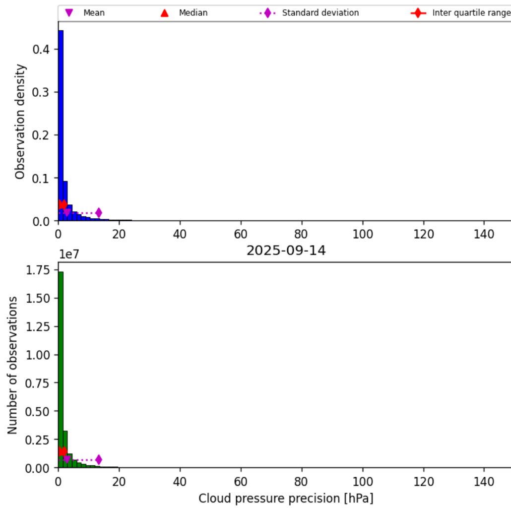
Figure 29: Histogram of “Cloud pressure precision” for 2025-09-14 to 2025-09-15
