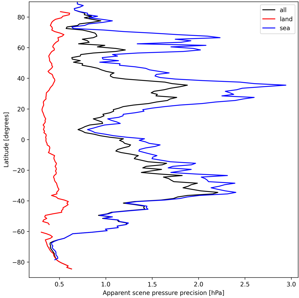
Figure 18: Zonal average of “Apparent scene pressure precision” for 2025-09-14 to 2025-09-15.
