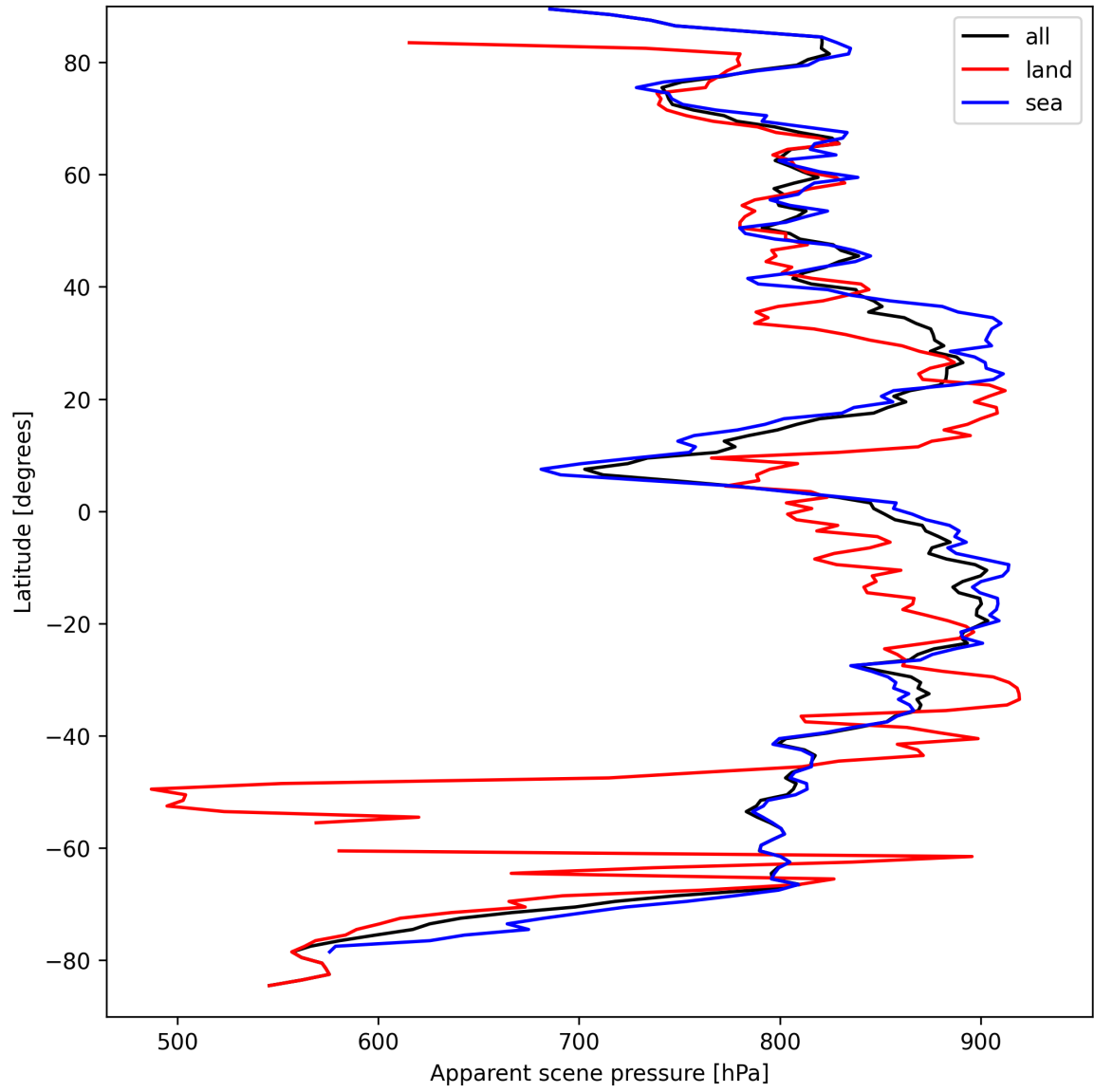
Figure 17: Zonal average of “Apparent scene pressure” for 2025-09-14 to 2025-09-15.
