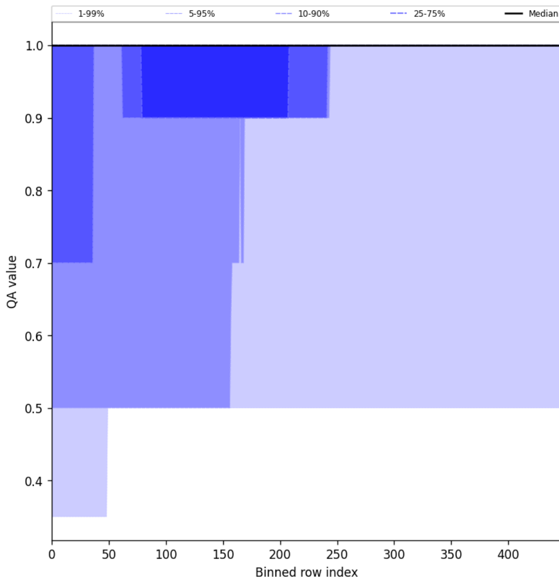
Figure 44: Along track statistics of “QA value” for 2025-09-14 to 2025-09-15
