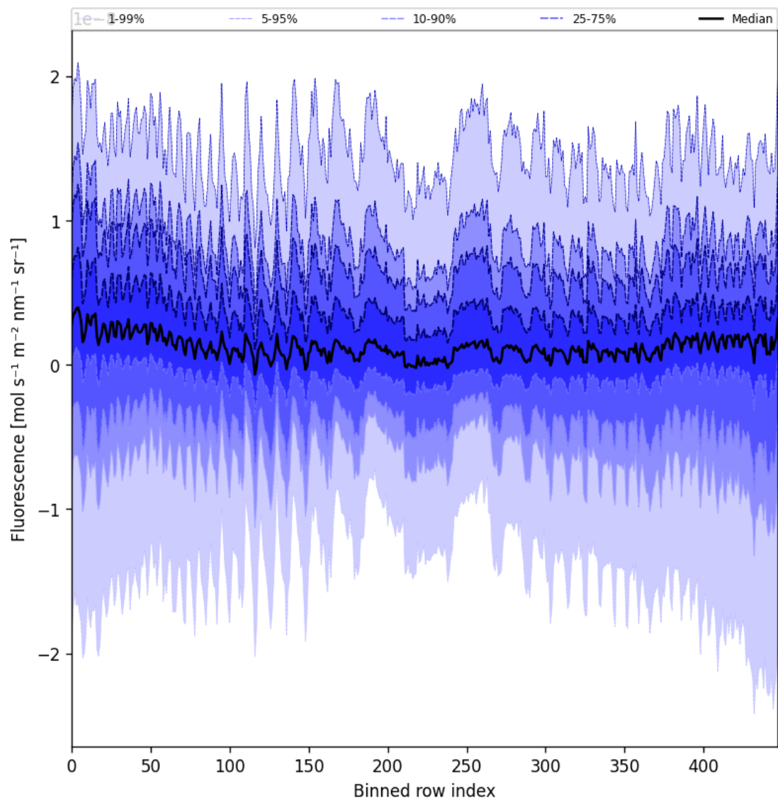
Figure 55: Along track statistics of “Fluorescence” for 2025-09-14 to 2025-09-15
