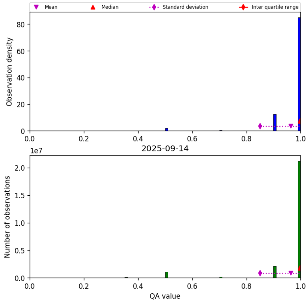
Figure 27: Histogram of “QA value” for 2025-09-14 to 2025-09-15
