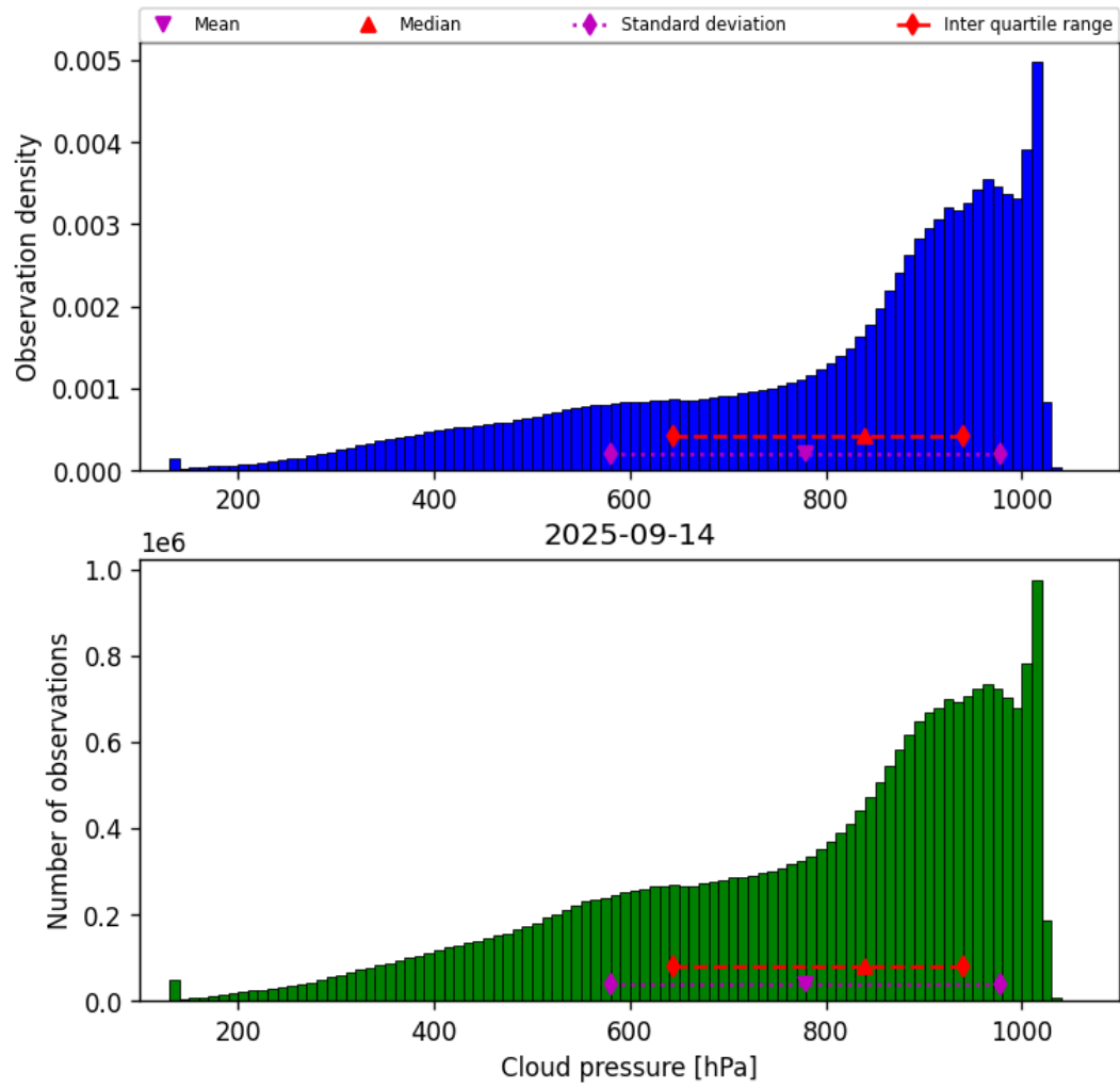
Figure 28: Histogram of “Cloud pressure” for 2025-09-14 to 2025-09-15
