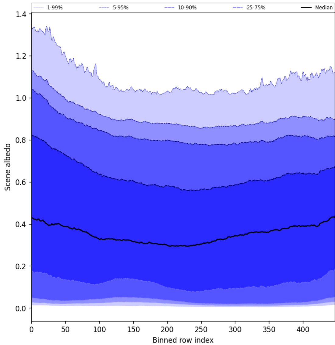
Figure 49: Along track statistics of “Scene albedo” for 2025-09-14 to 2025-09-15
