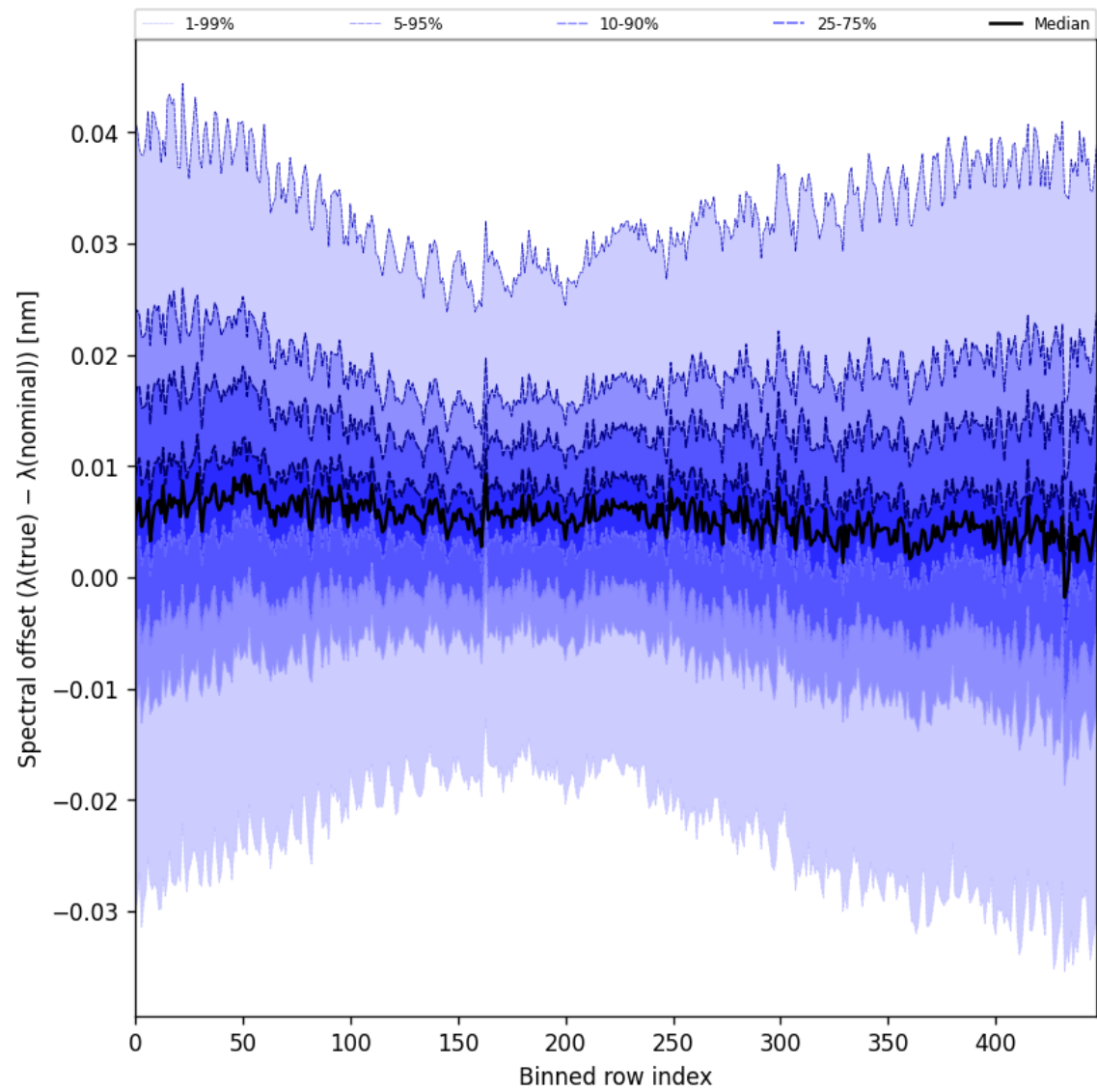
Figure 60: Along track statistics of “Spectral offset ( \lambda_{\text{true}} - \lambda_{\text{nominal}} )” for 2025-09-14 to 2025-09-15
