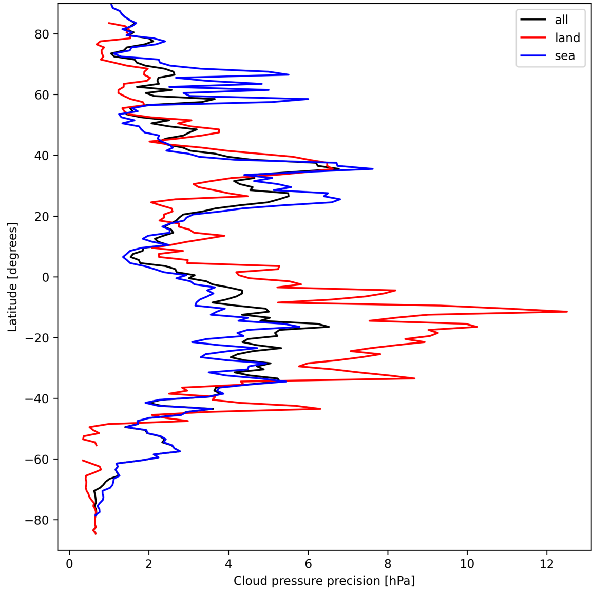
Figure 12: Zonal average of “Cloud pressure precision” for 2025-09-14 to 2025-09-15.
