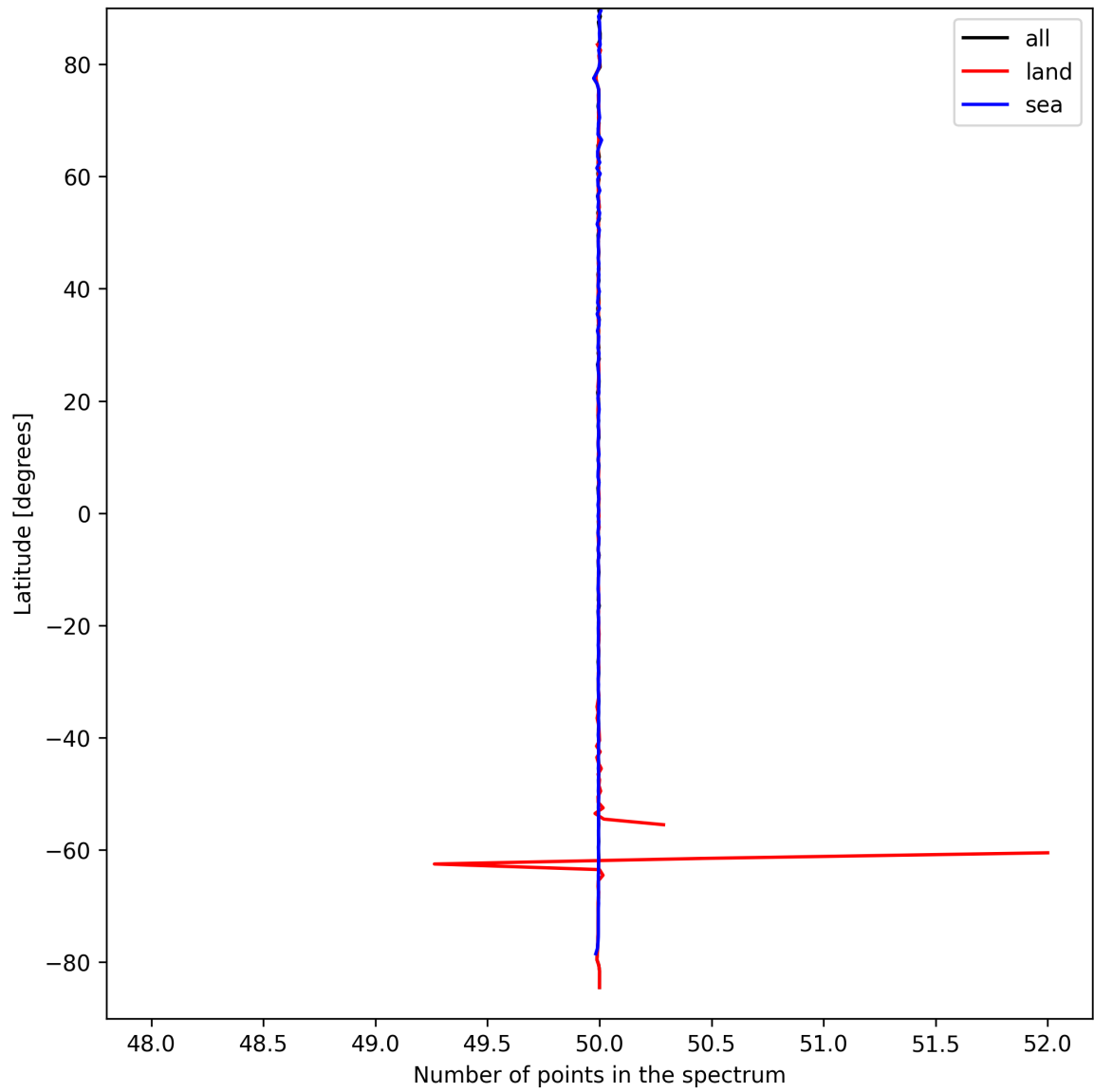
Figure 25: Zonal average of “Number of points in the spectrum” for 2025-09-14 to 2025-09-15.
