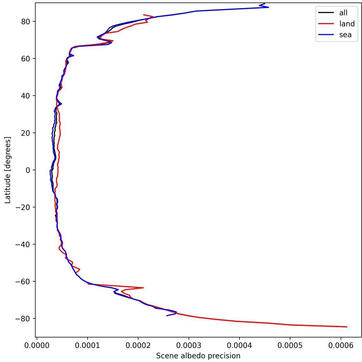
Figure 16: Zonal average of “Scene albedo precision” for 2025-09-14 to 2025-09-15.
