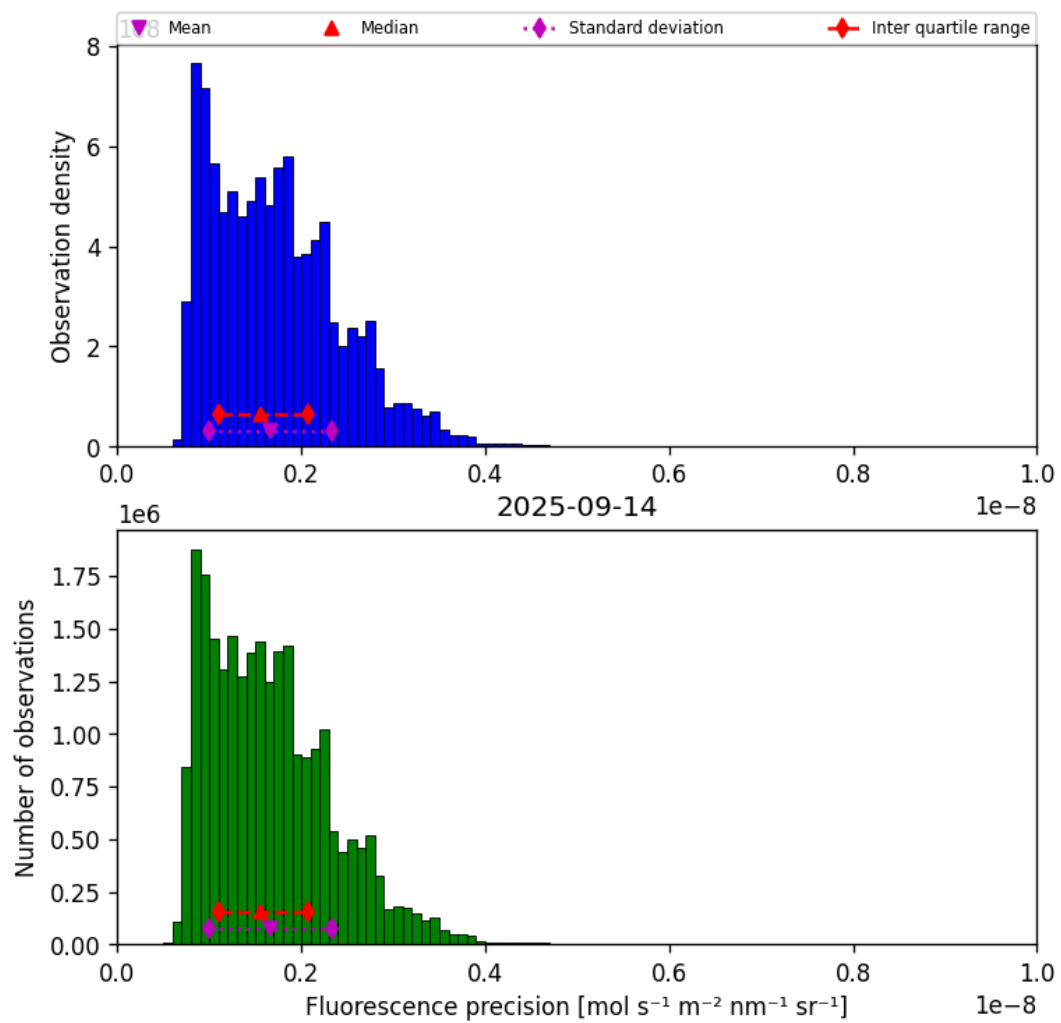
Figure 39: Histogram of “Fluorescence precision” for 2025-09-14 to 2025-09-15
