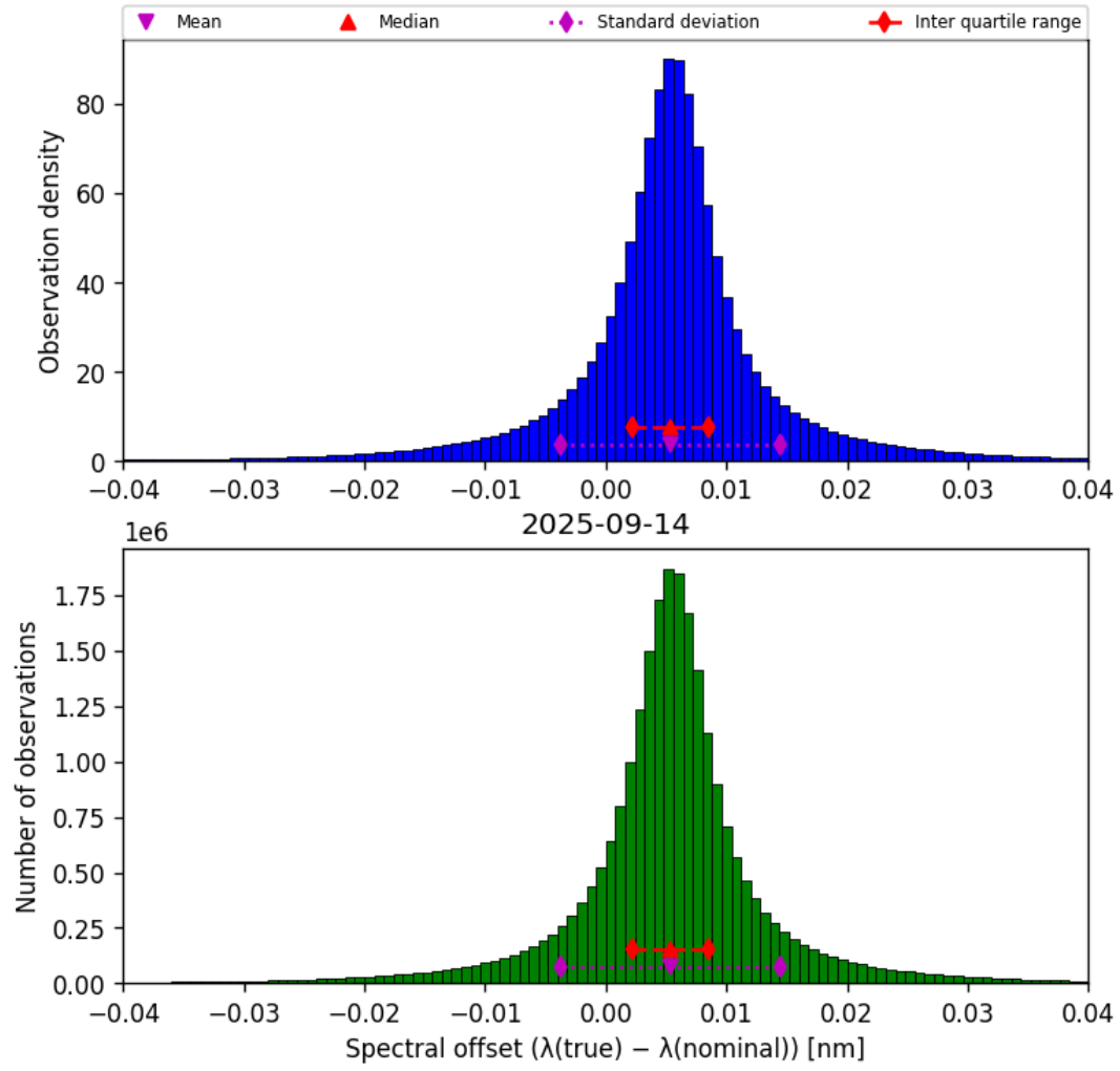
Figure 43: Histogram of “Spectral offset ( \lambda_{\text{true}} - \lambda_{\text{nominal}} )” for 2025-09-14 to 2025-09-15
