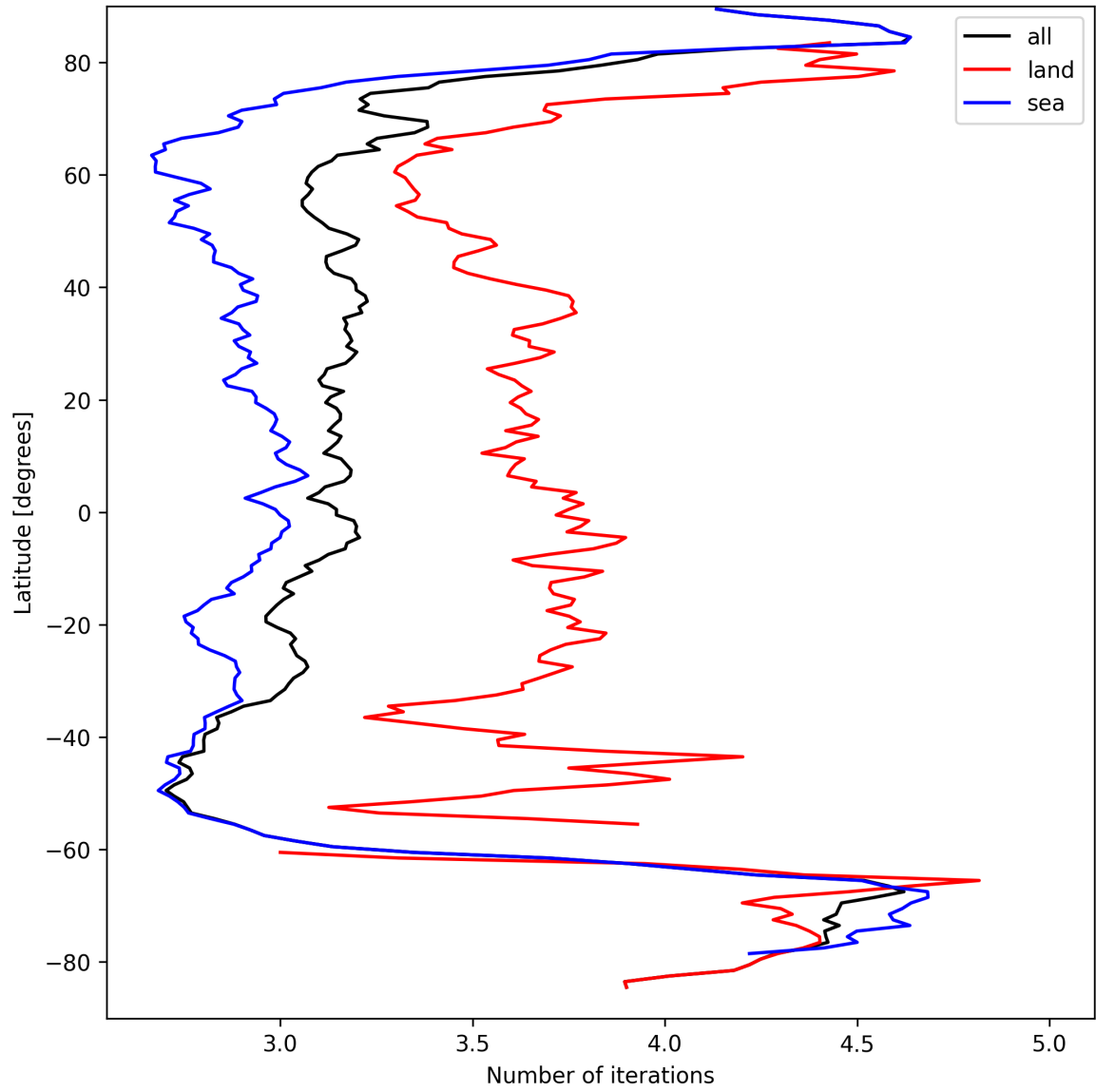
Figure 20: Zonal average of “Number of iterations” for 2025-09-14 to 2025-09-15.
