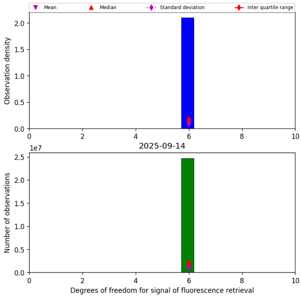
Figure 41: Histogram of “Degrees of freedom for signal of fluorescence retrieval” for 2025-09-14 to 2025-09-15
