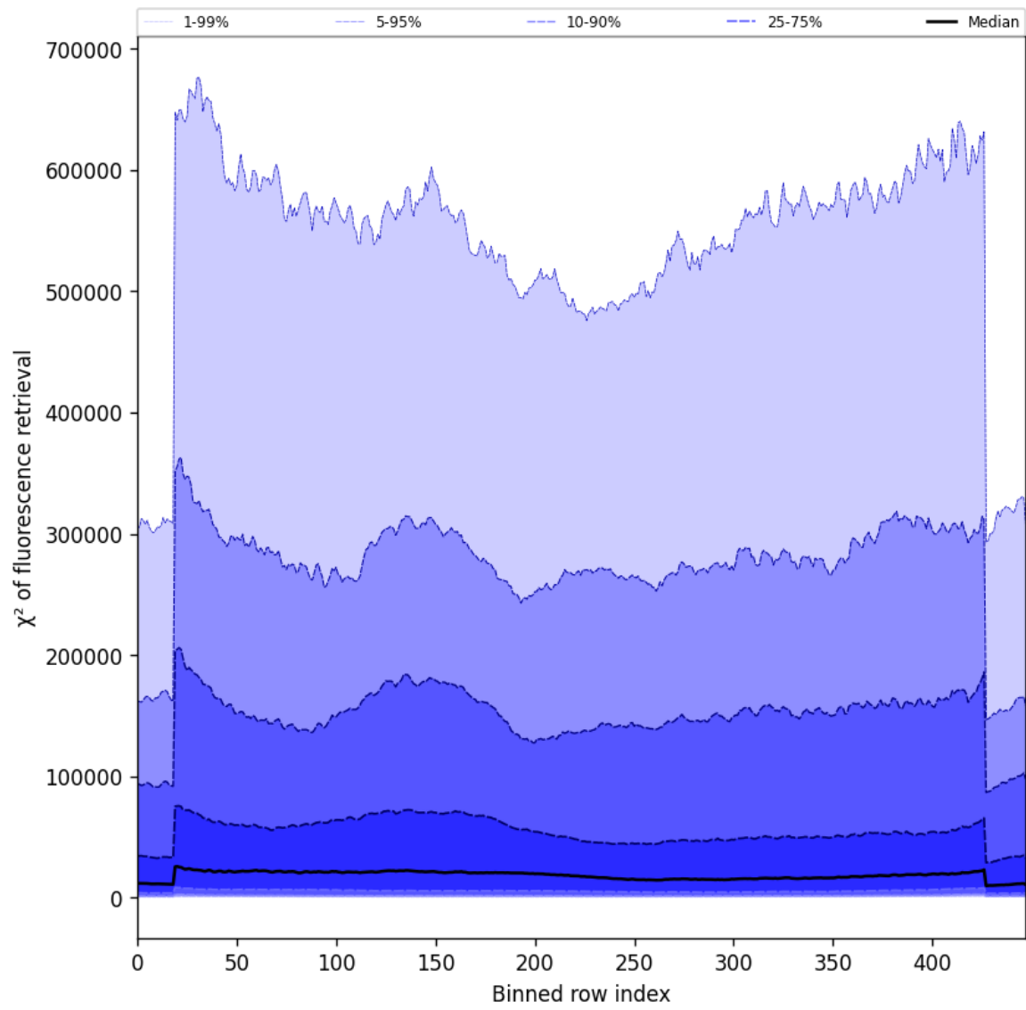
Figure 57: Along track statistics of “ \chi^2 of fluorescence retrieval” for 2025-09-14 to 2025-09-15
