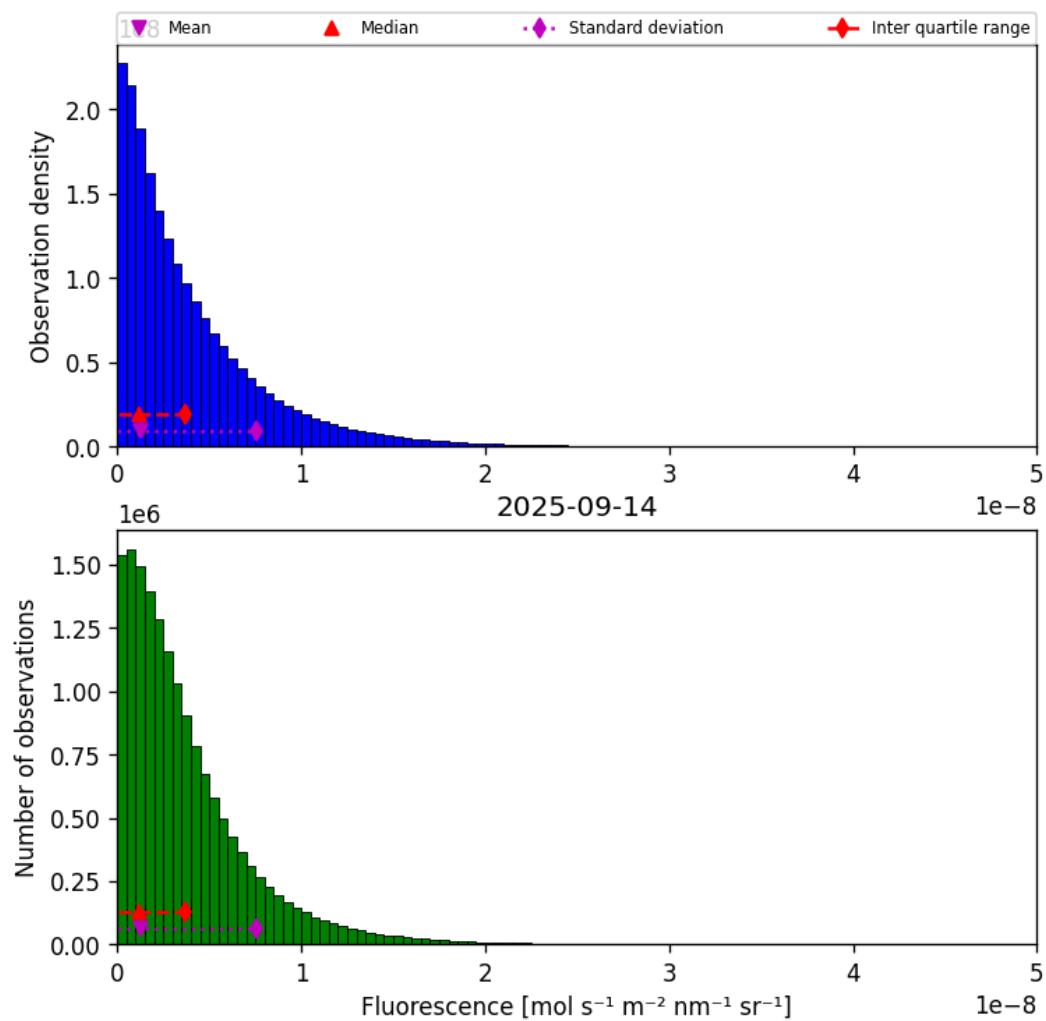
Figure 38: Histogram of “Fluorescence” for 2025-09-14 to 2025-09-15
