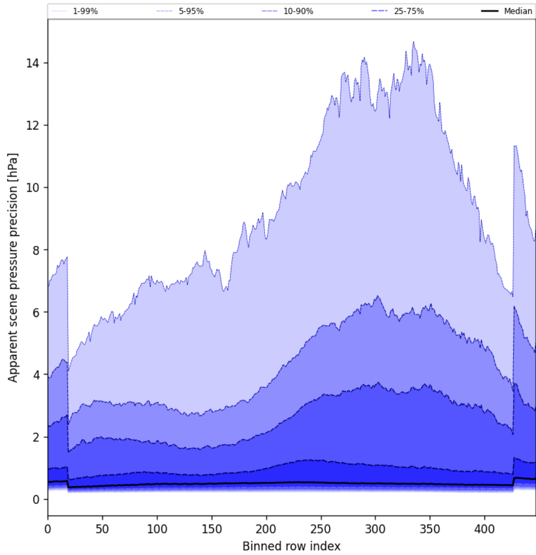
Figure 52: Along track statistics of “Apparent scene pressure precision” for 2025-09-14 to 2025-09-15
