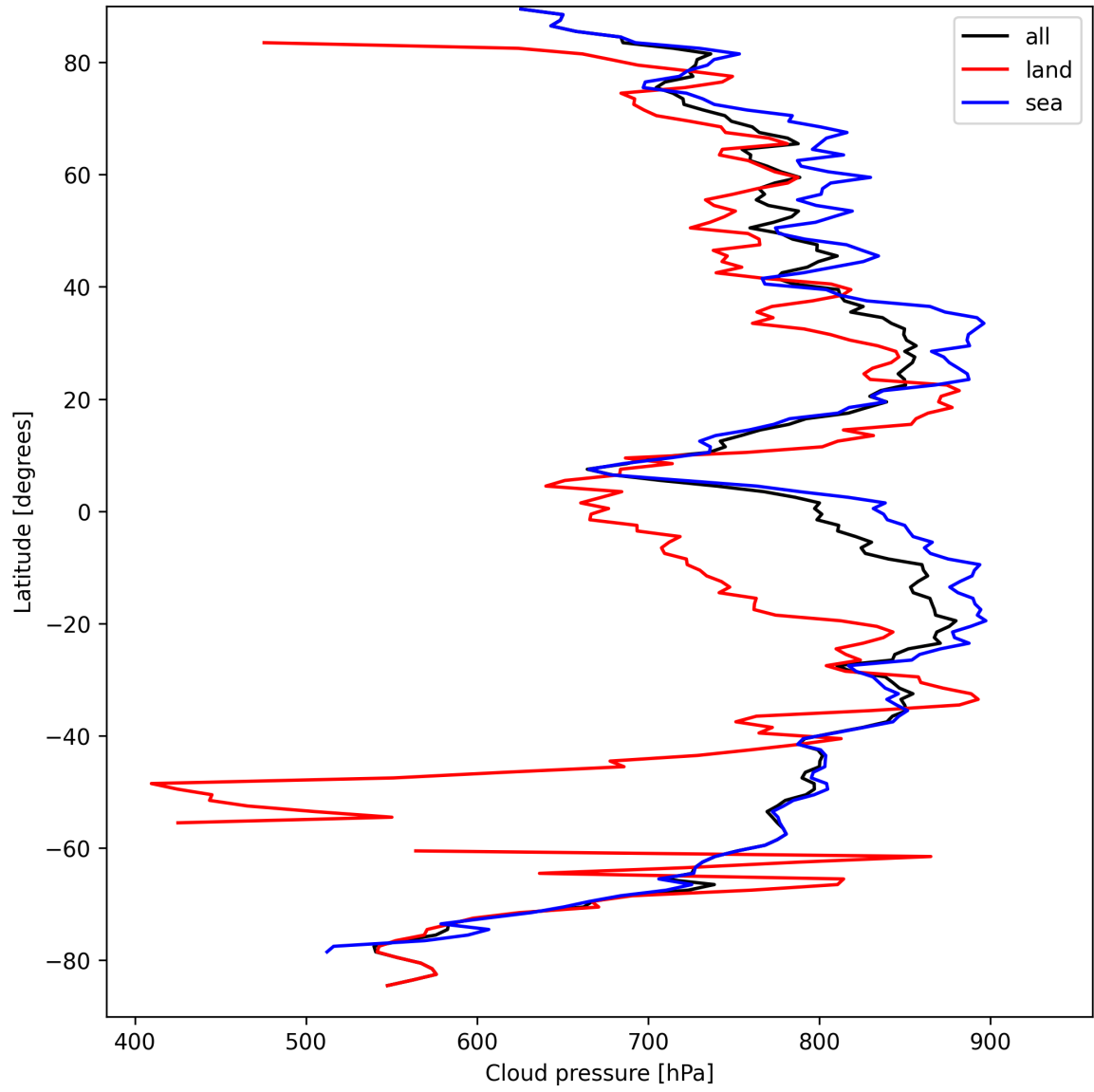
Figure 11: Zonal average of “Cloud pressure” for 2025-09-14 to 2025-09-15.
