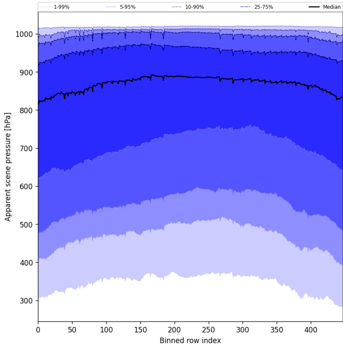
Figure 51: Along track statistics of “Apparent scene pressure” for 2025-09-14 to 2025-09-15
