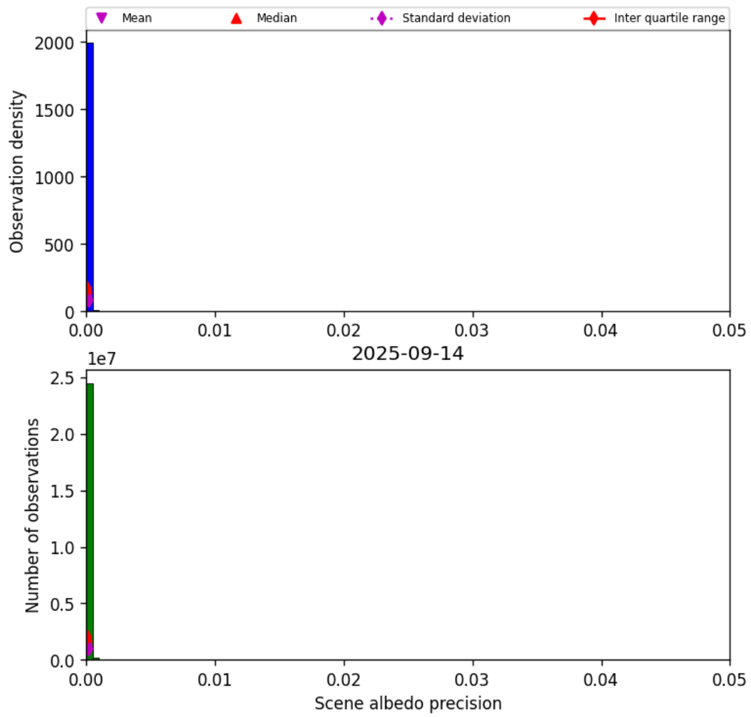
Figure 33: Histogram of “Scene albedo precision” for 2025-09-14 to 2025-09-15
