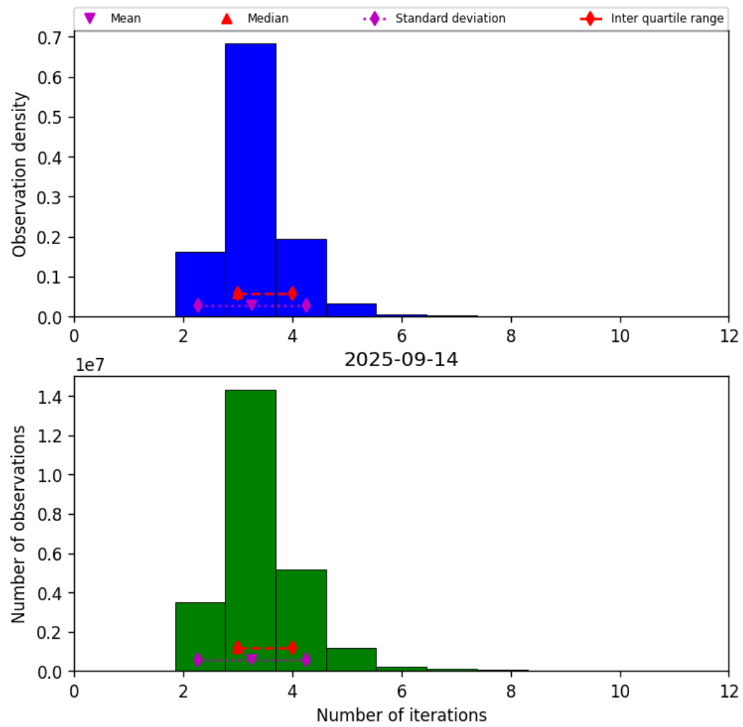
Figure 37: Histogram of “Number of iterations” for 2025-09-14 to 2025-09-15
