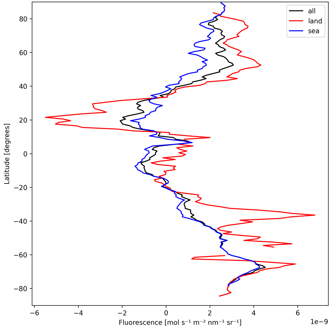
Figure 21: Zonal average of “Fluorescence” for 2025-09-14 to 2025-09-15.
