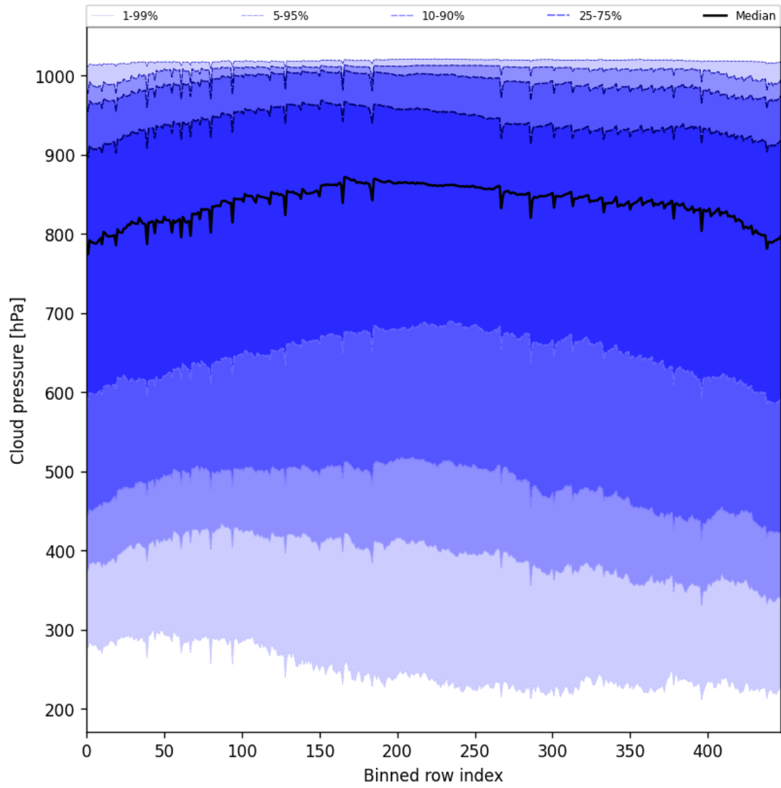
Figure 45: Along track statistics of “Cloud pressure” for 2025-09-14 to 2025-09-15
