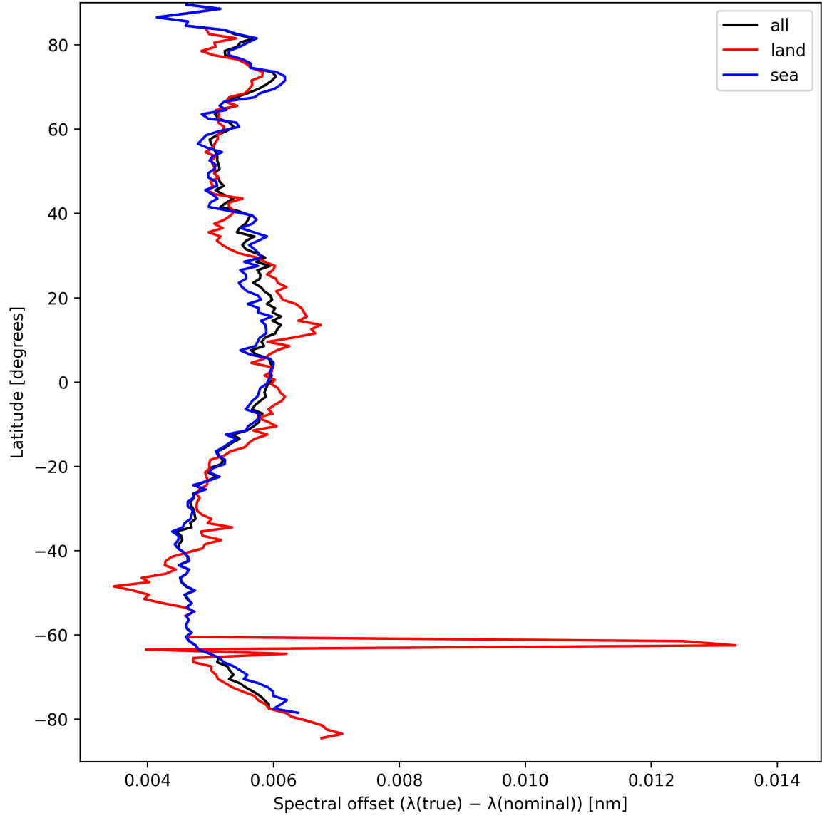
Figure 26: Zonal average of “Spectral offset ( \lambda_{\text{true}} - \lambda_{\text{nominal}} )” for 2025-09-14 to 2025-09-15.
