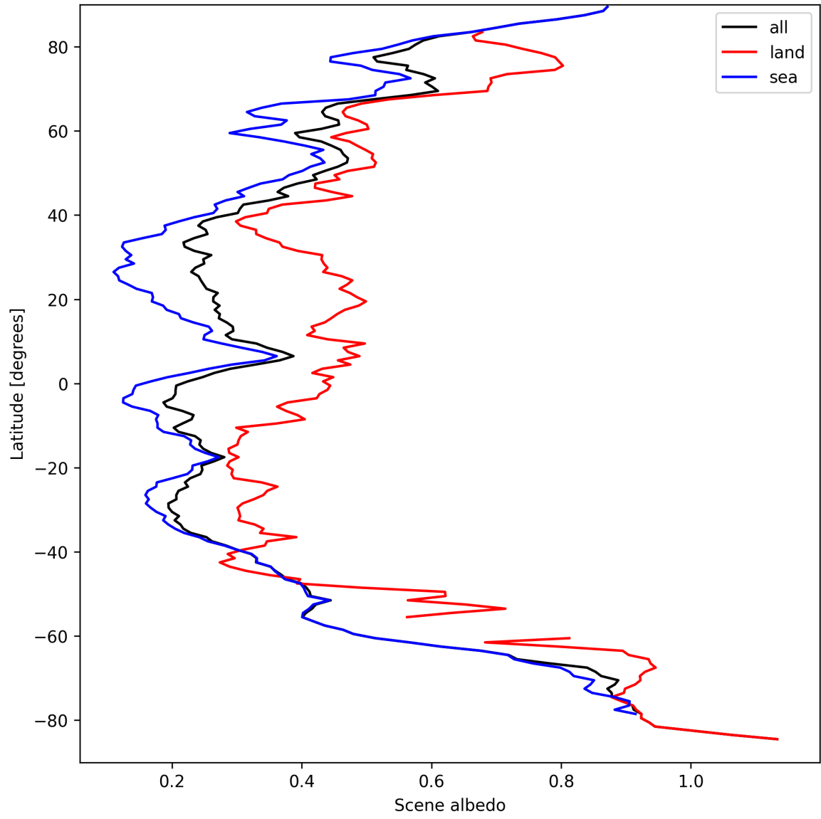
Figure 15: Zonal average of “Scene albedo” for 2025-09-14 to 2025-09-15.
