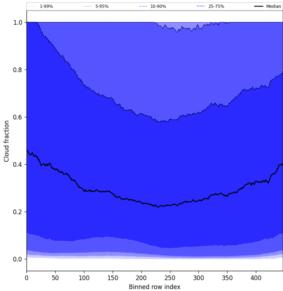
Figure 47: Along track statistics of “Cloud fraction” for 2025-09-14 to 2025-09-15
