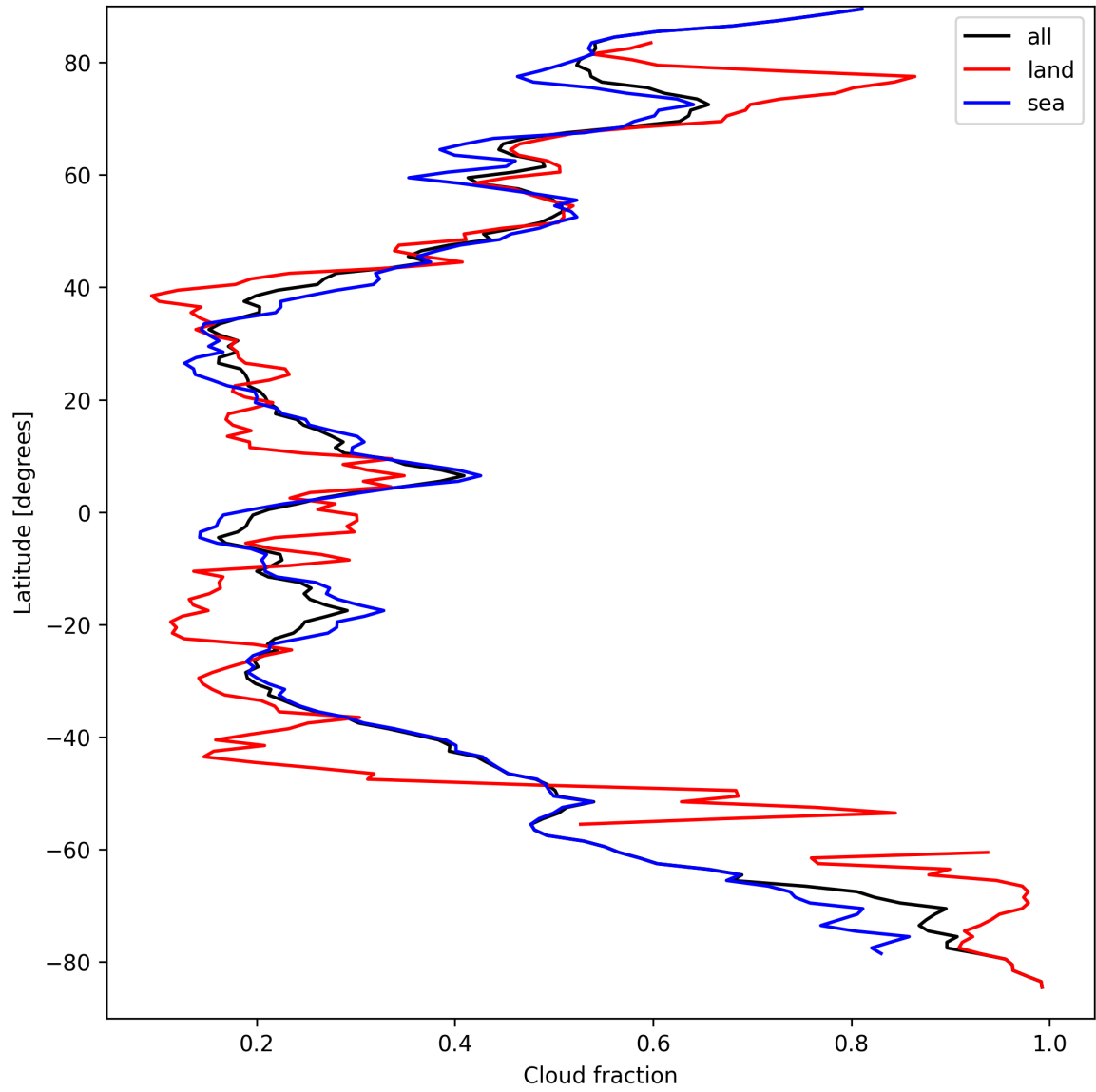
Figure 13: Zonal average of “Cloud fraction” for 2025-09-14 to 2025-09-15.
