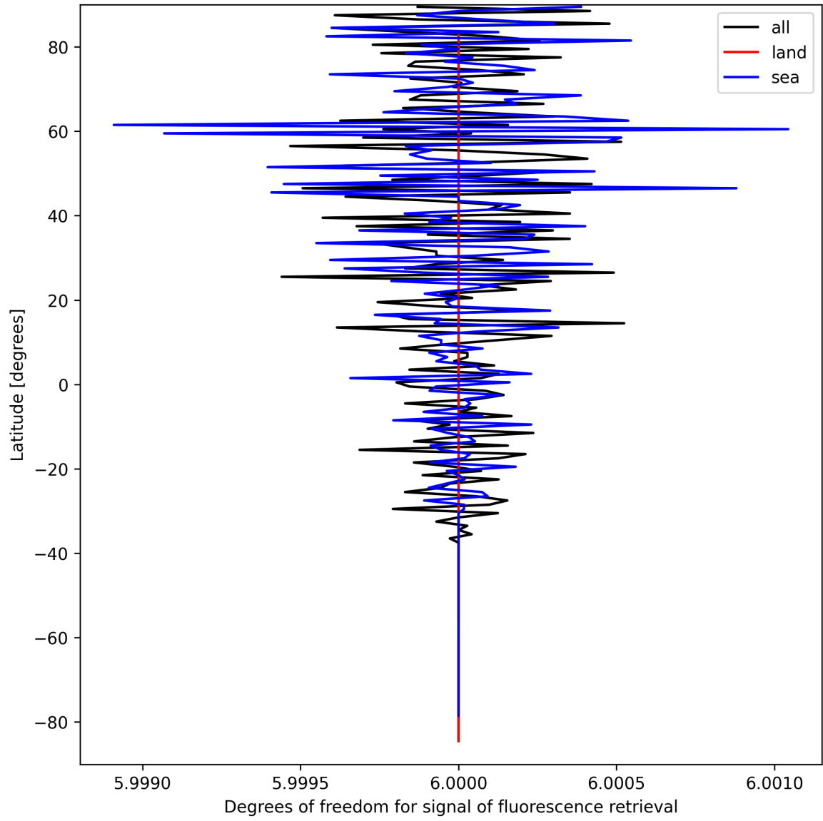
Figure 24: Zonal average of “Degrees of freedom for signal of fluorescence retrieval” for 2025-09-14 to 2025-09-15.
