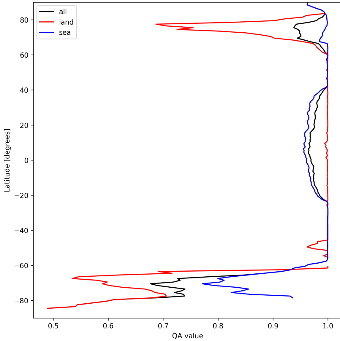
Figure 10: Zonal average of "QA value" for 2025-09-14 to 2025-09-15.
