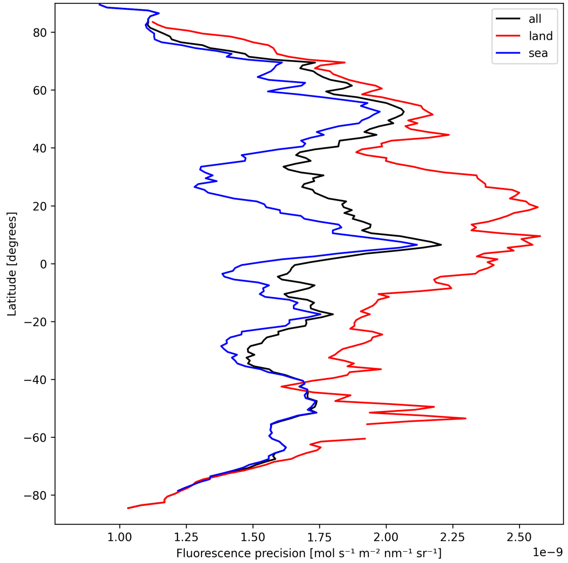
Figure 22: Zonal average of “Fluorescence precision” for 2025-09-14 to 2025-09-15.
