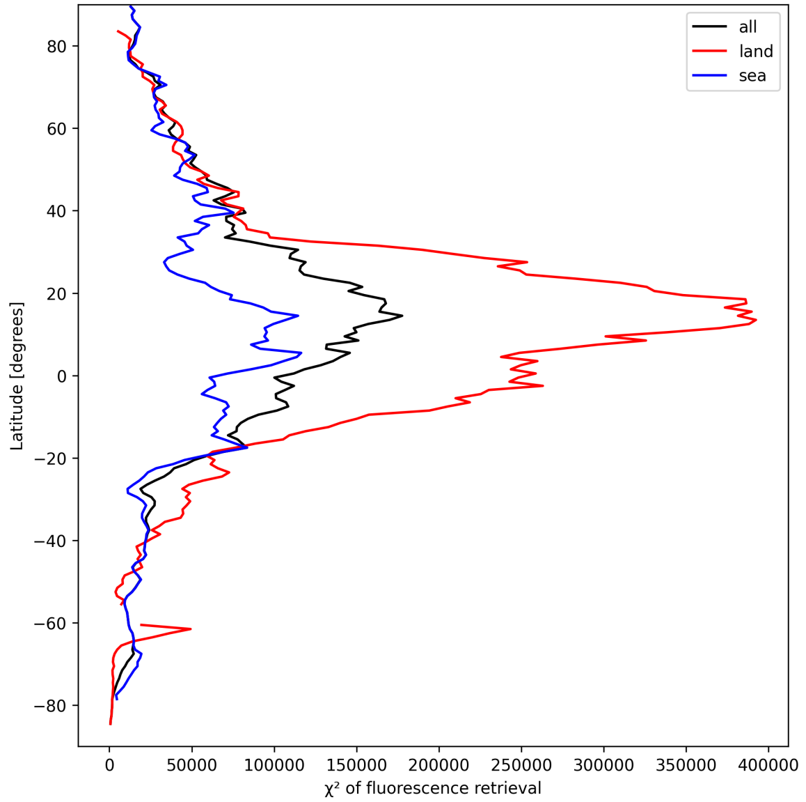
Figure 23: Zonal average of “ \chi^2 of fluorescence retrieval” for 2025-09-14 to 2025-09-15.
