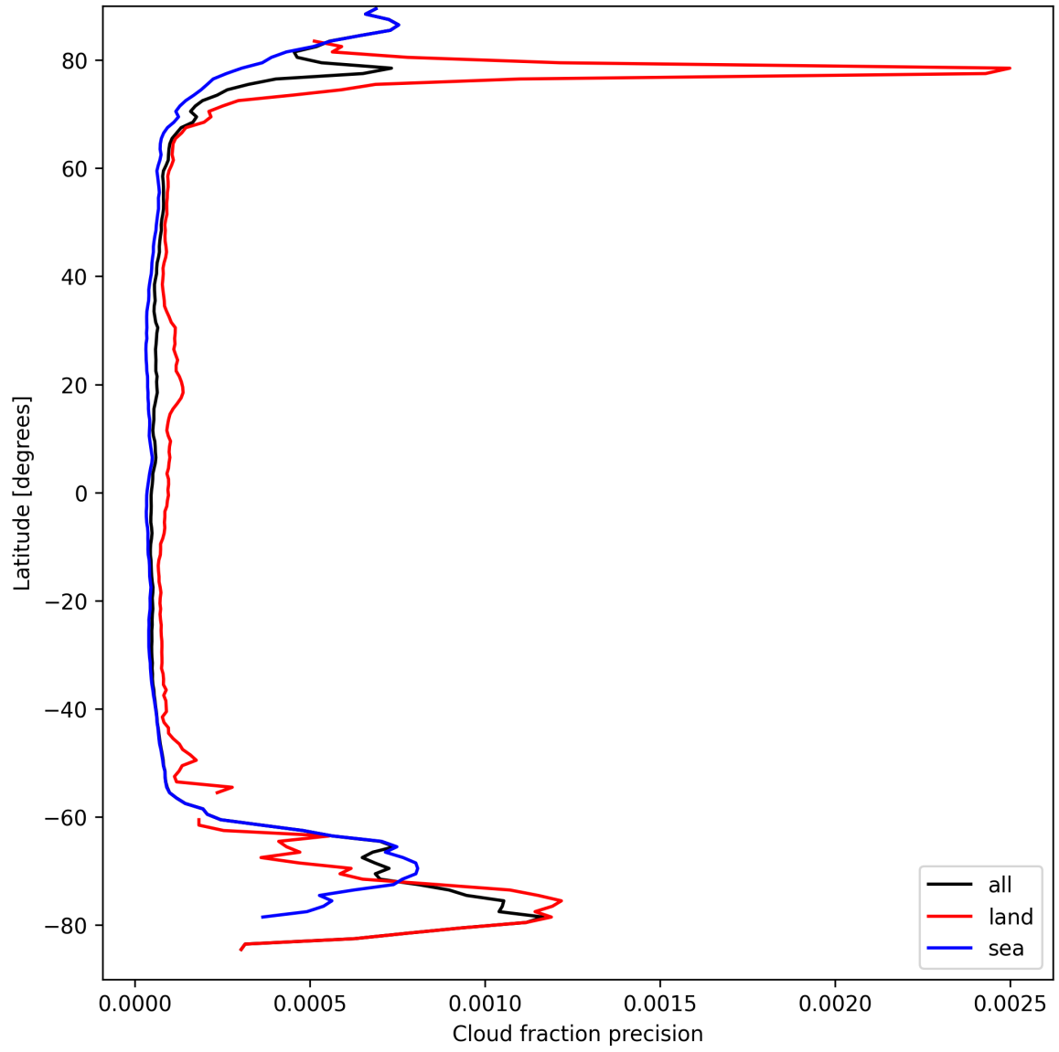
Figure 14: Zonal average of “Cloud fraction precision” for 2025-09-14 to 2025-09-15.
