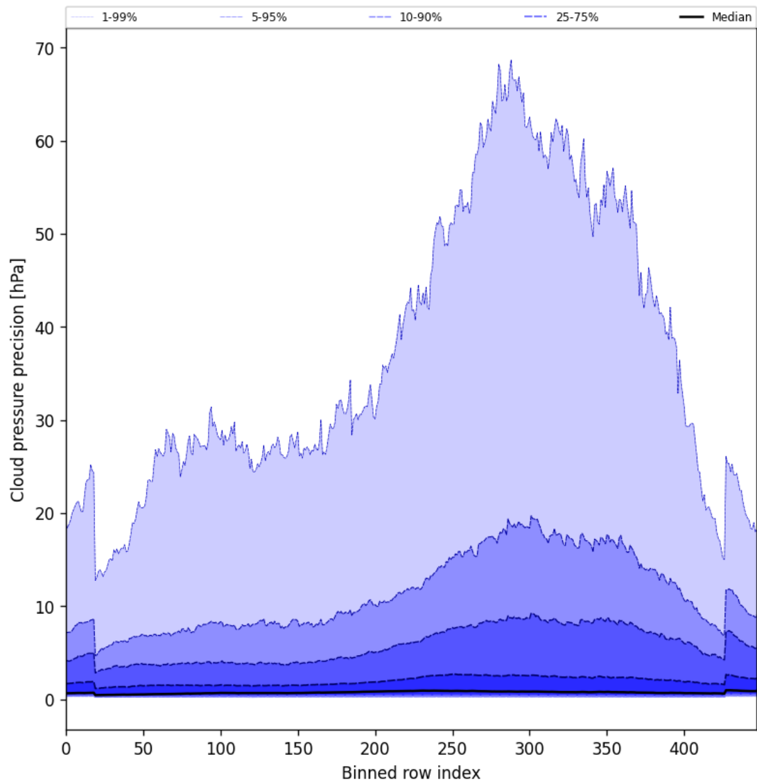
Figure 46: Along track statistics of “Cloud pressure precision” for 2025-09-14 to 2025-09-15
