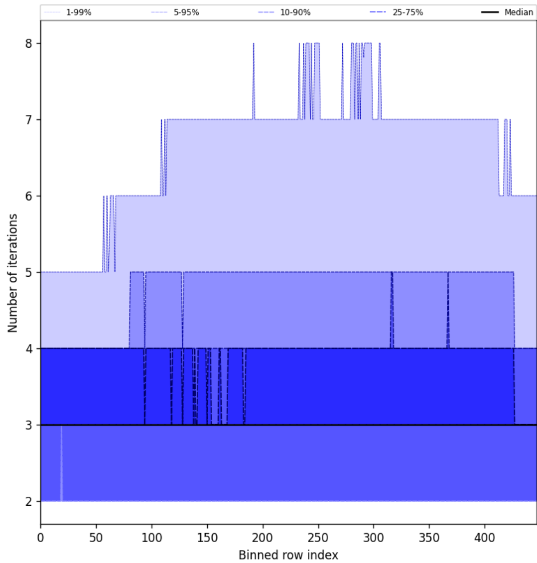
Figure 54: Along track statistics of “Number of iterations” for 2025-09-14 to 2025-09-15
