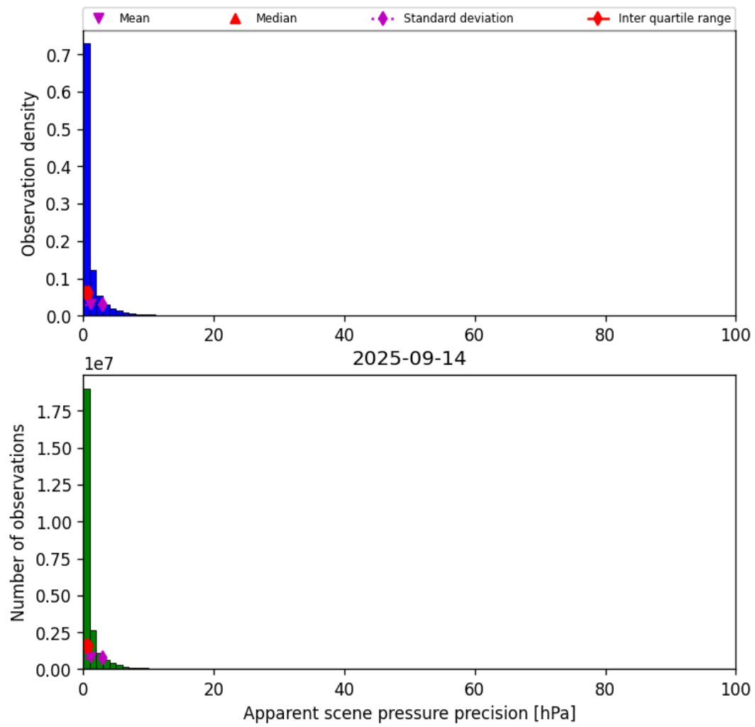
Figure 35: Histogram of “Apparent scene pressure precision” for 2025-09-14 to 2025-09-15
