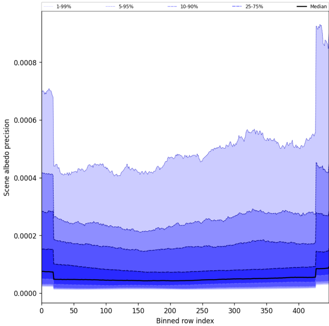
Figure 50: Along track statistics of “Scene albedo precision” for 2025-09-14 to 2025-09-15
