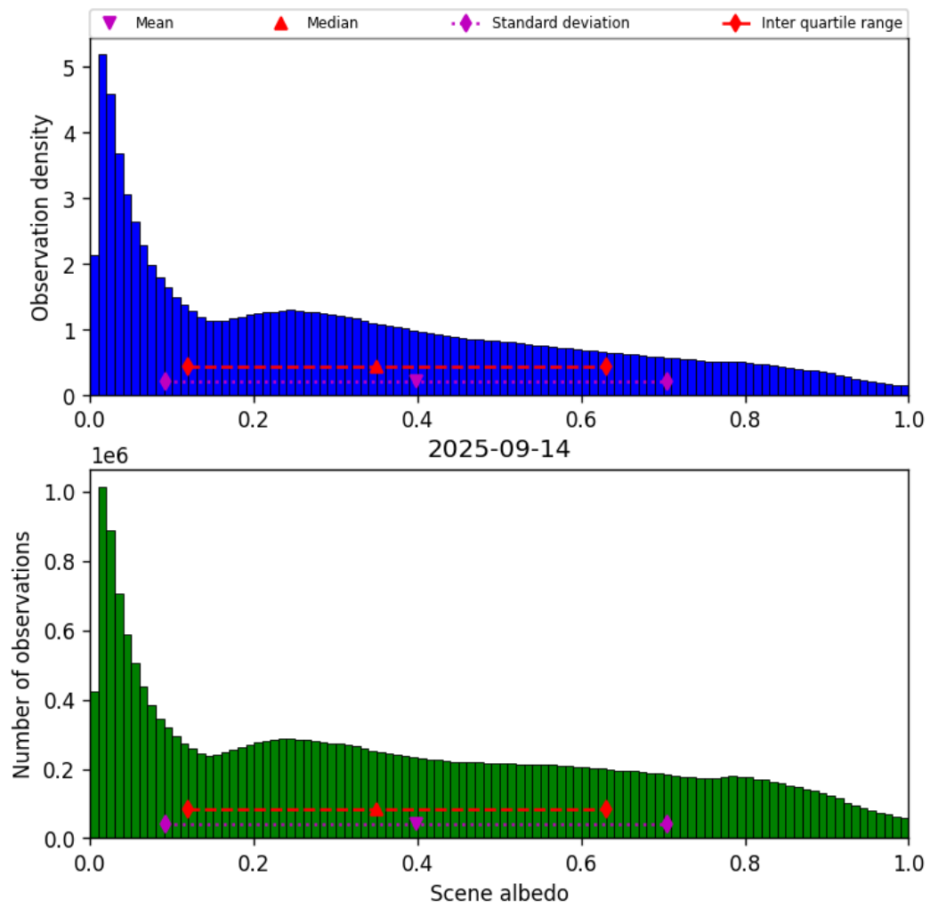
Figure 32: Histogram of “Scene albedo” for 2025-09-14 to 2025-09-15
