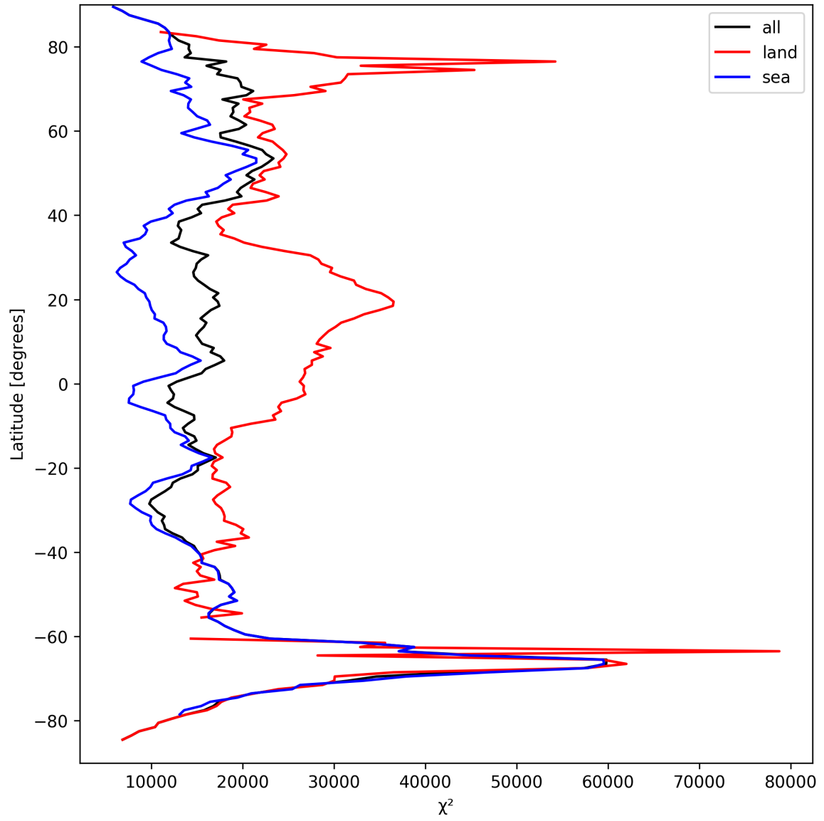
Figure 19: Zonal average of “ \chi^2 ” for 2025-09-14 to 2025-09-15.
