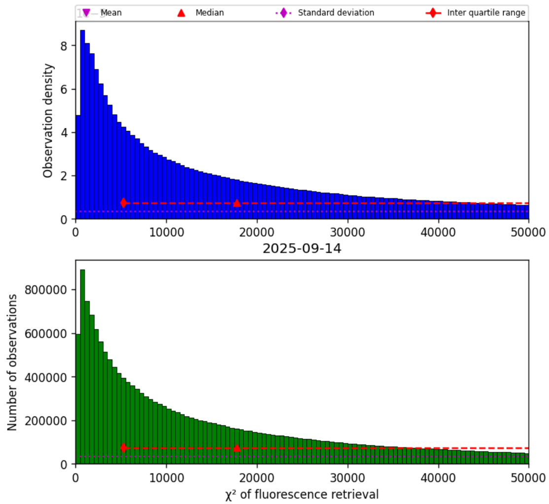
Figure 40: Histogram of “ \chi^2 of fluorescence retrieval” for 2025-09-14 to 2025-09-15
