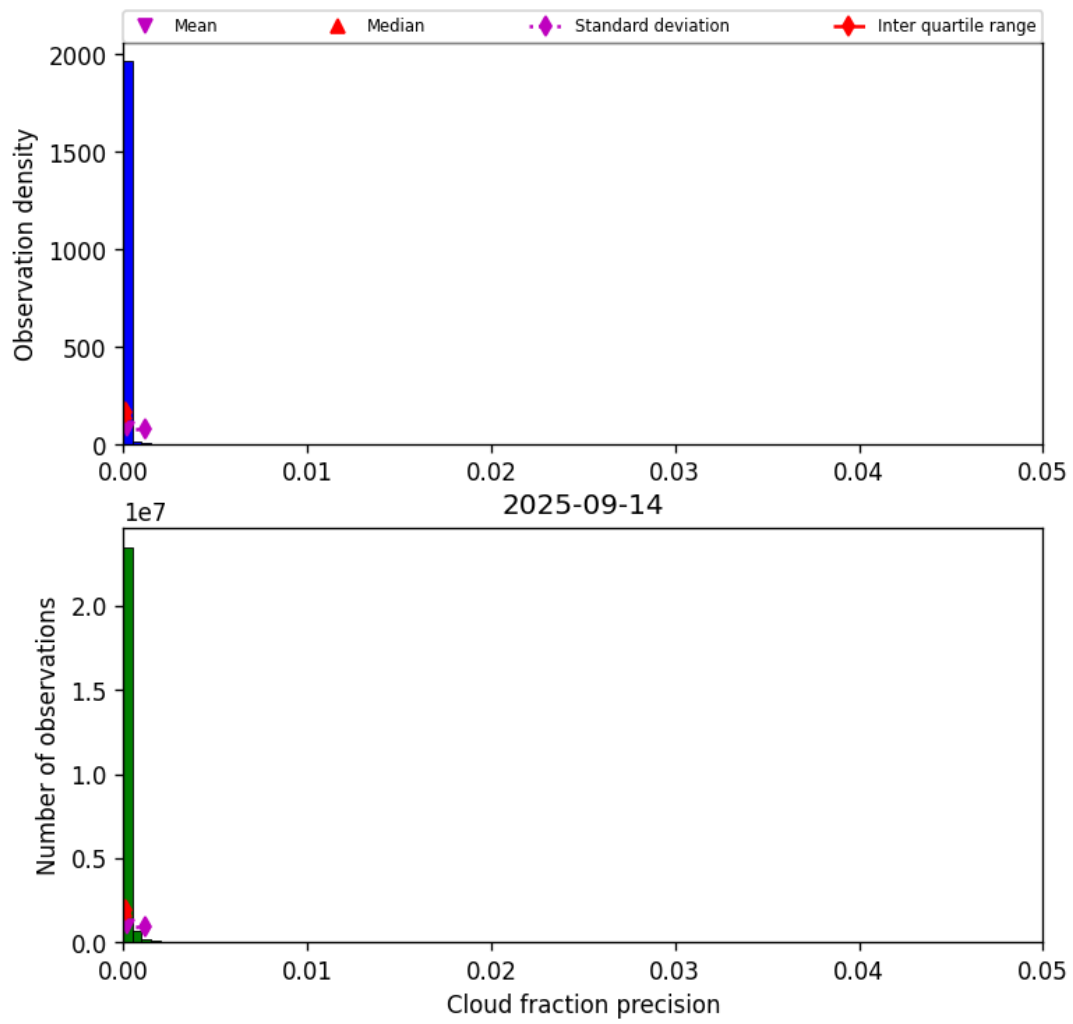
Figure 31: Histogram of “Cloud fraction precision” for 2025-09-14 to 2025-09-15
