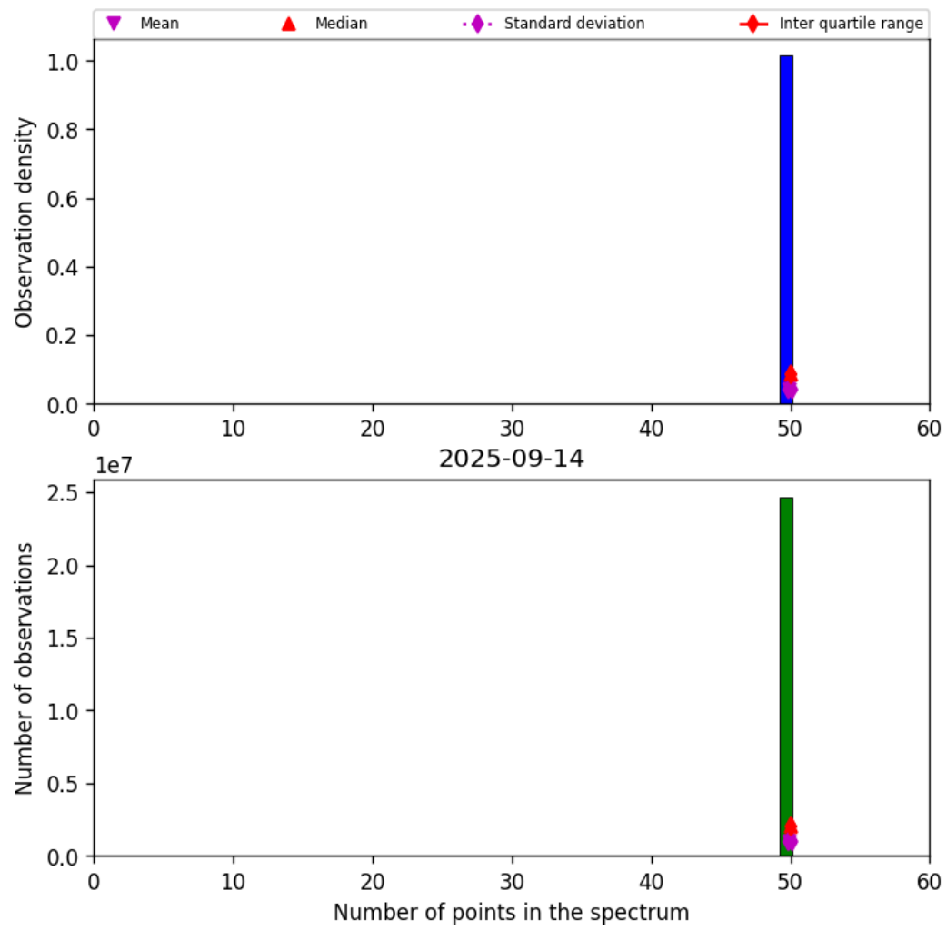
Figure 42: Histogram of "Number of points in the spectrum" for 2025-09-14 to 2025-09-15
