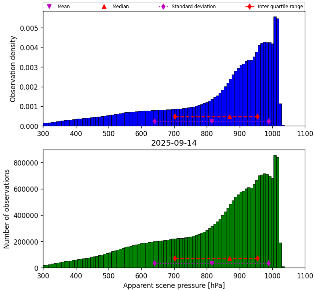
Figure 34: Histogram of “Apparent scene pressure” for 2025-09-14 to 2025-09-15
