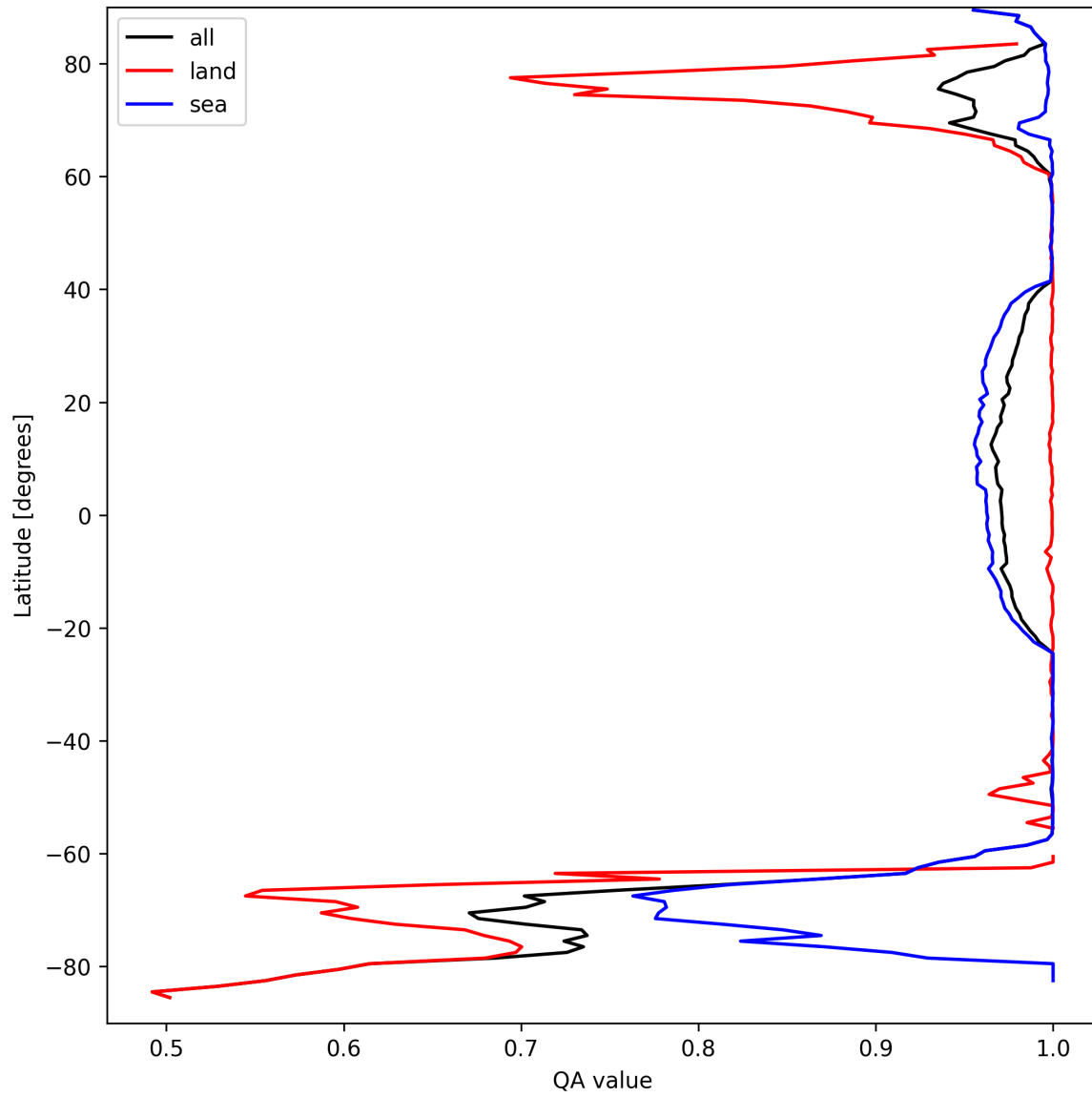
Figure 10: Zonal average of "QA value" for 2025-09-15 to 2025-09-16.
