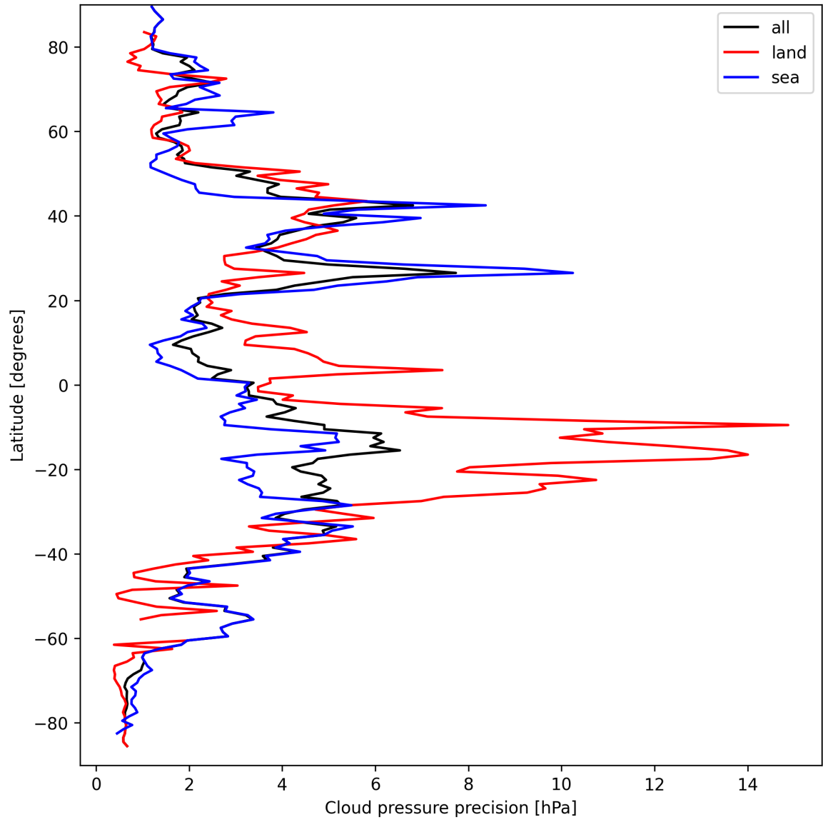
Figure 12: Zonal average of “Cloud pressure precision” for 2025-09-15 to 2025-09-16.
