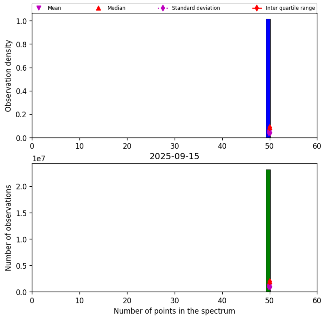
Figure 42: Histogram of “Number of points in the spectrum” for 2025-09-15 to 2025-09-16
