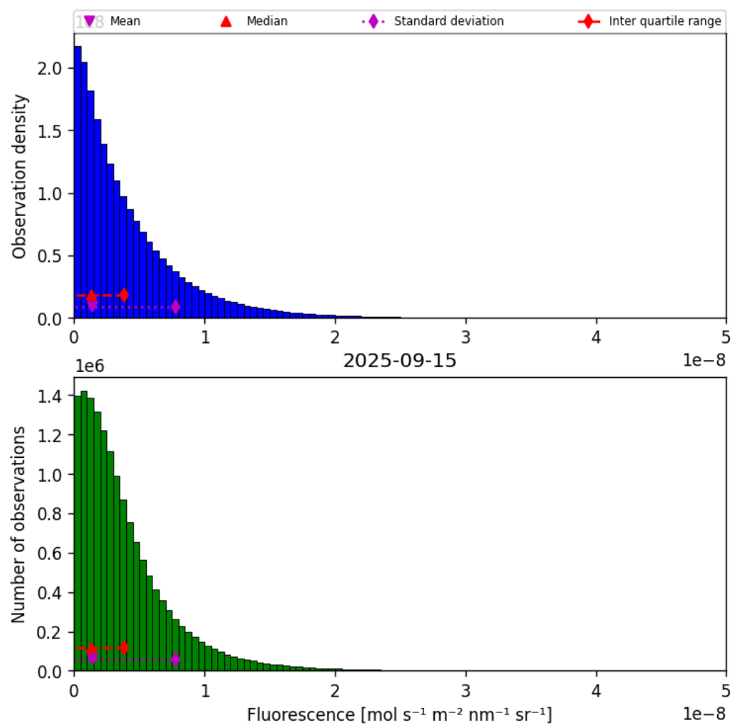
Figure 38: Histogram of “Fluorescence” for 2025-09-15 to 2025-09-16
