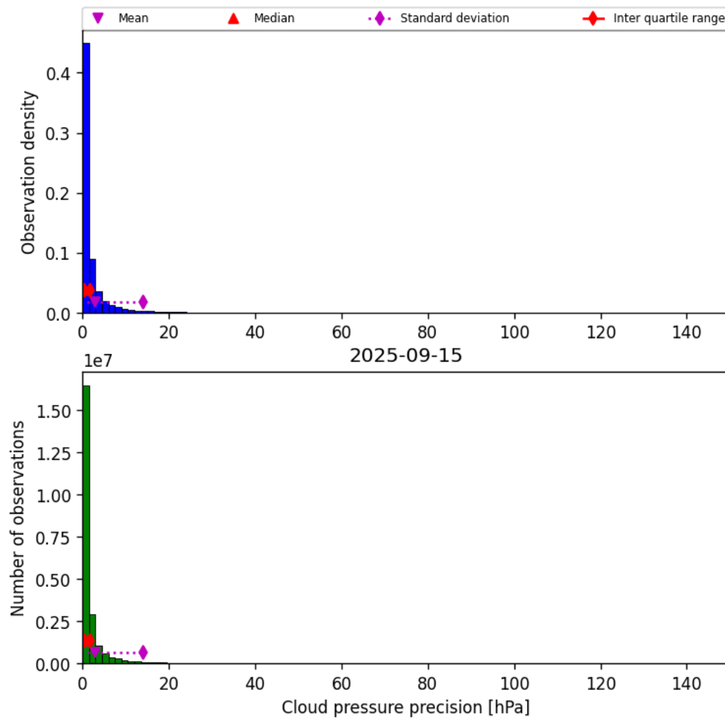
Figure 29: Histogram of “Cloud pressure precision” for 2025-09-15 to 2025-09-16
