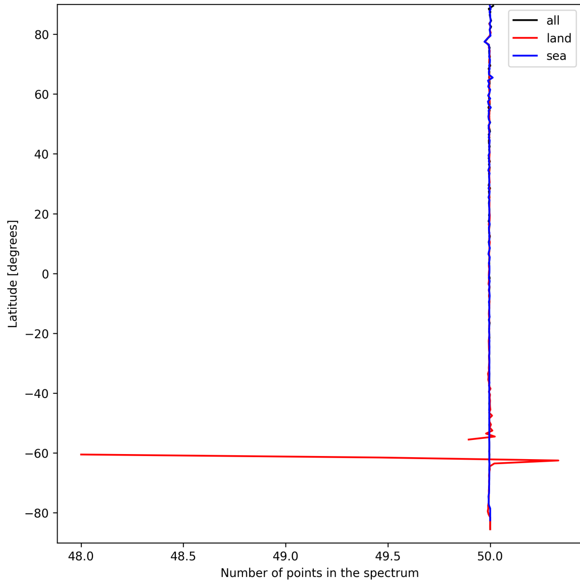
Figure 25: Zonal average of “Number of points in the spectrum” for 2025-09-15 to 2025-09-16.
