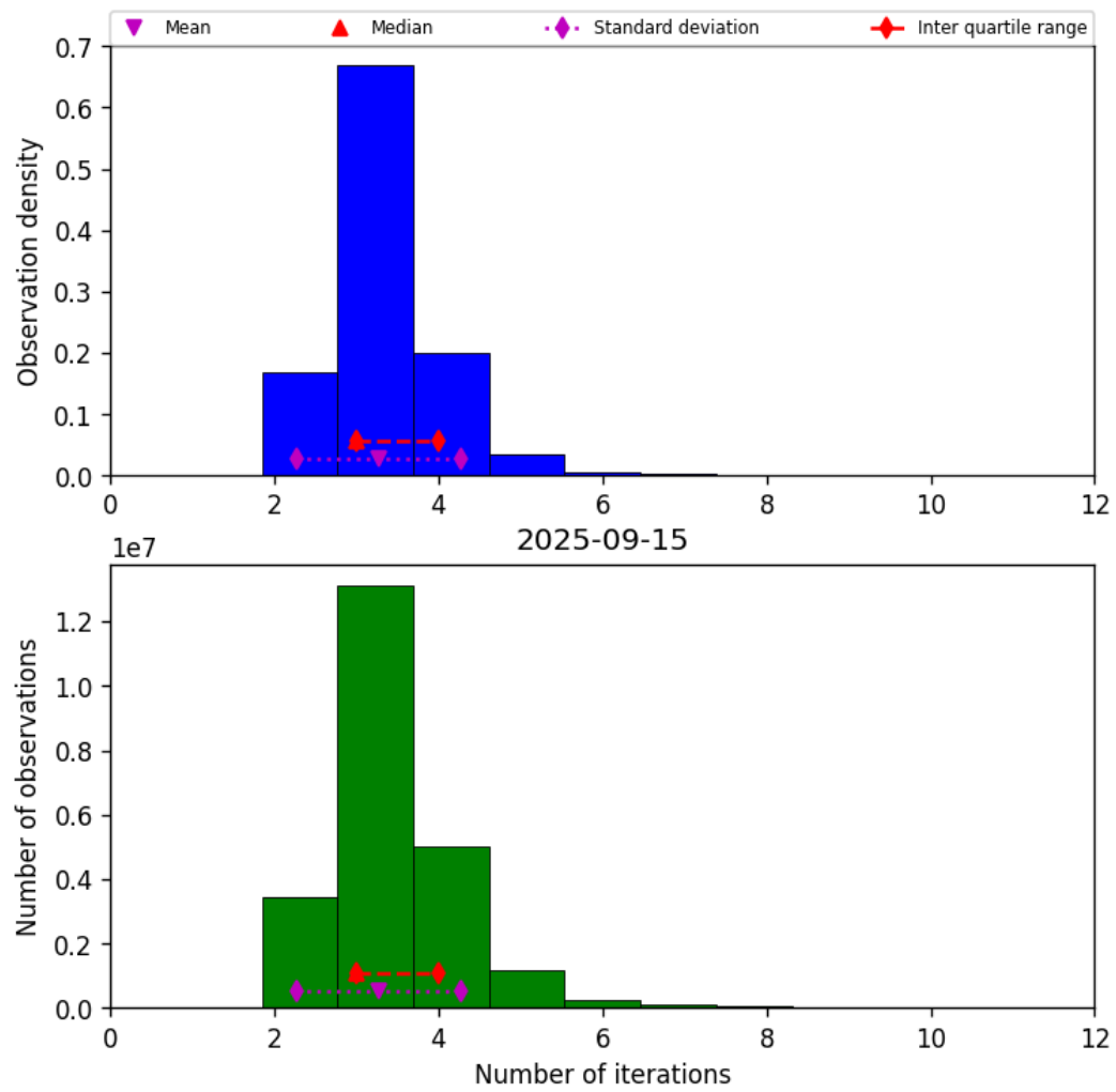
Figure 37: Histogram of “Number of iterations” for 2025-09-15 to 2025-09-16
