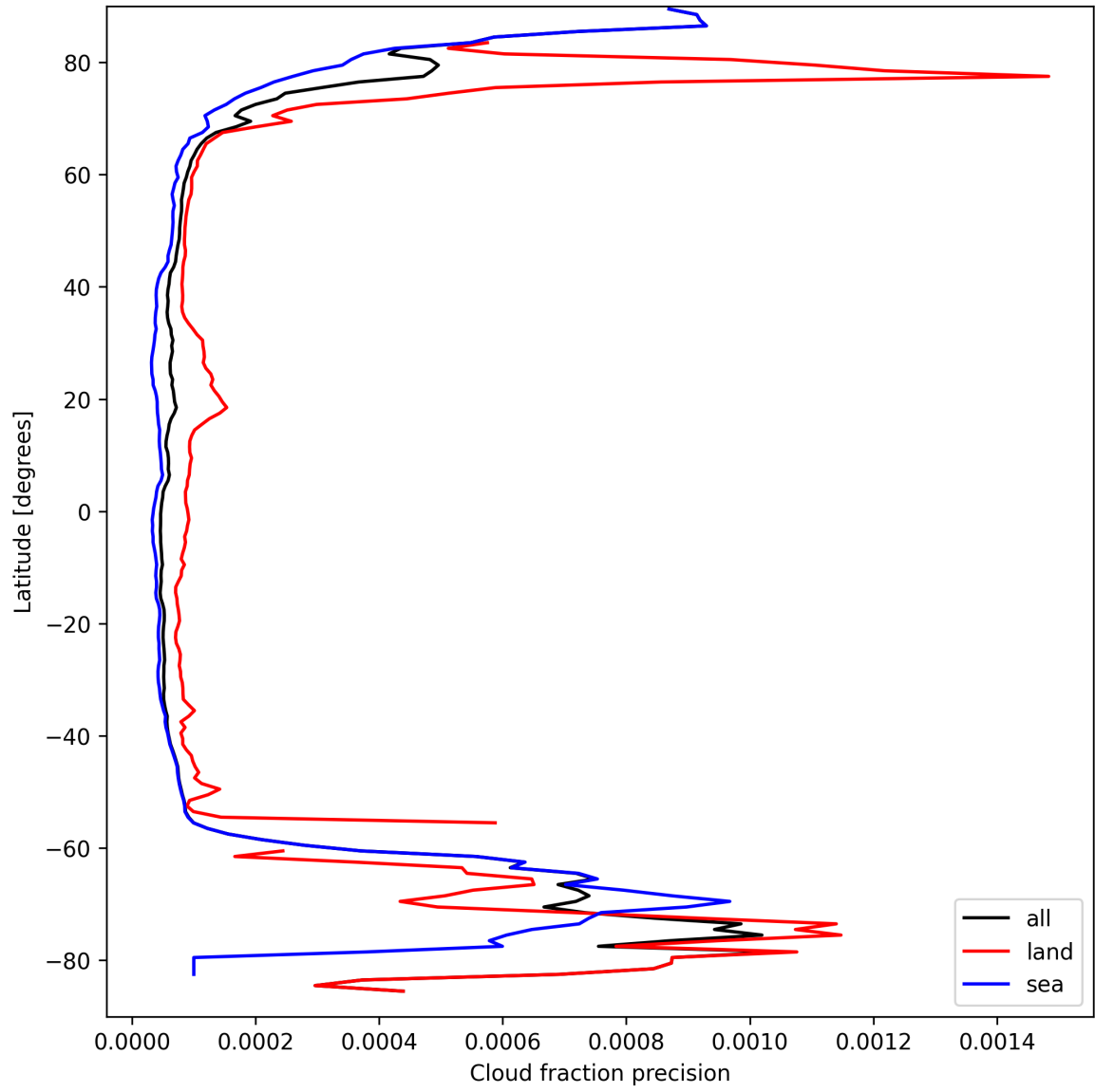
Figure 14: Zonal average of “Cloud fraction precision” for 2025-09-15 to 2025-09-16.
