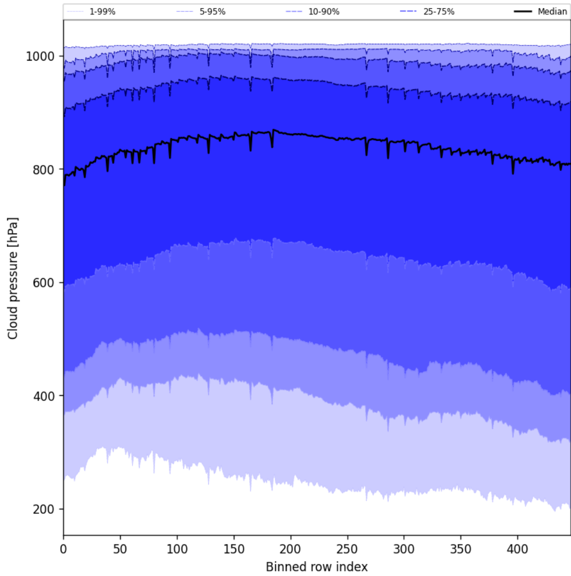
Figure 45: Along track statistics of “Cloud pressure” for 2025-09-15 to 2025-09-16
