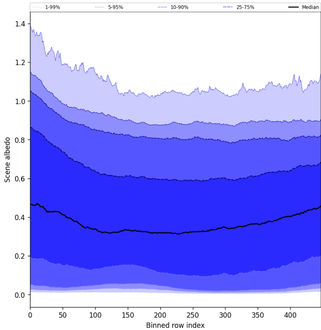
Figure 49: Along track statistics of “Scene albedo” for 2025-09-15 to 2025-09-16
