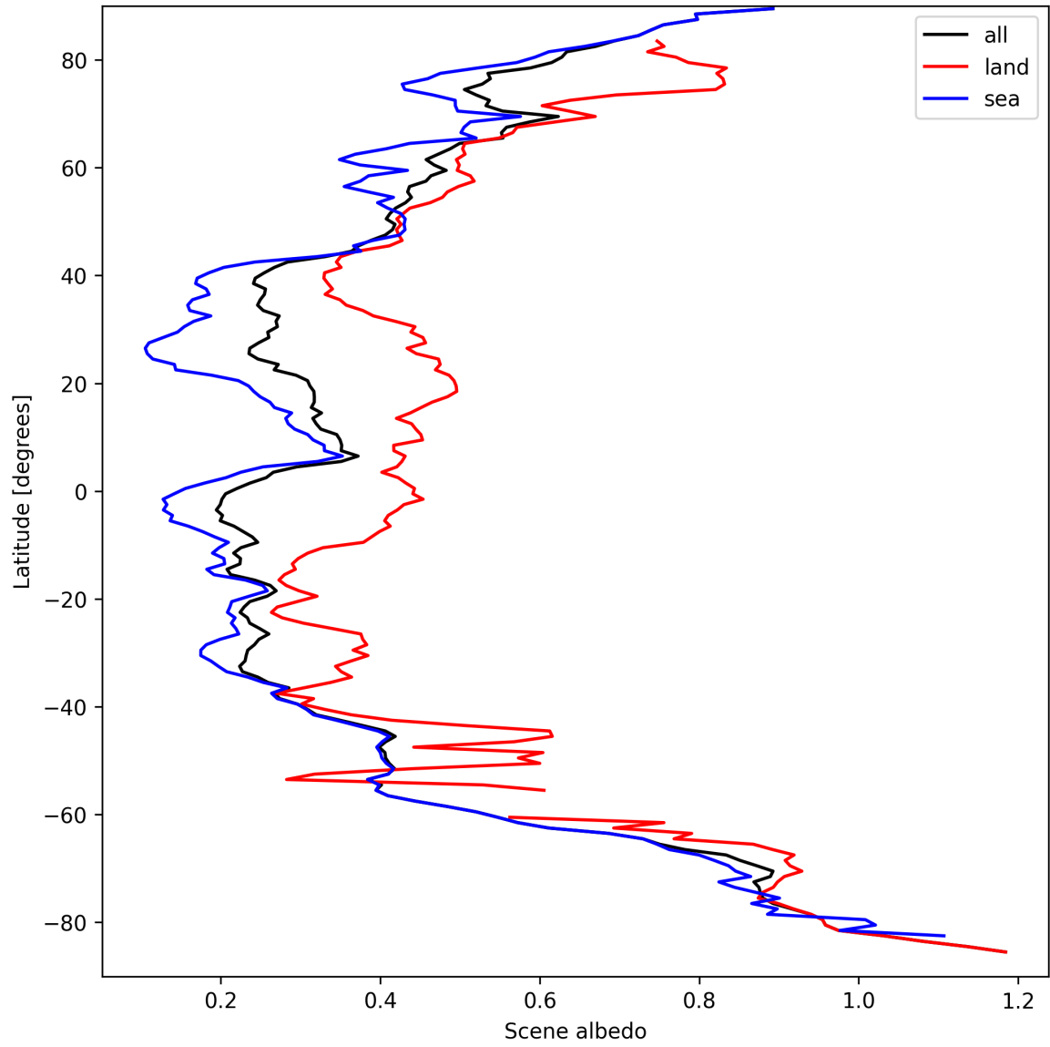
Figure 15: Zonal average of “Scene albedo” for 2025-09-15 to 2025-09-16.
