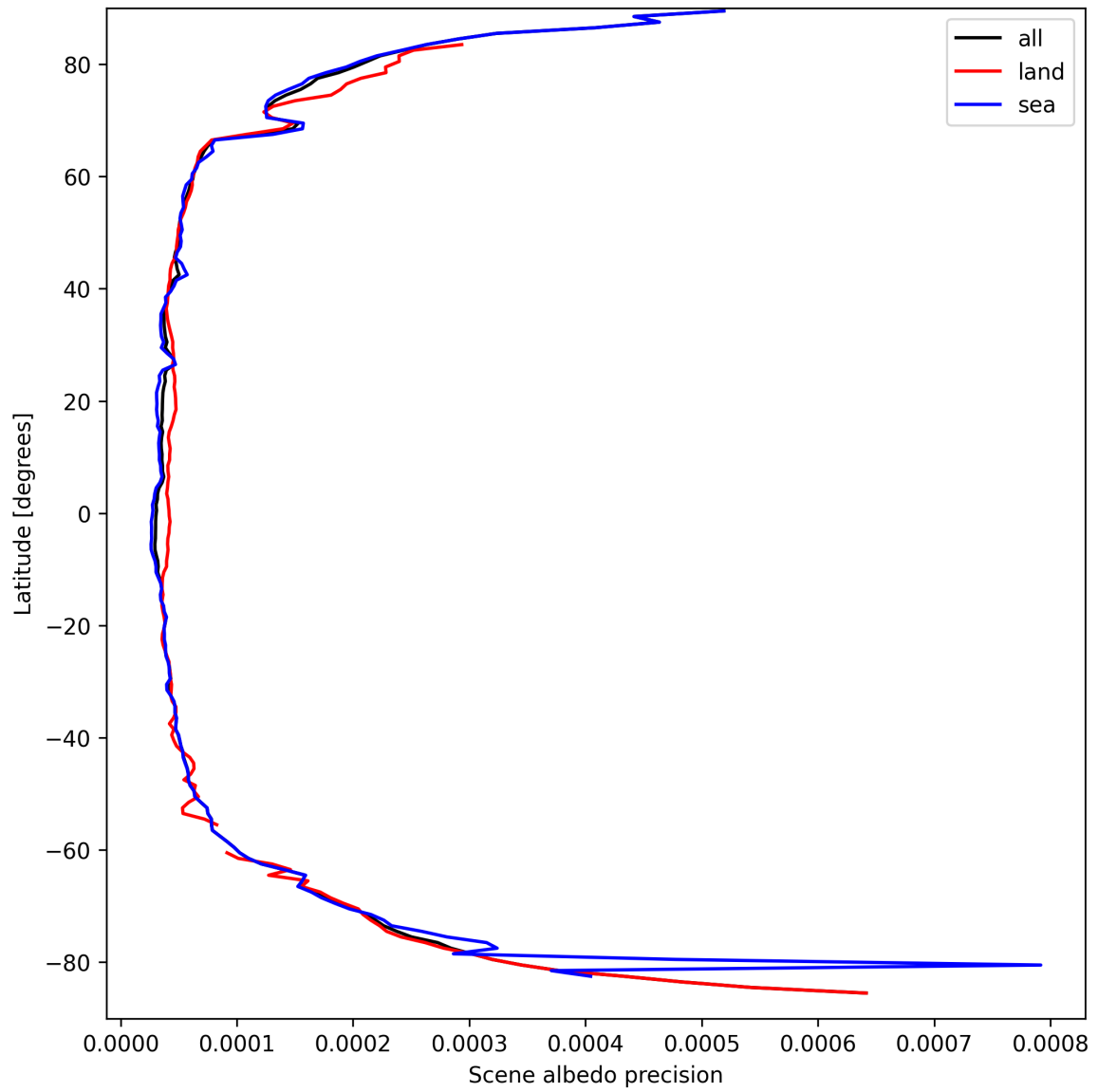
Figure 16: Zonal average of “Scene albedo precision” for 2025-09-15 to 2025-09-16.
