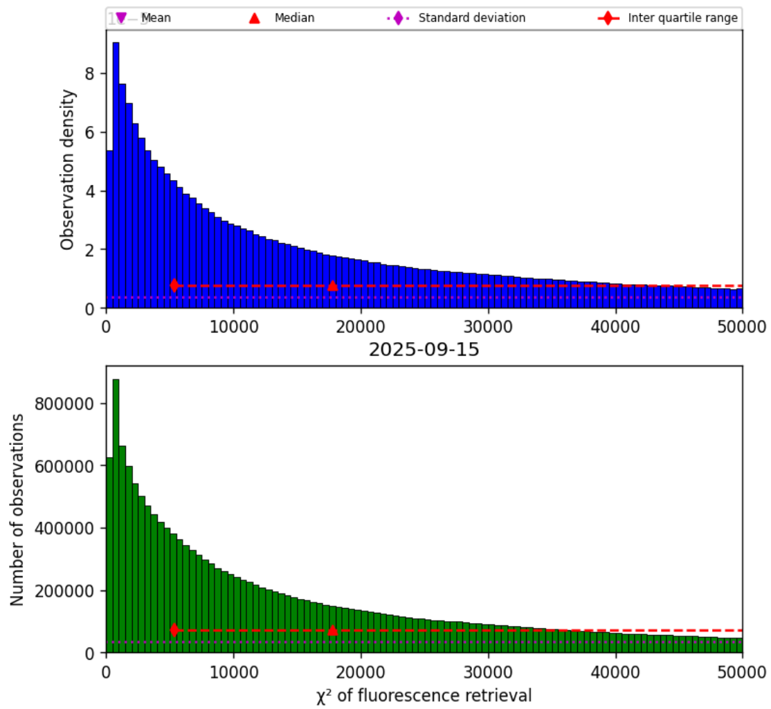
Figure 40: Histogram of “ \chi^2 of fluorescence retrieval” for 2025-09-15 to 2025-09-16
