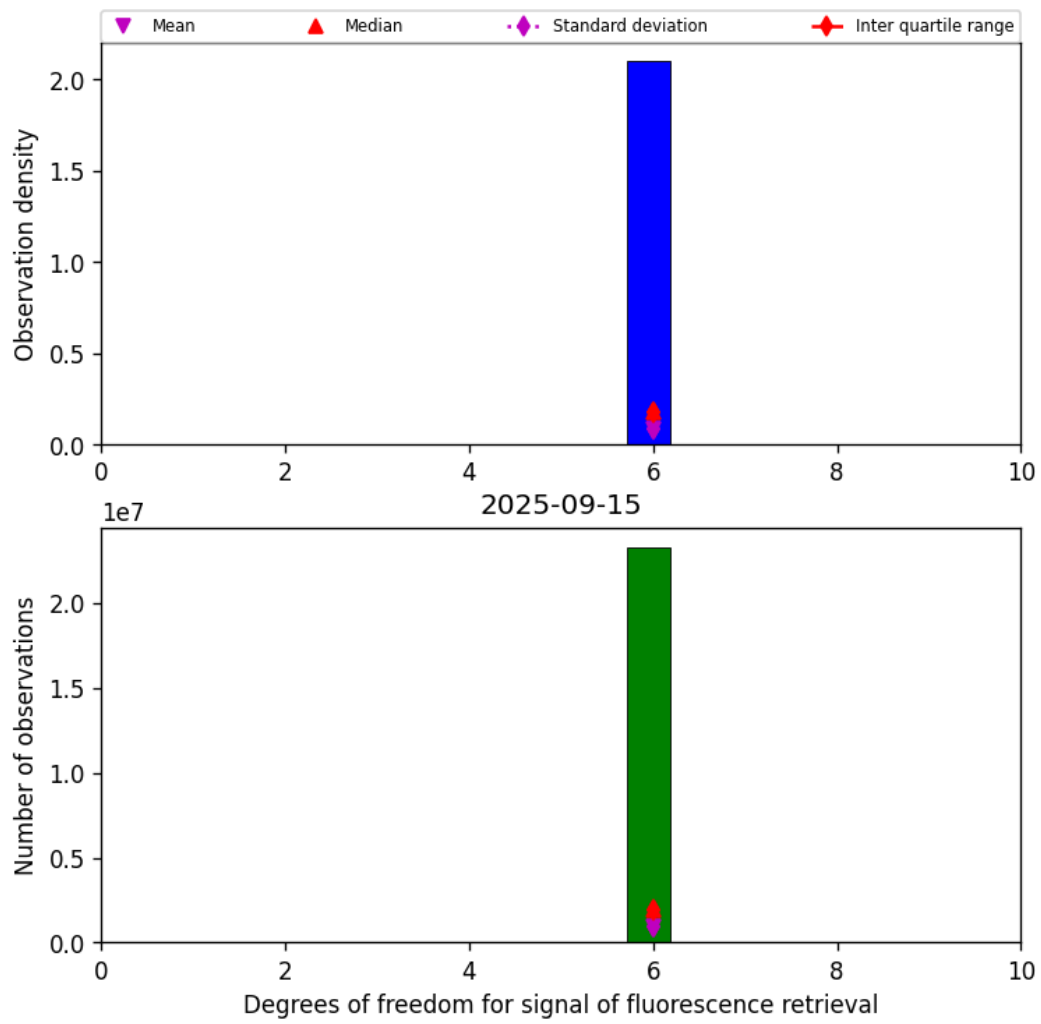
Figure 41: Histogram of “Degrees of freedom for signal of fluorescence retrieval” for 2025-09-15 to 2025-09-16
