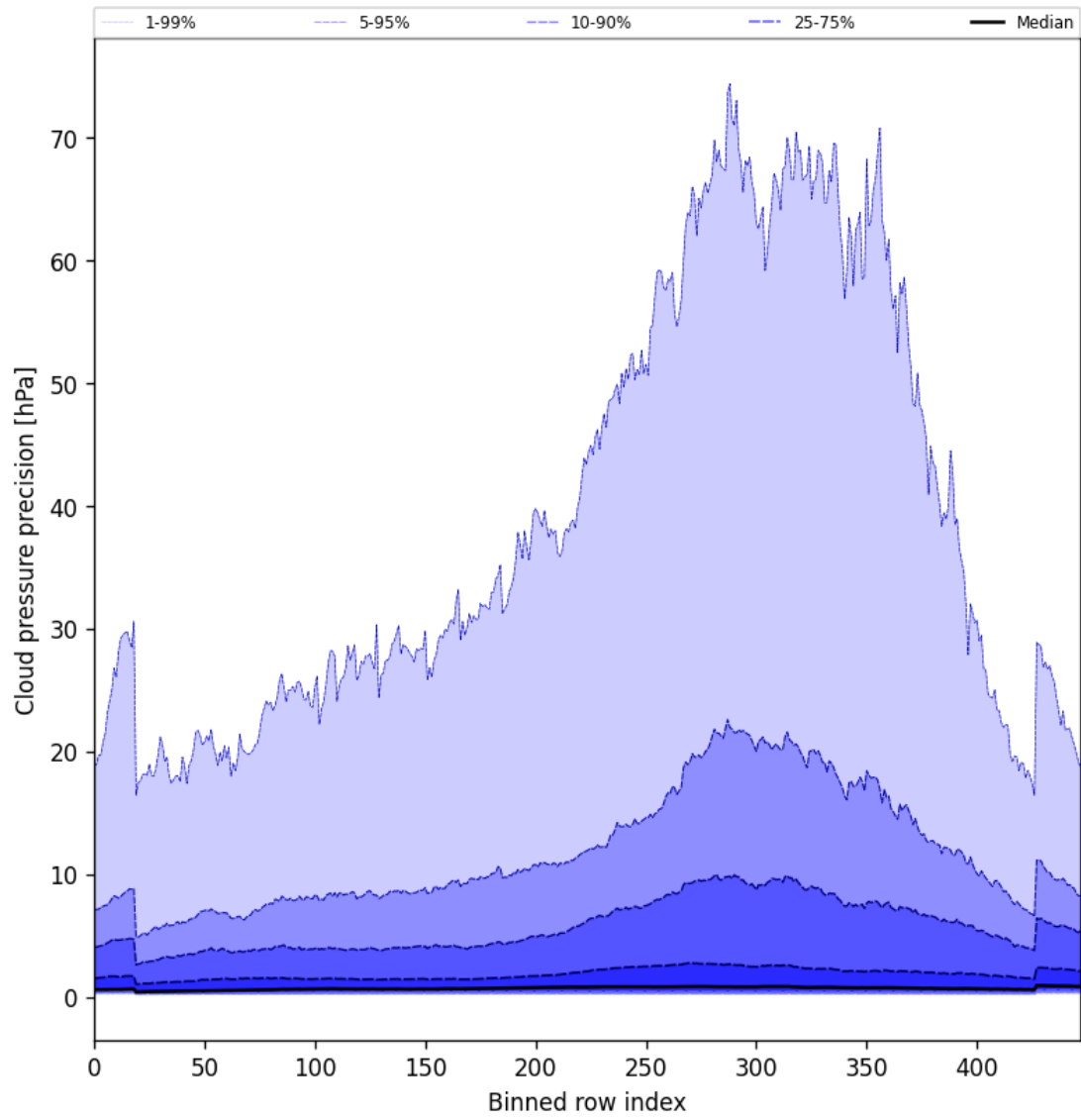
Figure 46: Along track statistics of “Cloud pressure precision” for 2025-09-15 to 2025-09-16
