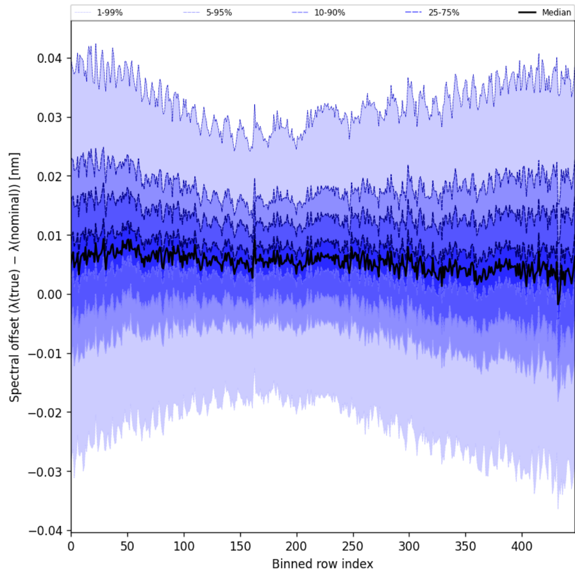
Figure 60: Along track statistics of “Spectral offset ( \lambda_{\text{true}} - \lambda_{\text{nominal}} )” for 2025-09-15 to 2025-09-16
