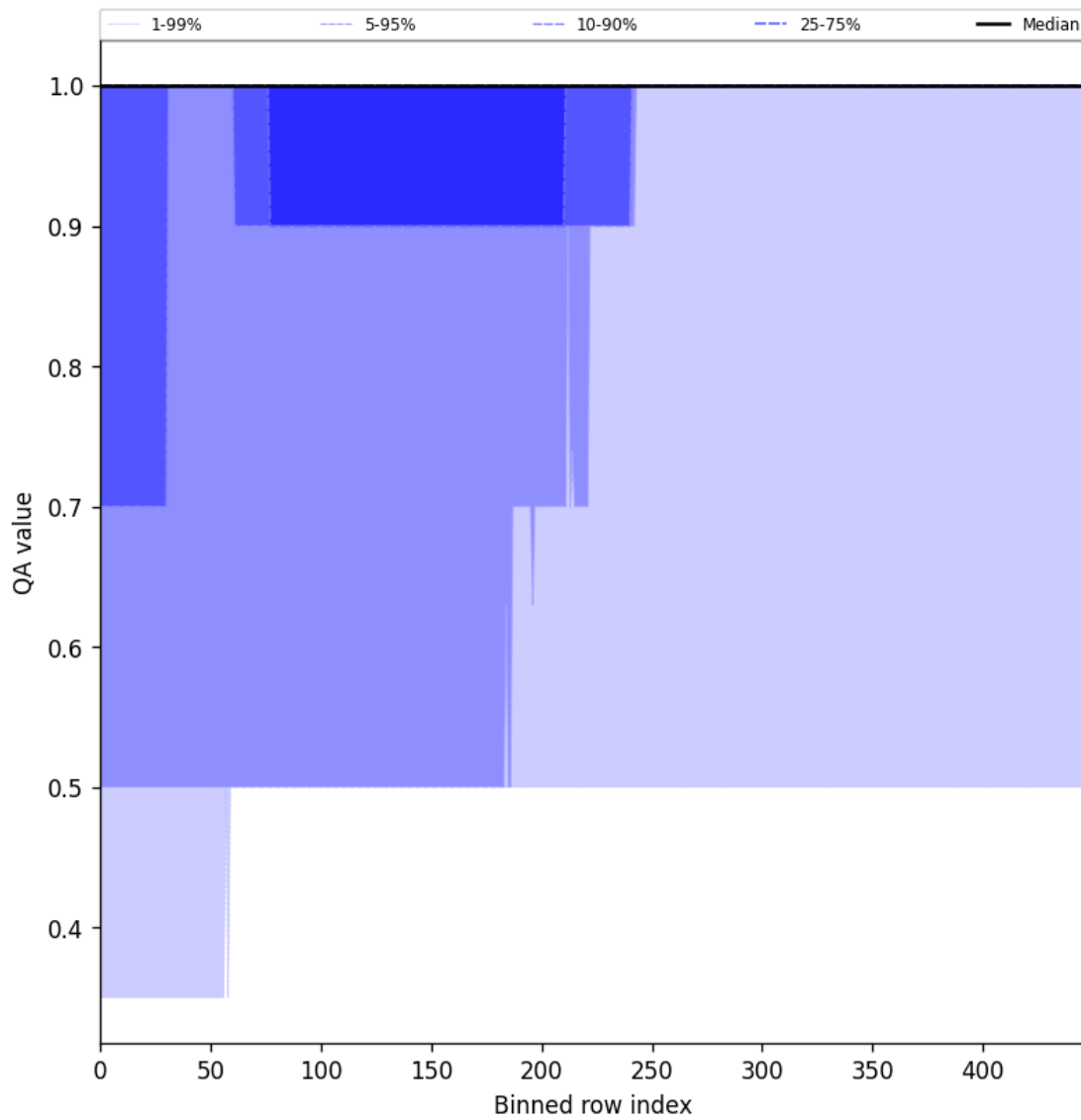
Figure 44: Along track statistics of “QA value” for 2025-09-15 to 2025-09-16
