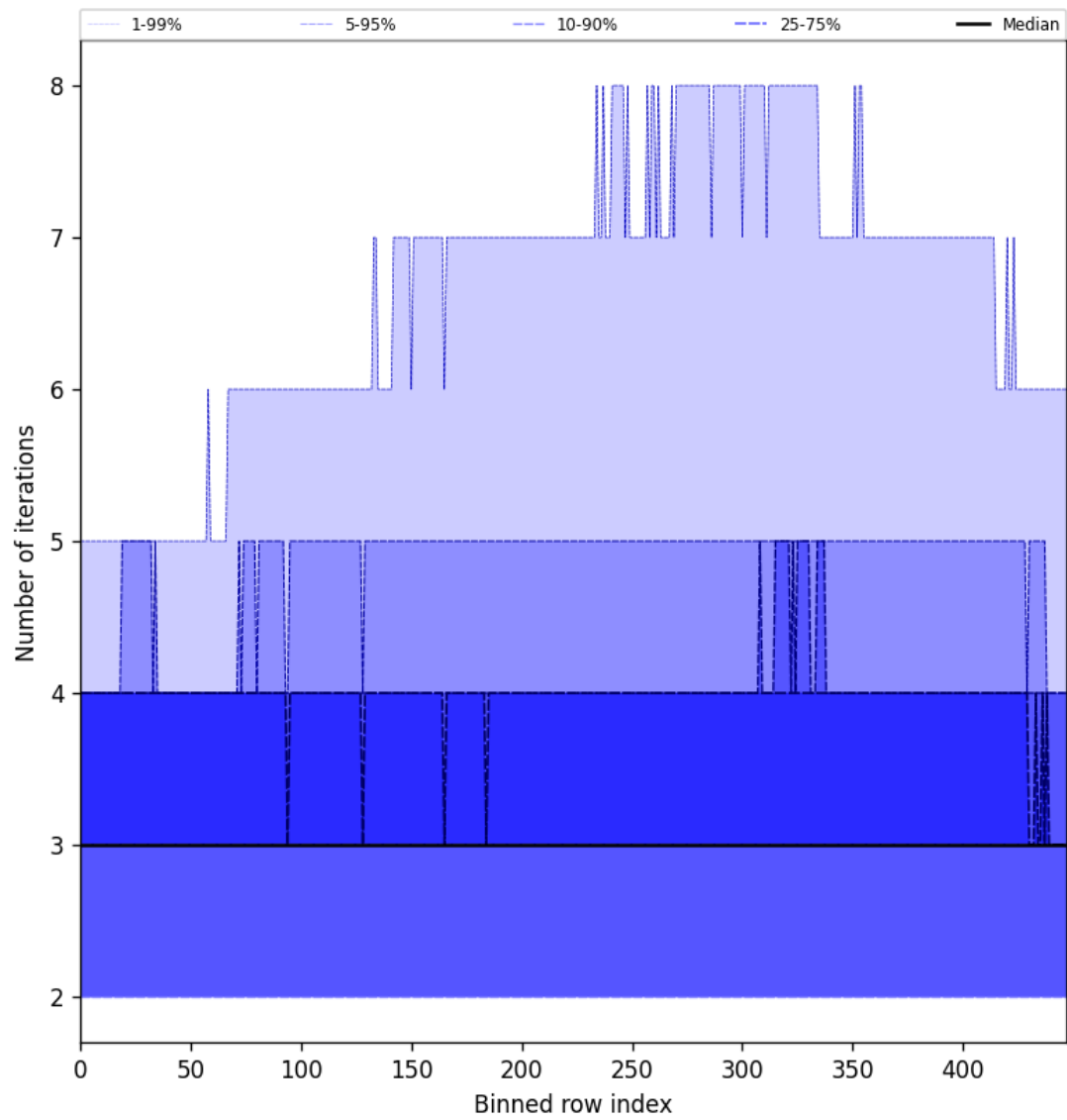
Figure 54: Along track statistics of “Number of iterations” for 2025-09-15 to 2025-09-16
