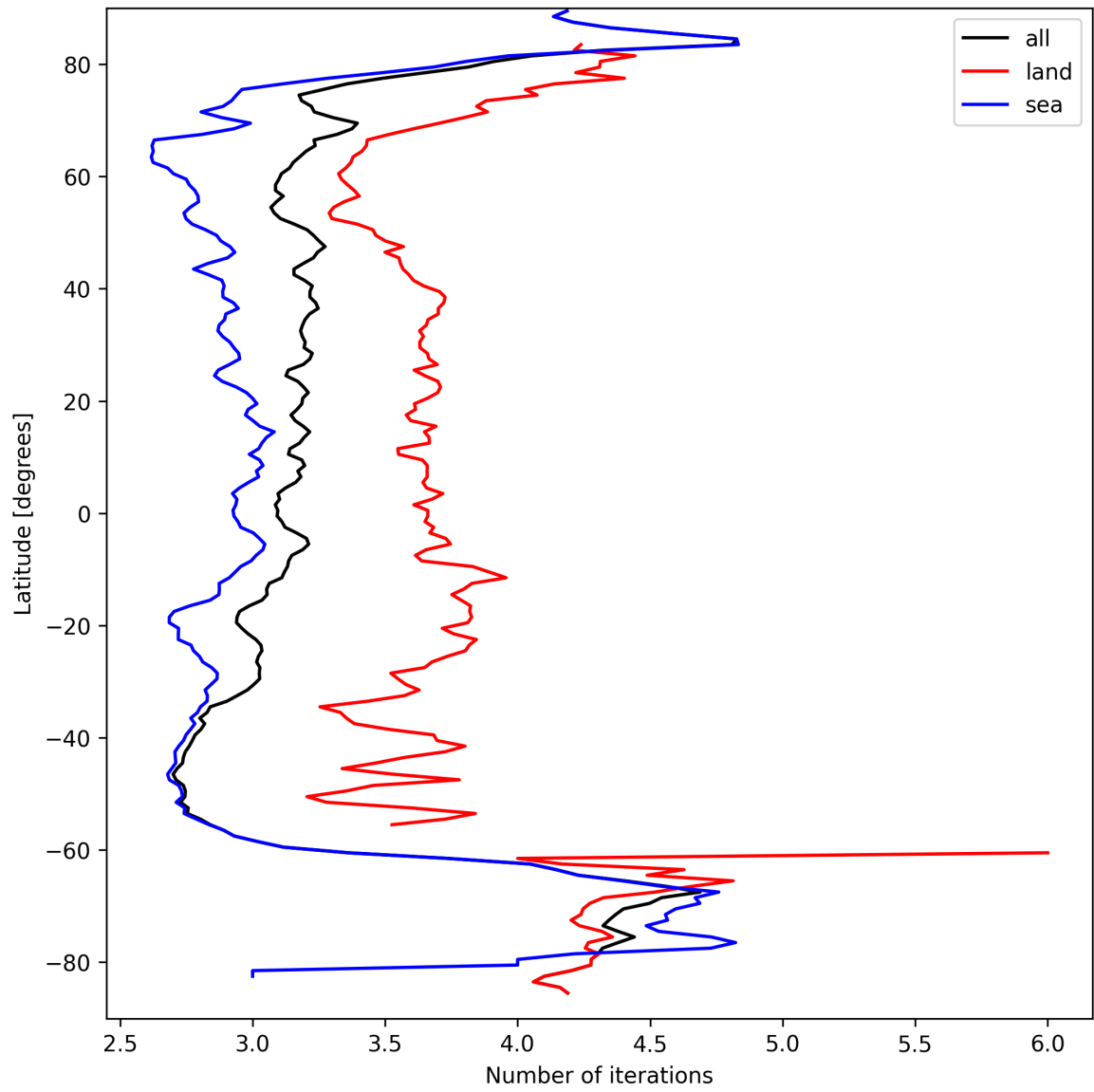
Figure 20: Zonal average of “Number of iterations” for 2025-09-15 to 2025-09-16.
