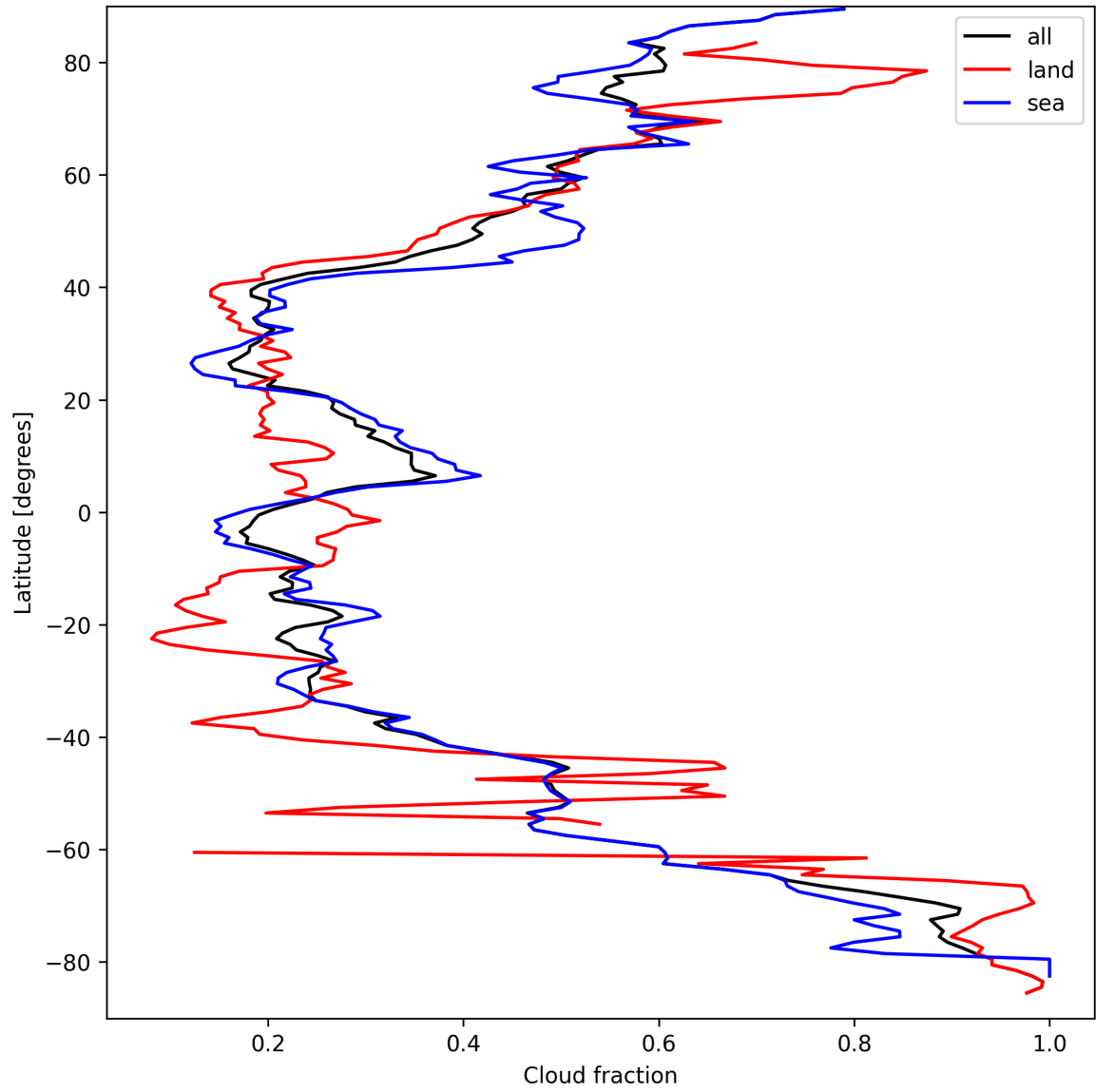
Figure 13: Zonal average of “Cloud fraction” for 2025-09-15 to 2025-09-16.
