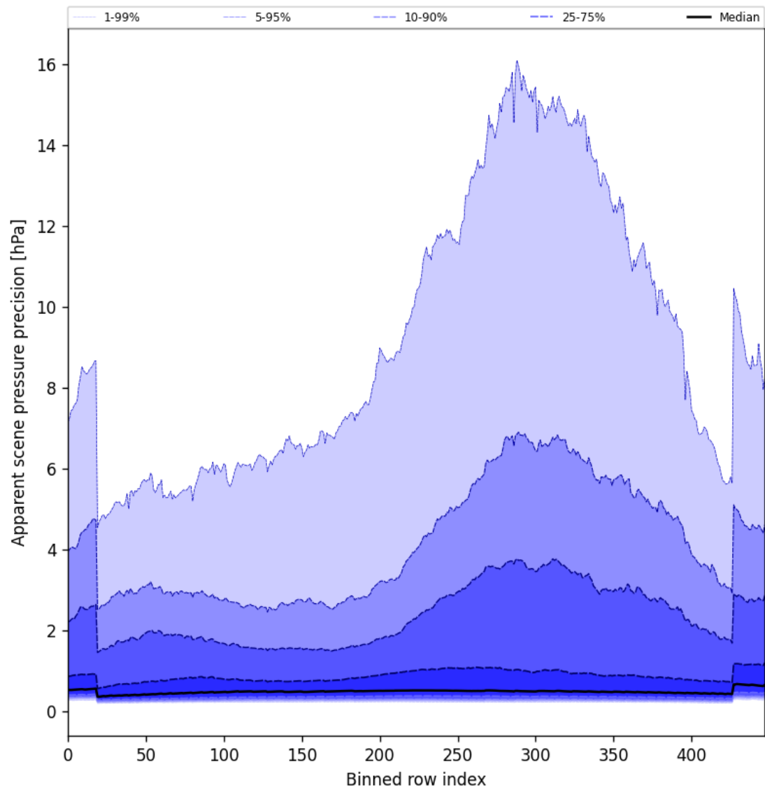
Figure 52: Along track statistics of “Apparent scene pressure precision” for 2025-09-15 to 2025-09-16
