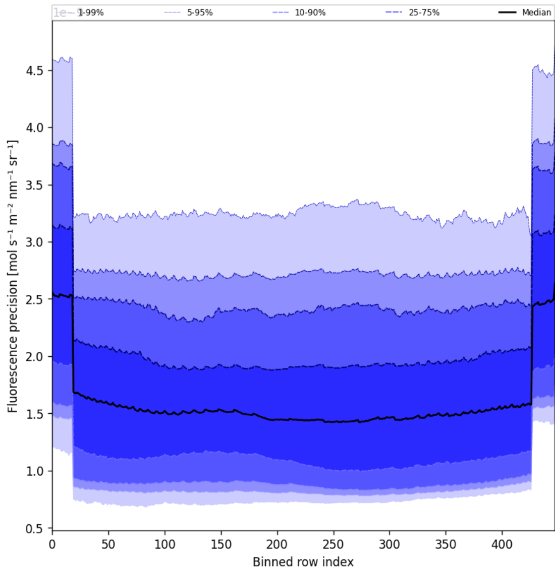
Figure 56: Along track statistics of “Fluorescence precision” for 2025-09-15 to 2025-09-16
