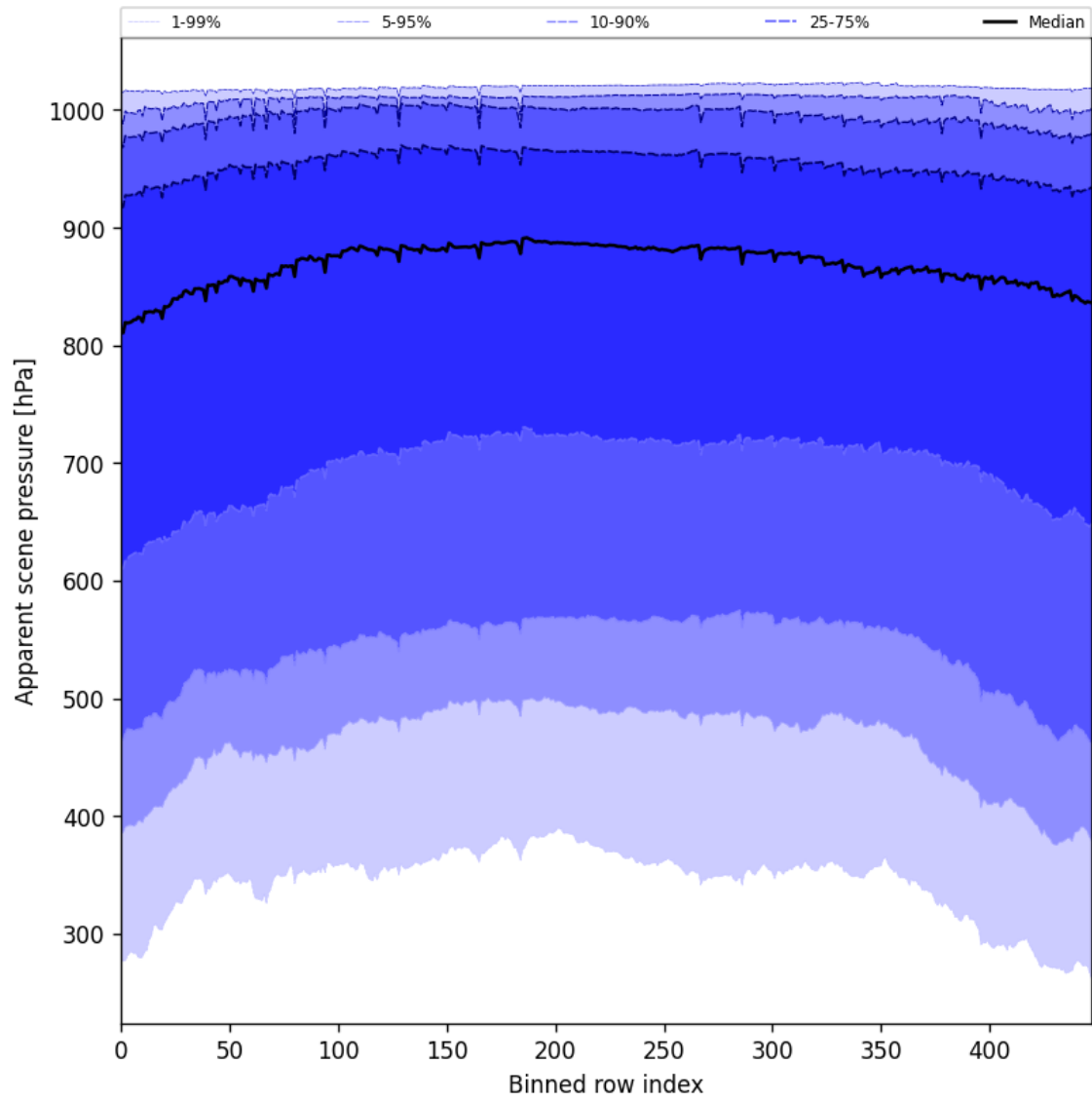
Figure 51: Along track statistics of “Apparent scene pressure” for 2025-09-15 to 2025-09-16
