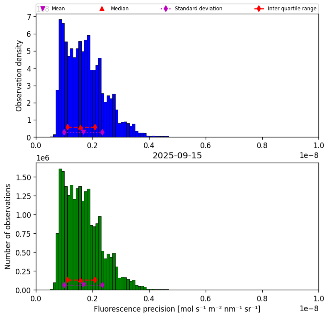
Figure 39: Histogram of “Fluorescence precision” for 2025-09-15 to 2025-09-16
