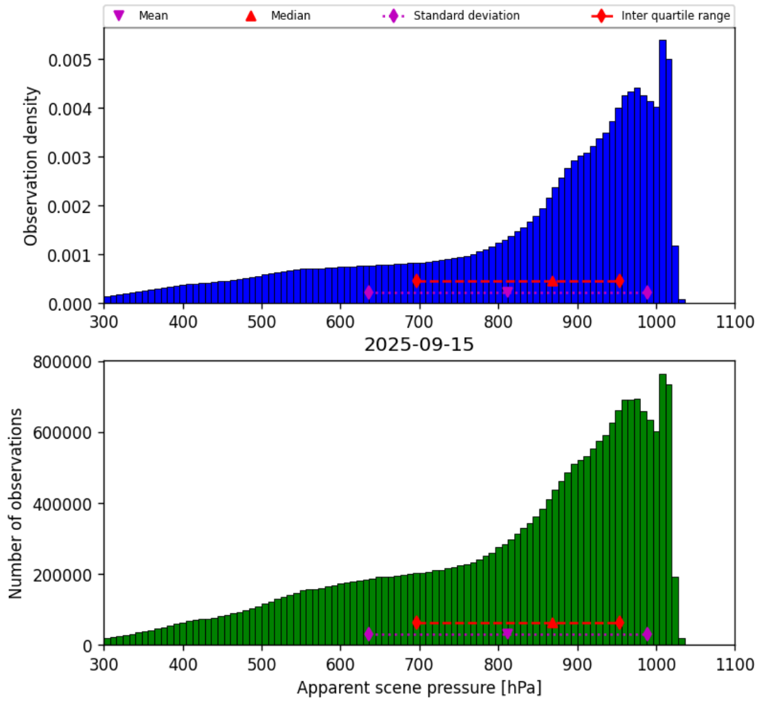
Figure 34: Histogram of “Apparent scene pressure” for 2025-09-15 to 2025-09-16
