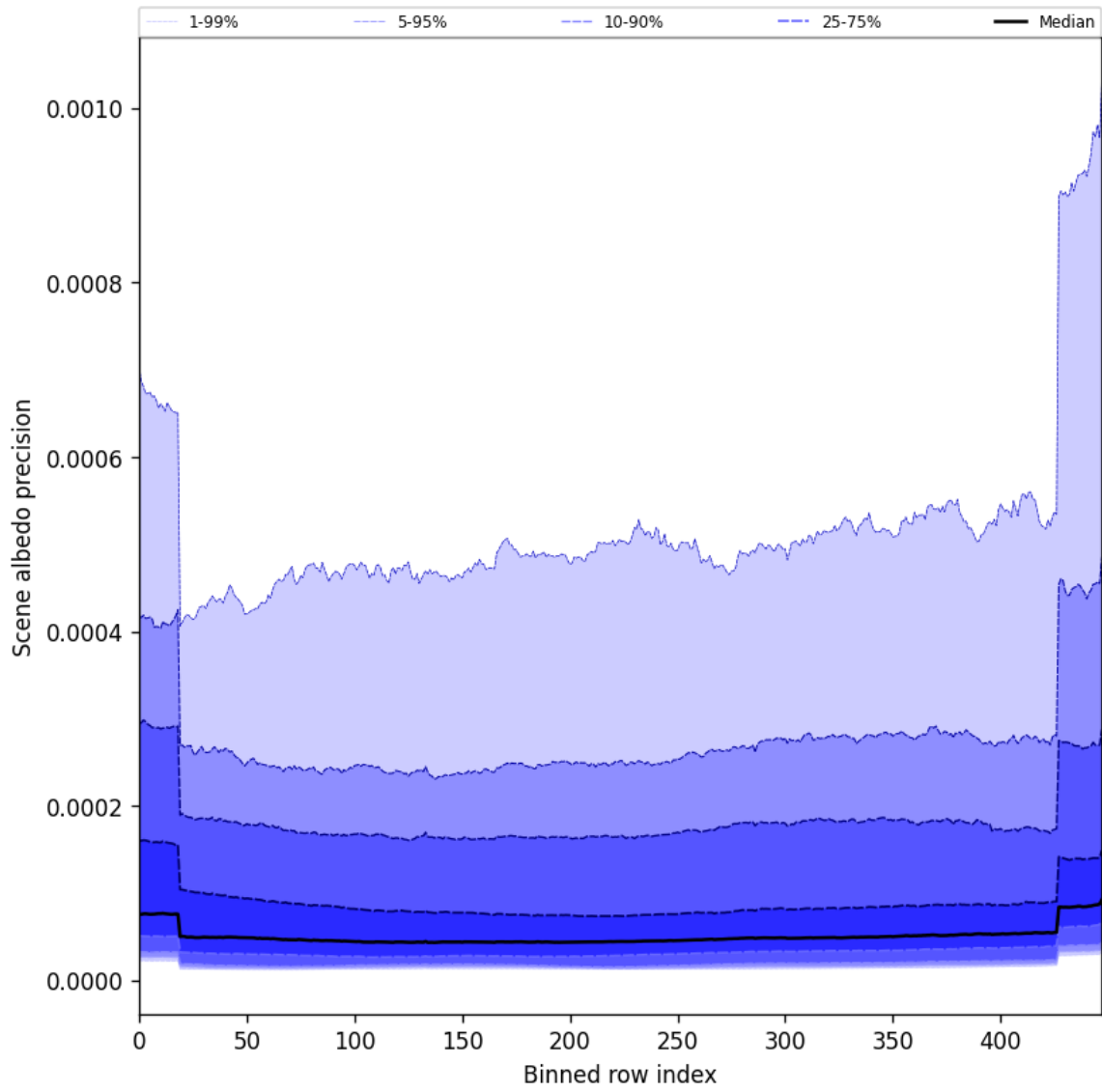
Figure 50: Along track statistics of “Scene albedo precision” for 2025-09-15 to 2025-09-16
