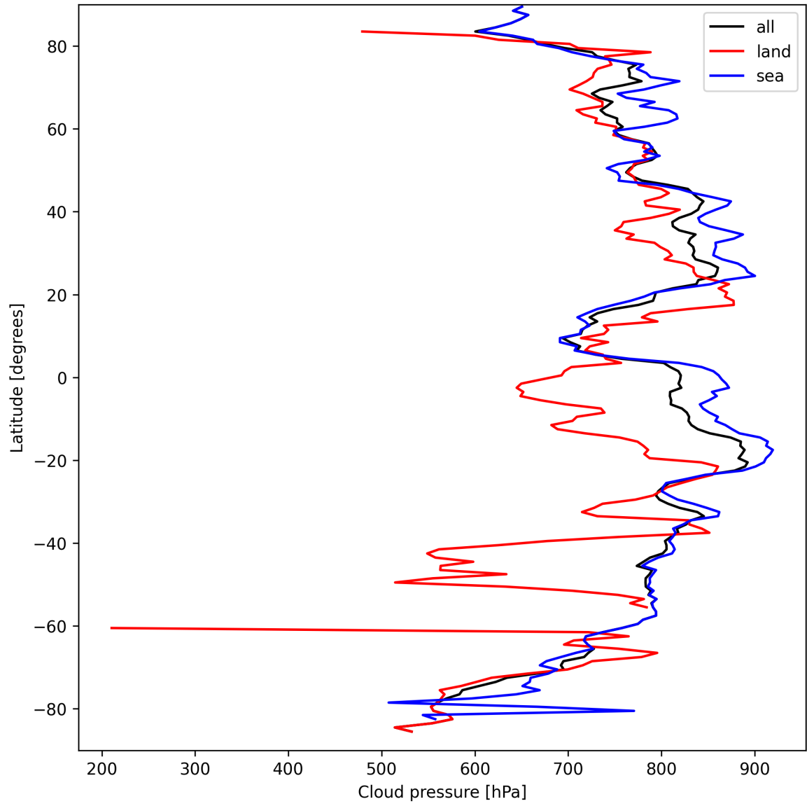
Figure 11: Zonal average of “Cloud pressure” for 2025-09-15 to 2025-09-16.
