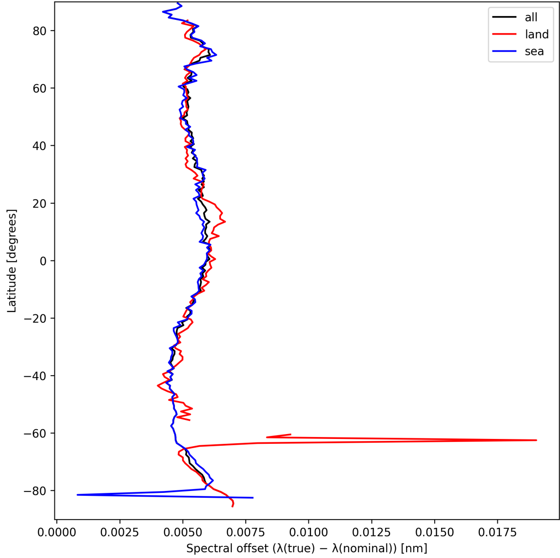
Figure 26: Zonal average of “Spectral offset ( \lambda_{\text{true}} - \lambda_{\text{nominal}} )” for 2025-09-15 to 2025-09-16.
