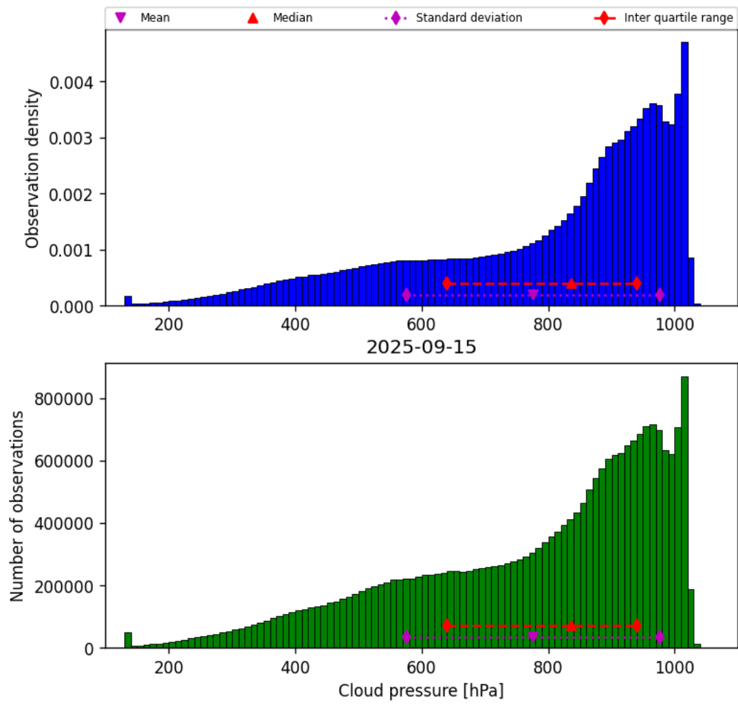
Figure 28: Histogram of “Cloud pressure” for 2025-09-15 to 2025-09-16
