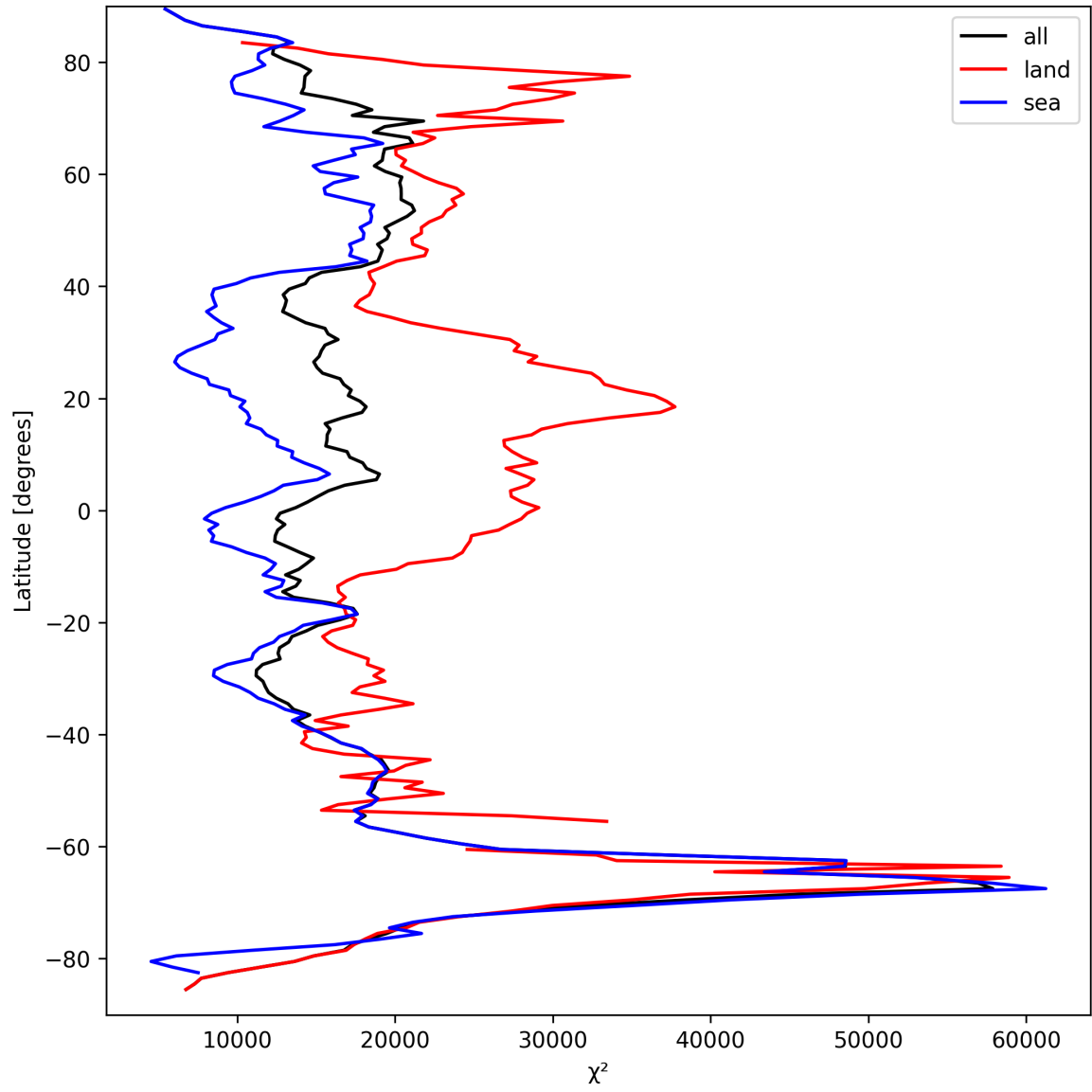
Figure 19: Zonal average of “ \chi^2 ” for 2025-09-15 to 2025-09-16.
