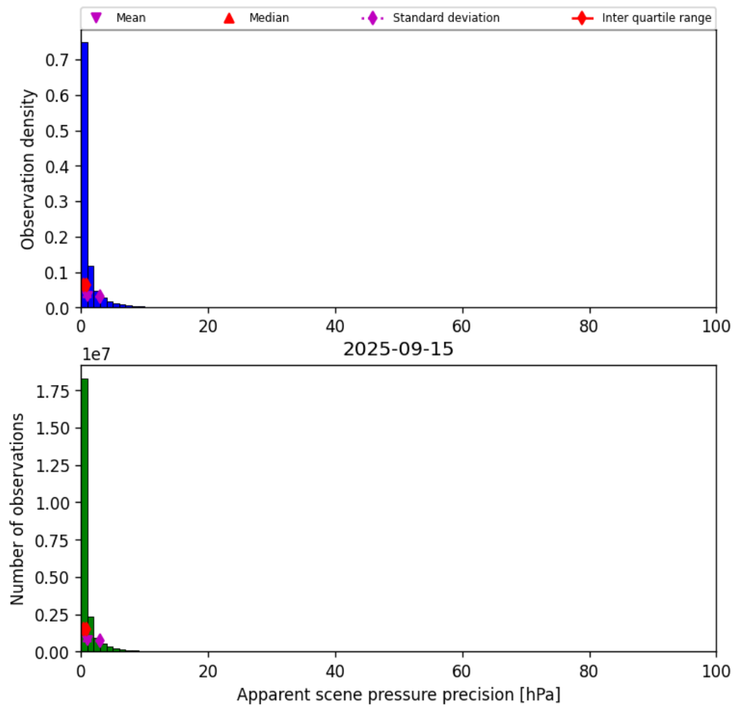
Figure 35: Histogram of “Apparent scene pressure precision” for 2025-09-15 to 2025-09-16
