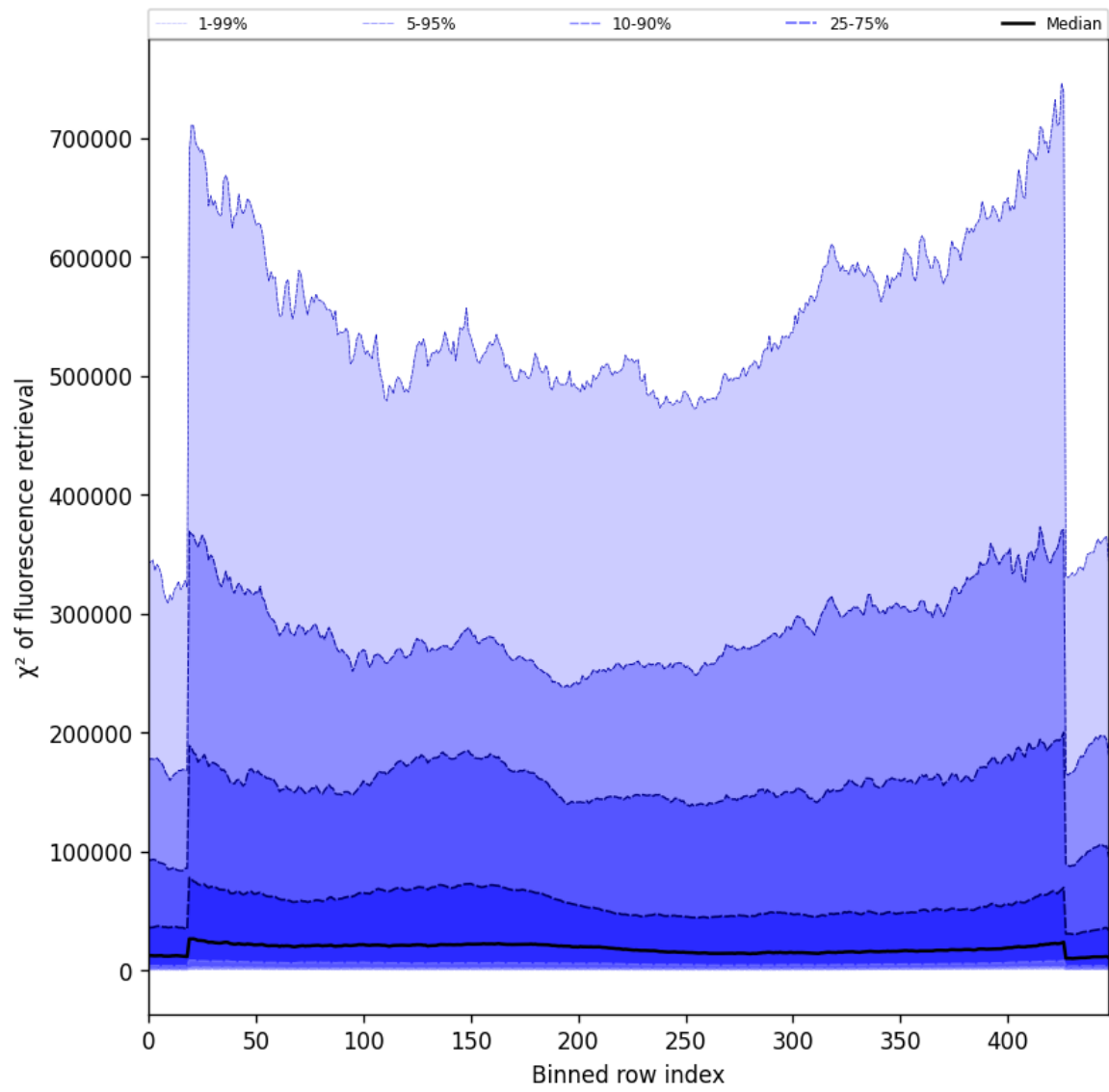
Figure 57: Along track statistics of “ \chi^2 of fluorescence retrieval” for 2025-09-15 to 2025-09-16
