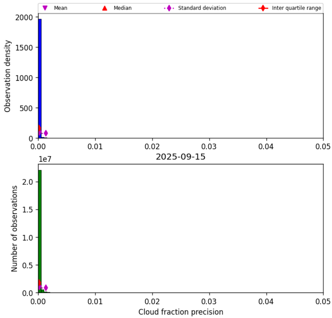
Figure 31: Histogram of “Cloud fraction precision” for 2025-09-15 to 2025-09-16
