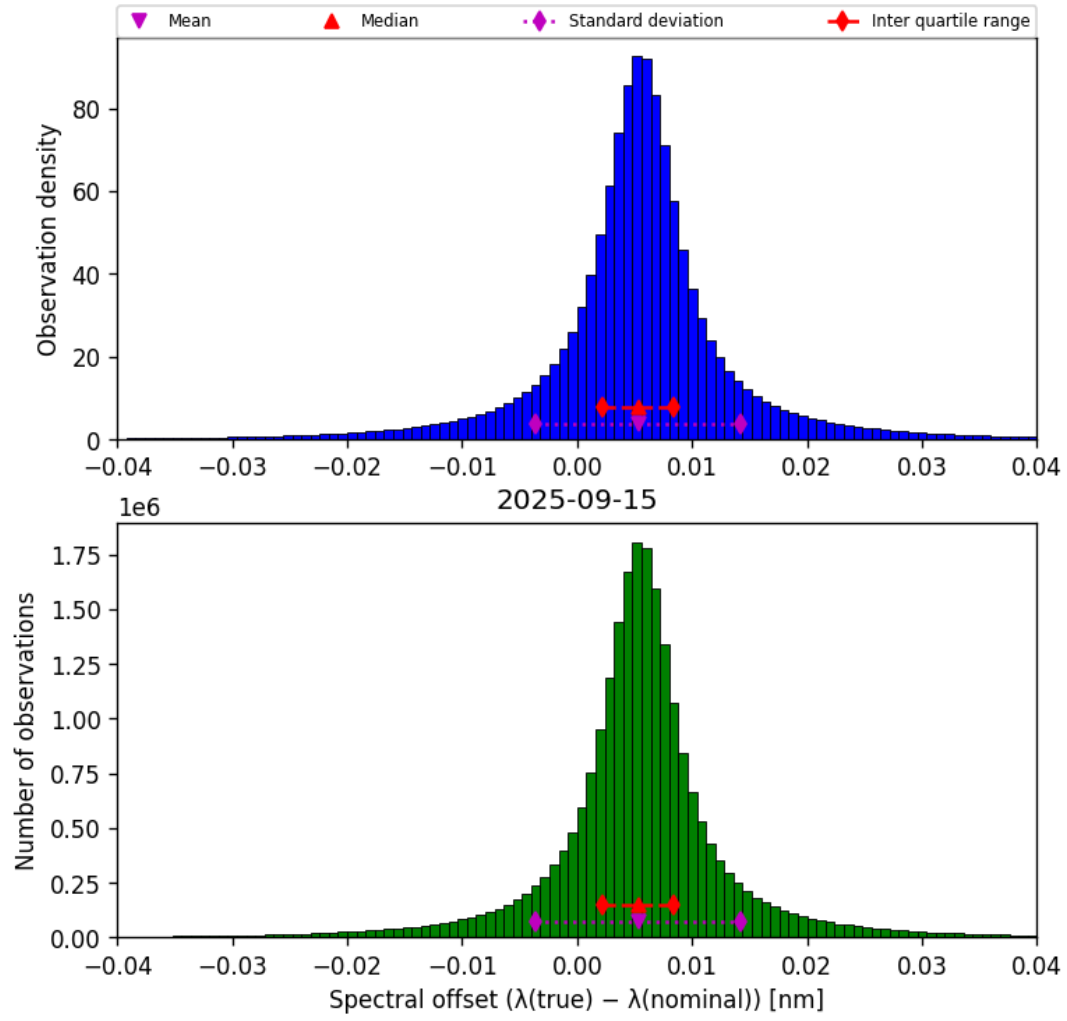
Figure 43: Histogram of “Spectral offset ( \lambda_{\text{true}} - \lambda_{\text{nominal}} )” for 2025-09-15 to 2025-09-16
