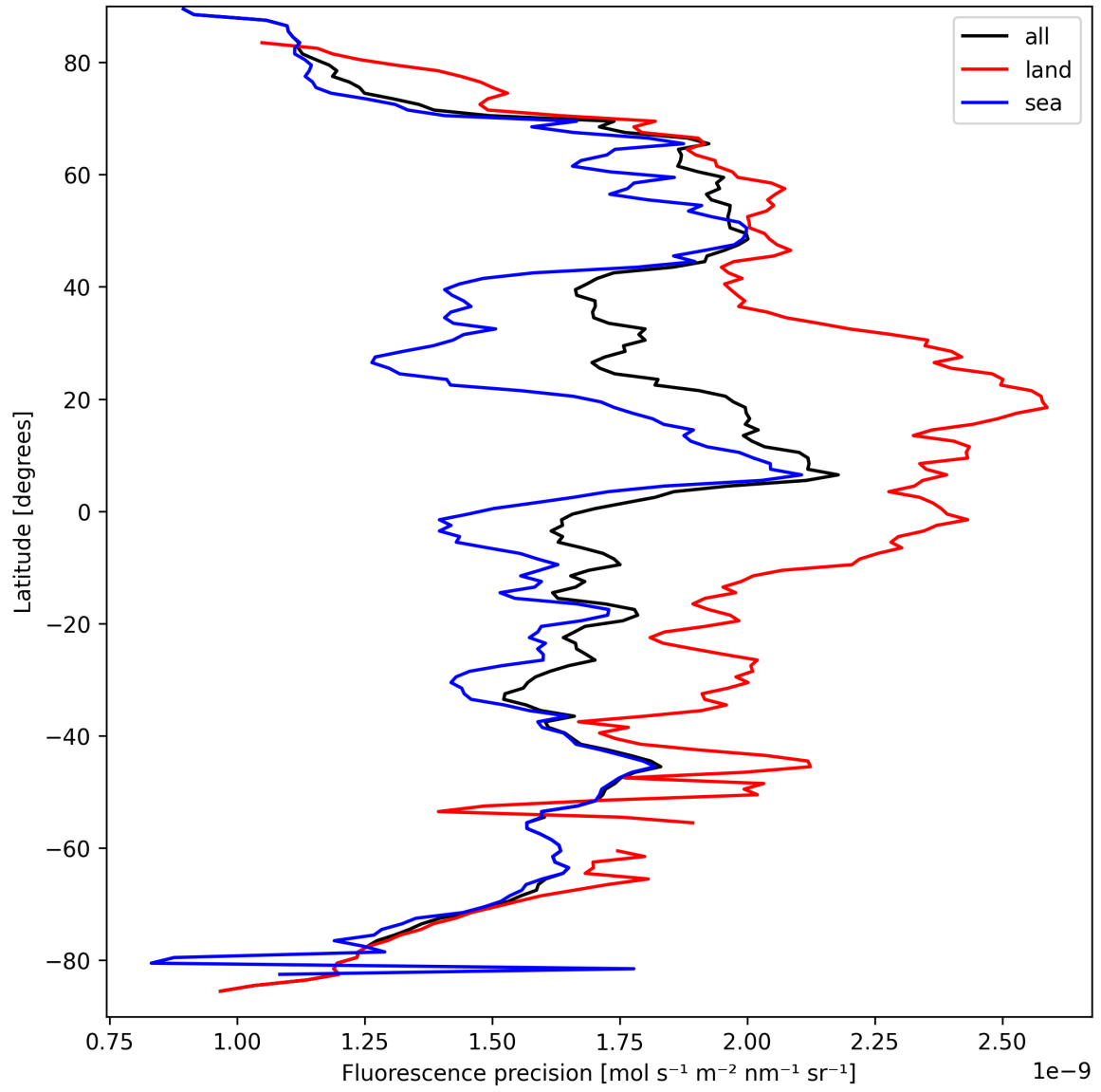
Figure 22: Zonal average of “Fluorescence precision” for 2025-09-15 to 2025-09-16.
