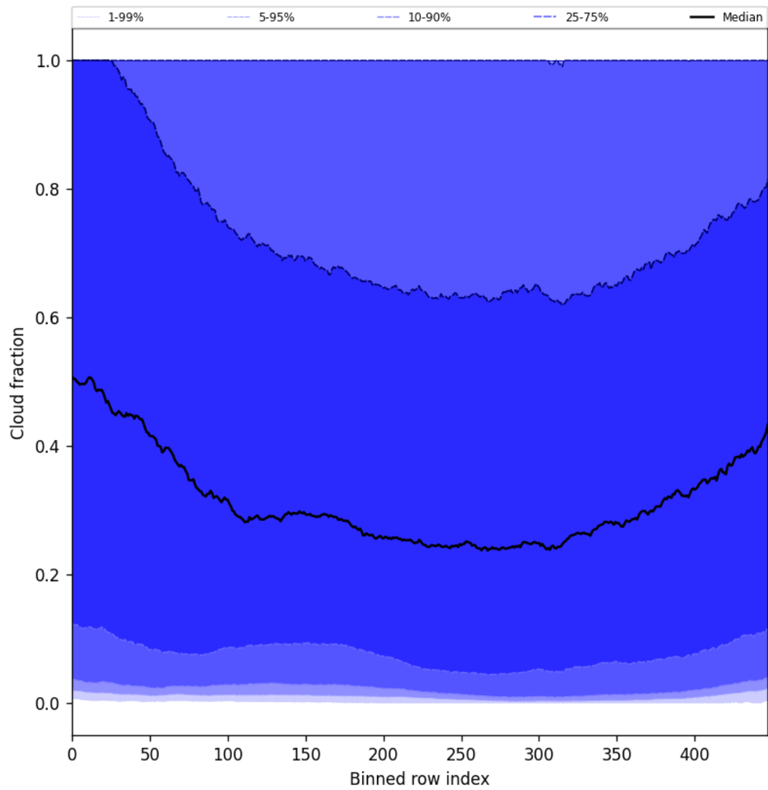
Figure 47: Along track statistics of “Cloud fraction” for 2025-09-15 to 2025-09-16
