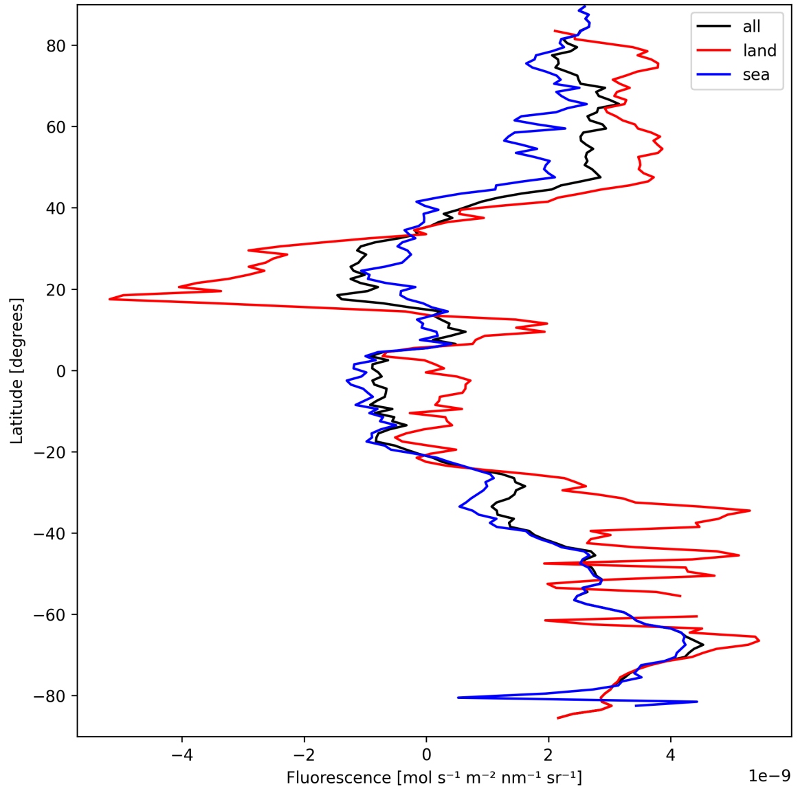
Figure 21: Zonal average of “Fluorescence” for 2025-09-15 to 2025-09-16.
