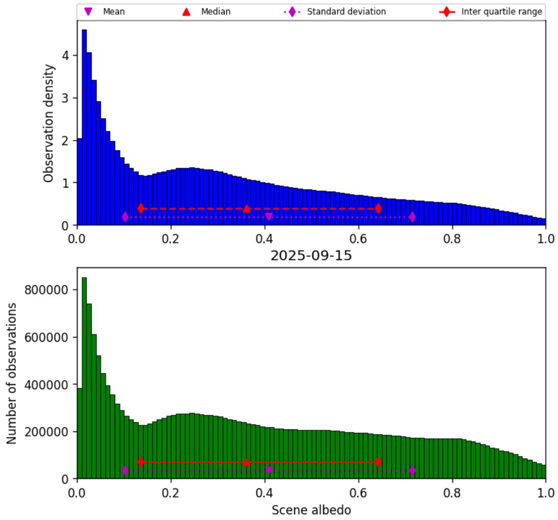
Figure 32: Histogram of “Scene albedo” for 2025-09-15 to 2025-09-16
