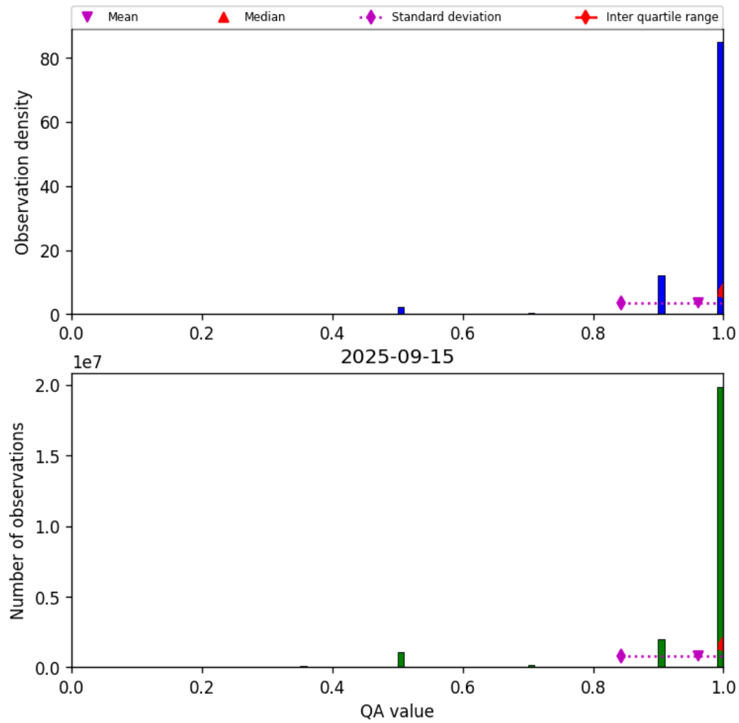
Figure 27: Histogram of “QA value” for 2025-09-15 to 2025-09-16
