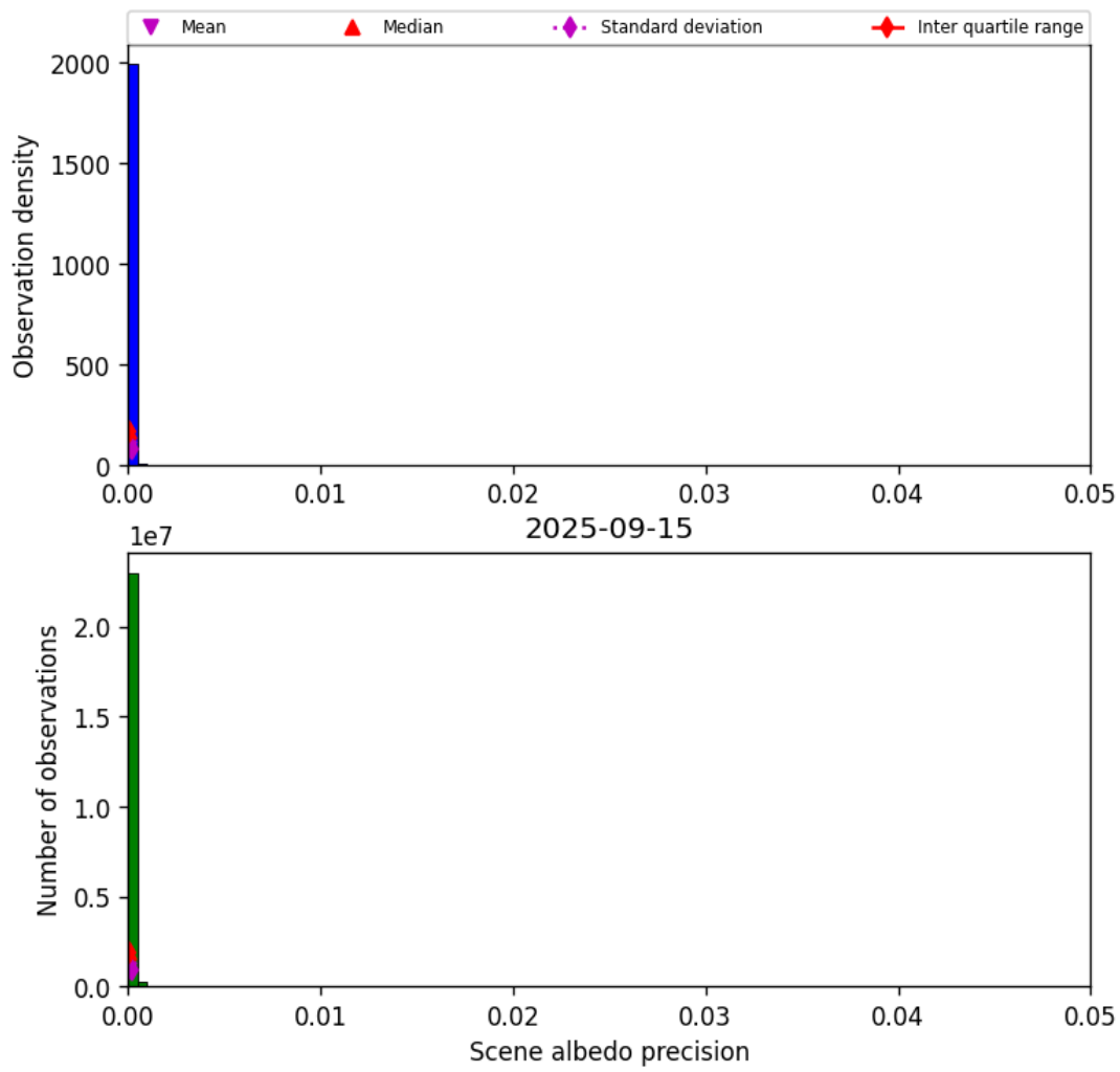
Figure 33: Histogram of “Scene albedo precision” for 2025-09-15 to 2025-09-16
