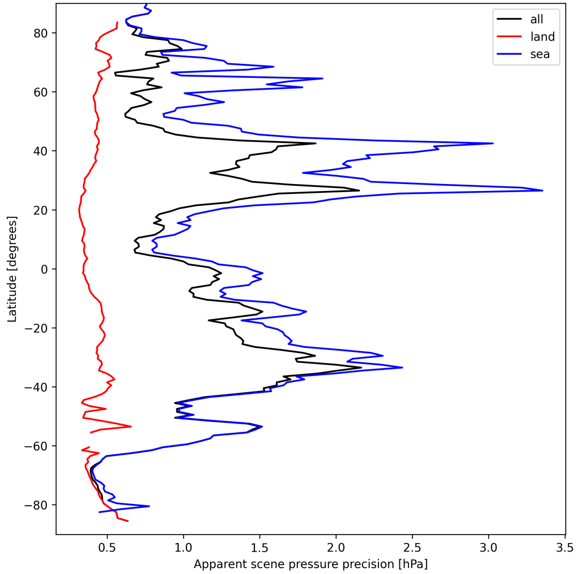
Figure 18: Zonal average of “Apparent scene pressure precision” for 2025-09-15 to 2025-09-16.
