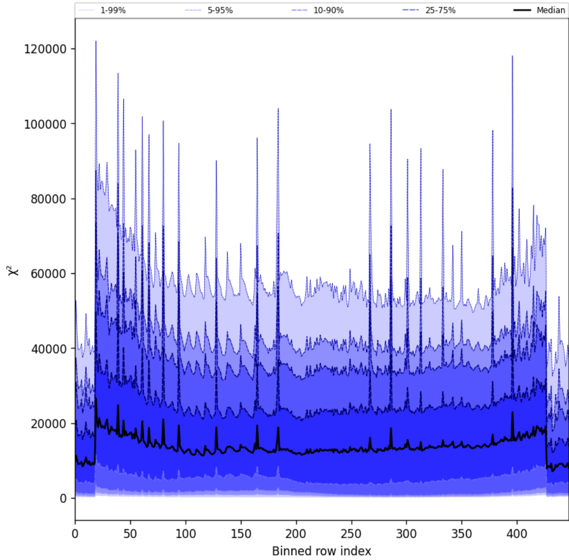
Figure 53: Along track statistics of “ \chi^2 ” for 2025-09-15 to 2025-09-16
