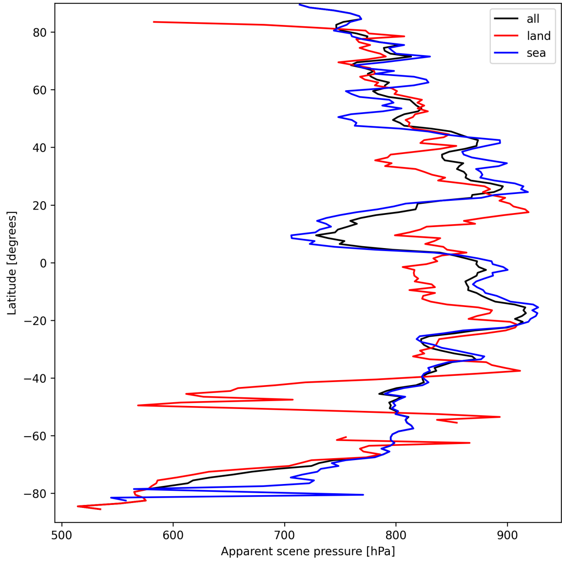
Figure 17: Zonal average of “Apparent scene pressure” for 2025-09-15 to 2025-09-16.
