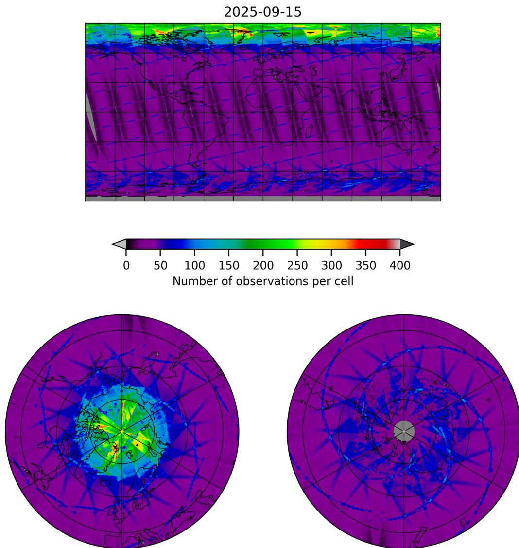
Figure 9: Map of the number of observations for 2025-09-15 to 2025-09-16
