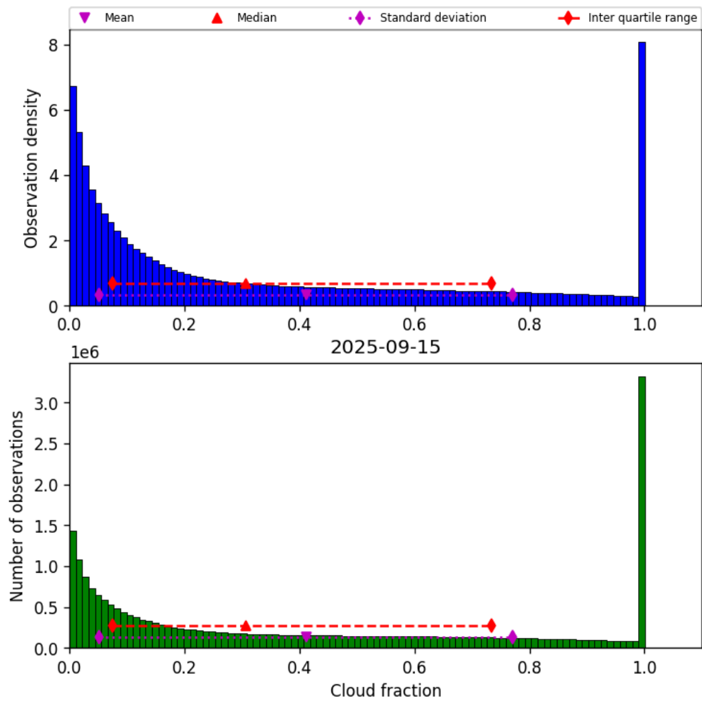
Figure 30: Histogram of “Cloud fraction” for 2025-09-15 to 2025-09-16
