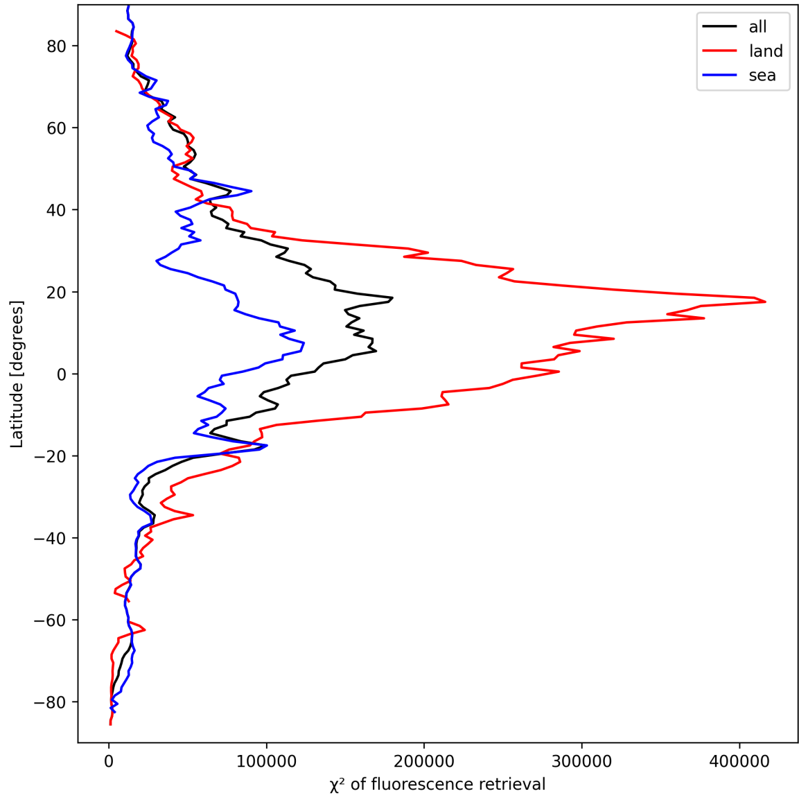
Figure 23: Zonal average of “ \chi^2 of fluorescence retrieval” for 2025-09-15 to 2025-09-16.
