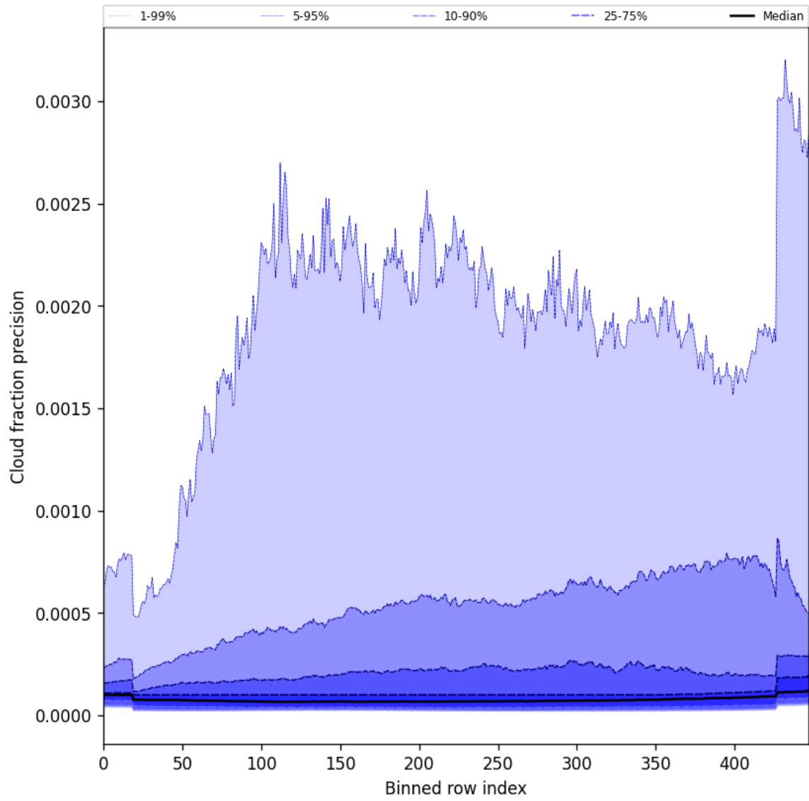
Figure 48: Along track statistics of “Cloud fraction precision” for 2025-09-15 to 2025-09-16
