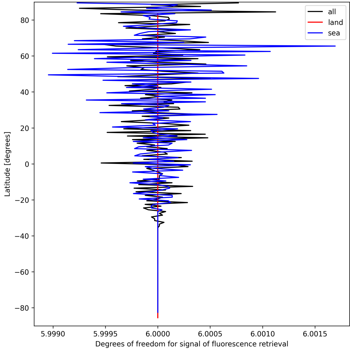
Figure 24: Zonal average of “Degrees of freedom for signal of fluorescence retrieval” for 2025-09-15 to 2025-09-16.
