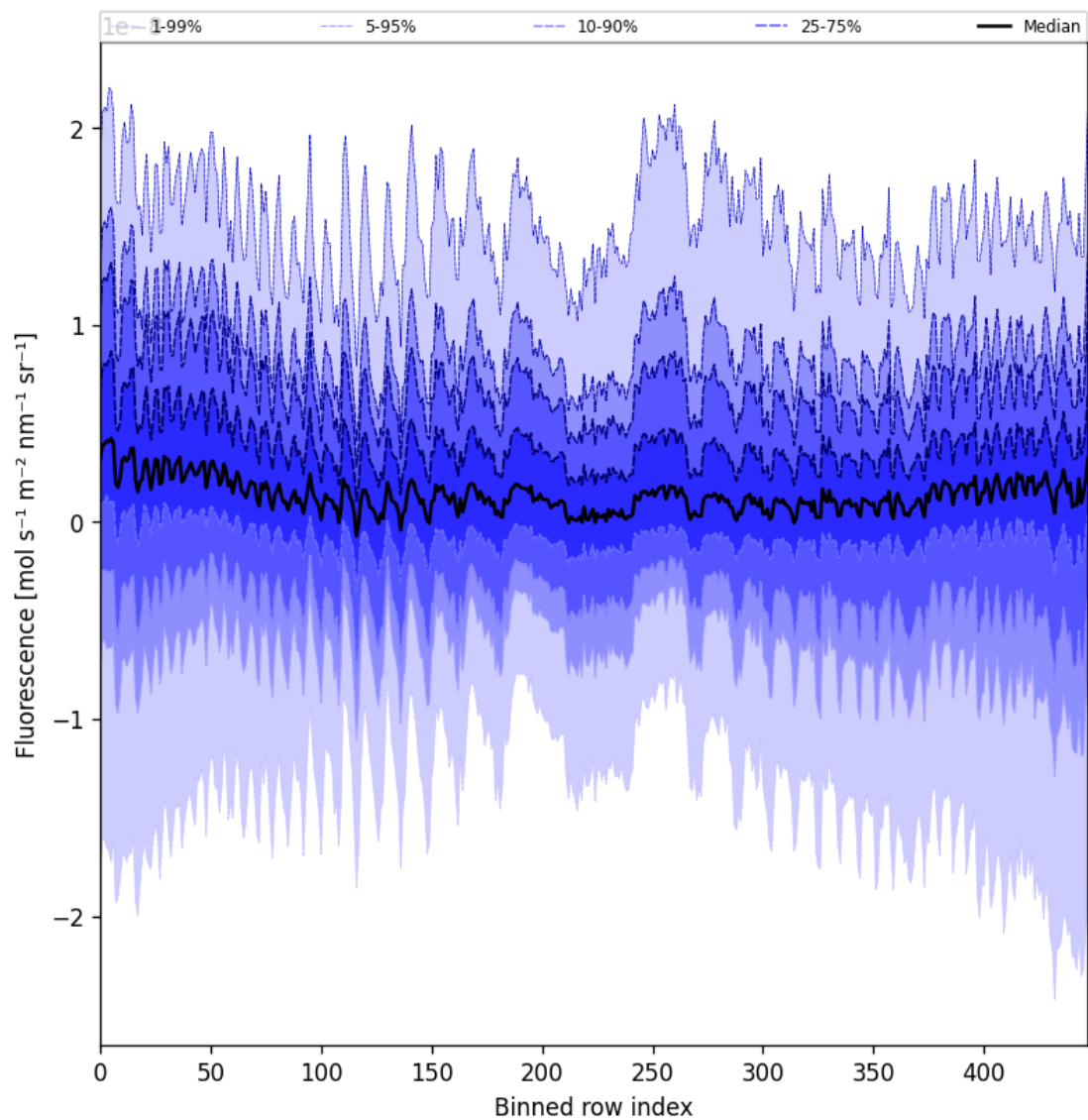
Figure 55: Along track statistics of “Fluorescence” for 2025-09-15 to 2025-09-16
