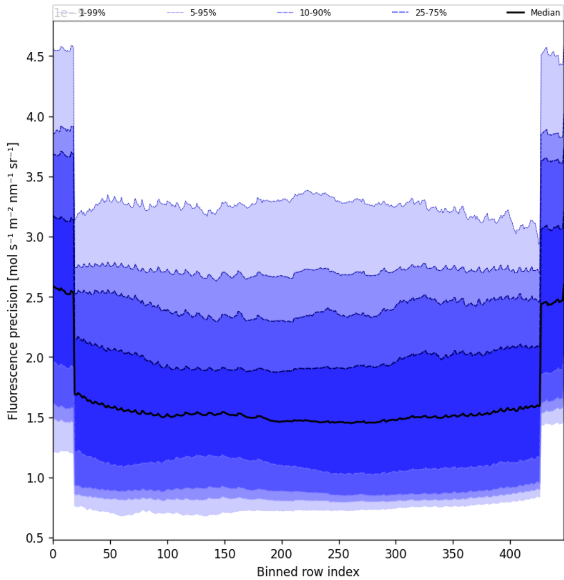
Figure 56: Along track statistics of “Fluorescence precision” for 2025-09-16 to 2025-09-17
