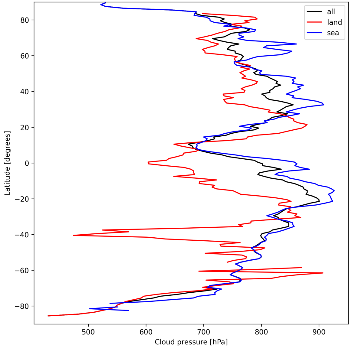
Figure 11: Zonal average of “Cloud pressure” for 2025-09-16 to 2025-09-17.
