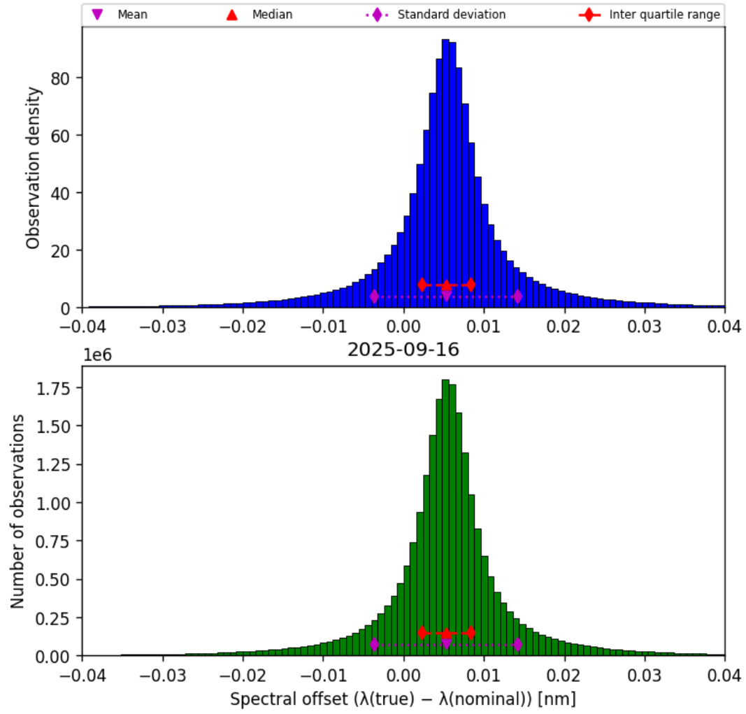
Figure 43: Histogram of “Spectral offset ( \lambda_{\text{true}} - \lambda_{\text{nominal}} )” for 2025-09-16 to 2025-09-17
