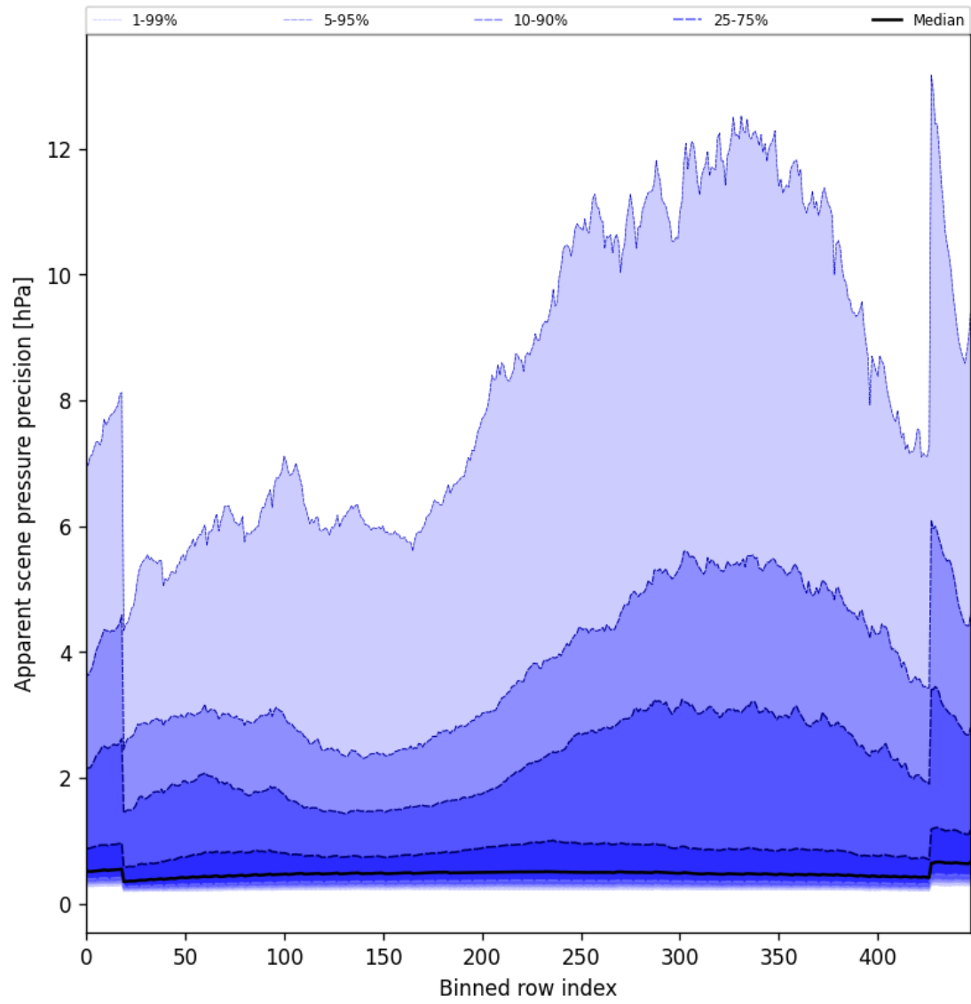
Figure 52: Along track statistics of “Apparent scene pressure precision” for 2025-09-16 to 2025-09-17
