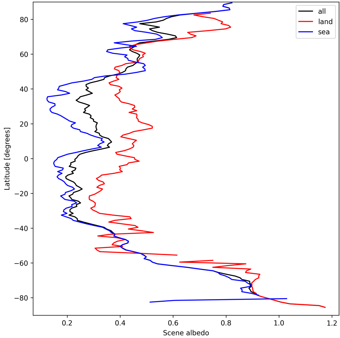
Figure 15: Zonal average of “Scene albedo” for 2025-09-16 to 2025-09-17.
