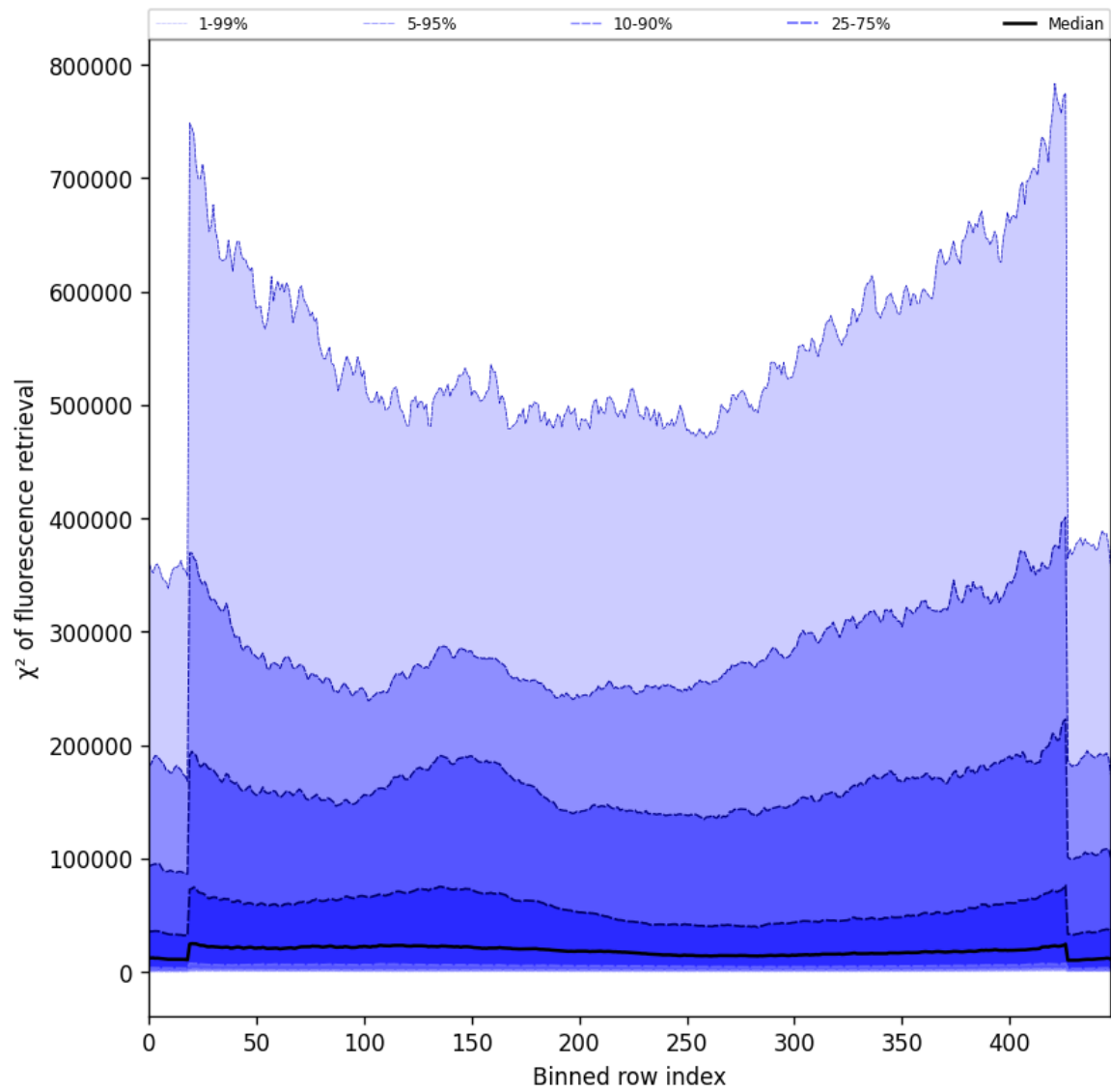
Figure 57: Along track statistics of “ \chi^2 of fluorescence retrieval” for 2025-09-16 to 2025-09-17
