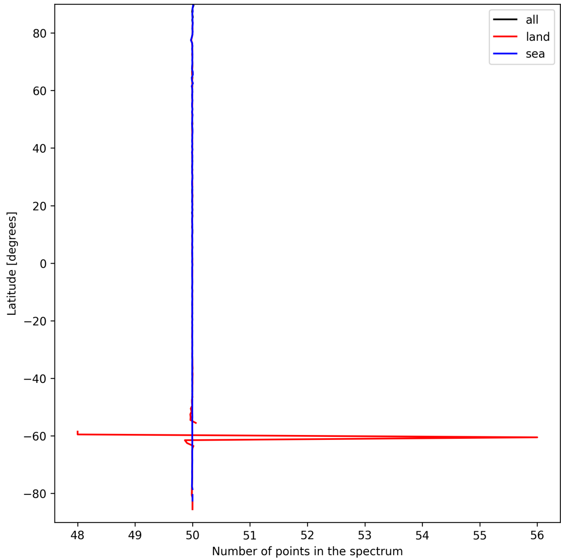
Figure 25: Zonal average of “Number of points in the spectrum” for 2025-09-16 to 2025-09-17.
