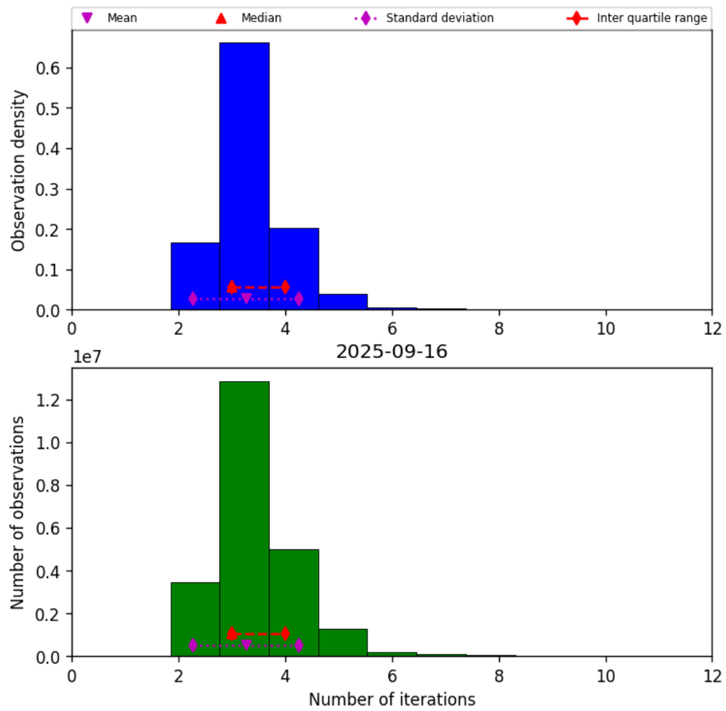
Figure 37: Histogram of “Number of iterations” for 2025-09-16 to 2025-09-17
