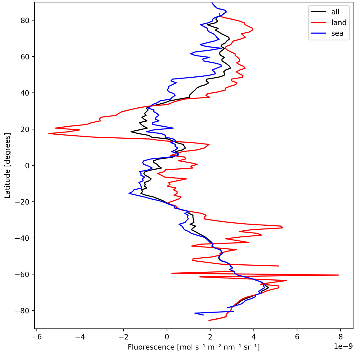
Figure 21: Zonal average of “Fluorescence” for 2025-09-16 to 2025-09-17.
