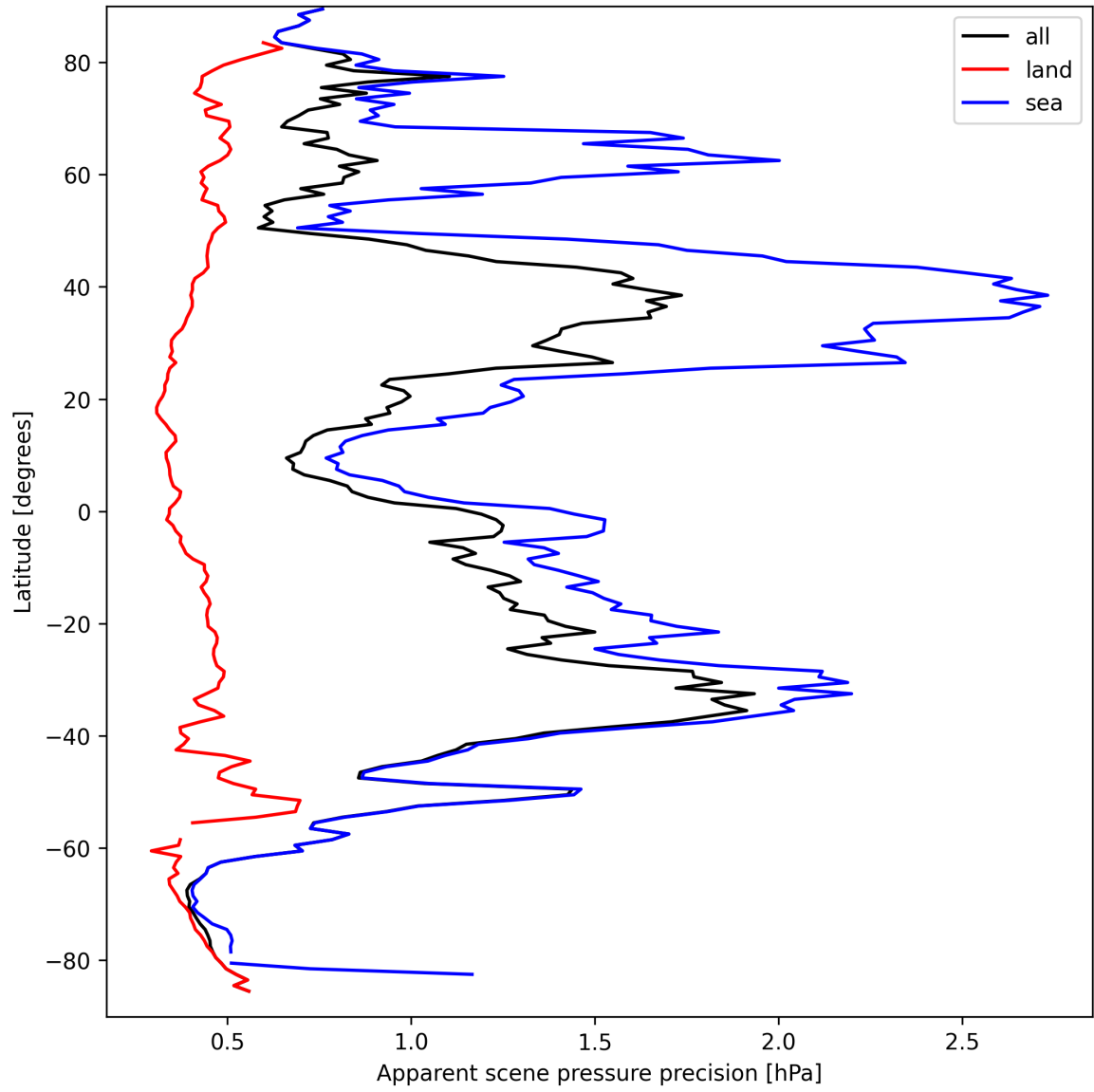
Figure 18: Zonal average of “Apparent scene pressure precision” for 2025-09-16 to 2025-09-17.
