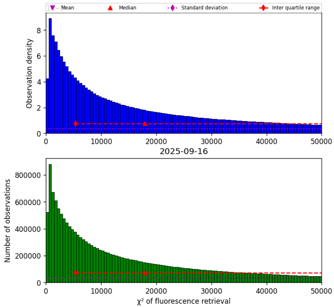
Figure 40: Histogram of “ \chi^2 of fluorescence retrieval” for 2025-09-16 to 2025-09-17
