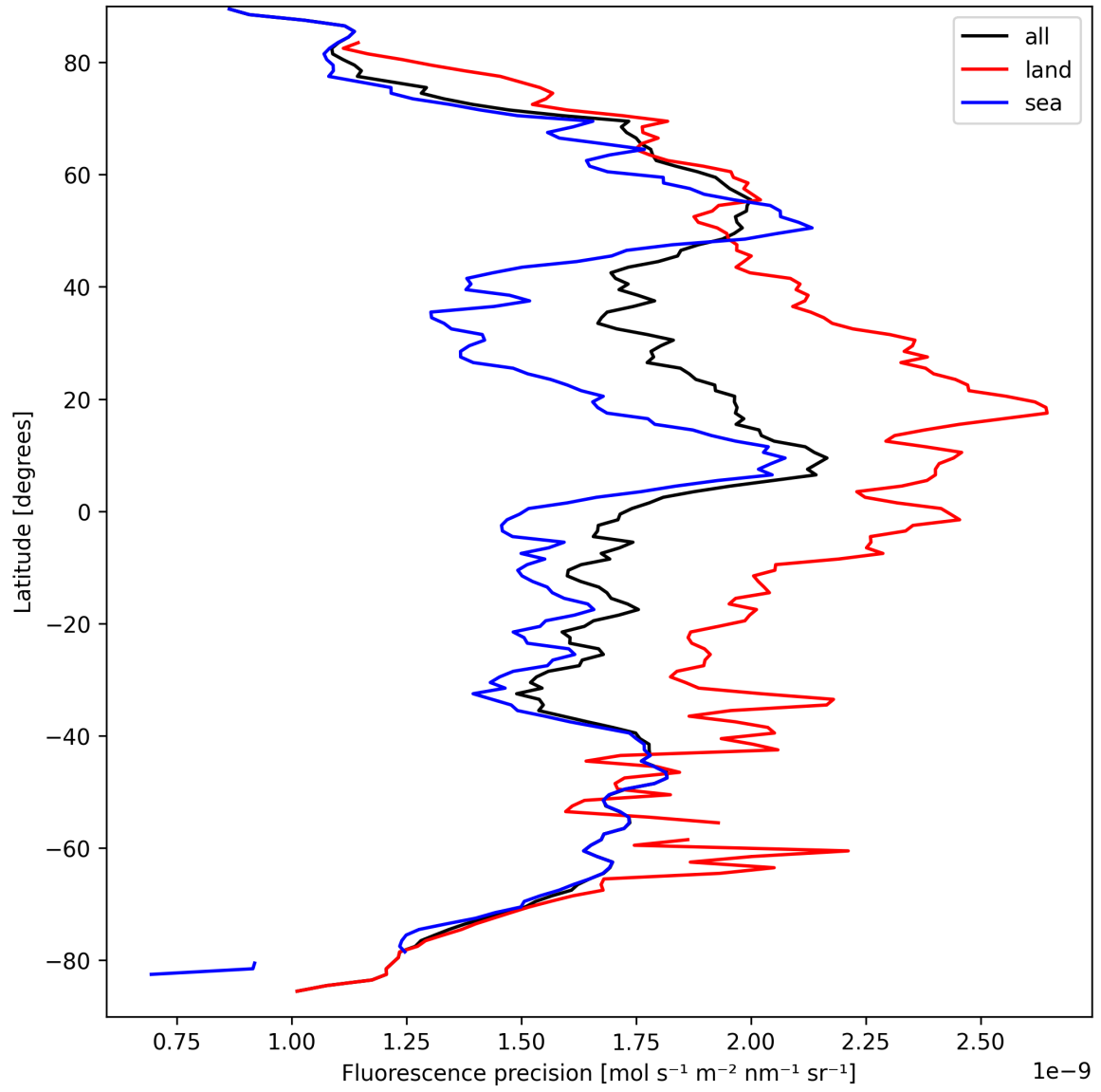
Figure 22: Zonal average of “Fluorescence precision” for 2025-09-16 to 2025-09-17.
