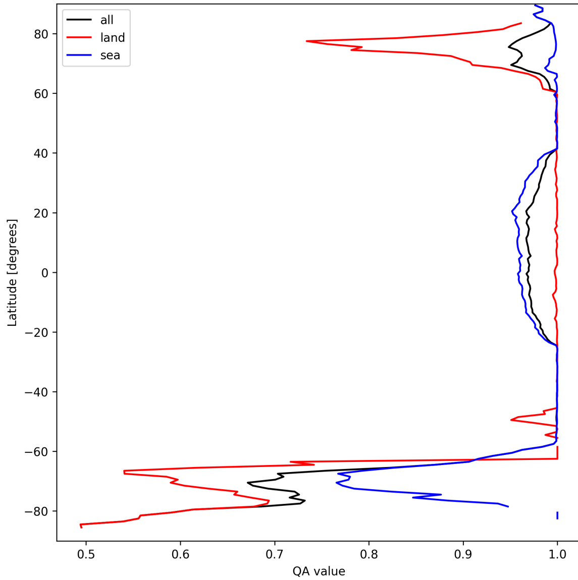
Figure 10: Zonal average of “QA value” for 2025-09-16 to 2025-09-17.
