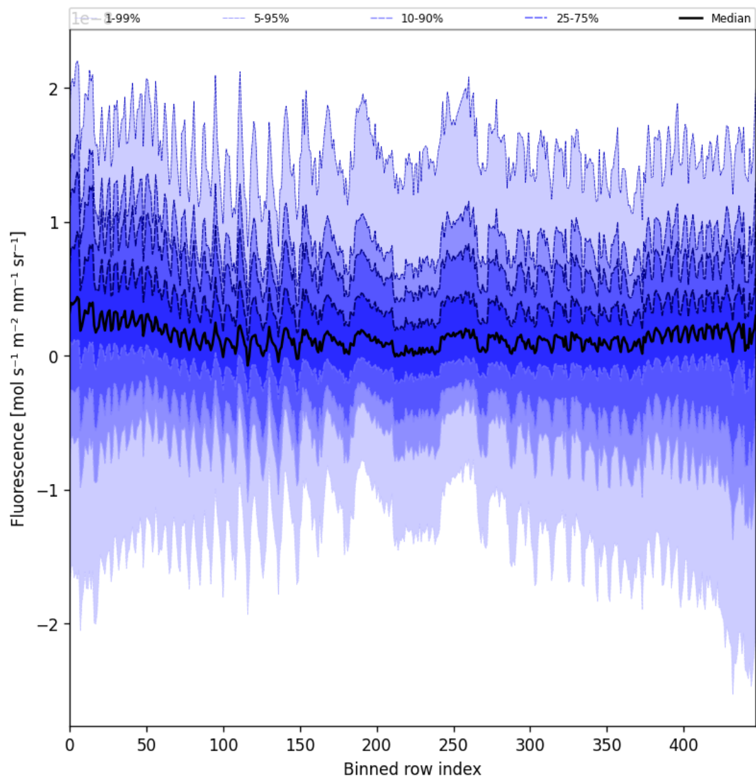
Figure 55: Along track statistics of “Fluorescence” for 2025-09-16 to 2025-09-17
