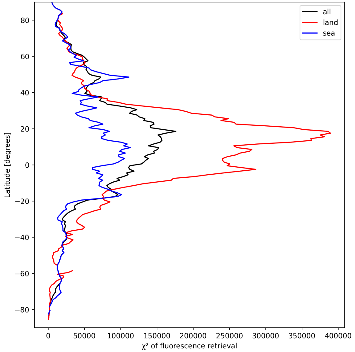
Figure 23: Zonal average of “ \chi^2 of fluorescence retrieval” for 2025-09-16 to 2025-09-17.
