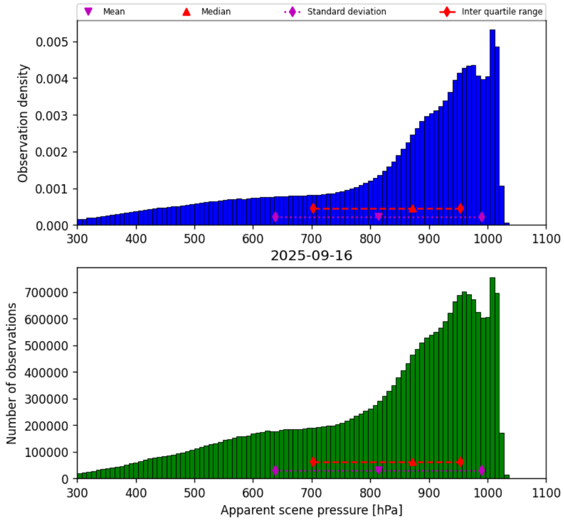
Figure 34: Histogram of “Apparent scene pressure” for 2025-09-16 to 2025-09-17
