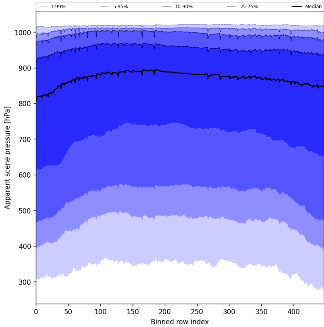
Figure 51: Along track statistics of “Apparent scene pressure” for 2025-09-16 to 2025-09-17
