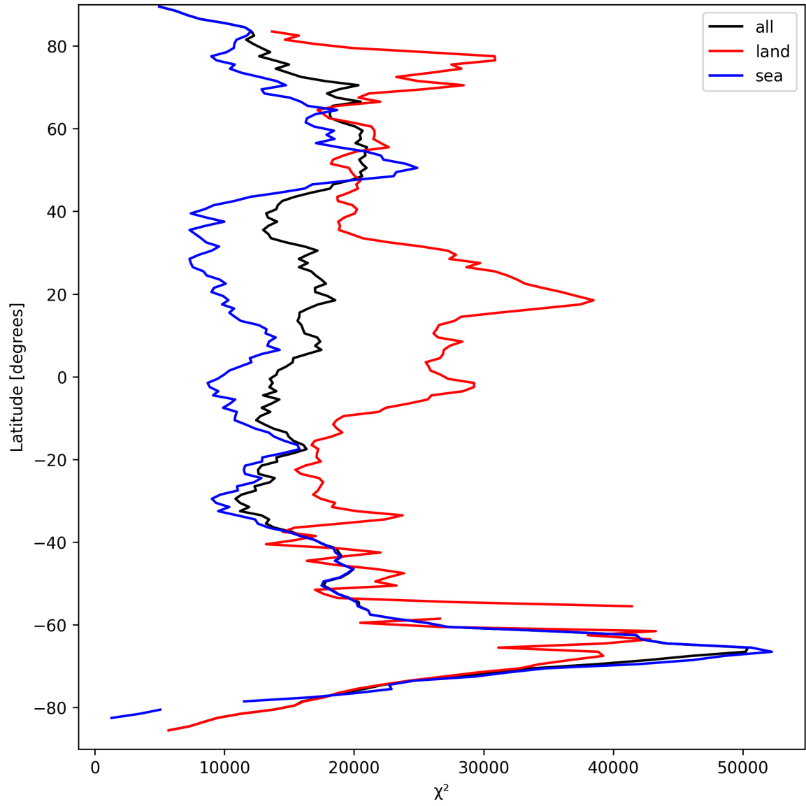
Figure 19: Zonal average of “ \chi^2 ” for 2025-09-16 to 2025-09-17.
