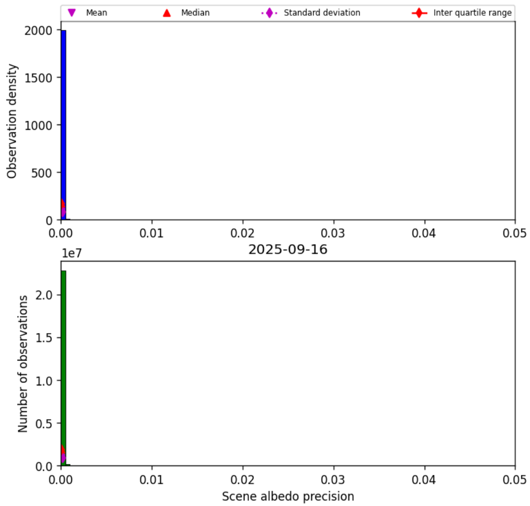
Figure 33: Histogram of “Scene albedo precision” for 2025-09-16 to 2025-09-17
