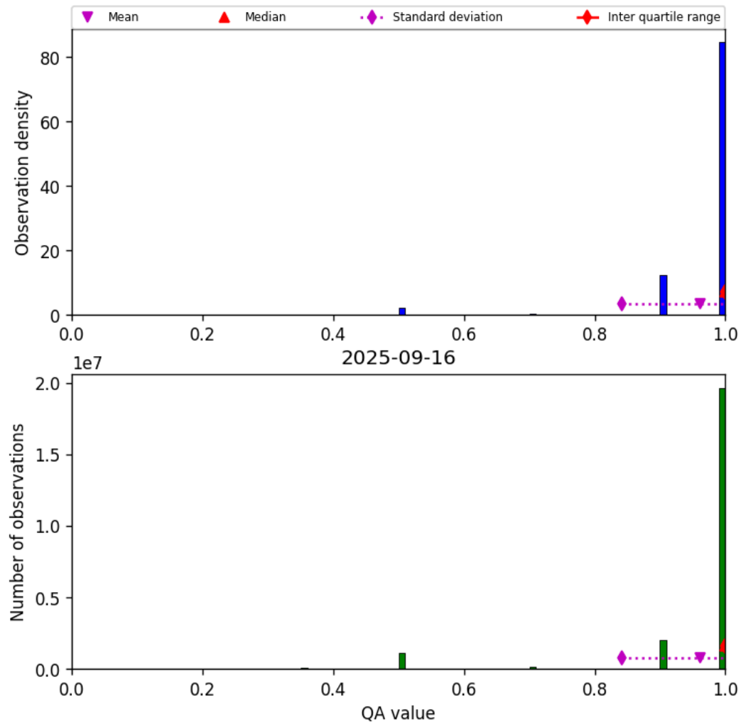
Figure 27: Histogram of “QA value” for 2025-09-16 to 2025-09-17
