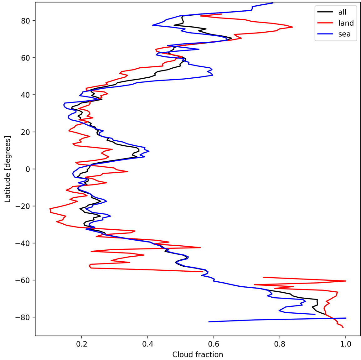
Figure 13: Zonal average of “Cloud fraction” for 2025-09-16 to 2025-09-17.
