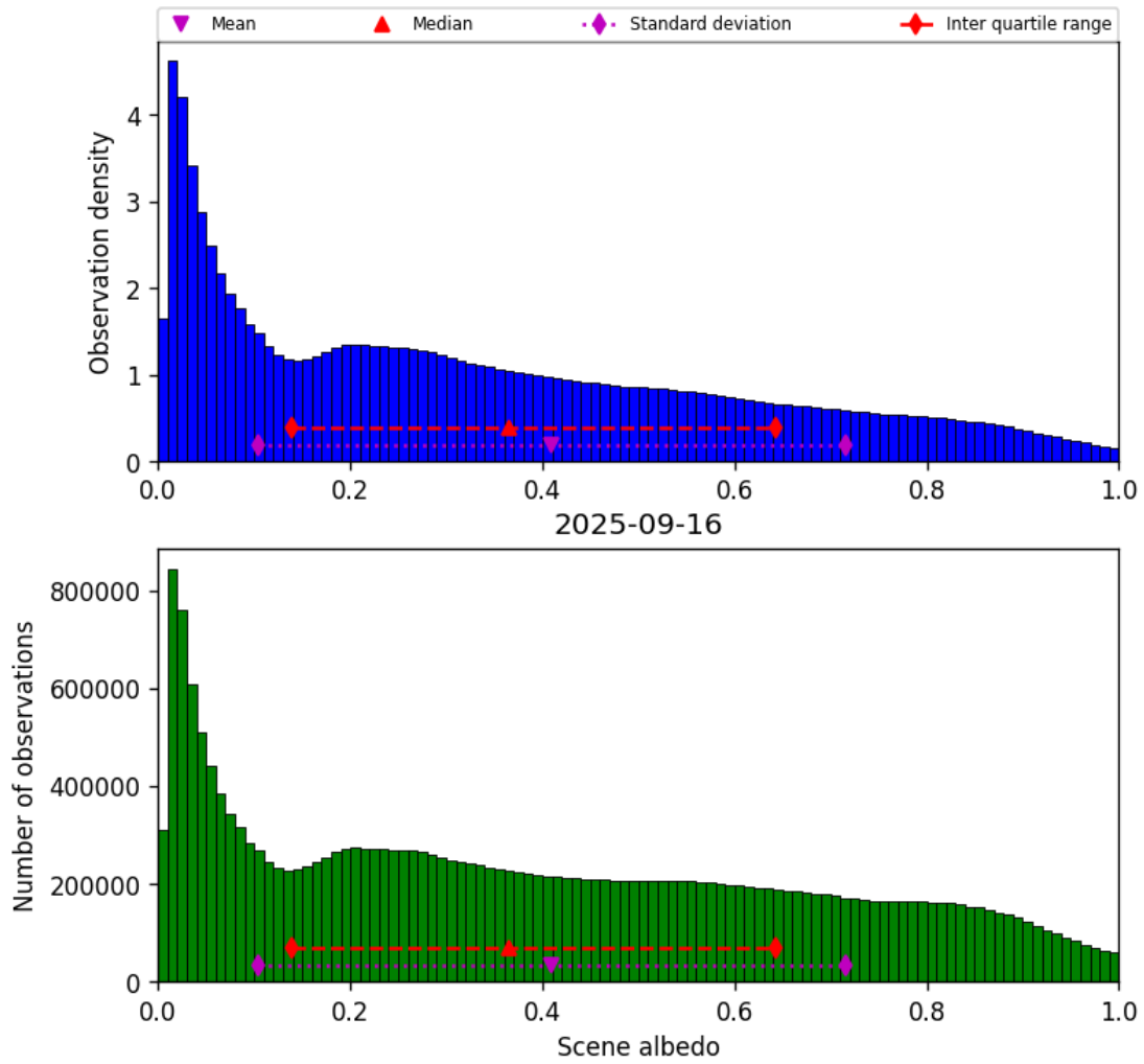
Figure 32: Histogram of “Scene albedo” for 2025-09-16 to 2025-09-17
