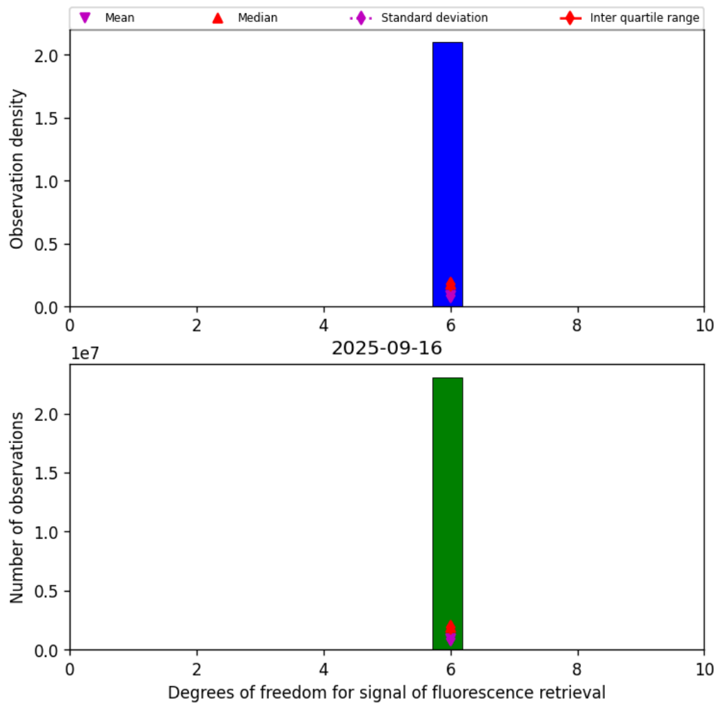
Figure 41: Histogram of “Degrees of freedom for signal of fluorescence retrieval” for 2025-09-16 to 2025-09-17
