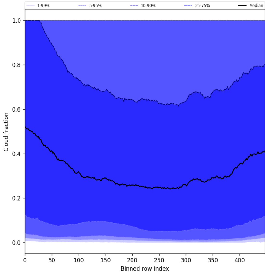
Figure 47: Along track statistics of “Cloud fraction” for 2025-09-16 to 2025-09-17
