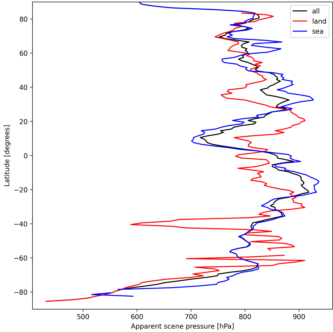
Figure 17: Zonal average of “Apparent scene pressure” for 2025-09-16 to 2025-09-17.
