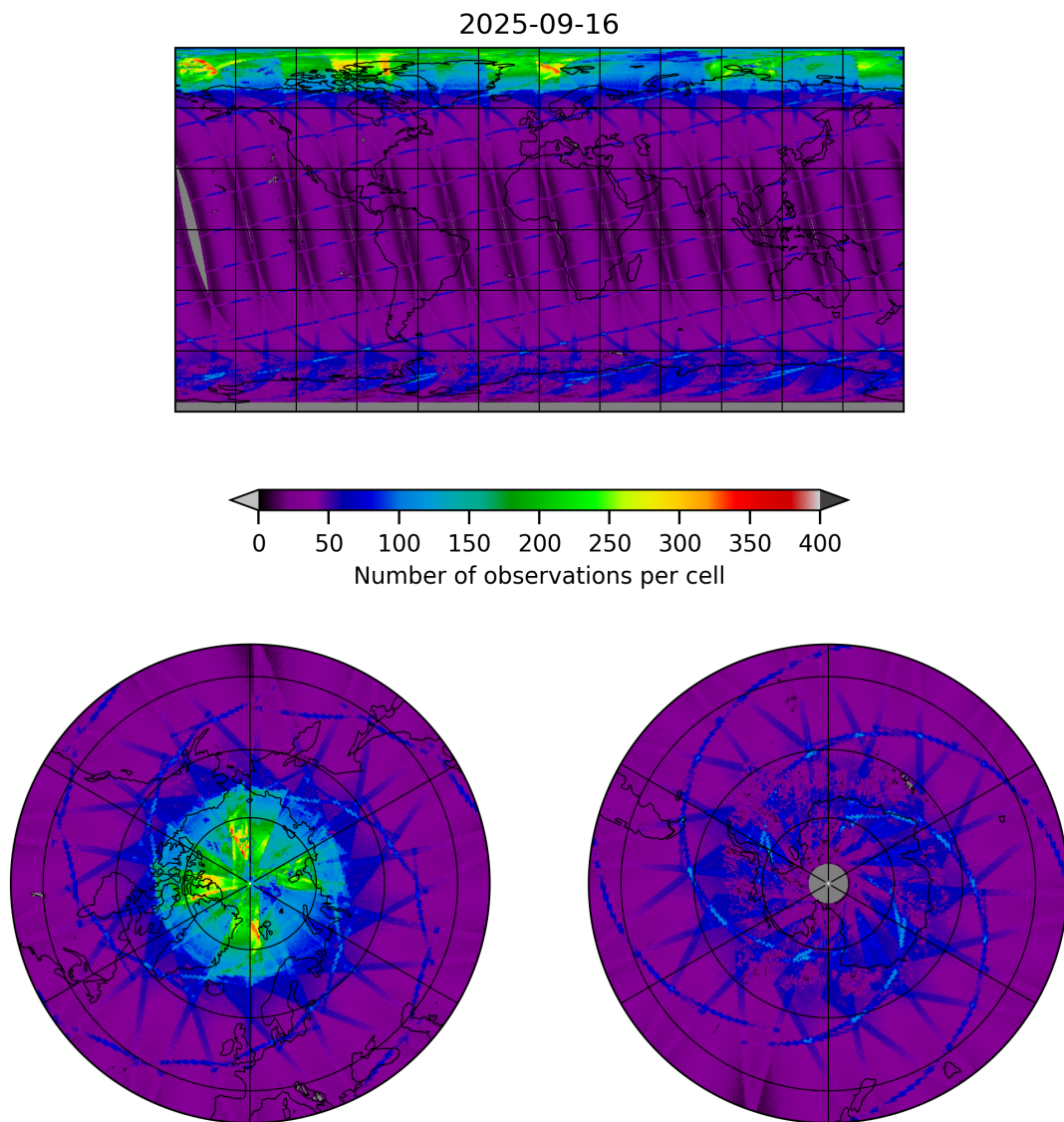
Figure 9: Map of the number of observations for 2025-09-16 to 2025-09-17
