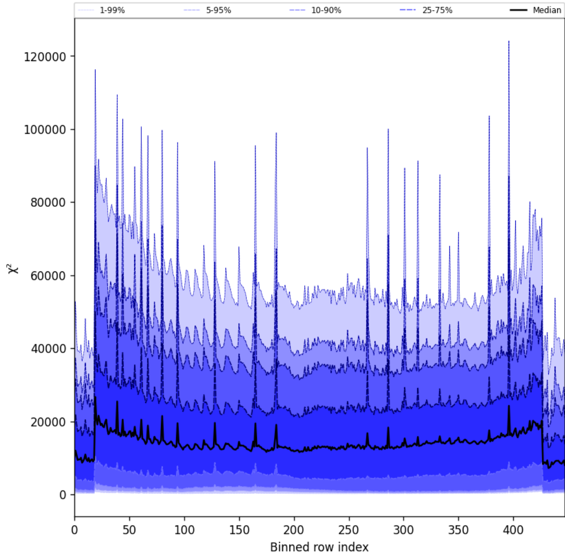
Figure 53: Along track statistics of “ \chi^2 ” for 2025-09-16 to 2025-09-17
