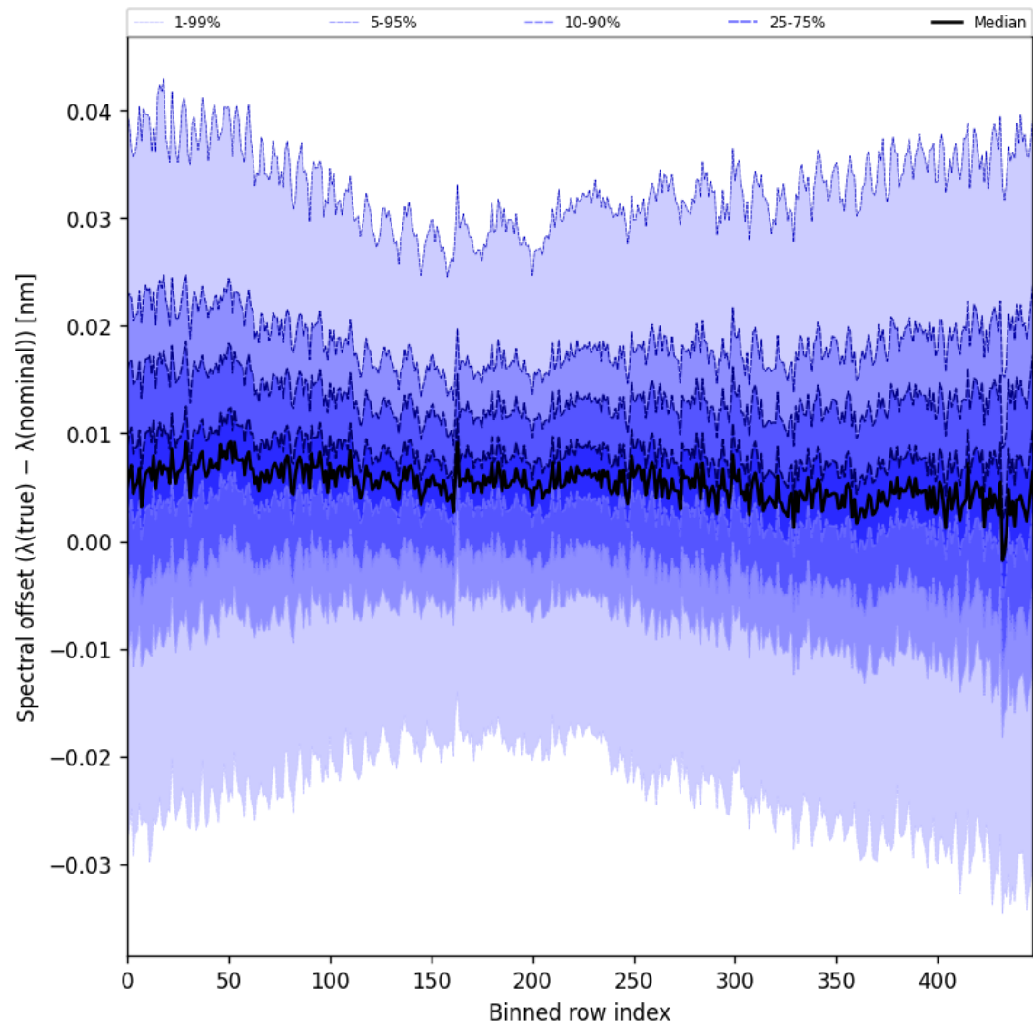
Figure 60: Along track statistics of “Spectral offset ( \lambda_{\text{true}} - \lambda_{\text{nominal}} )” for 2025-09-16 to 2025-09-17
