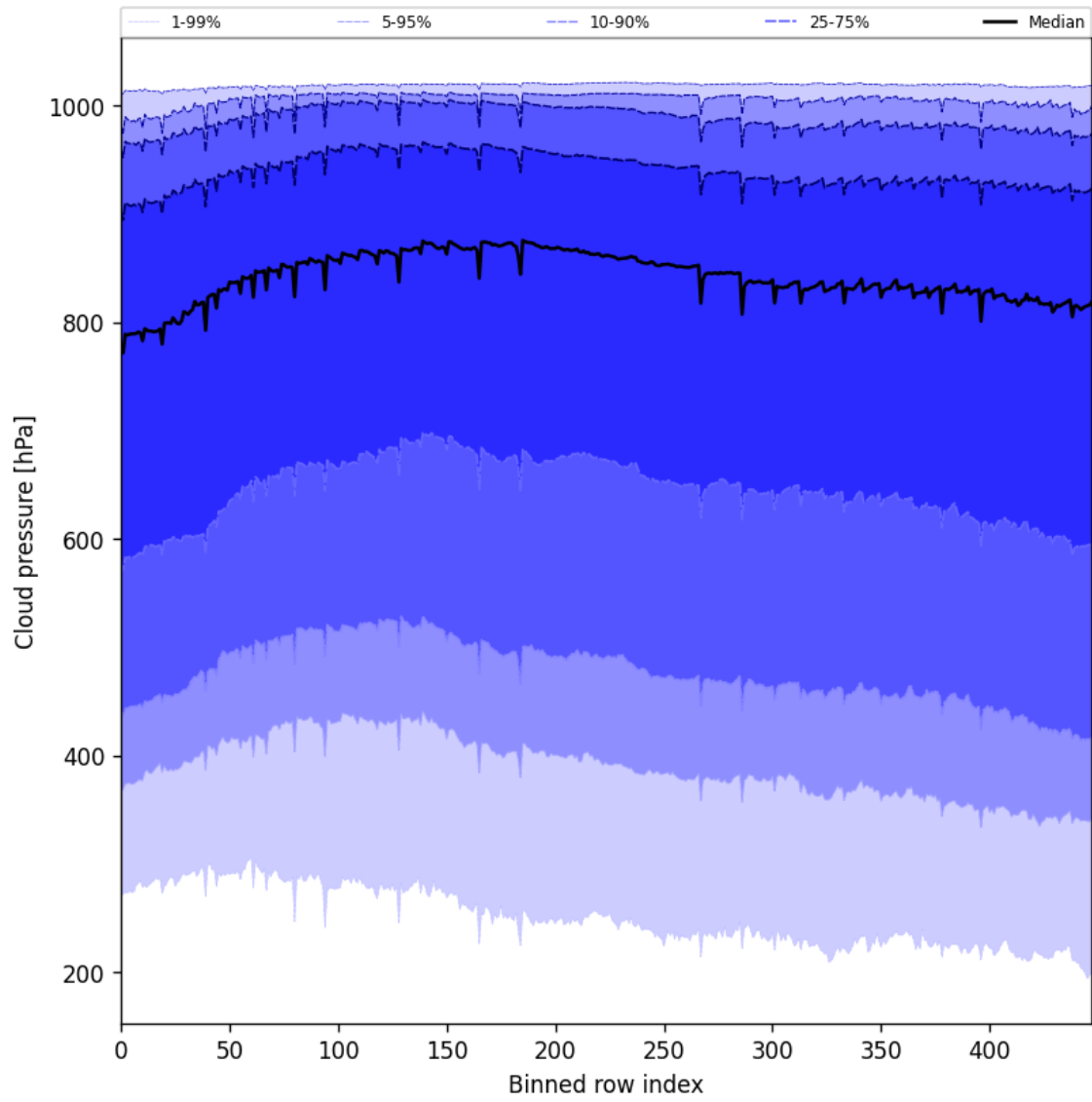
Figure 45: Along track statistics of “Cloud pressure” for 2025-09-16 to 2025-09-17
