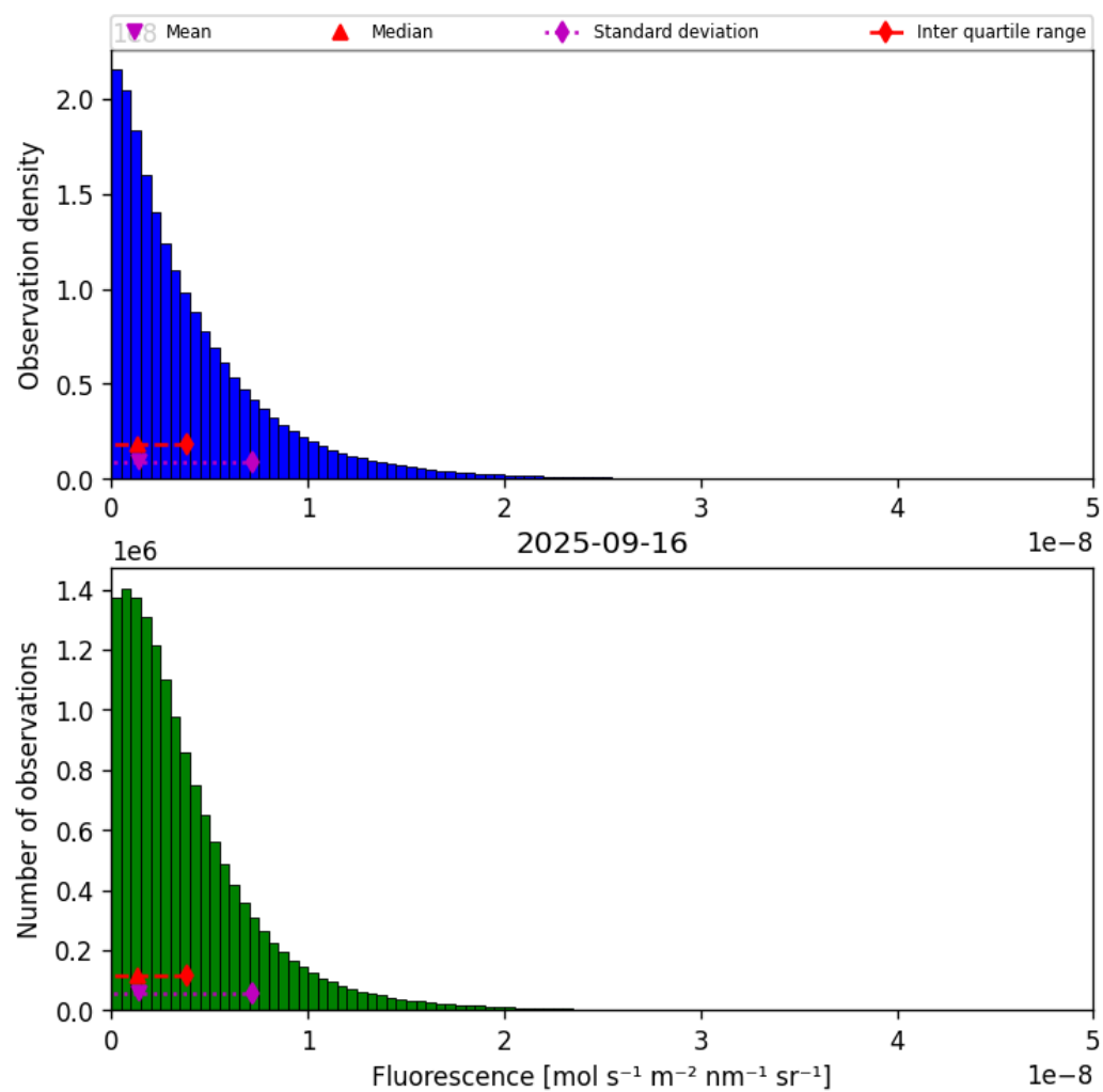
Figure 38: Histogram of “Fluorescence” for 2025-09-16 to 2025-09-17
