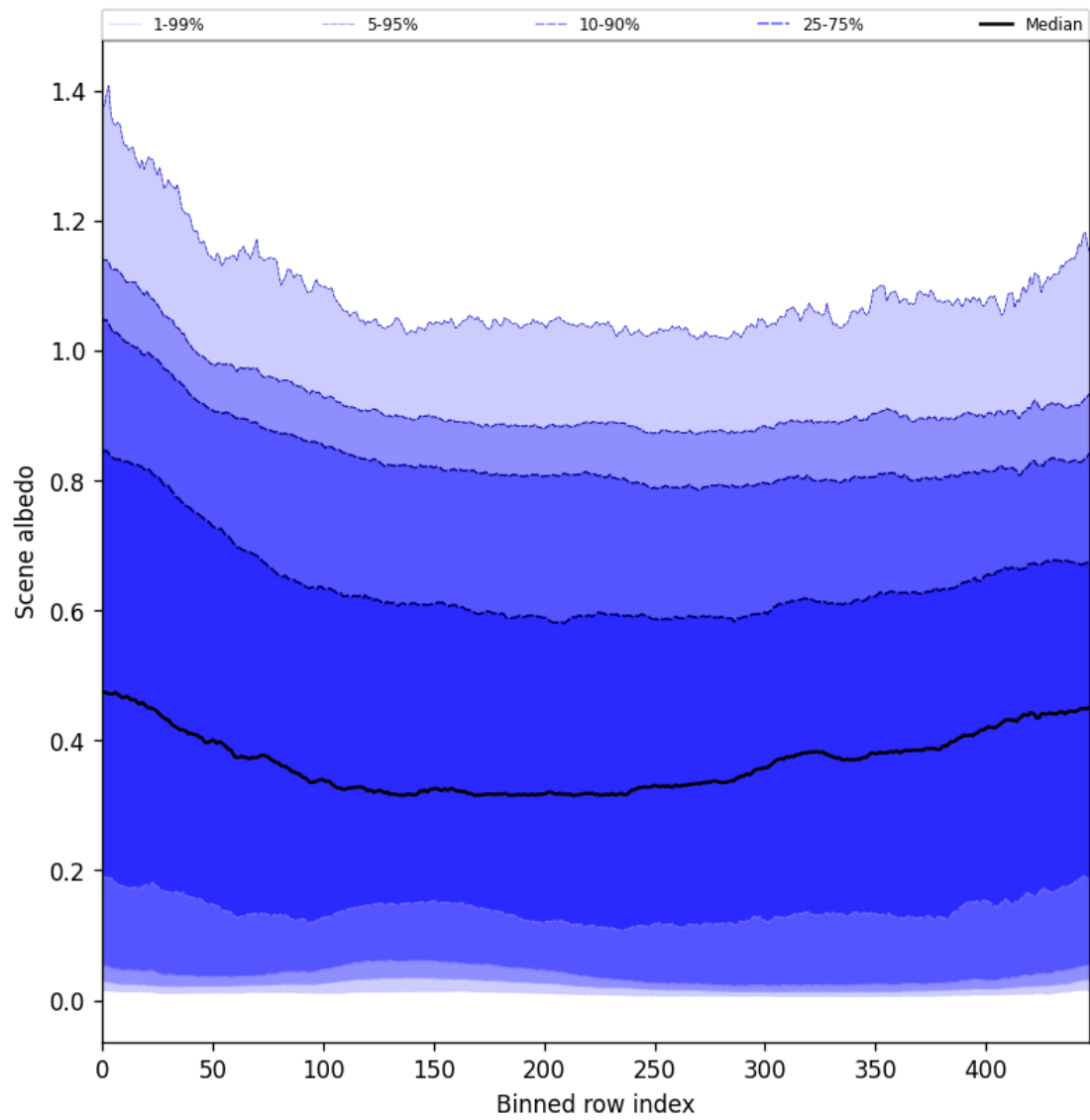
Figure 49: Along track statistics of “Scene albedo” for 2025-09-16 to 2025-09-17
