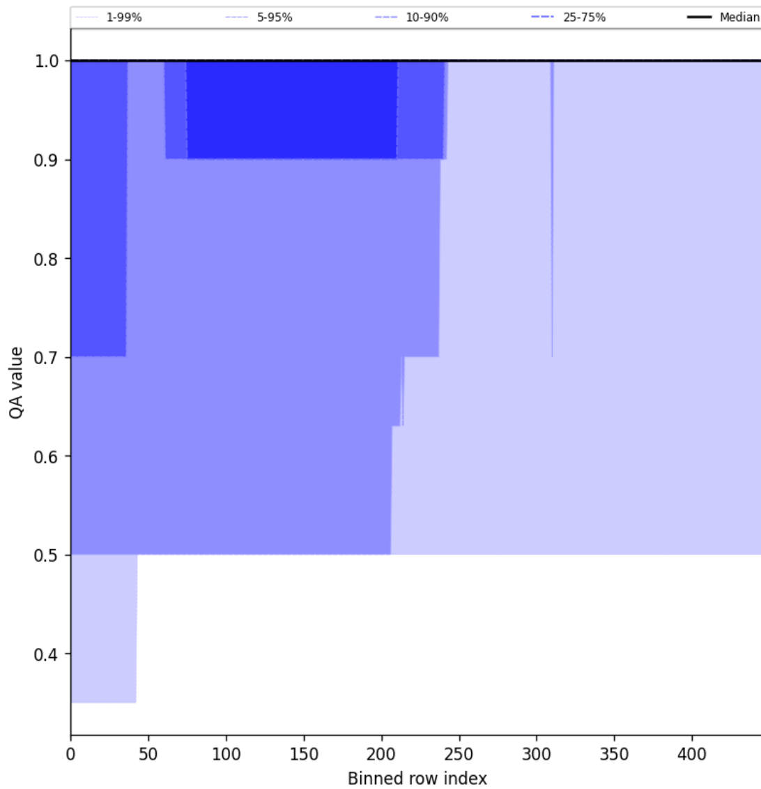
Figure 44: Along track statistics of “QA value” for 2025-09-16 to 2025-09-17
