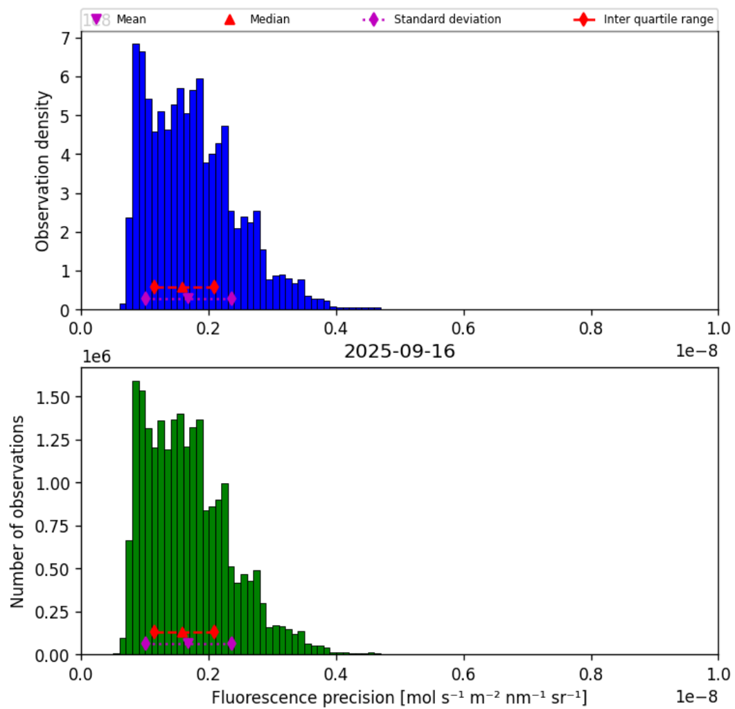
Figure 39: Histogram of “Fluorescence precision” for 2025-09-16 to 2025-09-17
