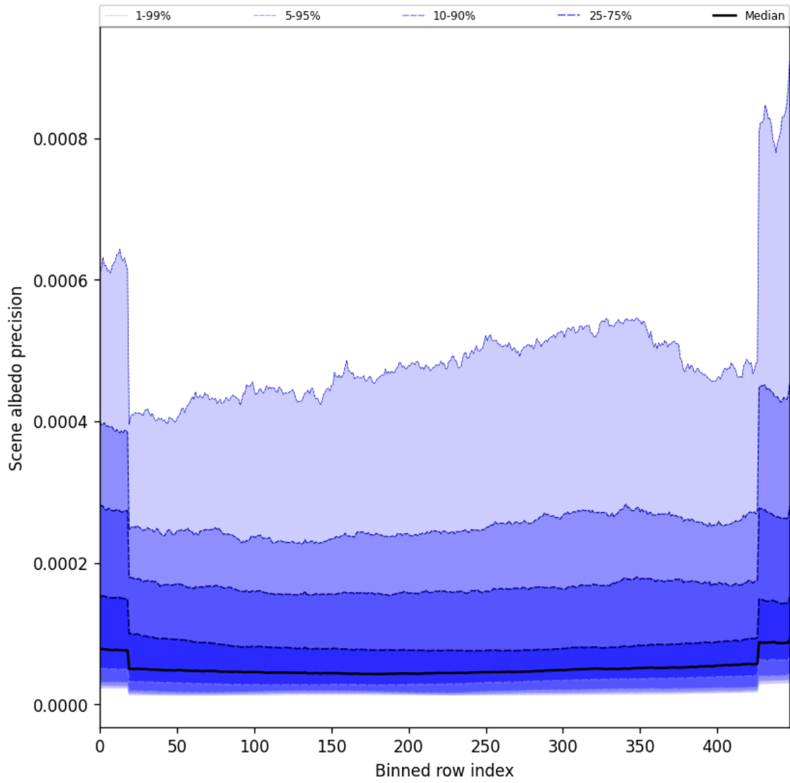
Figure 50: Along track statistics of “Scene albedo precision” for 2025-09-16 to 2025-09-17
