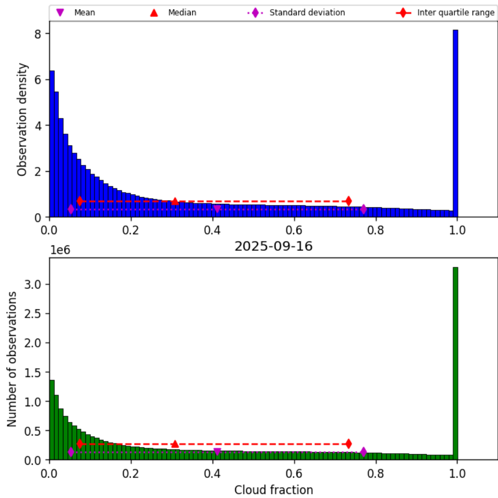
Figure 30: Histogram of “Cloud fraction” for 2025-09-16 to 2025-09-17
