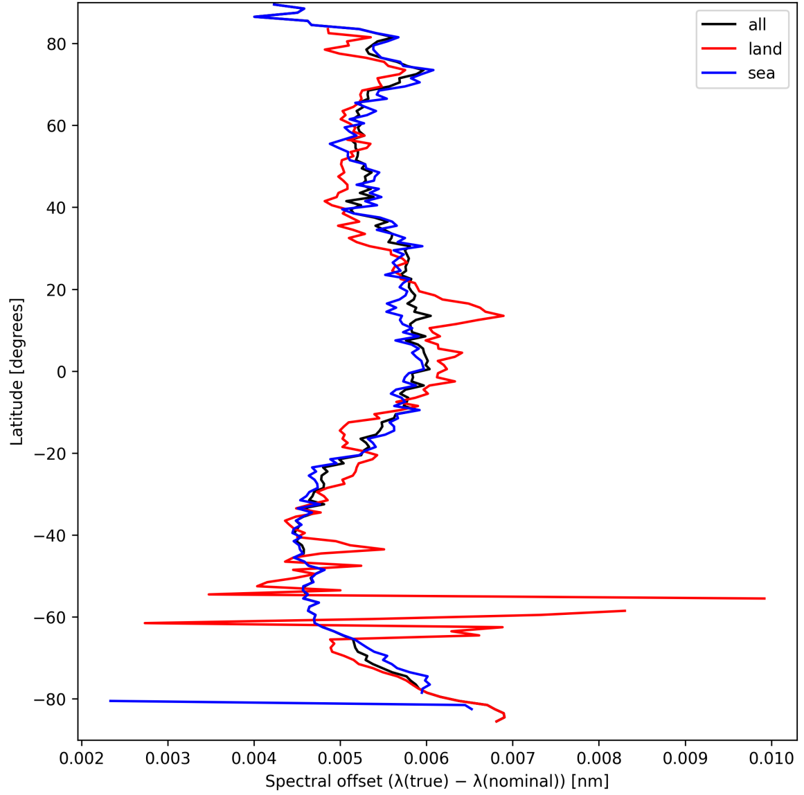
Figure 26: Zonal average of “Spectral offset ( \lambda_{\text{true}} - \lambda_{\text{nominal}} )” for 2025-09-16 to 2025-09-17.
