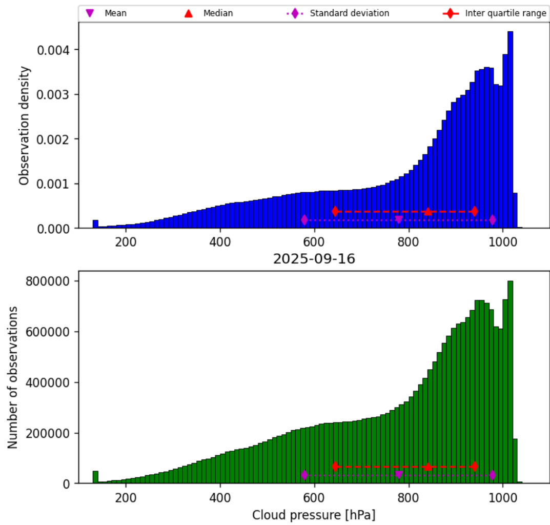
Figure 28: Histogram of “Cloud pressure” for 2025-09-16 to 2025-09-17
