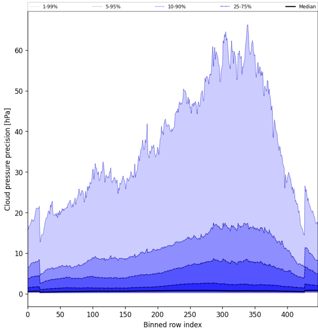
Figure 46: Along track statistics of “Cloud pressure precision” for 2025-09-16 to 2025-09-17
