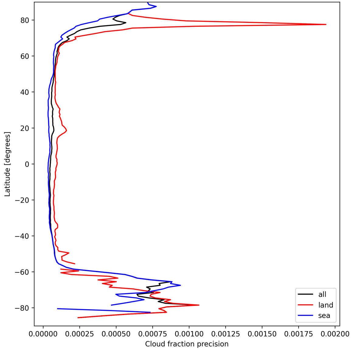
Figure 14: Zonal average of “Cloud fraction precision” for 2025-09-16 to 2025-09-17.
