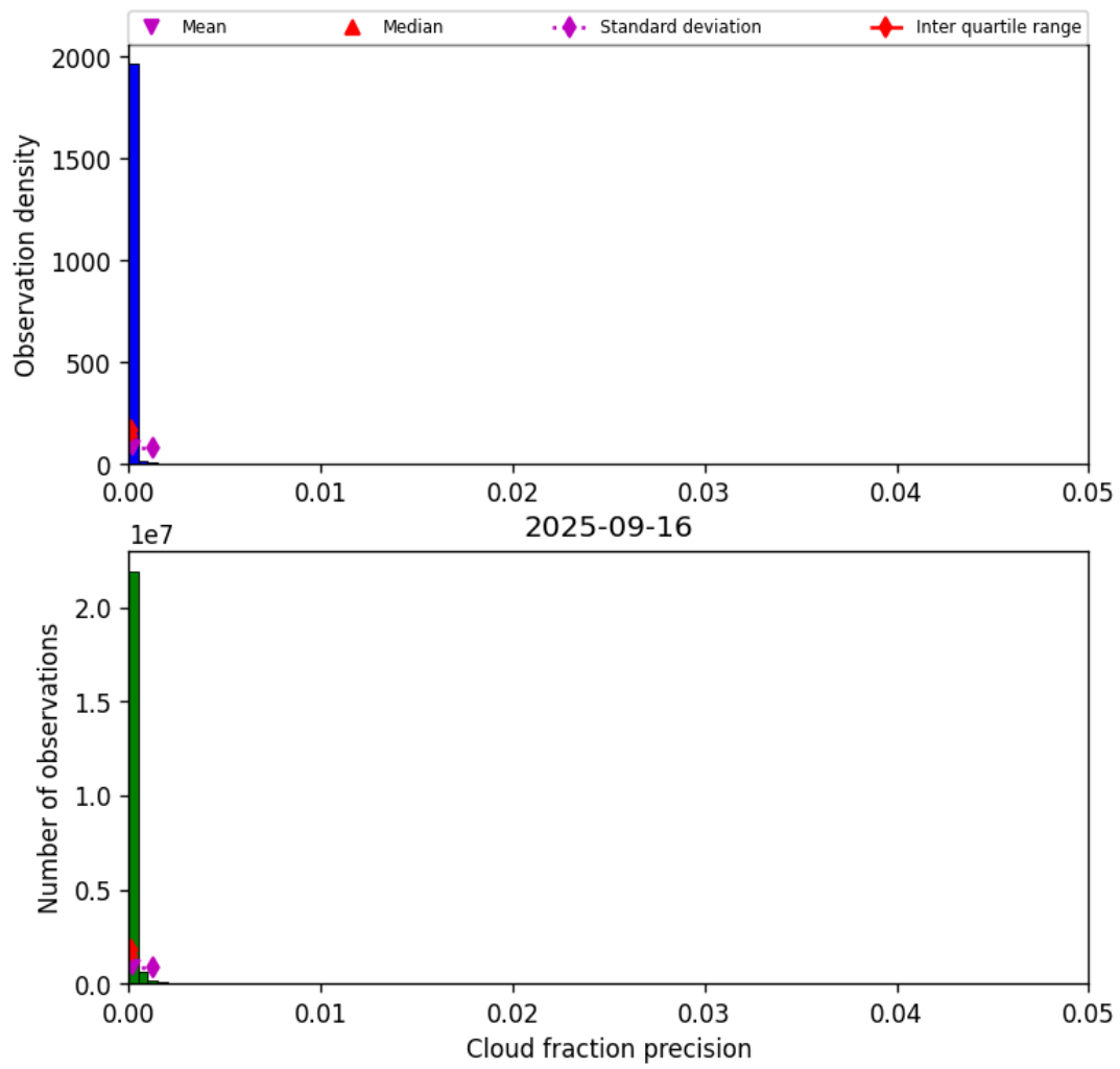
Figure 31: Histogram of “Cloud fraction precision” for 2025-09-16 to 2025-09-17
