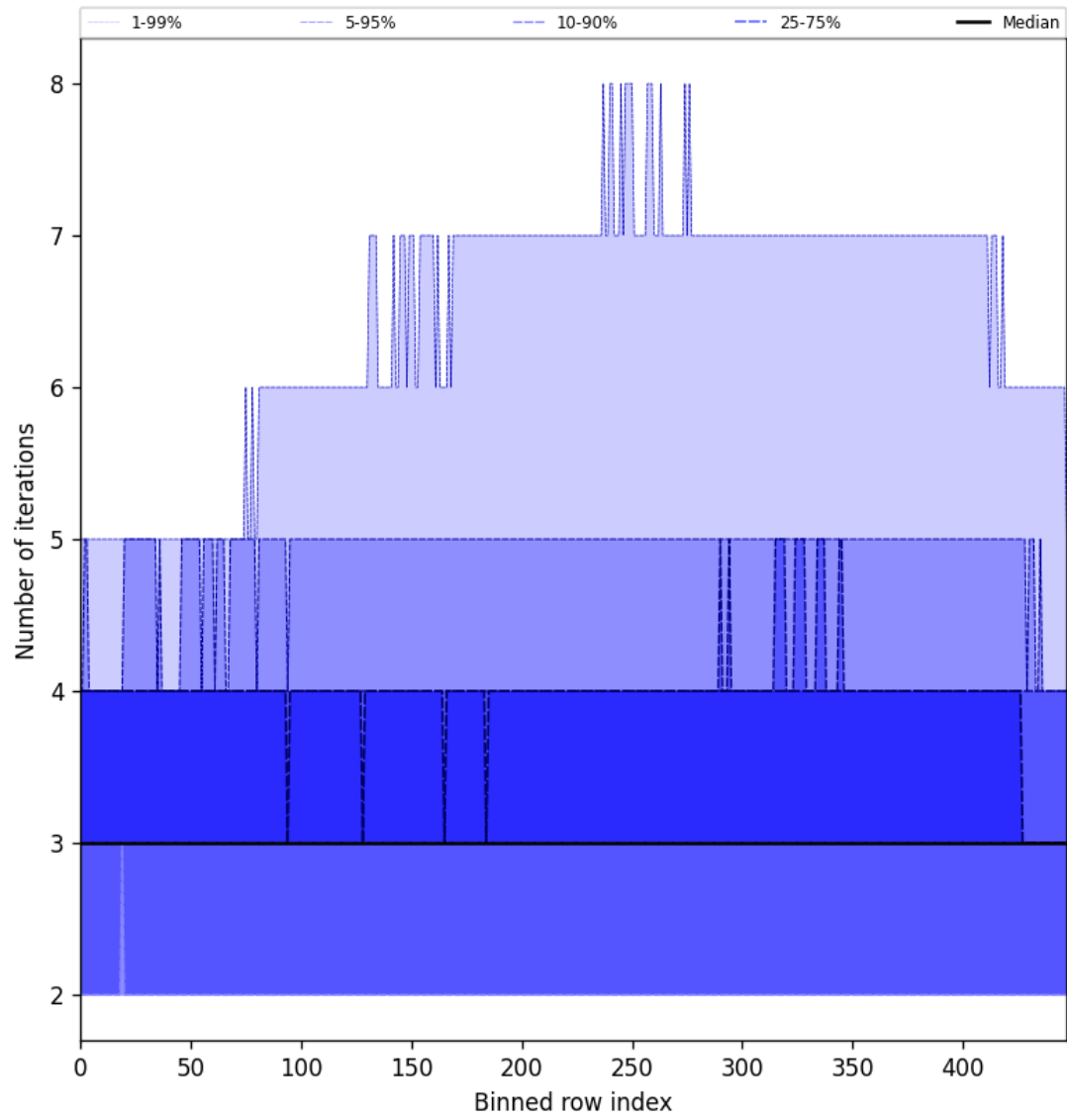
Figure 54: Along track statistics of “Number of iterations” for 2025-09-16 to 2025-09-17
