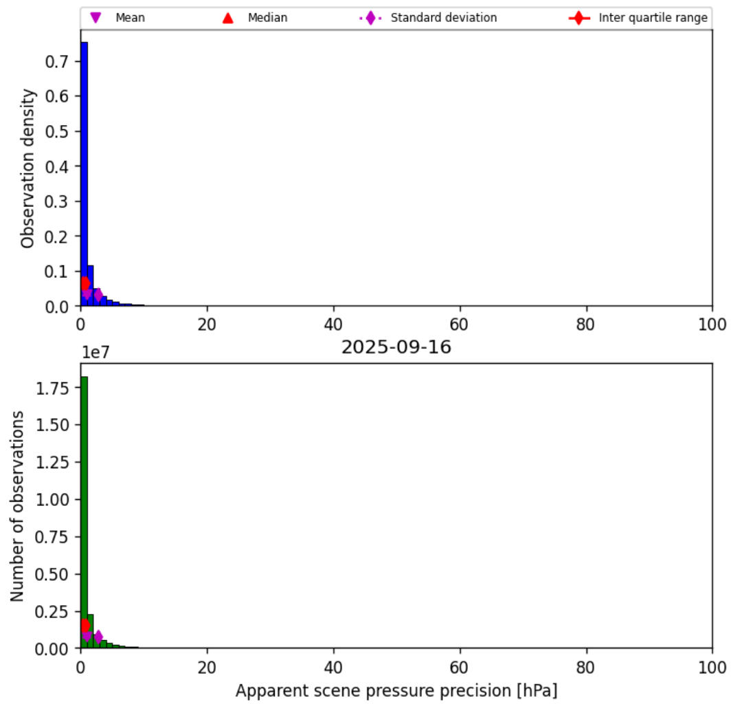
Figure 35: Histogram of “Apparent scene pressure precision” for 2025-09-16 to 2025-09-17
