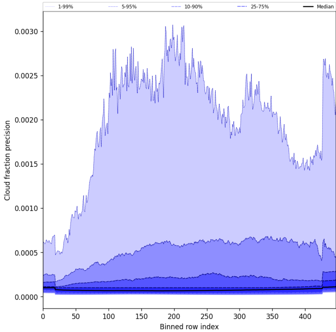
Figure 48: Along track statistics of “Cloud fraction precision” for 2025-09-16 to 2025-09-17
