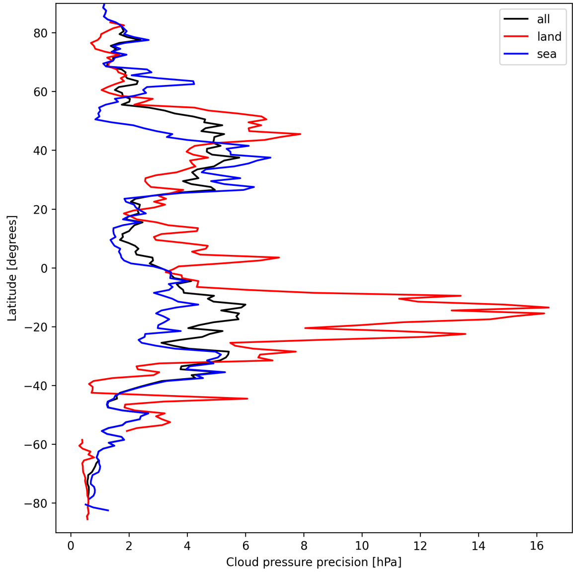
Figure 12: Zonal average of “Cloud pressure precision” for 2025-09-16 to 2025-09-17.
