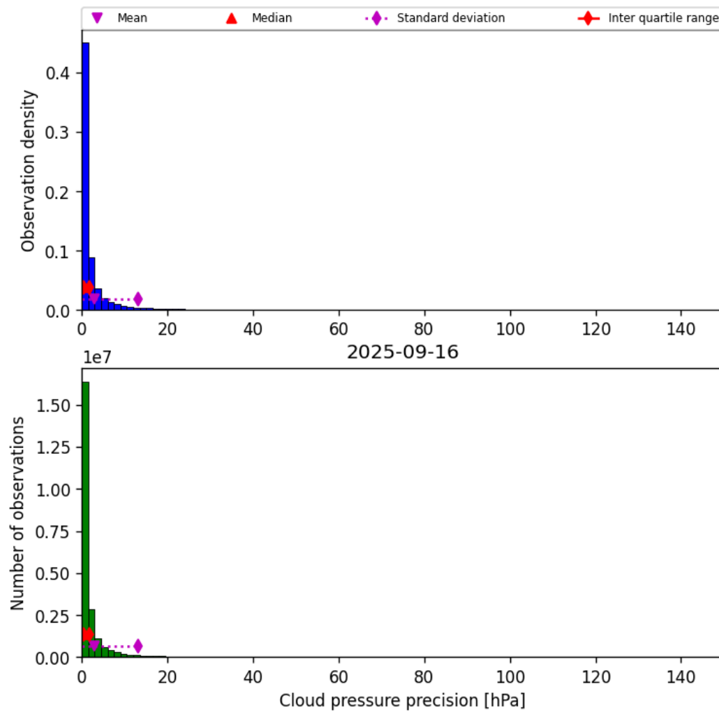
Figure 29: Histogram of “Cloud pressure precision” for 2025-09-16 to 2025-09-17
