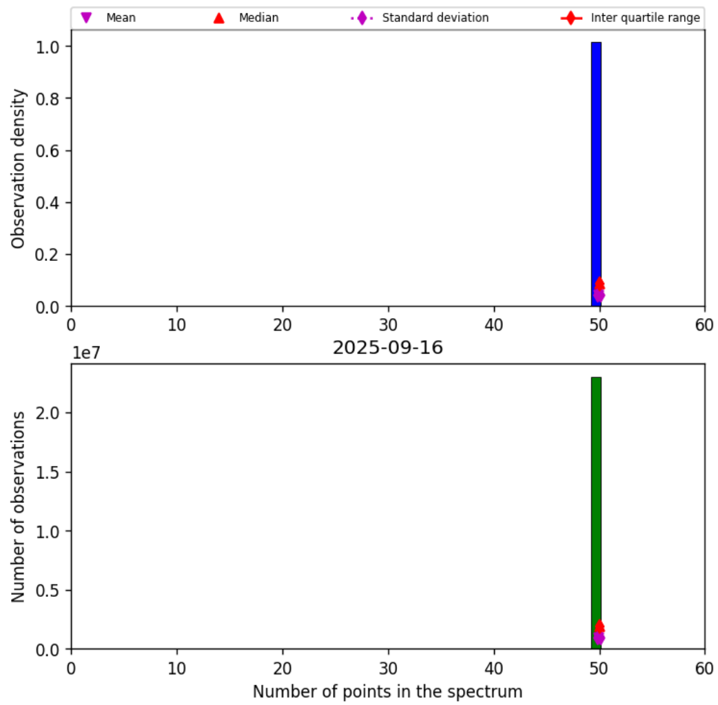
Figure 42: Histogram of “Number of points in the spectrum” for 2025-09-16 to 2025-09-17
