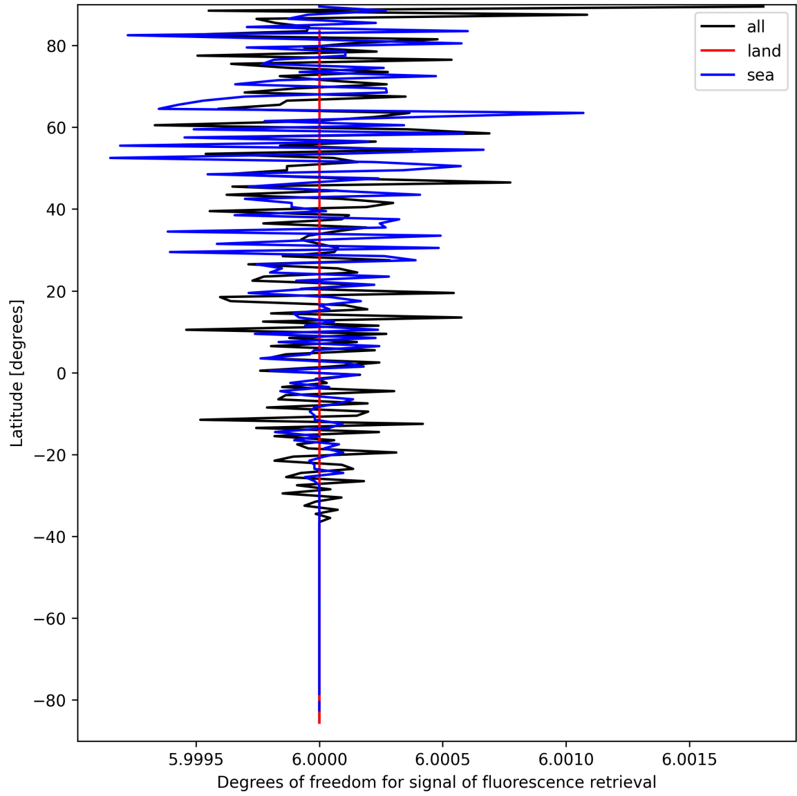
Figure 24: Zonal average of “Degrees of freedom for signal of fluorescence retrieval” for 2025-09-16 to 2025-09-17.
