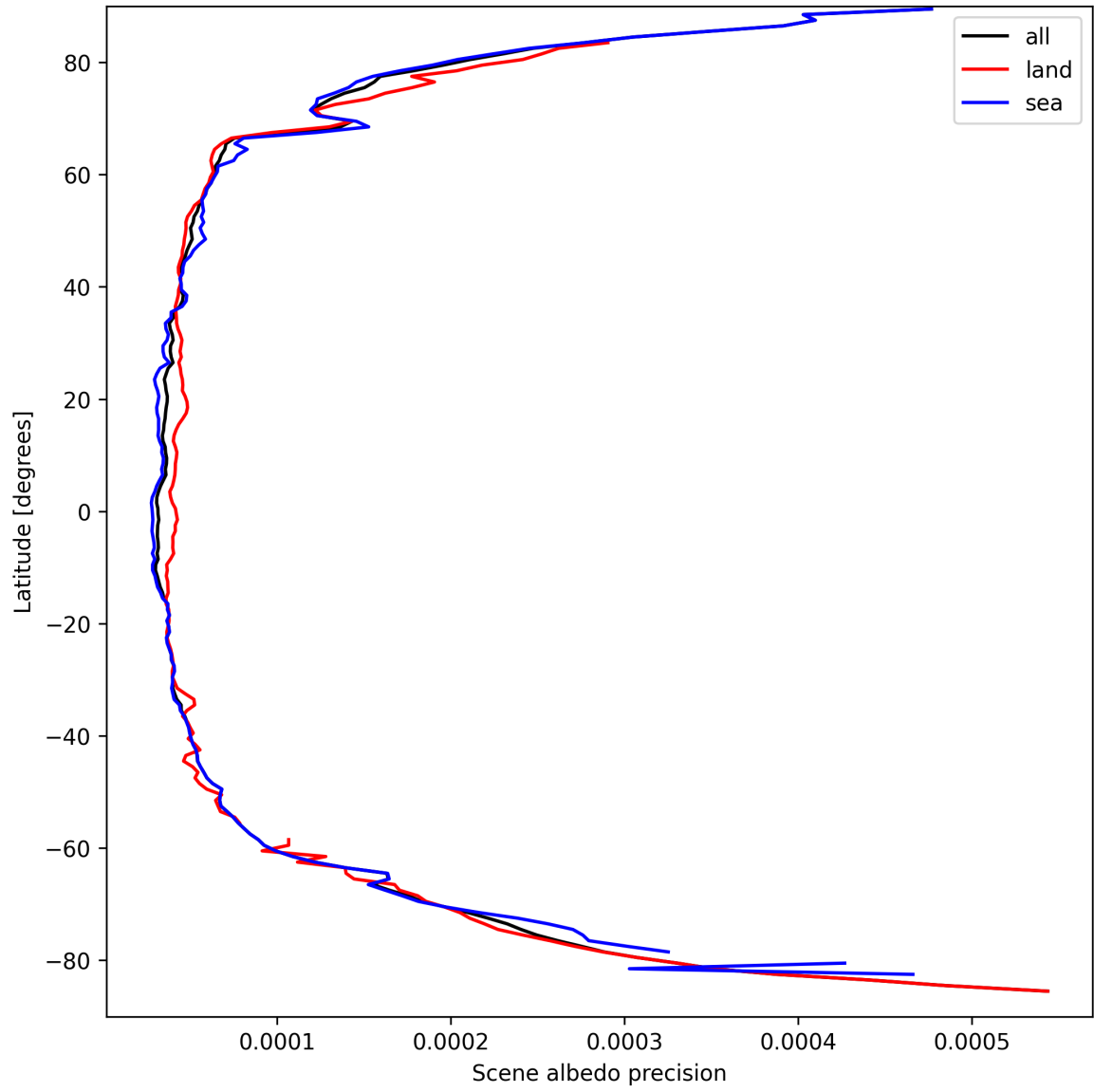
Figure 16: Zonal average of “Scene albedo precision” for 2025-09-16 to 2025-09-17.
