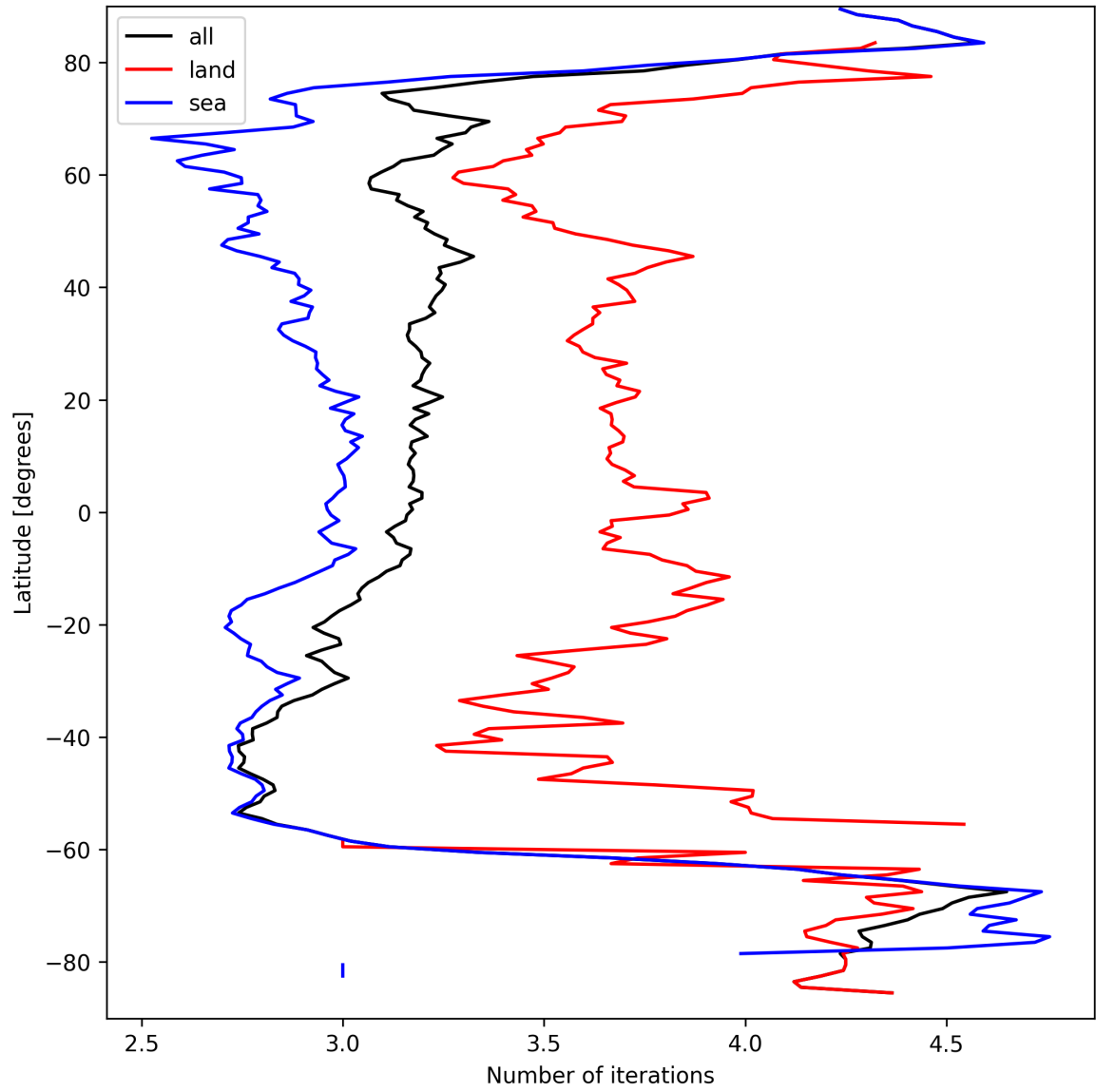
Figure 20: Zonal average of “Number of iterations” for 2025-09-16 to 2025-09-17.
