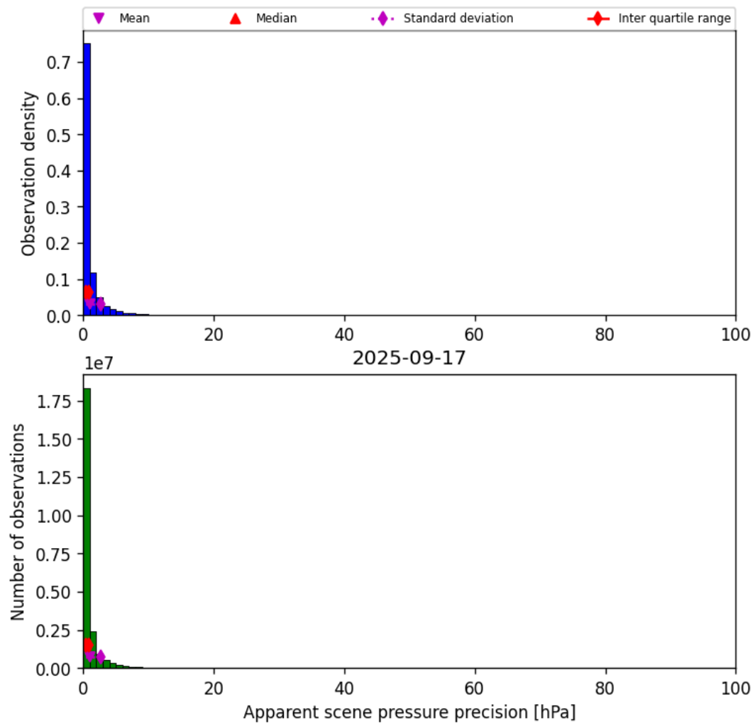
Figure 35: Histogram of “Apparent scene pressure precision” for 2025-09-17 to 2025-09-18
