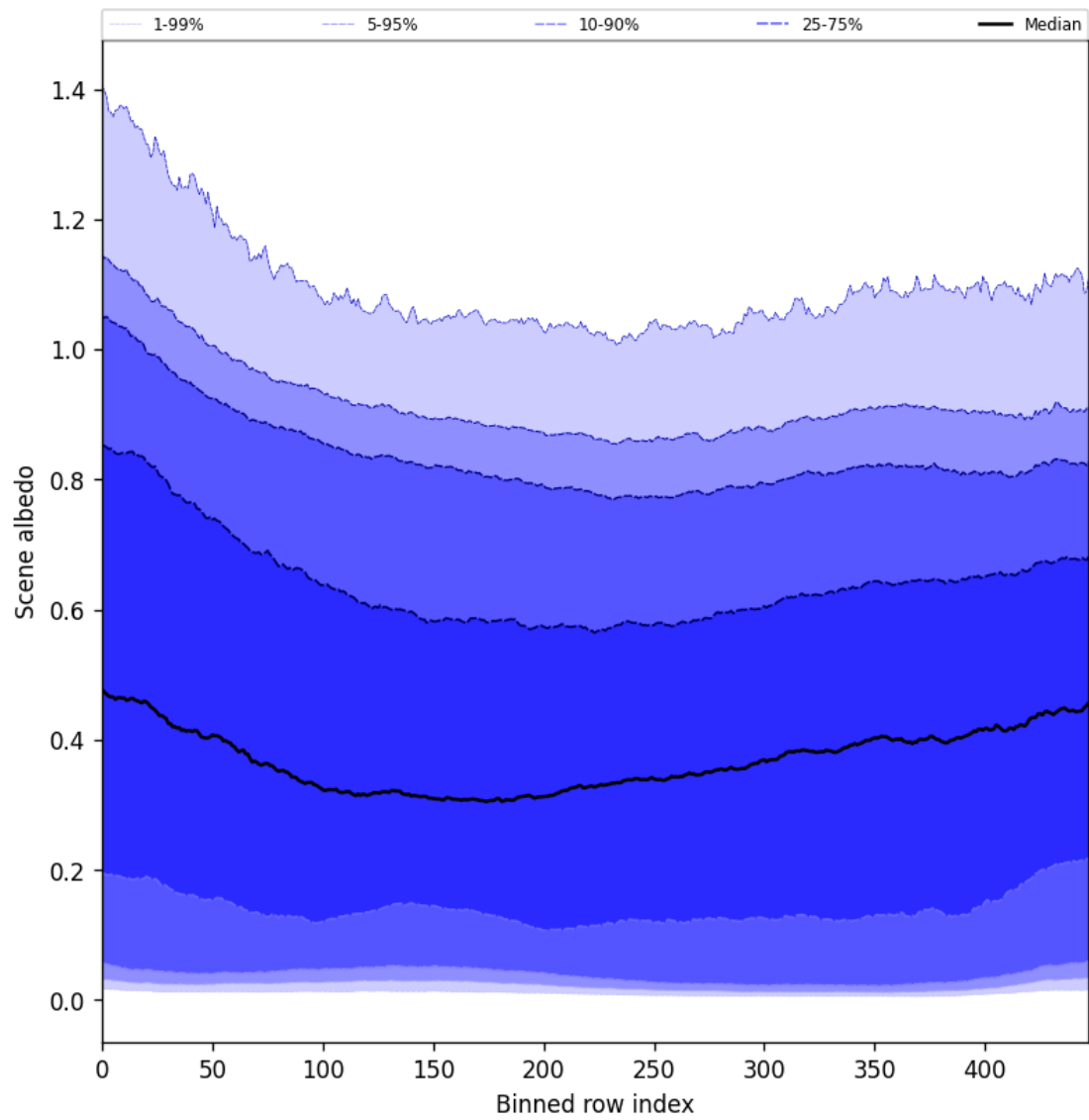
Figure 49: Along track statistics of “Scene albedo” for 2025-09-17 to 2025-09-18
