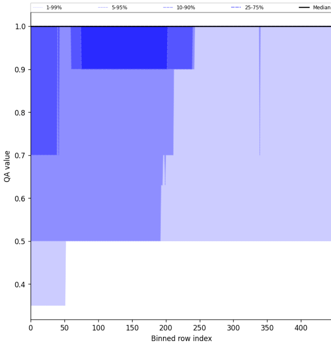
Figure 44: Along track statistics of “QA value” for 2025-09-17 to 2025-09-18
