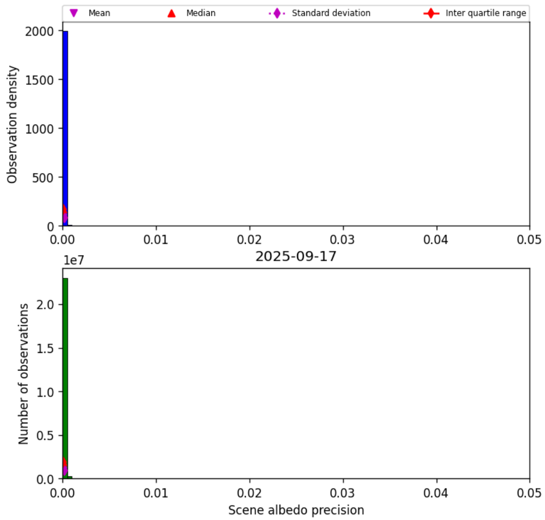
Figure 33: Histogram of “Scene albedo precision” for 2025-09-17 to 2025-09-18
