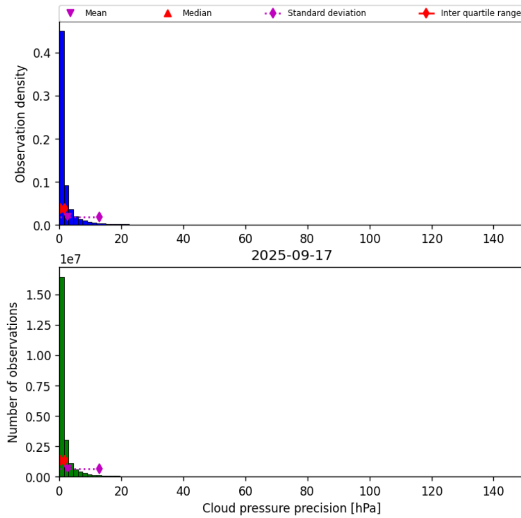
Figure 29: Histogram of "Cloud pressure precision" for 2025-09-17 to 2025-09-18
