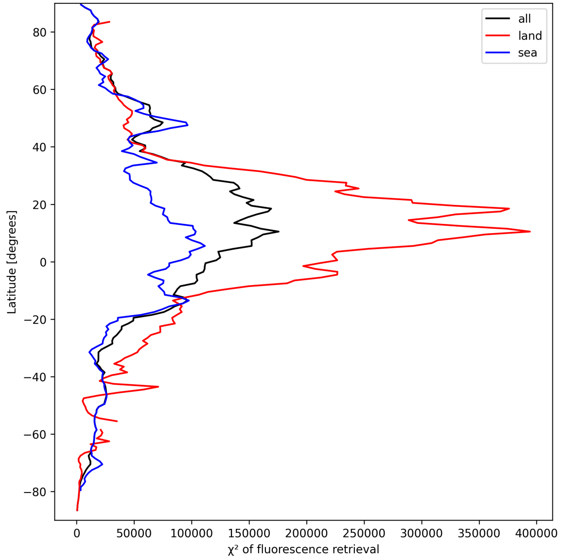
Figure 23: Zonal average of “ \chi^2 of fluorescence retrieval” for 2025-09-17 to 2025-09-18.
