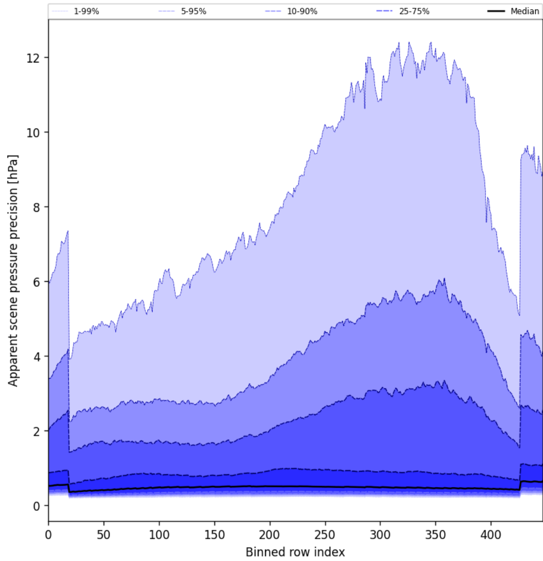
Figure 52: Along track statistics of “Apparent scene pressure precision” for 2025-09-17 to 2025-09-18
