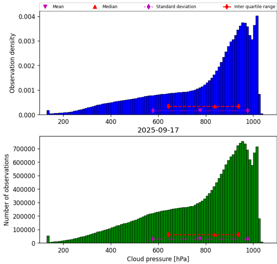
Figure 28: Histogram of “Cloud pressure” for 2025-09-17 to 2025-09-18
