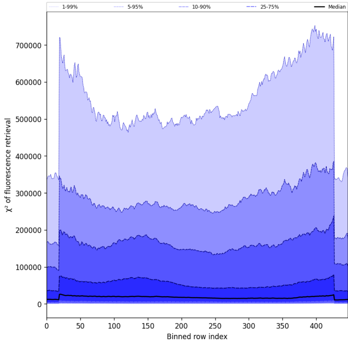
Figure 57: Along track statistics of “ \chi^2 of fluorescence retrieval” for 2025-09-17 to 2025-09-18
