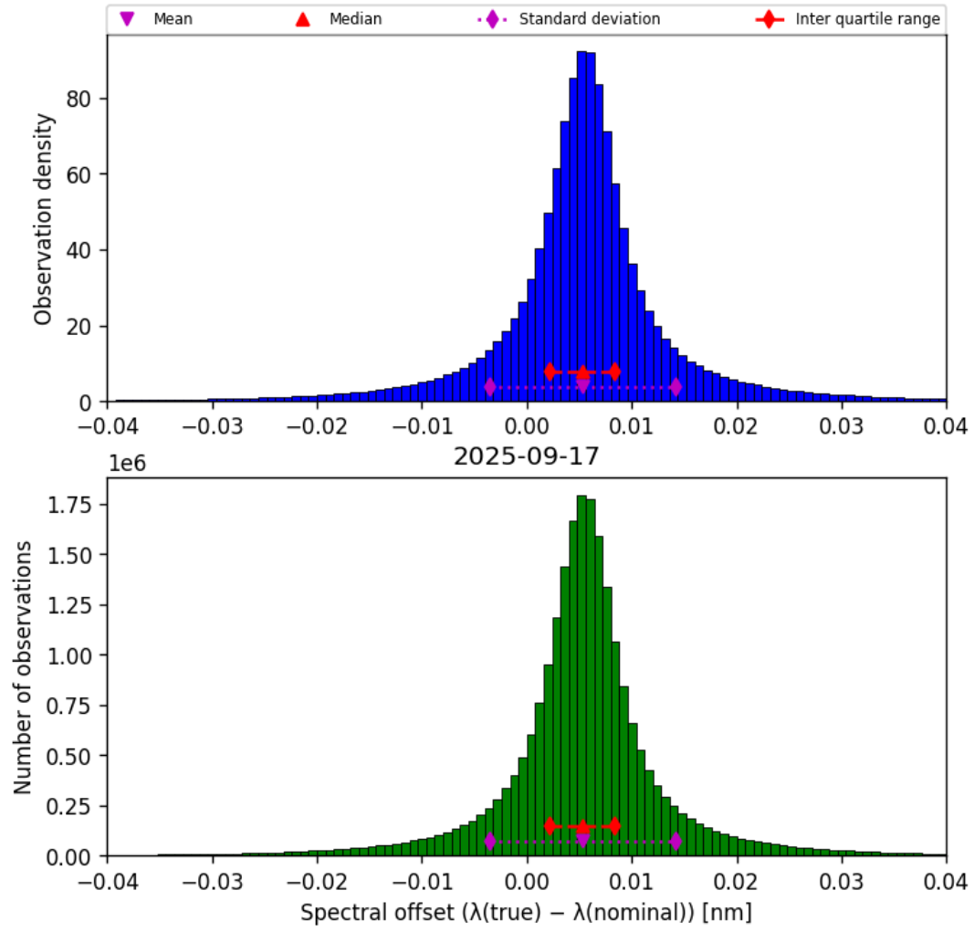
Figure 43: Histogram of “Spectral offset ( \lambda_{\text{true}} - \lambda_{\text{nominal}} )” for 2025-09-17 to 2025-09-18
