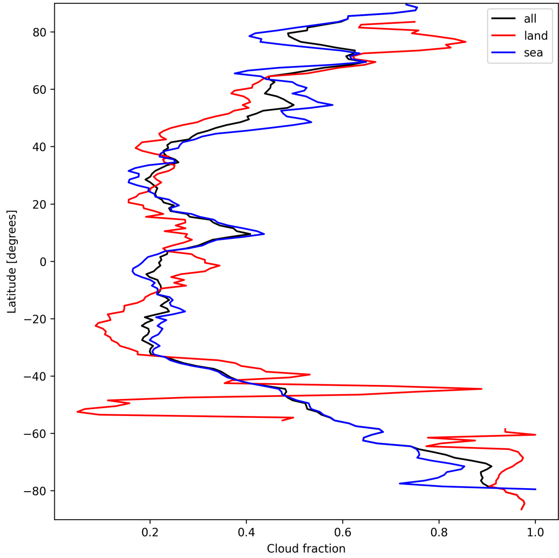
Figure 13: Zonal average of “Cloud fraction” for 2025-09-17 to 2025-09-18.
