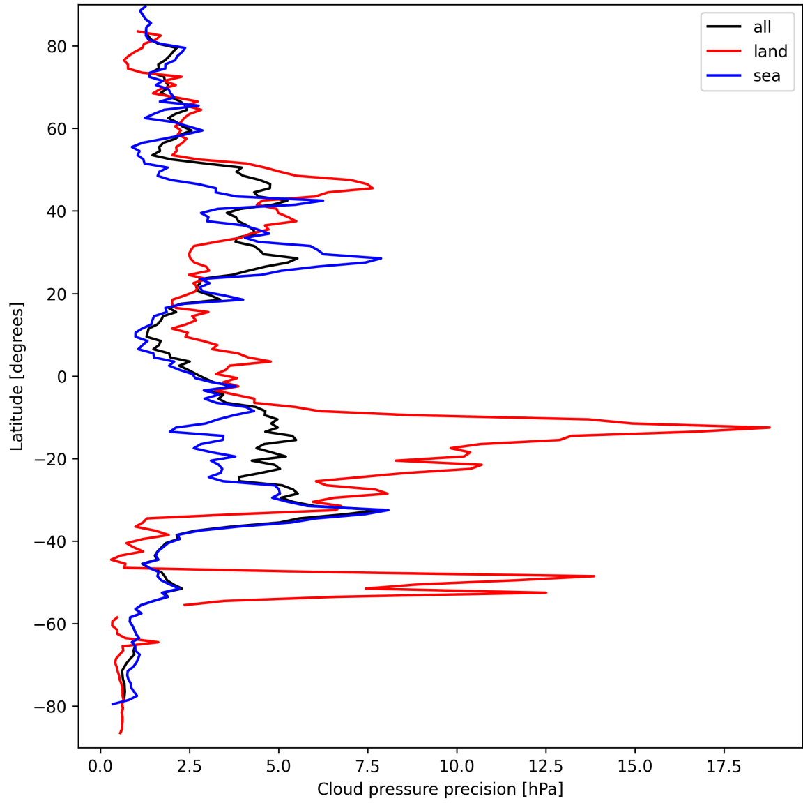
Figure 12: Zonal average of “Cloud pressure precision” for 2025-09-17 to 2025-09-18.
