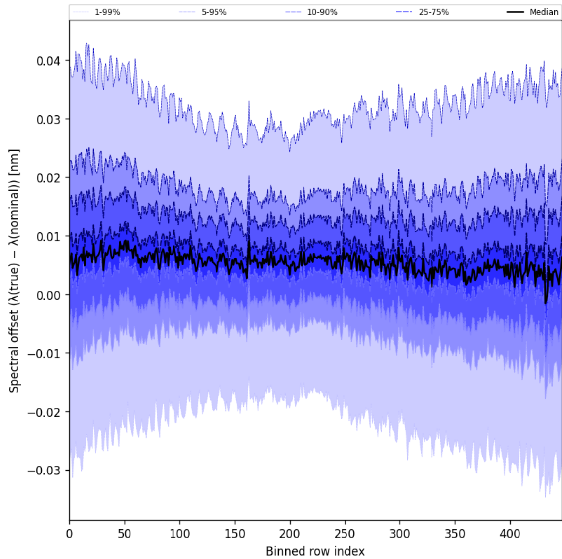
Figure 60: Along track statistics of “Spectral offset ( \lambda_{\text{true}} - \lambda_{\text{nominal}} )” for 2025-09-17 to 2025-09-18
