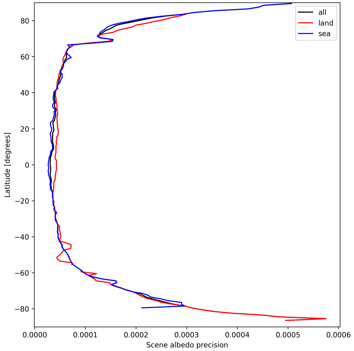
Figure 16: Zonal average of “Scene albedo precision” for 2025-09-17 to 2025-09-18.
