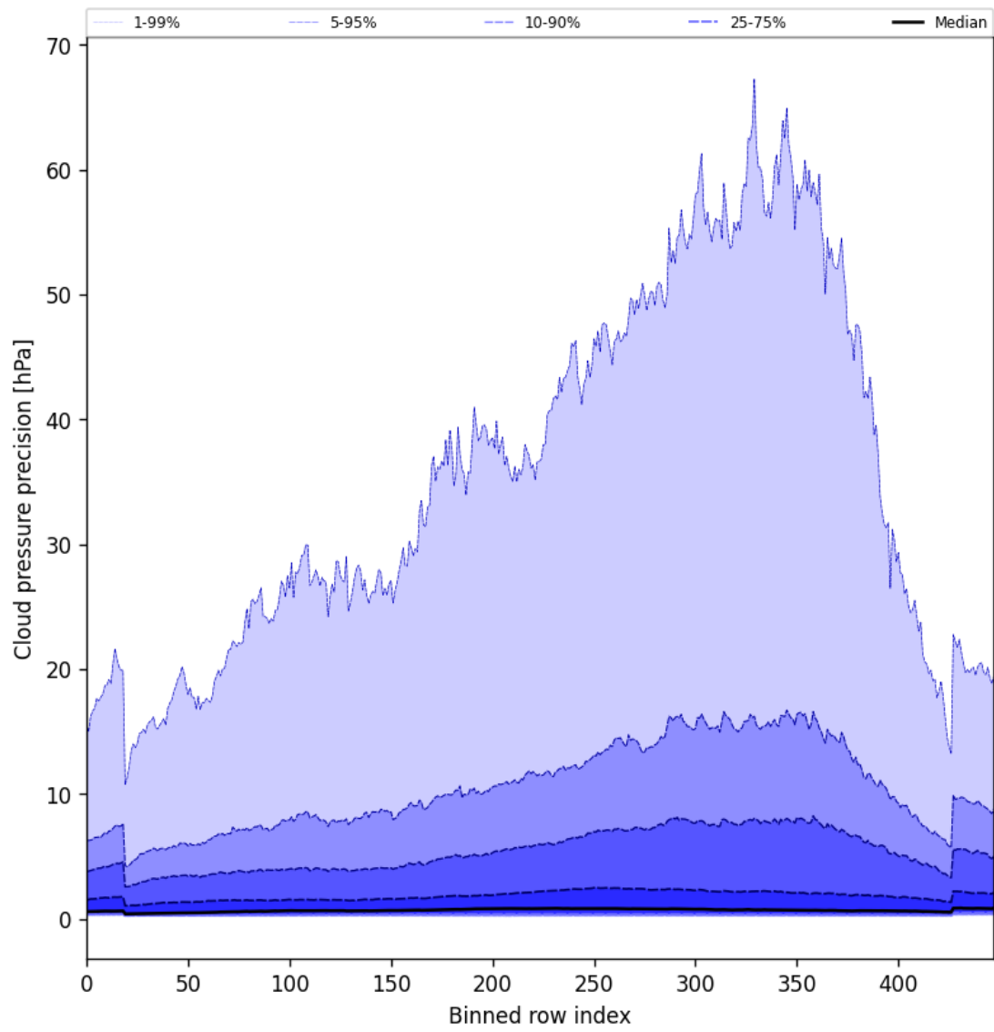
Figure 46: Along track statistics of “Cloud pressure precision” for 2025-09-17 to 2025-09-18
