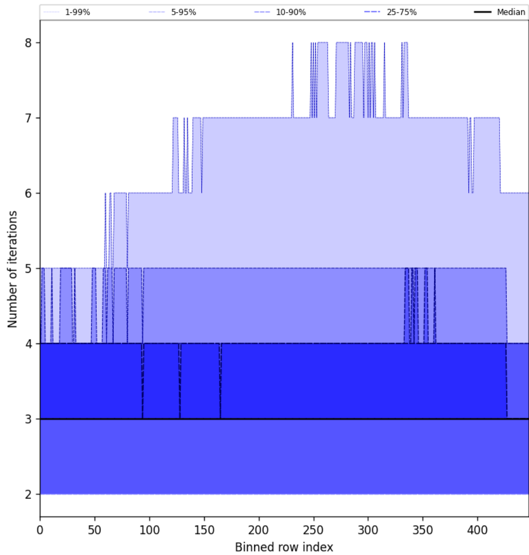
Figure 54: Along track statistics of “Number of iterations” for 2025-09-17 to 2025-09-18
