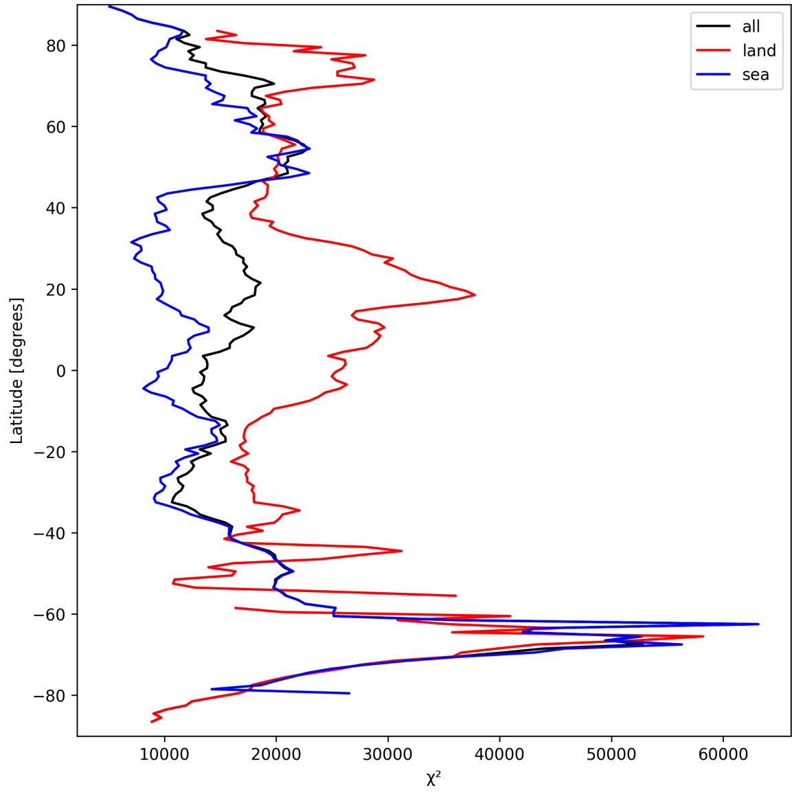
Figure 19: Zonal average of “ \chi^2 ” for 2025-09-17 to 2025-09-18.
