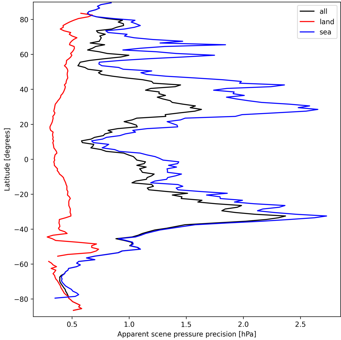
Figure 18: Zonal average of “Apparent scene pressure precision” for 2025-09-17 to 2025-09-18.
