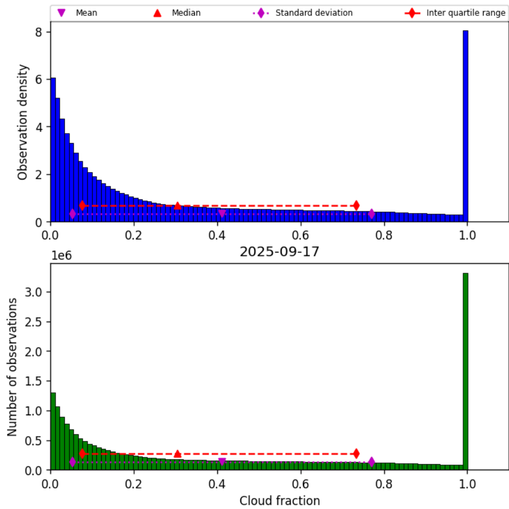
Figure 30: Histogram of “Cloud fraction” for 2025-09-17 to 2025-09-18
