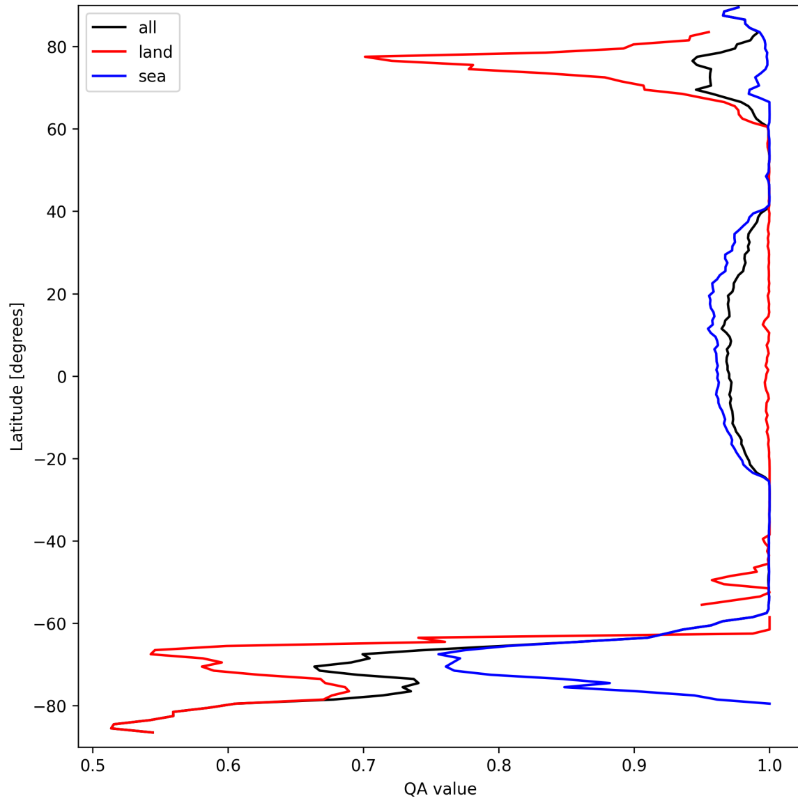
Figure 10: Zonal average of “QA value” for 2025-09-17 to 2025-09-18.
