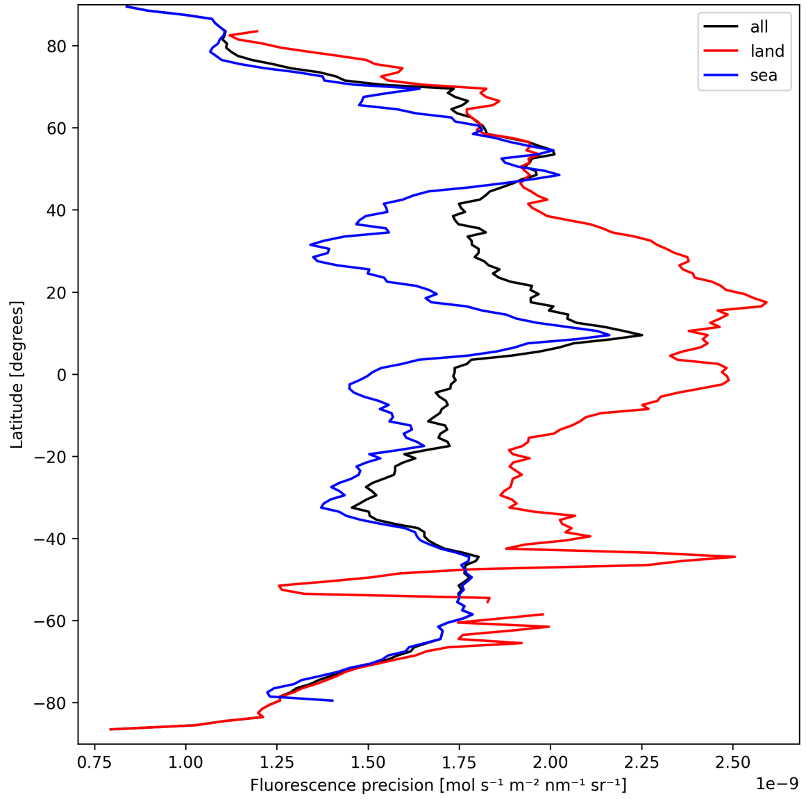
Figure 22: Zonal average of “Fluorescence precision” for 2025-09-17 to 2025-09-18.
