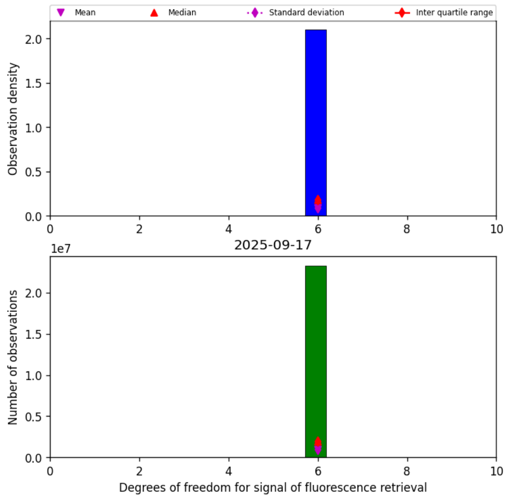
Figure 41: Histogram of “Degrees of freedom for signal of fluorescence retrieval” for 2025-09-17 to 2025-09-18
