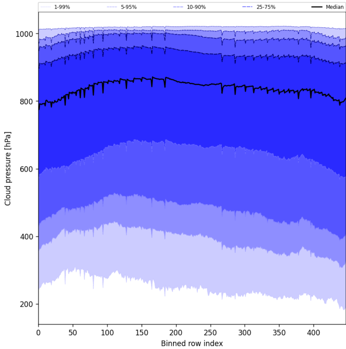
Figure 45: Along track statistics of “Cloud pressure” for 2025-09-17 to 2025-09-18
