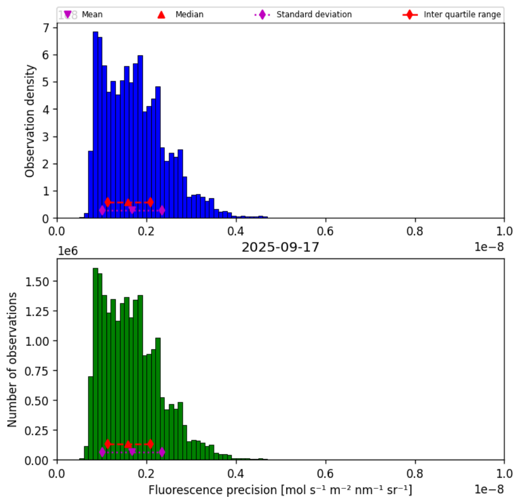
Figure 39: Histogram of “Fluorescence precision” for 2025-09-17 to 2025-09-18
