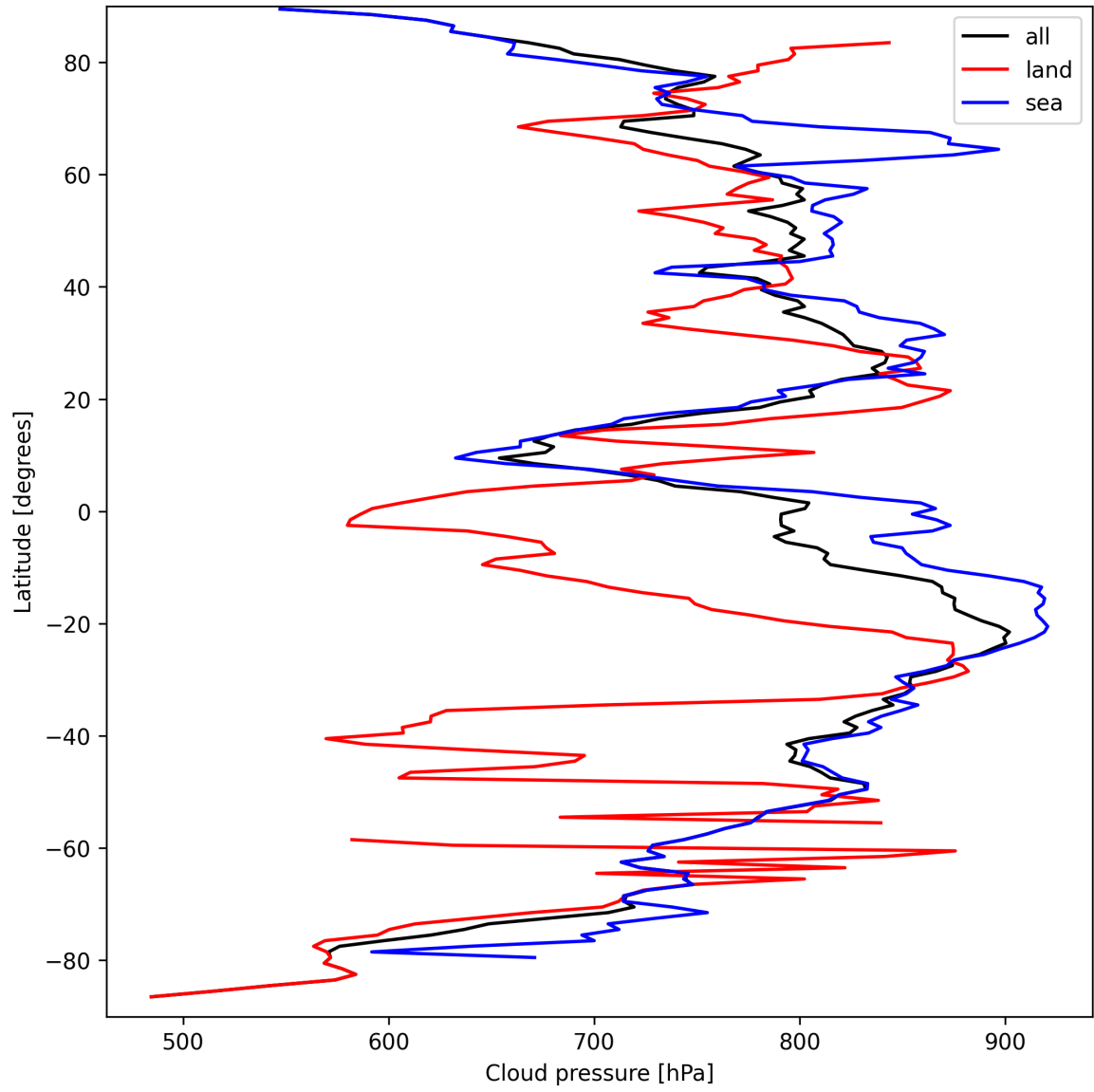
Figure 11: Zonal average of “Cloud pressure” for 2025-09-17 to 2025-09-18.
