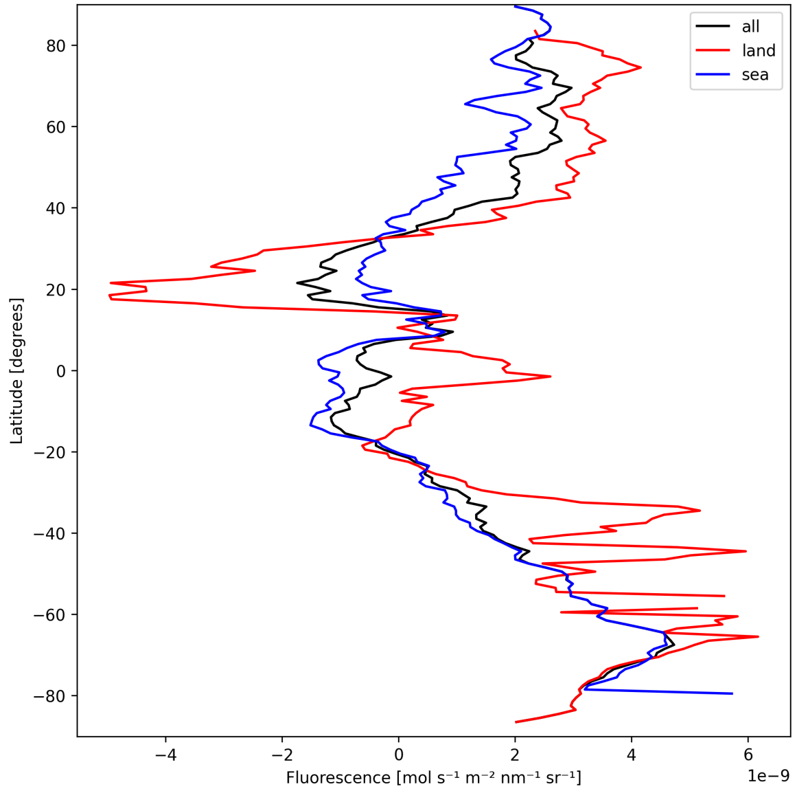
Figure 21: Zonal average of “Fluorescence” for 2025-09-17 to 2025-09-18.
