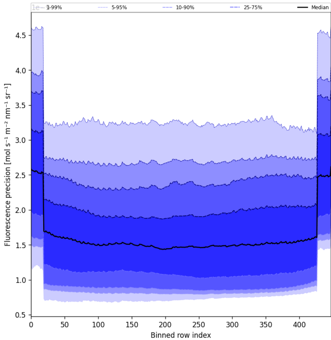
Figure 56: Along track statistics of “Fluorescence precision” for 2025-09-17 to 2025-09-18
