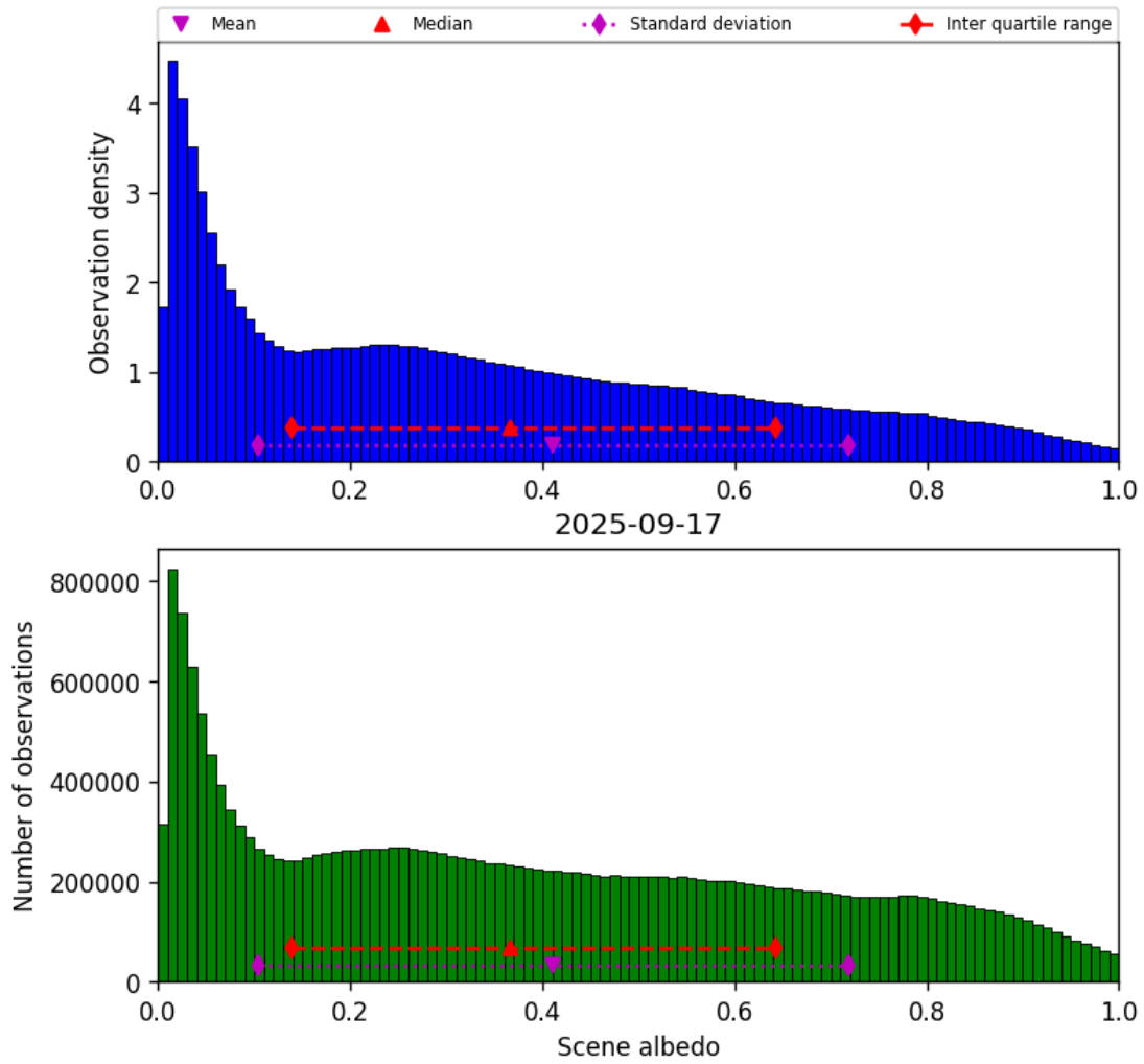
Figure 32: Histogram of “Scene albedo” for 2025-09-17 to 2025-09-18
