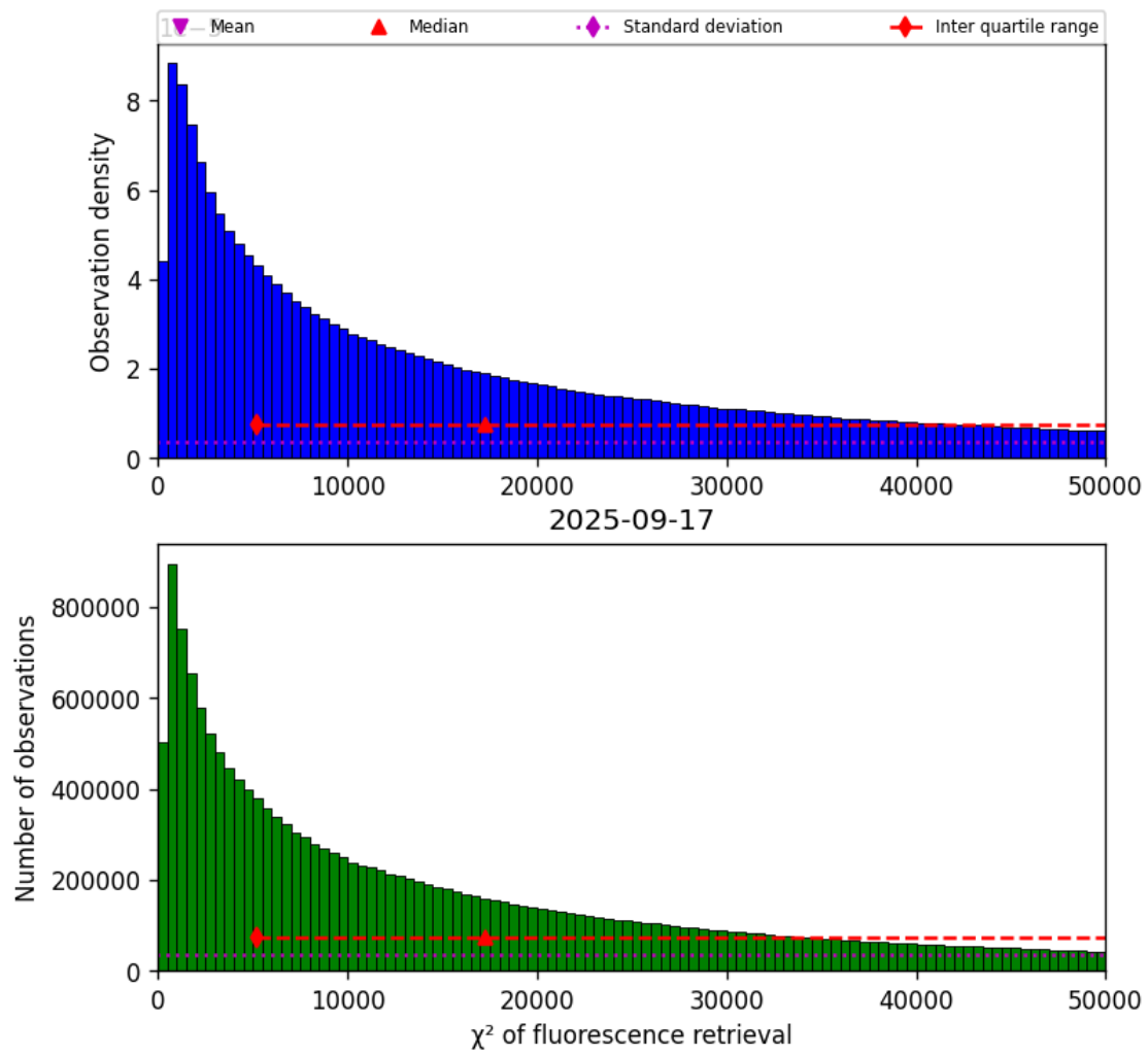
Figure 40: Histogram of “ \chi^2 of fluorescence retrieval” for 2025-09-17 to 2025-09-18
