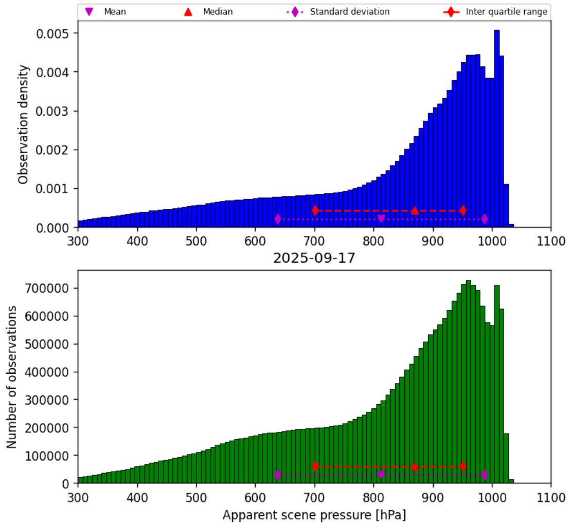
Figure 34: Histogram of “Apparent scene pressure” for 2025-09-17 to 2025-09-18
