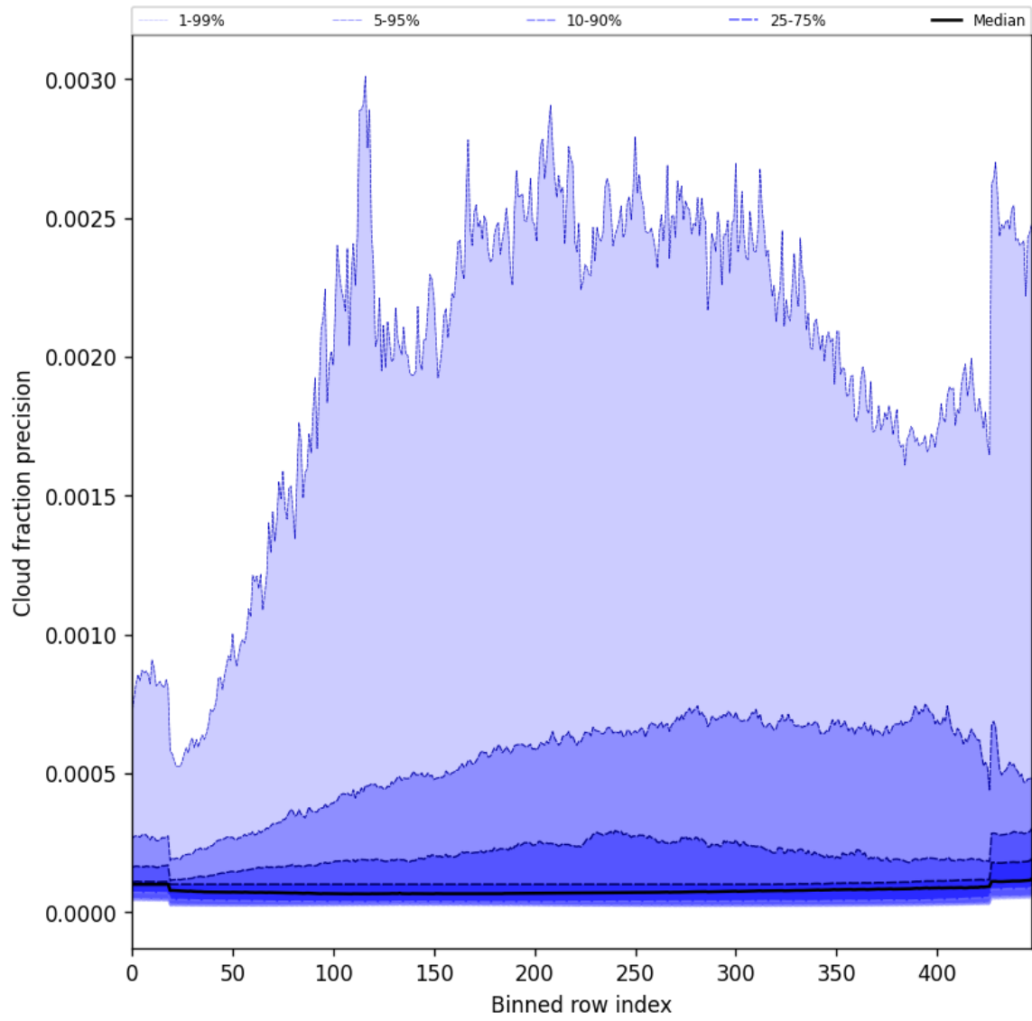
Figure 48: Along track statistics of “Cloud fraction precision” for 2025-09-17 to 2025-09-18
