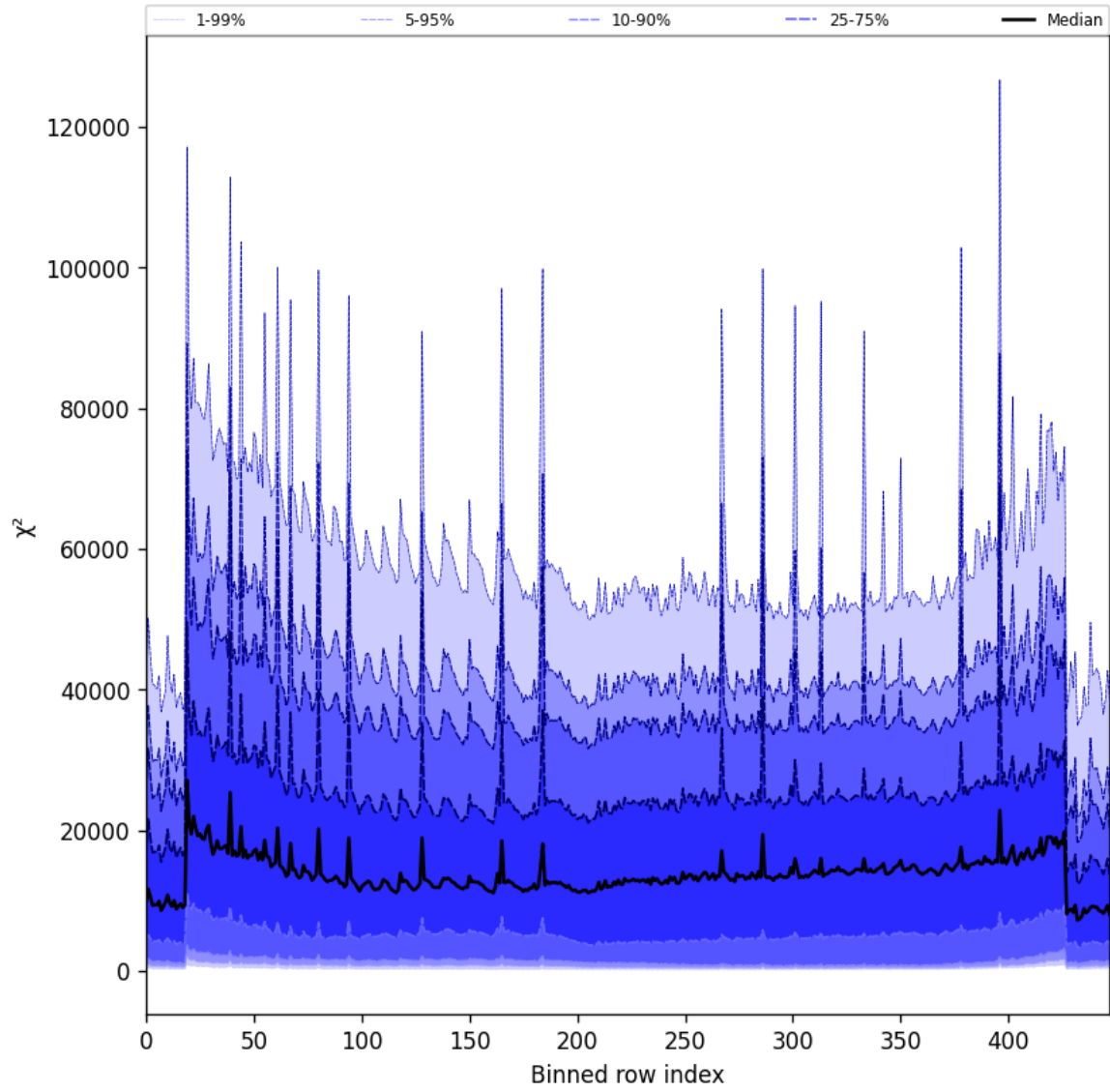
Figure 53: Along track statistics of “ \chi^2 ” for 2025-09-17 to 2025-09-18
