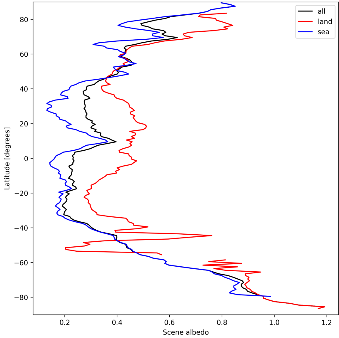
Figure 15: Zonal average of “Scene albedo” for 2025-09-17 to 2025-09-18.
