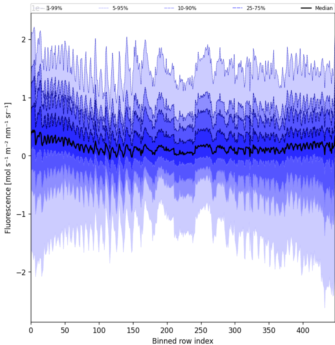
Figure 55: Along track statistics of “Fluorescence” for 2025-09-17 to 2025-09-18
