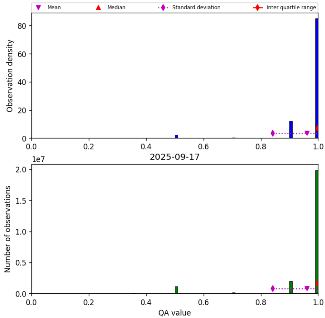
Figure 27: Histogram of “QA value” for 2025-09-17 to 2025-09-18
