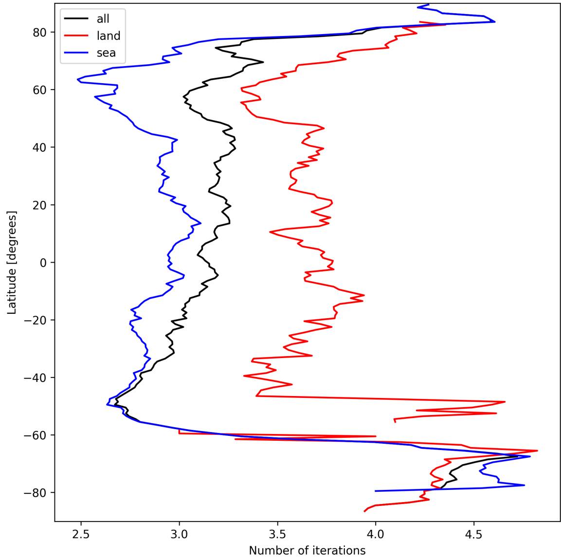
Figure 20: Zonal average of “Number of iterations” for 2025-09-17 to 2025-09-18.
