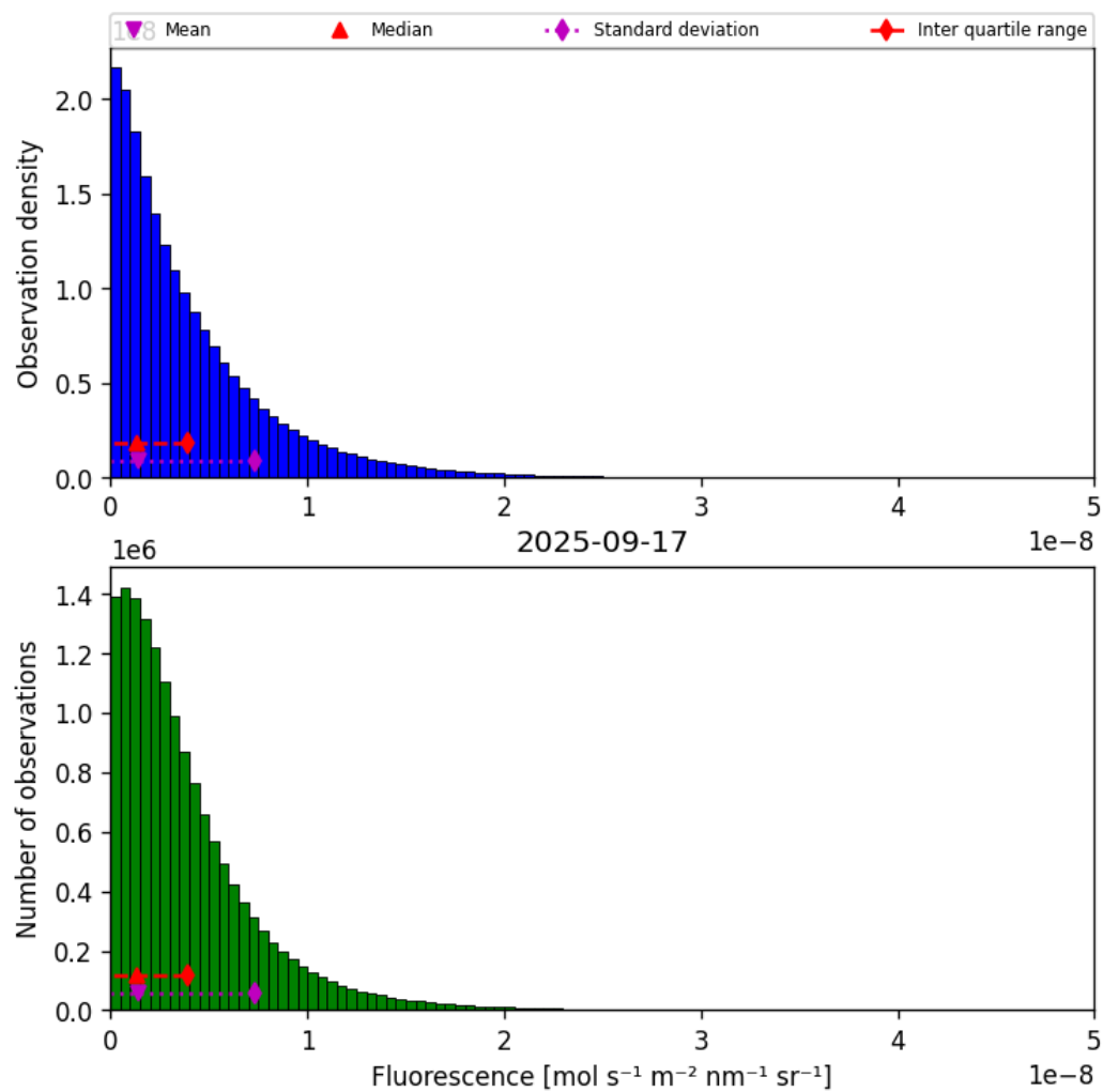
Figure 38: Histogram of “Fluorescence” for 2025-09-17 to 2025-09-18
