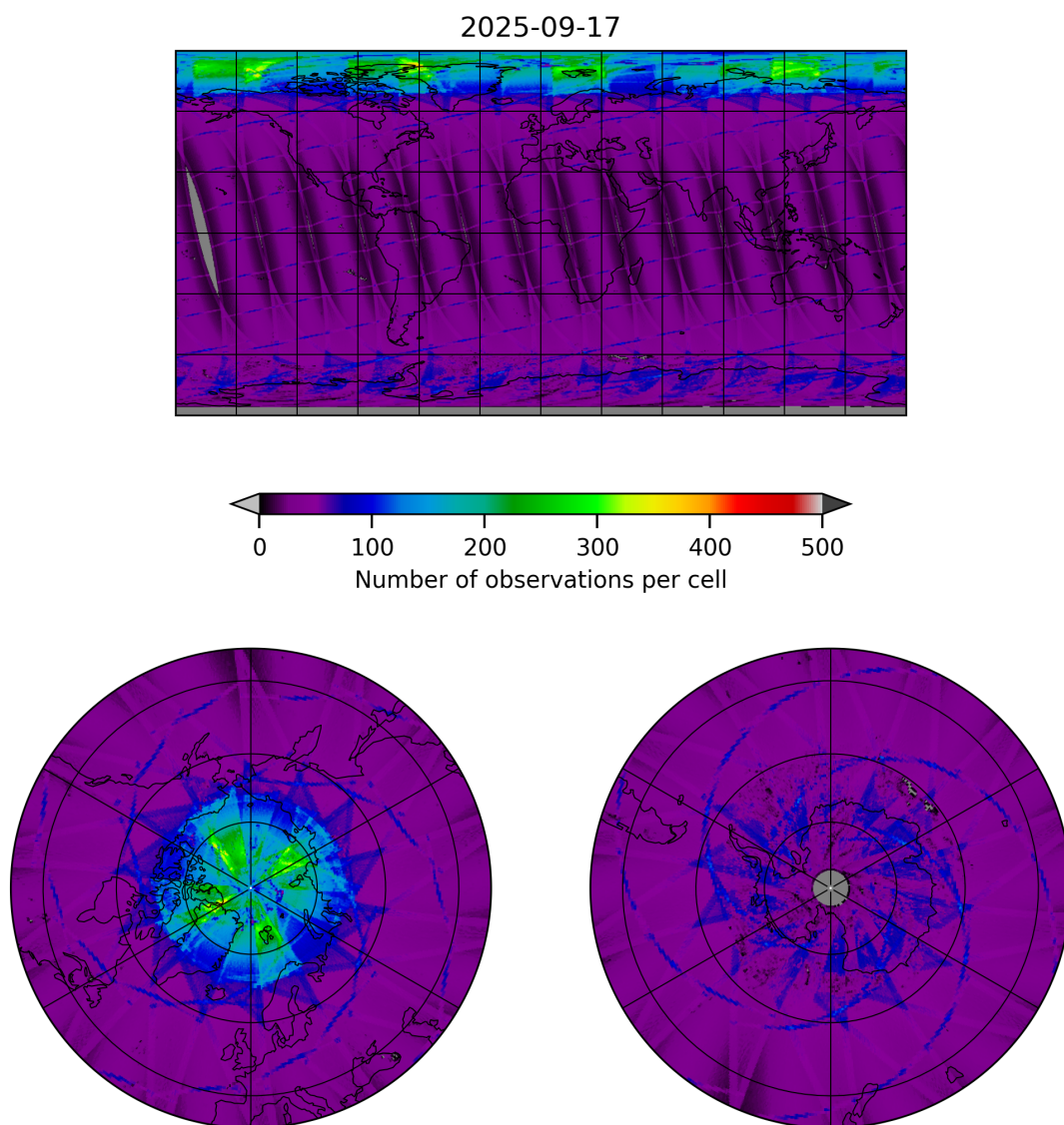
Figure 9: Map of the number of observations for 2025-09-17 to 2025-09-18
