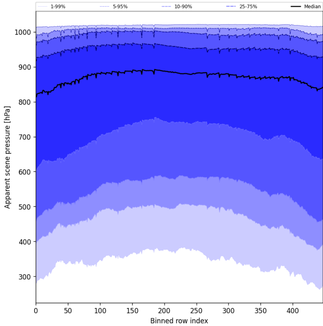
Figure 51: Along track statistics of “Apparent scene pressure” for 2025-09-17 to 2025-09-18
