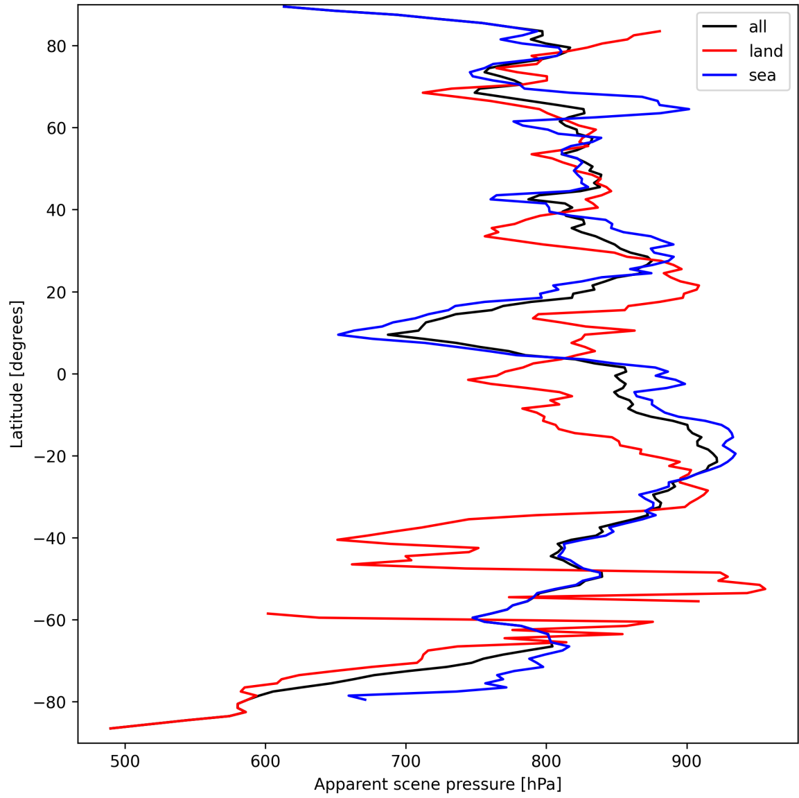
Figure 17: Zonal average of “Apparent scene pressure” for 2025-09-17 to 2025-09-18.
