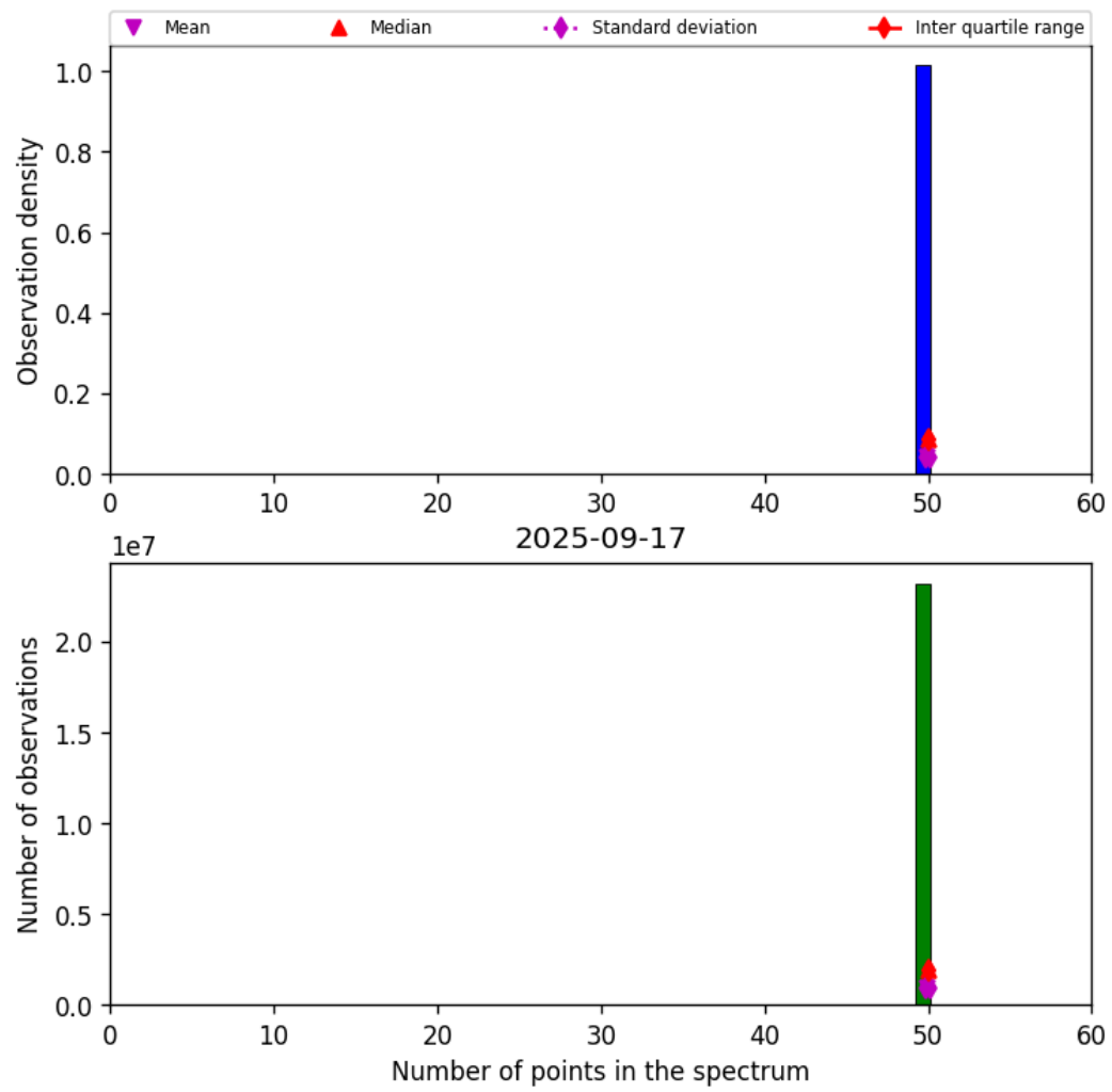
Figure 42: Histogram of “Number of points in the spectrum” for 2025-09-17 to 2025-09-18
