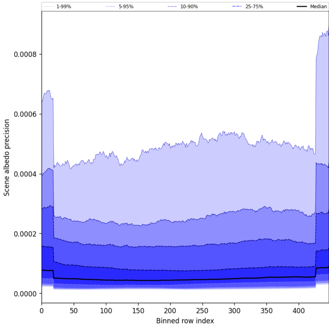
Figure 50: Along track statistics of “Scene albedo precision” for 2025-09-17 to 2025-09-18
