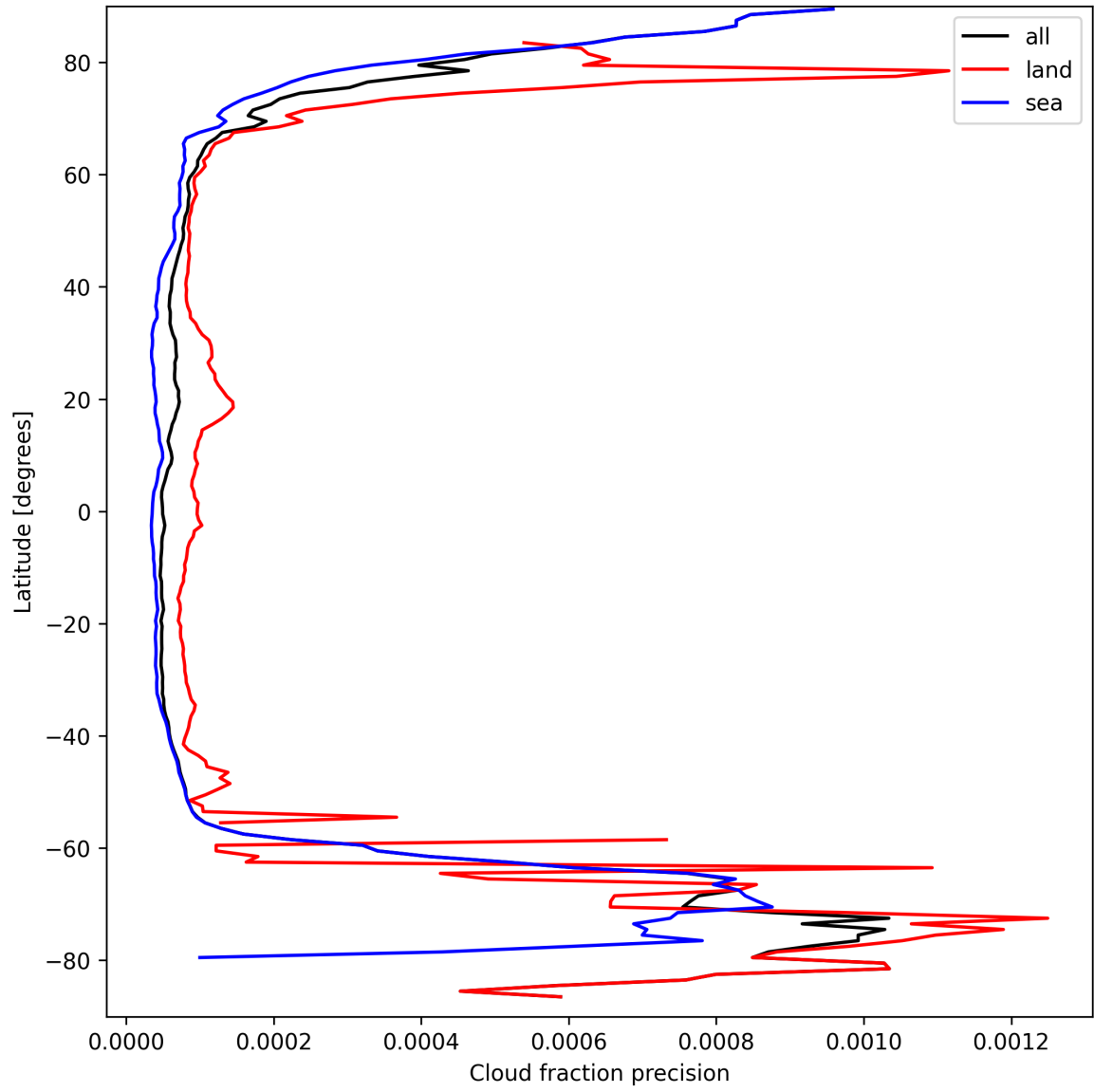
Figure 14: Zonal average of “Cloud fraction precision” for 2025-09-17 to 2025-09-18.
