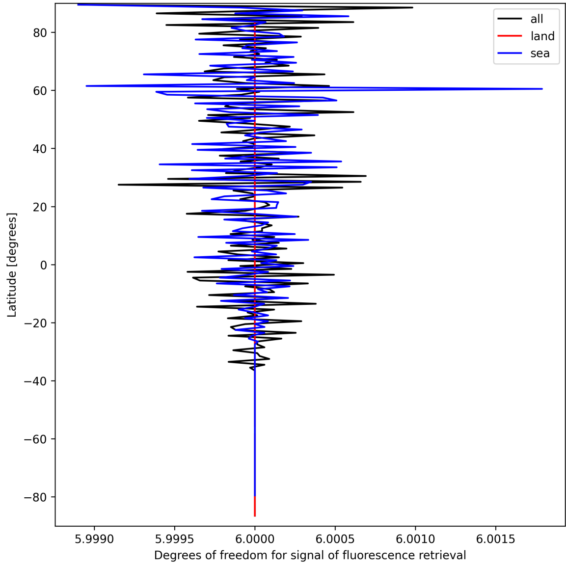
Figure 24: Zonal average of “Degrees of freedom for signal of fluorescence retrieval” for 2025-09-17 to 2025-09-18.
