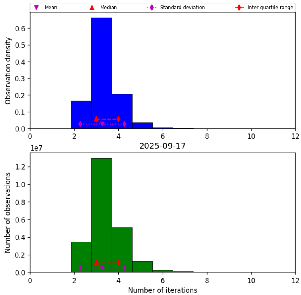
Figure 37: Histogram of “Number of iterations” for 2025-09-17 to 2025-09-18
