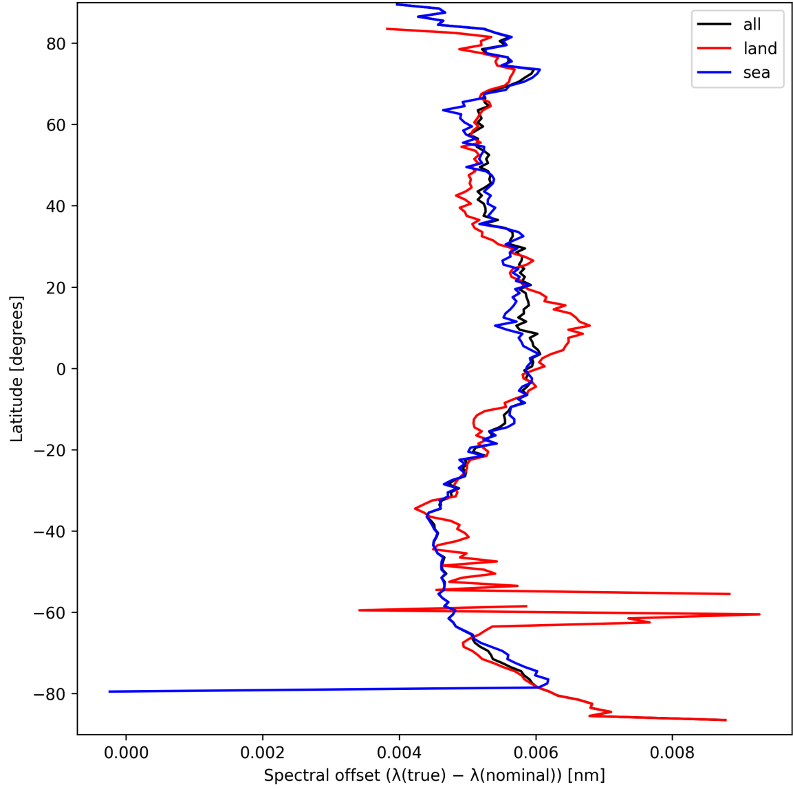
Figure 26: Zonal average of “Spectral offset ( \lambda_{\text{true}} - \lambda_{\text{nominal}} )” for 2025-09-17 to 2025-09-18.
