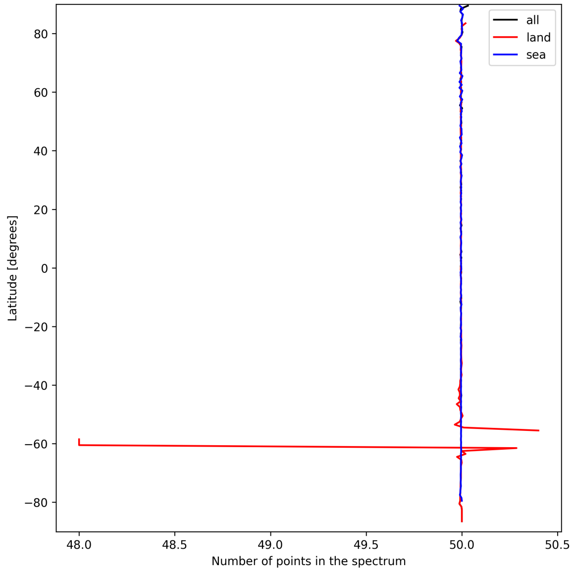
Figure 25: Zonal average of “Number of points in the spectrum” for 2025-09-17 to 2025-09-18.
