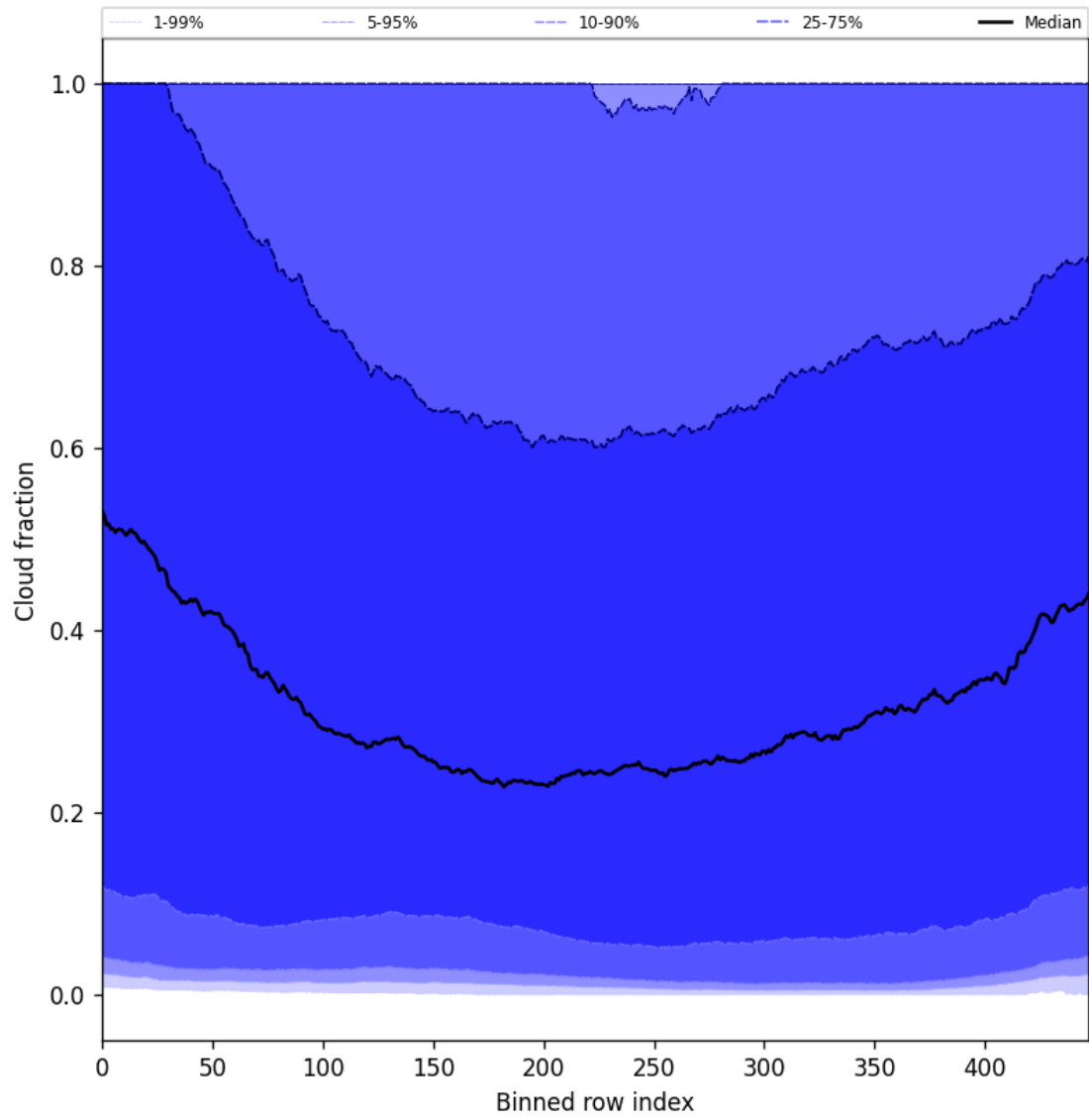
Figure 47: Along track statistics of “Cloud fraction” for 2025-09-17 to 2025-09-18
