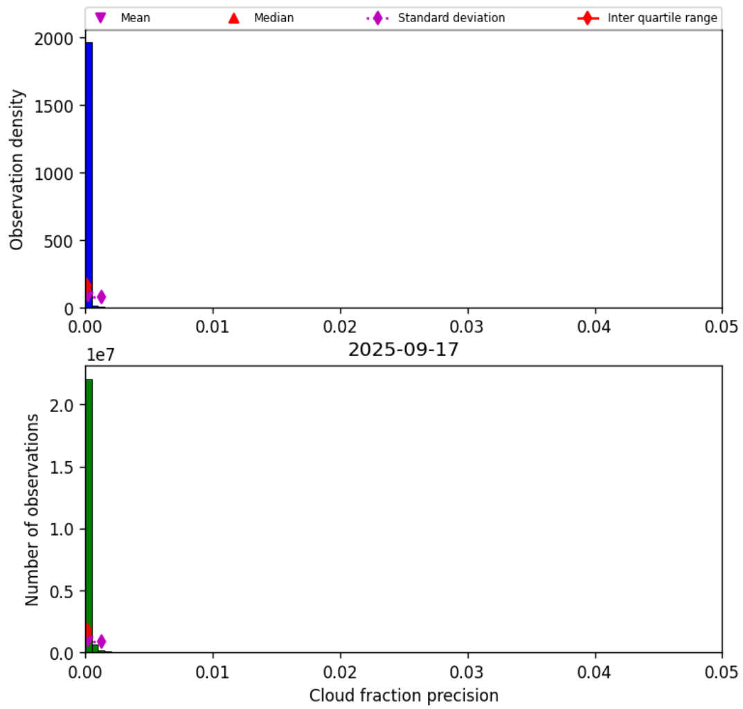
Figure 31: Histogram of “Cloud fraction precision” for 2025-09-17 to 2025-09-18
