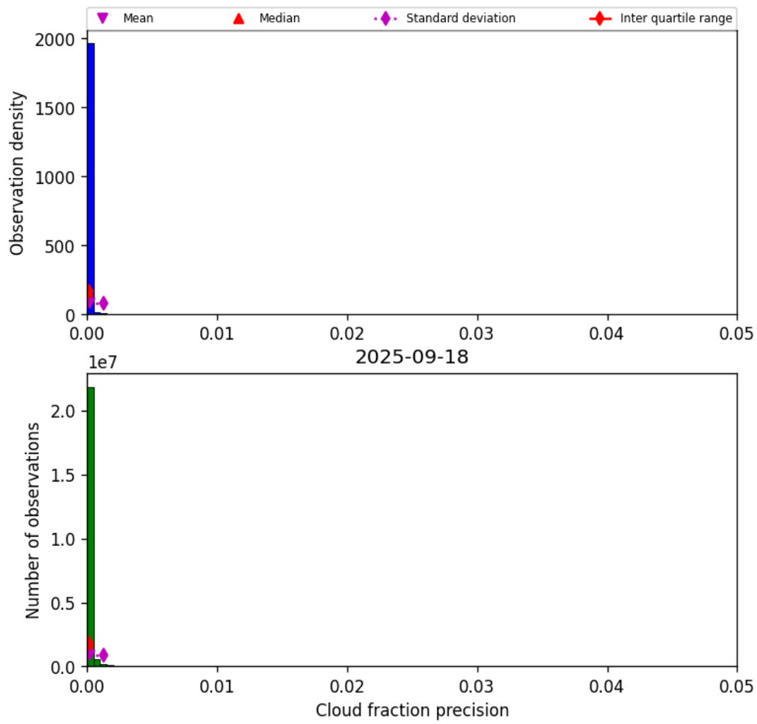
Figure 31: Histogram of “Cloud fraction precision” for 2025-09-18 to 2025-09-18
