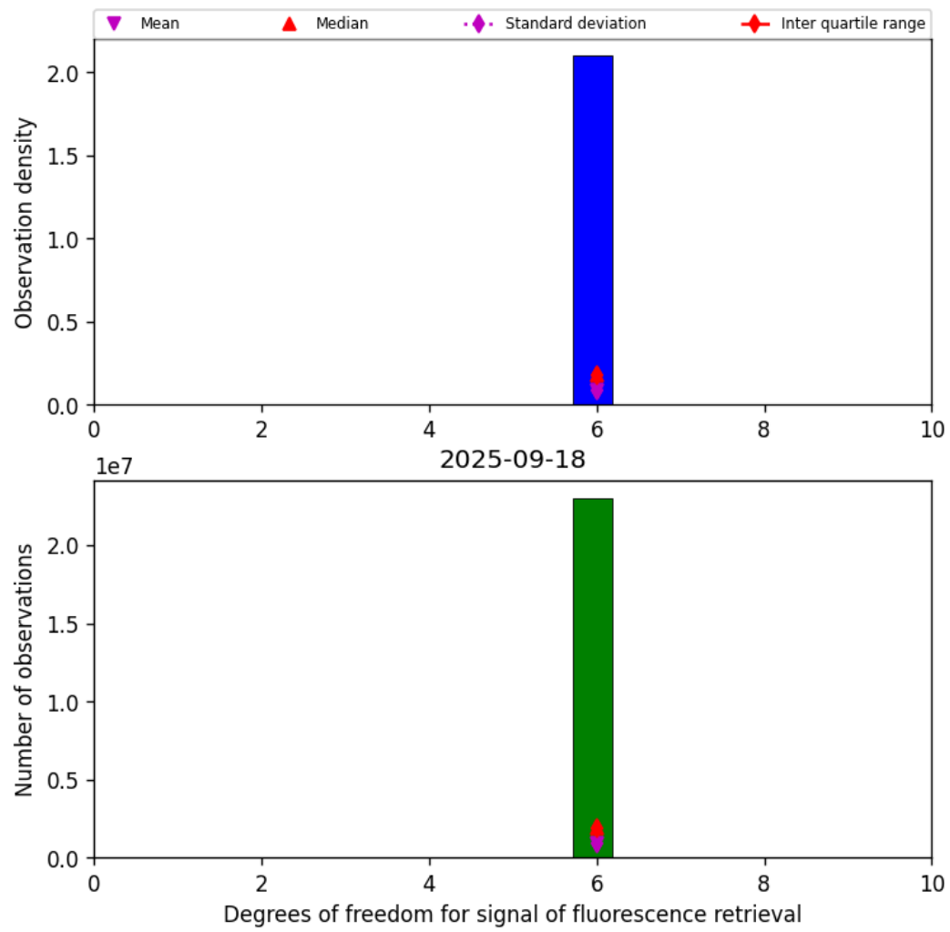
Figure 41: Histogram of “Degrees of freedom for signal of fluorescence retrieval” for 2025-09-18 to 2025-09-18
