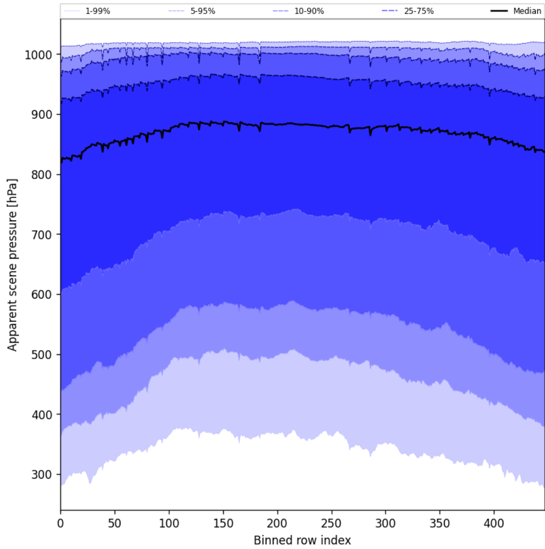
Figure 51: Along track statistics of “Apparent scene pressure” for 2025-09-18 to 2025-09-18
