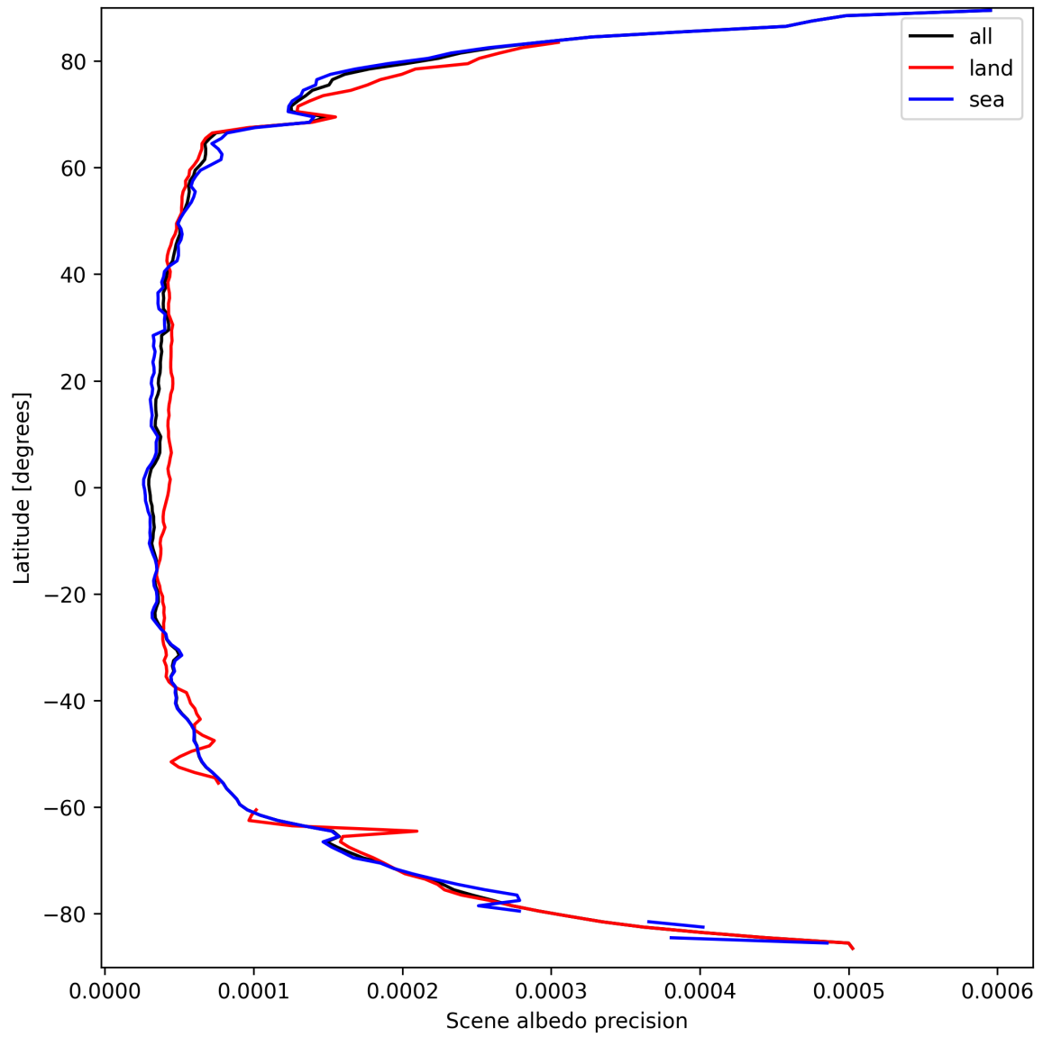
Figure 16: Zonal average of “Scene albedo precision” for 2025-09-18 to 2025-09-18.
