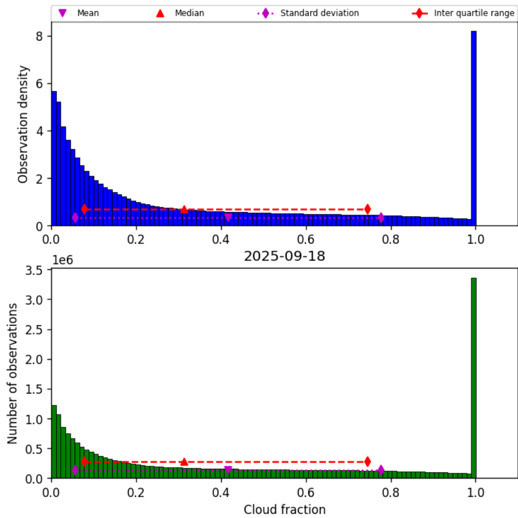
Figure 30: Histogram of “Cloud fraction” for 2025-09-18 to 2025-09-18
