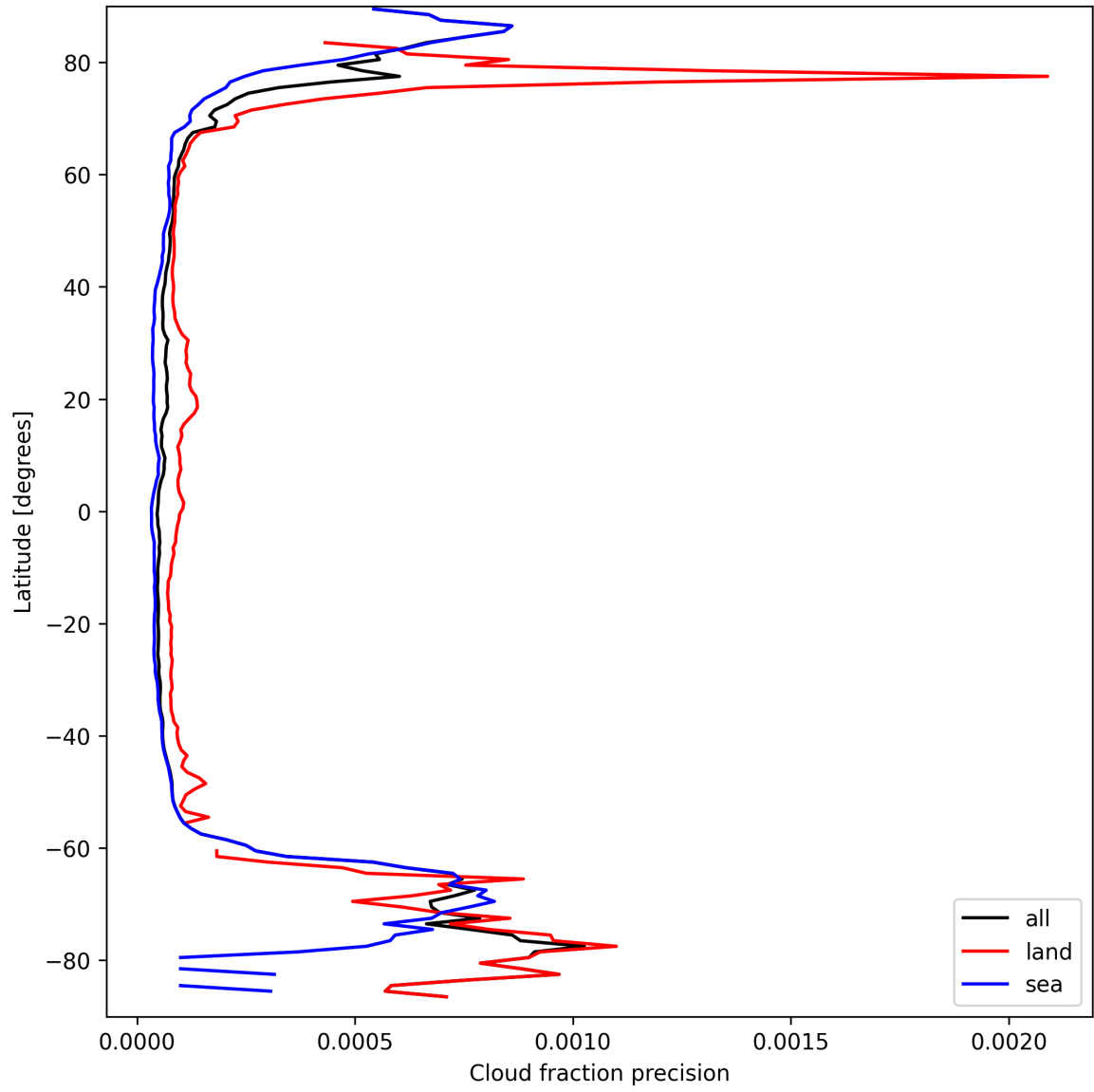
Figure 14: Zonal average of “Cloud fraction precision” for 2025-09-18 to 2025-09-18.
