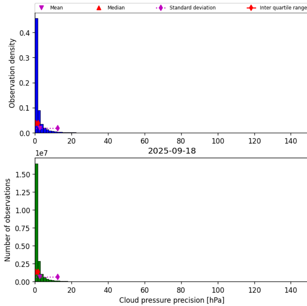
Figure 29: Histogram of “Cloud pressure precision” for 2025-09-18 to 2025-09-18
