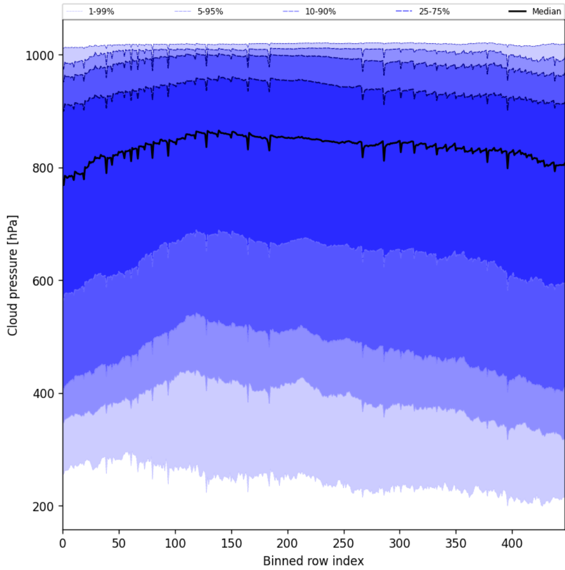
Figure 45: Along track statistics of “Cloud pressure” for 2025-09-18 to 2025-09-18
