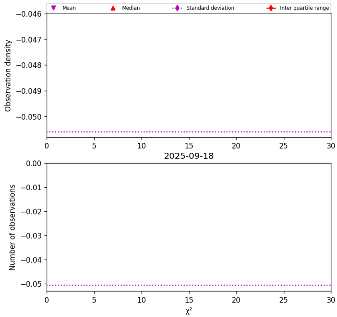
Figure 36: Histogram of " \chi^2 " for 2025-09-18 to 2025-09-18
