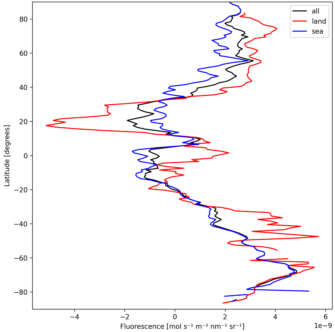
Figure 21: Zonal average of “Fluorescence” for 2025-09-18 to 2025-09-18.
