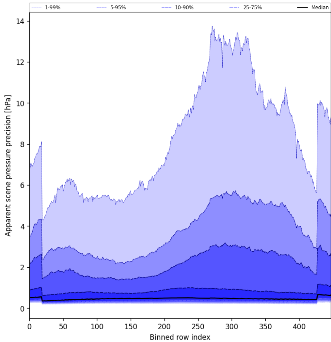
Figure 52: Along track statistics of “Apparent scene pressure precision” for 2025-09-18 to 2025-09-18
