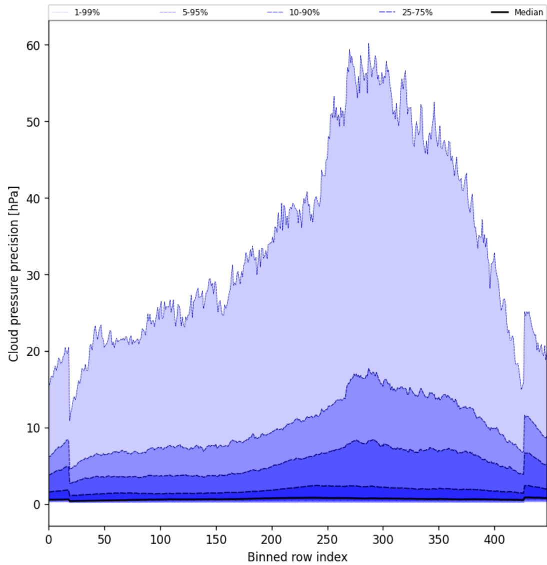
Figure 46: Along track statistics of “Cloud pressure precision” for 2025-09-18 to 2025-09-18
