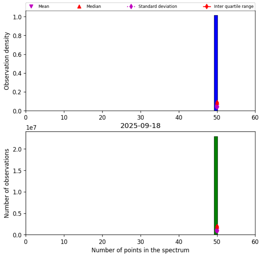
Figure 42: Histogram of “Number of points in the spectrum” for 2025-09-18 to 2025-09-18
