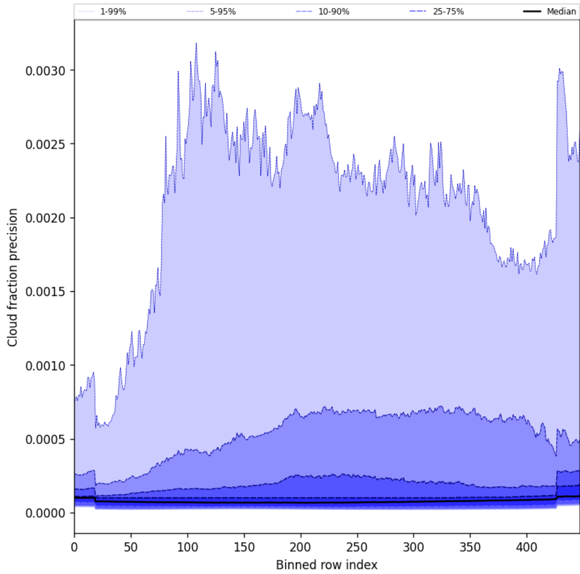
Figure 48: Along track statistics of “Cloud fraction precision” for 2025-09-18 to 2025-09-18
