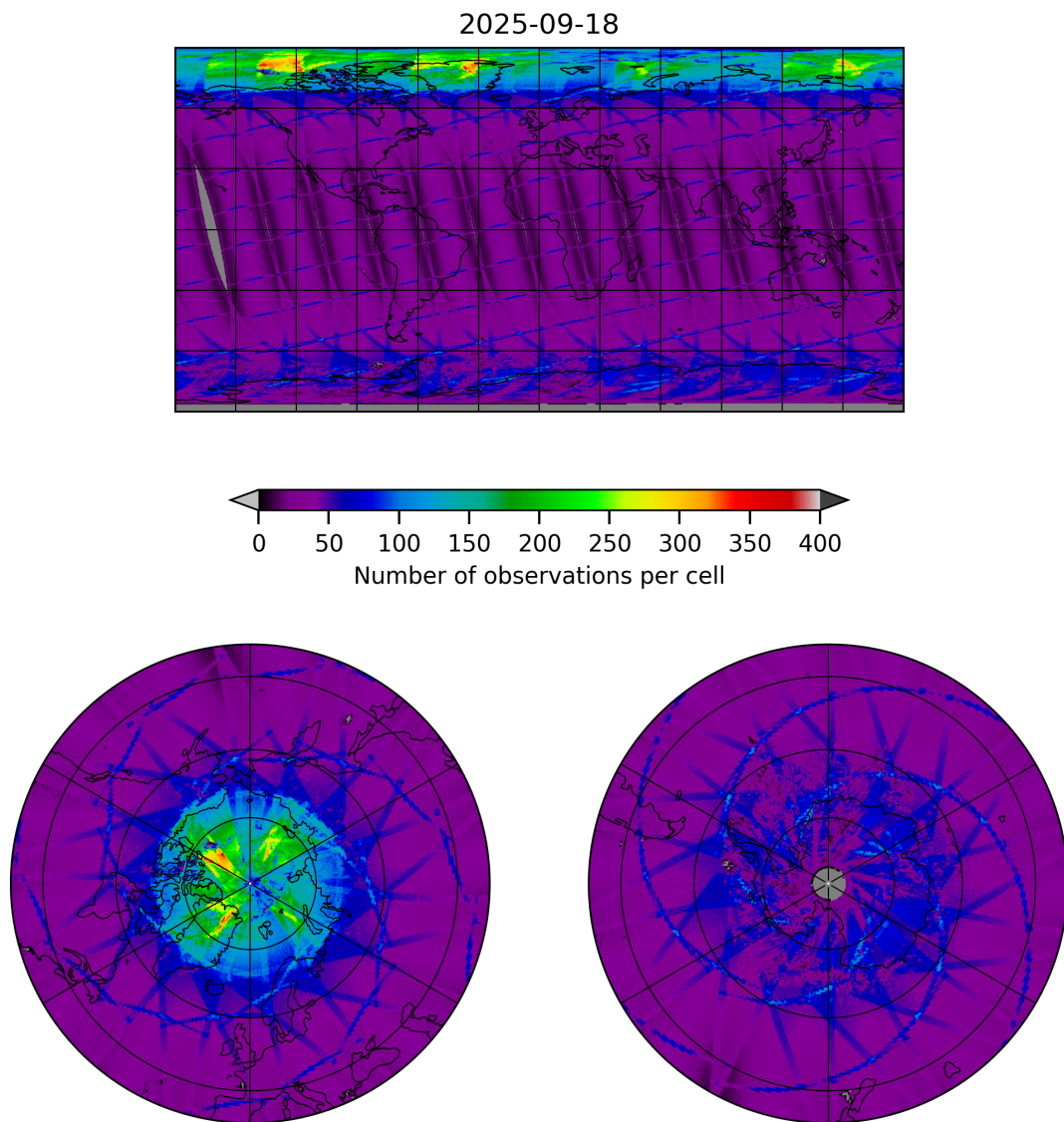
Figure 9: Map of the number of observations for 2025-09-18 to 2025-09-18
