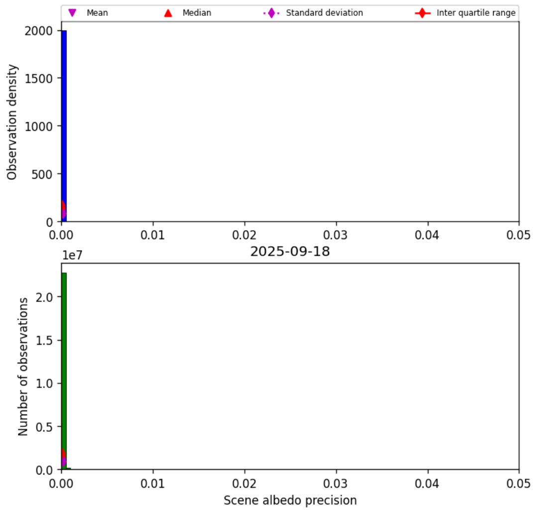
Figure 33: Histogram of “Scene albedo precision” for 2025-09-18 to 2025-09-18
