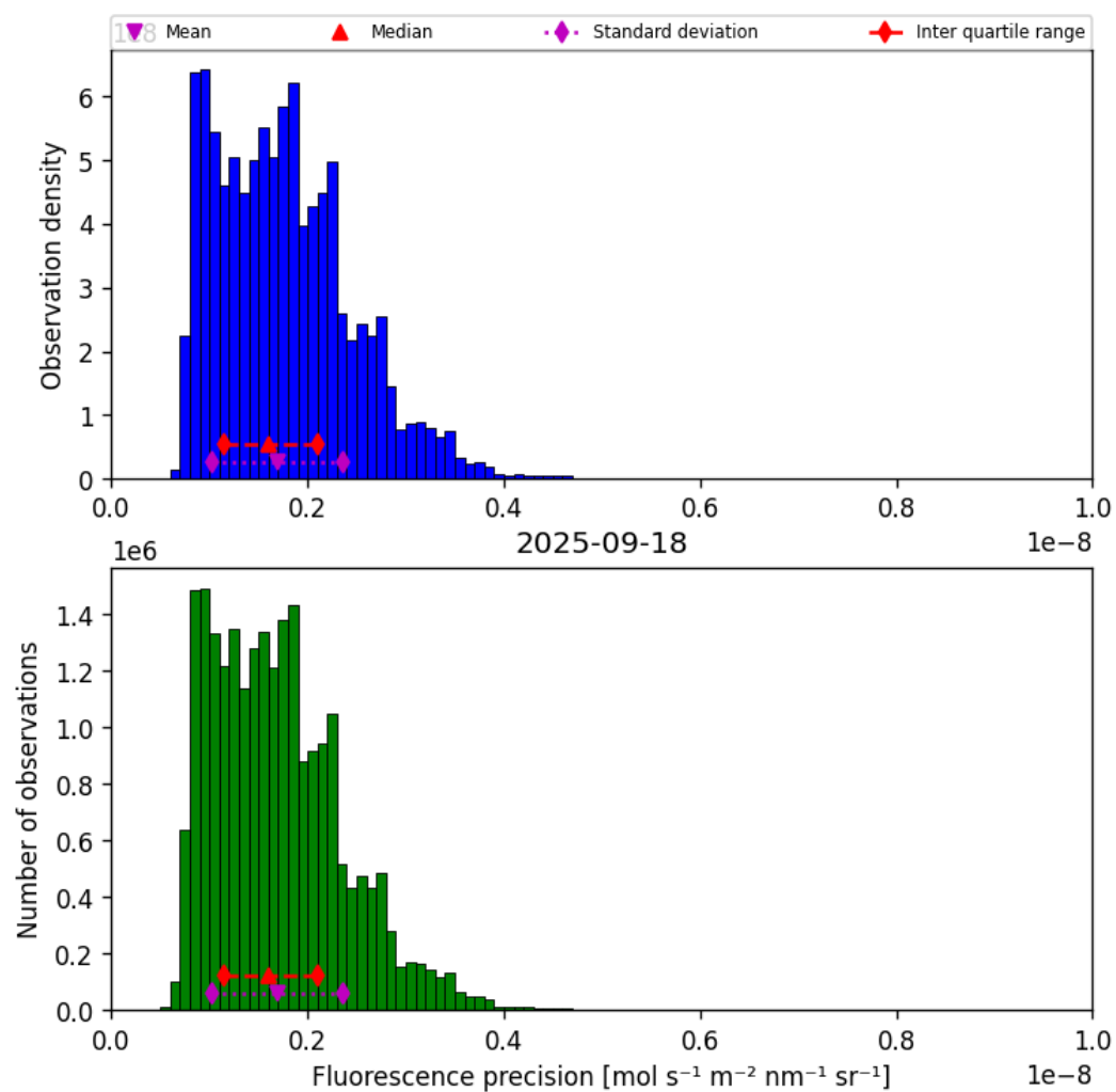
Figure 39: Histogram of “Fluorescence precision” for 2025-09-18 to 2025-09-18
