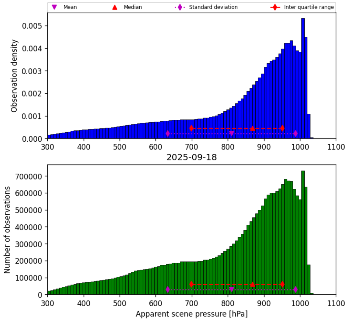
Figure 34: Histogram of “Apparent scene pressure” for 2025-09-18 to 2025-09-18
