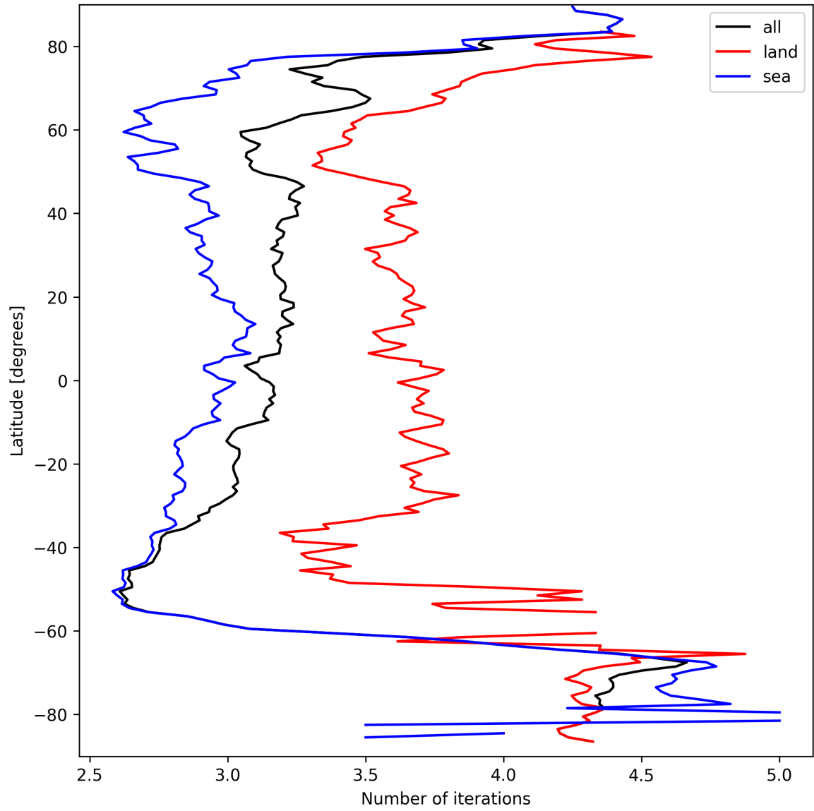
Figure 20: Zonal average of “Number of iterations” for 2025-09-18 to 2025-09-18.
