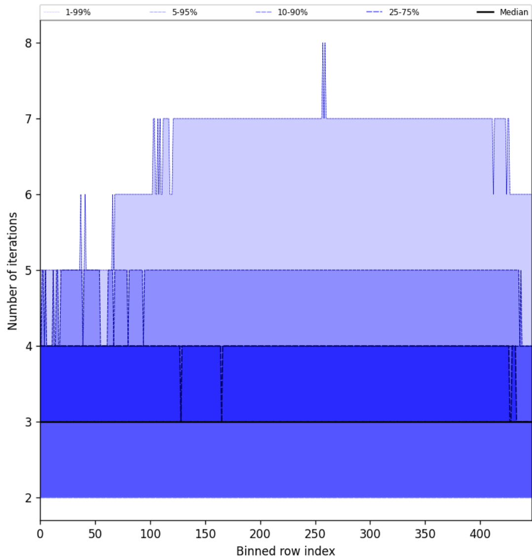
Figure 54: Along track statistics of “Number of iterations” for 2025-09-18 to 2025-09-18
