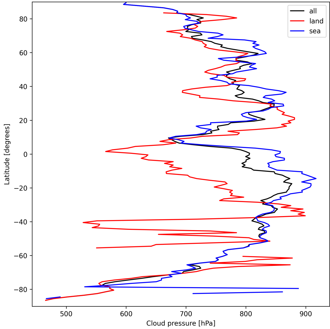
Figure 11: Zonal average of “Cloud pressure” for 2025-09-18 to 2025-09-18.
