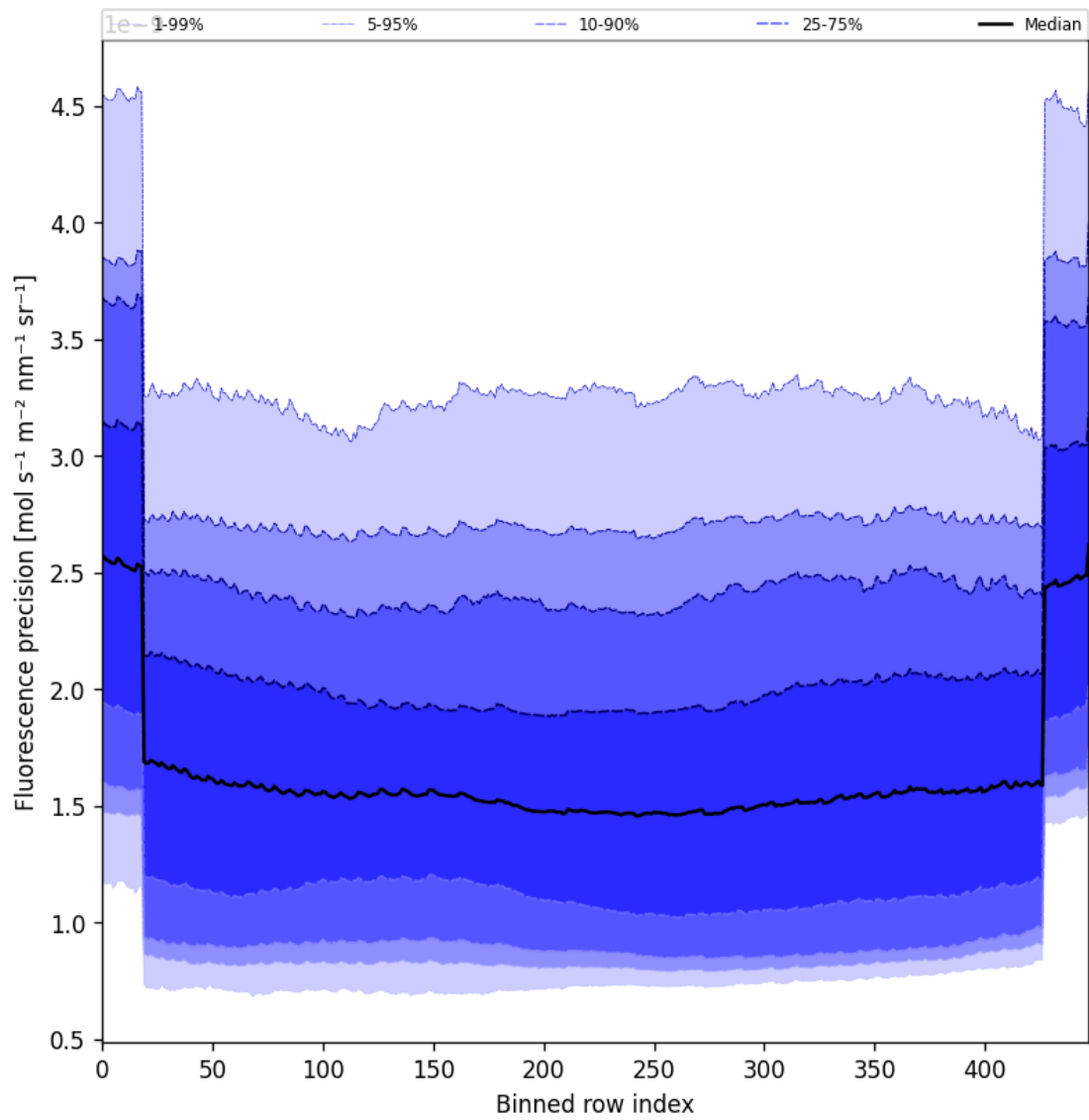
Figure 56: Along track statistics of “Fluorescence precision” for 2025-09-18 to 2025-09-18
