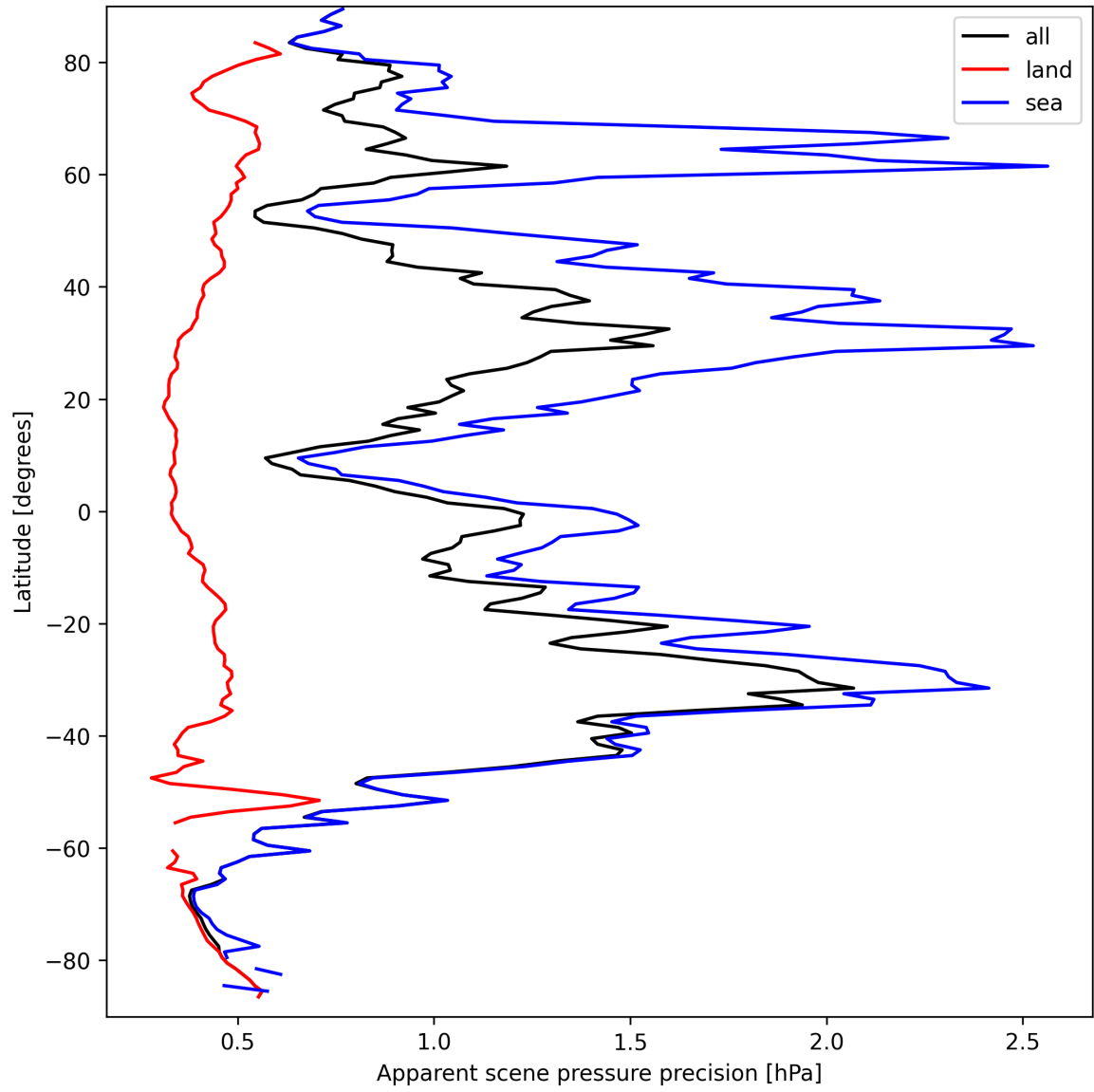
Figure 18: Zonal average of “Apparent scene pressure precision” for 2025-09-18 to 2025-09-18.
