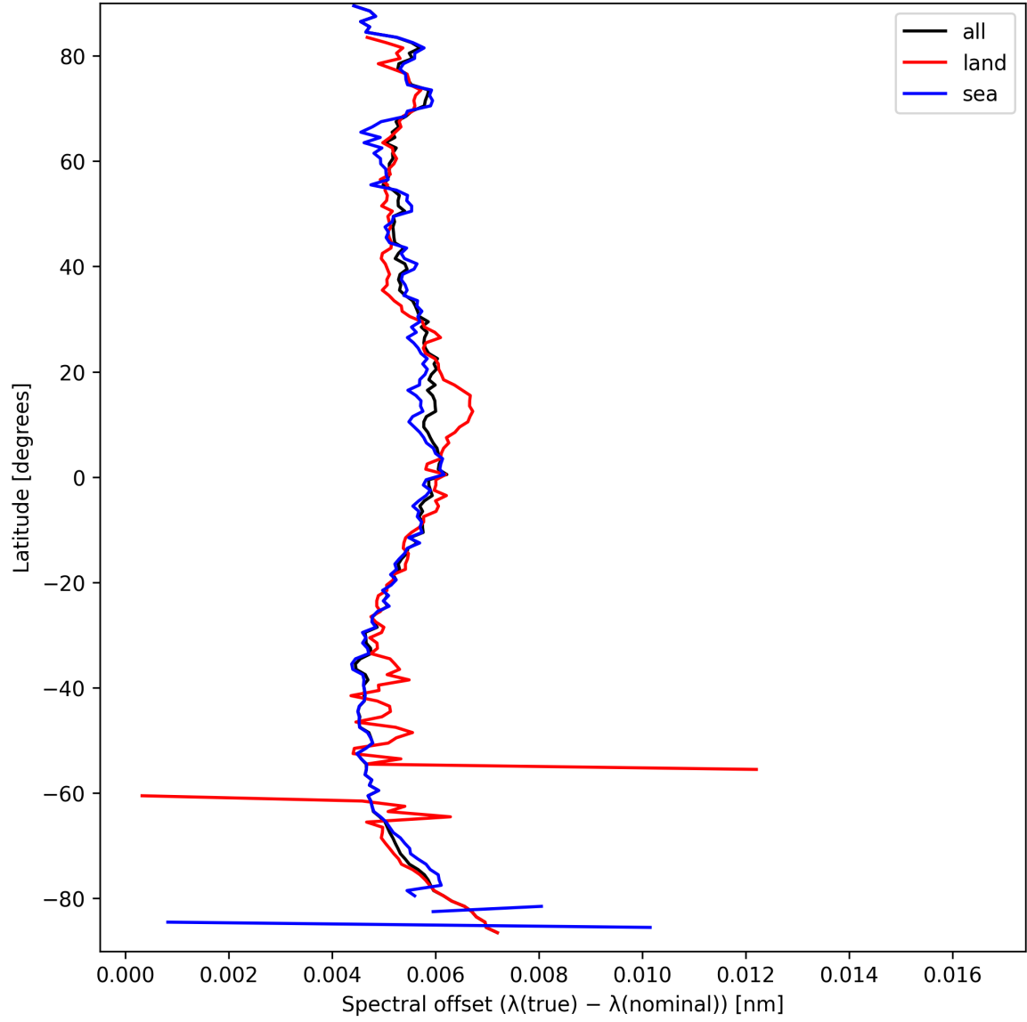
Figure 26: Zonal average of “Spectral offset ( \lambda_{\text{true}} - \lambda_{\text{nominal}} )” for 2025-09-18 to 2025-09-18.
