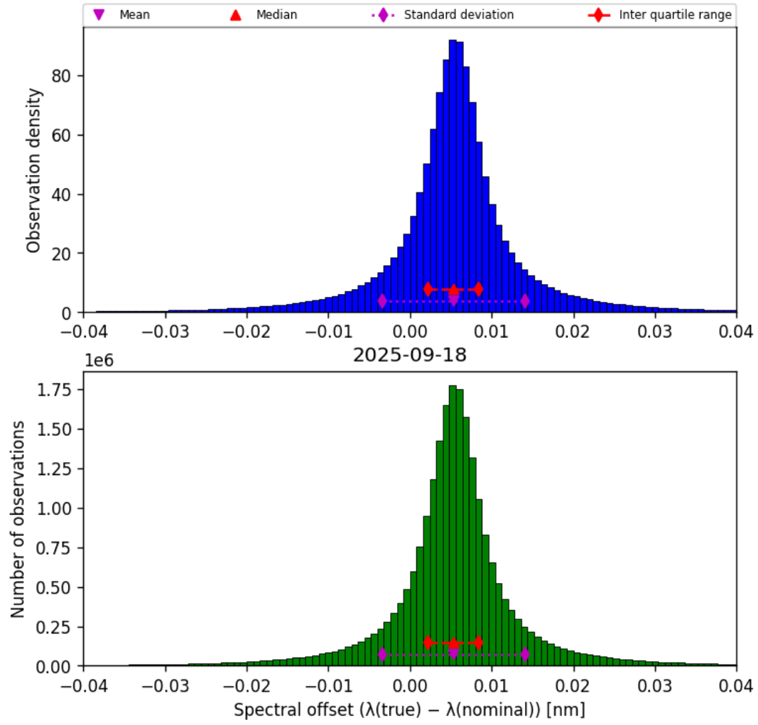
Figure 43: Histogram of “Spectral offset ( \lambda_{\text{true}} - \lambda_{\text{nominal}} )” for 2025-09-18 to 2025-09-18
