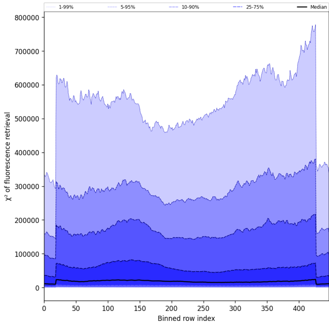
Figure 57: Along track statistics of “ \chi^2 of fluorescence retrieval” for 2025-09-18 to 2025-09-18
