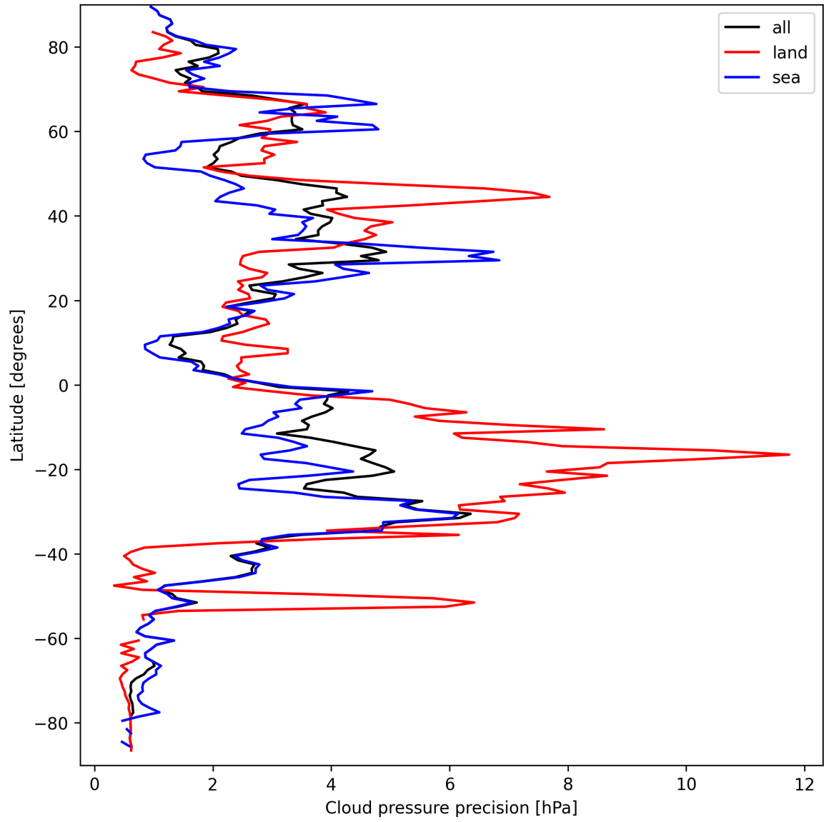
Figure 12: Zonal average of “Cloud pressure precision” for 2025-09-18 to 2025-09-18.
