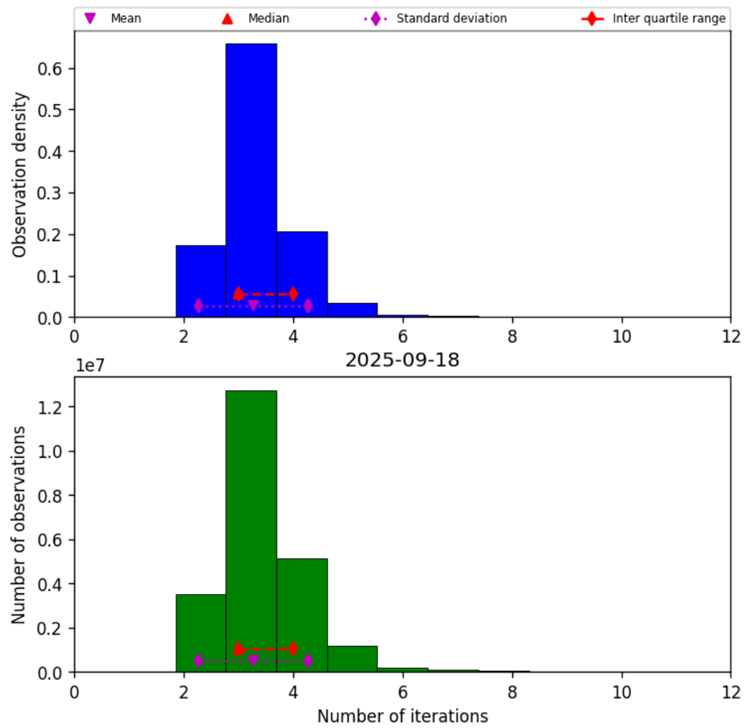
Figure 37: Histogram of “Number of iterations” for 2025-09-18 to 2025-09-18
