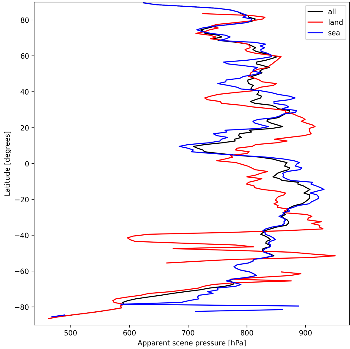
Figure 17: Zonal average of “Apparent scene pressure” for 2025-09-18 to 2025-09-18.
