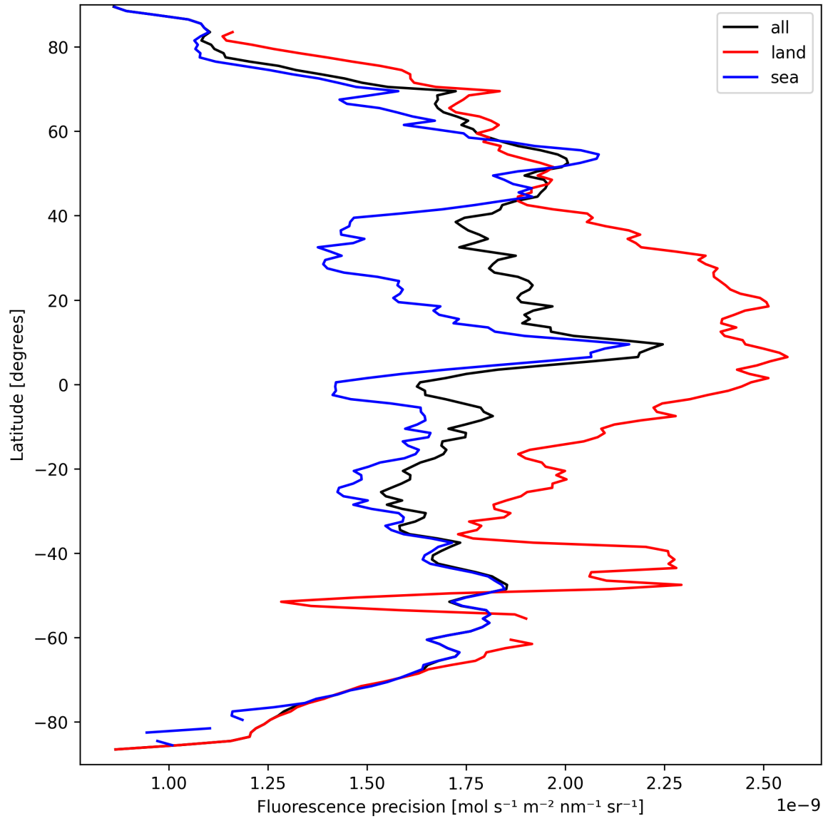
Figure 22: Zonal average of “Fluorescence precision” for 2025-09-18 to 2025-09-18.
