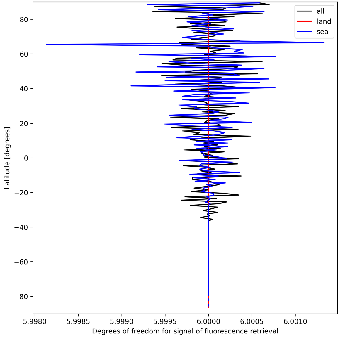
Figure 24: Zonal average of “Degrees of freedom for signal of fluorescence retrieval” for 2025-09-18 to 2025-09-18.
