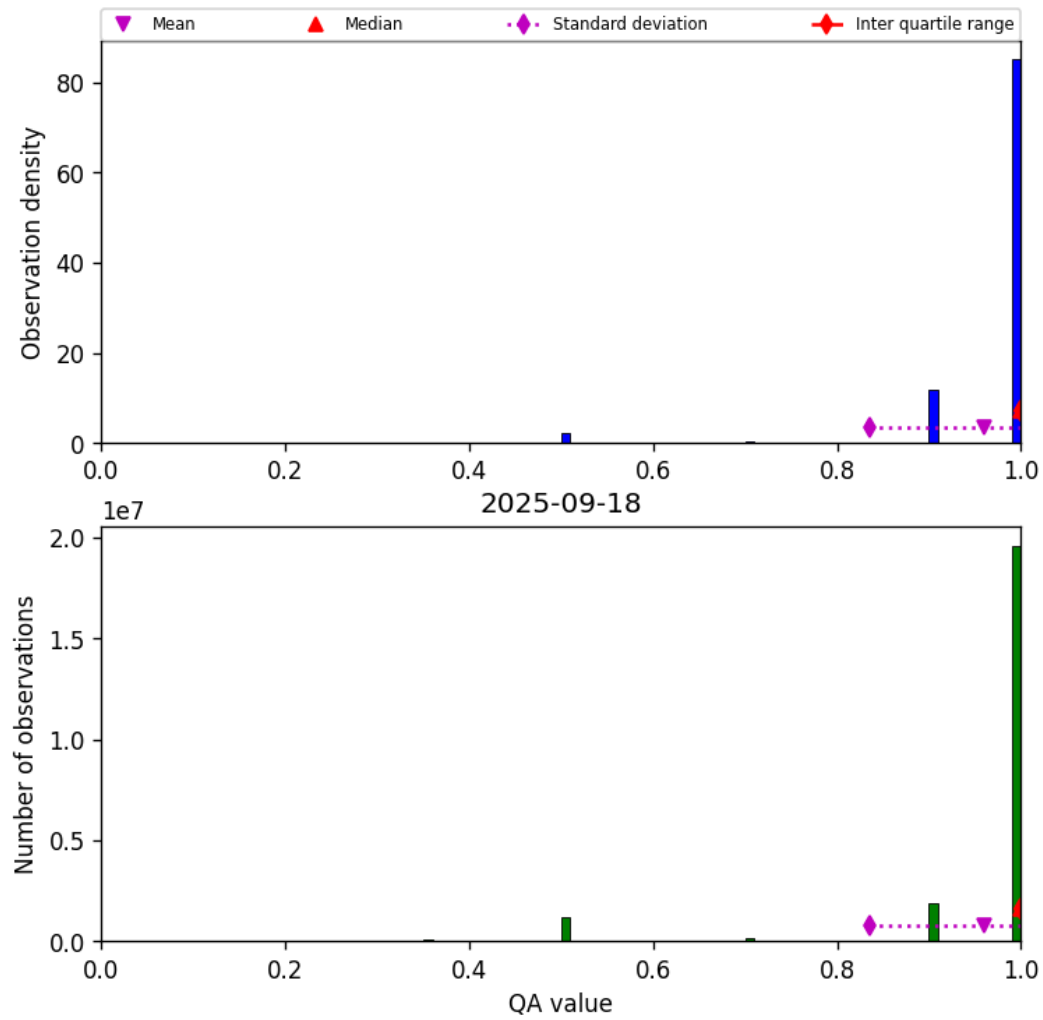
Figure 27: Histogram of “QA value” for 2025-09-18 to 2025-09-18
