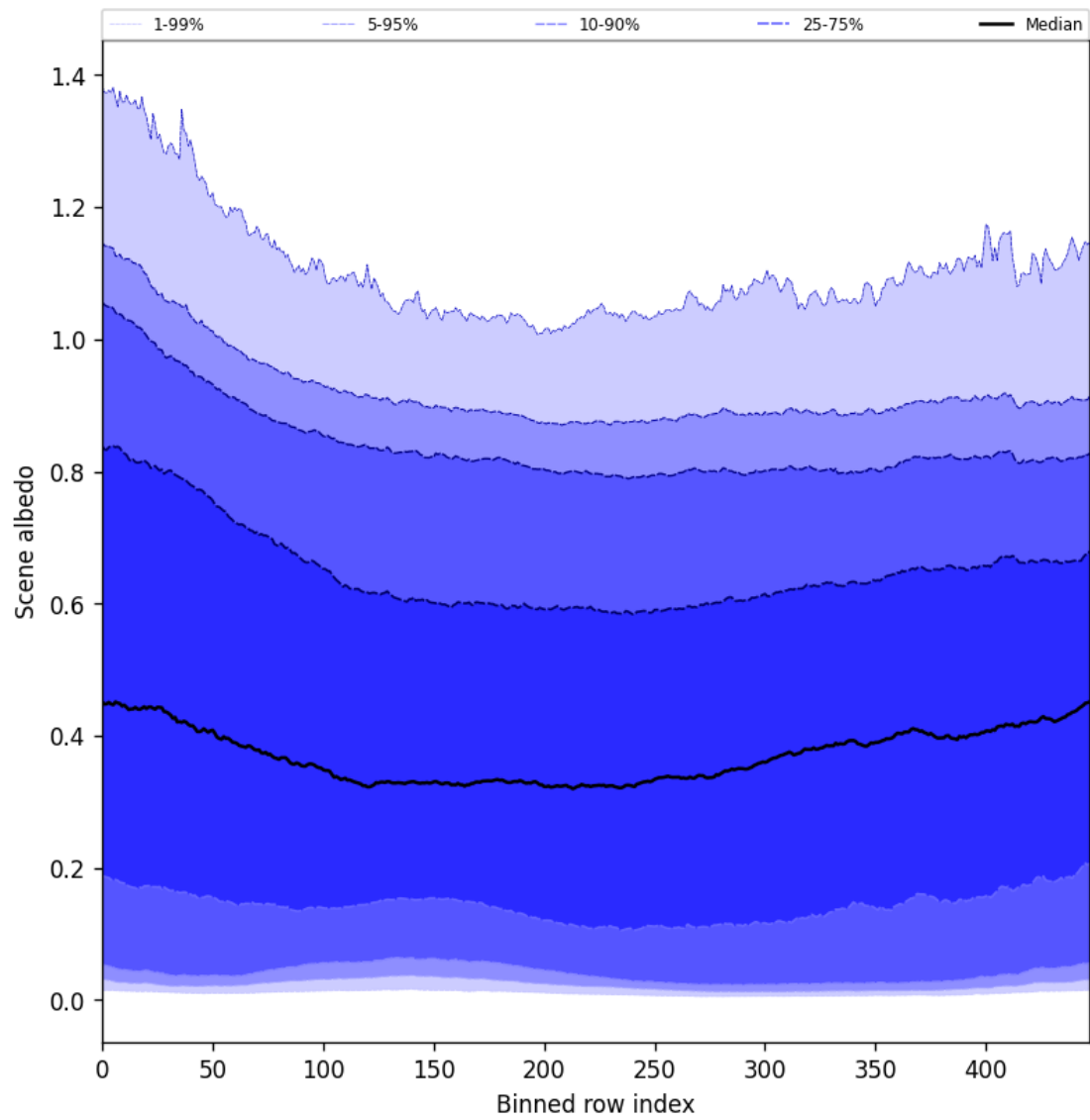
Figure 49: Along track statistics of “Scene albedo” for 2025-09-18 to 2025-09-18
