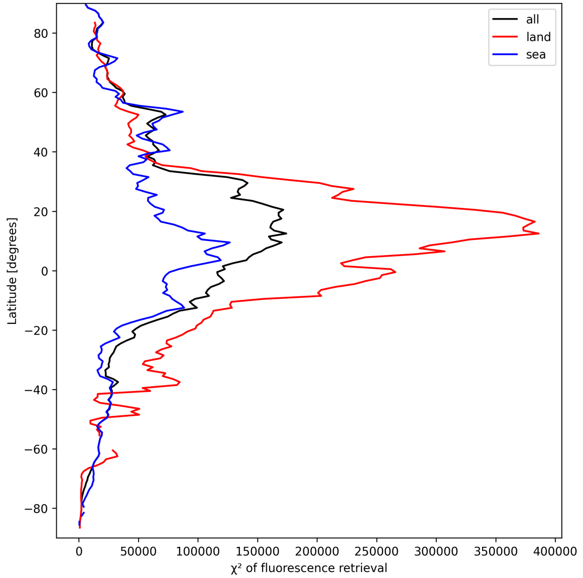
Figure 23: Zonal average of “ \chi^2 of fluorescence retrieval” for 2025-09-18 to 2025-09-18.
