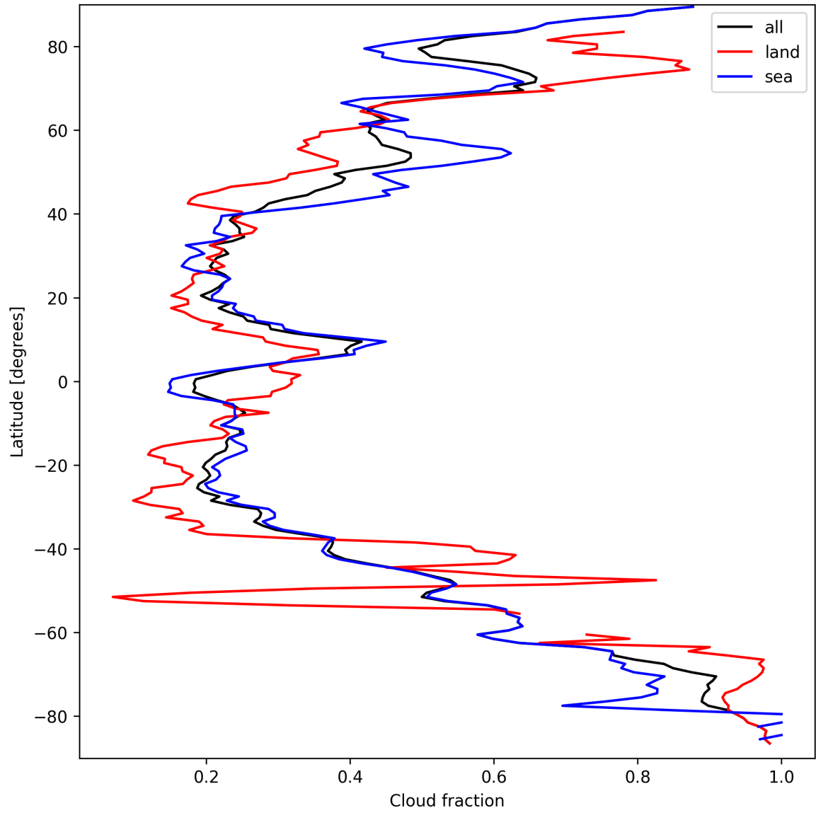
Figure 13: Zonal average of “Cloud fraction” for 2025-09-18 to 2025-09-18.
