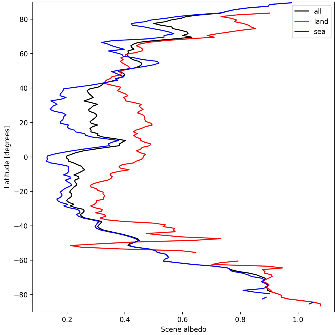
Figure 15: Zonal average of “Scene albedo” for 2025-09-18 to 2025-09-18.
