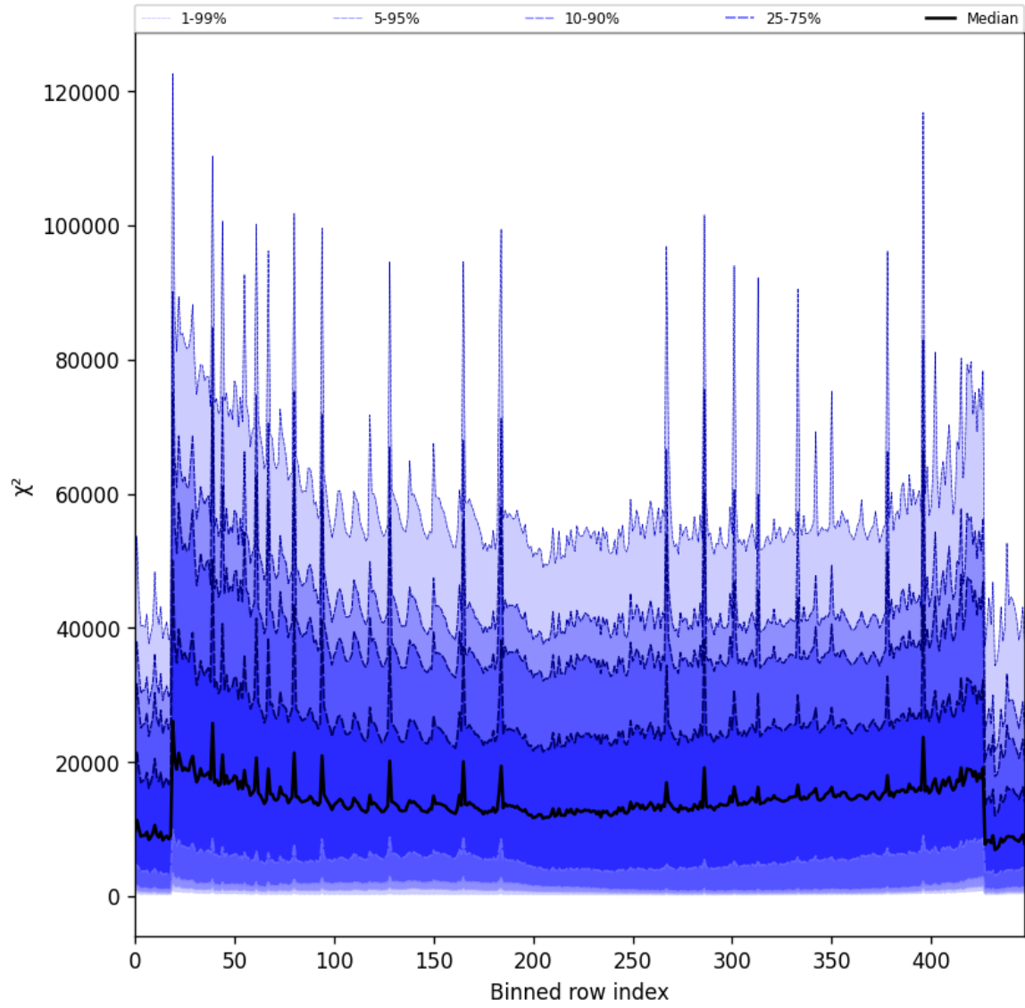
Figure 53: Along track statistics of “ \chi^2 ” for 2025-09-18 to 2025-09-18
