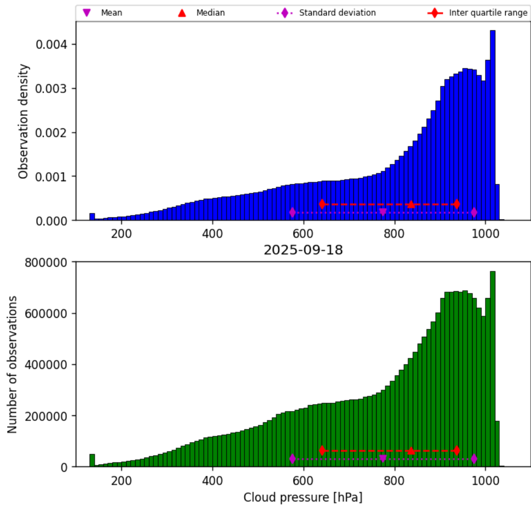
Figure 28: Histogram of “Cloud pressure” for 2025-09-18 to 2025-09-18
