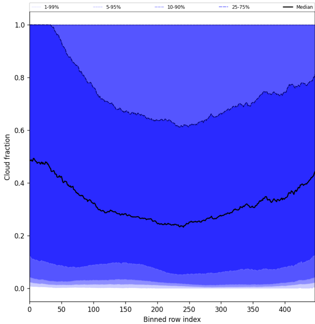
Figure 47: Along track statistics of “Cloud fraction” for 2025-09-18 to 2025-09-18
