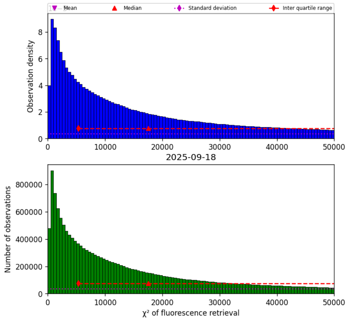
Figure 40: Histogram of “ \chi^2 of fluorescence retrieval” for 2025-09-18 to 2025-09-18
