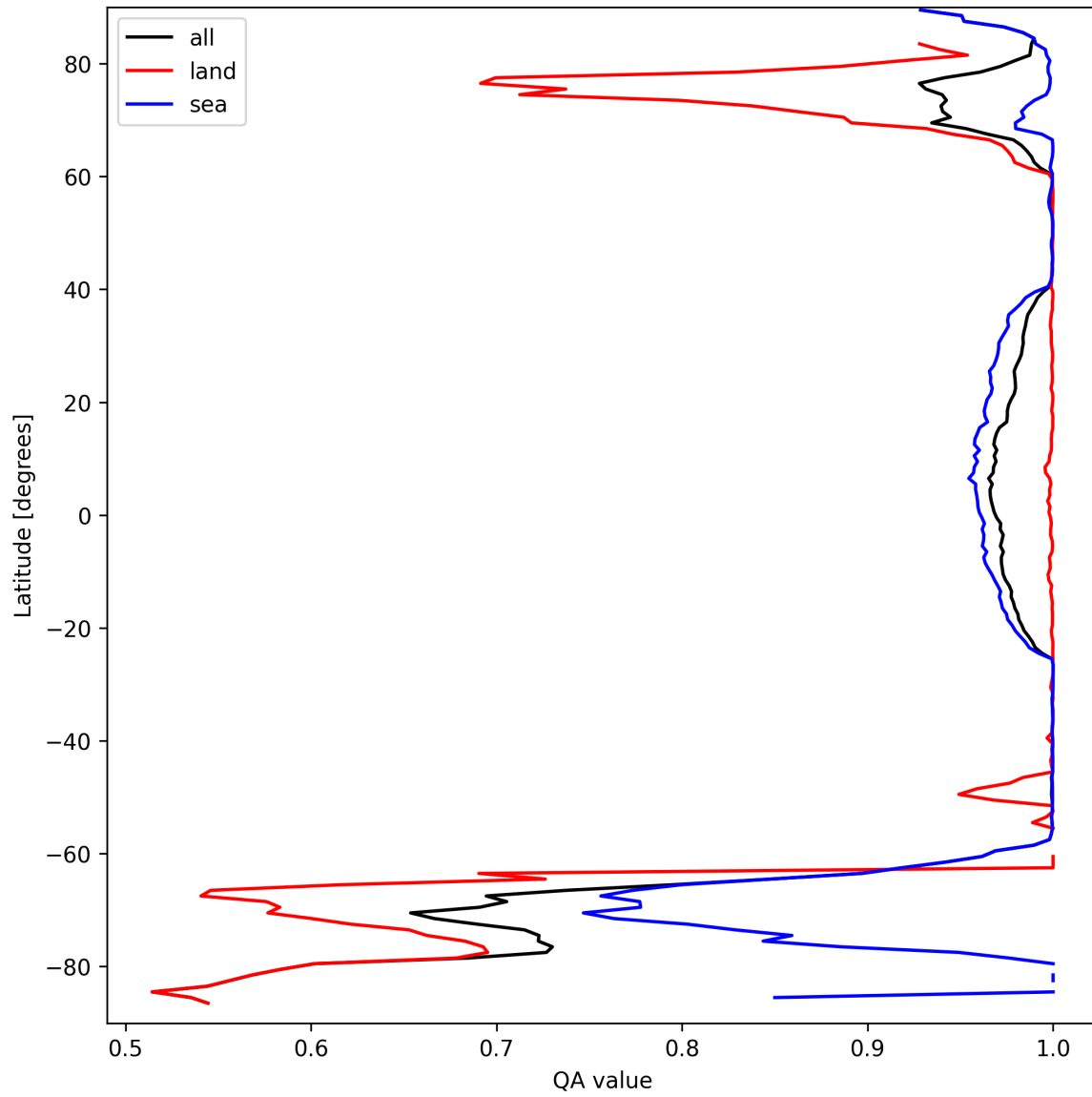
Figure 10: Zonal average of "QA value" for 2025-09-18 to 2025-09-18.
