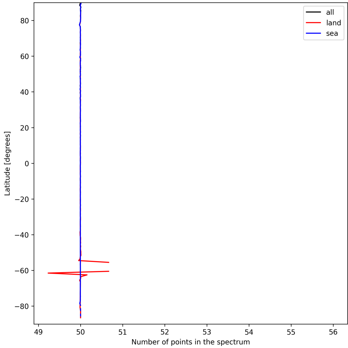
Figure 25: Zonal average of “Number of points in the spectrum” for 2025-09-18 to 2025-09-18.
