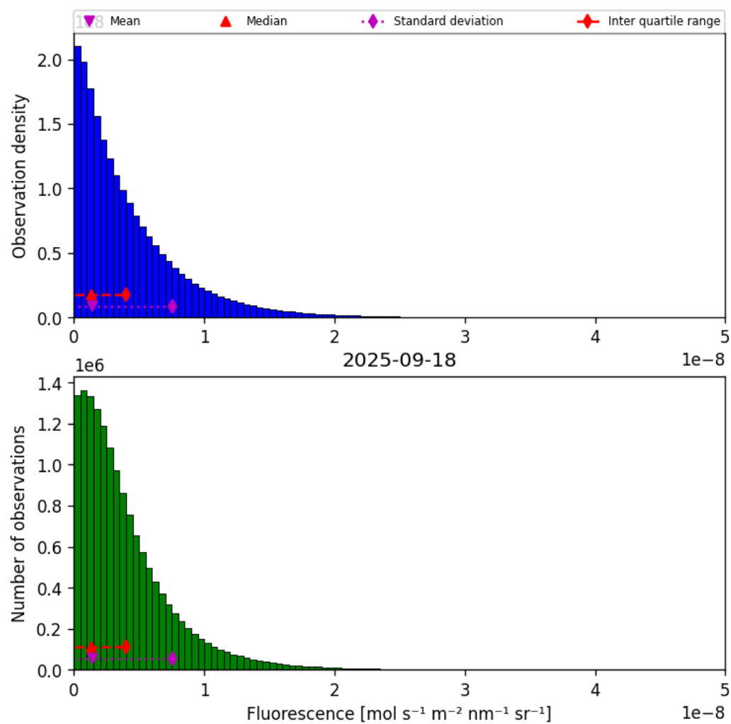
Figure 38: Histogram of “Fluorescence” for 2025-09-18 to 2025-09-18
