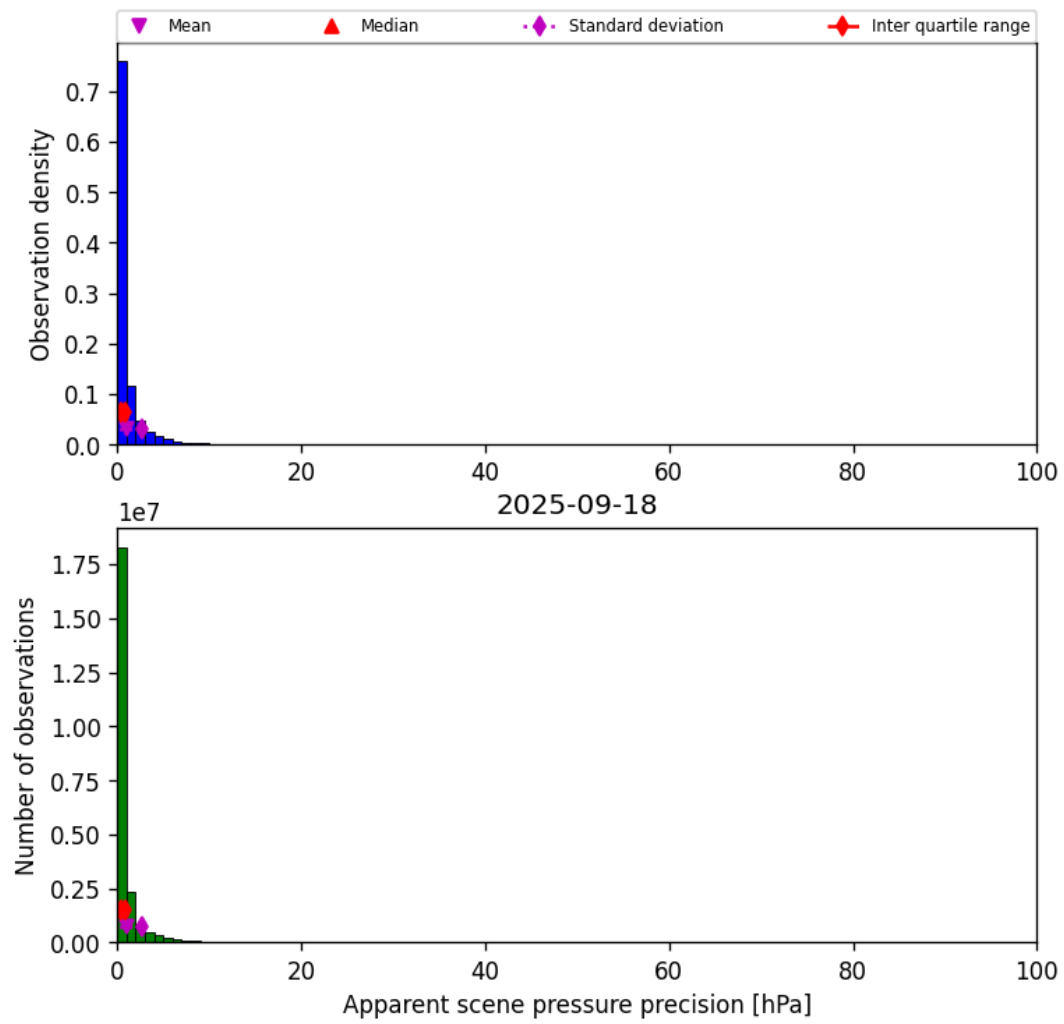
Figure 35: Histogram of “Apparent scene pressure precision” for 2025-09-18 to 2025-09-18
