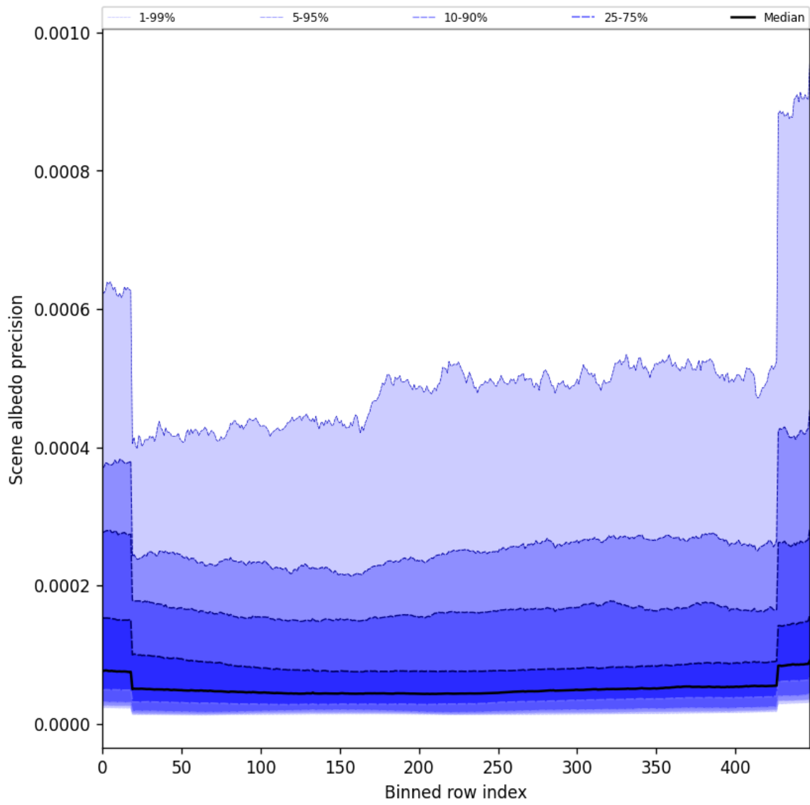
Figure 50: Along track statistics of “Scene albedo precision” for 2025-09-18 to 2025-09-18
