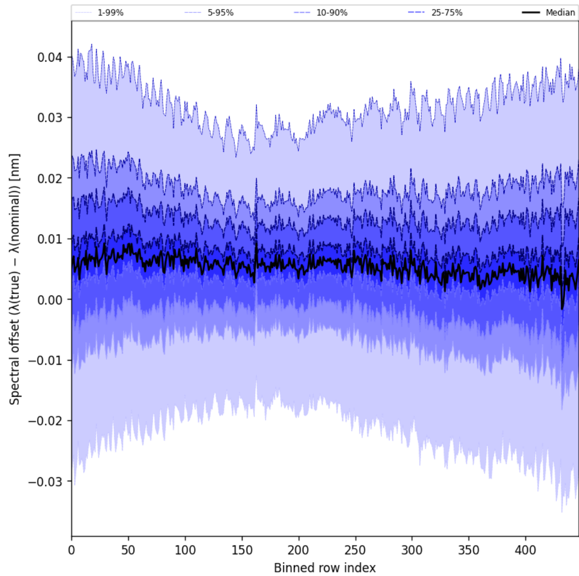
Figure 60: Along track statistics of “Spectral offset ( \lambda_{\text{true}} - \lambda_{\text{nominal}} )” for 2025-09-18 to 2025-09-18
