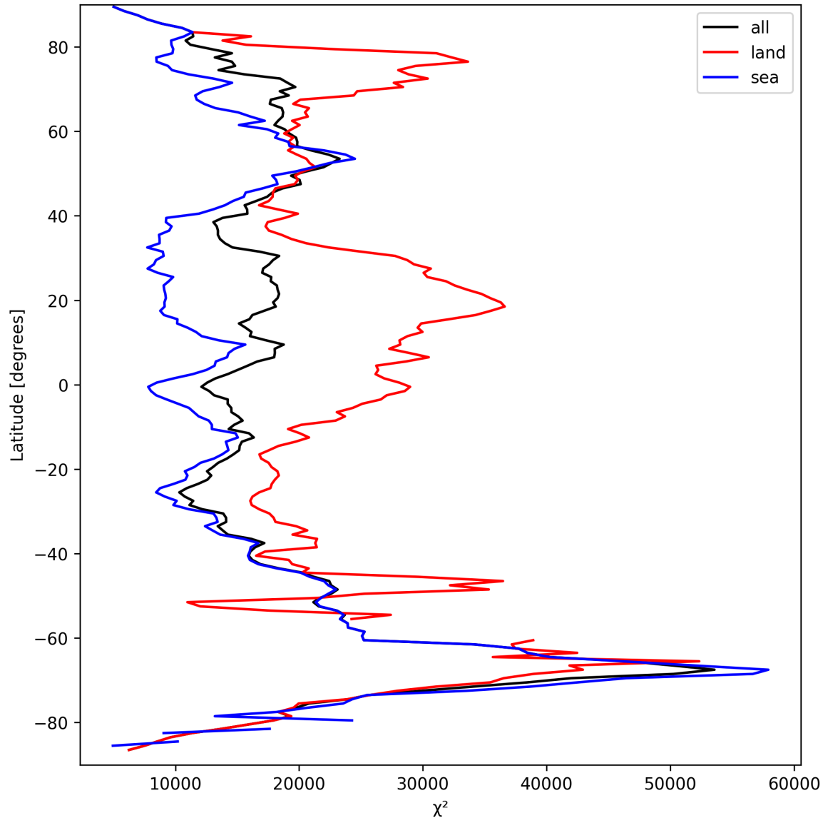
Figure 19: Zonal average of “ \chi^2 ” for 2025-09-18 to 2025-09-18.
