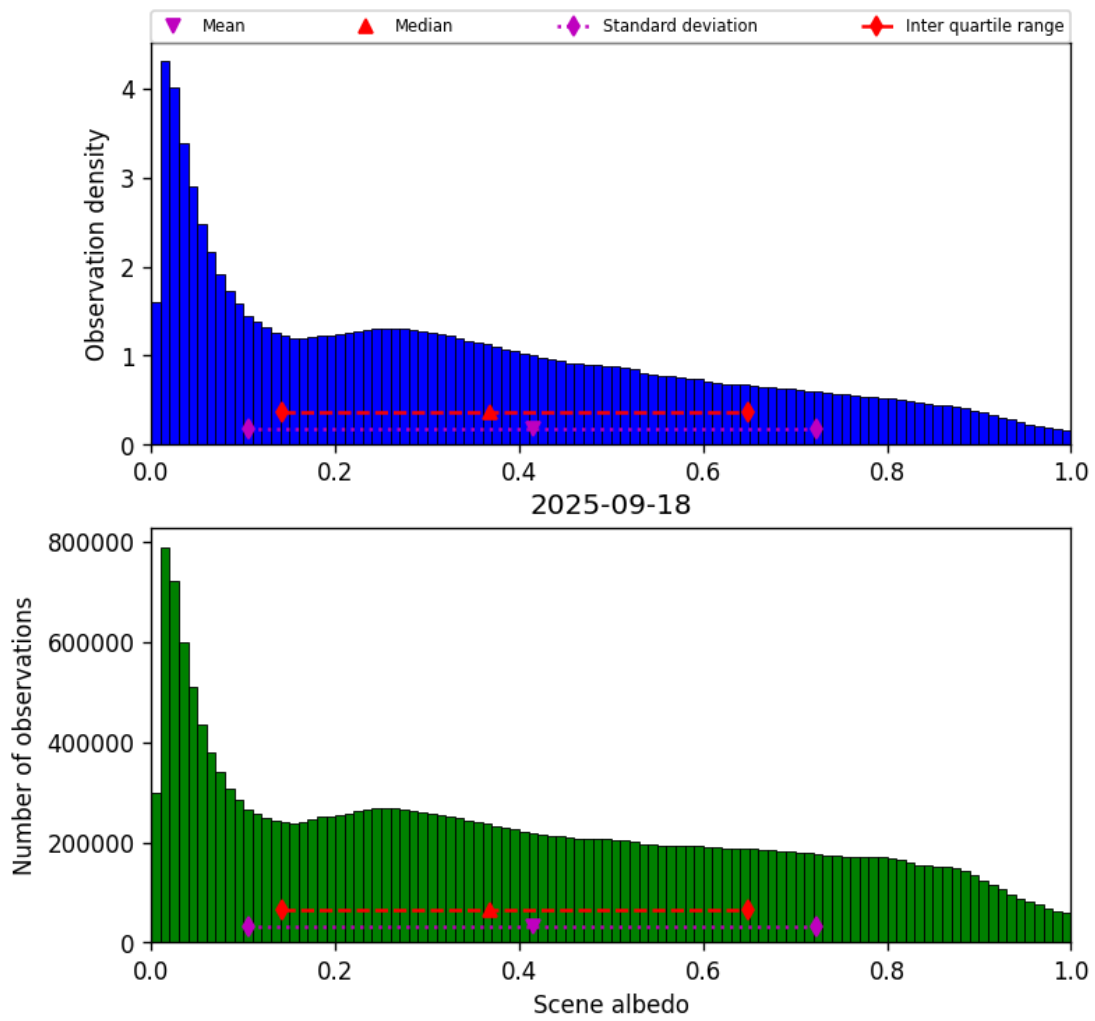
Figure 32: Histogram of “Scene albedo” for 2025-09-18 to 2025-09-18
