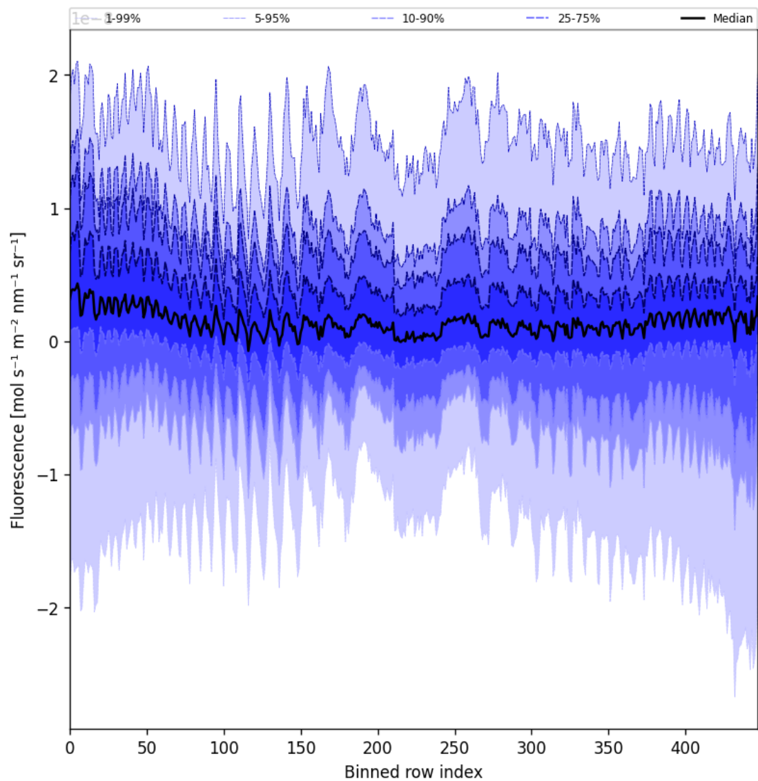
Figure 55: Along track statistics of “Fluorescence” for 2025-09-18 to 2025-09-18
