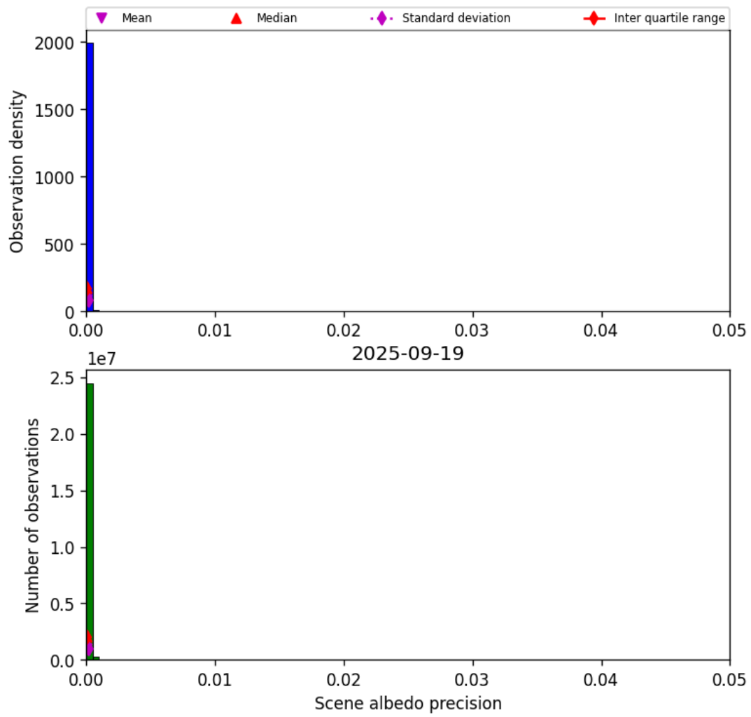
Figure 33: Histogram of “Scene albedo precision” for 2025-09-19 to 2025-09-20
