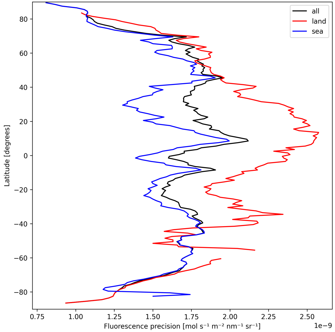
Figure 22: Zonal average of “Fluorescence precision” for 2025-09-19 to 2025-09-20.
