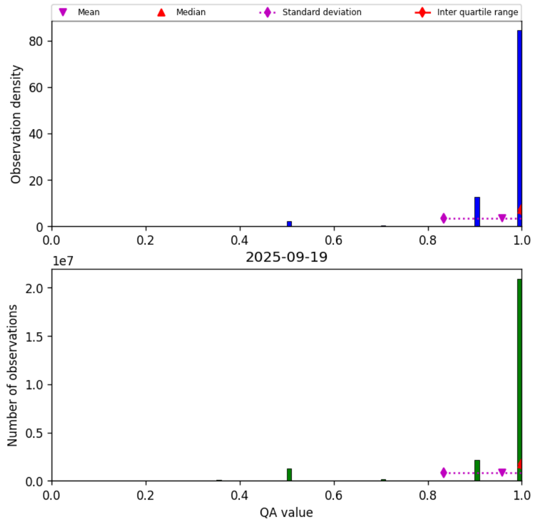
Figure 27: Histogram of “QA value” for 2025-09-19 to 2025-09-20
