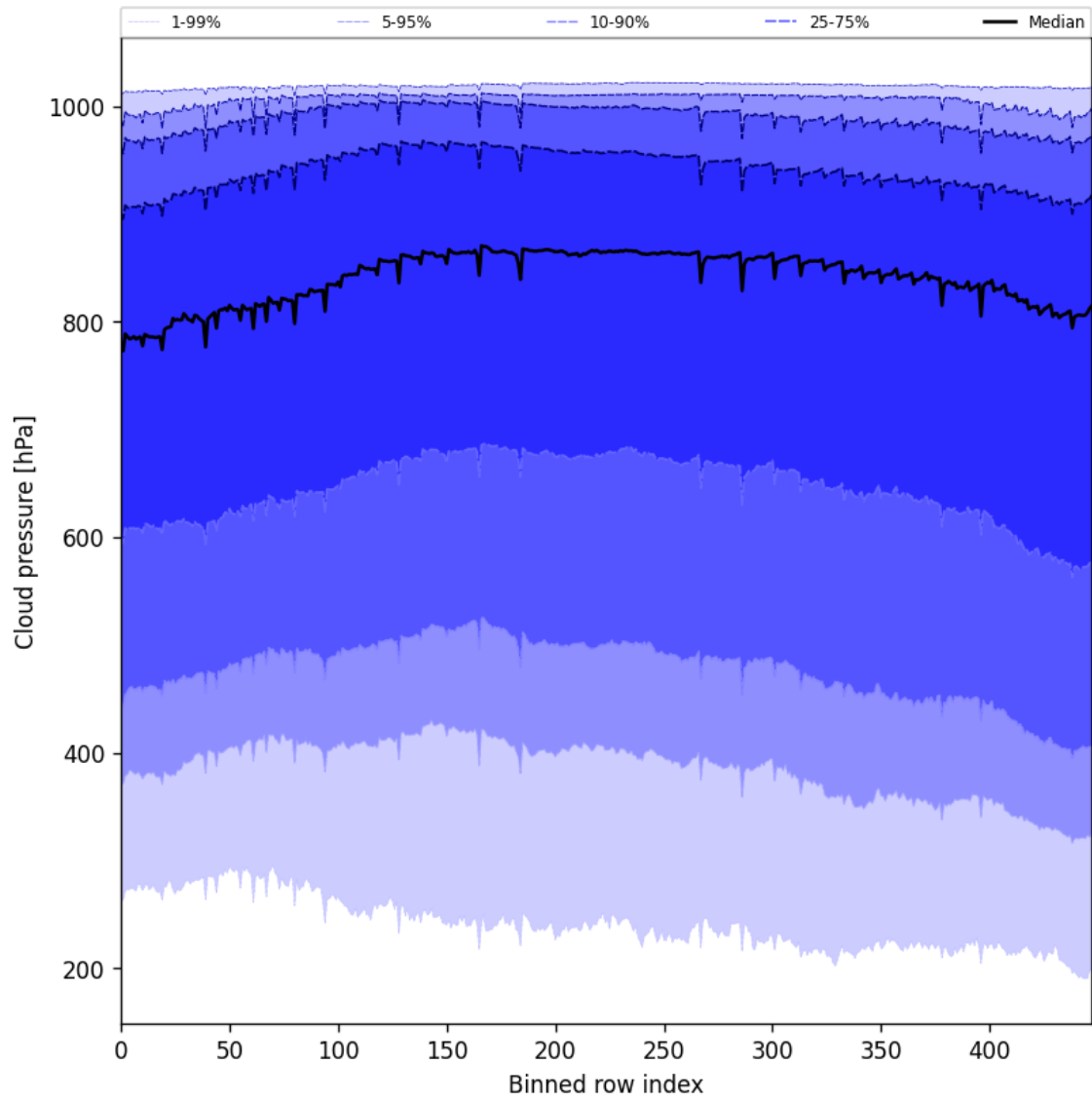
Figure 45: Along track statistics of “Cloud pressure” for 2025-09-19 to 2025-09-20
