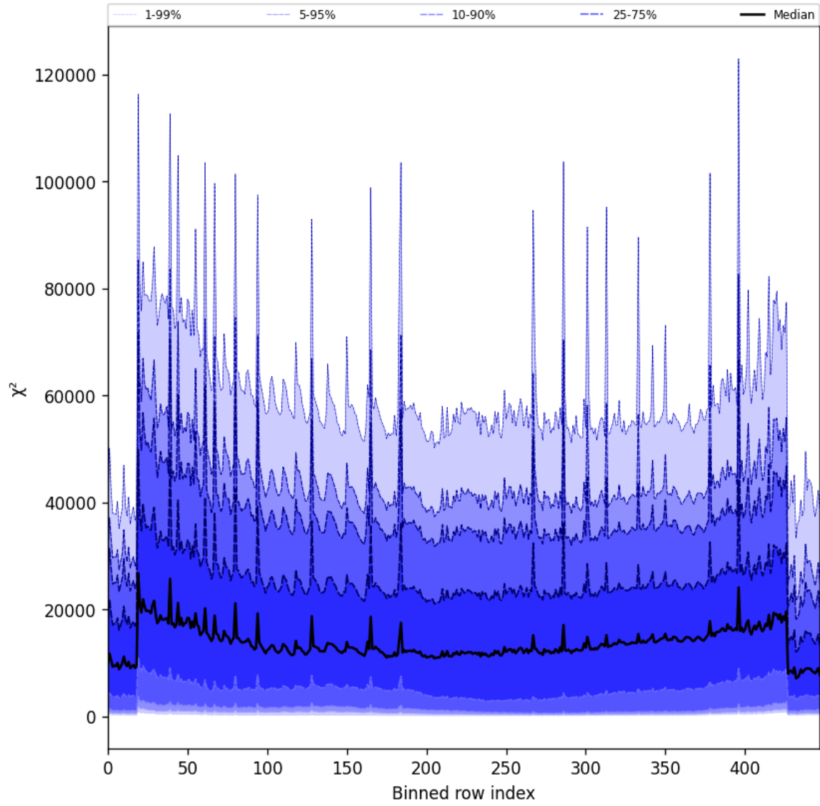
Figure 53: Along track statistics of “ \chi^2 ” for 2025-09-19 to 2025-09-20
