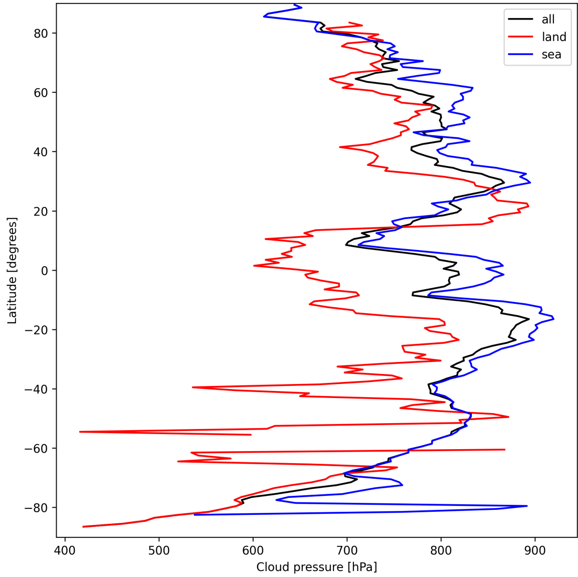
Figure 11: Zonal average of “Cloud pressure” for 2025-09-19 to 2025-09-20.
