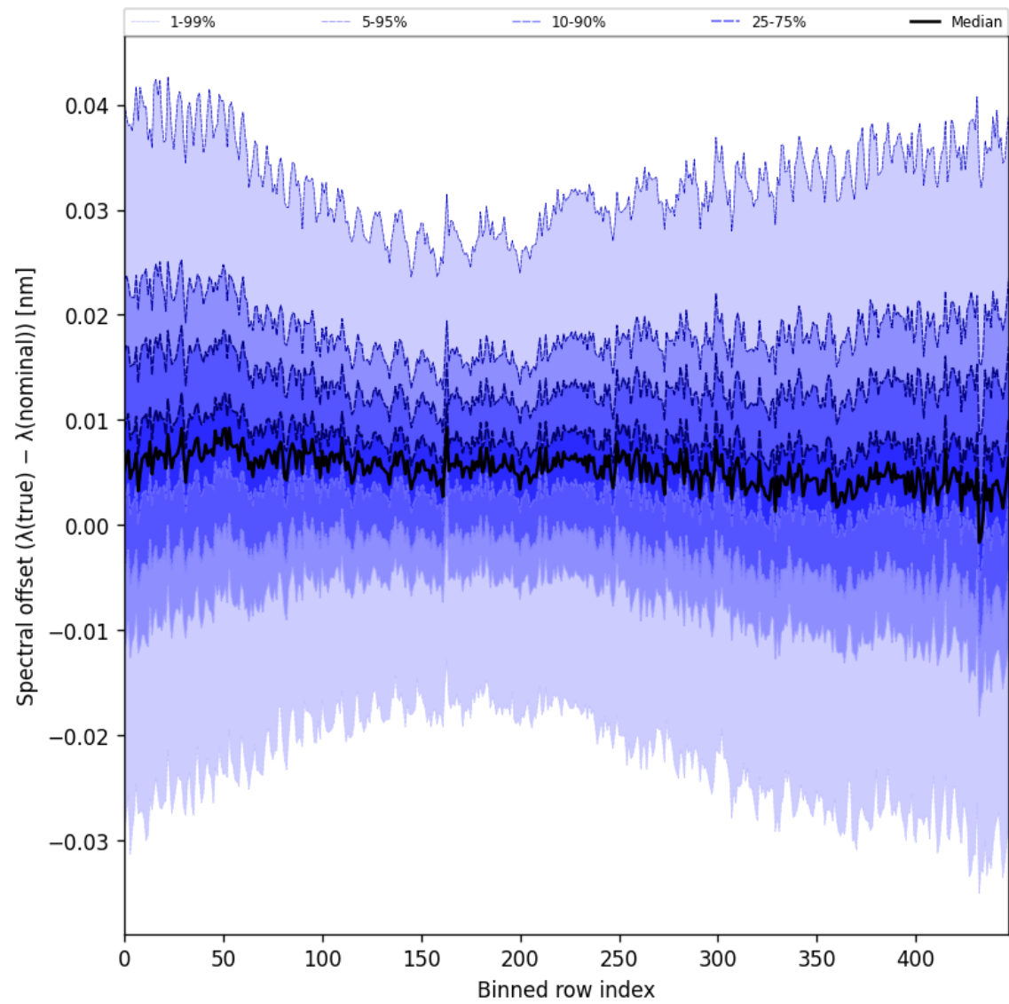
Figure 60: Along track statistics of “Spectral offset ( \lambda_{\text{true}} - \lambda_{\text{nominal}} )” for 2025-09-19 to 2025-09-20
