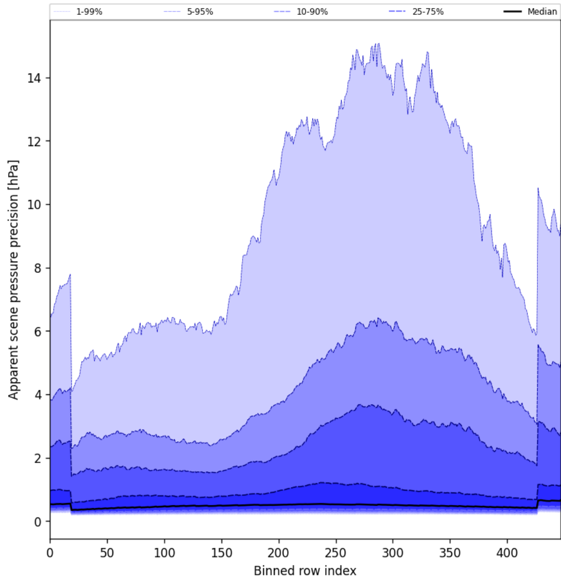
Figure 52: Along track statistics of “Apparent scene pressure precision” for 2025-09-19 to 2025-09-20
