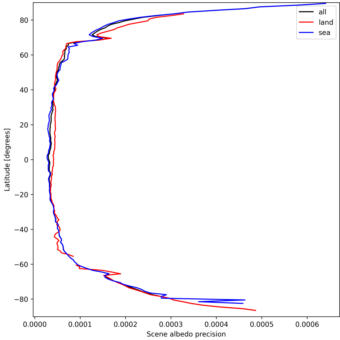
Figure 16: Zonal average of “Scene albedo precision” for 2025-09-19 to 2025-09-20.
