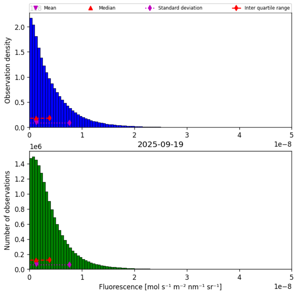
Figure 38: Histogram of “Fluorescence” for 2025-09-19 to 2025-09-20
