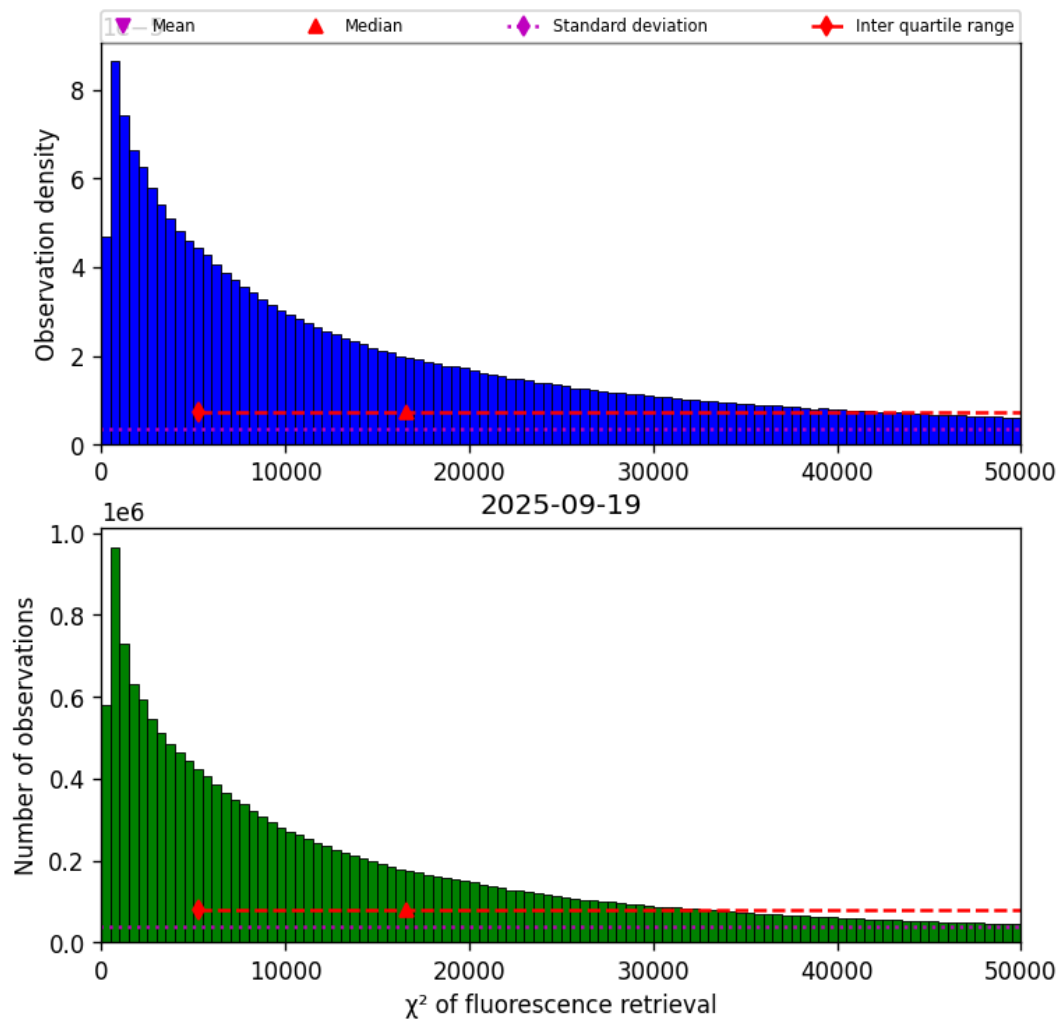
Figure 40: Histogram of “ \chi^2 of fluorescence retrieval” for 2025-09-19 to 2025-09-20
