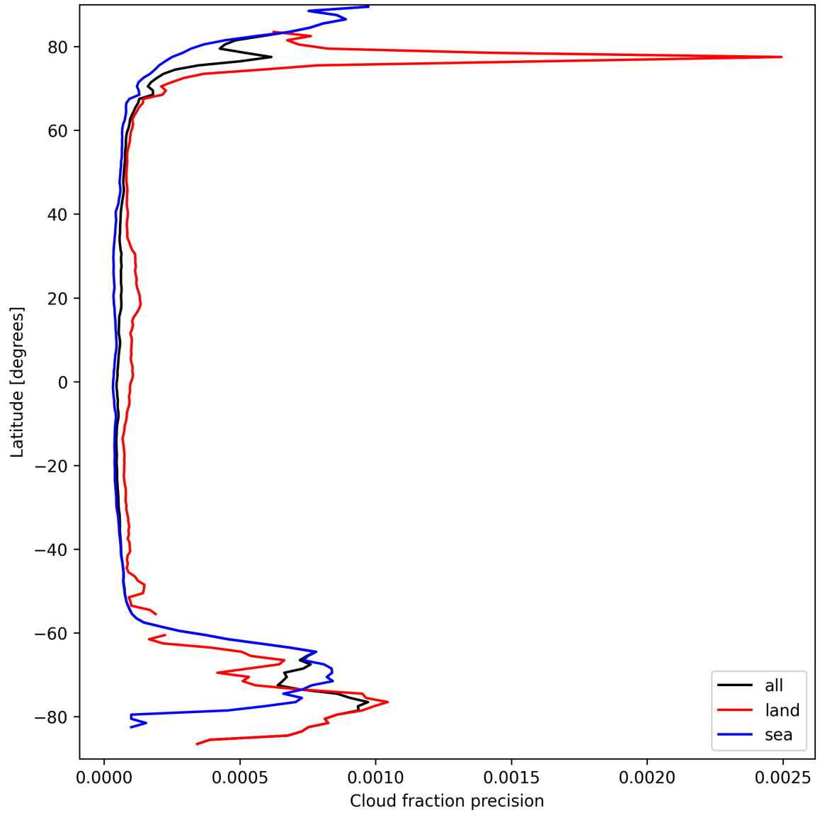
Figure 14: Zonal average of “Cloud fraction precision” for 2025-09-19 to 2025-09-20.
