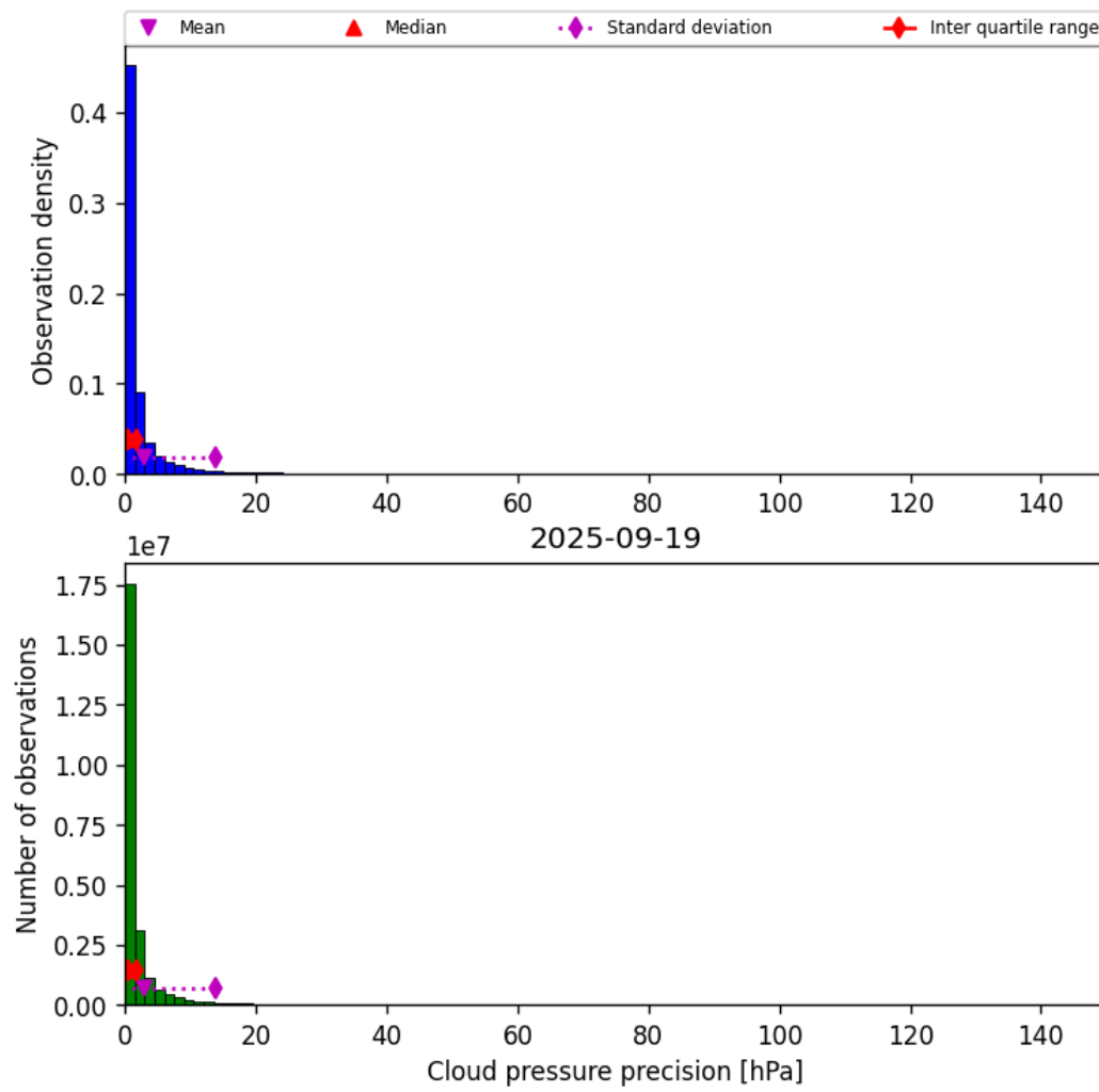
Figure 29: Histogram of “Cloud pressure precision” for 2025-09-19 to 2025-09-20
