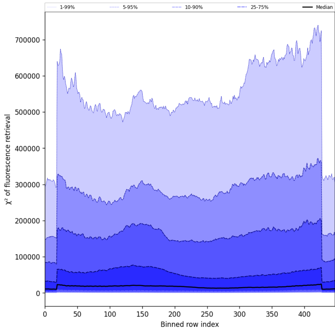
Figure 57: Along track statistics of “ \chi^2 of fluorescence retrieval” for 2025-09-19 to 2025-09-20
