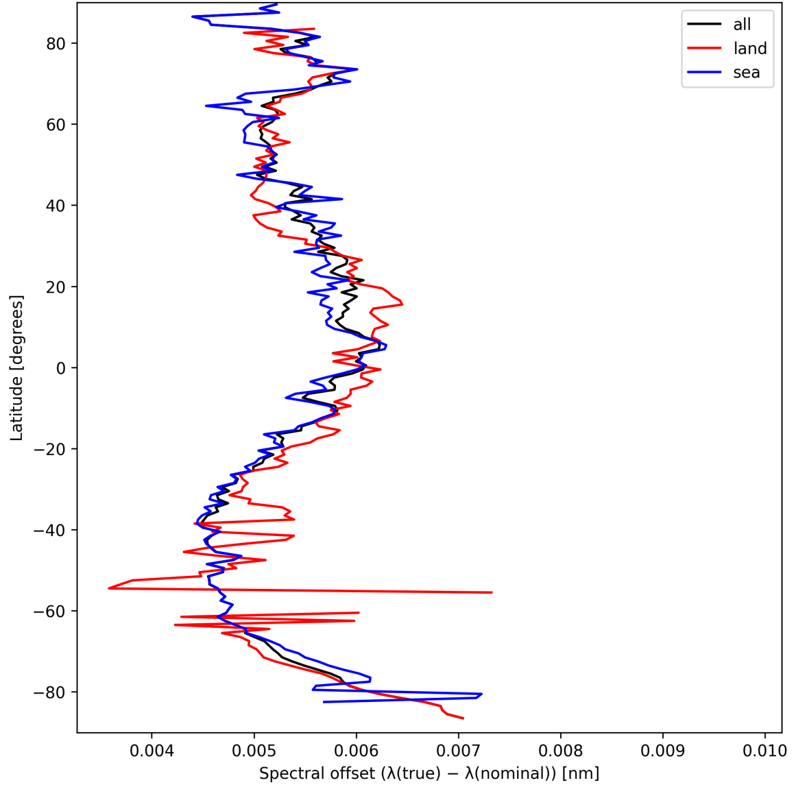
Figure 26: Zonal average of “Spectral offset ( \lambda_{\text{true}} - \lambda_{\text{nominal}} )” for 2025-09-19 to 2025-09-20.
