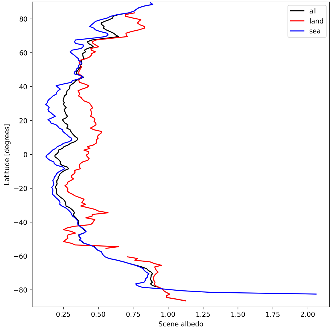
Figure 15: Zonal average of “Scene albedo” for 2025-09-19 to 2025-09-20.
