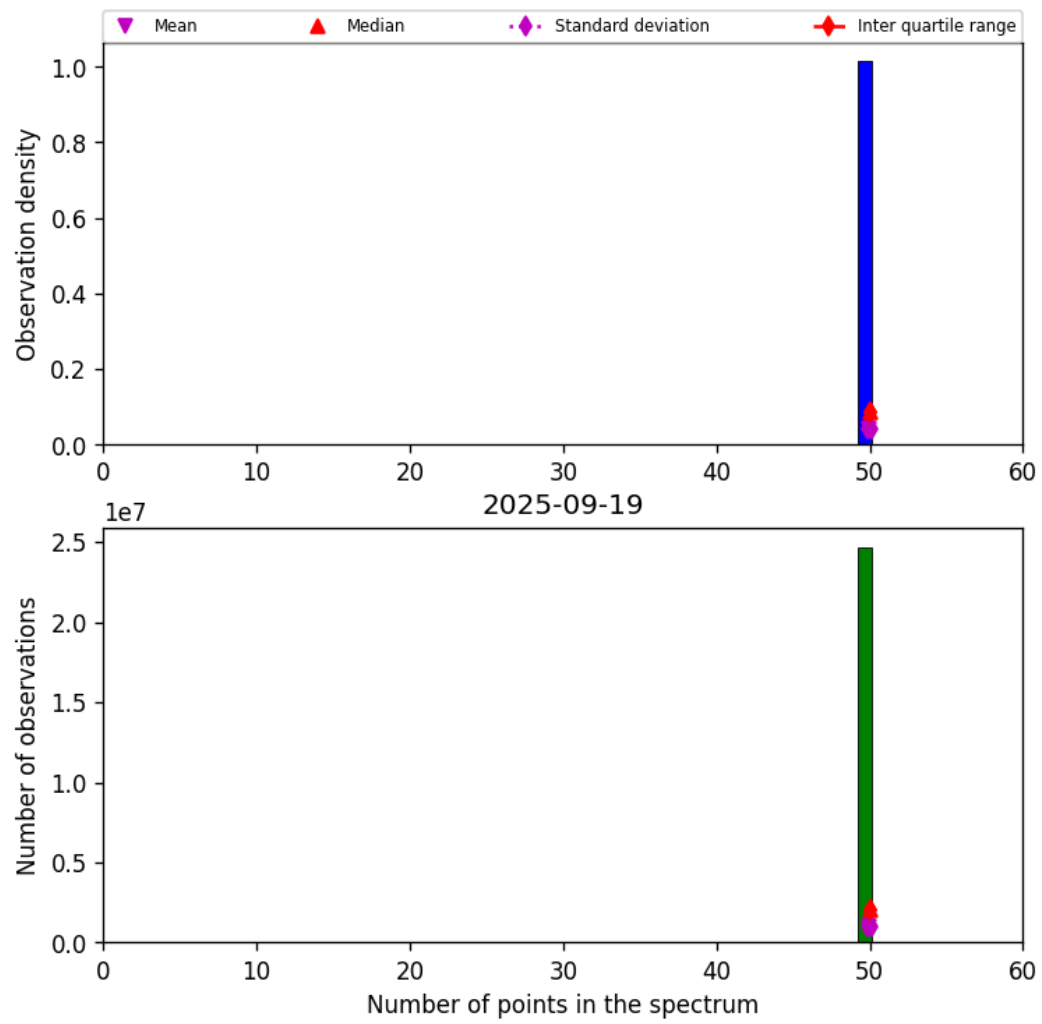
Figure 42: Histogram of "Number of points in the spectrum" for 2025-09-19 to 2025-09-20
