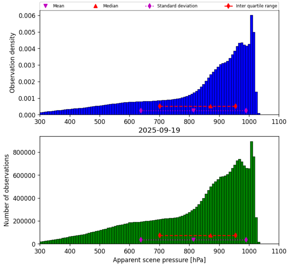
Figure 34: Histogram of “Apparent scene pressure” for 2025-09-19 to 2025-09-20
