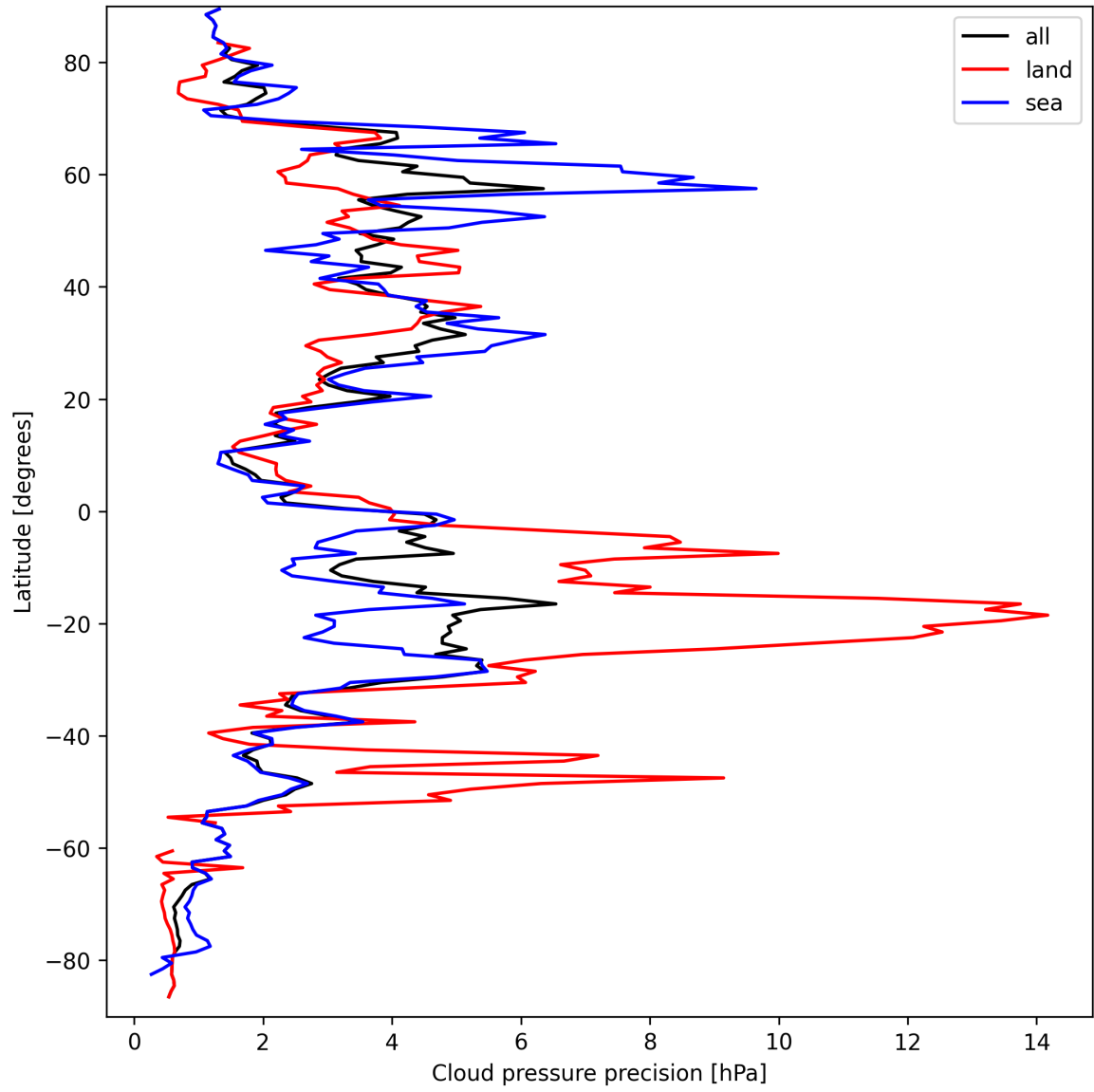
Figure 12: Zonal average of “Cloud pressure precision” for 2025-09-19 to 2025-09-20.
