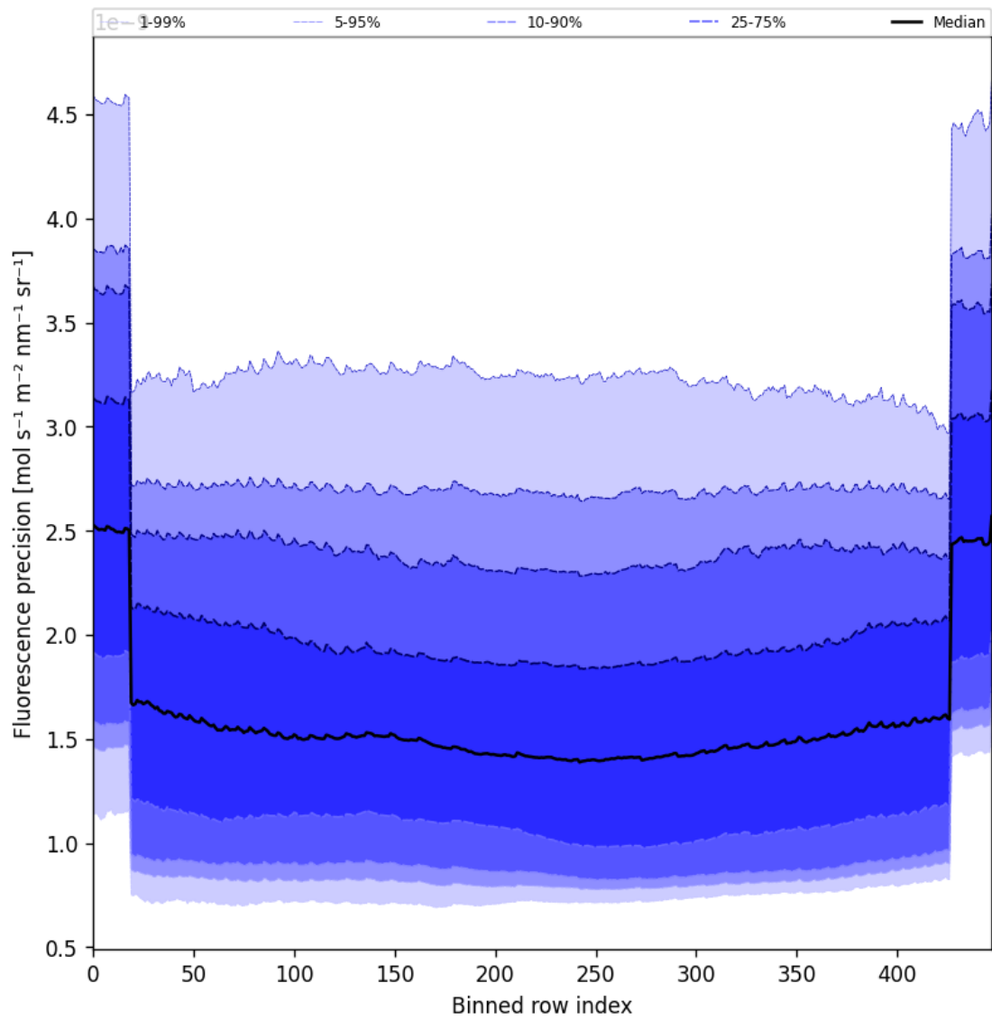
Figure 56: Along track statistics of “Fluorescence precision” for 2025-09-19 to 2025-09-20
