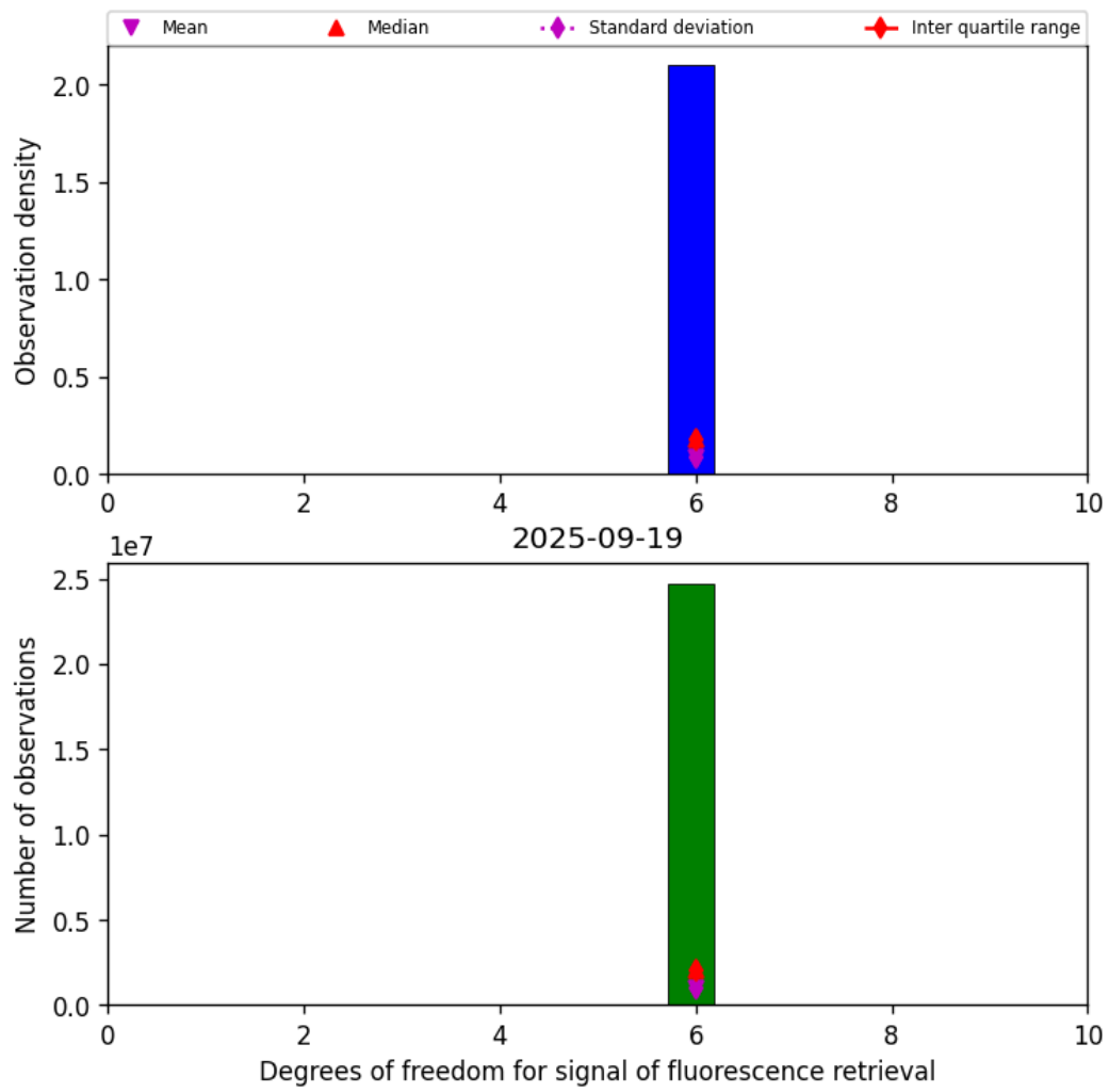
Figure 41: Histogram of “Degrees of freedom for signal of fluorescence retrieval” for 2025-09-19 to 2025-09-20
