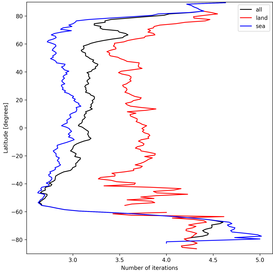
Figure 20: Zonal average of “Number of iterations” for 2025-09-19 to 2025-09-20.
