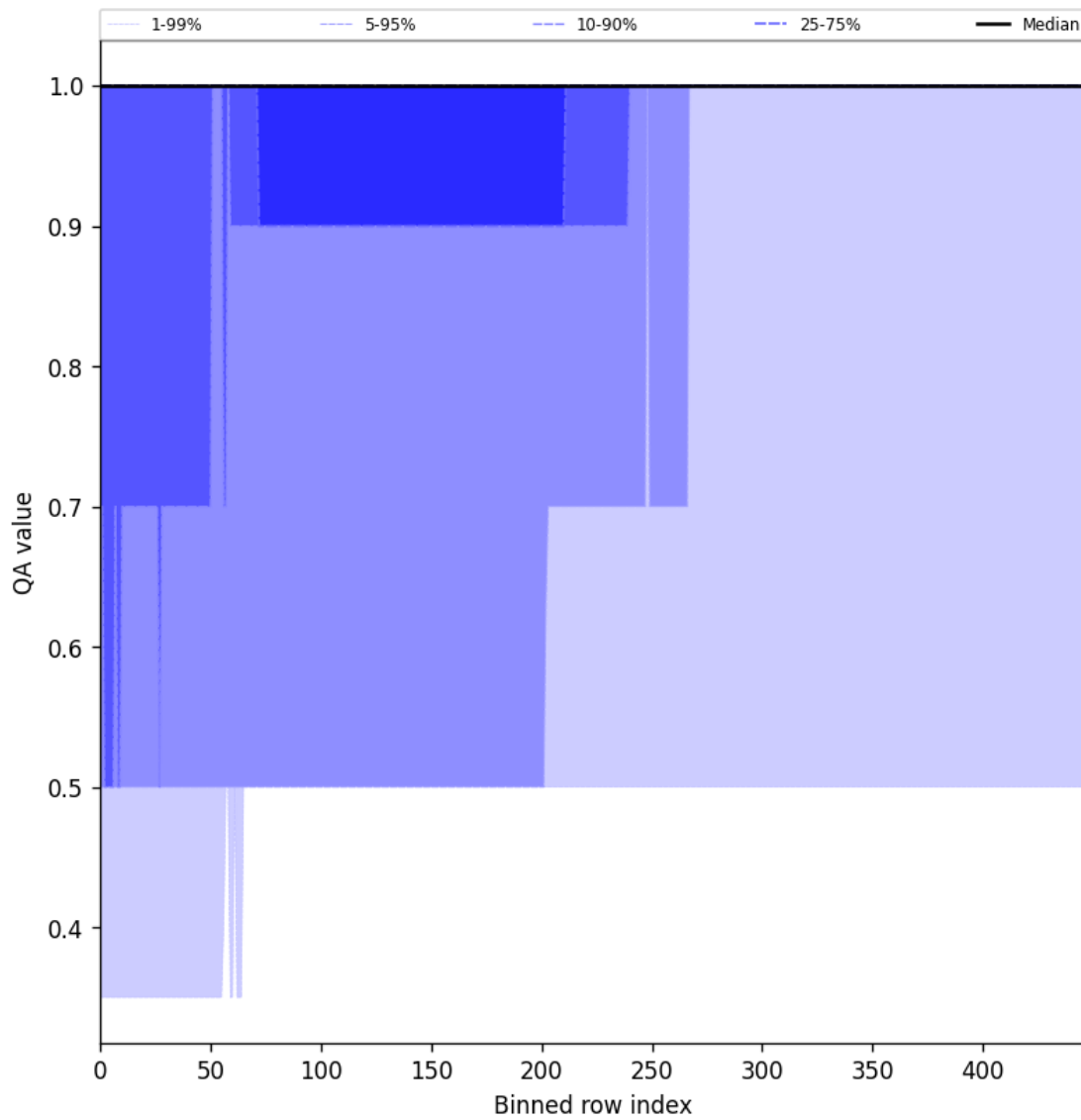
Figure 44: Along track statistics of “QA value” for 2025-09-19 to 2025-09-20
