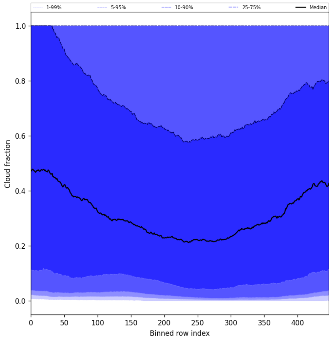
Figure 47: Along track statistics of “Cloud fraction” for 2025-09-19 to 2025-09-20
