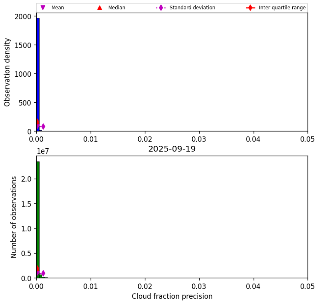
Figure 31: Histogram of “Cloud fraction precision” for 2025-09-19 to 2025-09-20
