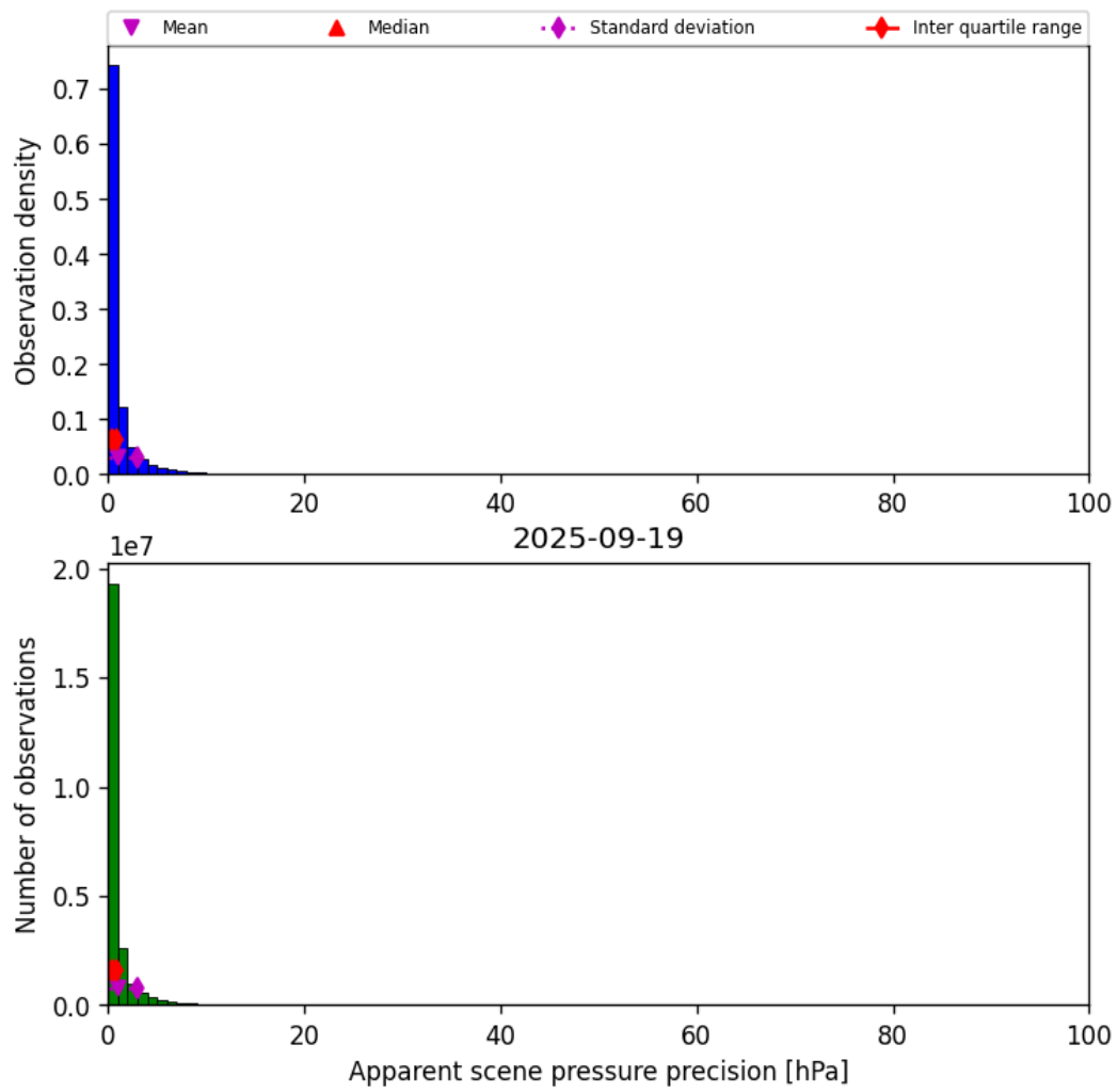
Figure 35: Histogram of “Apparent scene pressure precision” for 2025-09-19 to 2025-09-20
