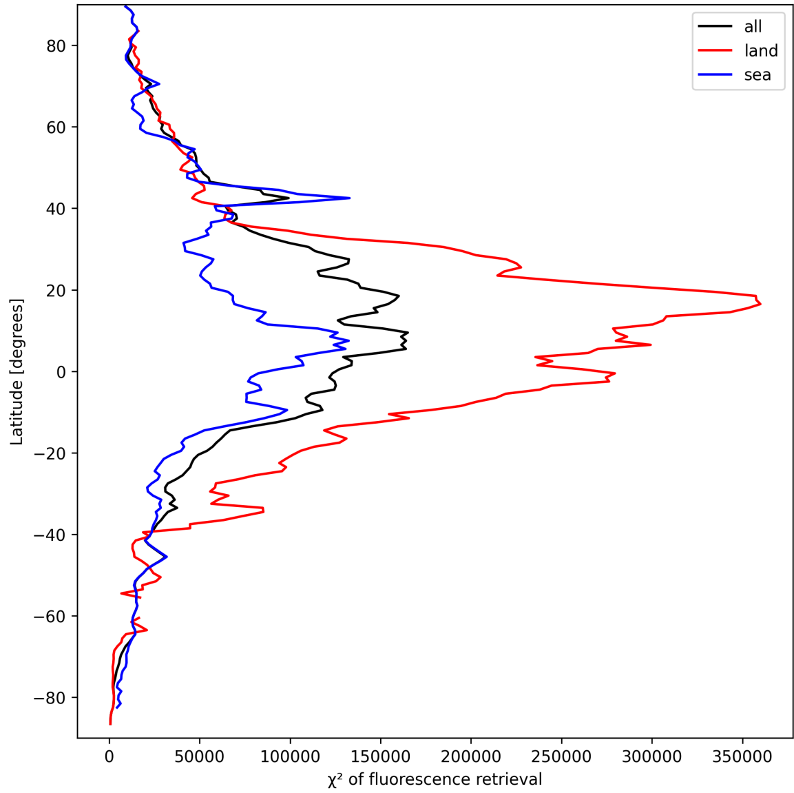
Figure 23: Zonal average of “ \chi^2 of fluorescence retrieval” for 2025-09-19 to 2025-09-20.
