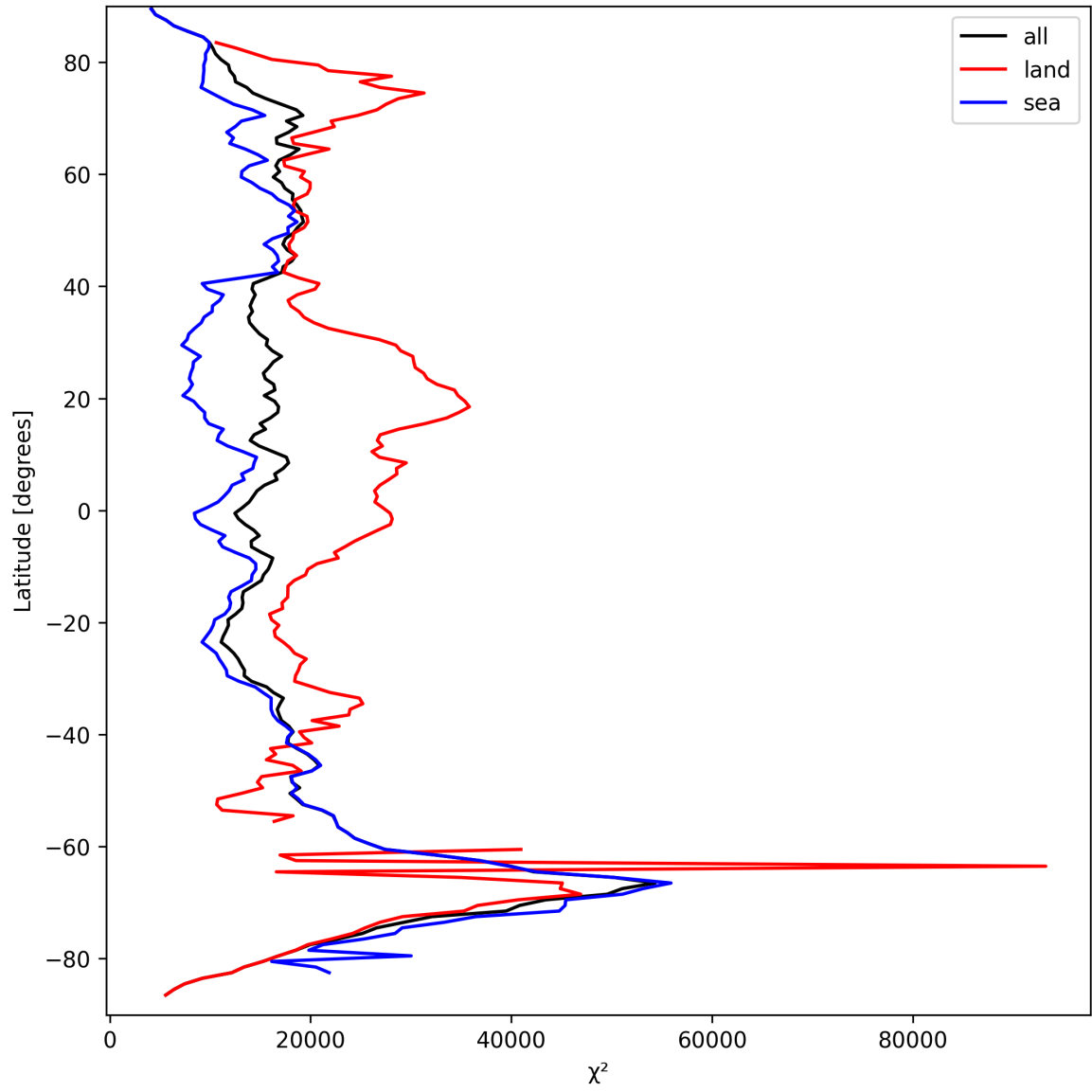
Figure 19: Zonal average of “ \chi^2 ” for 2025-09-19 to 2025-09-20.
