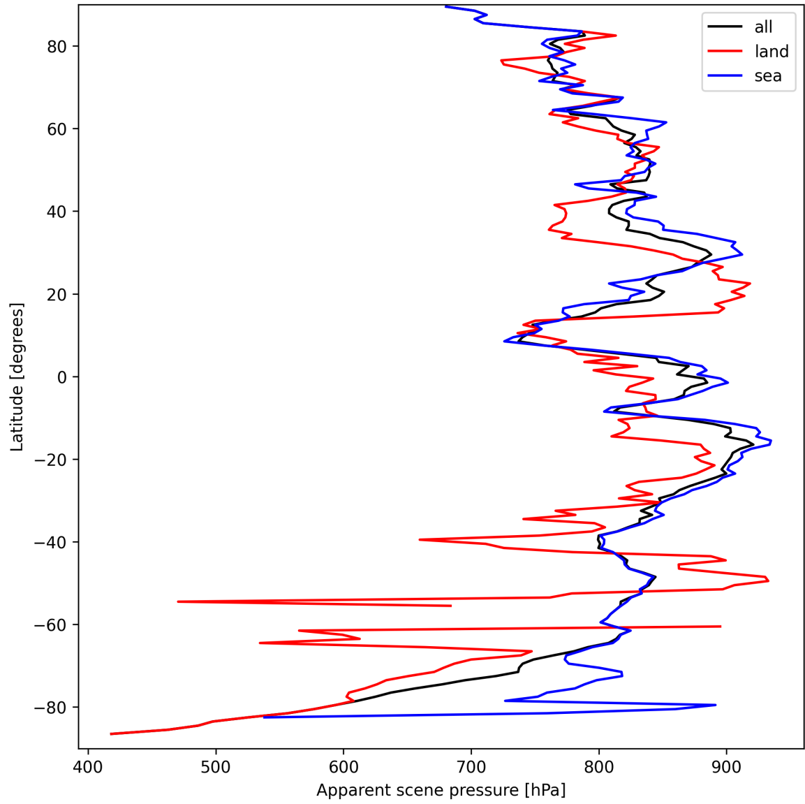
Figure 17: Zonal average of “Apparent scene pressure” for 2025-09-19 to 2025-09-20.
