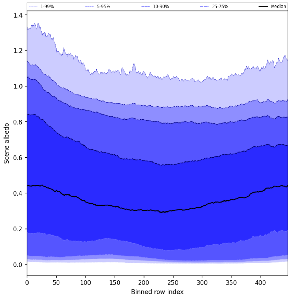
Figure 49: Along track statistics of “Scene albedo” for 2025-09-19 to 2025-09-20
