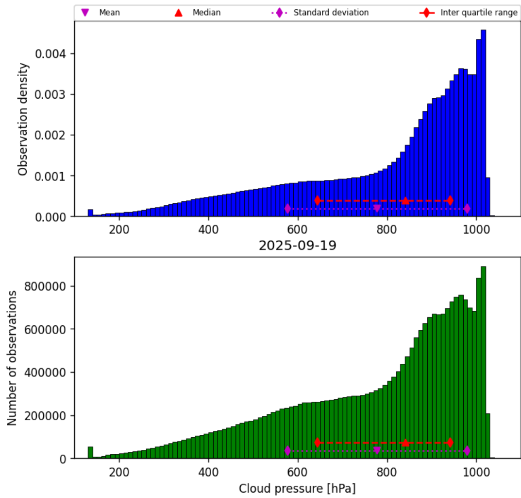
Figure 28: Histogram of “Cloud pressure” for 2025-09-19 to 2025-09-20
