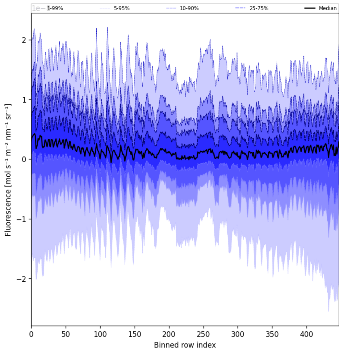
Figure 55: Along track statistics of “Fluorescence” for 2025-09-19 to 2025-09-20
