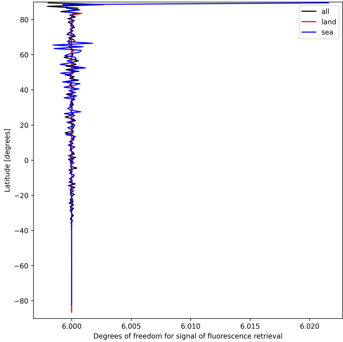
Figure 24: Zonal average of “Degrees of freedom for signal of fluorescence retrieval” for 2025-09-19 to 2025-09-20.
