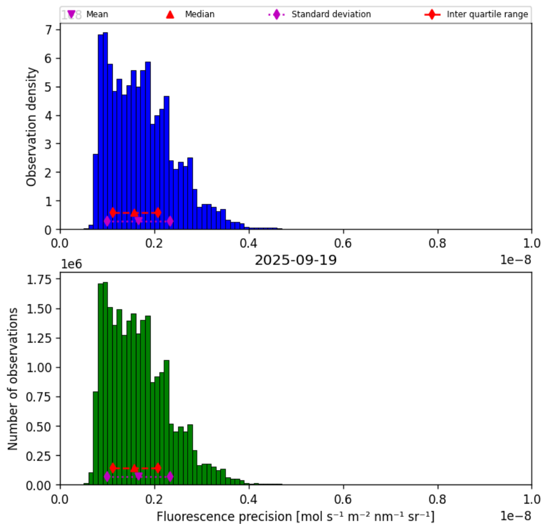
Figure 39: Histogram of “Fluorescence precision” for 2025-09-19 to 2025-09-20
