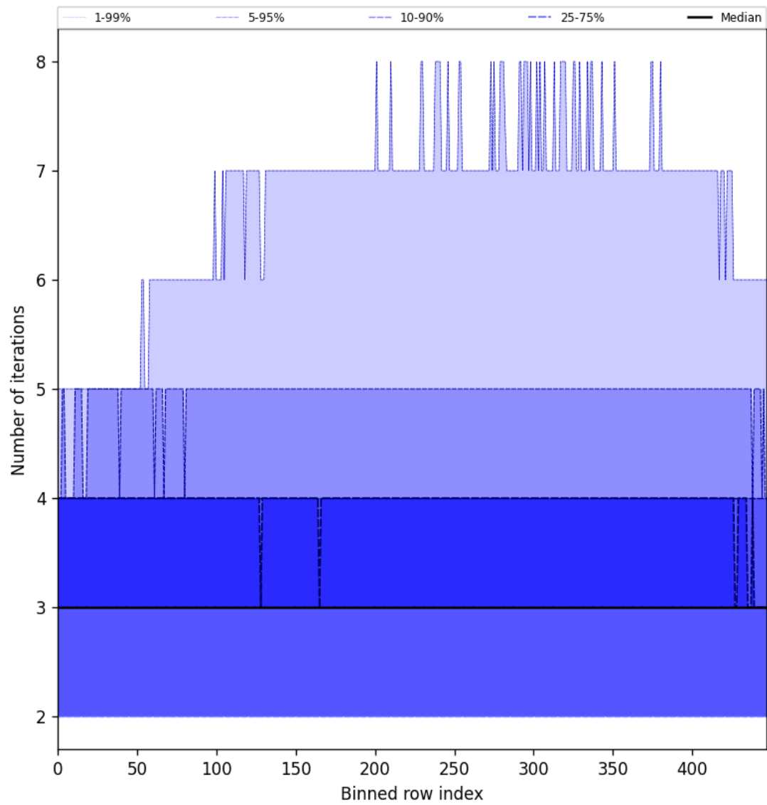
Figure 54: Along track statistics of “Number of iterations” for 2025-09-19 to 2025-09-20
