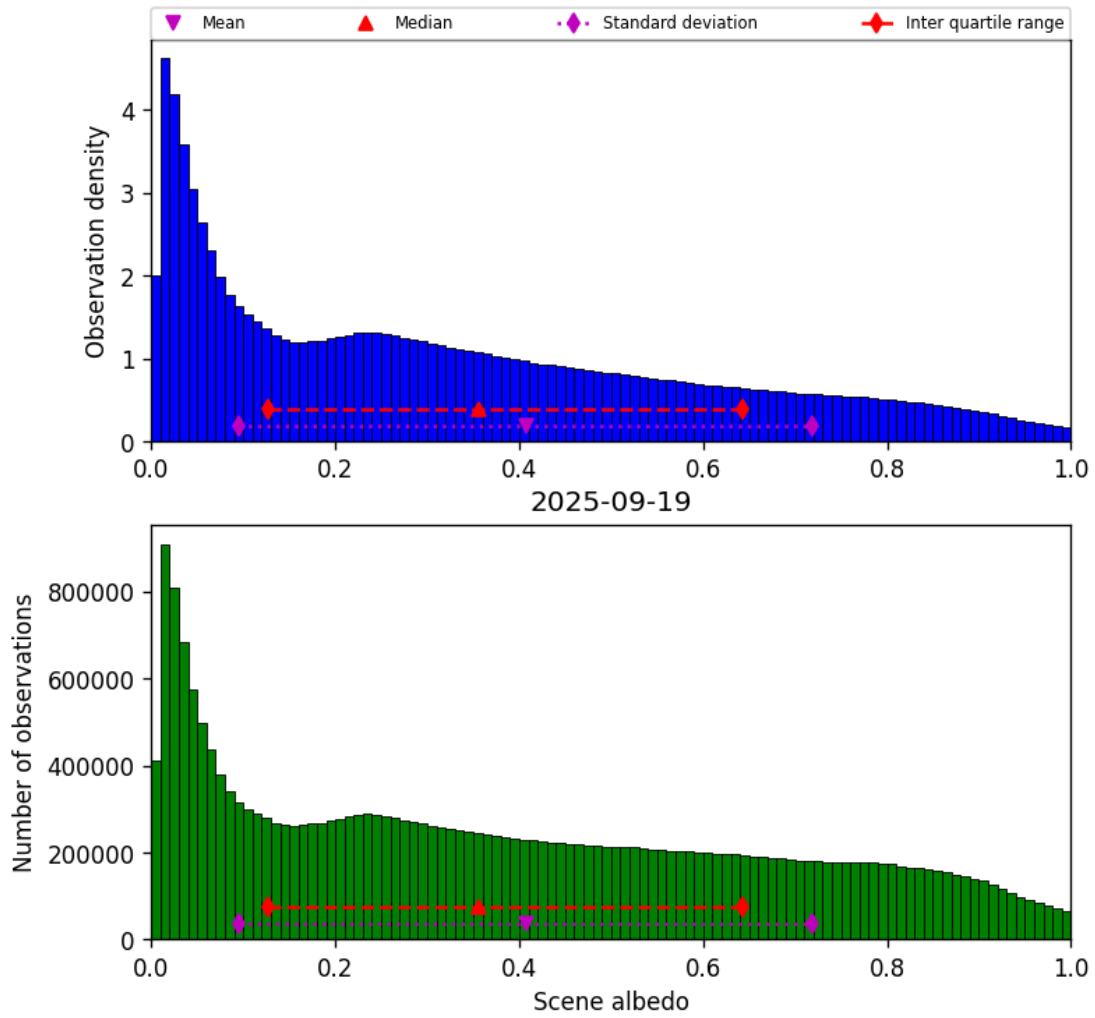
Figure 32: Histogram of “Scene albedo” for 2025-09-19 to 2025-09-20
