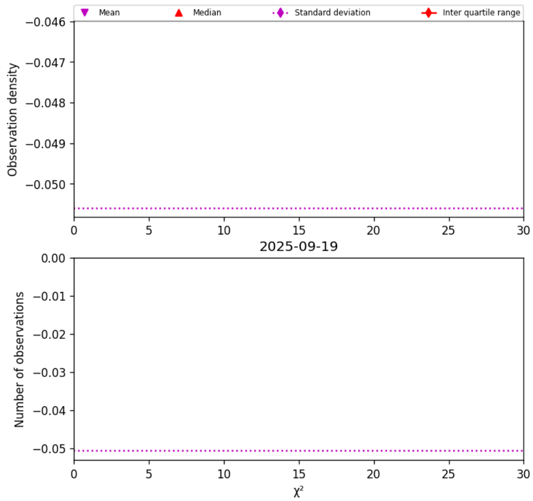
Figure 36: Histogram of " \chi^2 " for 2025-09-19 to 2025-09-20
