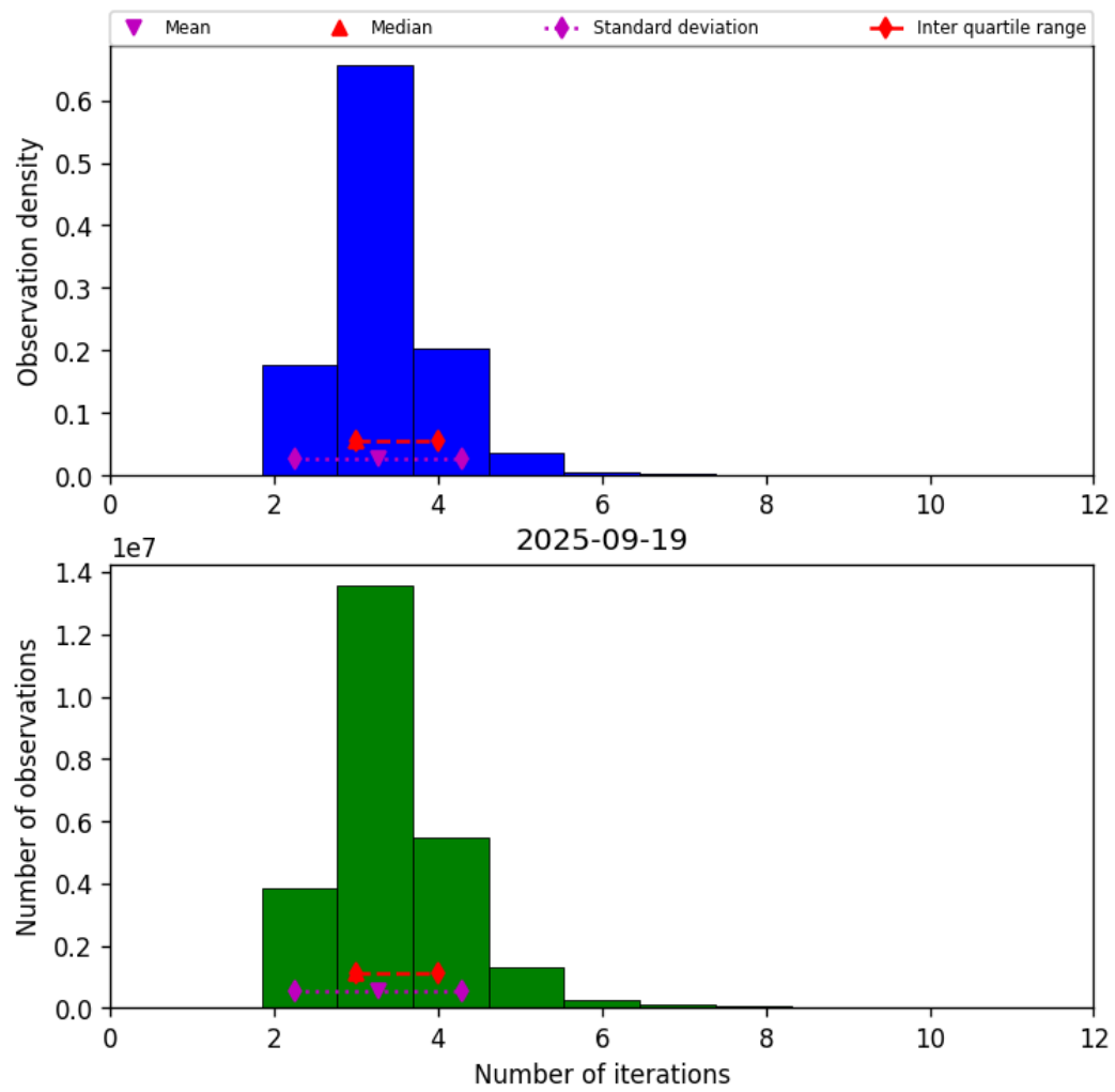
Figure 37: Histogram of “Number of iterations” for 2025-09-19 to 2025-09-20
