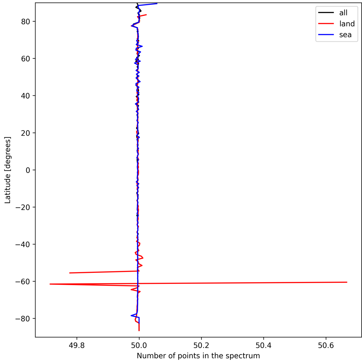
Figure 25: Zonal average of “Number of points in the spectrum” for 2025-09-19 to 2025-09-20.
