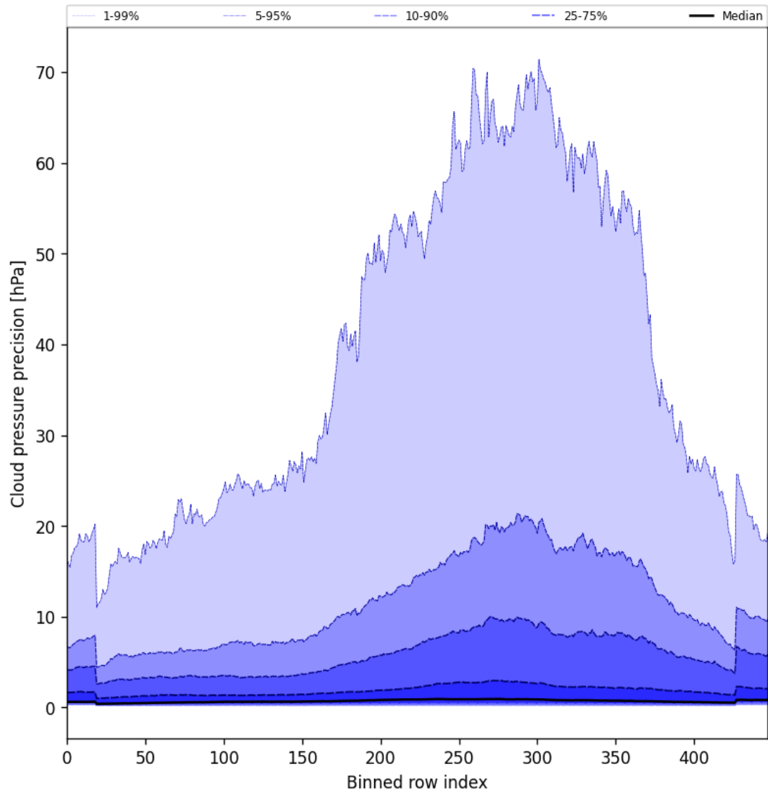
Figure 46: Along track statistics of “Cloud pressure precision” for 2025-09-19 to 2025-09-20
