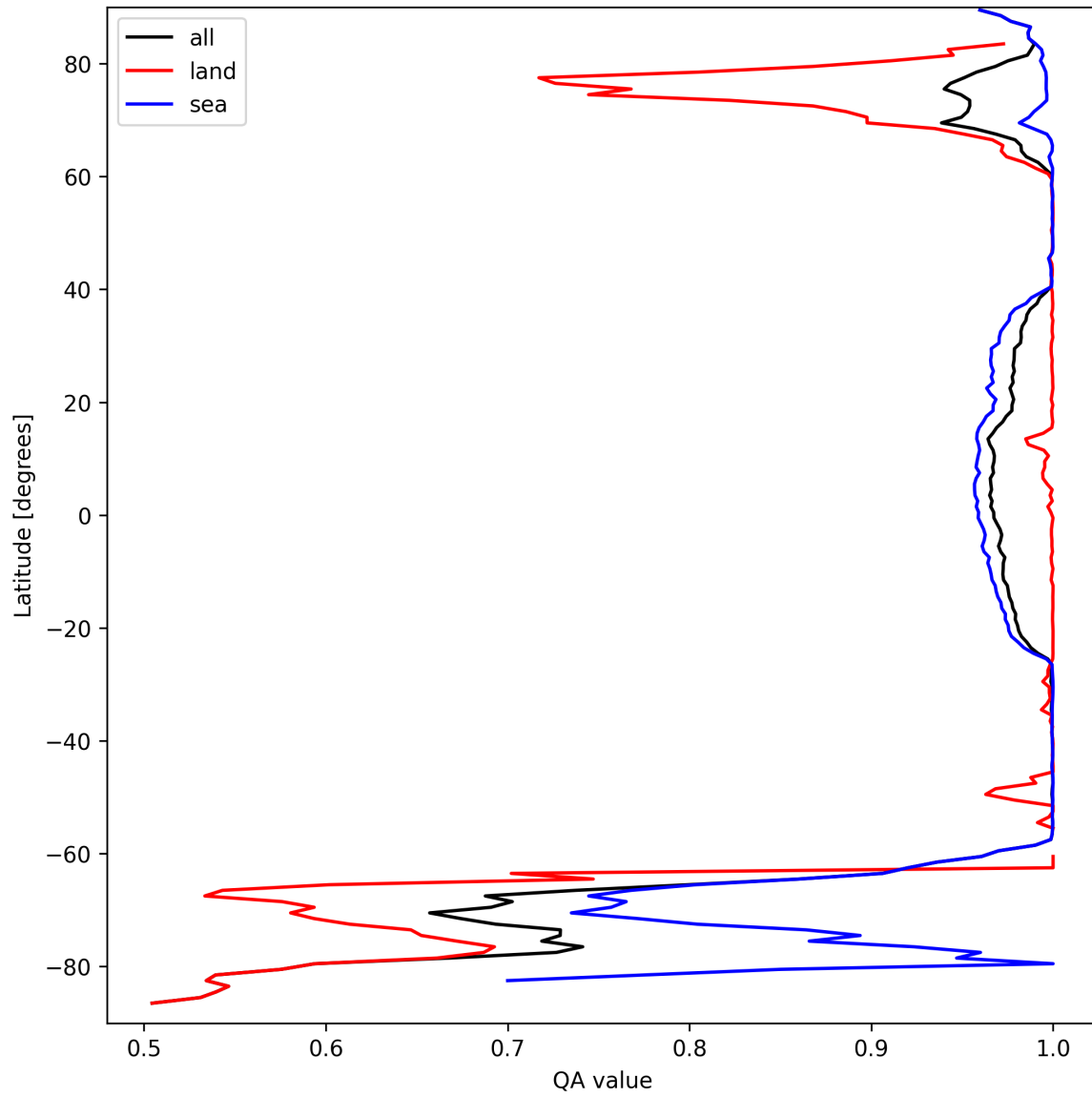
Figure 10: Zonal average of “QA value” for 2025-09-19 to 2025-09-20.
