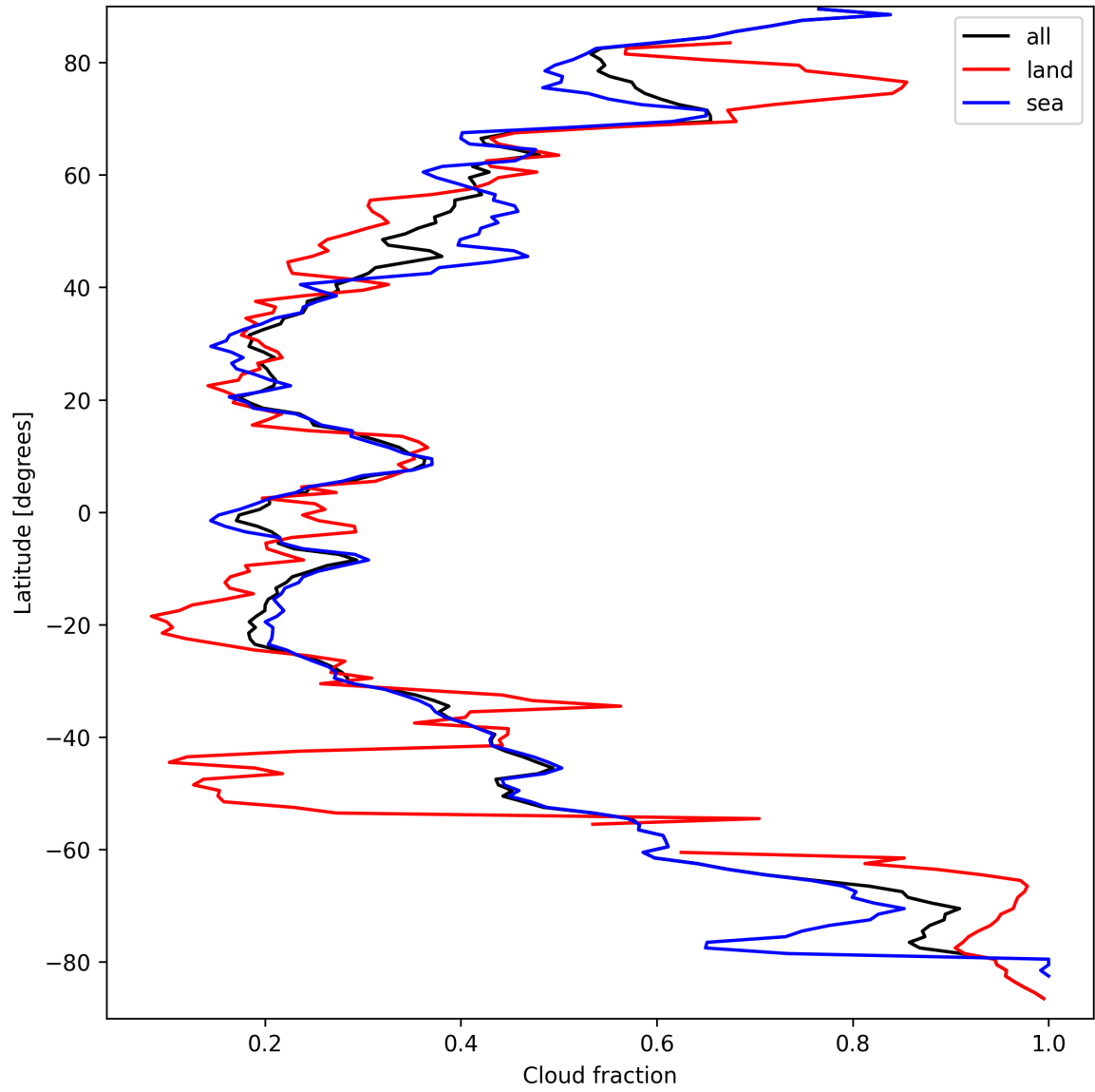
Figure 13: Zonal average of “Cloud fraction” for 2025-09-19 to 2025-09-20.
