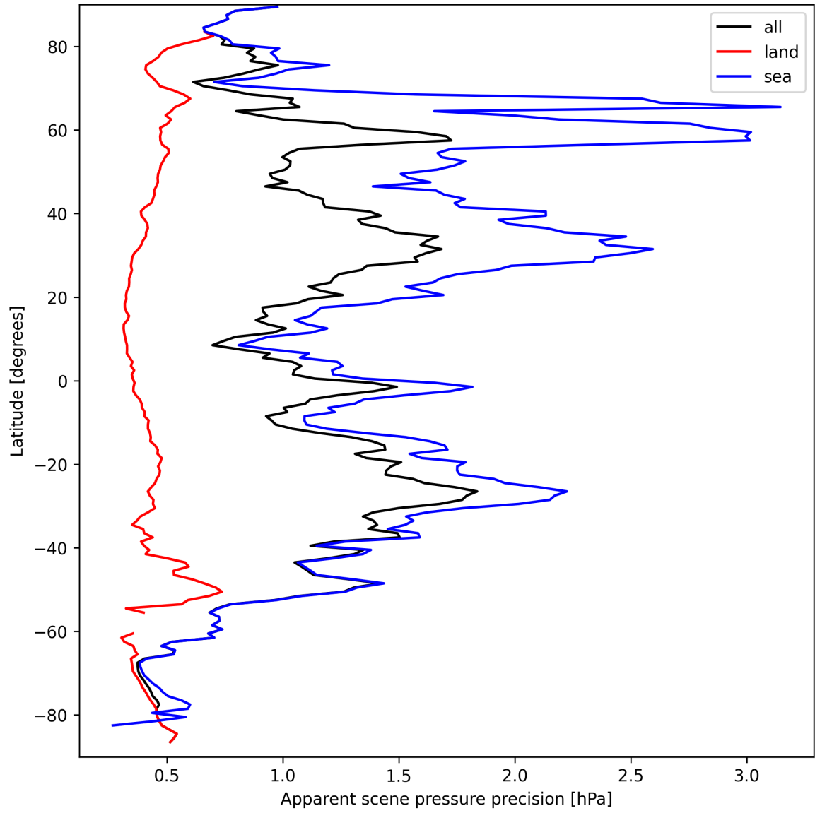
Figure 18: Zonal average of “Apparent scene pressure precision” for 2025-09-19 to 2025-09-20.
