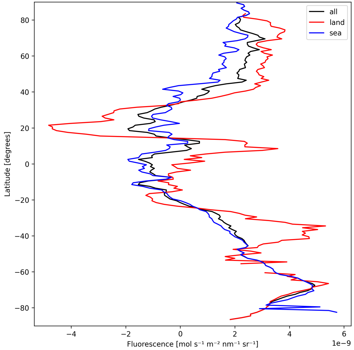
Figure 21: Zonal average of “Fluorescence” for 2025-09-19 to 2025-09-20.
