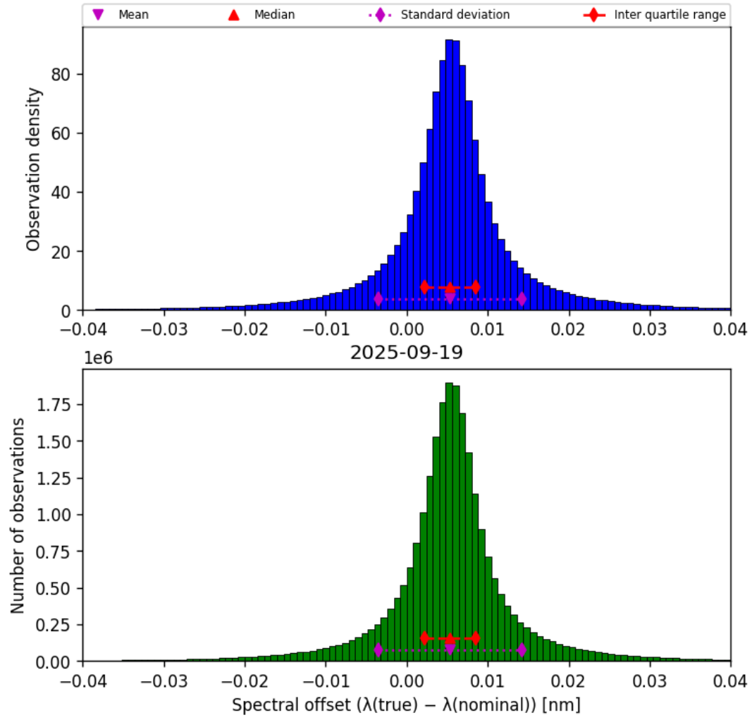
Figure 43: Histogram of “Spectral offset ( \lambda_{\text{true}} - \lambda_{\text{nominal}} )” for 2025-09-19 to 2025-09-20
