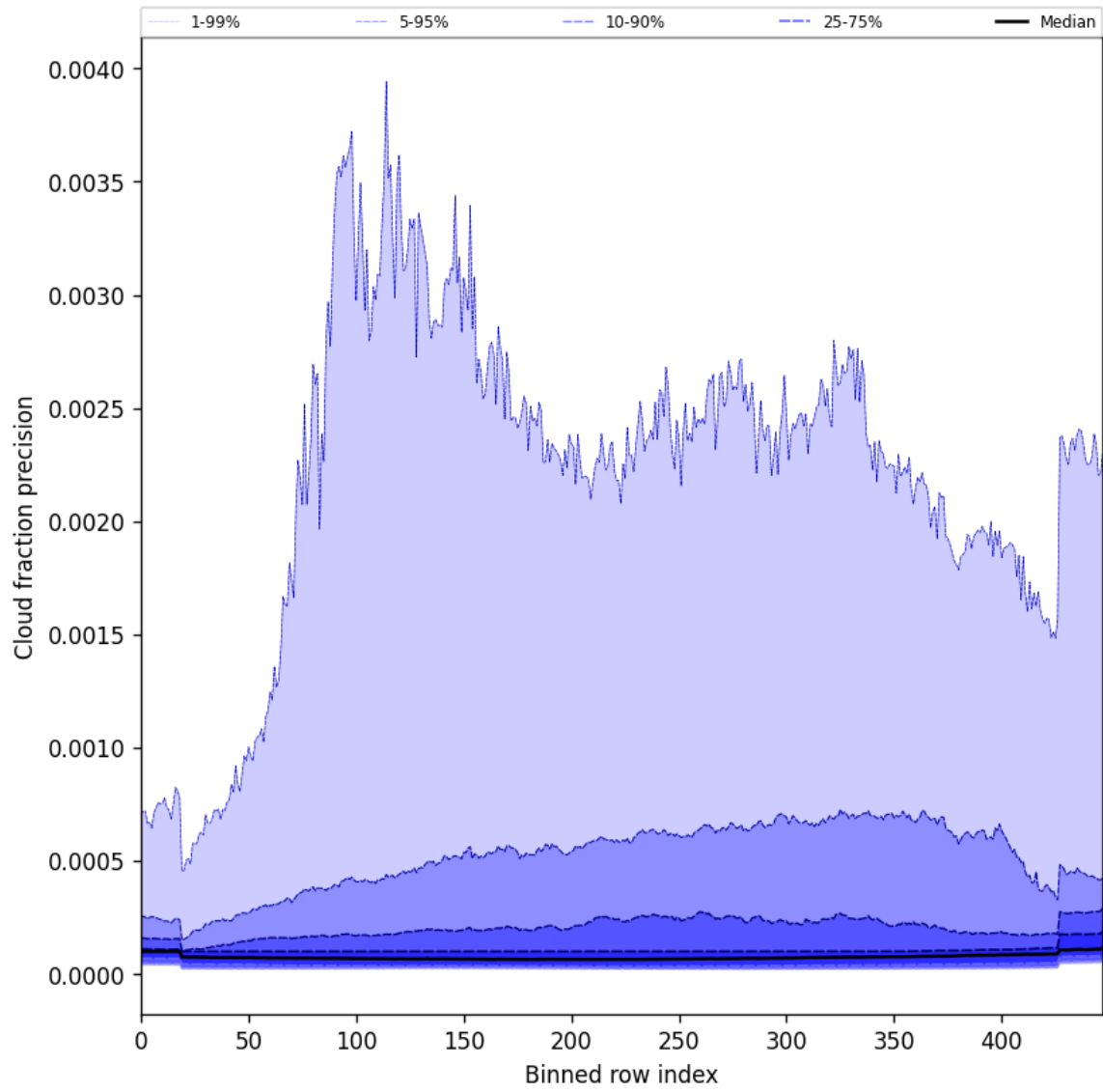
Figure 48: Along track statistics of “Cloud fraction precision” for 2025-09-19 to 2025-09-20
