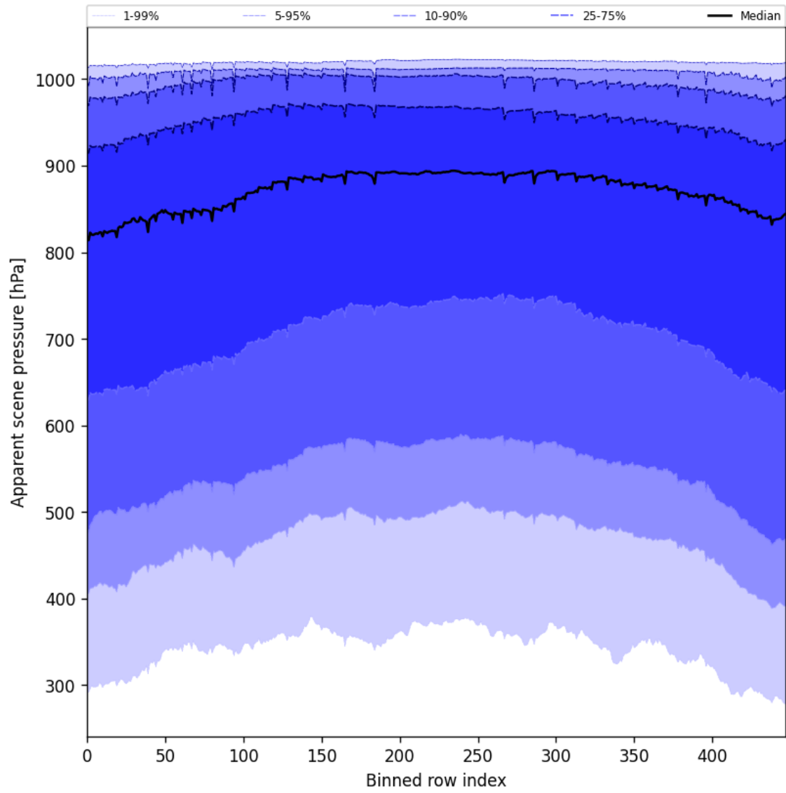
Figure 51: Along track statistics of “Apparent scene pressure” for 2025-09-19 to 2025-09-20
