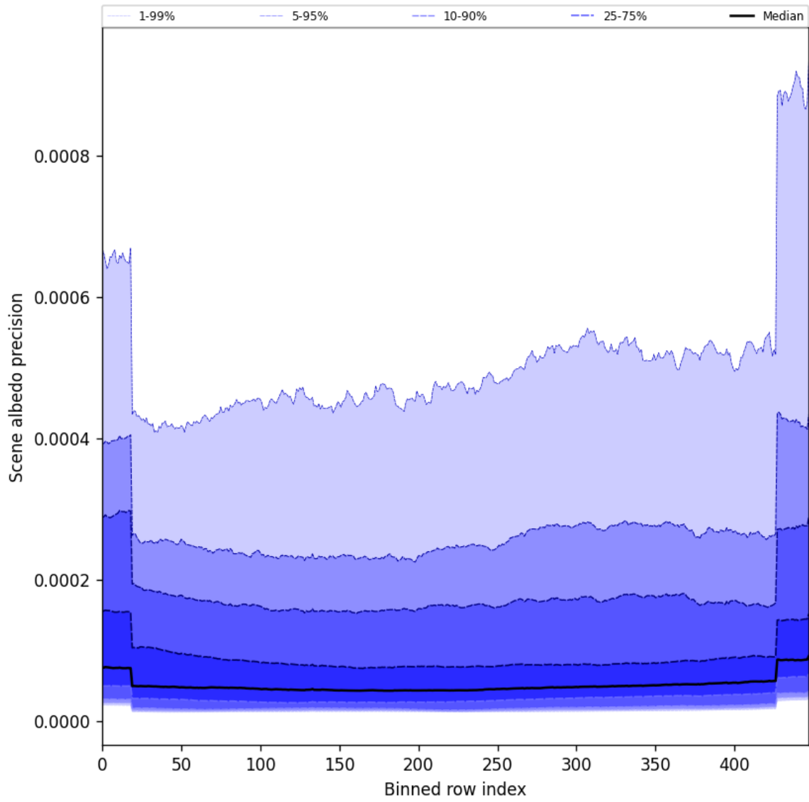
Figure 50: Along track statistics of “Scene albedo precision” for 2025-09-19 to 2025-09-20
