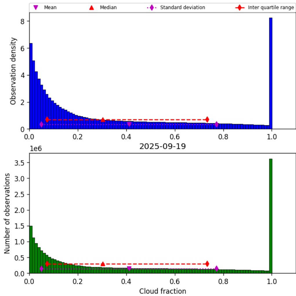
Figure 30: Histogram of “Cloud fraction” for 2025-09-19 to 2025-09-20
