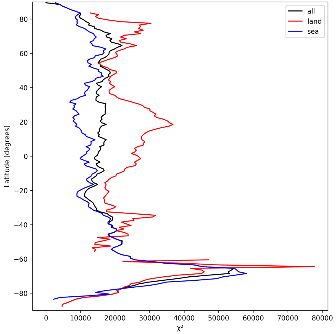
Figure 19: Zonal average of “ \chi^2 ” for 2025-09-20 to 2025-09-21.
