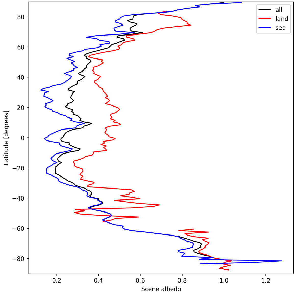
Figure 15: Zonal average of “Scene albedo” for 2025-09-20 to 2025-09-21.
