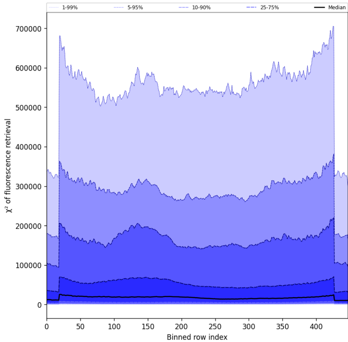
Figure 57: Along track statistics of “ \chi^2 of fluorescence retrieval” for 2025-09-20 to 2025-09-21
