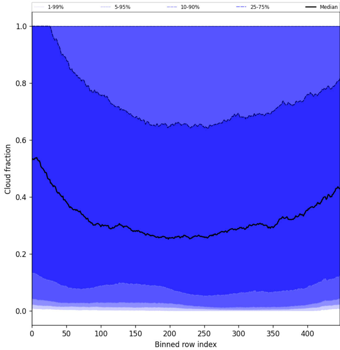
Figure 47: Along track statistics of “Cloud fraction” for 2025-09-20 to 2025-09-21
