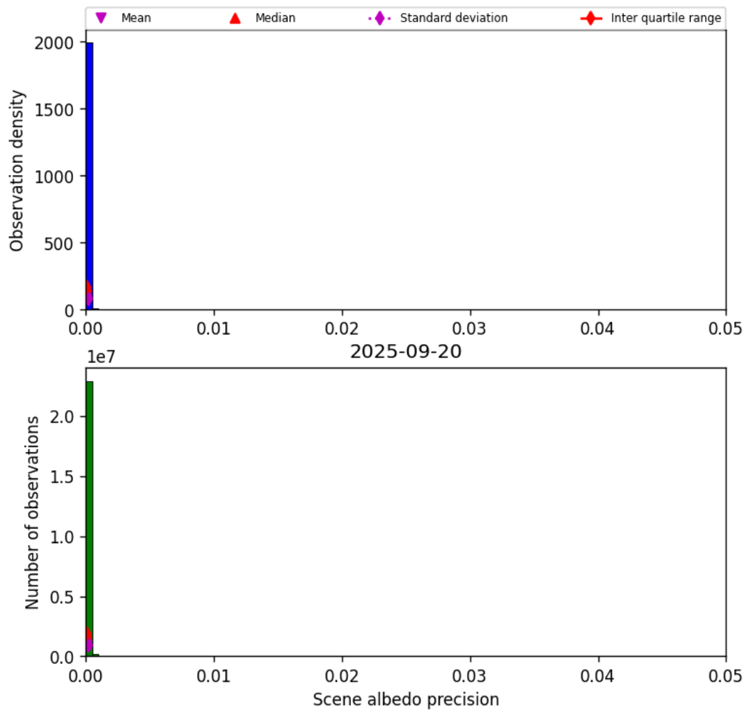
Figure 33: Histogram of “Scene albedo precision” for 2025-09-20 to 2025-09-21
