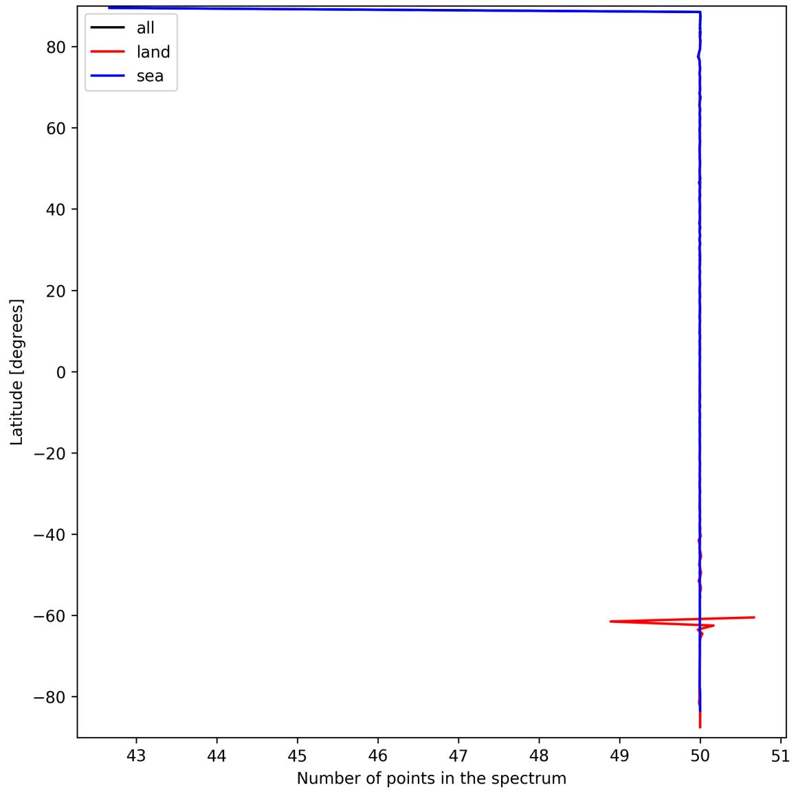
Figure 25: Zonal average of “Number of points in the spectrum” for 2025-09-20 to 2025-09-21.
