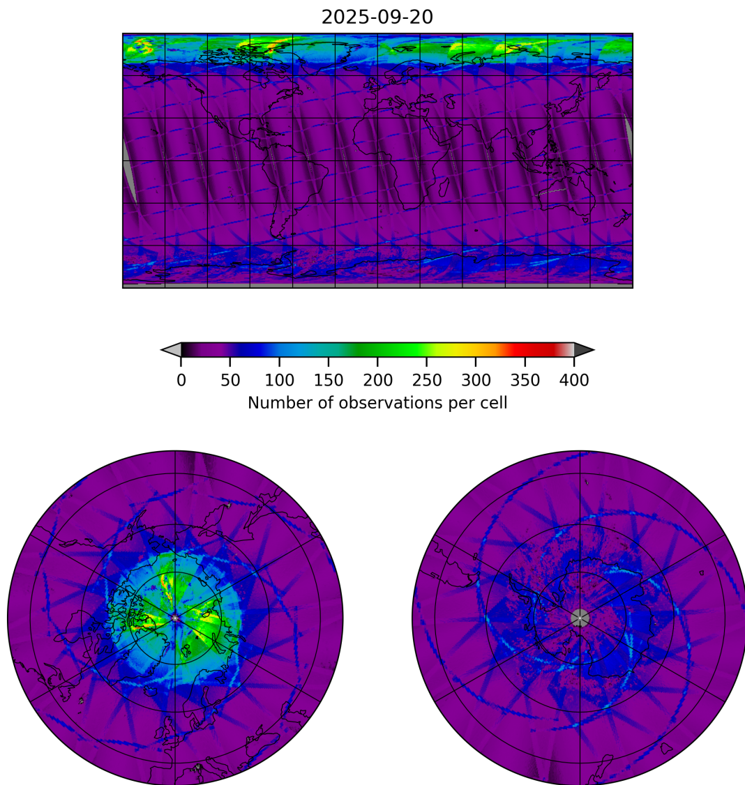
Figure 9: Map of the number of observations for 2025-09-20 to 2025-09-21
