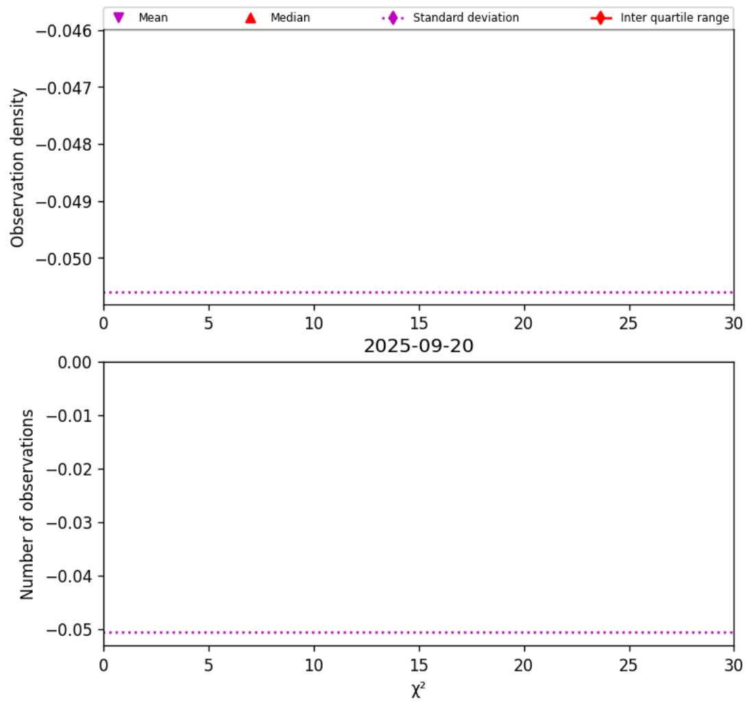
Figure 36: Histogram of " \chi^2 " for 2025-09-20 to 2025-09-21
