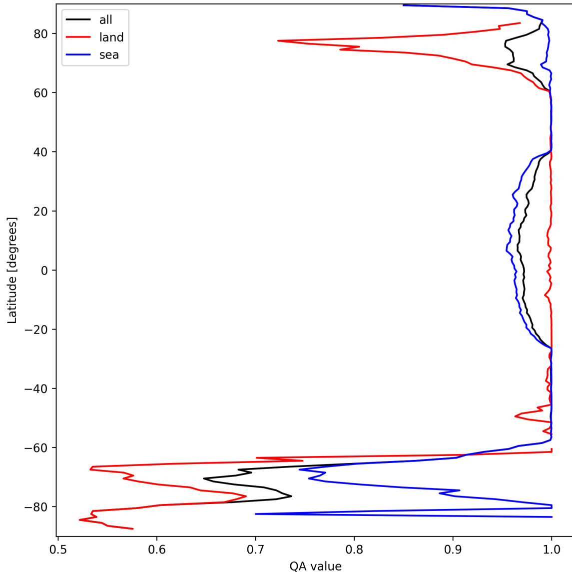
Figure 10: Zonal average of "QA value" for 2025-09-20 to 2025-09-21.
