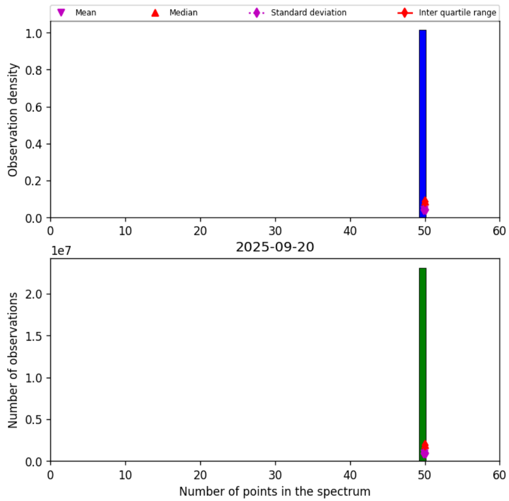
Figure 42: Histogram of “Number of points in the spectrum” for 2025-09-20 to 2025-09-21
