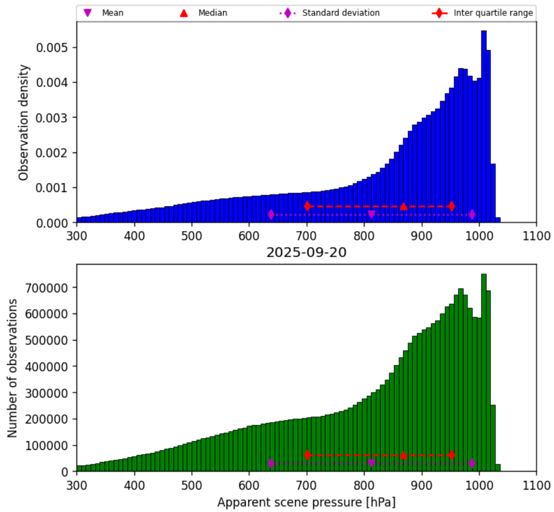
Figure 34: Histogram of “Apparent scene pressure” for 2025-09-20 to 2025-09-21
