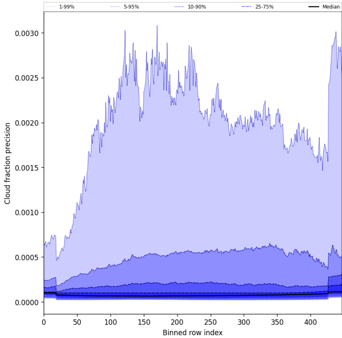
Figure 48: Along track statistics of “Cloud fraction precision” for 2025-09-20 to 2025-09-21
