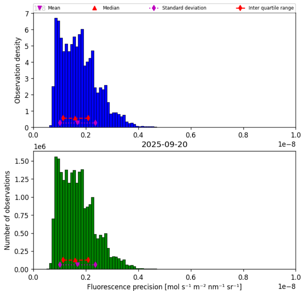
Figure 39: Histogram of “Fluorescence precision” for 2025-09-20 to 2025-09-21
