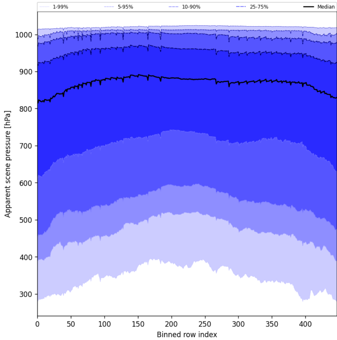
Figure 51: Along track statistics of “Apparent scene pressure” for 2025-09-20 to 2025-09-21
