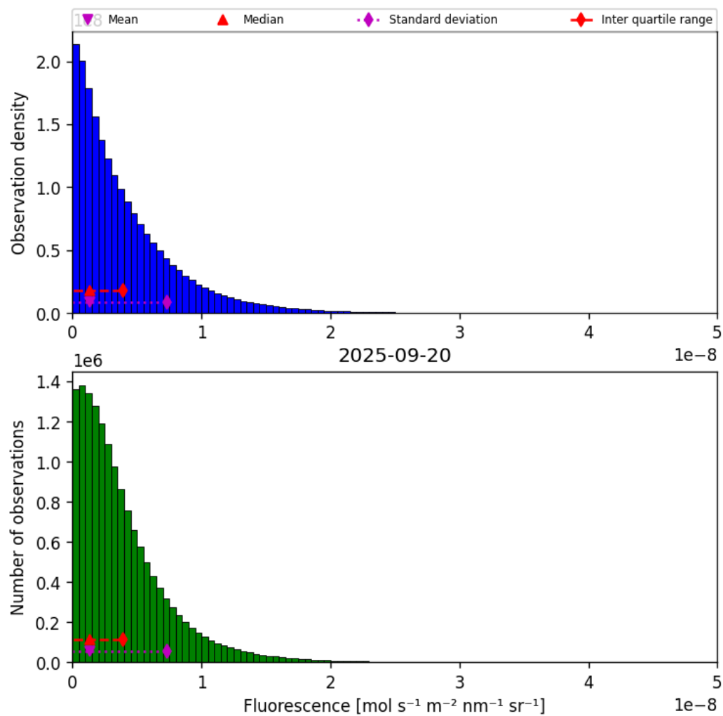
Figure 38: Histogram of “Fluorescence” for 2025-09-20 to 2025-09-21
