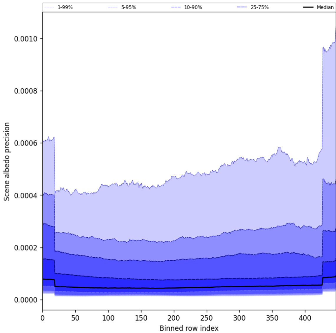
Figure 50: Along track statistics of “Scene albedo precision” for 2025-09-20 to 2025-09-21
