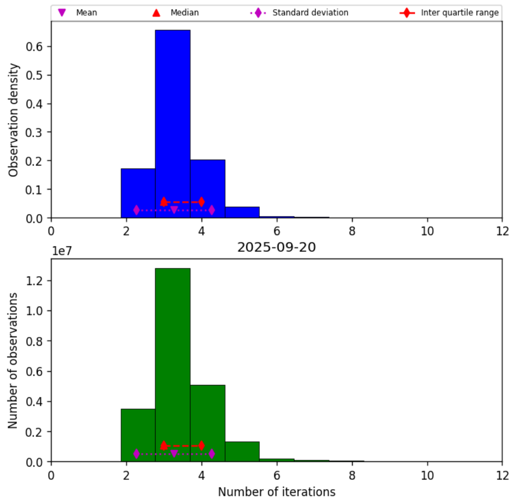
Figure 37: Histogram of “Number of iterations” for 2025-09-20 to 2025-09-21
