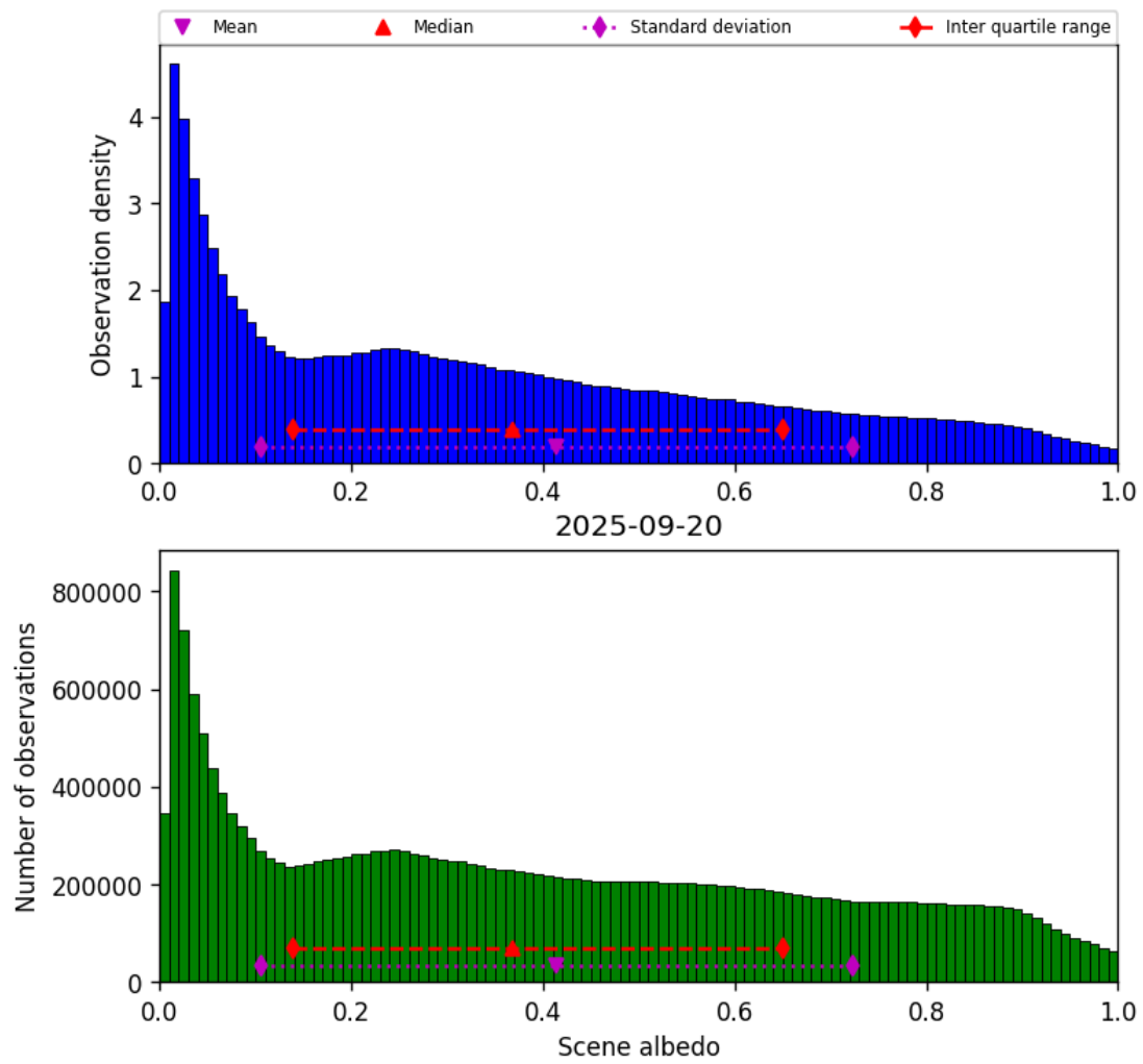
Figure 32: Histogram of “Scene albedo” for 2025-09-20 to 2025-09-21
