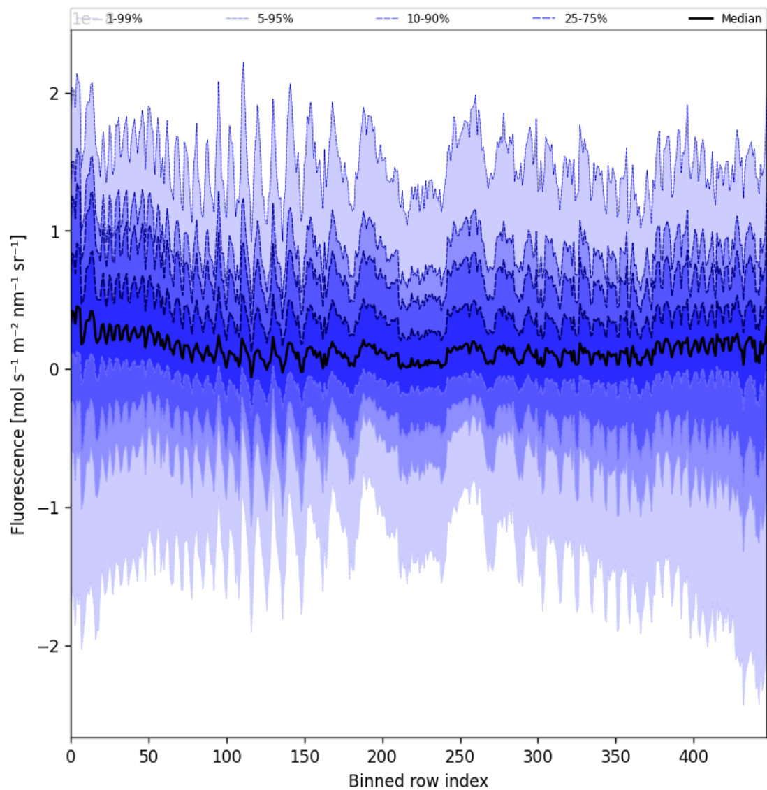
Figure 55: Along track statistics of “Fluorescence” for 2025-09-20 to 2025-09-21
