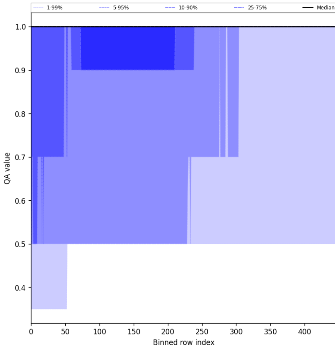
Figure 44: Along track statistics of “QA value” for 2025-09-20 to 2025-09-21
