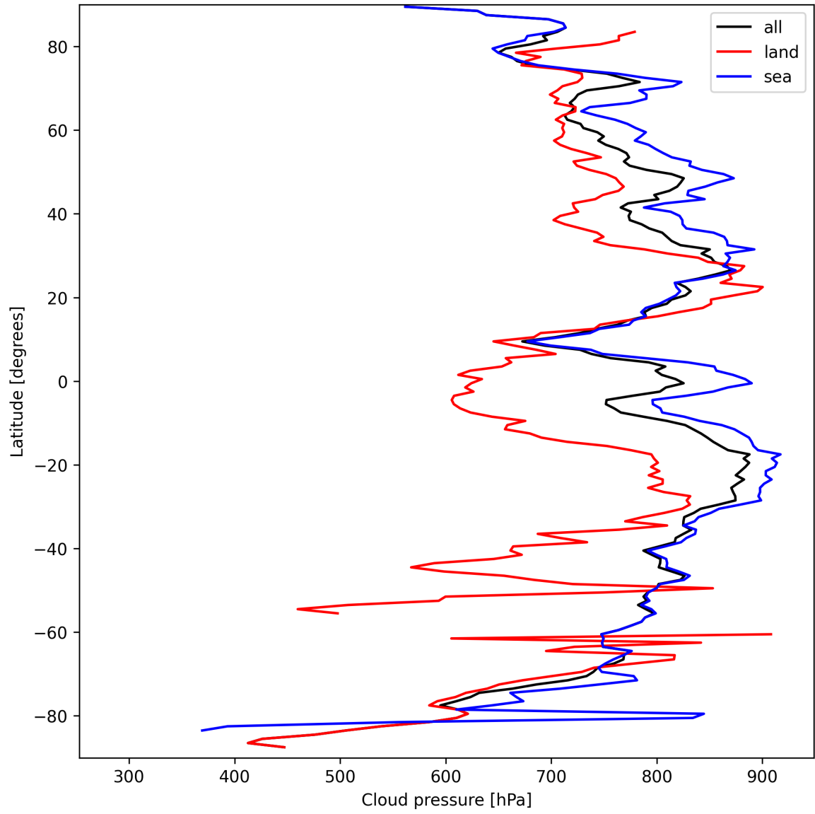
Figure 11: Zonal average of “Cloud pressure” for 2025-09-20 to 2025-09-21.
