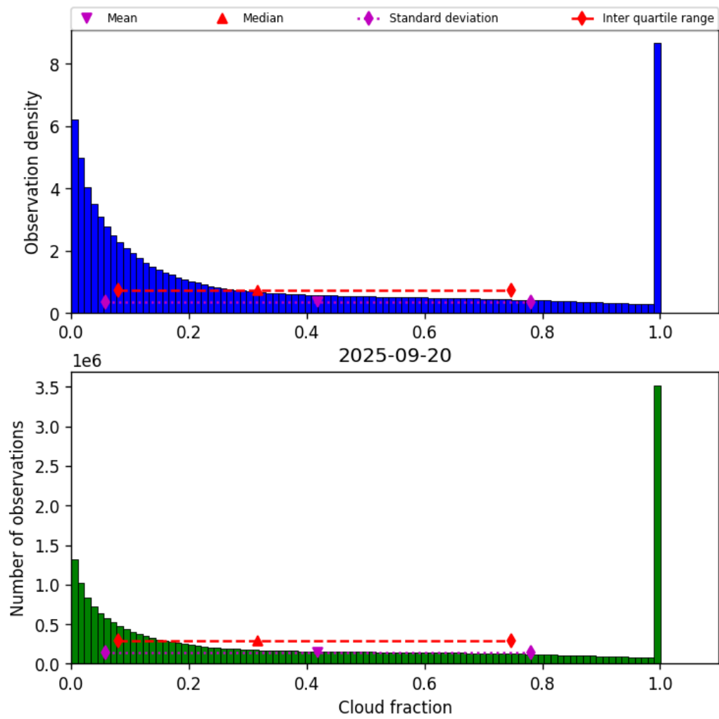
Figure 30: Histogram of “Cloud fraction” for 2025-09-20 to 2025-09-21
