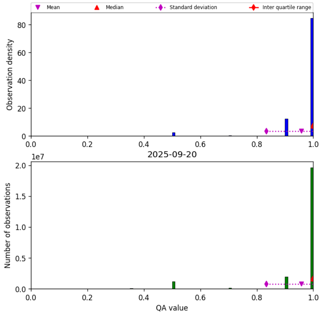
Figure 27: Histogram of “QA value” for 2025-09-20 to 2025-09-21
