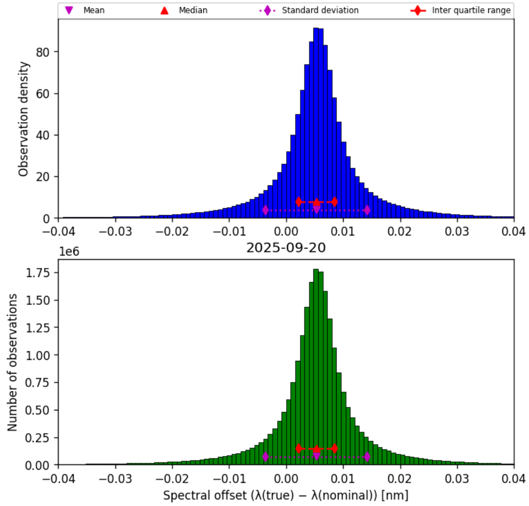
Figure 43: Histogram of “Spectral offset ( \lambda_{\text{true}} - \lambda_{\text{nominal}} )” for 2025-09-20 to 2025-09-21
