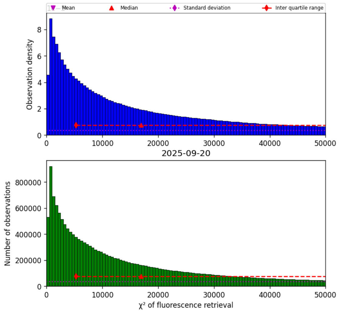
Figure 40: Histogram of “ \chi^2 of fluorescence retrieval” for 2025-09-20 to 2025-09-21
