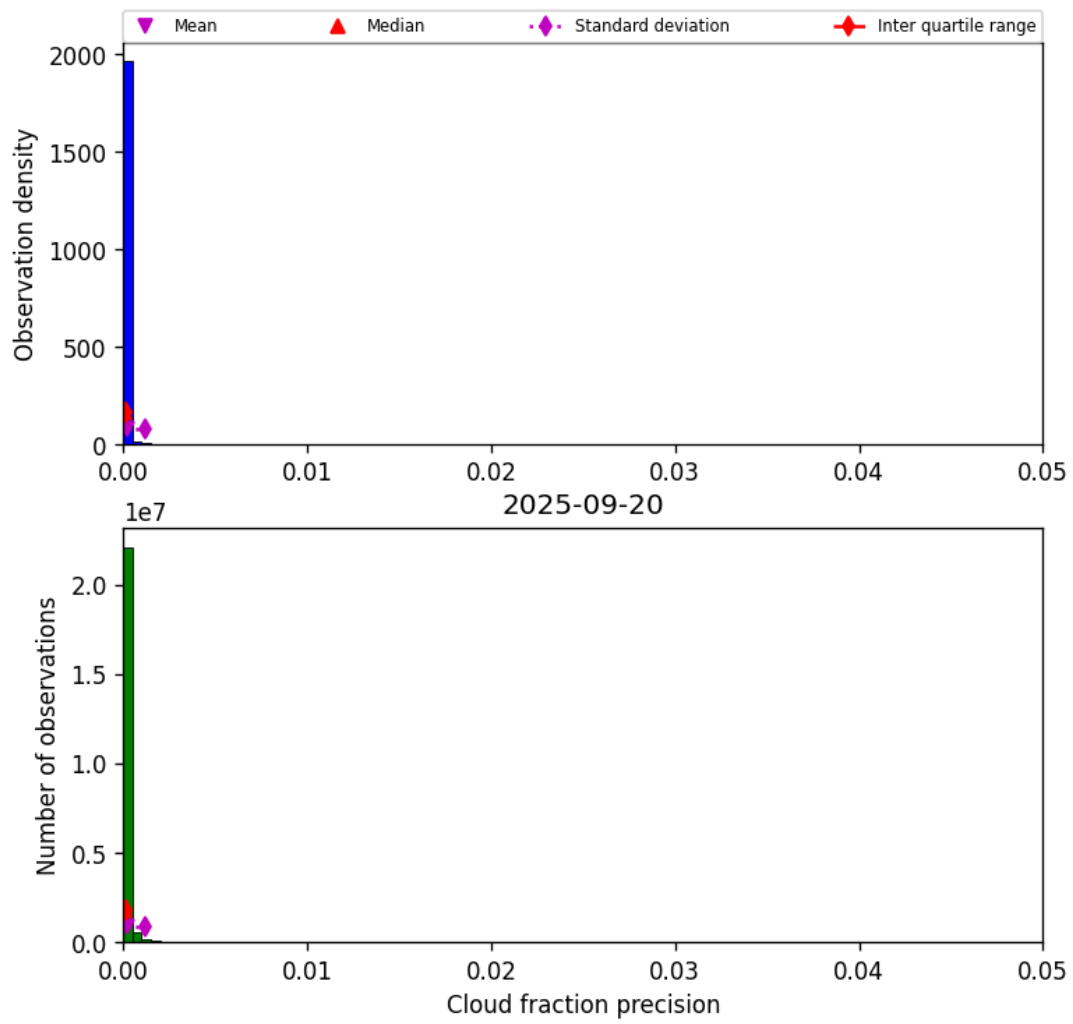
Figure 31: Histogram of “Cloud fraction precision” for 2025-09-20 to 2025-09-21
