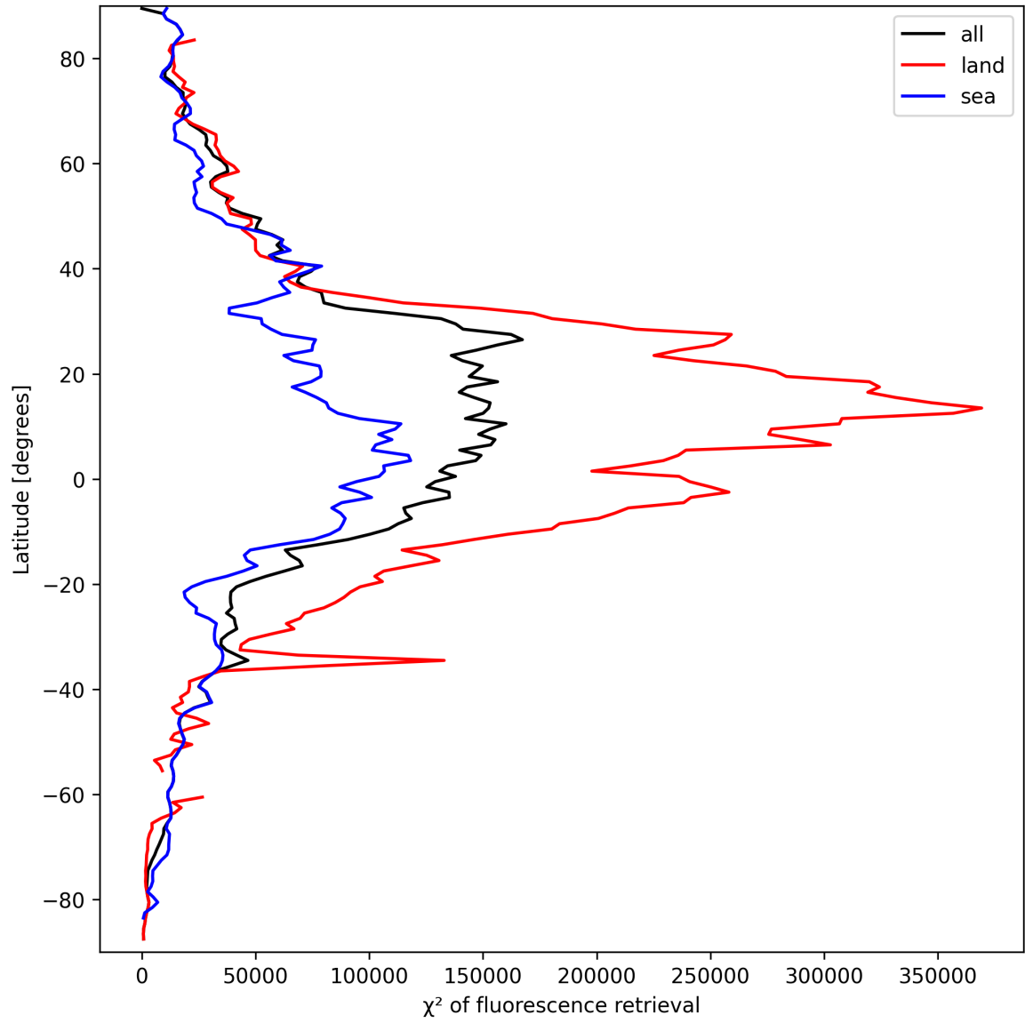
Figure 23: Zonal average of “ \chi^2 of fluorescence retrieval” for 2025-09-20 to 2025-09-21.
