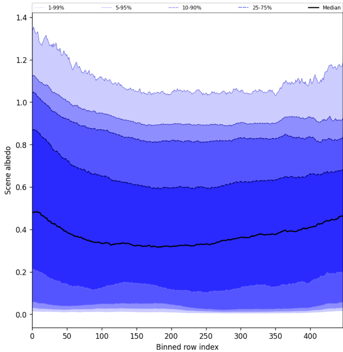
Figure 49: Along track statistics of “Scene albedo” for 2025-09-20 to 2025-09-21
