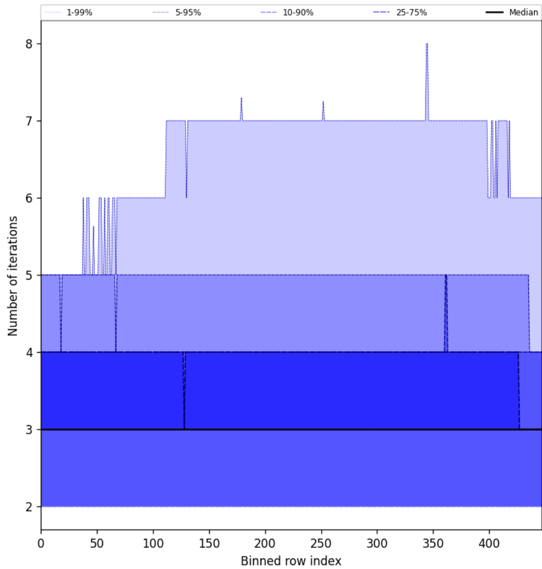
Figure 54: Along track statistics of “Number of iterations” for 2025-09-20 to 2025-09-21
