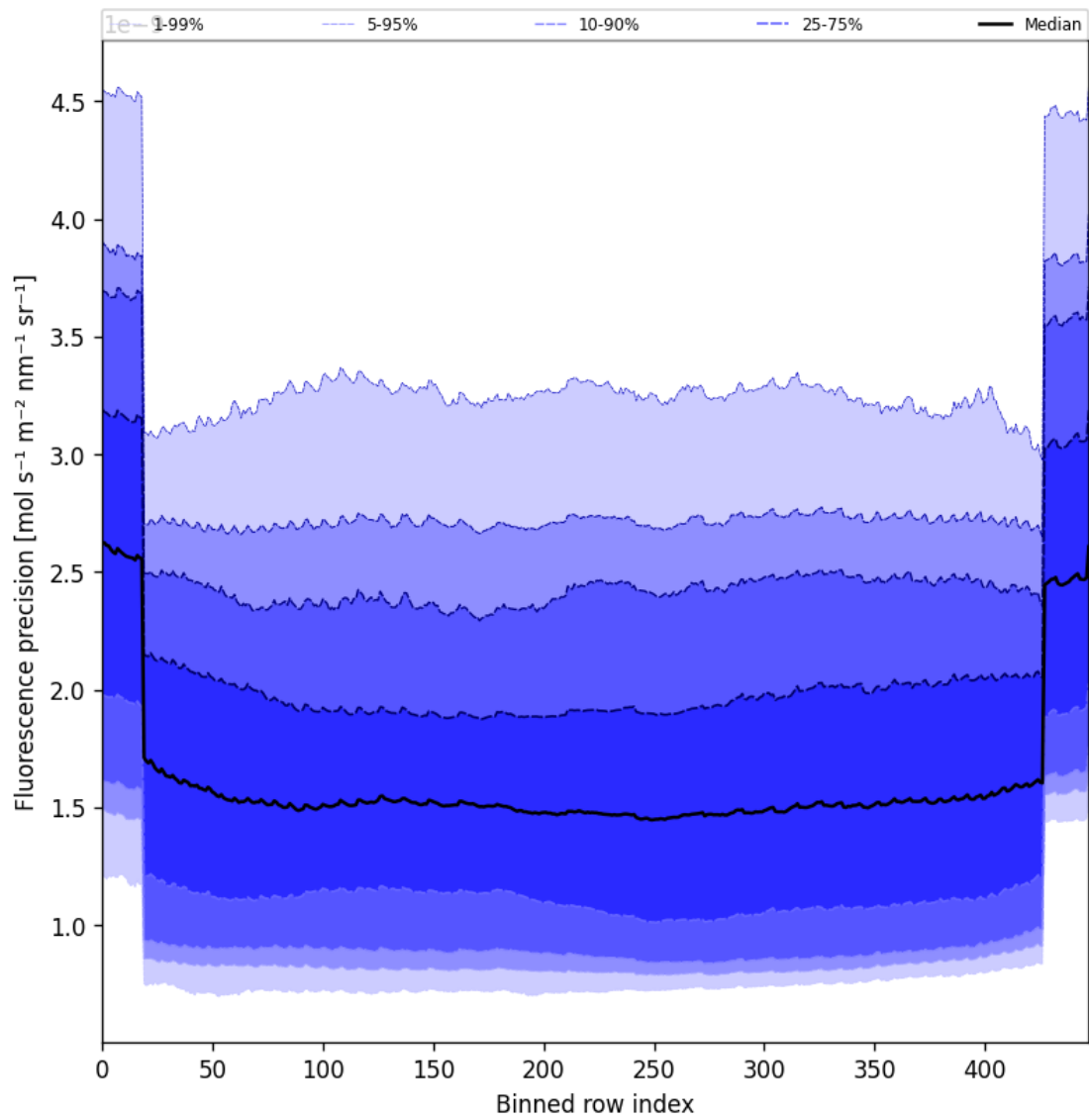
Figure 56: Along track statistics of “Fluorescence precision” for 2025-09-20 to 2025-09-21
