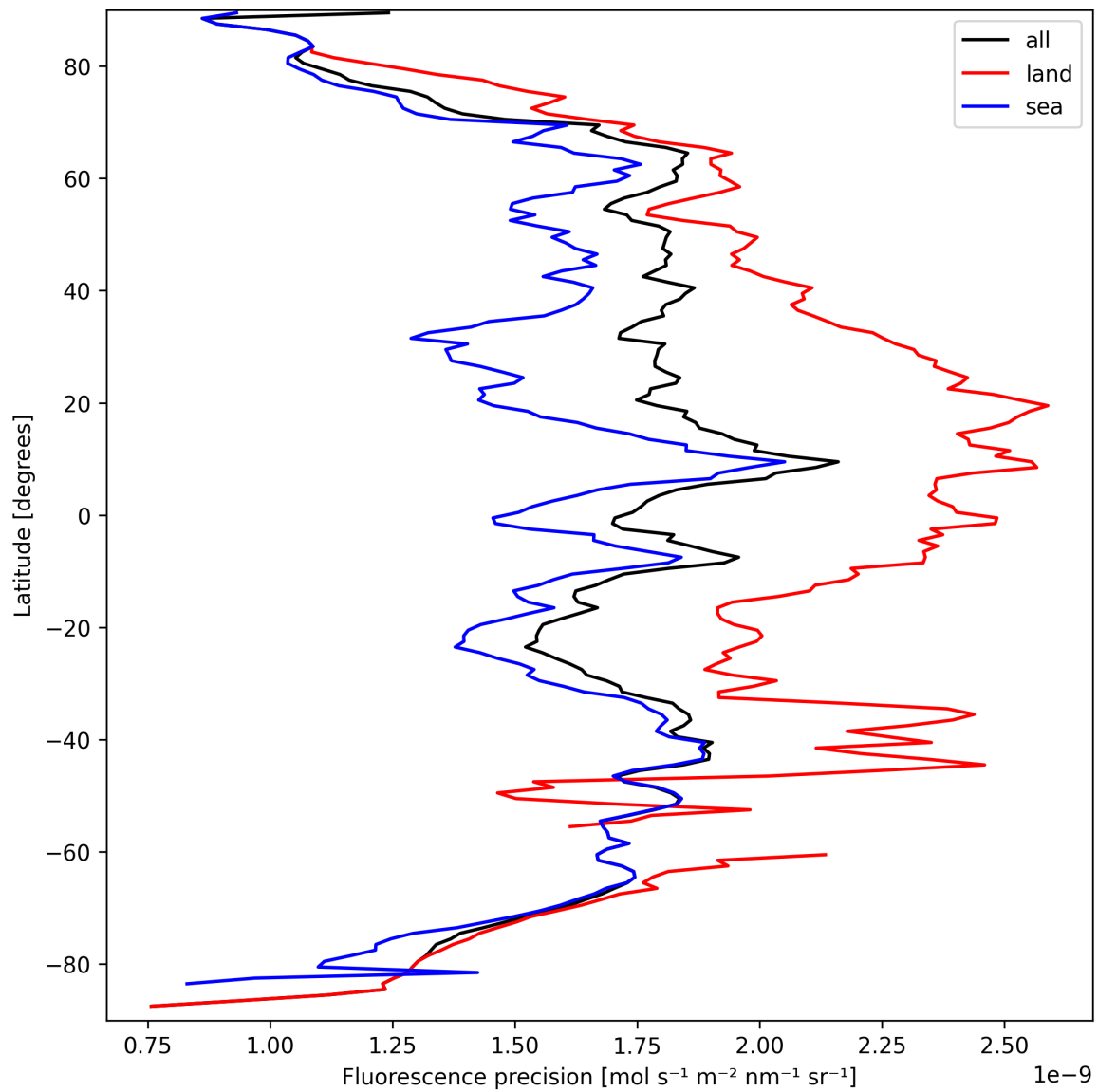
Figure 22: Zonal average of “Fluorescence precision” for 2025-09-20 to 2025-09-21.
