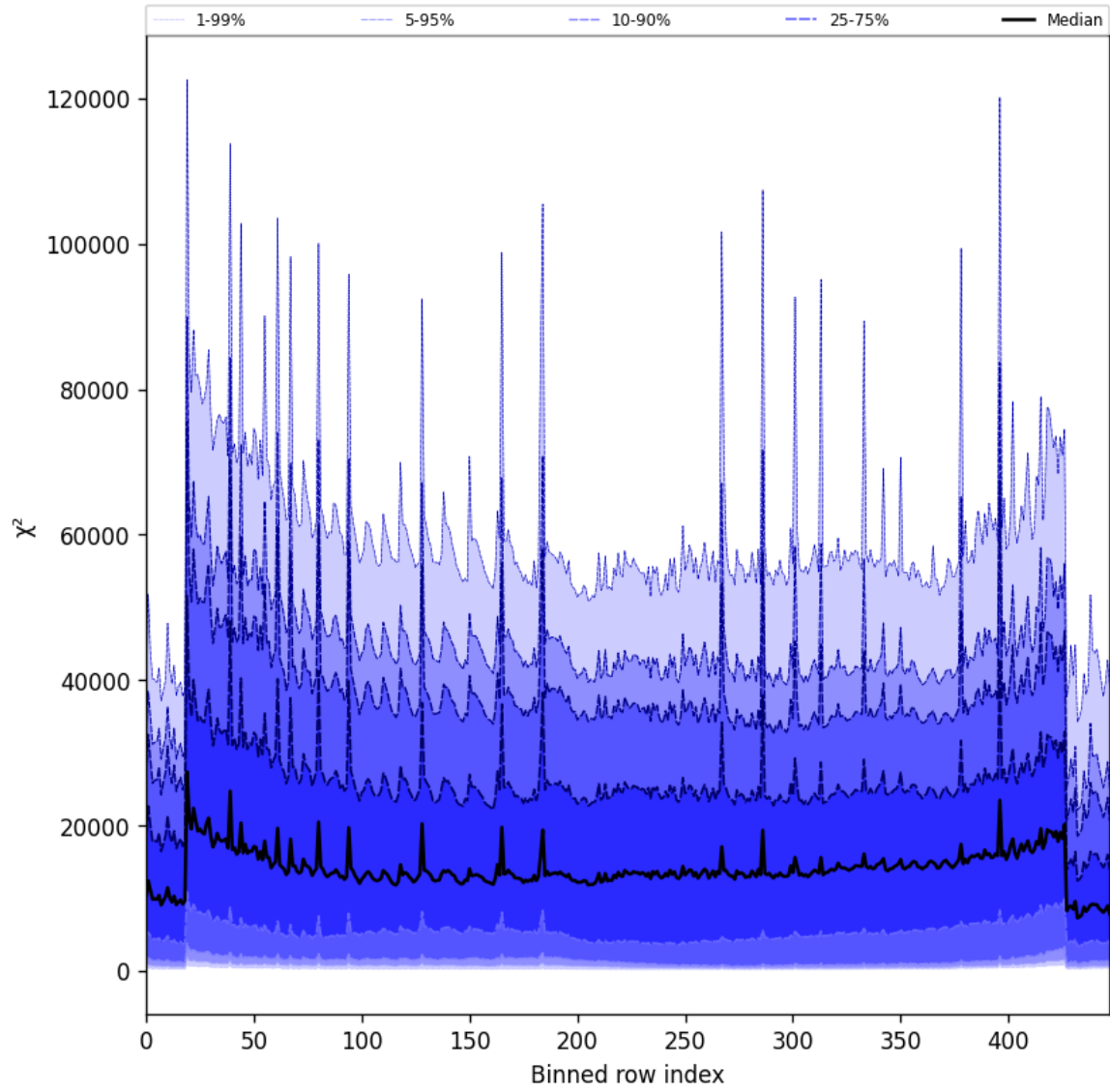
Figure 53: Along track statistics of “ \chi^2 ” for 2025-09-20 to 2025-09-21
