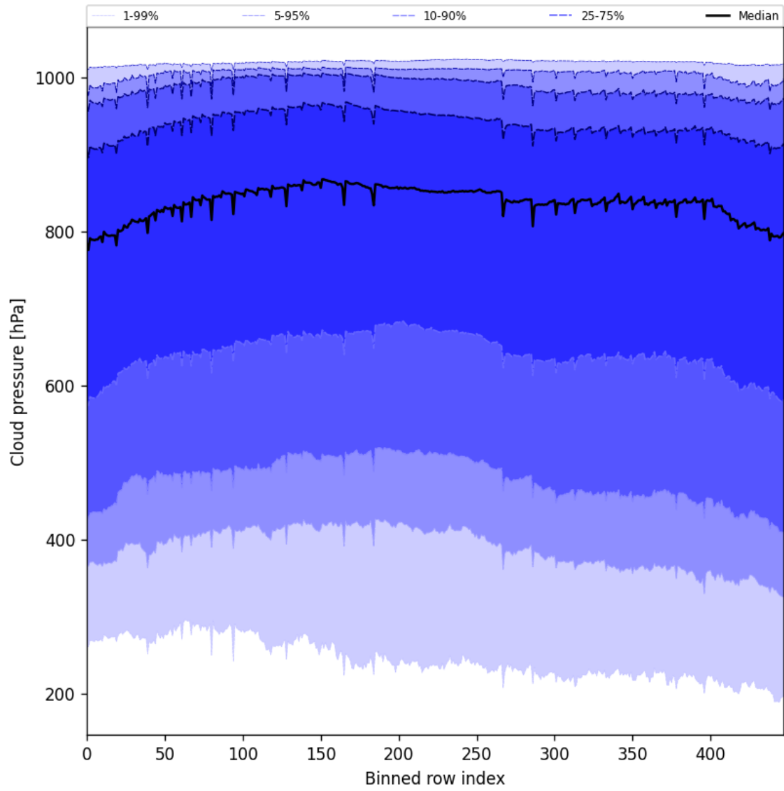
Figure 45: Along track statistics of “Cloud pressure” for 2025-09-20 to 2025-09-21
