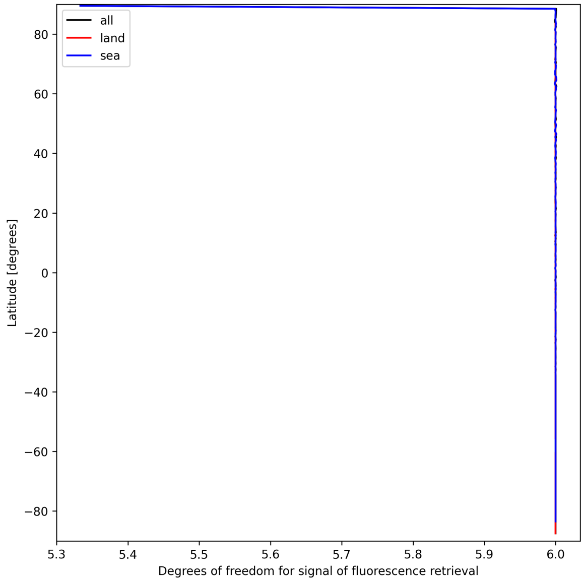
Figure 24: Zonal average of “Degrees of freedom for signal of fluorescence retrieval” for 2025-09-20 to 2025-09-21.
