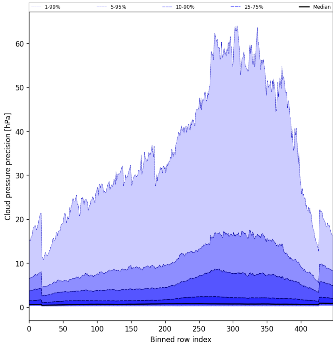
Figure 46: Along track statistics of “Cloud pressure precision” for 2025-09-20 to 2025-09-21
