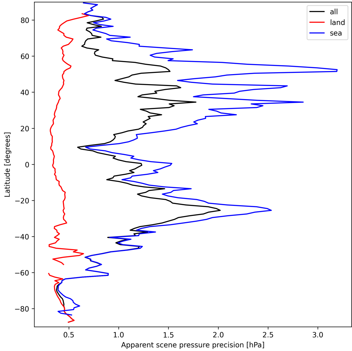
Figure 18: Zonal average of “Apparent scene pressure precision” for 2025-09-20 to 2025-09-21.
