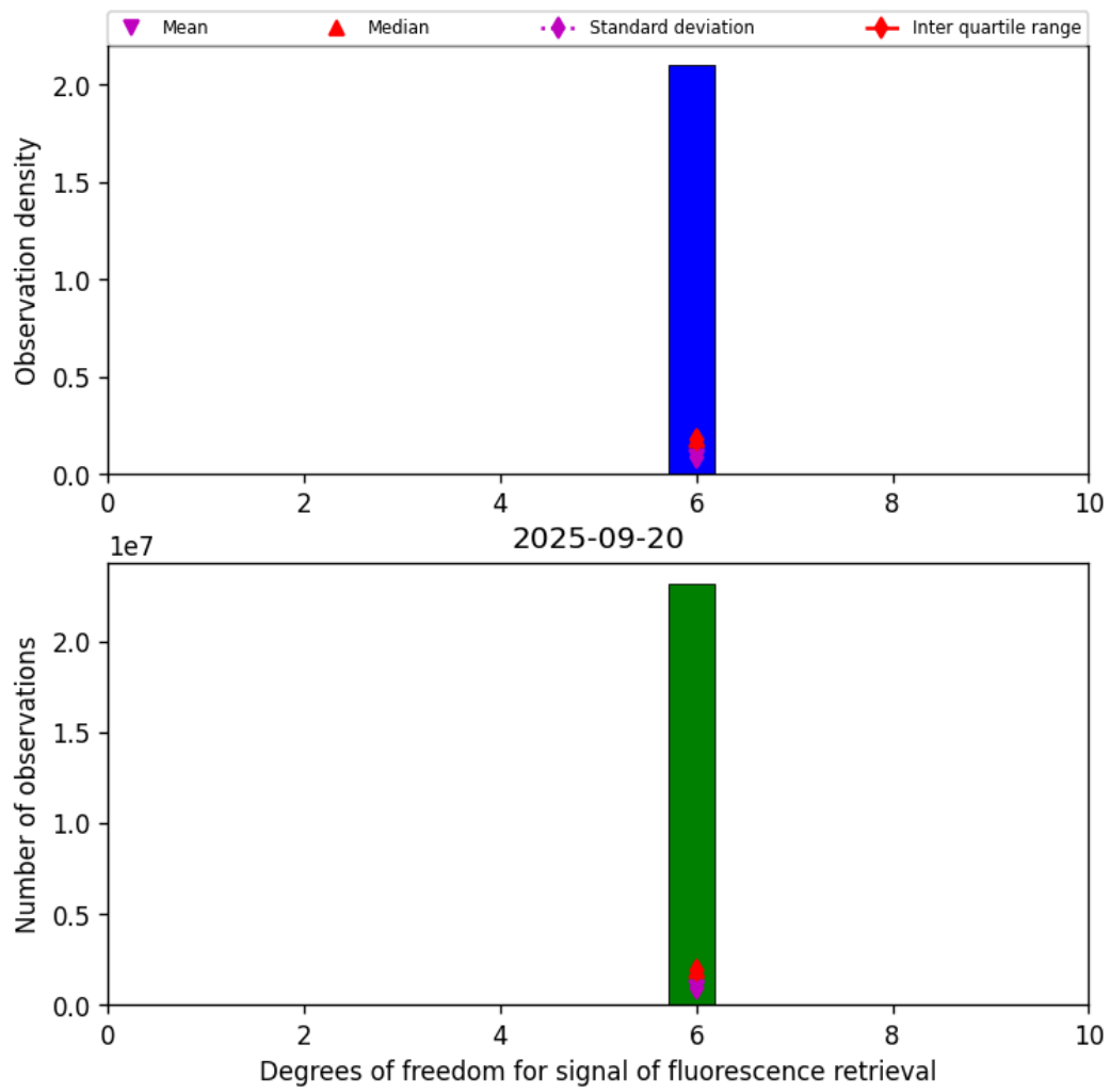
Figure 41: Histogram of “Degrees of freedom for signal of fluorescence retrieval” for 2025-09-20 to 2025-09-21
