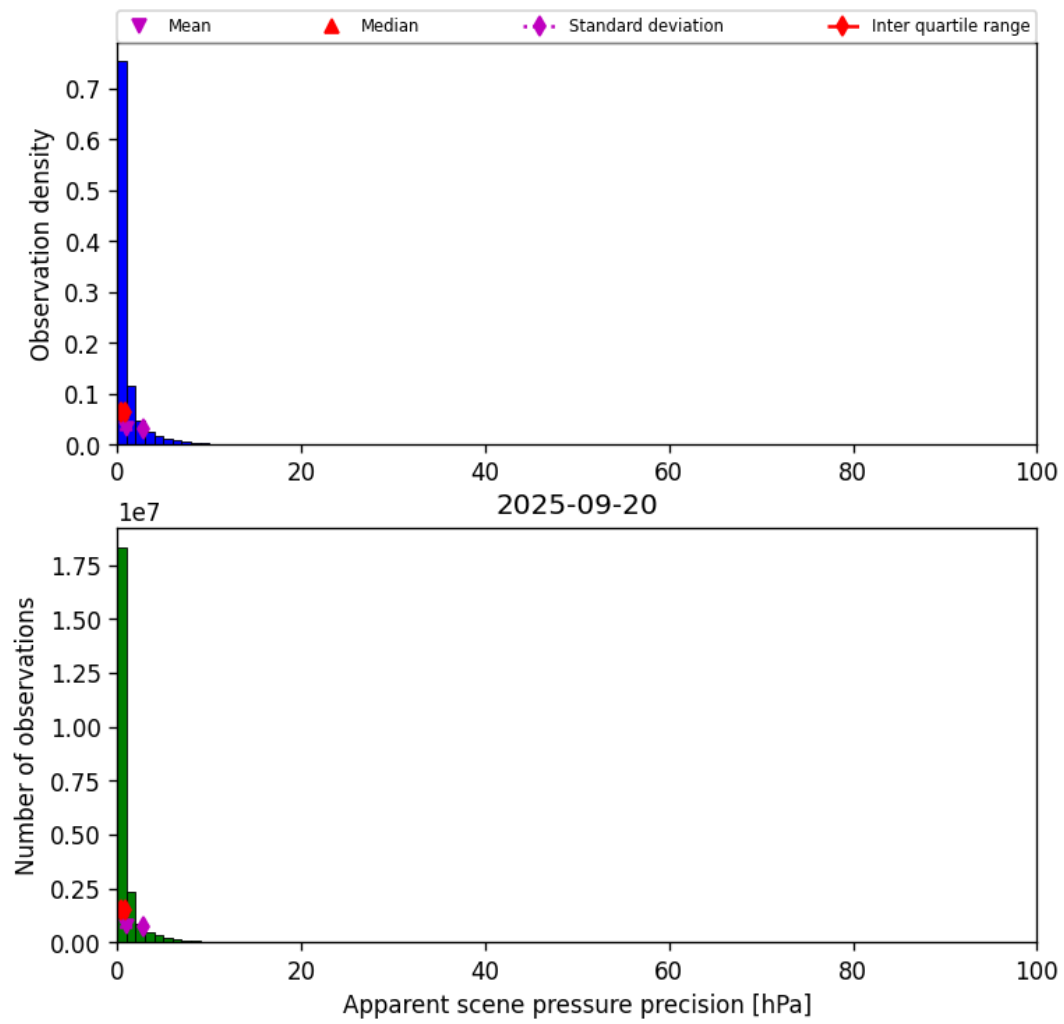
Figure 35: Histogram of “Apparent scene pressure precision” for 2025-09-20 to 2025-09-21
