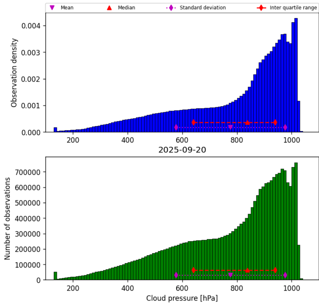
Figure 28: Histogram of “Cloud pressure” for 2025-09-20 to 2025-09-21
