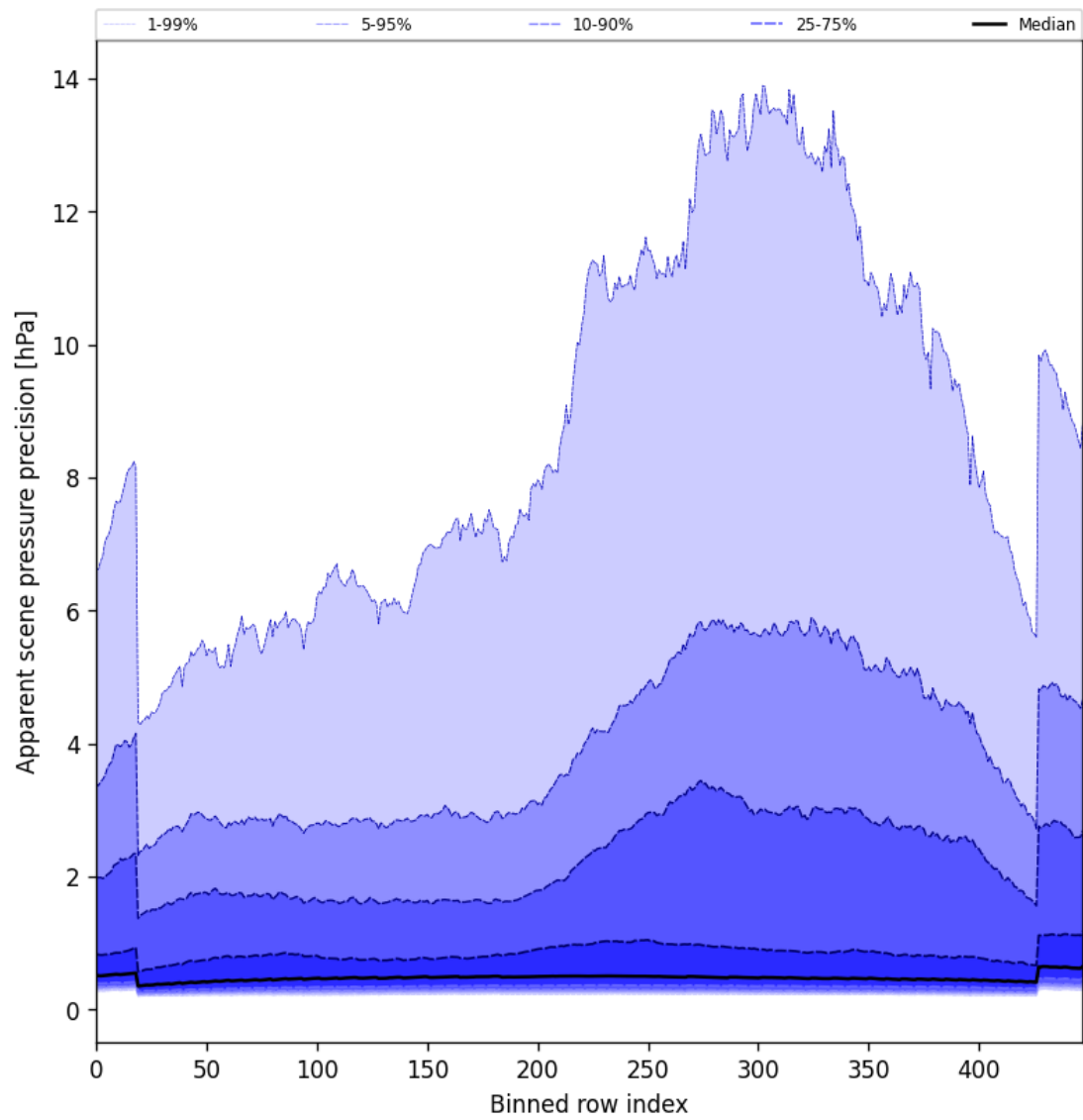
Figure 52: Along track statistics of “Apparent scene pressure precision” for 2025-09-20 to 2025-09-21
