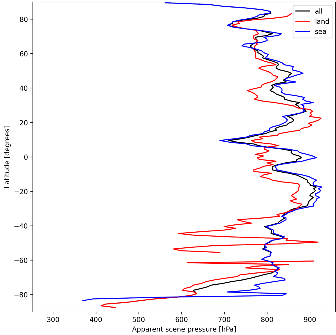
Figure 17: Zonal average of “Apparent scene pressure” for 2025-09-20 to 2025-09-21.
