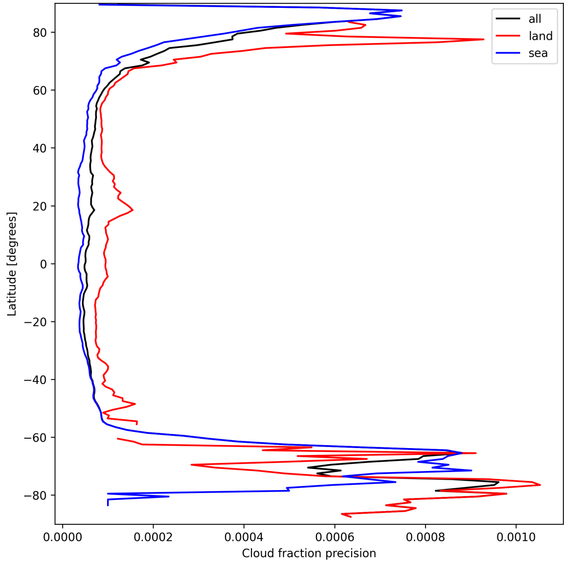
Figure 14: Zonal average of “Cloud fraction precision” for 2025-09-20 to 2025-09-21.
