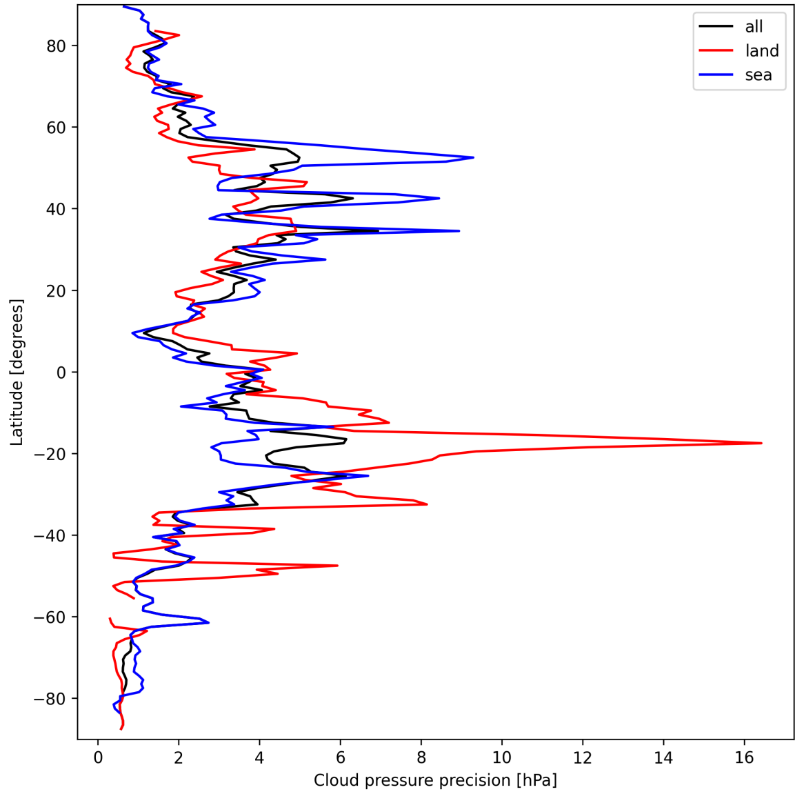
Figure 12: Zonal average of “Cloud pressure precision” for 2025-09-20 to 2025-09-21.
