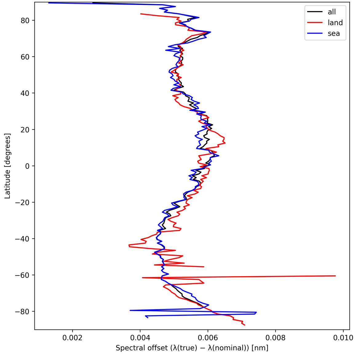
Figure 26: Zonal average of “Spectral offset ( \lambda_{\text{true}} - \lambda_{\text{nominal}} )” for 2025-09-20 to 2025-09-21.
