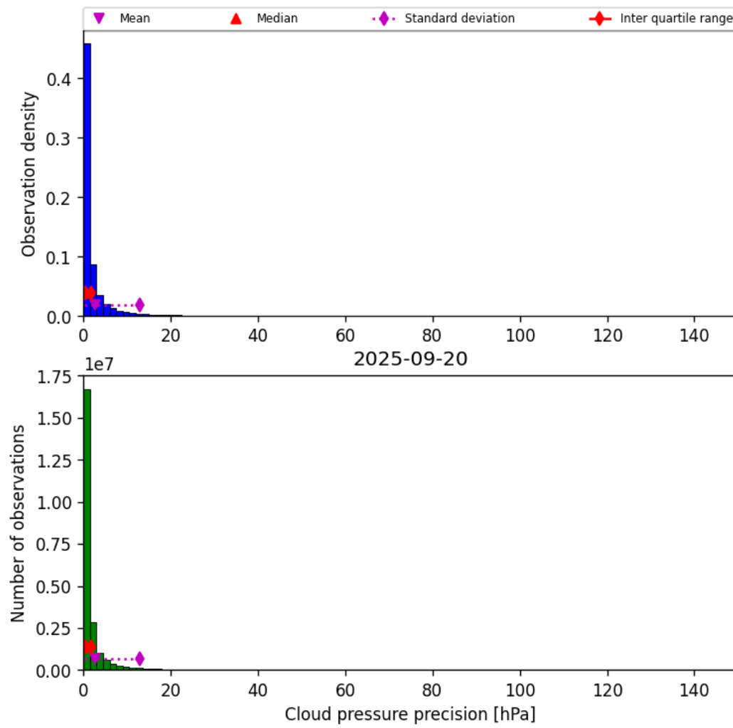
Figure 29: Histogram of “Cloud pressure precision” for 2025-09-20 to 2025-09-21
