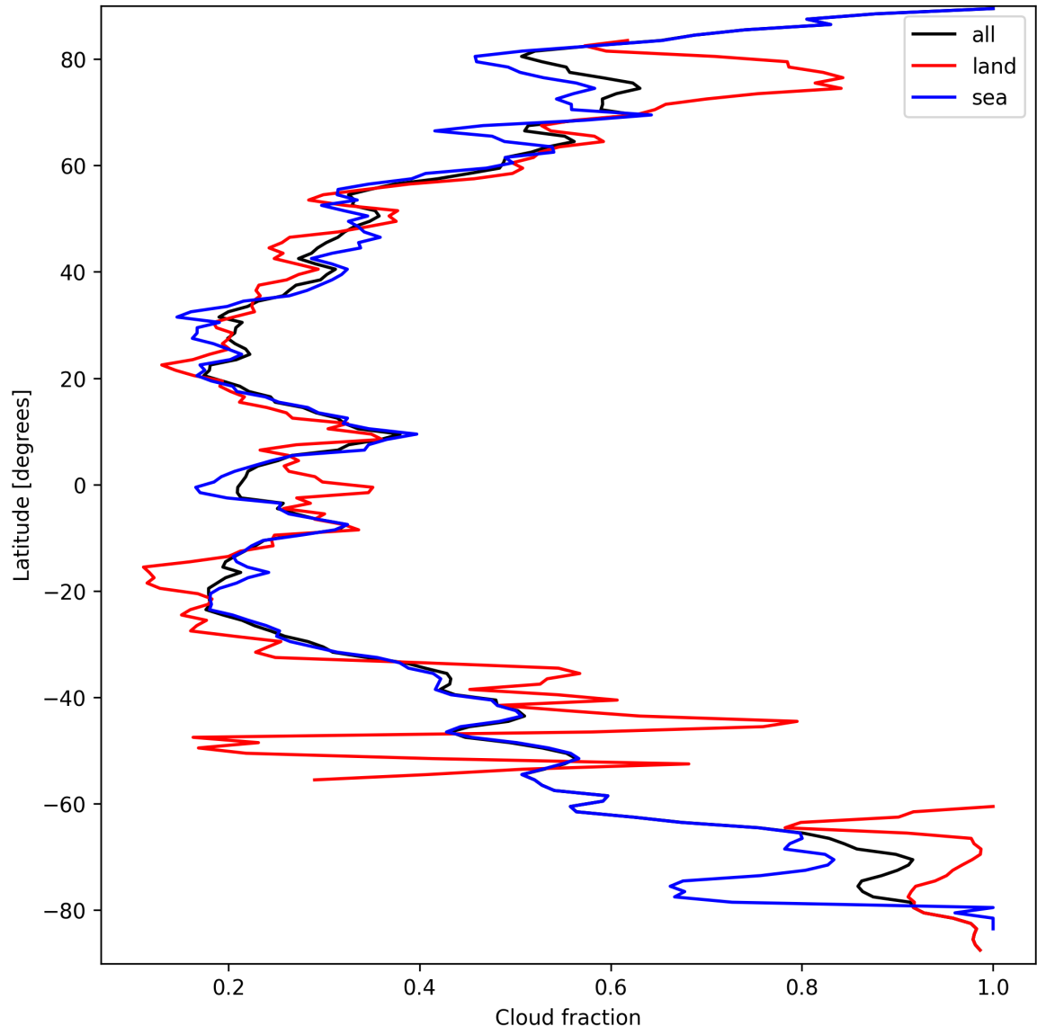
Figure 13: Zonal average of “Cloud fraction” for 2025-09-20 to 2025-09-21.
