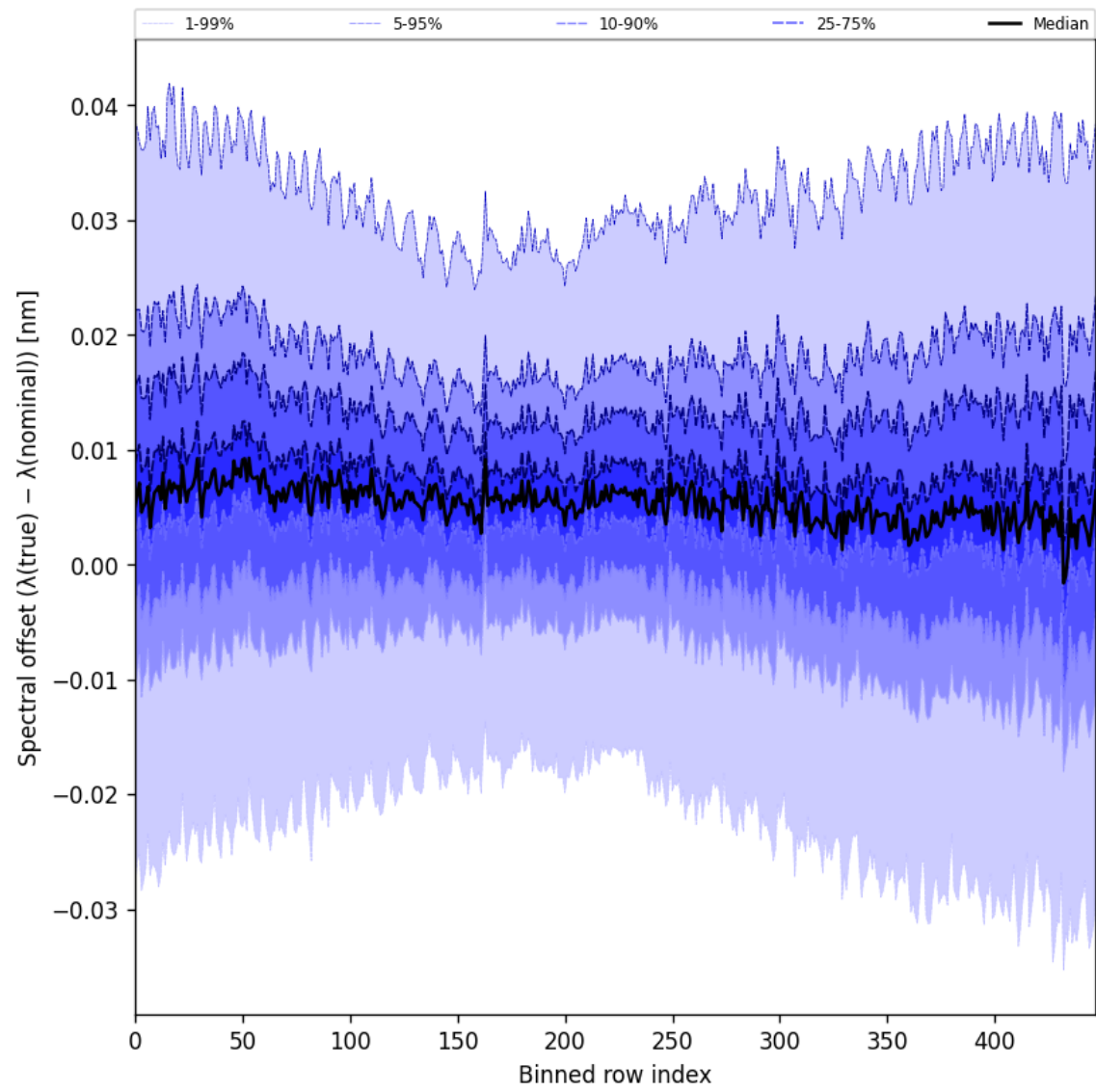
Figure 60: Along track statistics of “Spectral offset ( \lambda_{\text{true}} - \lambda_{\text{nominal}} )” for 2025-09-20 to 2025-09-21
