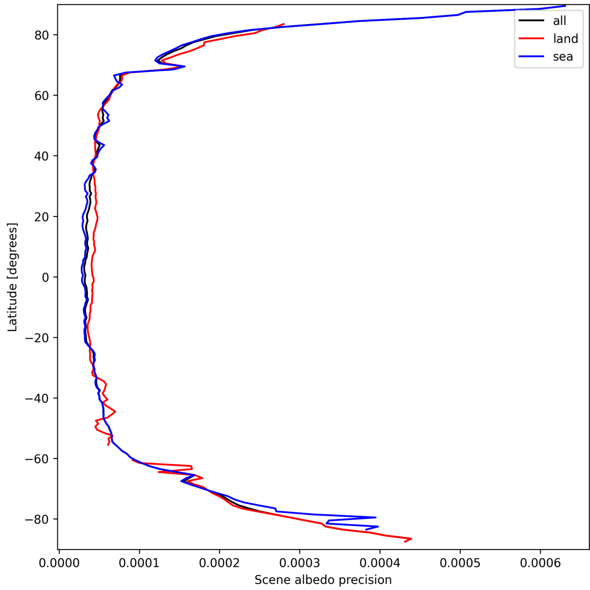
Figure 16: Zonal average of “Scene albedo precision” for 2025-09-20 to 2025-09-21.
