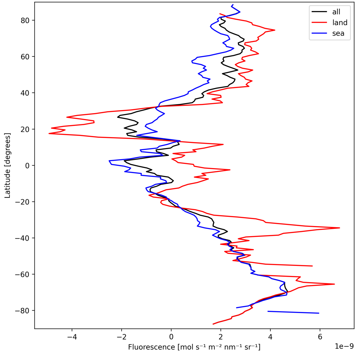
Figure 21: Zonal average of “Fluorescence” for 2025-09-21 to 2025-09-22.
