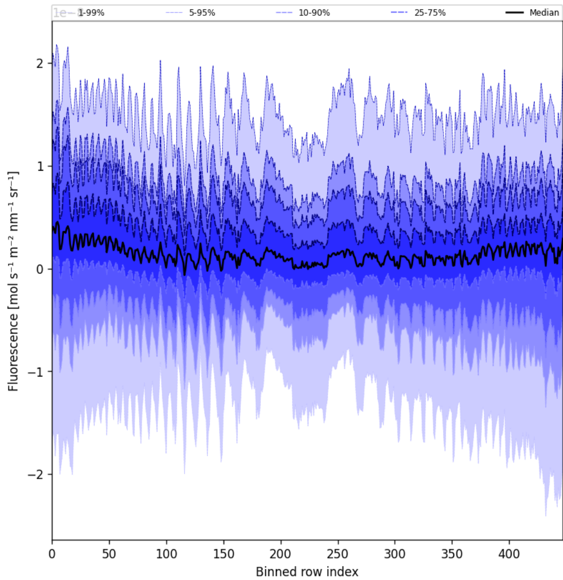
Figure 55: Along track statistics of “Fluorescence” for 2025-09-21 to 2025-09-22
