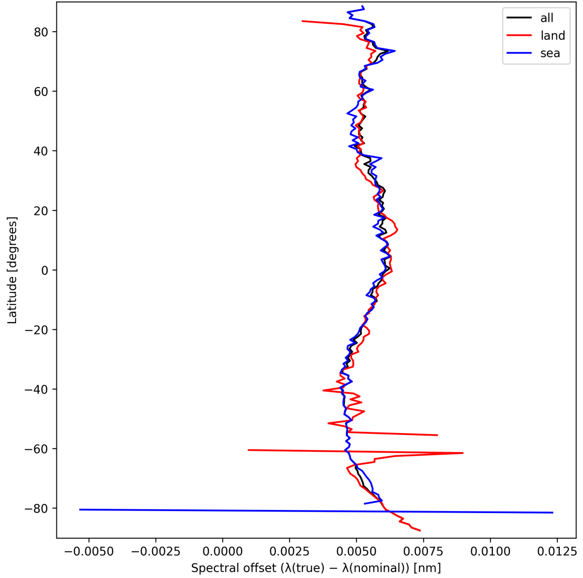
Figure 26: Zonal average of “Spectral offset ( \lambda_{\text{true}} - \lambda_{\text{nominal}} )” for 2025-09-21 to 2025-09-22.
