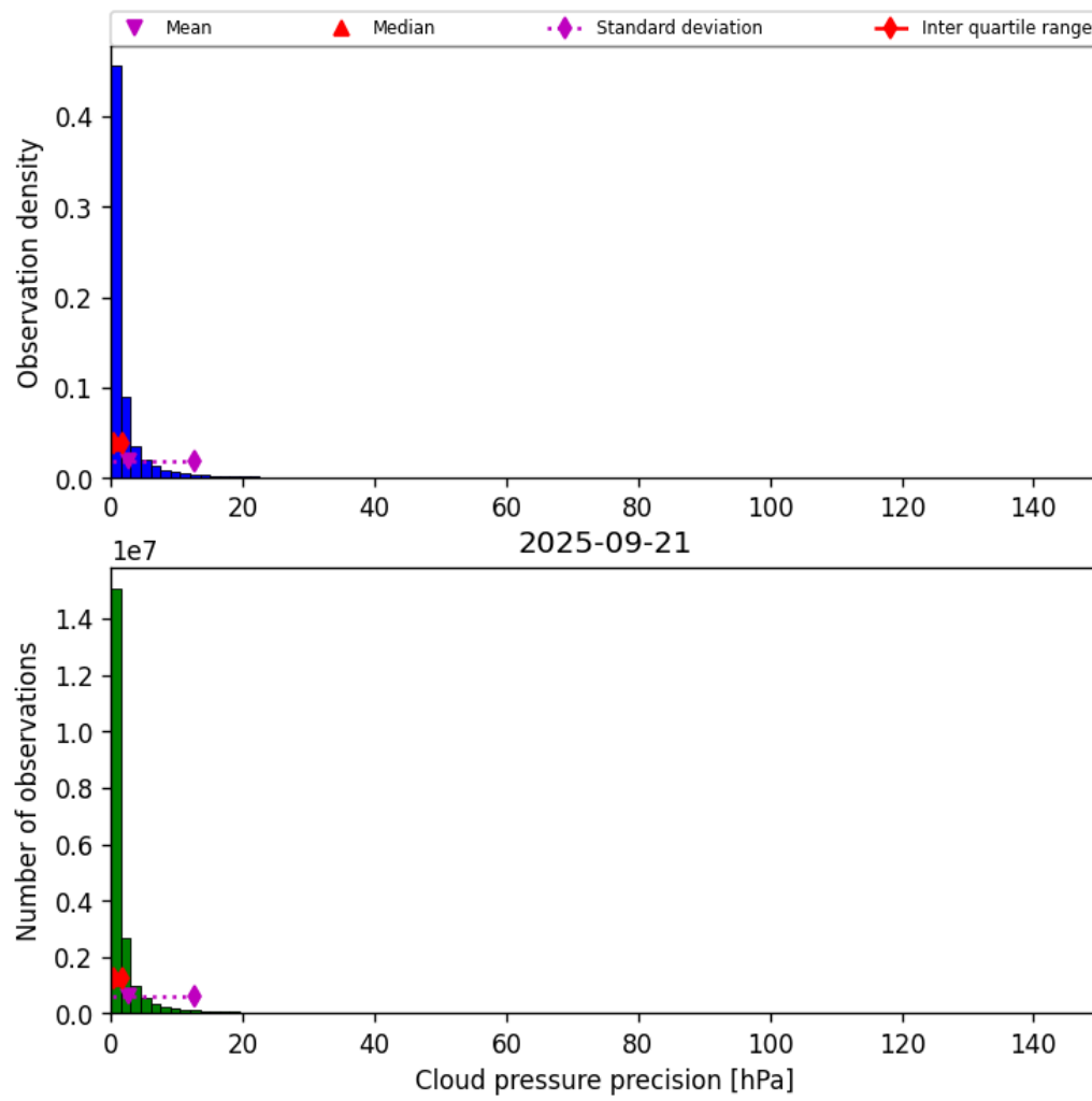
Figure 29: Histogram of “Cloud pressure precision” for 2025-09-21 to 2025-09-22
