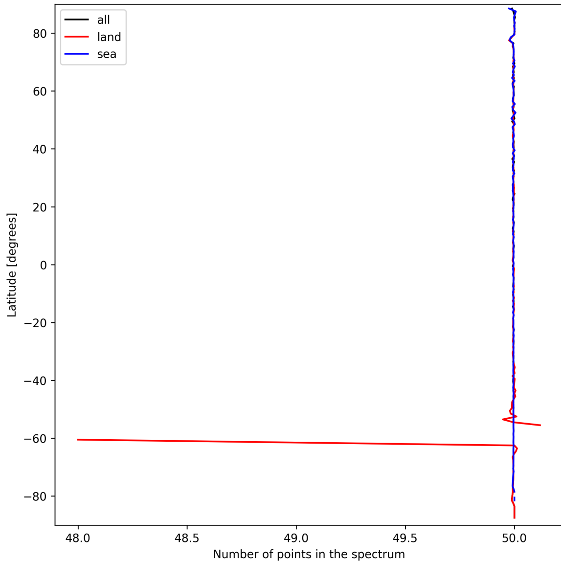
Figure 25: Zonal average of “Number of points in the spectrum” for 2025-09-21 to 2025-09-22.
