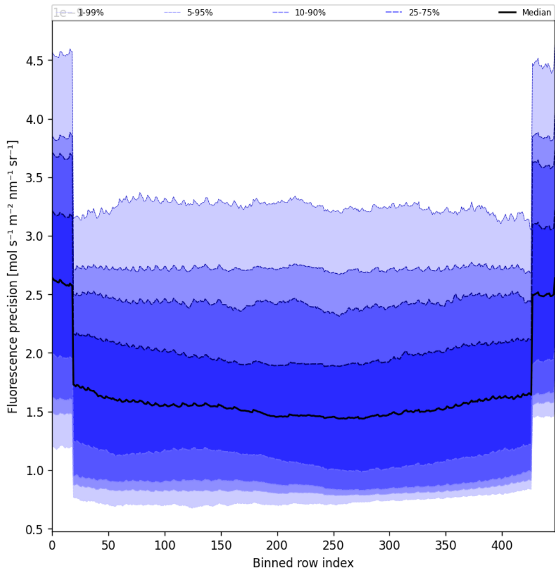
Figure 56: Along track statistics of “Fluorescence precision” for 2025-09-21 to 2025-09-22
