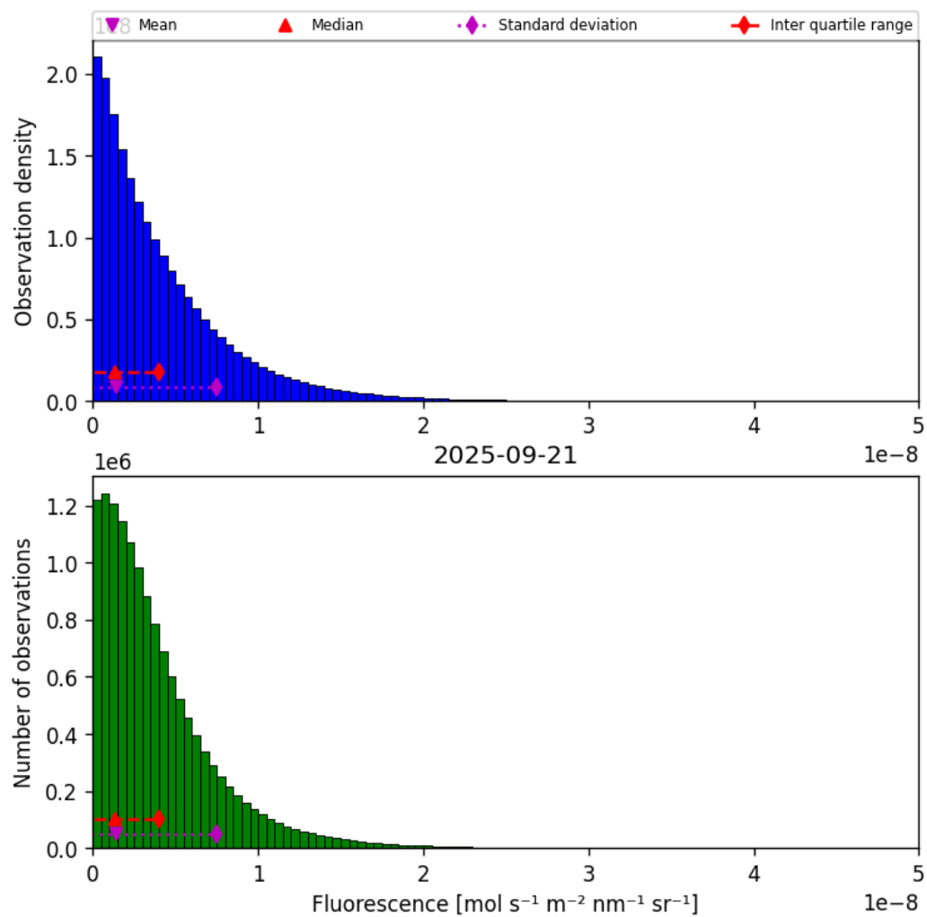
Figure 38: Histogram of “Fluorescence” for 2025-09-21 to 2025-09-22
