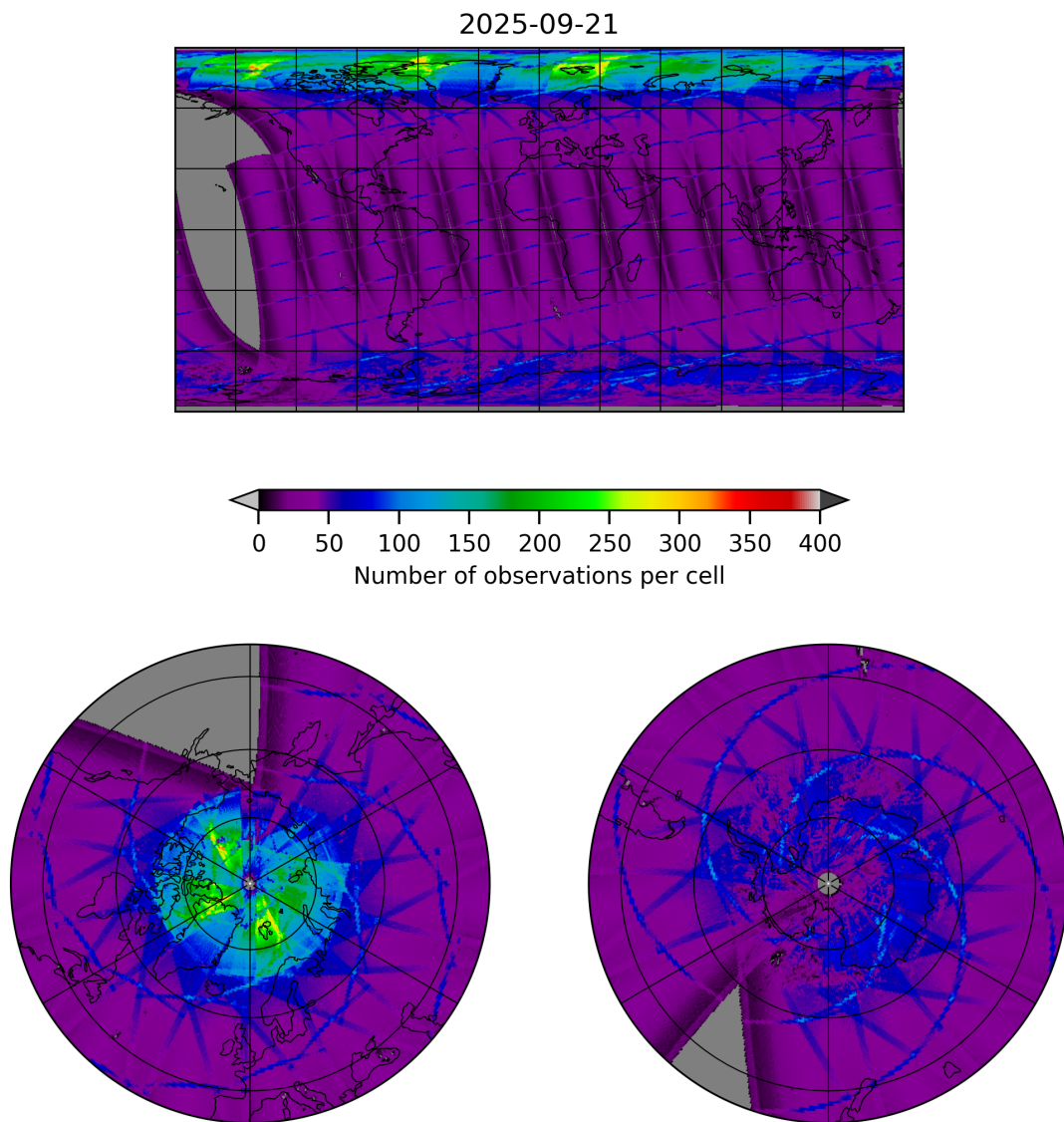
Figure 9: Map of the number of observations for 2025-09-21 to 2025-09-22
