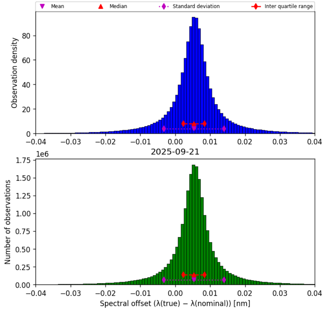
Figure 43: Histogram of “Spectral offset ( \lambda_{\text{true}} - \lambda_{\text{nominal}} )” for 2025-09-21 to 2025-09-22
