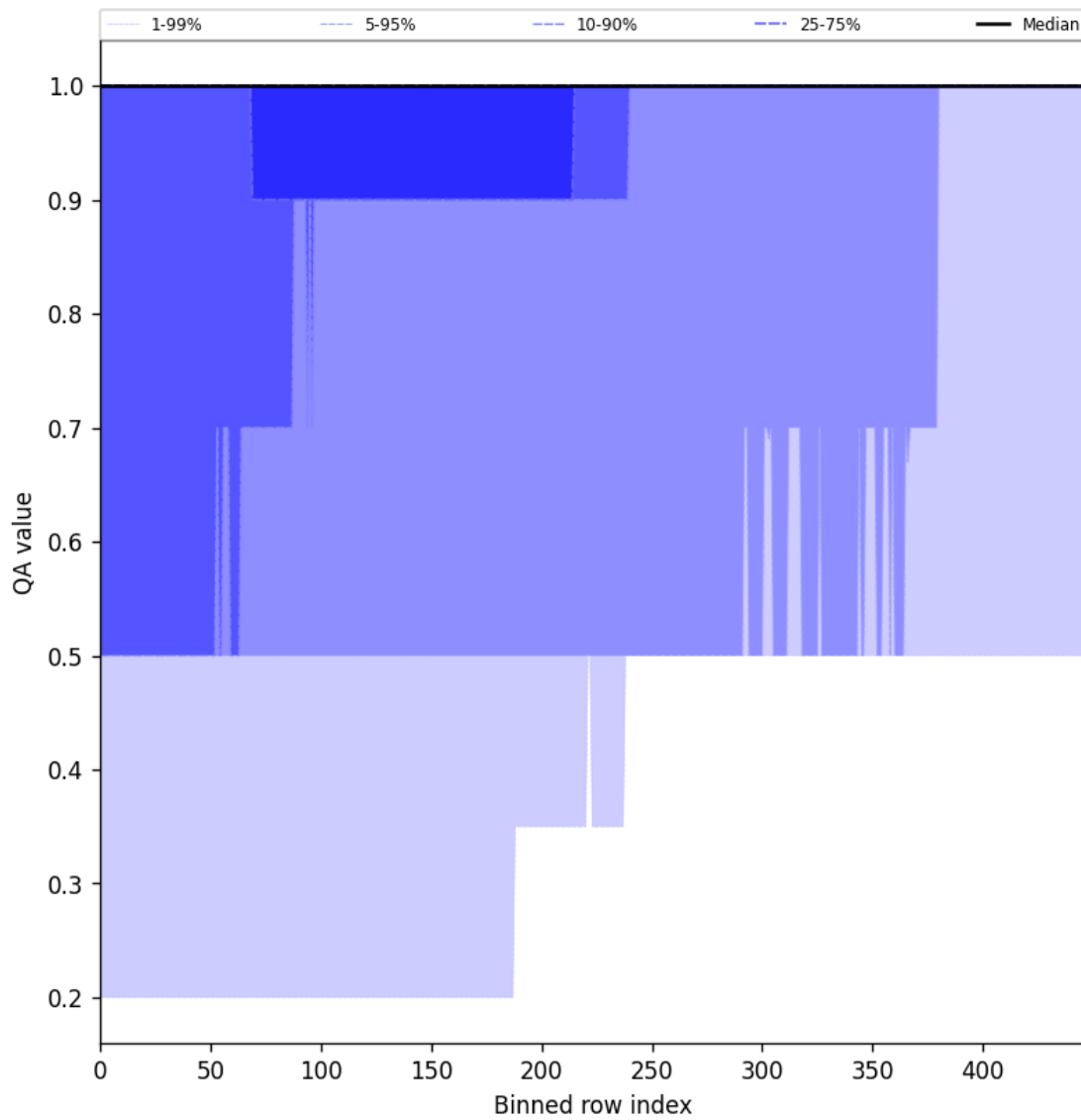
Figure 44: Along track statistics of “QA value” for 2025-09-21 to 2025-09-22
