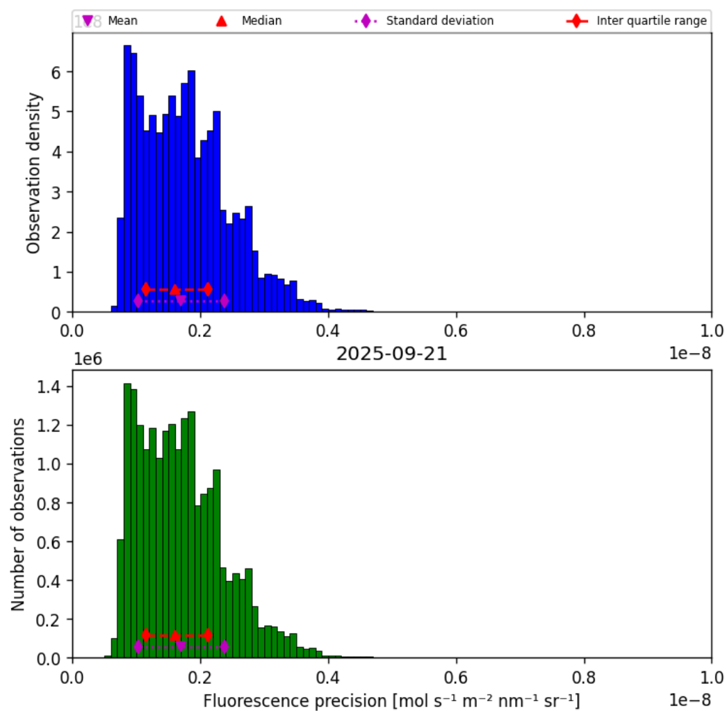
Figure 39: Histogram of “Fluorescence precision” for 2025-09-21 to 2025-09-22
