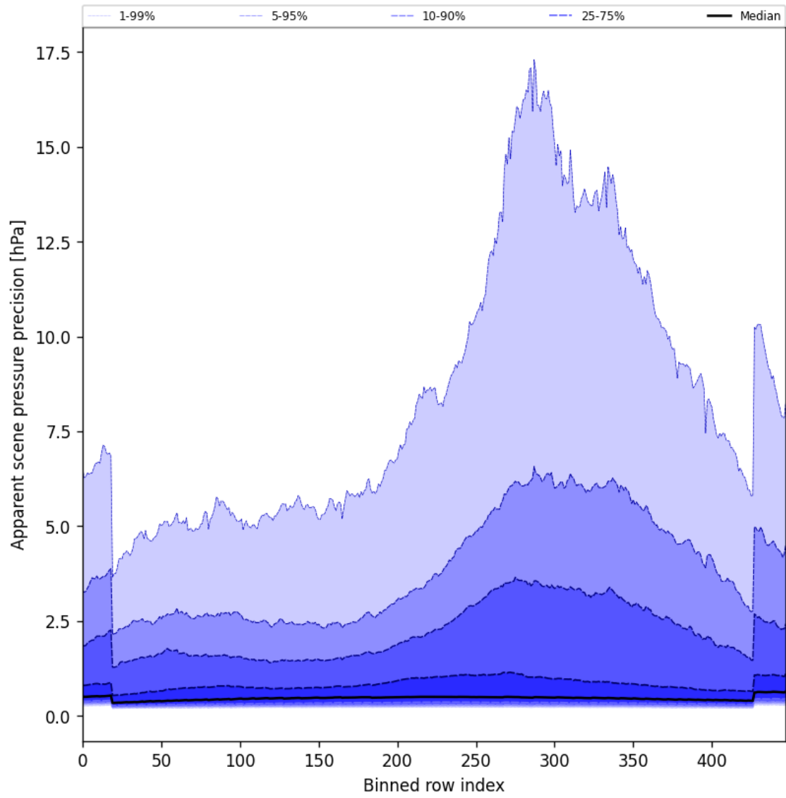
Figure 52: Along track statistics of “Apparent scene pressure precision” for 2025-09-21 to 2025-09-22
