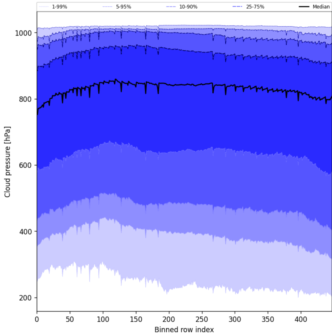
Figure 45: Along track statistics of “Cloud pressure” for 2025-09-21 to 2025-09-22
