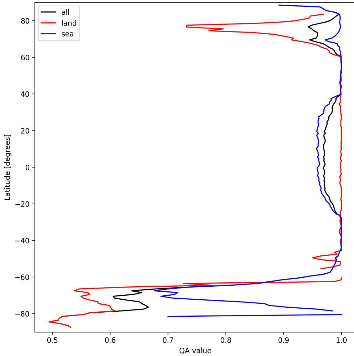
Figure 10: Zonal average of "QA value" for 2025-09-21 to 2025-09-22.
