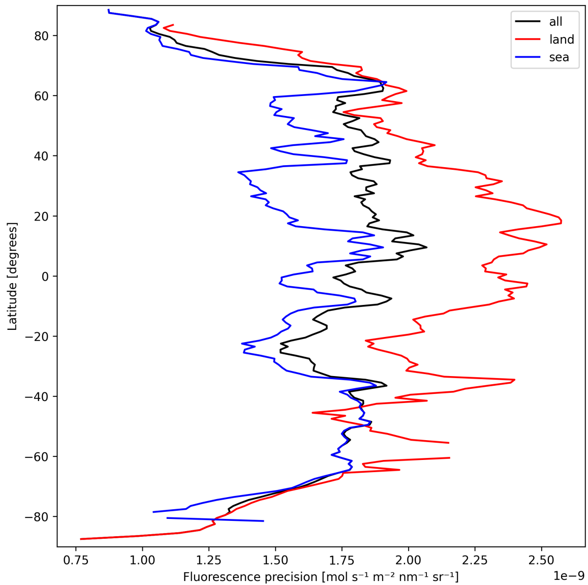
Figure 22: Zonal average of “Fluorescence precision” for 2025-09-21 to 2025-09-22.
