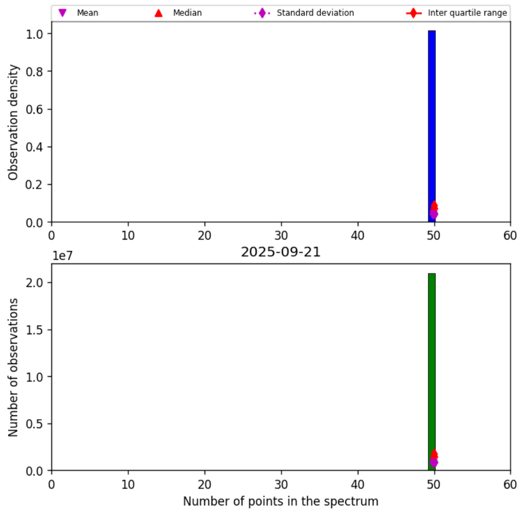
Figure 42: Histogram of “Number of points in the spectrum” for 2025-09-21 to 2025-09-22
