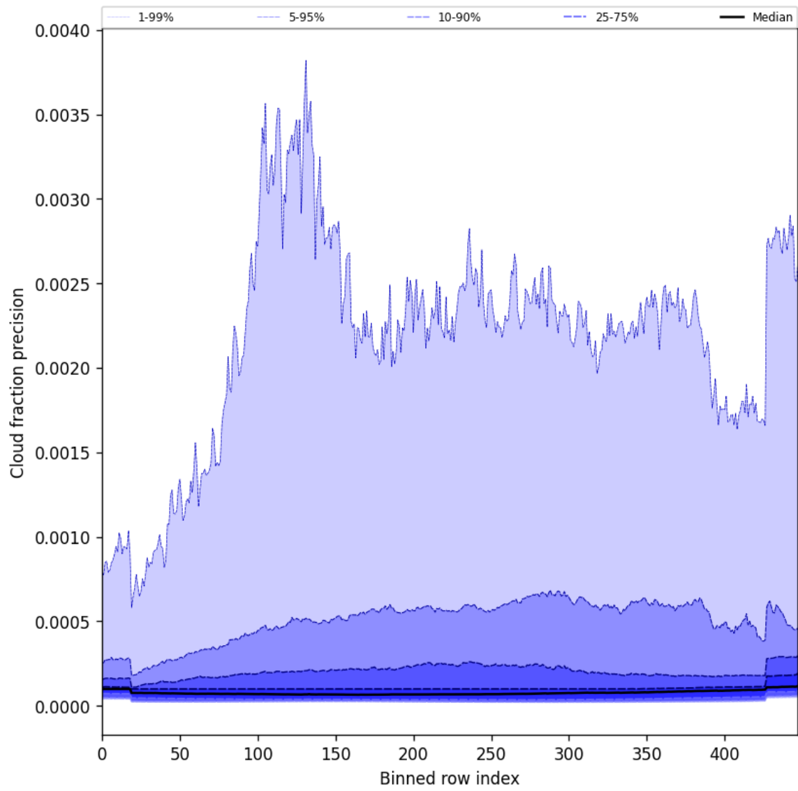
Figure 48: Along track statistics of “Cloud fraction precision” for 2025-09-21 to 2025-09-22
