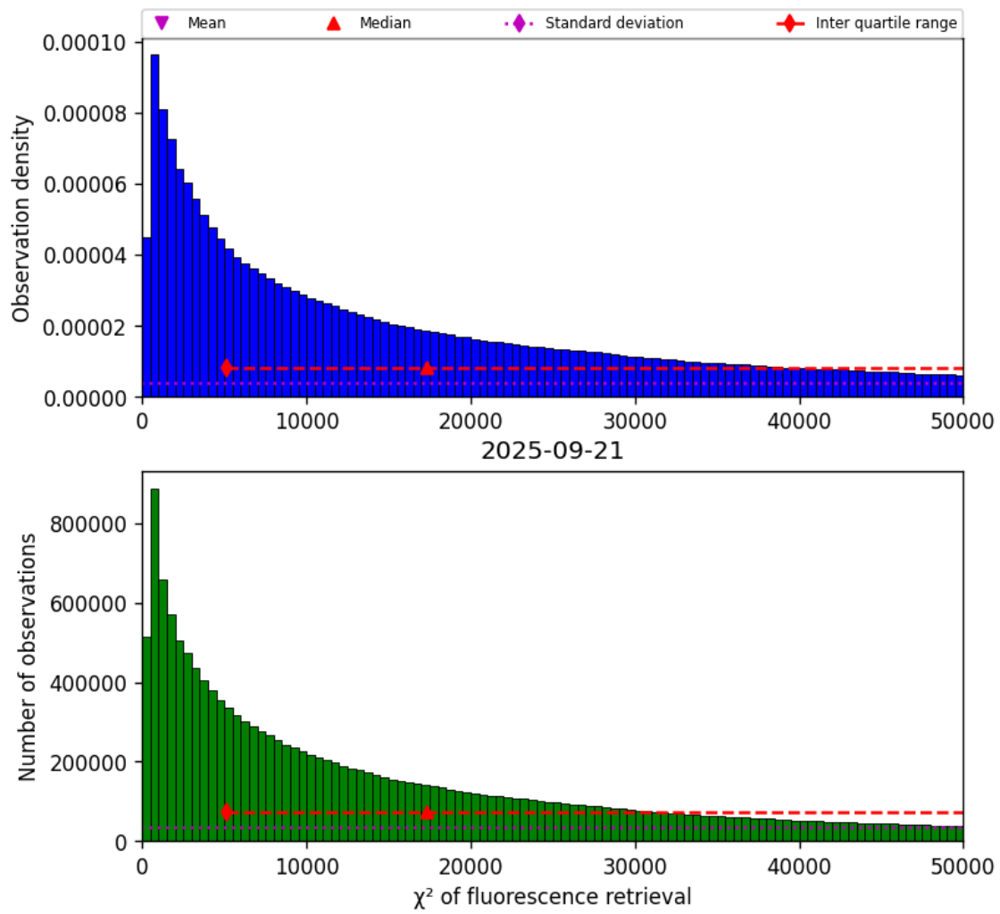
Figure 40: Histogram of “ \chi^2 of fluorescence retrieval” for 2025-09-21 to 2025-09-22
