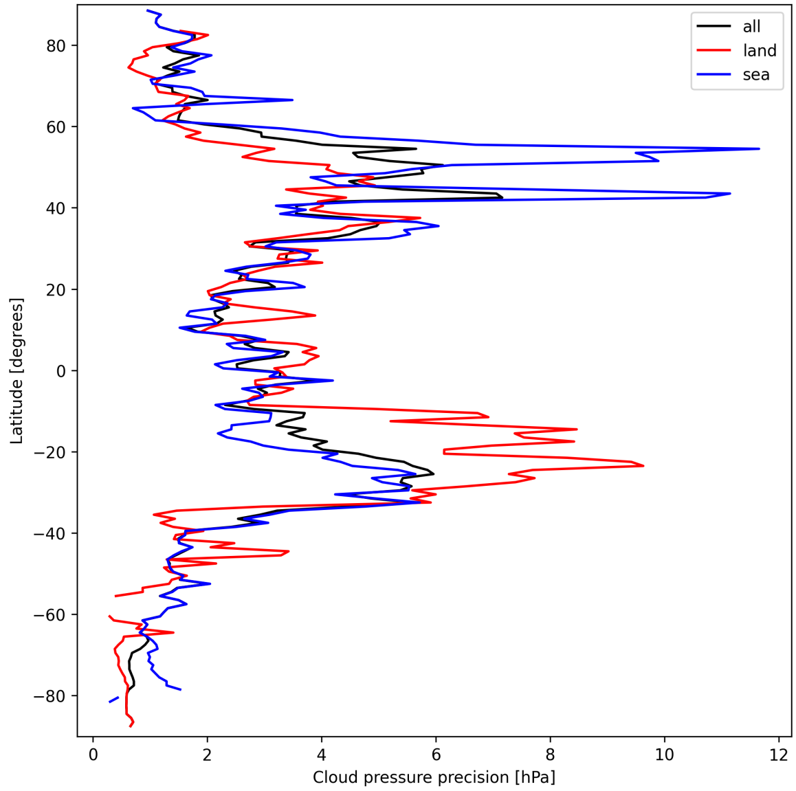
Figure 12: Zonal average of “Cloud pressure precision” for 2025-09-21 to 2025-09-22.
