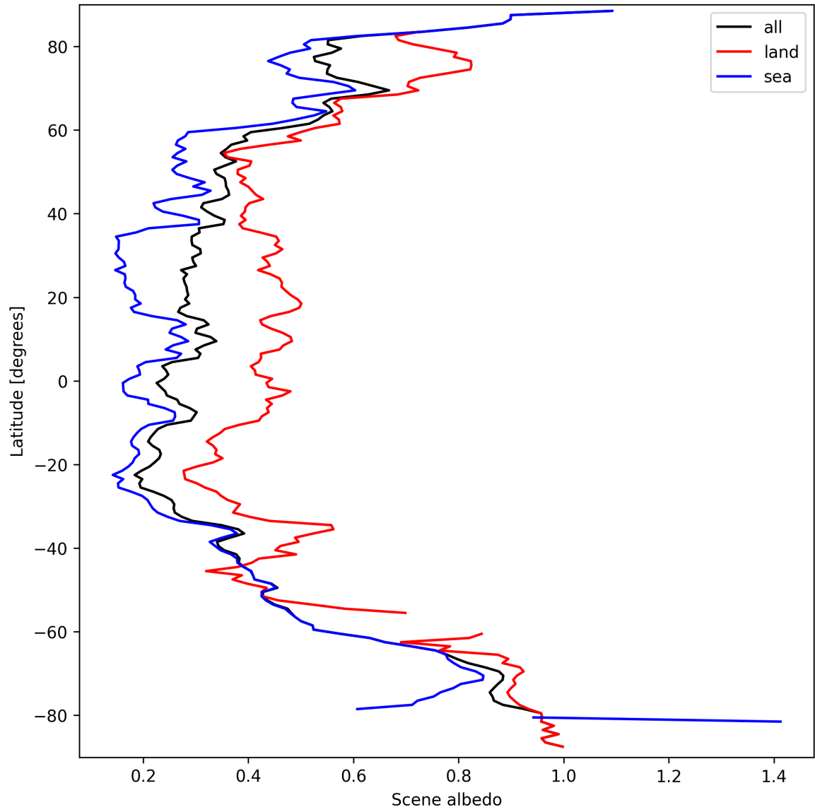
Figure 15: Zonal average of “Scene albedo” for 2025-09-21 to 2025-09-22.
