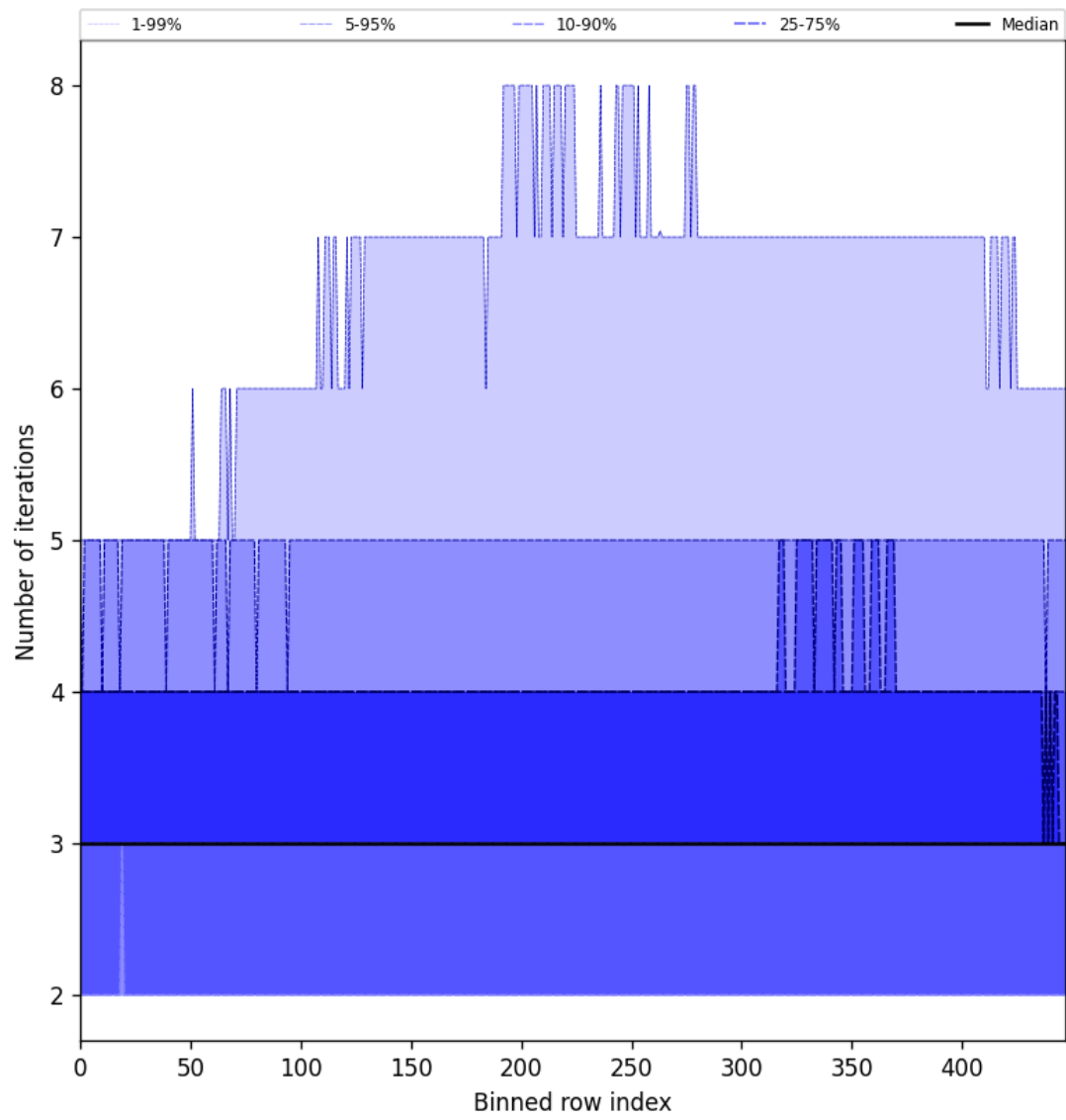
Figure 54: Along track statistics of “Number of iterations” for 2025-09-21 to 2025-09-22
