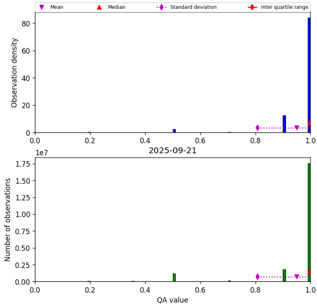
Figure 27: Histogram of “QA value” for 2025-09-21 to 2025-09-22
