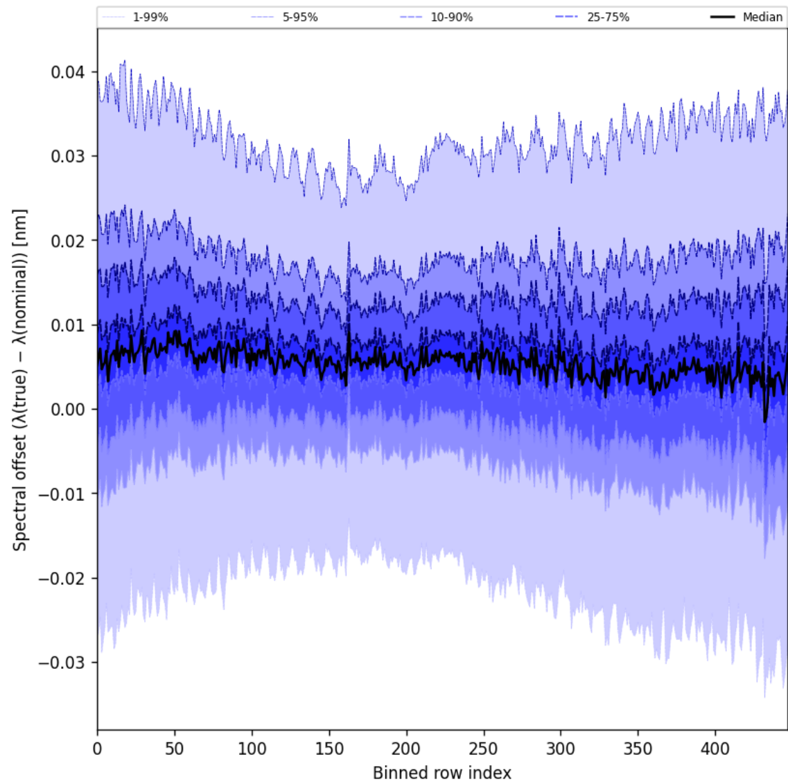
Figure 60: Along track statistics of “Spectral offset ( \lambda_{\text{true}} - \lambda_{\text{nominal}} )” for 2025-09-21 to 2025-09-22
