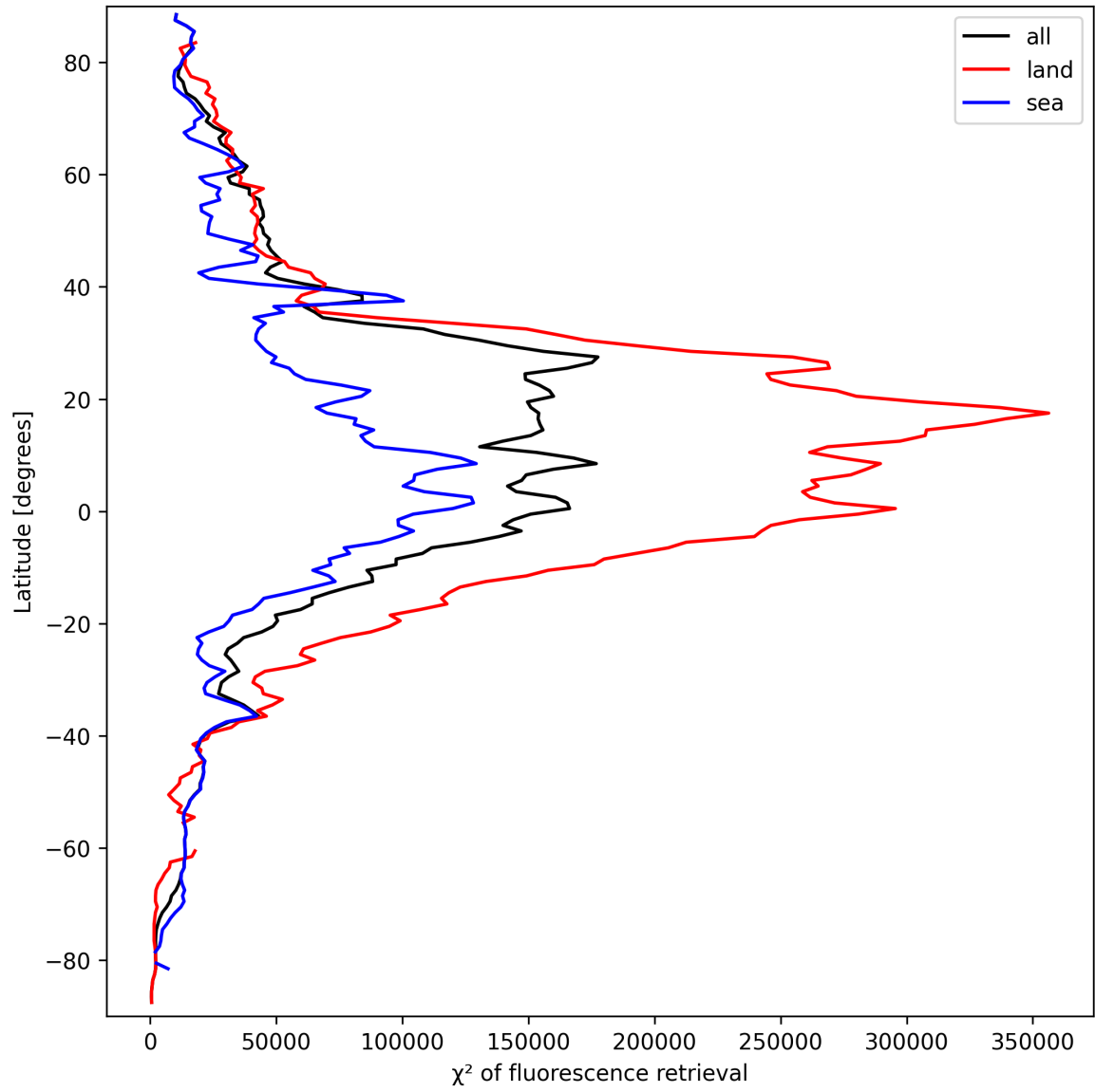
Figure 23: Zonal average of “ \chi^2 of fluorescence retrieval” for 2025-09-21 to 2025-09-22.
