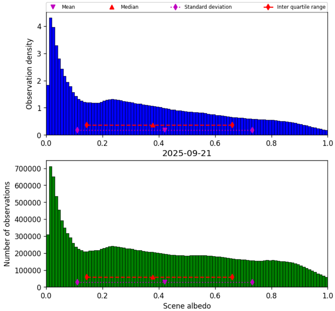
Figure 32: Histogram of “Scene albedo” for 2025-09-21 to 2025-09-22
