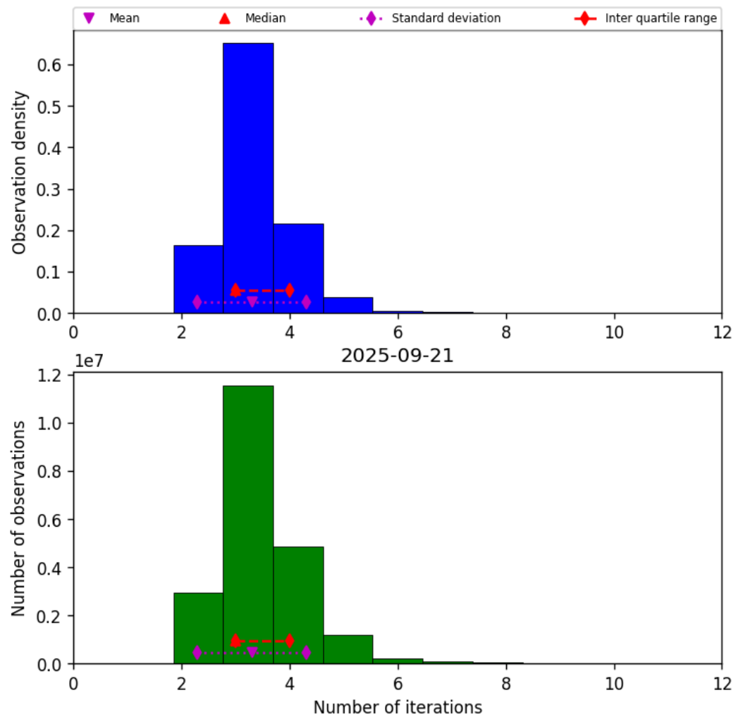
Figure 37: Histogram of “Number of iterations” for 2025-09-21 to 2025-09-22
