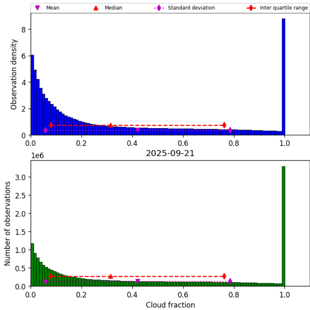
Figure 30: Histogram of “Cloud fraction” for 2025-09-21 to 2025-09-22
