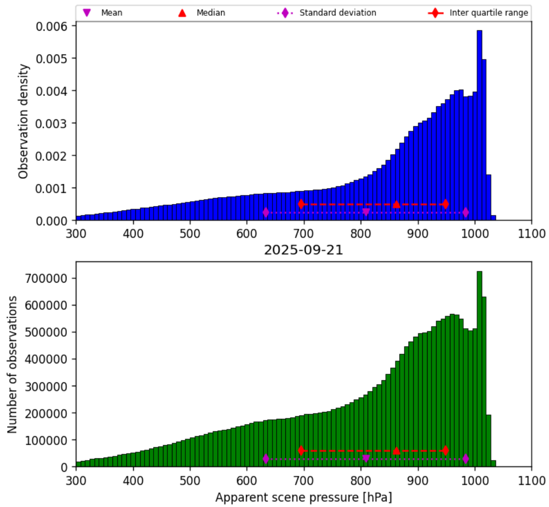
Figure 34: Histogram of “Apparent scene pressure” for 2025-09-21 to 2025-09-22
