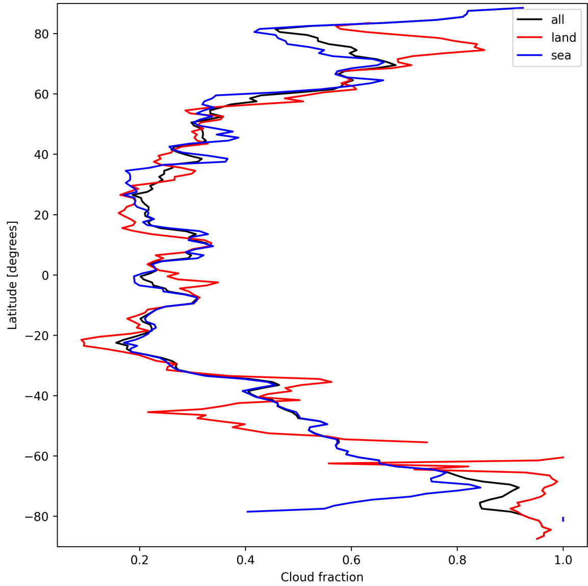
Figure 13: Zonal average of “Cloud fraction” for 2025-09-21 to 2025-09-22.
