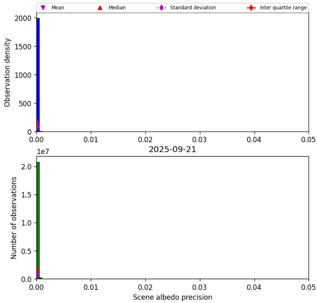
Figure 33: Histogram of “Scene albedo precision” for 2025-09-21 to 2025-09-22
