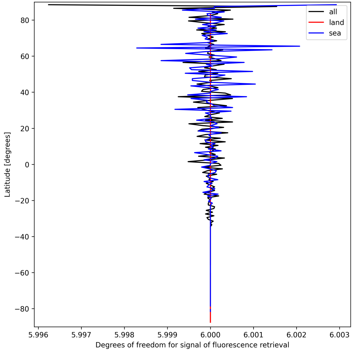
Figure 24: Zonal average of “Degrees of freedom for signal of fluorescence retrieval” for 2025-09-21 to 2025-09-22.
