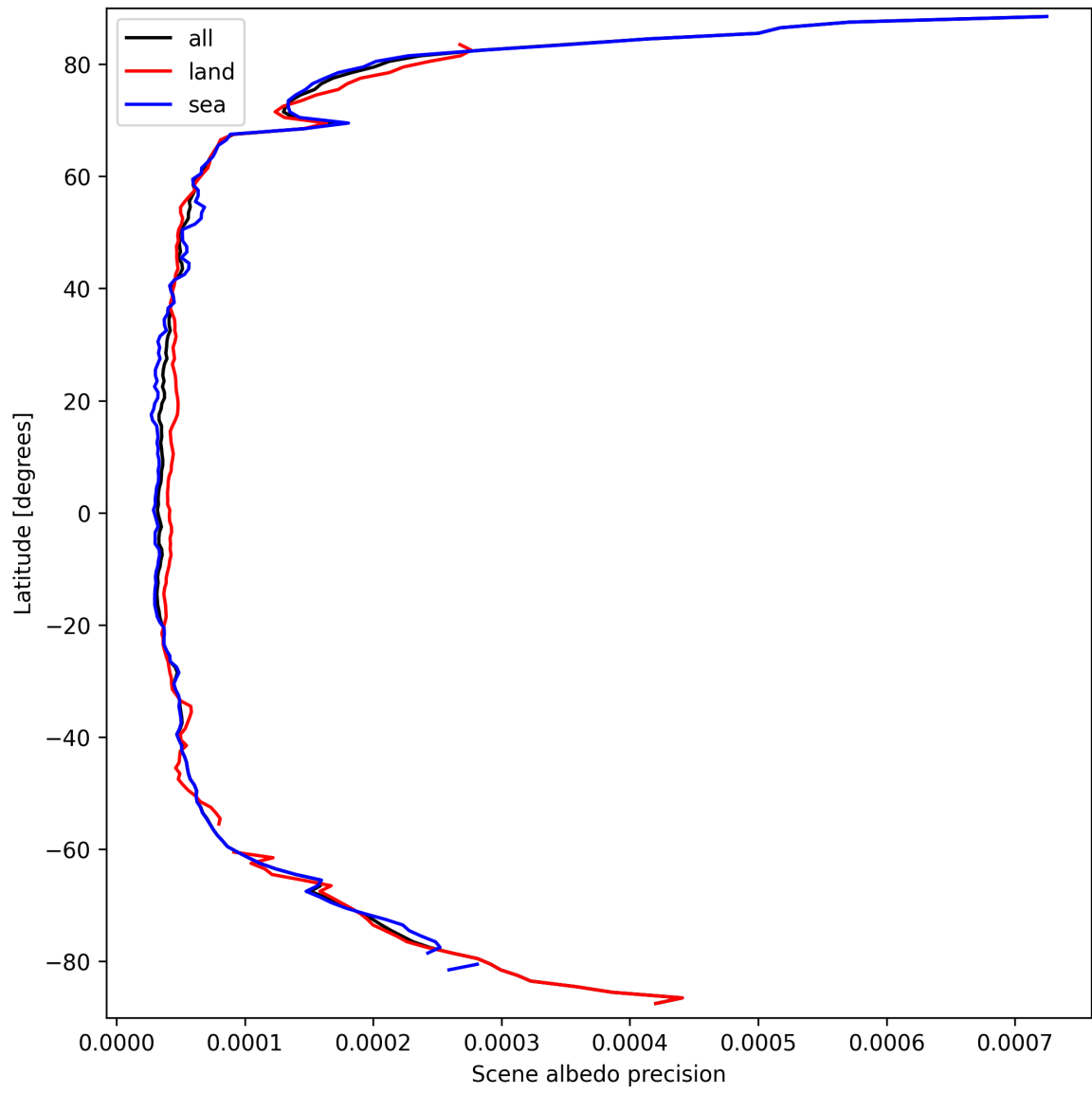
Figure 16: Zonal average of “Scene albedo precision” for 2025-09-21 to 2025-09-22.
