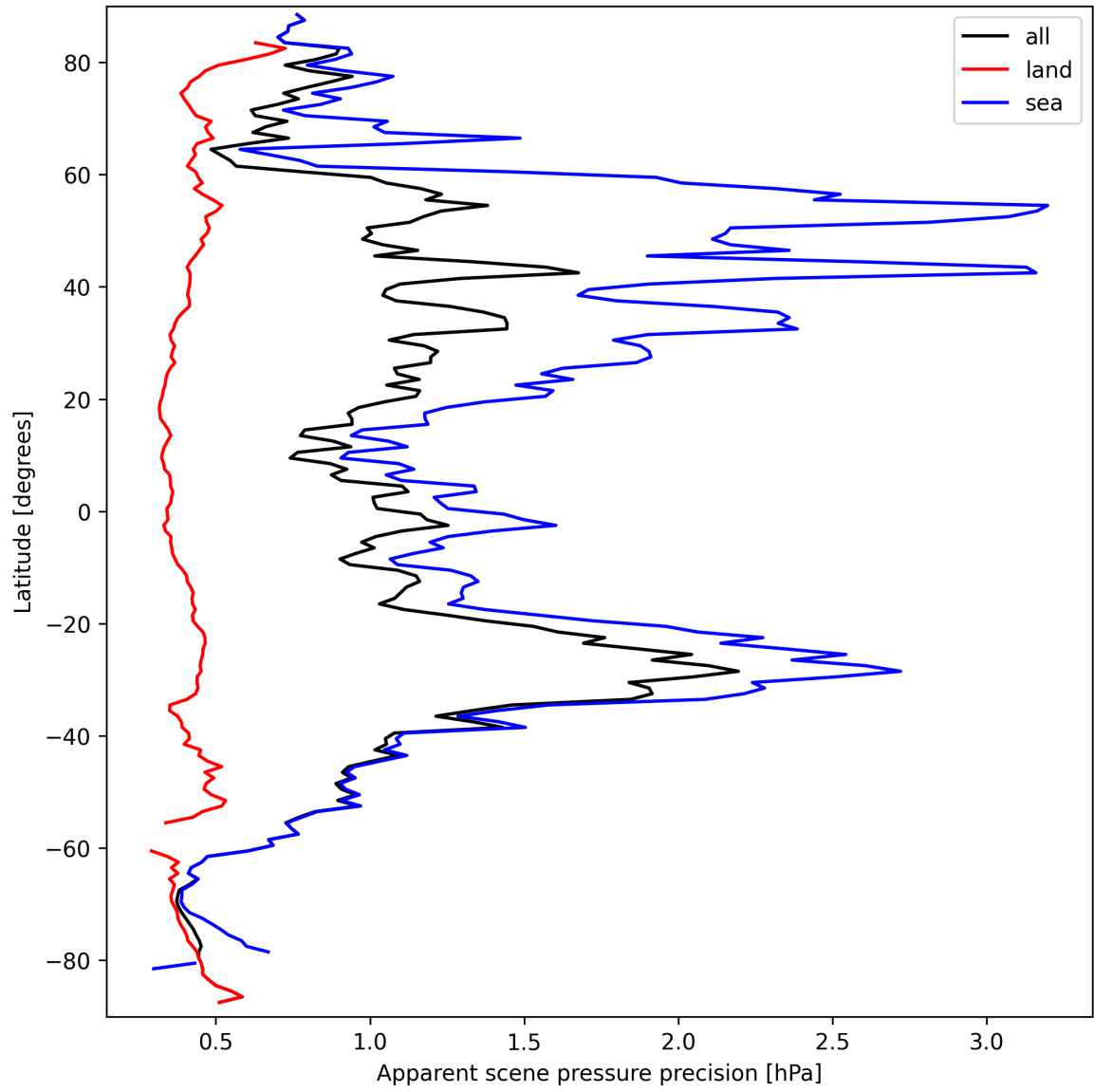
Figure 18: Zonal average of “Apparent scene pressure precision” for 2025-09-21 to 2025-09-22.
