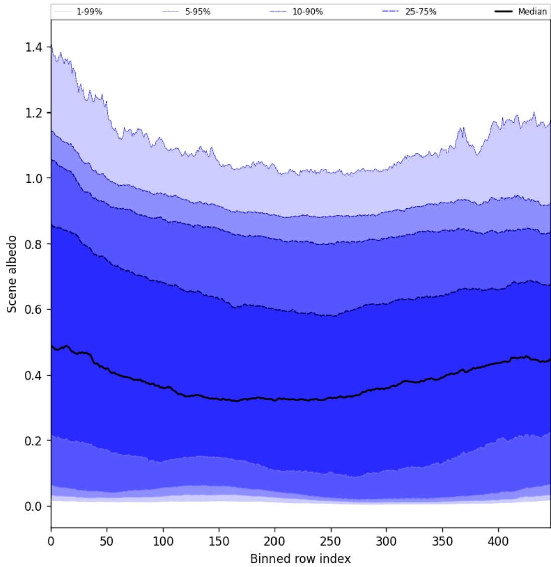
Figure 49: Along track statistics of “Scene albedo” for 2025-09-21 to 2025-09-22
