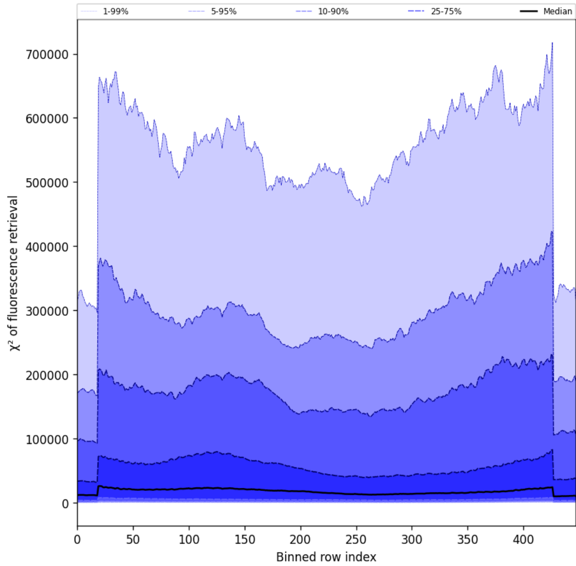
Figure 57: Along track statistics of “ \chi^2 of fluorescence retrieval” for 2025-09-21 to 2025-09-22
