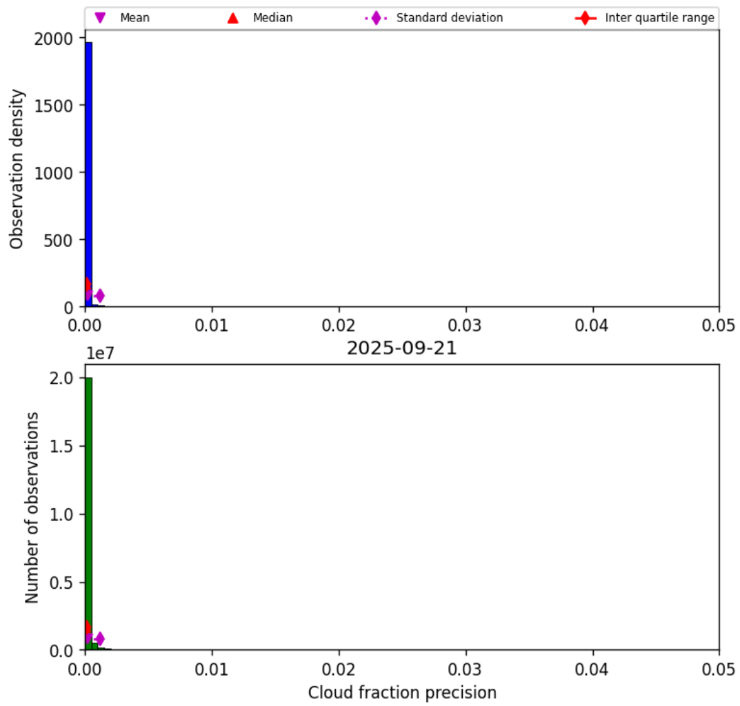
Figure 31: Histogram of “Cloud fraction precision” for 2025-09-21 to 2025-09-22
