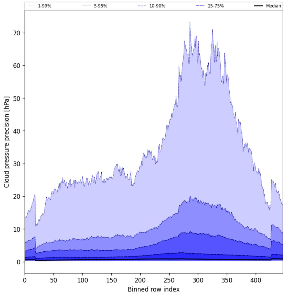
Figure 46: Along track statistics of “Cloud pressure precision” for 2025-09-21 to 2025-09-22
