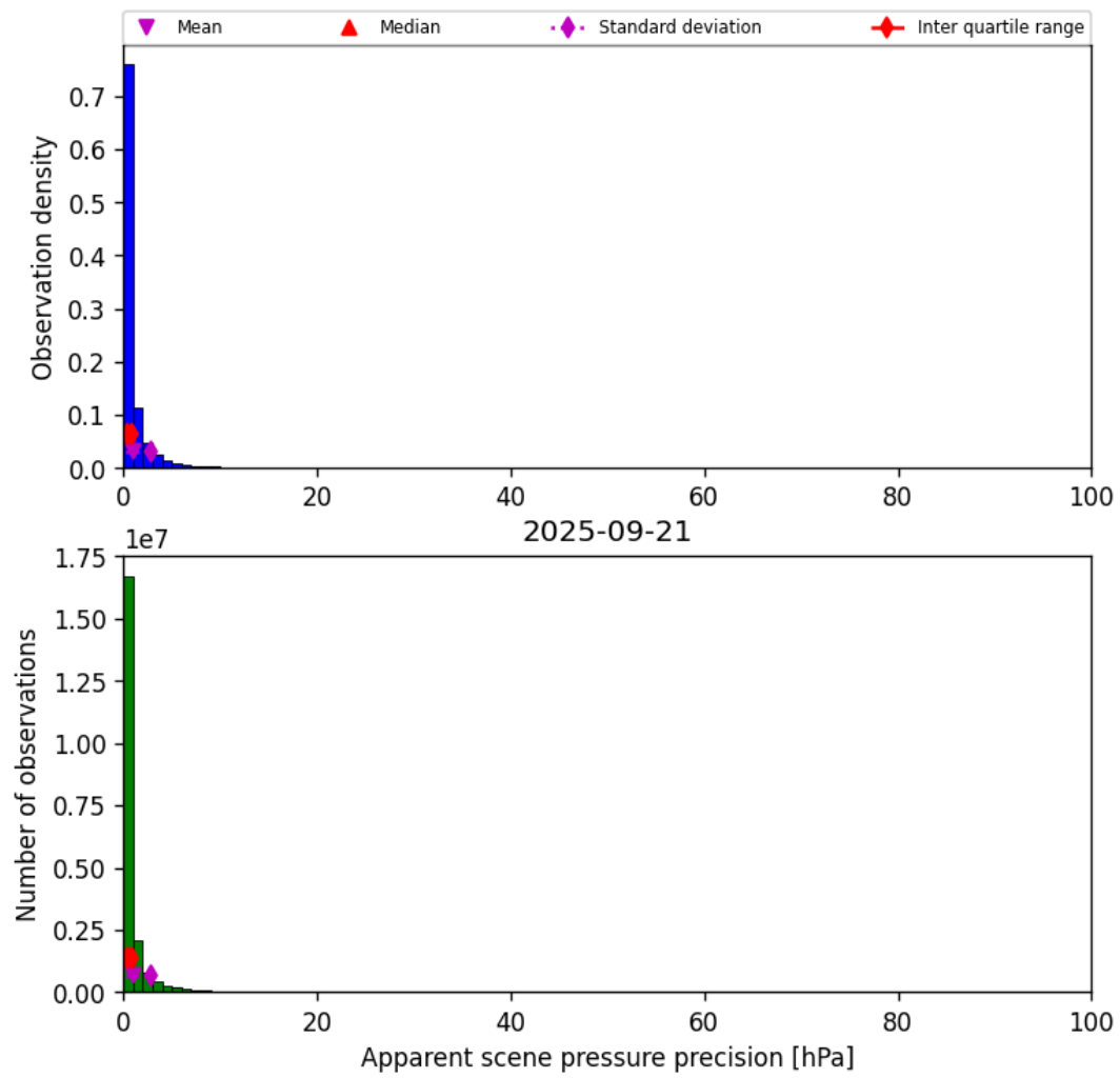
Figure 35: Histogram of “Apparent scene pressure precision” for 2025-09-21 to 2025-09-22
