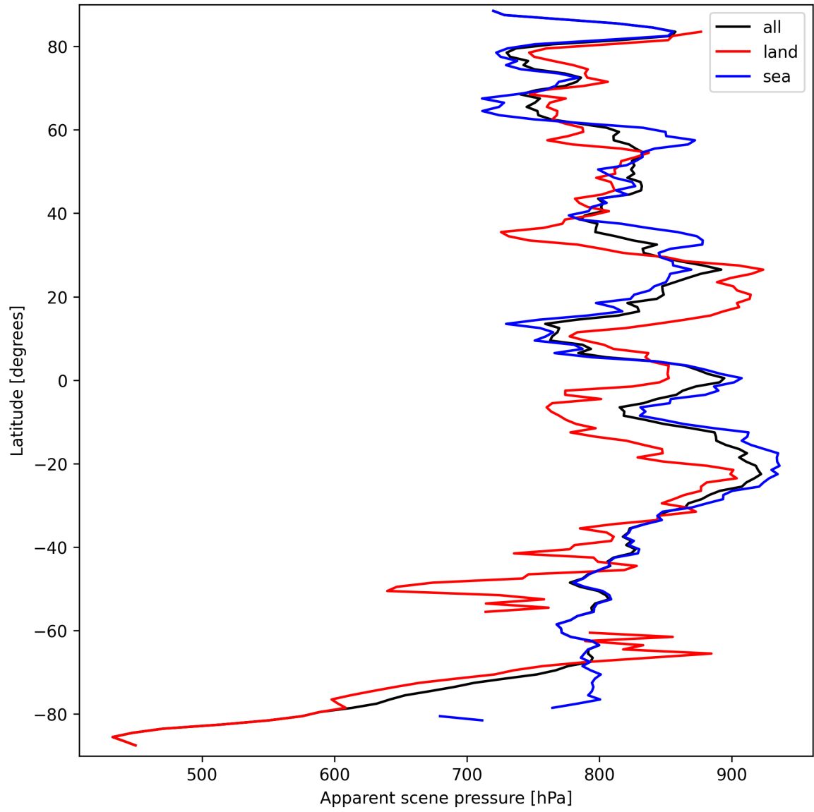
Figure 17: Zonal average of “Apparent scene pressure” for 2025-09-21 to 2025-09-22.
