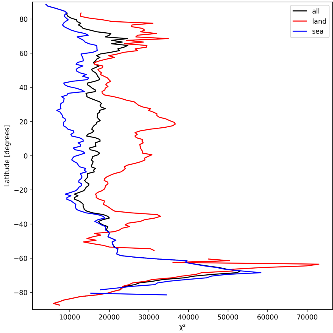
Figure 19: Zonal average of “ \chi^2 ” for 2025-09-21 to 2025-09-22.
