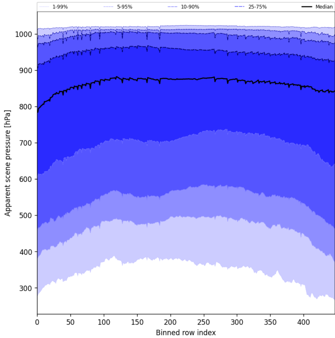
Figure 51: Along track statistics of “Apparent scene pressure” for 2025-09-21 to 2025-09-22
