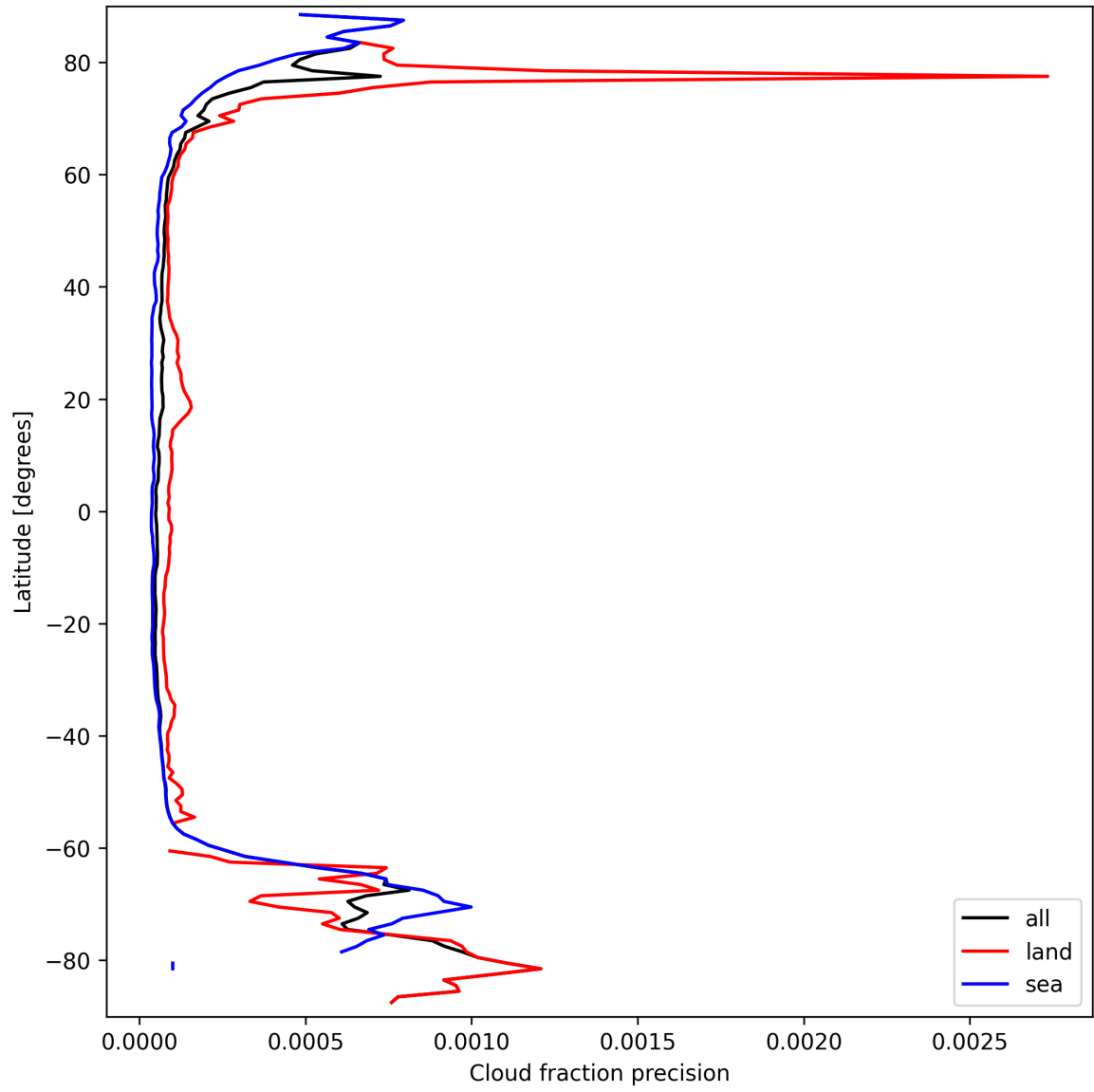
Figure 14: Zonal average of “Cloud fraction precision” for 2025-09-21 to 2025-09-22.
