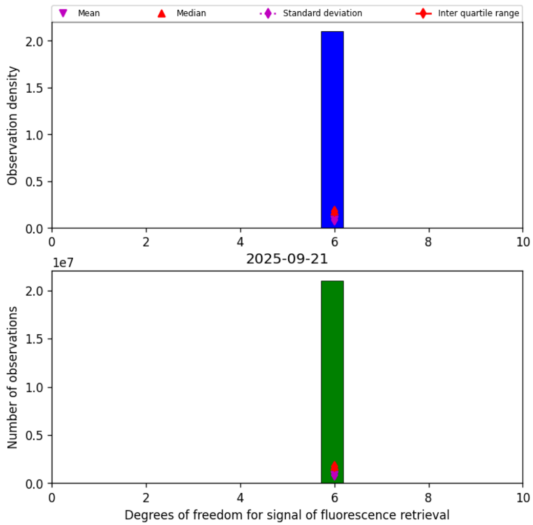
Figure 41: Histogram of “Degrees of freedom for signal of fluorescence retrieval” for 2025-09-21 to 2025-09-22
