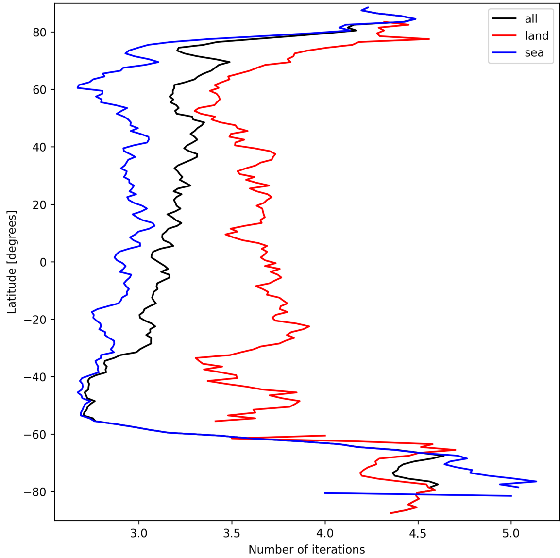
Figure 20: Zonal average of “Number of iterations” for 2025-09-21 to 2025-09-22.
