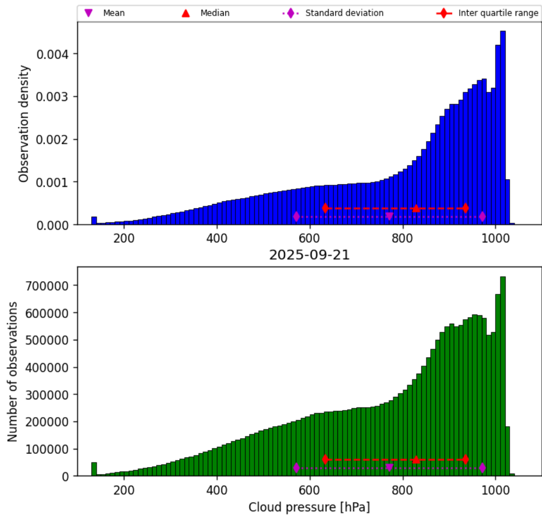
Figure 28: Histogram of “Cloud pressure” for 2025-09-21 to 2025-09-22
