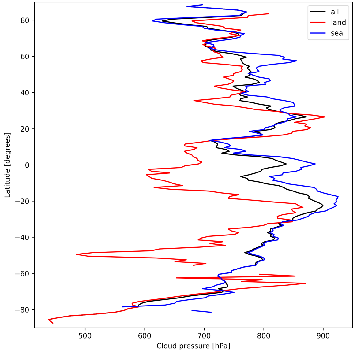
Figure 11: Zonal average of “Cloud pressure” for 2025-09-21 to 2025-09-22.
