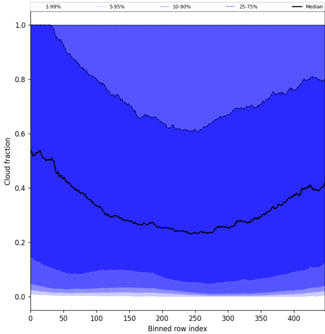
Figure 47: Along track statistics of “Cloud fraction” for 2025-09-21 to 2025-09-22
