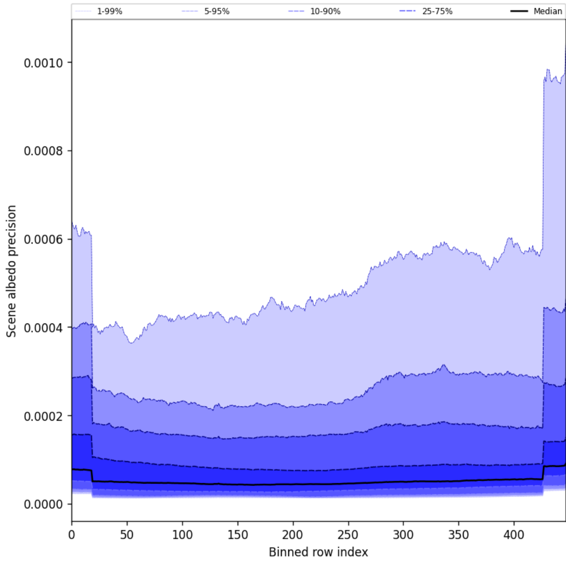
Figure 50: Along track statistics of “Scene albedo precision” for 2025-09-21 to 2025-09-22
