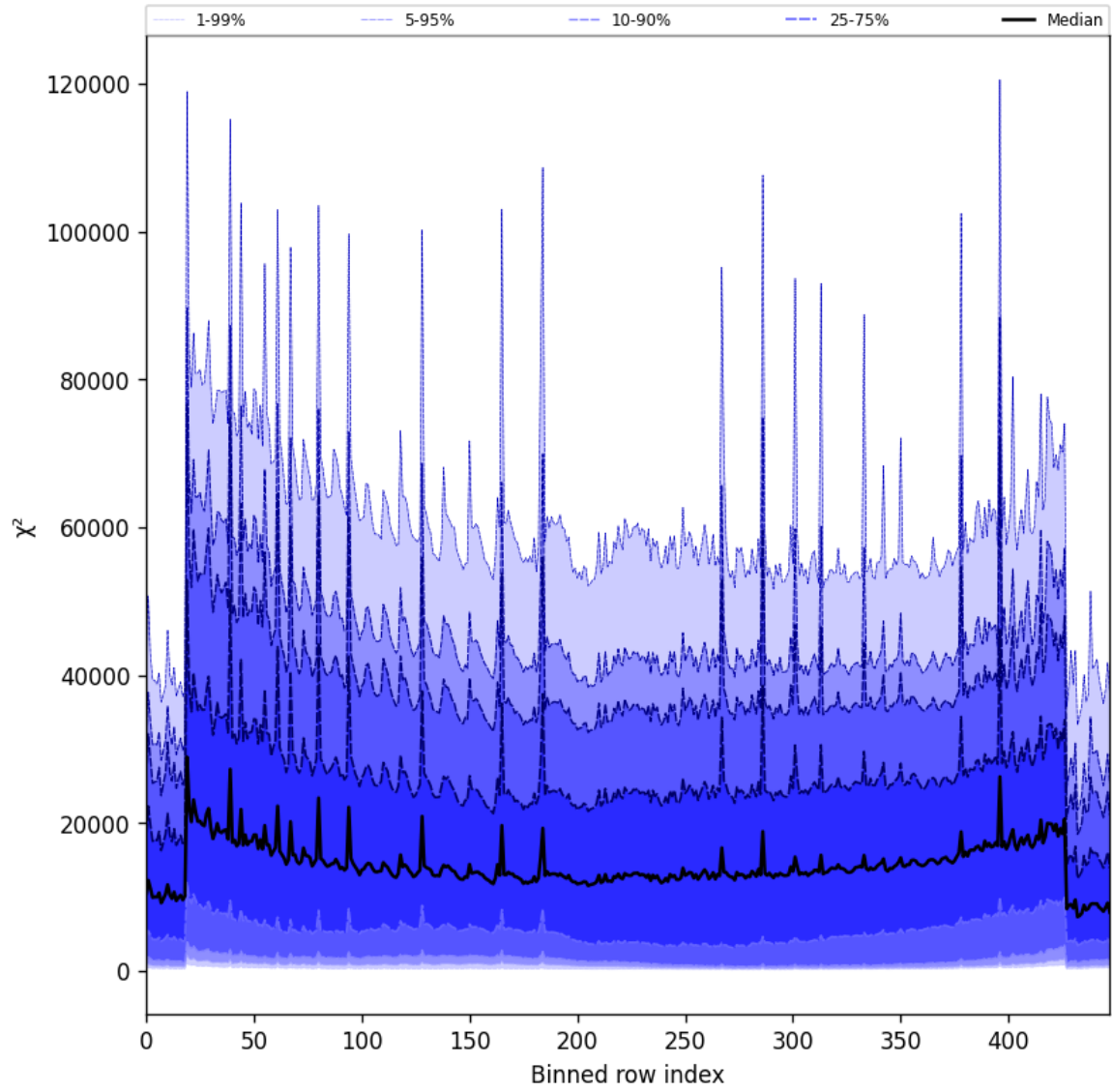
Figure 53: Along track statistics of “ \chi^2 ” for 2025-09-21 to 2025-09-22
