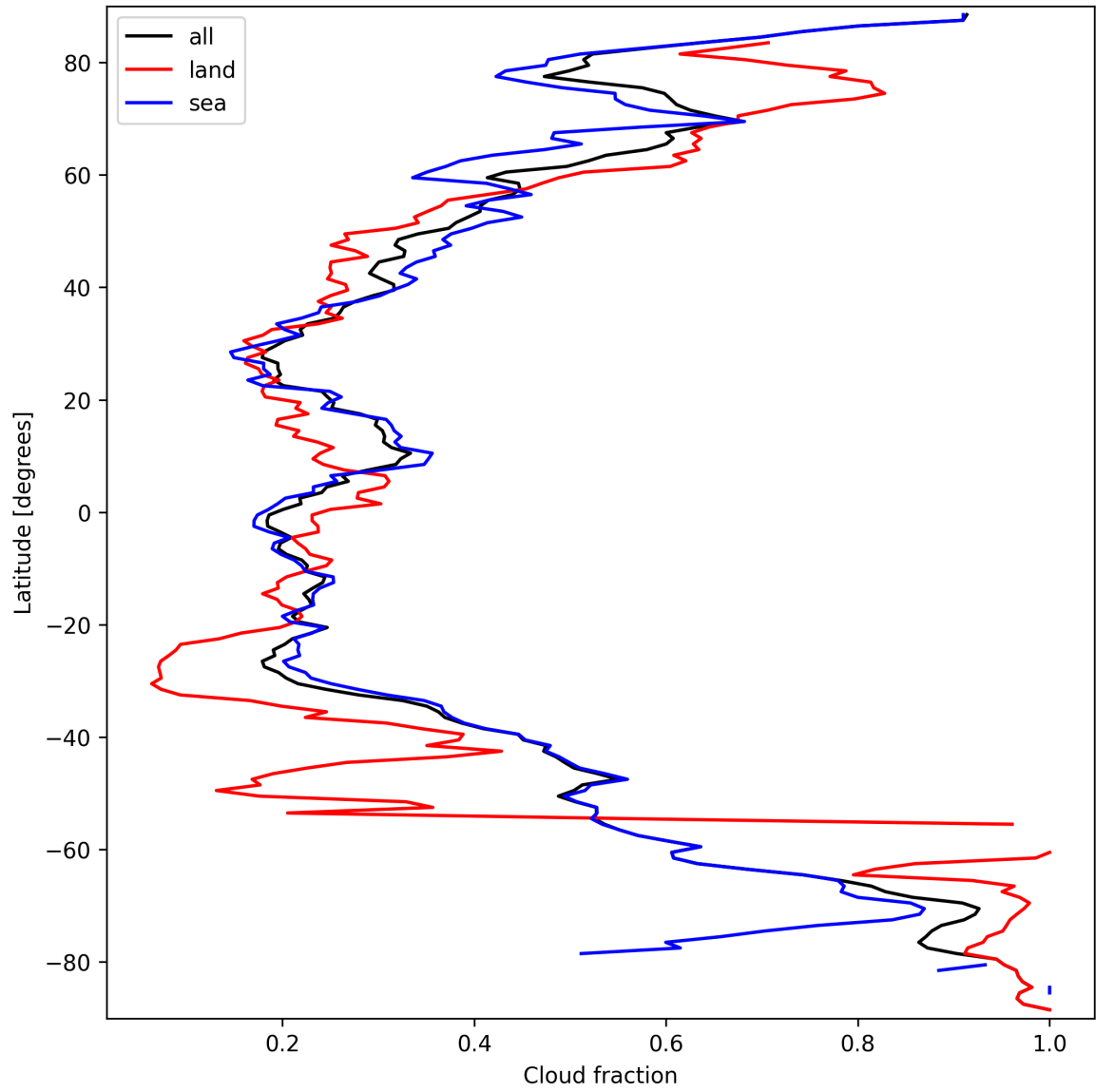
Figure 13: Zonal average of “Cloud fraction” for 2025-09-22 to 2025-09-23.
