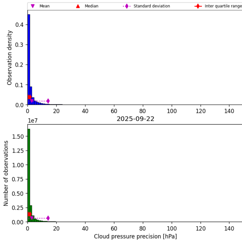
Figure 29: Histogram of “Cloud pressure precision” for 2025-09-22 to 2025-09-23
