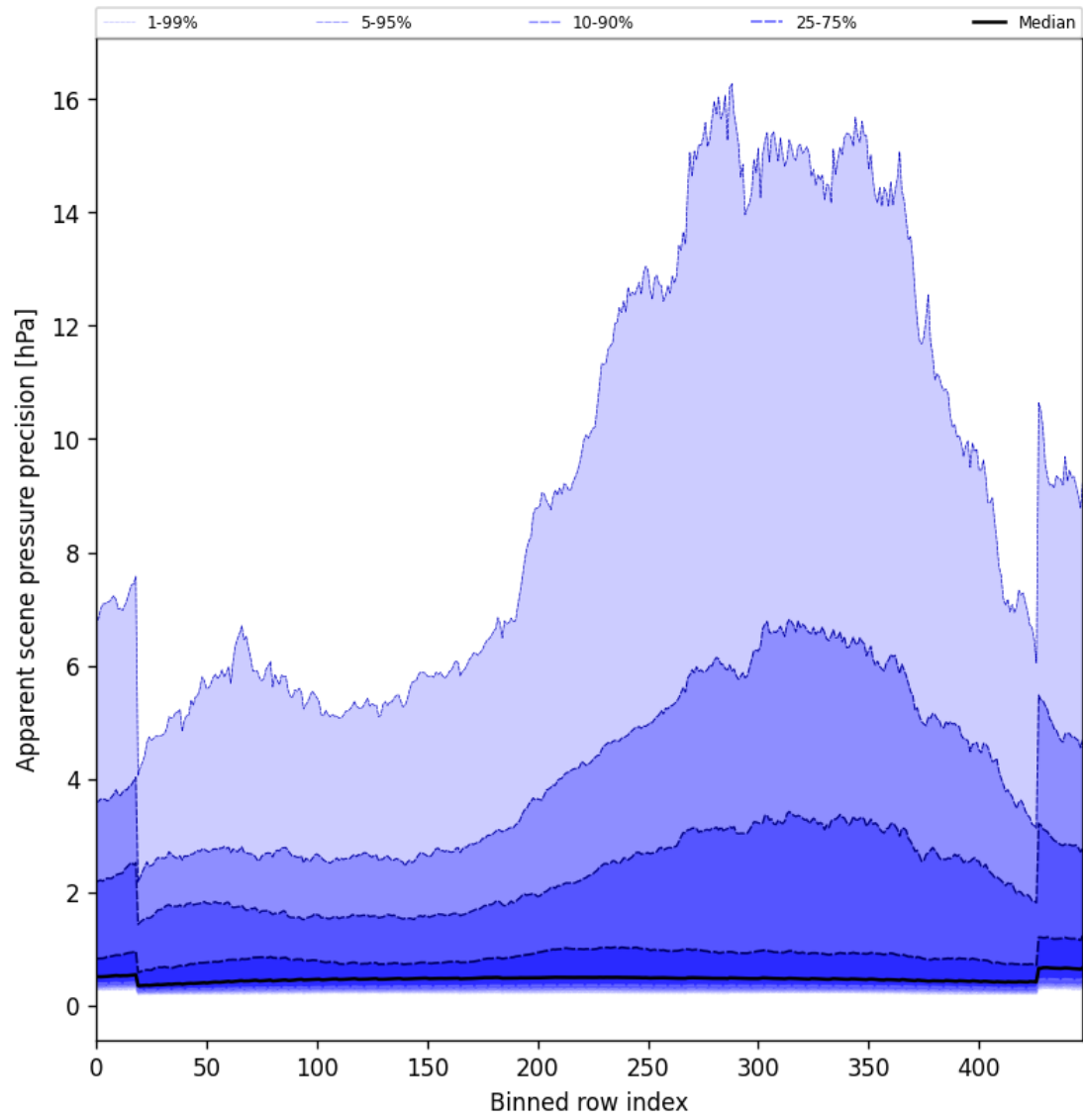
Figure 52: Along track statistics of “Apparent scene pressure precision” for 2025-09-22 to 2025-09-23
