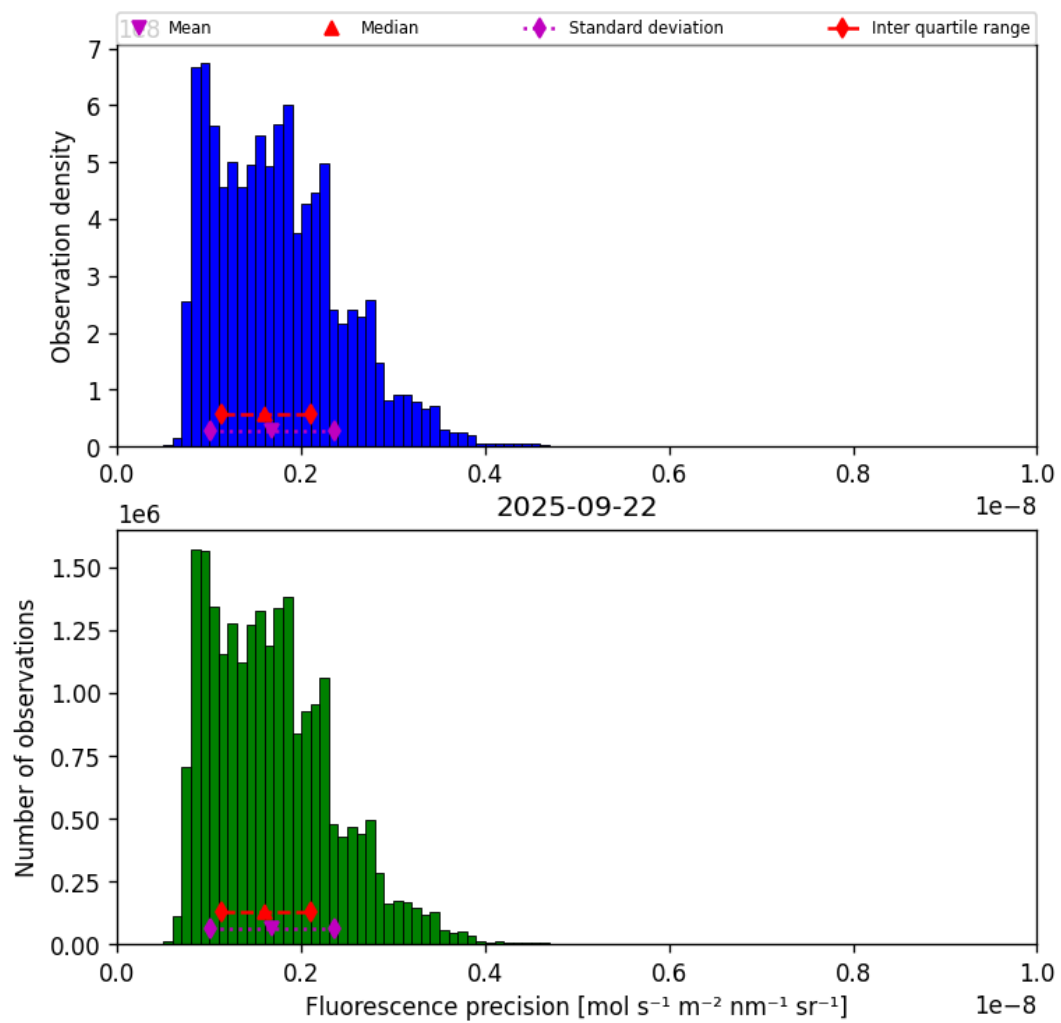
Figure 39: Histogram of “Fluorescence precision” for 2025-09-22 to 2025-09-23
