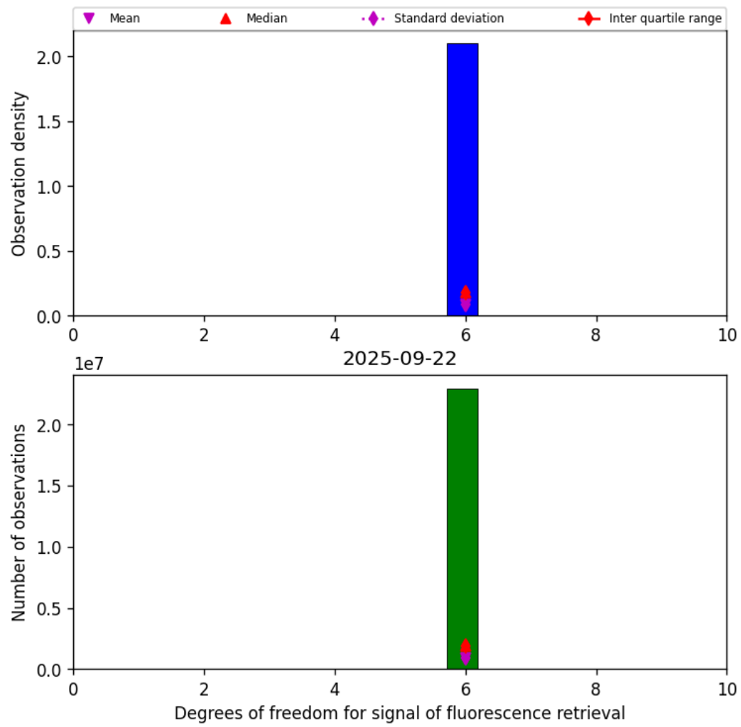
Figure 41: Histogram of “Degrees of freedom for signal of fluorescence retrieval” for 2025-09-22 to 2025-09-23
