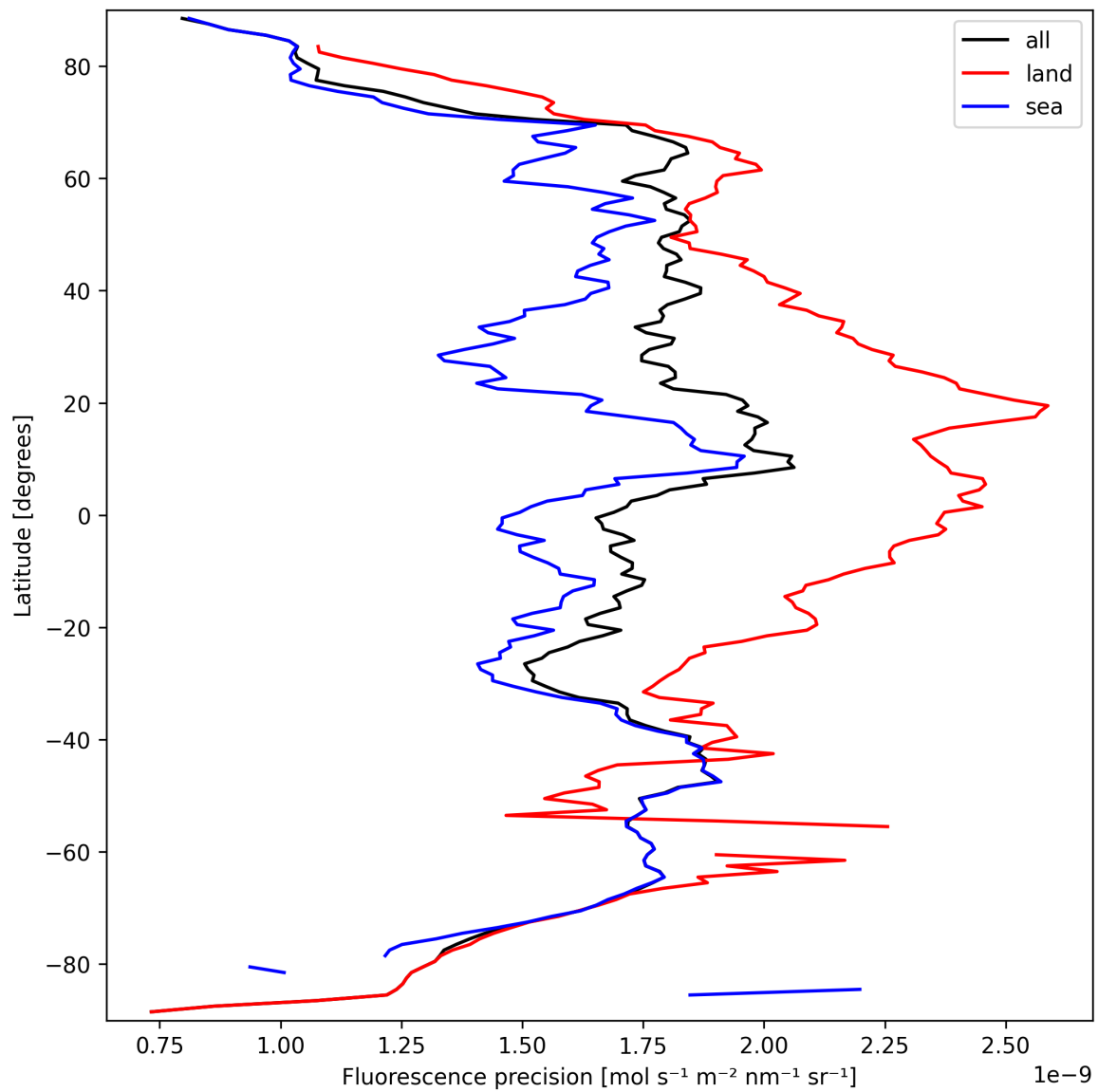
Figure 22: Zonal average of “Fluorescence precision” for 2025-09-22 to 2025-09-23.
