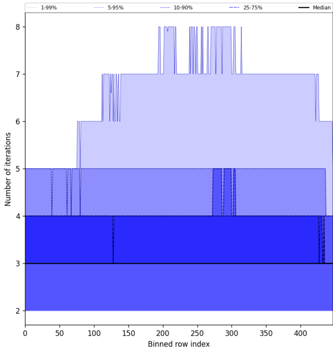
Figure 54: Along track statistics of “Number of iterations” for 2025-09-22 to 2025-09-23
