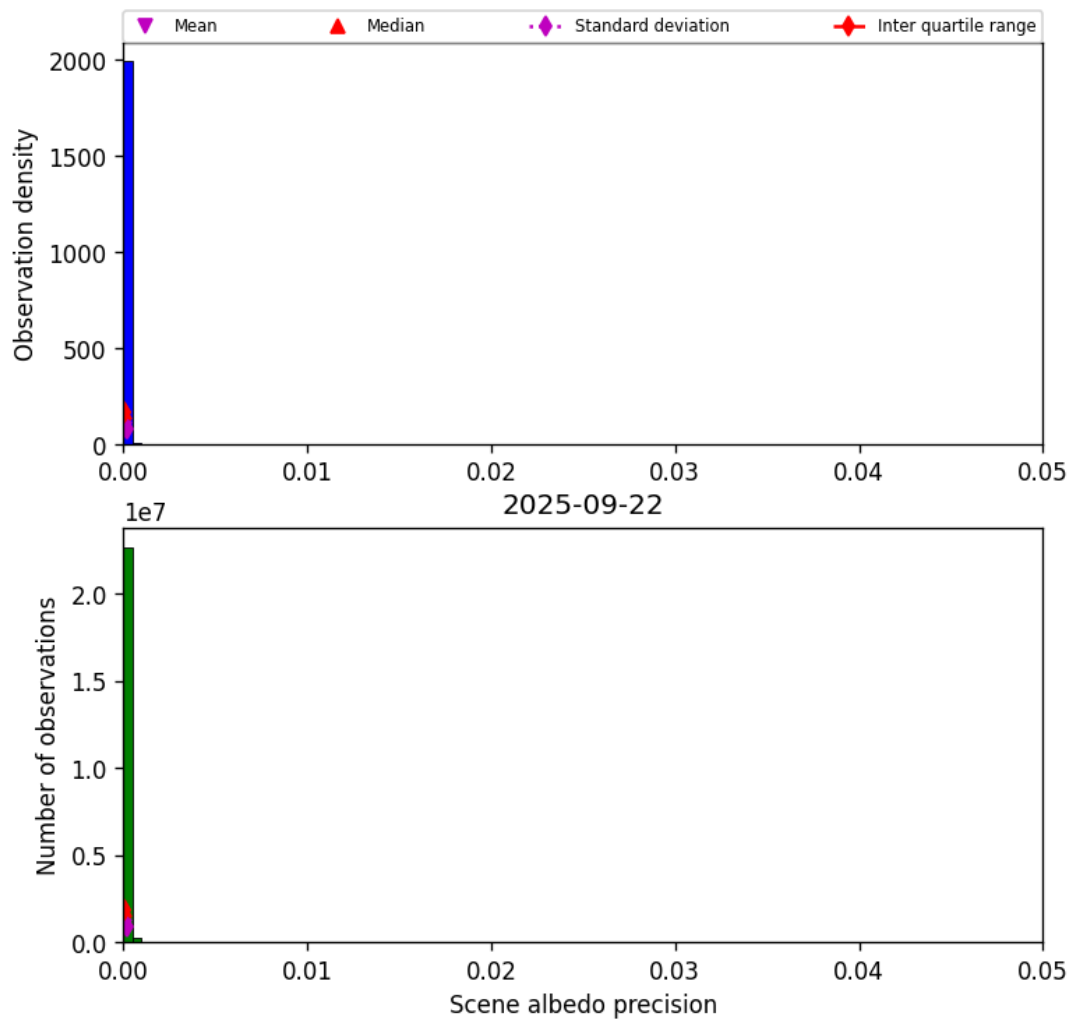
Figure 33: Histogram of “Scene albedo precision” for 2025-09-22 to 2025-09-23
