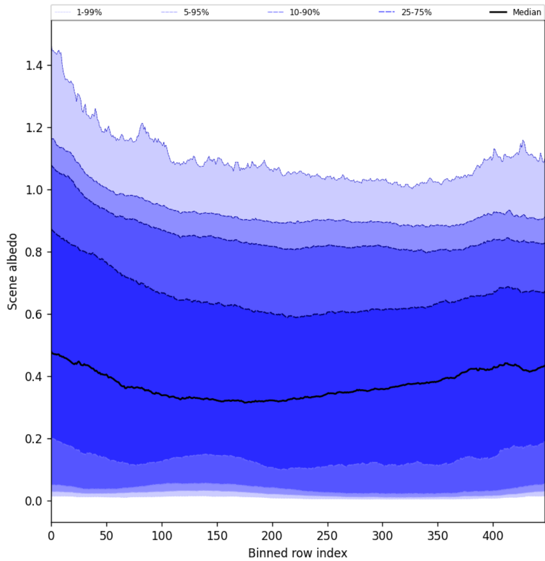
Figure 49: Along track statistics of “Scene albedo” for 2025-09-22 to 2025-09-23
