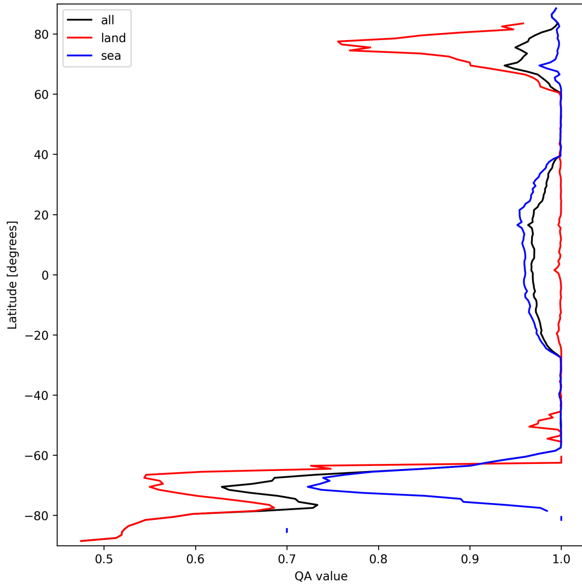
Figure 10: Zonal average of "QA value" for 2025-09-22 to 2025-09-23.
