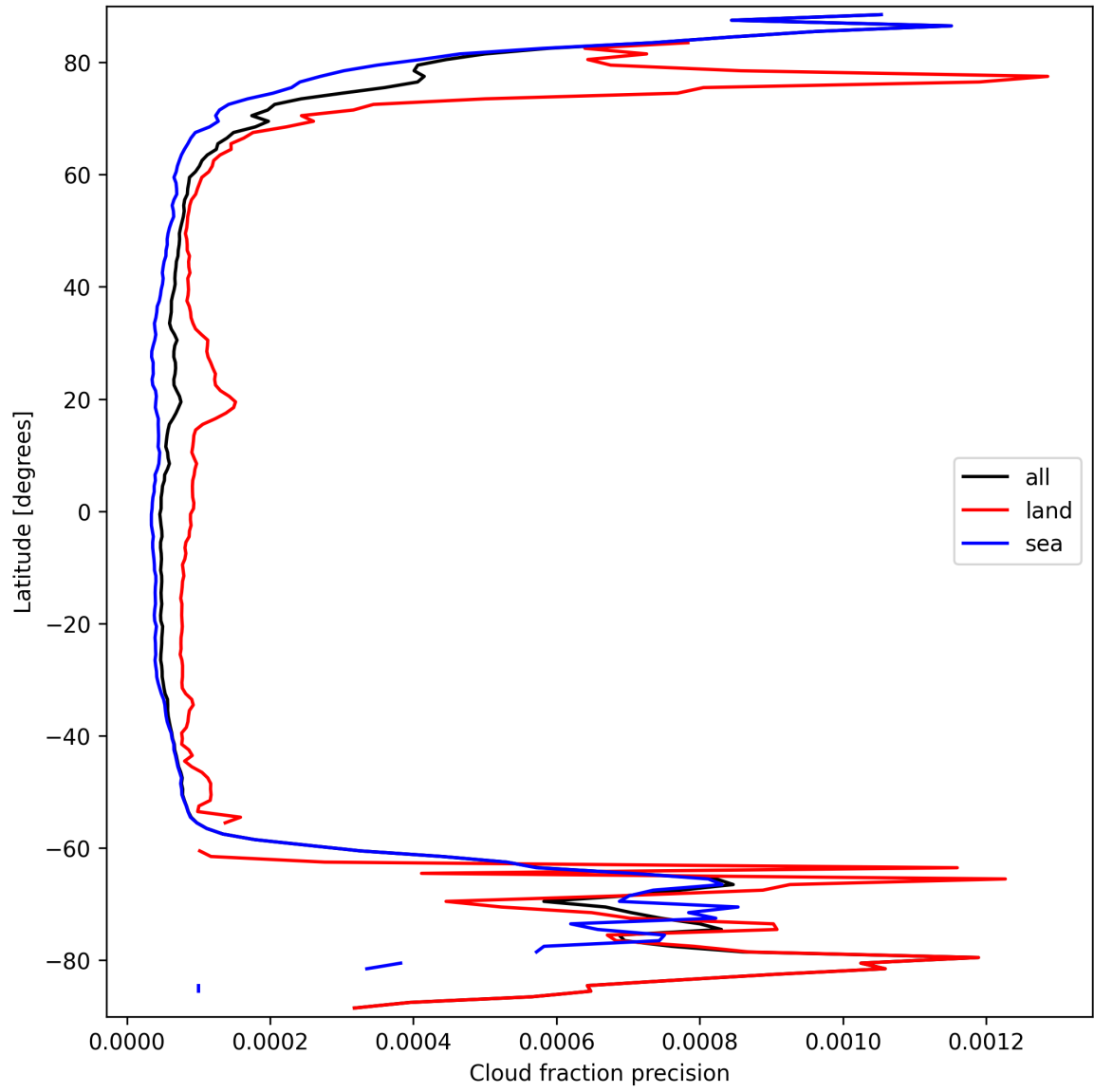
Figure 14: Zonal average of “Cloud fraction precision” for 2025-09-22 to 2025-09-23.
