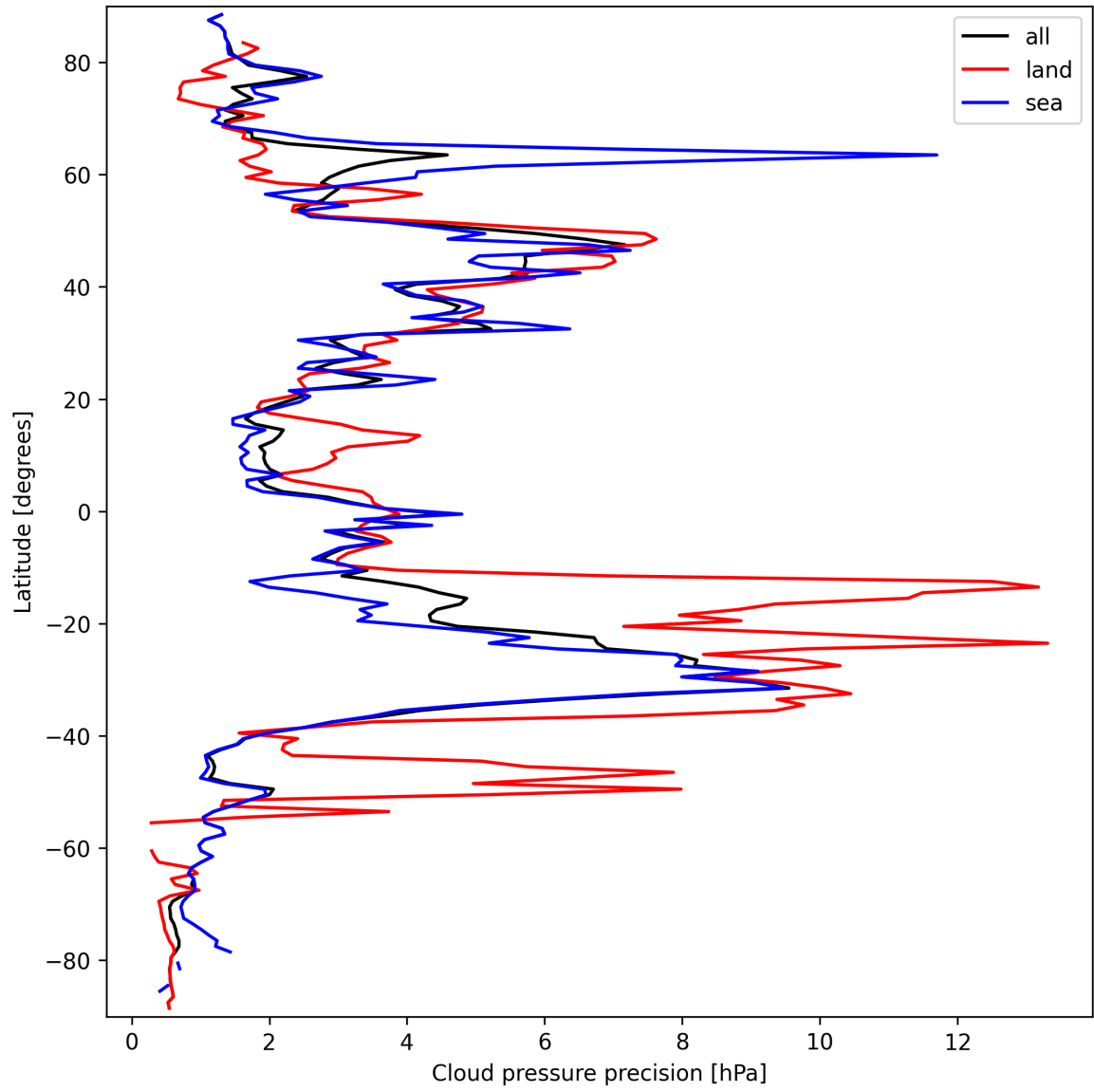
Figure 12: Zonal average of “Cloud pressure precision” for 2025-09-22 to 2025-09-23.
