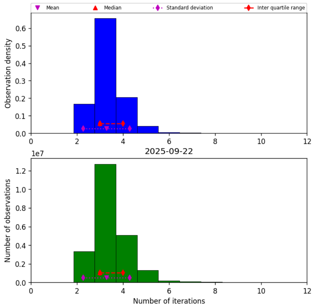
Figure 37: Histogram of “Number of iterations” for 2025-09-22 to 2025-09-23
