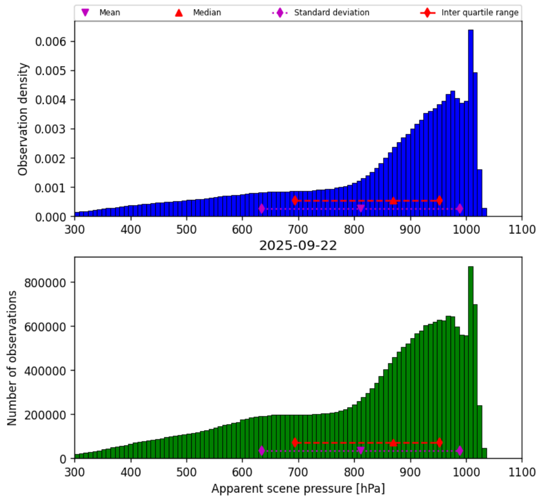
Figure 34: Histogram of “Apparent scene pressure” for 2025-09-22 to 2025-09-23
