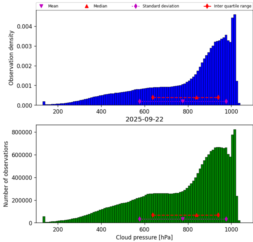
Figure 28: Histogram of “Cloud pressure” for 2025-09-22 to 2025-09-23
