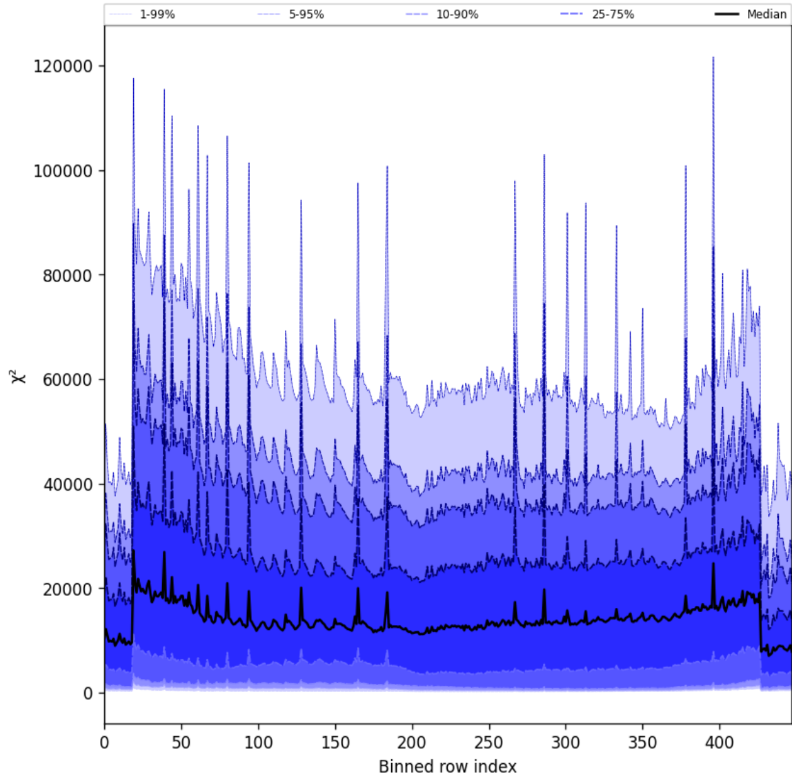
Figure 53: Along track statistics of “ \chi^2 ” for 2025-09-22 to 2025-09-23
