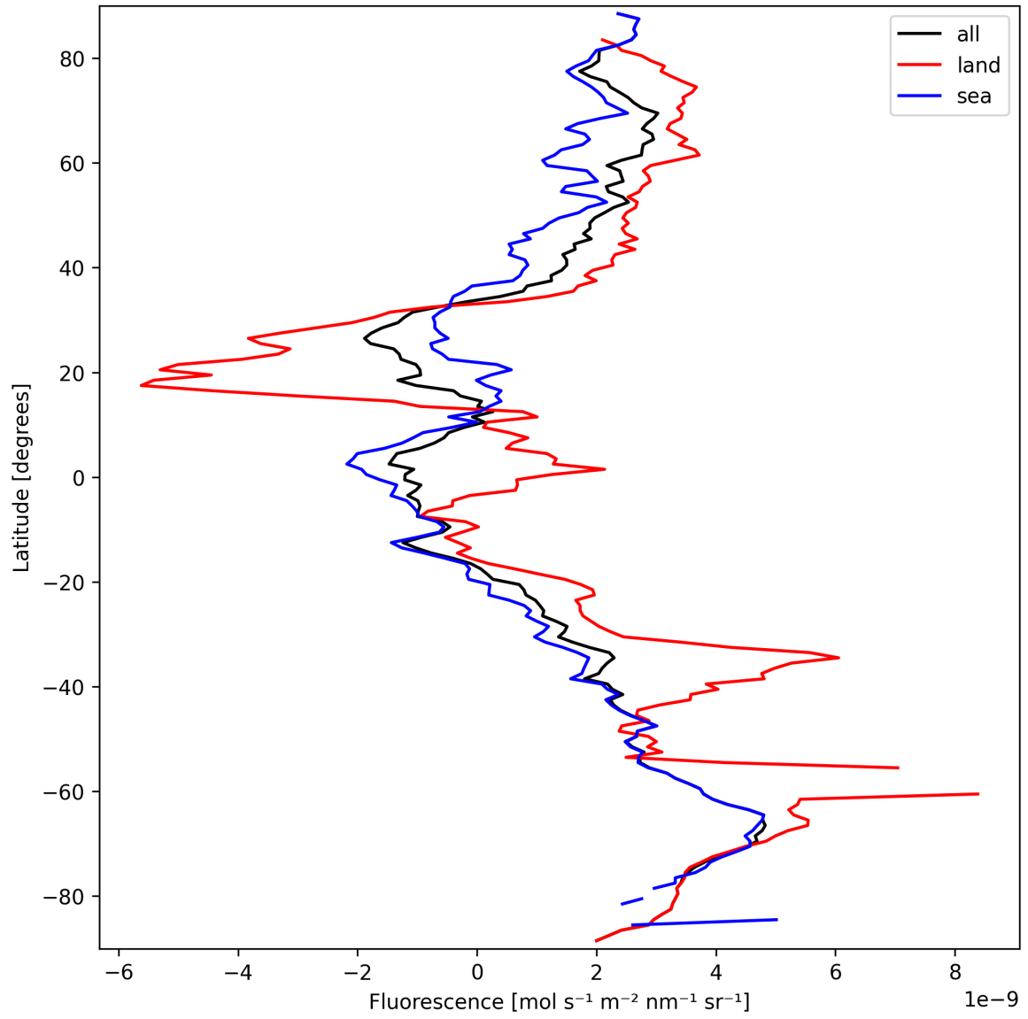
Figure 21: Zonal average of “Fluorescence” for 2025-09-22 to 2025-09-23.
