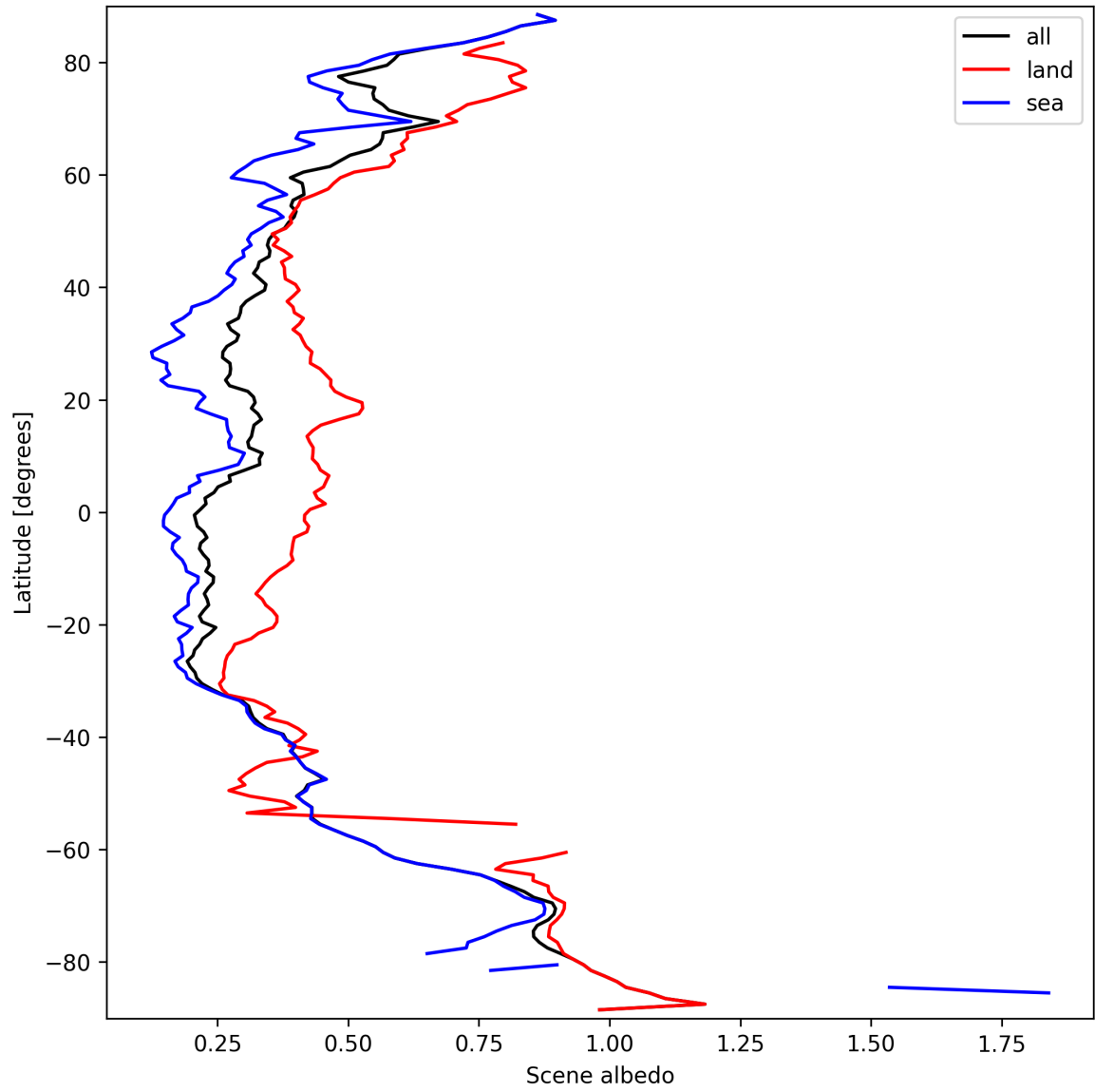
Figure 15: Zonal average of “Scene albedo” for 2025-09-22 to 2025-09-23.
