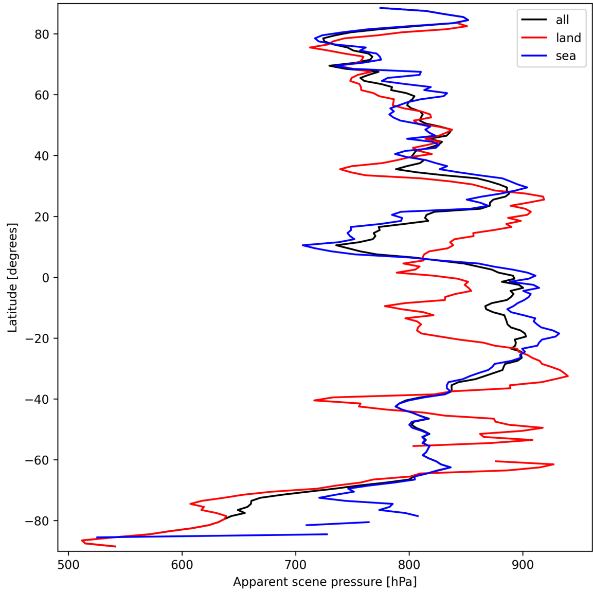
Figure 17: Zonal average of “Apparent scene pressure” for 2025-09-22 to 2025-09-23.
