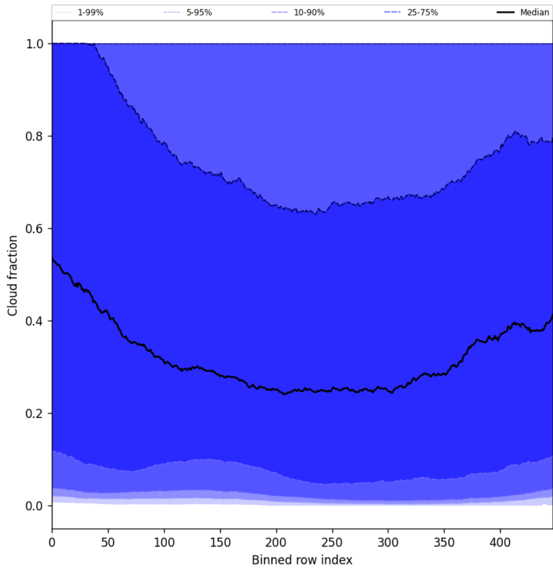
Figure 47: Along track statistics of “Cloud fraction” for 2025-09-22 to 2025-09-23
