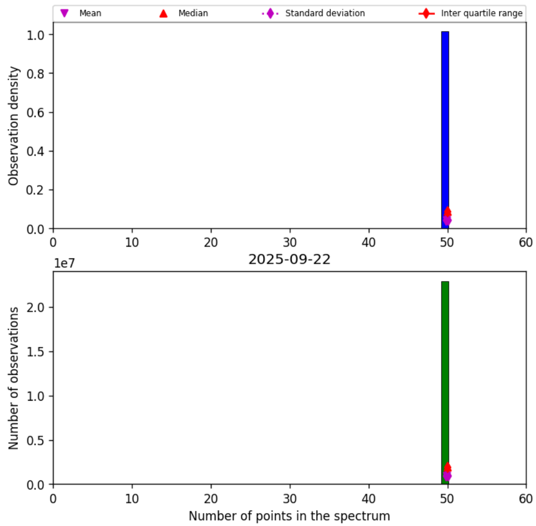
Figure 42: Histogram of “Number of points in the spectrum” for 2025-09-22 to 2025-09-23
