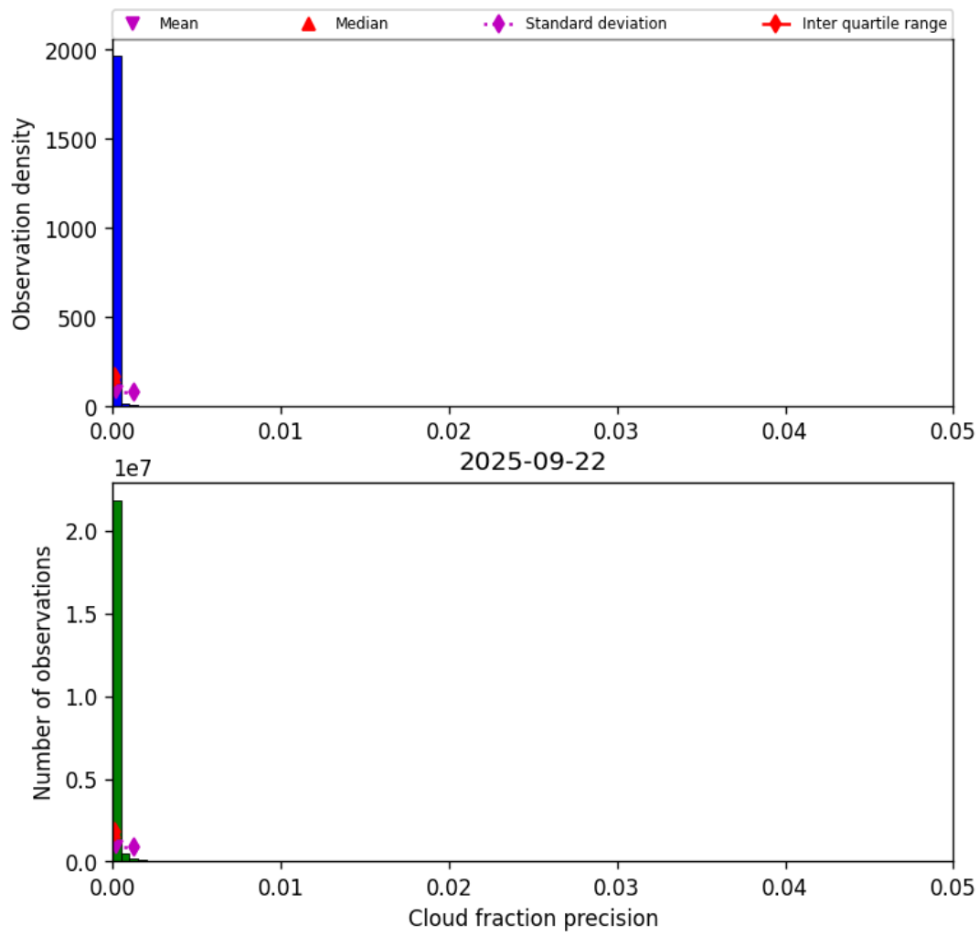
Figure 31: Histogram of “Cloud fraction precision” for 2025-09-22 to 2025-09-23
