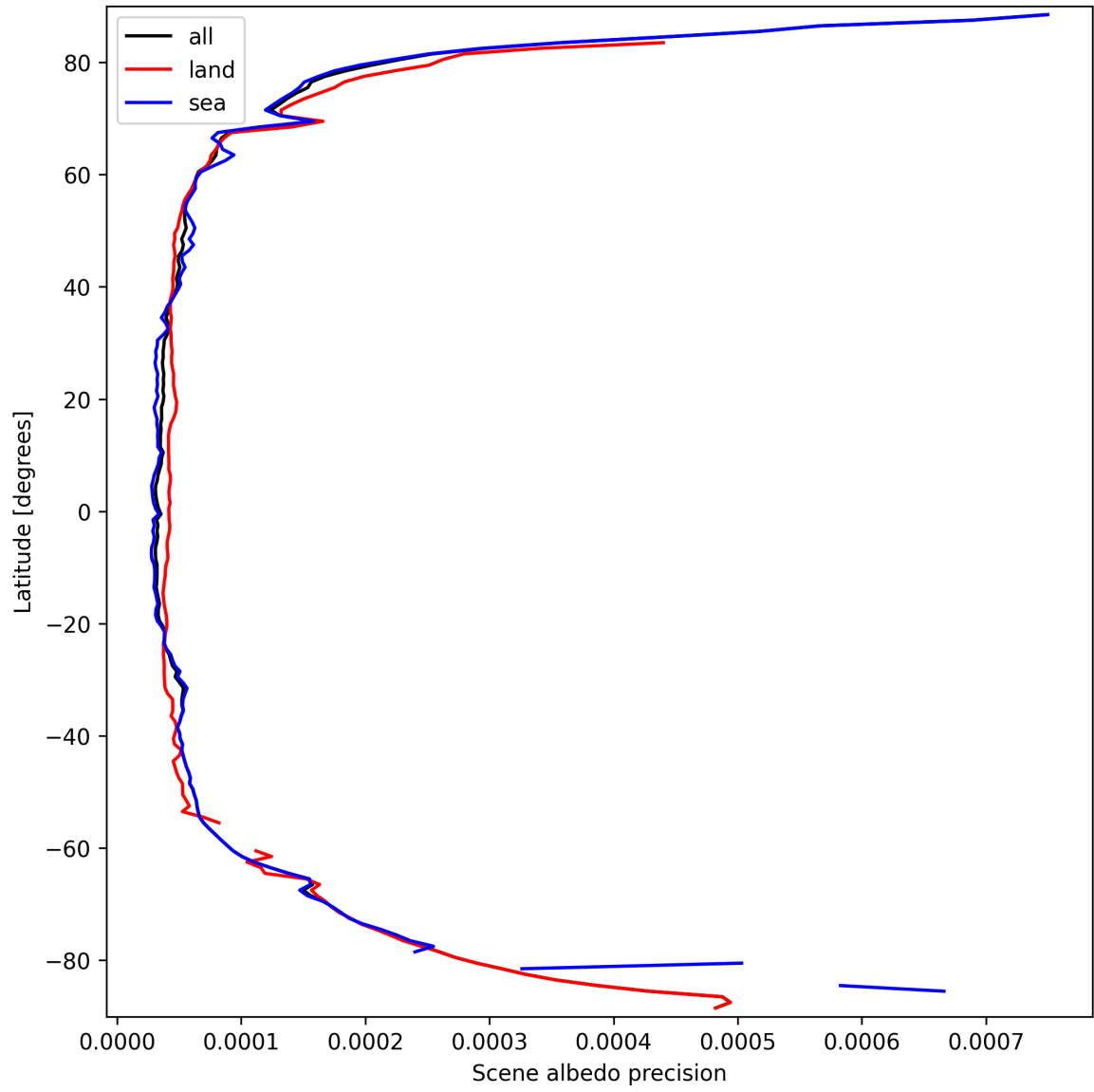
Figure 16: Zonal average of “Scene albedo precision” for 2025-09-22 to 2025-09-23.
