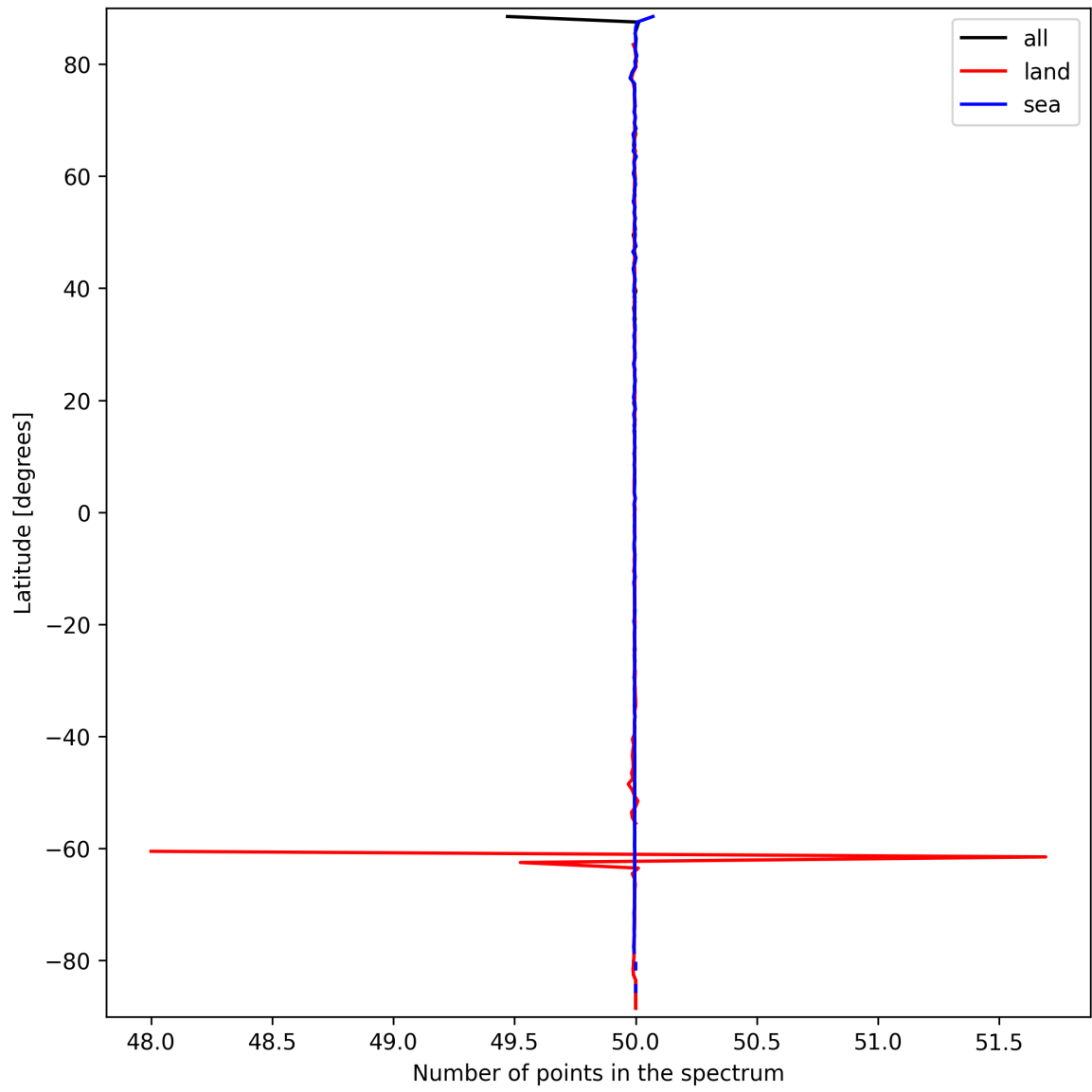
Figure 25: Zonal average of “Number of points in the spectrum” for 2025-09-22 to 2025-09-23.
