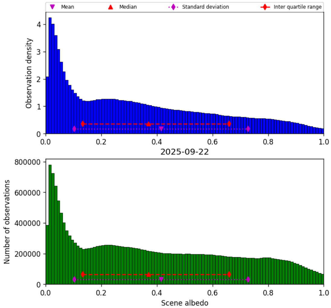
Figure 32: Histogram of “Scene albedo” for 2025-09-22 to 2025-09-23
