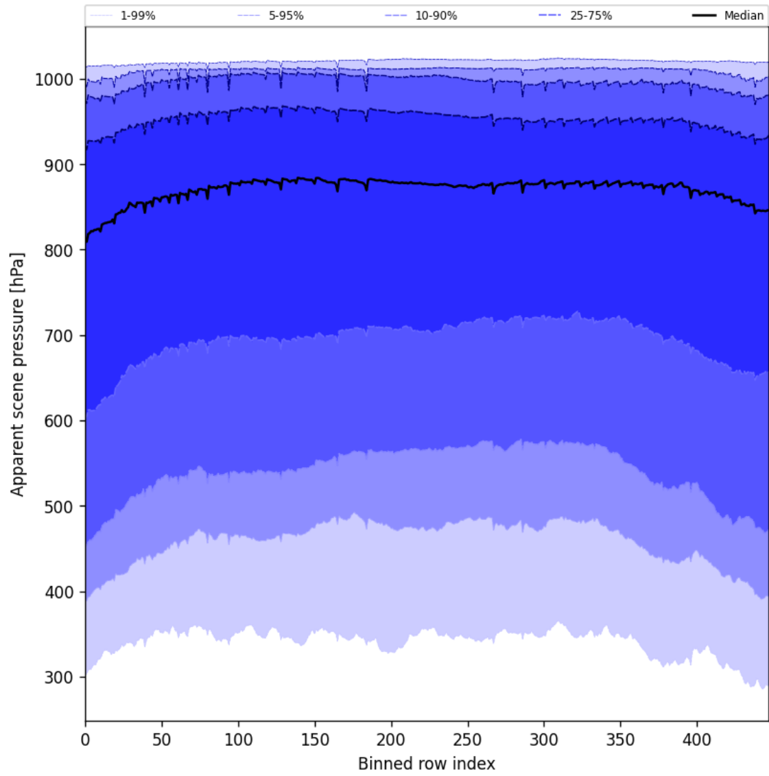
Figure 51: Along track statistics of “Apparent scene pressure” for 2025-09-22 to 2025-09-23
