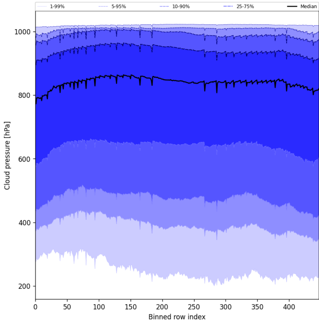
Figure 45: Along track statistics of “Cloud pressure” for 2025-09-22 to 2025-09-23
