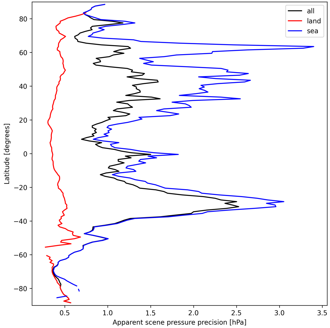
Figure 18: Zonal average of “Apparent scene pressure precision” for 2025-09-22 to 2025-09-23.
