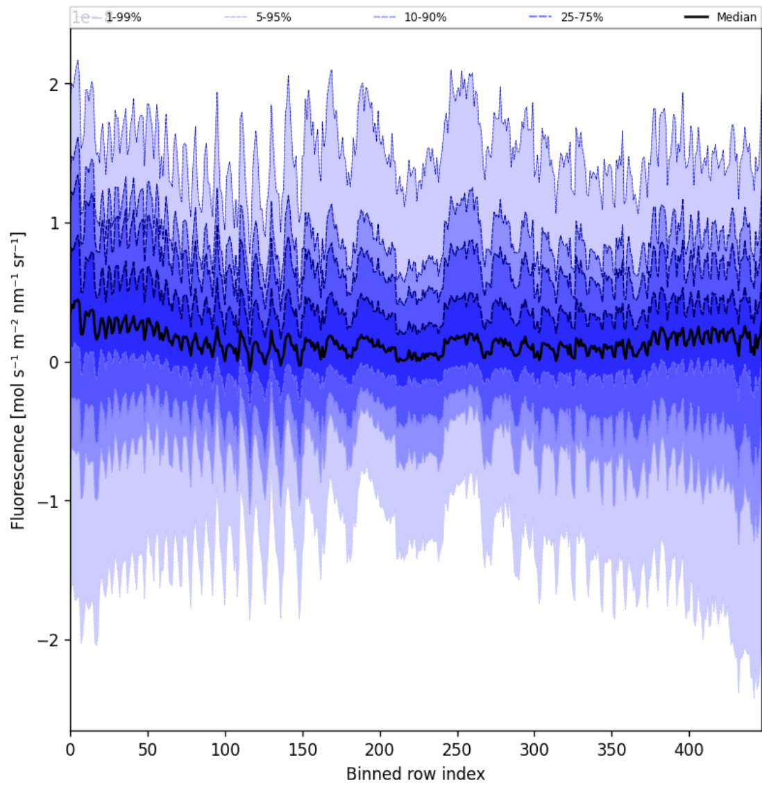
Figure 55: Along track statistics of “Fluorescence” for 2025-09-22 to 2025-09-23
