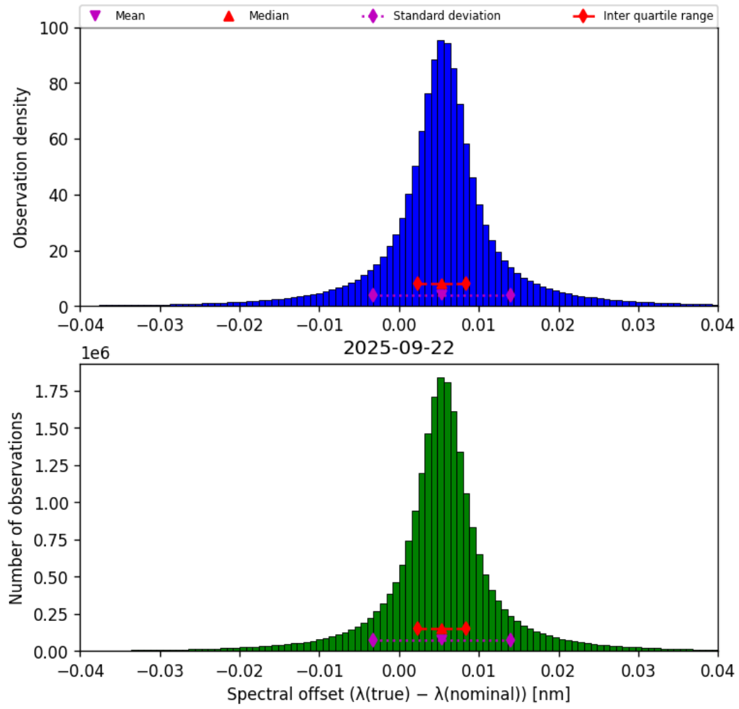
Figure 43: Histogram of “Spectral offset ( \lambda_{\text{true}} - \lambda_{\text{nominal}} )” for 2025-09-22 to 2025-09-23
