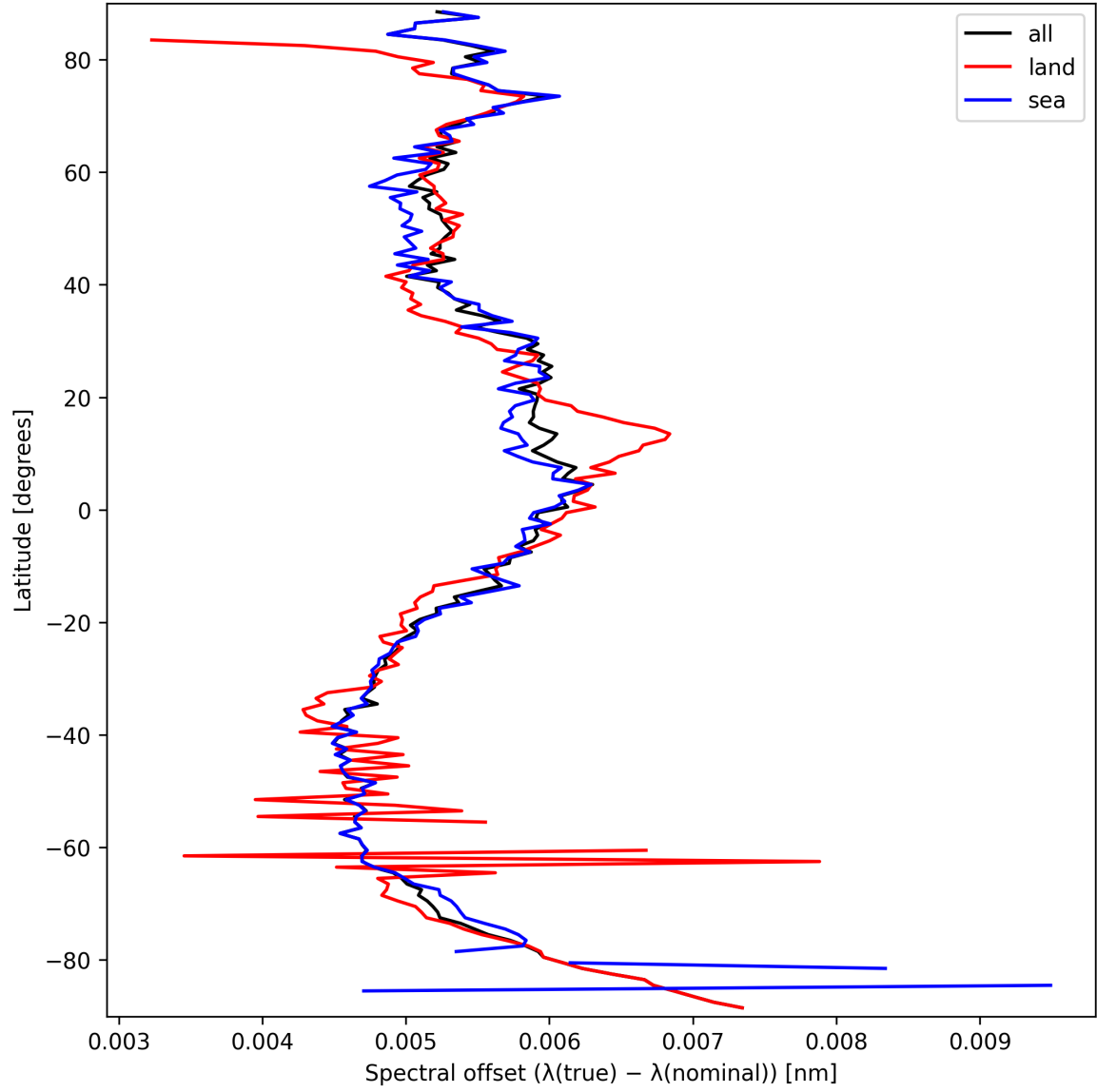
Figure 26: Zonal average of “Spectral offset ( \lambda_{\text{true}} - \lambda_{\text{nominal}} )” for 2025-09-22 to 2025-09-23.
