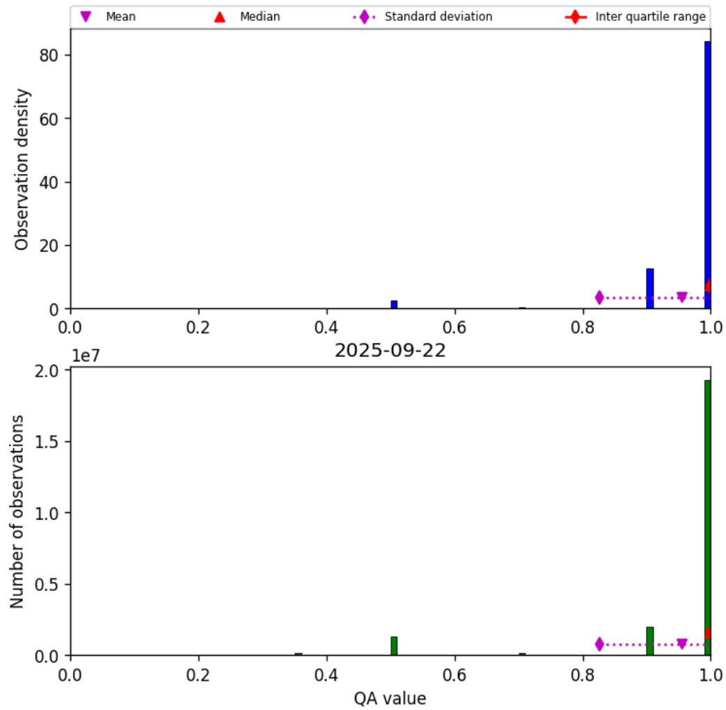
Figure 27: Histogram of “QA value” for 2025-09-22 to 2025-09-23
