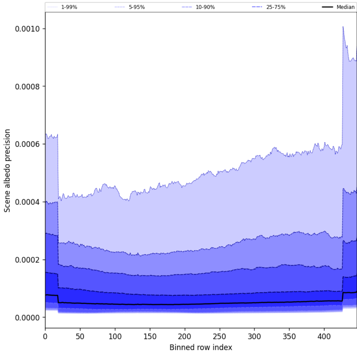
Figure 50: Along track statistics of “Scene albedo precision” for 2025-09-22 to 2025-09-23
