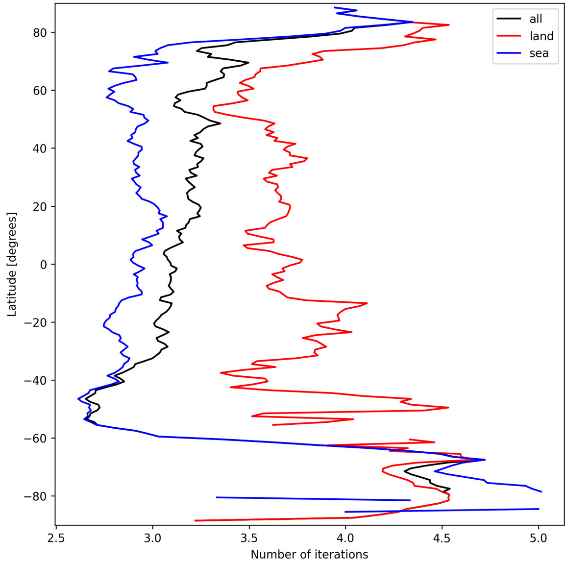
Figure 20: Zonal average of “Number of iterations” for 2025-09-22 to 2025-09-23.
