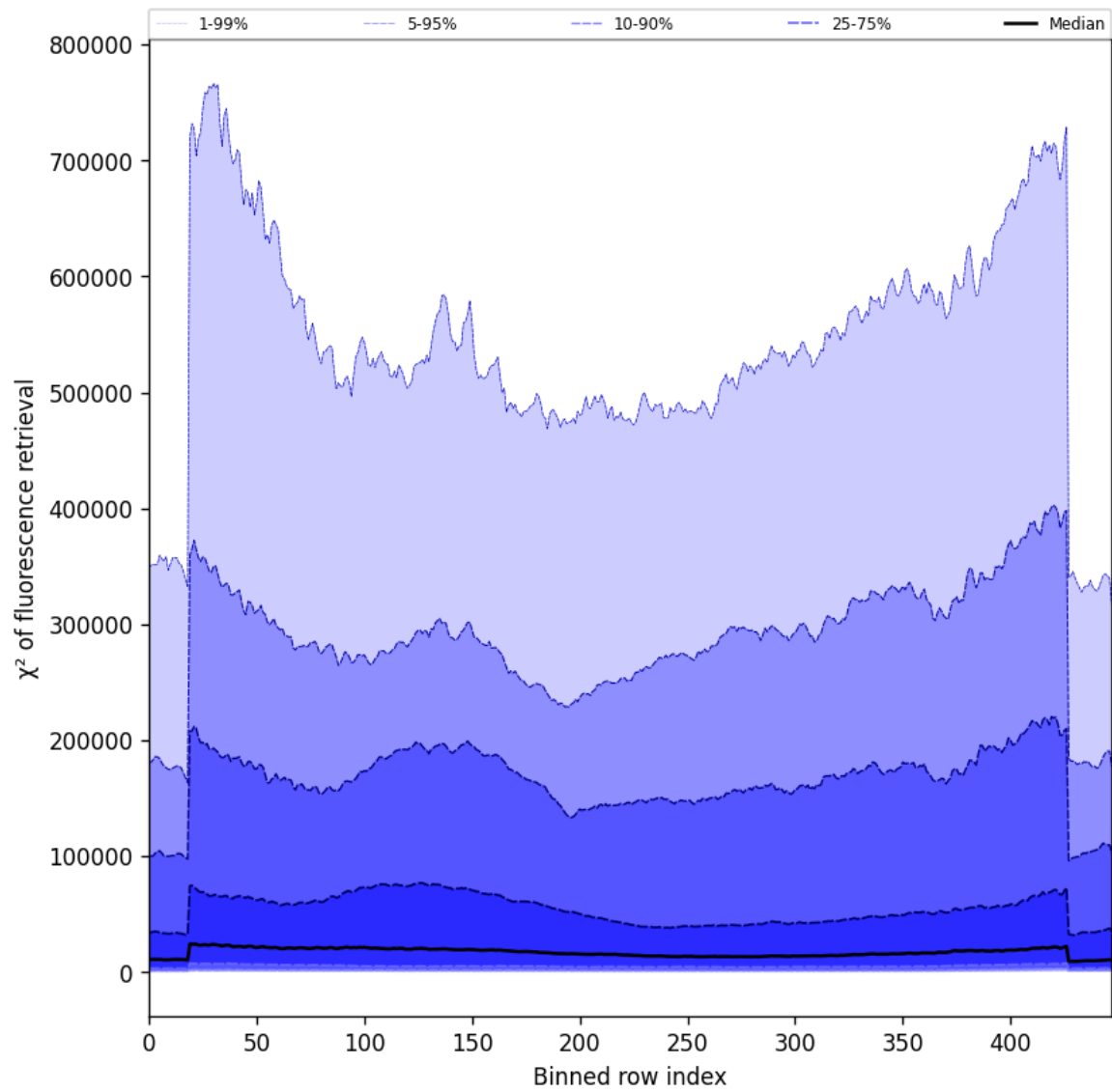
Figure 57: Along track statistics of “ \chi^2 of fluorescence retrieval” for 2025-09-22 to 2025-09-23
