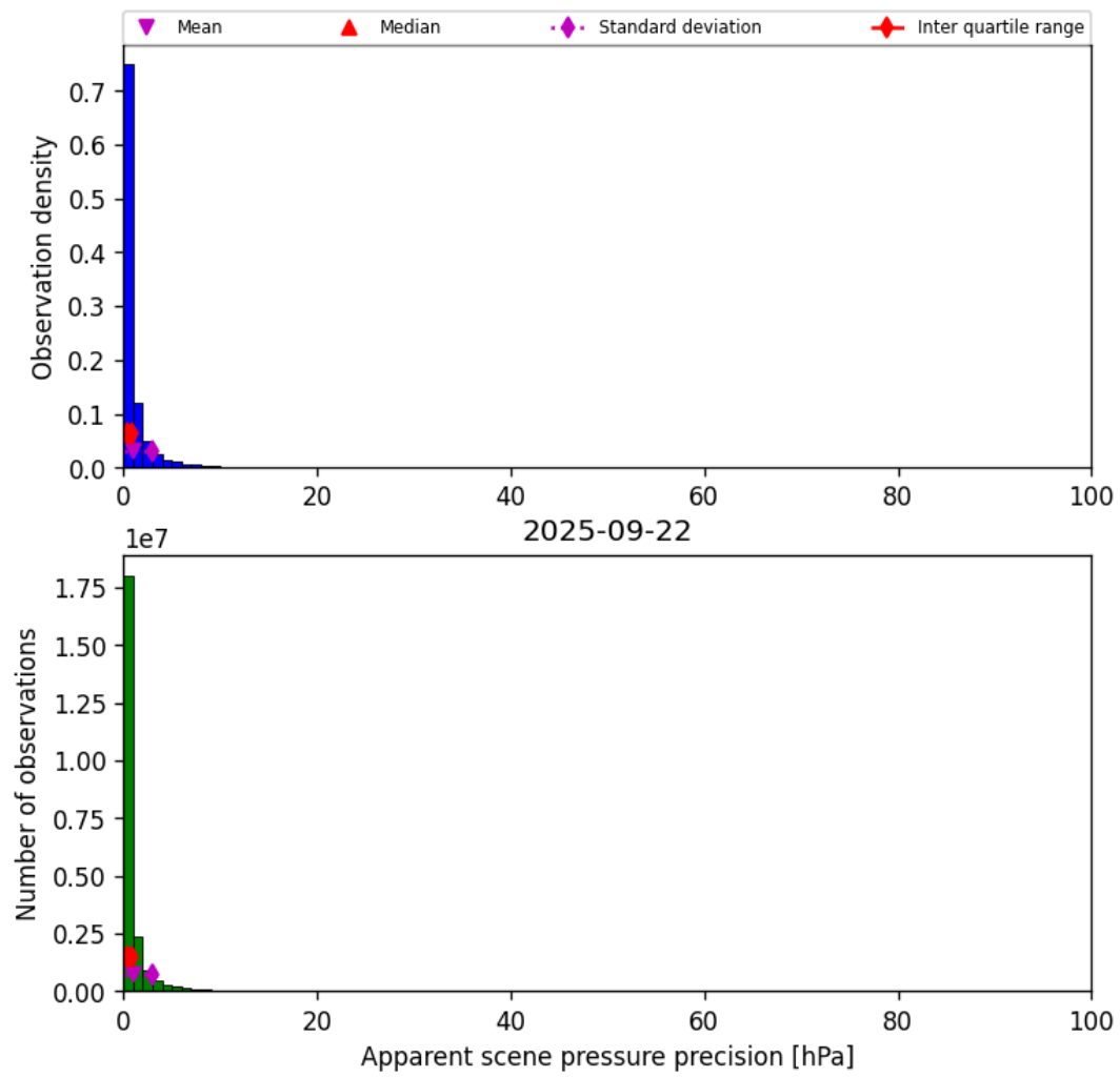
Figure 35: Histogram of “Apparent scene pressure precision” for 2025-09-22 to 2025-09-23
