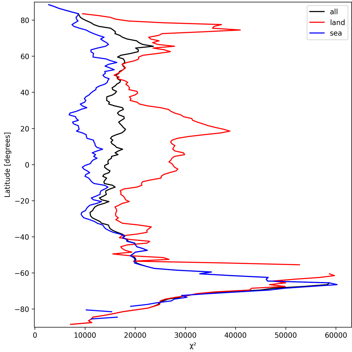
Figure 19: Zonal average of “ \chi^2 ” for 2025-09-22 to 2025-09-23.
