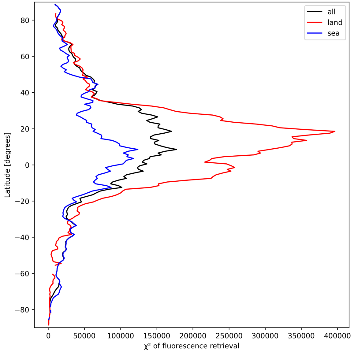
Figure 23: Zonal average of “ \chi^2 of fluorescence retrieval” for 2025-09-22 to 2025-09-23.
