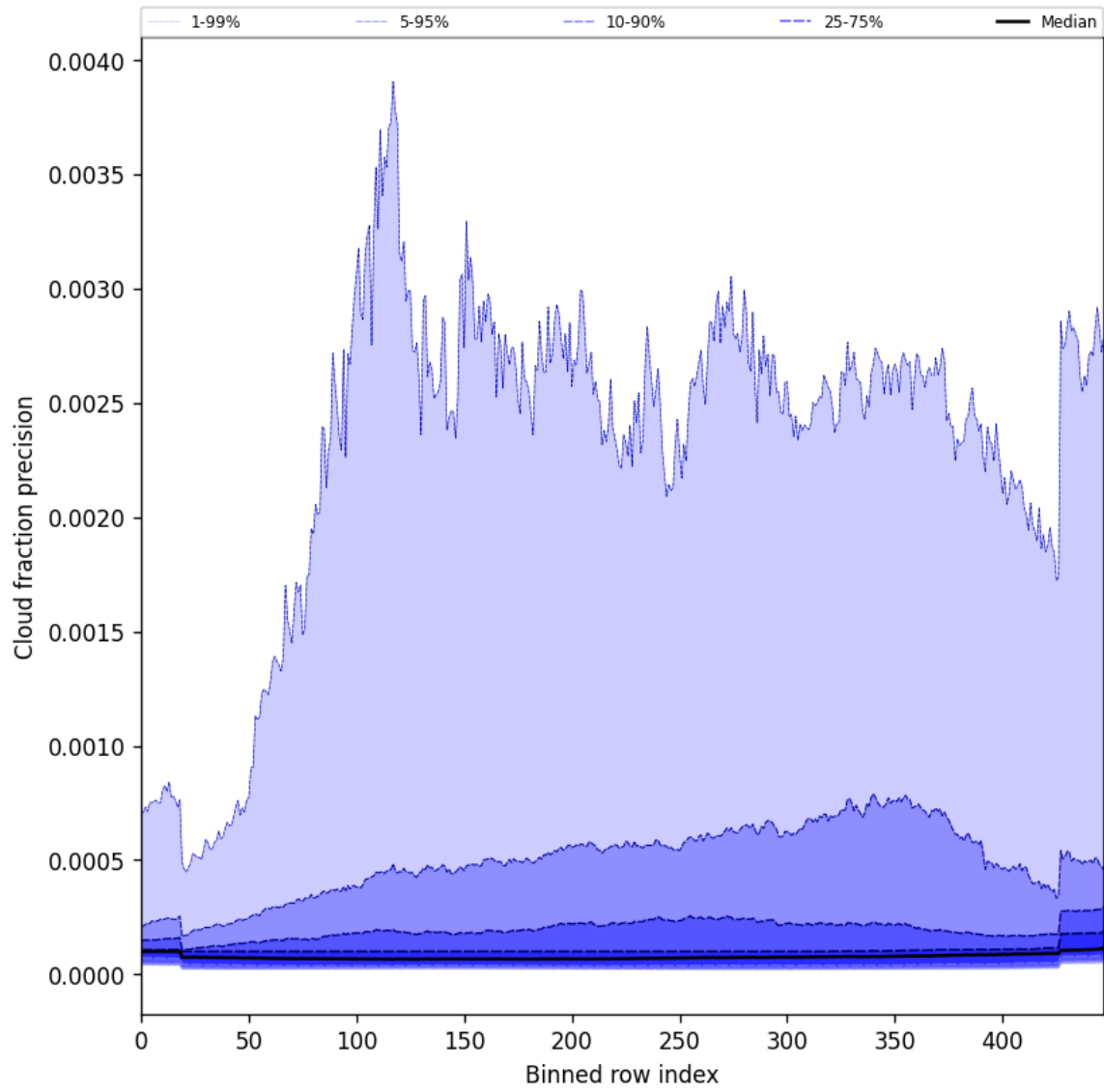
Figure 48: Along track statistics of “Cloud fraction precision” for 2025-09-22 to 2025-09-23
