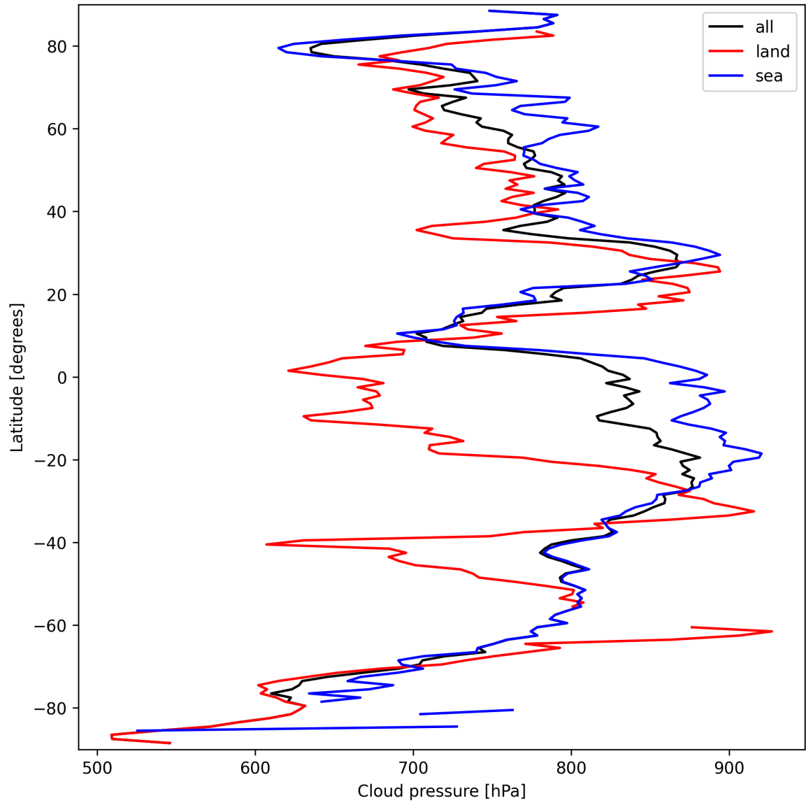
Figure 11: Zonal average of “Cloud pressure” for 2025-09-22 to 2025-09-23.
