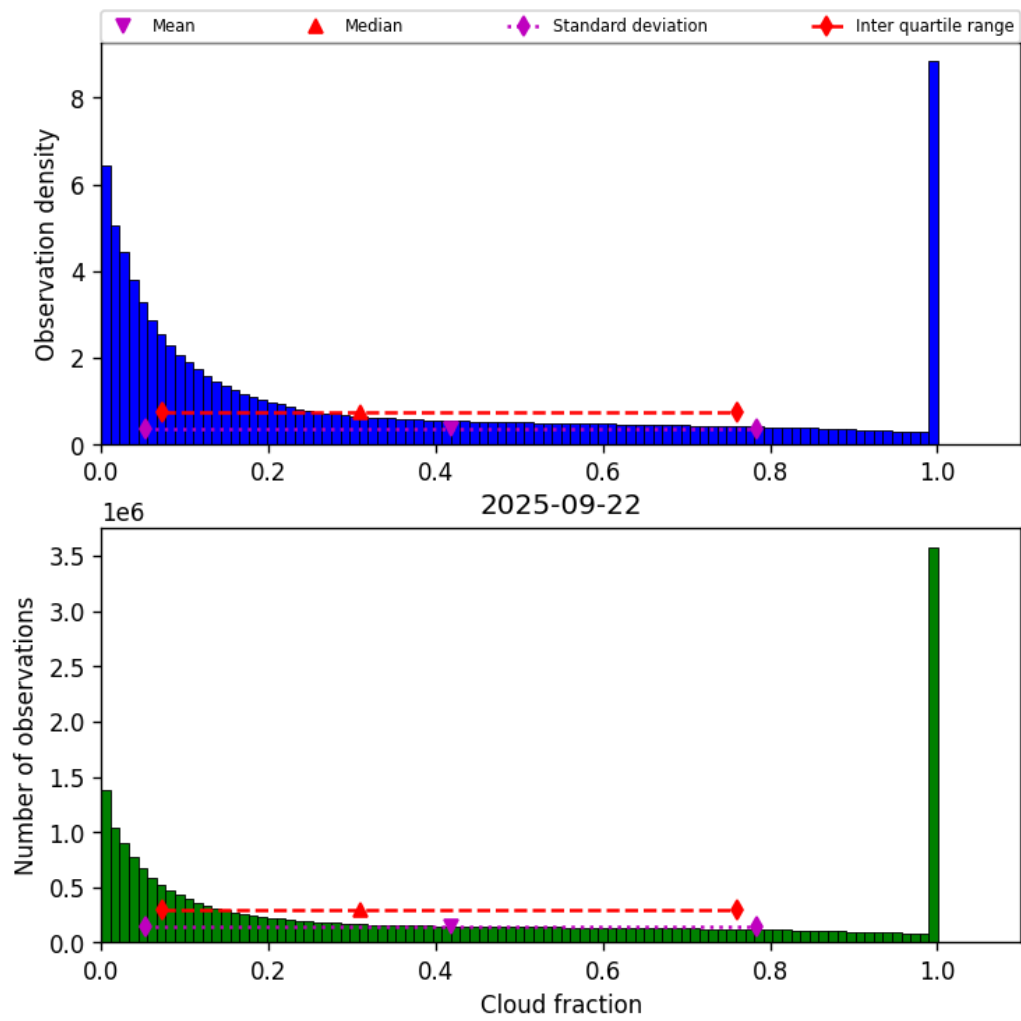
Figure 30: Histogram of “Cloud fraction” for 2025-09-22 to 2025-09-23
