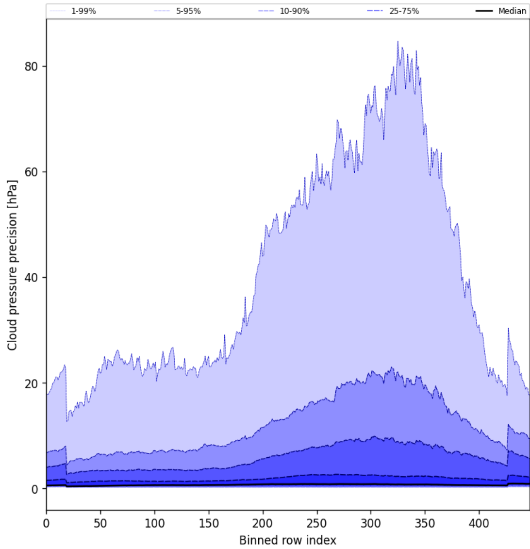
Figure 46: Along track statistics of “Cloud pressure precision” for 2025-09-22 to 2025-09-23
