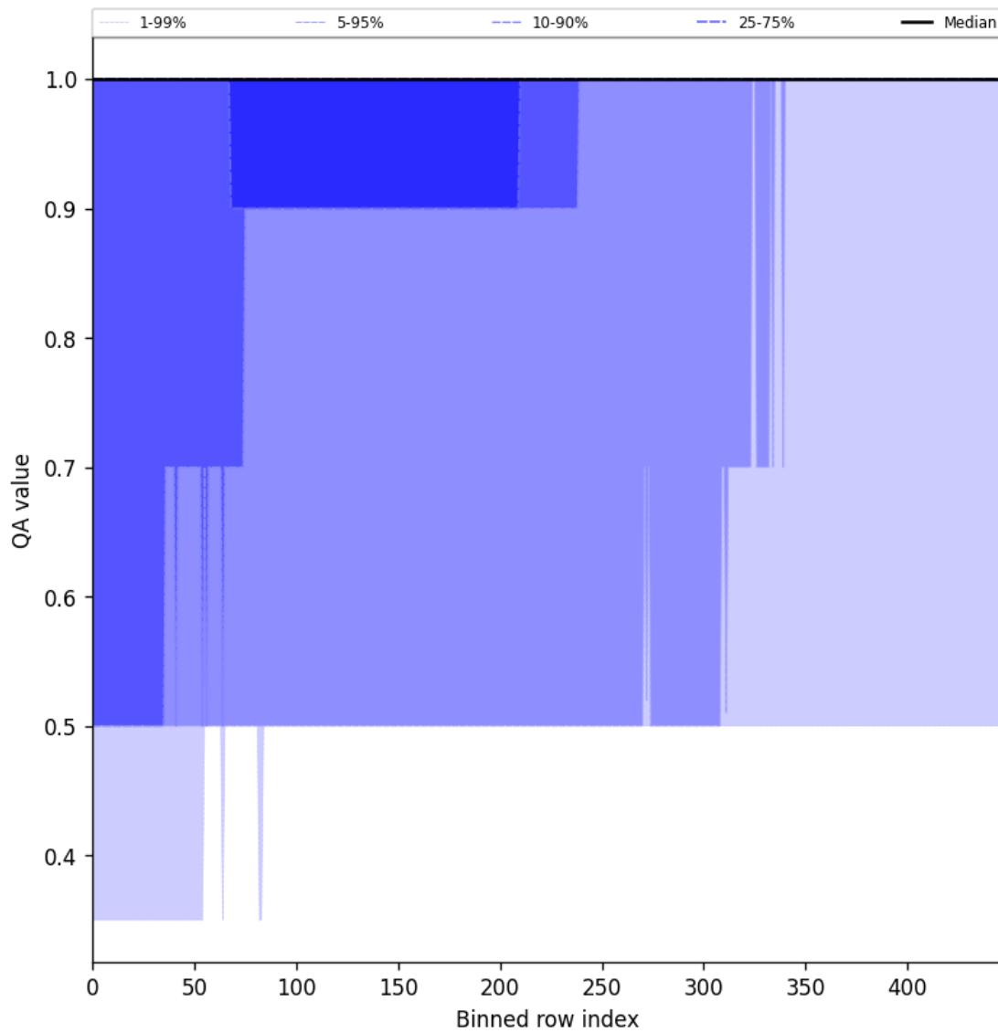
Figure 44: Along track statistics of “QA value” for 2025-09-22 to 2025-09-23
