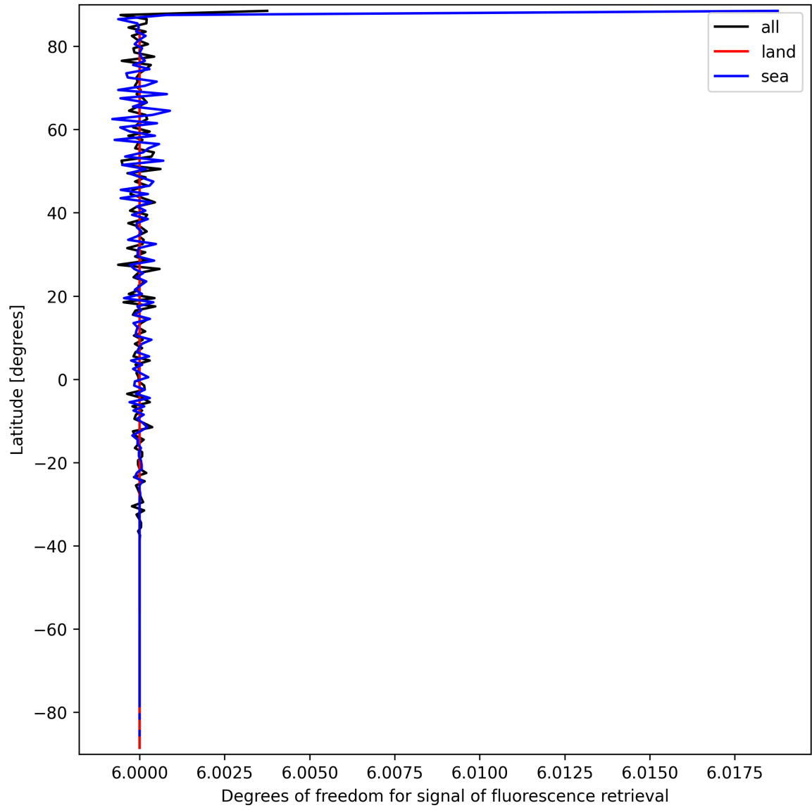
Figure 24: Zonal average of “Degrees of freedom for signal of fluorescence retrieval” for 2025-09-22 to 2025-09-23.
