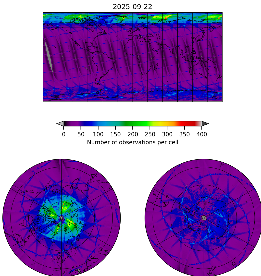
Figure 9: Map of the number of observations for 2025-09-22 to 2025-09-23
