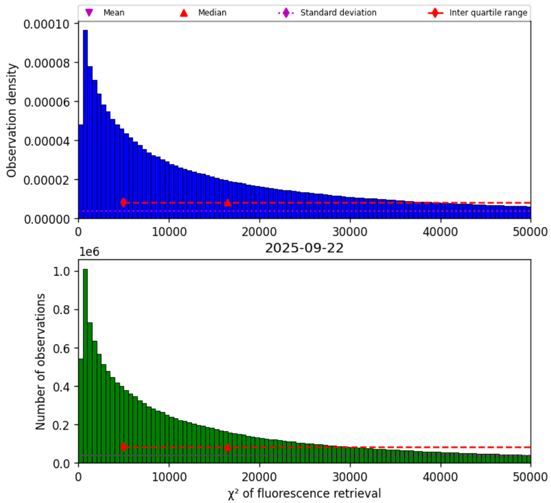
Figure 40: Histogram of “ \chi^2 of fluorescence retrieval” for 2025-09-22 to 2025-09-23
