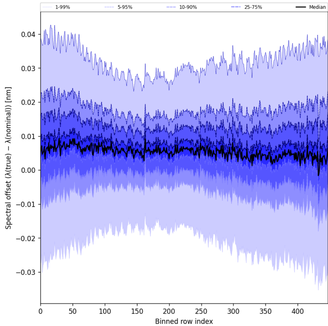
Figure 60: Along track statistics of “Spectral offset ( \lambda_{\text{true}} - \lambda_{\text{nominal}} )” for 2025-09-22 to 2025-09-23
