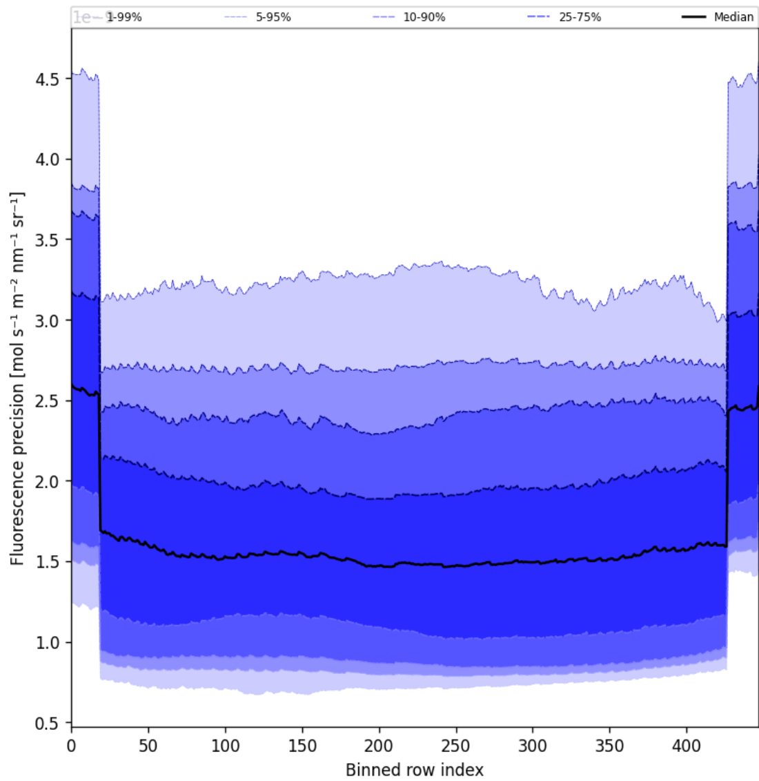
Figure 56: Along track statistics of “Fluorescence precision” for 2025-09-22 to 2025-09-23
