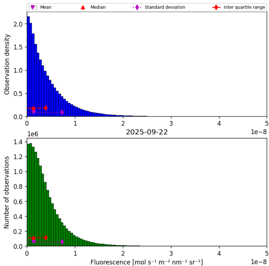
Figure 38: Histogram of “Fluorescence” for 2025-09-22 to 2025-09-23
