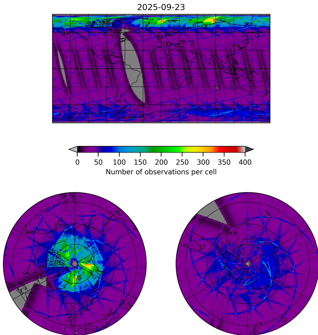
Figure 9: Map of the number of observations for 2025-09-23 to 2025-09-23
