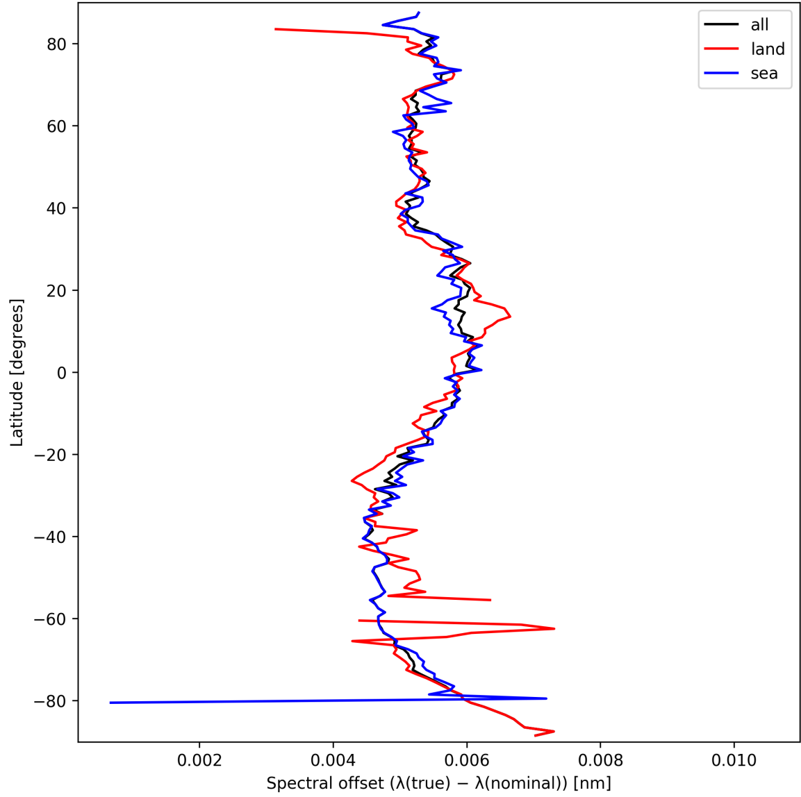
Figure 26: Zonal average of “Spectral offset ( \lambda_{\text{true}} - \lambda_{\text{nominal}} )” for 2025-09-23 to 2025-09-23.
