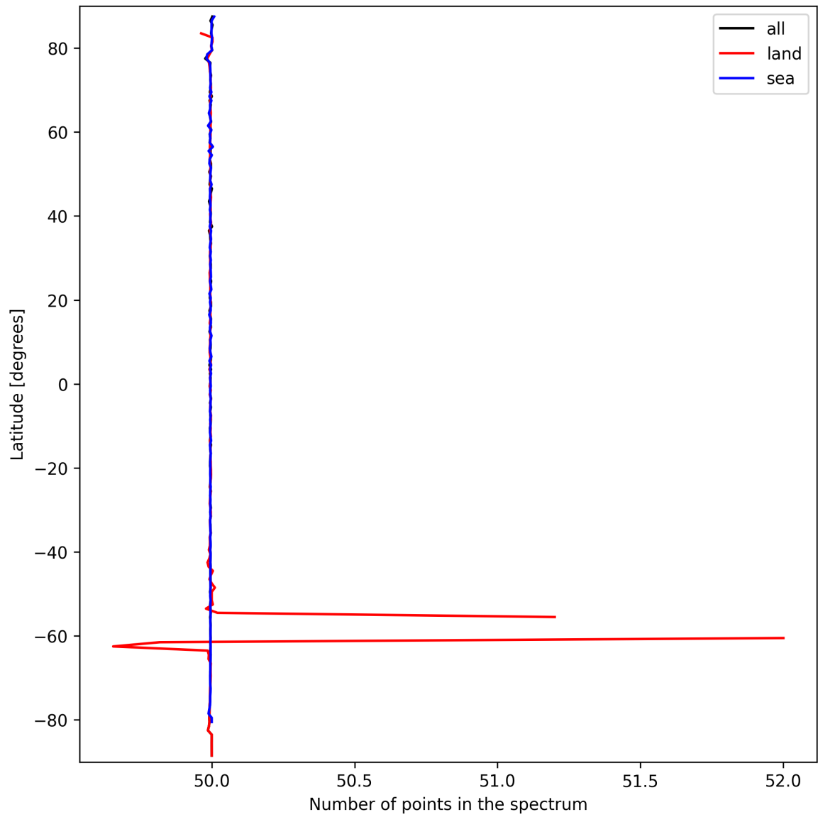
Figure 25: Zonal average of “Number of points in the spectrum” for 2025-09-23 to 2025-09-23.
