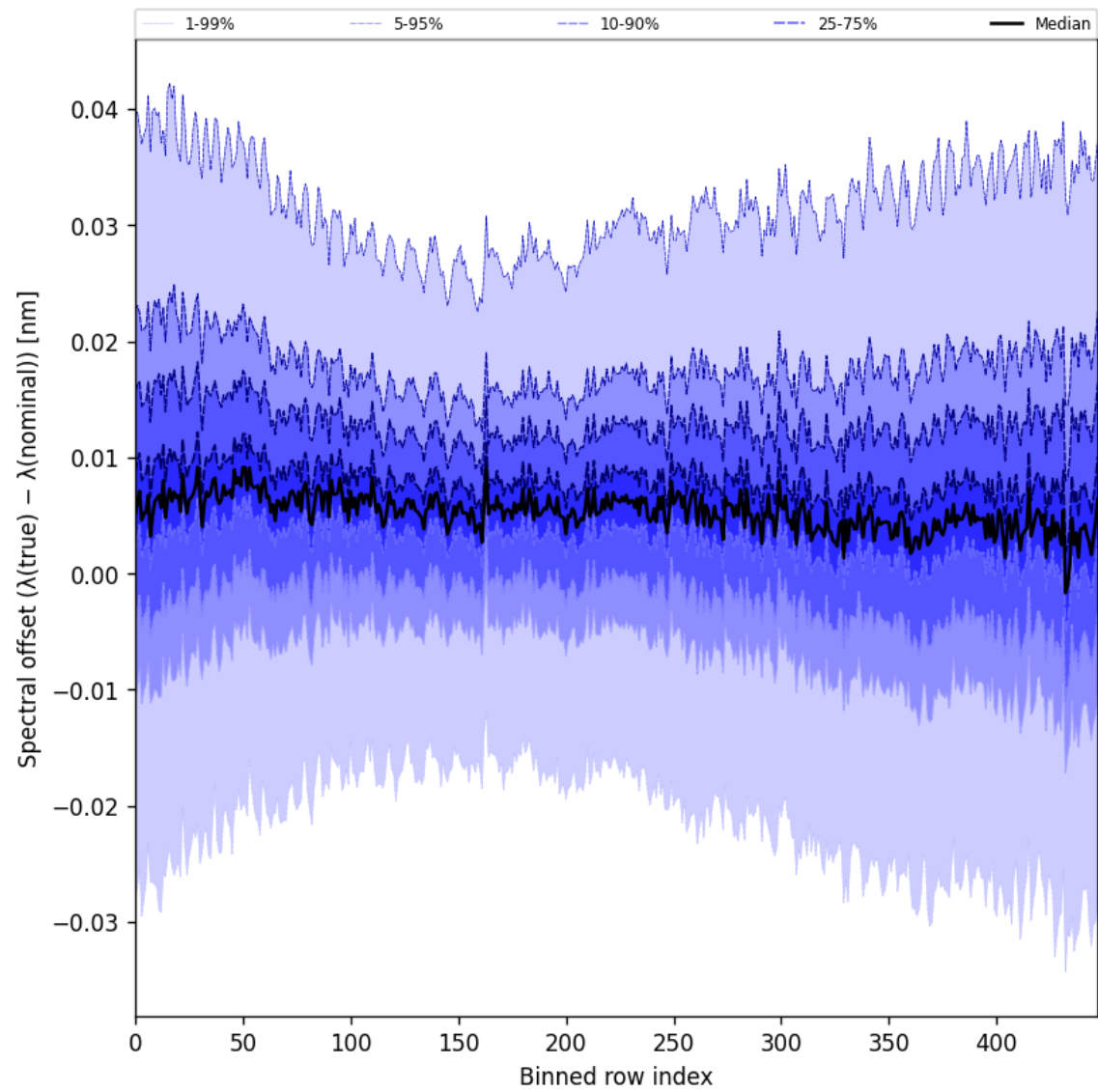
Figure 60: Along track statistics of “Spectral offset ( \lambda_{\text{true}} - \lambda_{\text{nominal}} )” for 2025-09-23 to 2025-09-23
