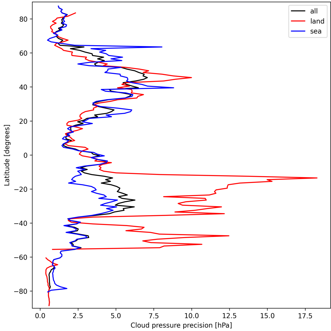
Figure 12: Zonal average of “Cloud pressure precision” for 2025-09-23 to 2025-09-23.
