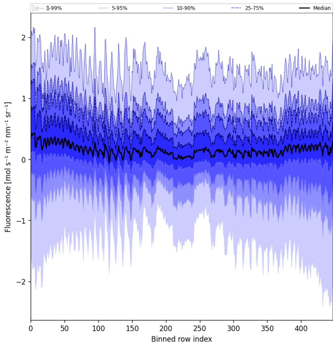
Figure 55: Along track statistics of “Fluorescence” for 2025-09-23 to 2025-09-23
