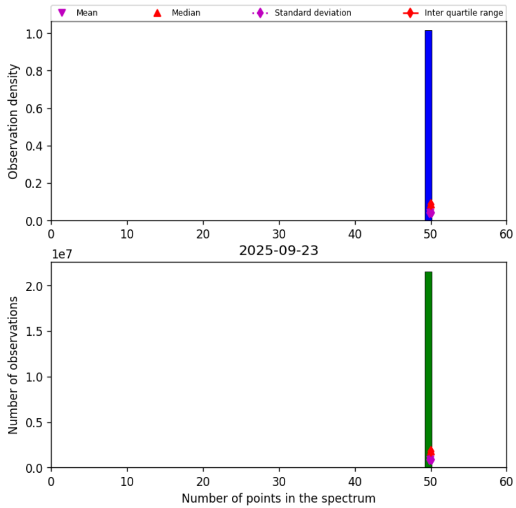
Figure 42: Histogram of "Number of points in the spectrum" for 2025-09-23 to 2025-09-23
