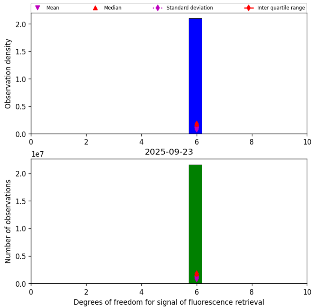
Figure 41: Histogram of “Degrees of freedom for signal of fluorescence retrieval” for 2025-09-23 to 2025-09-23
