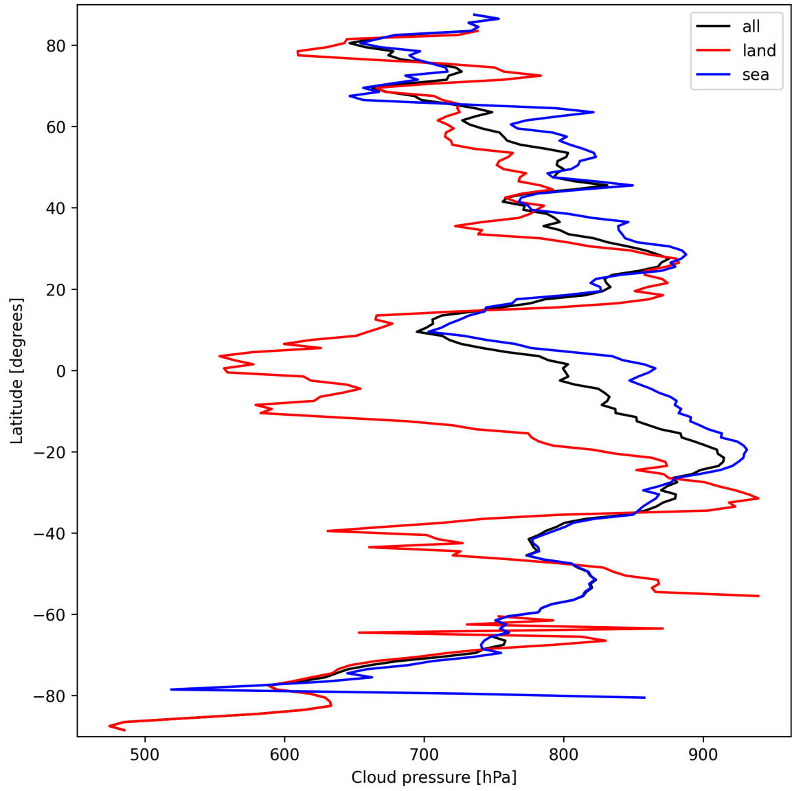
Figure 11: Zonal average of “Cloud pressure” for 2025-09-23 to 2025-09-23.
