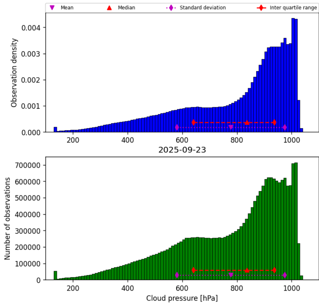
Figure 28: Histogram of “Cloud pressure” for 2025-09-23 to 2025-09-23
