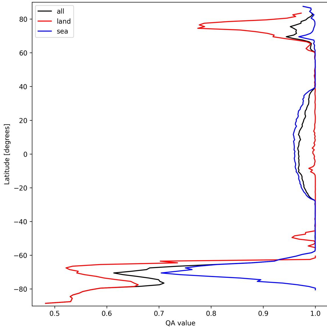
Figure 10: Zonal average of “QA value” for 2025-09-23 to 2025-09-23.
