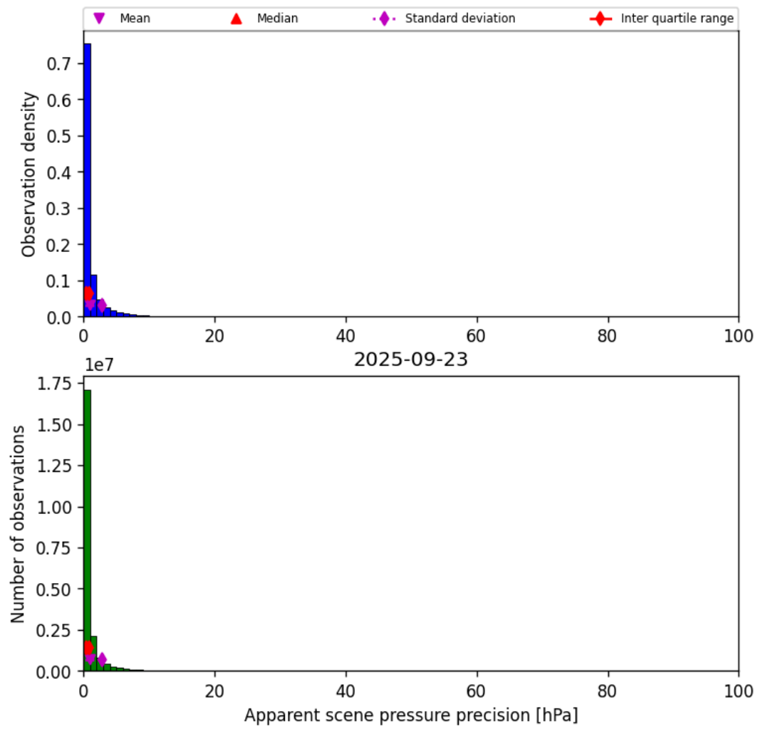
Figure 35: Histogram of “Apparent scene pressure precision” for 2025-09-23 to 2025-09-23
