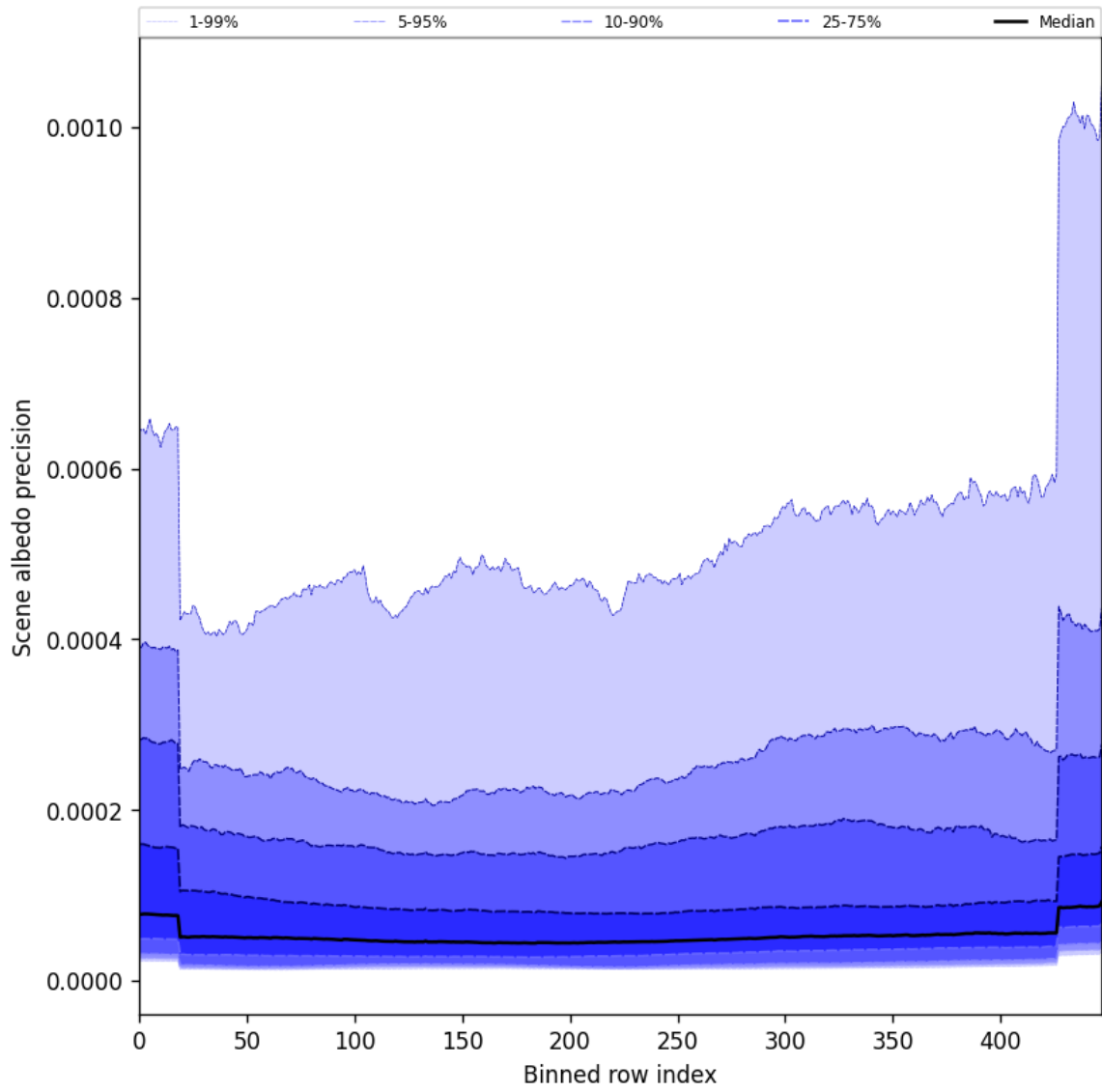
Figure 50: Along track statistics of “Scene albedo precision” for 2025-09-23 to 2025-09-23
