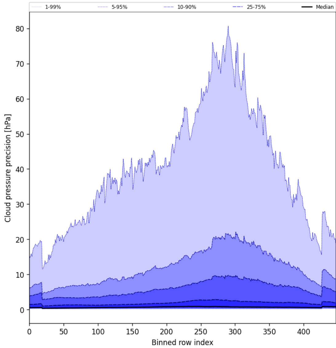
Figure 46: Along track statistics of “Cloud pressure precision” for 2025-09-23 to 2025-09-23
