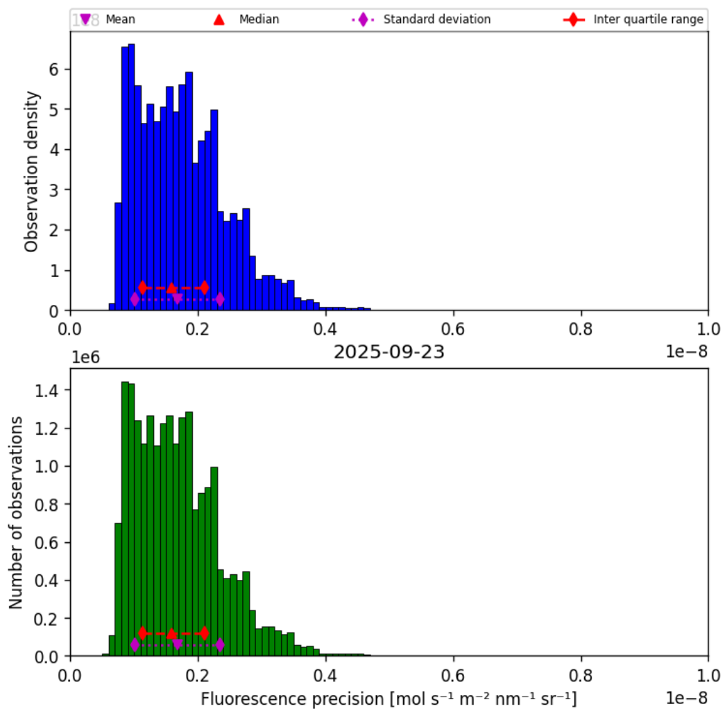
Figure 39: Histogram of “Fluorescence precision” for 2025-09-23 to 2025-09-23
