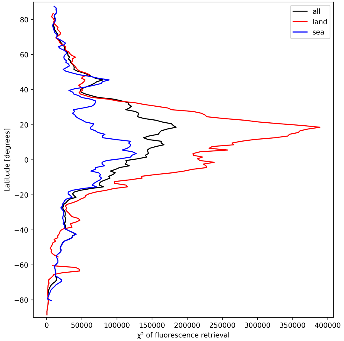
Figure 23: Zonal average of “ \chi^2 of fluorescence retrieval” for 2025-09-23 to 2025-09-23.
