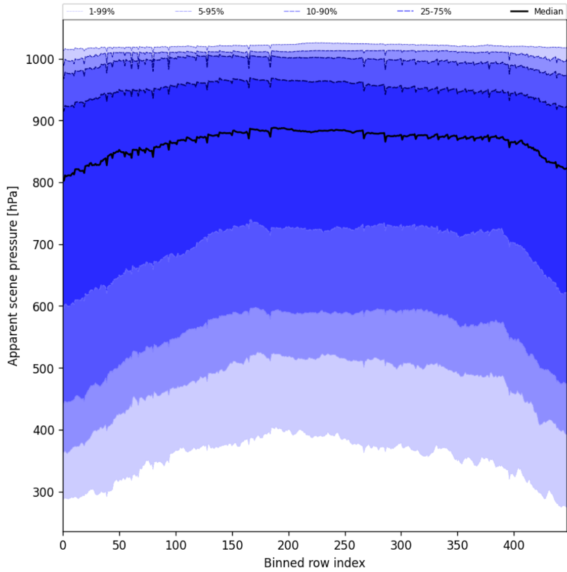
Figure 51: Along track statistics of “Apparent scene pressure” for 2025-09-23 to 2025-09-23
