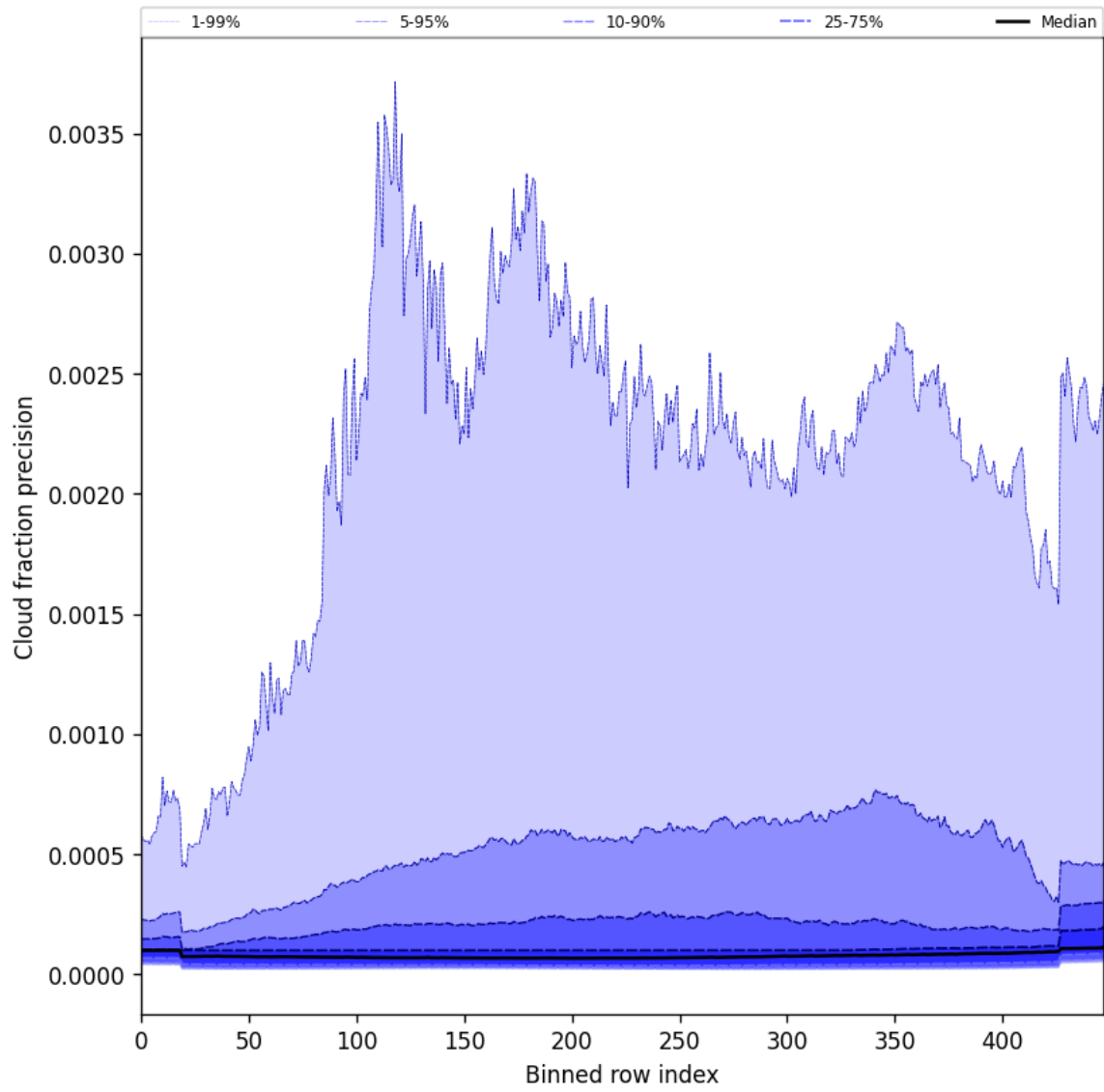
Figure 48: Along track statistics of “Cloud fraction precision” for 2025-09-23 to 2025-09-23
