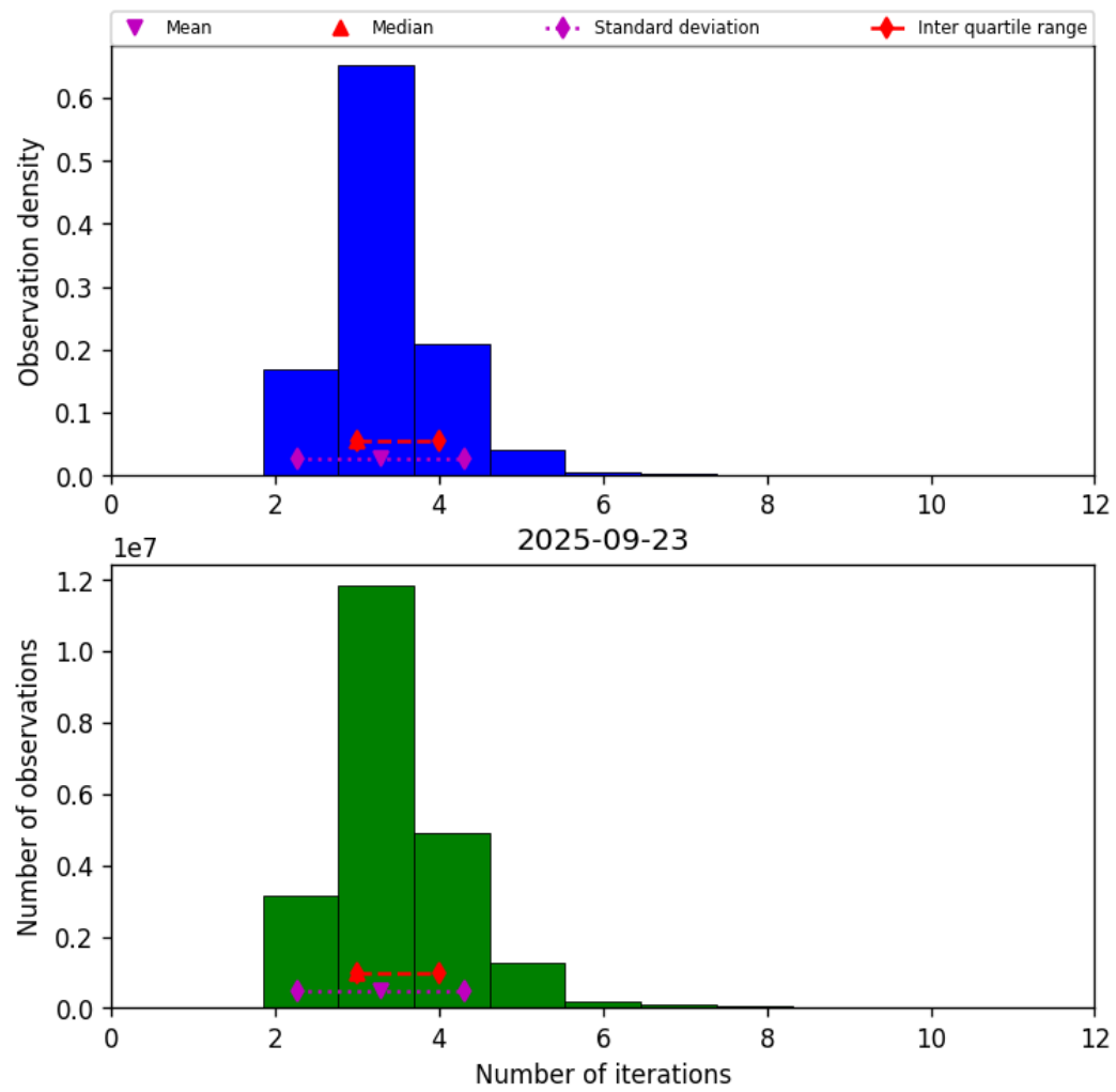
Figure 37: Histogram of “Number of iterations” for 2025-09-23 to 2025-09-23
