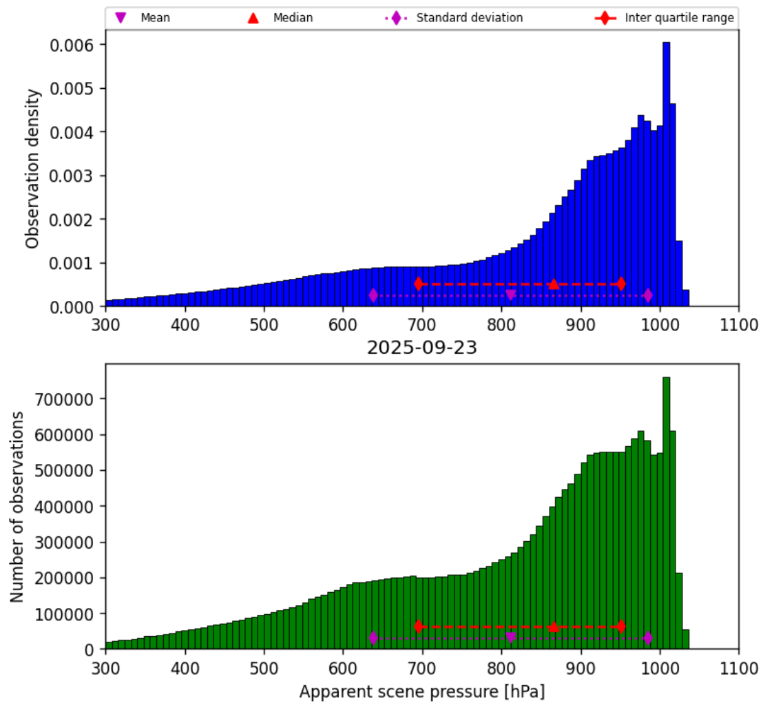
Figure 34: Histogram of “Apparent scene pressure” for 2025-09-23 to 2025-09-23
