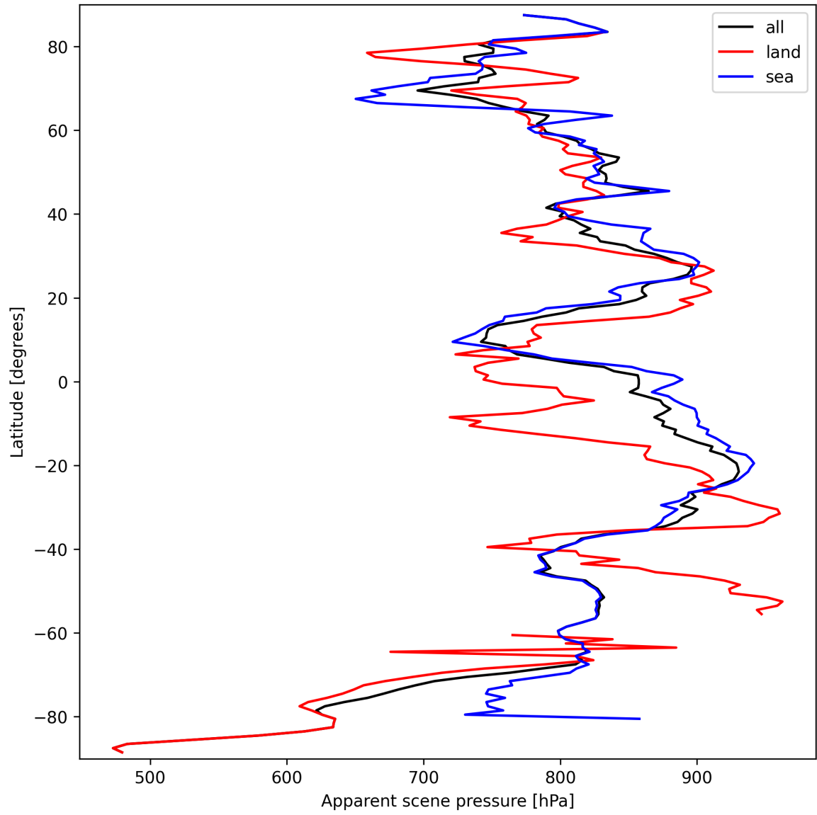
Figure 17: Zonal average of “Apparent scene pressure” for 2025-09-23 to 2025-09-23.
