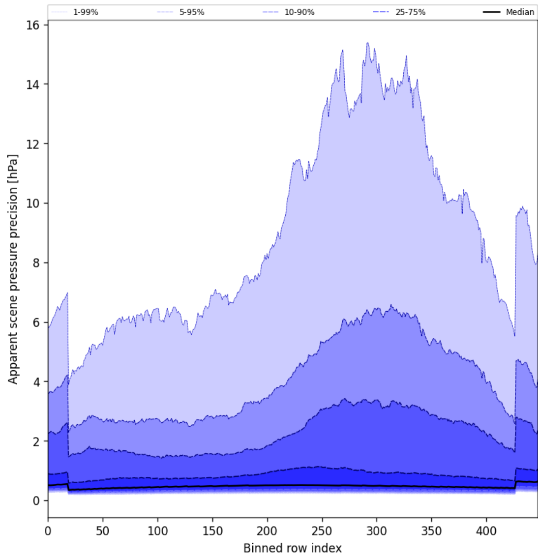
Figure 52: Along track statistics of “Apparent scene pressure precision” for 2025-09-23 to 2025-09-23
