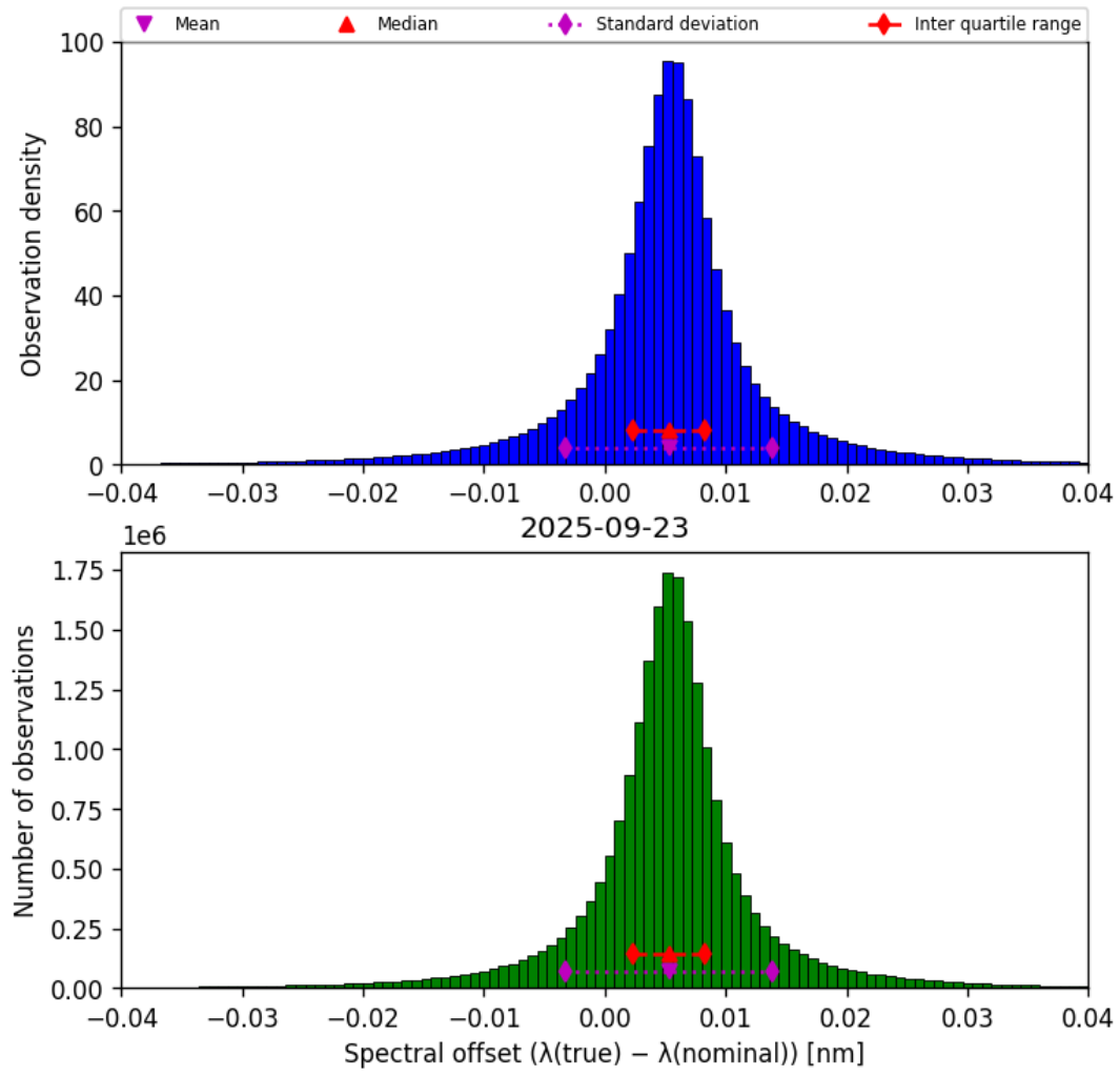
Figure 43: Histogram of “Spectral offset ( \lambda_{\text{true}} - \lambda_{\text{nominal}} )” for 2025-09-23 to 2025-09-23
