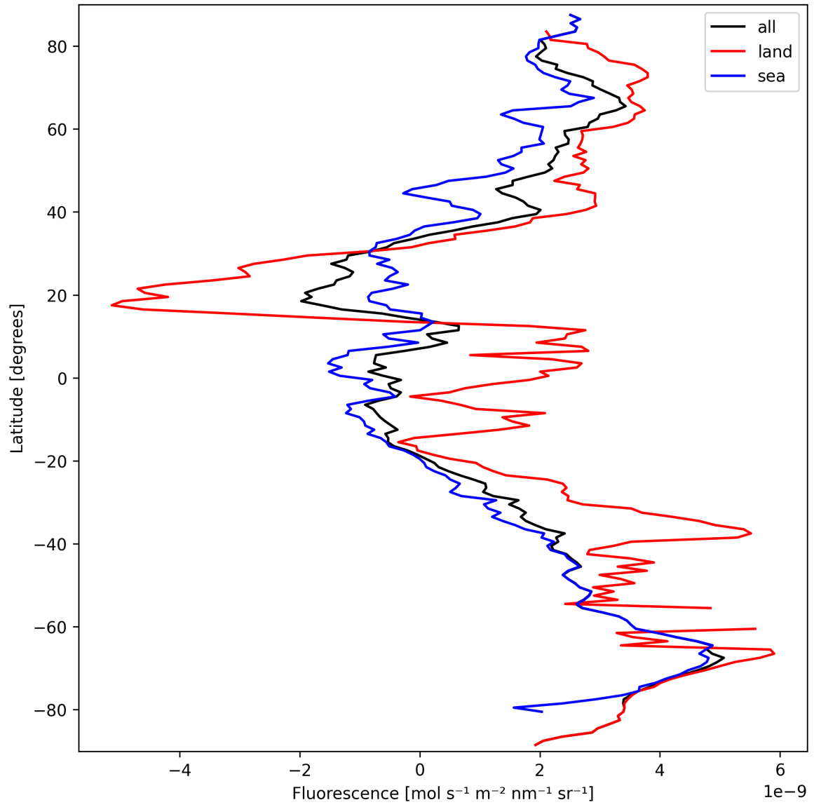
Figure 21: Zonal average of “Fluorescence” for 2025-09-23 to 2025-09-23.
