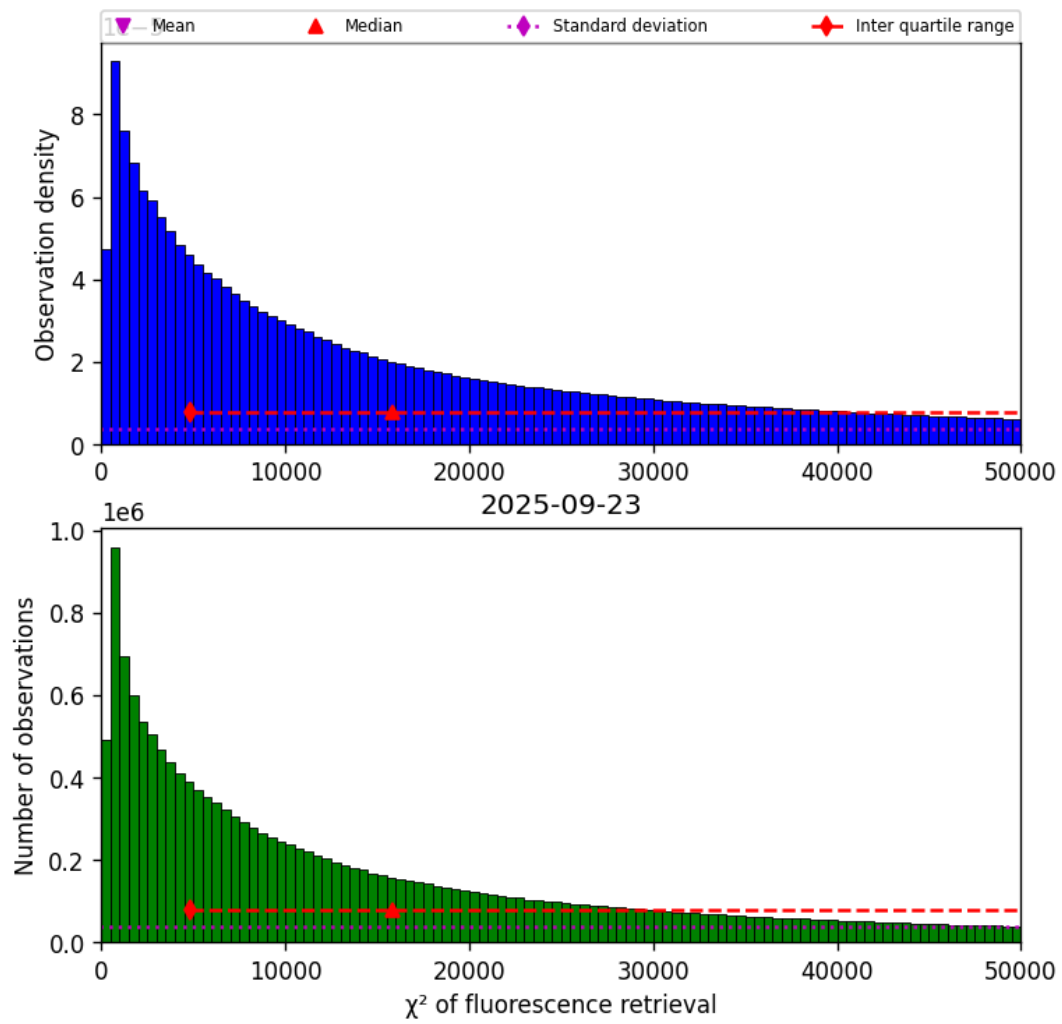
Figure 40: Histogram of “ \chi^2 of fluorescence retrieval” for 2025-09-23 to 2025-09-23
