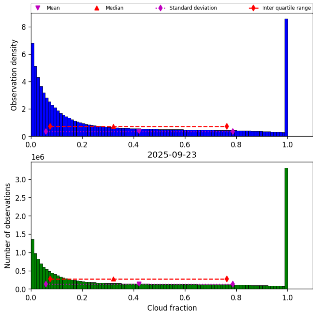
Figure 30: Histogram of “Cloud fraction” for 2025-09-23 to 2025-09-23
