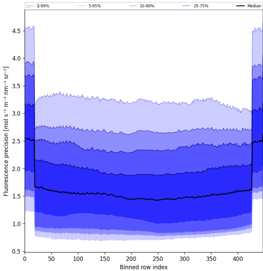
Figure 56: Along track statistics of “Fluorescence precision” for 2025-09-23 to 2025-09-23
