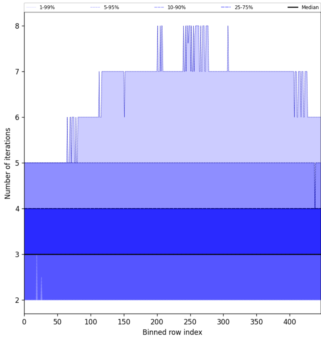
Figure 54: Along track statistics of “Number of iterations” for 2025-09-23 to 2025-09-23
