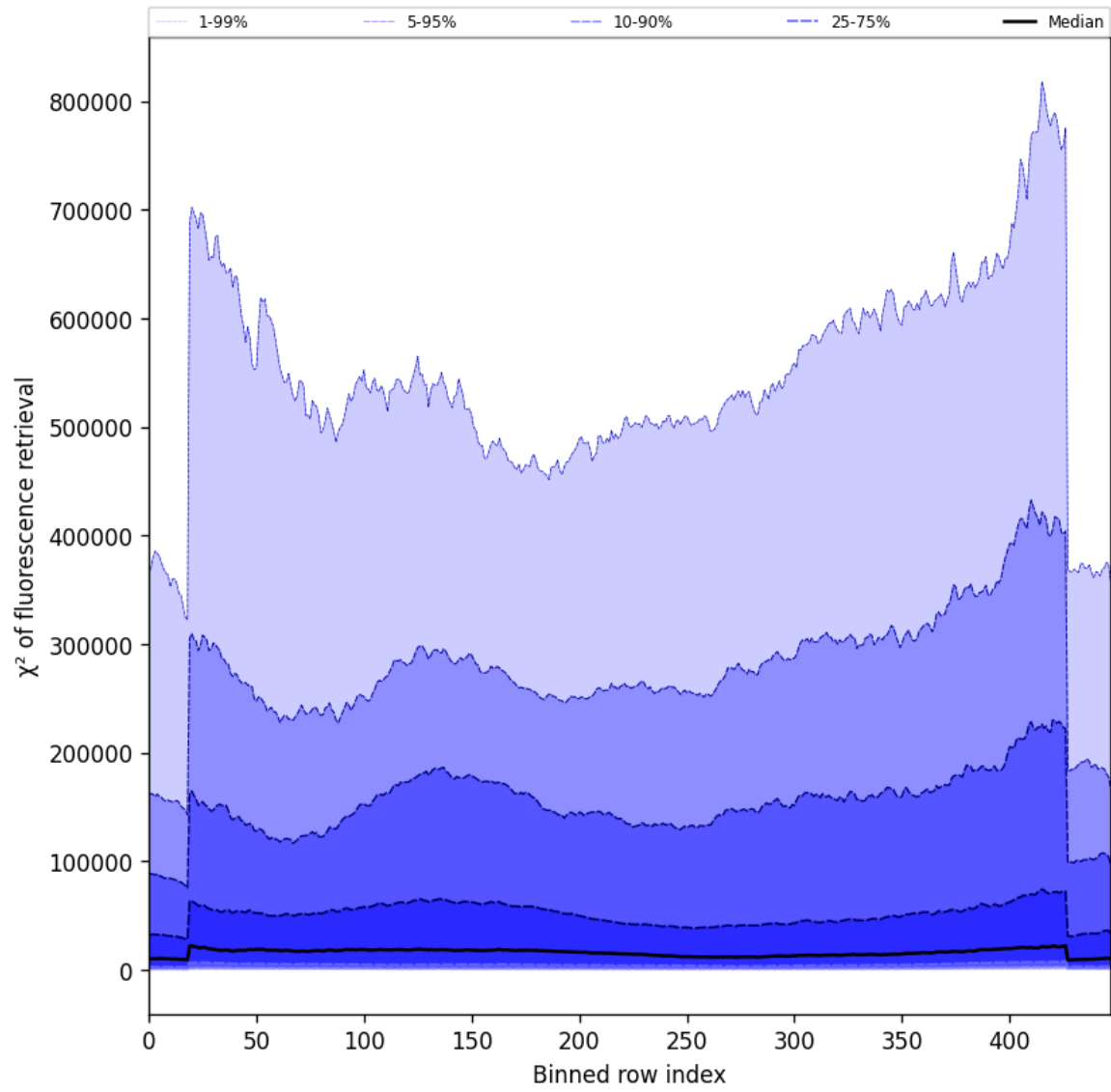
Figure 57: Along track statistics of “ \chi^2 of fluorescence retrieval” for 2025-09-23 to 2025-09-23
