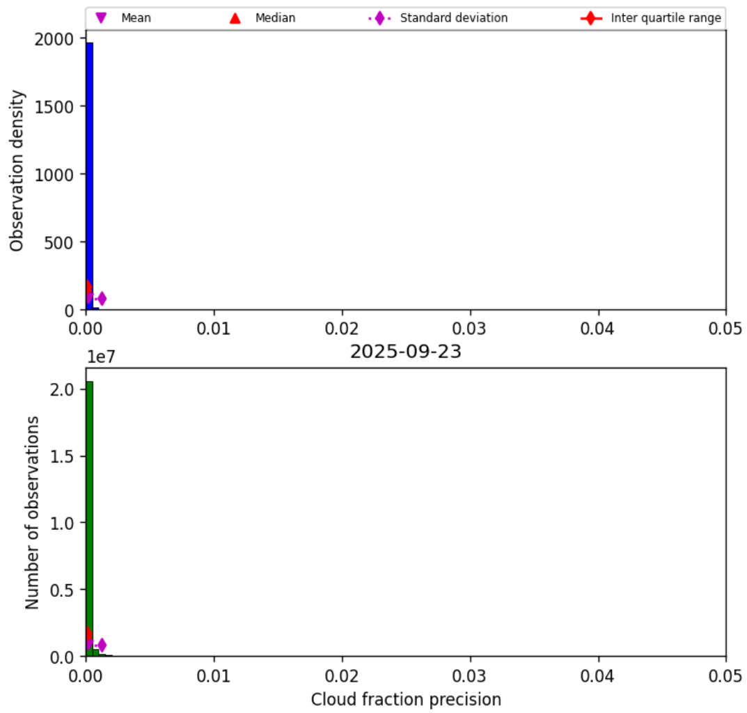
Figure 31: Histogram of “Cloud fraction precision” for 2025-09-23 to 2025-09-23
