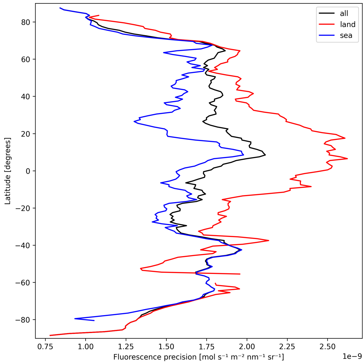
Figure 22: Zonal average of “Fluorescence precision” for 2025-09-23 to 2025-09-23.
