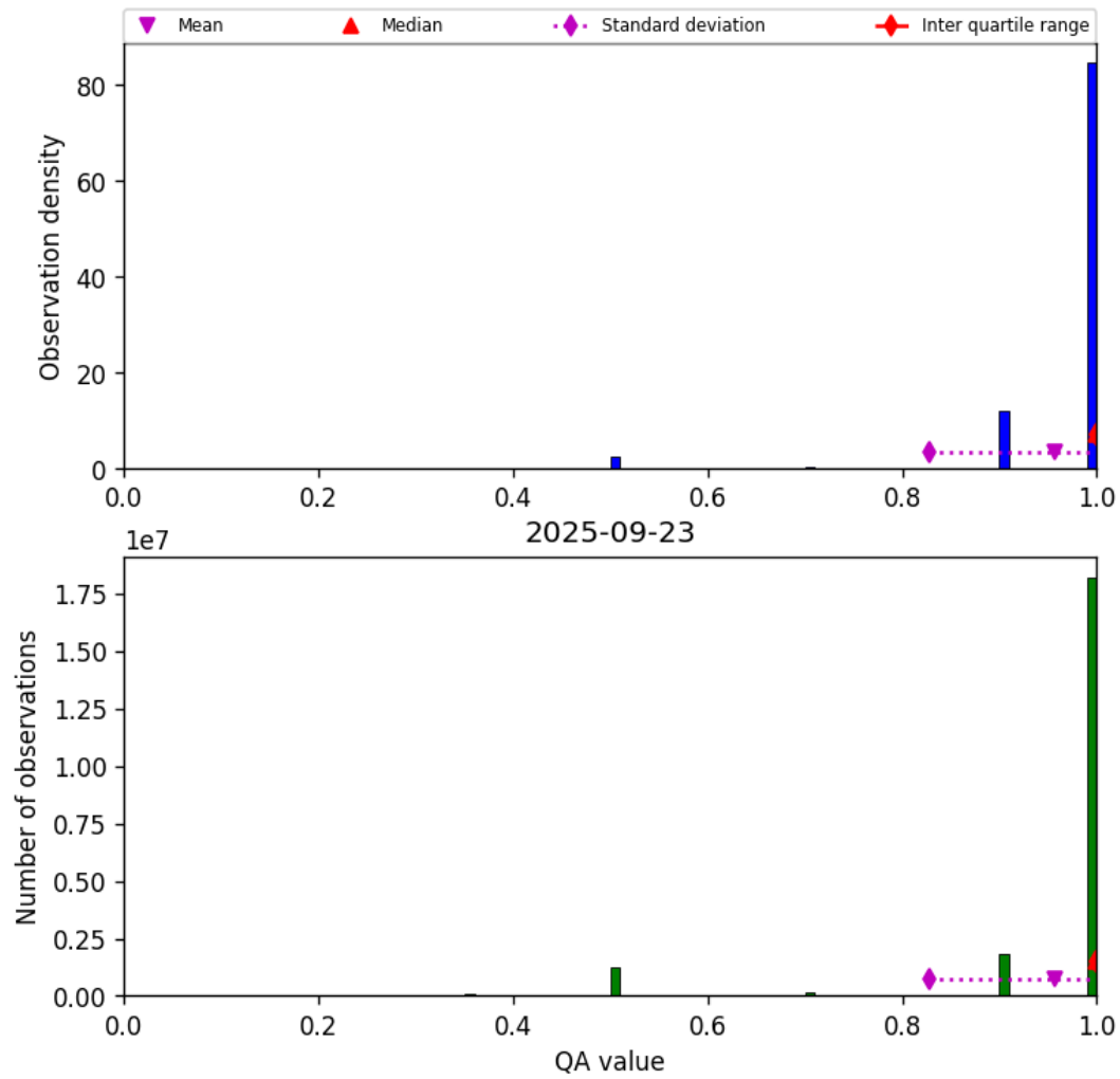
Figure 27: Histogram of “QA value” for 2025-09-23 to 2025-09-23
