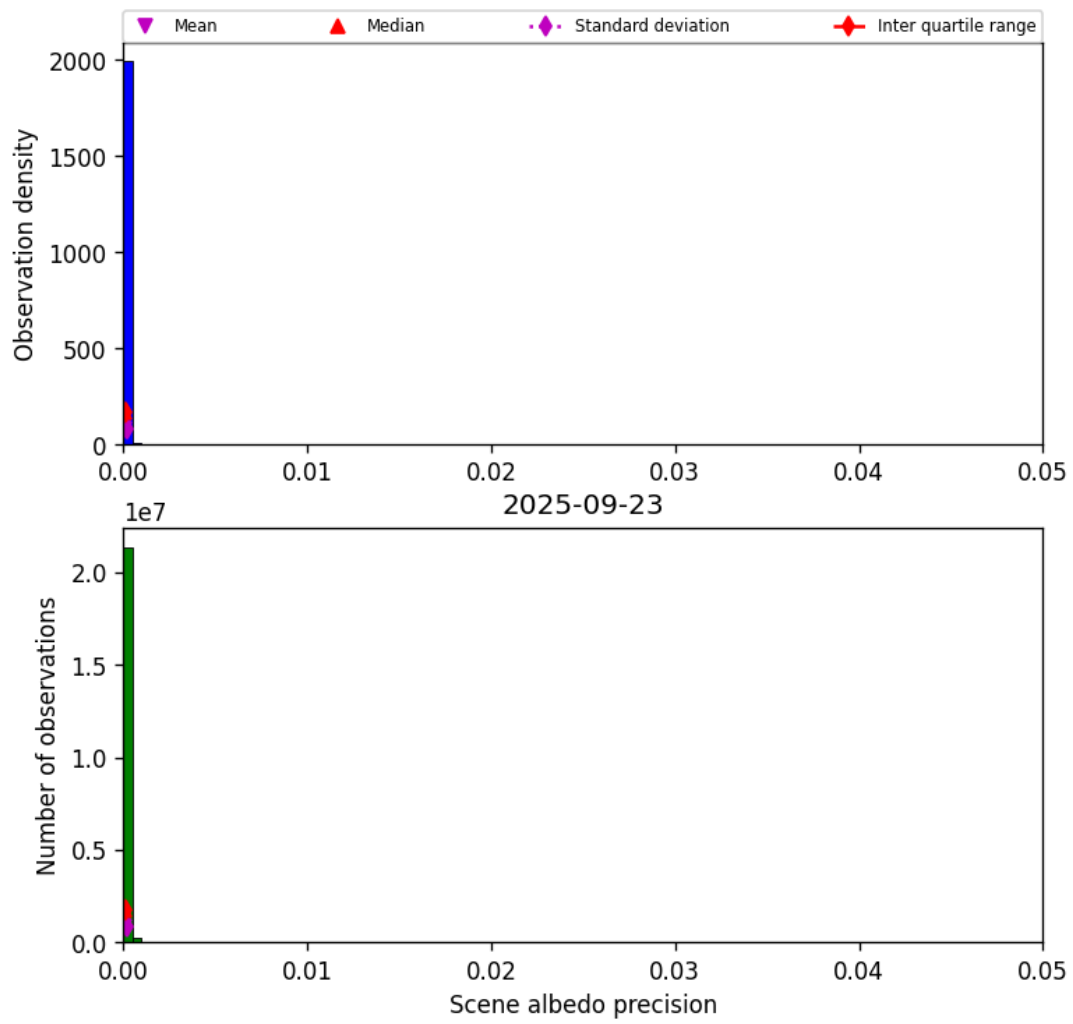
Figure 33: Histogram of “Scene albedo precision” for 2025-09-23 to 2025-09-23
