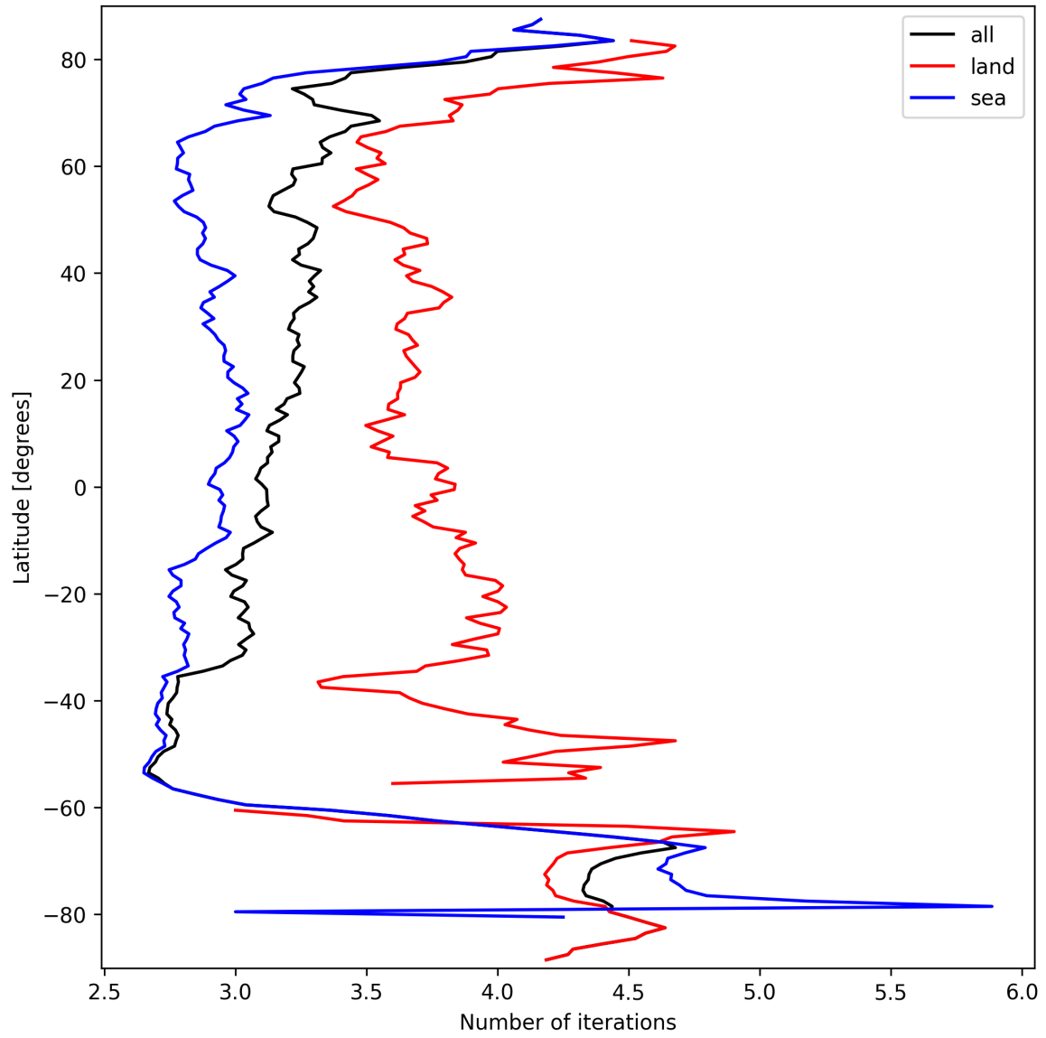
Figure 20: Zonal average of “Number of iterations” for 2025-09-23 to 2025-09-23.
