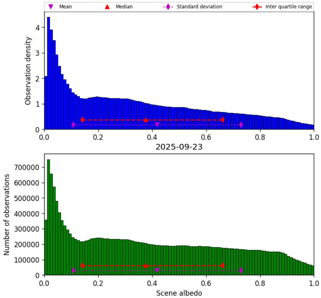
Figure 32: Histogram of “Scene albedo” for 2025-09-23 to 2025-09-23
