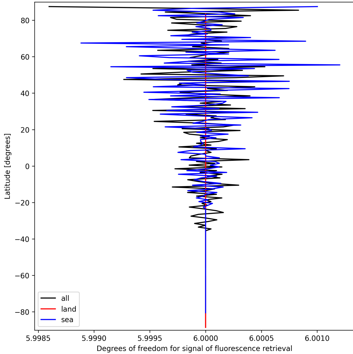
Figure 24: Zonal average of “Degrees of freedom for signal of fluorescence retrieval” for 2025-09-23 to 2025-09-23.
