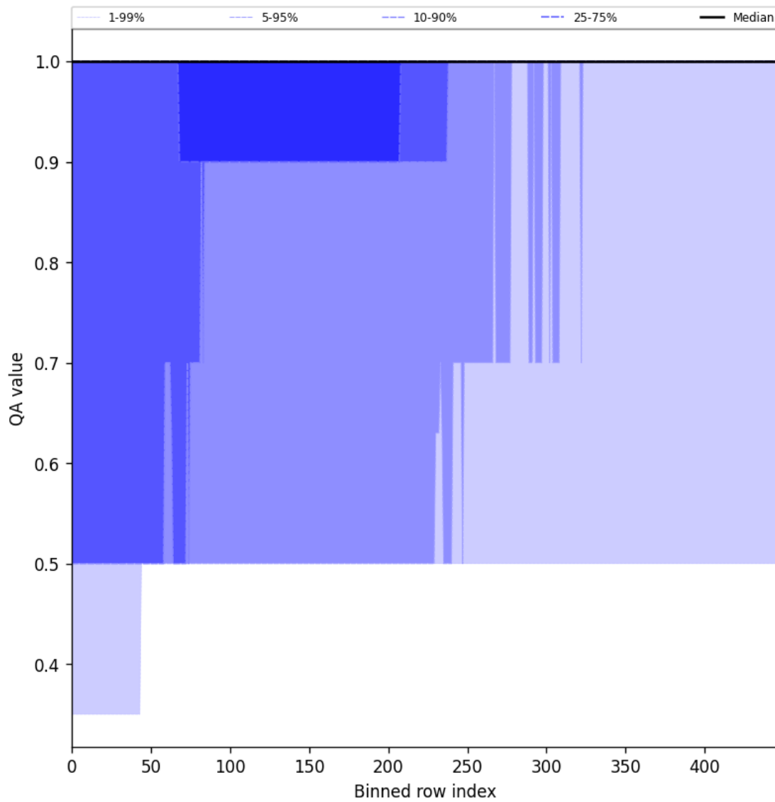
Figure 44: Along track statistics of “QA value” for 2025-09-23 to 2025-09-23
