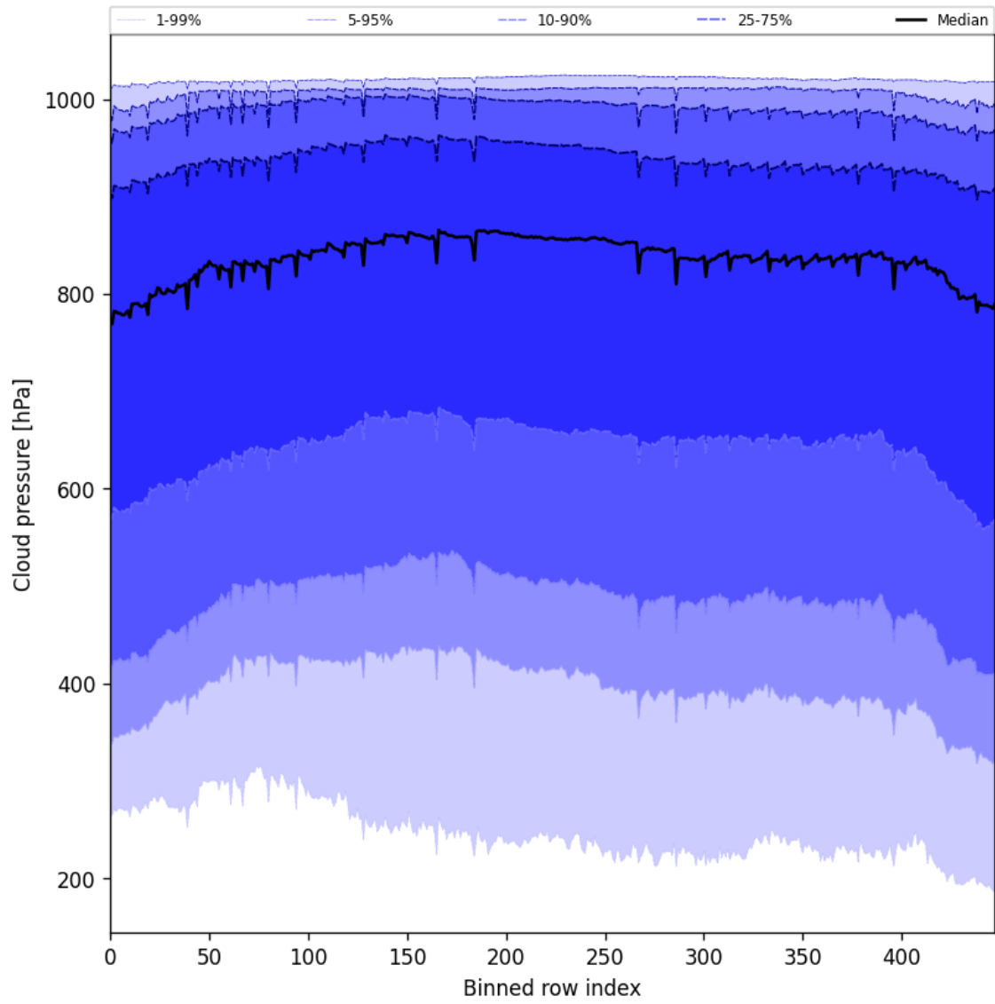
Figure 45: Along track statistics of “Cloud pressure” for 2025-09-23 to 2025-09-23
