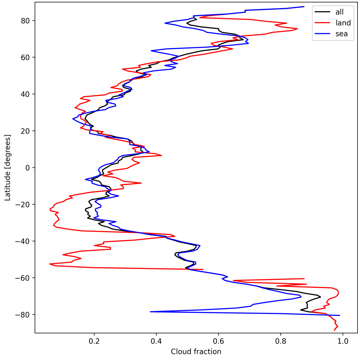
Figure 13: Zonal average of “Cloud fraction” for 2025-09-23 to 2025-09-23.
