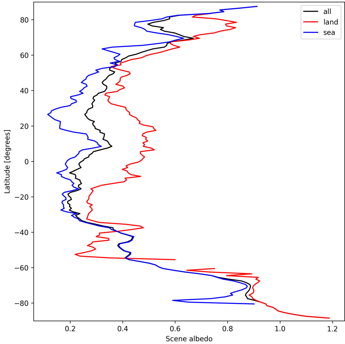
Figure 15: Zonal average of "Scene albedo" for 2025-09-23 to 2025-09-23.
