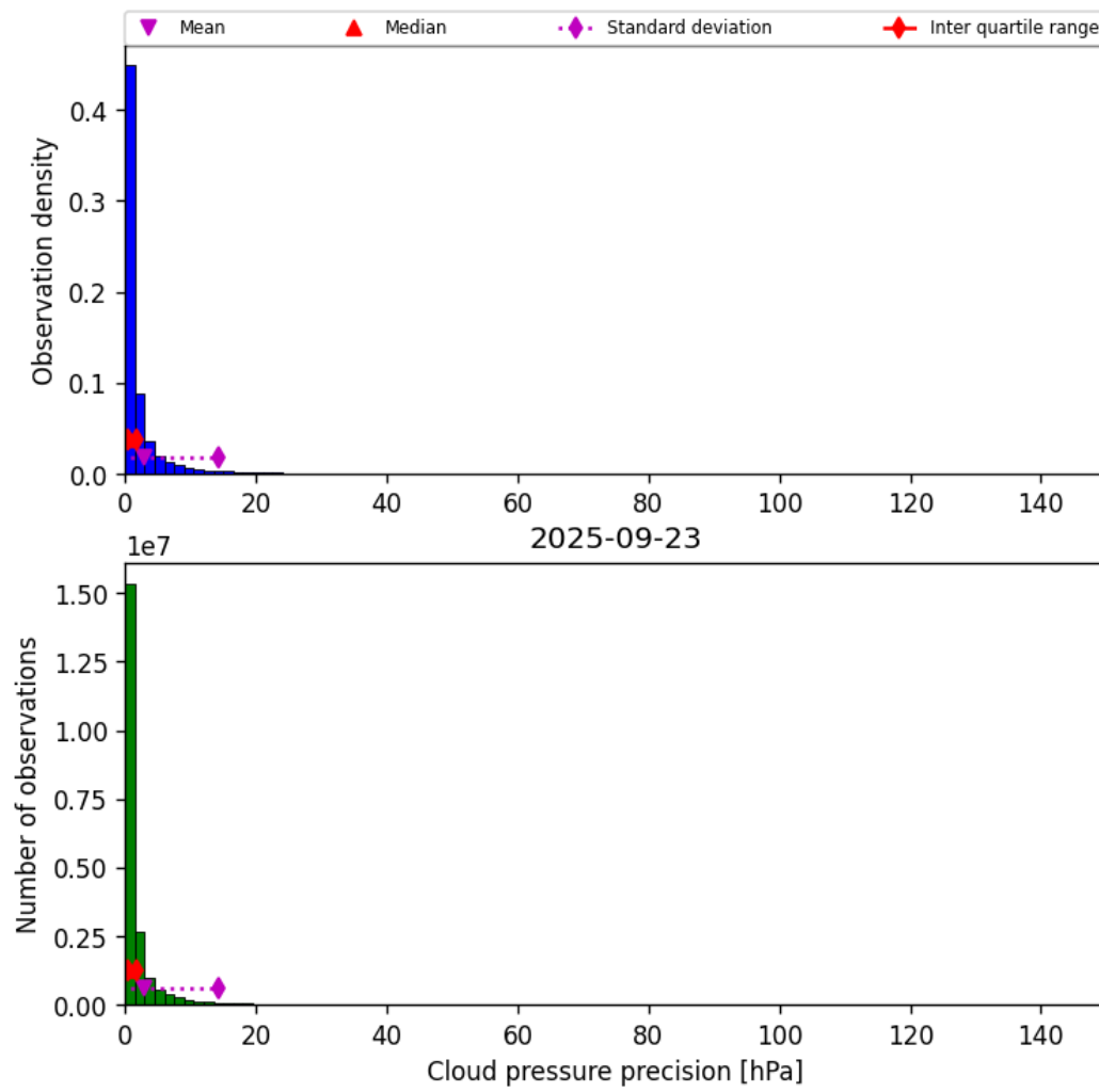
Figure 29: Histogram of “Cloud pressure precision” for 2025-09-23 to 2025-09-23
