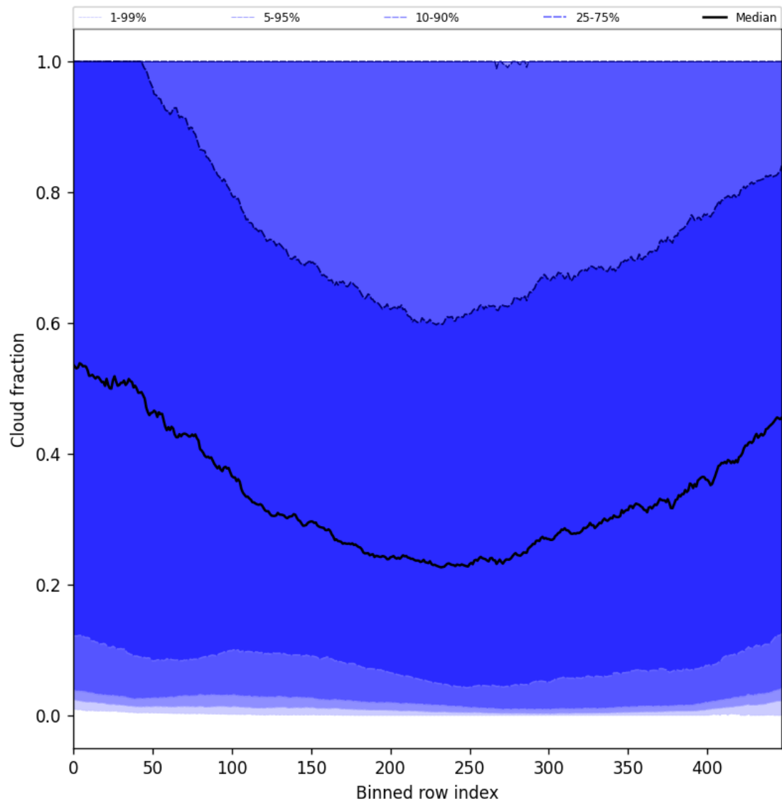
Figure 47: Along track statistics of “Cloud fraction” for 2025-09-23 to 2025-09-23
