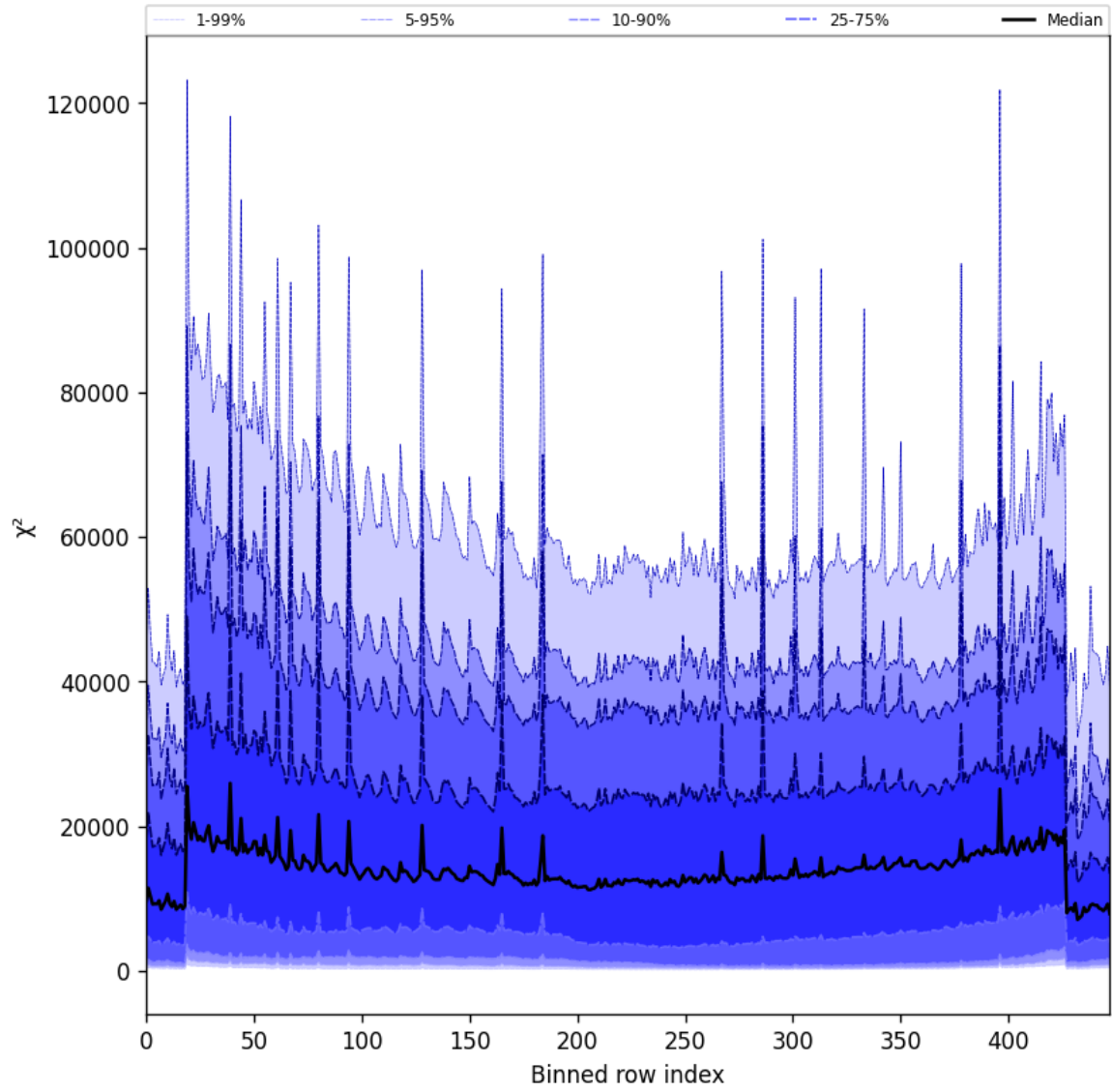
Figure 53: Along track statistics of “ \chi^2 ” for 2025-09-23 to 2025-09-23
