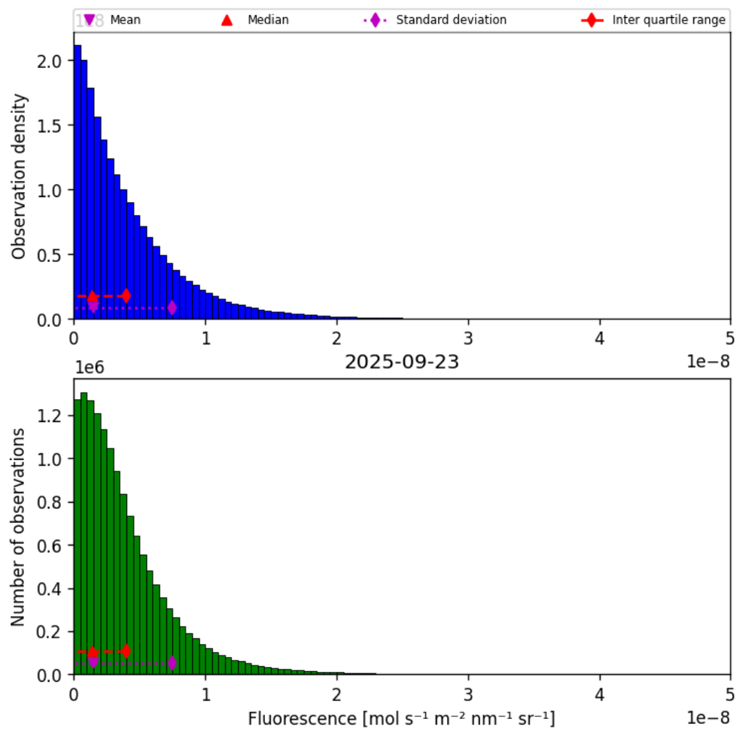
Figure 38: Histogram of “Fluorescence” for 2025-09-23 to 2025-09-23
