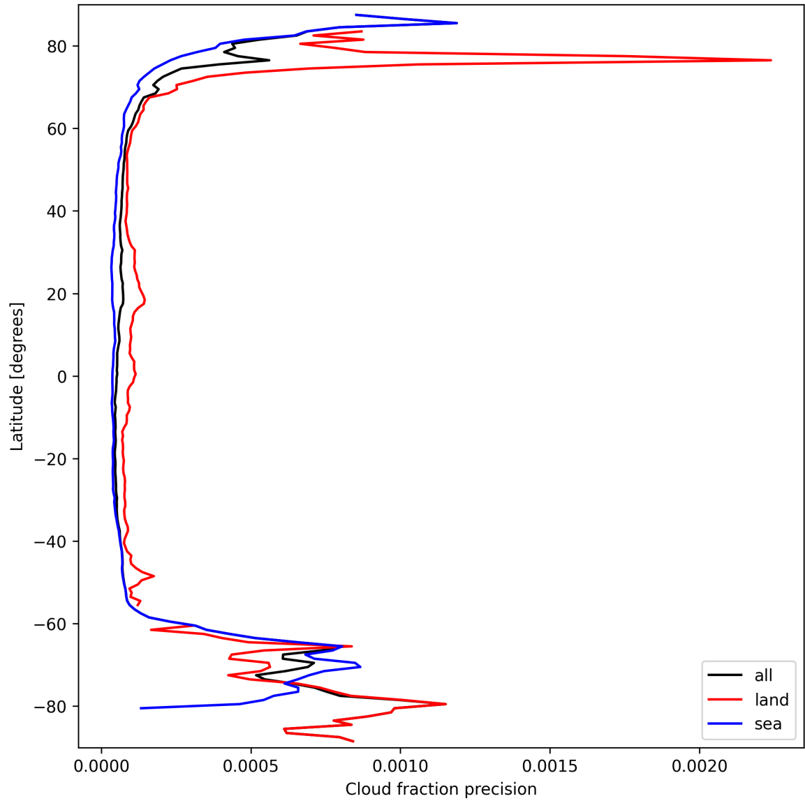
Figure 14: Zonal average of “Cloud fraction precision” for 2025-09-23 to 2025-09-23.
