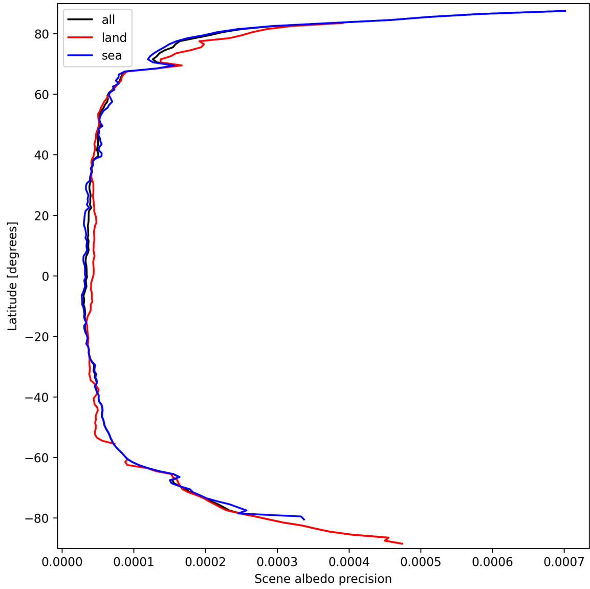
Figure 16: Zonal average of “Scene albedo precision” for 2025-09-23 to 2025-09-23.
