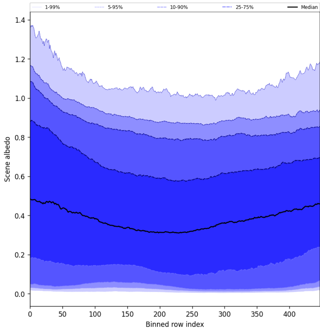
Figure 49: Along track statistics of “Scene albedo” for 2025-09-23 to 2025-09-23
