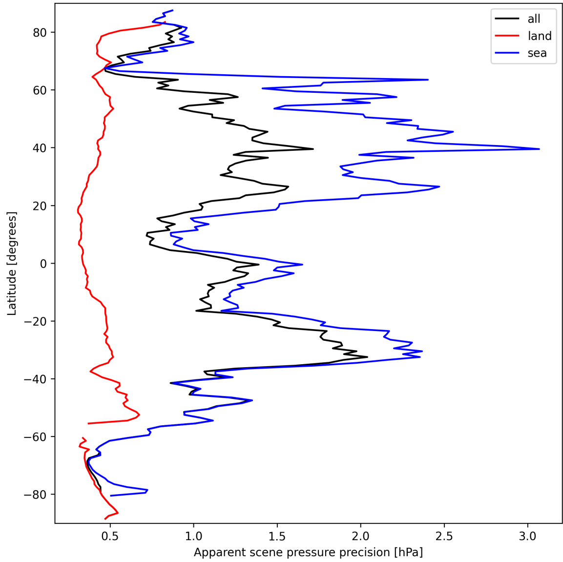
Figure 18: Zonal average of “Apparent scene pressure precision” for 2025-09-23 to 2025-09-23.
