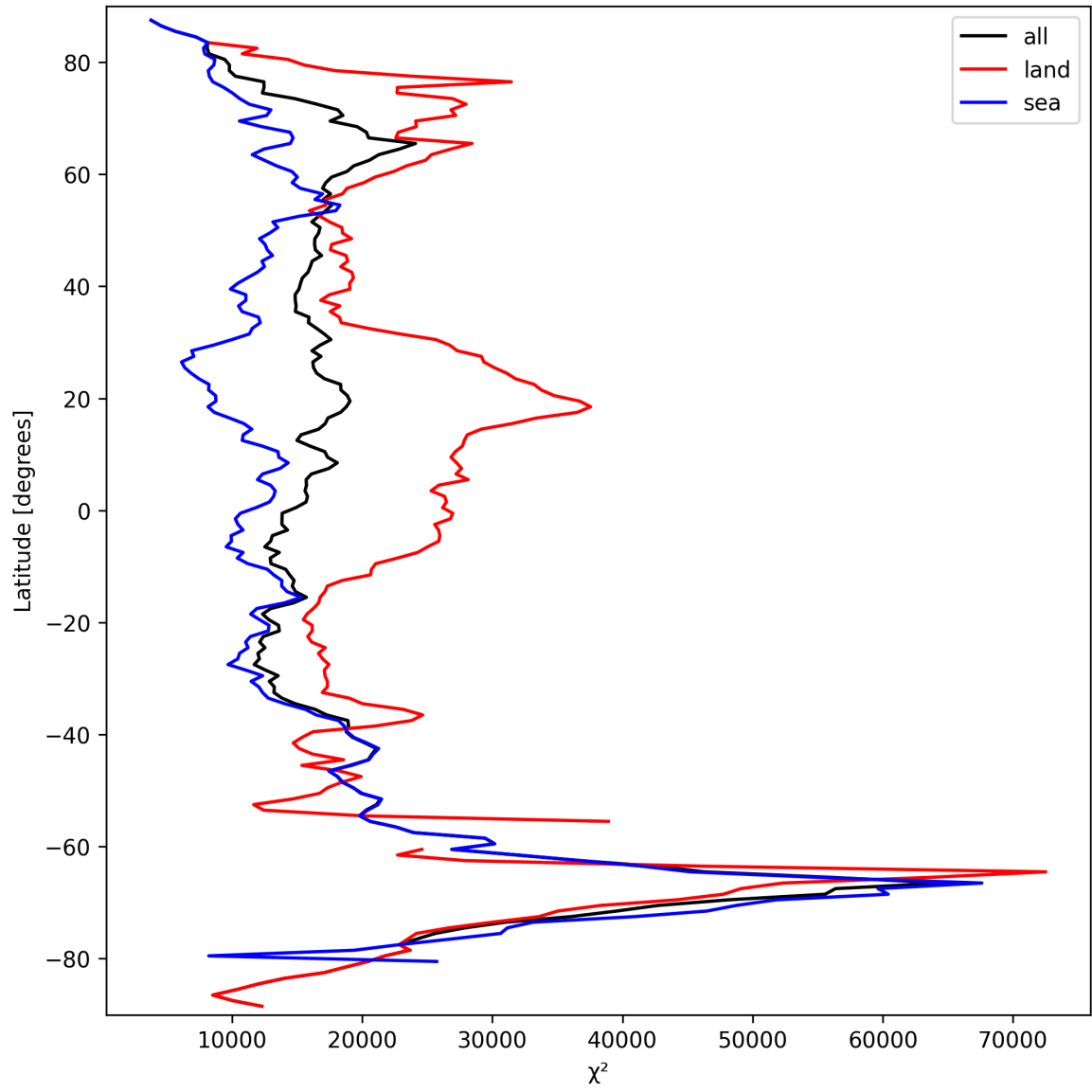
Figure 19: Zonal average of “ \chi^2 ” for 2025-09-23 to 2025-09-23.
