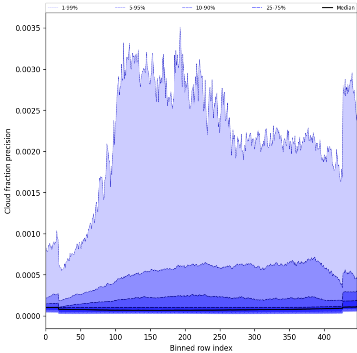
Figure 48: Along track statistics of “Cloud fraction precision” for 2025-09-24 to 2025-09-25
