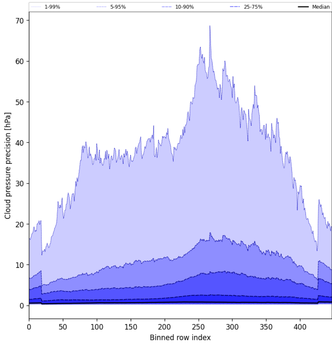
Figure 46: Along track statistics of “Cloud pressure precision” for 2025-09-24 to 2025-09-25
