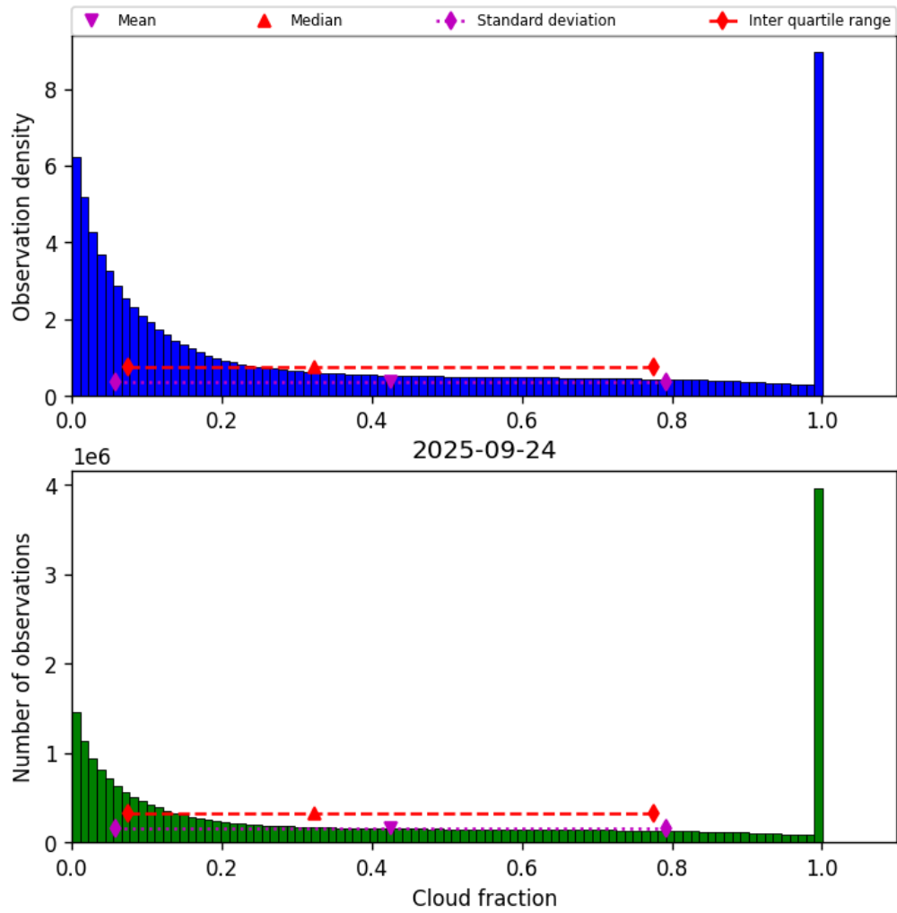
Figure 30: Histogram of “Cloud fraction” for 2025-09-24 to 2025-09-25
