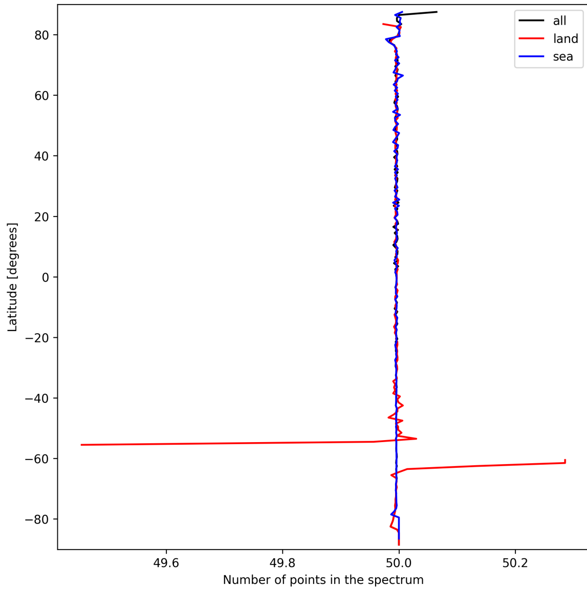
Figure 25: Zonal average of “Number of points in the spectrum” for 2025-09-24 to 2025-09-25.
