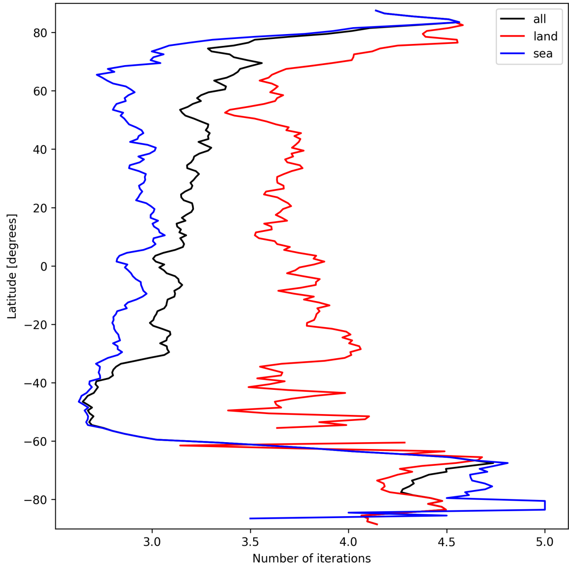
Figure 20: Zonal average of “Number of iterations” for 2025-09-24 to 2025-09-25.
