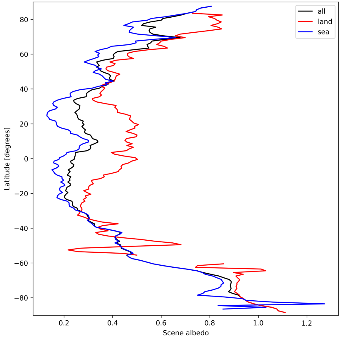
Figure 15: Zonal average of "Scene albedo" for 2025-09-24 to 2025-09-25.
