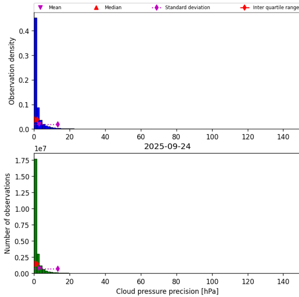
Figure 29: Histogram of “Cloud pressure precision” for 2025-09-24 to 2025-09-25
