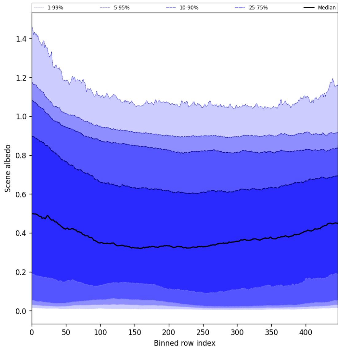
Figure 49: Along track statistics of “Scene albedo” for 2025-09-24 to 2025-09-25
