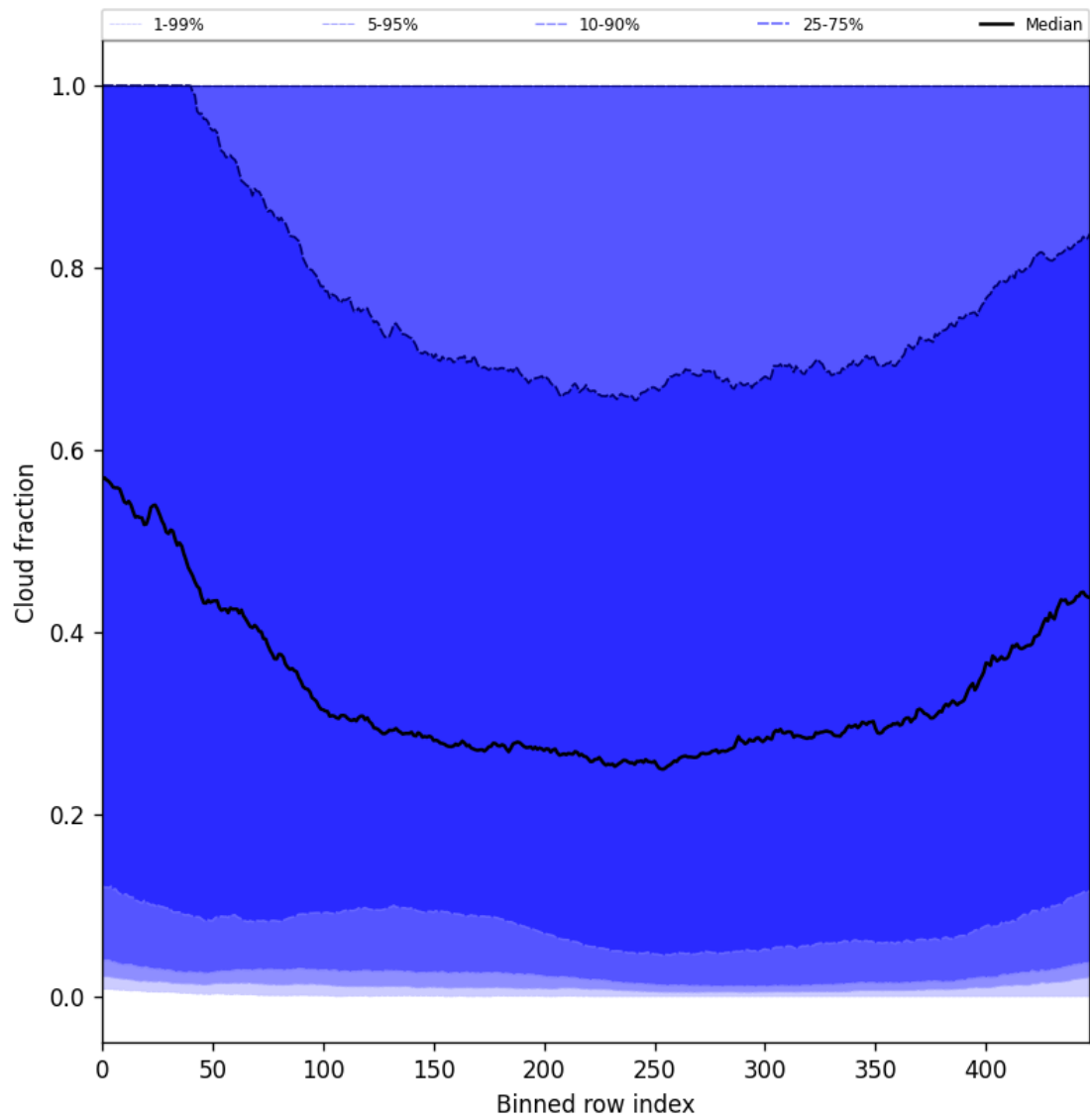
Figure 47: Along track statistics of “Cloud fraction” for 2025-09-24 to 2025-09-25
