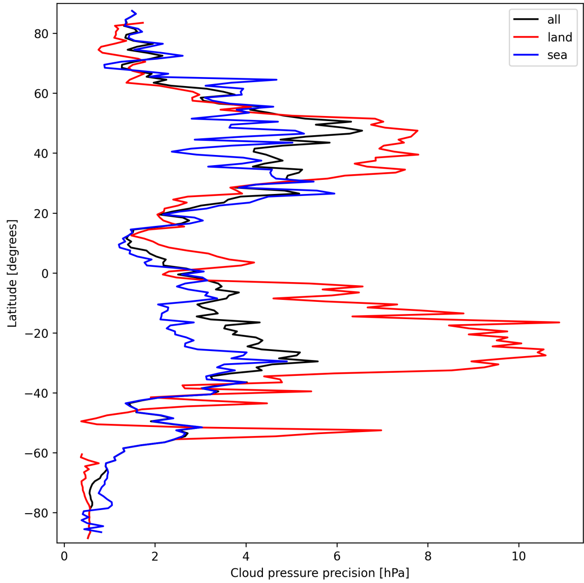
Figure 12: Zonal average of “Cloud pressure precision” for 2025-09-24 to 2025-09-25.
