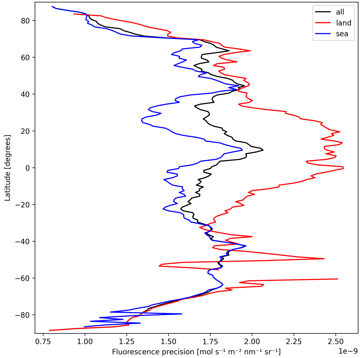
Figure 22: Zonal average of “Fluorescence precision” for 2025-09-24 to 2025-09-25.
