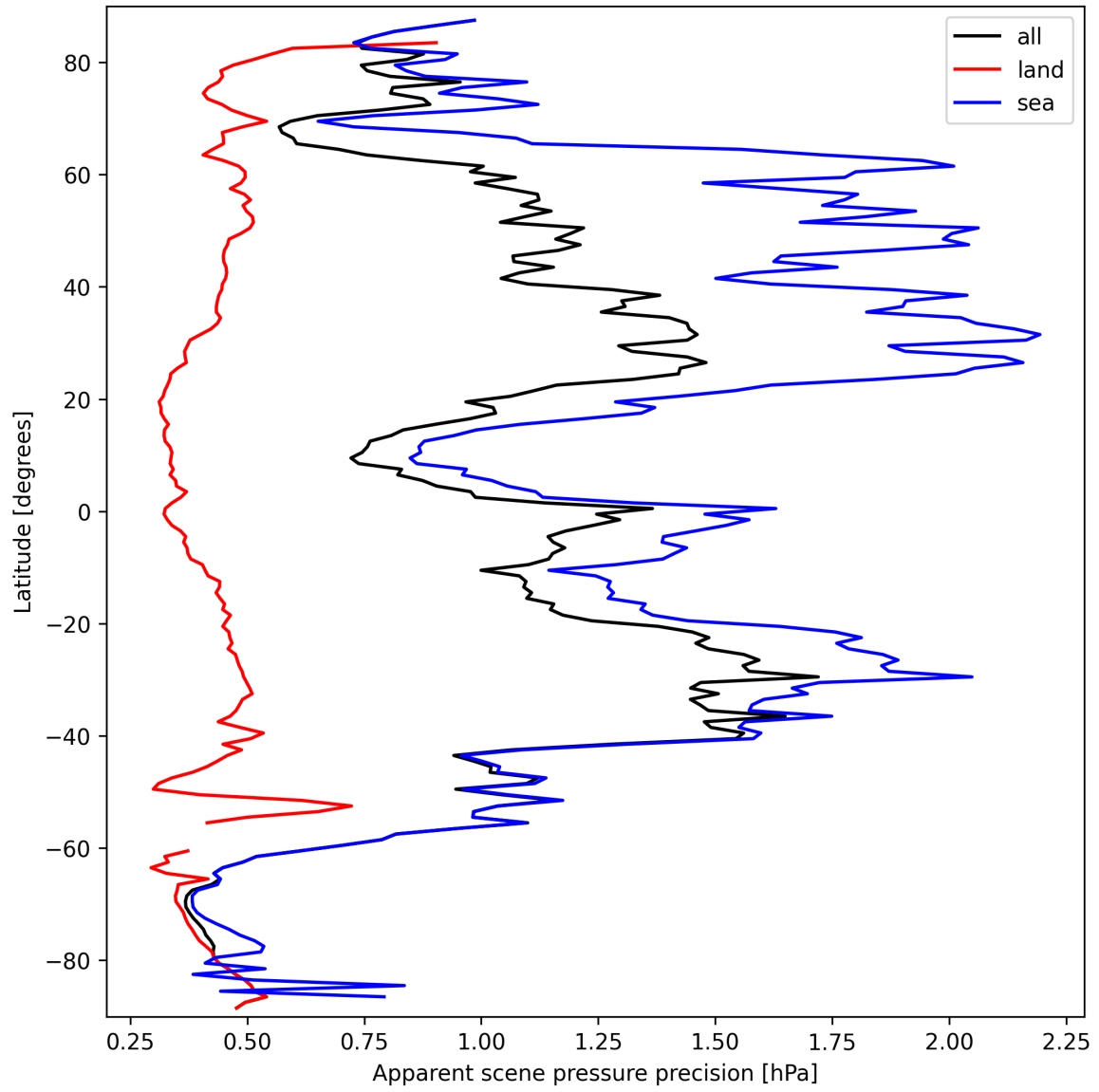
Figure 18: Zonal average of “Apparent scene pressure precision” for 2025-09-24 to 2025-09-25.
