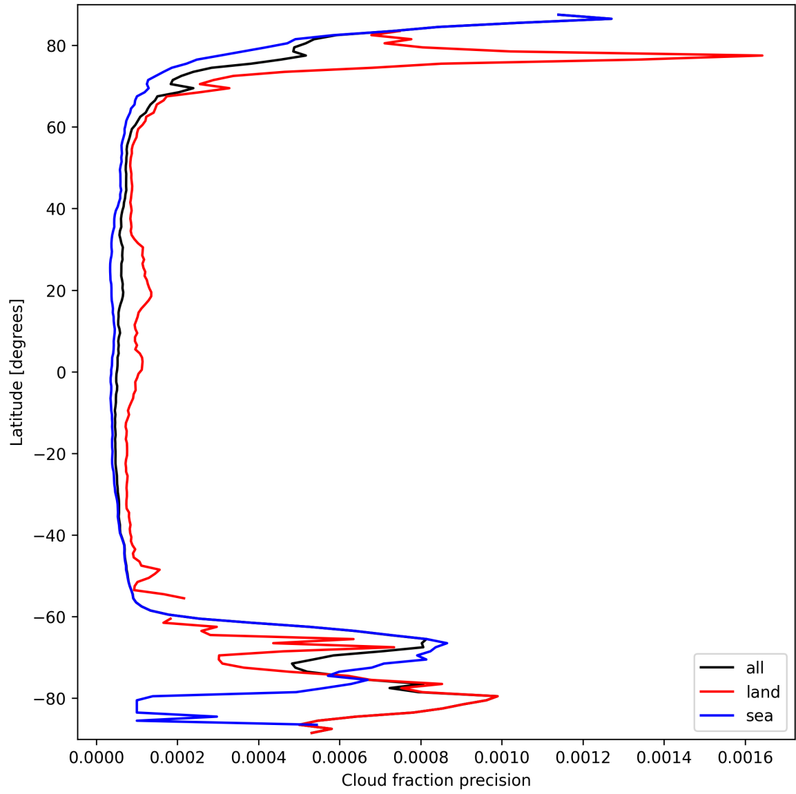
Figure 14: Zonal average of “Cloud fraction precision” for 2025-09-24 to 2025-09-25.
