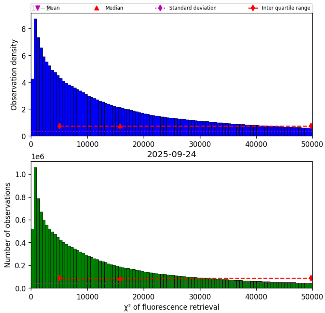
Figure 40: Histogram of “ \chi^2 of fluorescence retrieval” for 2025-09-24 to 2025-09-25
