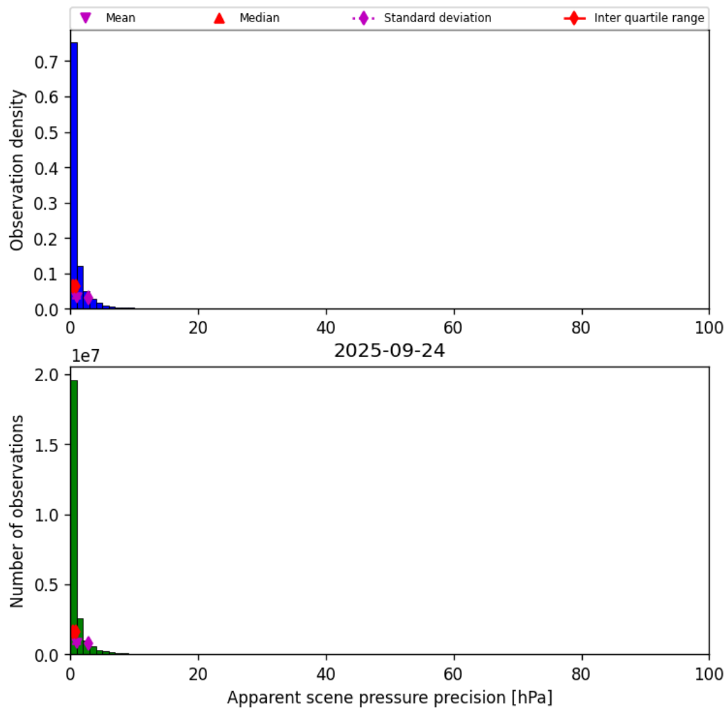
Figure 35: Histogram of “Apparent scene pressure precision” for 2025-09-24 to 2025-09-25
