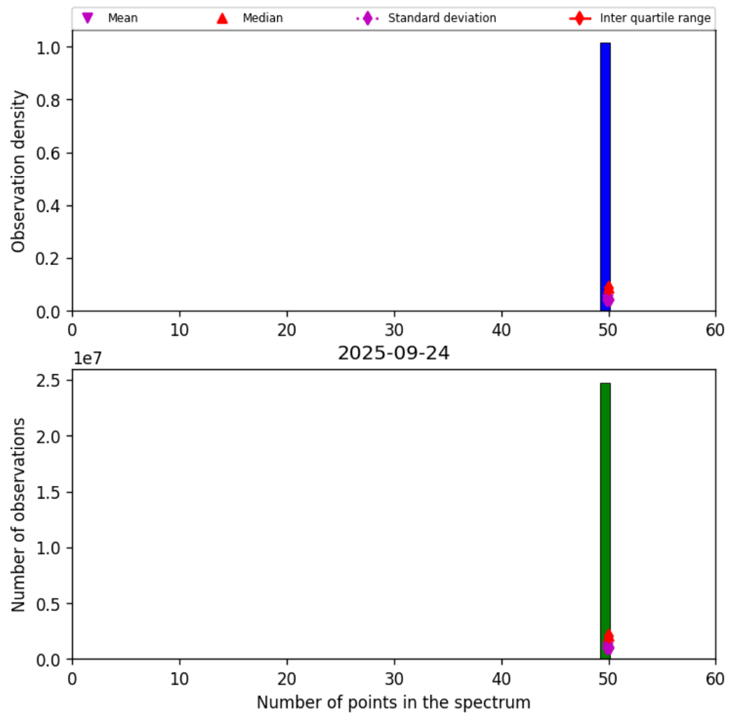
Figure 42: Histogram of “Number of points in the spectrum” for 2025-09-24 to 2025-09-25
