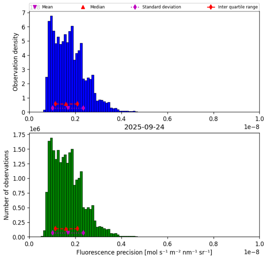
Figure 39: Histogram of “Fluorescence precision” for 2025-09-24 to 2025-09-25
