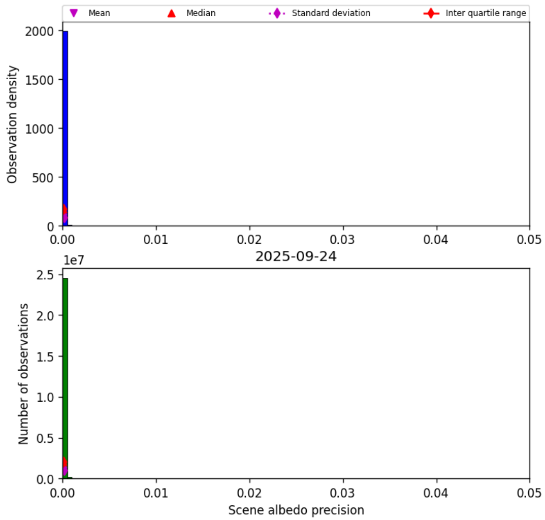
Figure 33: Histogram of “Scene albedo precision” for 2025-09-24 to 2025-09-25
