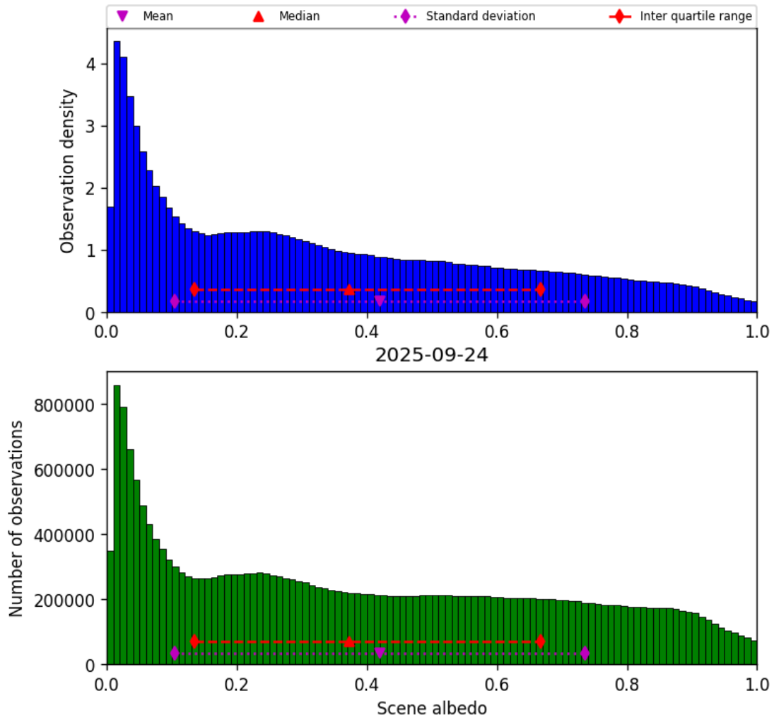
Figure 32: Histogram of “Scene albedo” for 2025-09-24 to 2025-09-25
