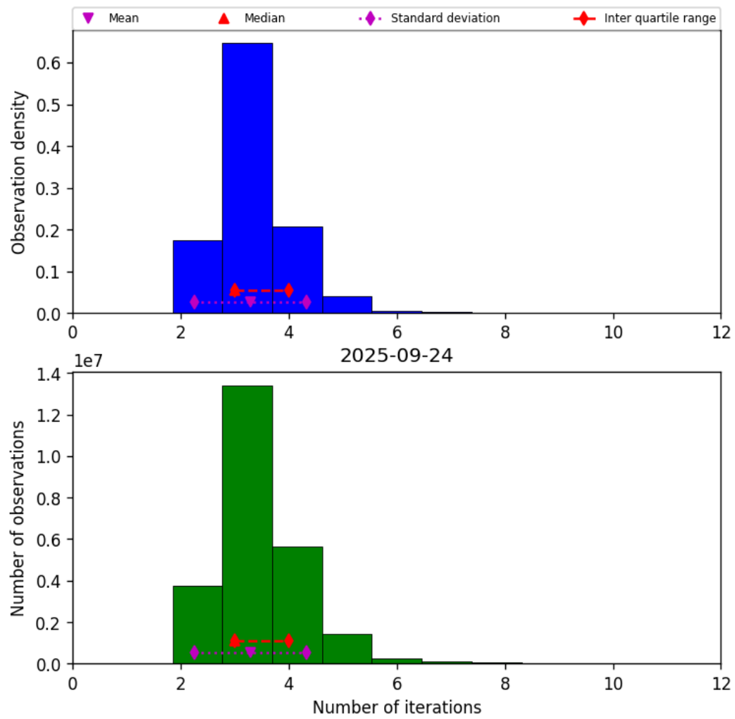
Figure 37: Histogram of “Number of iterations” for 2025-09-24 to 2025-09-25
