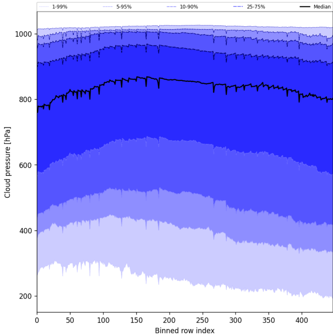
Figure 45: Along track statistics of “Cloud pressure” for 2025-09-24 to 2025-09-25
