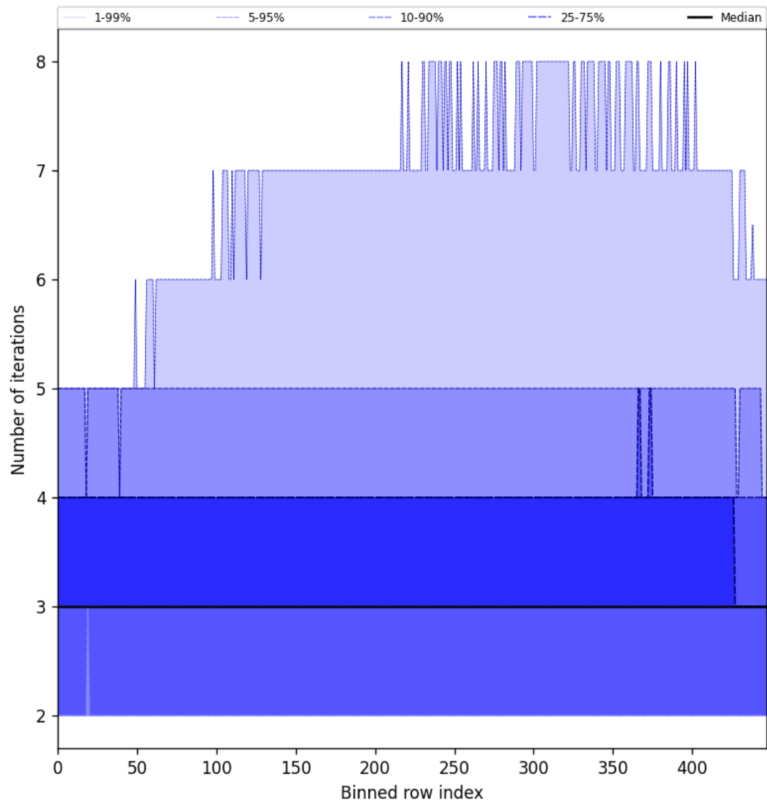
Figure 54: Along track statistics of “Number of iterations” for 2025-09-24 to 2025-09-25
