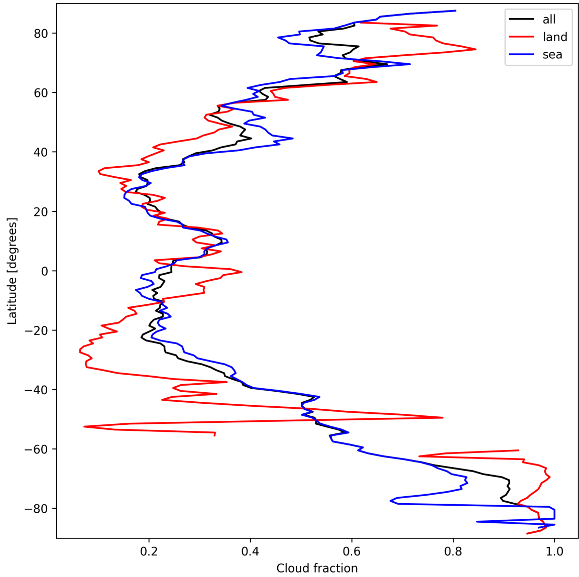
Figure 13: Zonal average of “Cloud fraction” for 2025-09-24 to 2025-09-25.
