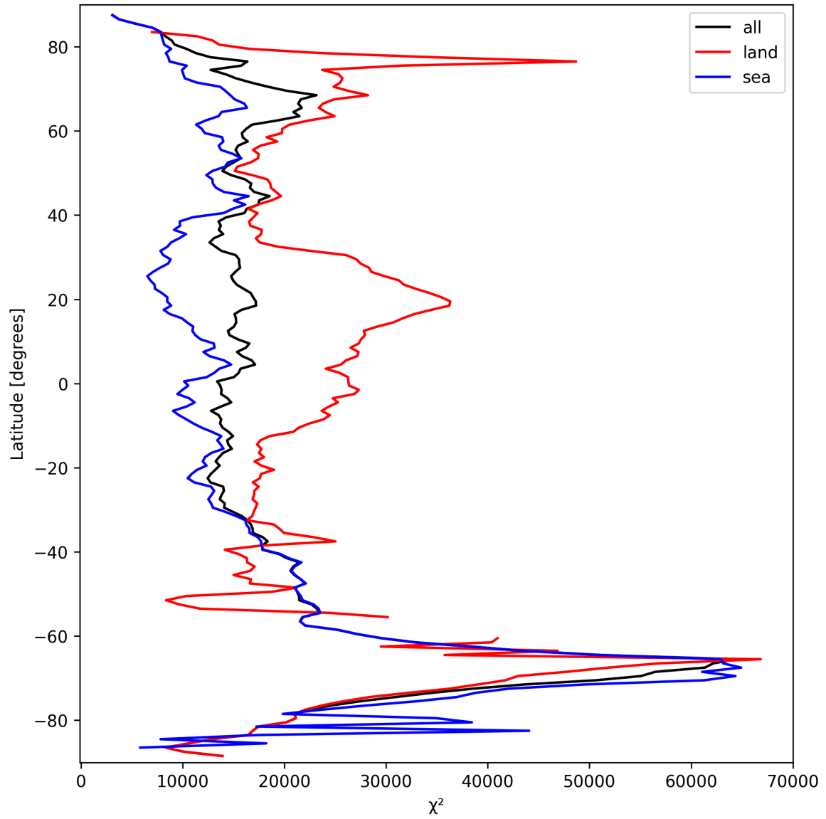
Figure 19: Zonal average of “ \chi^2 ” for 2025-09-24 to 2025-09-25.
