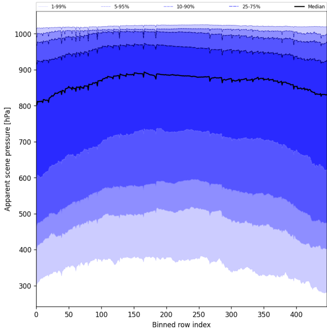
Figure 51: Along track statistics of “Apparent scene pressure” for 2025-09-24 to 2025-09-25
