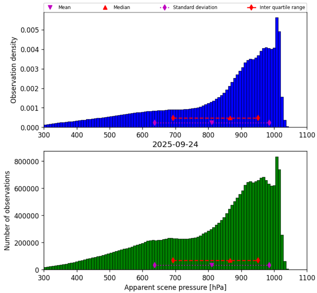
Figure 34: Histogram of “Apparent scene pressure” for 2025-09-24 to 2025-09-25
