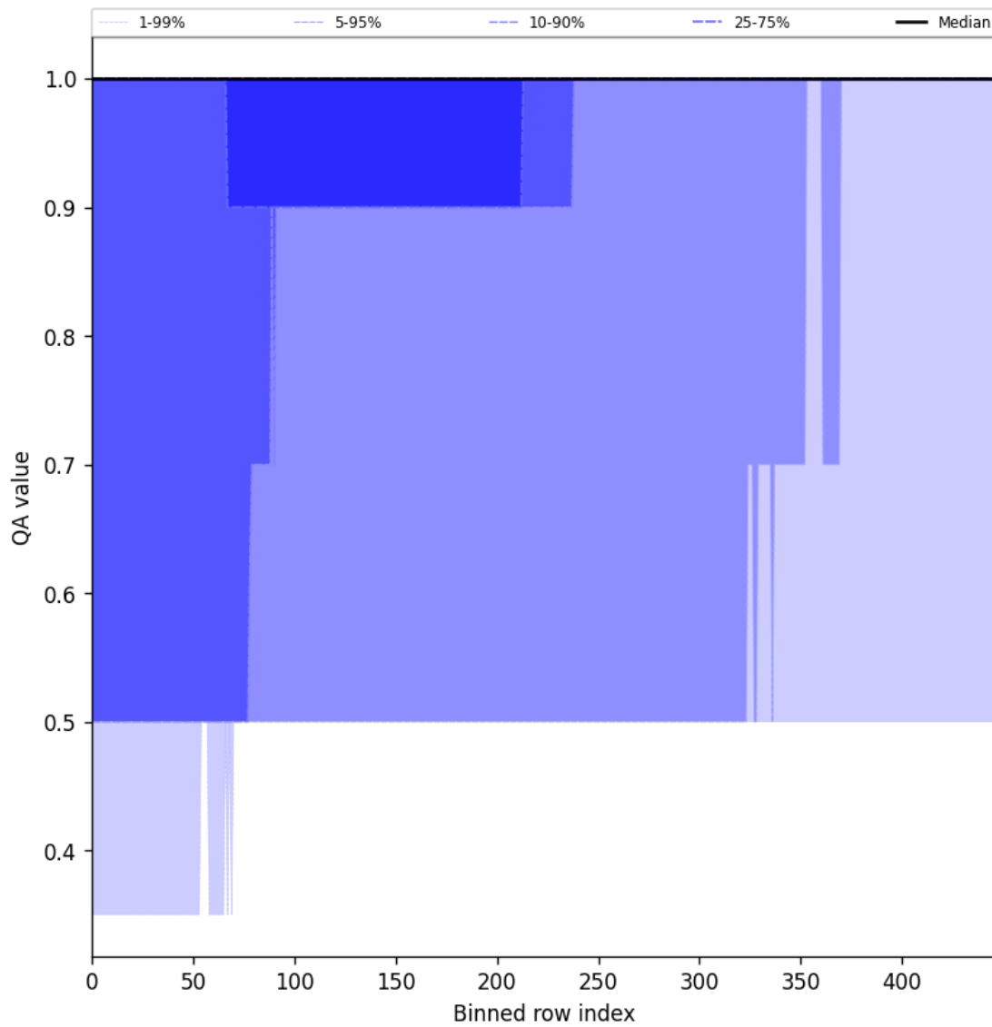
Figure 44: Along track statistics of “QA value” for 2025-09-24 to 2025-09-25
