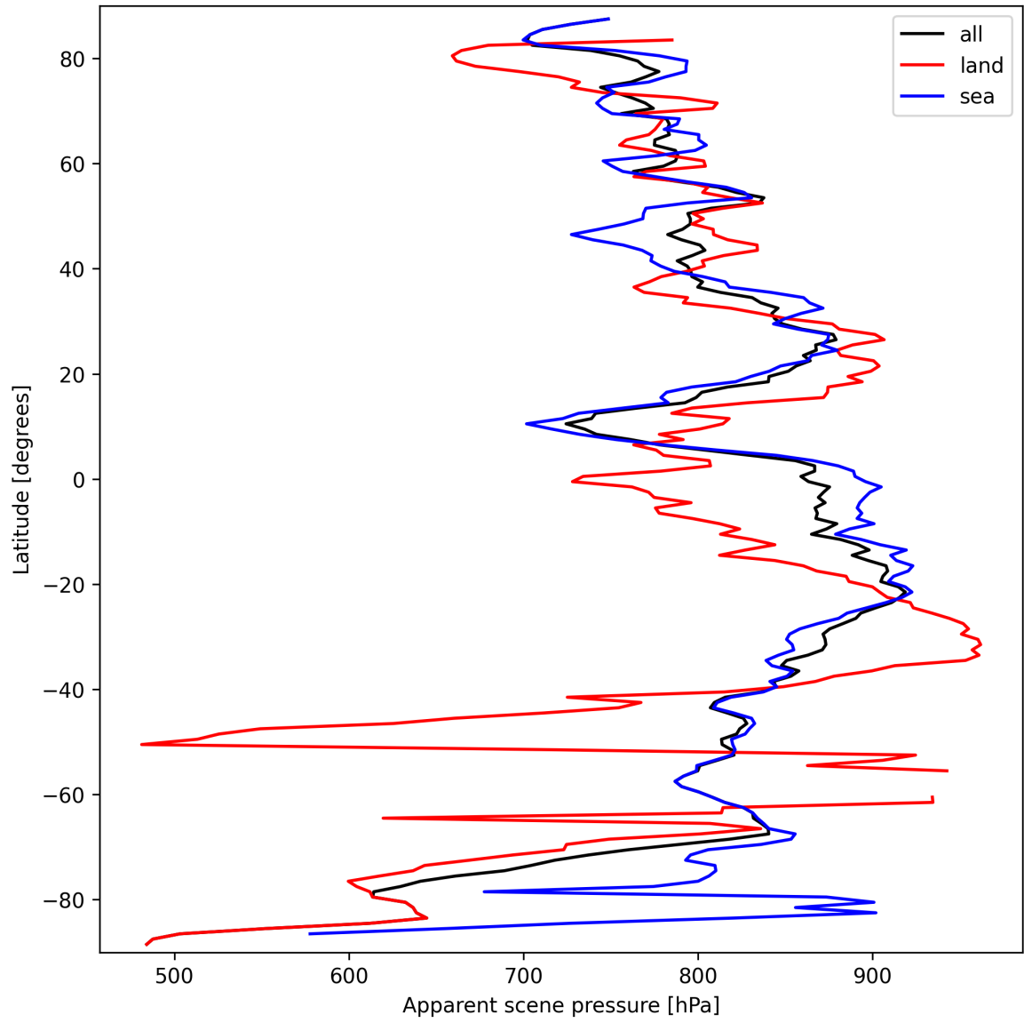
Figure 17: Zonal average of “Apparent scene pressure” for 2025-09-24 to 2025-09-25.
