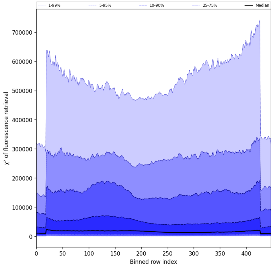
Figure 57: Along track statistics of “ \chi^2 of fluorescence retrieval” for 2025-09-24 to 2025-09-25
