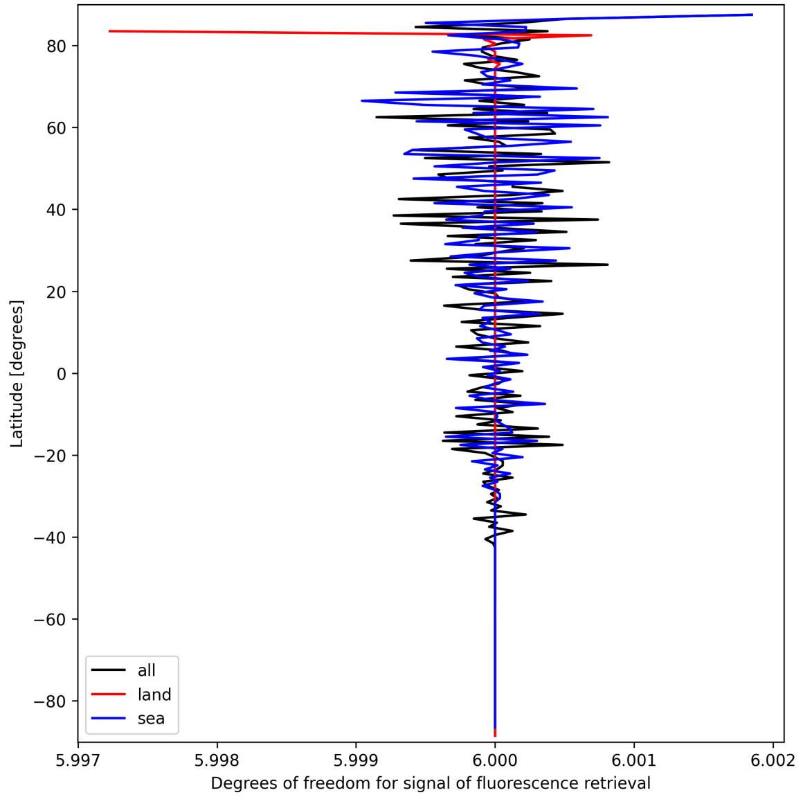
Figure 24: Zonal average of “Degrees of freedom for signal of fluorescence retrieval” for 2025-09-24 to 2025-09-25.
