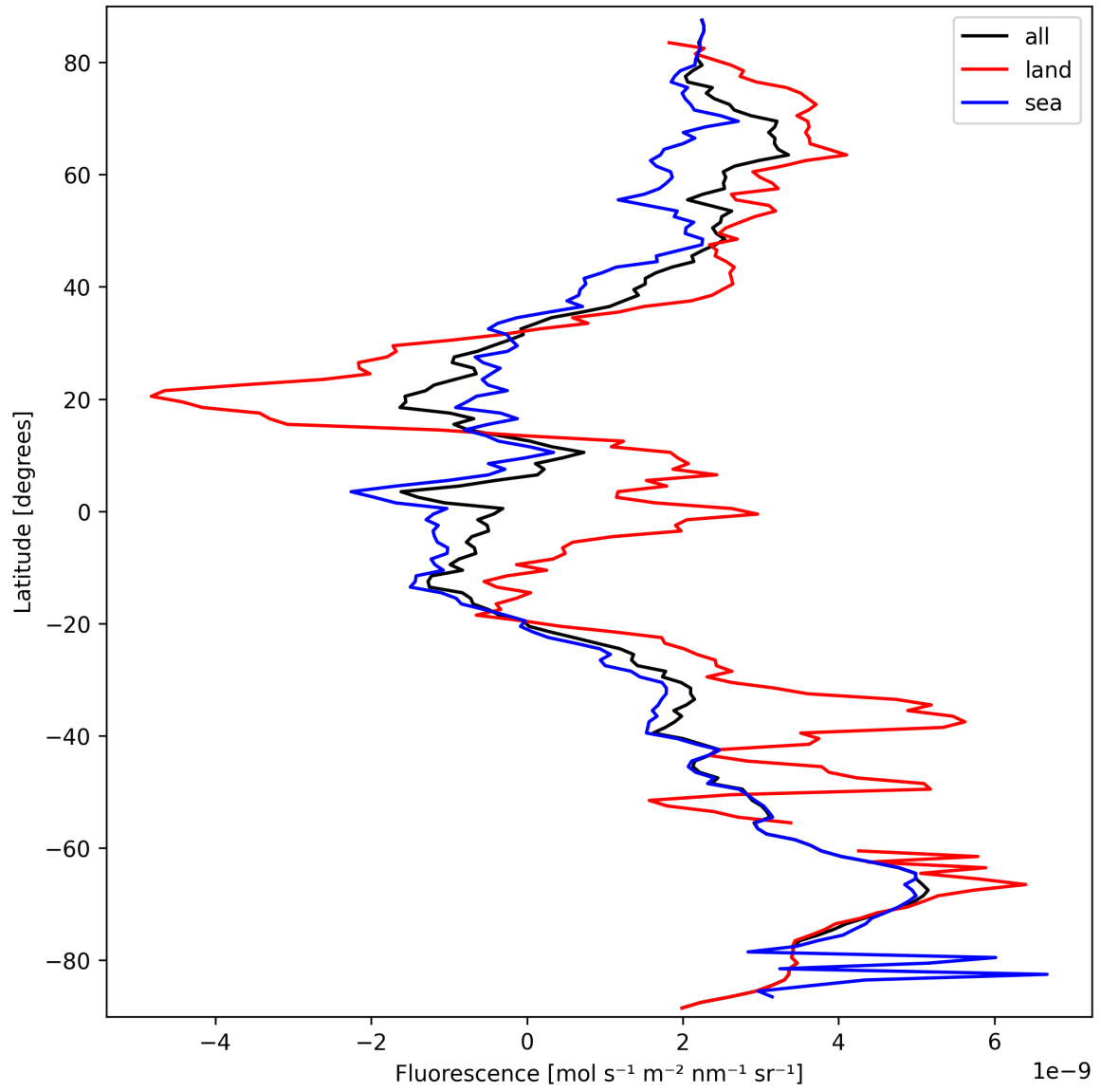
Figure 21: Zonal average of “Fluorescence” for 2025-09-24 to 2025-09-25.
