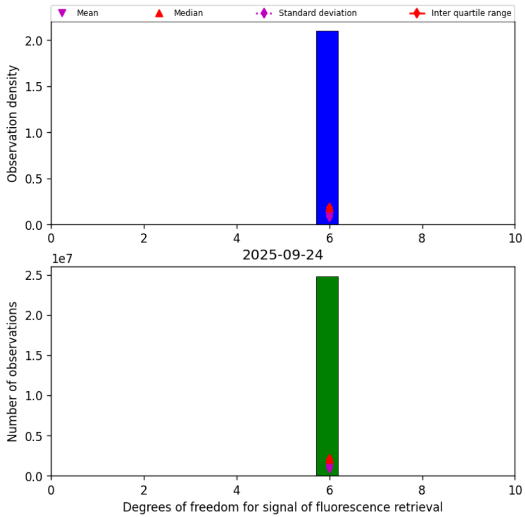
Figure 41: Histogram of “Degrees of freedom for signal of fluorescence retrieval” for 2025-09-24 to 2025-09-25
