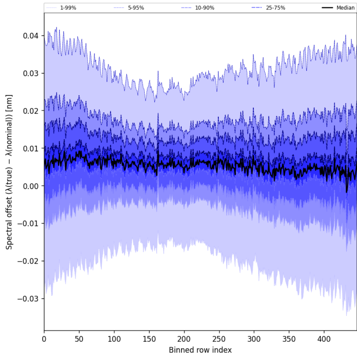
Figure 60: Along track statistics of “Spectral offset ( \lambda_{\text{true}} - \lambda_{\text{nominal}} )” for 2025-09-24 to 2025-09-25
