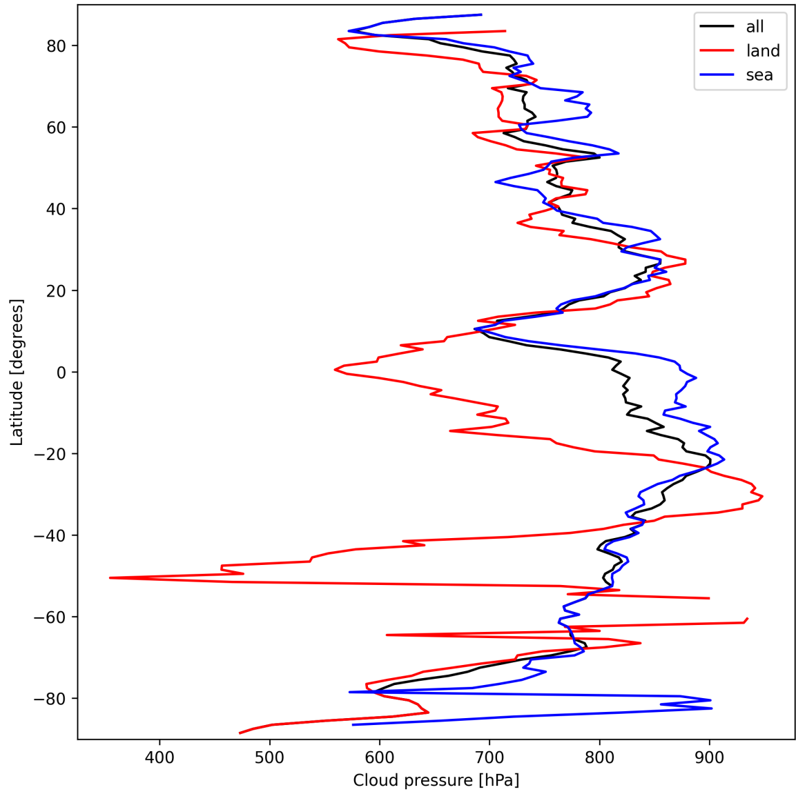
Figure 11: Zonal average of “Cloud pressure” for 2025-09-24 to 2025-09-25.
