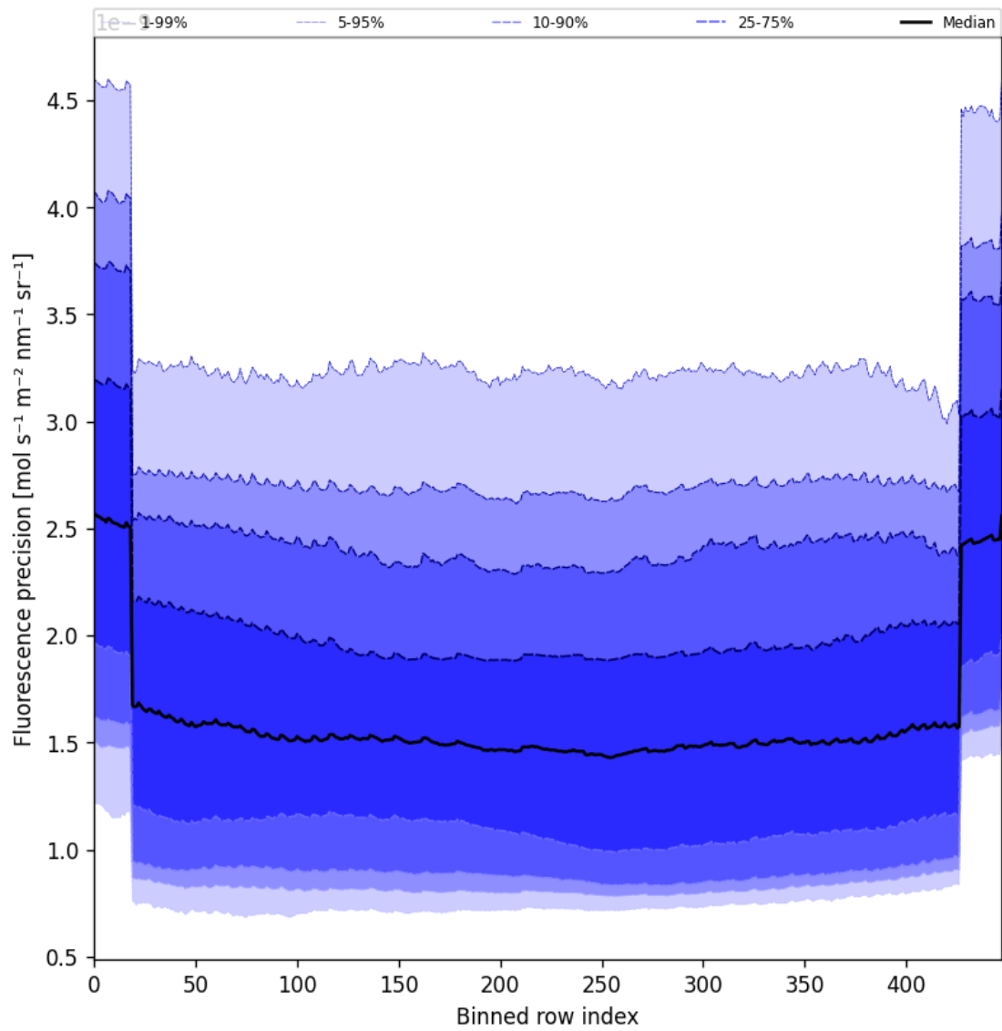
Figure 56: Along track statistics of “Fluorescence precision” for 2025-09-24 to 2025-09-25
