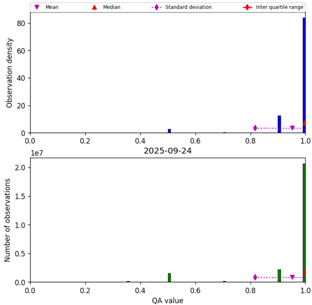
Figure 27: Histogram of “QA value” for 2025-09-24 to 2025-09-25
