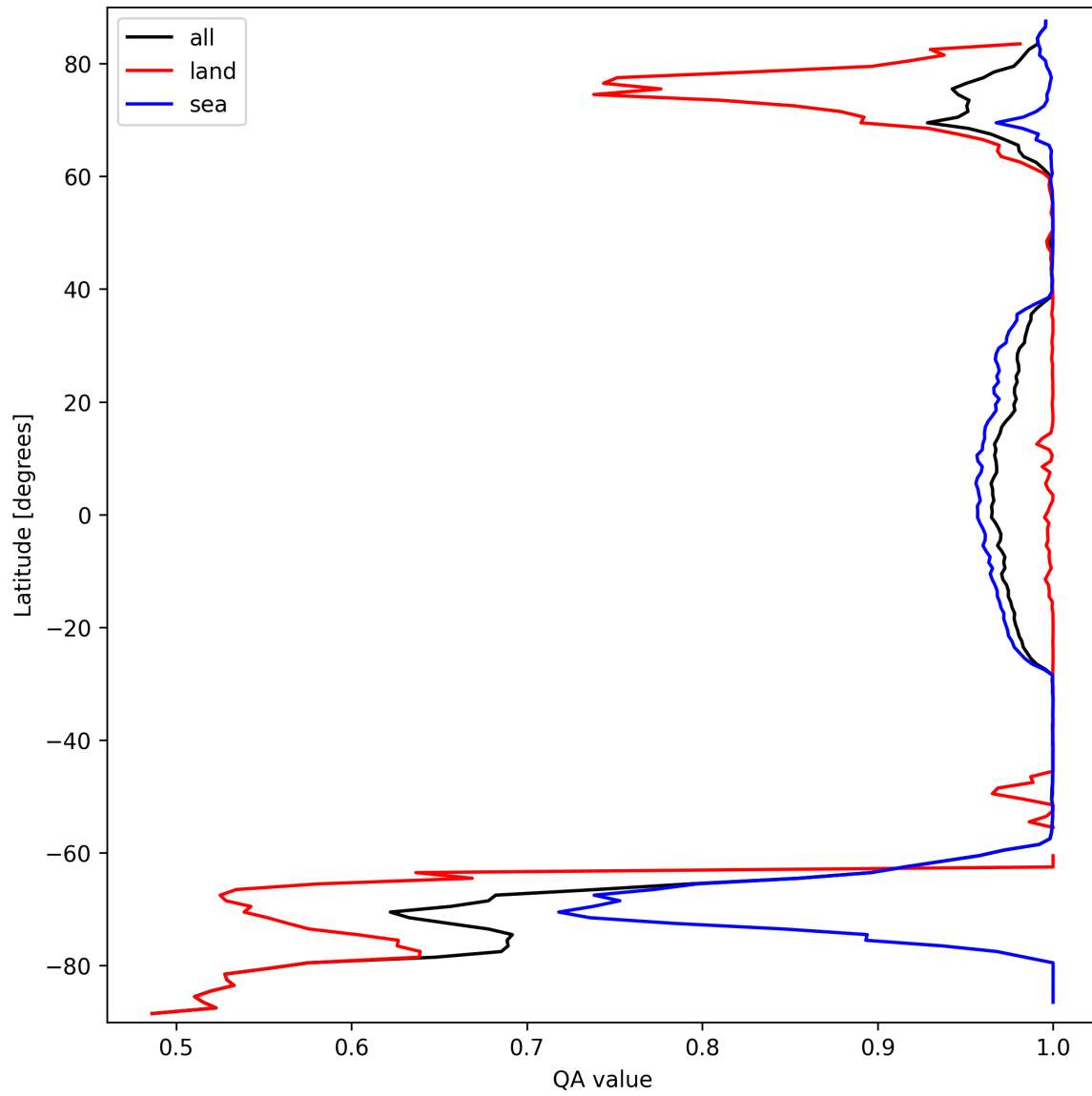
Figure 10: Zonal average of “QA value” for 2025-09-24 to 2025-09-25.
