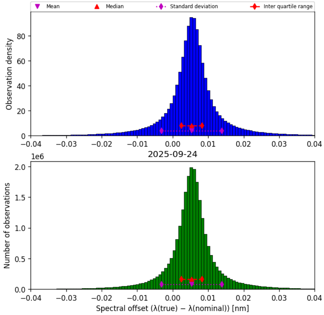
Figure 43: Histogram of “Spectral offset ( \lambda_{\text{true}} - \lambda_{\text{nominal}} )” for 2025-09-24 to 2025-09-25
