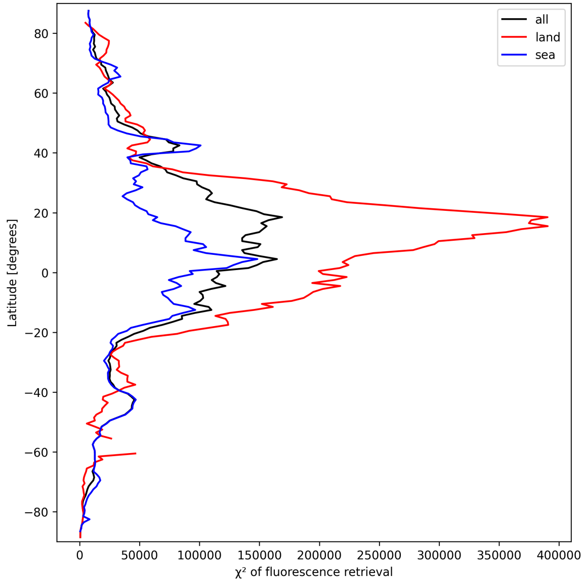
Figure 23: Zonal average of “ \chi^2 of fluorescence retrieval” for 2025-09-24 to 2025-09-25.
