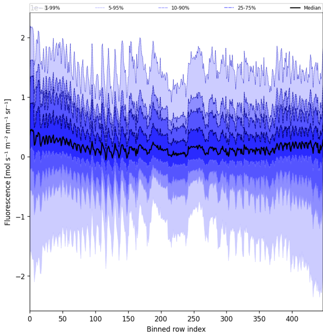
Figure 55: Along track statistics of "Fluorescence" for 2025-09-24 to 2025-09-25
