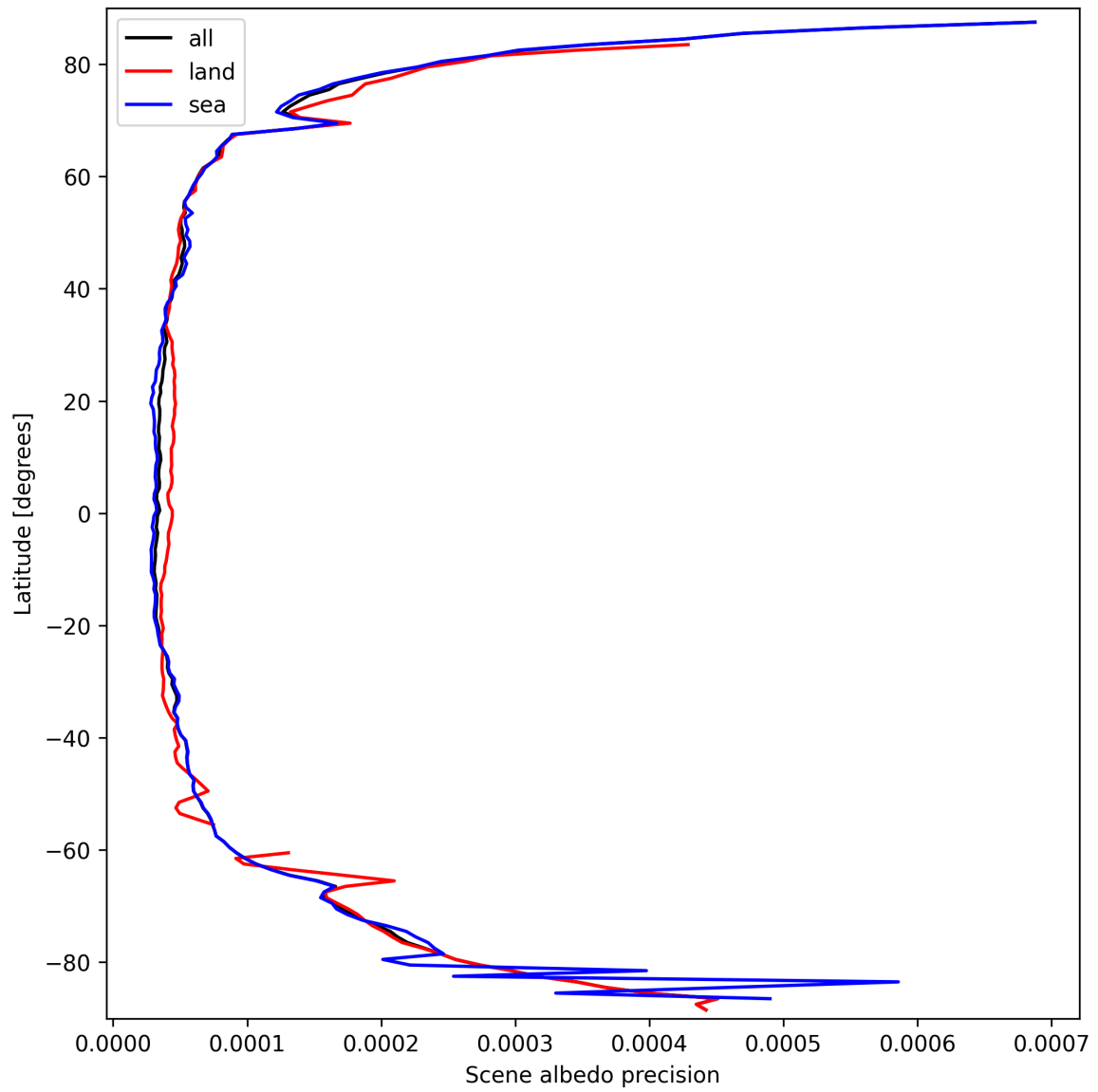
Figure 16: Zonal average of “Scene albedo precision” for 2025-09-24 to 2025-09-25.
