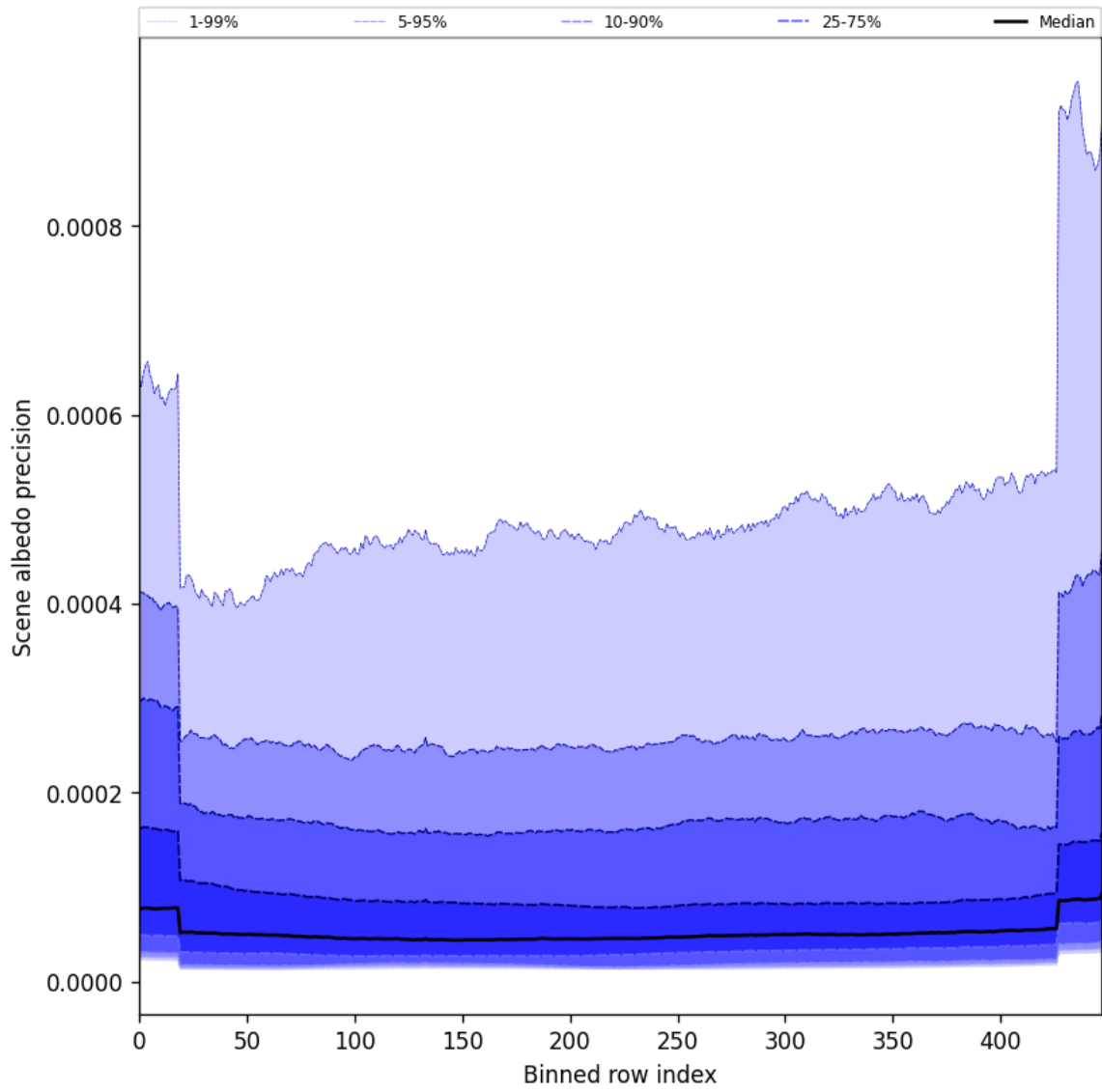
Figure 50: Along track statistics of “Scene albedo precision” for 2025-09-24 to 2025-09-25
