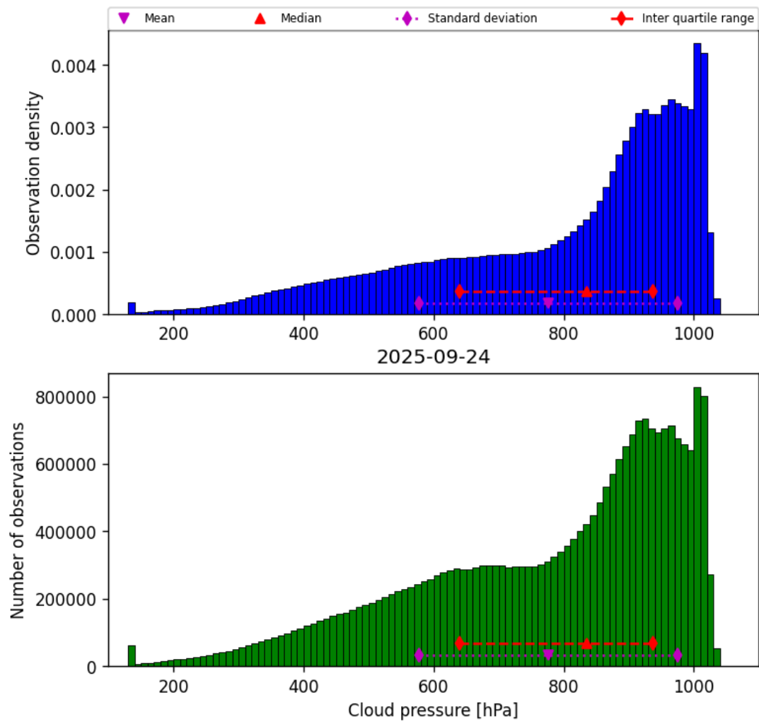
Figure 28: Histogram of “Cloud pressure” for 2025-09-24 to 2025-09-25
