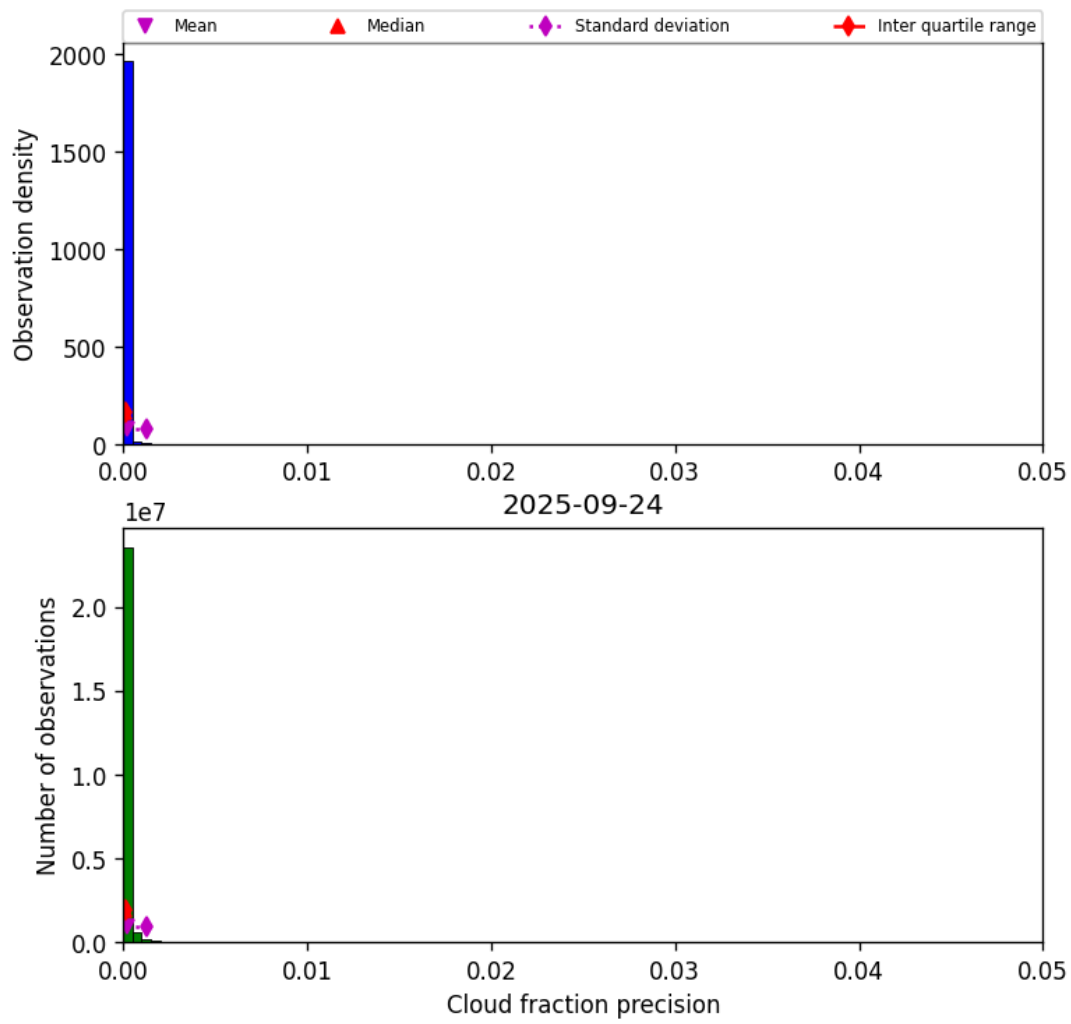
Figure 31: Histogram of “Cloud fraction precision” for 2025-09-24 to 2025-09-25
