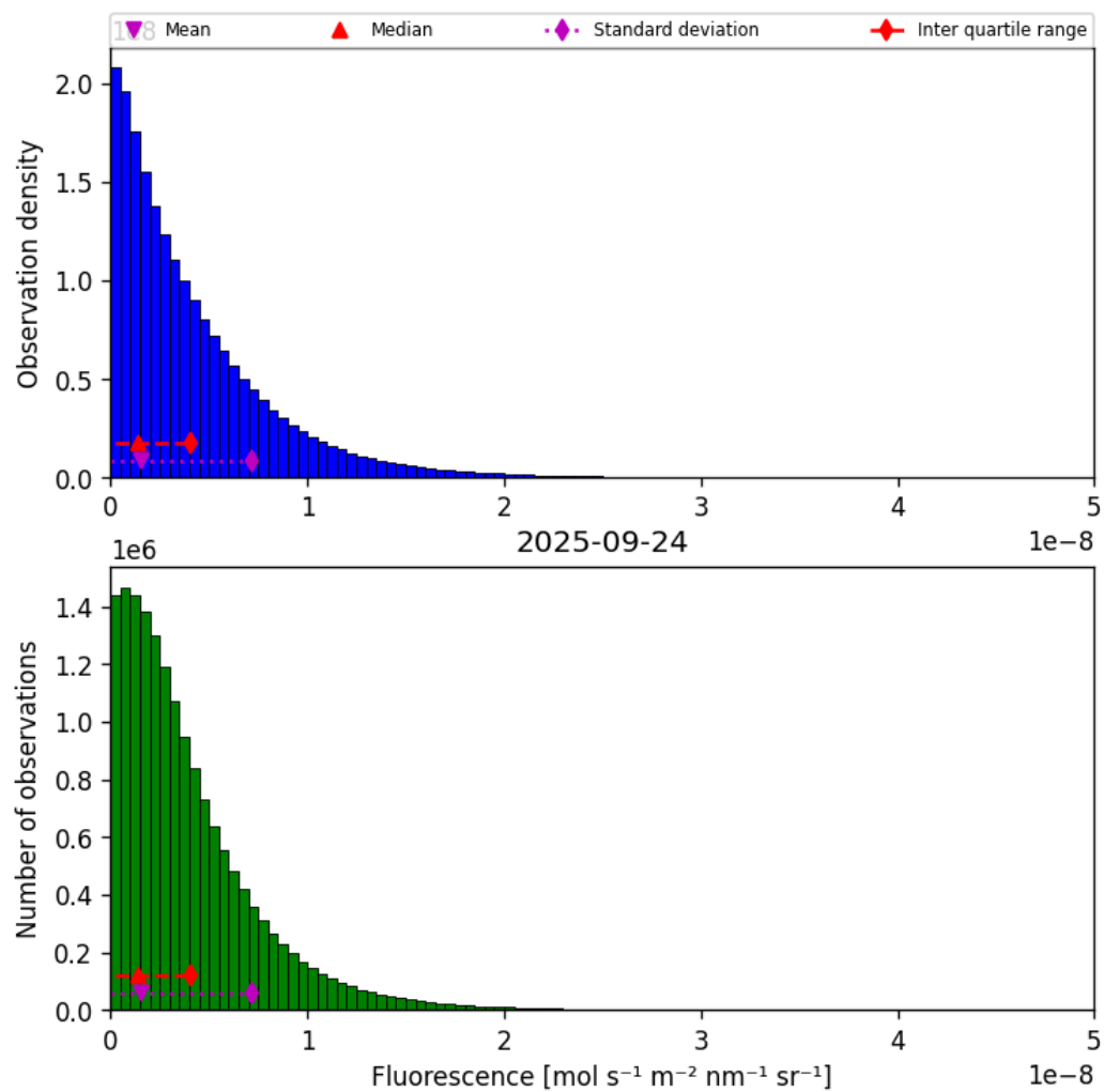
Figure 38: Histogram of “Fluorescence” for 2025-09-24 to 2025-09-25
