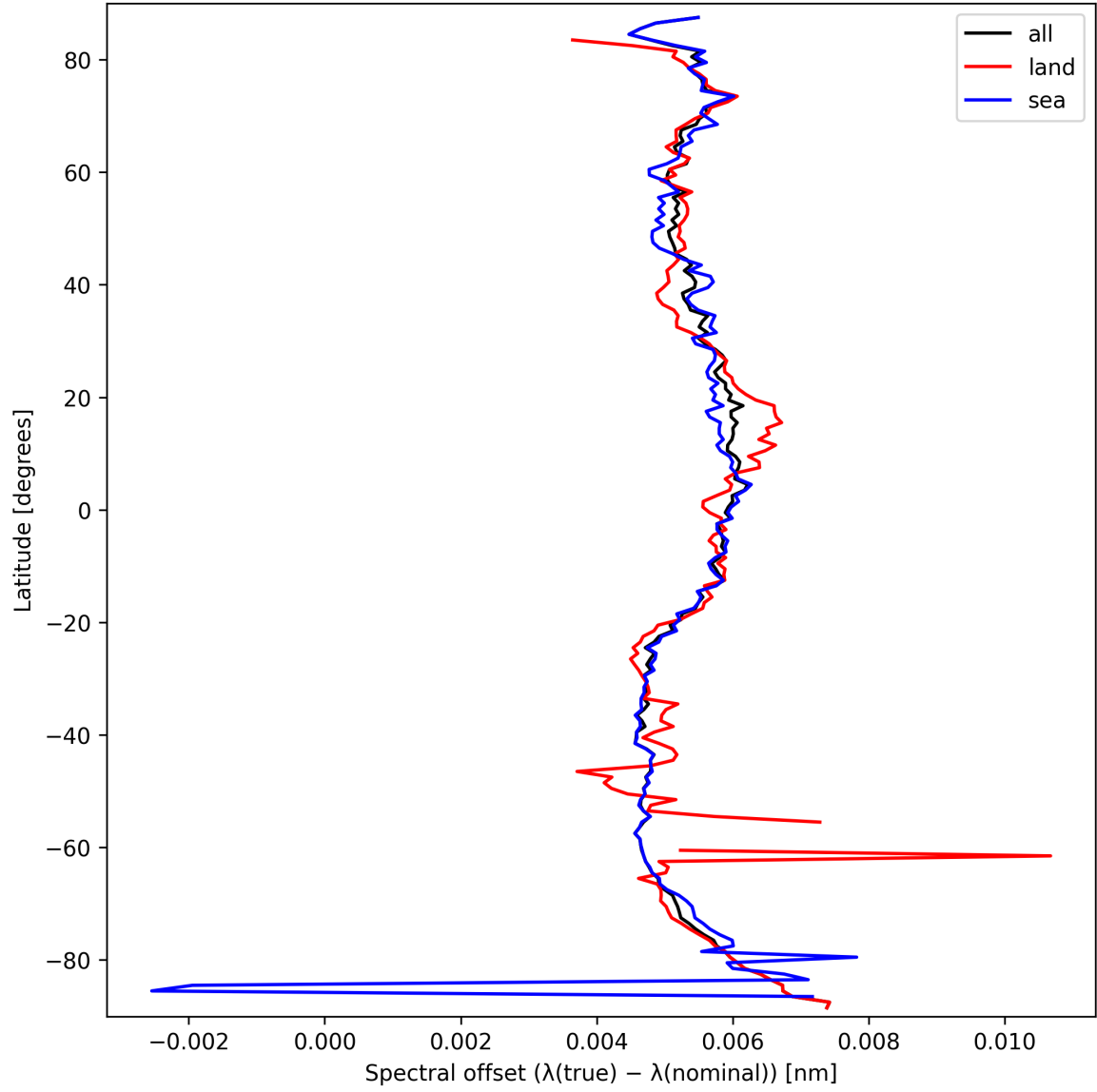
Figure 26: Zonal average of “Spectral offset ( \lambda_{\text{true}} - \lambda_{\text{nominal}} )” for 2025-09-24 to 2025-09-25.
