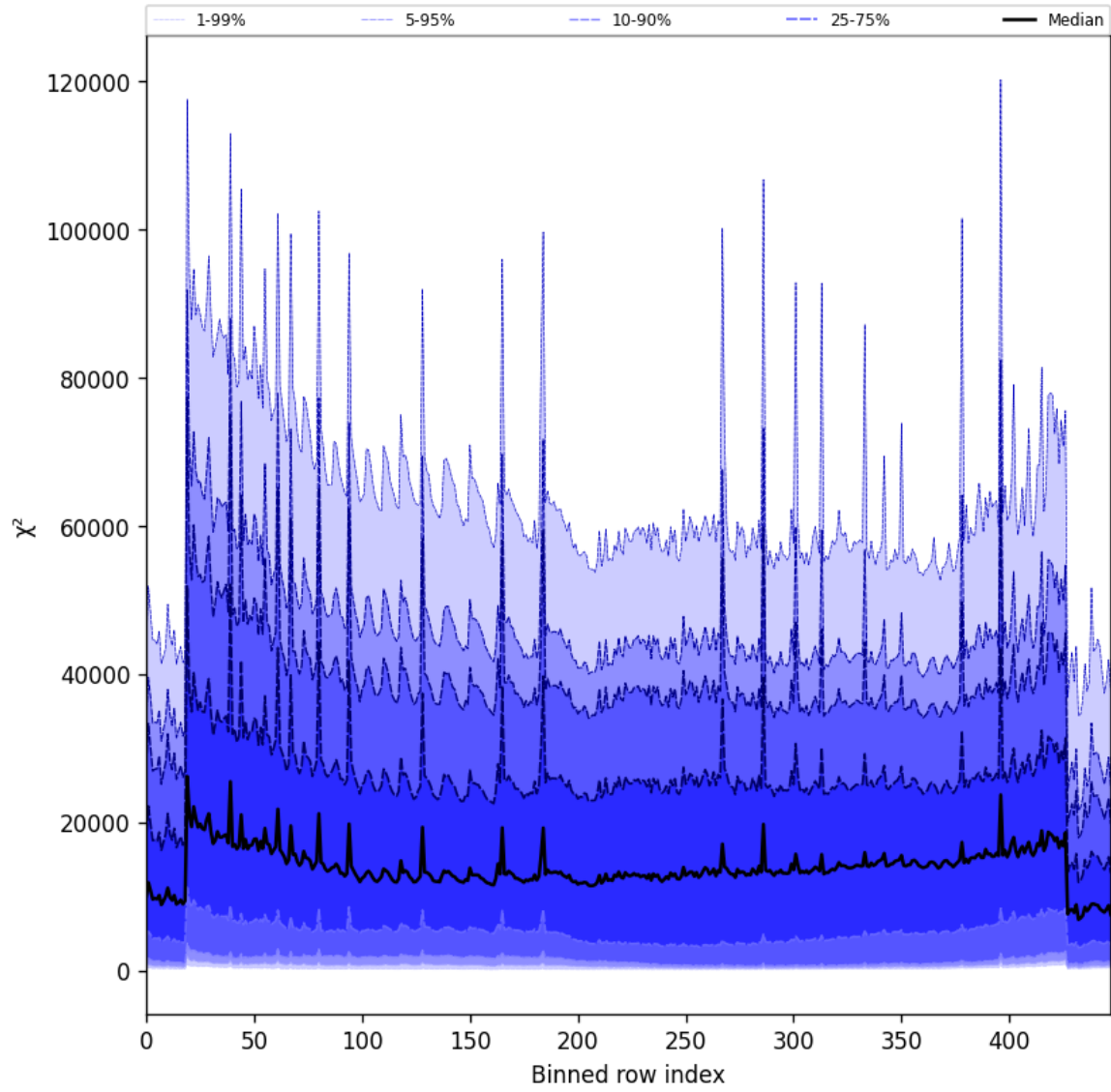
Figure 53: Along track statistics of “ \chi^2 ” for 2025-09-24 to 2025-09-25
