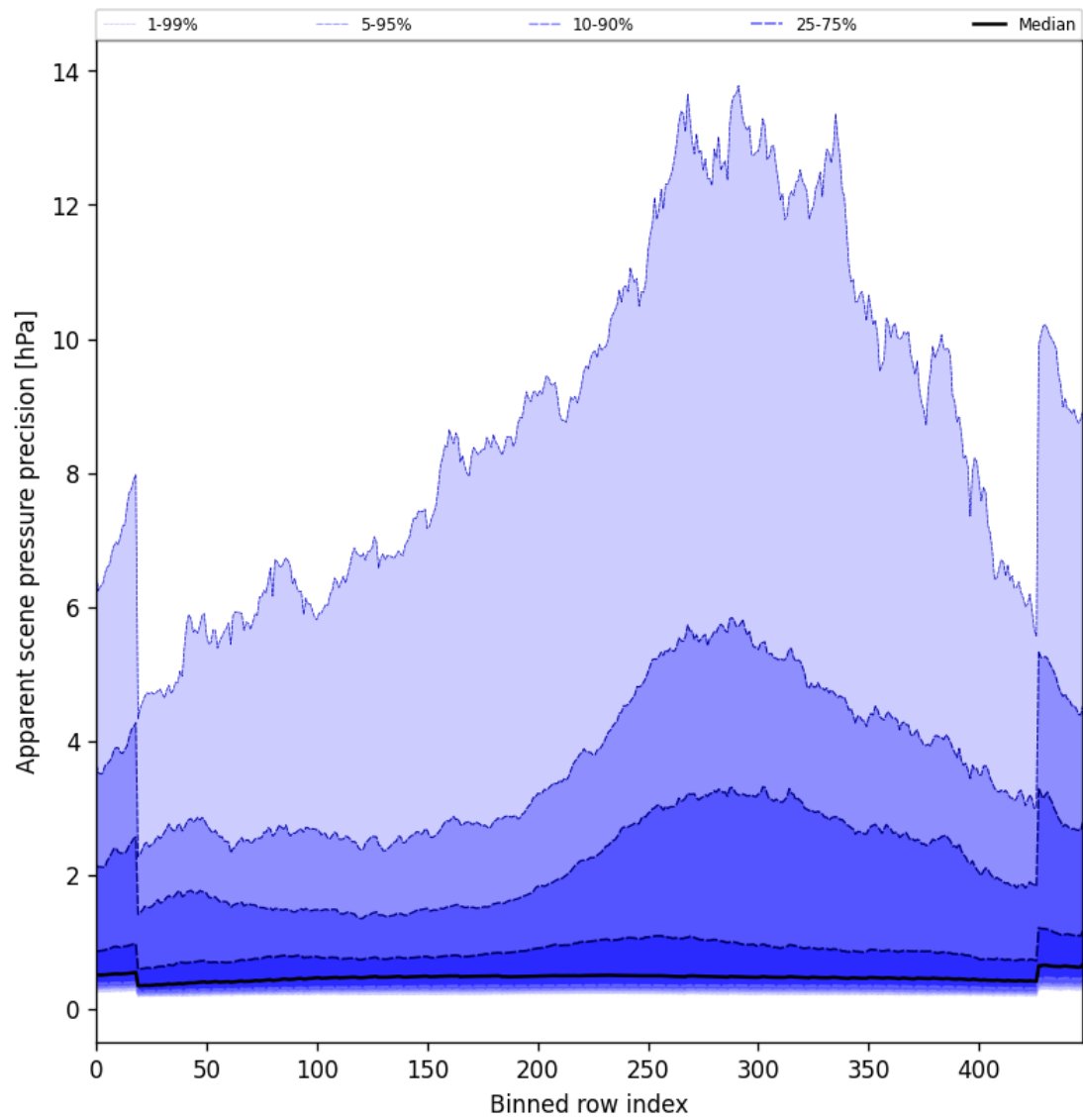
Figure 52: Along track statistics of “Apparent scene pressure precision” for 2025-09-24 to 2025-09-25
