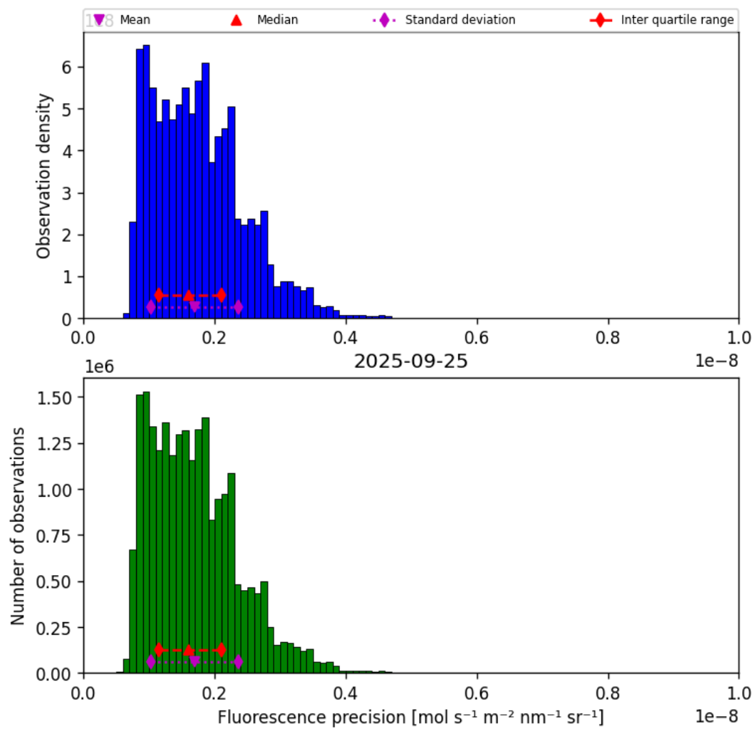
Figure 39: Histogram of “Fluorescence precision” for 2025-09-25 to 2025-09-26
