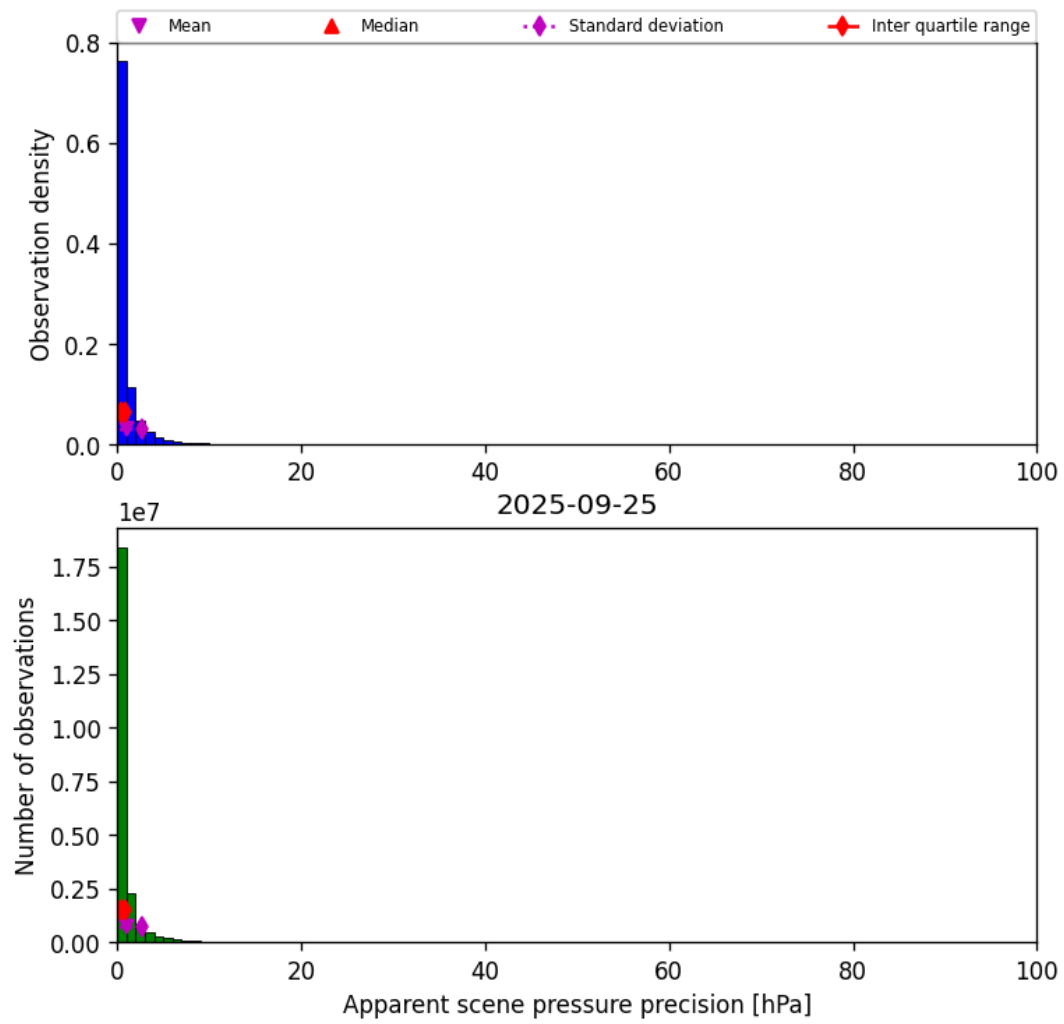
Figure 35: Histogram of “Apparent scene pressure precision” for 2025-09-25 to 2025-09-26
