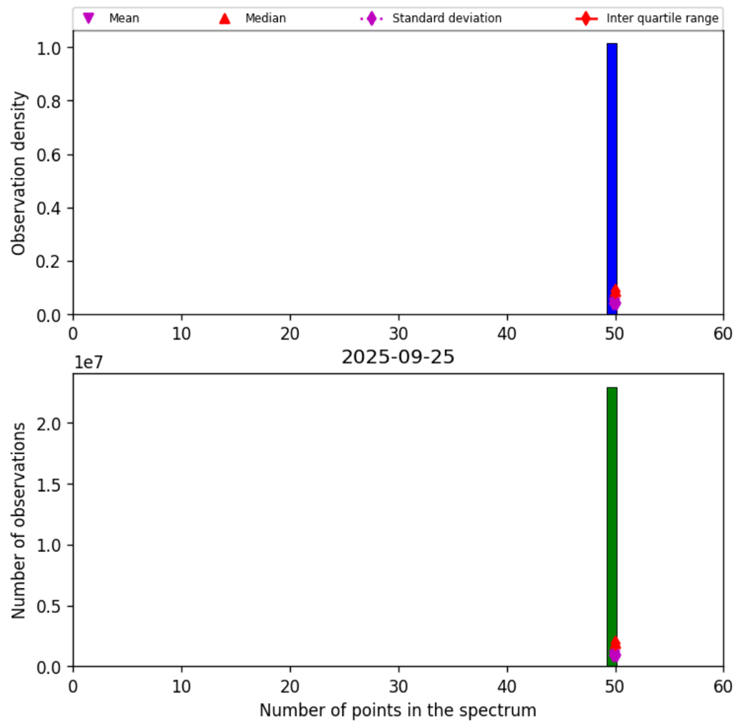
Figure 42: Histogram of “Number of points in the spectrum” for 2025-09-25 to 2025-09-26
