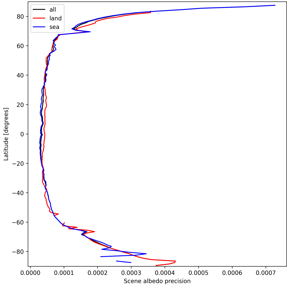
Figure 16: Zonal average of “Scene albedo precision” for 2025-09-25 to 2025-09-26.
