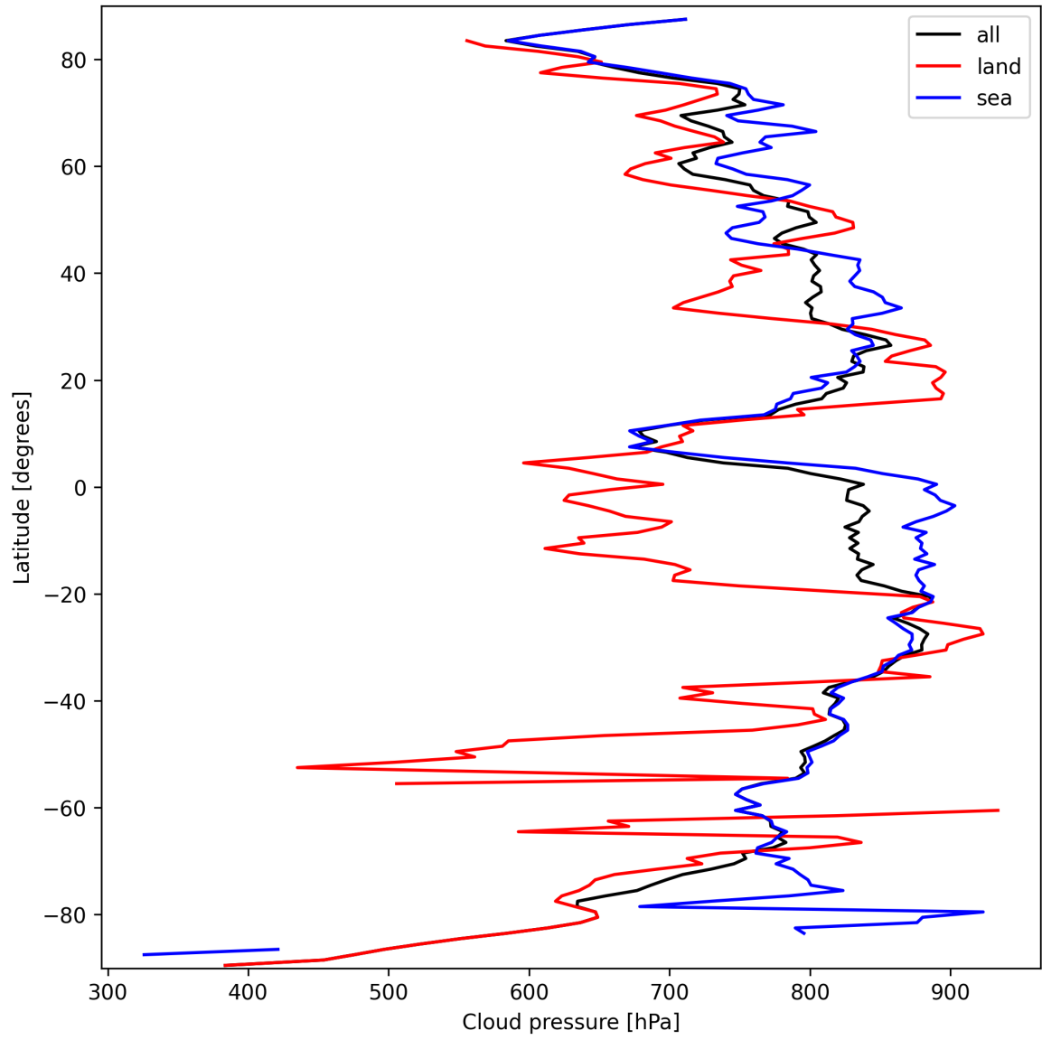
Figure 11: Zonal average of “Cloud pressure” for 2025-09-25 to 2025-09-26.
