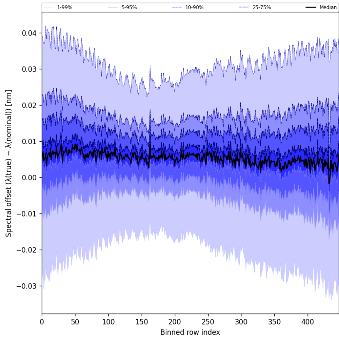
Figure 60: Along track statistics of “Spectral offset ( \lambda_{\text{true}} - \lambda_{\text{nominal}} )” for 2025-09-25 to 2025-09-26
