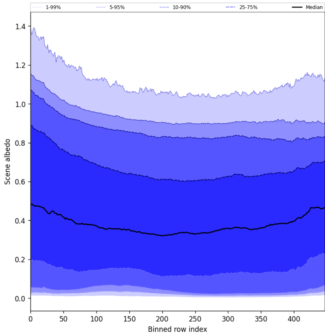
Figure 49: Along track statistics of “Scene albedo” for 2025-09-25 to 2025-09-26
