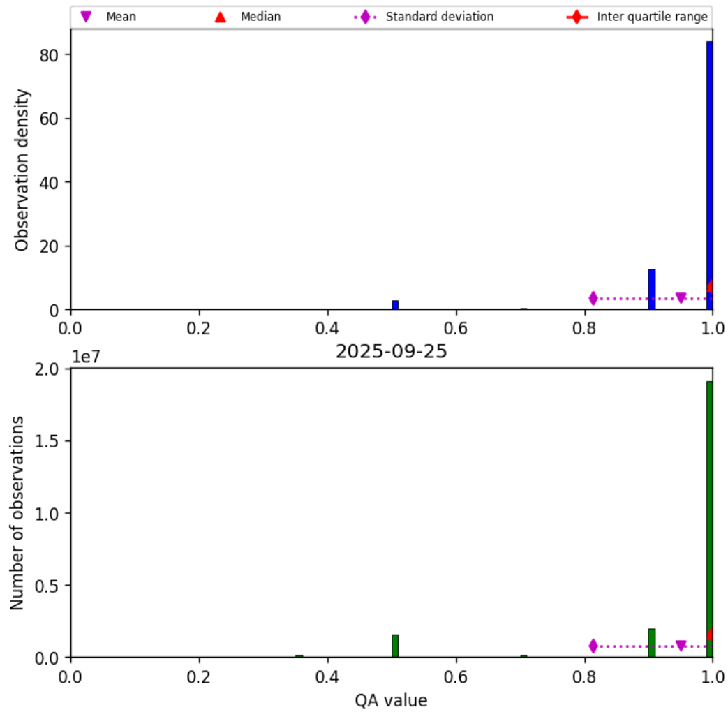
Figure 27: Histogram of "QA value" for 2025-09-25 to 2025-09-26
