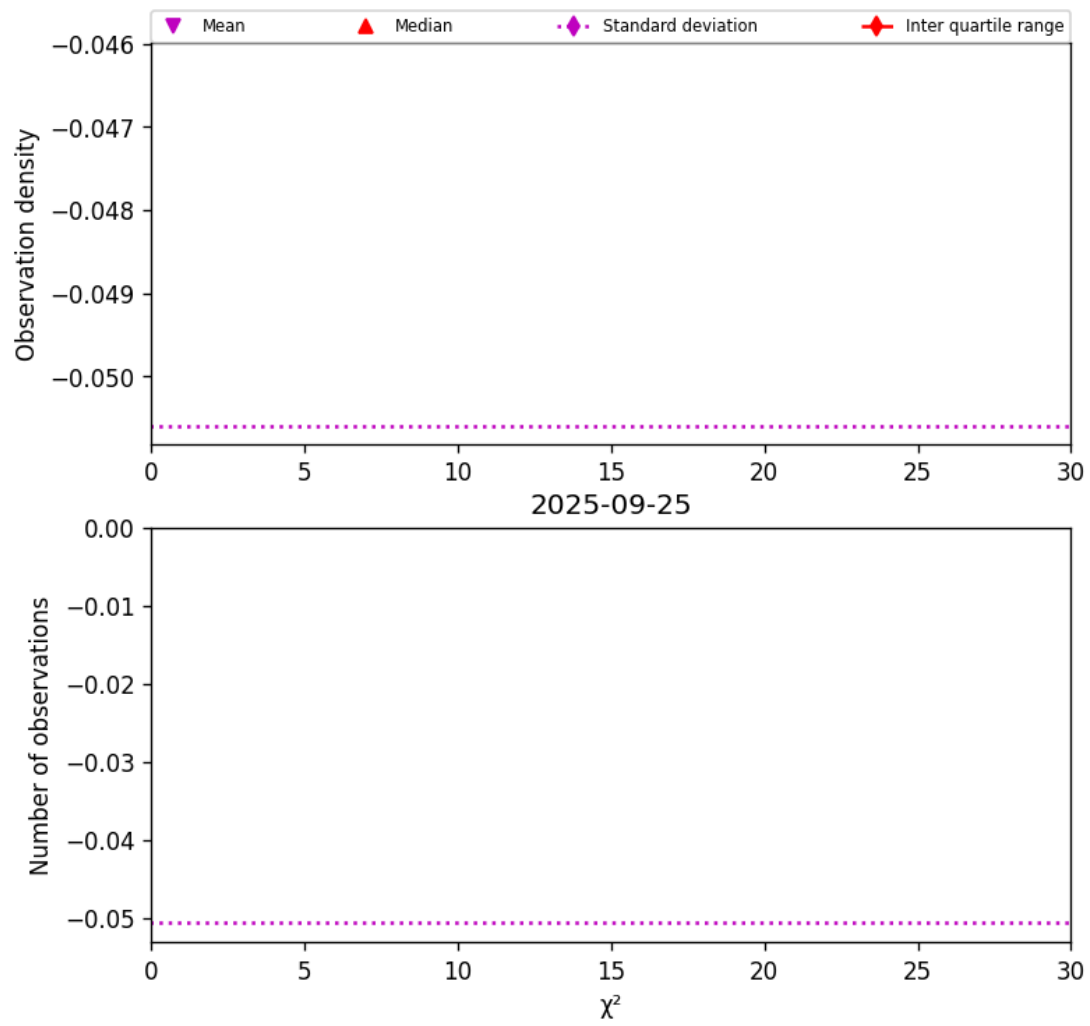
Figure 36: Histogram of " \chi^2 " for 2025-09-25 to 2025-09-26
