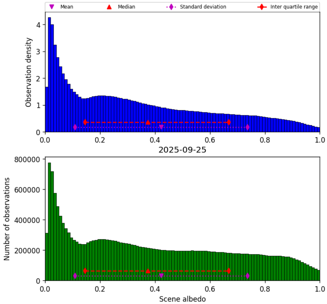
Figure 32: Histogram of “Scene albedo” for 2025-09-25 to 2025-09-26
