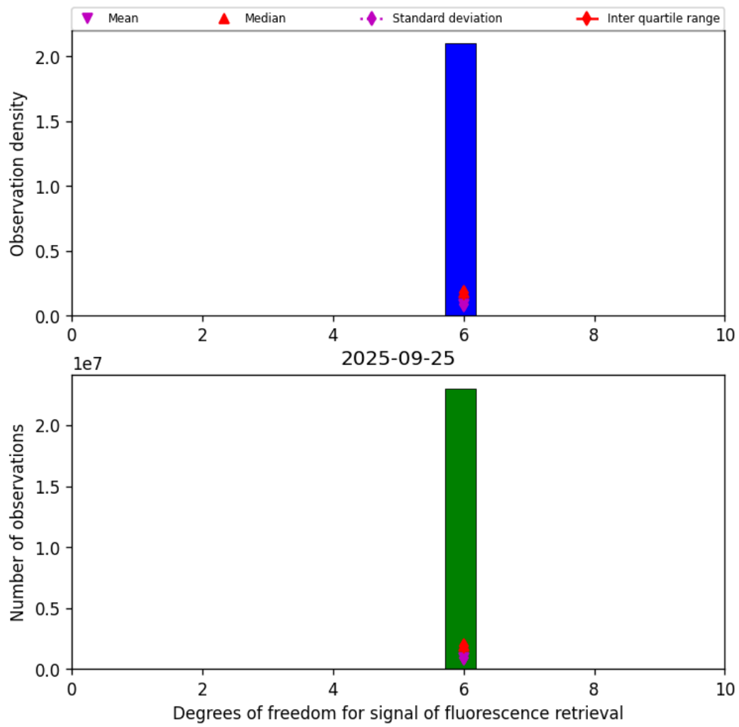
Figure 41: Histogram of “Degrees of freedom for signal of fluorescence retrieval” for 2025-09-25 to 2025-09-26
