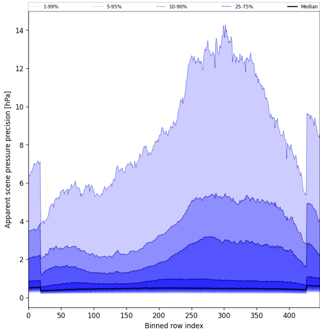
Figure 52: Along track statistics of “Apparent scene pressure precision” for 2025-09-25 to 2025-09-26
