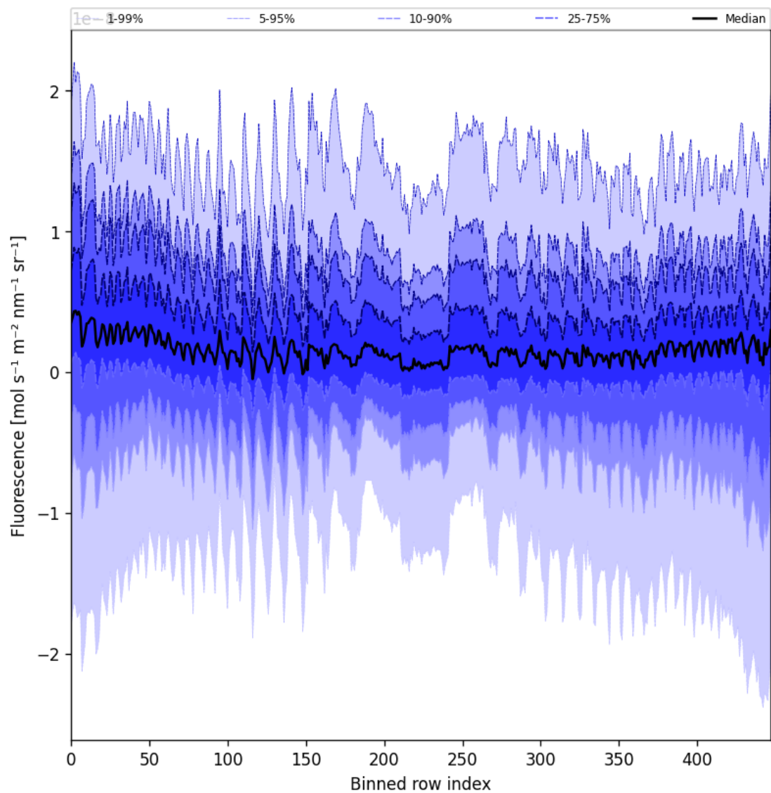
Figure 55: Along track statistics of "Fluorescence" for 2025-09-25 to 2025-09-26
