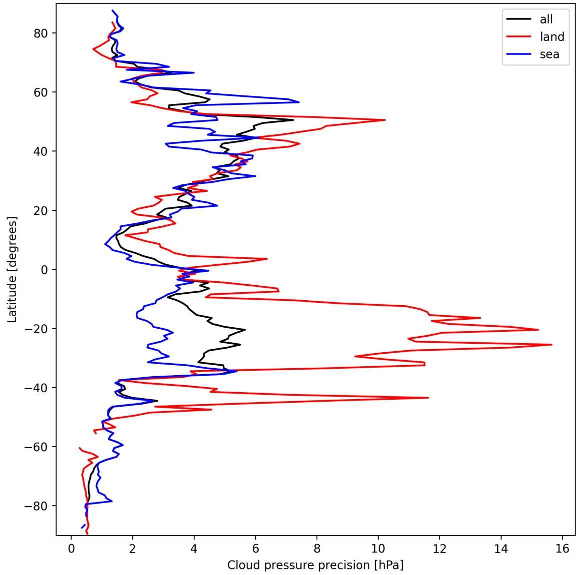
Figure 12: Zonal average of “Cloud pressure precision” for 2025-09-25 to 2025-09-26.
