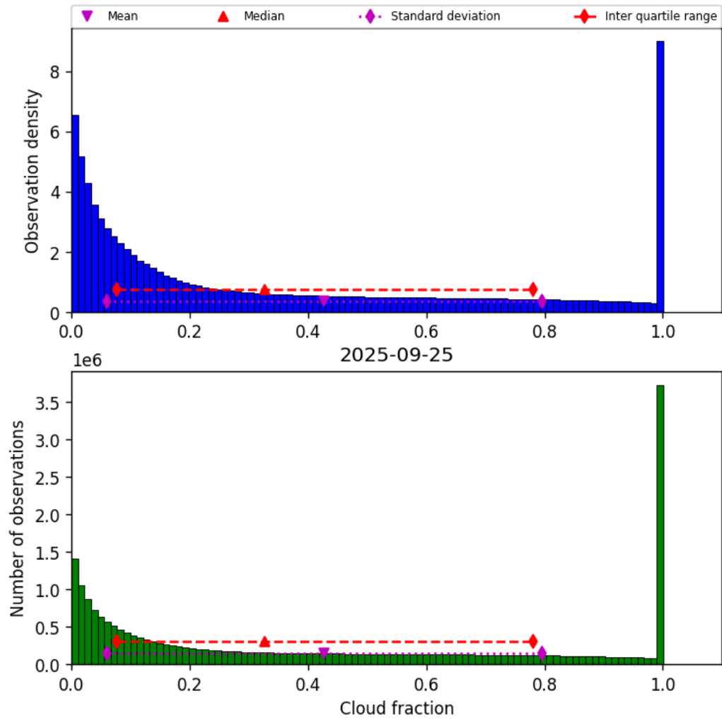
Figure 30: Histogram of “Cloud fraction” for 2025-09-25 to 2025-09-26
