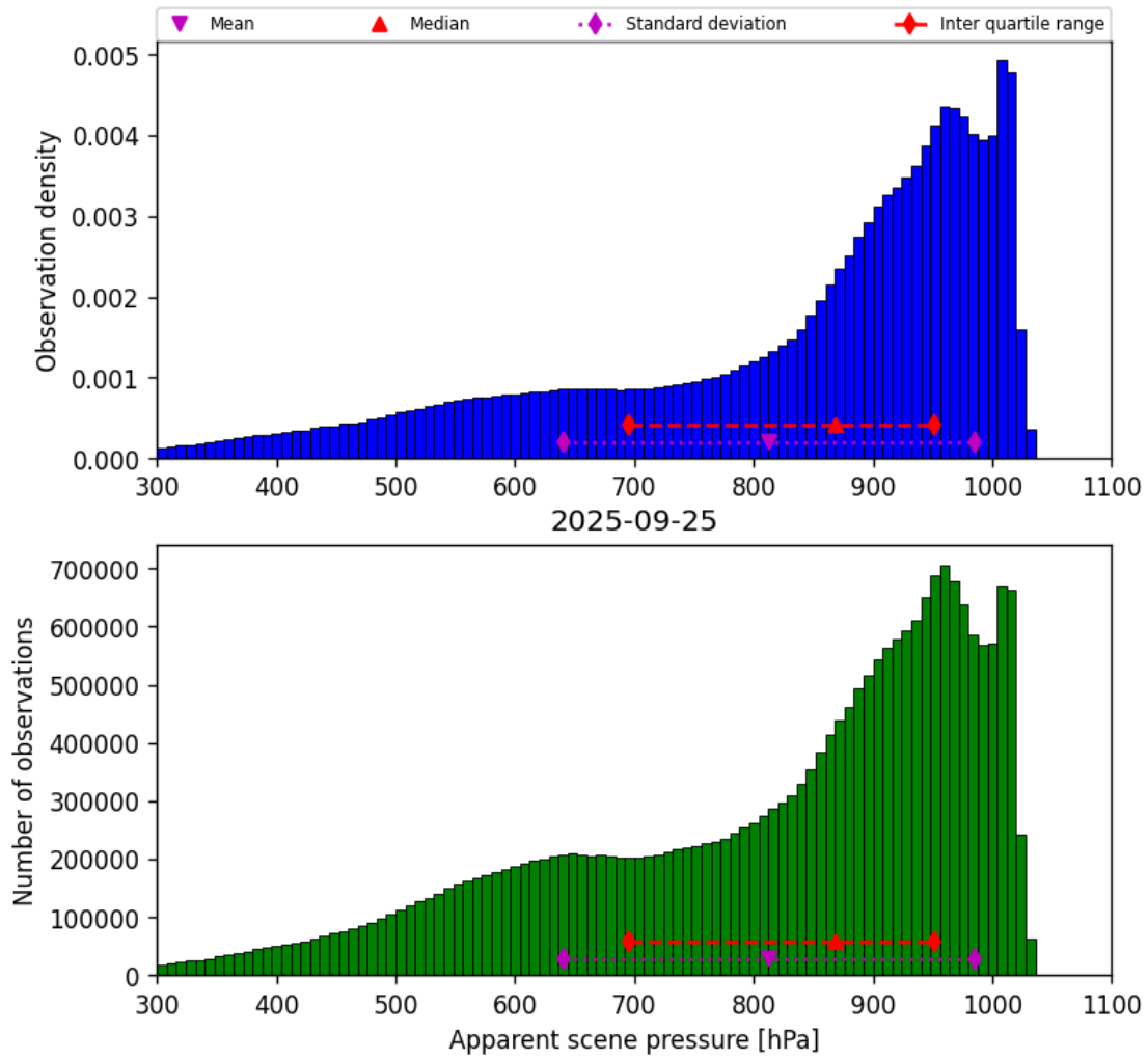
Figure 34: Histogram of “Apparent scene pressure” for 2025-09-25 to 2025-09-26
