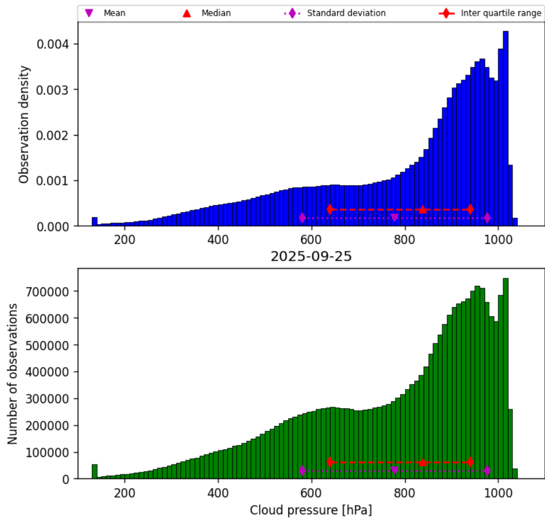
Figure 28: Histogram of “Cloud pressure” for 2025-09-25 to 2025-09-26
