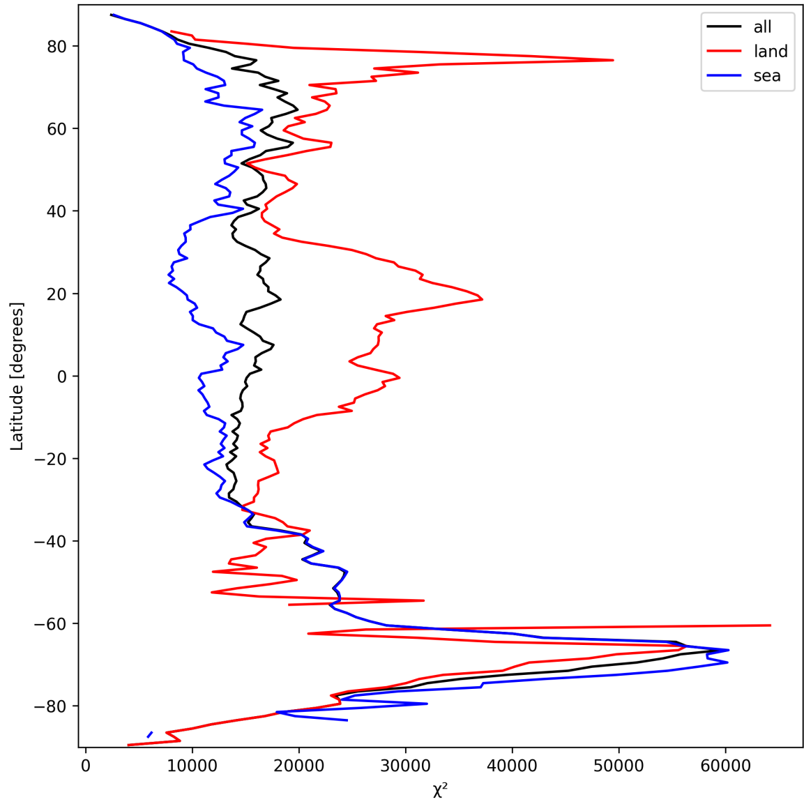
Figure 19: Zonal average of “ \chi^2 ” for 2025-09-25 to 2025-09-26.
