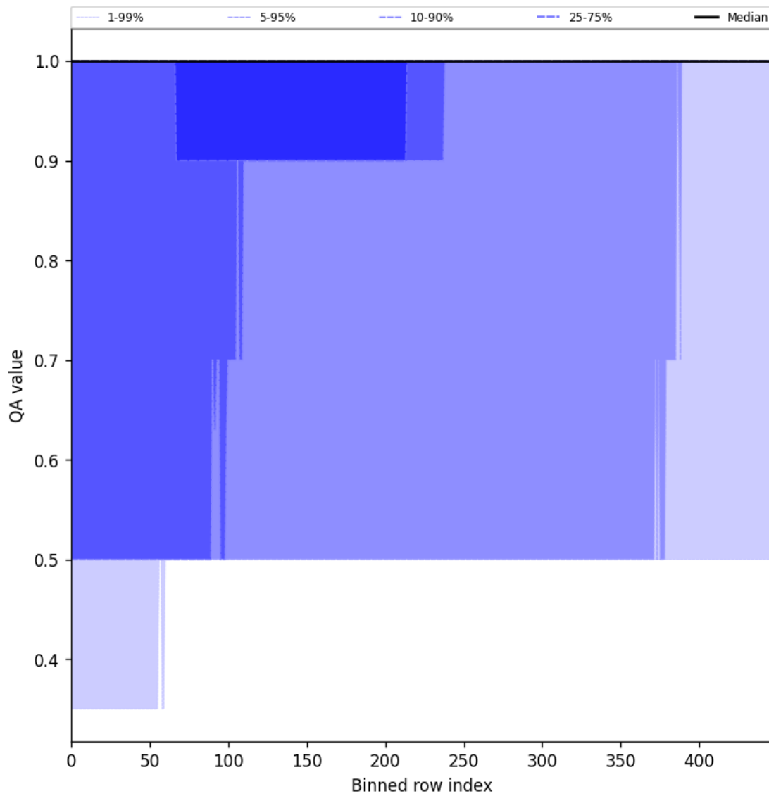
Figure 44: Along track statistics of “QA value” for 2025-09-25 to 2025-09-26
