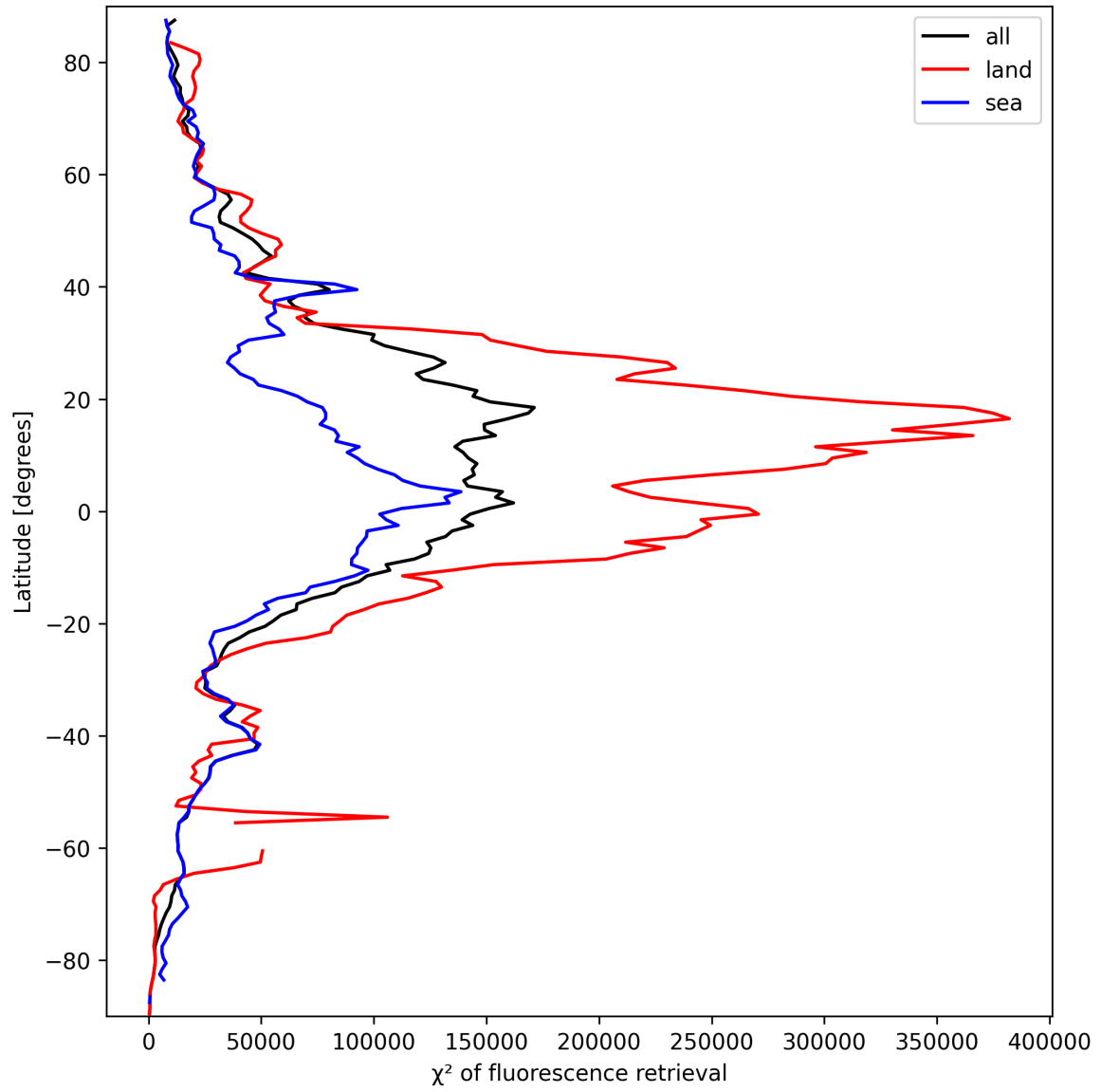
Figure 23: Zonal average of “ \chi^2 of fluorescence retrieval” for 2025-09-25 to 2025-09-26.
