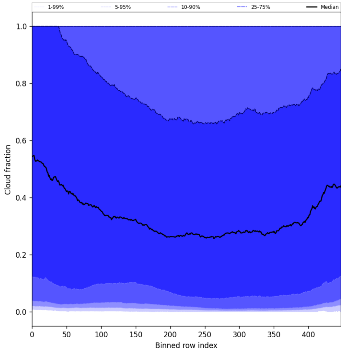
Figure 47: Along track statistics of “Cloud fraction” for 2025-09-25 to 2025-09-26
