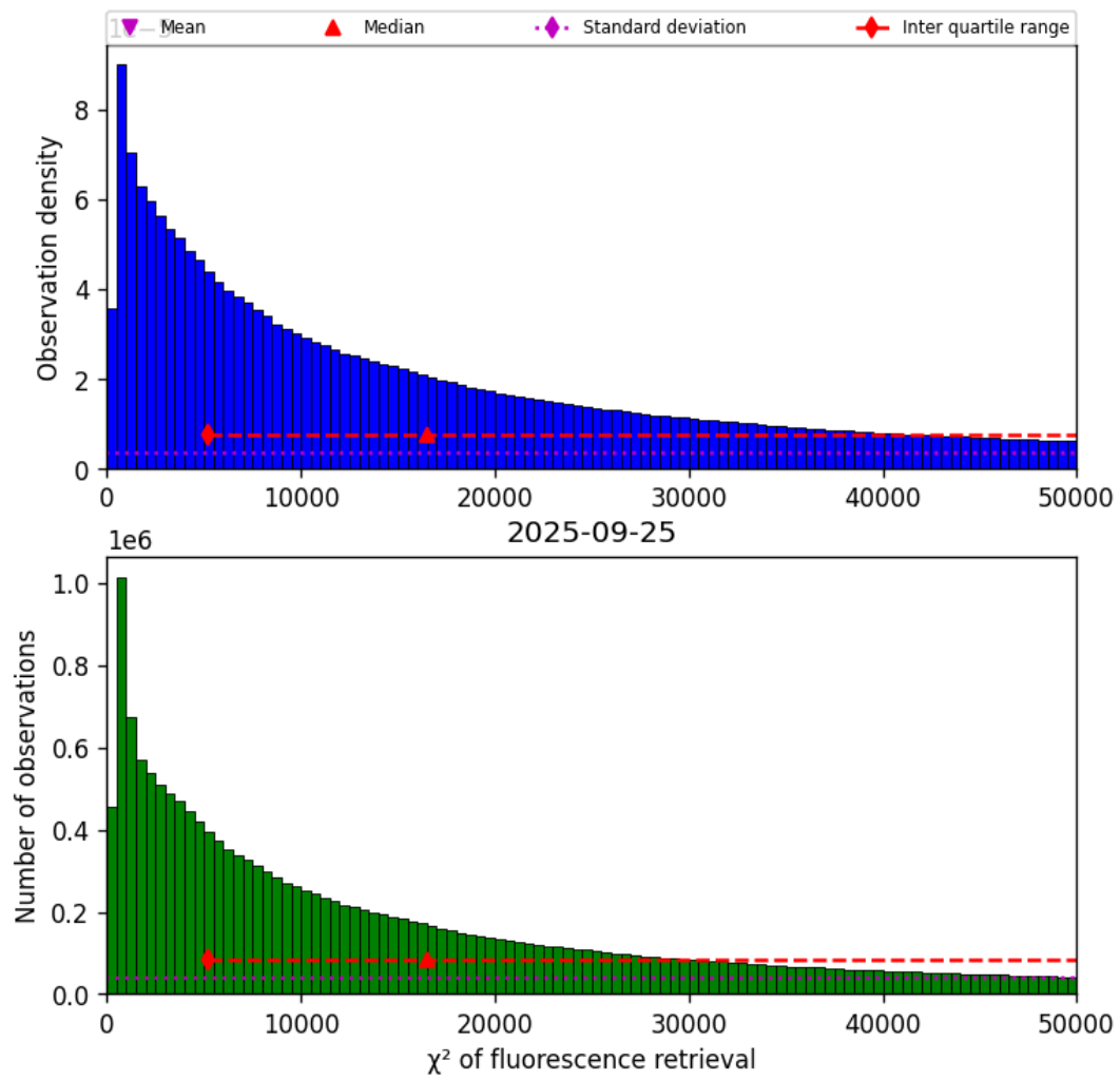
Figure 40: Histogram of “ \chi^2 of fluorescence retrieval” for 2025-09-25 to 2025-09-26
