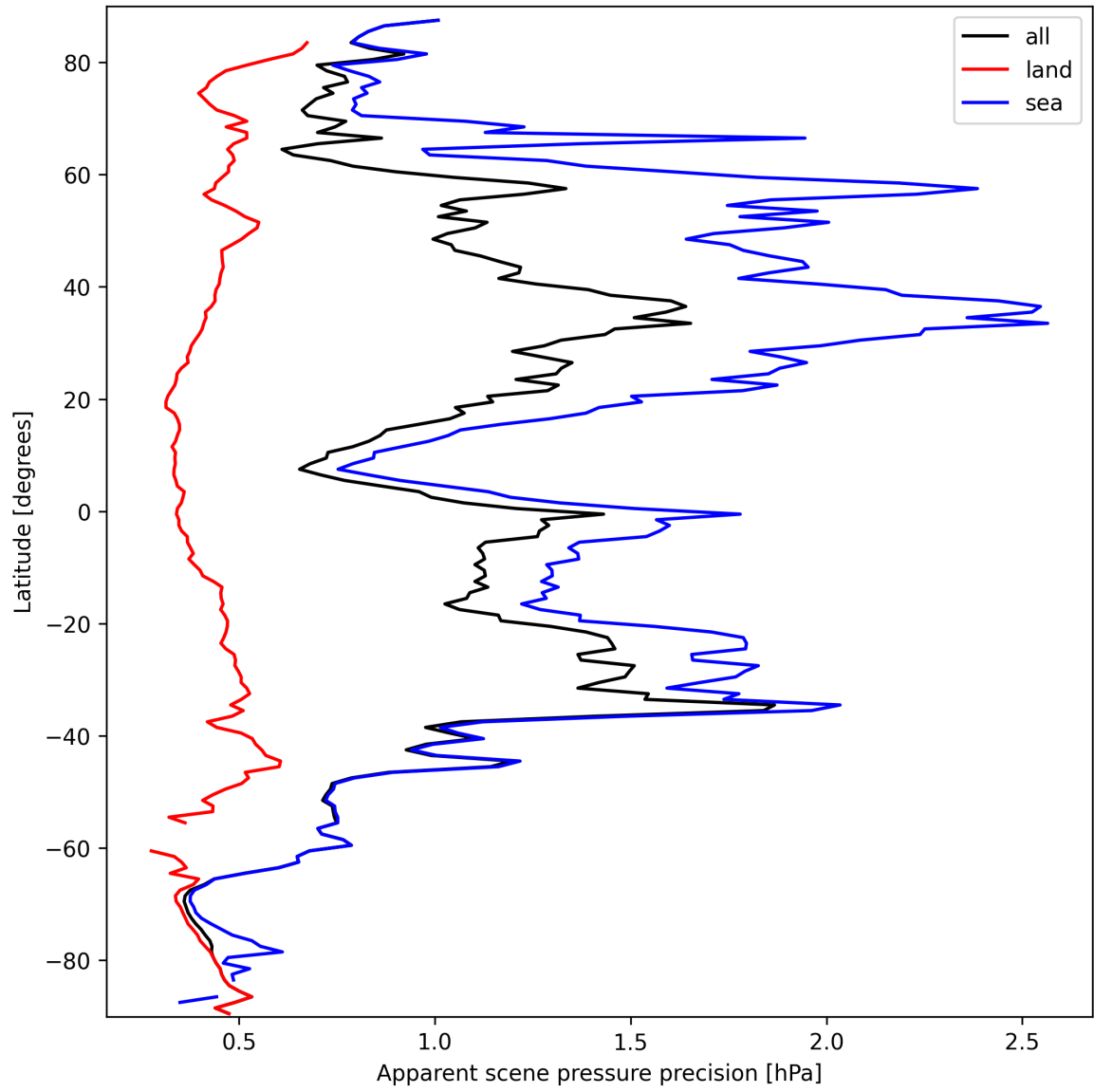
Figure 18: Zonal average of “Apparent scene pressure precision” for 2025-09-25 to 2025-09-26.
