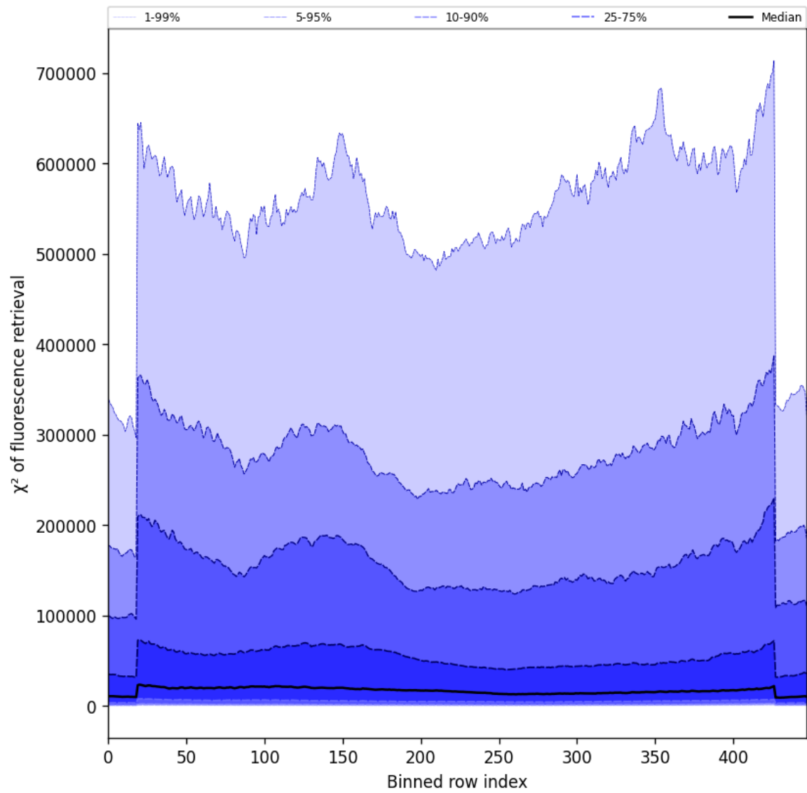
Figure 57: Along track statistics of “ \chi^2 of fluorescence retrieval” for 2025-09-25 to 2025-09-26
