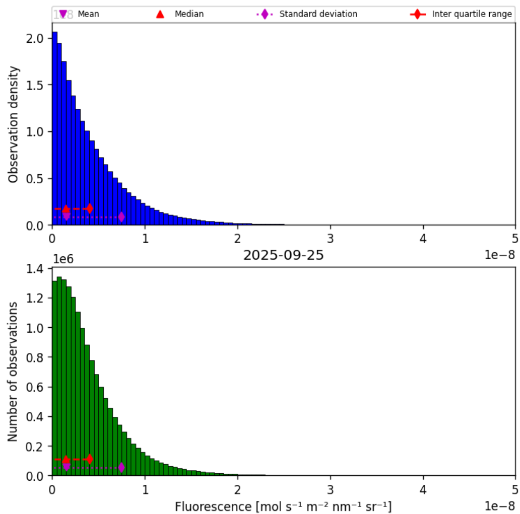
Figure 38: Histogram of “Fluorescence” for 2025-09-25 to 2025-09-26
