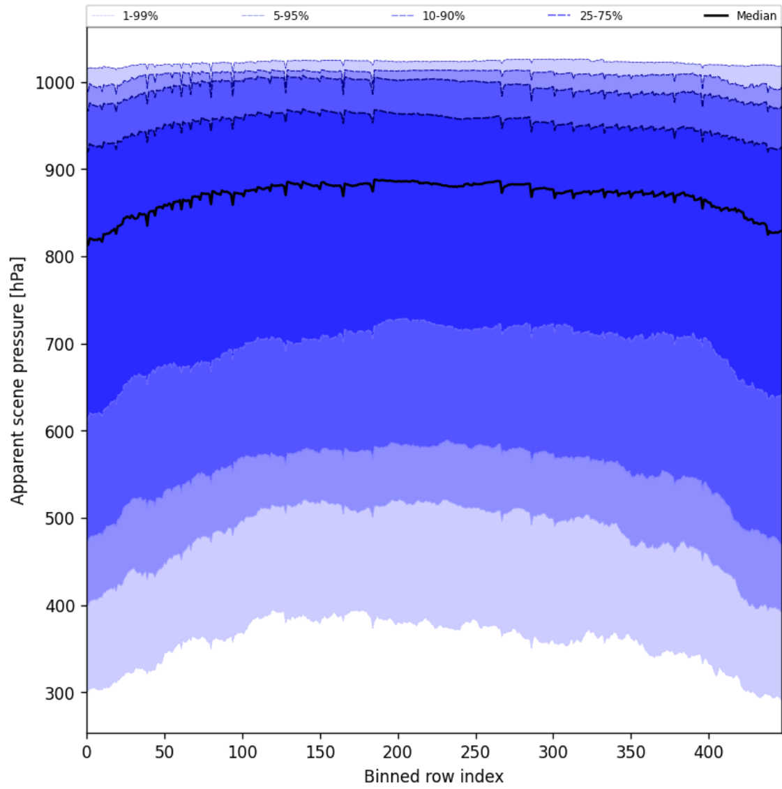
Figure 51: Along track statistics of “Apparent scene pressure” for 2025-09-25 to 2025-09-26
