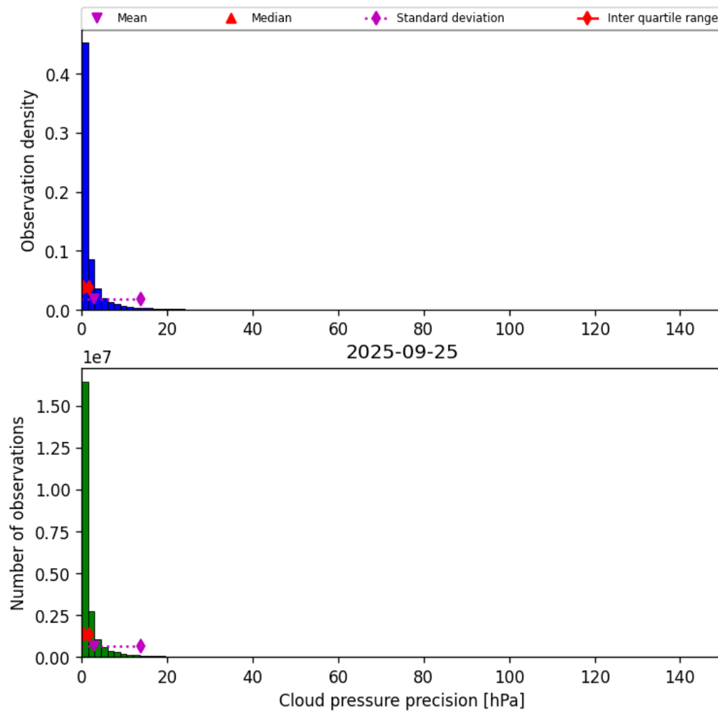
Figure 29: Histogram of “Cloud pressure precision” for 2025-09-25 to 2025-09-26
