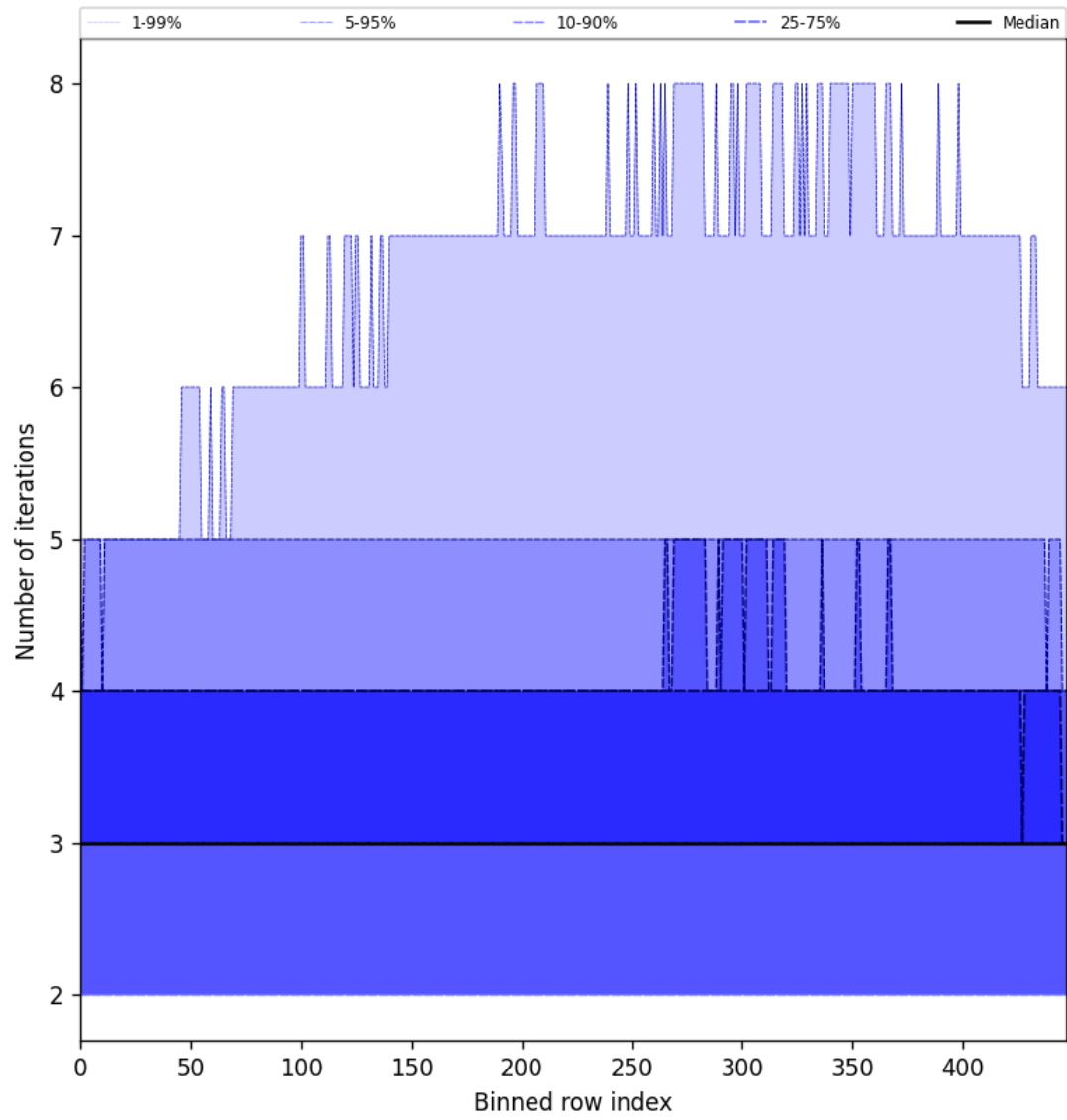
Figure 54: Along track statistics of “Number of iterations” for 2025-09-25 to 2025-09-26
