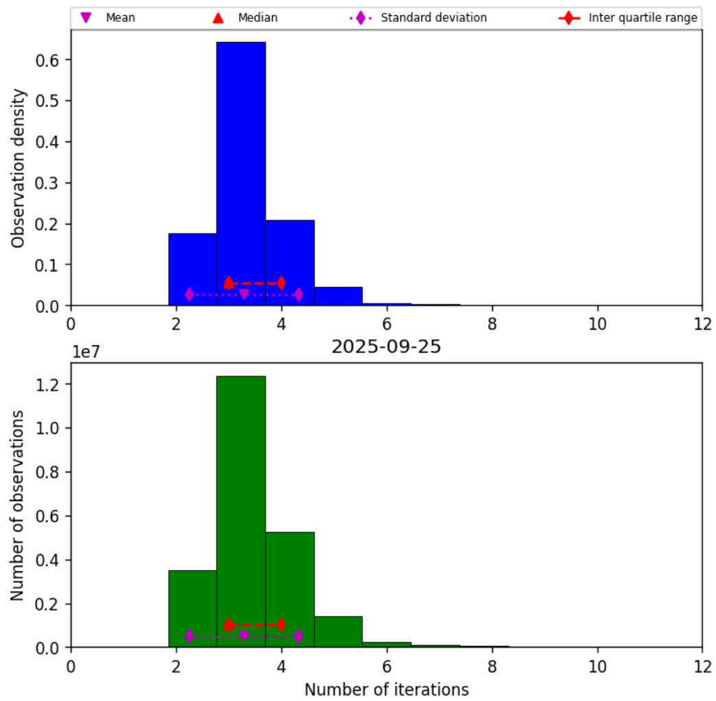
Figure 37: Histogram of “Number of iterations” for 2025-09-25 to 2025-09-26
