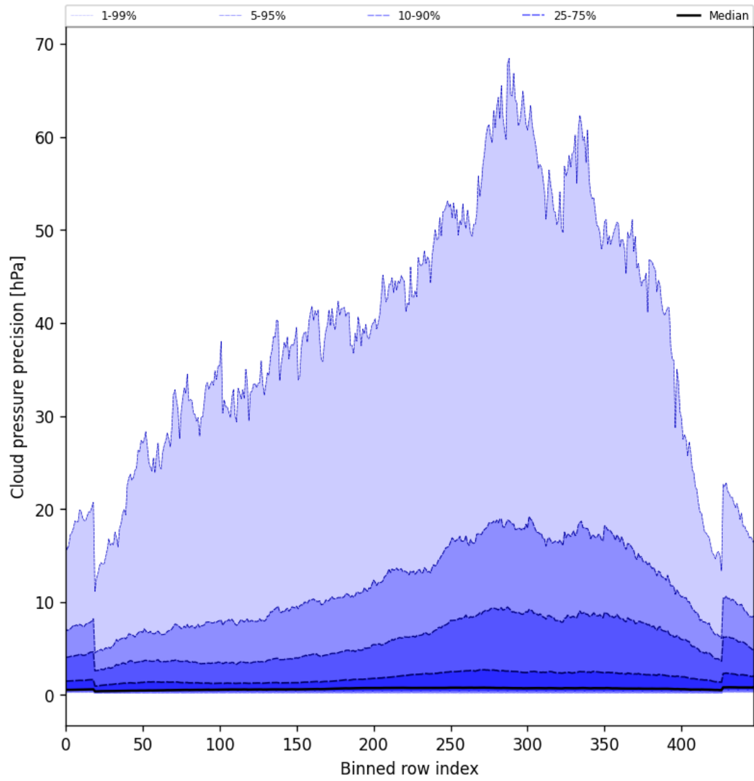
Figure 46: Along track statistics of “Cloud pressure precision” for 2025-09-25 to 2025-09-26
