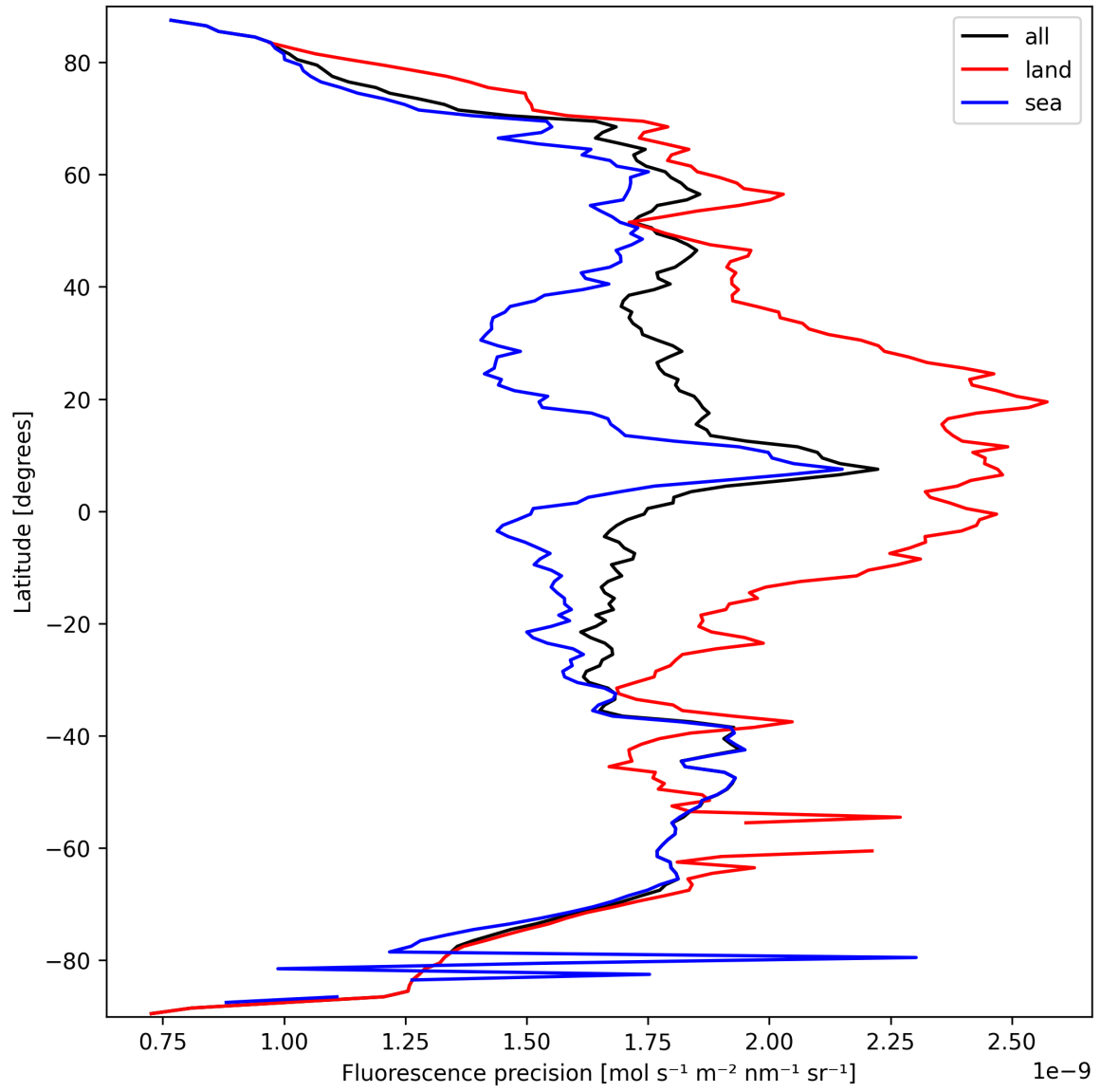
Figure 22: Zonal average of “Fluorescence precision” for 2025-09-25 to 2025-09-26.
