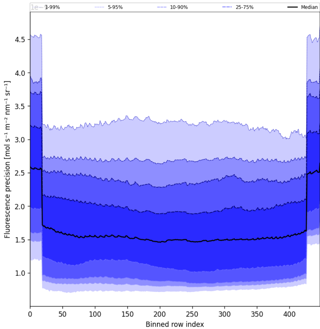
Figure 56: Along track statistics of “Fluorescence precision” for 2025-09-25 to 2025-09-26
