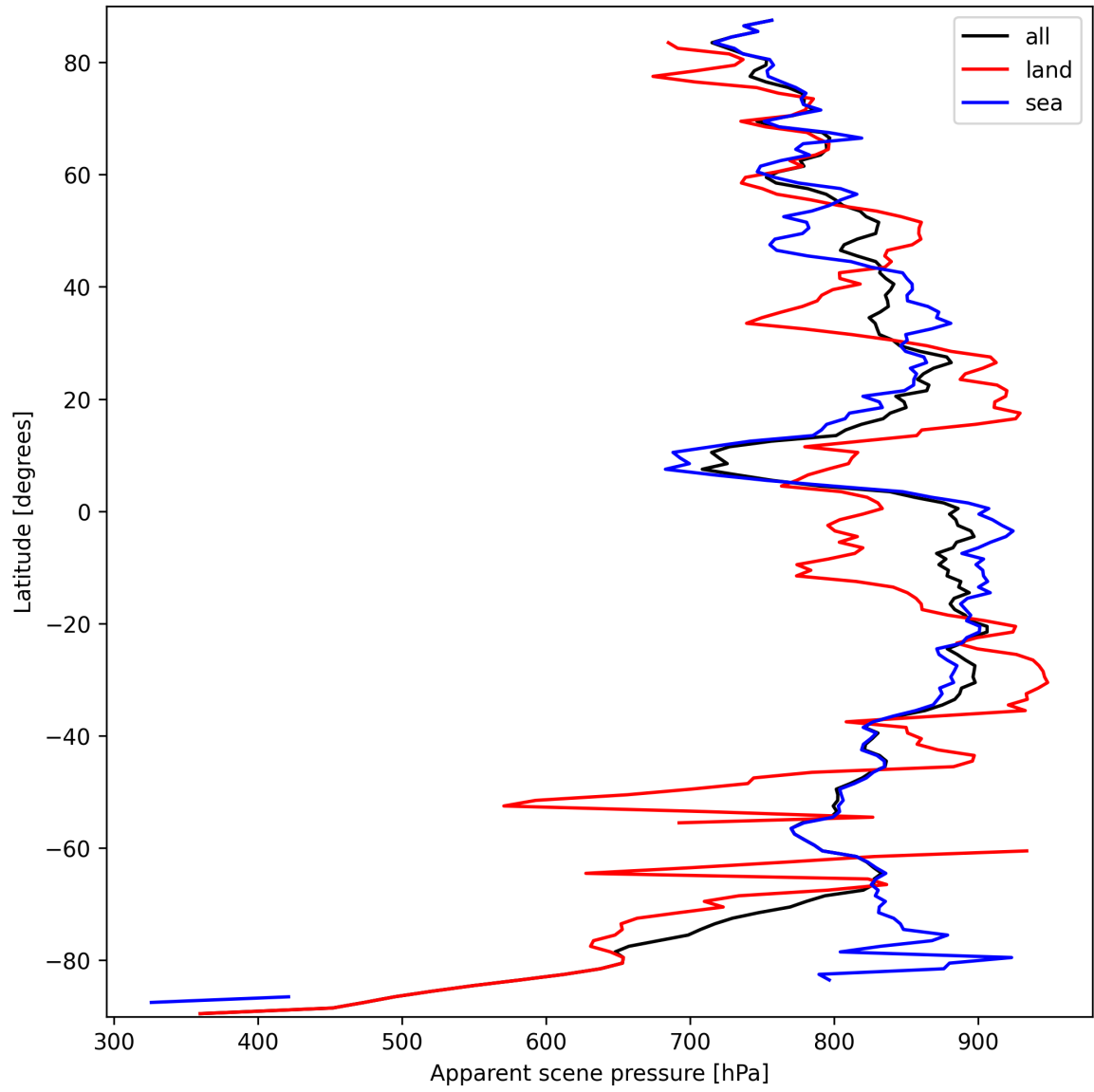
Figure 17: Zonal average of “Apparent scene pressure” for 2025-09-25 to 2025-09-26.
