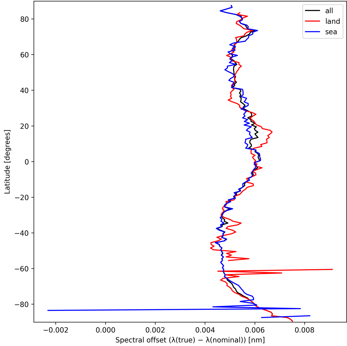
Figure 26: Zonal average of “Spectral offset ( \lambda_{\text{true}} - \lambda_{\text{nominal}} )” for 2025-09-25 to 2025-09-26.
