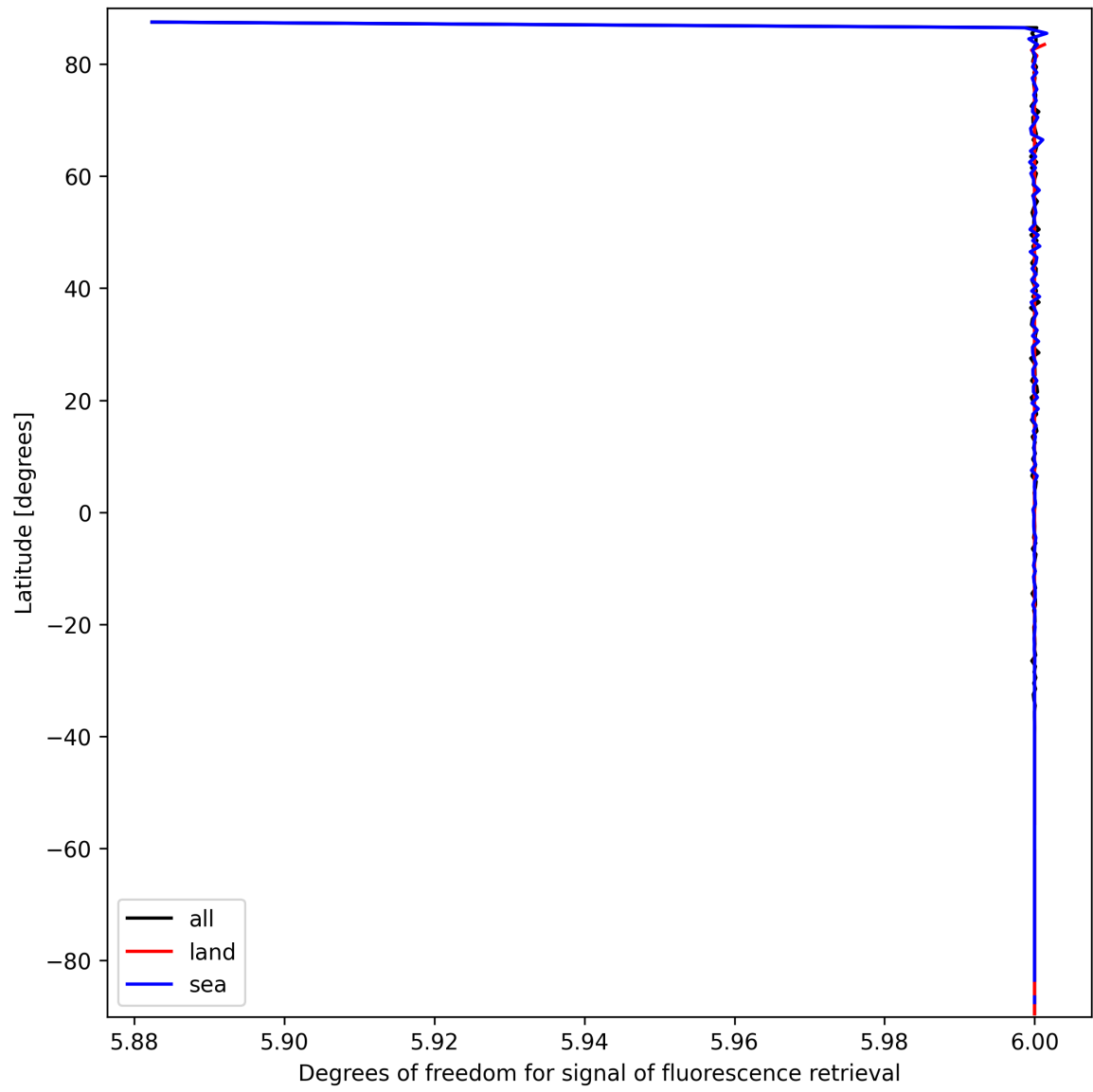
Figure 24: Zonal average of “Degrees of freedom for signal of fluorescence retrieval” for 2025-09-25 to 2025-09-26.
