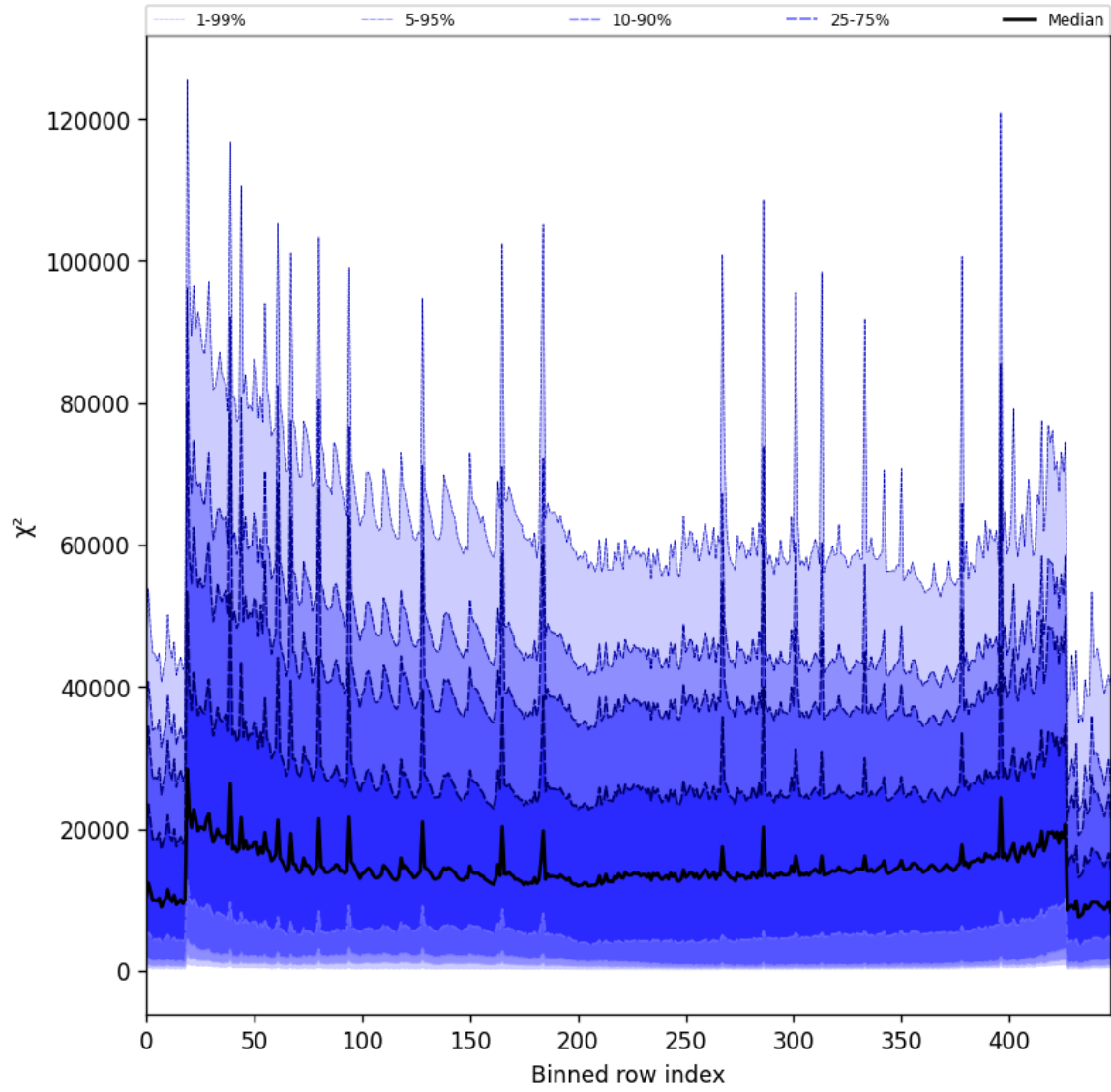
Figure 53: Along track statistics of “ \chi^2 ” for 2025-09-25 to 2025-09-26
