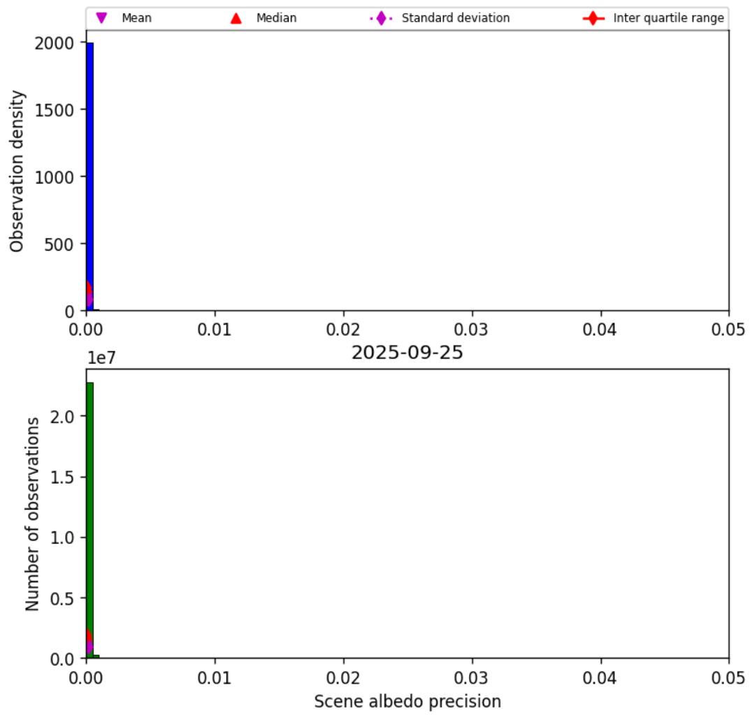
Figure 33: Histogram of “Scene albedo precision” for 2025-09-25 to 2025-09-26
