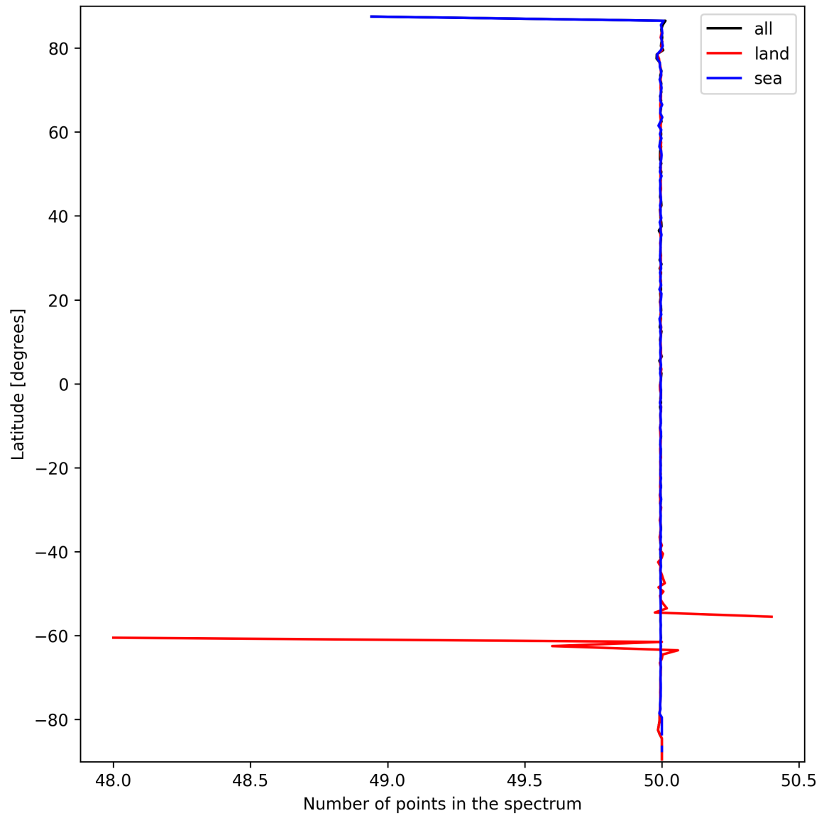
Figure 25: Zonal average of “Number of points in the spectrum” for 2025-09-25 to 2025-09-26.
