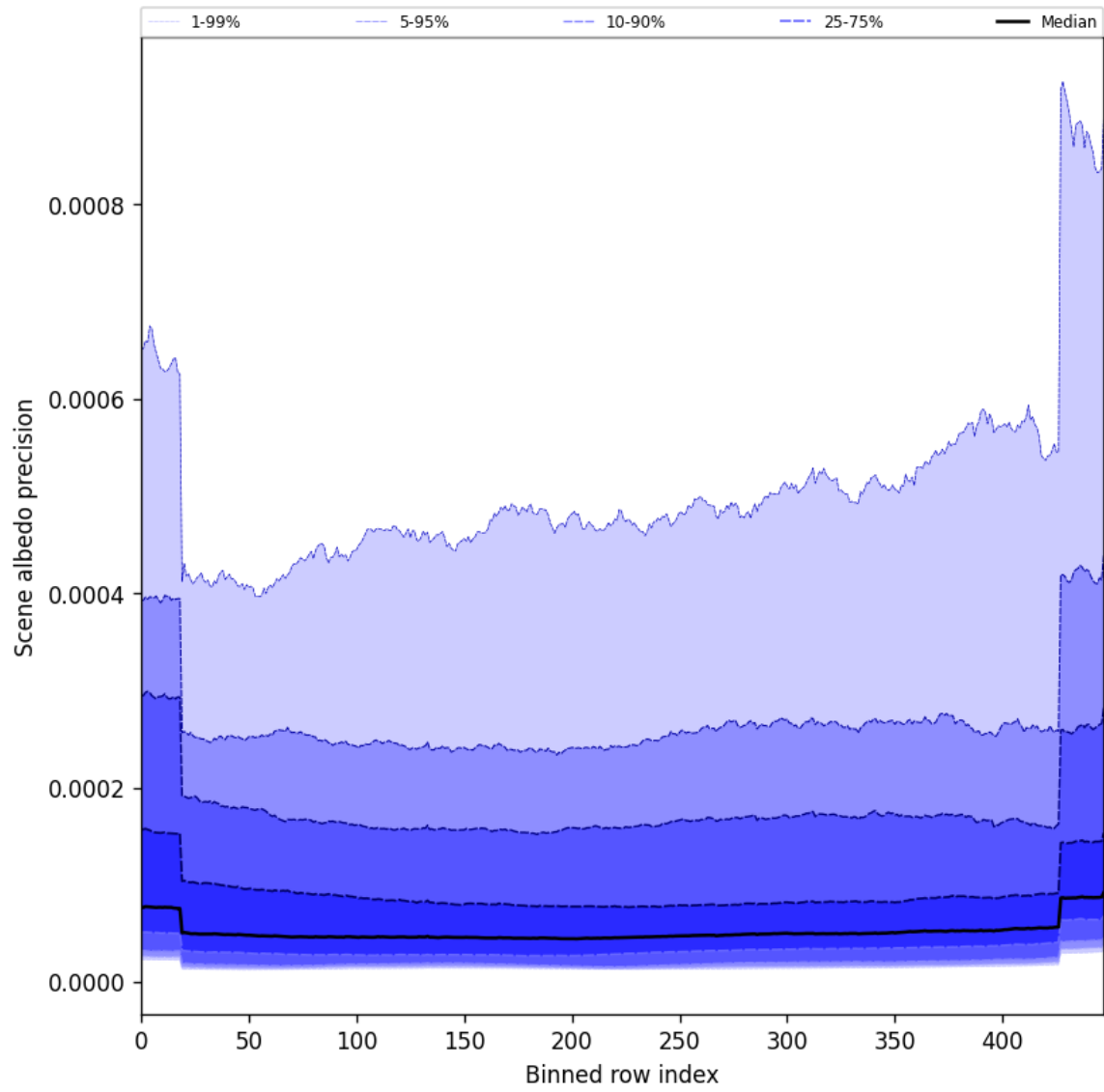
Figure 50: Along track statistics of “Scene albedo precision” for 2025-09-25 to 2025-09-26
