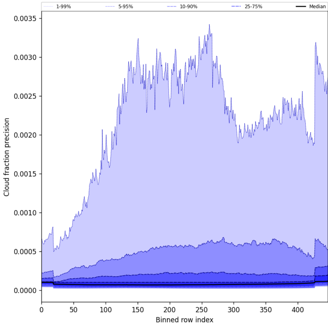
Figure 48: Along track statistics of “Cloud fraction precision” for 2025-09-25 to 2025-09-26
