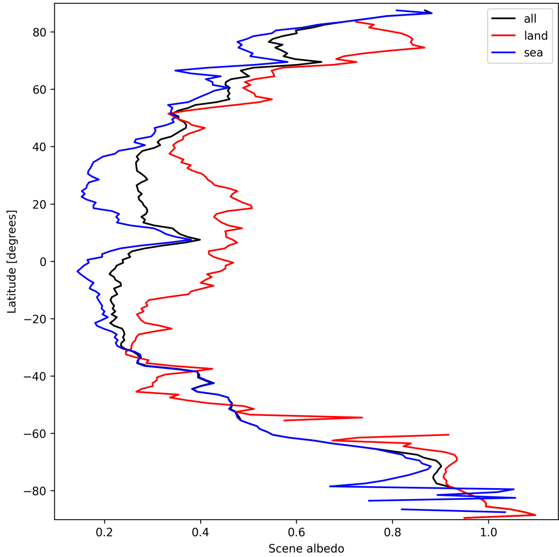
Figure 15: Zonal average of “Scene albedo” for 2025-09-25 to 2025-09-26.
