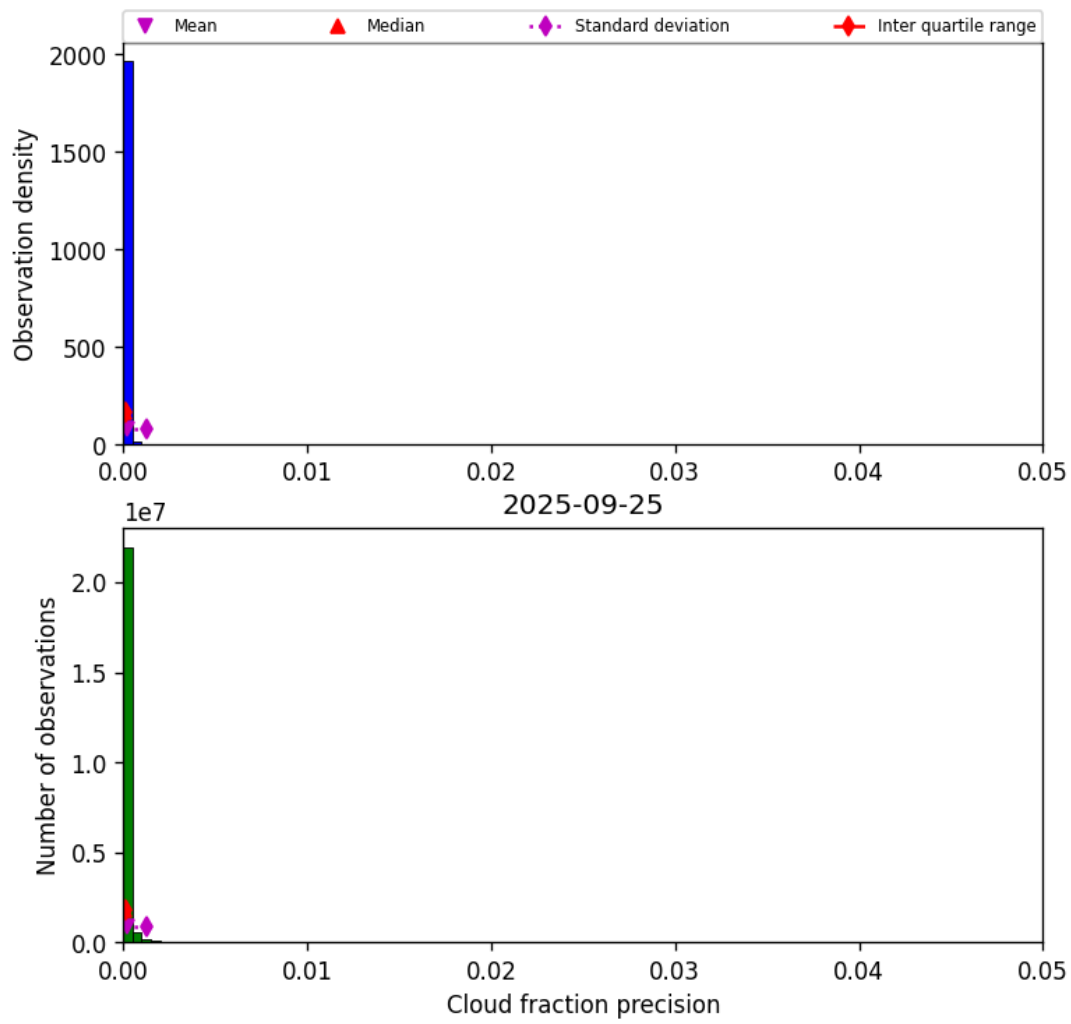
Figure 31: Histogram of “Cloud fraction precision” for 2025-09-25 to 2025-09-26
