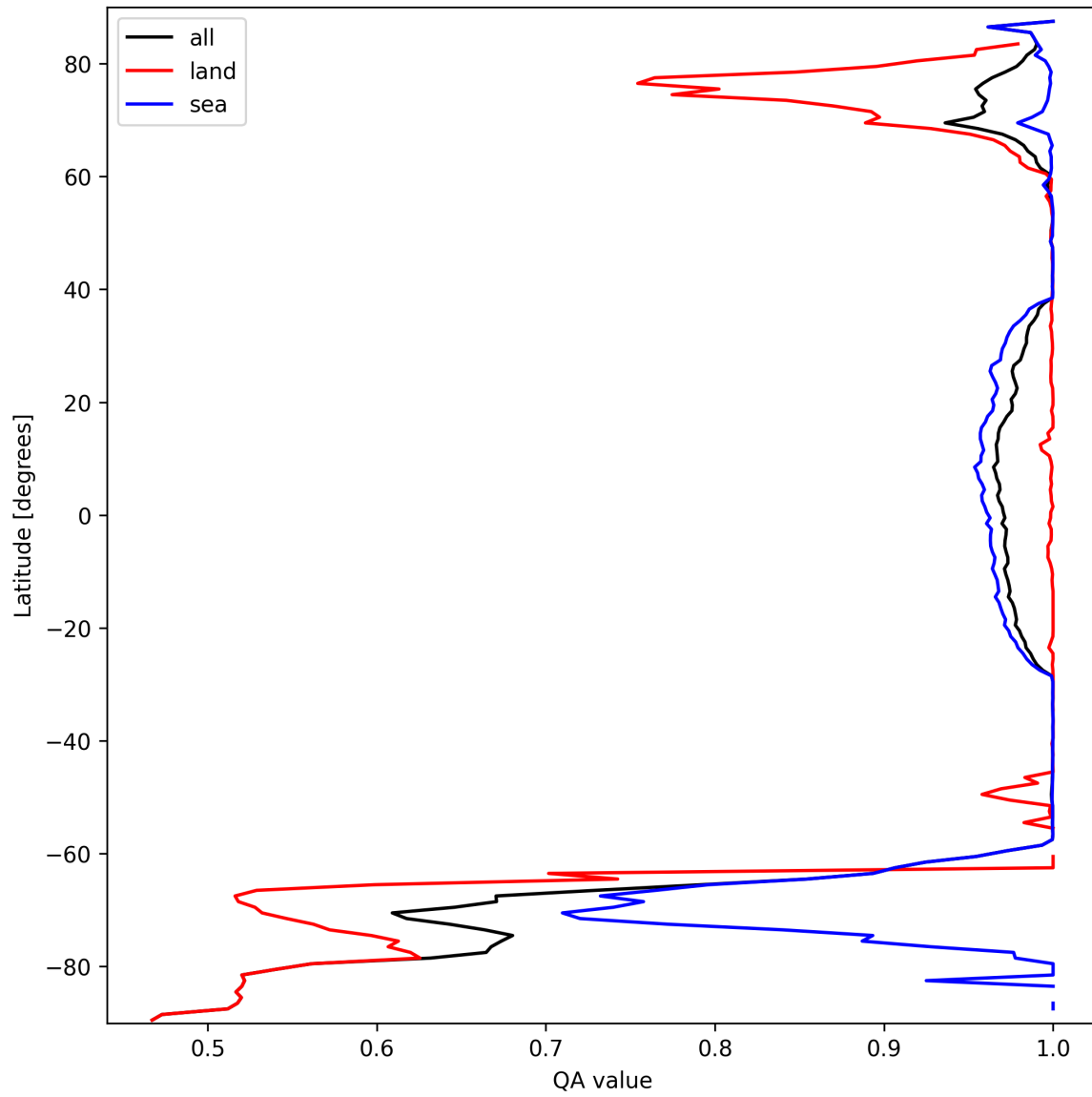
Figure 10: Zonal average of “QA value” for 2025-09-25 to 2025-09-26.
