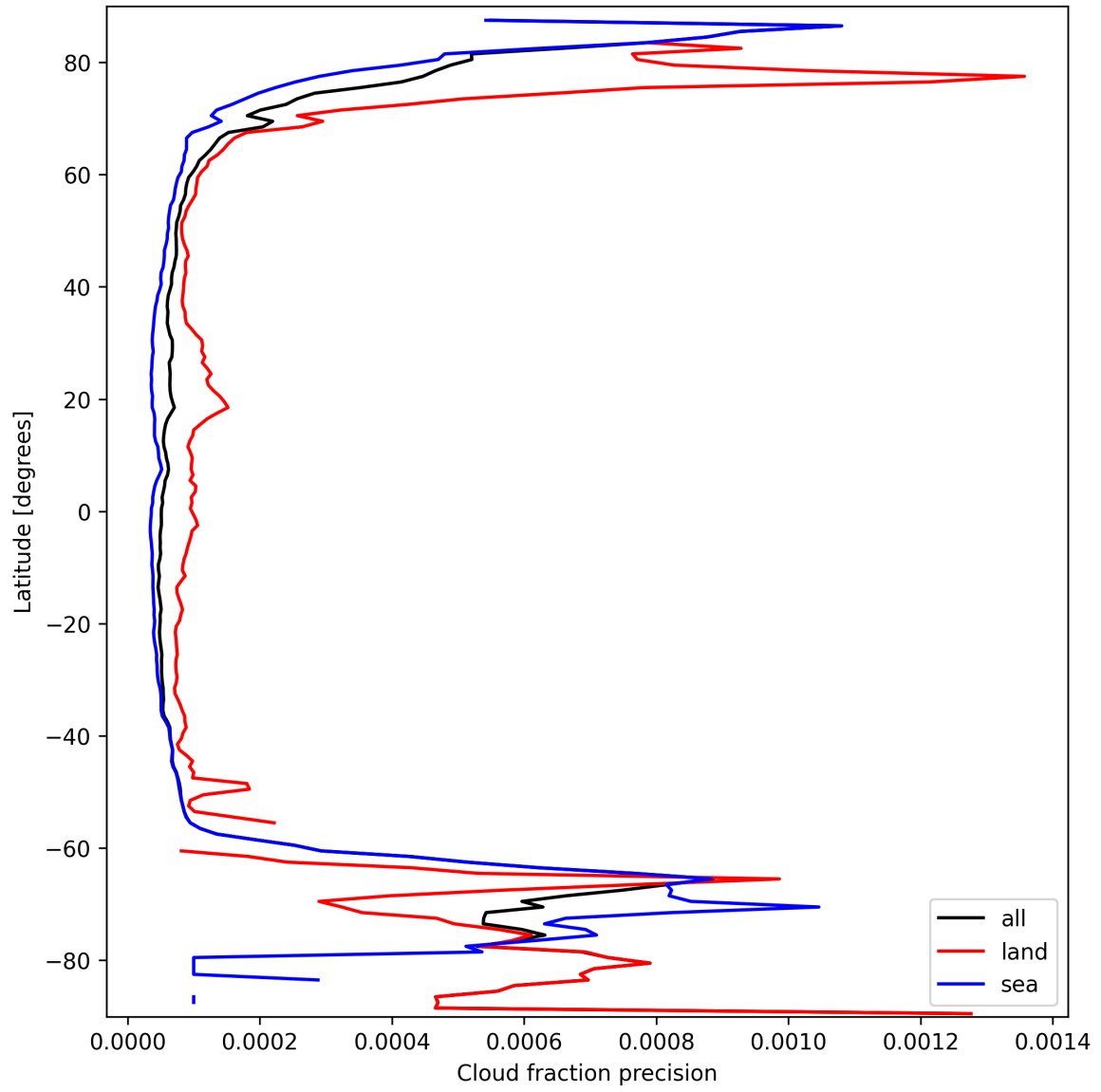
Figure 14: Zonal average of “Cloud fraction precision” for 2025-09-25 to 2025-09-26.
