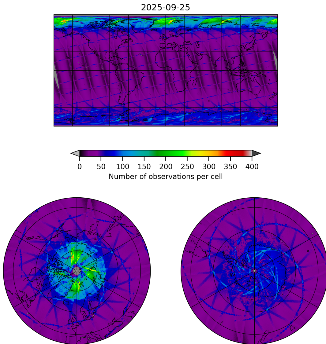
Figure 9: Map of the number of observations for 2025-09-25 to 2025-09-26
