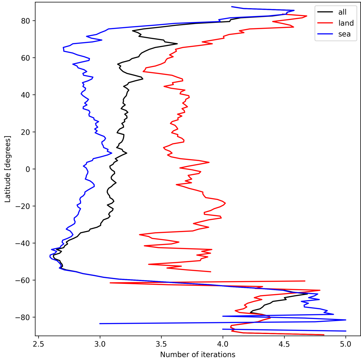
Figure 20: Zonal average of “Number of iterations” for 2025-09-25 to 2025-09-26.
