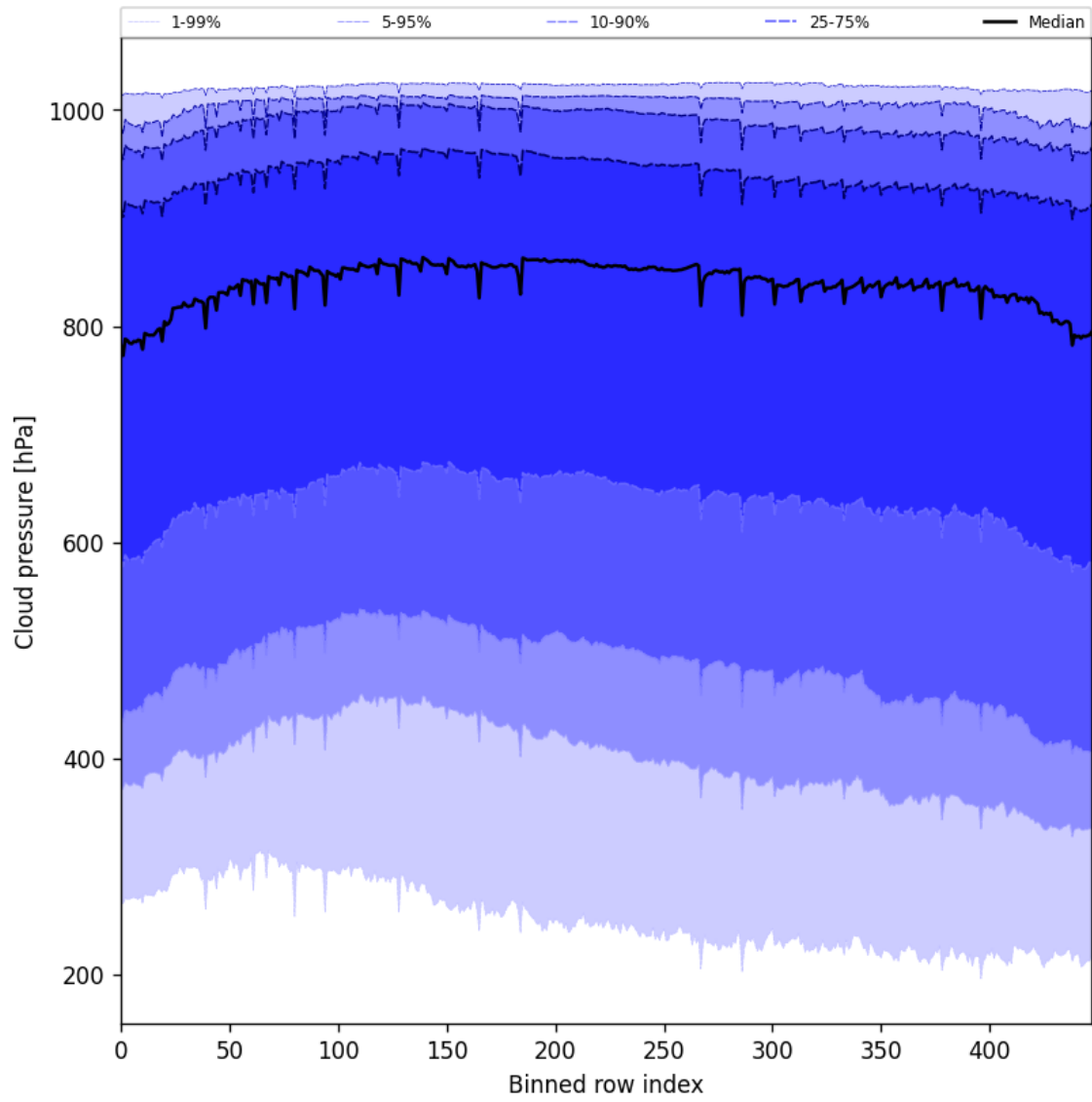
Figure 45: Along track statistics of “Cloud pressure” for 2025-09-25 to 2025-09-26
