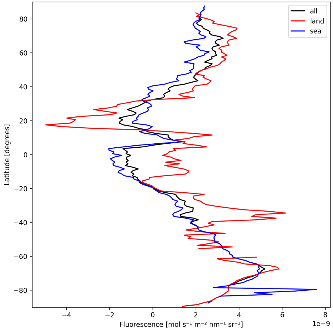
Figure 21: Zonal average of “Fluorescence” for 2025-09-25 to 2025-09-26.
