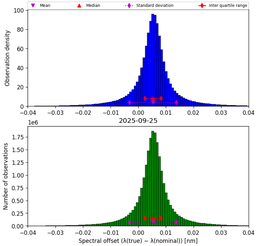
Figure 43: Histogram of “Spectral offset ( \lambda_{\text{true}} - \lambda_{\text{nominal}} )” for 2025-09-25 to 2025-09-26
