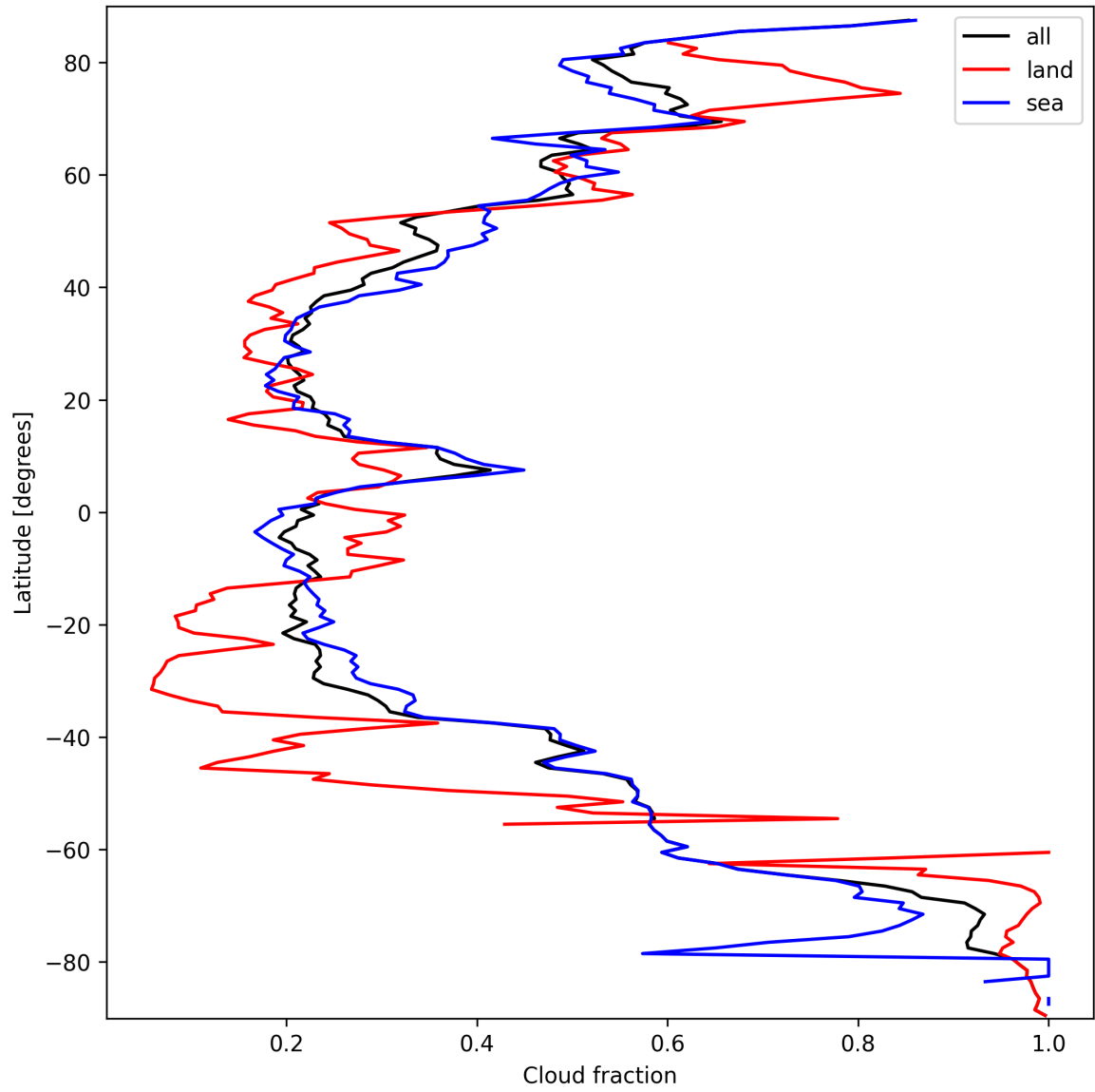
Figure 13: Zonal average of “Cloud fraction” for 2025-09-25 to 2025-09-26.
