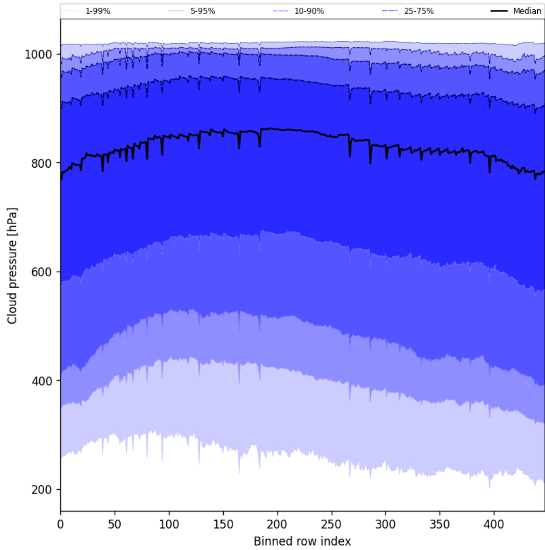
Figure 45: Along track statistics of “Cloud pressure” for 2025-09-26 to 2025-09-27
