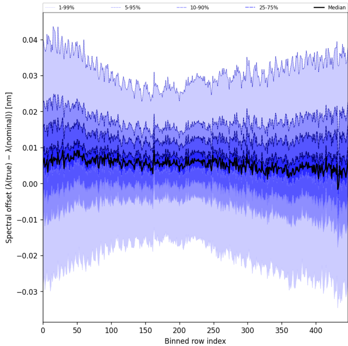
Figure 60: Along track statistics of “Spectral offset ( \lambda_{\text{true}} - \lambda_{\text{nominal}} )” for 2025-09-26 to 2025-09-27
