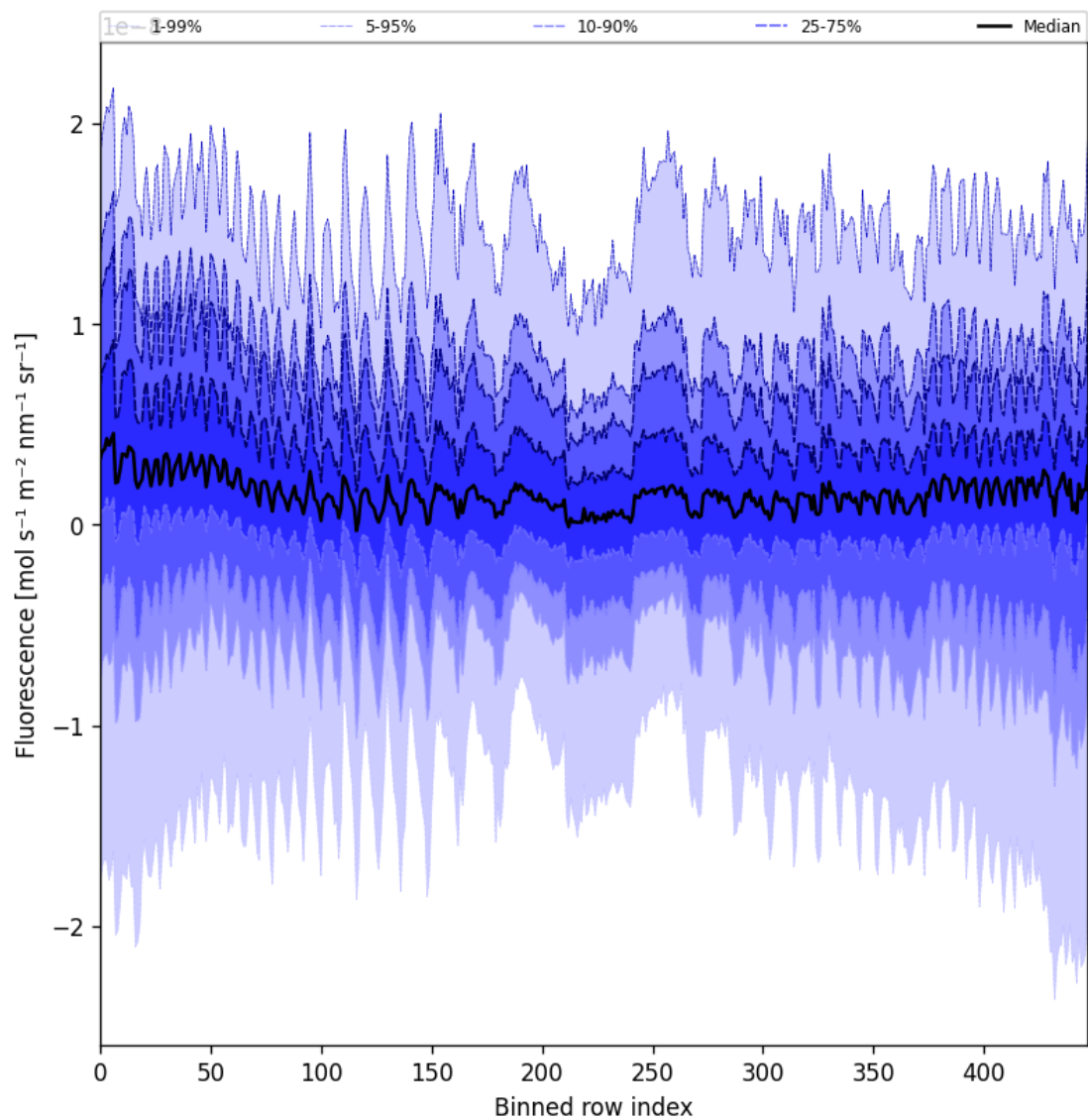
Figure 55: Along track statistics of “Fluorescence” for 2025-09-26 to 2025-09-27
