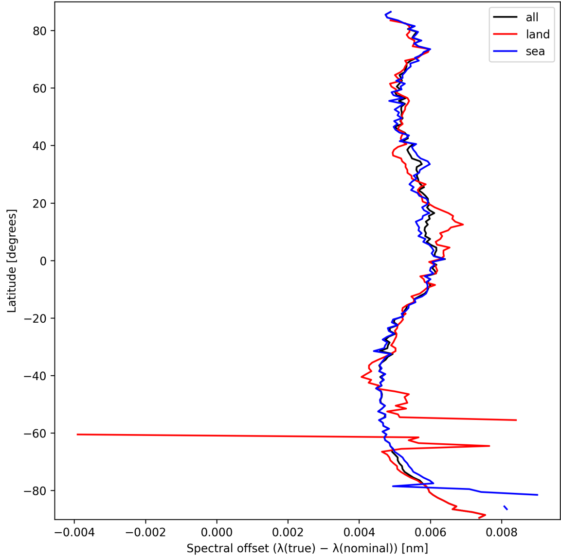
Figure 26: Zonal average of “Spectral offset ( \lambda_{\text{true}} - \lambda_{\text{nominal}} )” for 2025-09-26 to 2025-09-27.
