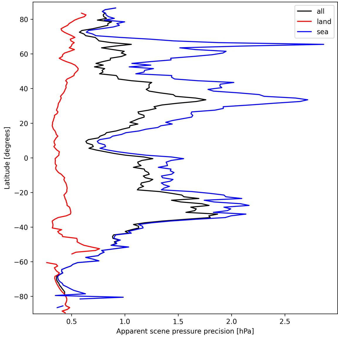
Figure 18: Zonal average of “Apparent scene pressure precision” for 2025-09-26 to 2025-09-27.
