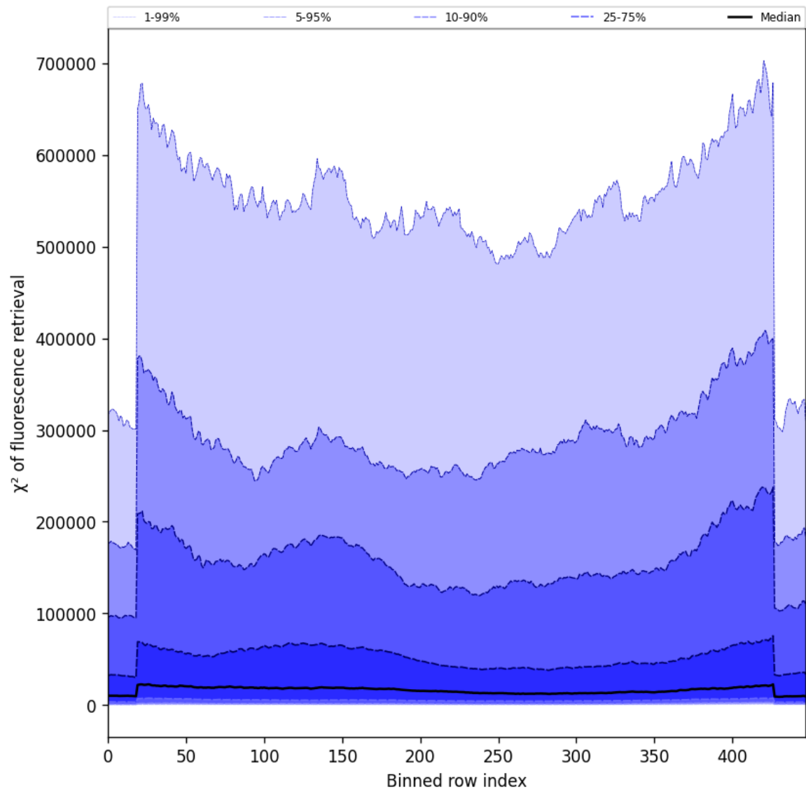
Figure 57: Along track statistics of “ \chi^2 of fluorescence retrieval” for 2025-09-26 to 2025-09-27
