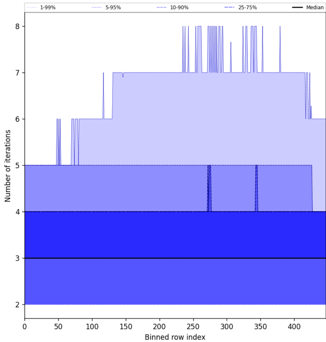
Figure 54: Along track statistics of “Number of iterations” for 2025-09-26 to 2025-09-27
