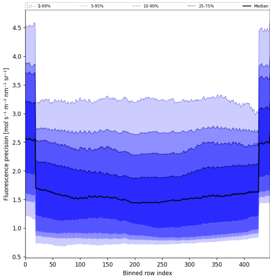
Figure 56: Along track statistics of “Fluorescence precision” for 2025-09-26 to 2025-09-27
