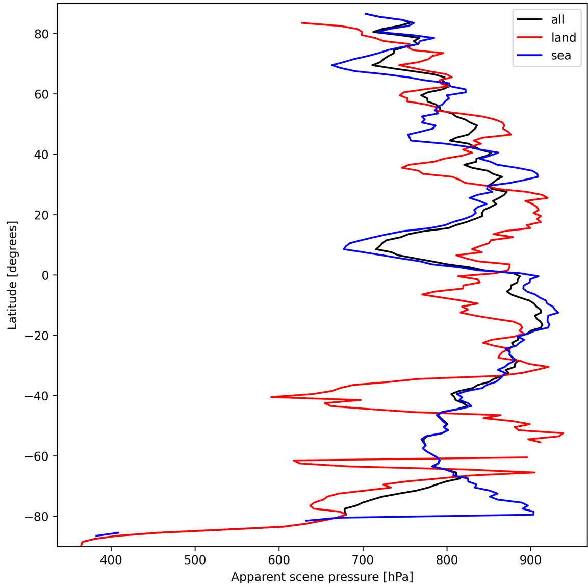
Figure 17: Zonal average of “Apparent scene pressure” for 2025-09-26 to 2025-09-27.
