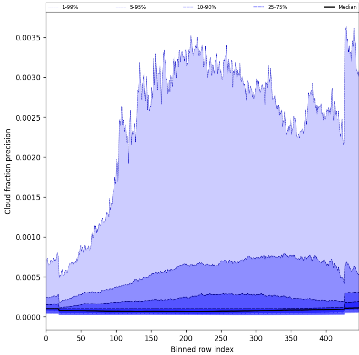
Figure 48: Along track statistics of “Cloud fraction precision” for 2025-09-26 to 2025-09-27
