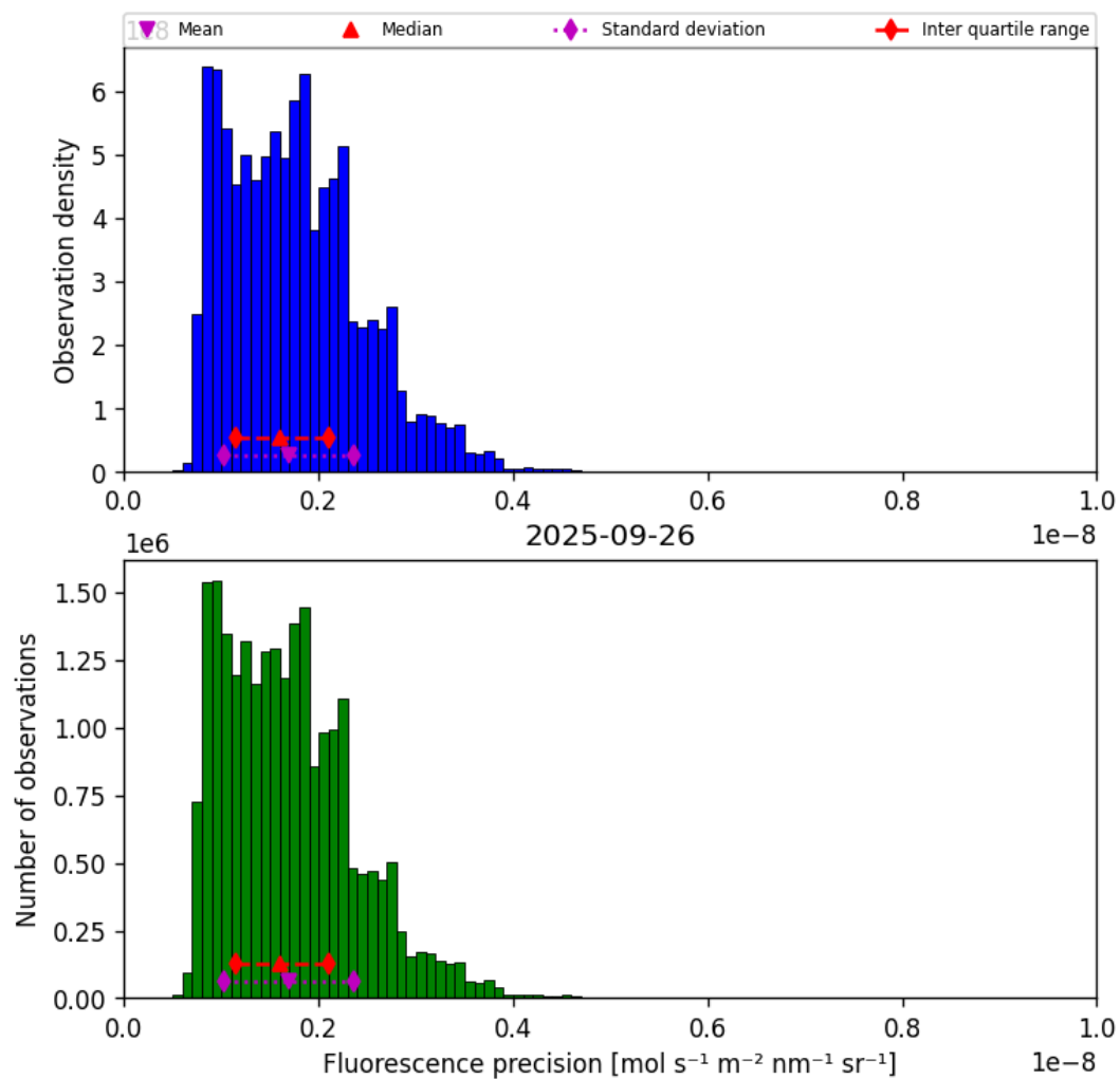
Figure 39: Histogram of “Fluorescence precision” for 2025-09-26 to 2025-09-27
