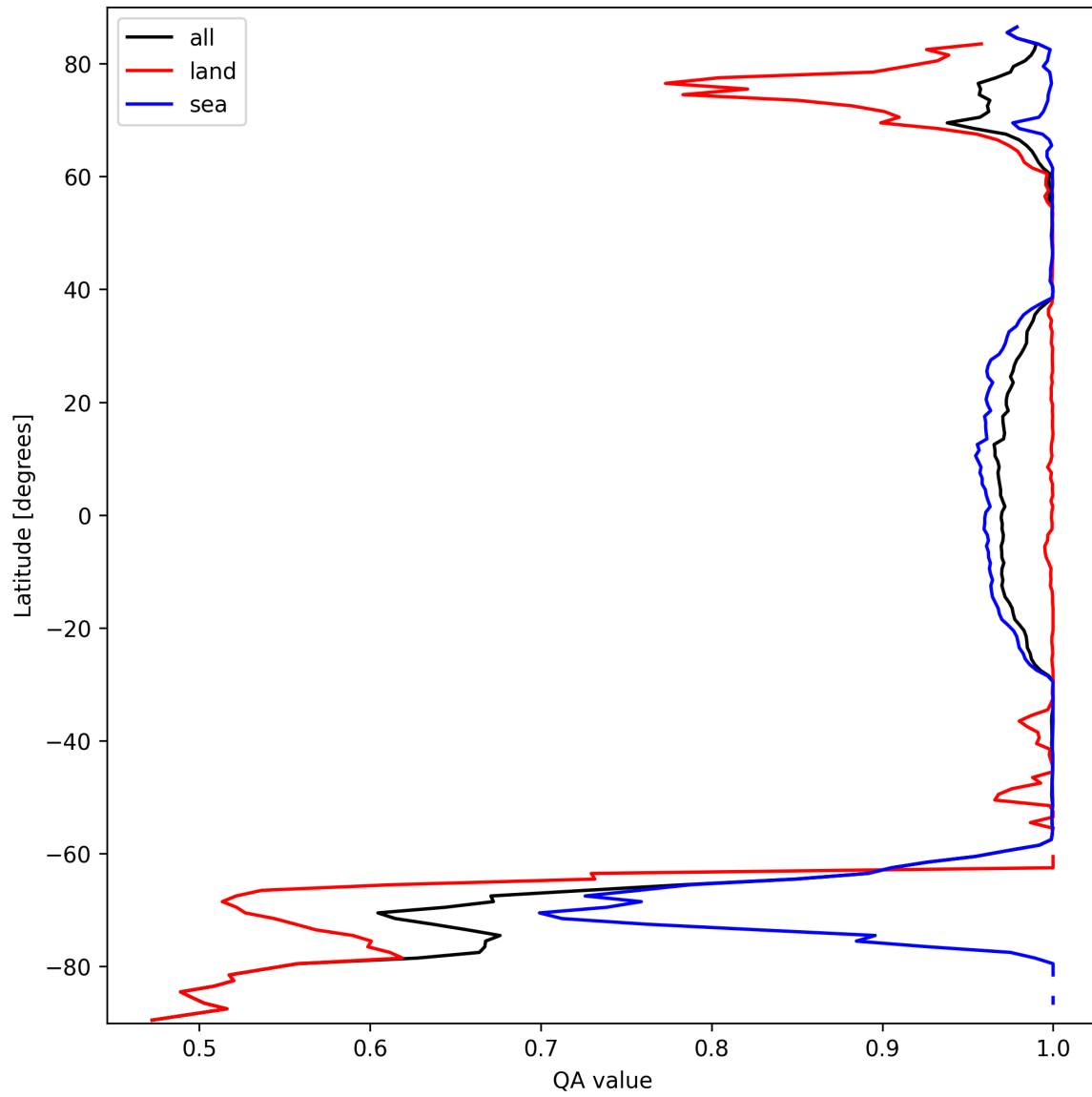
Figure 10: Zonal average of “QA value” for 2025-09-26 to 2025-09-27.
