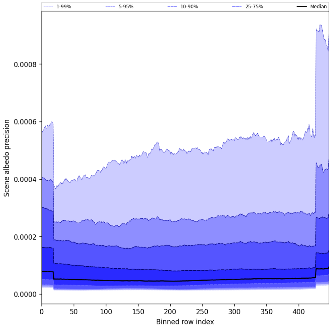
Figure 50: Along track statistics of “Scene albedo precision” for 2025-09-26 to 2025-09-27
