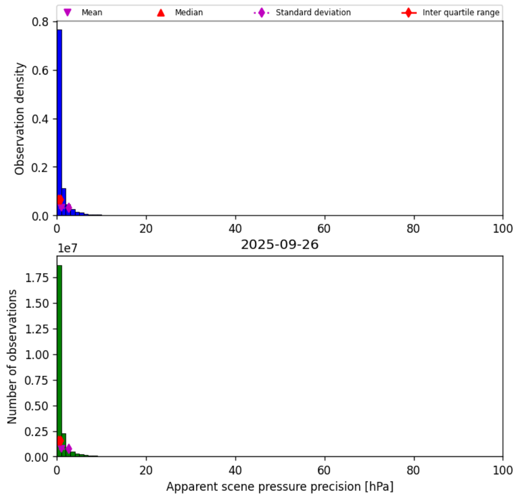
Figure 35: Histogram of “Apparent scene pressure precision” for 2025-09-26 to 2025-09-27
