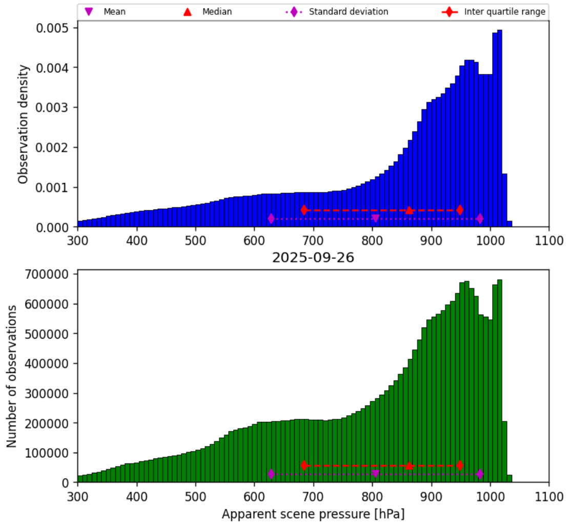
Figure 34: Histogram of “Apparent scene pressure” for 2025-09-26 to 2025-09-27
