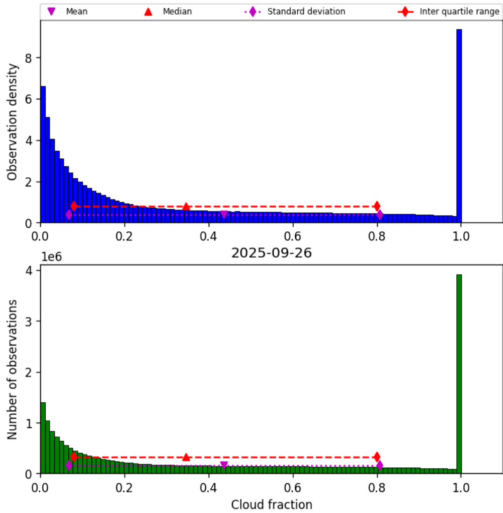
Figure 30: Histogram of “Cloud fraction” for 2025-09-26 to 2025-09-27
