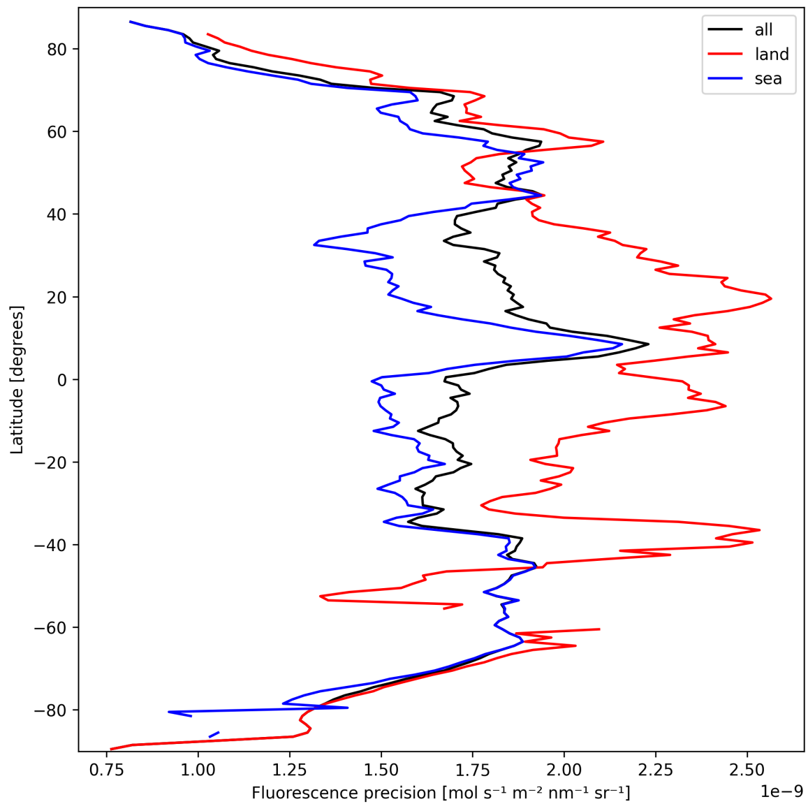
Figure 22: Zonal average of “Fluorescence precision” for 2025-09-26 to 2025-09-27.
