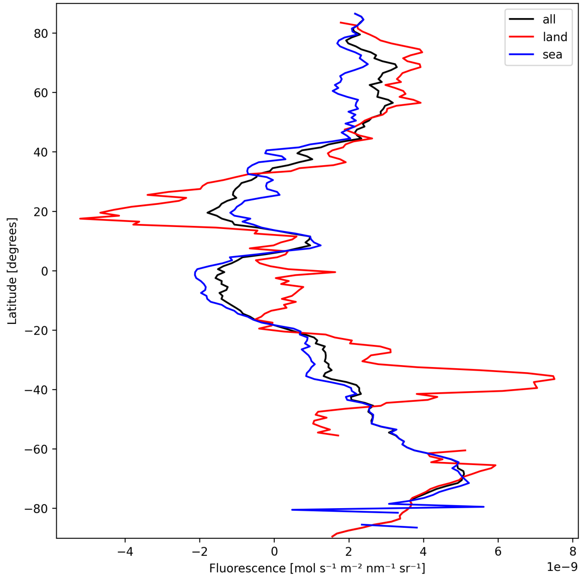
Figure 21: Zonal average of “Fluorescence” for 2025-09-26 to 2025-09-27.
