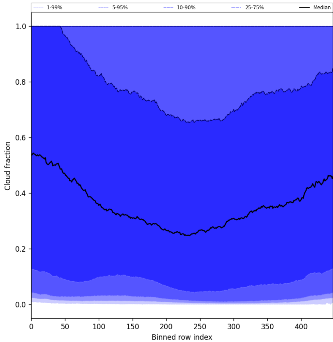
Figure 47: Along track statistics of “Cloud fraction” for 2025-09-26 to 2025-09-27
