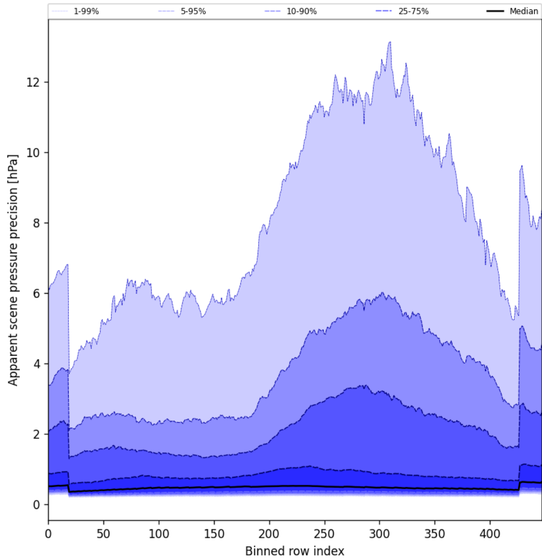
Figure 52: Along track statistics of “Apparent scene pressure precision” for 2025-09-26 to 2025-09-27
