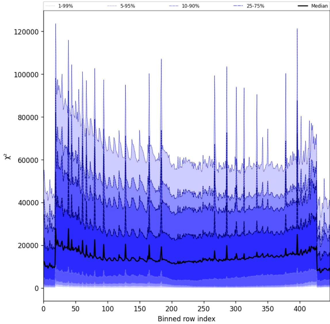
Figure 53: Along track statistics of “ \chi^2 ” for 2025-09-26 to 2025-09-27
