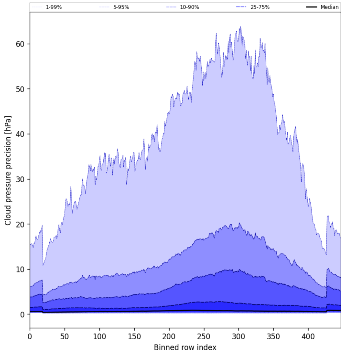
Figure 46: Along track statistics of “Cloud pressure precision” for 2025-09-26 to 2025-09-27
