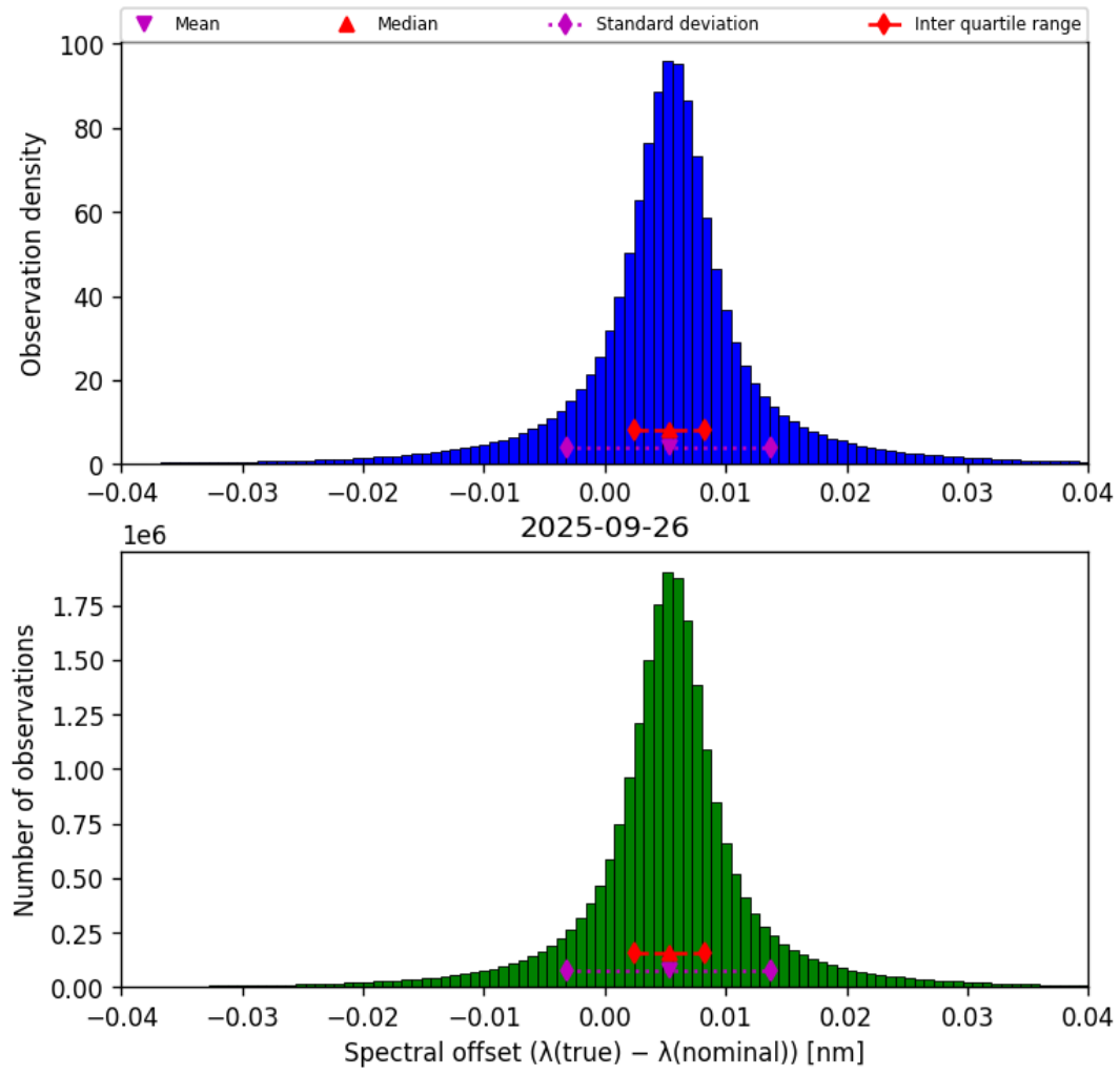
Figure 43: Histogram of “Spectral offset ( \lambda_{\text{true}} - \lambda_{\text{nominal}} )” for 2025-09-26 to 2025-09-27
