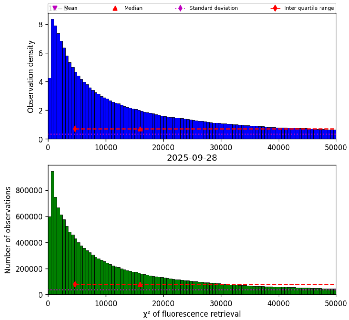
Figure 40: Histogram of “ \chi^2 of fluorescence retrieval” for 2025-09-28 to 2025-09-29
