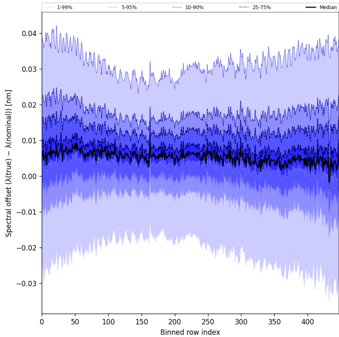
Figure 60: Along track statistics of “Spectral offset ( \lambda_{\text{true}} - \lambda_{\text{nominal}} )” for 2025-09-28 to 2025-09-29
