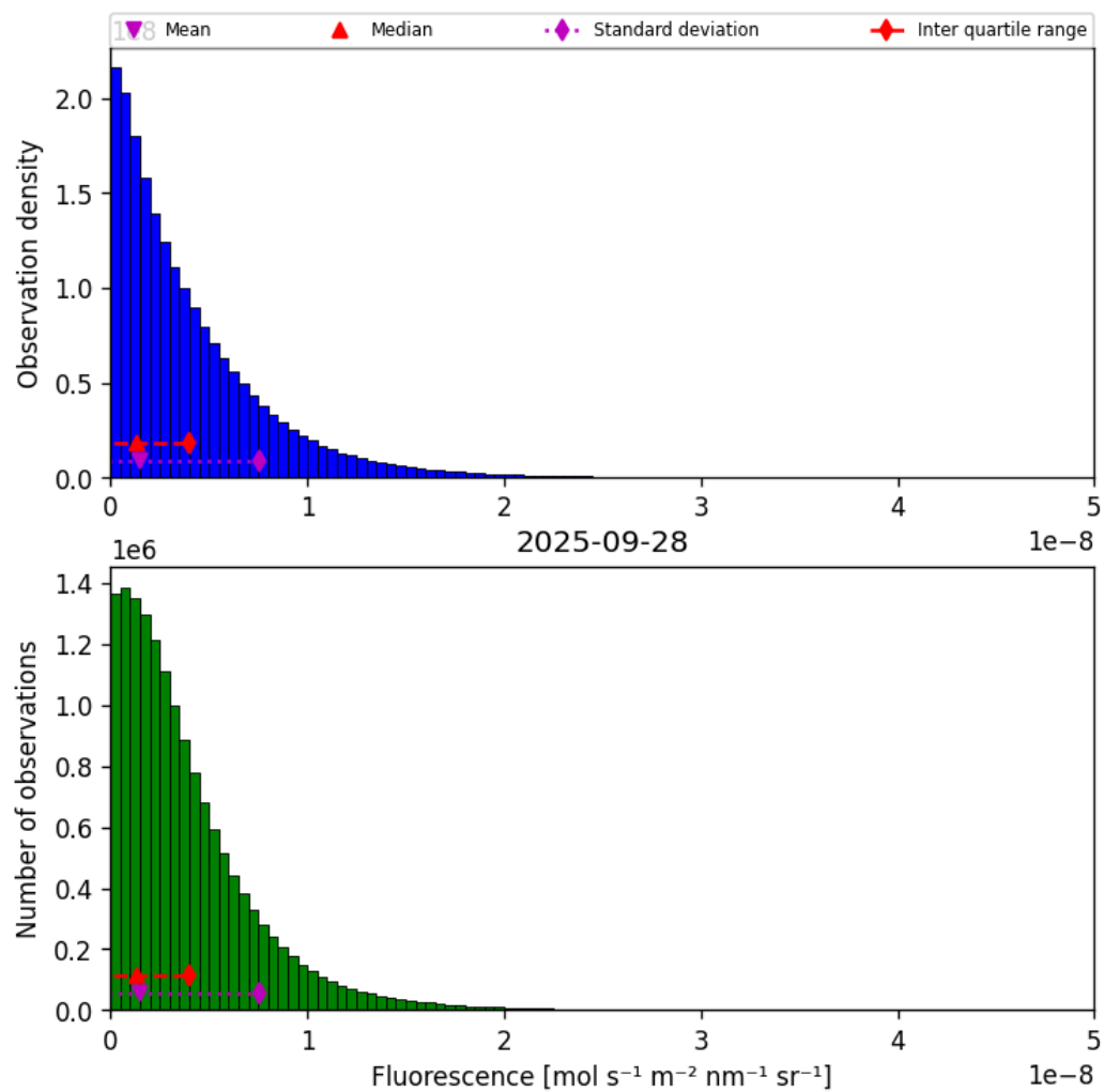
Figure 38: Histogram of “Fluorescence” for 2025-09-28 to 2025-09-29
