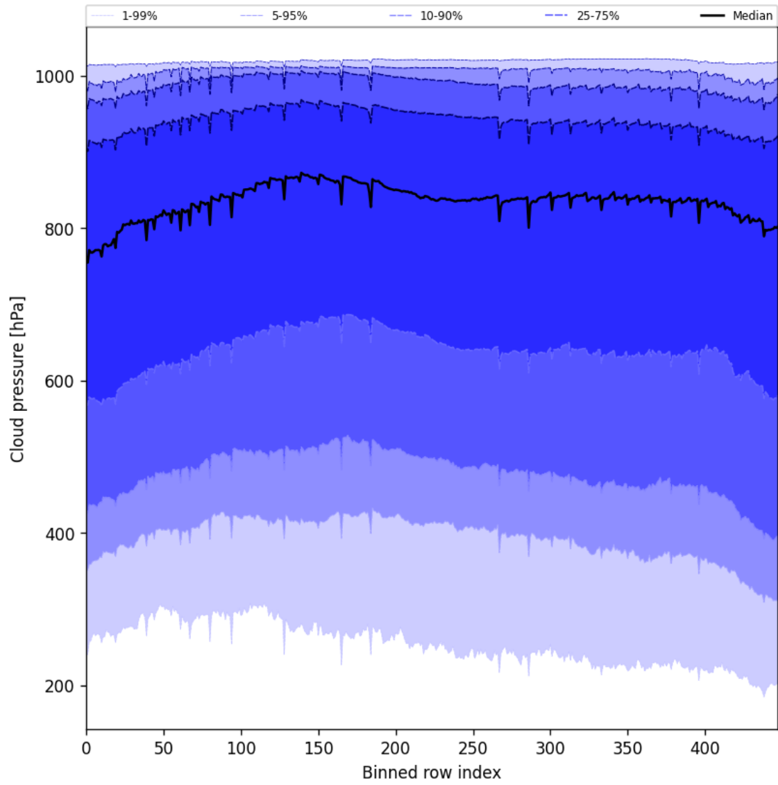
Figure 45: Along track statistics of “Cloud pressure” for 2025-09-28 to 2025-09-29
