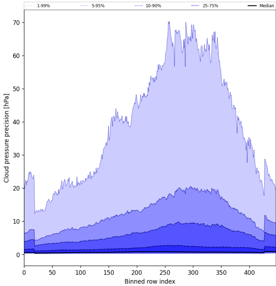
Figure 46: Along track statistics of “Cloud pressure precision” for 2025-09-28 to 2025-09-29
