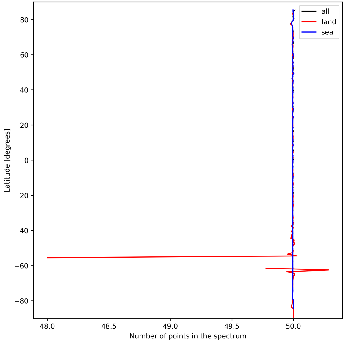
Figure 25: Zonal average of “Number of points in the spectrum” for 2025-09-28 to 2025-09-29.
