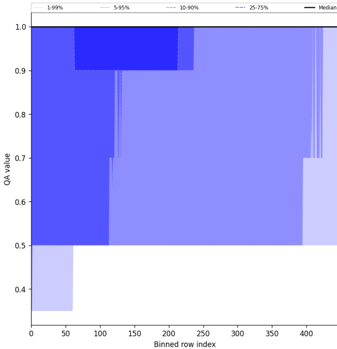
Figure 44: Along track statistics of “QA value” for 2025-09-28 to 2025-09-29
