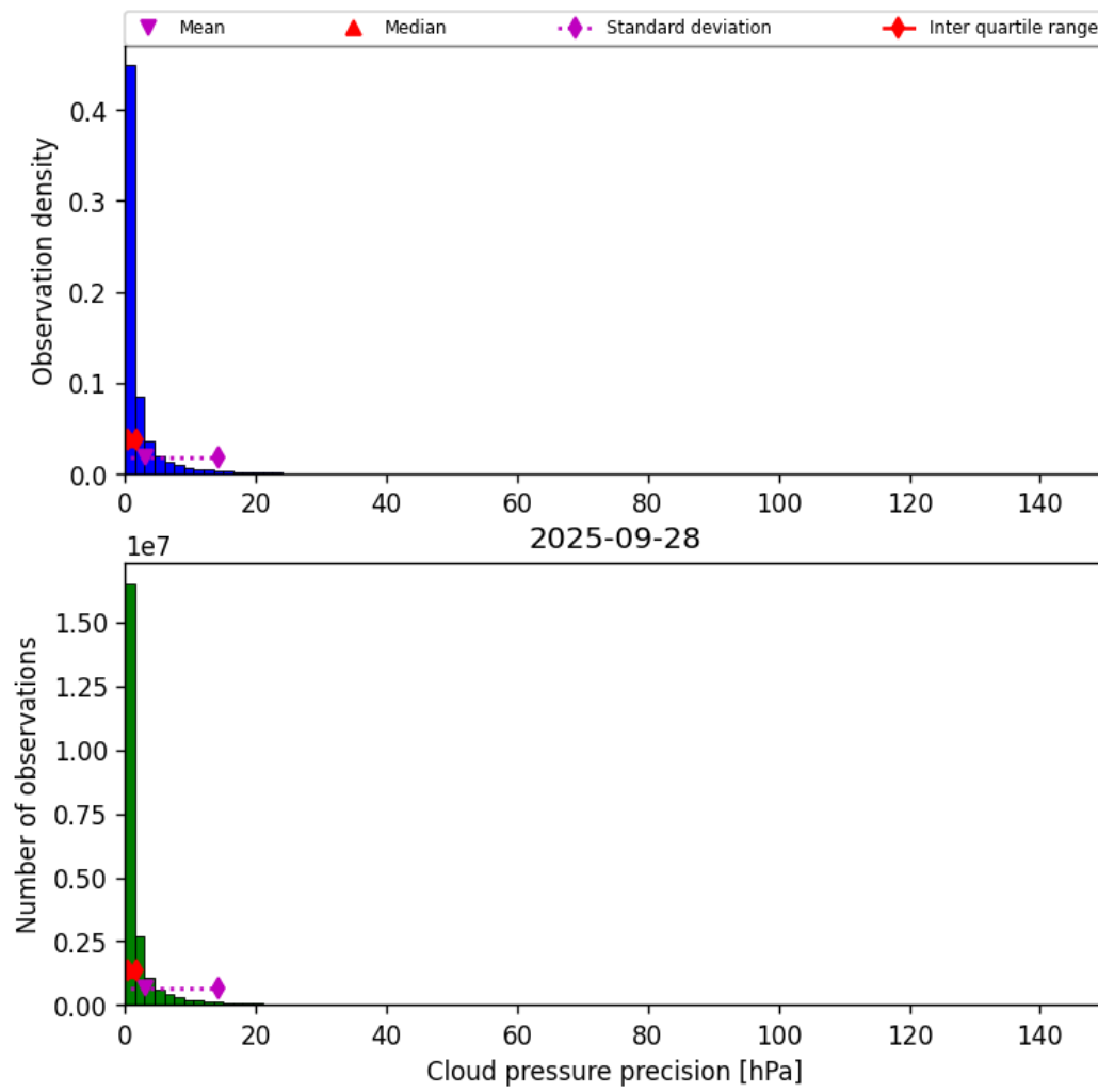
Figure 29: Histogram of “Cloud pressure precision” for 2025-09-28 to 2025-09-29
