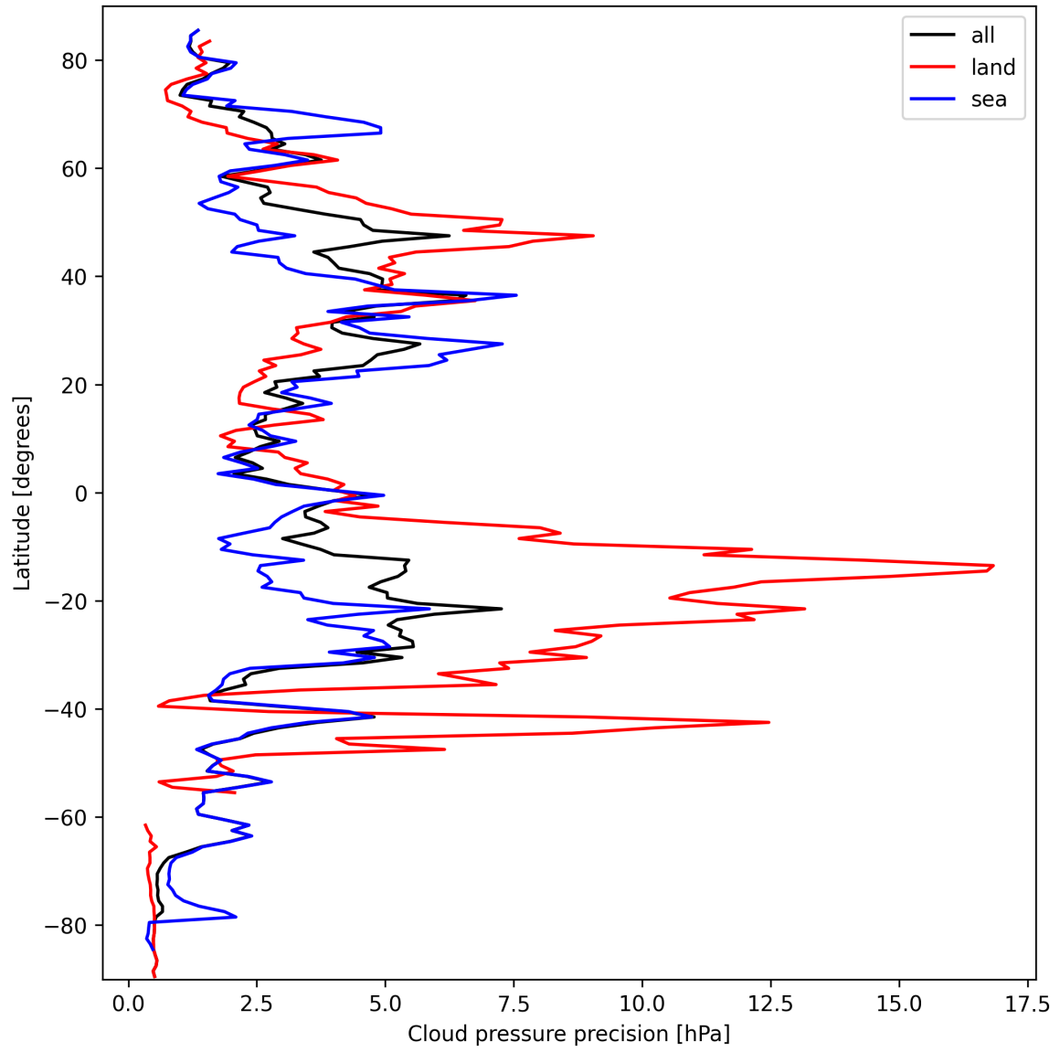
Figure 12: Zonal average of “Cloud pressure precision” for 2025-09-28 to 2025-09-29.
