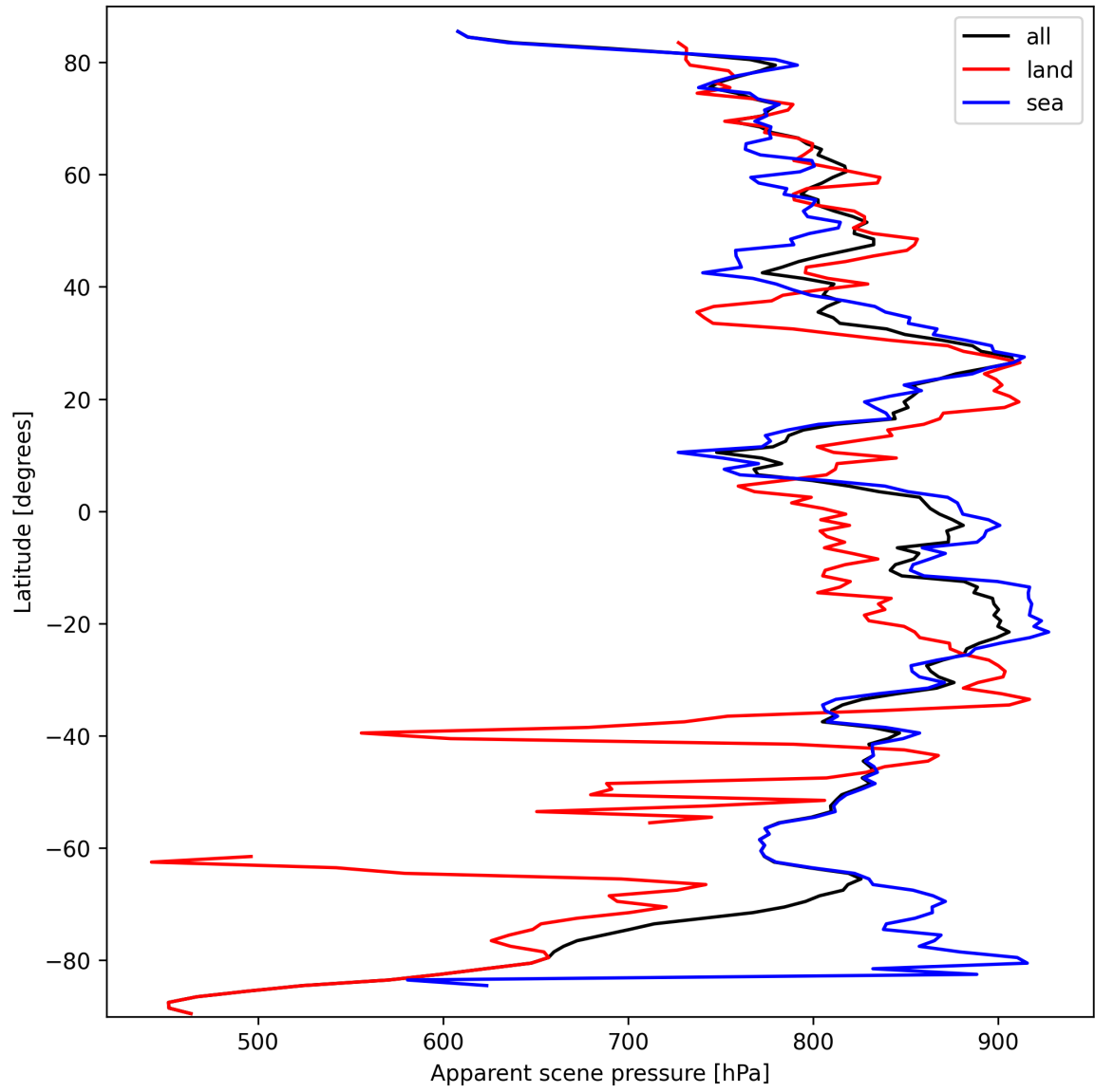
Figure 17: Zonal average of “Apparent scene pressure” for 2025-09-28 to 2025-09-29.
