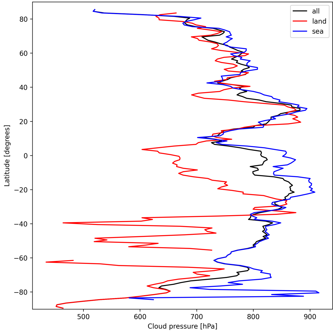
Figure 11: Zonal average of “Cloud pressure” for 2025-09-28 to 2025-09-29.
