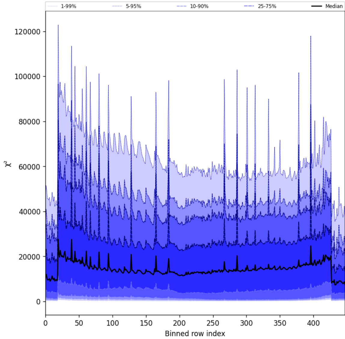
Figure 53: Along track statistics of “ \chi^2 ” for 2025-09-28 to 2025-09-29
