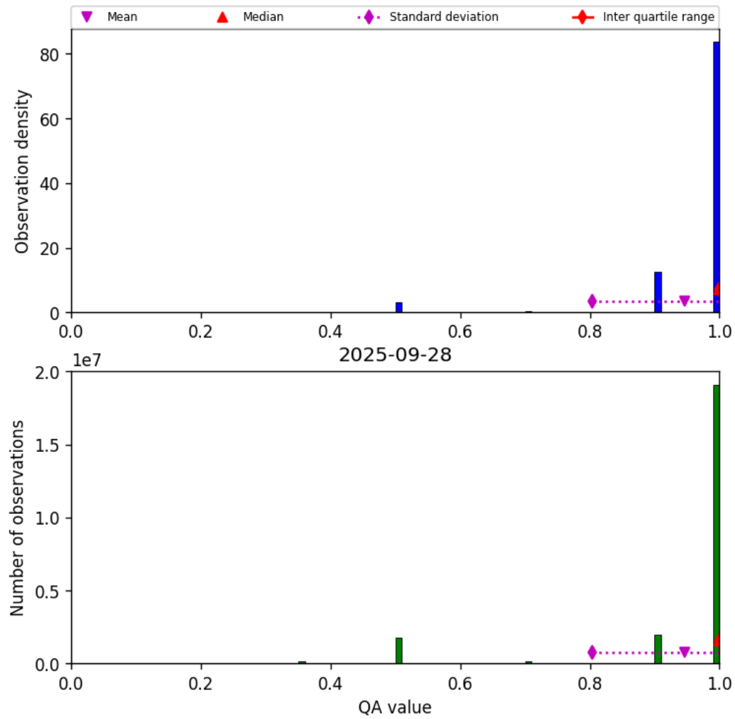
Figure 27: Histogram of “QA value” for 2025-09-28 to 2025-09-29
