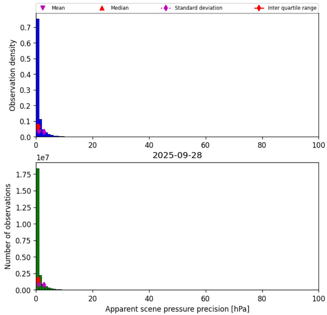
Figure 35: Histogram of “Apparent scene pressure precision” for 2025-09-28 to 2025-09-29
