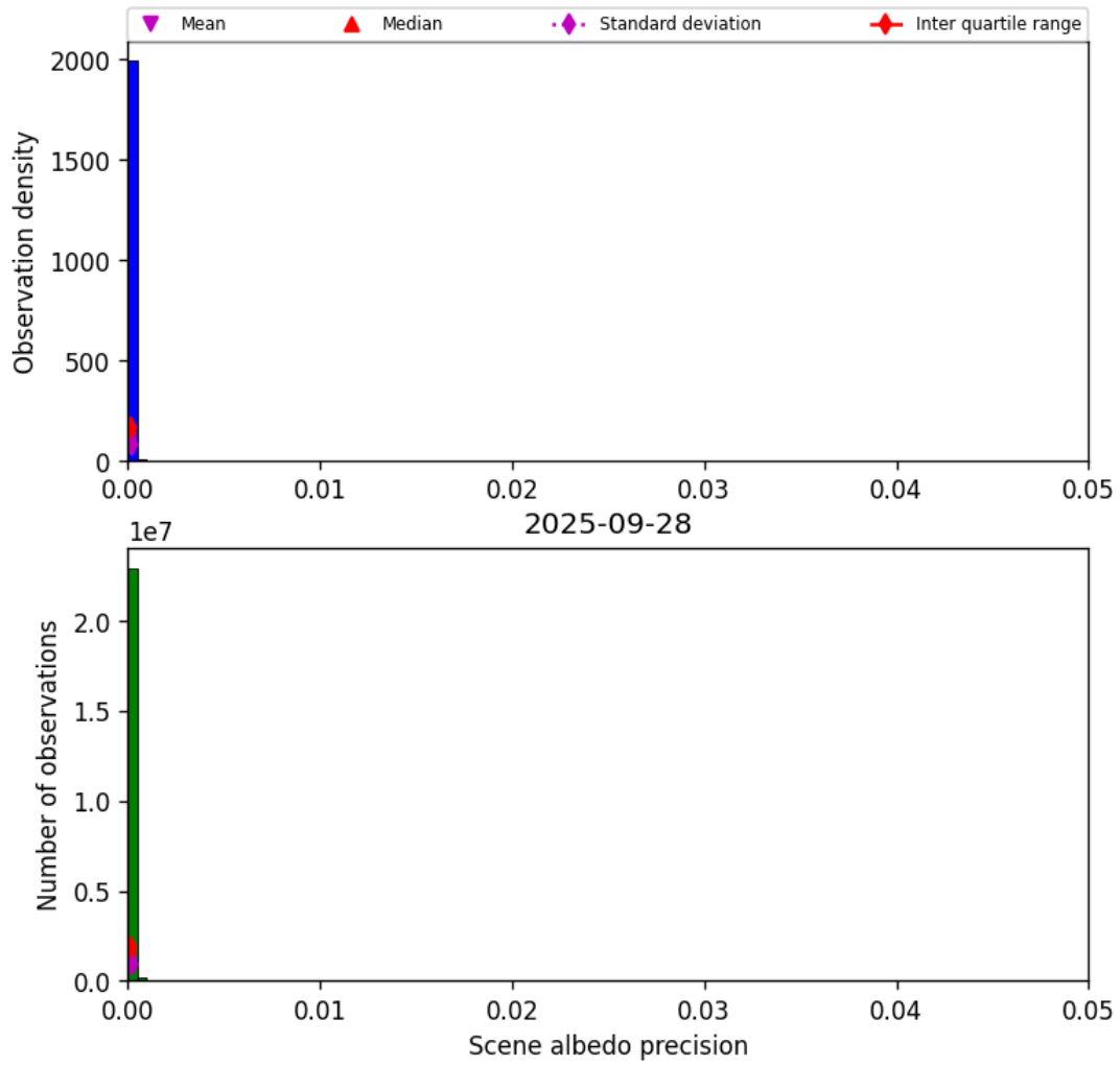
Figure 33: Histogram of “Scene albedo precision” for 2025-09-28 to 2025-09-29
