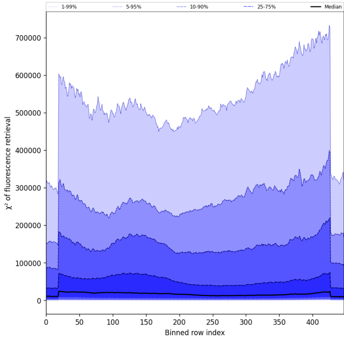
Figure 57: Along track statistics of “ \chi^2 of fluorescence retrieval” for 2025-09-28 to 2025-09-29
