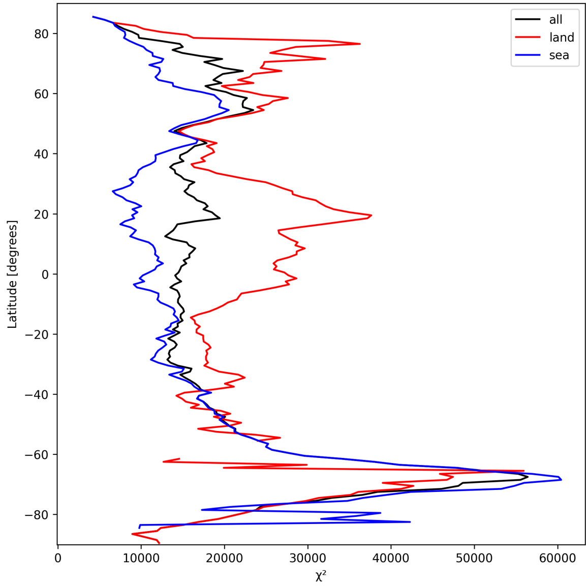
Figure 19: Zonal average of “ \chi^2 ” for 2025-09-28 to 2025-09-29.
