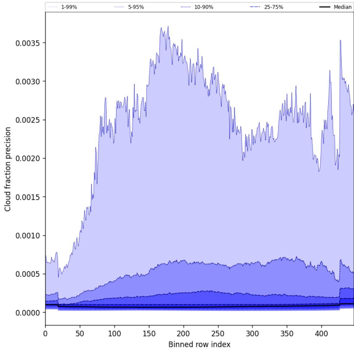
Figure 48: Along track statistics of “Cloud fraction precision” for 2025-09-28 to 2025-09-29
