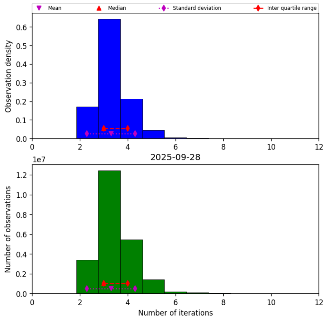
Figure 37: Histogram of “Number of iterations” for 2025-09-28 to 2025-09-29
