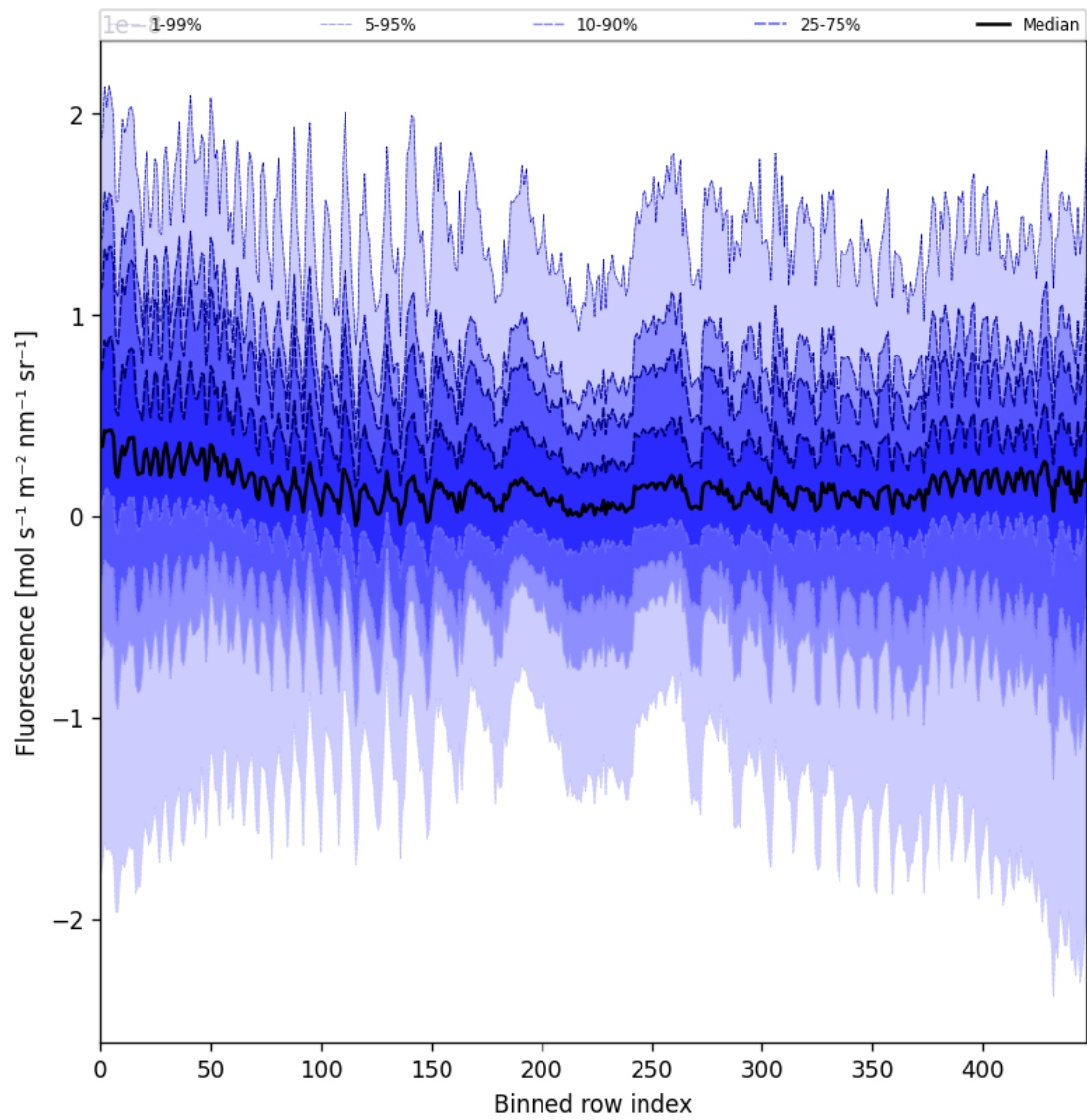
Figure 55: Along track statistics of “Fluorescence” for 2025-09-28 to 2025-09-29
