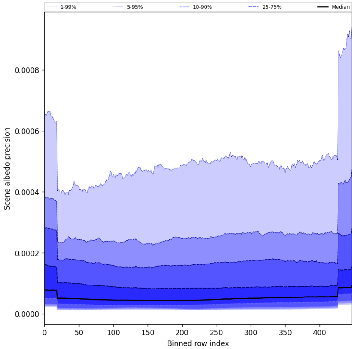
Figure 50: Along track statistics of “Scene albedo precision” for 2025-09-28 to 2025-09-29
