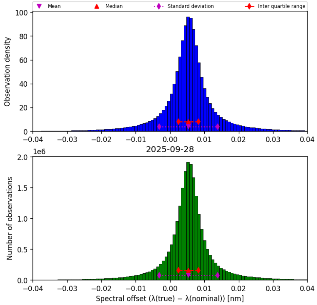
Figure 43: Histogram of “Spectral offset ( \lambda_{\text{true}} - \lambda_{\text{nominal}} )” for 2025-09-28 to 2025-09-29
