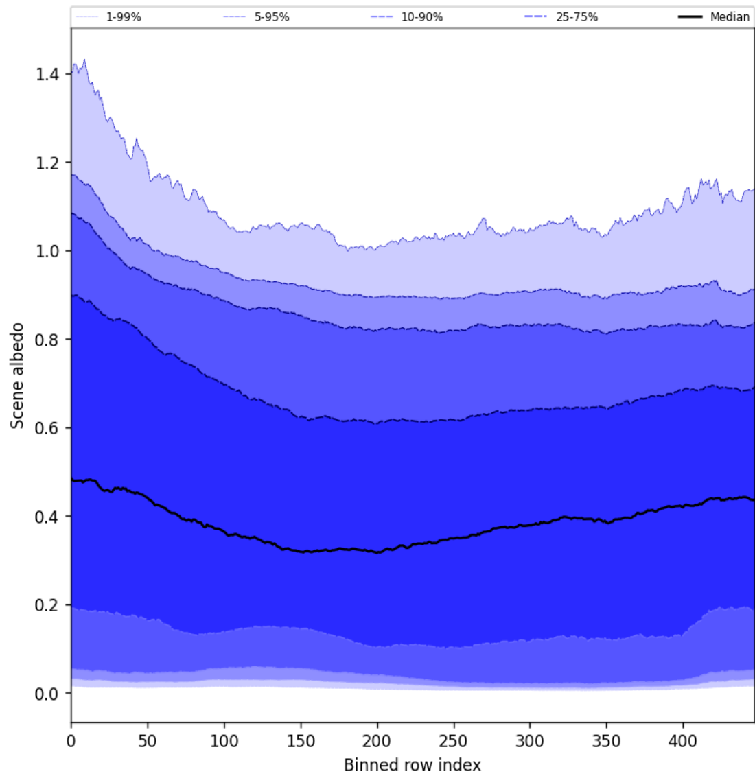
Figure 49: Along track statistics of “Scene albedo” for 2025-09-28 to 2025-09-29
