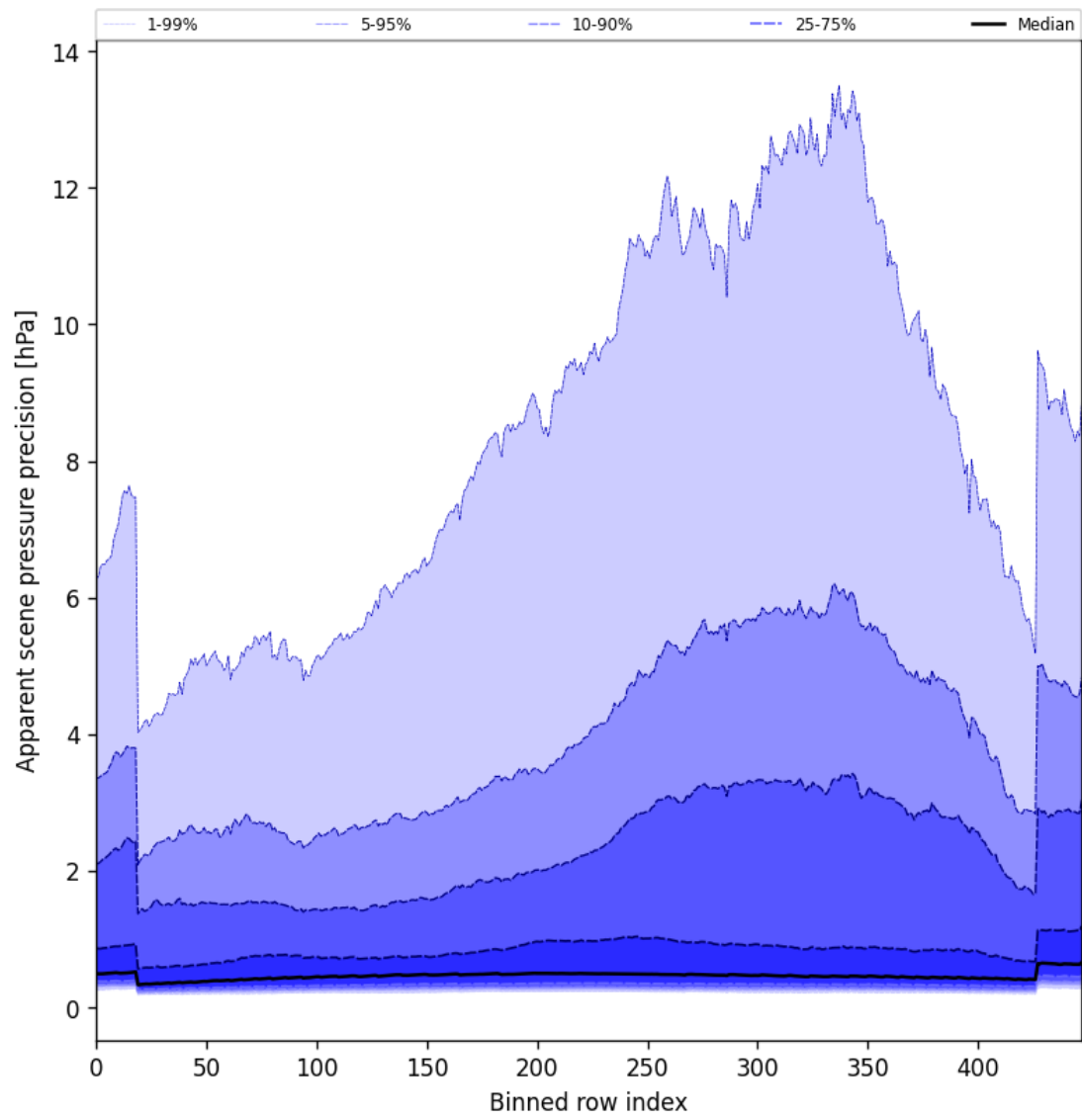
Figure 52: Along track statistics of “Apparent scene pressure precision” for 2025-09-28 to 2025-09-29
