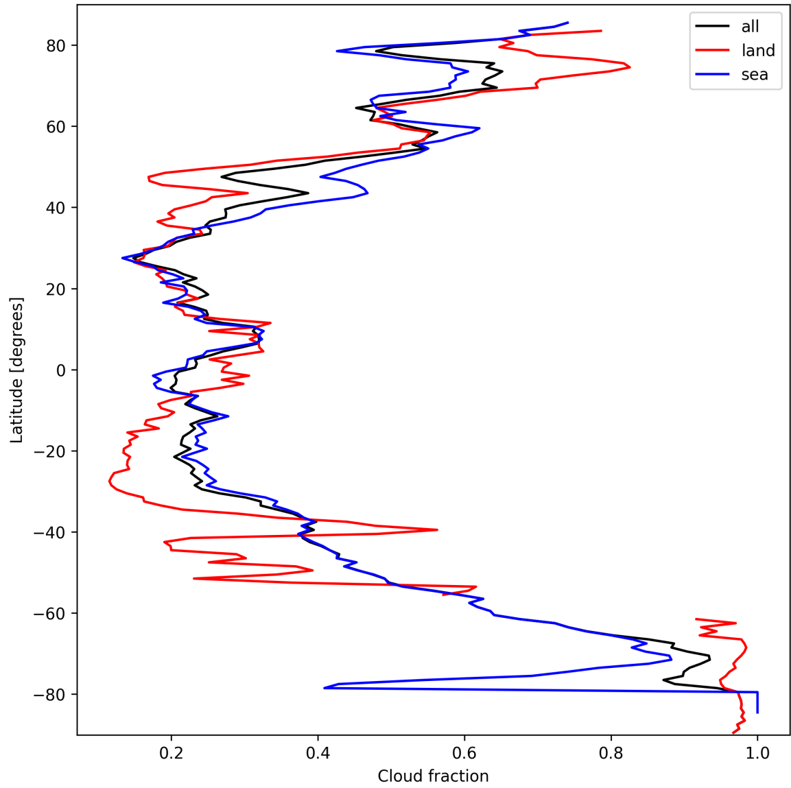
Figure 13: Zonal average of “Cloud fraction” for 2025-09-28 to 2025-09-29.
