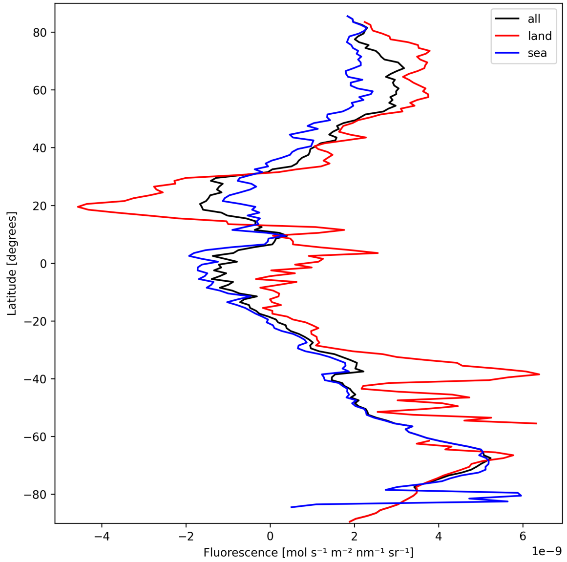
Figure 21: Zonal average of “Fluorescence” for 2025-09-28 to 2025-09-29.
