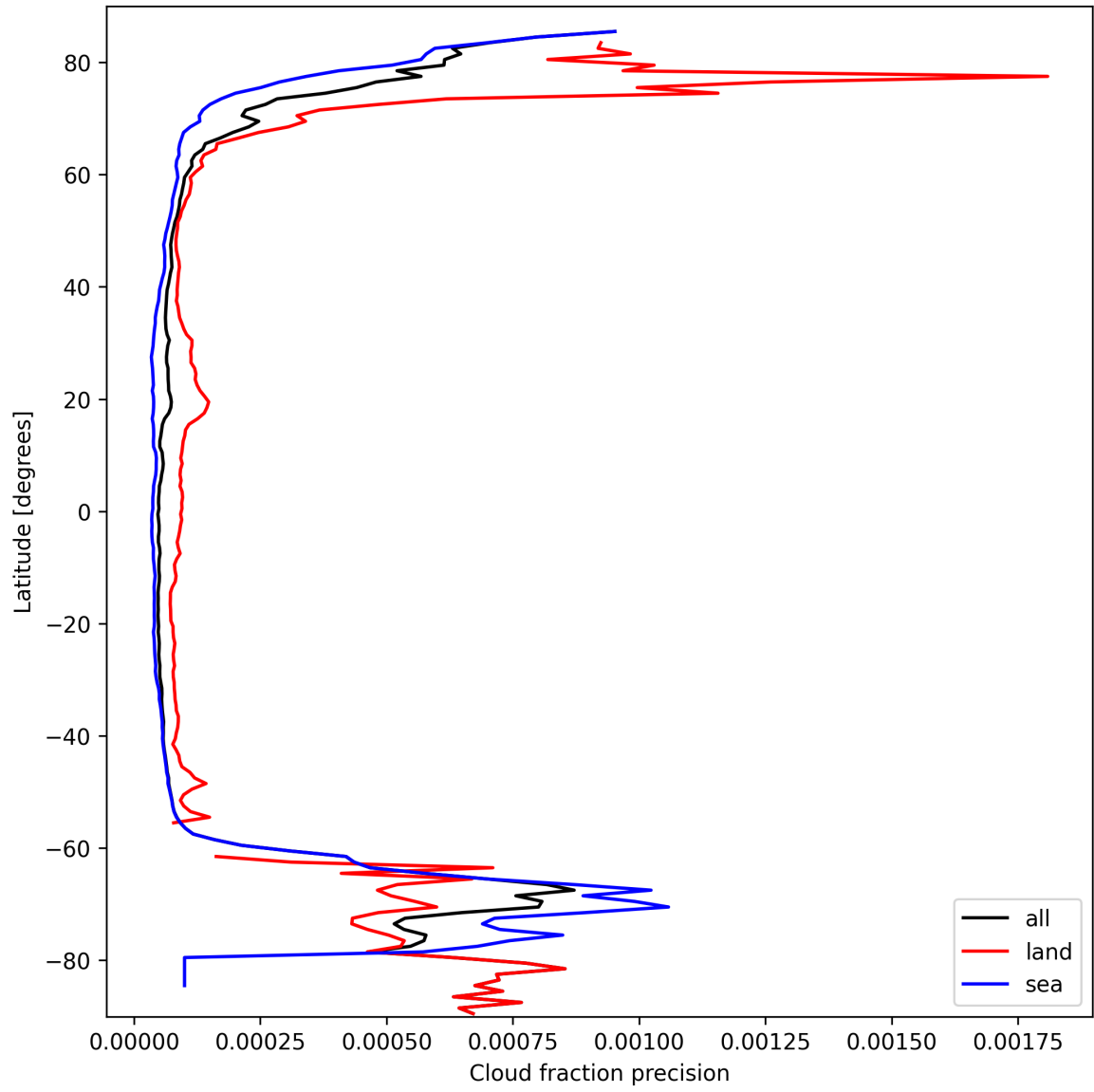
Figure 14: Zonal average of “Cloud fraction precision” for 2025-09-28 to 2025-09-29.
