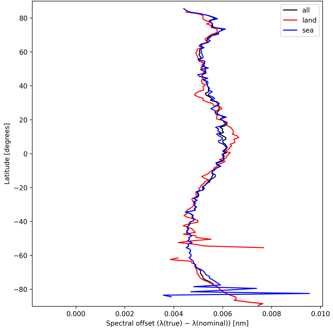
Figure 26: Zonal average of “Spectral offset ( \lambda_{\text{true}} - \lambda_{\text{nominal}} )” for 2025-09-28 to 2025-09-29.
