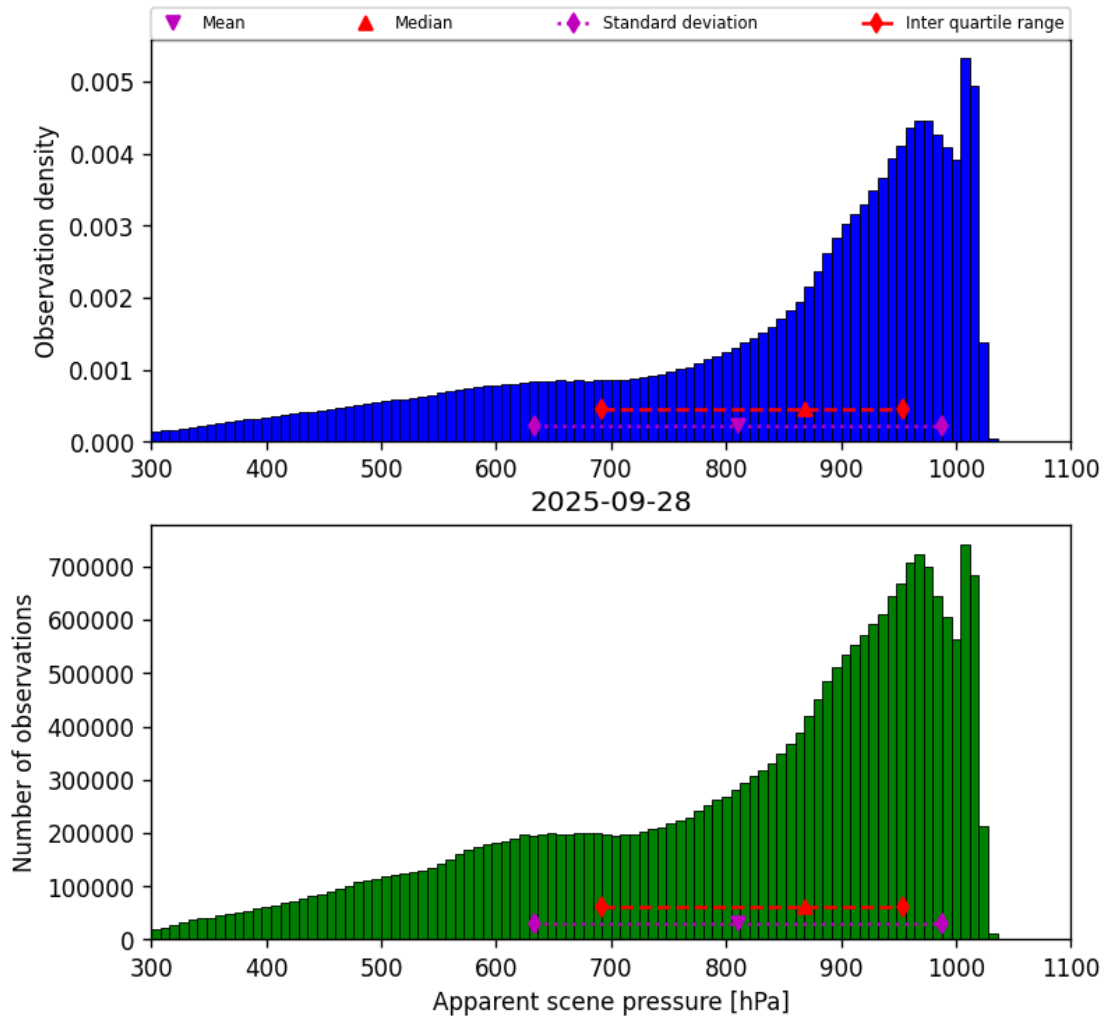
Figure 34: Histogram of “Apparent scene pressure” for 2025-09-28 to 2025-09-29
