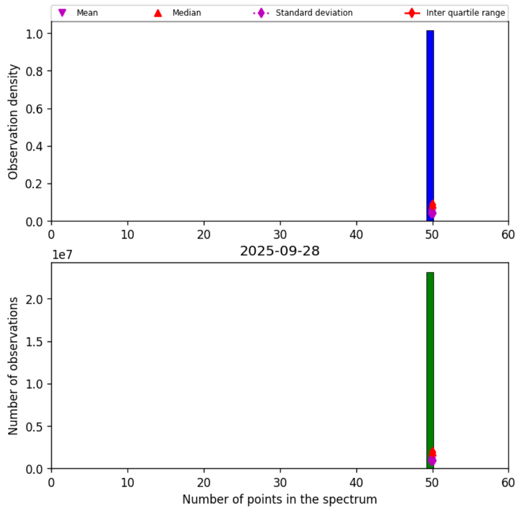
Figure 42: Histogram of “Number of points in the spectrum” for 2025-09-28 to 2025-09-29
