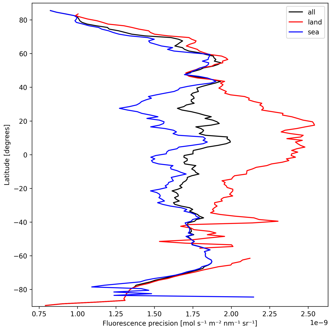
Figure 22: Zonal average of “Fluorescence precision” for 2025-09-28 to 2025-09-29.
