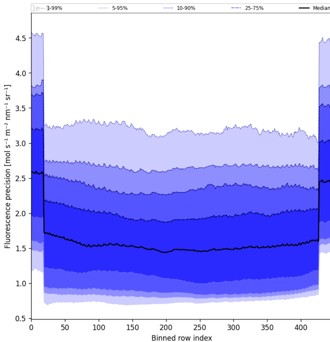
Figure 56: Along track statistics of “Fluorescence precision” for 2025-09-28 to 2025-09-29
