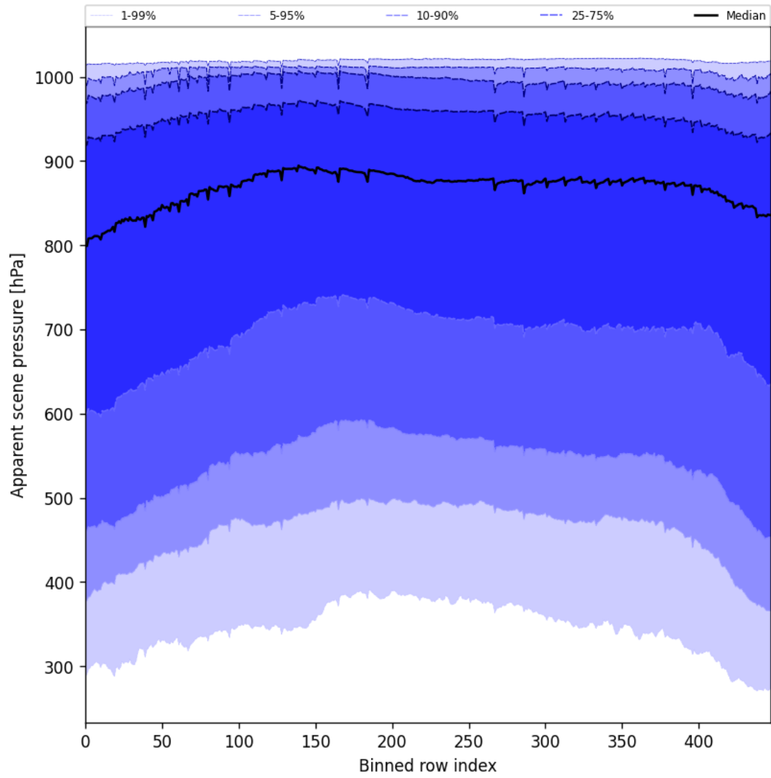
Figure 51: Along track statistics of “Apparent scene pressure” for 2025-09-28 to 2025-09-29
