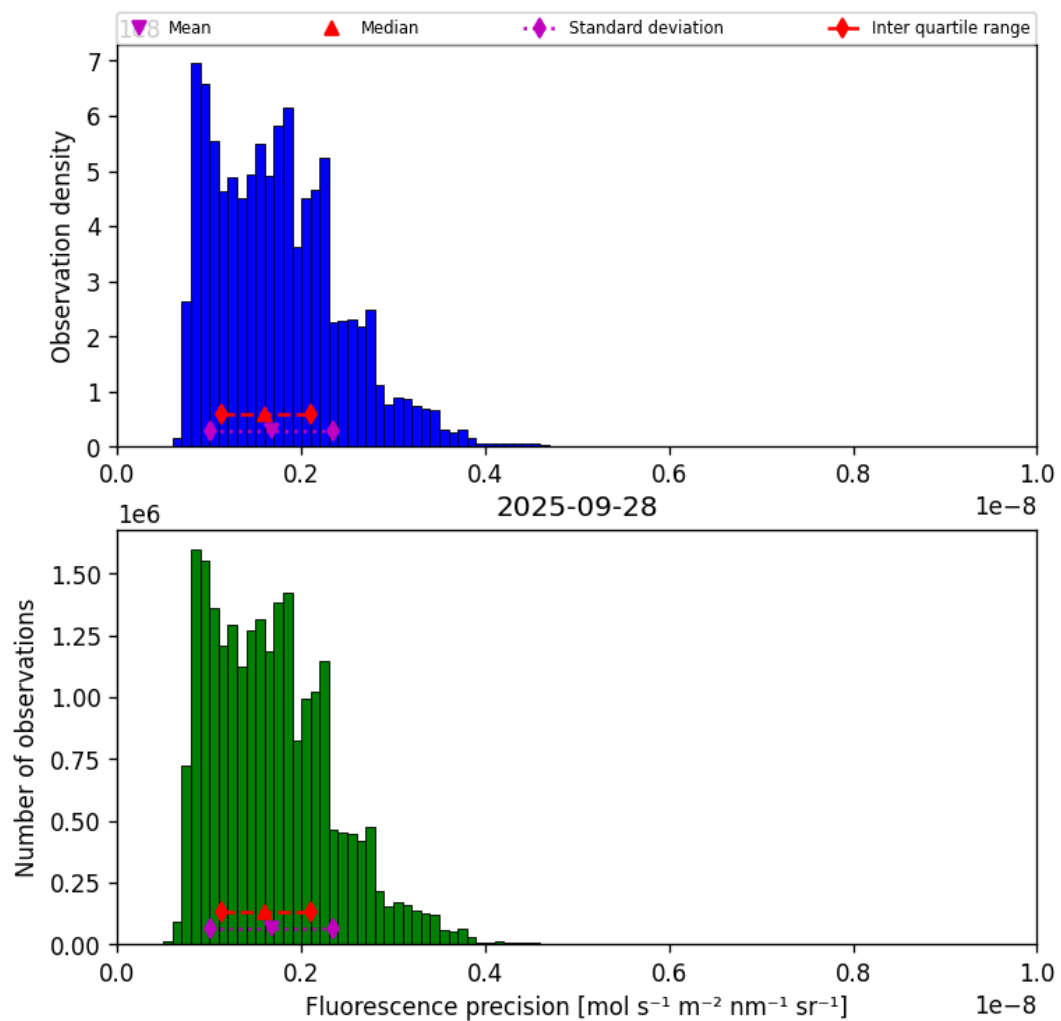
Figure 39: Histogram of “Fluorescence precision” for 2025-09-28 to 2025-09-29
