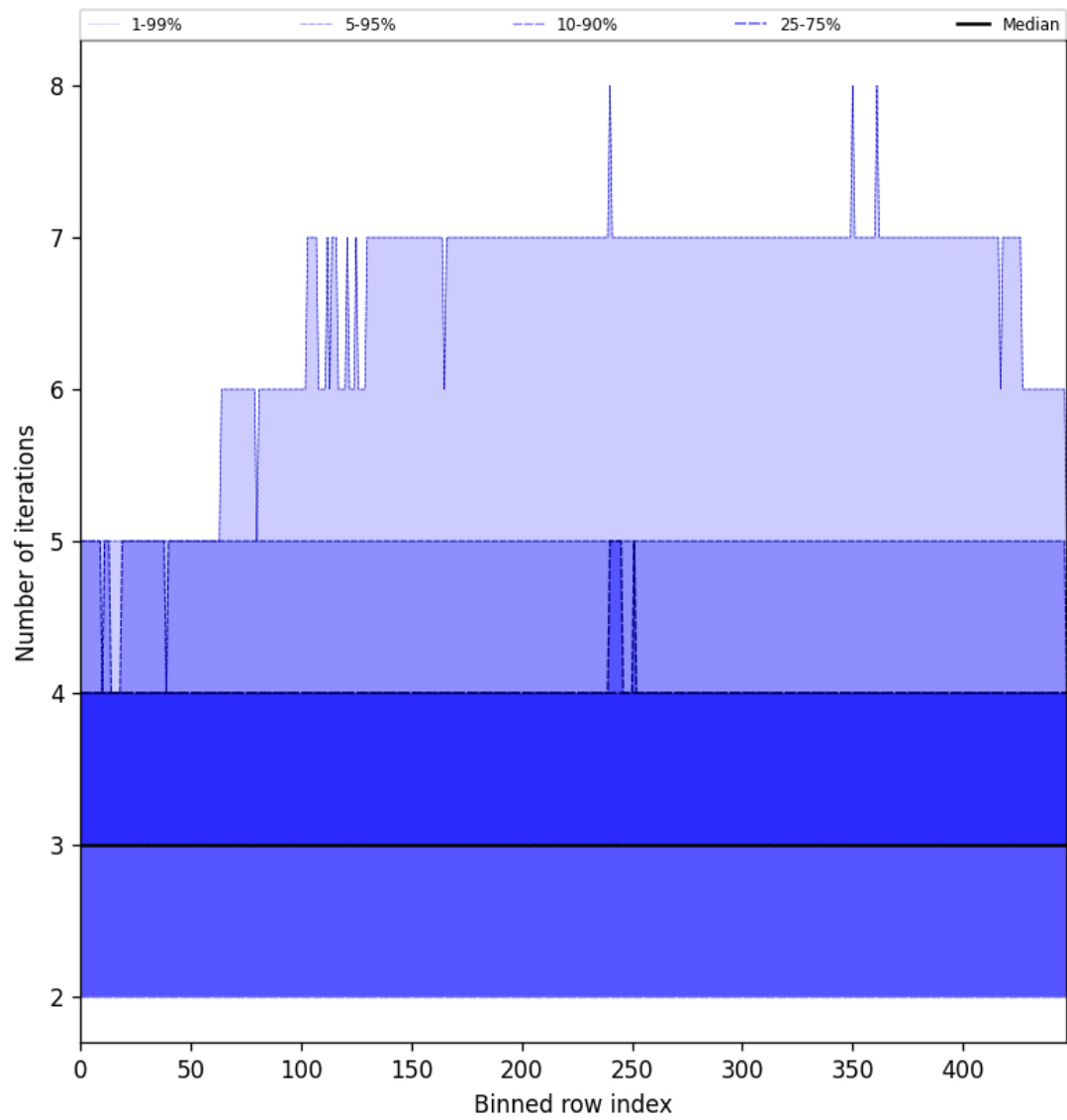
Figure 54: Along track statistics of “Number of iterations” for 2025-09-28 to 2025-09-29
