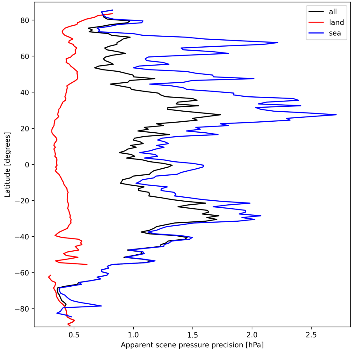
Figure 18: Zonal average of “Apparent scene pressure precision” for 2025-09-28 to 2025-09-29.
