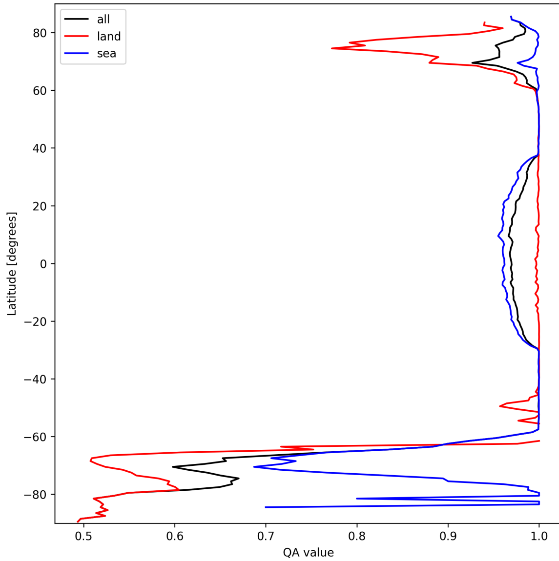
Figure 10: Zonal average of “QA value” for 2025-09-28 to 2025-09-29.
