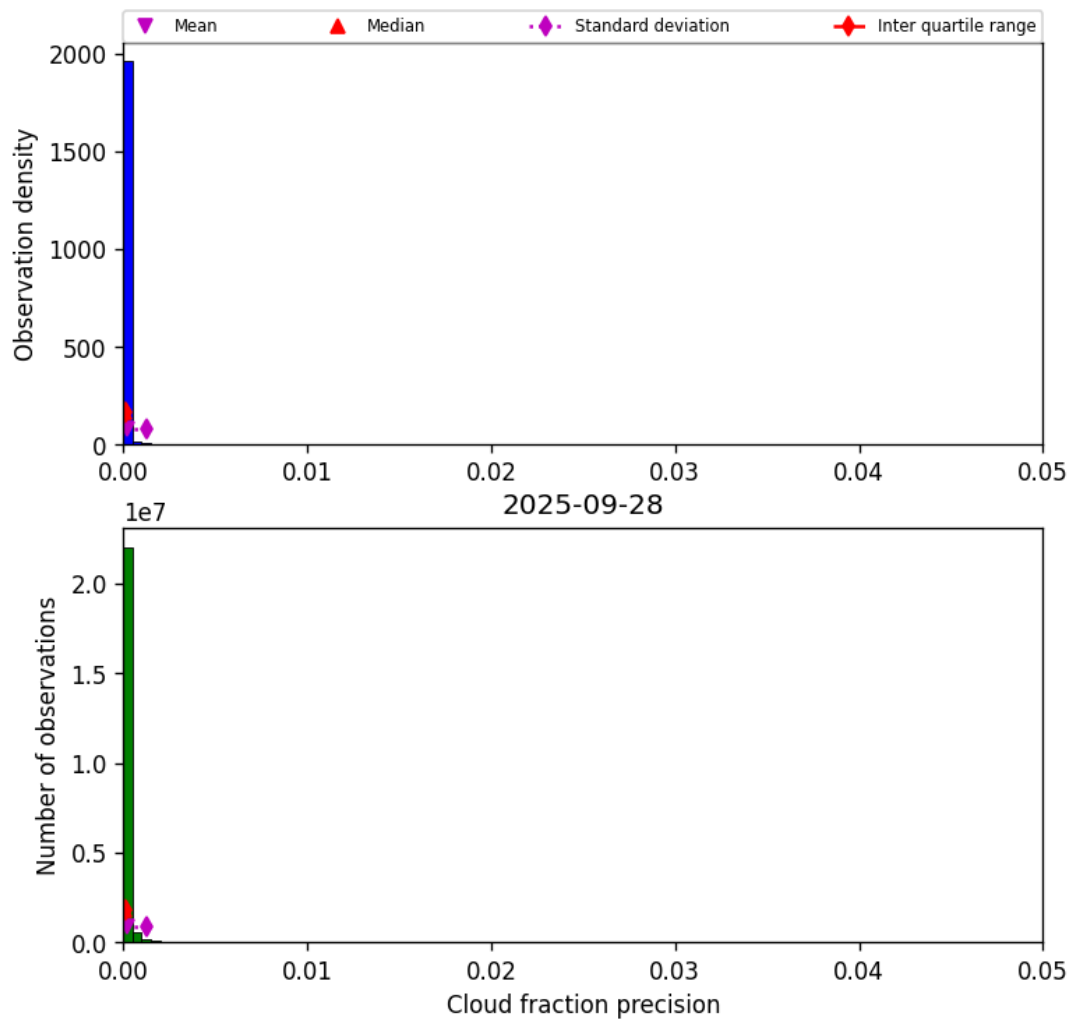
Figure 31: Histogram of “Cloud fraction precision” for 2025-09-28 to 2025-09-29
