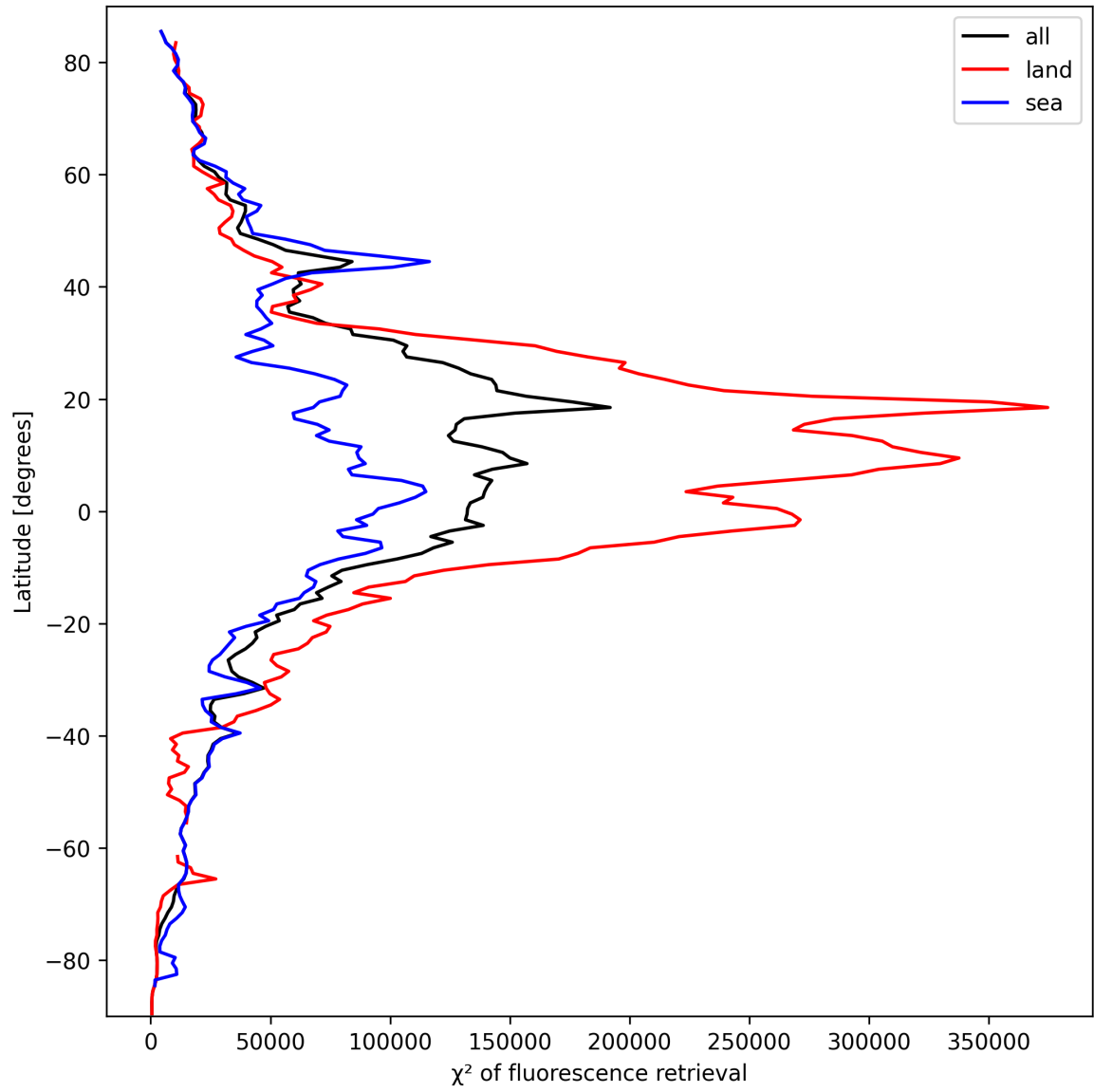
Figure 23: Zonal average of “ \chi^2 of fluorescence retrieval” for 2025-09-28 to 2025-09-29.
