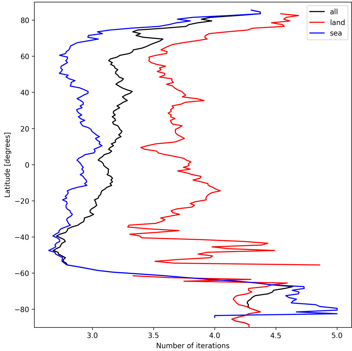
Figure 20: Zonal average of “Number of iterations” for 2025-09-28 to 2025-09-29.
