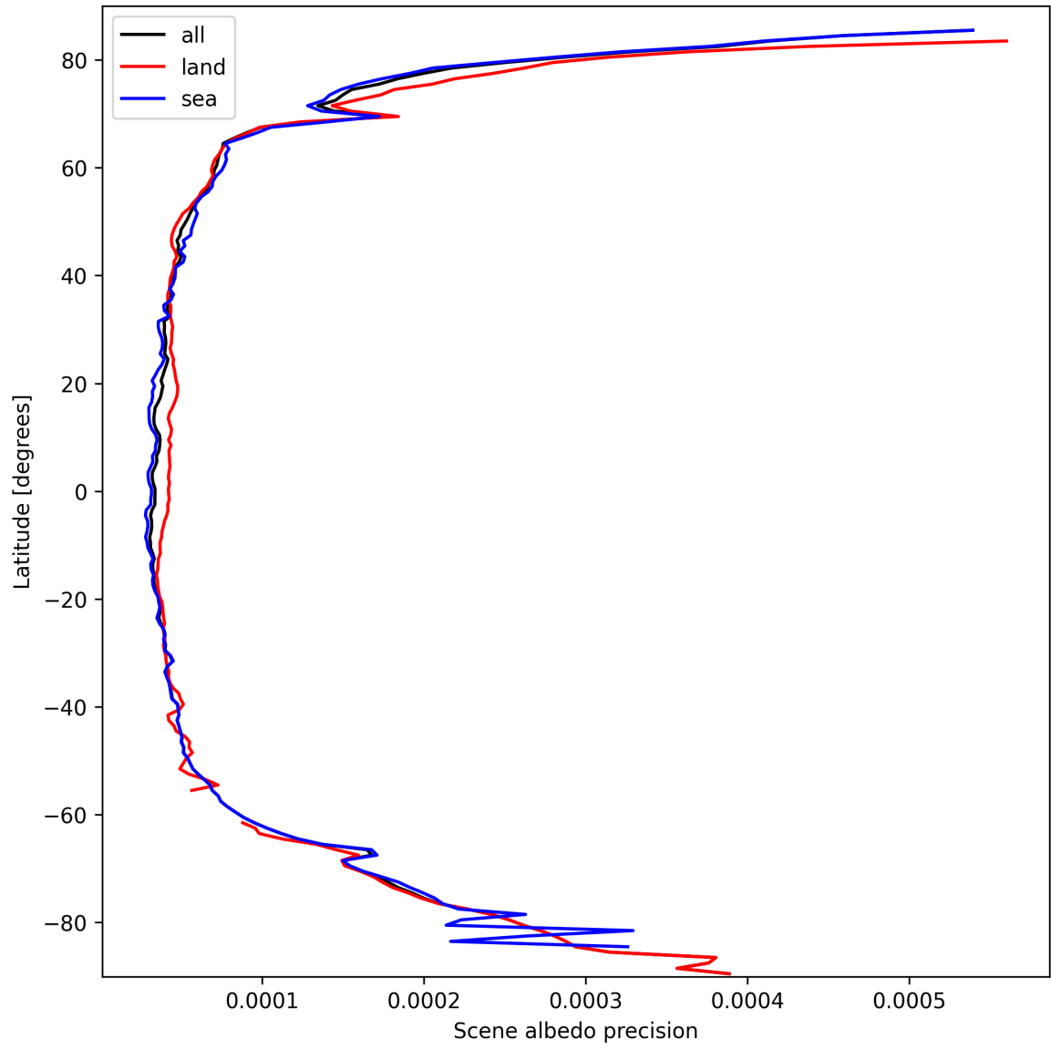
Figure 16: Zonal average of “Scene albedo precision” for 2025-09-28 to 2025-09-29.
