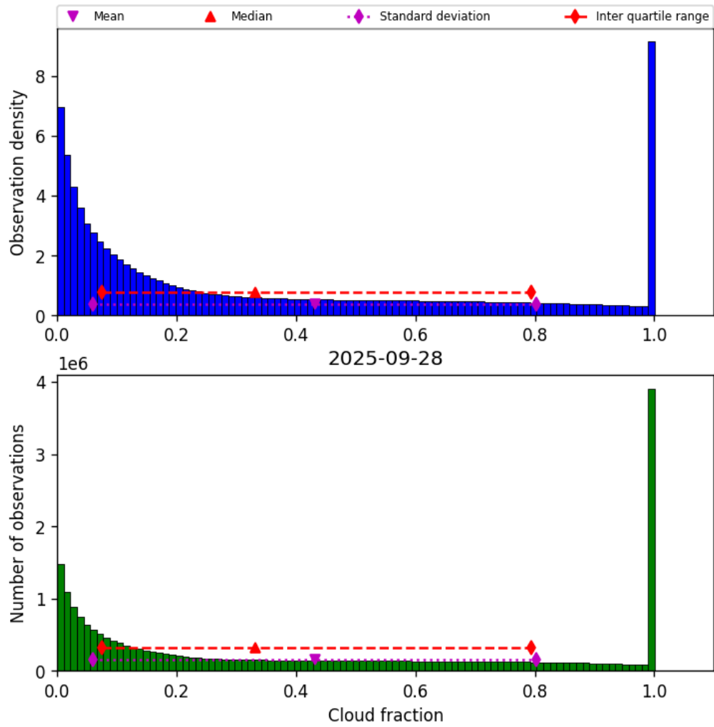
Figure 30: Histogram of “Cloud fraction” for 2025-09-28 to 2025-09-29
