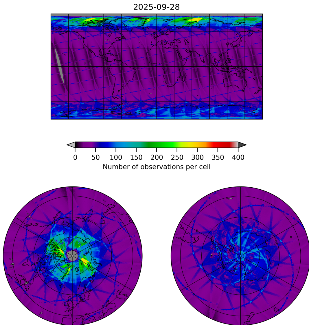
Figure 9: Map of the number of observations for 2025-09-28 to 2025-09-29
