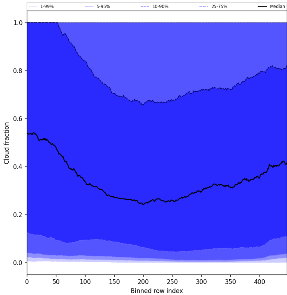
Figure 47: Along track statistics of “Cloud fraction” for 2025-09-28 to 2025-09-29
