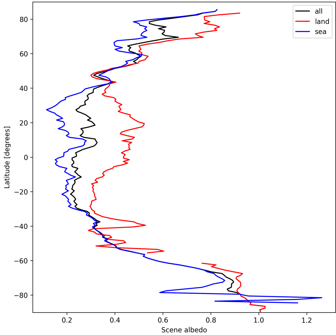
Figure 15: Zonal average of “Scene albedo” for 2025-09-28 to 2025-09-29.
