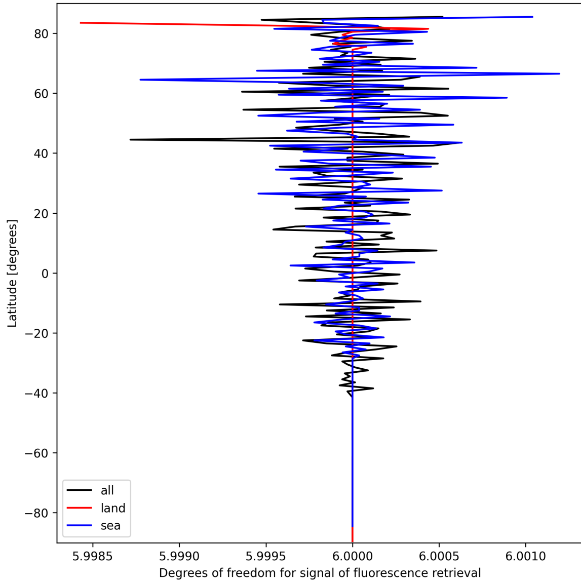
Figure 24: Zonal average of “Degrees of freedom for signal of fluorescence retrieval” for 2025-09-28 to 2025-09-29.
