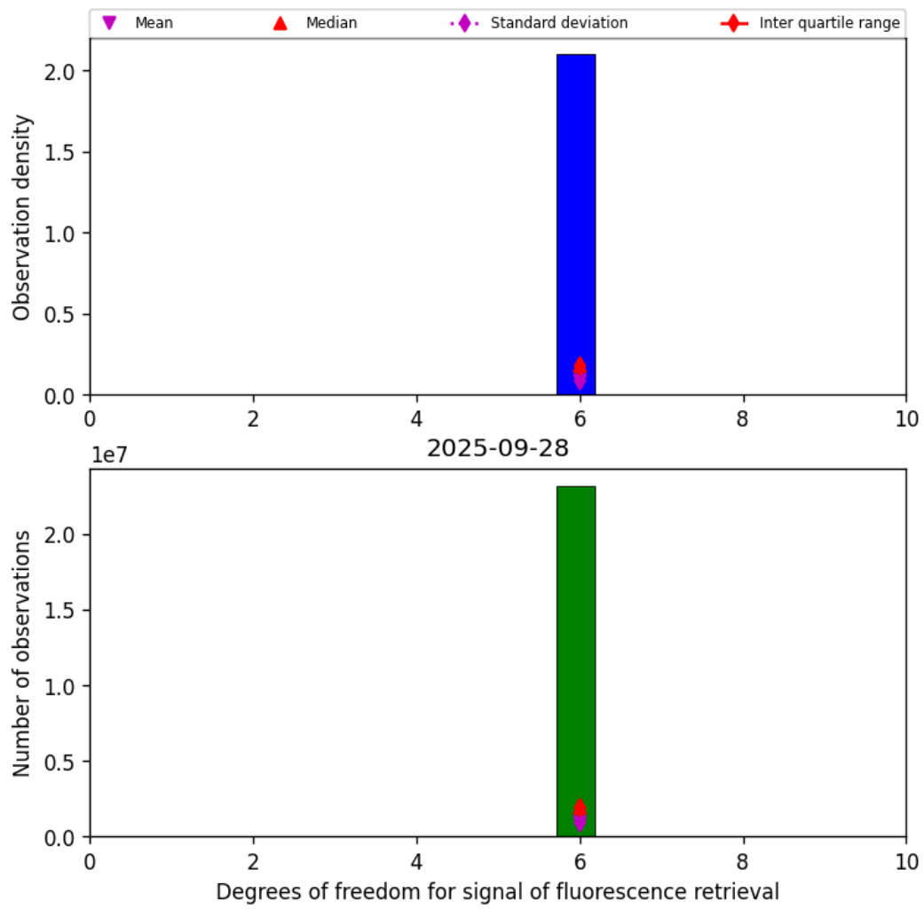
Figure 41: Histogram of “Degrees of freedom for signal of fluorescence retrieval” for 2025-09-28 to 2025-09-29
