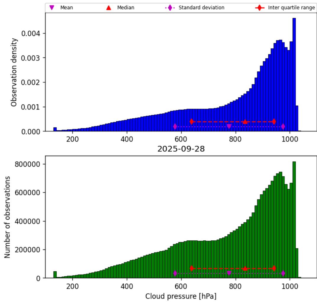
Figure 28: Histogram of “Cloud pressure” for 2025-09-28 to 2025-09-29
