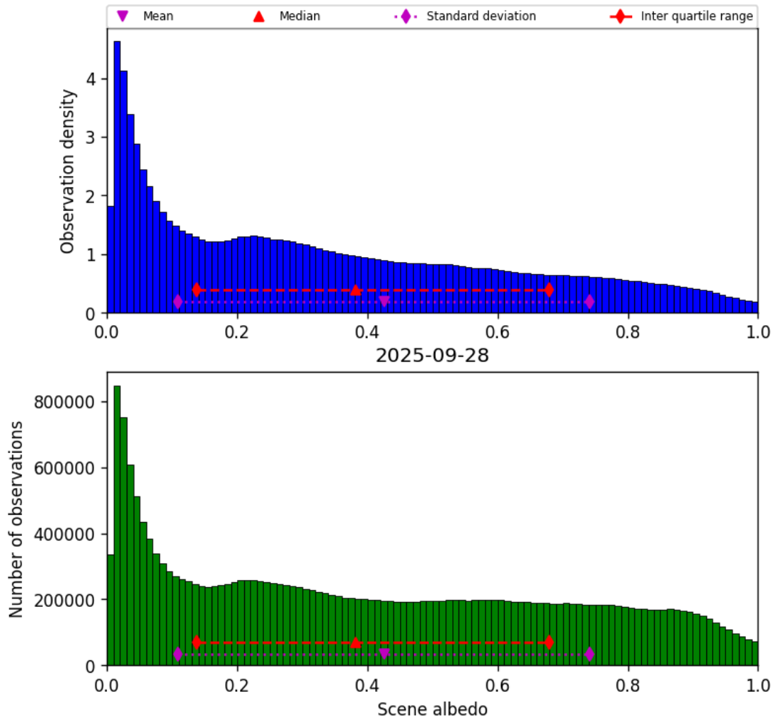
Figure 32: Histogram of “Scene albedo” for 2025-09-28 to 2025-09-29
