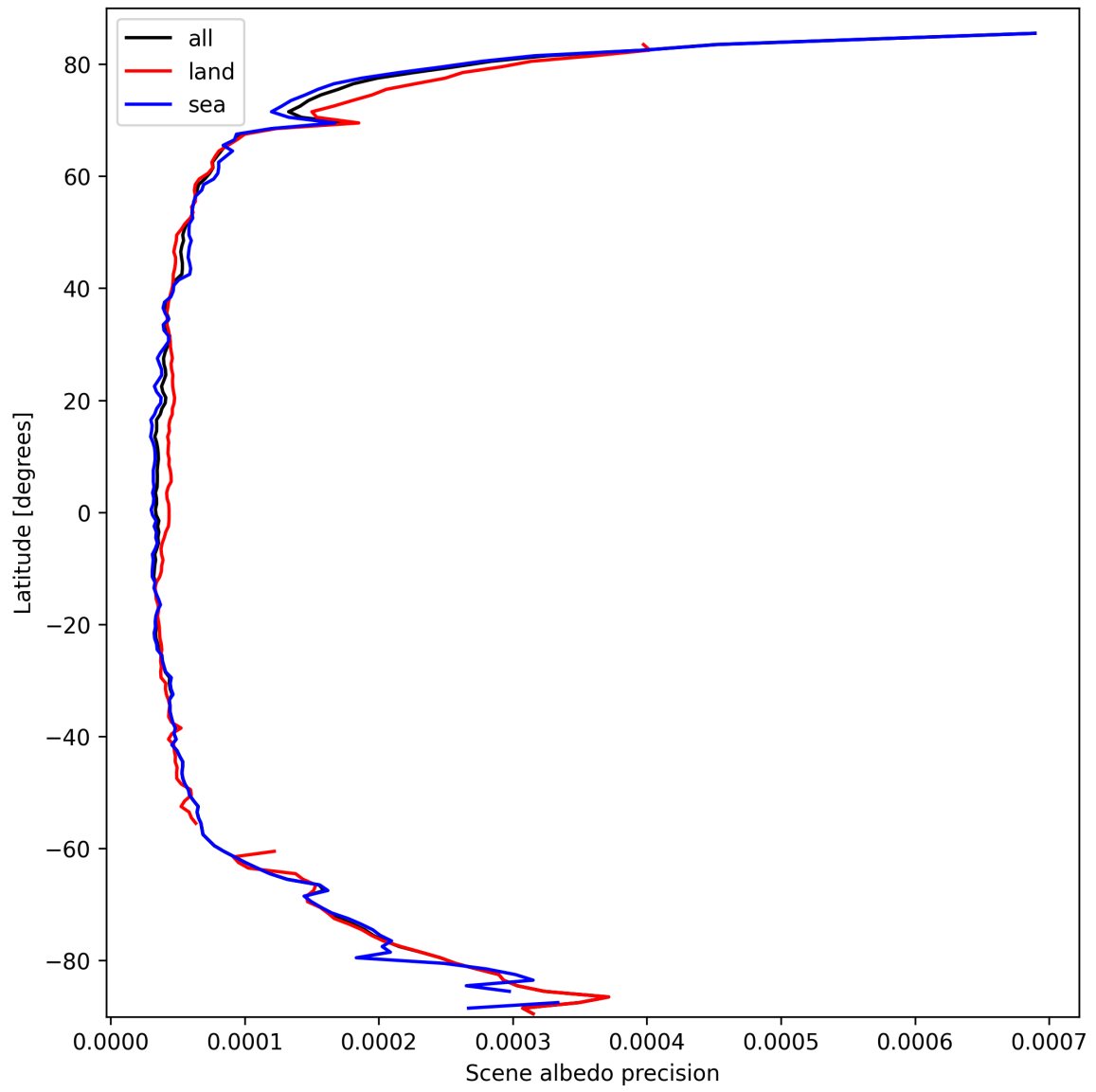
Figure 16: Zonal average of “Scene albedo precision” for 2025-09-29 to 2025-09-29.
