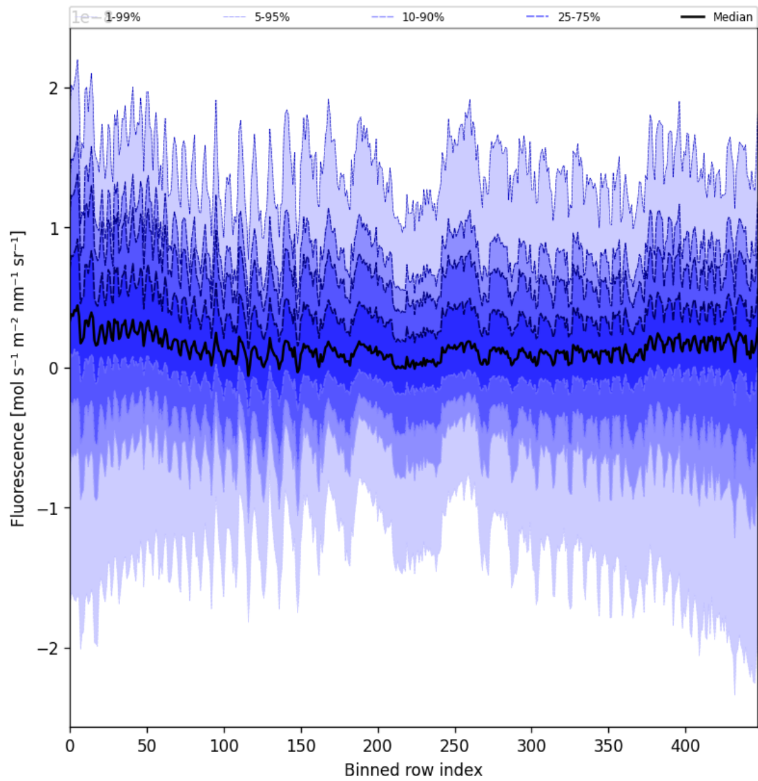
Figure 55: Along track statistics of “Fluorescence” for 2025-09-29 to 2025-09-29
