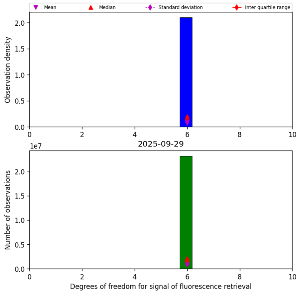
Figure 41: Histogram of “Degrees of freedom for signal of fluorescence retrieval” for 2025-09-29 to 2025-09-29
