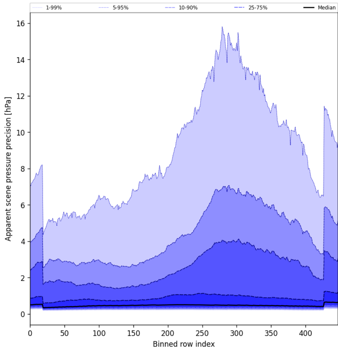
Figure 52: Along track statistics of “Apparent scene pressure precision” for 2025-09-29 to 2025-09-29
