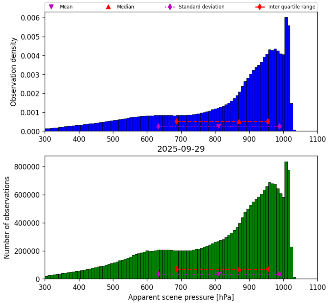
Figure 34: Histogram of “Apparent scene pressure” for 2025-09-29 to 2025-09-29
