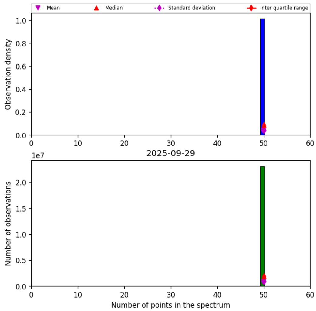
Figure 42: Histogram of "Number of points in the spectrum" for 2025-09-29 to 2025-09-29
