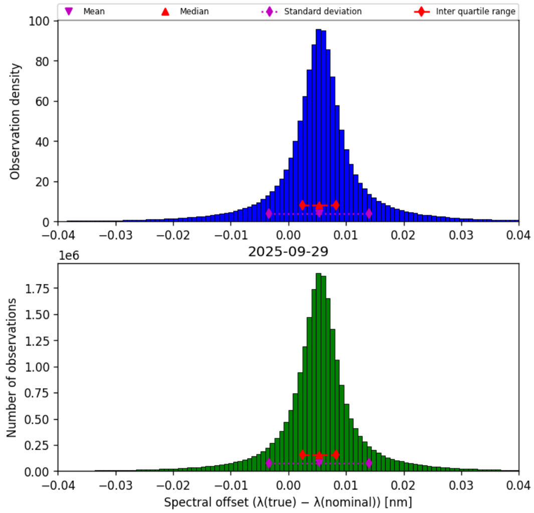
Figure 43: Histogram of “Spectral offset ( \lambda_{\text{true}} - \lambda_{\text{nominal}} )” for 2025-09-29 to 2025-09-29
