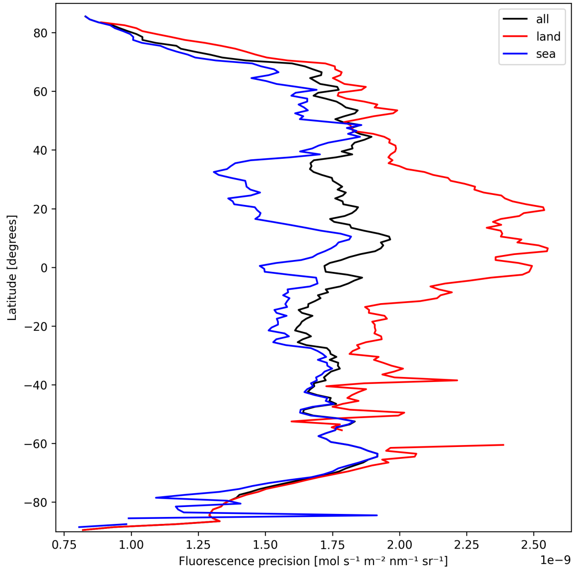
Figure 22: Zonal average of “Fluorescence precision” for 2025-09-29 to 2025-09-29.
