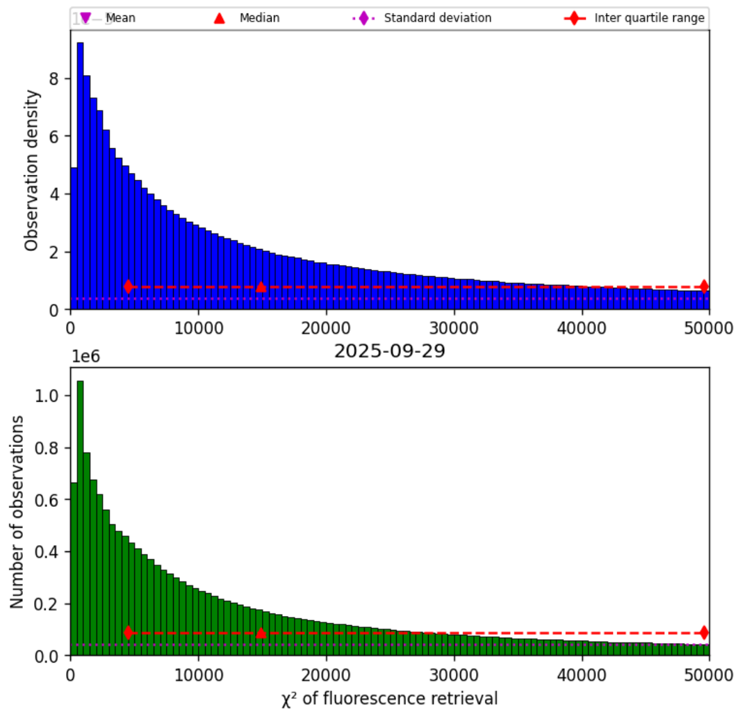
Figure 40: Histogram of “ \chi^2 of fluorescence retrieval” for 2025-09-29 to 2025-09-29
