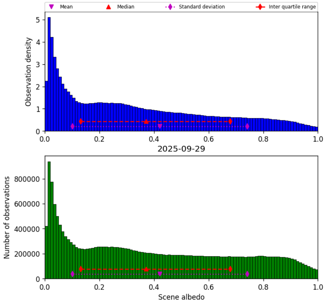
Figure 32: Histogram of “Scene albedo” for 2025-09-29 to 2025-09-29
