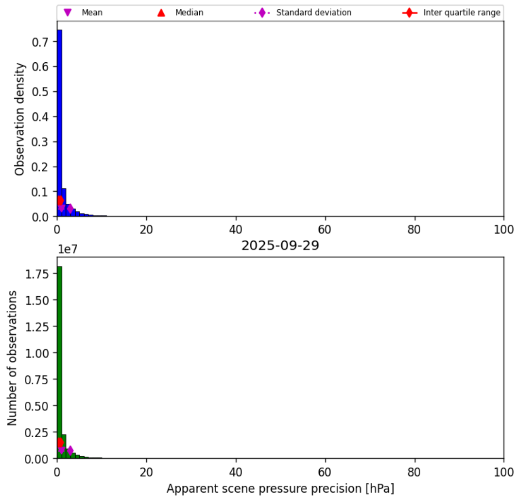
Figure 35: Histogram of “Apparent scene pressure precision” for 2025-09-29 to 2025-09-29
