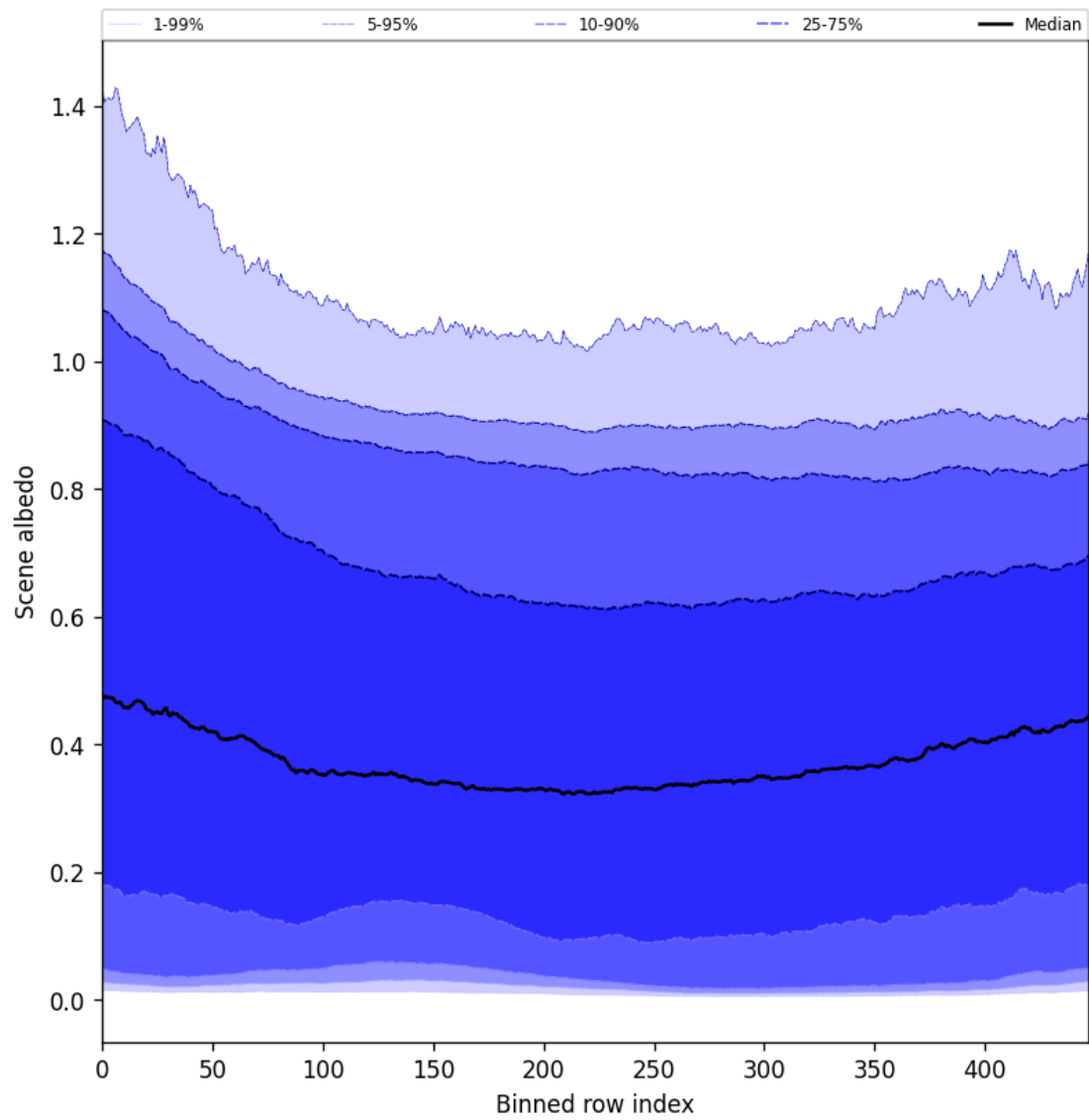
Figure 49: Along track statistics of “Scene albedo” for 2025-09-29 to 2025-09-29
