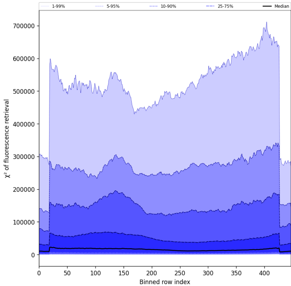
Figure 57: Along track statistics of “ \chi^2 of fluorescence retrieval” for 2025-09-29 to 2025-09-29
