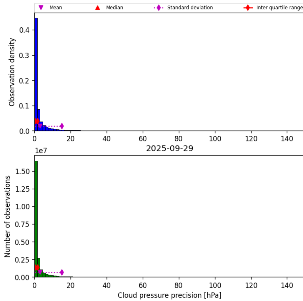
Figure 29: Histogram of “Cloud pressure precision” for 2025-09-29 to 2025-09-29
