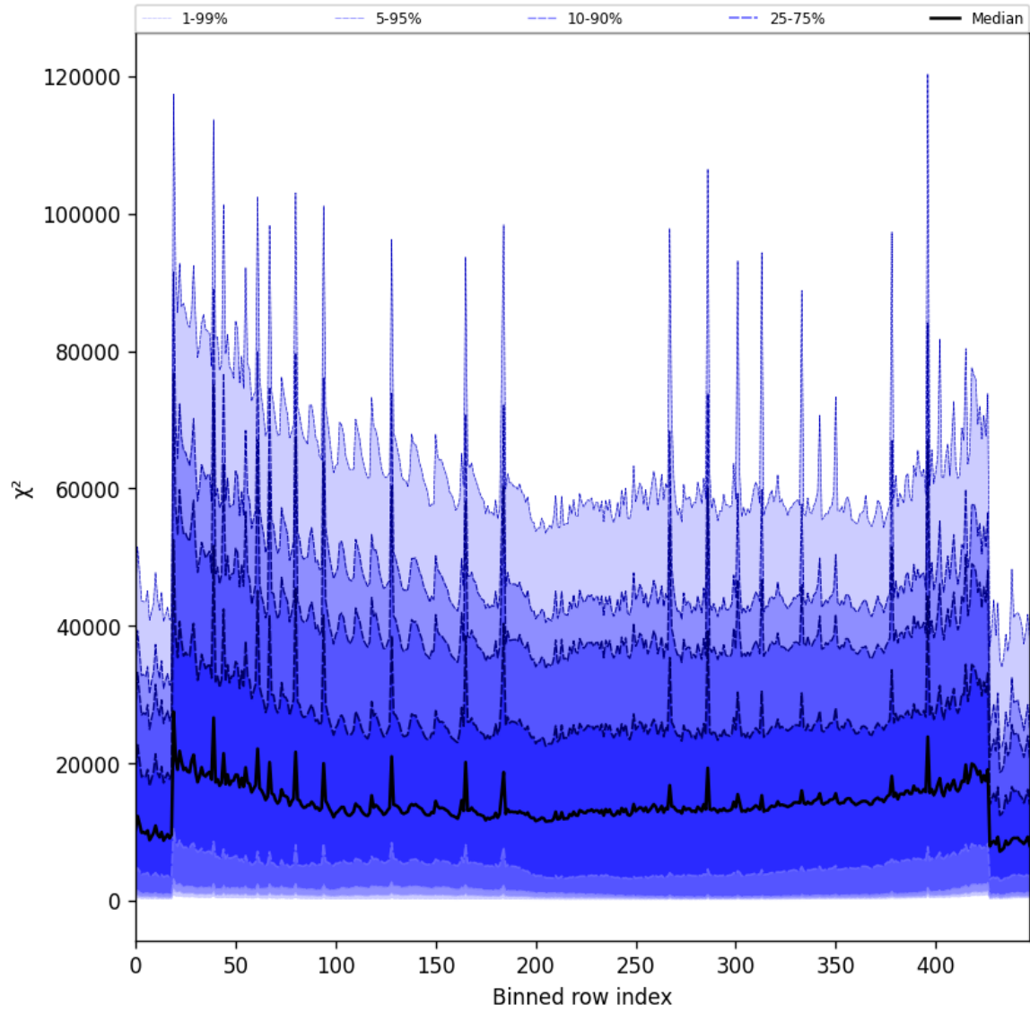
Figure 53: Along track statistics of “ \chi^2 ” for 2025-09-29 to 2025-09-29
