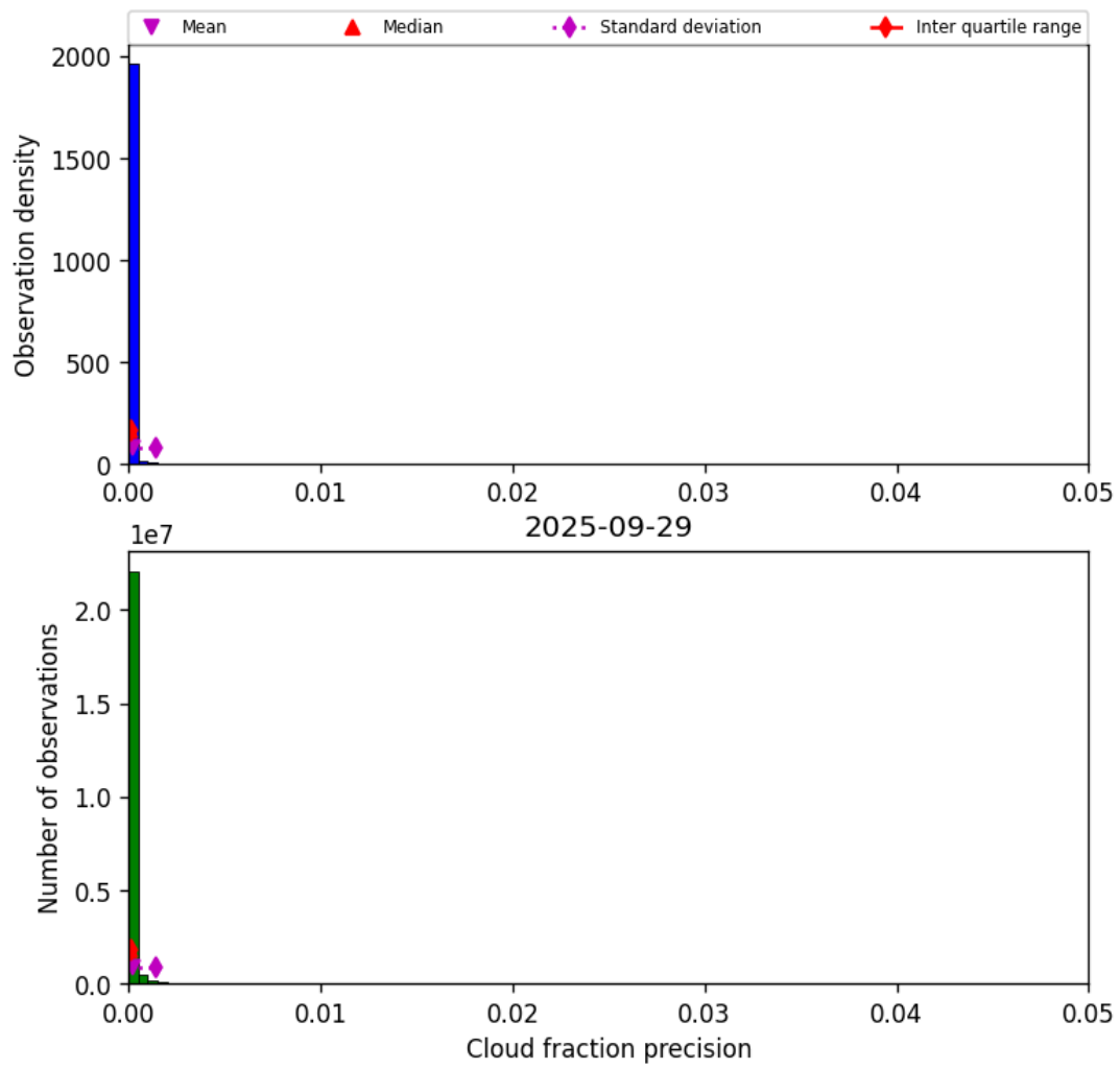
Figure 31: Histogram of “Cloud fraction precision” for 2025-09-29 to 2025-09-29
