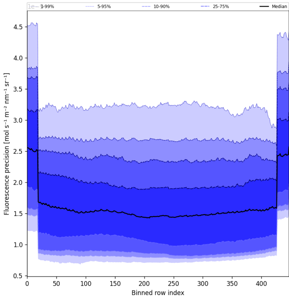
Figure 56: Along track statistics of “Fluorescence precision” for 2025-09-29 to 2025-09-29
