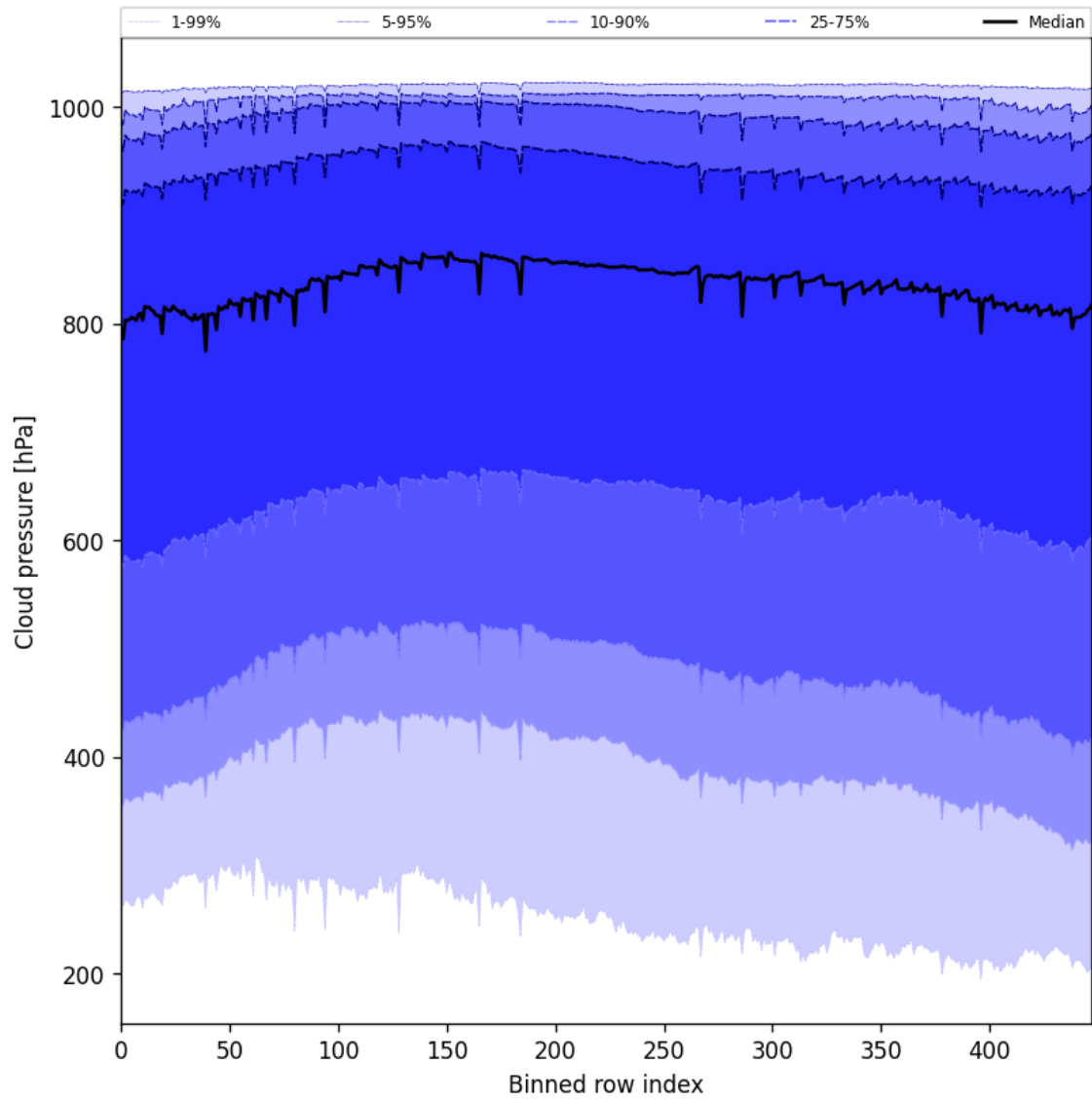
Figure 45: Along track statistics of “Cloud pressure” for 2025-09-29 to 2025-09-29
