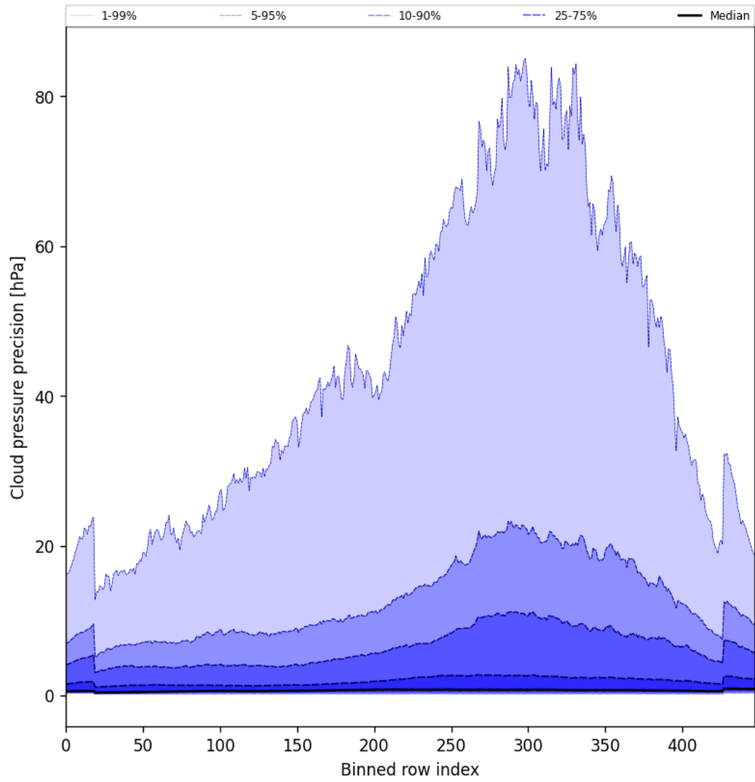
Figure 46: Along track statistics of “Cloud pressure precision” for 2025-09-29 to 2025-09-29
