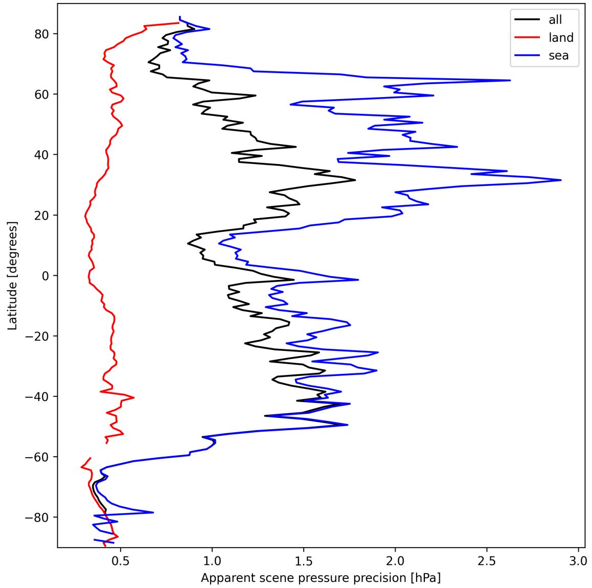
Figure 18: Zonal average of “Apparent scene pressure precision” for 2025-09-29 to 2025-09-29.
