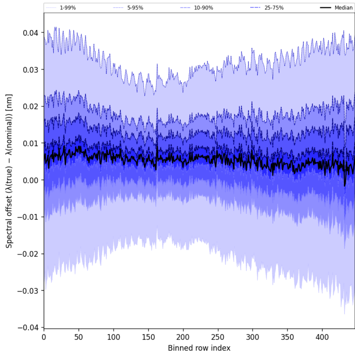
Figure 60: Along track statistics of “Spectral offset ( \lambda_{\text{true}} - \lambda_{\text{nominal}} )” for 2025-09-29 to 2025-09-29
