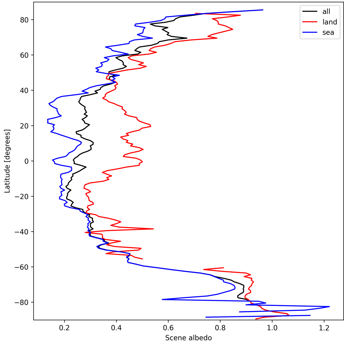
Figure 15: Zonal average of “Scene albedo” for 2025-09-29 to 2025-09-29.
