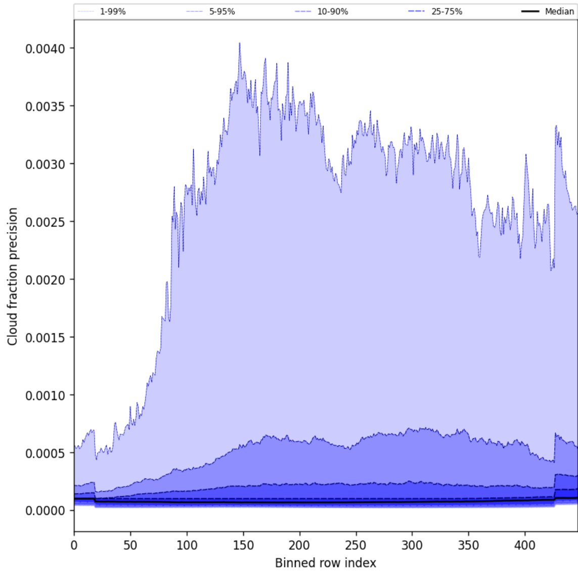
Figure 48: Along track statistics of “Cloud fraction precision” for 2025-09-29 to 2025-09-29
