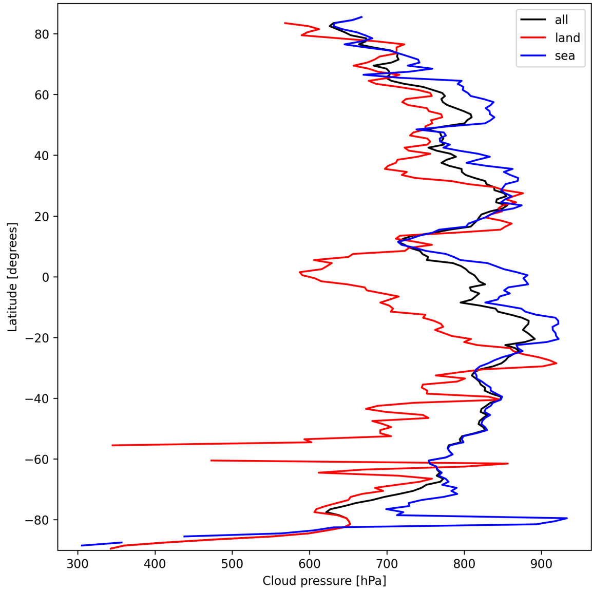
Figure 11: Zonal average of “Cloud pressure” for 2025-09-29 to 2025-09-29.
