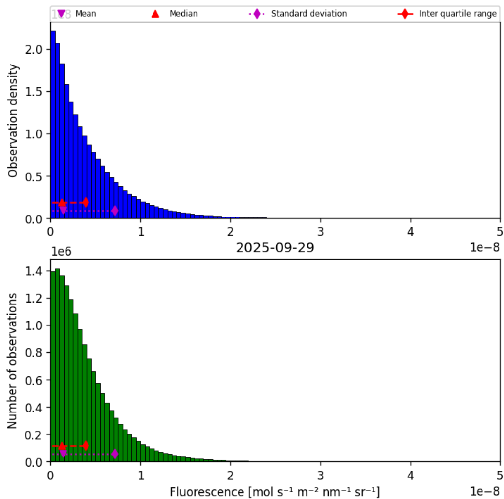
Figure 38: Histogram of “Fluorescence” for 2025-09-29 to 2025-09-29
