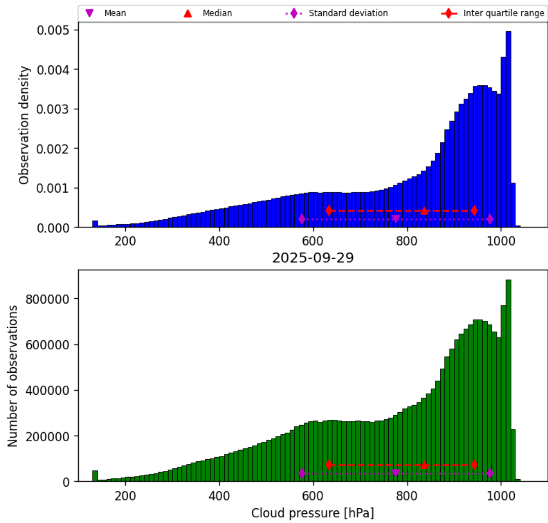
Figure 28: Histogram of “Cloud pressure” for 2025-09-29 to 2025-09-29
