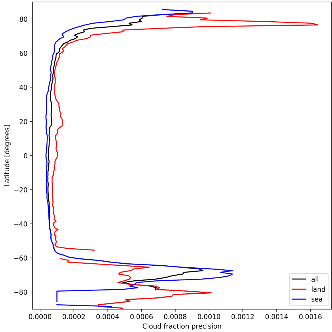
Figure 14: Zonal average of “Cloud fraction precision” for 2025-09-29 to 2025-09-29.
