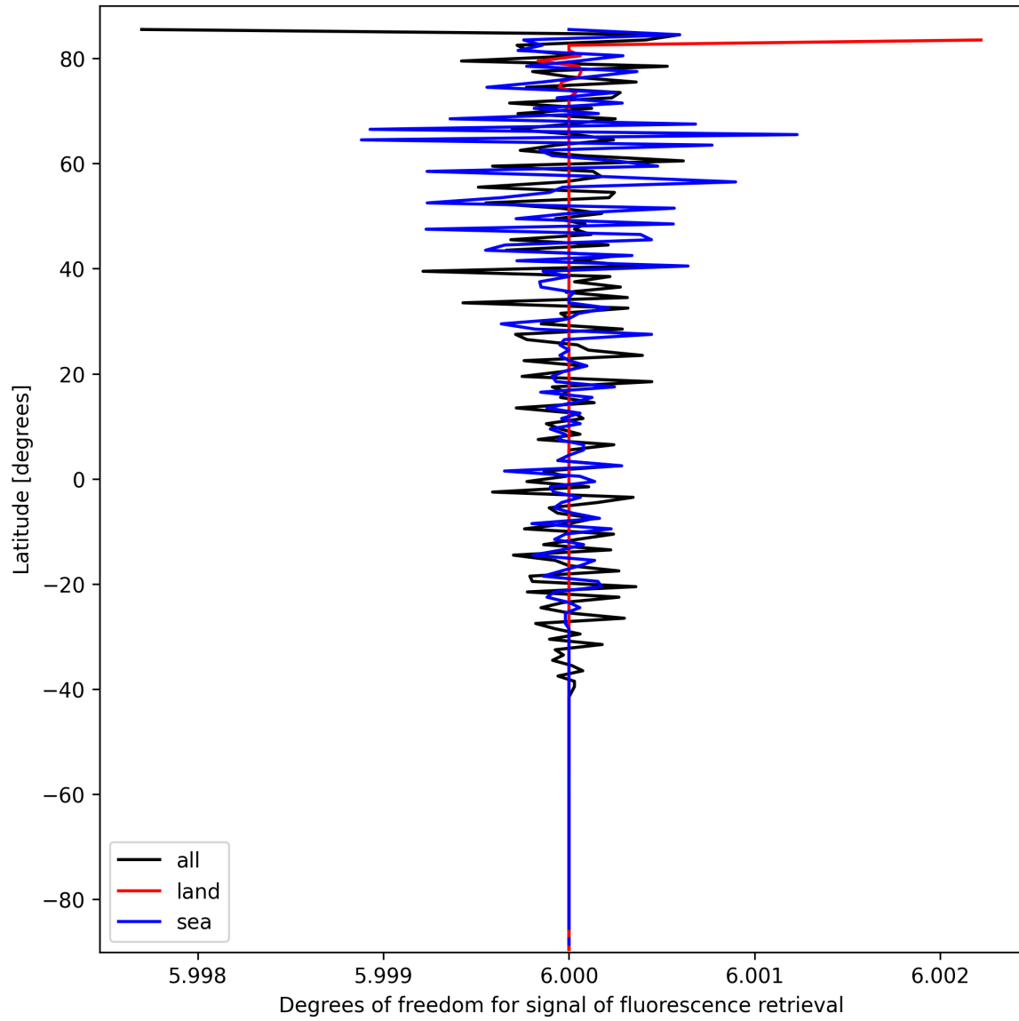
Figure 24: Zonal average of “Degrees of freedom for signal of fluorescence retrieval” for 2025-09-29 to 2025-09-29.
