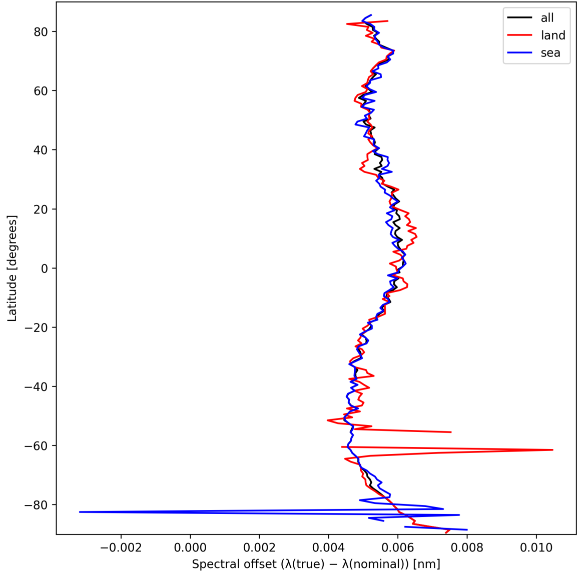
Figure 26: Zonal average of “Spectral offset ( \lambda_{\text{true}} - \lambda_{\text{nominal}} )” for 2025-09-29 to 2025-09-29.
