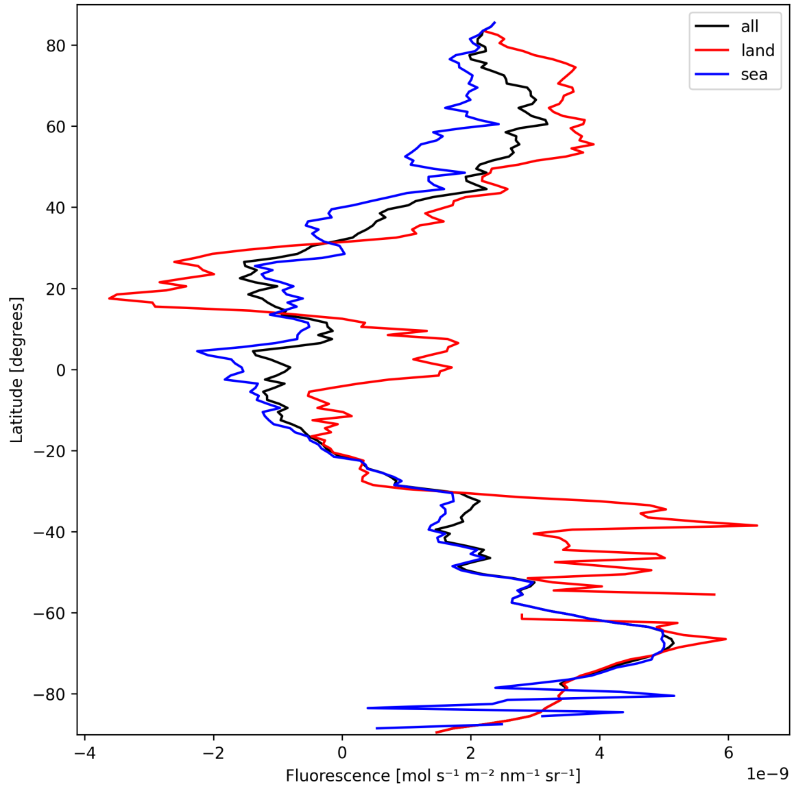
Figure 21: Zonal average of “Fluorescence” for 2025-09-29 to 2025-09-29.
