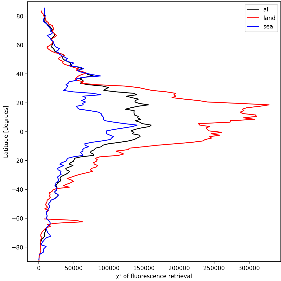
Figure 23: Zonal average of “ \chi^2 of fluorescence retrieval” for 2025-09-29 to 2025-09-29.
