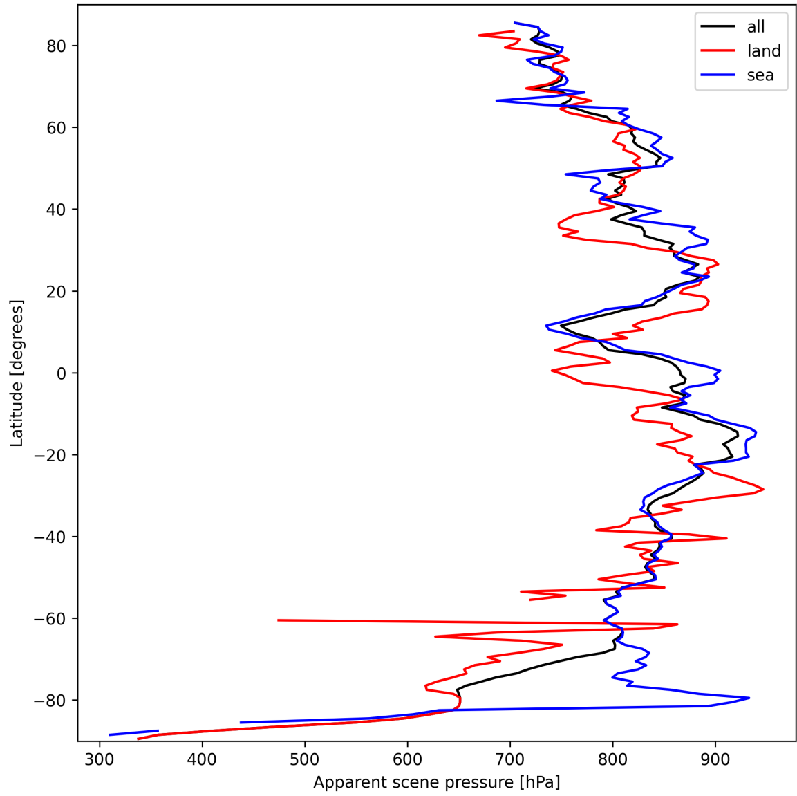
Figure 17: Zonal average of “Apparent scene pressure” for 2025-09-29 to 2025-09-29.
