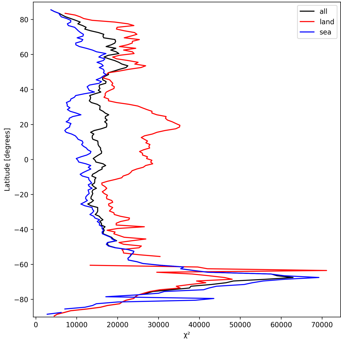
Figure 19: Zonal average of “ \chi^2 ” for 2025-09-29 to 2025-09-29.
