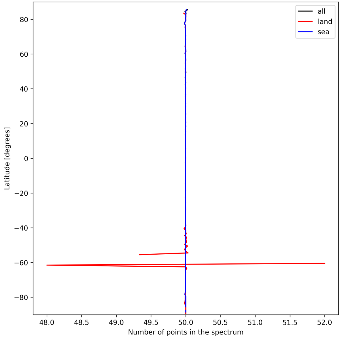
Figure 25: Zonal average of “Number of points in the spectrum” for 2025-09-29 to 2025-09-29.
