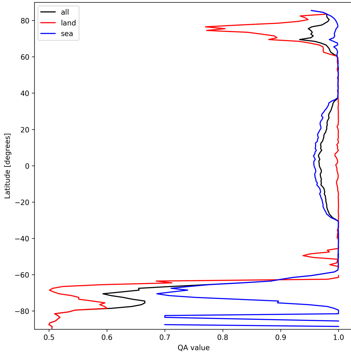
Figure 10: Zonal average of “QA value” for 2025-09-29 to 2025-09-29.
