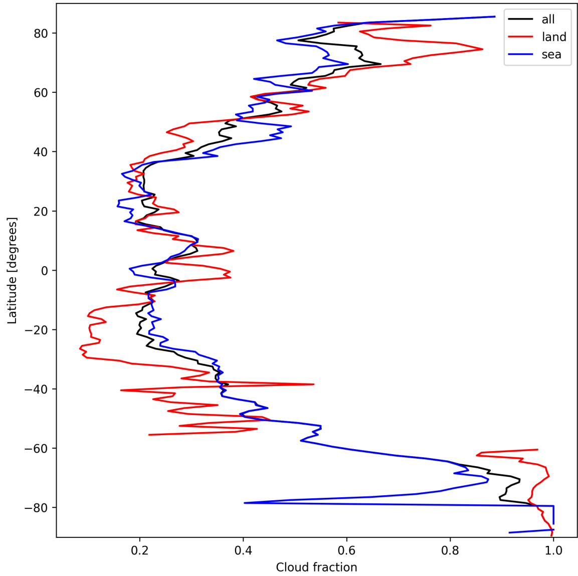
Figure 13: Zonal average of “Cloud fraction” for 2025-09-29 to 2025-09-29.
