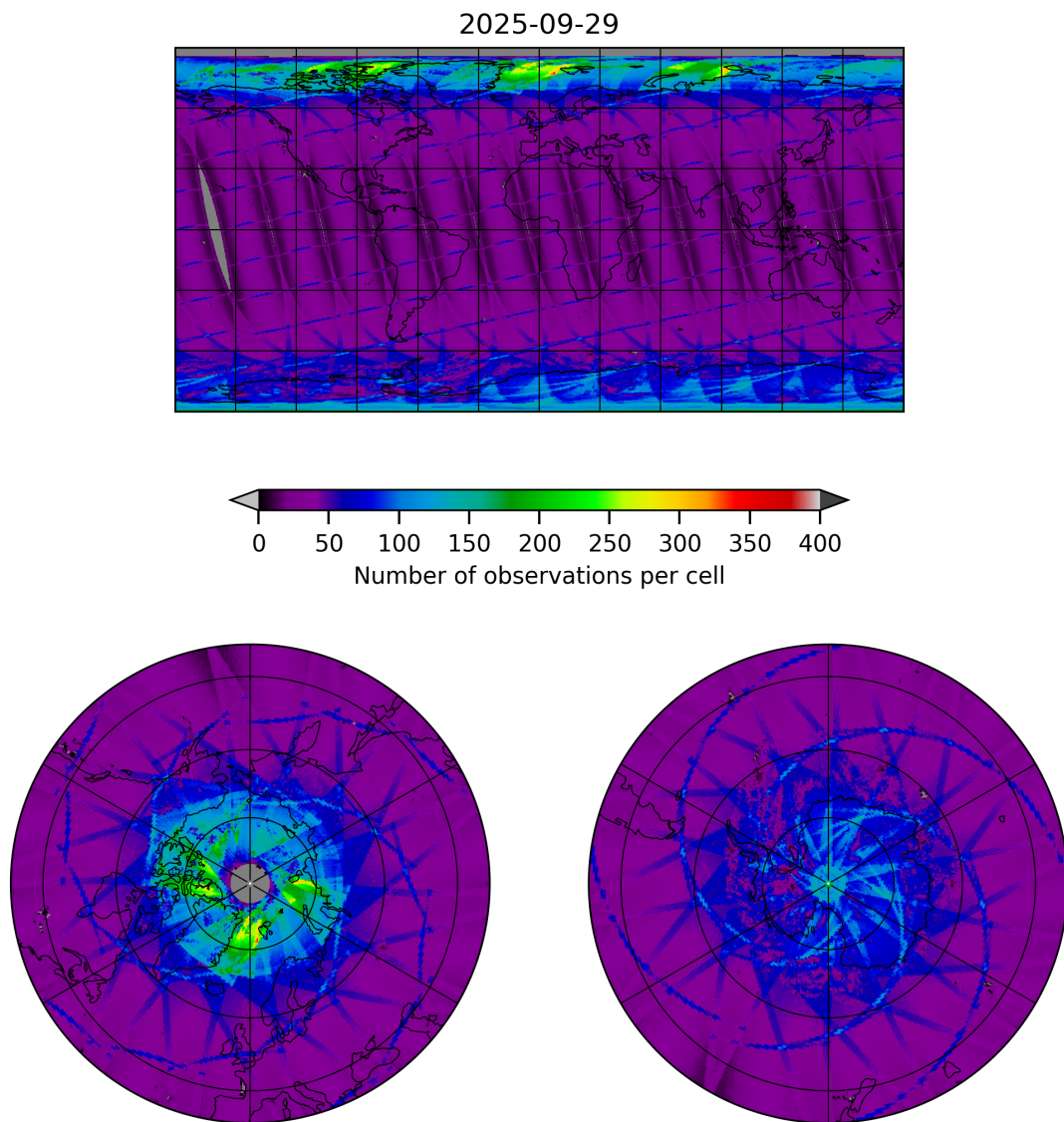
Figure 9: Map of the number of observations for 2025-09-29 to 2025-09-29
