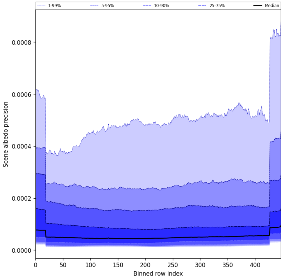
Figure 50: Along track statistics of “Scene albedo precision” for 2025-09-29 to 2025-09-29
