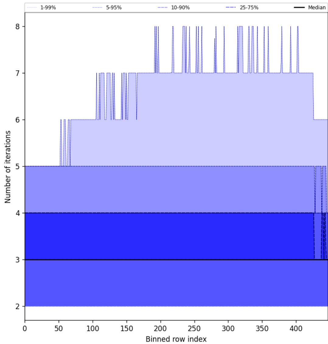
Figure 54: Along track statistics of “Number of iterations” for 2025-09-29 to 2025-09-29
