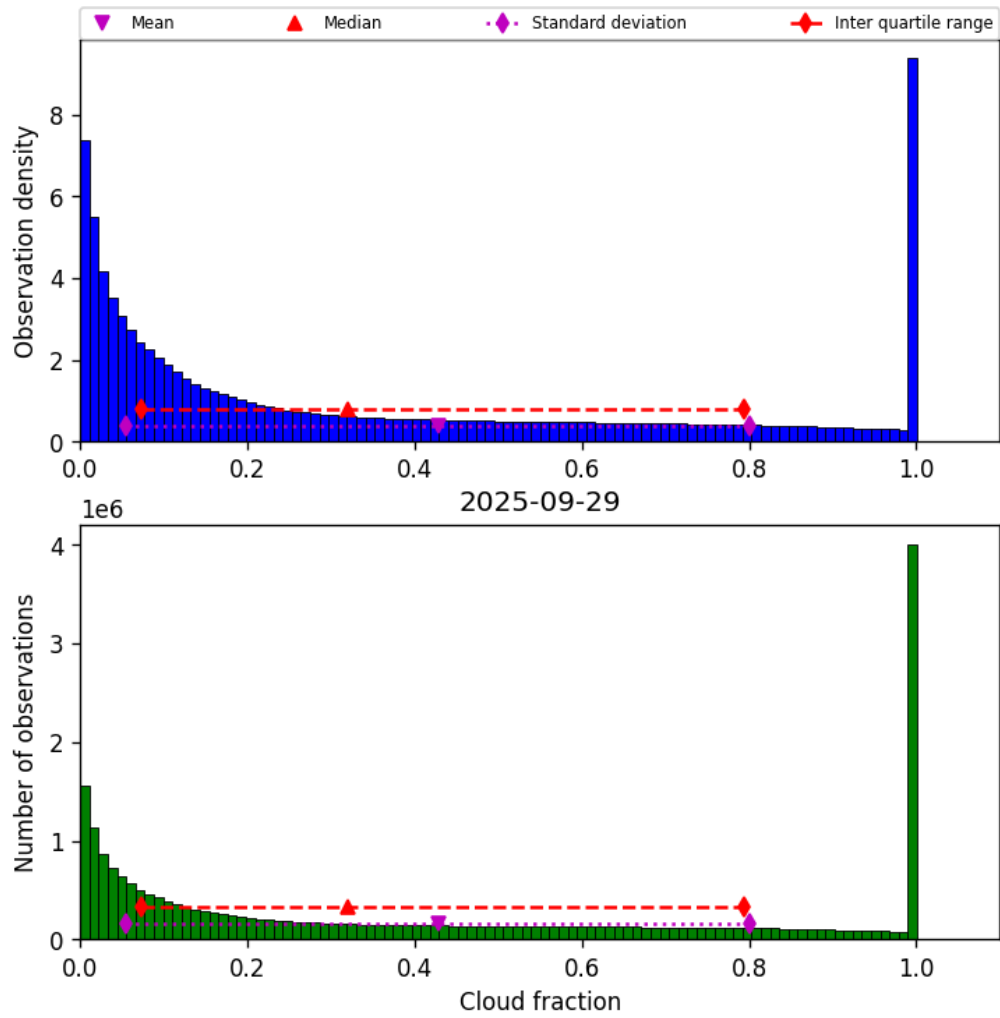
Figure 30: Histogram of “Cloud fraction” for 2025-09-29 to 2025-09-29
