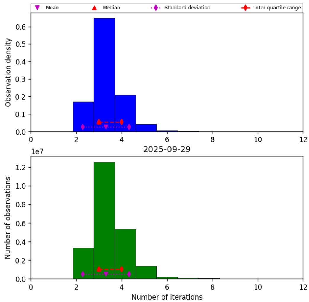
Figure 37: Histogram of “Number of iterations” for 2025-09-29 to 2025-09-29
