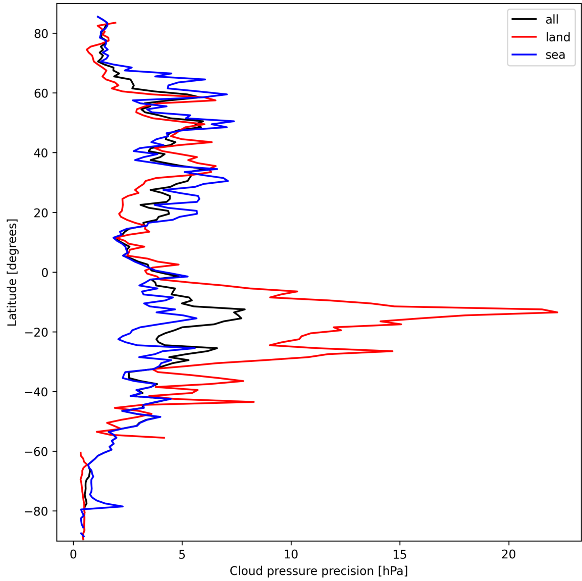
Figure 12: Zonal average of "Cloud pressure precision" for 2025-09-29 to 2025-09-29.
