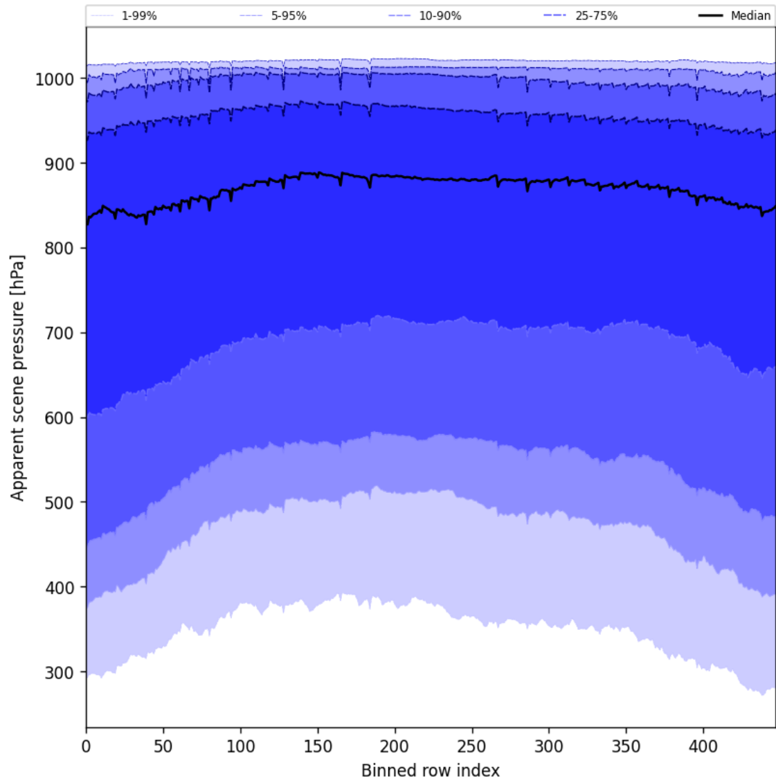
Figure 51: Along track statistics of “Apparent scene pressure” for 2025-09-29 to 2025-09-29
