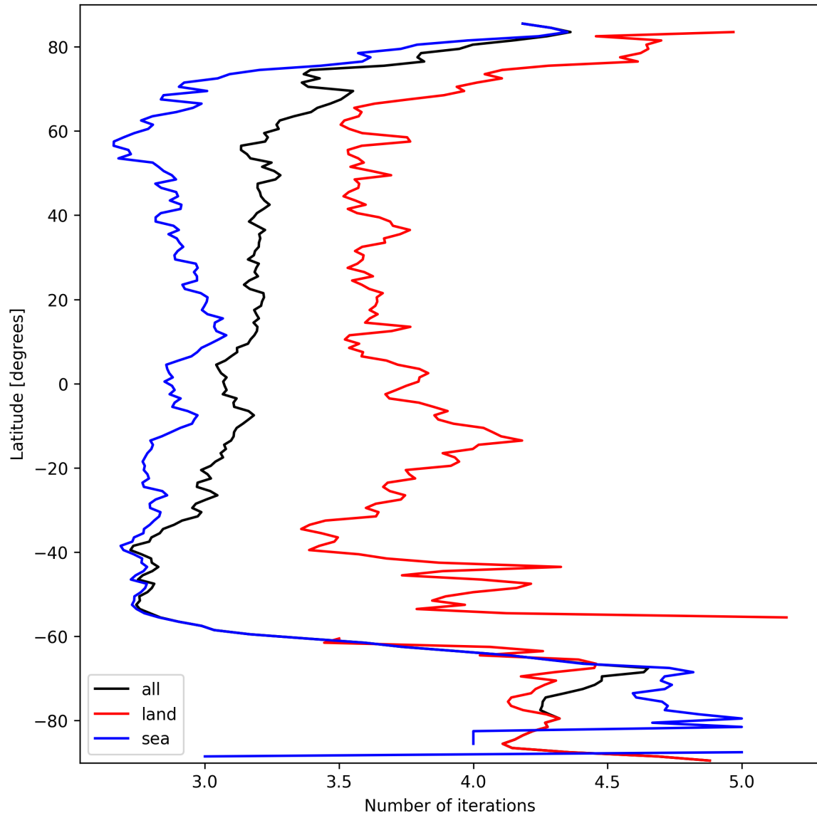
Figure 20: Zonal average of “Number of iterations” for 2025-09-29 to 2025-09-29.
