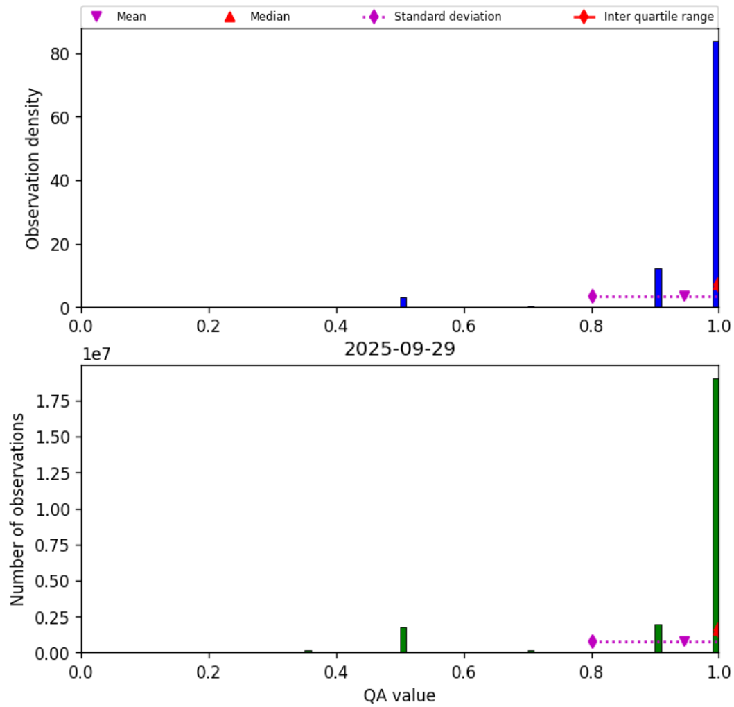
Figure 27: Histogram of “QA value” for 2025-09-29 to 2025-09-29
