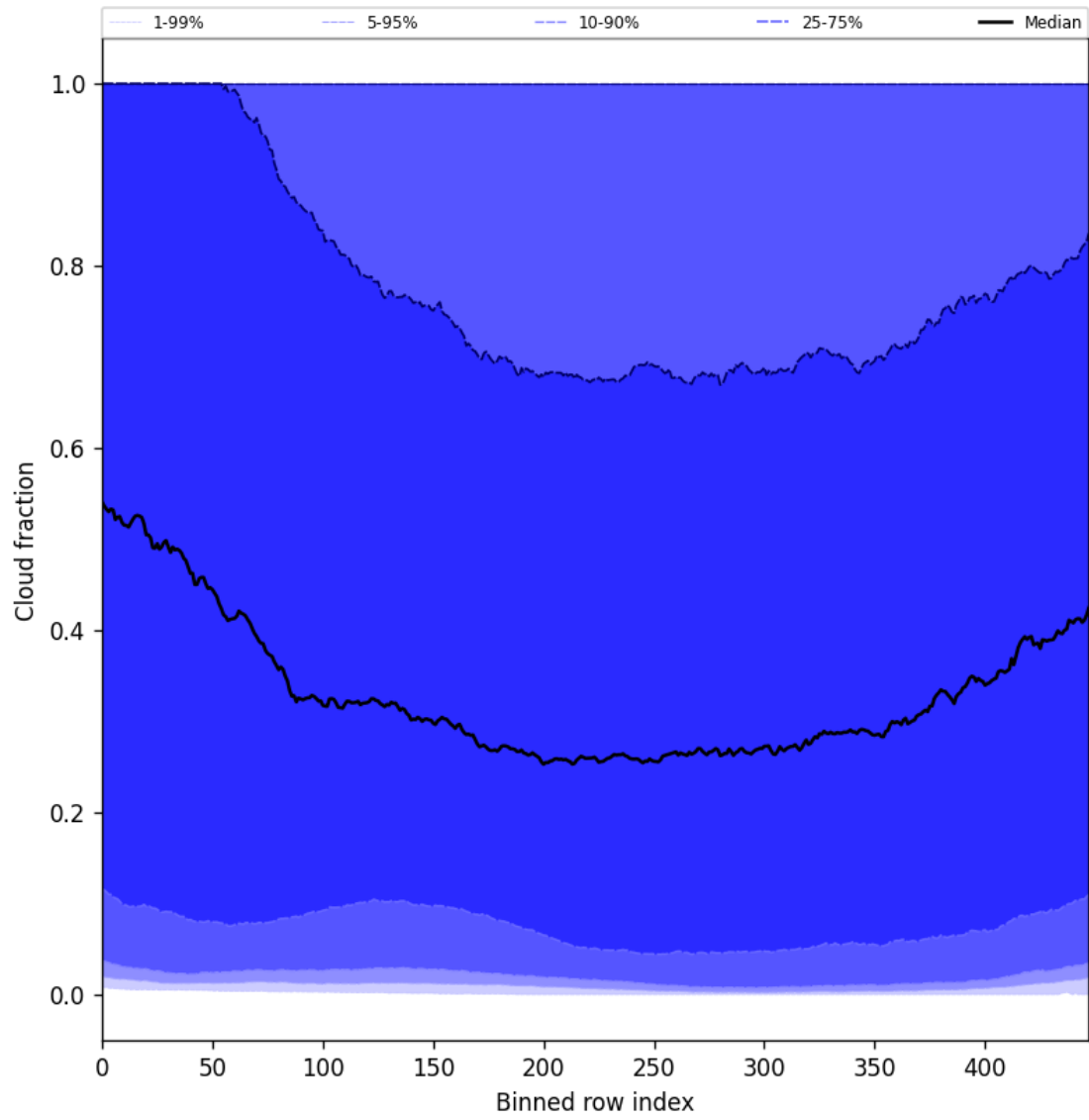
Figure 47: Along track statistics of “Cloud fraction” for 2025-09-29 to 2025-09-29
