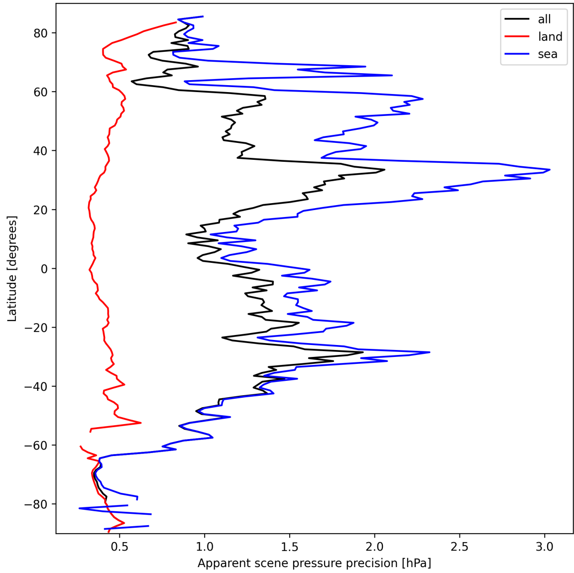
Figure 18: Zonal average of “Apparent scene pressure precision” for 2025-09-30 to 2025-10-01.
