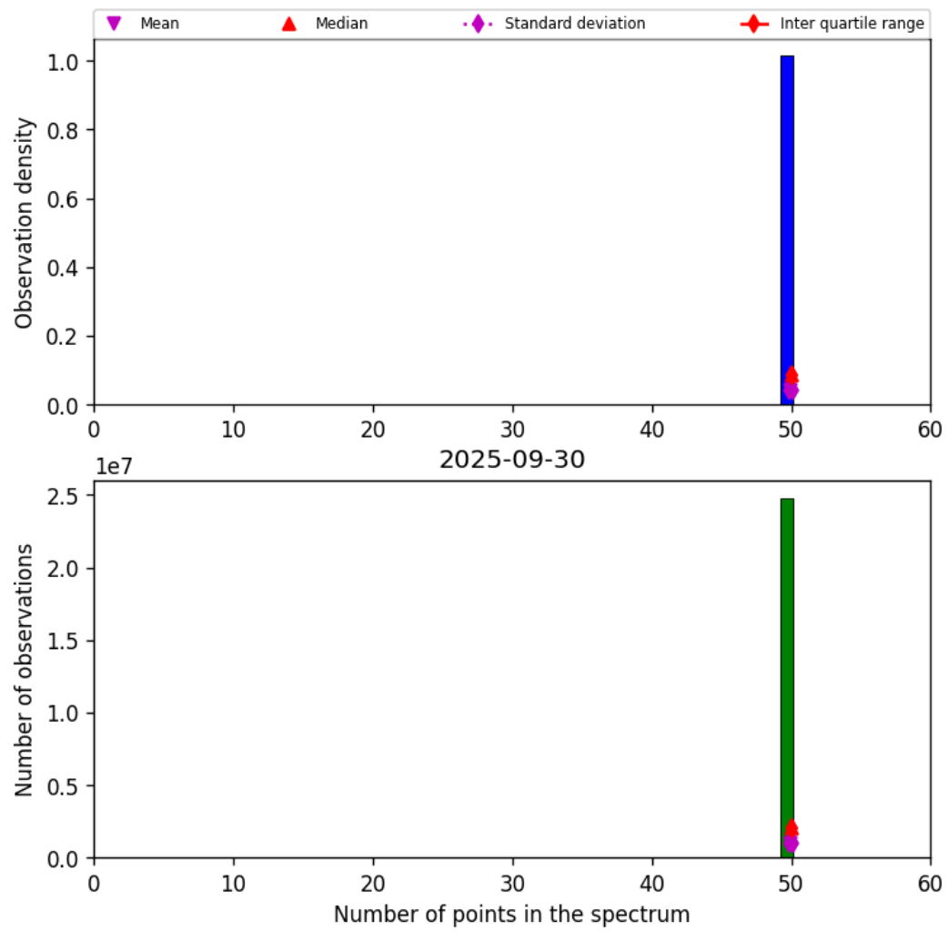
Figure 42: Histogram of “Number of points in the spectrum” for 2025-09-30 to 2025-10-01
