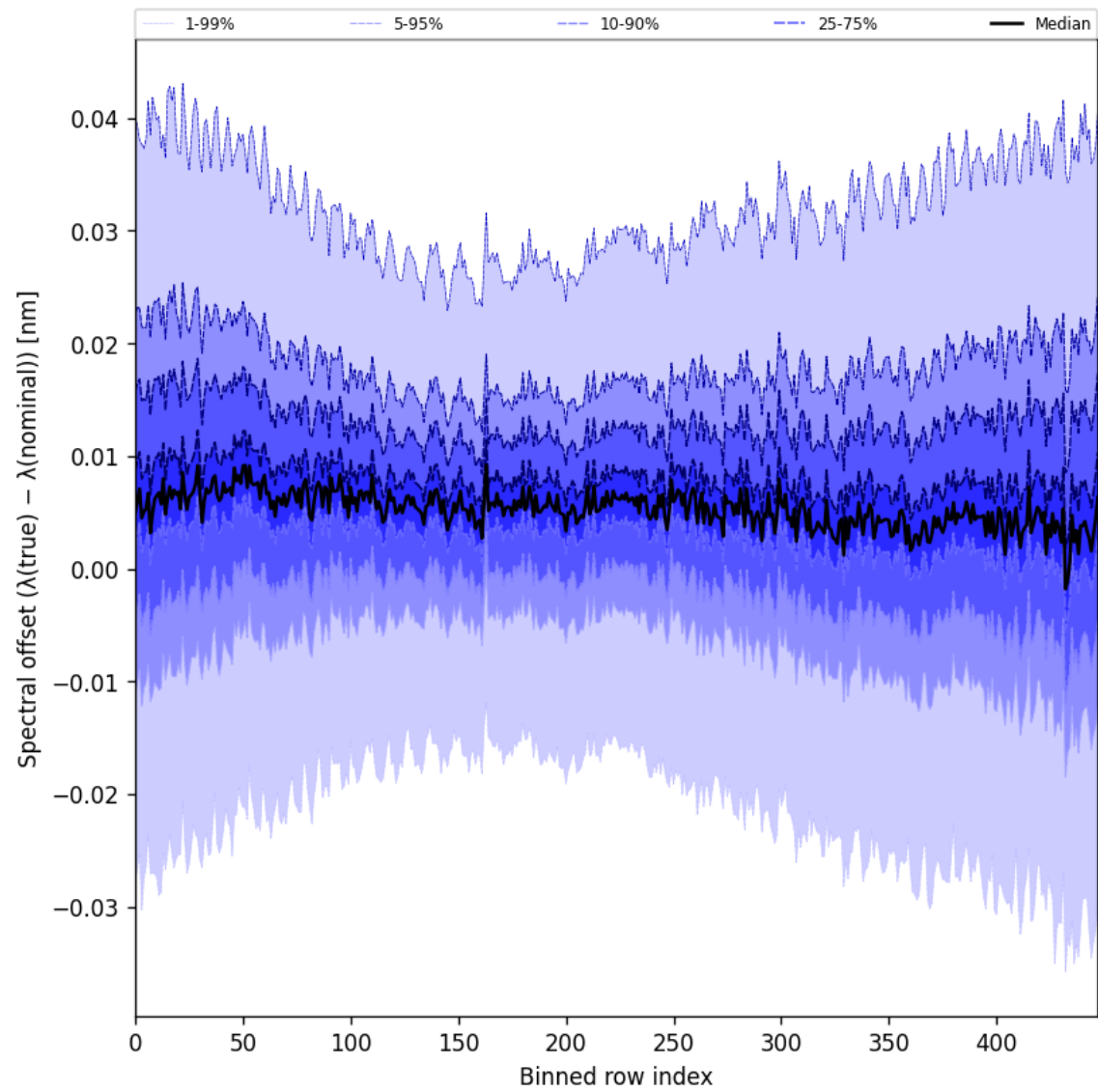
Figure 60: Along track statistics of “Spectral offset ( \lambda_{\text{true}} - \lambda_{\text{nominal}} )” for 2025-09-30 to 2025-10-01
