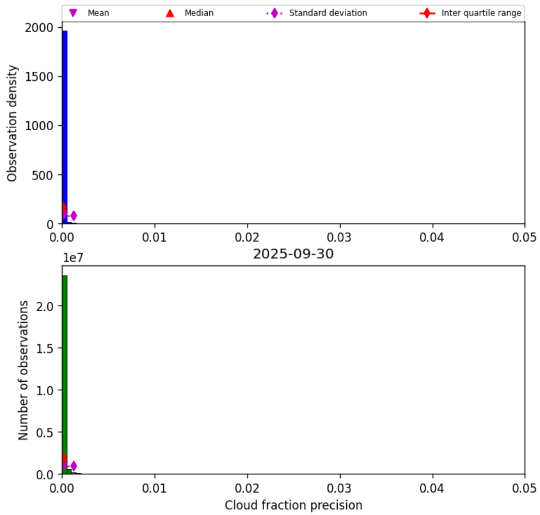
Figure 31: Histogram of “Cloud fraction precision” for 2025-09-30 to 2025-10-01
