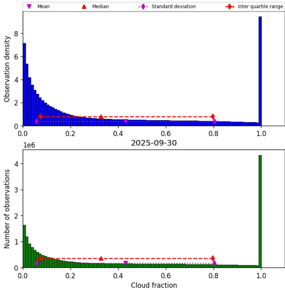
Figure 30: Histogram of “Cloud fraction” for 2025-09-30 to 2025-10-01
