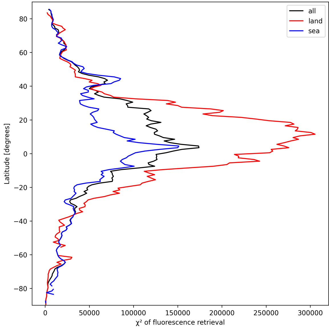
Figure 23: Zonal average of “ \chi^2 of fluorescence retrieval” for 2025-09-30 to 2025-10-01.
