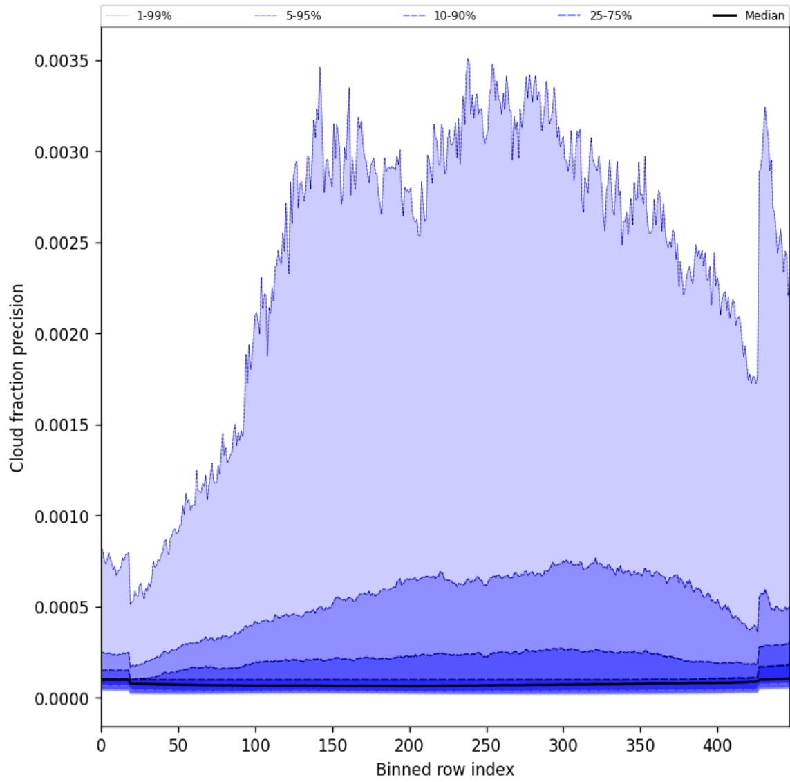
Figure 48: Along track statistics of “Cloud fraction precision” for 2025-09-30 to 2025-10-01
