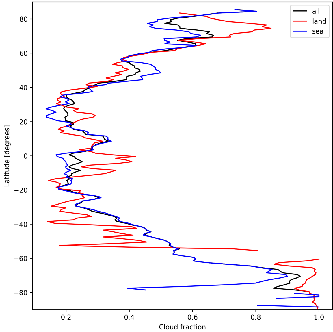
Figure 13: Zonal average of “Cloud fraction” for 2025-09-30 to 2025-10-01.
