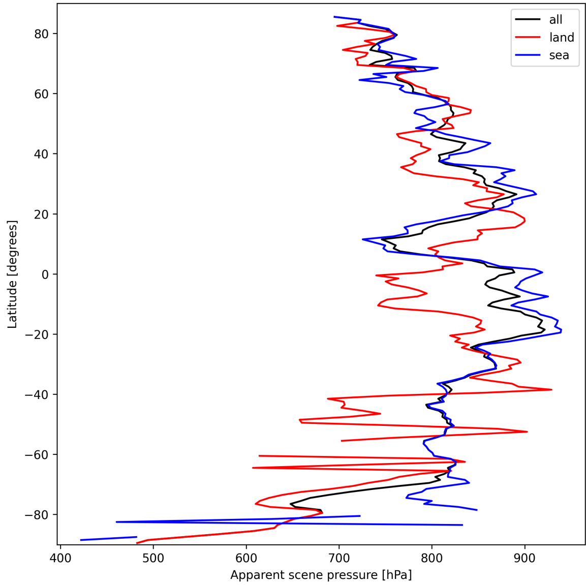
Figure 17: Zonal average of “Apparent scene pressure” for 2025-09-30 to 2025-10-01.
