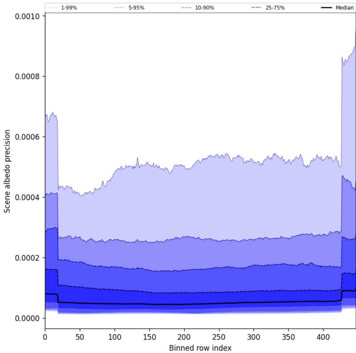
Figure 50: Along track statistics of “Scene albedo precision” for 2025-09-30 to 2025-10-01
