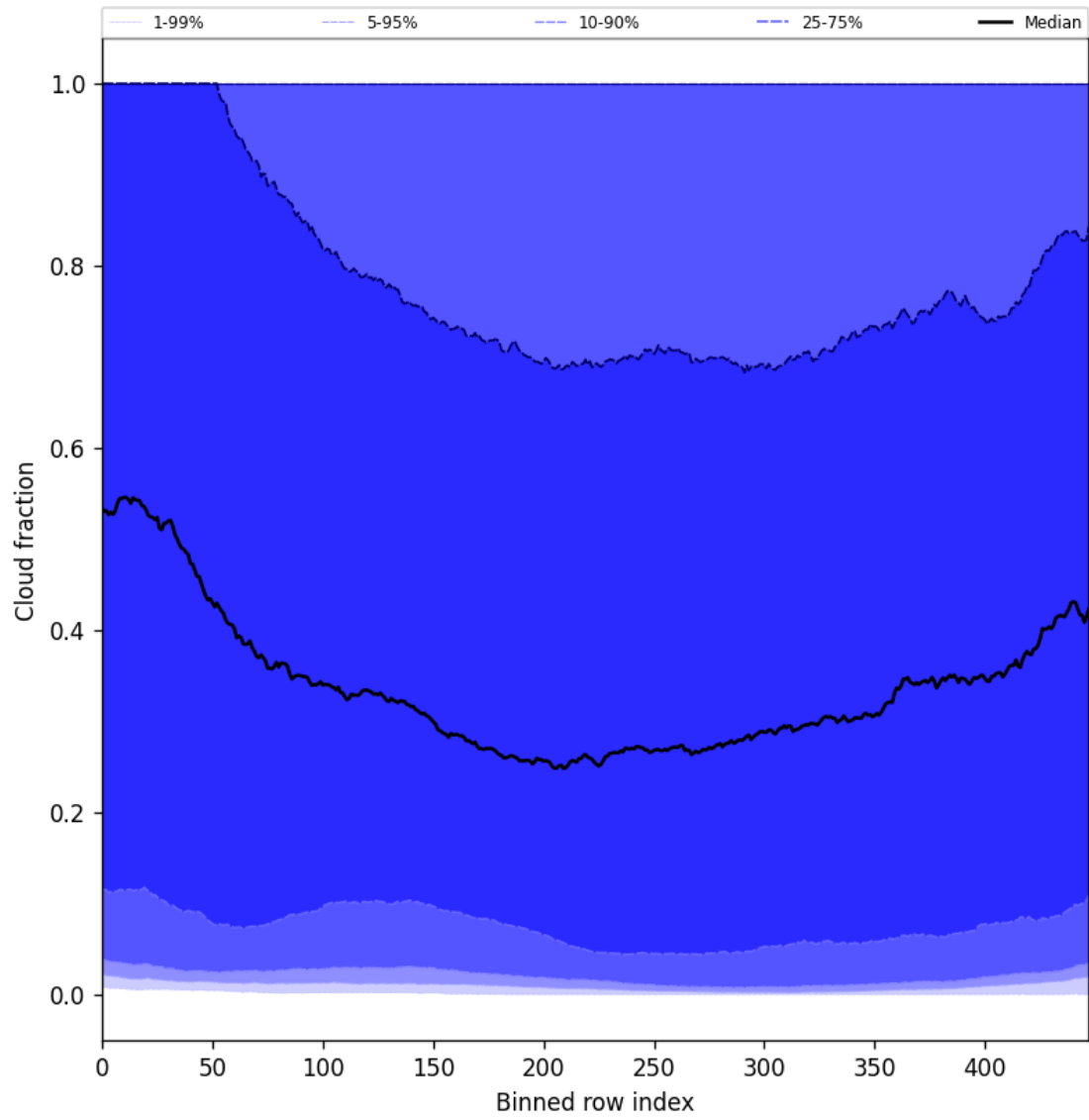
Figure 47: Along track statistics of “Cloud fraction” for 2025-09-30 to 2025-10-01
