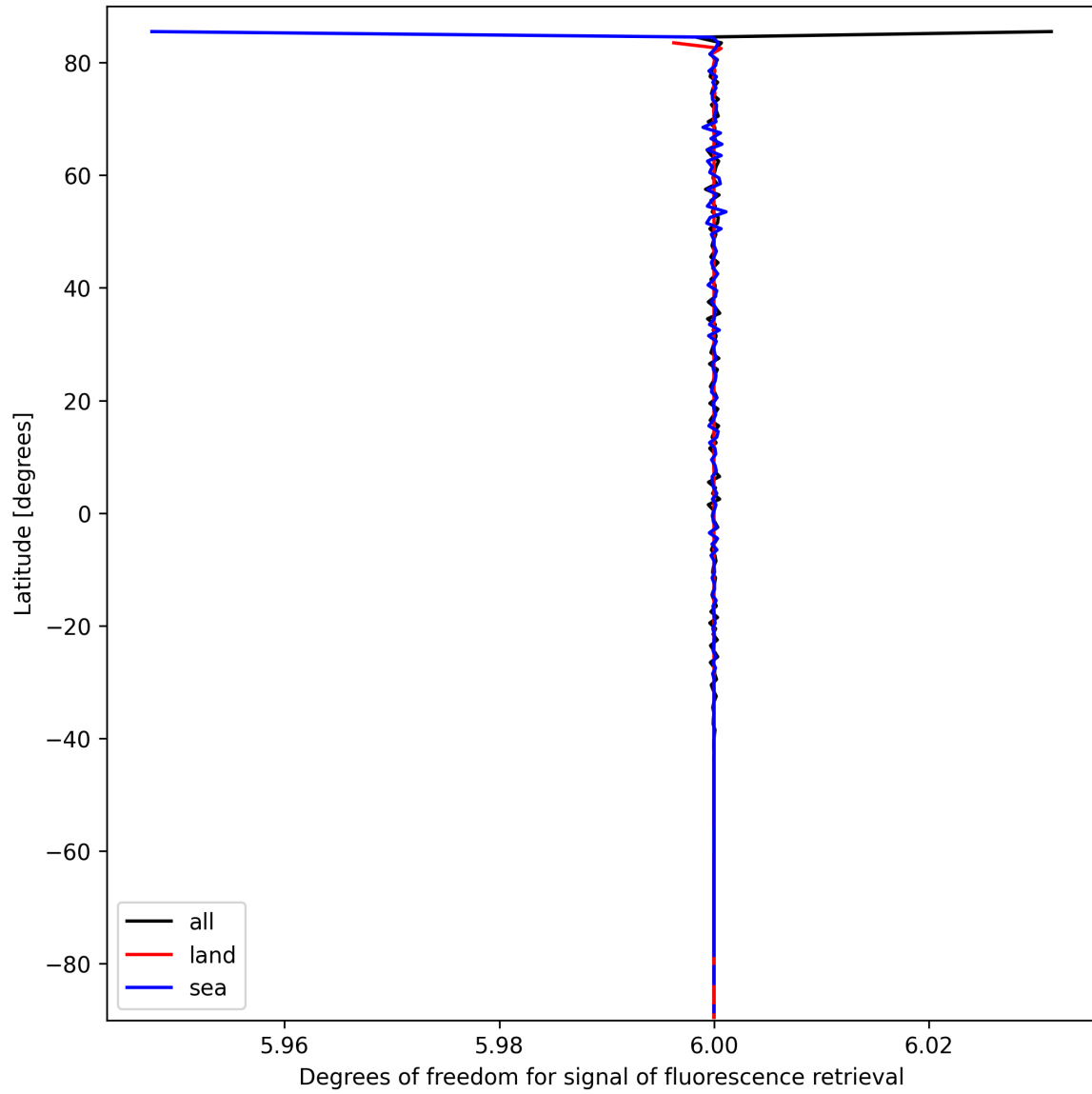
Figure 24: Zonal average of “Degrees of freedom for signal of fluorescence retrieval” for 2025-09-30 to 2025-10-01.
