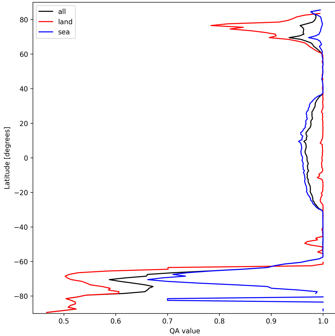
Figure 10: Zonal average of "QA value" for 2025-09-30 to 2025-10-01.
