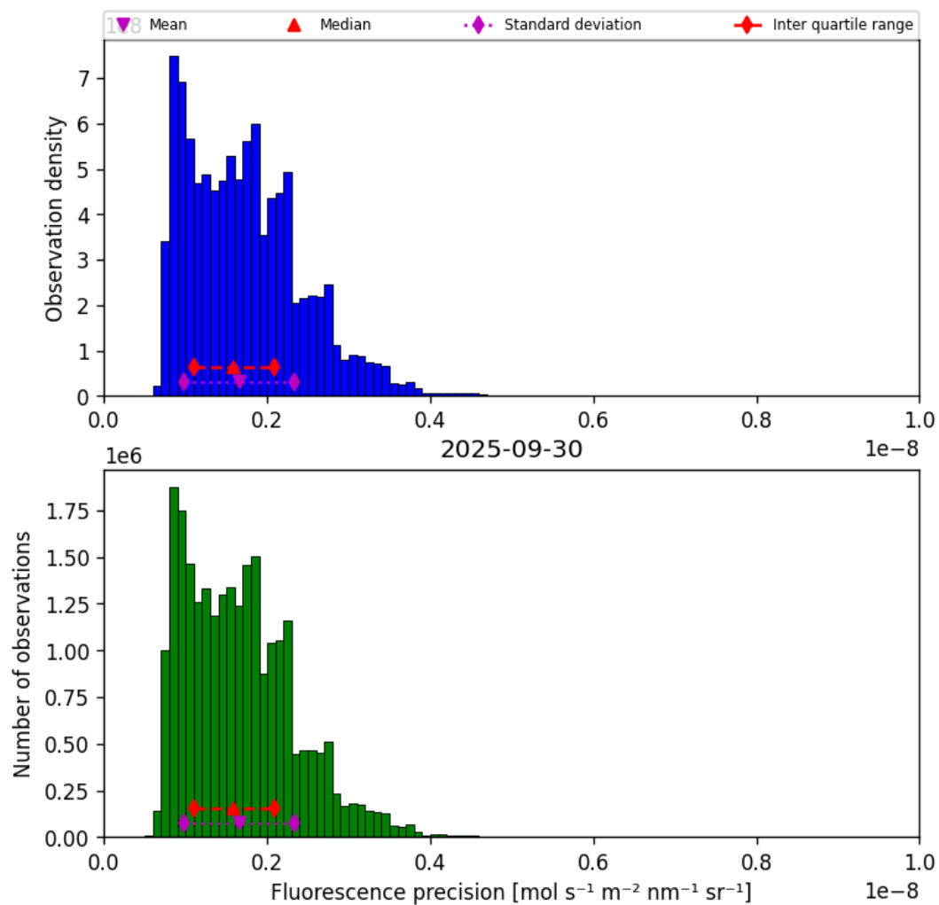
Figure 39: Histogram of “Fluorescence precision” for 2025-09-30 to 2025-10-01
