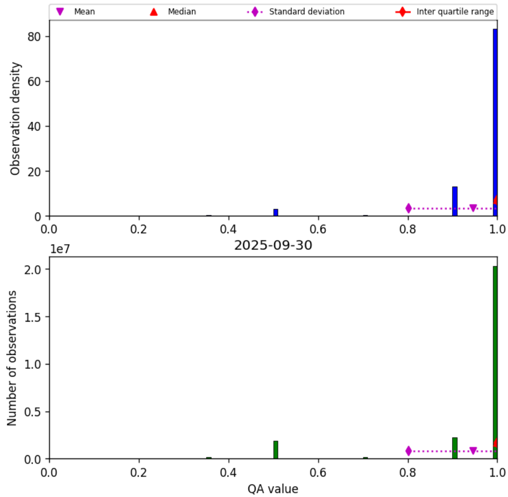
Figure 27: Histogram of “QA value” for 2025-09-30 to 2025-10-01
