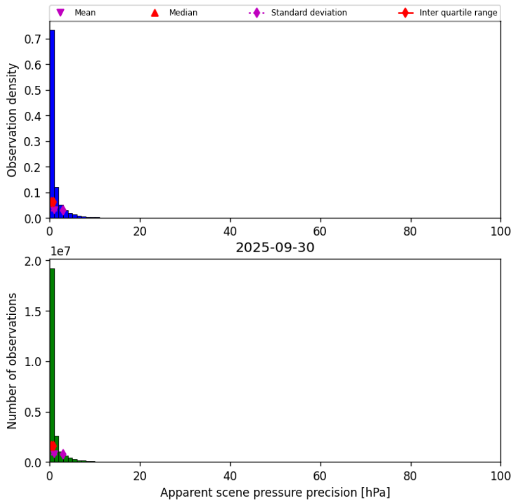
Figure 35: Histogram of “Apparent scene pressure precision” for 2025-09-30 to 2025-10-01
