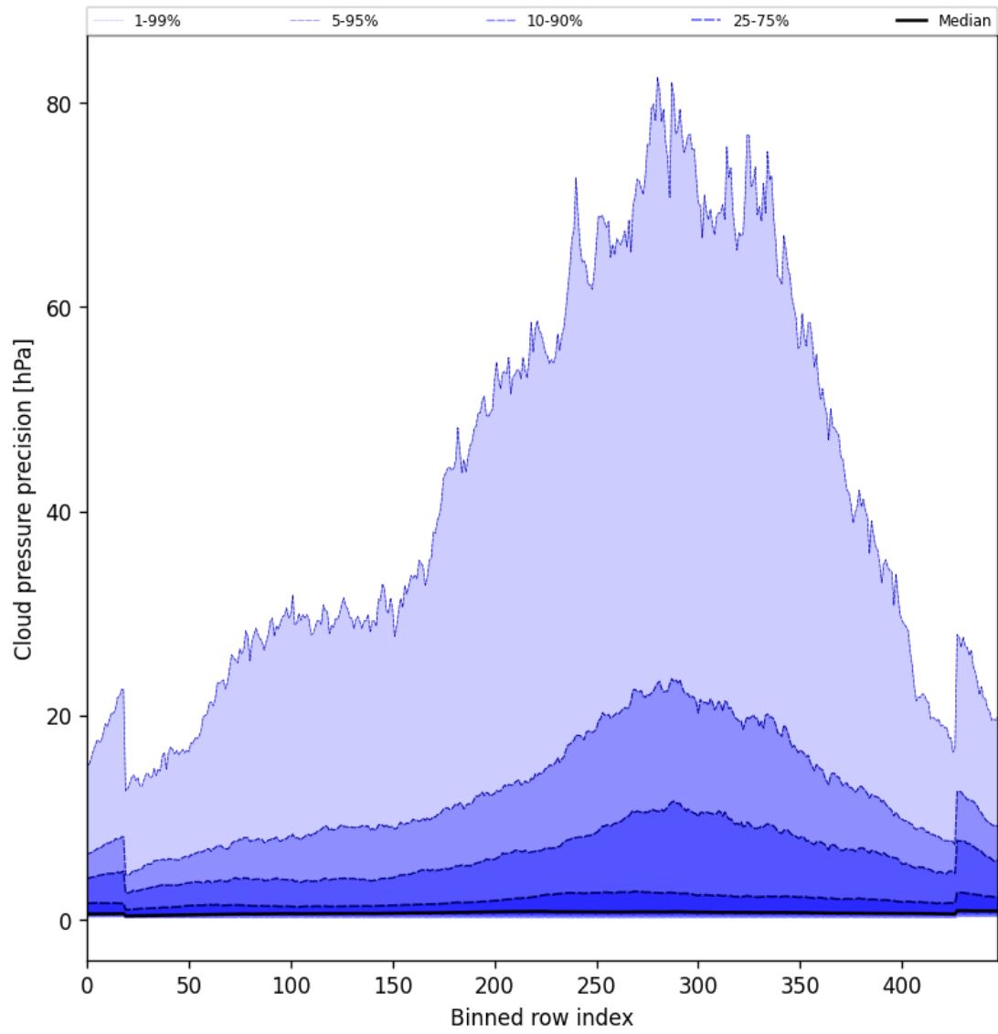
Figure 46: Along track statistics of “Cloud pressure precision” for 2025-09-30 to 2025-10-01
