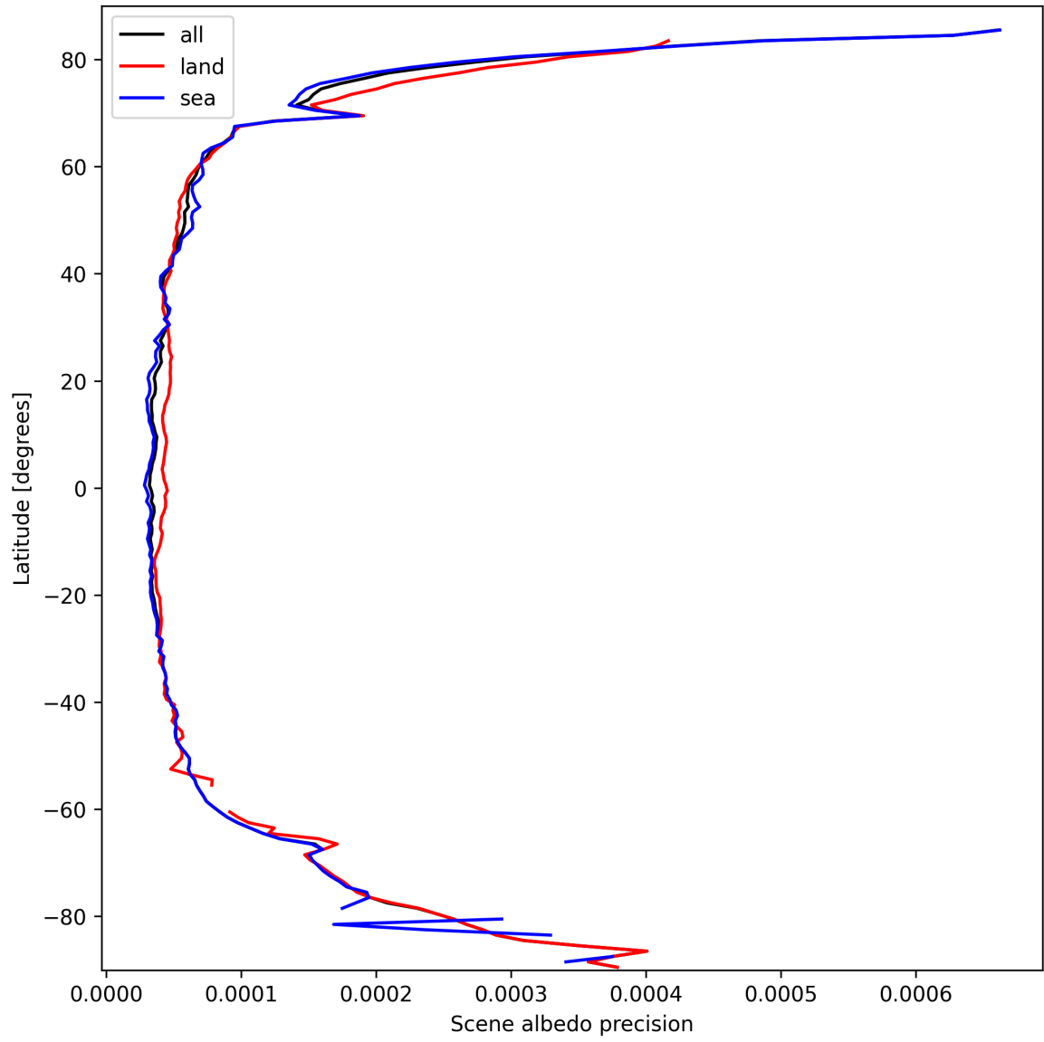
Figure 16: Zonal average of “Scene albedo precision” for 2025-09-30 to 2025-10-01.
