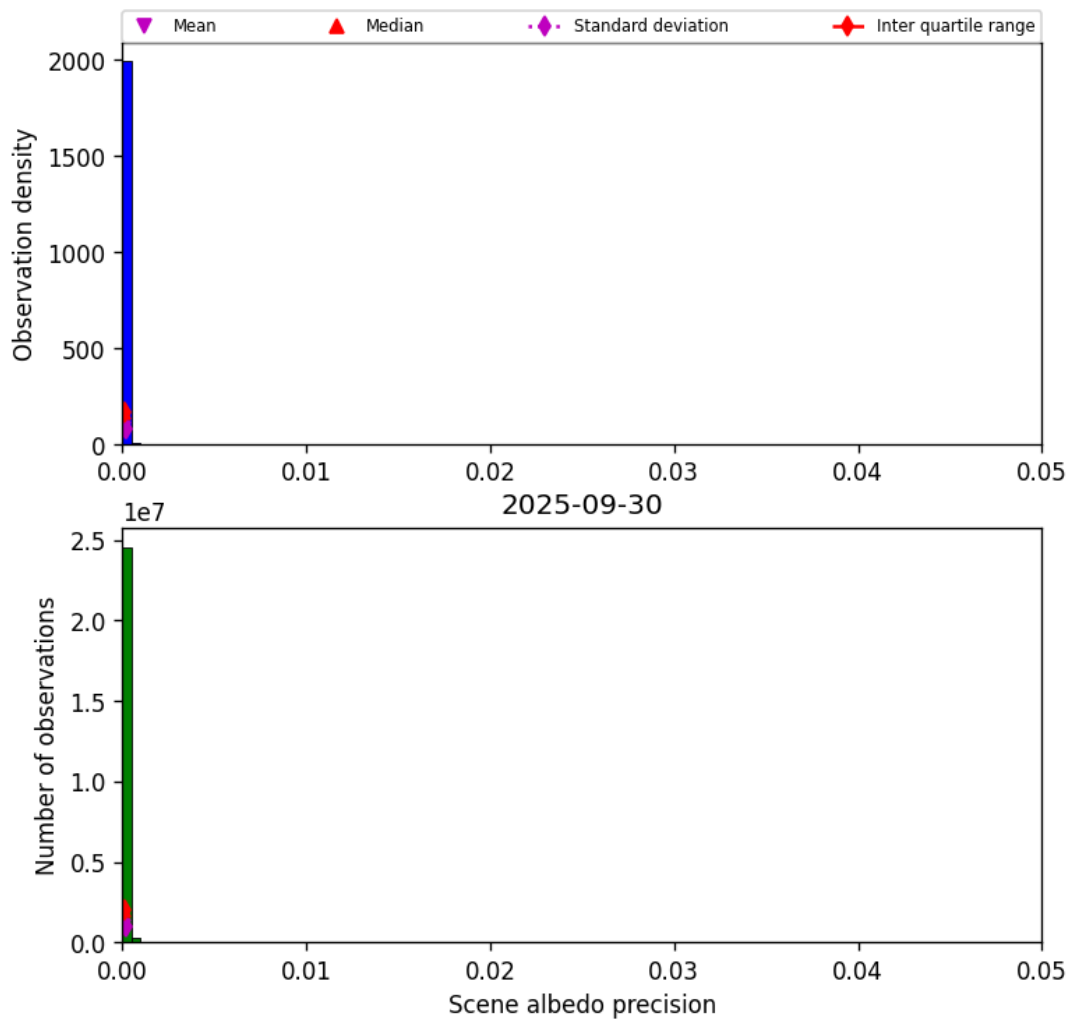
Figure 33: Histogram of “Scene albedo precision” for 2025-09-30 to 2025-10-01
