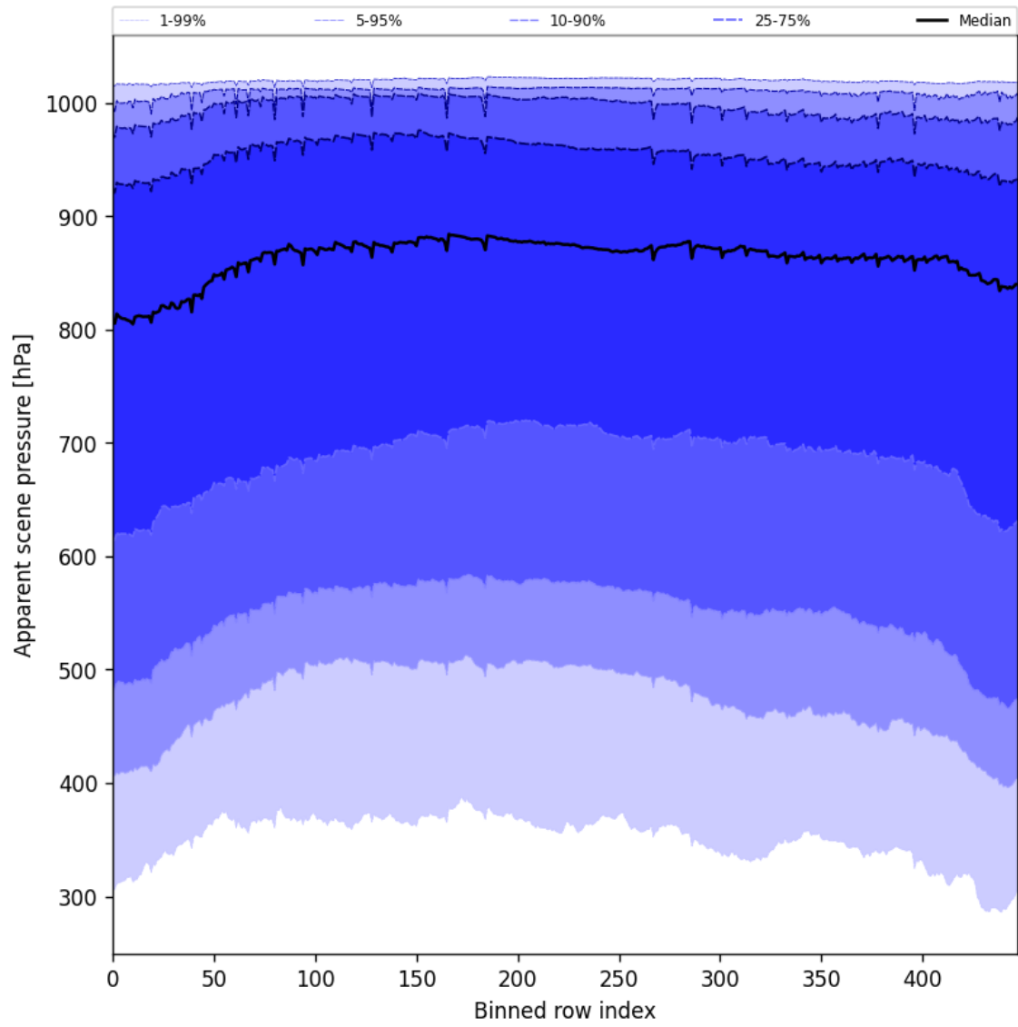
Figure 51: Along track statistics of “Apparent scene pressure” for 2025-09-30 to 2025-10-01
