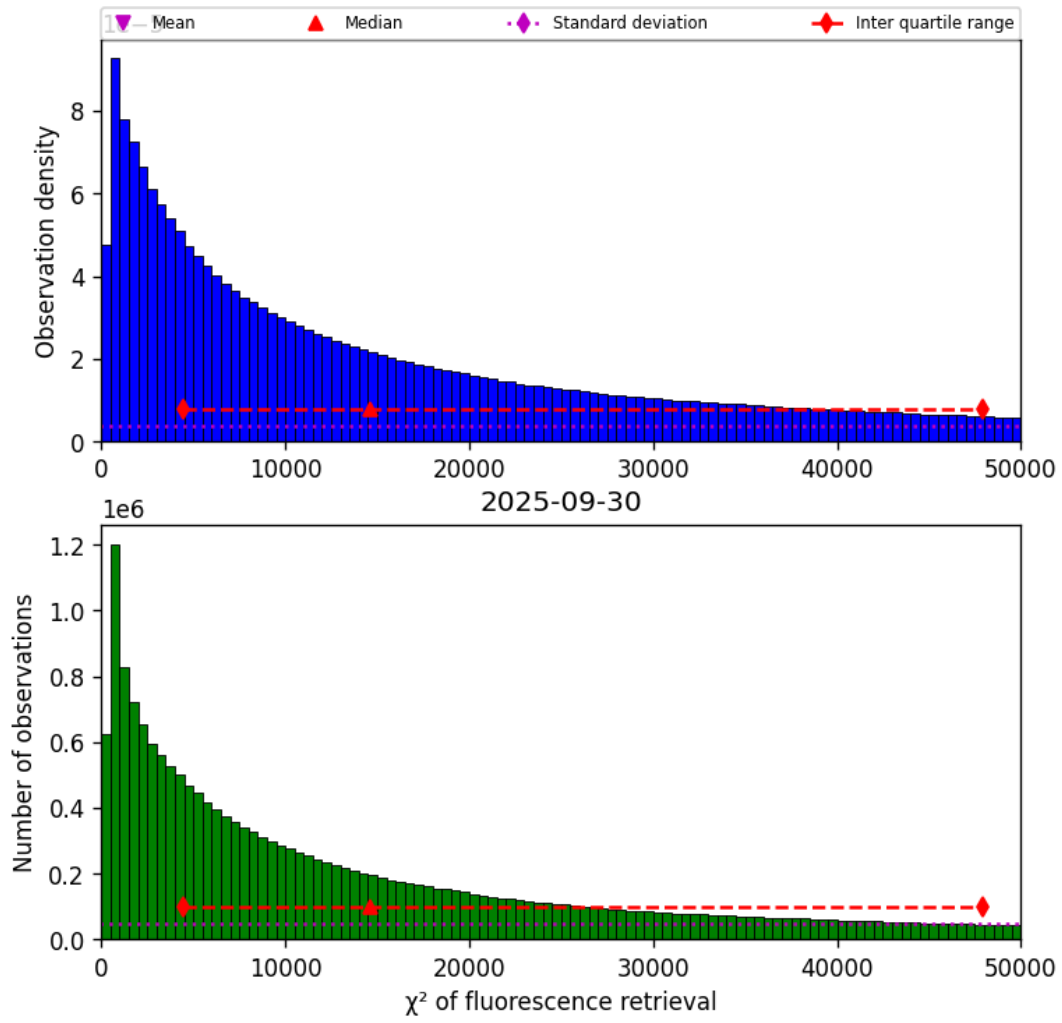
Figure 40: Histogram of “ \chi^2 of fluorescence retrieval” for 2025-09-30 to 2025-10-01
