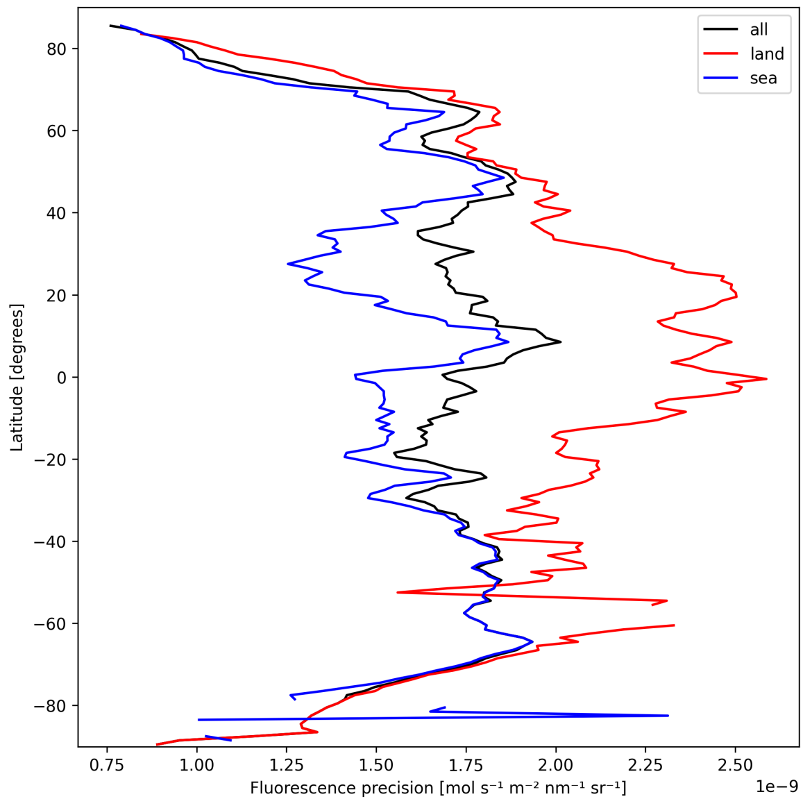
Figure 22: Zonal average of “Fluorescence precision” for 2025-09-30 to 2025-10-01.
