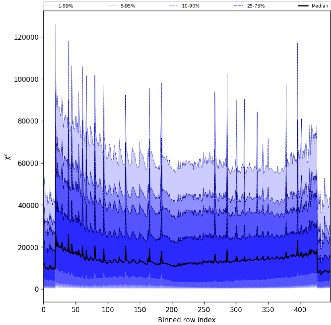
Figure 53: Along track statistics of “ \chi^2 ” for 2025-09-30 to 2025-10-01
