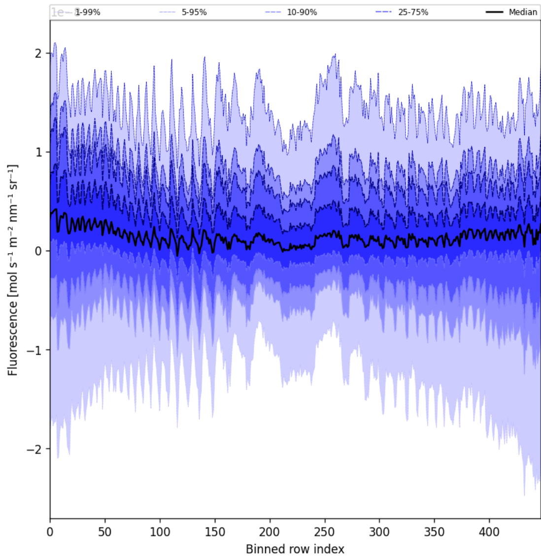
Figure 55: Along track statistics of “Fluorescence” for 2025-09-30 to 2025-10-01
