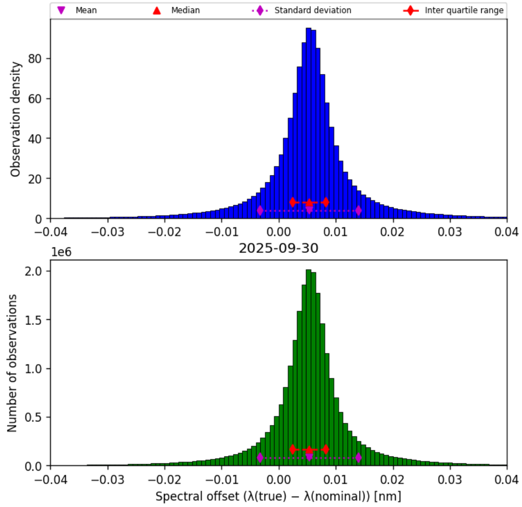
Figure 43: Histogram of “Spectral offset ( \lambda_{\text{true}} - \lambda_{\text{nominal}} )” for 2025-09-30 to 2025-10-01
