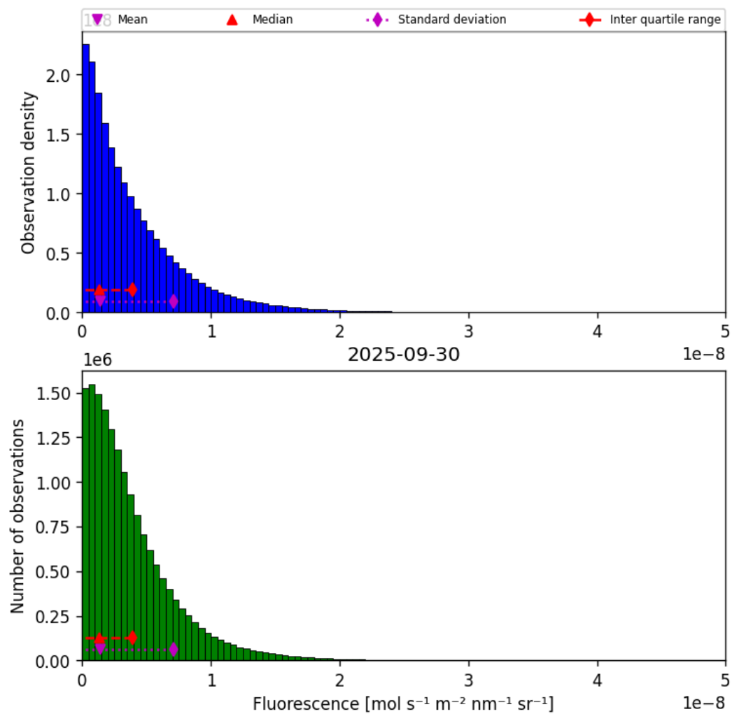
Figure 38: Histogram of “Fluorescence” for 2025-09-30 to 2025-10-01
