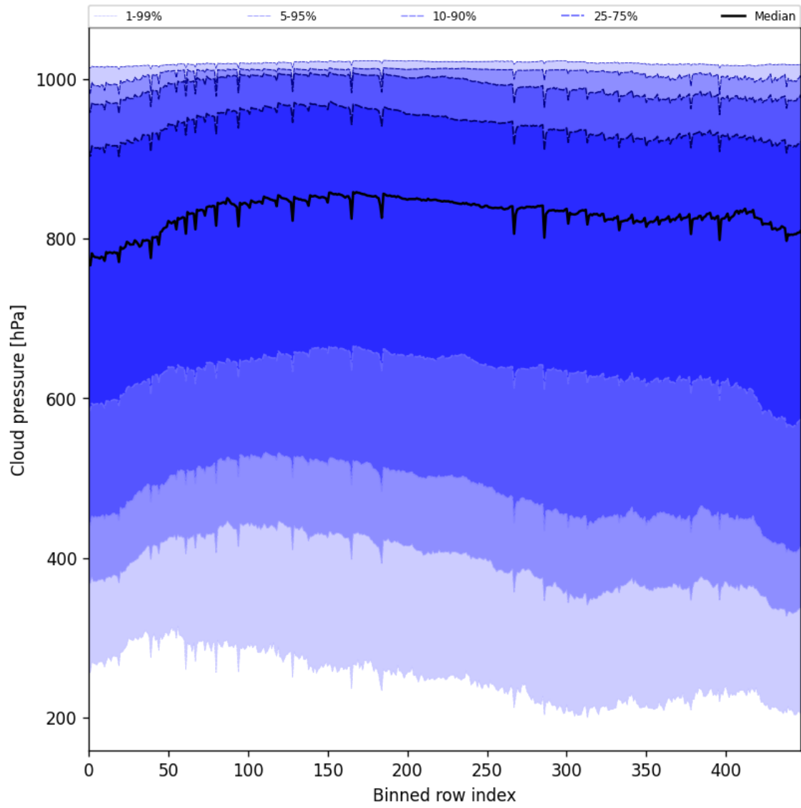
Figure 45: Along track statistics of “Cloud pressure” for 2025-09-30 to 2025-10-01
