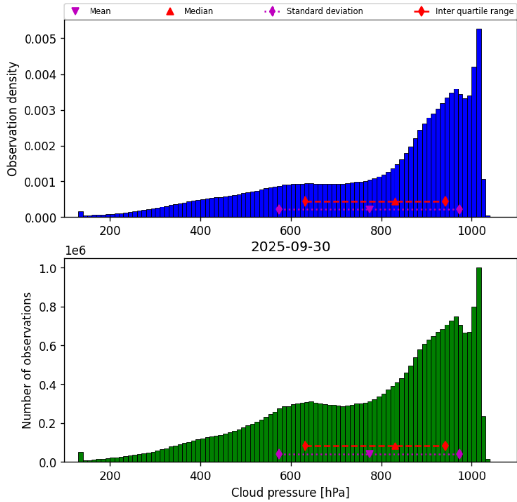
Figure 28: Histogram of “Cloud pressure” for 2025-09-30 to 2025-10-01
