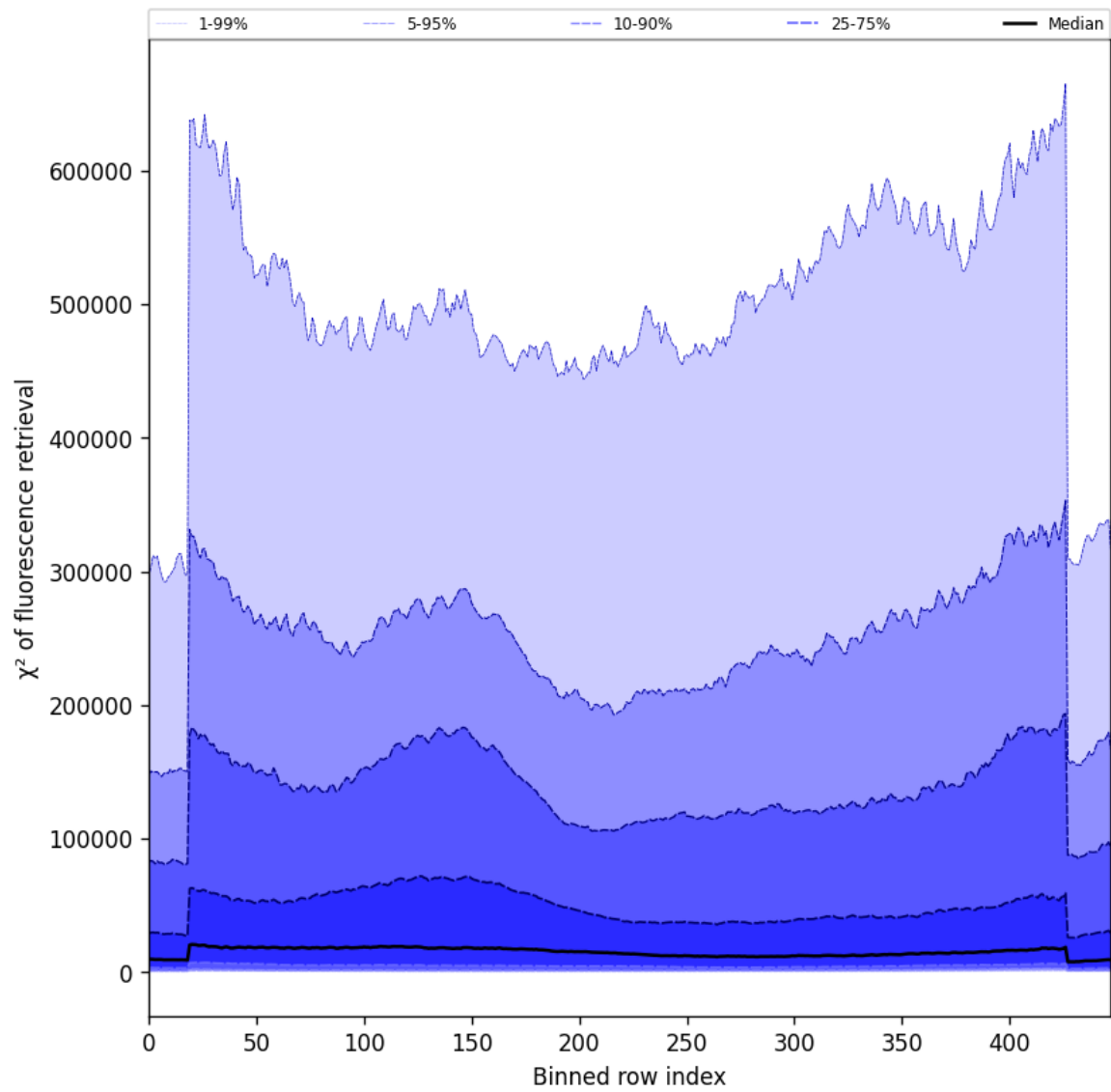
Figure 57: Along track statistics of “ \chi^2 of fluorescence retrieval” for 2025-09-30 to 2025-10-01
