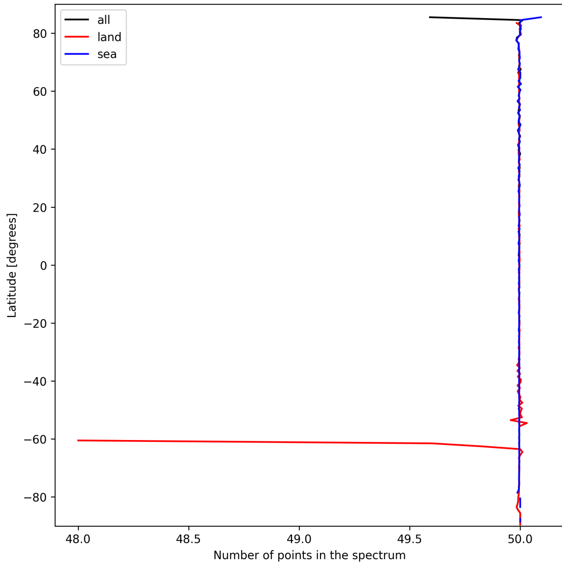
Figure 25: Zonal average of “Number of points in the spectrum” for 2025-09-30 to 2025-10-01.
