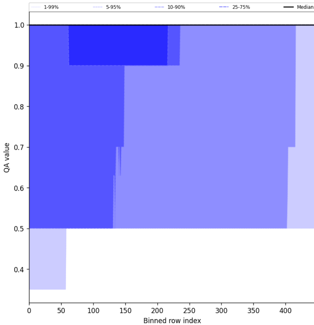
Figure 44: Along track statistics of “QA value” for 2025-09-30 to 2025-10-01
