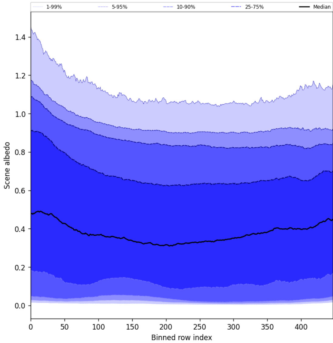
Figure 49: Along track statistics of “Scene albedo” for 2025-09-30 to 2025-10-01
