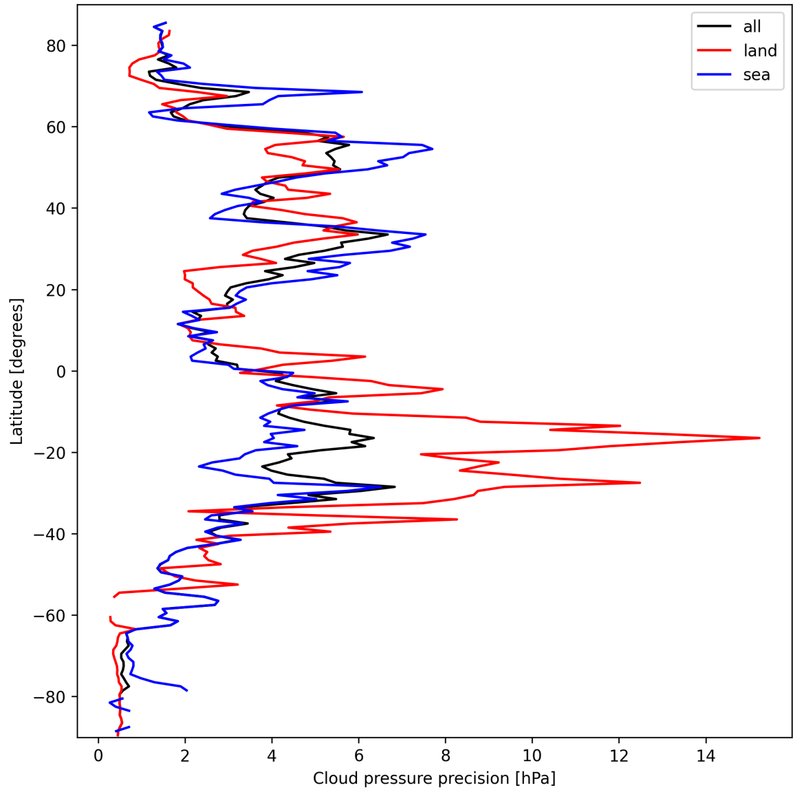
Figure 12: Zonal average of “Cloud pressure precision” for 2025-09-30 to 2025-10-01.
