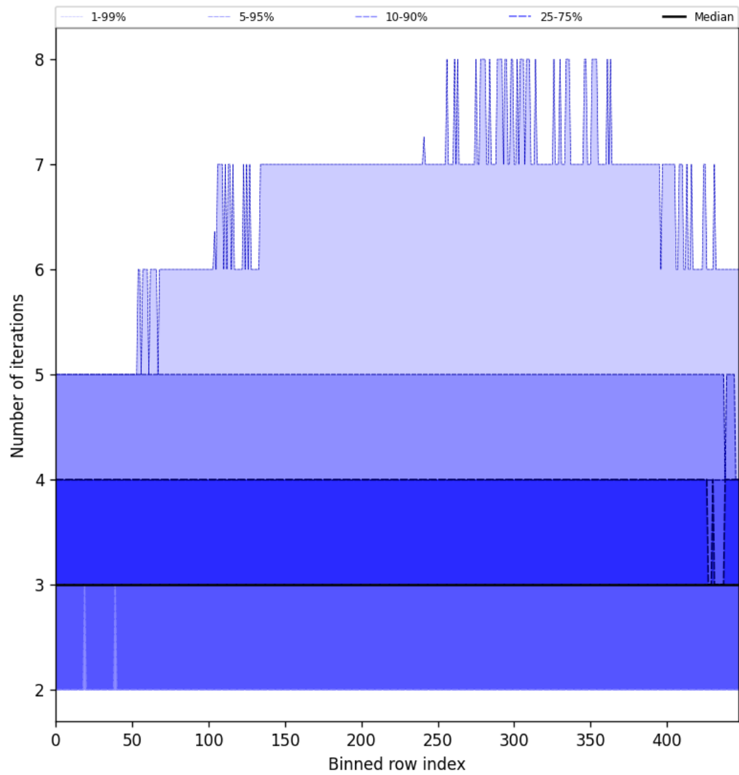
Figure 54: Along track statistics of “Number of iterations” for 2025-09-30 to 2025-10-01
