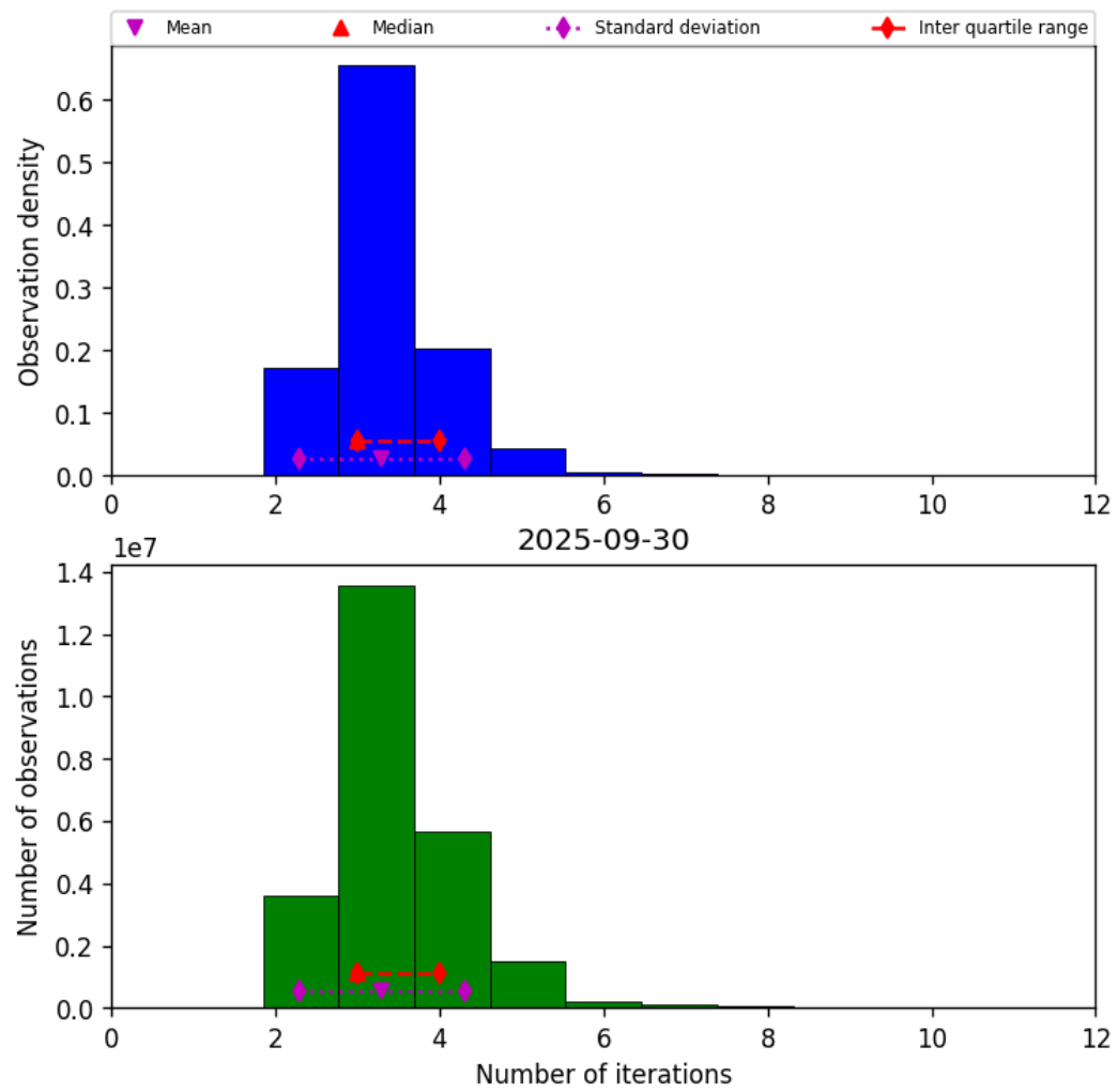
Figure 37: Histogram of “Number of iterations” for 2025-09-30 to 2025-10-01
