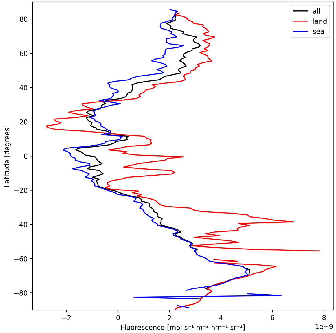
Figure 21: Zonal average of “Fluorescence” for 2025-09-30 to 2025-10-01.
