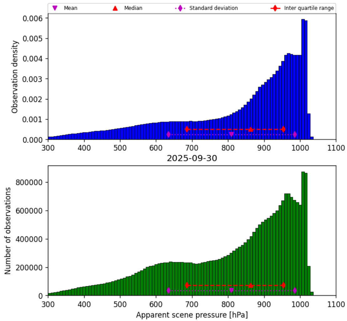
Figure 34: Histogram of “Apparent scene pressure” for 2025-09-30 to 2025-10-01
