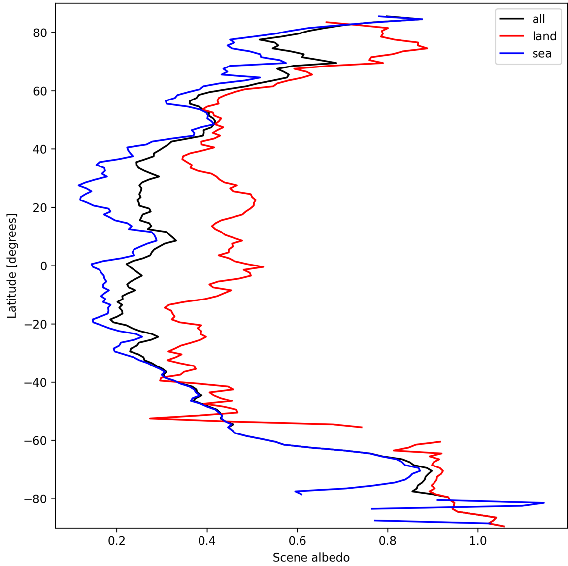
Figure 15: Zonal average of “Scene albedo” for 2025-09-30 to 2025-10-01.
