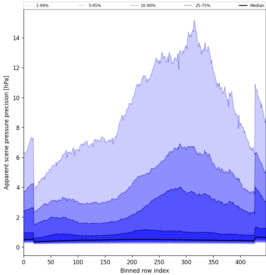
Figure 52: Along track statistics of “Apparent scene pressure precision” for 2025-09-30 to 2025-10-01
