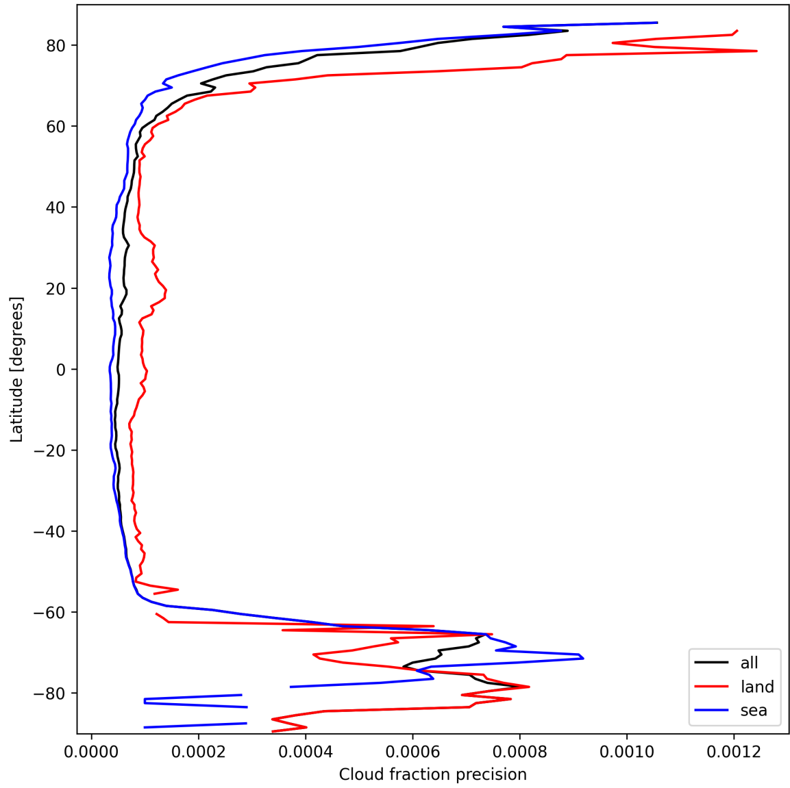
Figure 14: Zonal average of “Cloud fraction precision” for 2025-09-30 to 2025-10-01.
