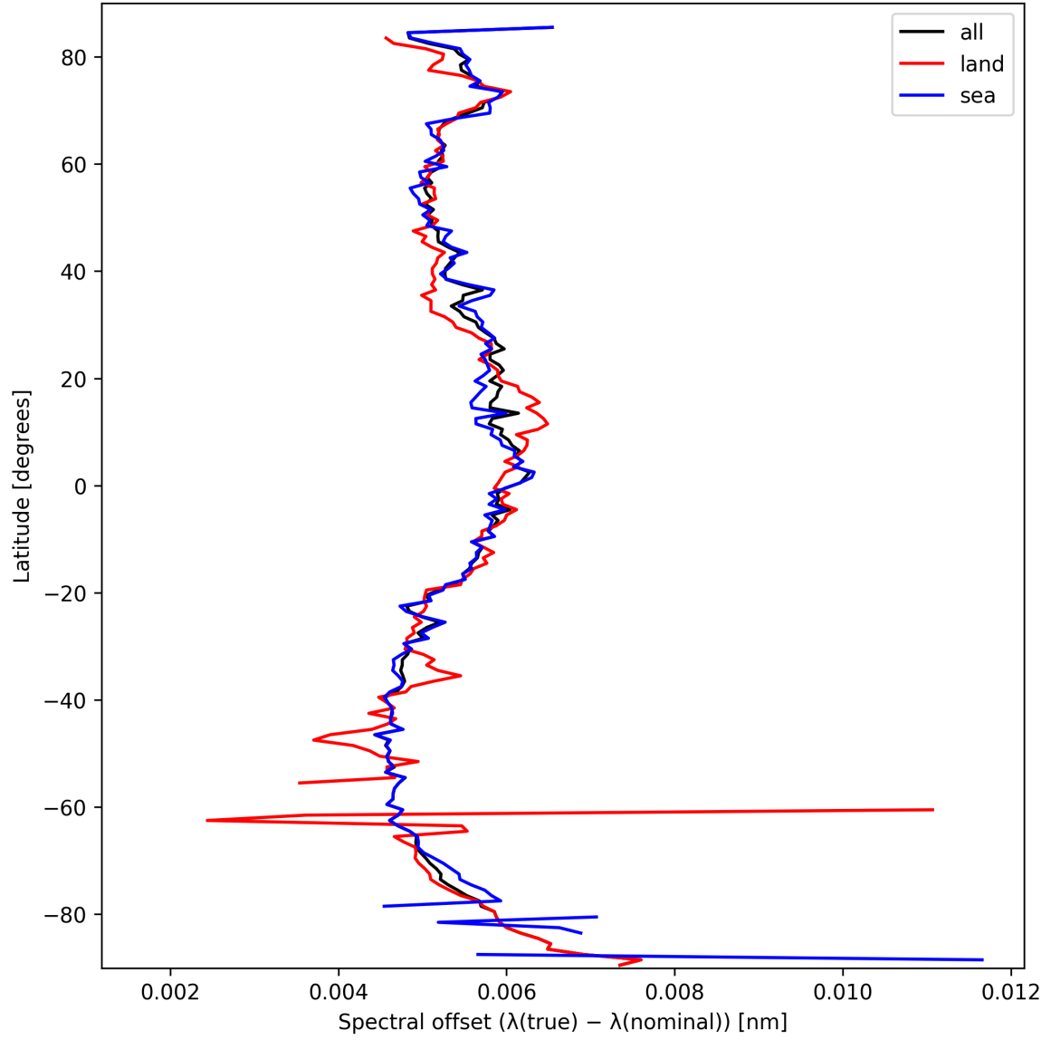
Figure 26: Zonal average of “Spectral offset ( \lambda_{\text{true}} - \lambda_{\text{nominal}} )” for 2025-09-30 to 2025-10-01.
