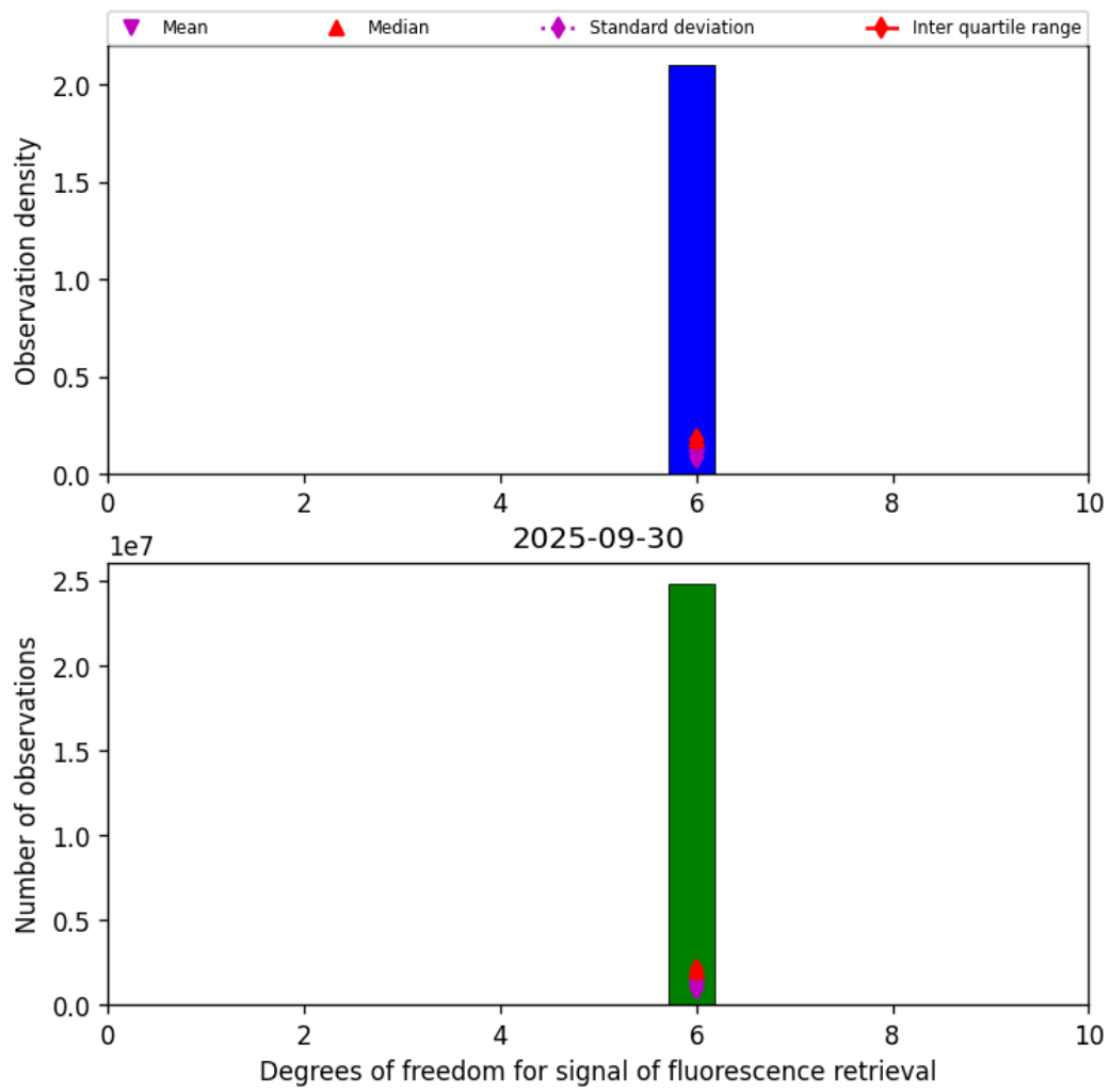
Figure 41: Histogram of “Degrees of freedom for signal of fluorescence retrieval” for 2025-09-30 to 2025-10-01
