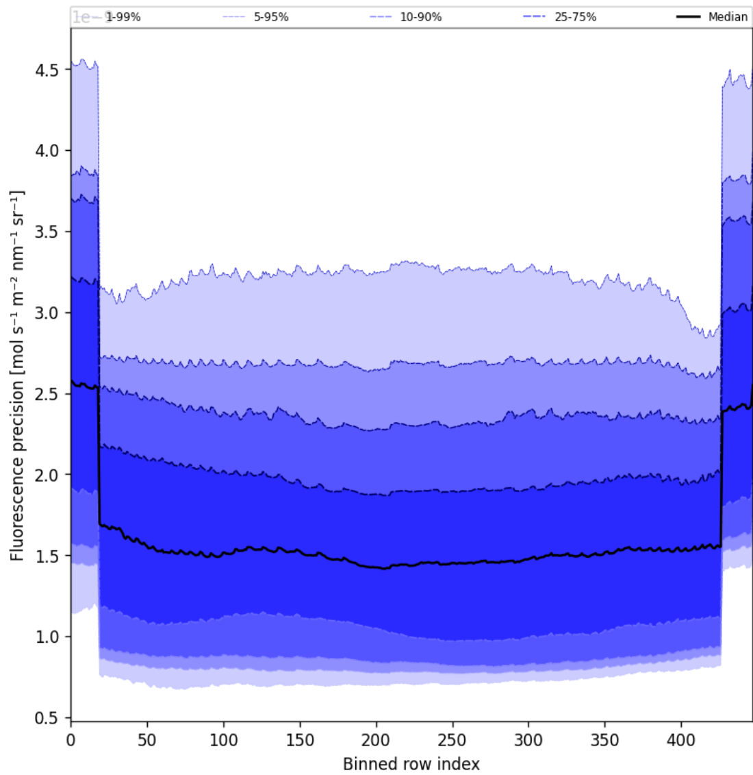
Figure 56: Along track statistics of “Fluorescence precision” for 2025-09-30 to 2025-10-01
