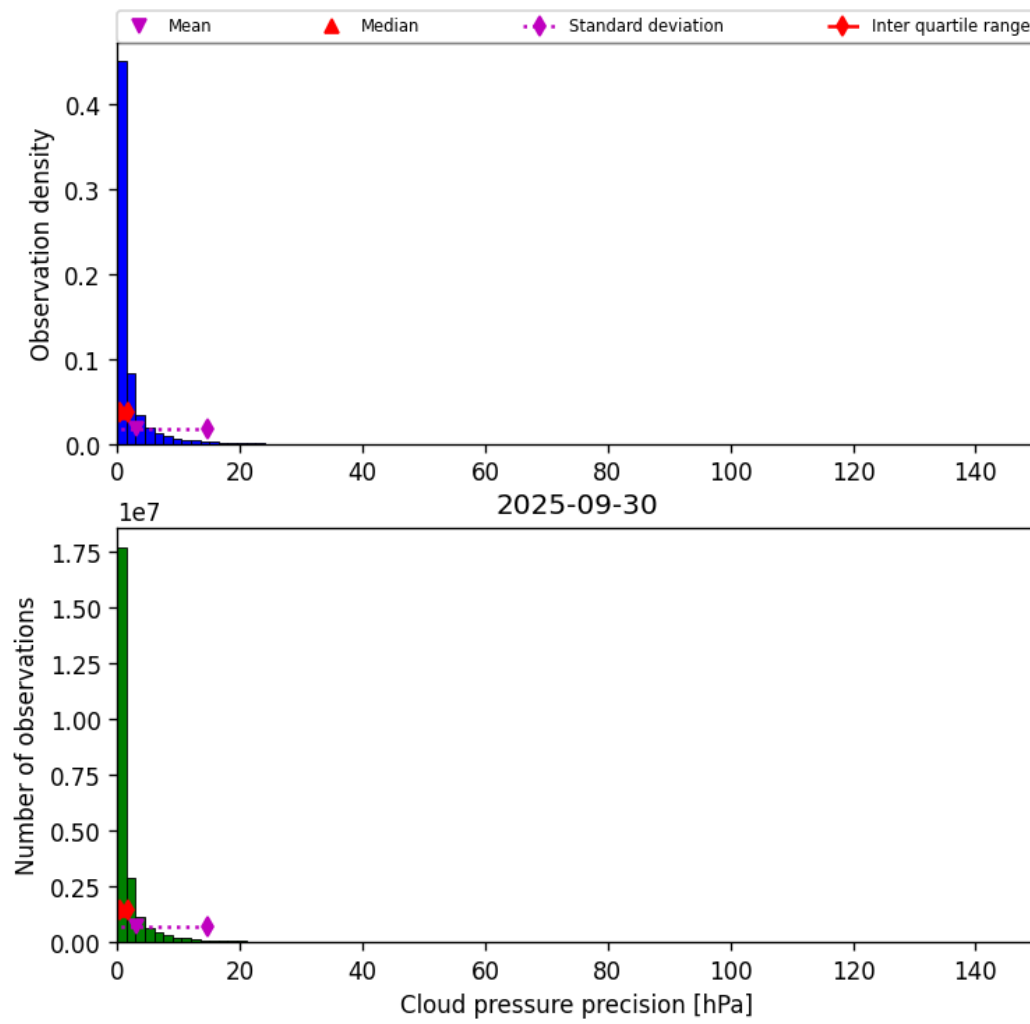
Figure 29: Histogram of “Cloud pressure precision” for 2025-09-30 to 2025-10-01
