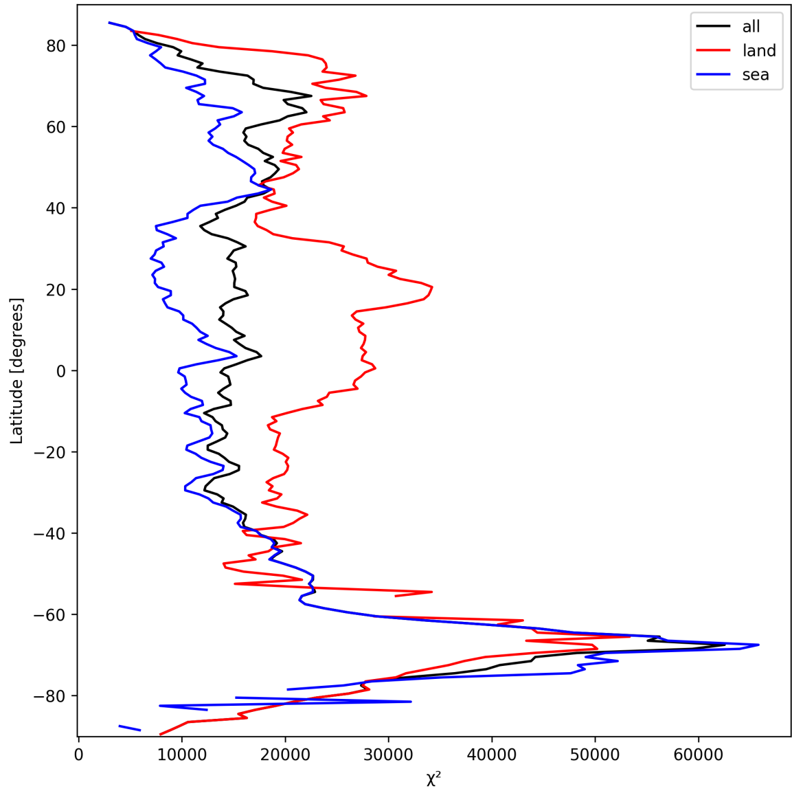
Figure 19: Zonal average of “ \chi^2 ” for 2025-09-30 to 2025-10-01.
