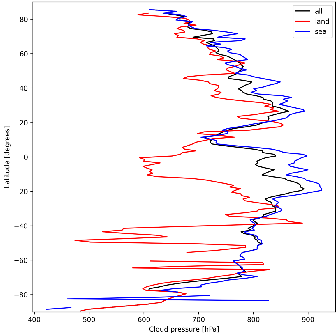
Figure 11: Zonal average of “Cloud pressure” for 2025-09-30 to 2025-10-01.
