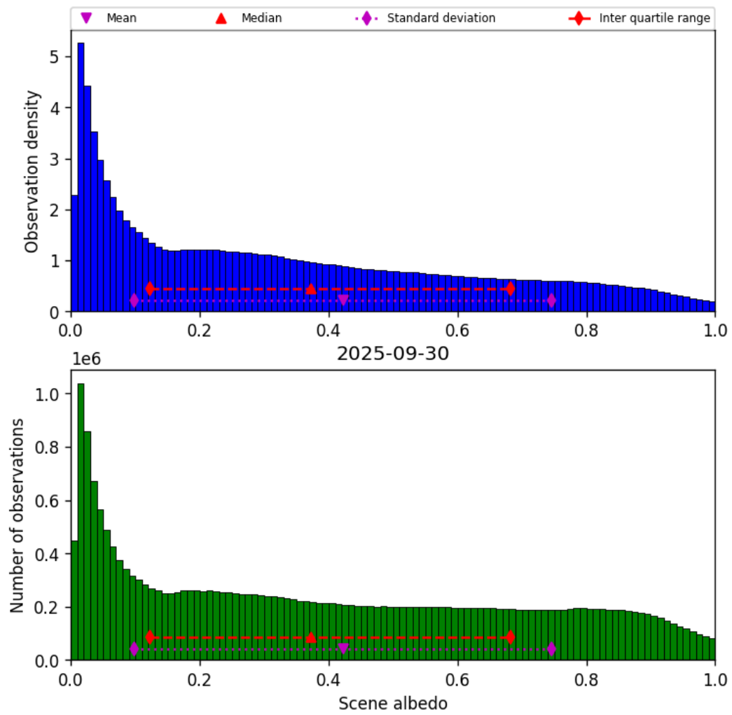
Figure 32: Histogram of “Scene albedo” for 2025-09-30 to 2025-10-01
