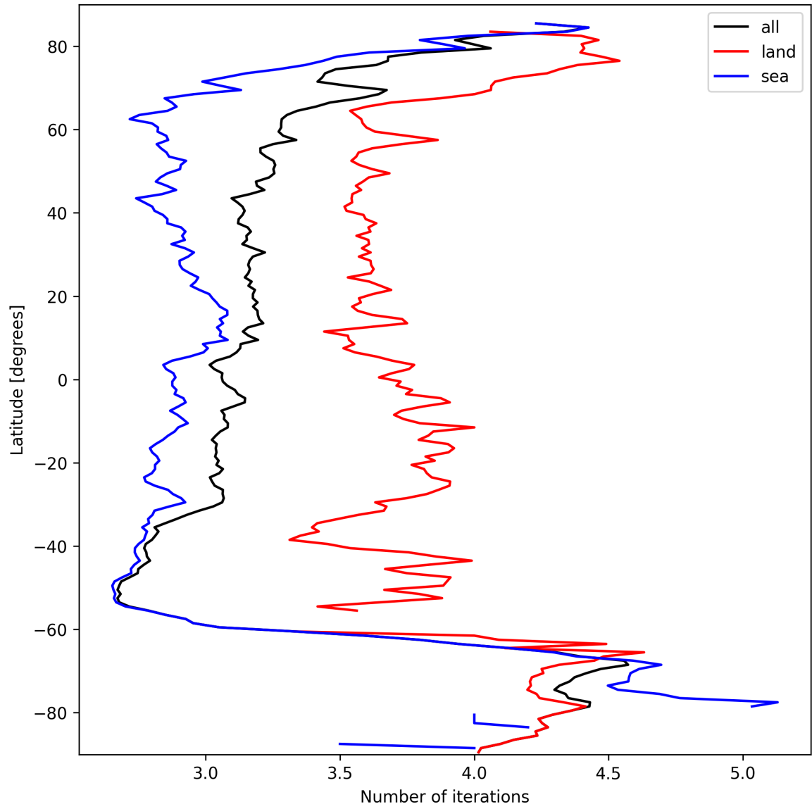
Figure 20: Zonal average of “Number of iterations” for 2025-09-30 to 2025-10-01.
