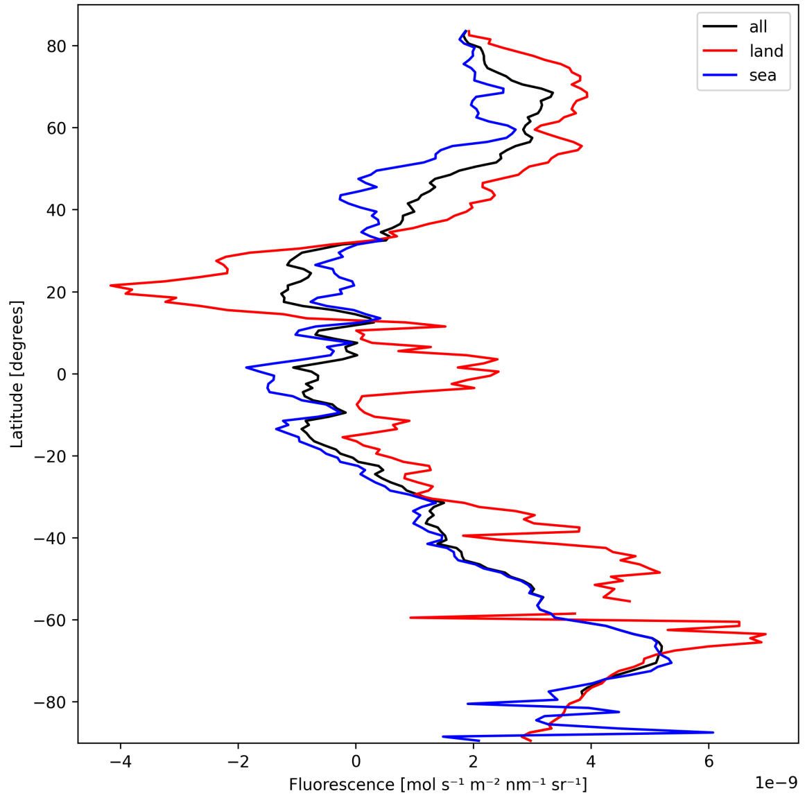
Figure 21: Zonal average of “Fluorescence” for 2025-10-03 to 2025-10-04.
