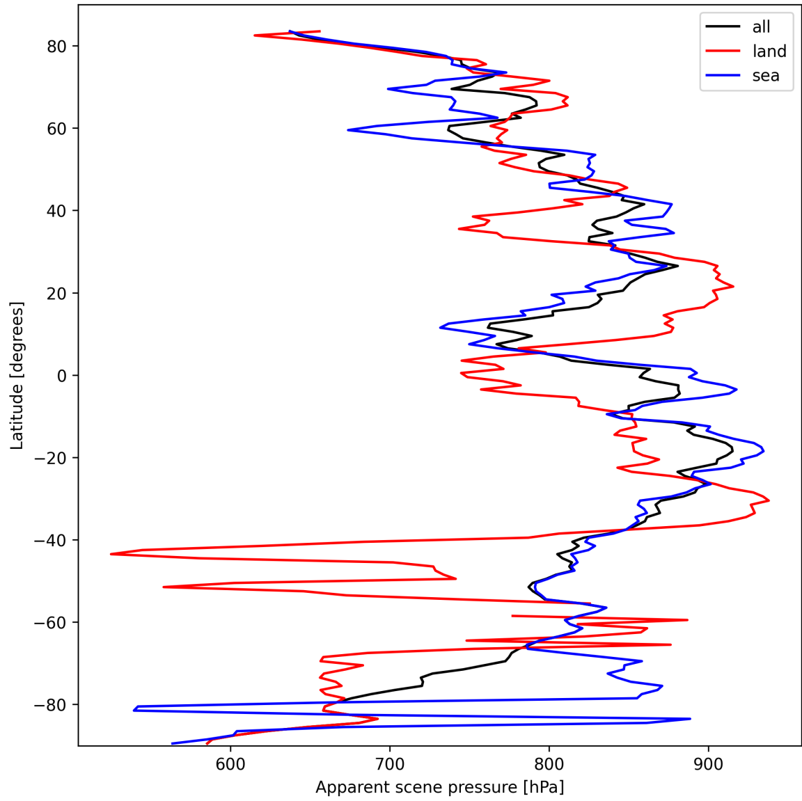
Figure 17: Zonal average of “Apparent scene pressure” for 2025-10-03 to 2025-10-04.
