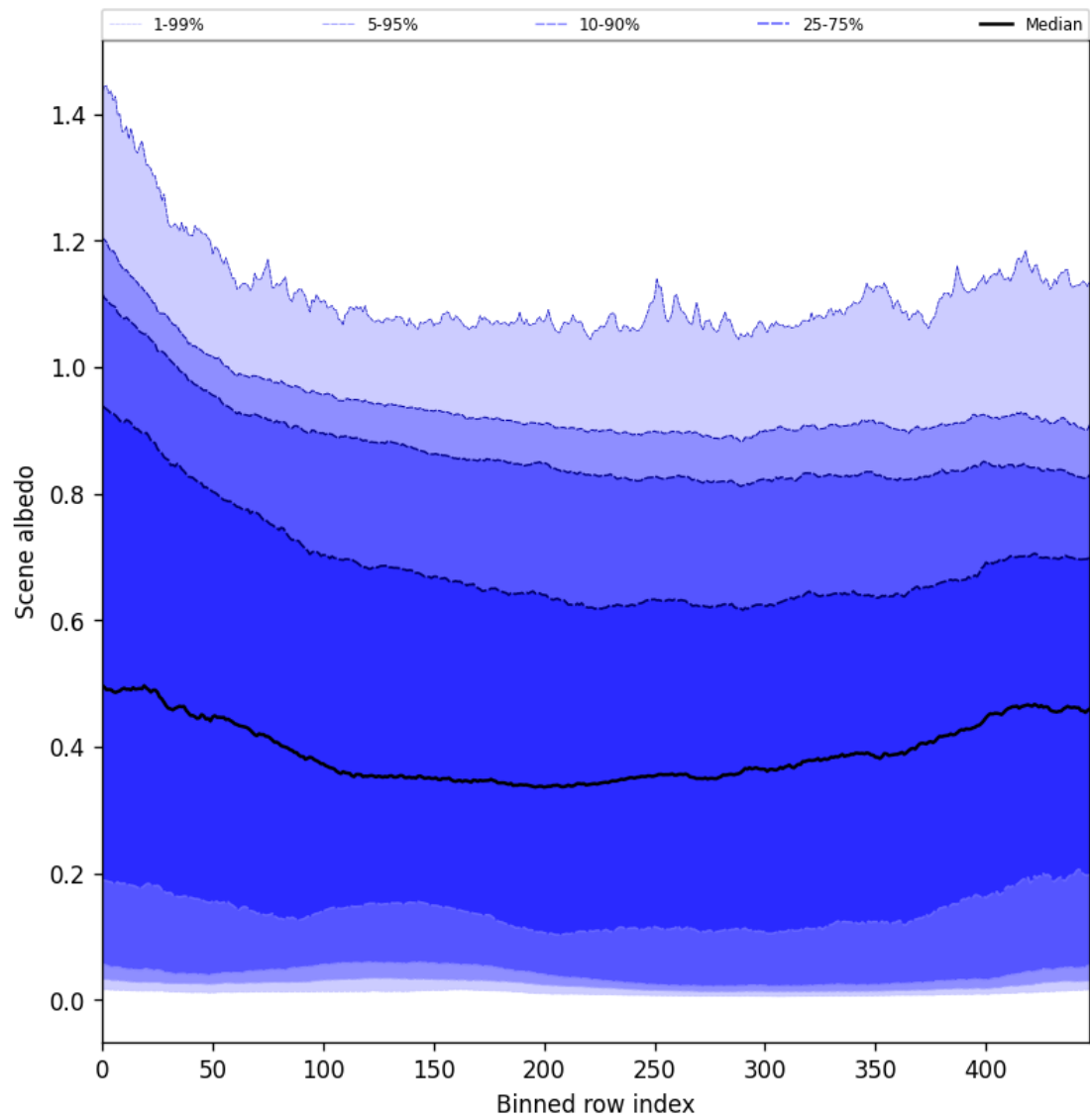
Figure 49: Along track statistics of “Scene albedo” for 2025-10-03 to 2025-10-04
