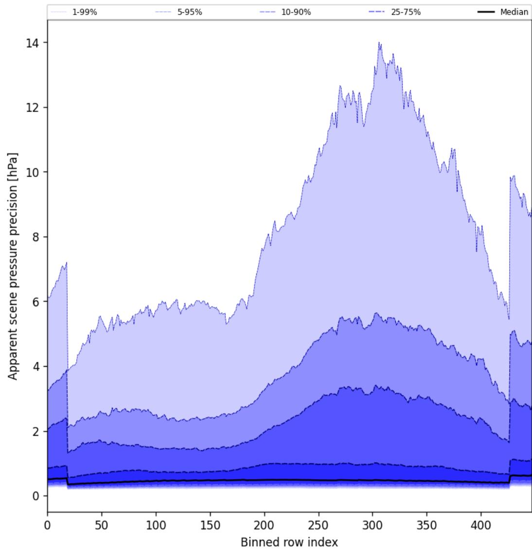
Figure 52: Along track statistics of “Apparent scene pressure precision” for 2025-10-03 to 2025-10-04
