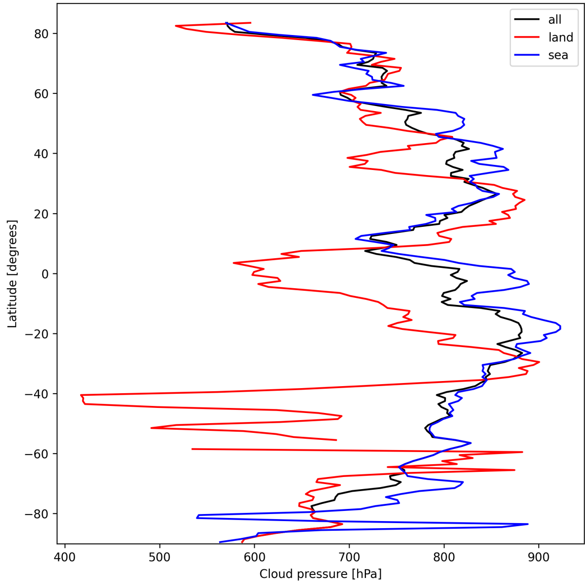
Figure 11: Zonal average of “Cloud pressure” for 2025-10-03 to 2025-10-04.
