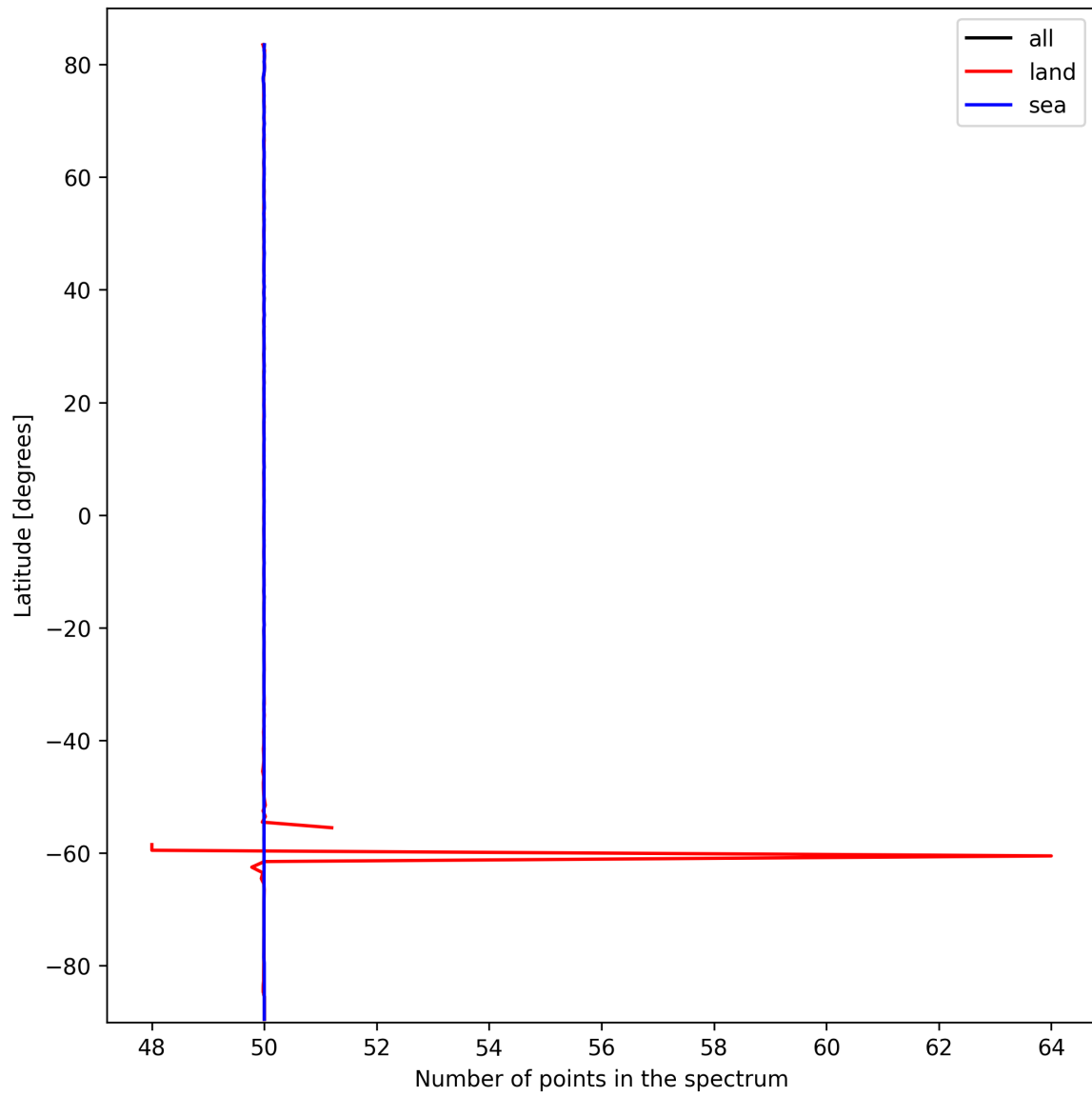
Figure 25: Zonal average of “Number of points in the spectrum” for 2025-10-03 to 2025-10-04.
