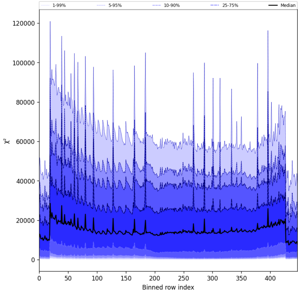
Figure 53: Along track statistics of “ \chi^2 ” for 2025-10-03 to 2025-10-04
