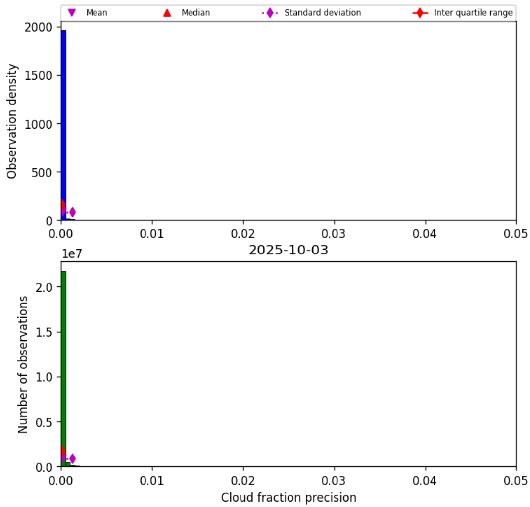
Figure 31: Histogram of “Cloud fraction precision” for 2025-10-03 to 2025-10-04
