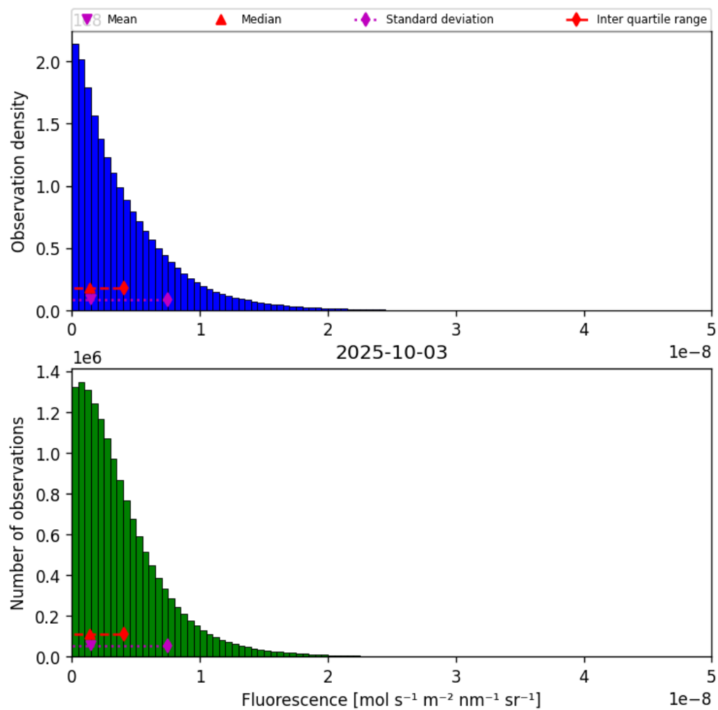
Figure 38: Histogram of “Fluorescence” for 2025-10-03 to 2025-10-04
