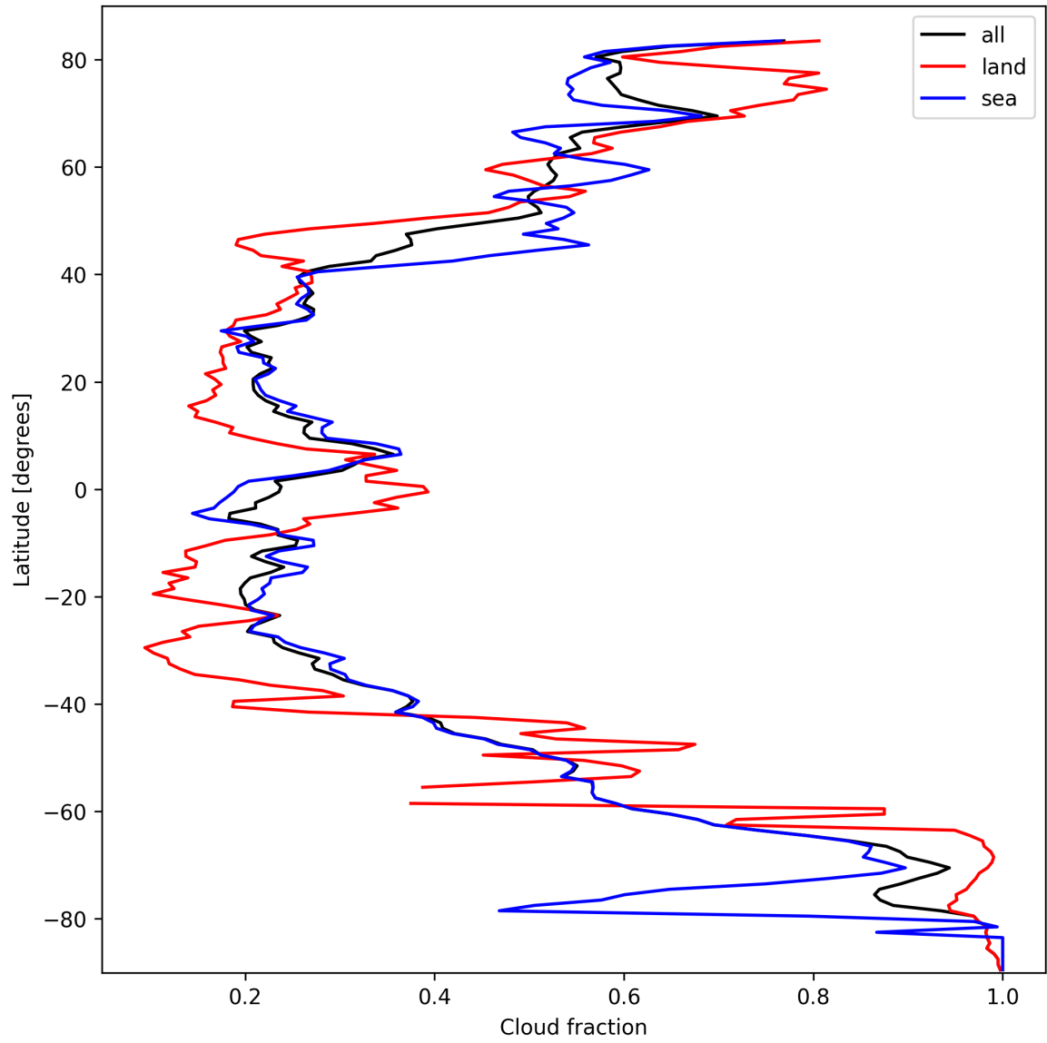
Figure 13: Zonal average of “Cloud fraction” for 2025-10-03 to 2025-10-04.
