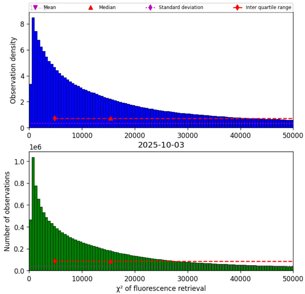
Figure 40: Histogram of “ \chi^2 of fluorescence retrieval” for 2025-10-03 to 2025-10-04
