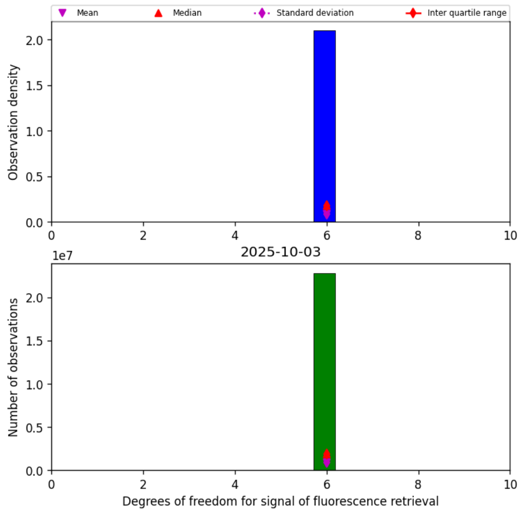
Figure 41: Histogram of “Degrees of freedom for signal of fluorescence retrieval” for 2025-10-03 to 2025-10-04
