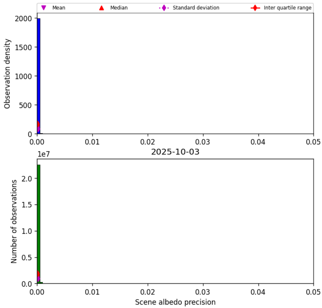
Figure 33: Histogram of “Scene albedo precision” for 2025-10-03 to 2025-10-04
