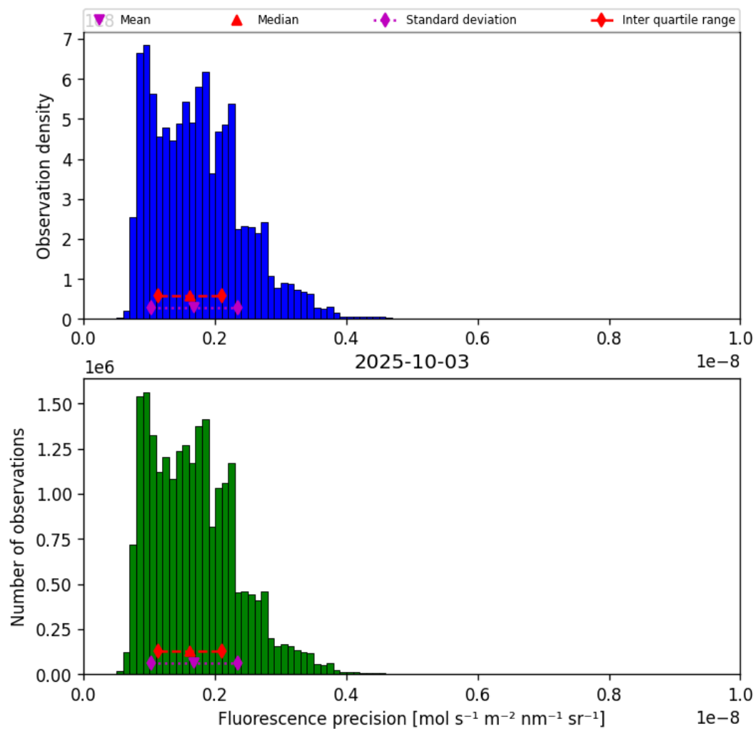
Figure 39: Histogram of “Fluorescence precision” for 2025-10-03 to 2025-10-04
