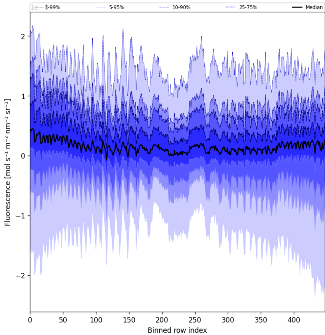
Figure 55: Along track statistics of "Fluorescence" for 2025-10-03 to 2025-10-04
