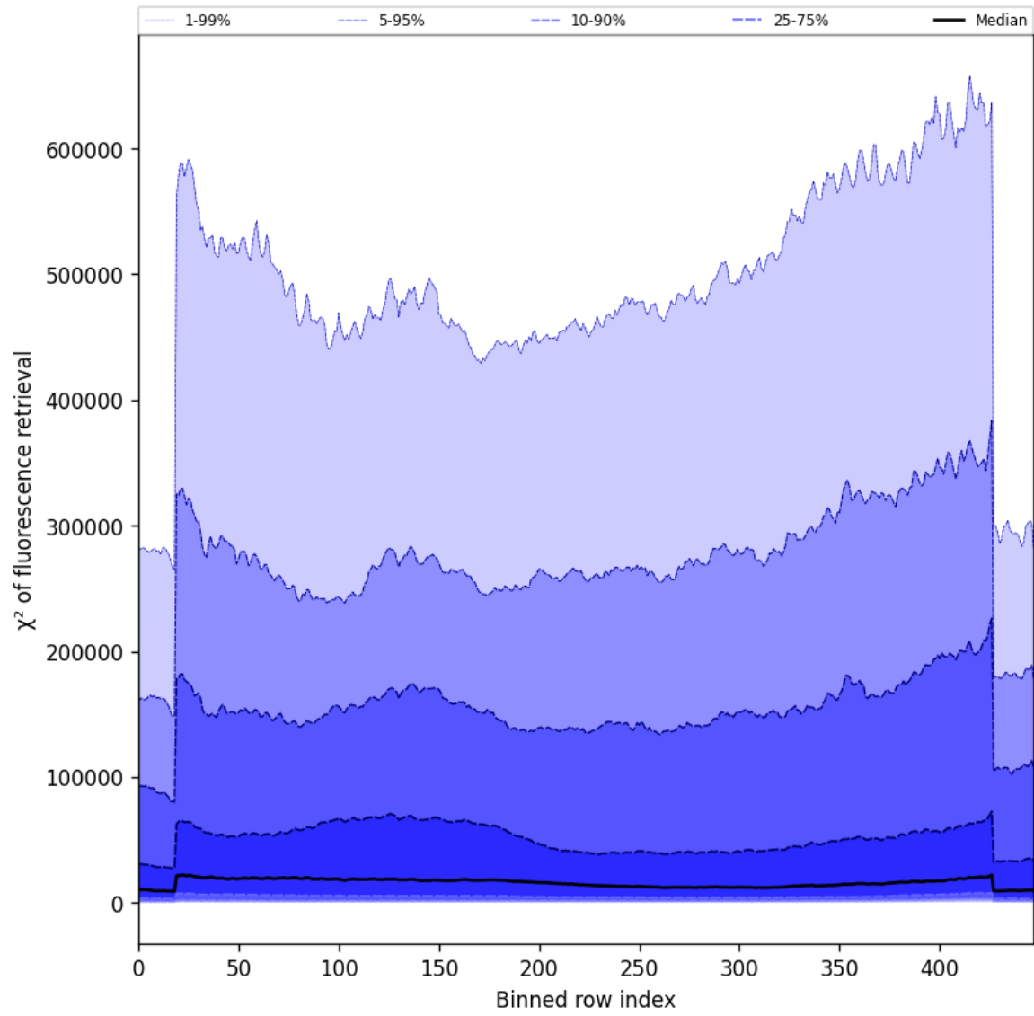
Figure 57: Along track statistics of " \chi^2 of fluorescence retrieval" for 2025-10-03 to 2025-10-04
