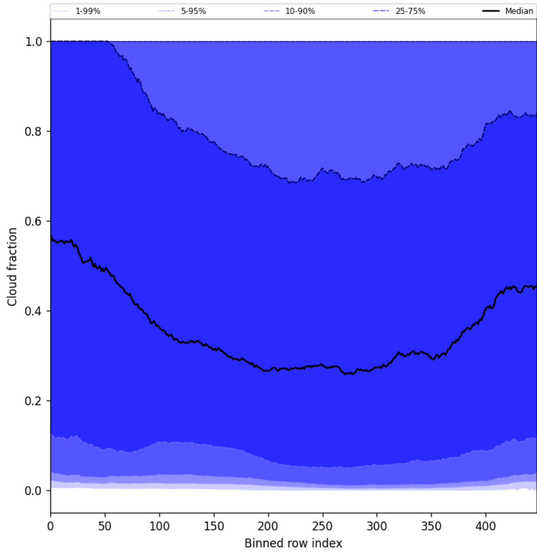
Figure 47: Along track statistics of “Cloud fraction” for 2025-10-03 to 2025-10-04
