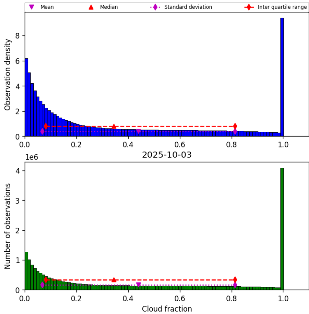
Figure 30: Histogram of “Cloud fraction” for 2025-10-03 to 2025-10-04
