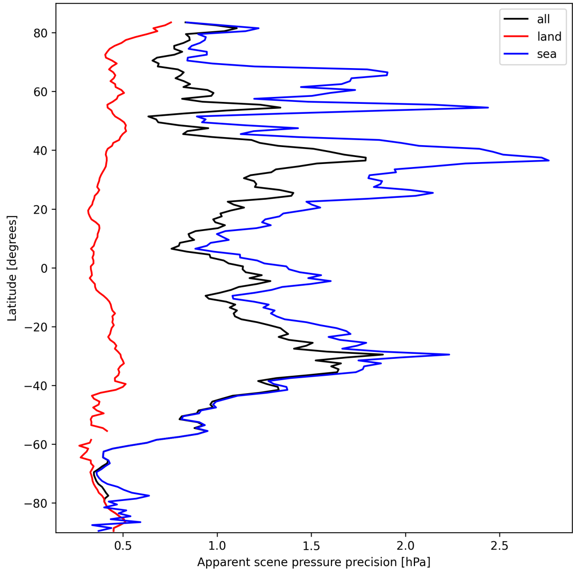
Figure 18: Zonal average of “Apparent scene pressure precision” for 2025-10-03 to 2025-10-04.
