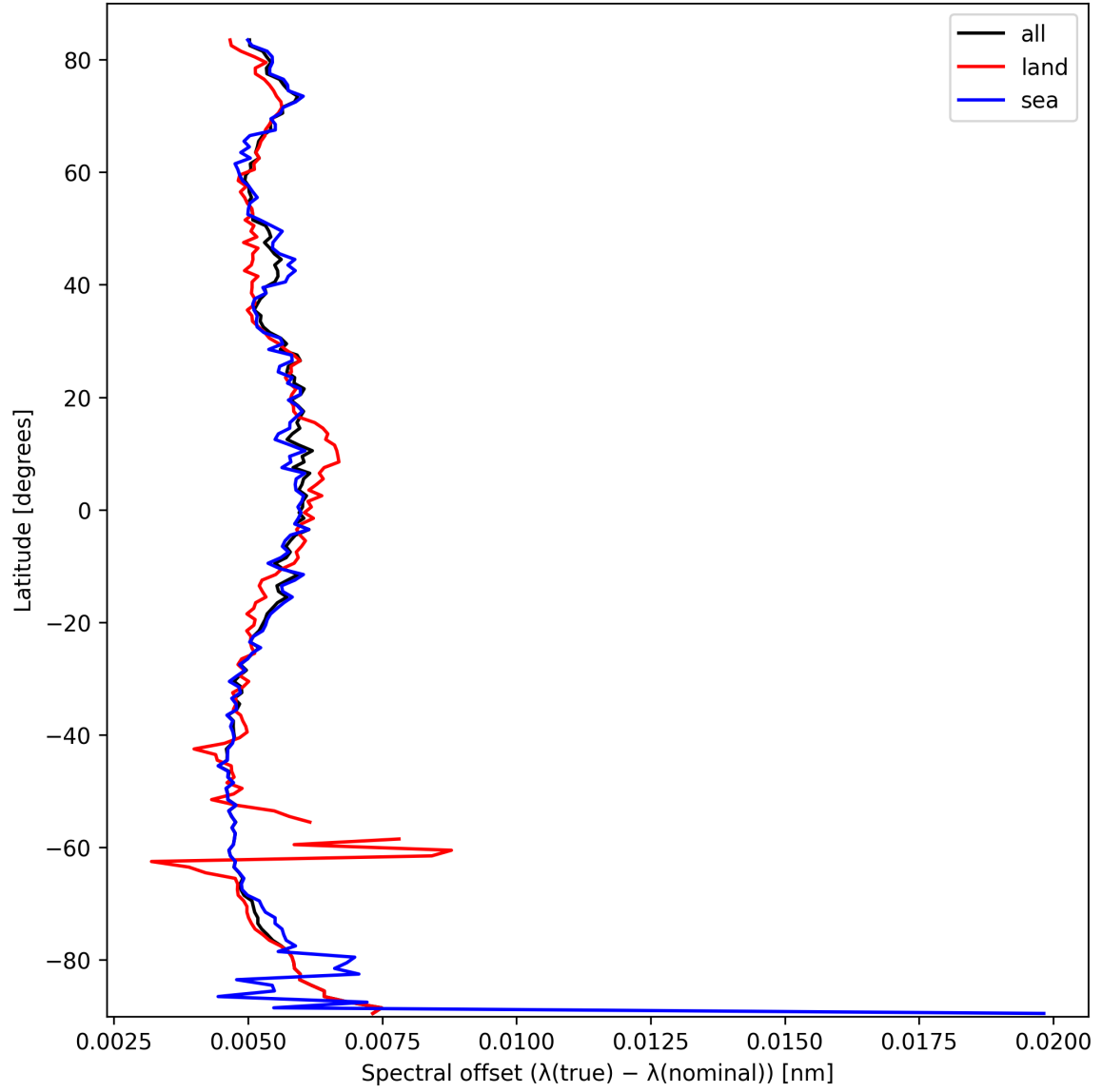
Figure 26: Zonal average of “Spectral offset ( \lambda_{\text{true}} - \lambda_{\text{nominal}} )” for 2025-10-03 to 2025-10-04.
