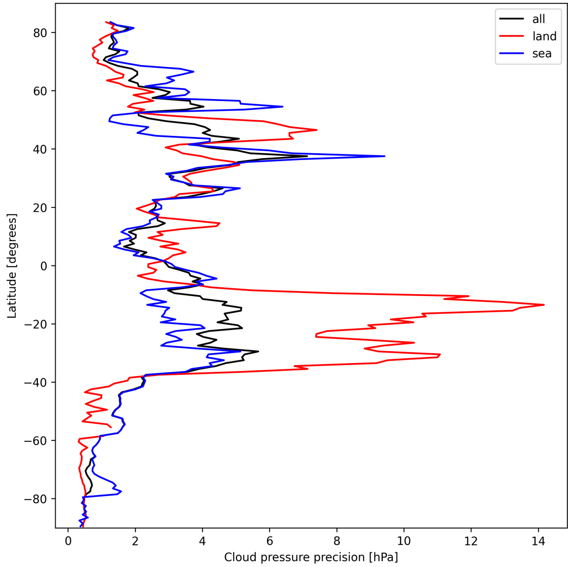
Figure 12: Zonal average of “Cloud pressure precision” for 2025-10-03 to 2025-10-04.
