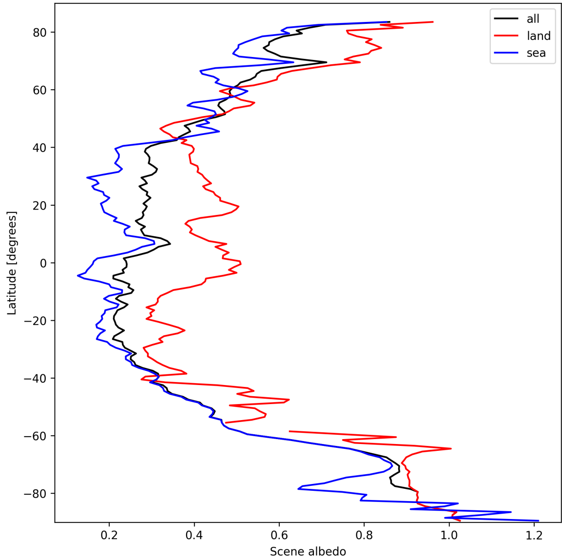
Figure 15: Zonal average of “Scene albedo” for 2025-10-03 to 2025-10-04.
