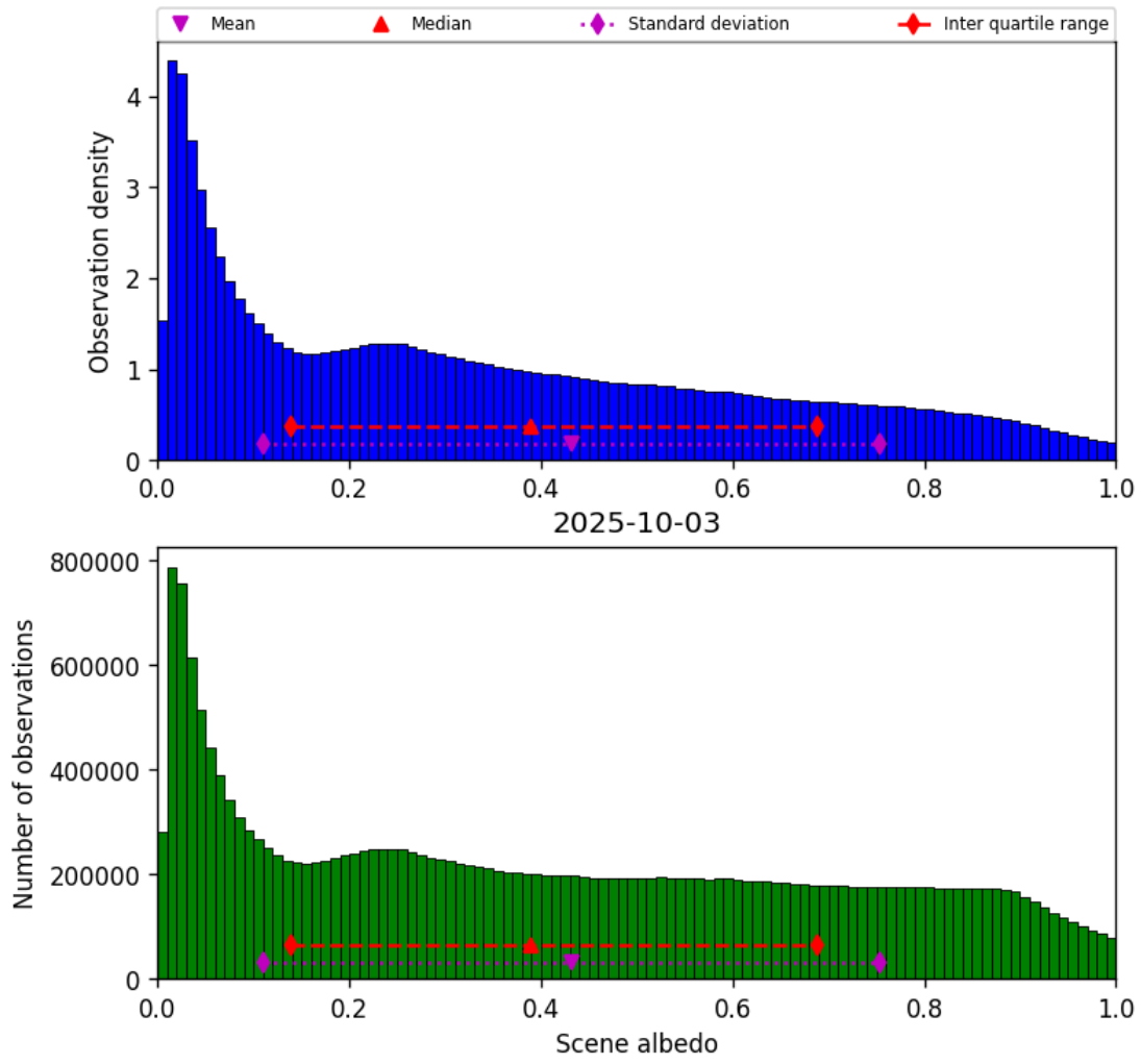
Figure 32: Histogram of “Scene albedo” for 2025-10-03 to 2025-10-04
