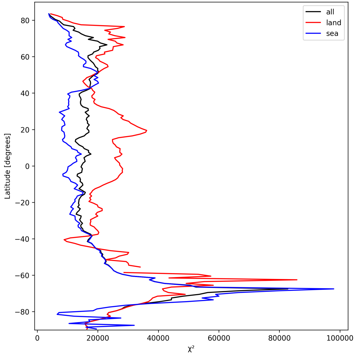
Figure 19: Zonal average of “ \chi^2 ” for 2025-10-03 to 2025-10-04.
