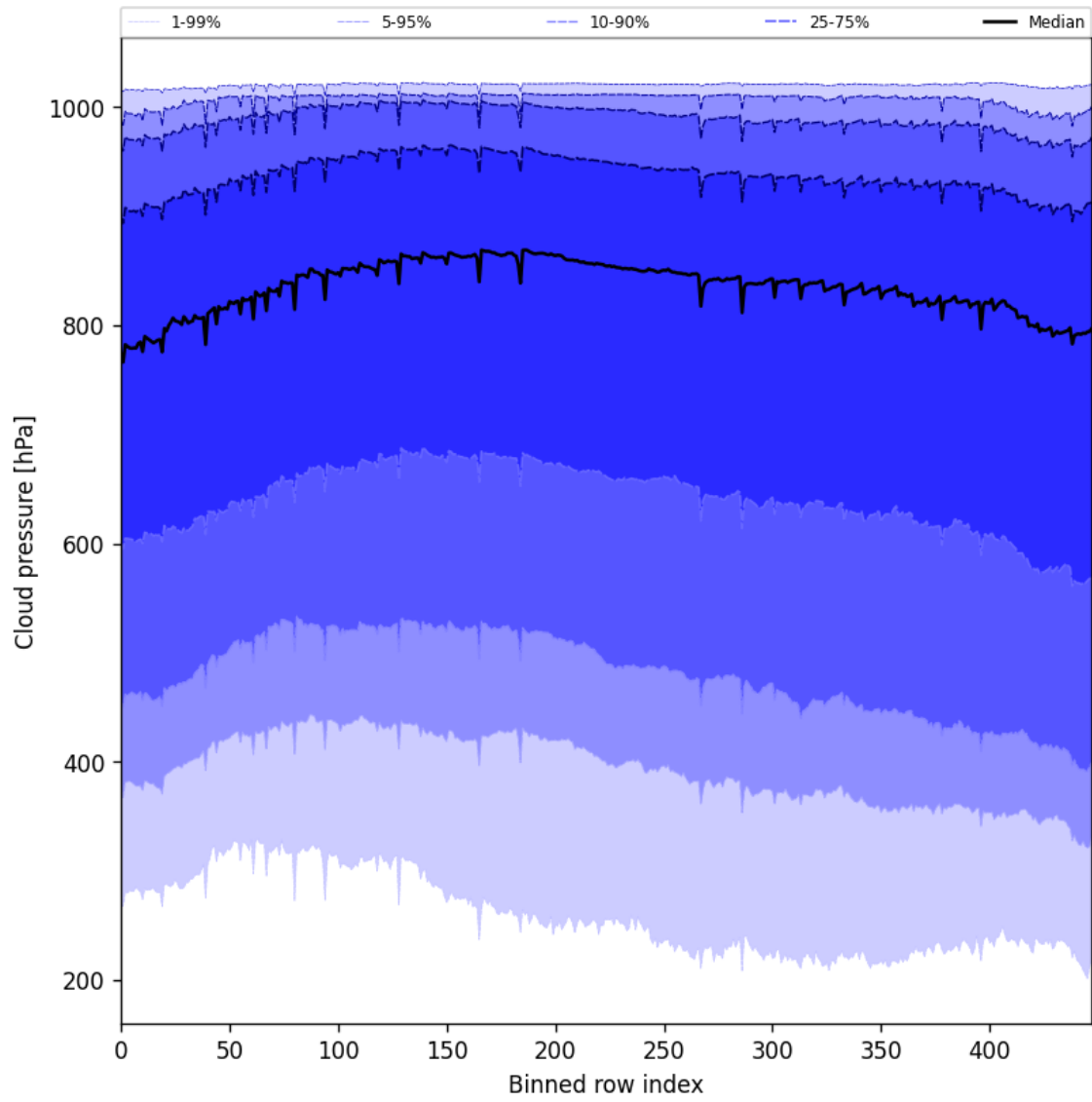
Figure 45: Along track statistics of “Cloud pressure” for 2025-10-03 to 2025-10-04
