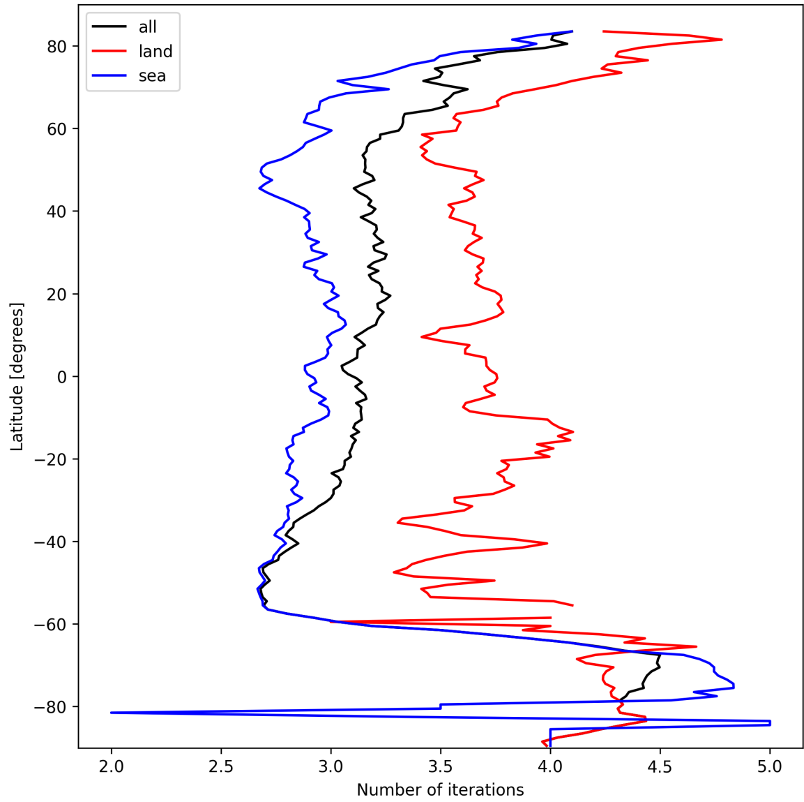
Figure 20: Zonal average of “Number of iterations” for 2025-10-03 to 2025-10-04.
