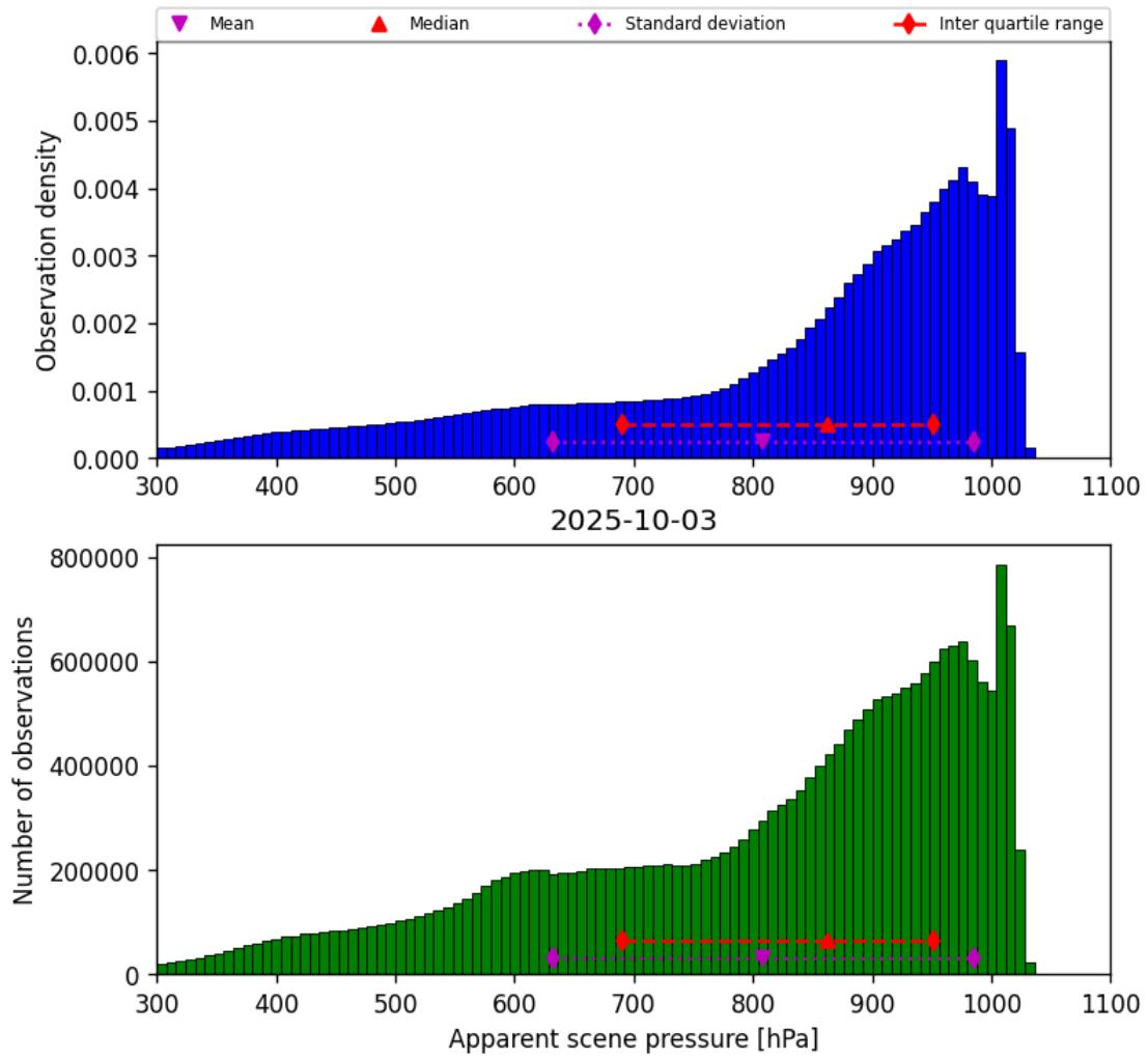
Figure 34: Histogram of “Apparent scene pressure” for 2025-10-03 to 2025-10-04
