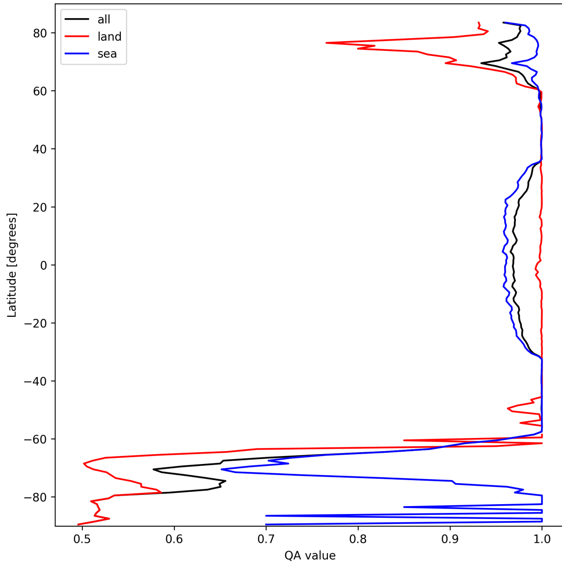
Figure 10: Zonal average of “QA value” for 2025-10-03 to 2025-10-04.
