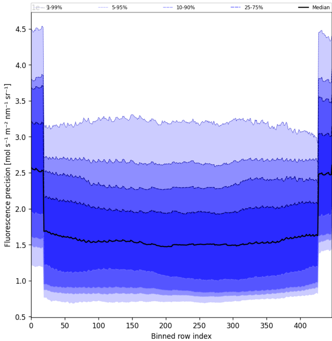
Figure 56: Along track statistics of “Fluorescence precision” for 2025-10-03 to 2025-10-04
