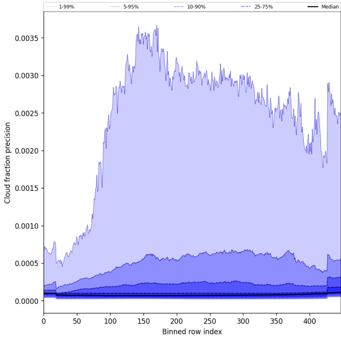
Figure 48: Along track statistics of “Cloud fraction precision” for 2025-10-03 to 2025-10-04
