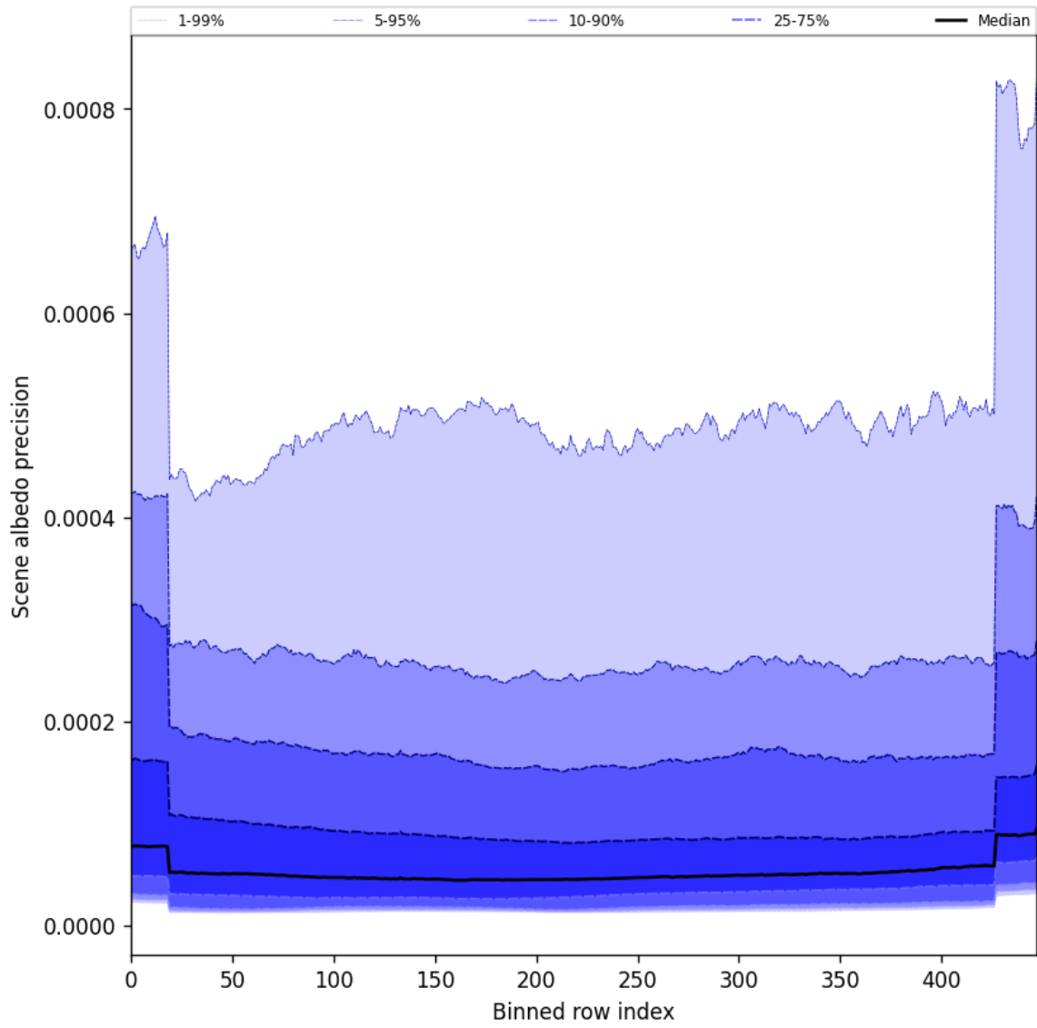
Figure 50: Along track statistics of “Scene albedo precision” for 2025-10-03 to 2025-10-04
