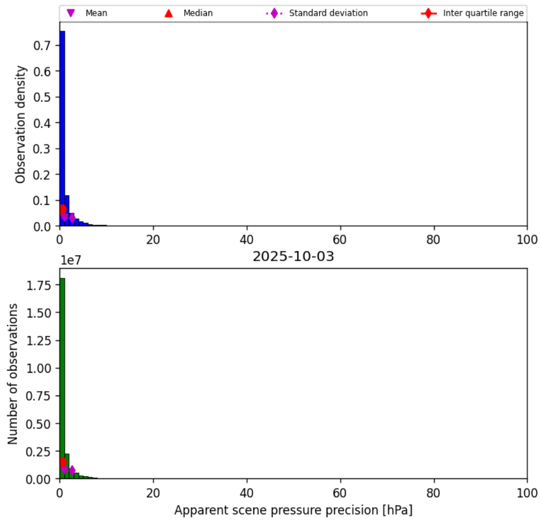
Figure 35: Histogram of “Apparent scene pressure precision” for 2025-10-03 to 2025-10-04
