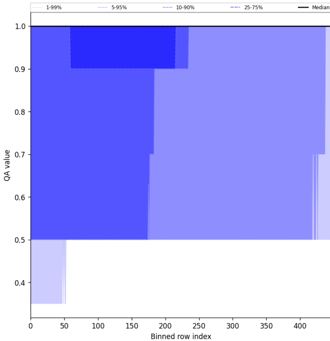
Figure 44: Along track statistics of “QA value” for 2025-10-03 to 2025-10-04
