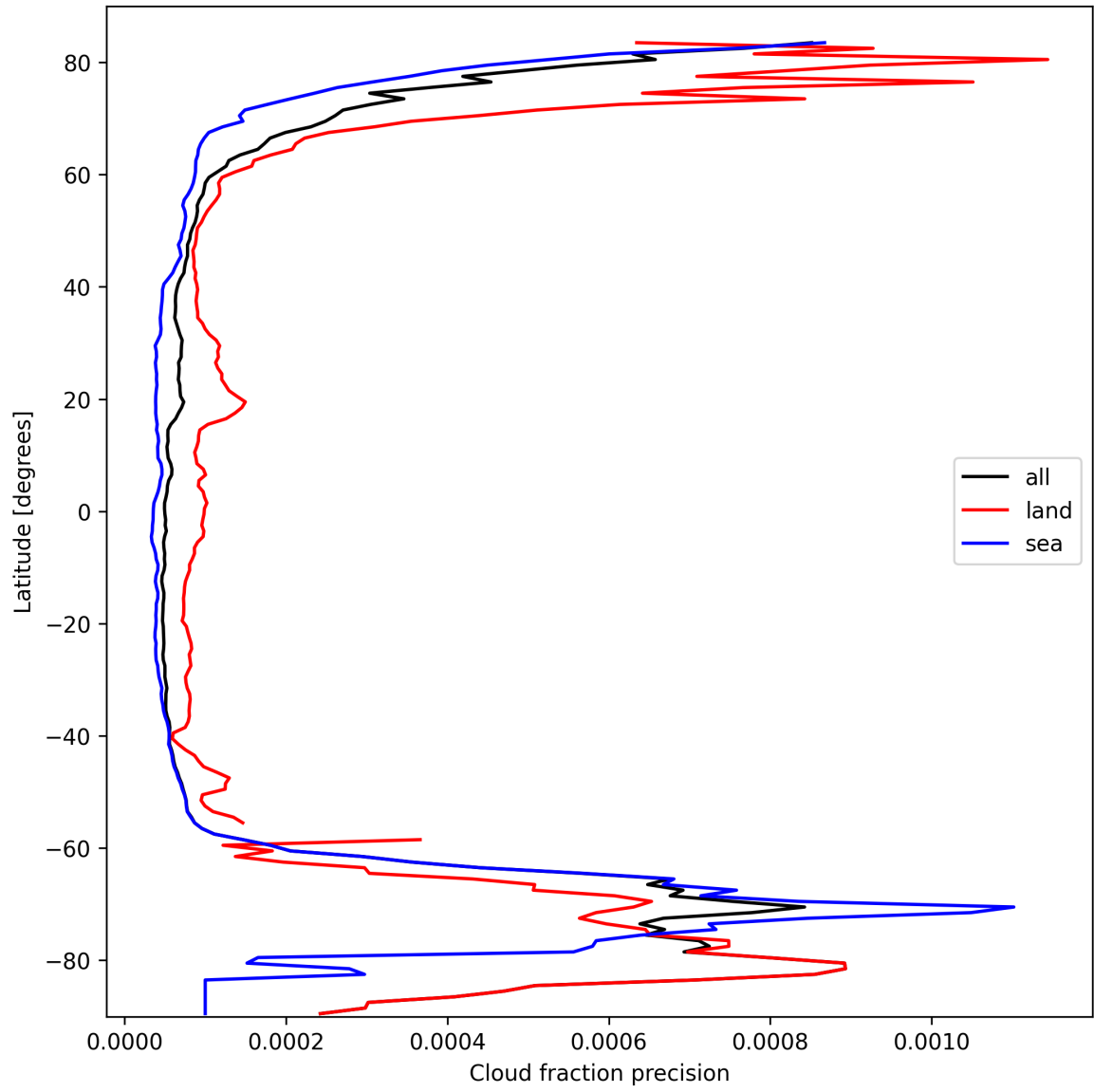
Figure 14: Zonal average of “Cloud fraction precision” for 2025-10-03 to 2025-10-04.
