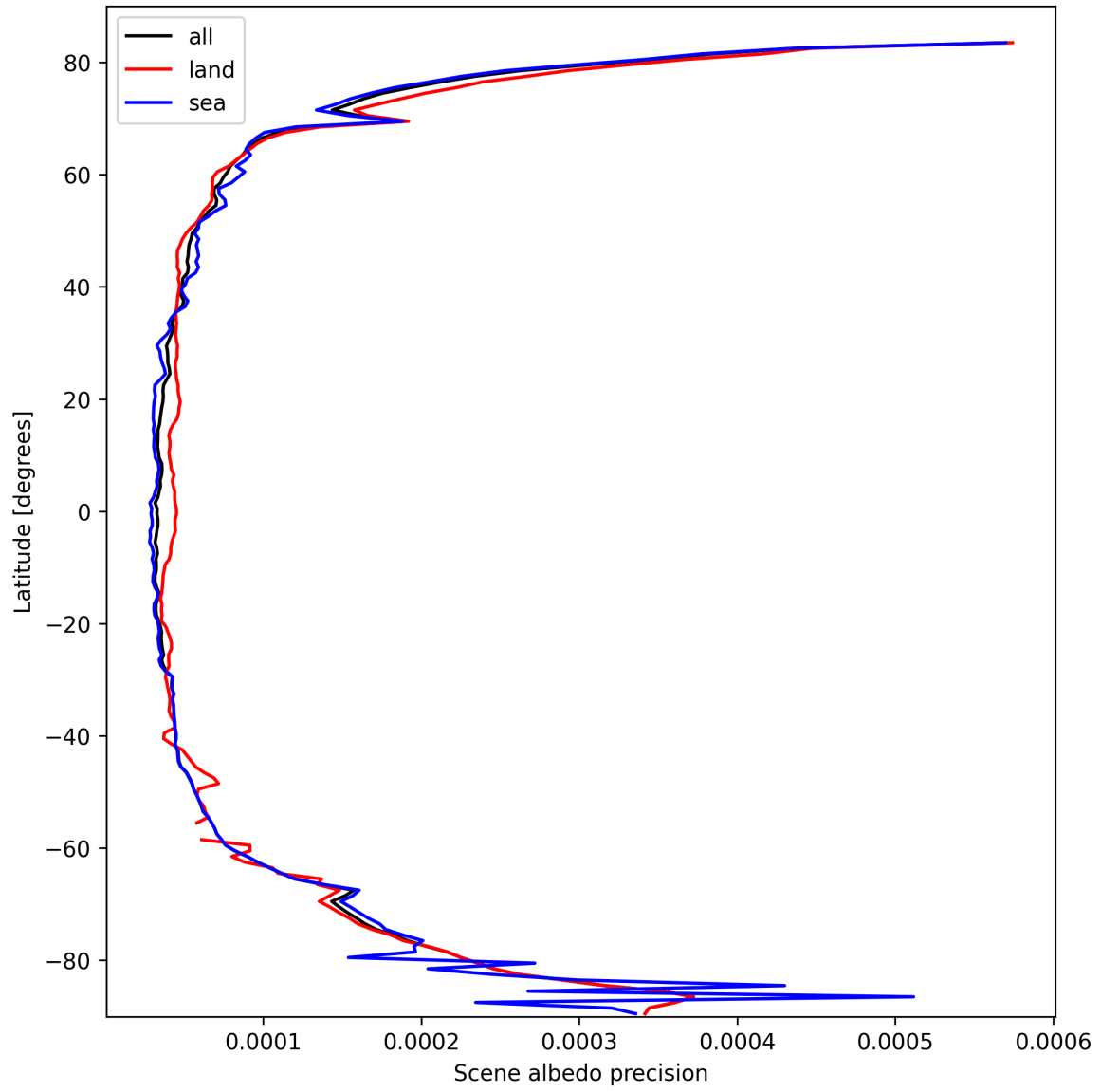
Figure 16: Zonal average of “Scene albedo precision” for 2025-10-03 to 2025-10-04.
