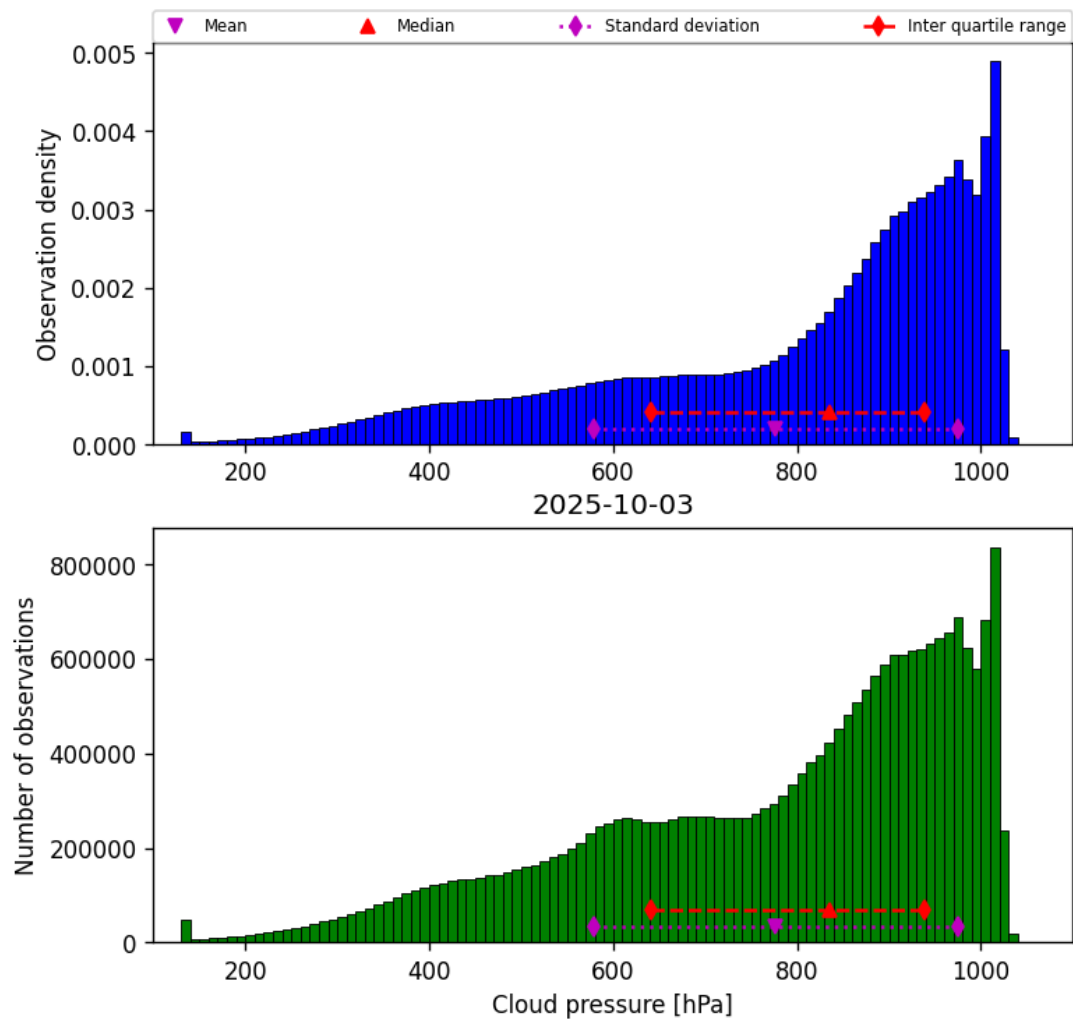
Figure 28: Histogram of “Cloud pressure” for 2025-10-03 to 2025-10-04
