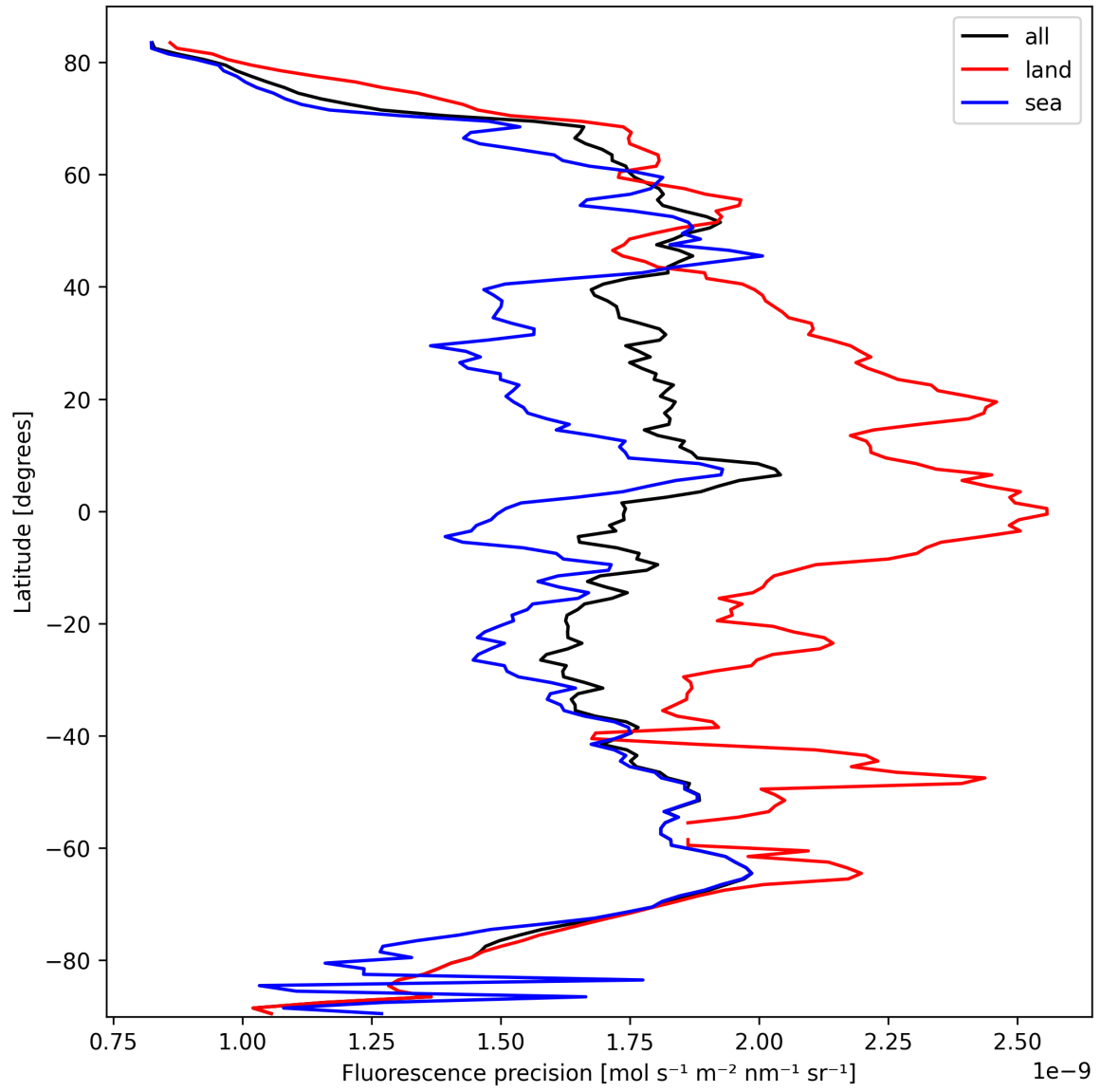
Figure 22: Zonal average of “Fluorescence precision” for 2025-10-03 to 2025-10-04.
