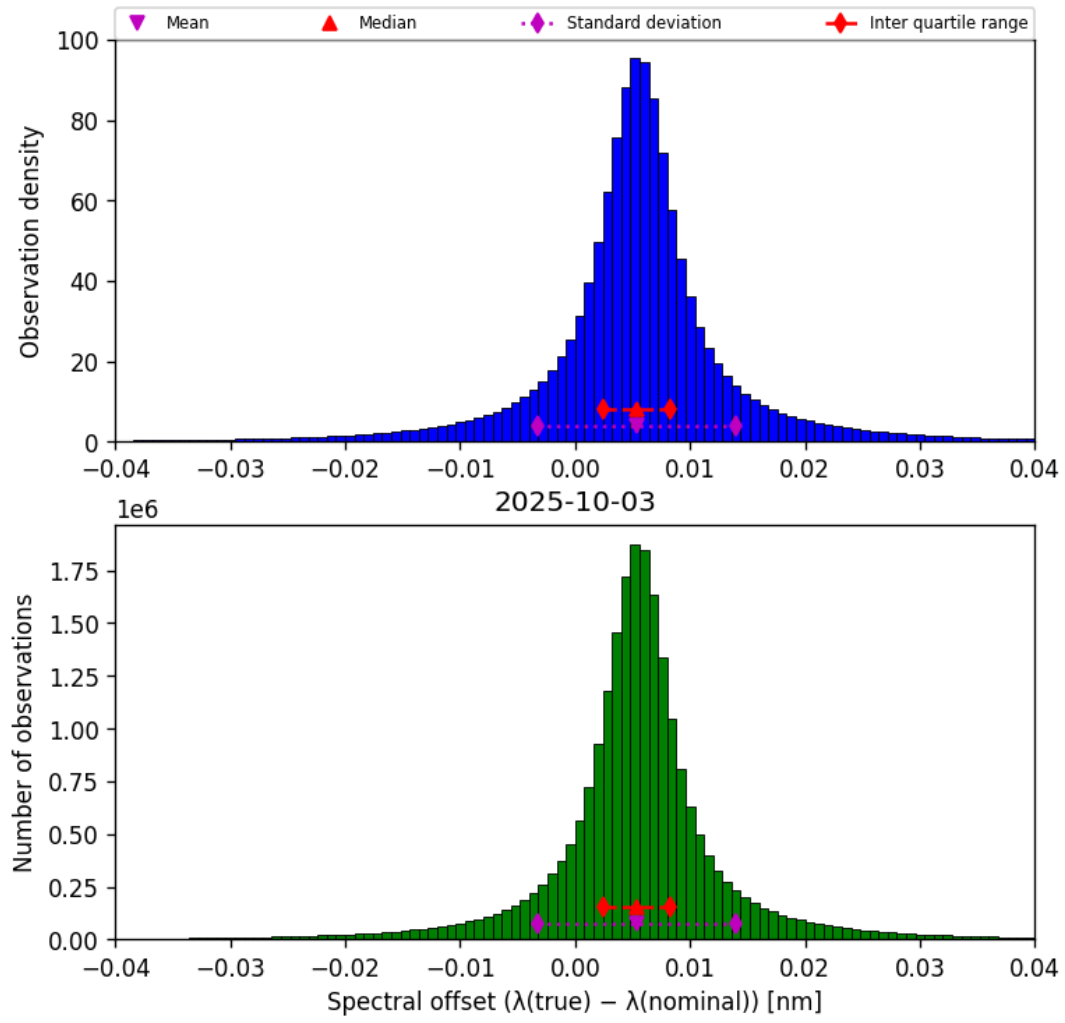
Figure 43: Histogram of “Spectral offset ( \lambda_{\text{true}} - \lambda_{\text{nominal}} )” for 2025-10-03 to 2025-10-04
