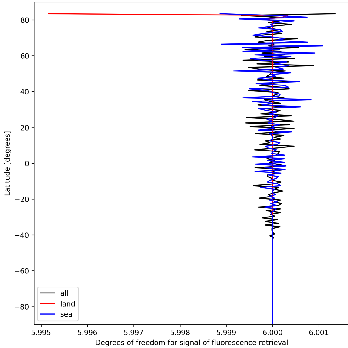
Figure 24: Zonal average of “Degrees of freedom for signal of fluorescence retrieval” for 2025-10-03 to 2025-10-04.
