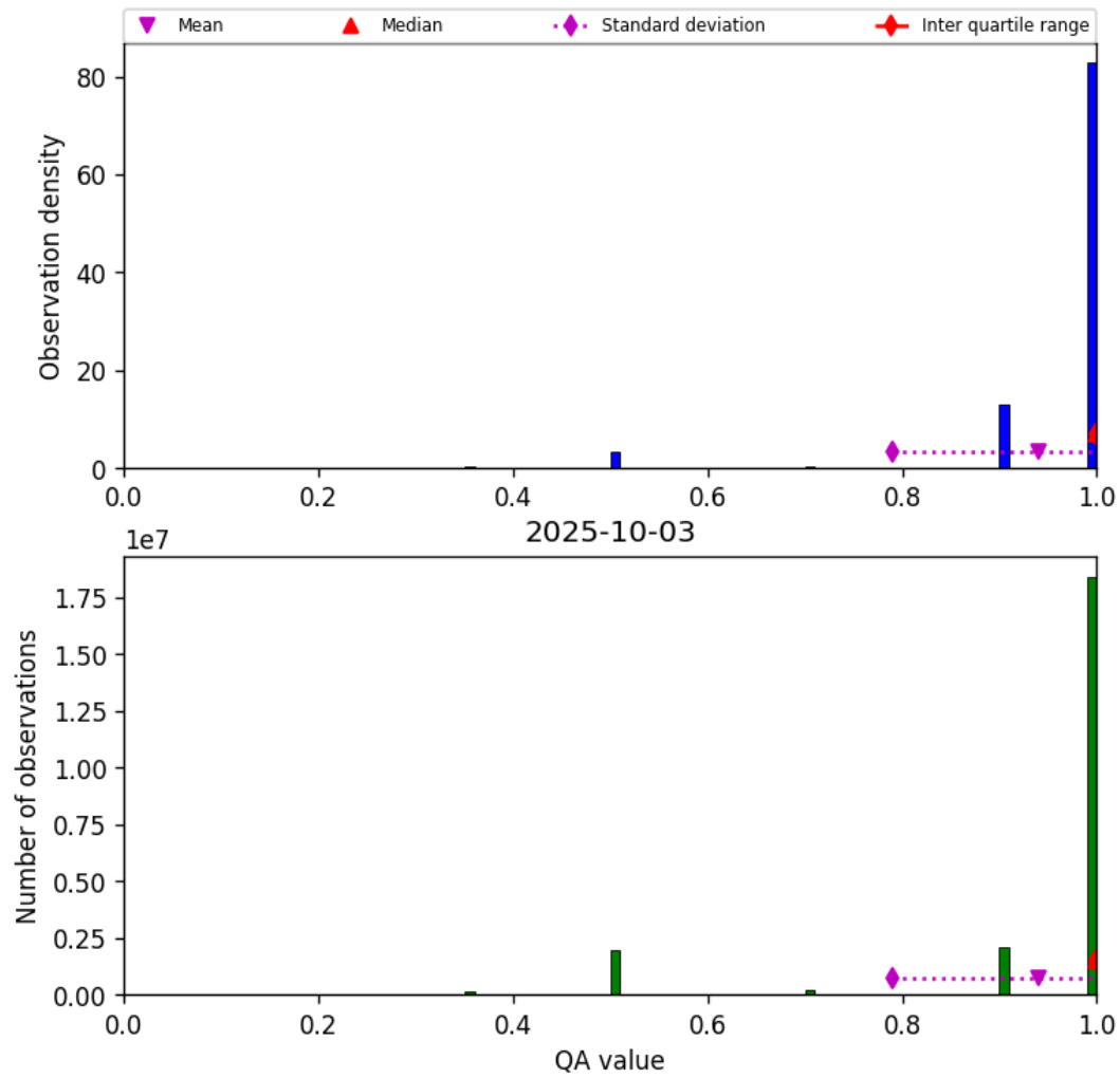
Figure 27: Histogram of “QA value” for 2025-10-03 to 2025-10-04
