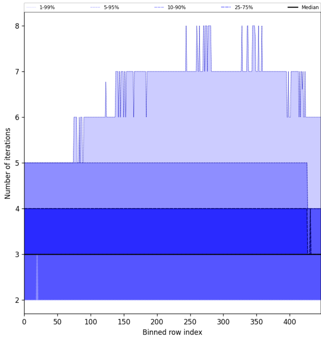
Figure 54: Along track statistics of “Number of iterations” for 2025-10-03 to 2025-10-04
