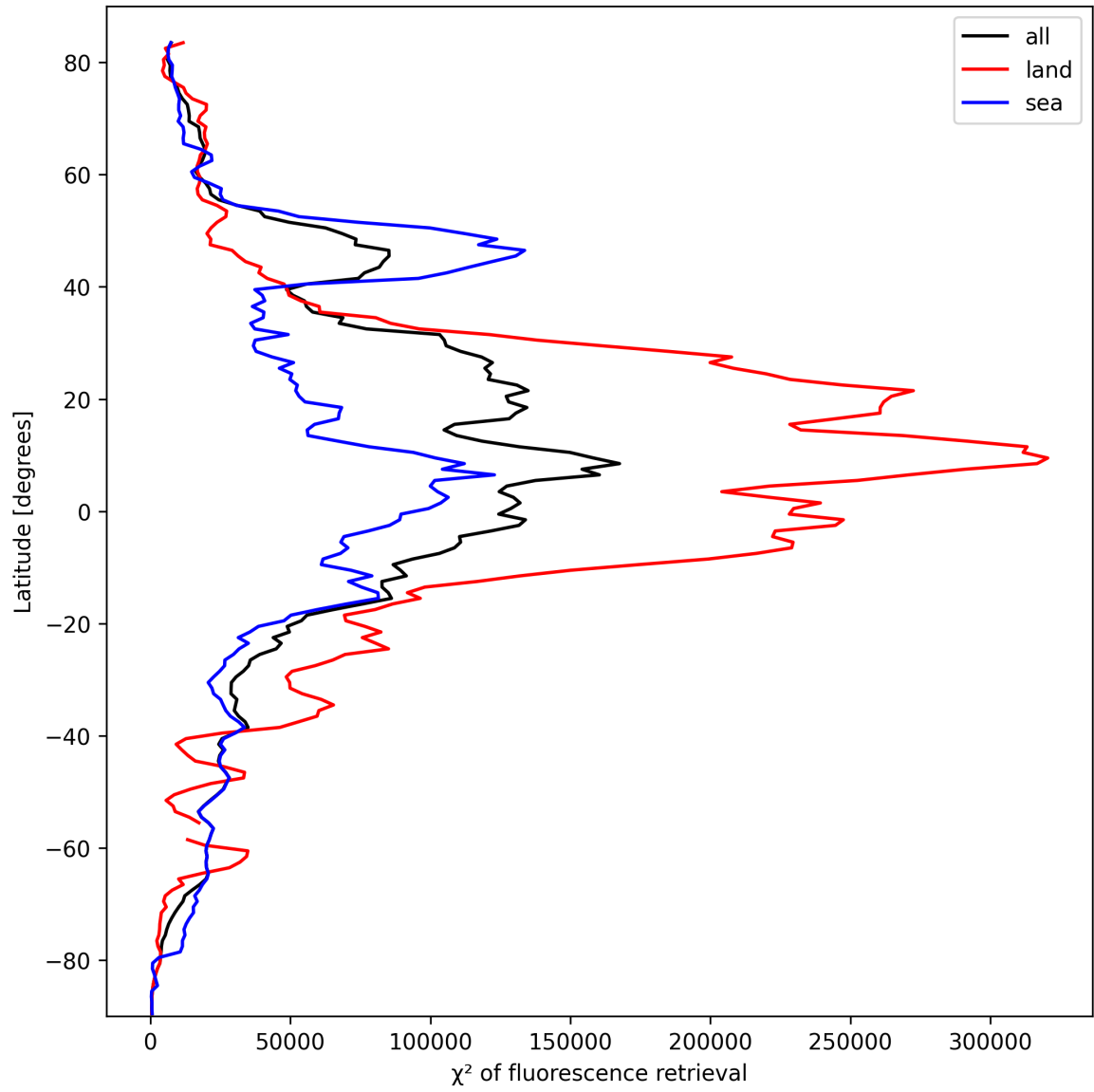
Figure 23: Zonal average of “ \chi^2 of fluorescence retrieval” for 2025-10-03 to 2025-10-04.
