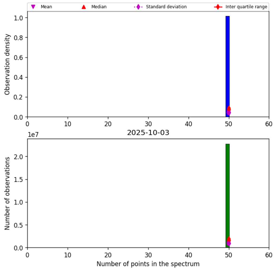
Figure 42: Histogram of “Number of points in the spectrum” for 2025-10-03 to 2025-10-04
