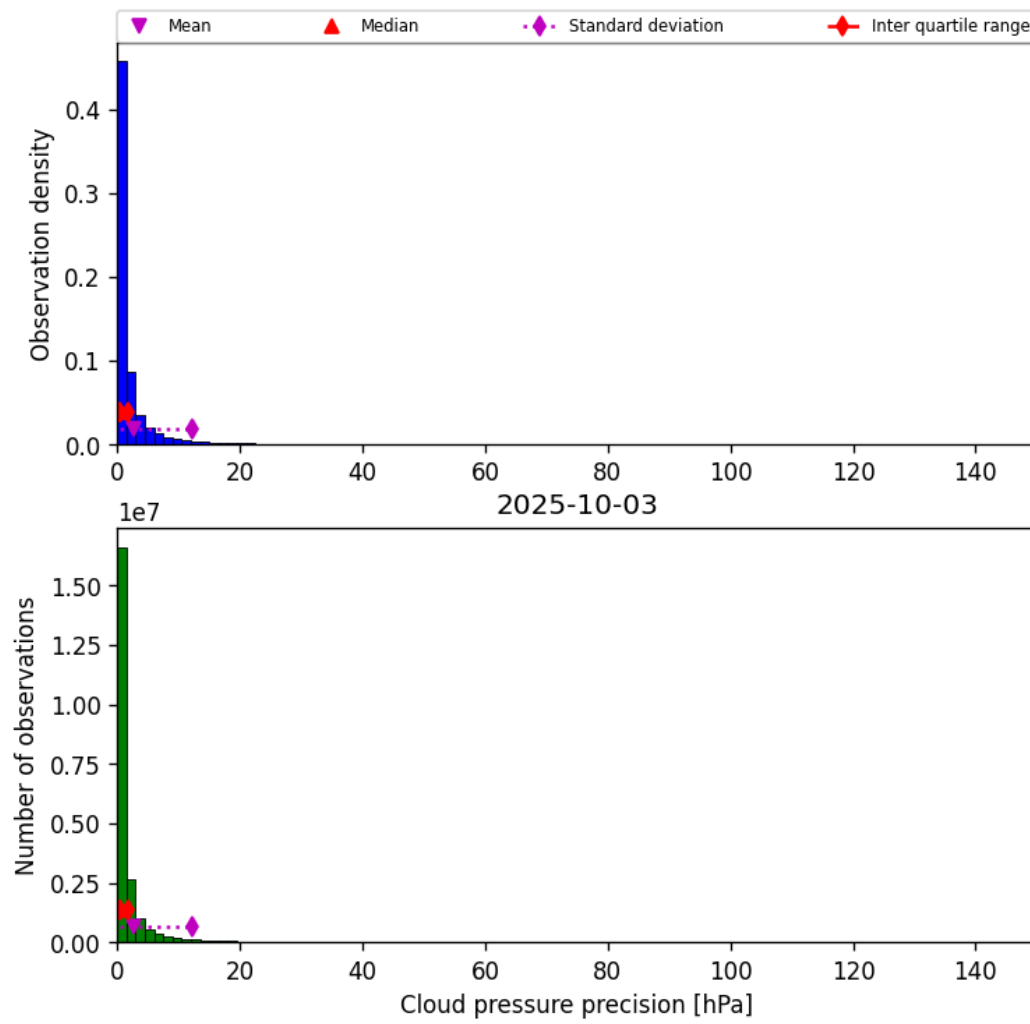
Figure 29: Histogram of “Cloud pressure precision” for 2025-10-03 to 2025-10-04
