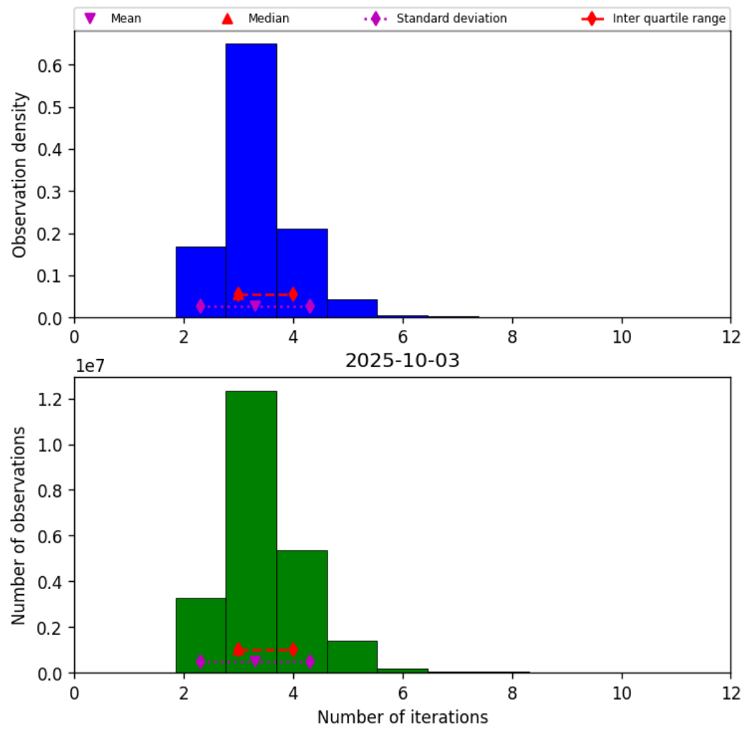
Figure 37: Histogram of “Number of iterations” for 2025-10-03 to 2025-10-04
