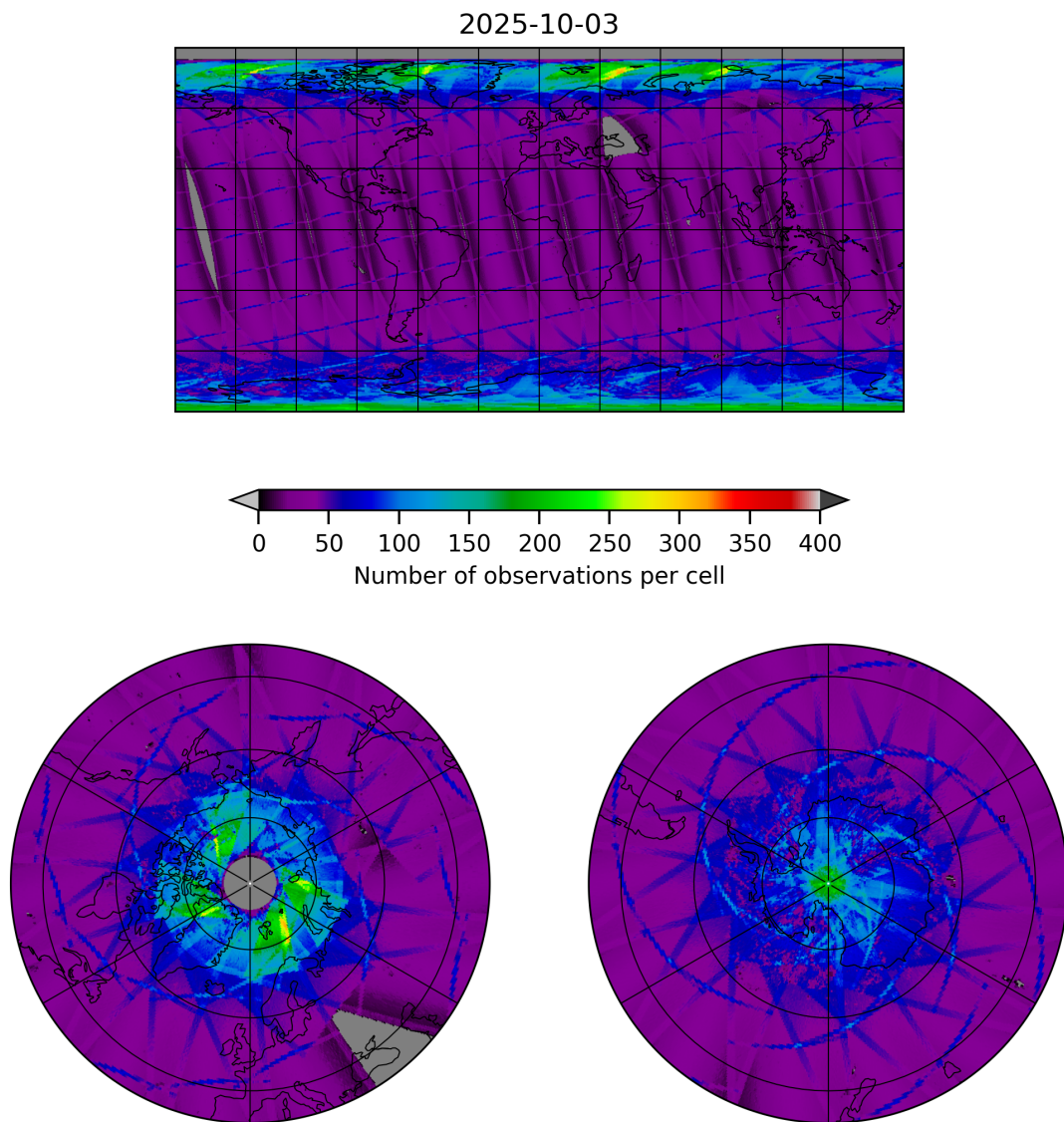
Figure 9: Map of the number of observations for 2025-10-03 to 2025-10-04
