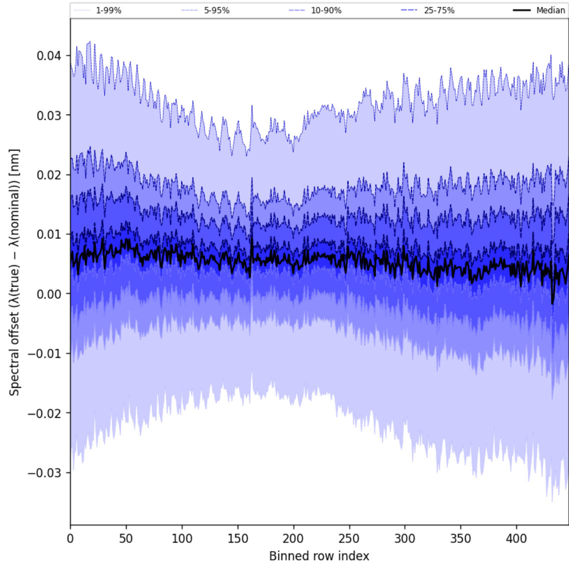
Figure 60: Along track statistics of “Spectral offset ( \lambda_{\text{true}} - \lambda_{\text{nominal}} )” for 2025-10-03 to 2025-10-04
