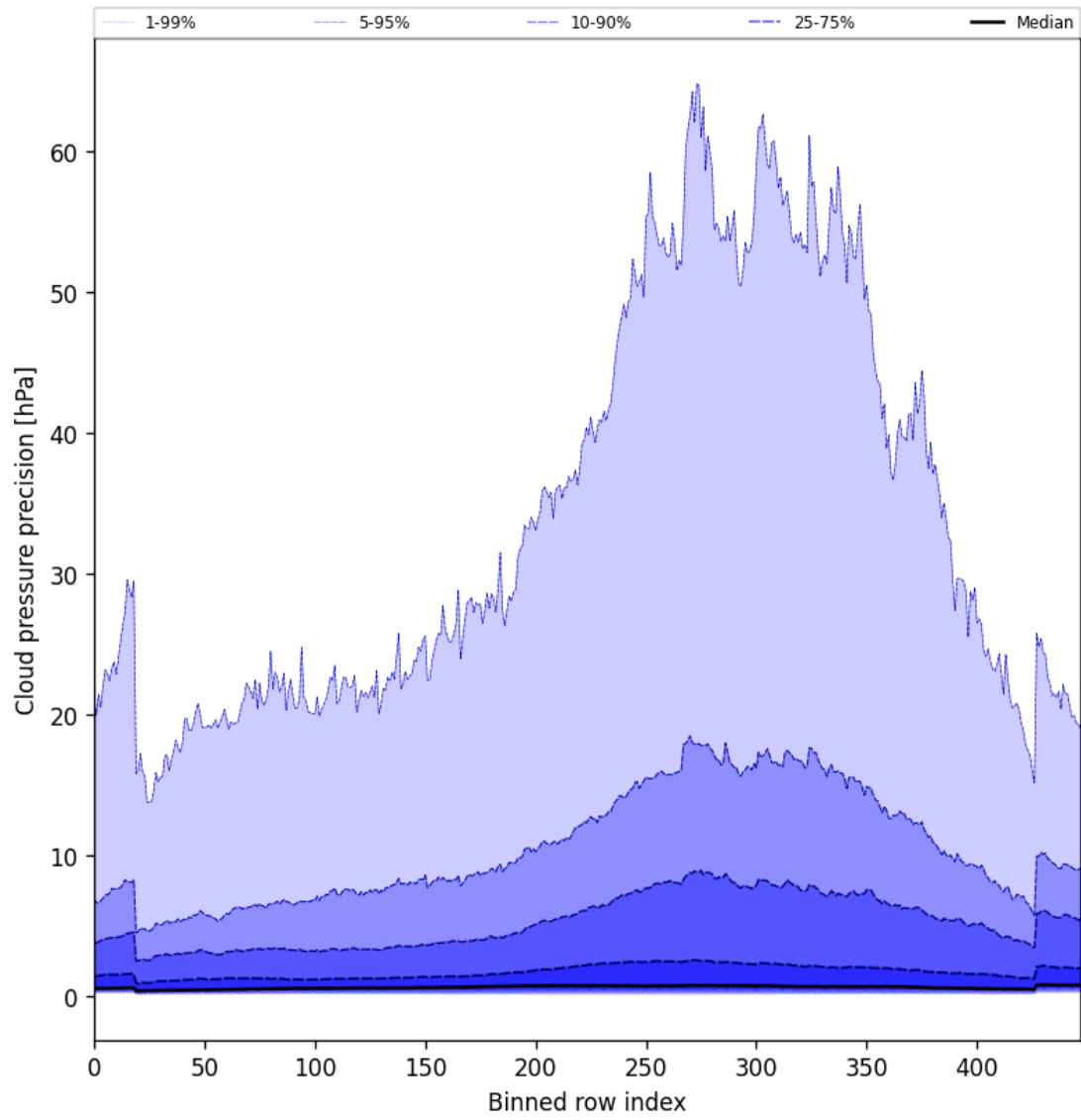
Figure 46: Along track statistics of “Cloud pressure precision” for 2025-10-03 to 2025-10-04
