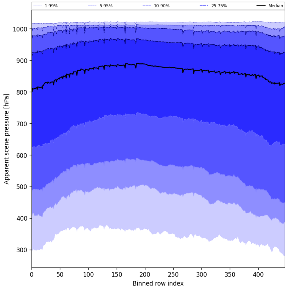
Figure 51: Along track statistics of “Apparent scene pressure” for 2025-10-03 to 2025-10-04
