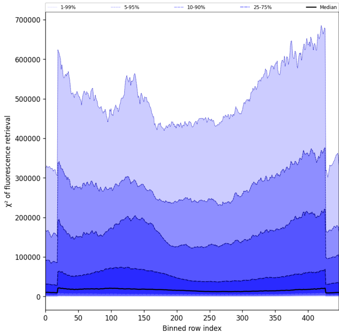
Figure 57: Along track statistics of “ \chi^2 of fluorescence retrieval” for 2025-10-04 to 2025-10-04
