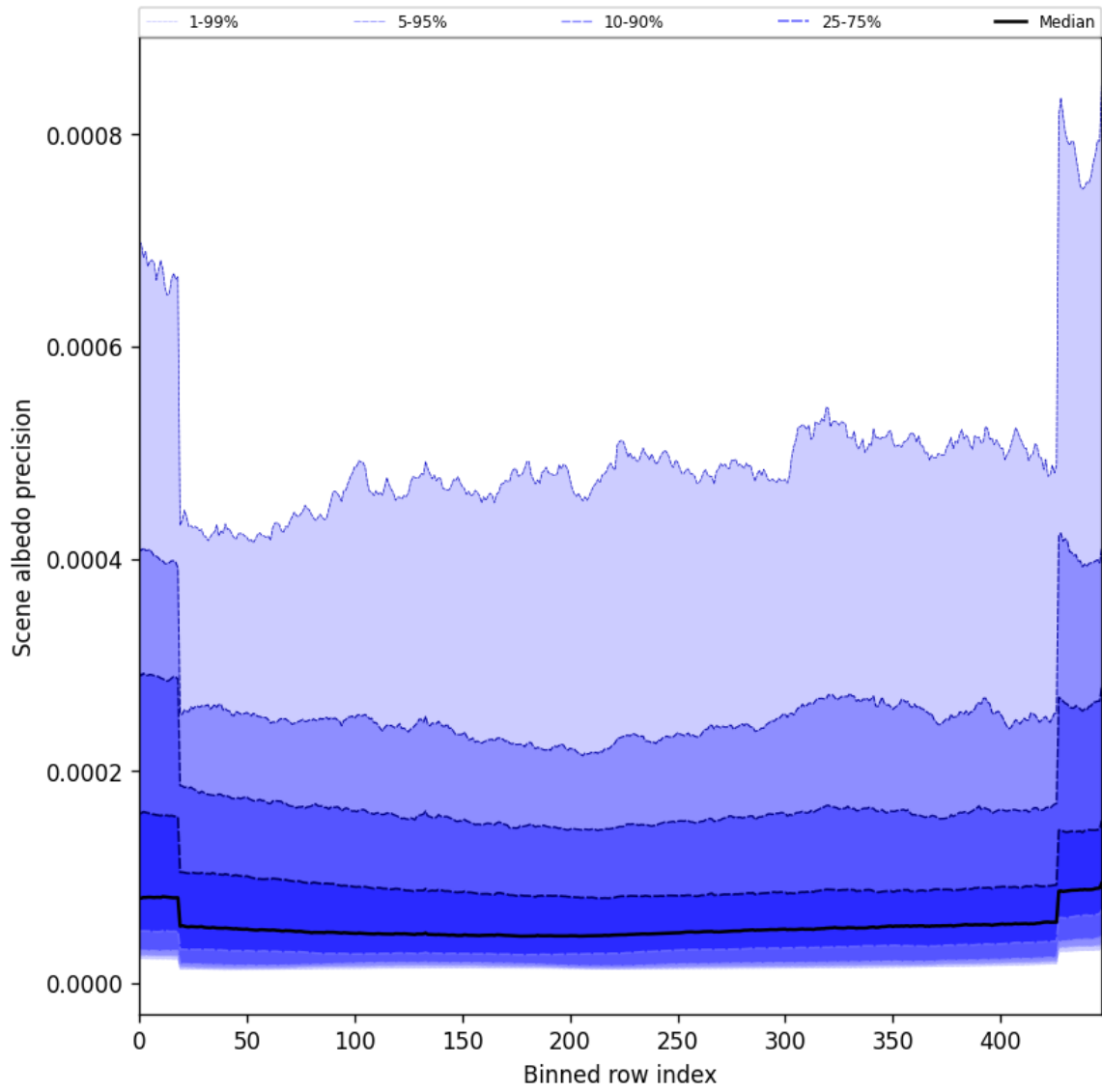
Figure 50: Along track statistics of “Scene albedo precision” for 2025-10-04 to 2025-10-04
