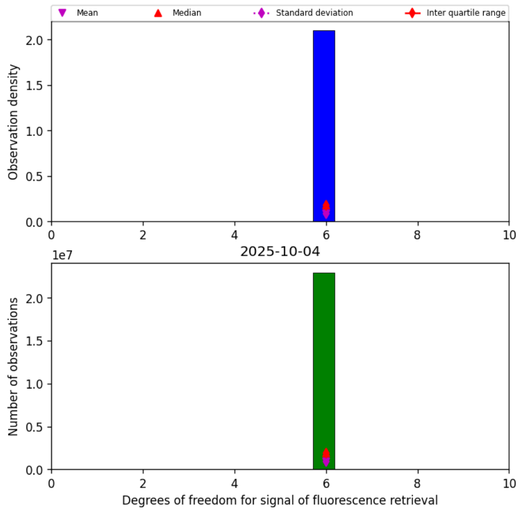
Figure 41: Histogram of “Degrees of freedom for signal of fluorescence retrieval” for 2025-10-04 to 2025-10-04
