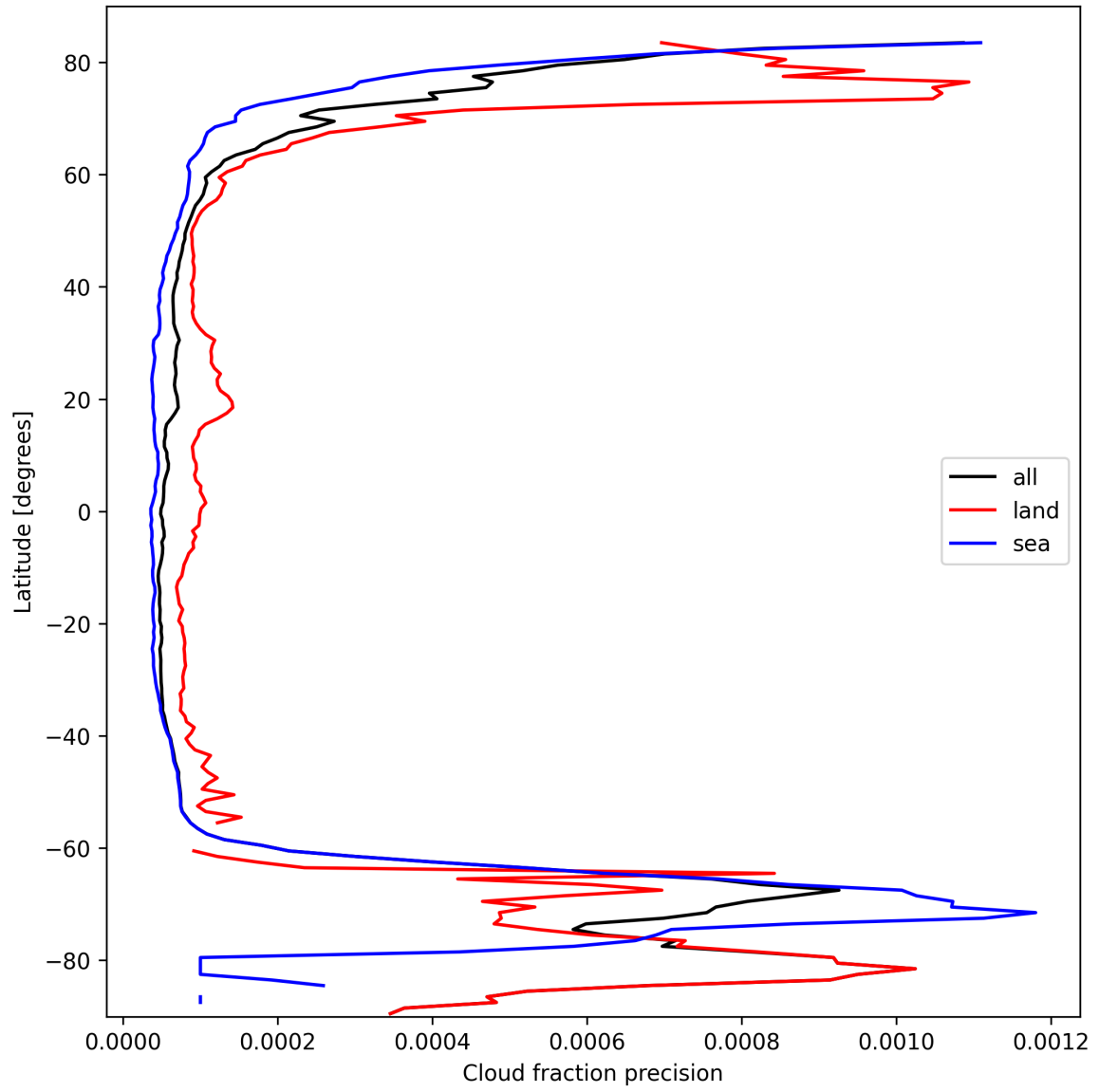
Figure 14: Zonal average of “Cloud fraction precision” for 2025-10-04 to 2025-10-04.
