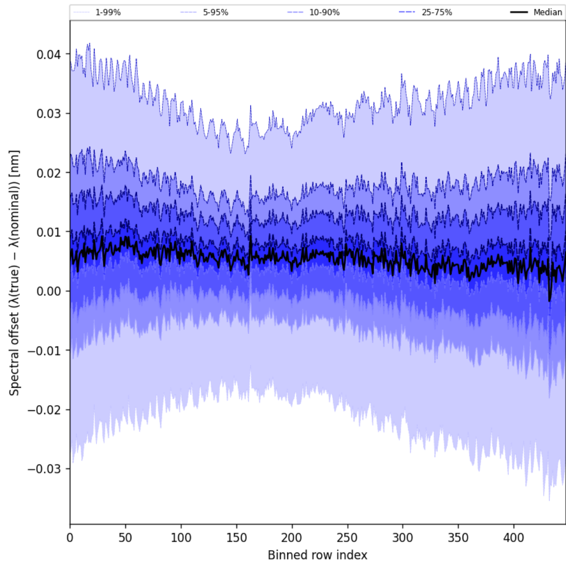
Figure 60: Along track statistics of “Spectral offset ( \lambda_{\text{true}} - \lambda_{\text{nominal}} )” for 2025-10-04 to 2025-10-04
