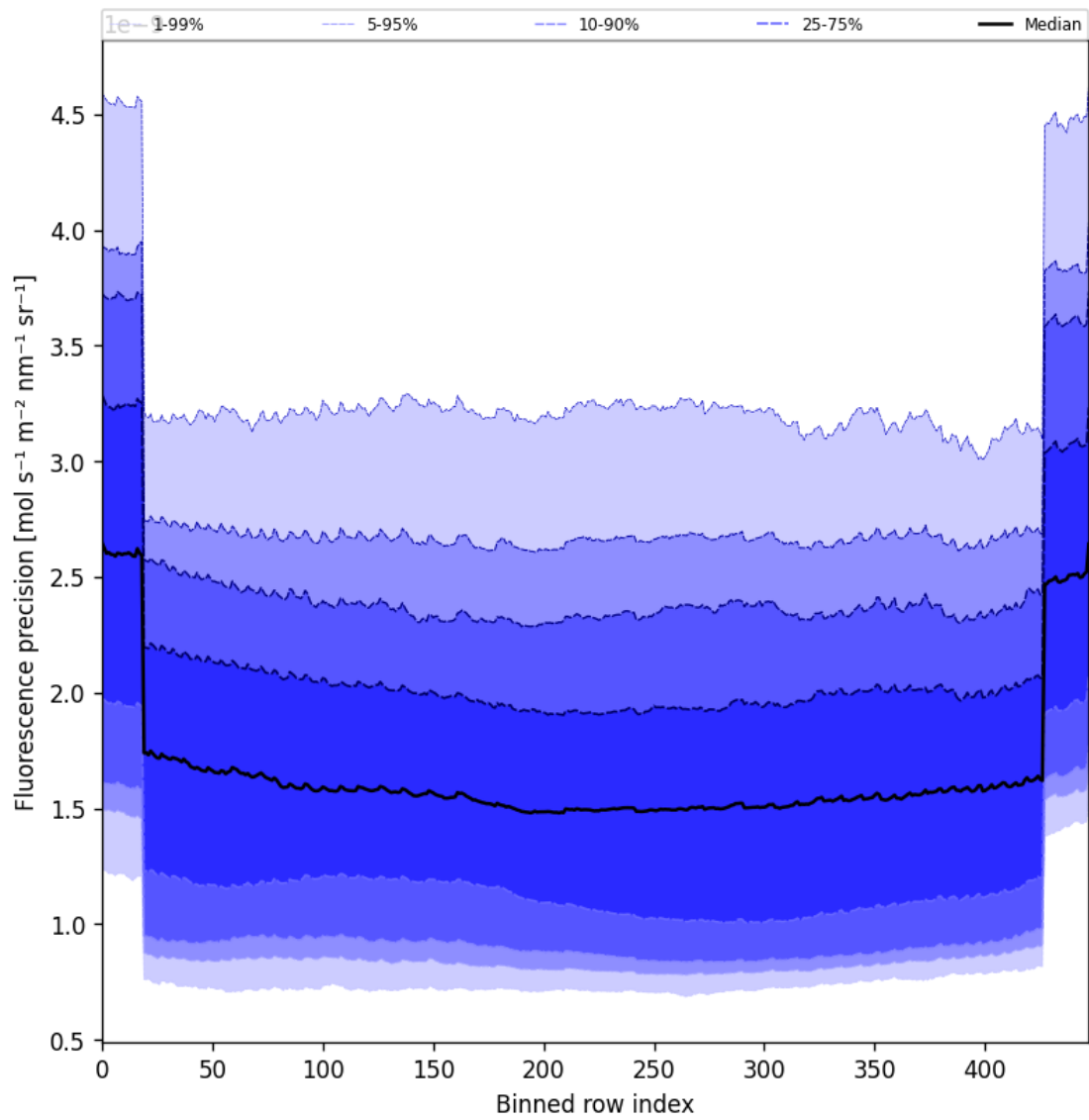
Figure 56: Along track statistics of “Fluorescence precision” for 2025-10-04 to 2025-10-04
