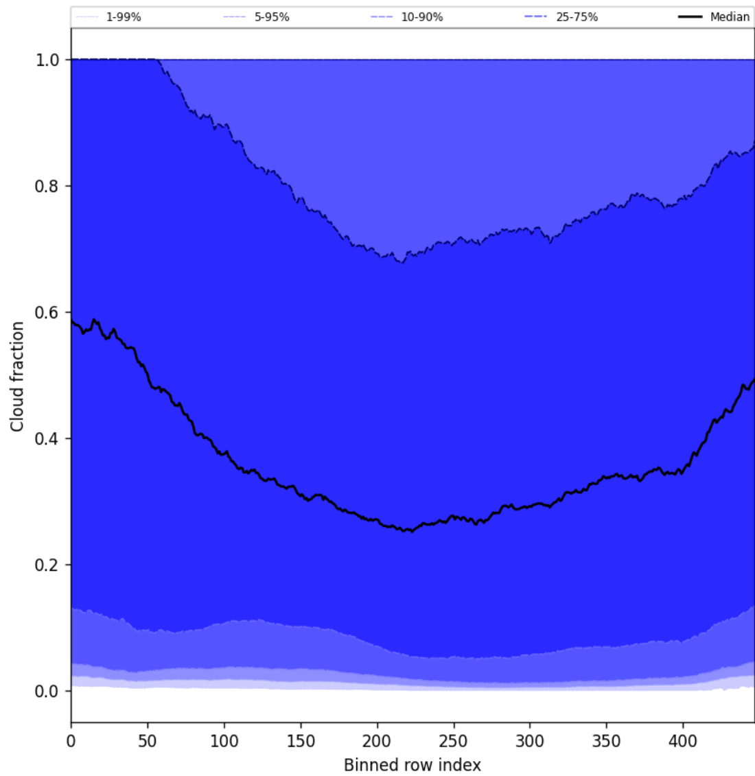
Figure 47: Along track statistics of “Cloud fraction” for 2025-10-04 to 2025-10-04
