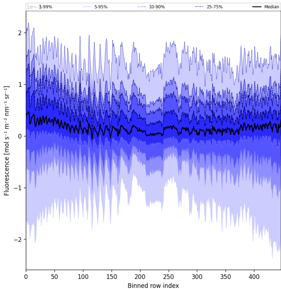
Figure 55: Along track statistics of “Fluorescence” for 2025-10-04 to 2025-10-04
