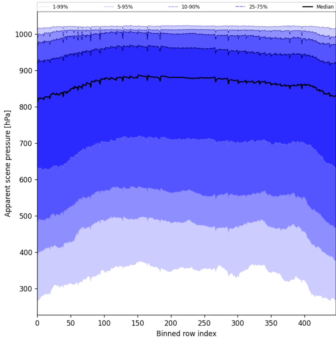
Figure 51: Along track statistics of “Apparent scene pressure” for 2025-10-04 to 2025-10-04
