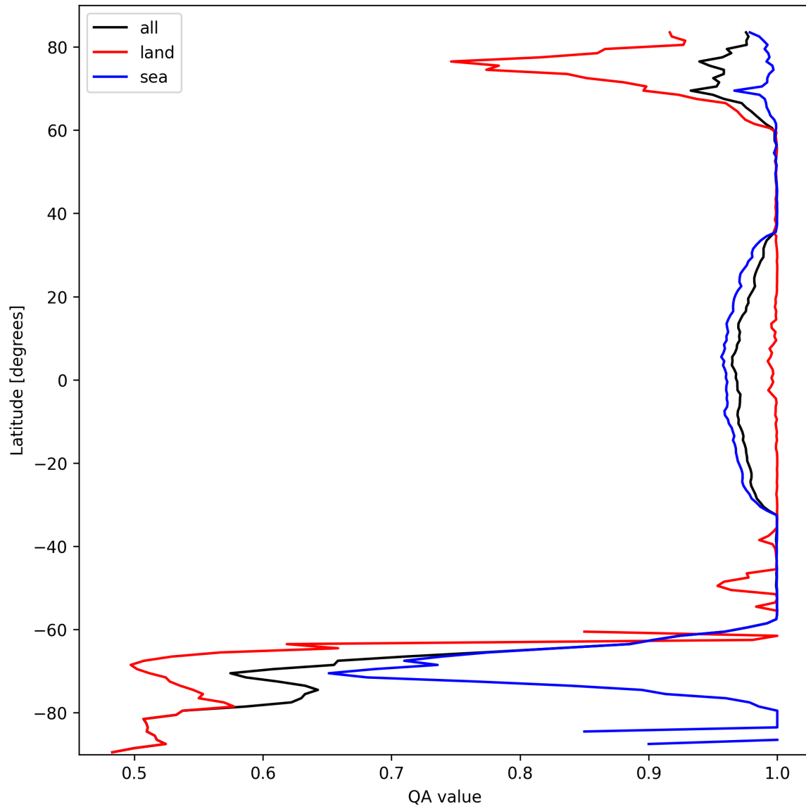
Figure 10: Zonal average of “QA value” for 2025-10-04 to 2025-10-04.
