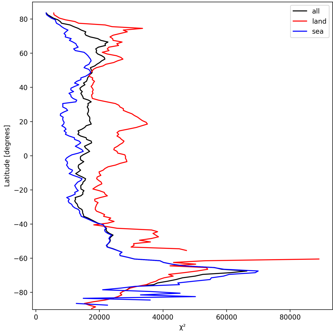
Figure 19: Zonal average of “ \chi^2 ” for 2025-10-04 to 2025-10-04.
