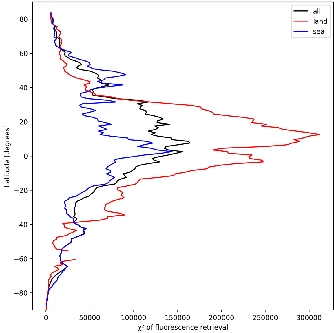
Figure 23: Zonal average of “ \chi^2 of fluorescence retrieval” for 2025-10-04 to 2025-10-04.
