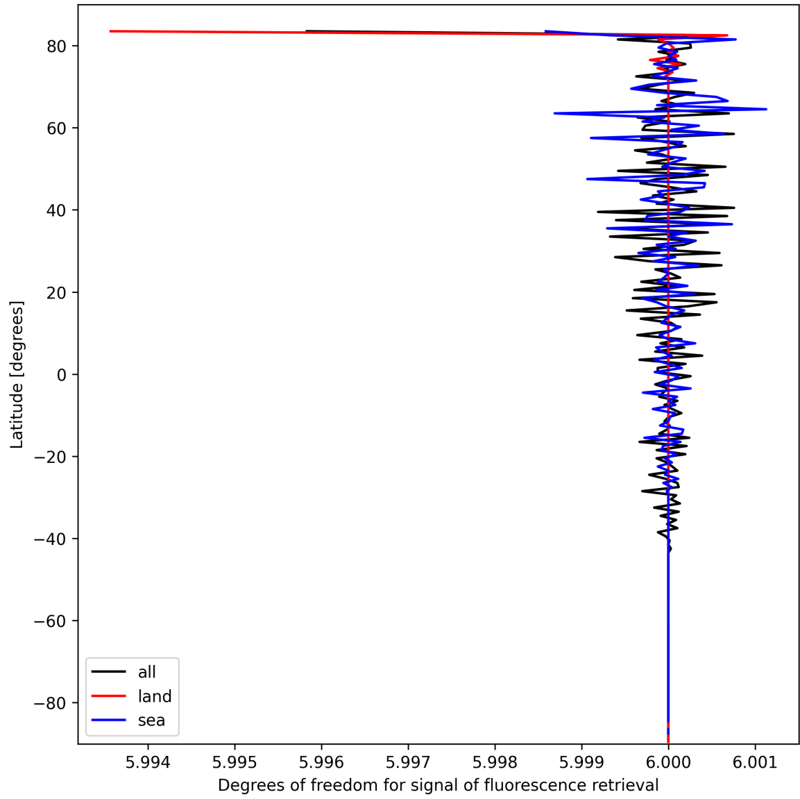
Figure 24: Zonal average of “Degrees of freedom for signal of fluorescence retrieval” for 2025-10-04 to 2025-10-04.
