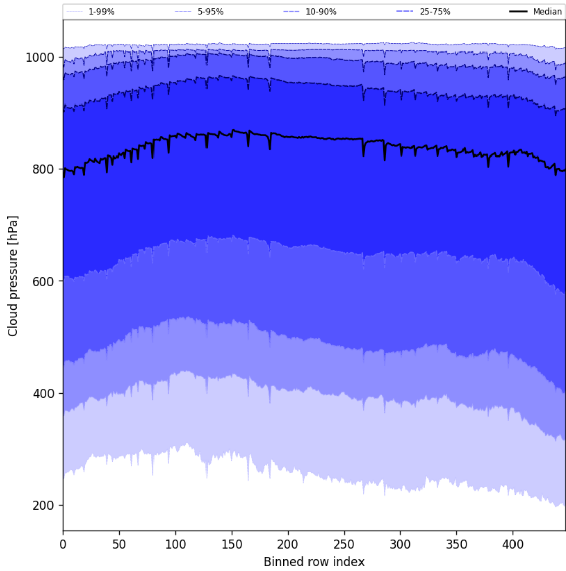
Figure 45: Along track statistics of “Cloud pressure” for 2025-10-04 to 2025-10-04
