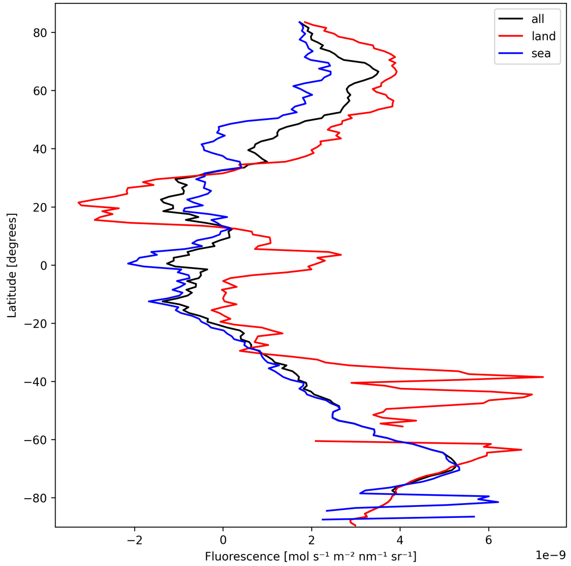
Figure 21: Zonal average of “Fluorescence” for 2025-10-04 to 2025-10-04.
