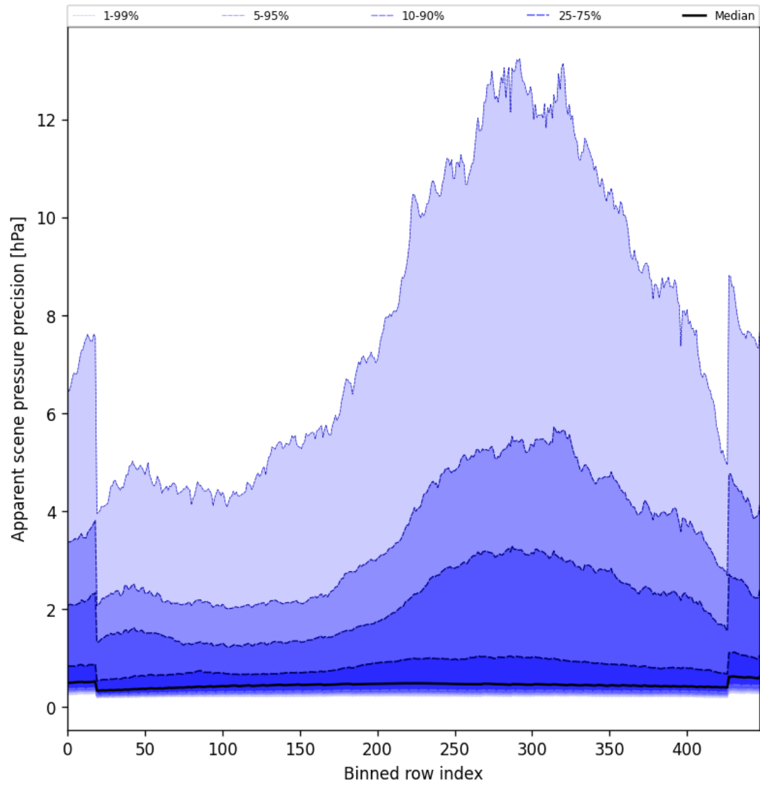
Figure 52: Along track statistics of “Apparent scene pressure precision” for 2025-10-04 to 2025-10-04
