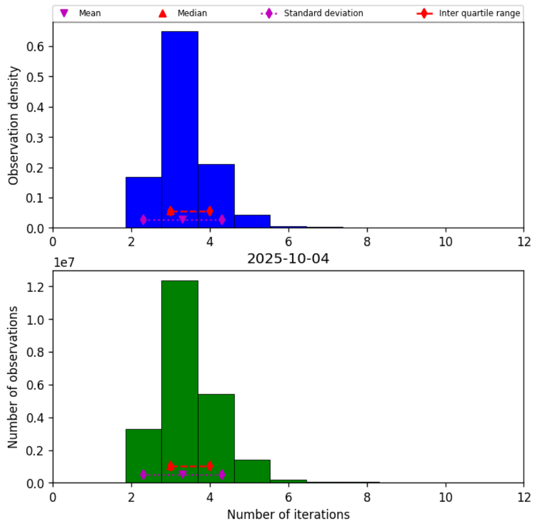
Figure 37: Histogram of “Number of iterations” for 2025-10-04 to 2025-10-04
