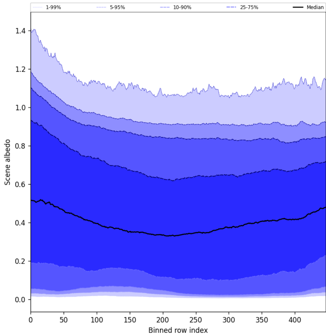
Figure 49: Along track statistics of “Scene albedo” for 2025-10-04 to 2025-10-04
