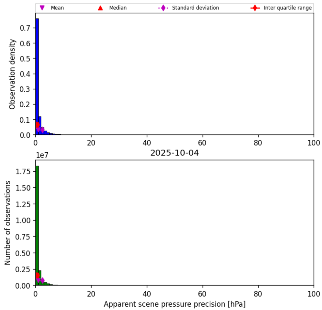
Figure 35: Histogram of “Apparent scene pressure precision” for 2025-10-04 to 2025-10-04
