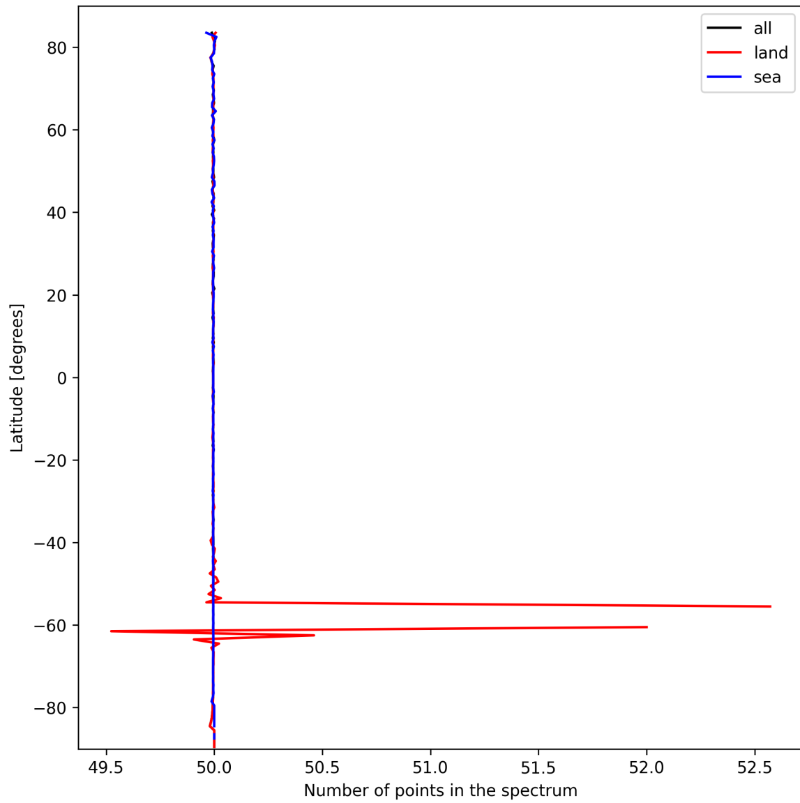
Figure 25: Zonal average of “Number of points in the spectrum” for 2025-10-04 to 2025-10-04.
