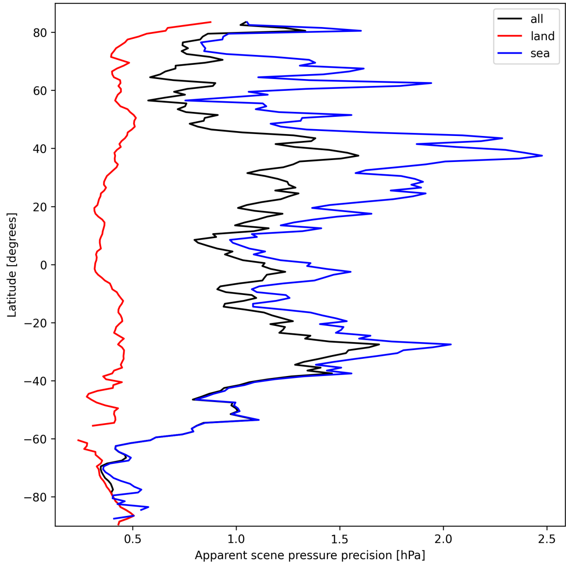
Figure 18: Zonal average of “Apparent scene pressure precision” for 2025-10-04 to 2025-10-04.
