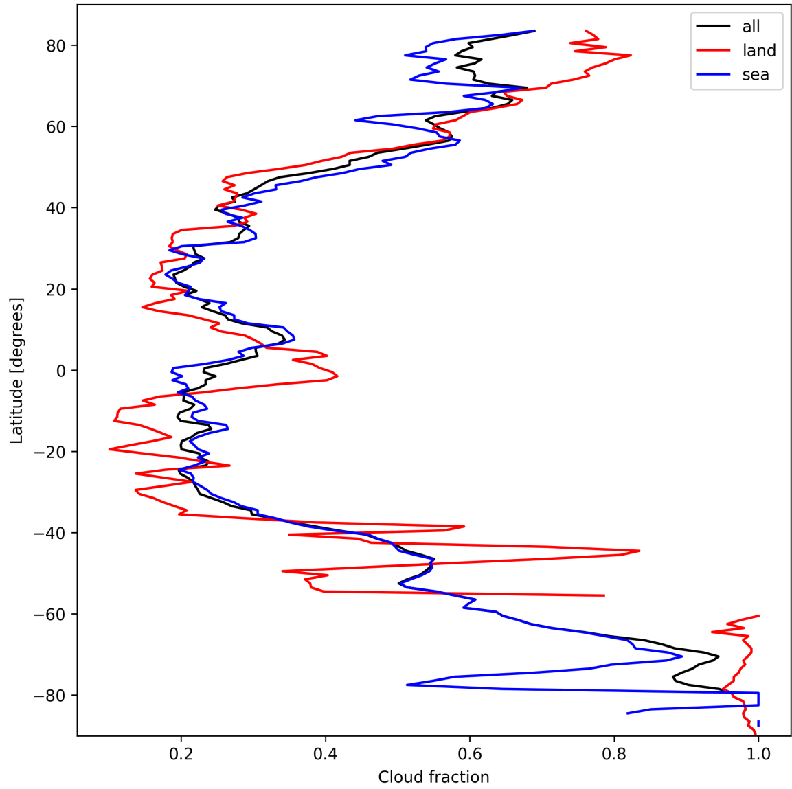
Figure 13: Zonal average of “Cloud fraction” for 2025-10-04 to 2025-10-04.
