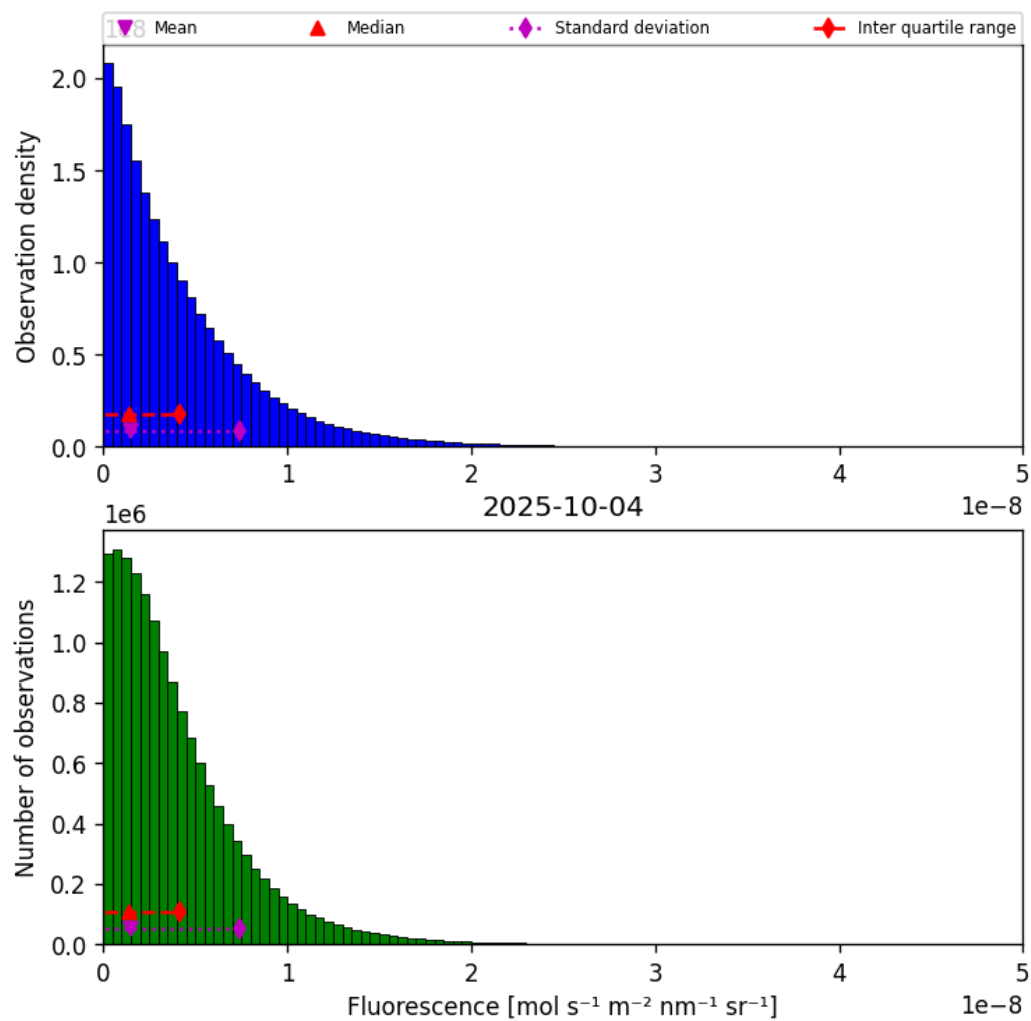
Figure 38: Histogram of “Fluorescence” for 2025-10-04 to 2025-10-04
