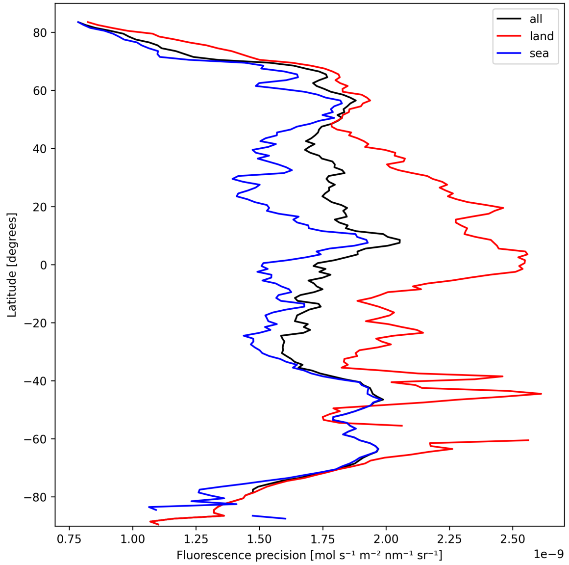
Figure 22: Zonal average of “Fluorescence precision” for 2025-10-04 to 2025-10-04.
