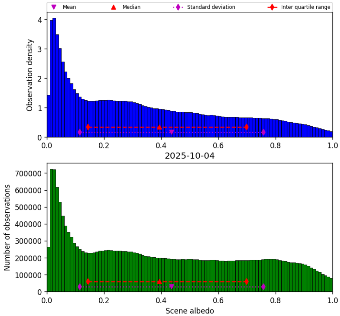
Figure 32: Histogram of “Scene albedo” for 2025-10-04 to 2025-10-04
