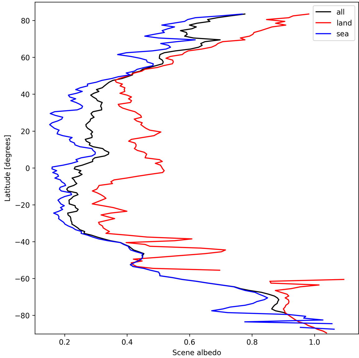
Figure 15: Zonal average of “Scene albedo” for 2025-10-04 to 2025-10-04.
