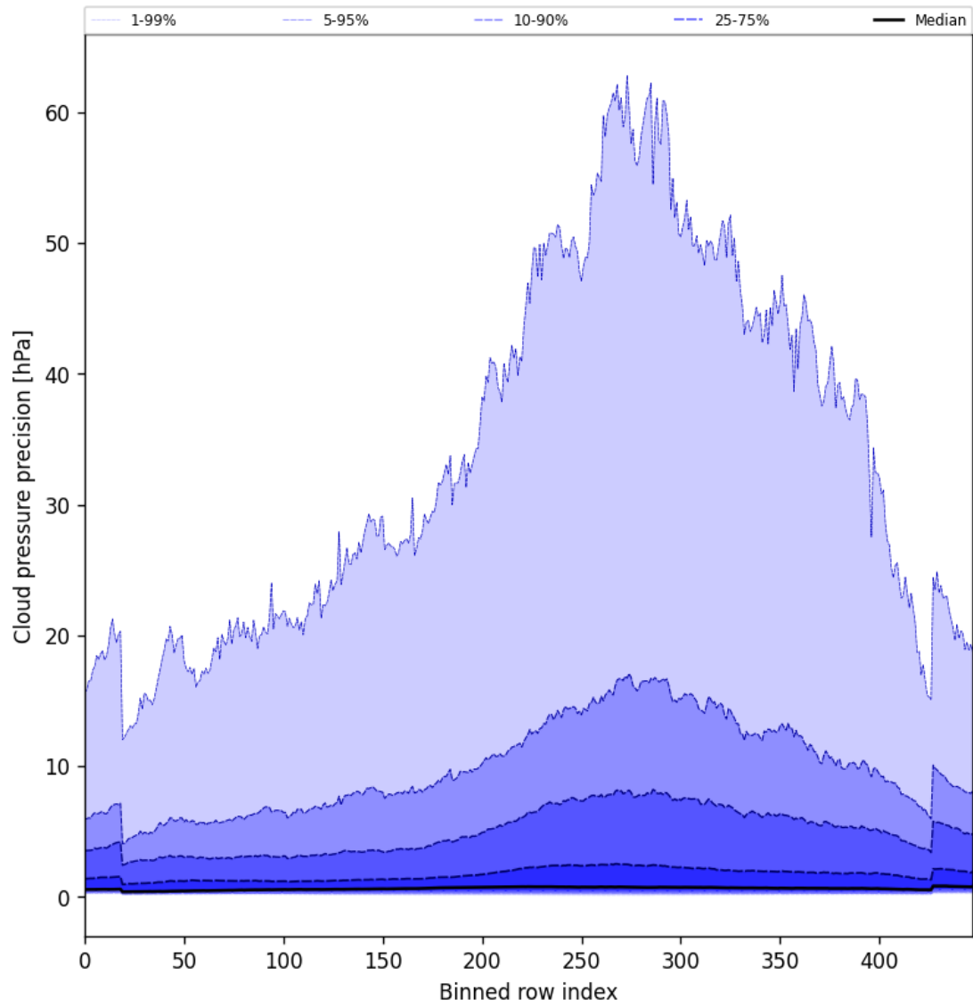
Figure 46: Along track statistics of “Cloud pressure precision” for 2025-10-04 to 2025-10-04
