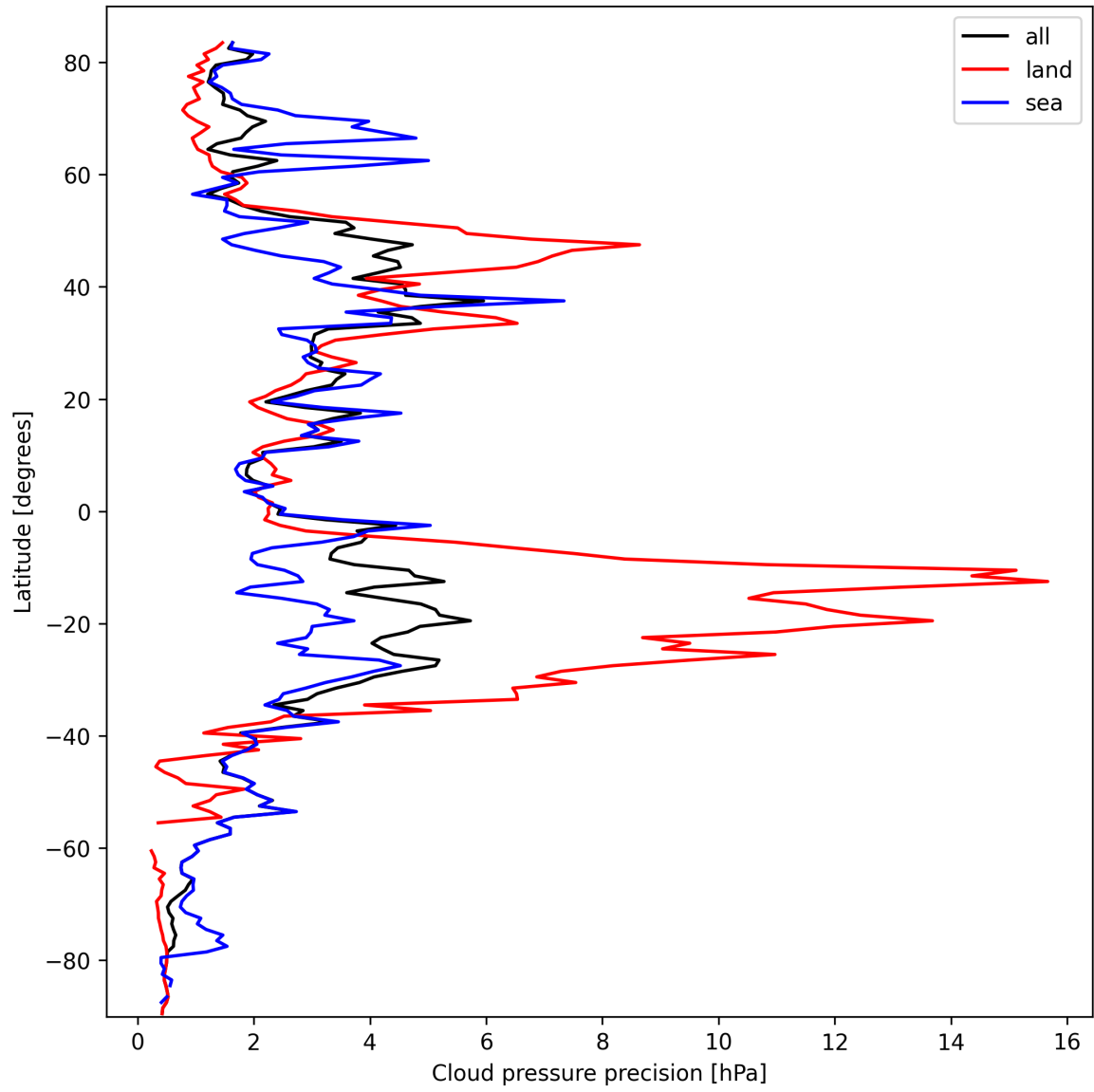
Figure 12: Zonal average of "Cloud pressure precision" for 2025-10-04 to 2025-10-04.
