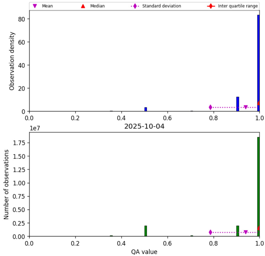
Figure 27: Histogram of “QA value” for 2025-10-04 to 2025-10-04
