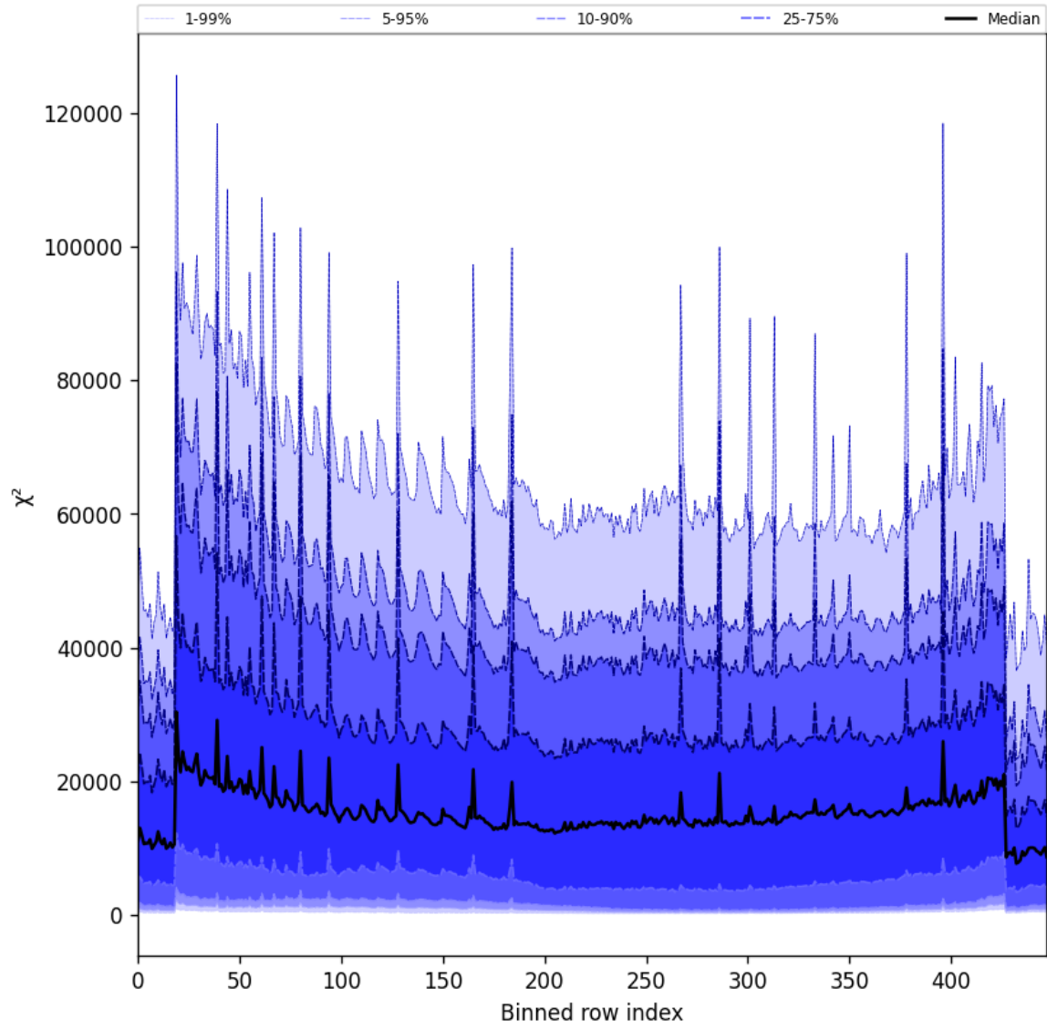
Figure 53: Along track statistics of “ \chi^2 ” for 2025-10-04 to 2025-10-04
