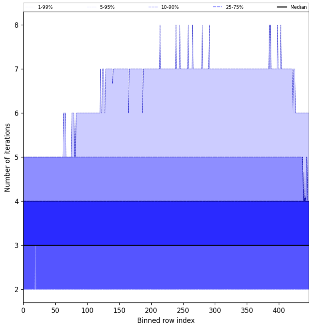
Figure 54: Along track statistics of “Number of iterations” for 2025-10-04 to 2025-10-04
