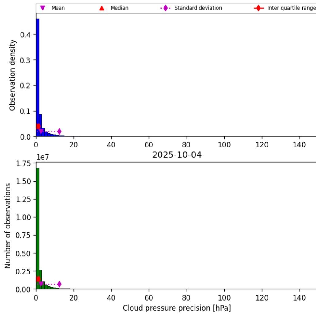
Figure 29: Histogram of “Cloud pressure precision” for 2025-10-04 to 2025-10-04
