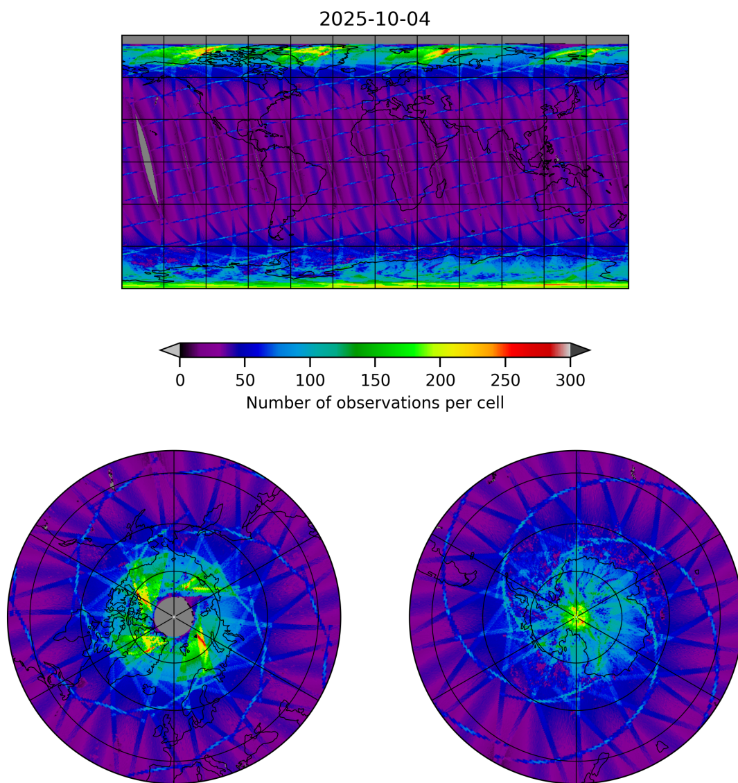
Figure 9: Map of the number of observations for 2025-10-04 to 2025-10-04
