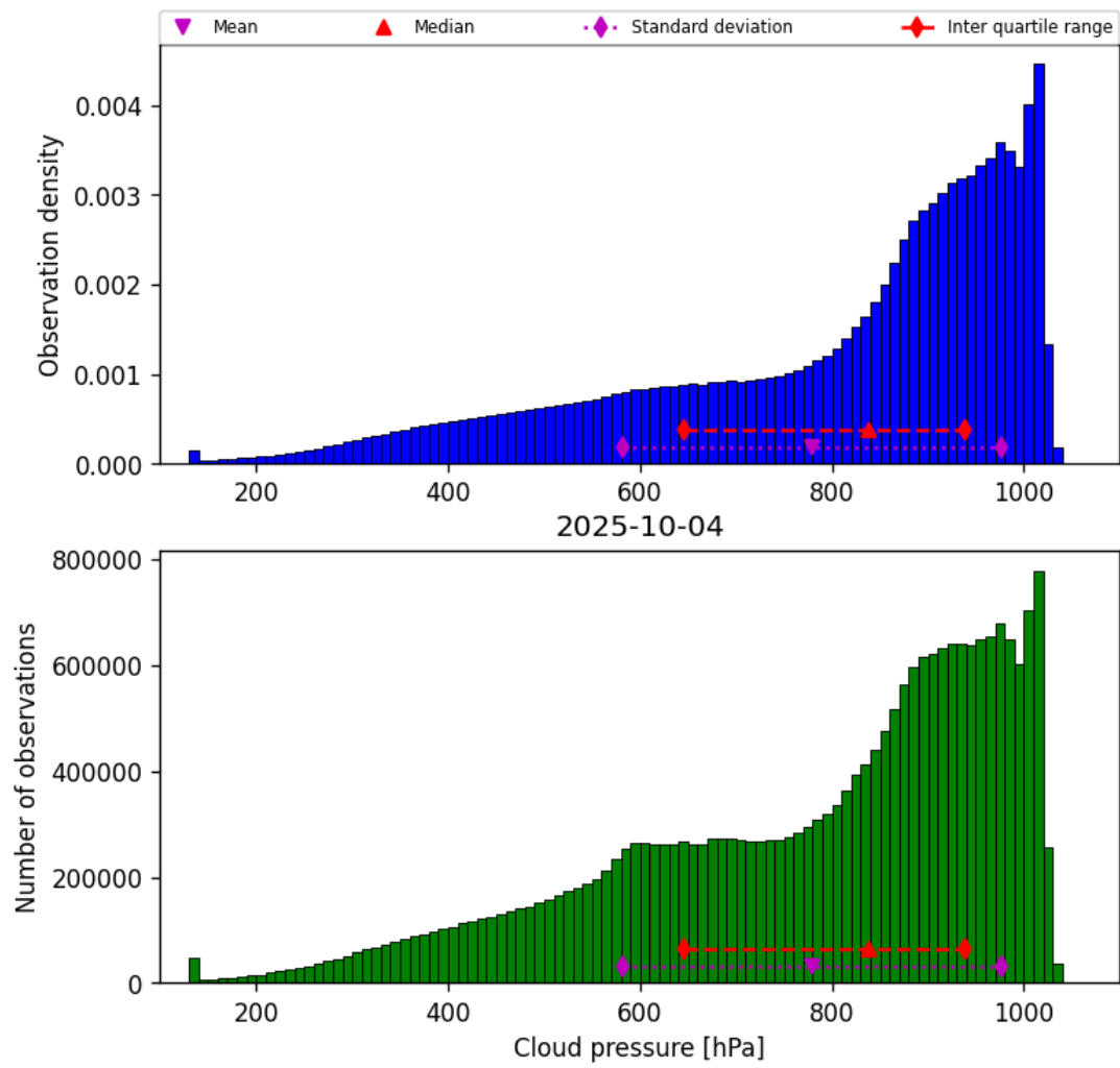
Figure 28: Histogram of “Cloud pressure” for 2025-10-04 to 2025-10-04
