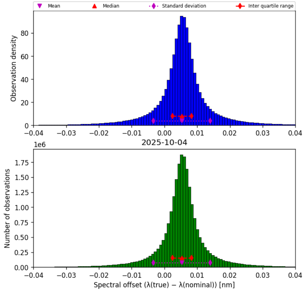
Figure 43: Histogram of “Spectral offset ( \lambda_{\text{true}} - \lambda_{\text{nominal}} )” for 2025-10-04 to 2025-10-04
