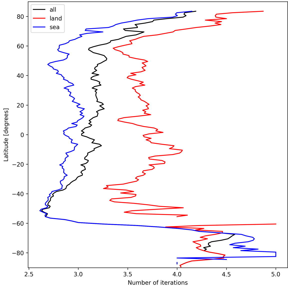
Figure 20: Zonal average of “Number of iterations” for 2025-10-04 to 2025-10-04.
