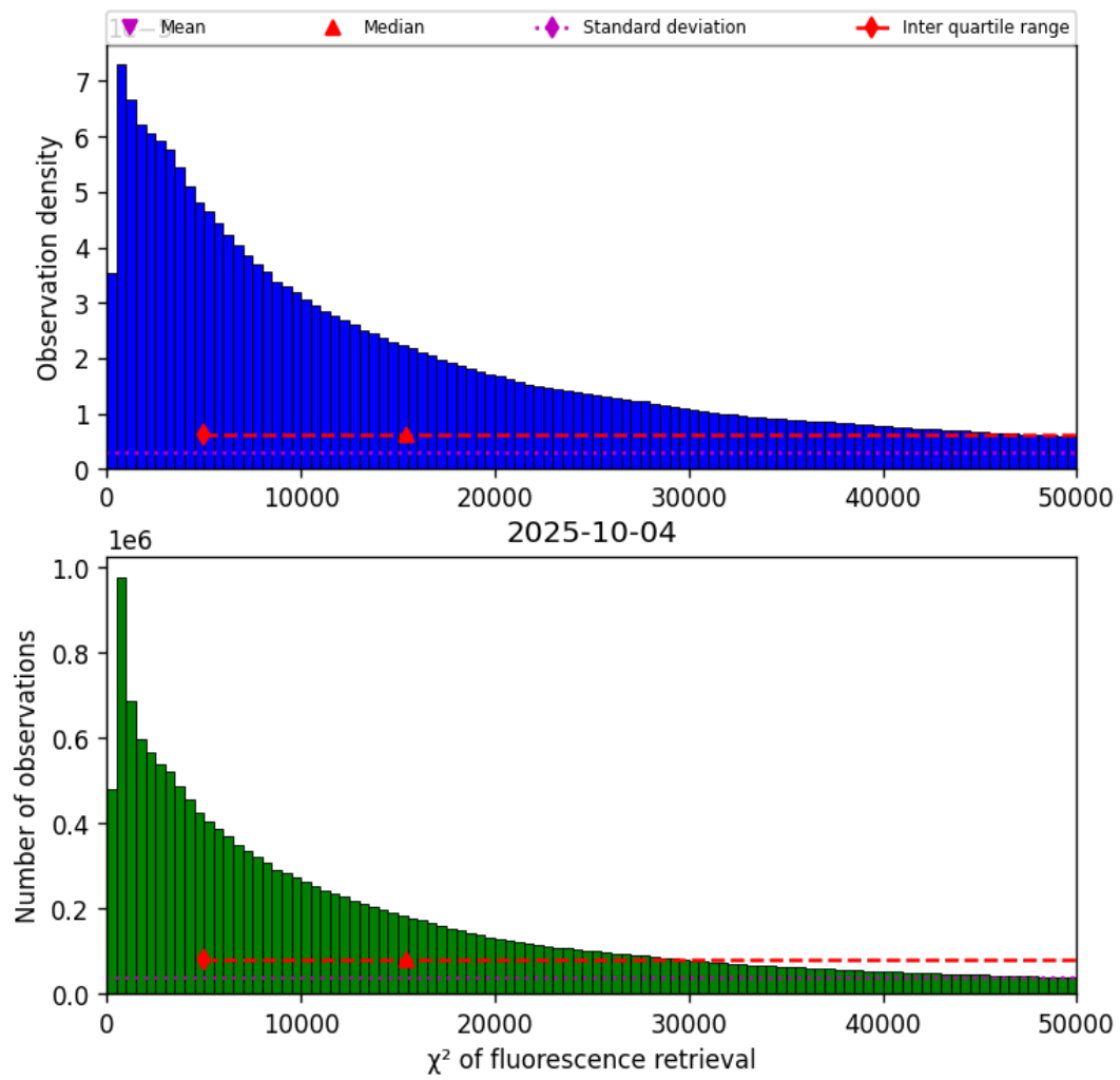
Figure 40: Histogram of “ \chi^2 of fluorescence retrieval” for 2025-10-04 to 2025-10-04
