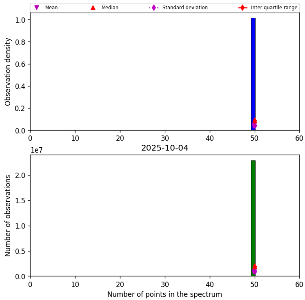
Figure 42: Histogram of “Number of points in the spectrum” for 2025-10-04 to 2025-10-04
