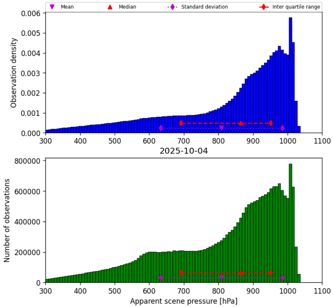
Figure 34: Histogram of “Apparent scene pressure” for 2025-10-04 to 2025-10-04
