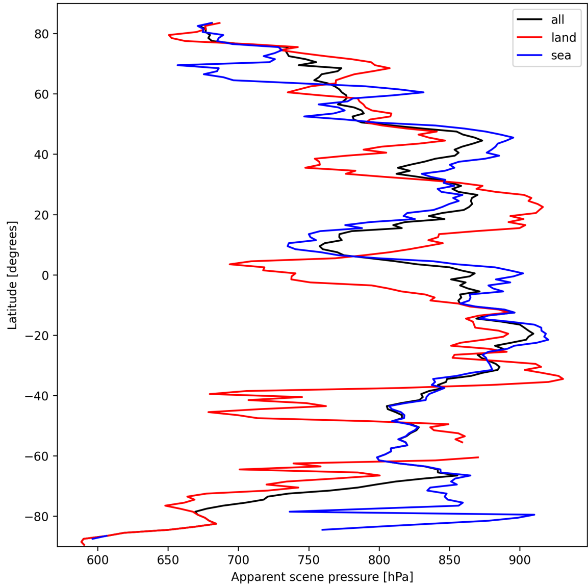
Figure 17: Zonal average of “Apparent scene pressure” for 2025-10-04 to 2025-10-04.
