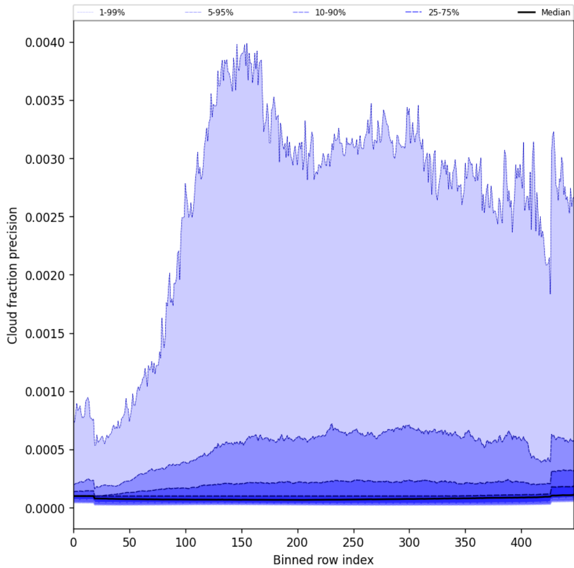
Figure 48: Along track statistics of “Cloud fraction precision” for 2025-10-04 to 2025-10-04
