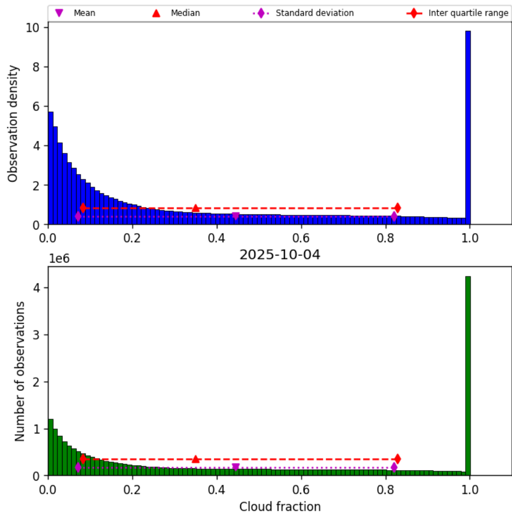
Figure 30: Histogram of “Cloud fraction” for 2025-10-04 to 2025-10-04
