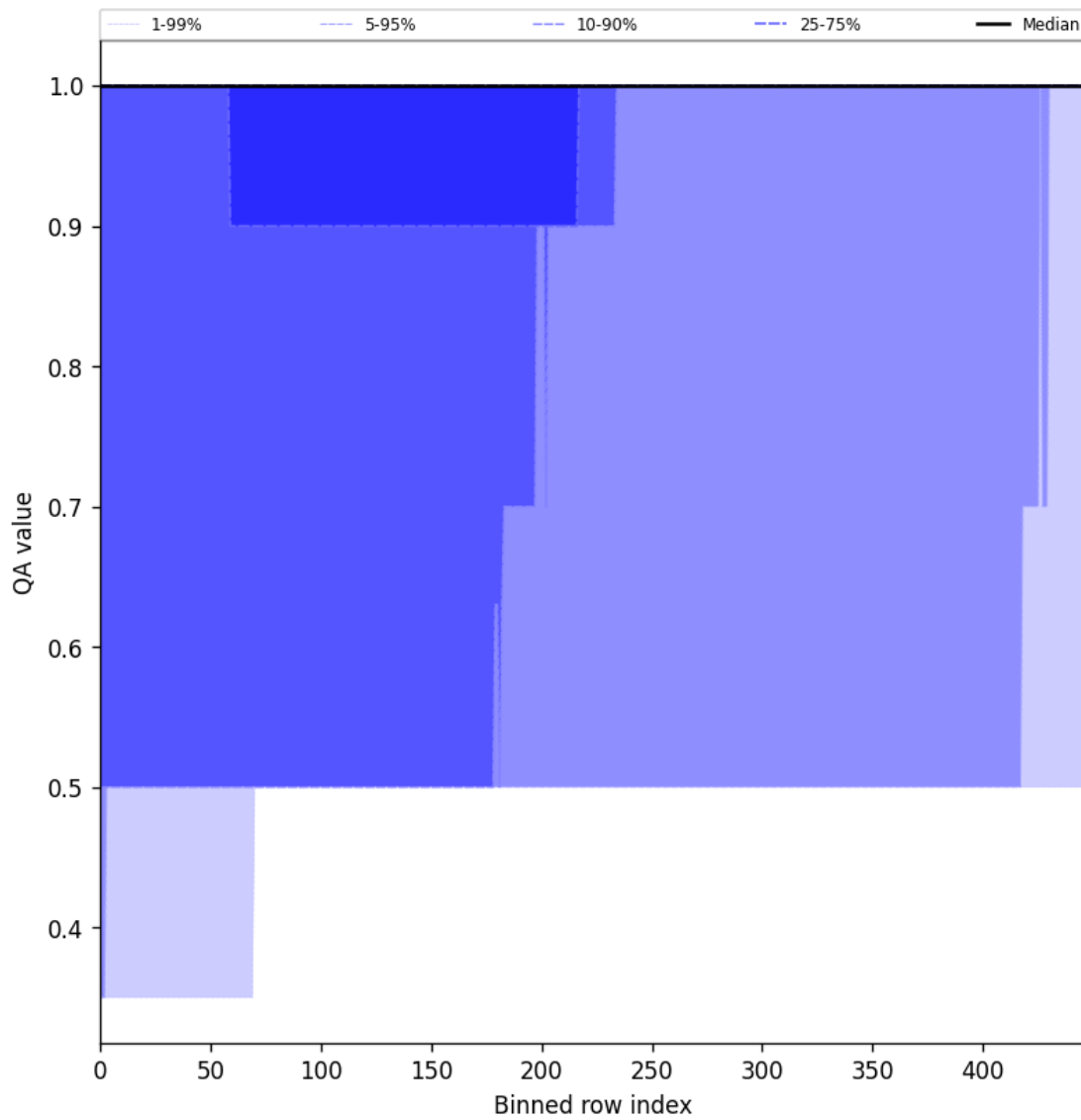
Figure 44: Along track statistics of “QA value” for 2025-10-04 to 2025-10-04
