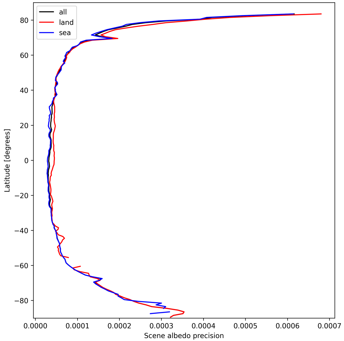
Figure 16: Zonal average of “Scene albedo precision” for 2025-10-04 to 2025-10-04.
