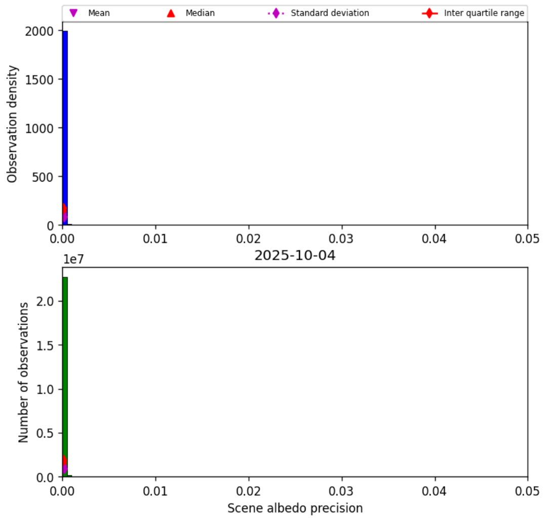
Figure 33: Histogram of “Scene albedo precision” for 2025-10-04 to 2025-10-04
