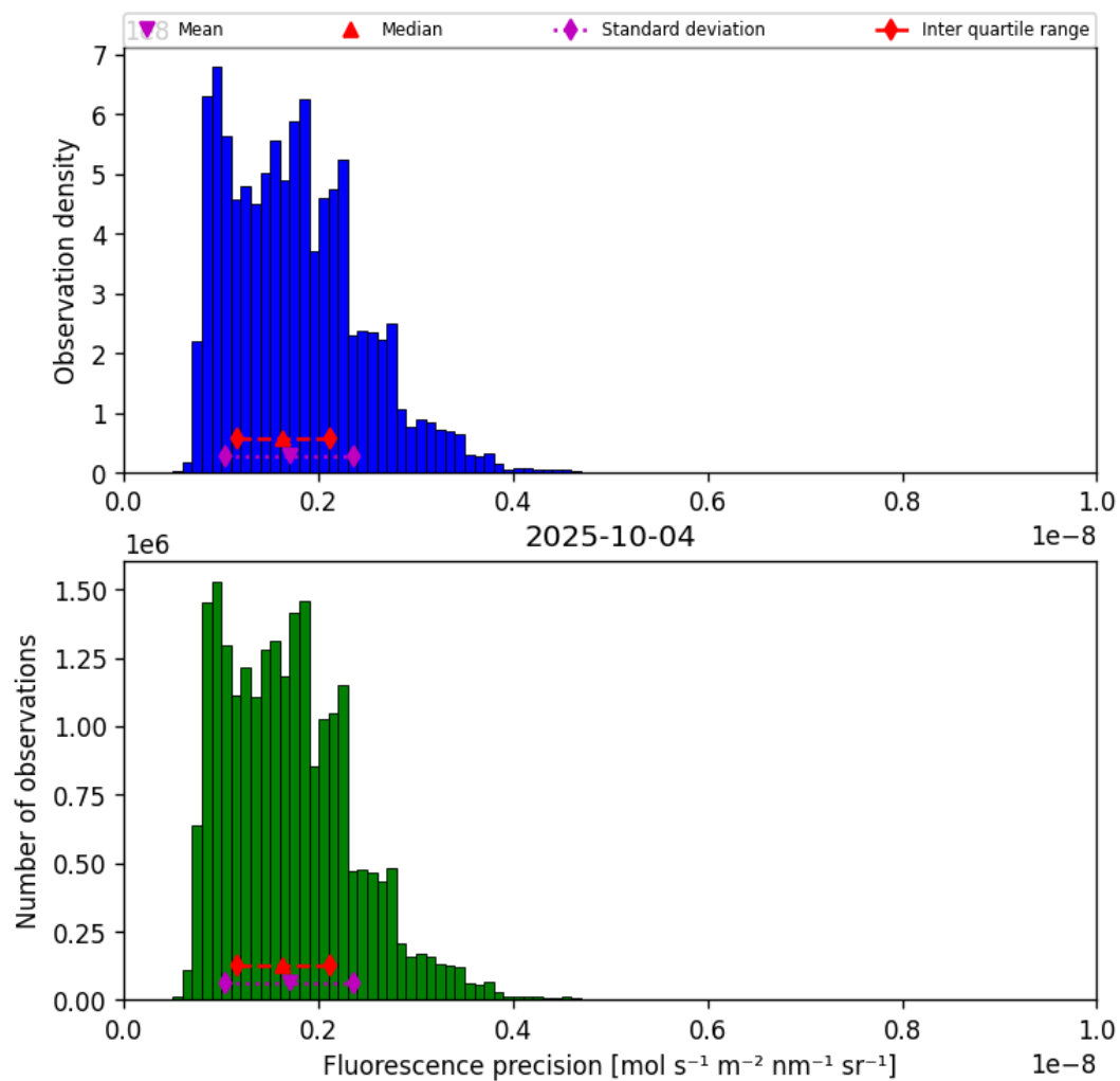
Figure 39: Histogram of “Fluorescence precision” for 2025-10-04 to 2025-10-04
