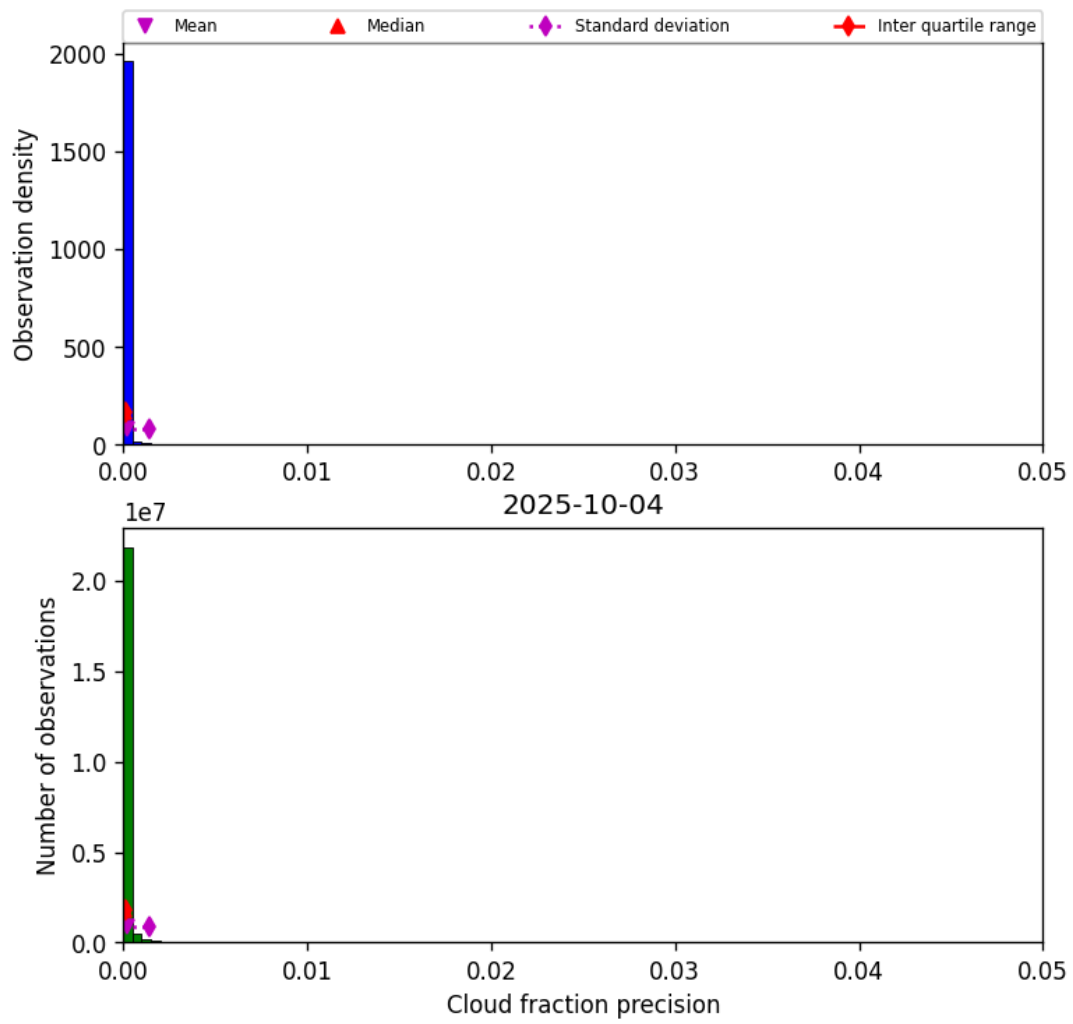
Figure 31: Histogram of “Cloud fraction precision” for 2025-10-04 to 2025-10-04
