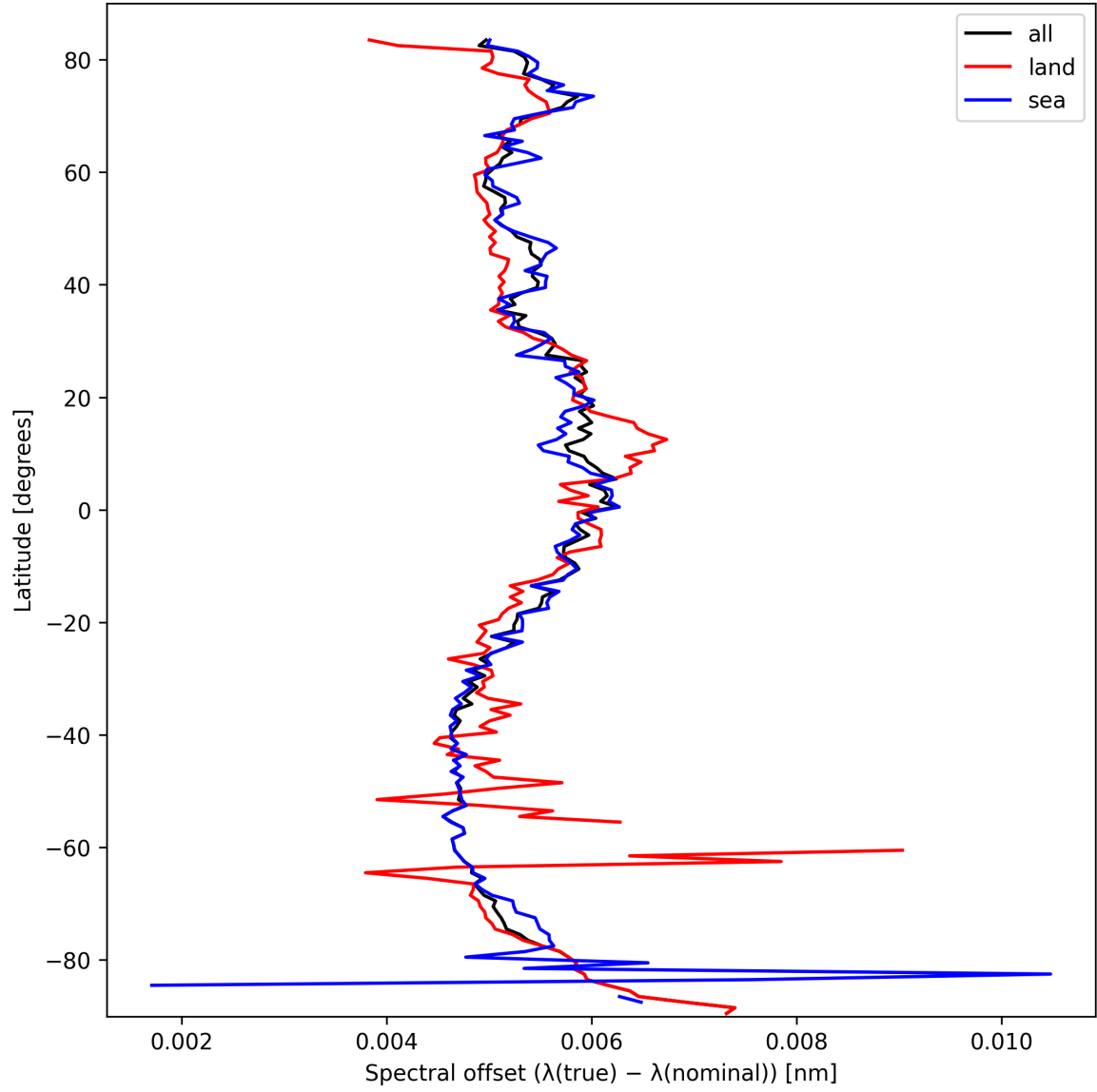
Figure 26: Zonal average of “Spectral offset ( \lambda_{\text{true}} - \lambda_{\text{nominal}} )” for 2025-10-04 to 2025-10-04.
