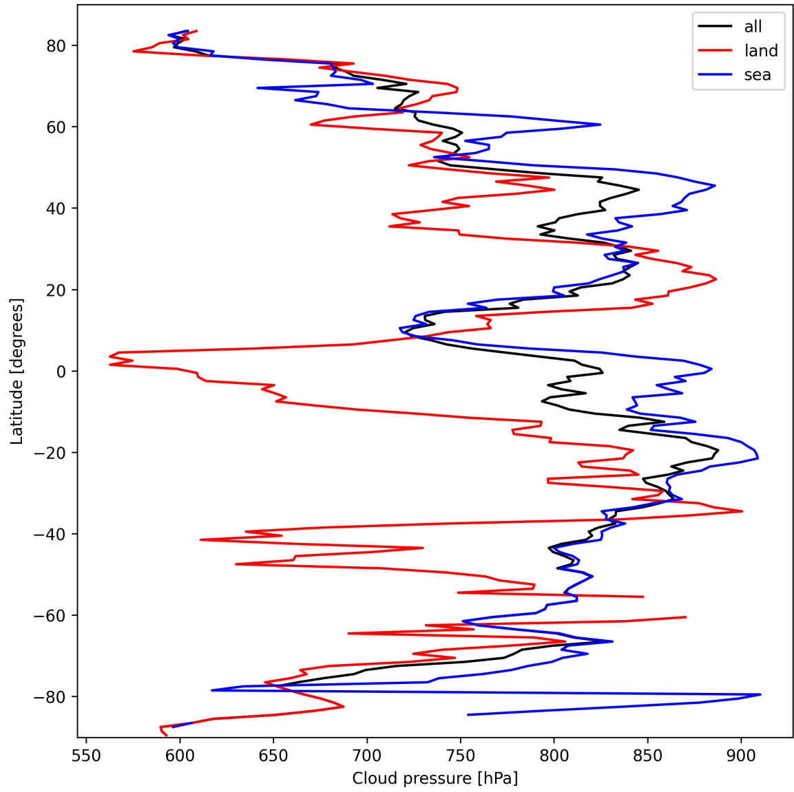
Figure 11: Zonal average of “Cloud pressure” for 2025-10-04 to 2025-10-04.
