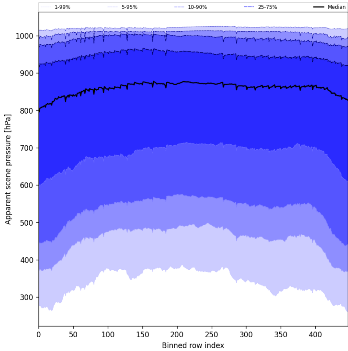
Figure 51: Along track statistics of “Apparent scene pressure” for 2025-10-05 to 2025-10-06
