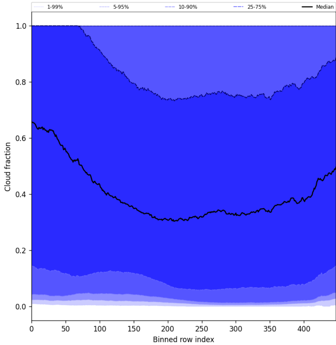
Figure 47: Along track statistics of “Cloud fraction” for 2025-10-05 to 2025-10-06
