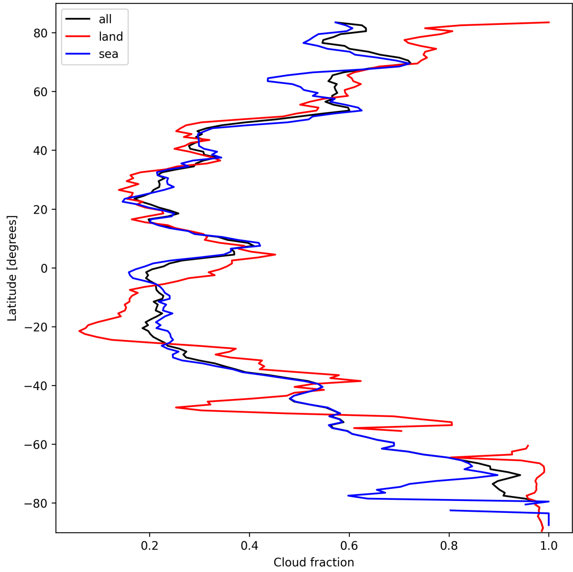
Figure 13: Zonal average of “Cloud fraction” for 2025-10-05 to 2025-10-06.
