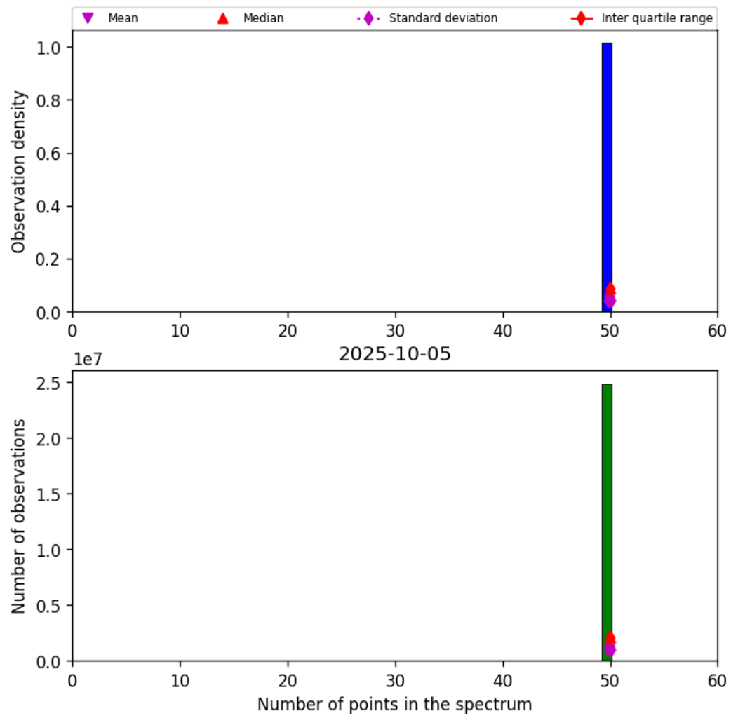
Figure 42: Histogram of “Number of points in the spectrum” for 2025-10-05 to 2025-10-06
