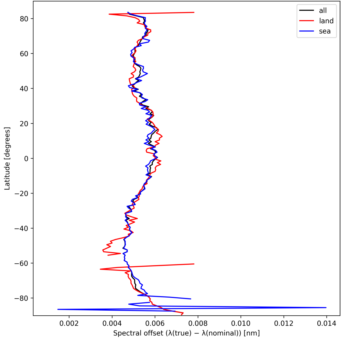
Figure 26: Zonal average of “Spectral offset ( \lambda_{\text{true}} - \lambda_{\text{nominal}} )” for 2025-10-05 to 2025-10-06.
