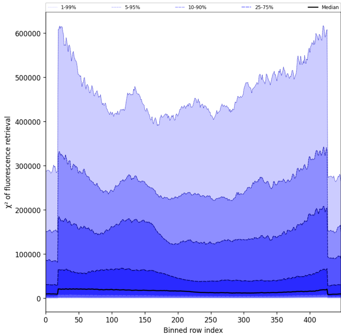
Figure 57: Along track statistics of “ \chi^2 of fluorescence retrieval” for 2025-10-05 to 2025-10-06
