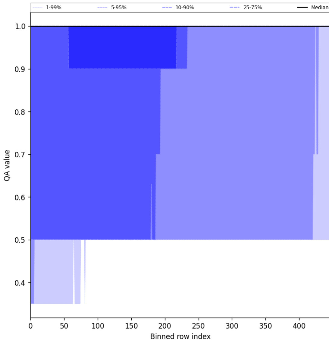
Figure 44: Along track statistics of “QA value” for 2025-10-05 to 2025-10-06
