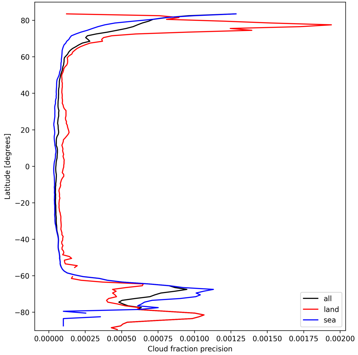
Figure 14: Zonal average of “Cloud fraction precision” for 2025-10-05 to 2025-10-06.
