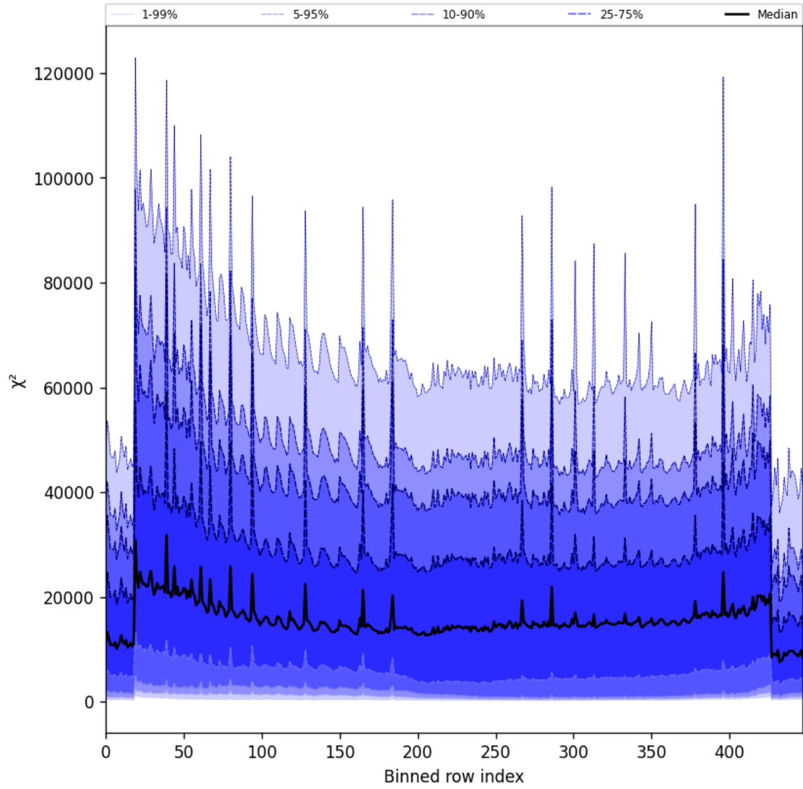
Figure 53: Along track statistics of “ \chi^2 ” for 2025-10-05 to 2025-10-06
