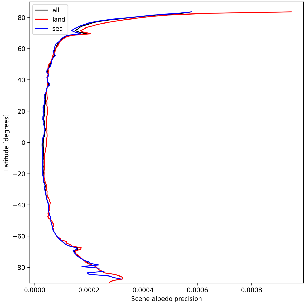
Figure 16: Zonal average of “Scene albedo precision” for 2025-10-05 to 2025-10-06.
