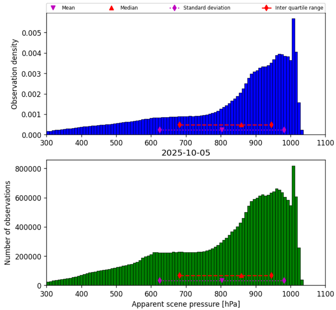
Figure 34: Histogram of “Apparent scene pressure” for 2025-10-05 to 2025-10-06
