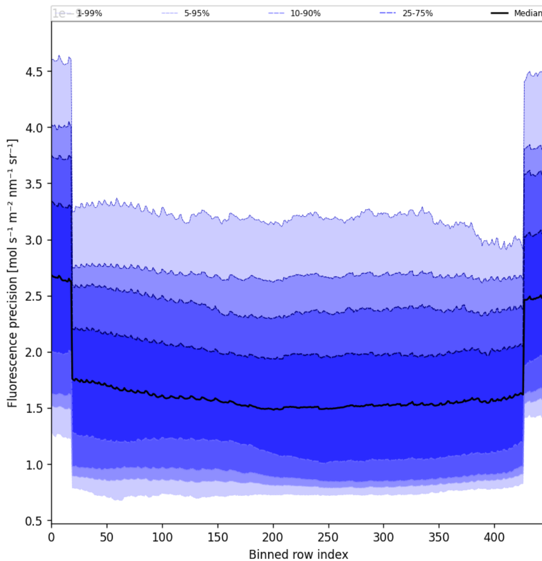
Figure 56: Along track statistics of “Fluorescence precision” for 2025-10-05 to 2025-10-06
