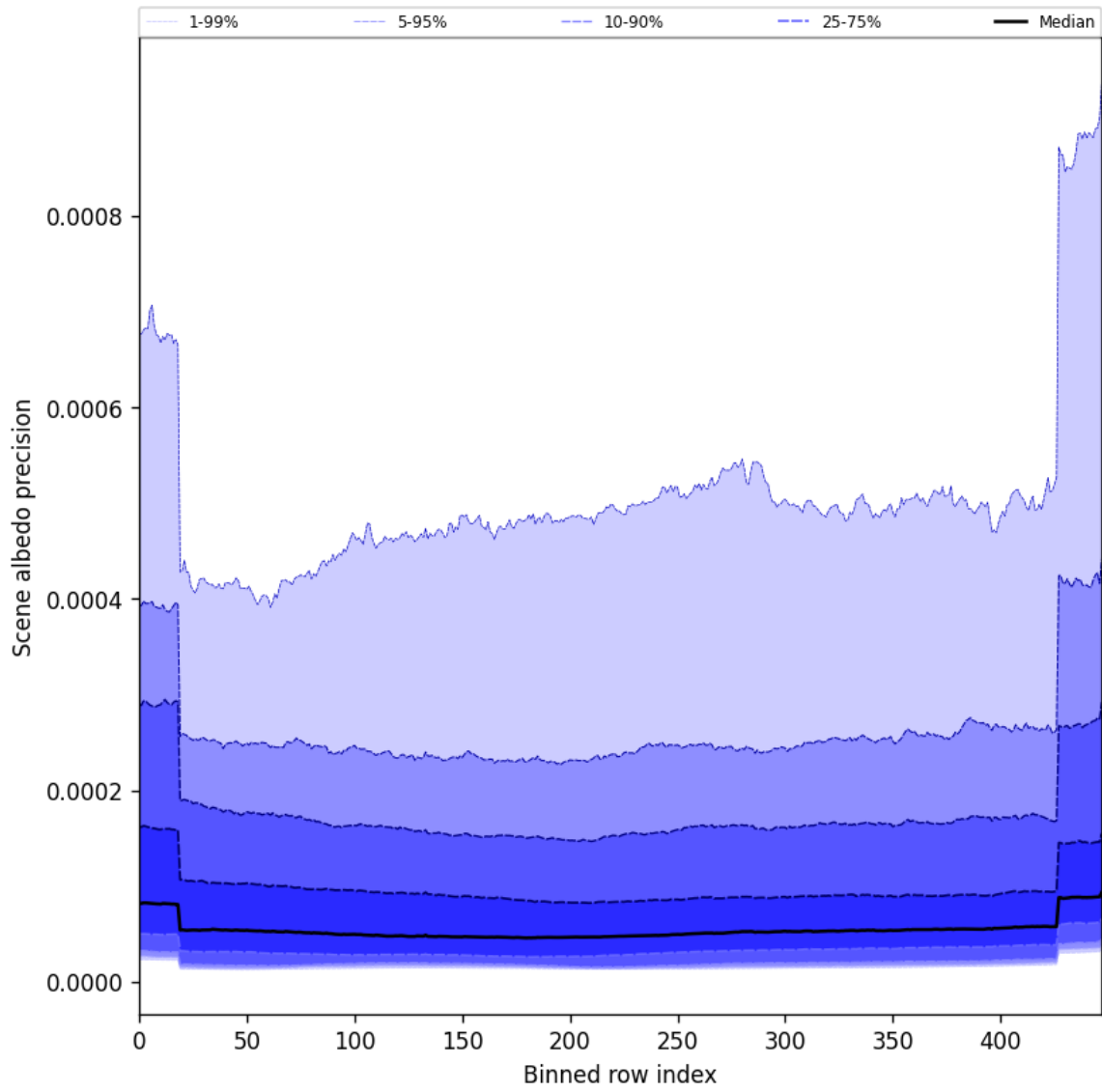
Figure 50: Along track statistics of “Scene albedo precision” for 2025-10-05 to 2025-10-06
