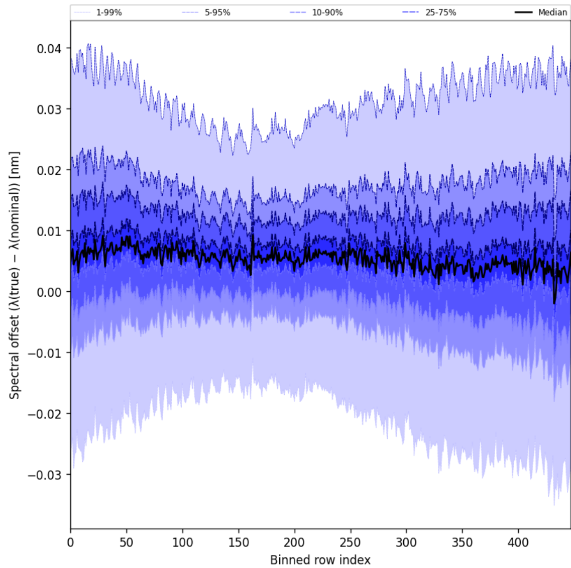
Figure 60: Along track statistics of “Spectral offset ( \lambda_{\text{true}} - \lambda_{\text{nominal}} )” for 2025-10-05 to 2025-10-06
