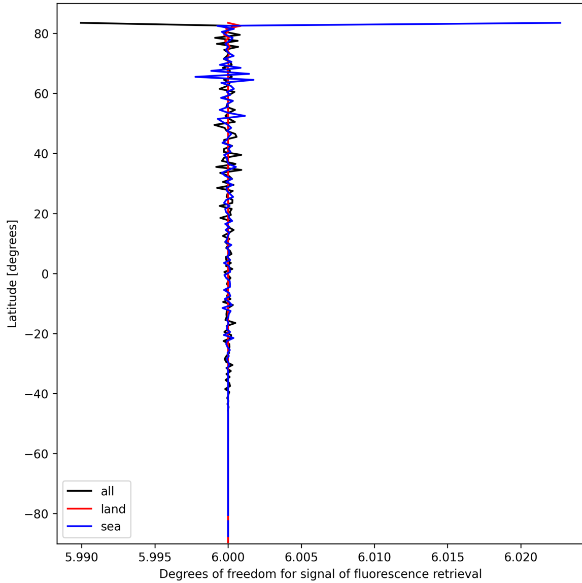
Figure 24: Zonal average of “Degrees of freedom for signal of fluorescence retrieval” for 2025-10-05 to 2025-10-06.
