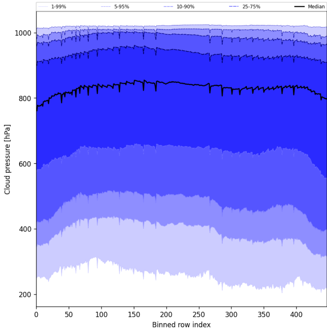
Figure 45: Along track statistics of “Cloud pressure” for 2025-10-05 to 2025-10-06
