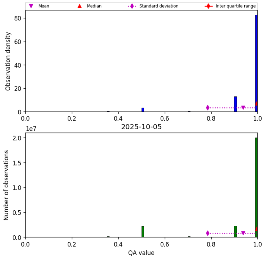
Figure 27: Histogram of “QA value” for 2025-10-05 to 2025-10-06
