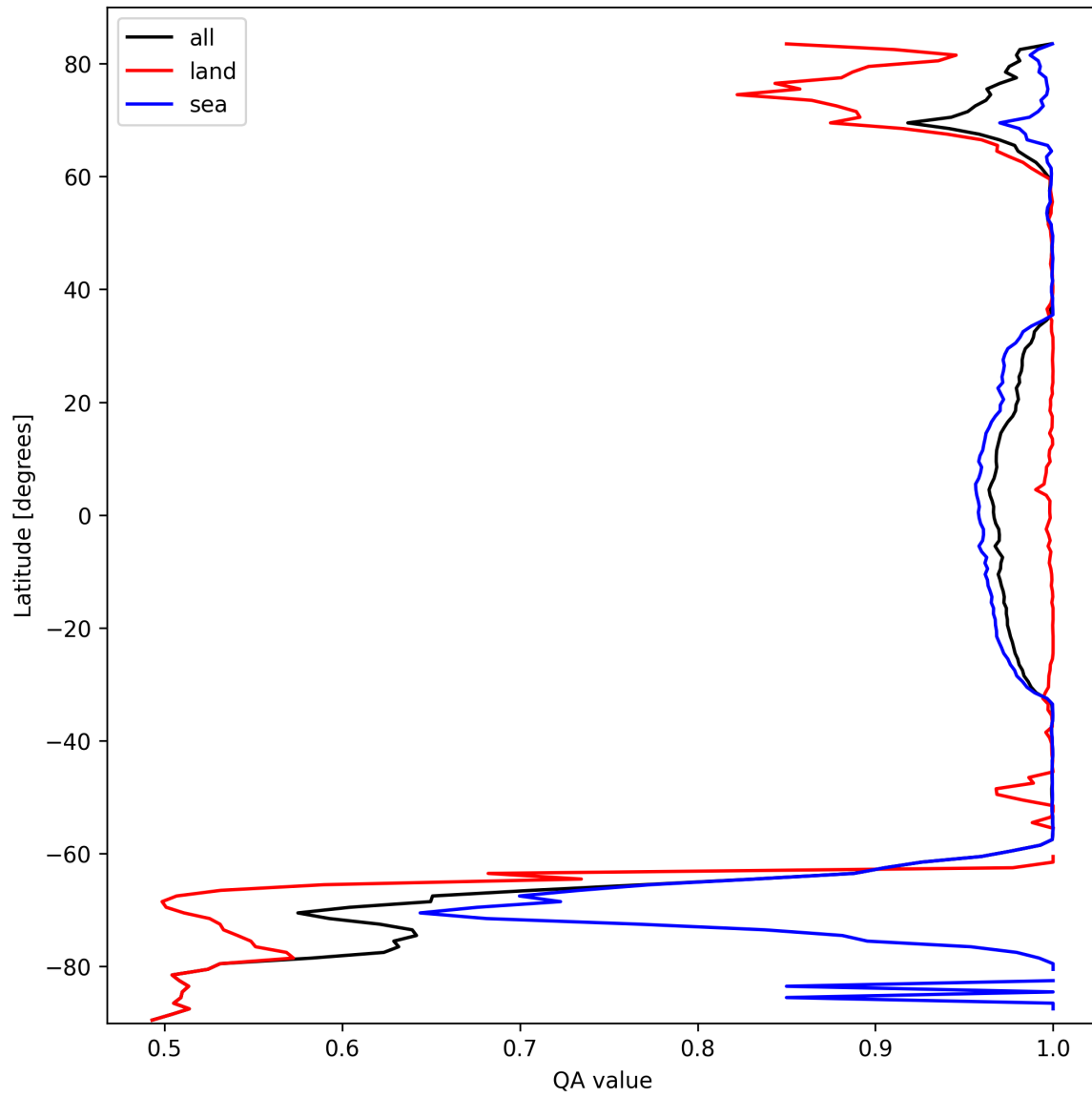
Figure 10: Zonal average of “QA value” for 2025-10-05 to 2025-10-06.
