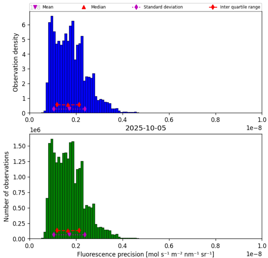
Figure 39: Histogram of “Fluorescence precision” for 2025-10-05 to 2025-10-06
