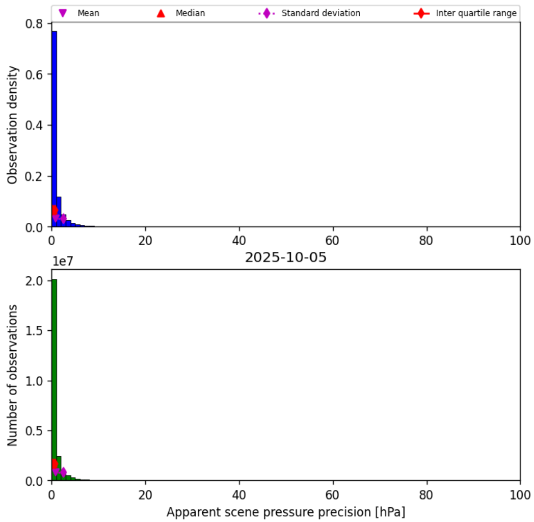
Figure 35: Histogram of “Apparent scene pressure precision” for 2025-10-05 to 2025-10-06
