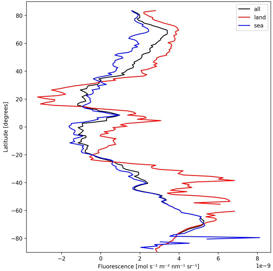
Figure 21: Zonal average of “Fluorescence” for 2025-10-05 to 2025-10-06.
