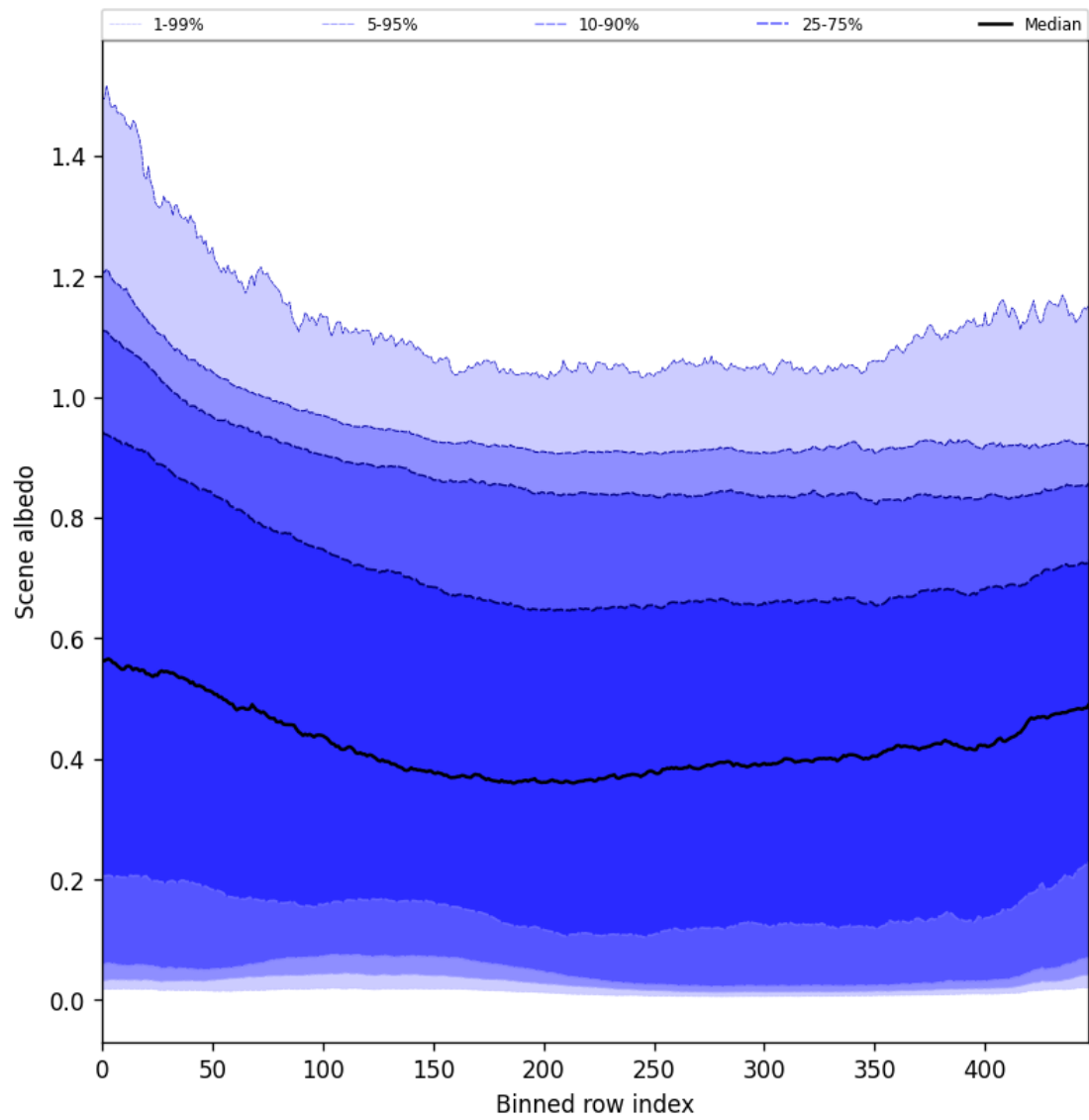
Figure 49: Along track statistics of “Scene albedo” for 2025-10-05 to 2025-10-06
