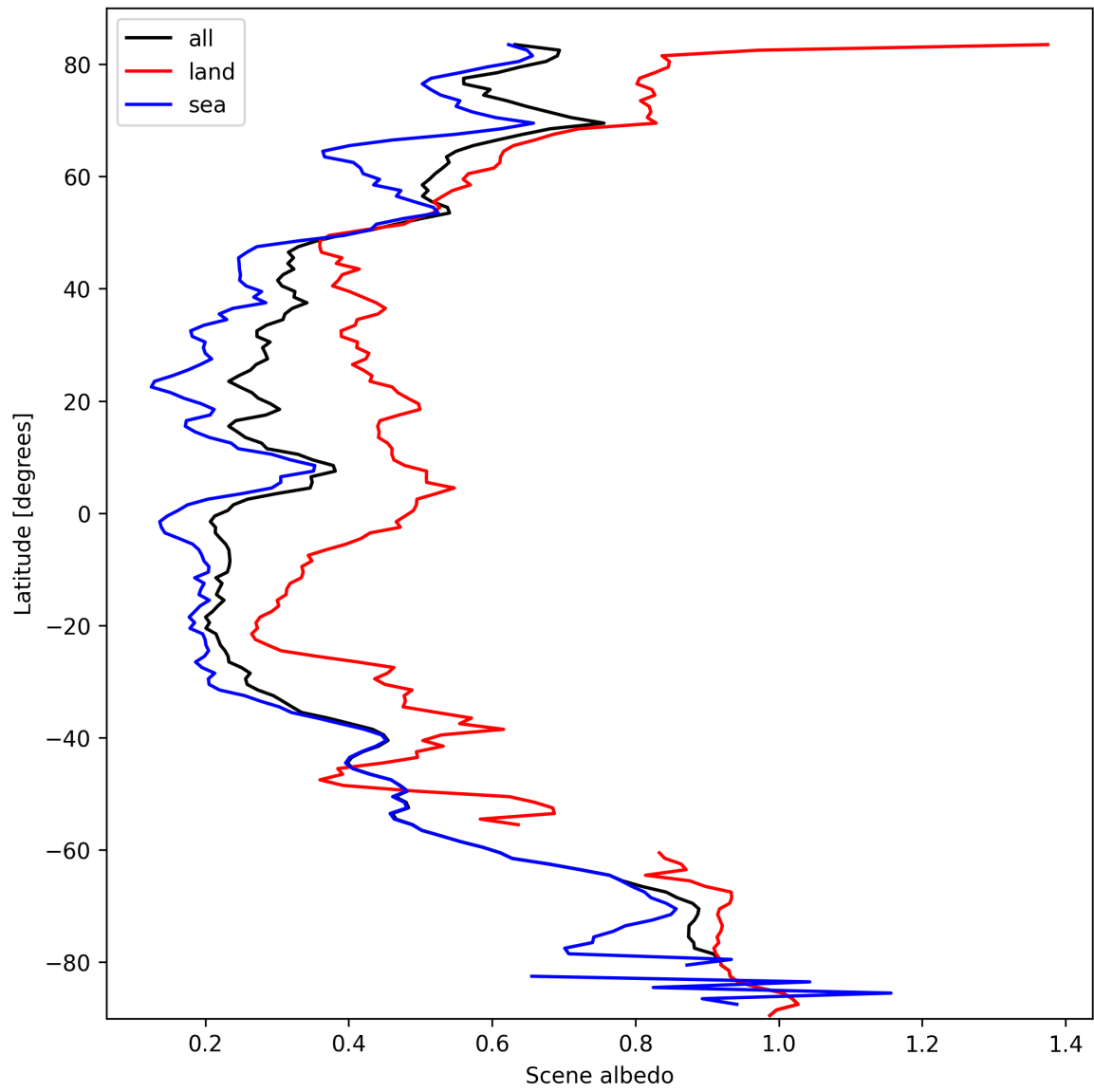
Figure 15: Zonal average of “Scene albedo” for 2025-10-05 to 2025-10-06.
