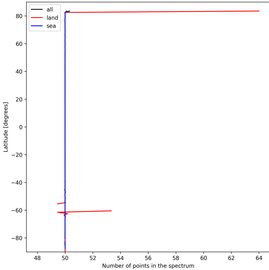
Figure 25: Zonal average of “Number of points in the spectrum” for 2025-10-05 to 2025-10-06.
