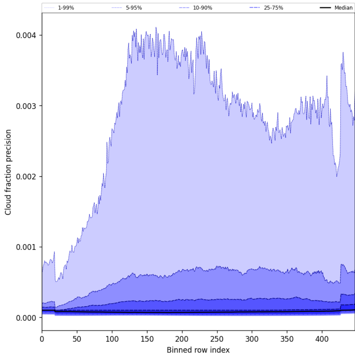
Figure 48: Along track statistics of “Cloud fraction precision” for 2025-10-05 to 2025-10-06
