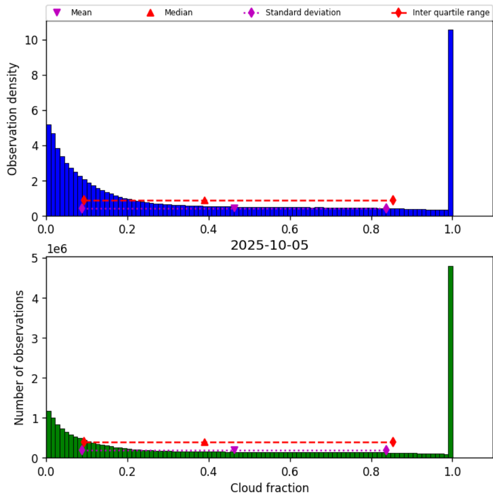
Figure 30: Histogram of “Cloud fraction” for 2025-10-05 to 2025-10-06
