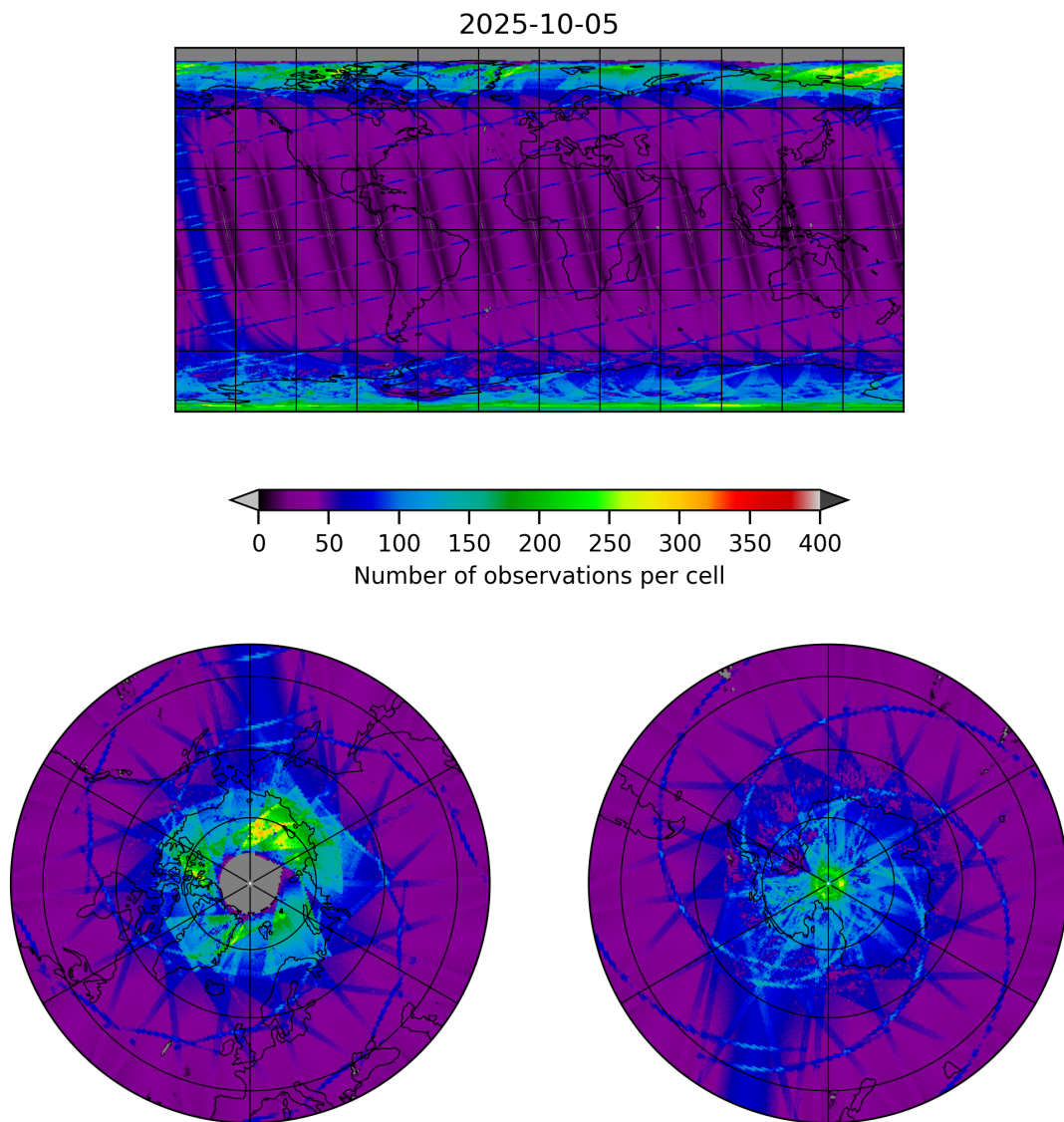
Figure 9: Map of the number of observations for 2025-10-05 to 2025-10-06
