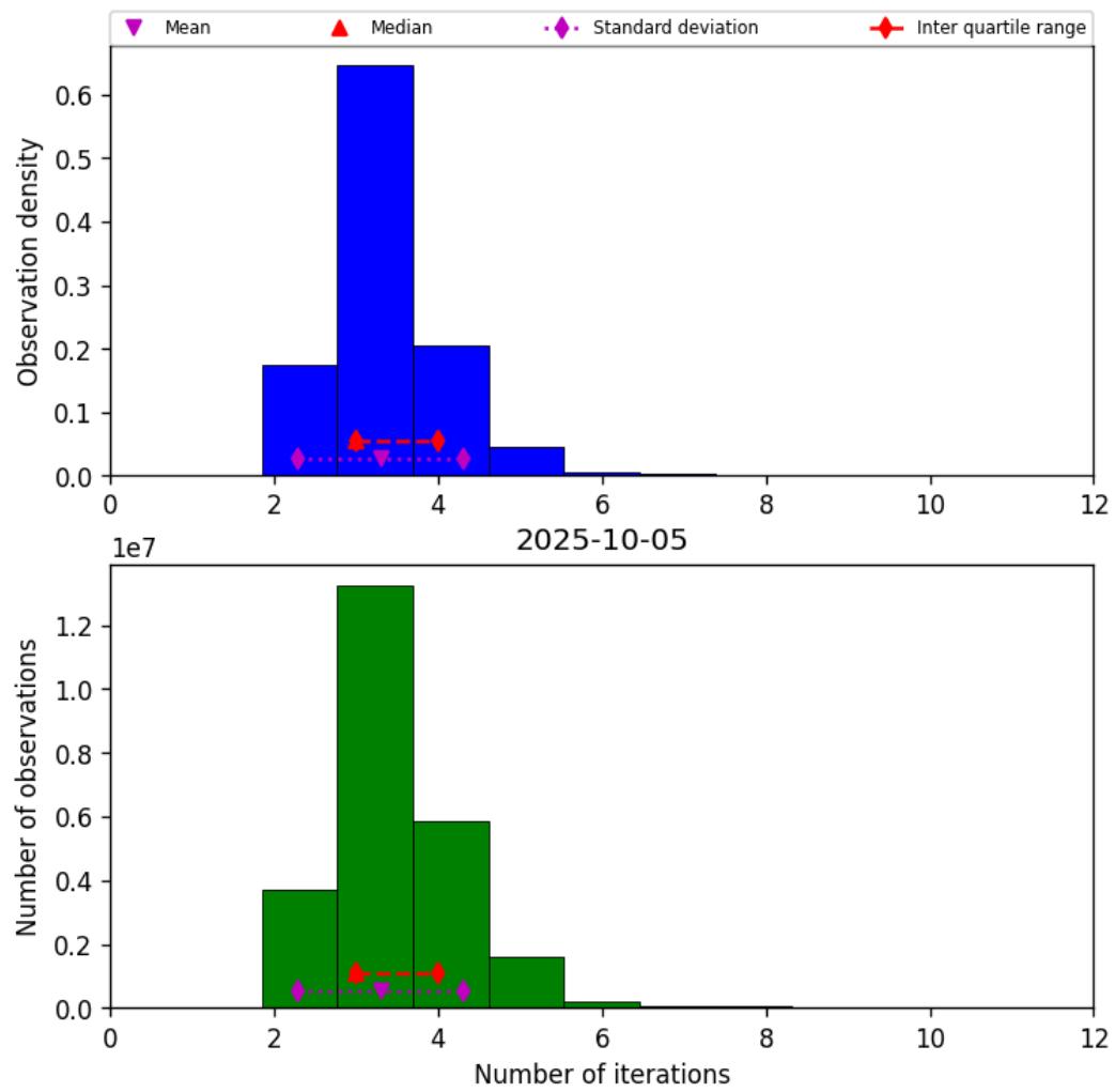
Figure 37: Histogram of “Number of iterations” for 2025-10-05 to 2025-10-06
