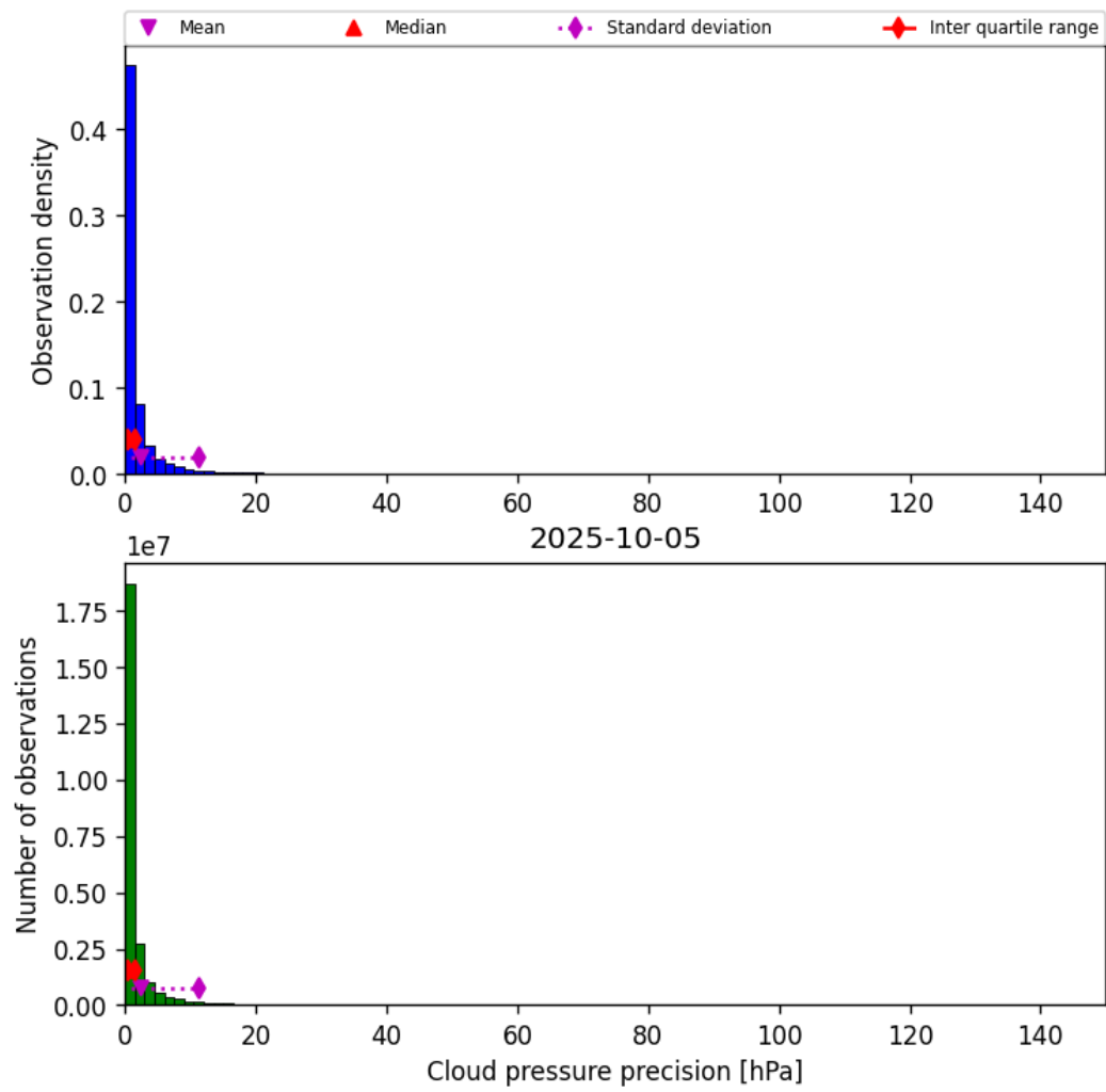
Figure 29: Histogram of “Cloud pressure precision” for 2025-10-05 to 2025-10-06
