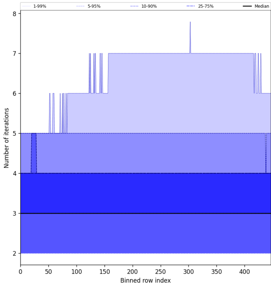
Figure 54: Along track statistics of “Number of iterations” for 2025-10-05 to 2025-10-06
