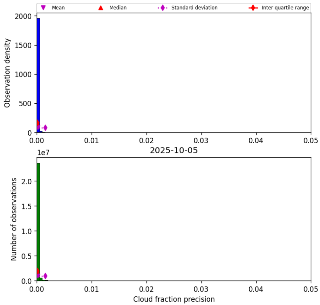
Figure 31: Histogram of “Cloud fraction precision” for 2025-10-05 to 2025-10-06
