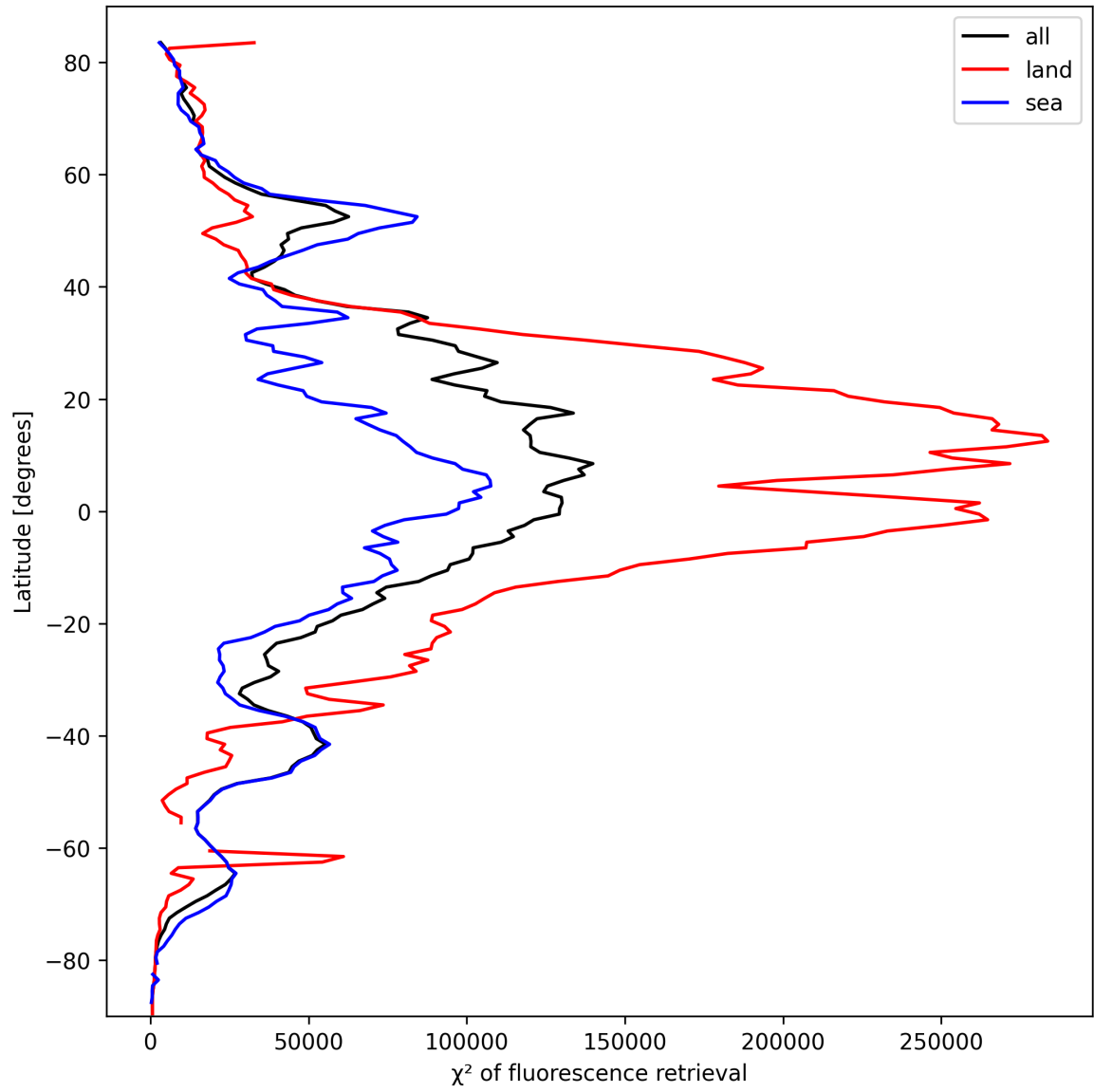
Figure 23: Zonal average of “ \chi^2 of fluorescence retrieval” for 2025-10-05 to 2025-10-06.
