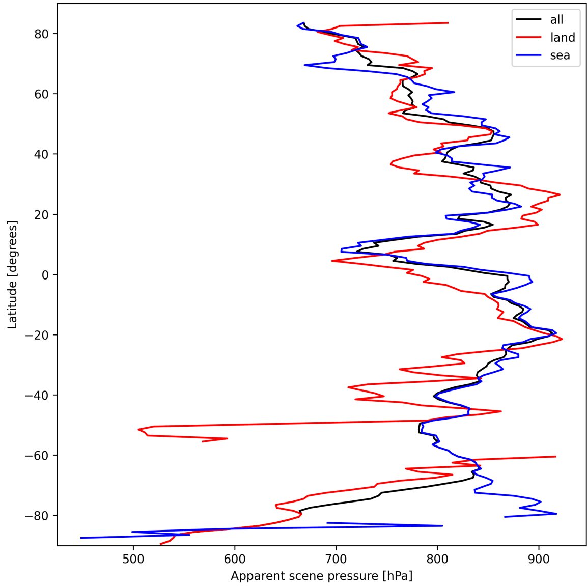
Figure 17: Zonal average of “Apparent scene pressure” for 2025-10-05 to 2025-10-06.
