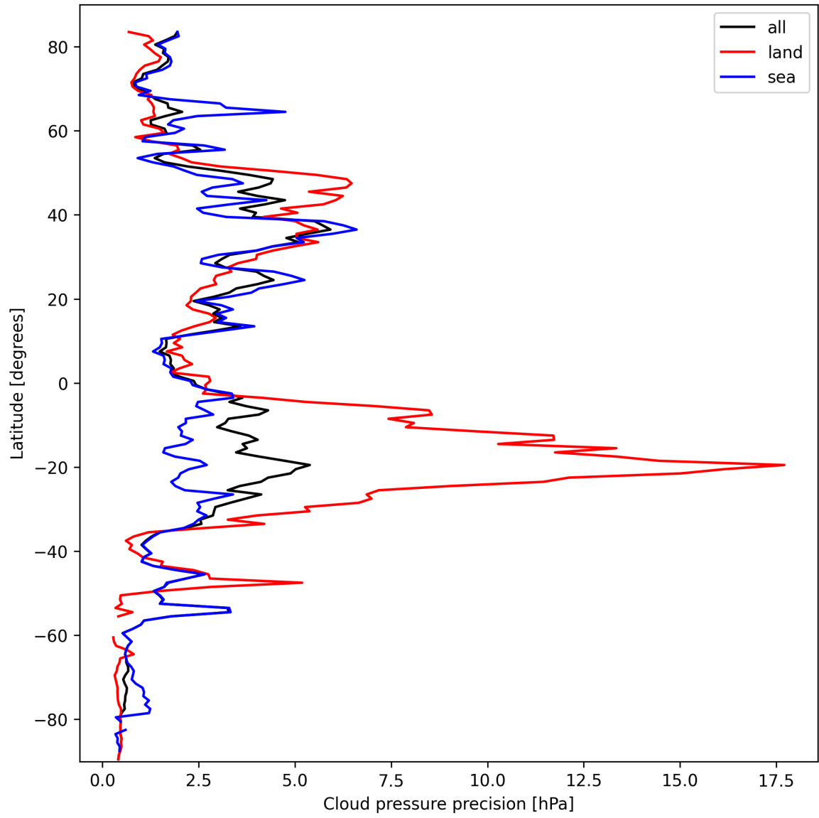
Figure 12: Zonal average of "Cloud pressure precision" for 2025-10-05 to 2025-10-06.
