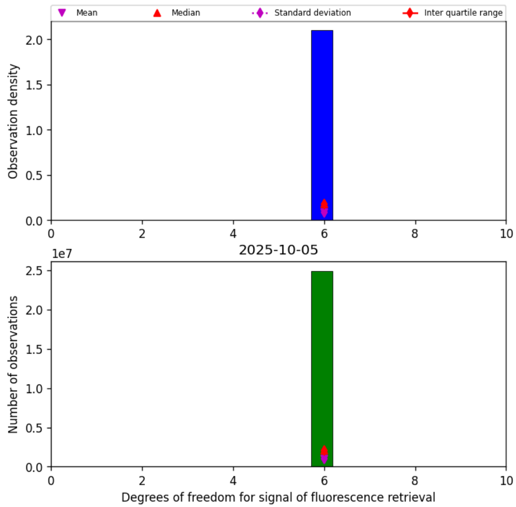
Figure 41: Histogram of “Degrees of freedom for signal of fluorescence retrieval” for 2025-10-05 to 2025-10-06
