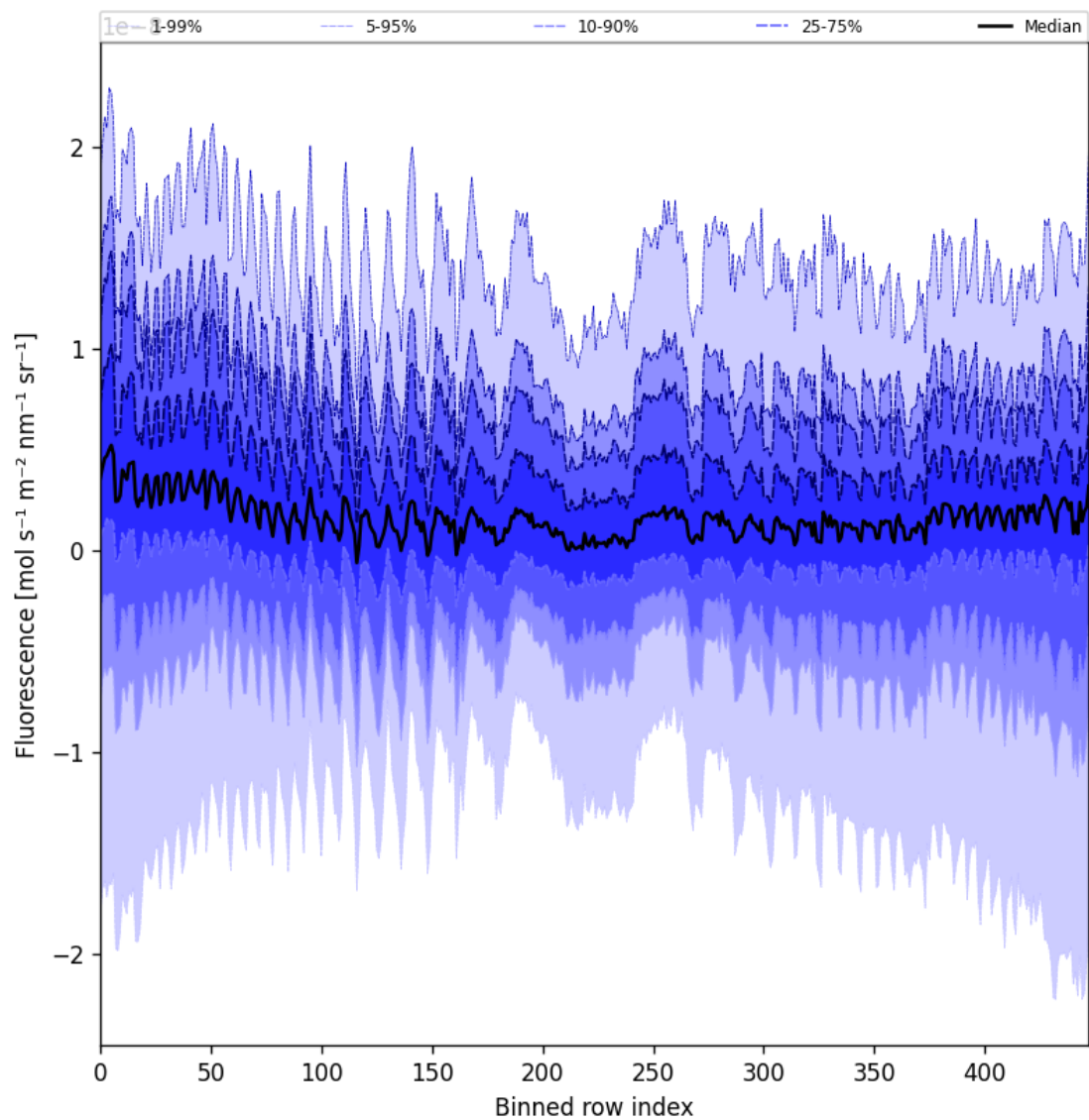
Figure 55: Along track statistics of “Fluorescence” for 2025-10-05 to 2025-10-06
