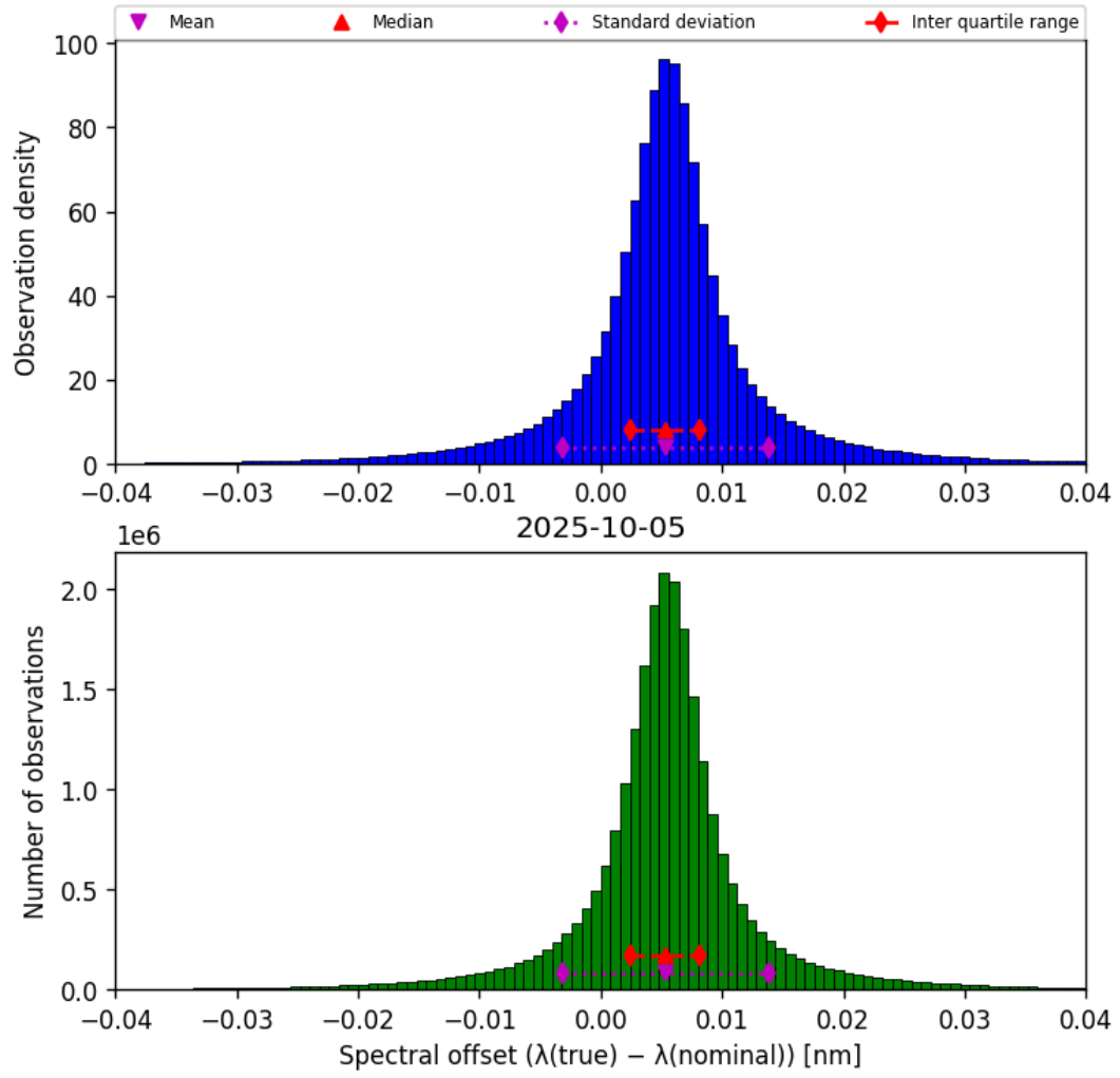
Figure 43: Histogram of “Spectral offset ( \lambda_{\text{true}} - \lambda_{\text{nominal}} )” for 2025-10-05 to 2025-10-06
