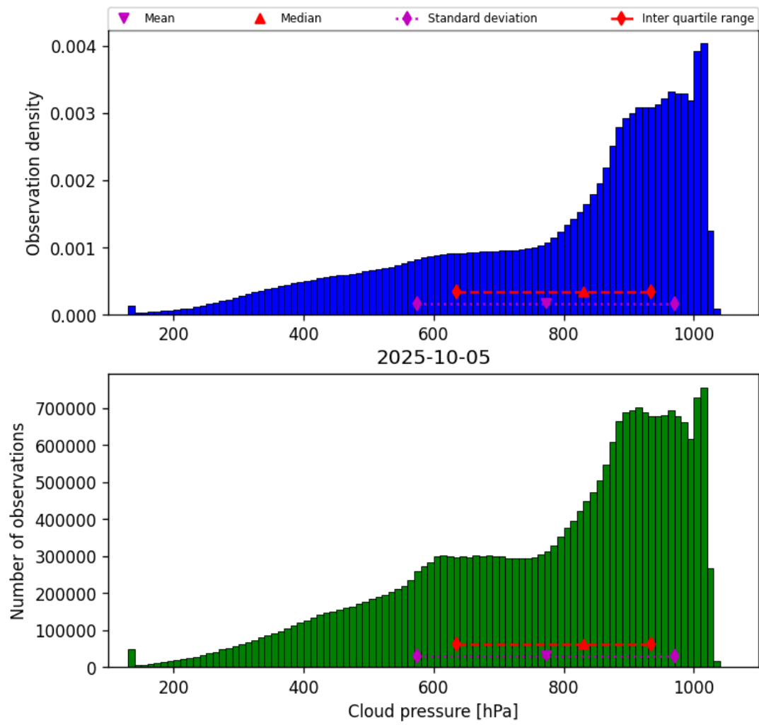
Figure 28: Histogram of “Cloud pressure” for 2025-10-05 to 2025-10-06
