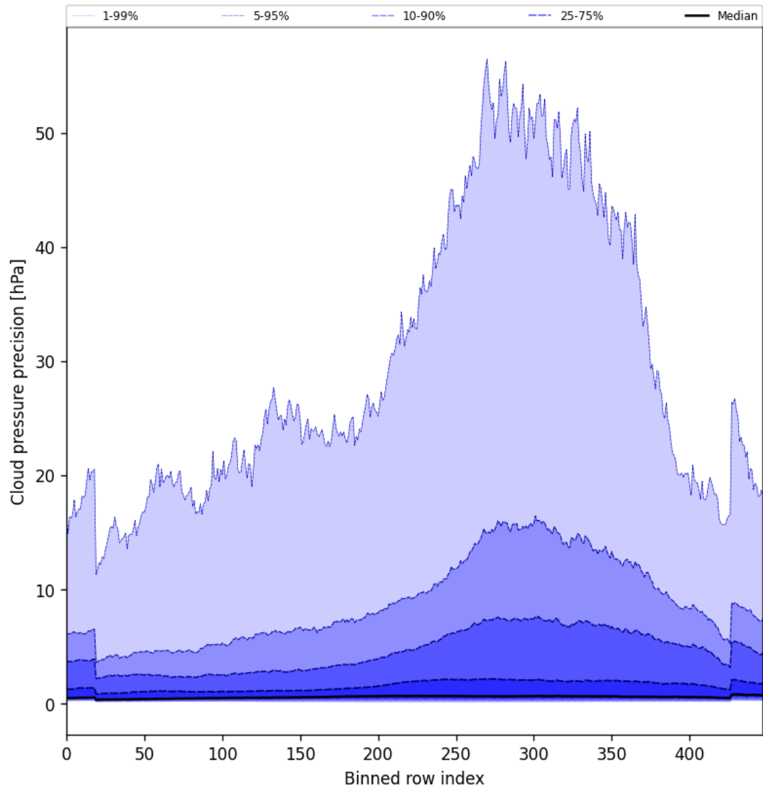
Figure 46: Along track statistics of “Cloud pressure precision” for 2025-10-05 to 2025-10-06
