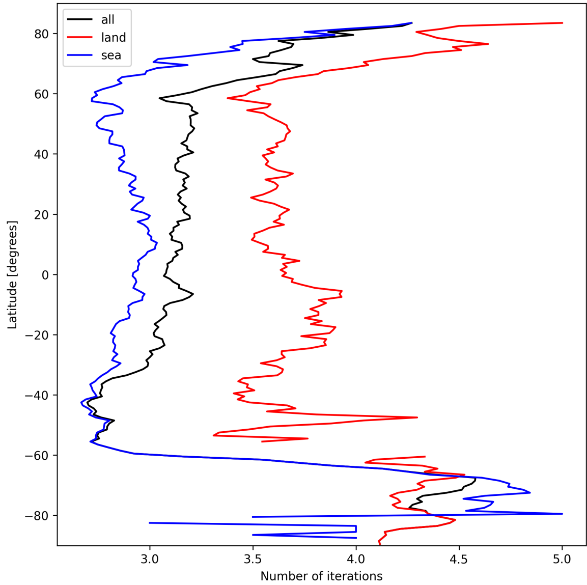
Figure 20: Zonal average of “Number of iterations” for 2025-10-05 to 2025-10-06.
