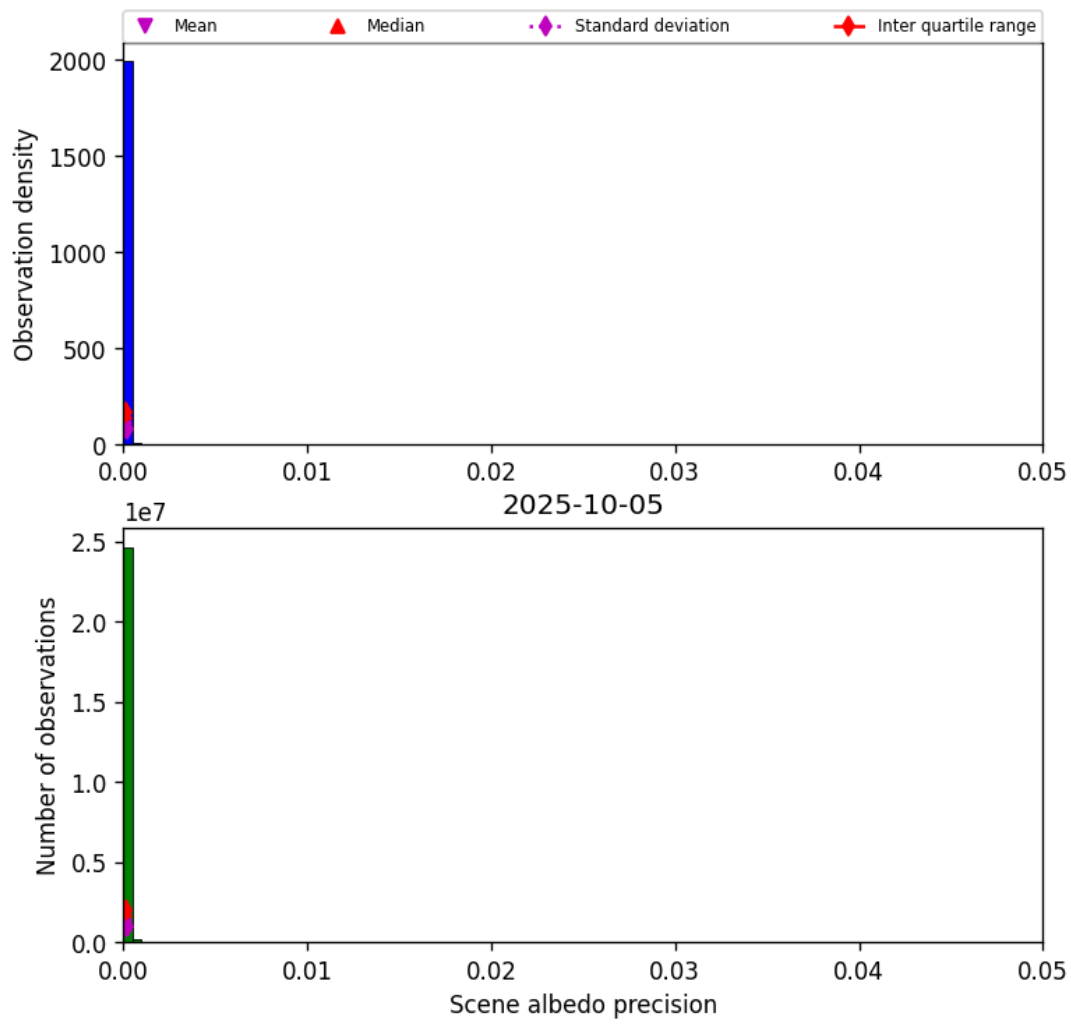
Figure 33: Histogram of “Scene albedo precision” for 2025-10-05 to 2025-10-06
