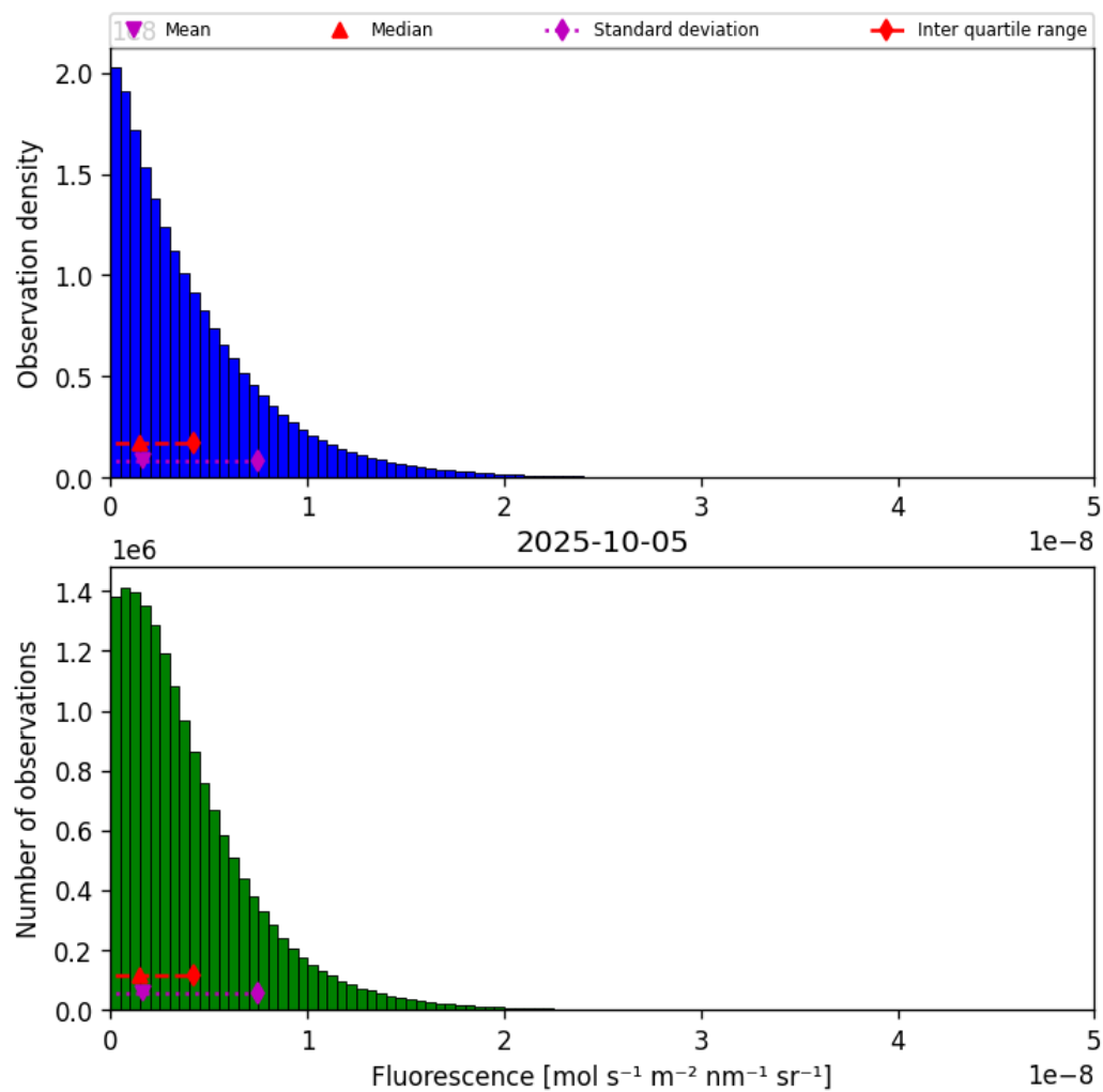
Figure 38: Histogram of “Fluorescence” for 2025-10-05 to 2025-10-06
