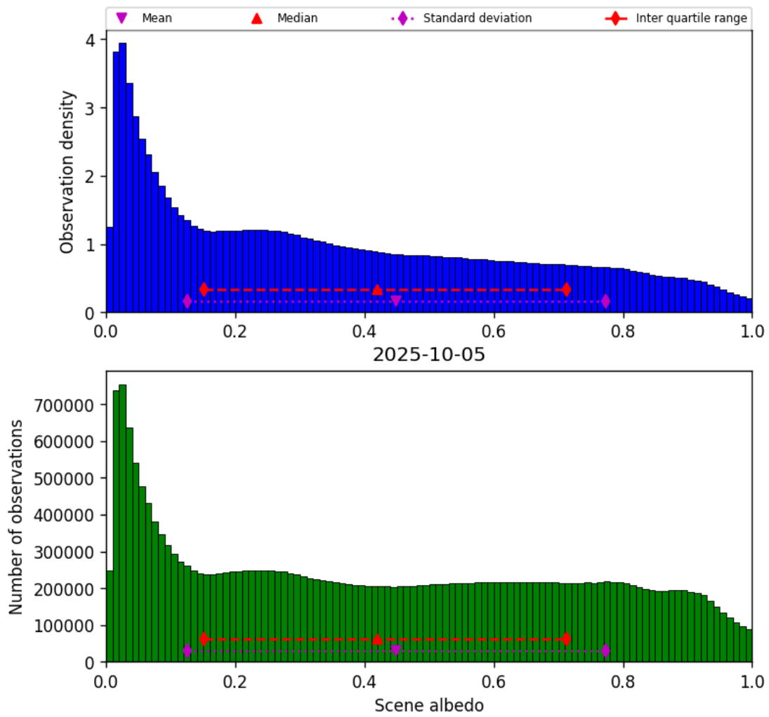
Figure 32: Histogram of “Scene albedo” for 2025-10-05 to 2025-10-06
