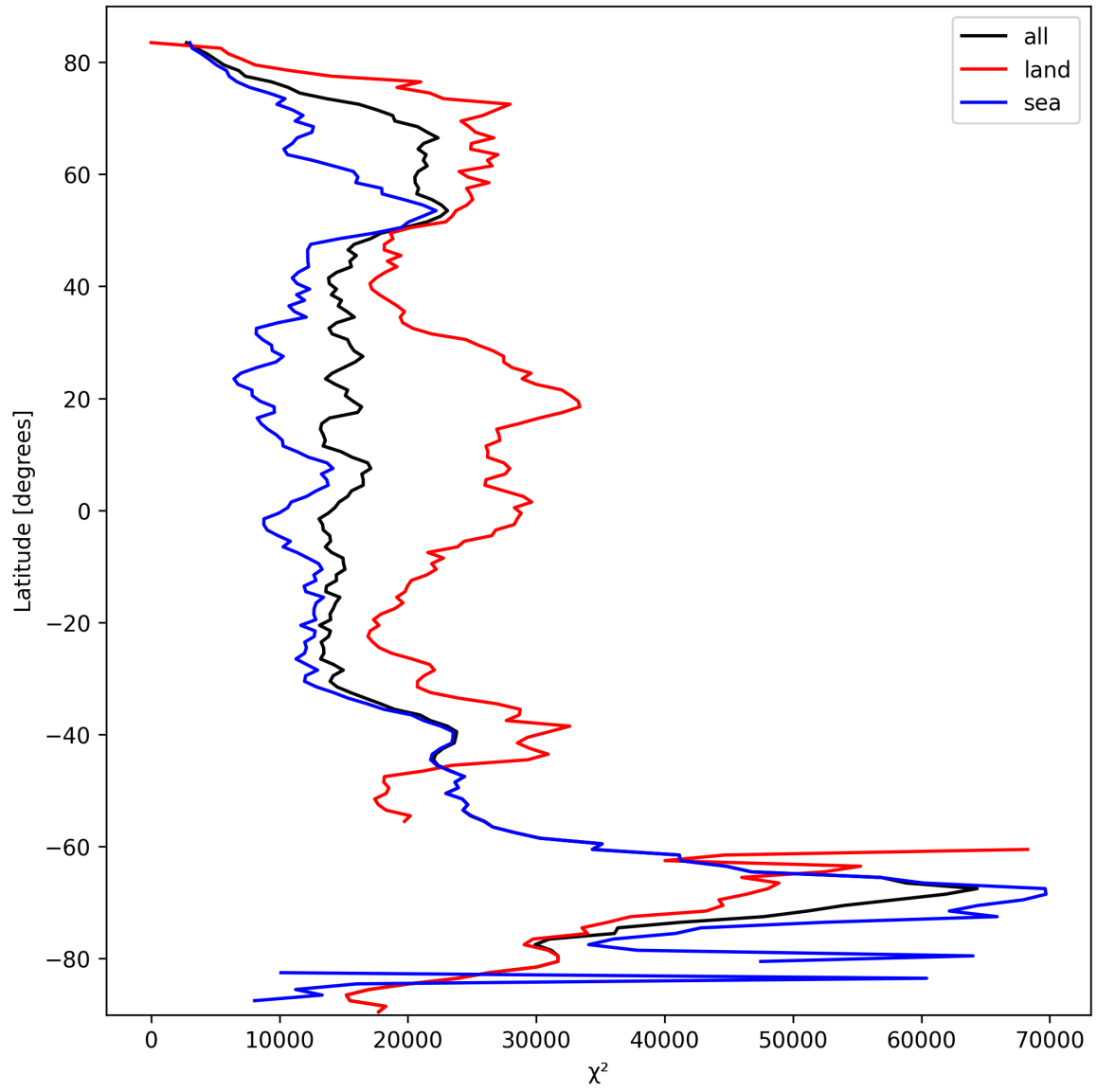
Figure 19: Zonal average of “ \chi^2 ” for 2025-10-05 to 2025-10-06.
