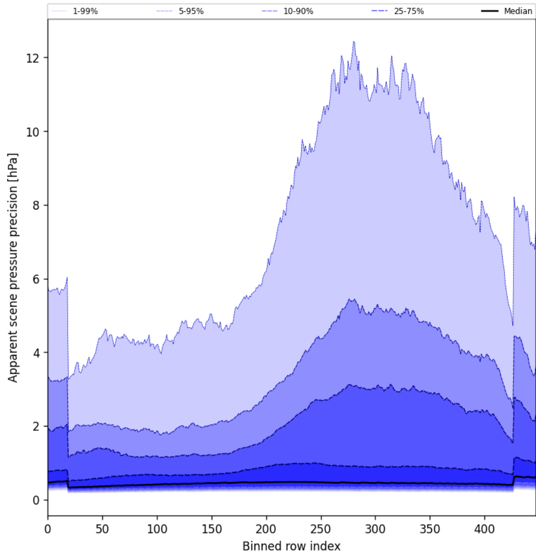
Figure 52: Along track statistics of “Apparent scene pressure precision” for 2025-10-05 to 2025-10-06
