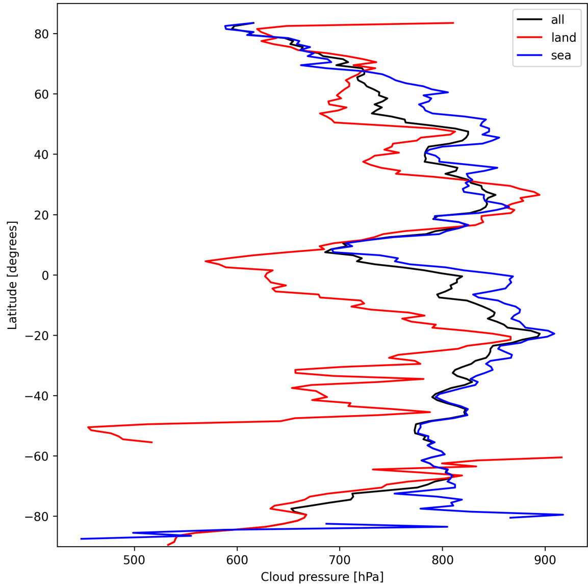
Figure 11: Zonal average of “Cloud pressure” for 2025-10-05 to 2025-10-06.
