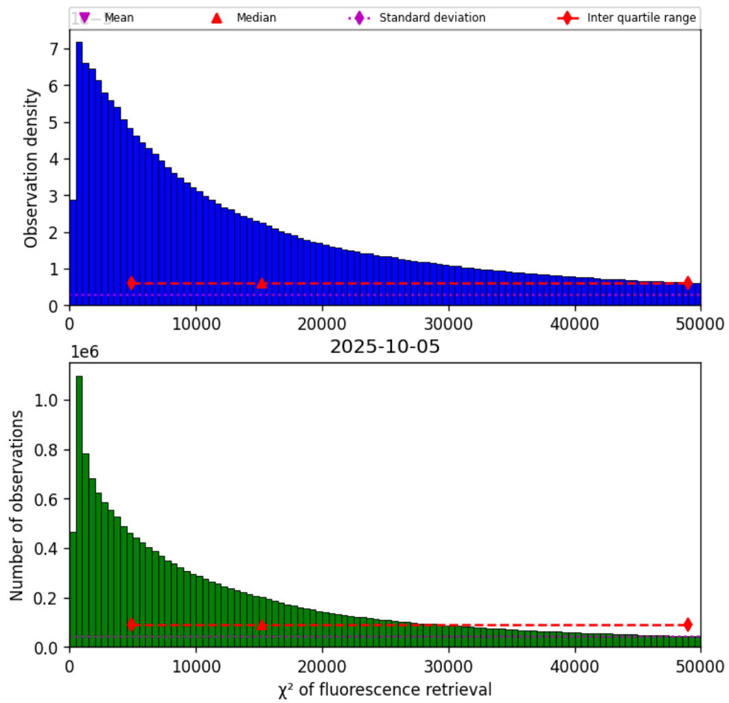
Figure 40: Histogram of “ \chi^2 of fluorescence retrieval” for 2025-10-05 to 2025-10-06
