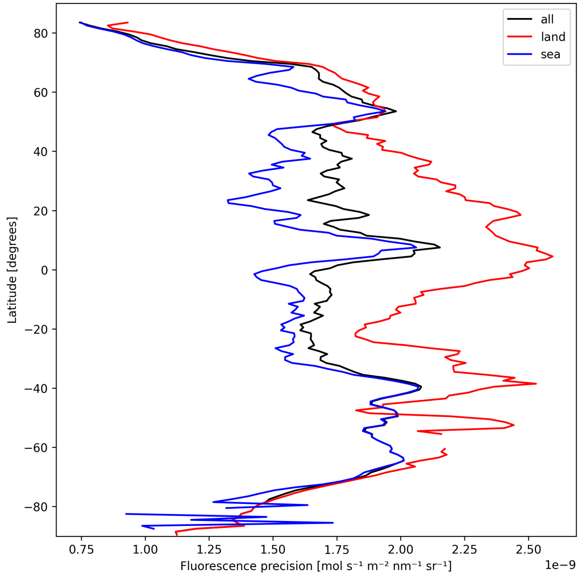
Figure 22: Zonal average of “Fluorescence precision” for 2025-10-05 to 2025-10-06.
