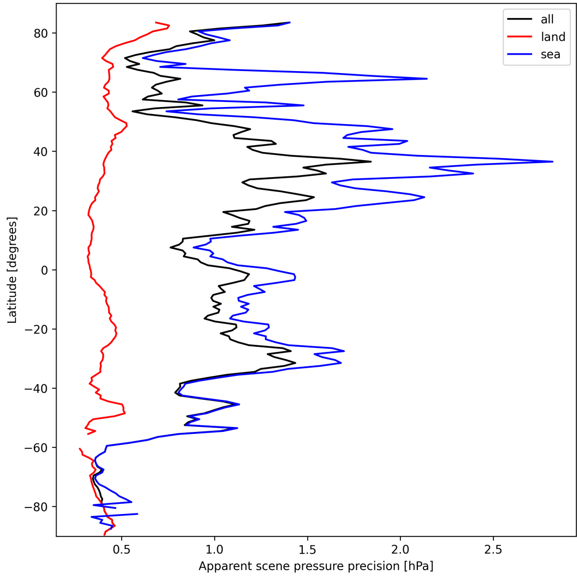
Figure 18: Zonal average of “Apparent scene pressure precision” for 2025-10-05 to 2025-10-06.
