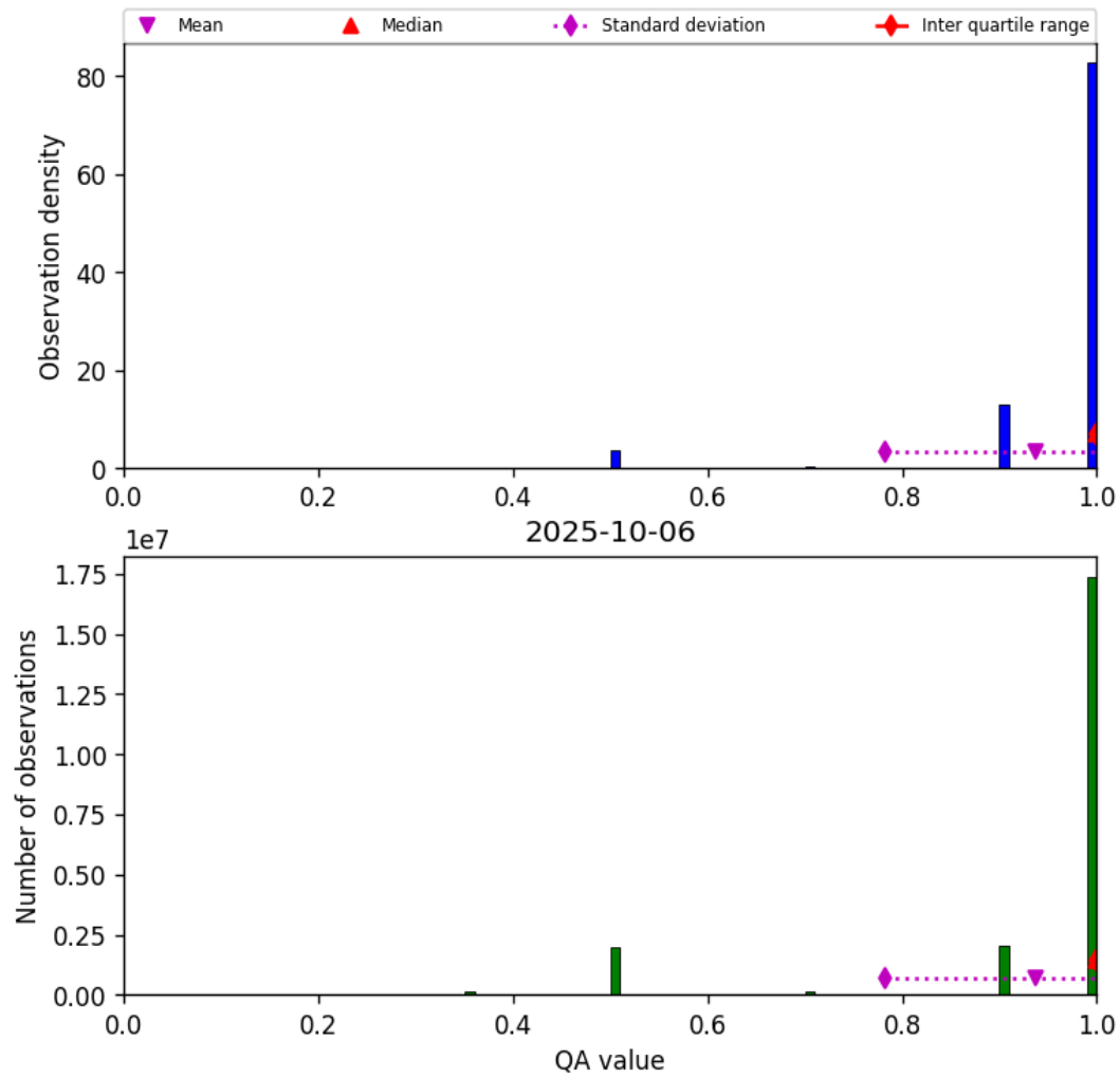
Figure 27: Histogram of “QA value” for 2025-10-06 to 2025-10-07
