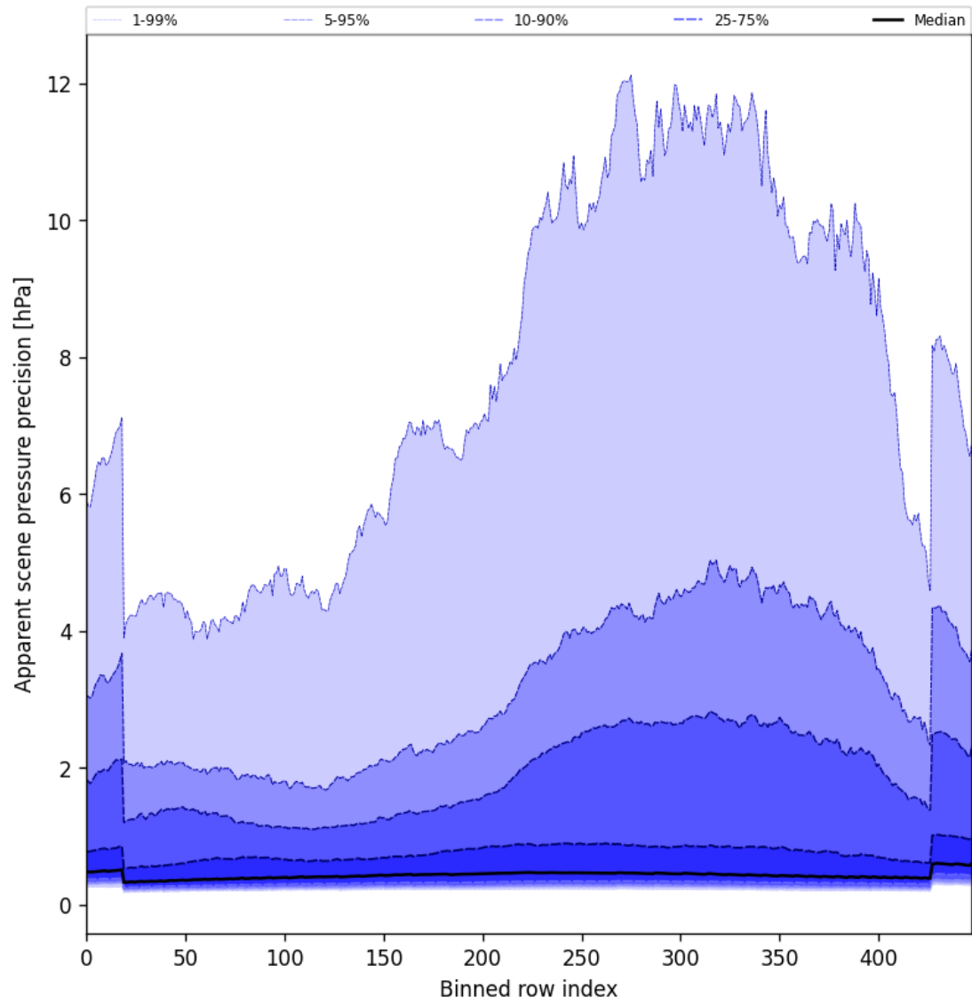
Figure 52: Along track statistics of “Apparent scene pressure precision” for 2025-10-06 to 2025-10-07
