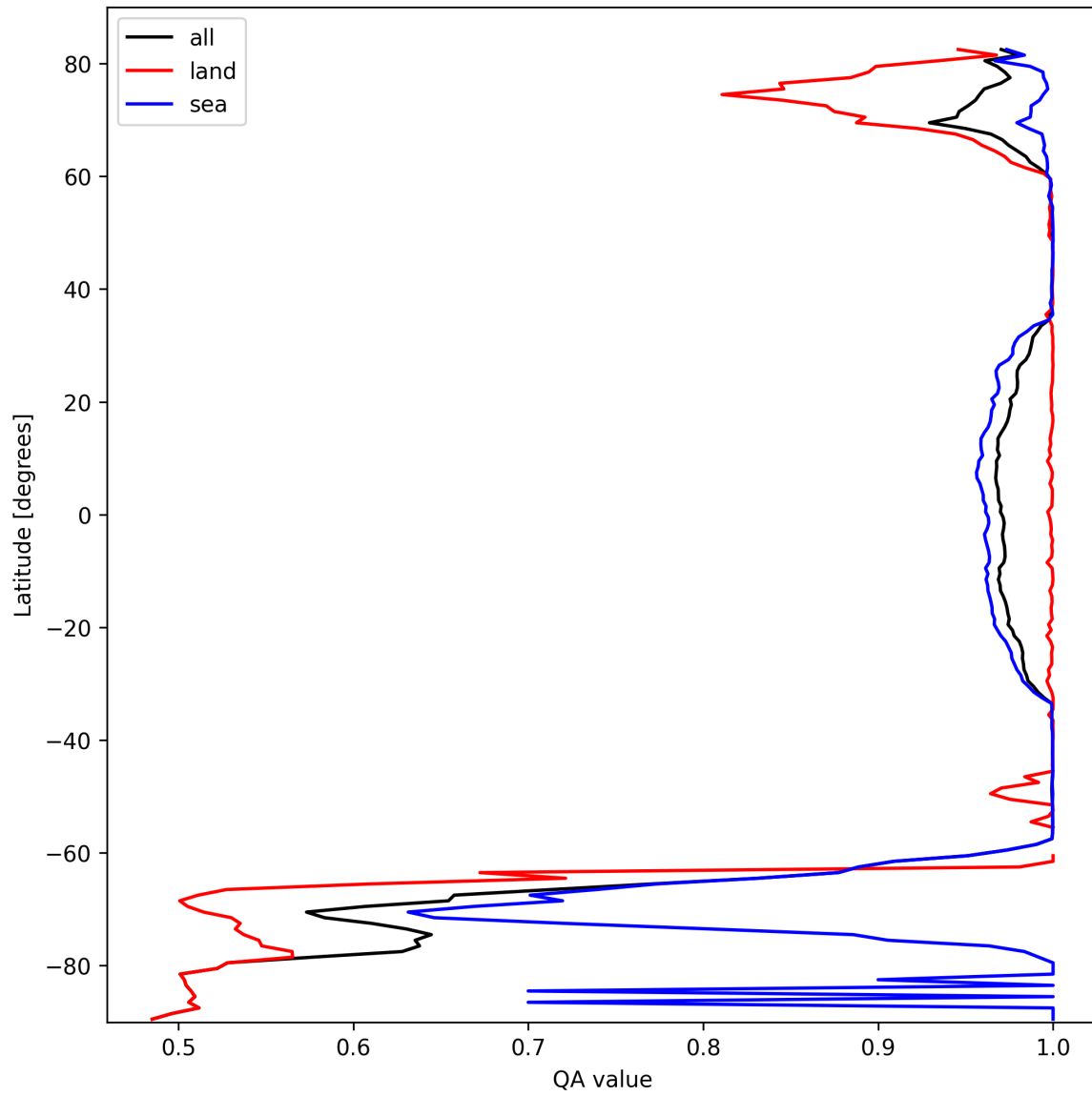
Figure 10: Zonal average of “QA value” for 2025-10-06 to 2025-10-07.
