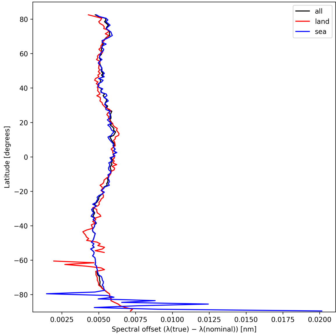
Figure 26: Zonal average of “Spectral offset ( \lambda_{\text{true}} - \lambda_{\text{nominal}} )” for 2025-10-06 to 2025-10-07.
