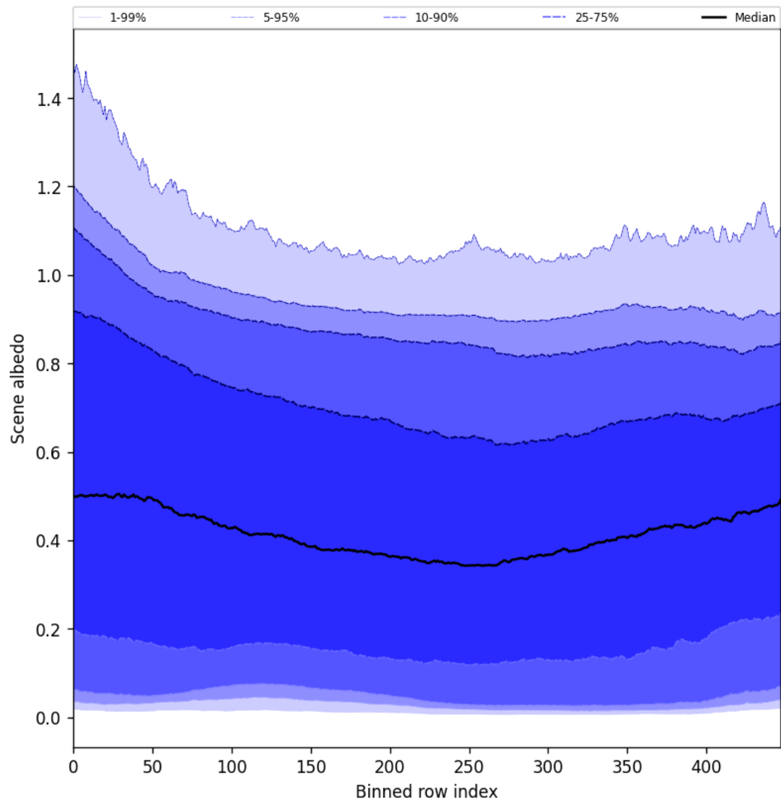
Figure 49: Along track statistics of “Scene albedo” for 2025-10-06 to 2025-10-07
