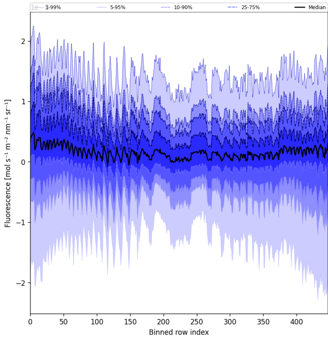
Figure 55: Along track statistics of “Fluorescence” for 2025-10-06 to 2025-10-07
