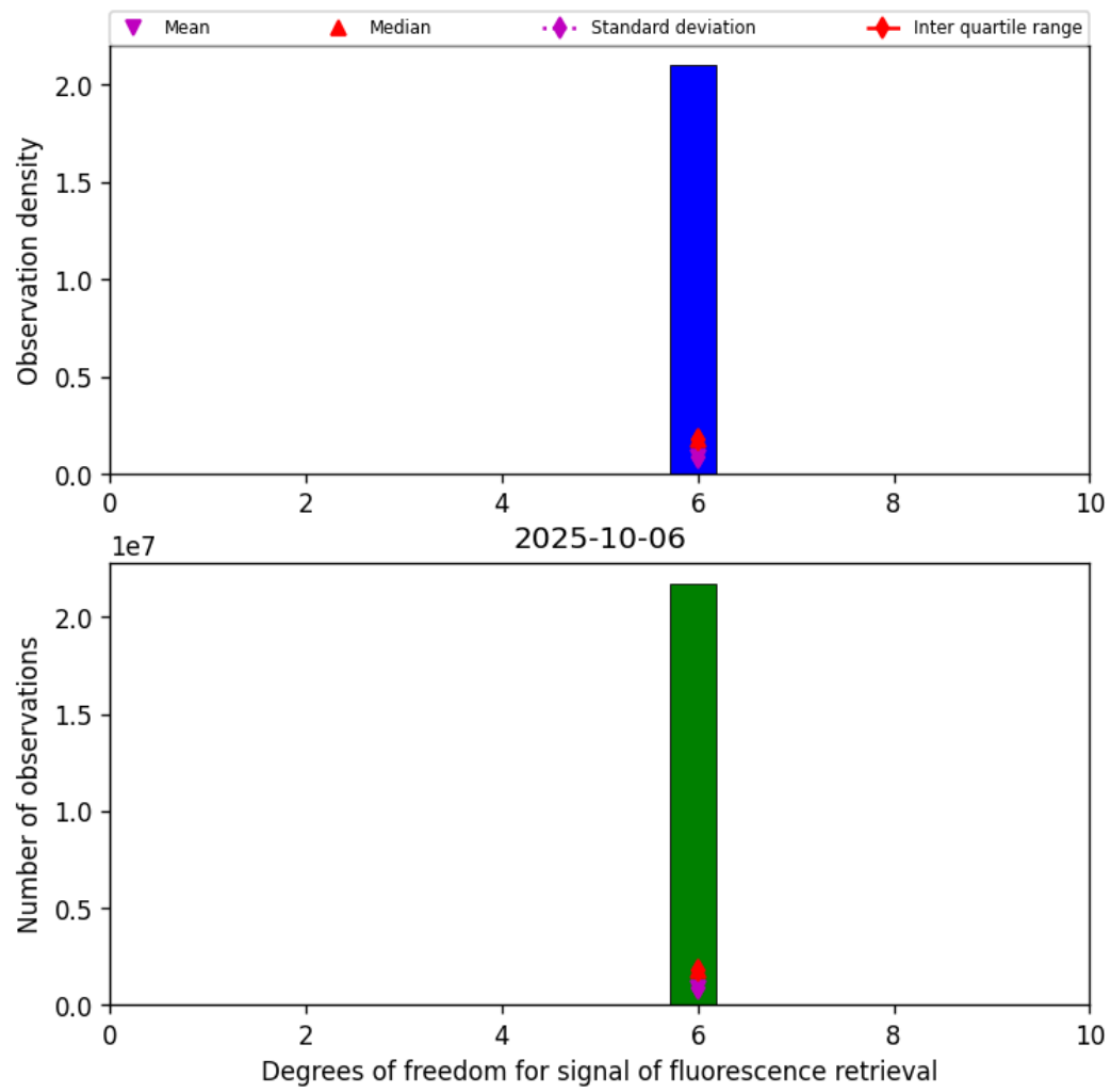
Figure 41: Histogram of "Degrees of freedom for signal of fluorescence retrieval" for 2025-10-06 to 2025-10-07
