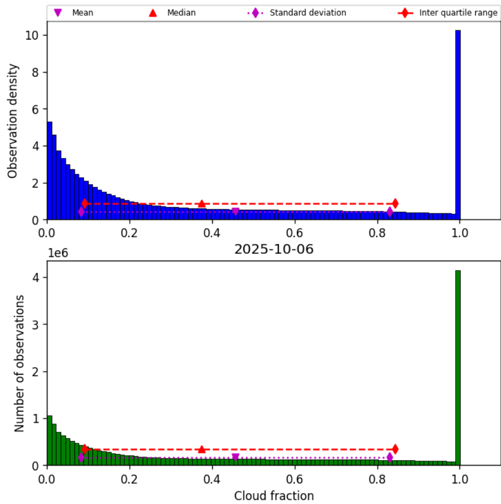
Figure 30: Histogram of “Cloud fraction” for 2025-10-06 to 2025-10-07
