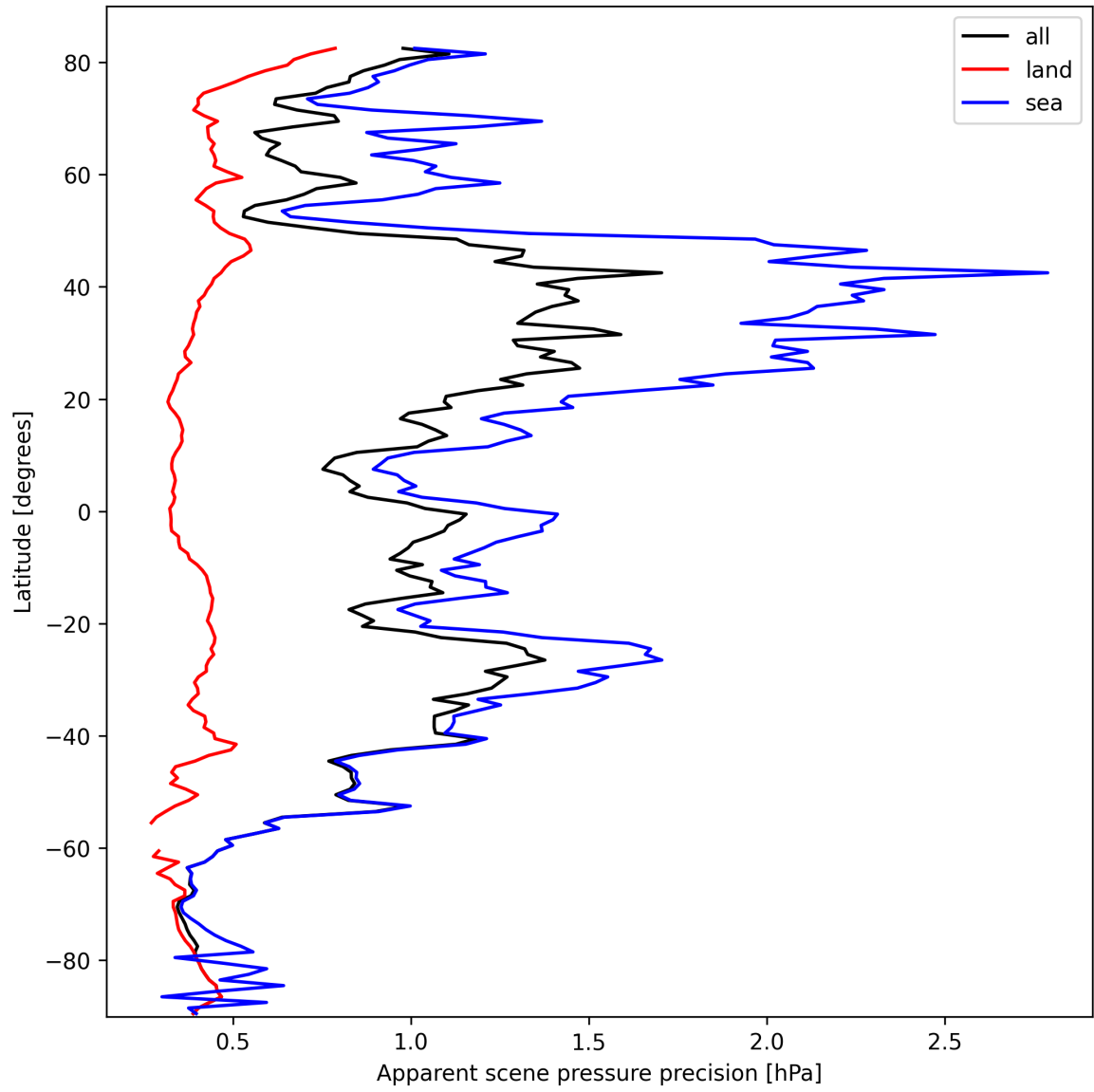
Figure 18: Zonal average of “Apparent scene pressure precision” for 2025-10-06 to 2025-10-07.
