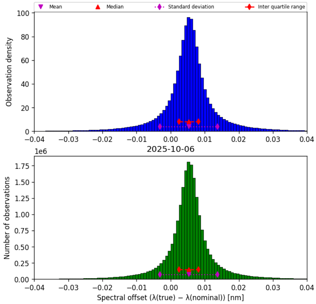
Figure 43: Histogram of “Spectral offset ( \lambda_{\text{true}} - \lambda_{\text{nominal}} )” for 2025-10-06 to 2025-10-07
