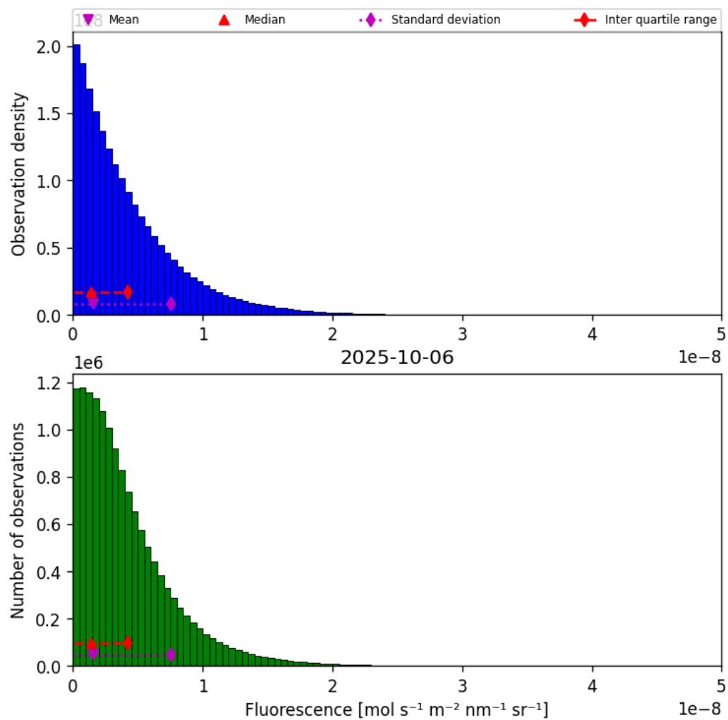
Figure 38: Histogram of “Fluorescence” for 2025-10-06 to 2025-10-07
