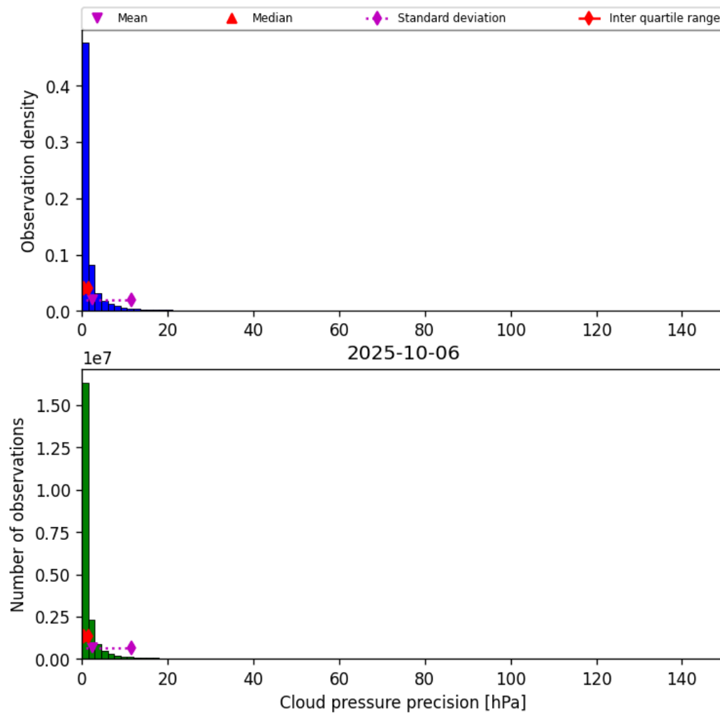
Figure 29: Histogram of “Cloud pressure precision” for 2025-10-06 to 2025-10-07
