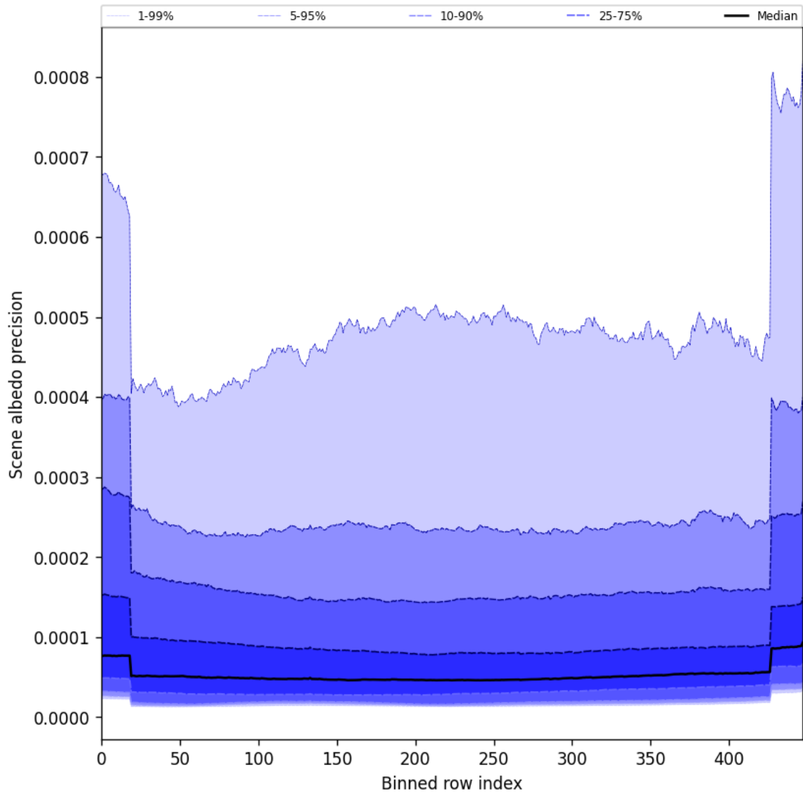
Figure 50: Along track statistics of “Scene albedo precision” for 2025-10-06 to 2025-10-07
