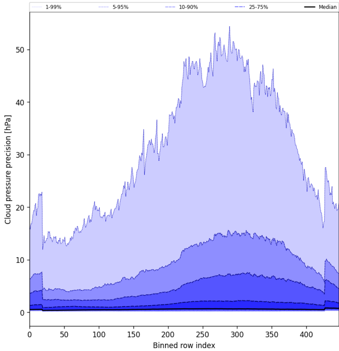
Figure 46: Along track statistics of “Cloud pressure precision” for 2025-10-06 to 2025-10-07
