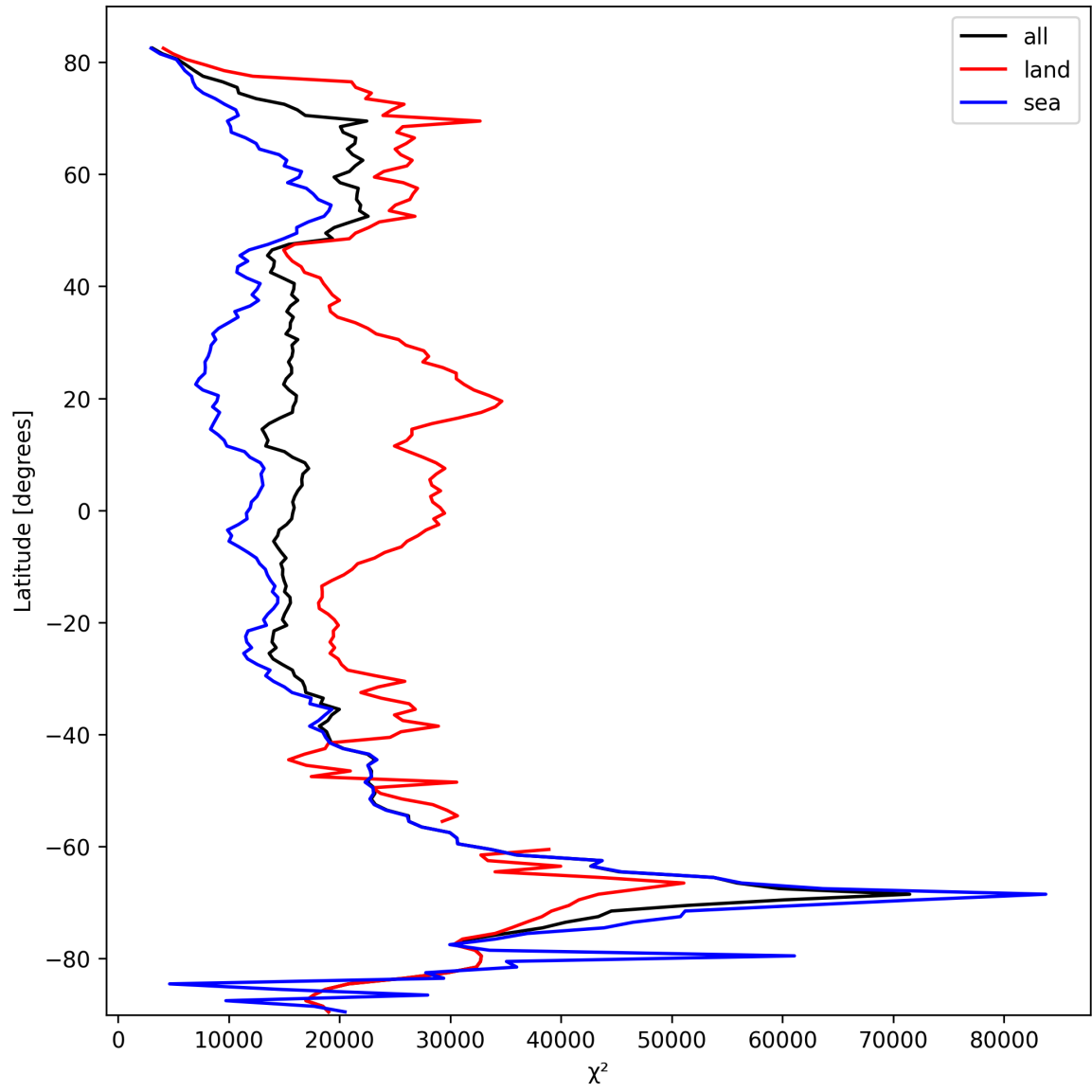
Figure 19: Zonal average of “ \chi^2 ” for 2025-10-06 to 2025-10-07.
