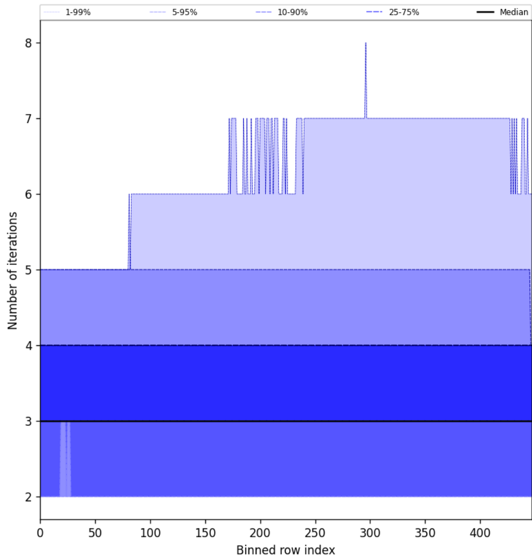
Figure 54: Along track statistics of “Number of iterations” for 2025-10-06 to 2025-10-07
