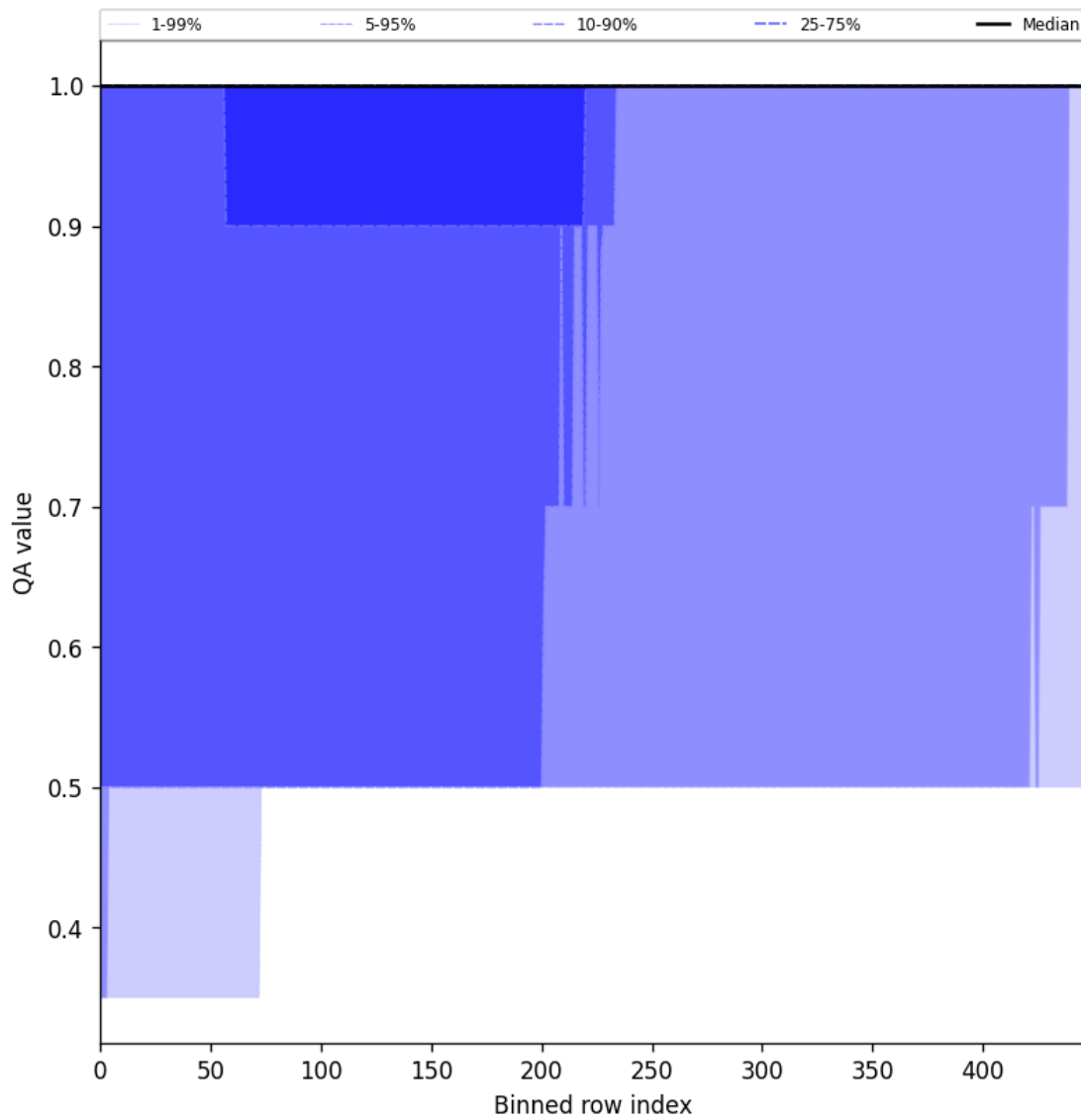
Figure 44: Along track statistics of “QA value” for 2025-10-06 to 2025-10-07
