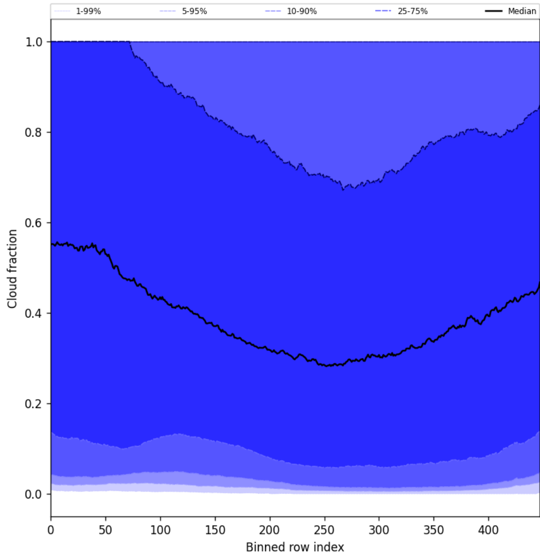
Figure 47: Along track statistics of “Cloud fraction” for 2025-10-06 to 2025-10-07
