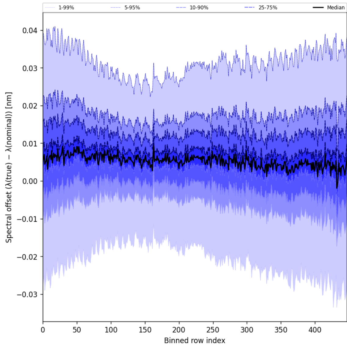
Figure 60: Along track statistics of “Spectral offset ( \lambda_{\text{true}} - \lambda_{\text{nominal}} )” for 2025-10-06 to 2025-10-07
