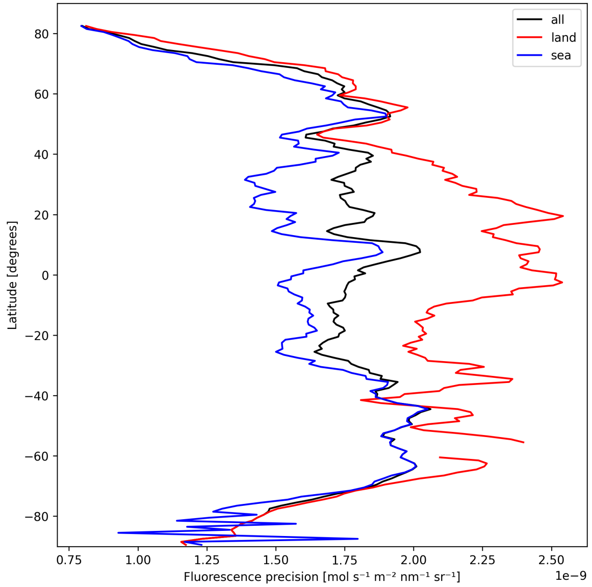
Figure 22: Zonal average of “Fluorescence precision” for 2025-10-06 to 2025-10-07.
