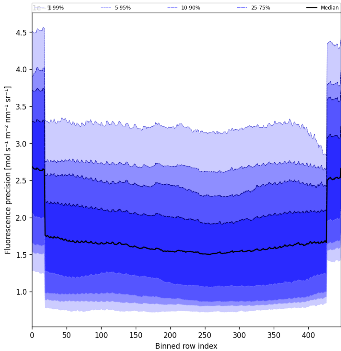
Figure 56: Along track statistics of “Fluorescence precision” for 2025-10-06 to 2025-10-07
