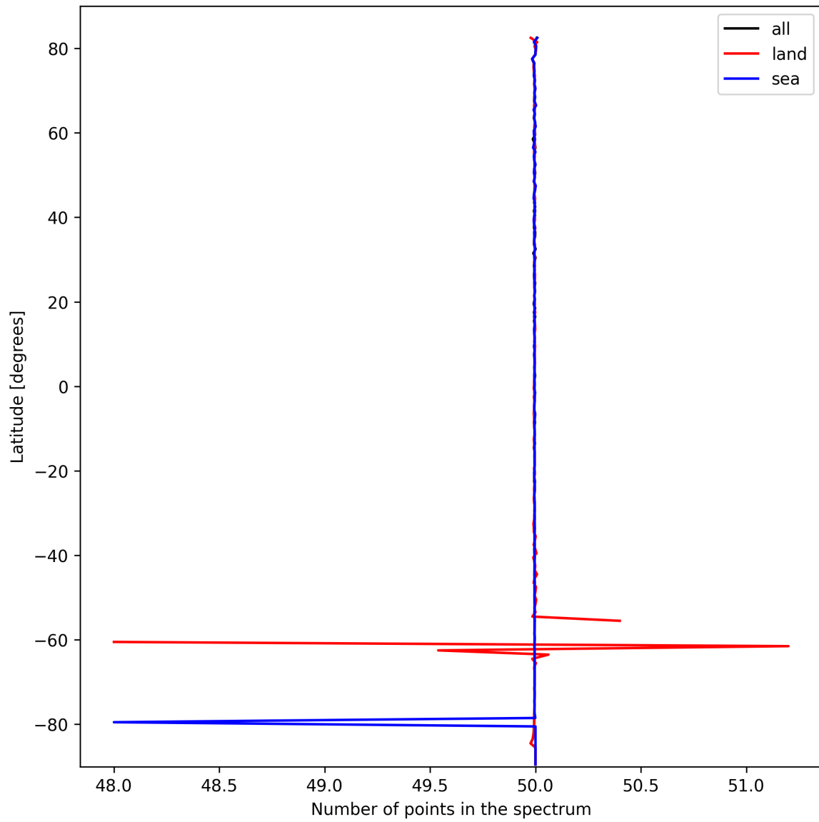
Figure 25: Zonal average of “Number of points in the spectrum” for 2025-10-06 to 2025-10-07.
