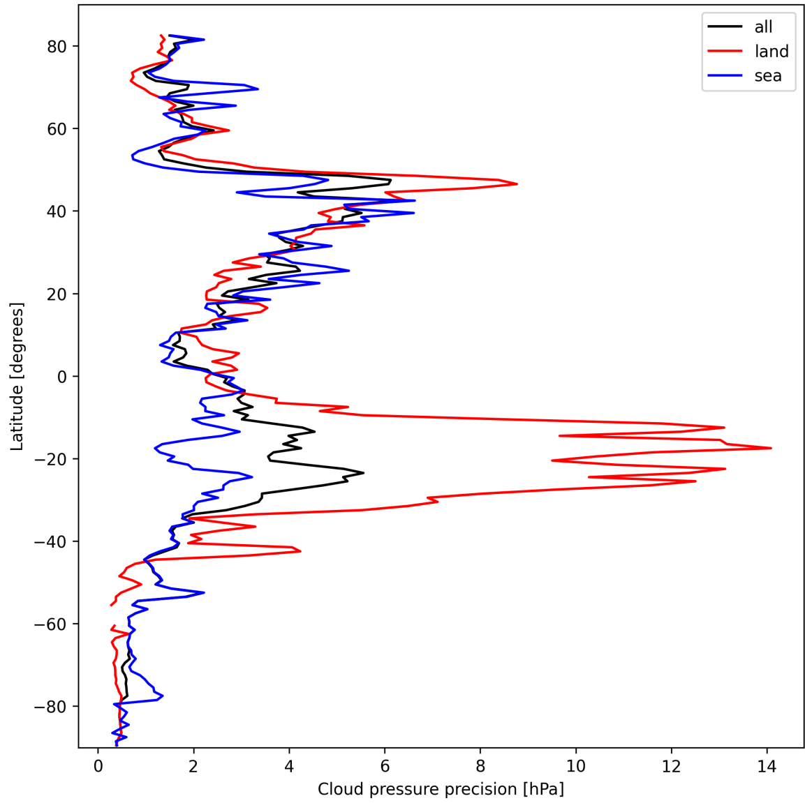
Figure 12: Zonal average of "Cloud pressure precision" for 2025-10-06 to 2025-10-07.
