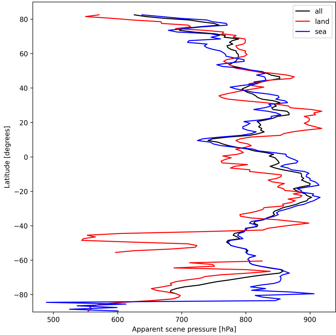
Figure 17: Zonal average of “Apparent scene pressure” for 2025-10-06 to 2025-10-07.
