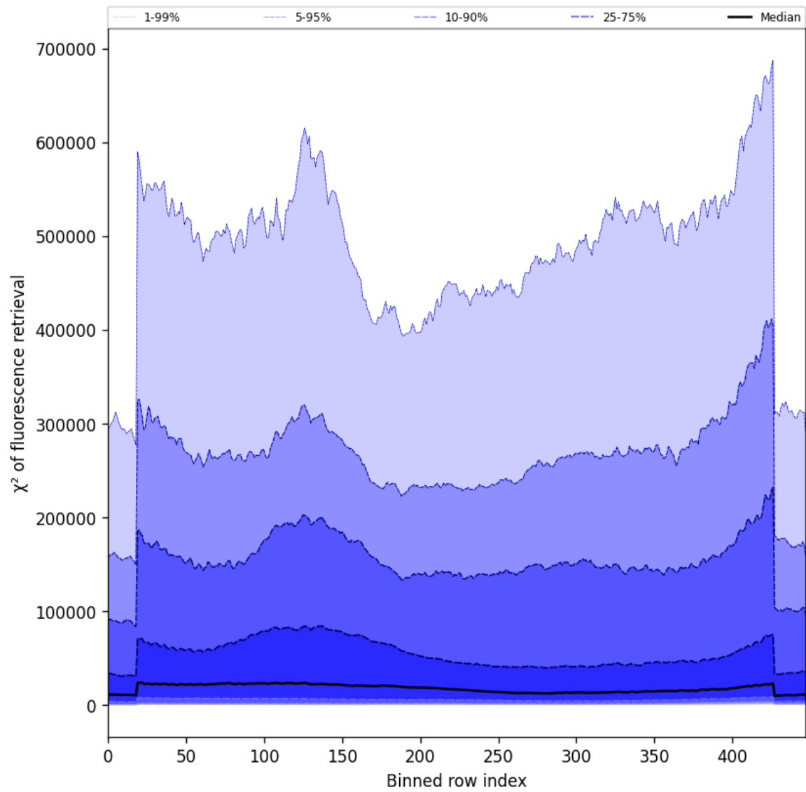
Figure 57: Along track statistics of “ \chi^2 of fluorescence retrieval” for 2025-10-06 to 2025-10-07
