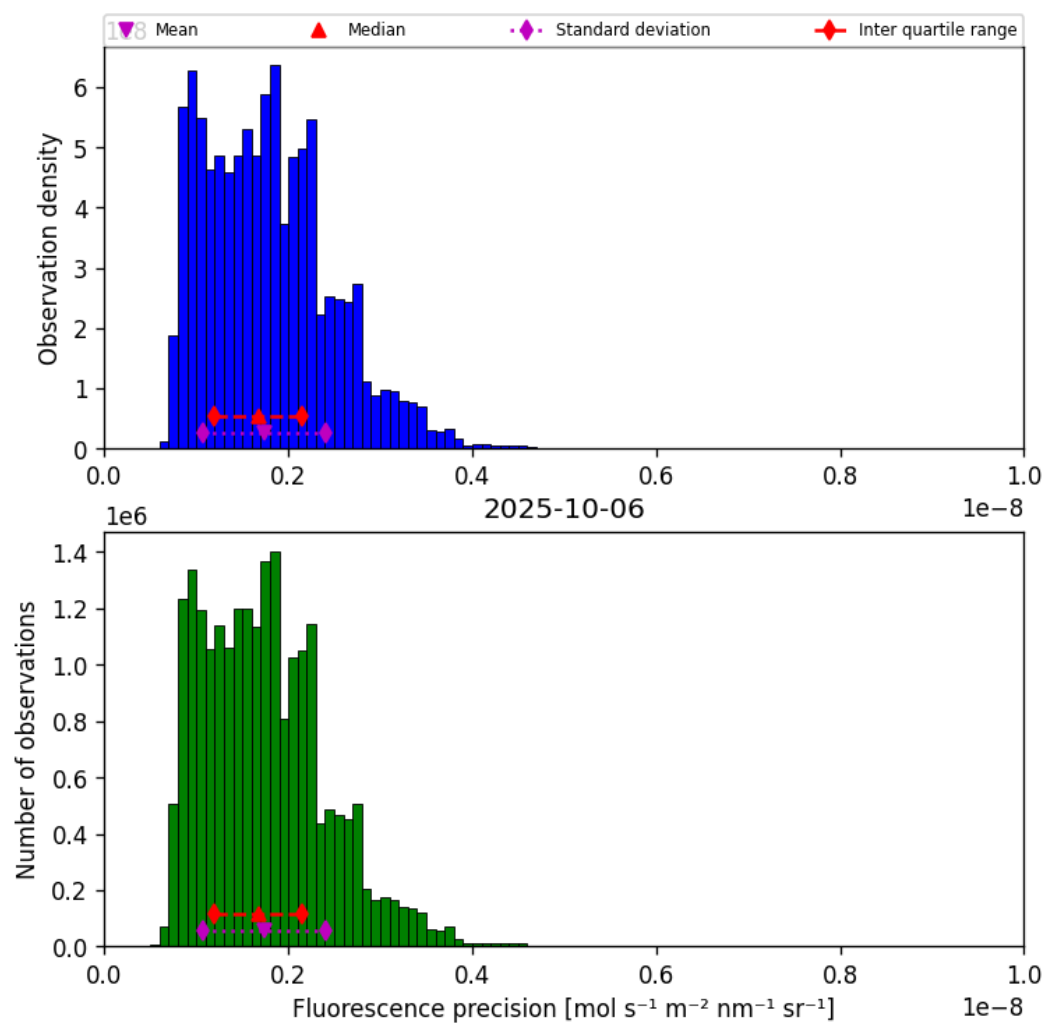
Figure 39: Histogram of “Fluorescence precision” for 2025-10-06 to 2025-10-07
