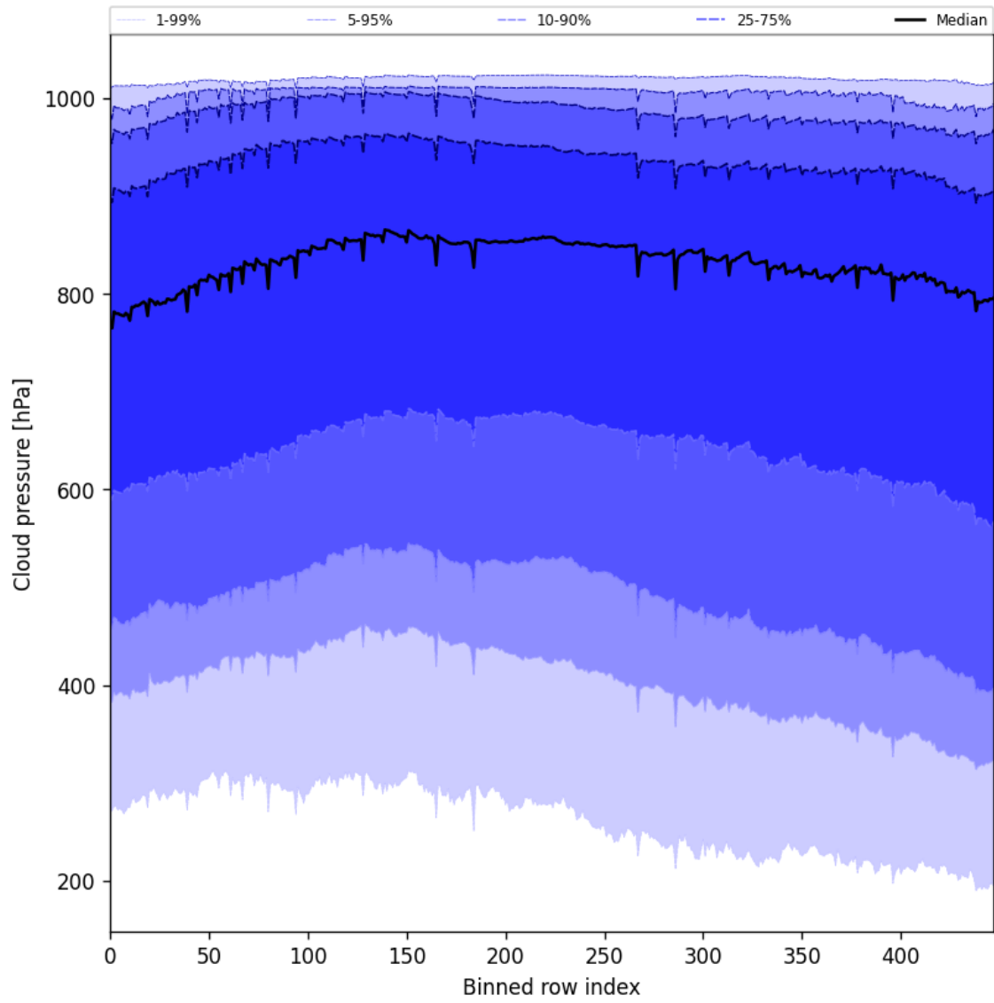
Figure 45: Along track statistics of “Cloud pressure” for 2025-10-06 to 2025-10-07
