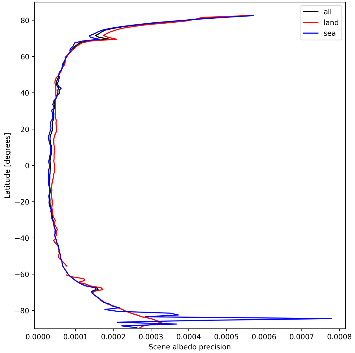
Figure 16: Zonal average of “Scene albedo precision” for 2025-10-06 to 2025-10-07.
