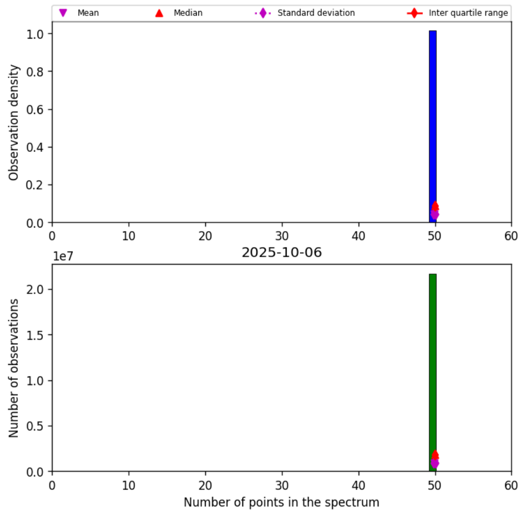
Figure 42: Histogram of “Number of points in the spectrum” for 2025-10-06 to 2025-10-07
