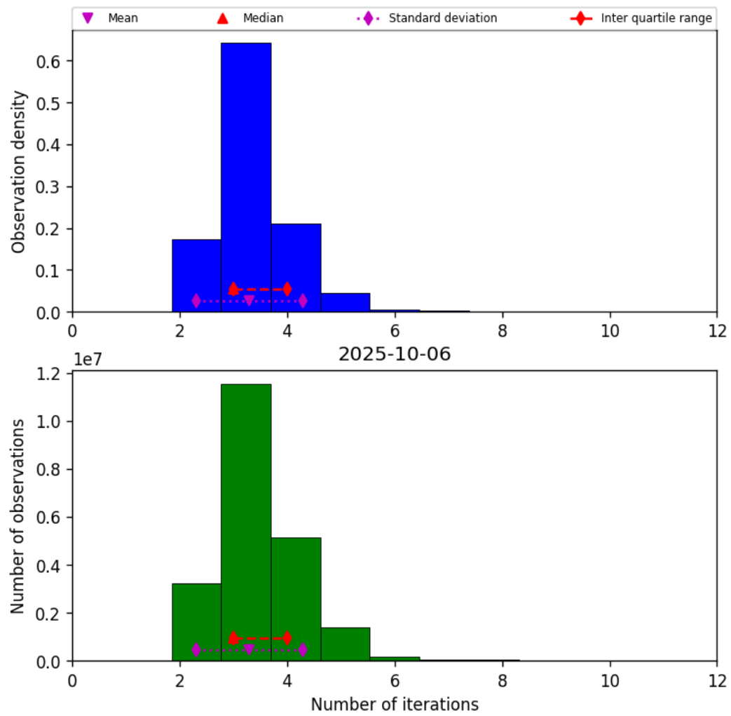
Figure 37: Histogram of “Number of iterations” for 2025-10-06 to 2025-10-07
