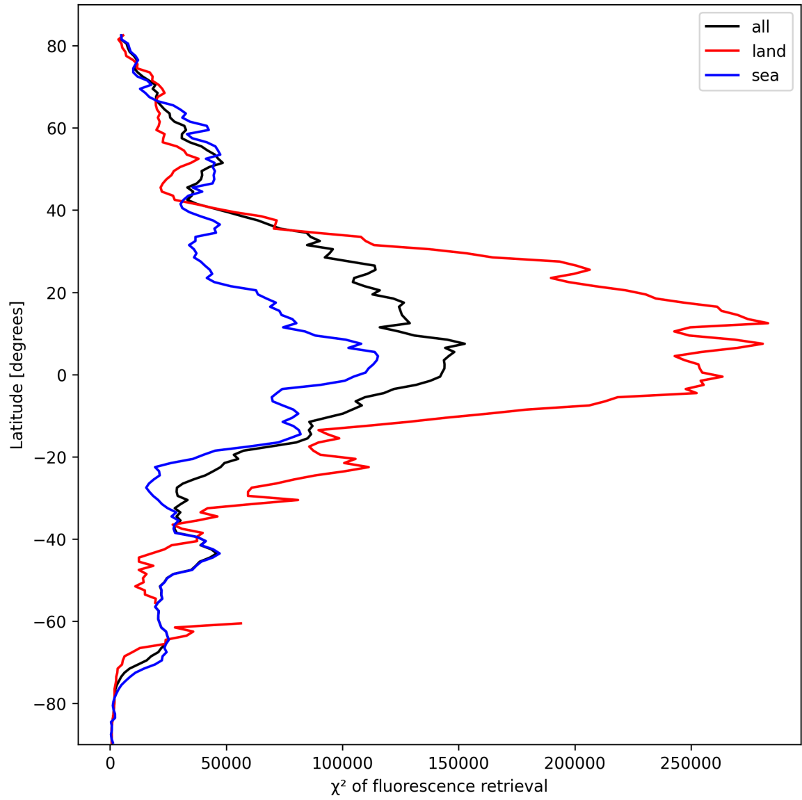
Figure 23: Zonal average of “ \chi^2 of fluorescence retrieval” for 2025-10-06 to 2025-10-07.
