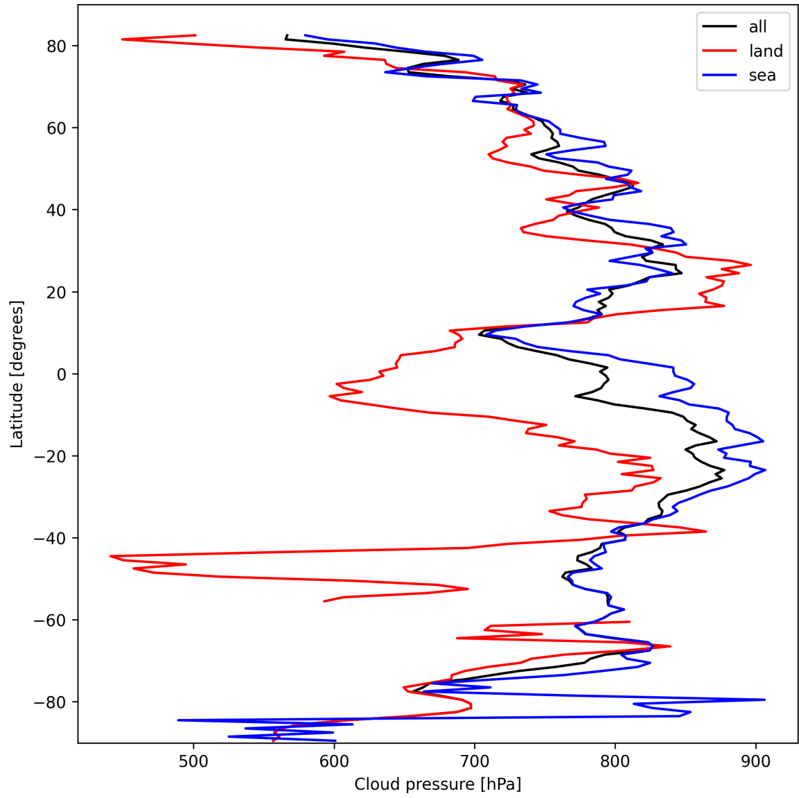
Figure 11: Zonal average of “Cloud pressure” for 2025-10-06 to 2025-10-07.
