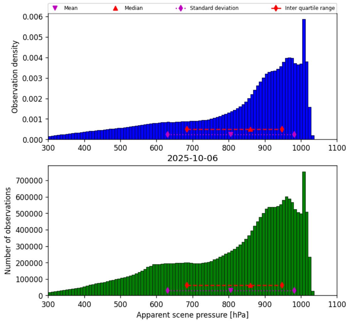
Figure 34: Histogram of “Apparent scene pressure” for 2025-10-06 to 2025-10-07
