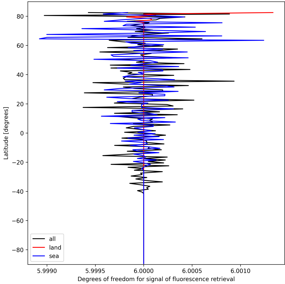
Figure 24: Zonal average of “Degrees of freedom for signal of fluorescence retrieval” for 2025-10-06 to 2025-10-07.
