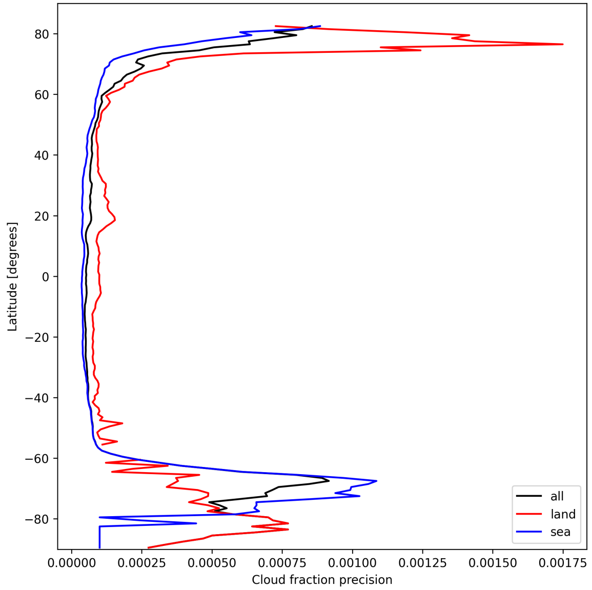
Figure 14: Zonal average of “Cloud fraction precision” for 2025-10-06 to 2025-10-07.
