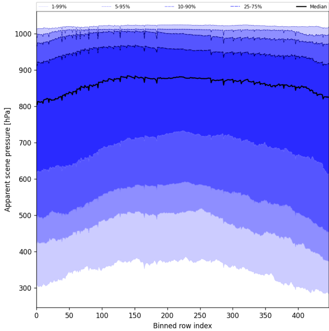
Figure 51: Along track statistics of “Apparent scene pressure” for 2025-10-06 to 2025-10-07
