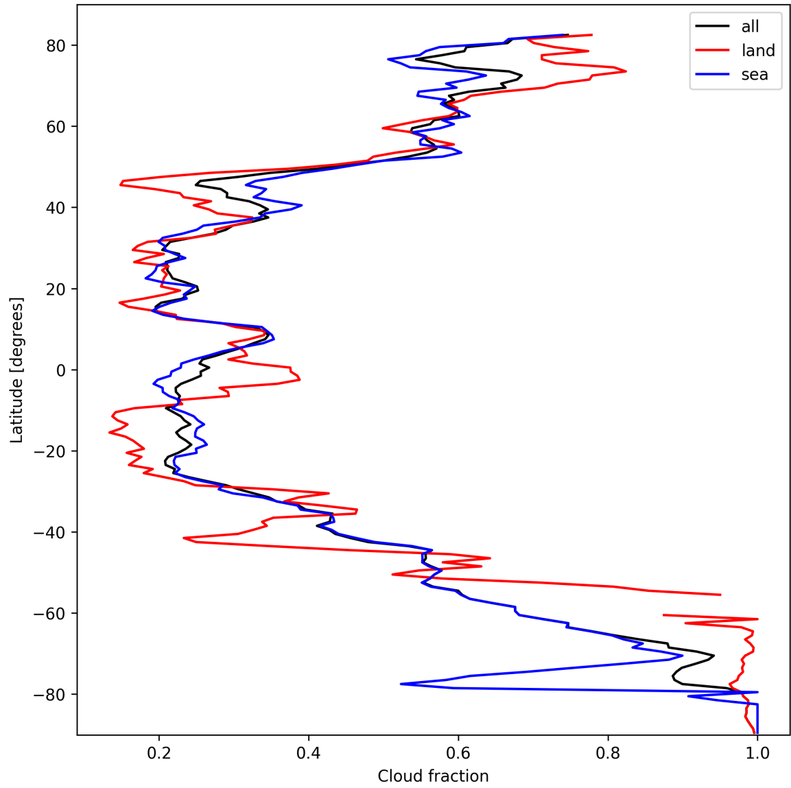
Figure 13: Zonal average of “Cloud fraction” for 2025-10-06 to 2025-10-07.
