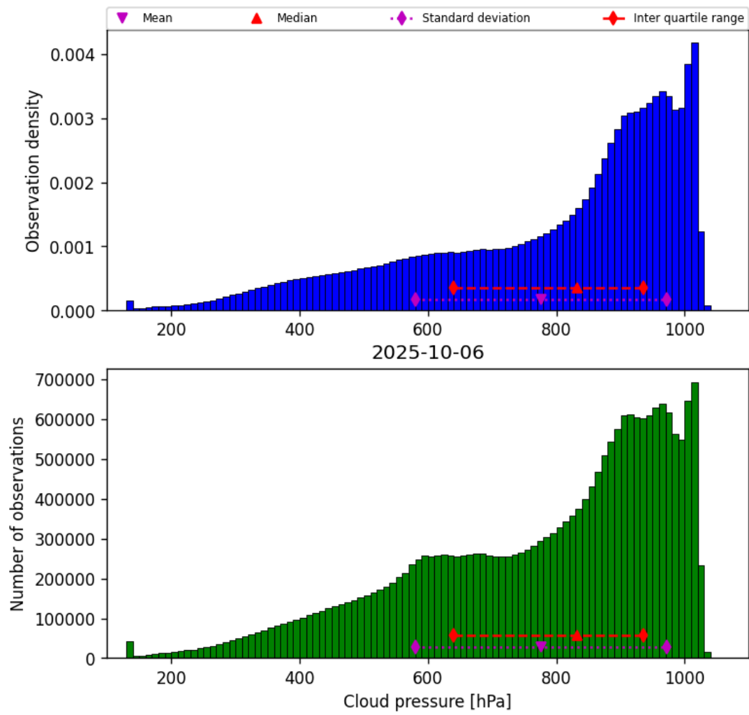
Figure 28: Histogram of “Cloud pressure” for 2025-10-06 to 2025-10-07
