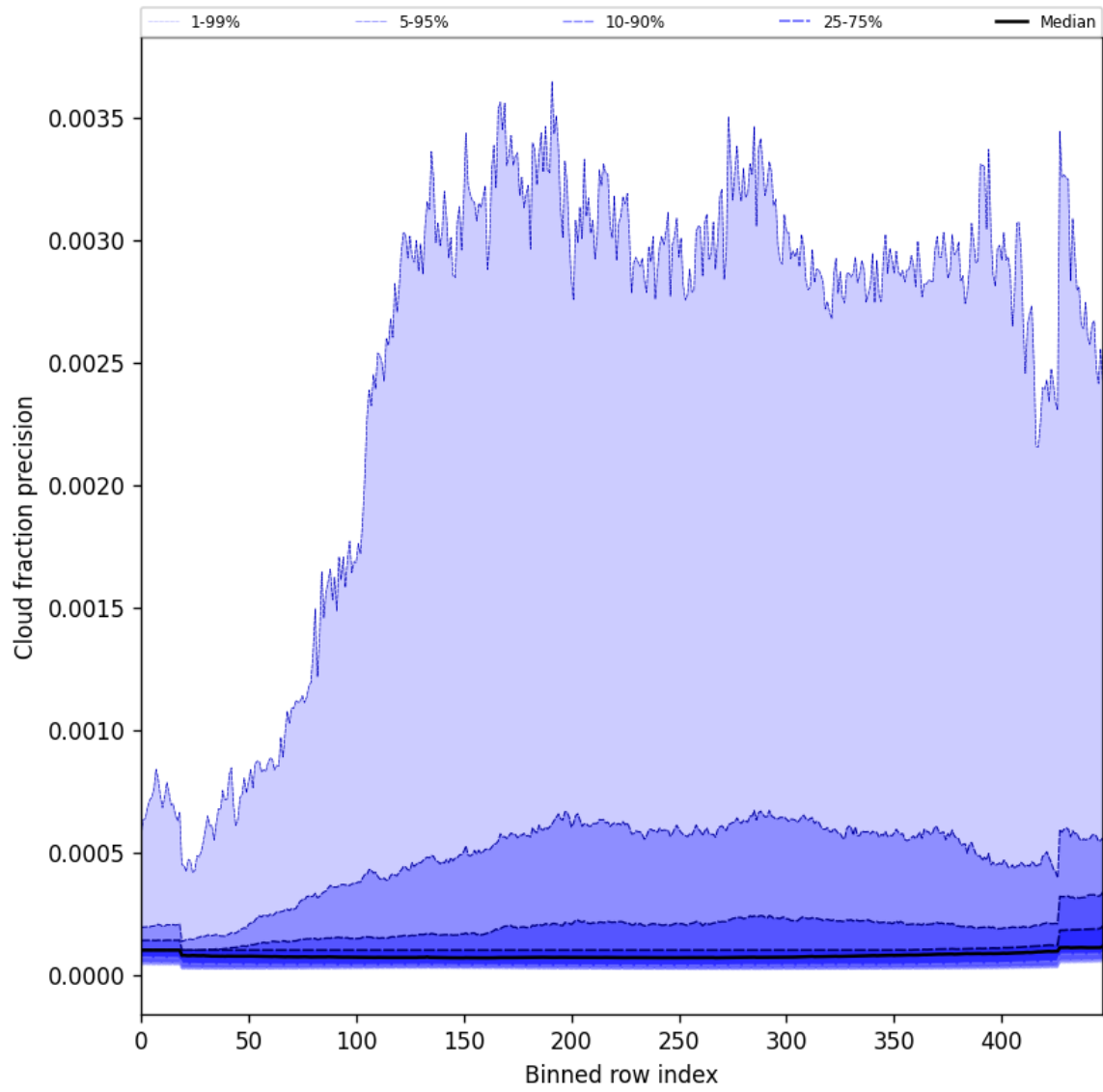
Figure 48: Along track statistics of “Cloud fraction precision” for 2025-10-06 to 2025-10-07
