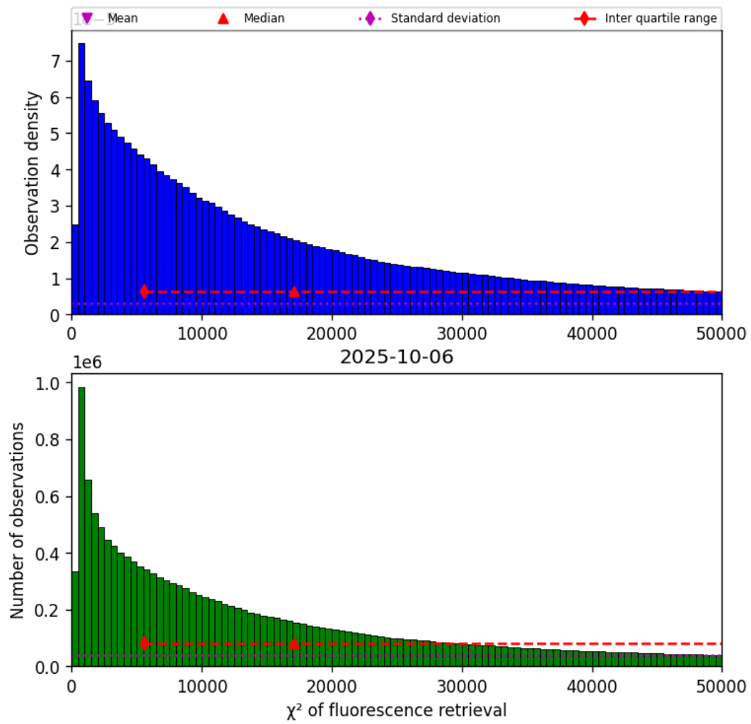
Figure 40: Histogram of “ \chi^2 of fluorescence retrieval” for 2025-10-06 to 2025-10-07
