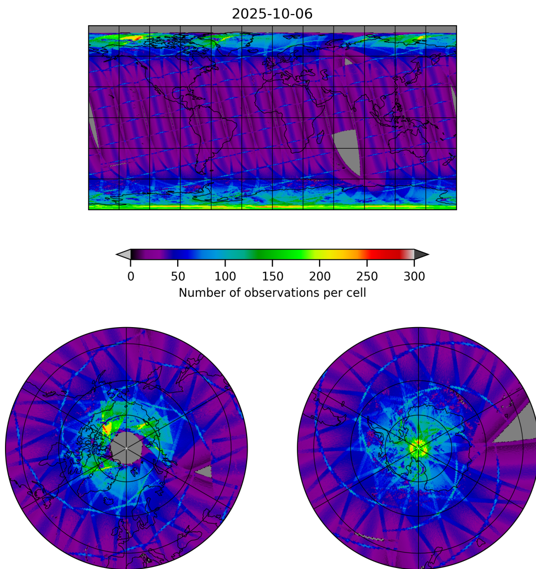
Figure 9: Map of the number of observations for 2025-10-06 to 2025-10-07
