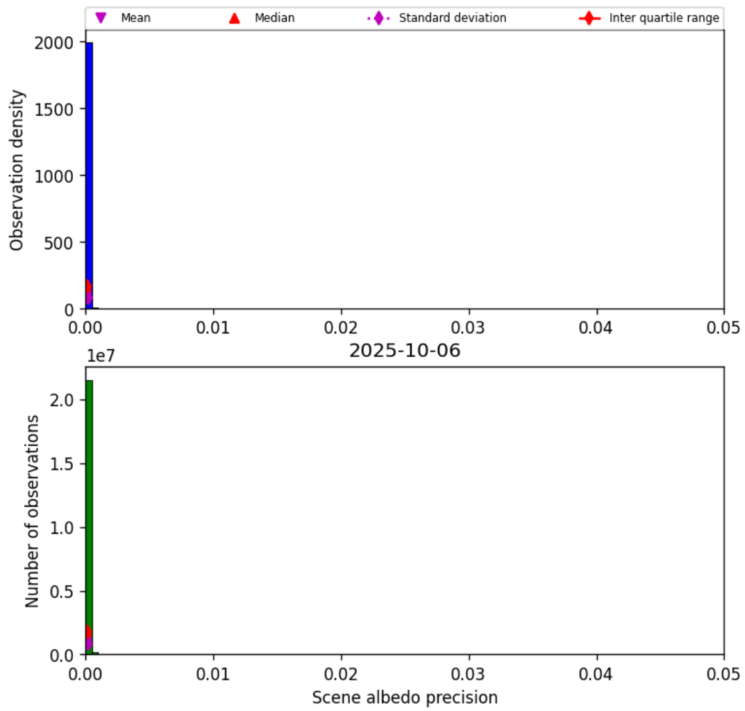
Figure 33: Histogram of “Scene albedo precision” for 2025-10-06 to 2025-10-07
