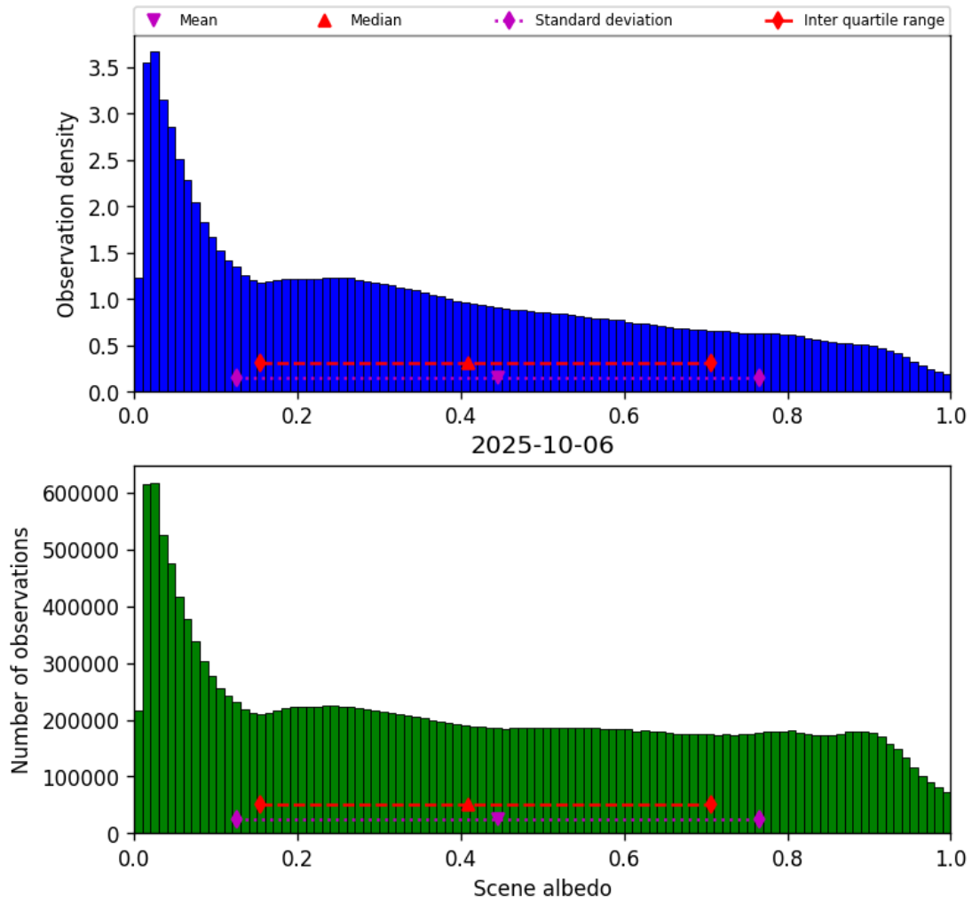
Figure 32: Histogram of “Scene albedo” for 2025-10-06 to 2025-10-07
