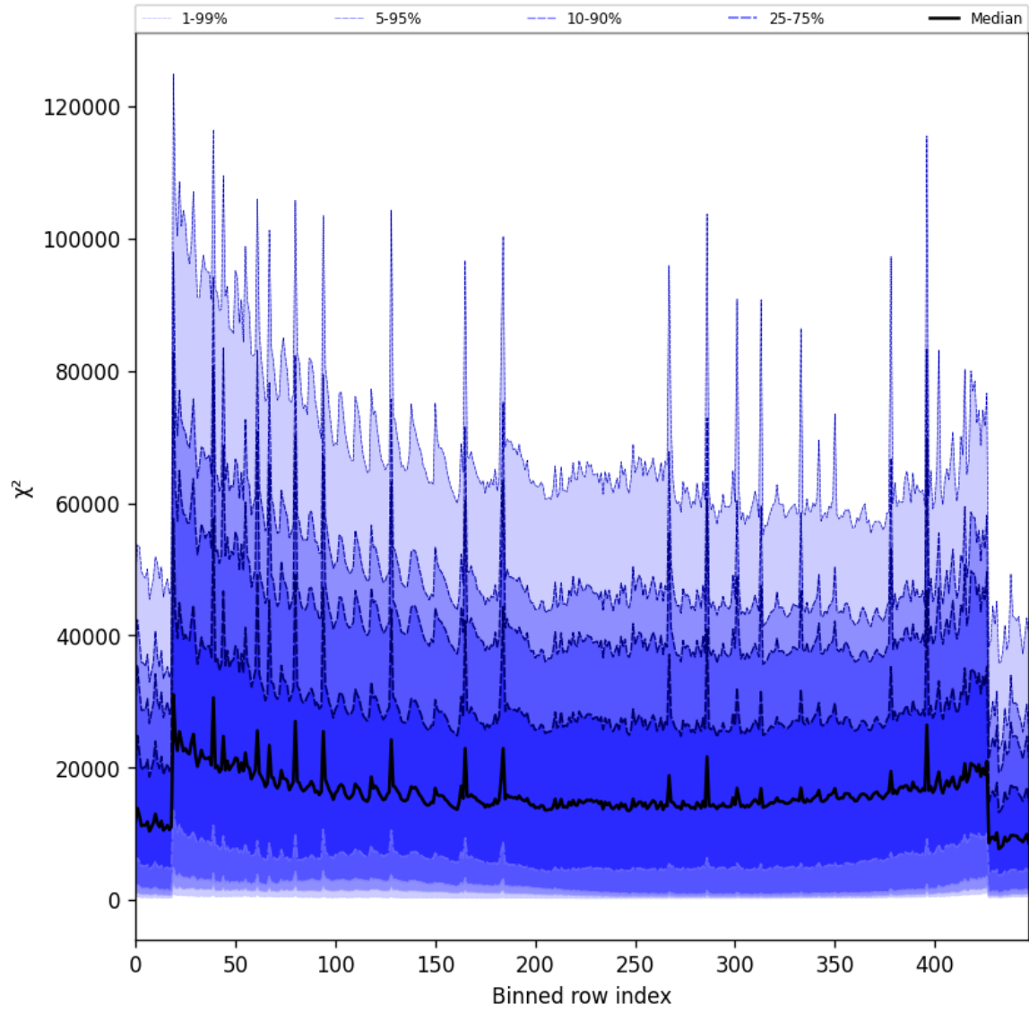
Figure 53: Along track statistics of “ \chi^2 ” for 2025-10-06 to 2025-10-07
