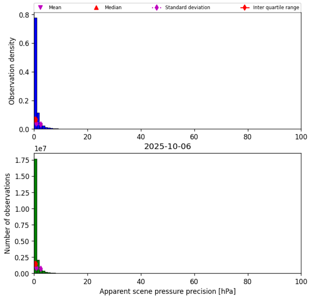
Figure 35: Histogram of “Apparent scene pressure precision” for 2025-10-06 to 2025-10-07
