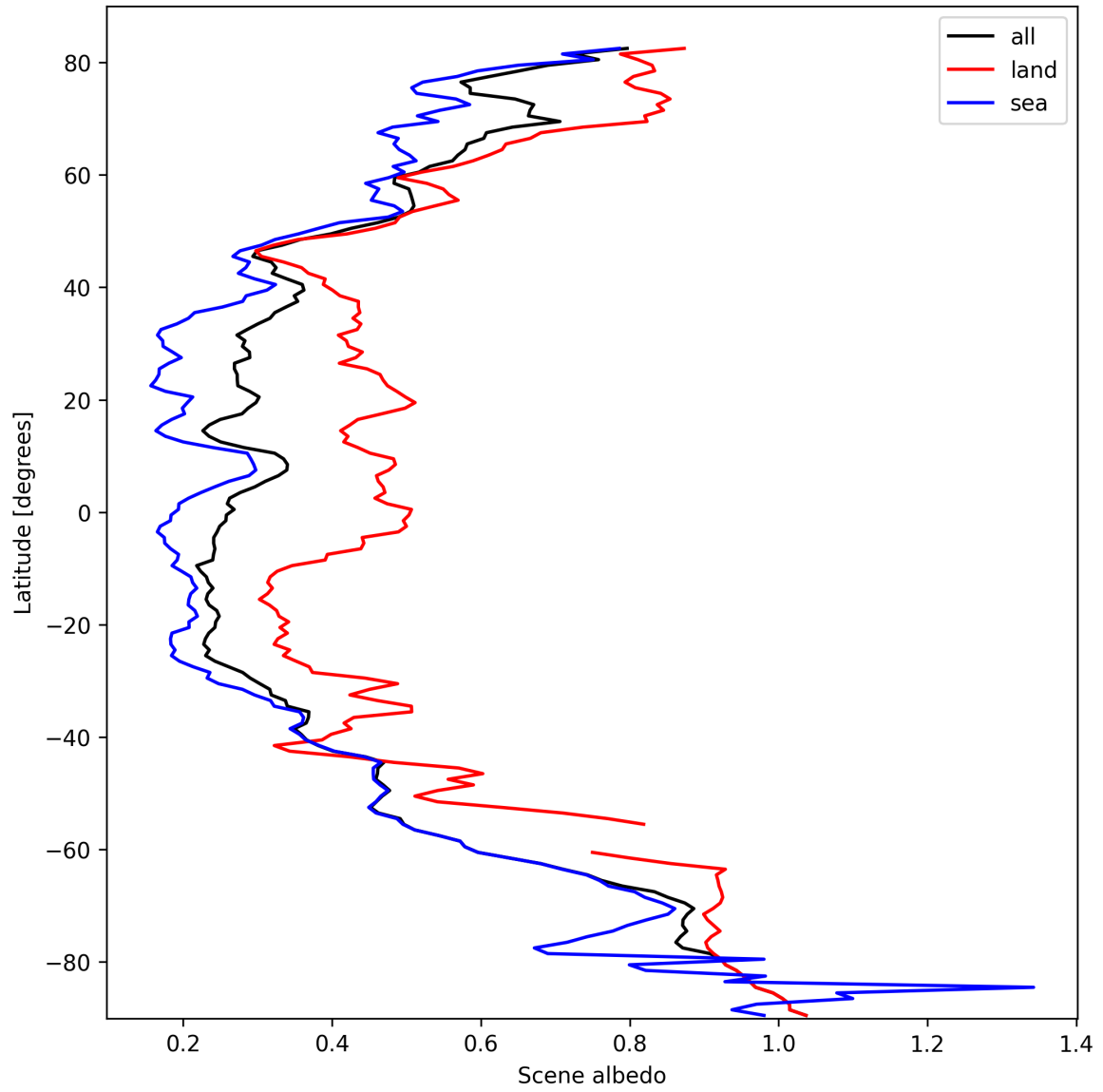
Figure 15: Zonal average of “Scene albedo” for 2025-10-06 to 2025-10-07.
