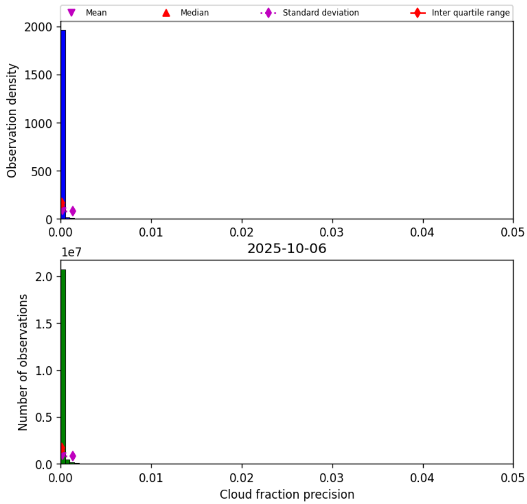
Figure 31: Histogram of “Cloud fraction precision” for 2025-10-06 to 2025-10-07
