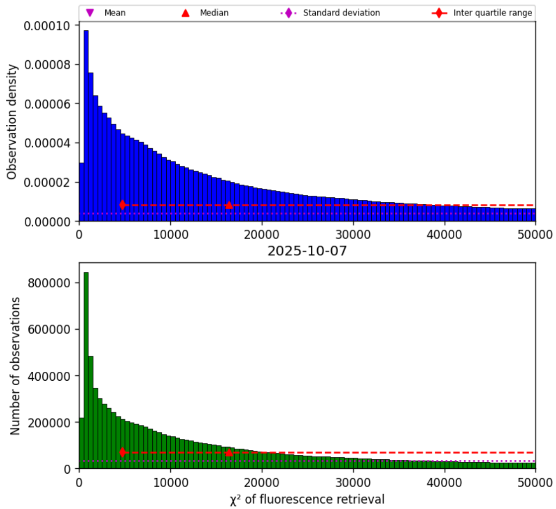
Figure 40: Histogram of “ \chi^2 of fluorescence retrieval” for 2025-10-07 to 2025-10-07
