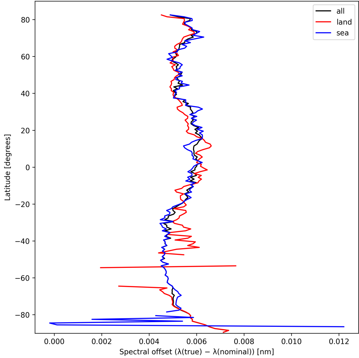
Figure 26: Zonal average of “Spectral offset ( \lambda_{\text{true}} - \lambda_{\text{nominal}} )” for 2025-10-07 to 2025-10-07.
