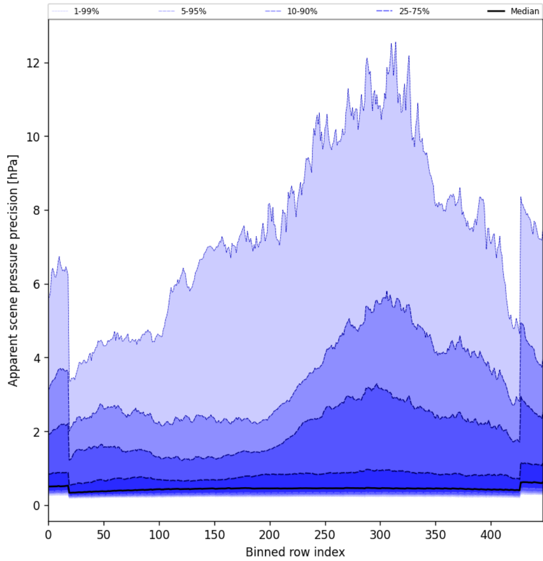
Figure 52: Along track statistics of “Apparent scene pressure precision” for 2025-10-07 to 2025-10-07
