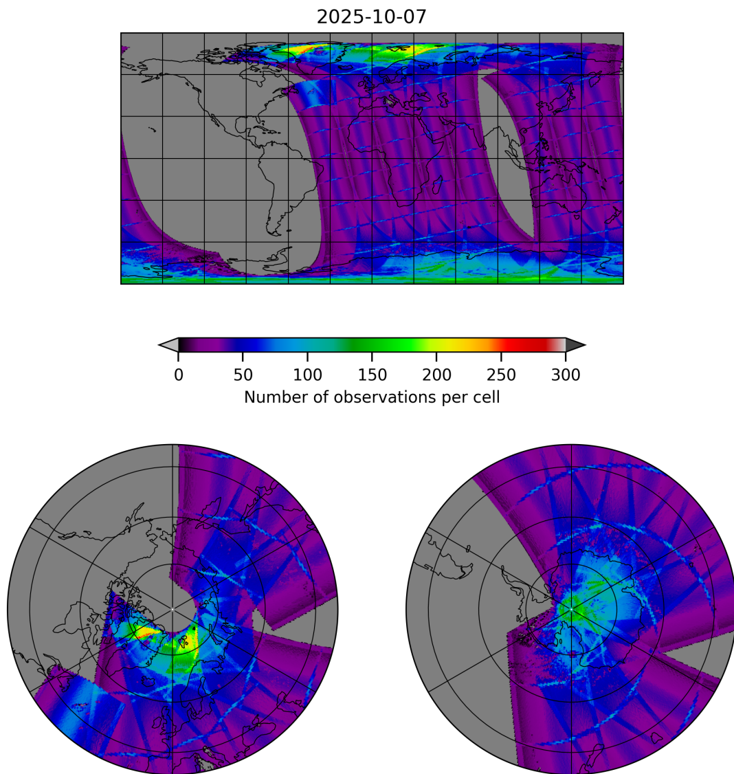
Figure 9: Map of the number of observations for 2025-10-07 to 2025-10-07
