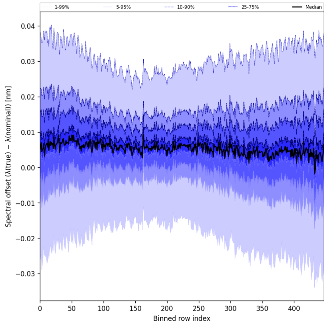
Figure 60: Along track statistics of “Spectral offset ( \lambda_{\text{true}} - \lambda_{\text{nominal}} )” for 2025-10-07 to 2025-10-07
