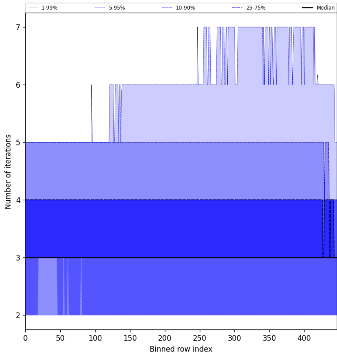
Figure 54: Along track statistics of “Number of iterations” for 2025-10-07 to 2025-10-07
