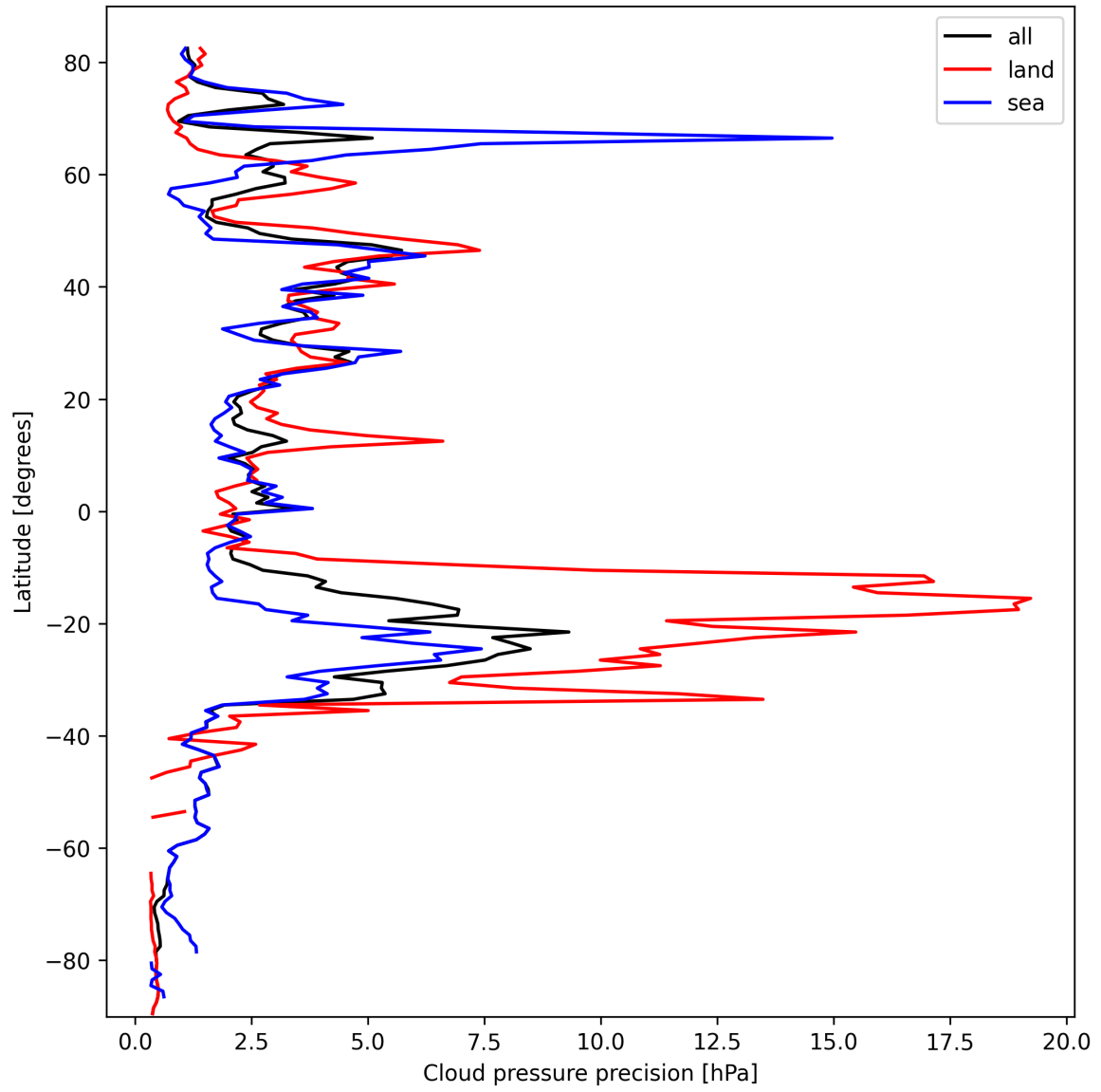
Figure 12: Zonal average of “Cloud pressure precision” for 2025-10-07 to 2025-10-07.
