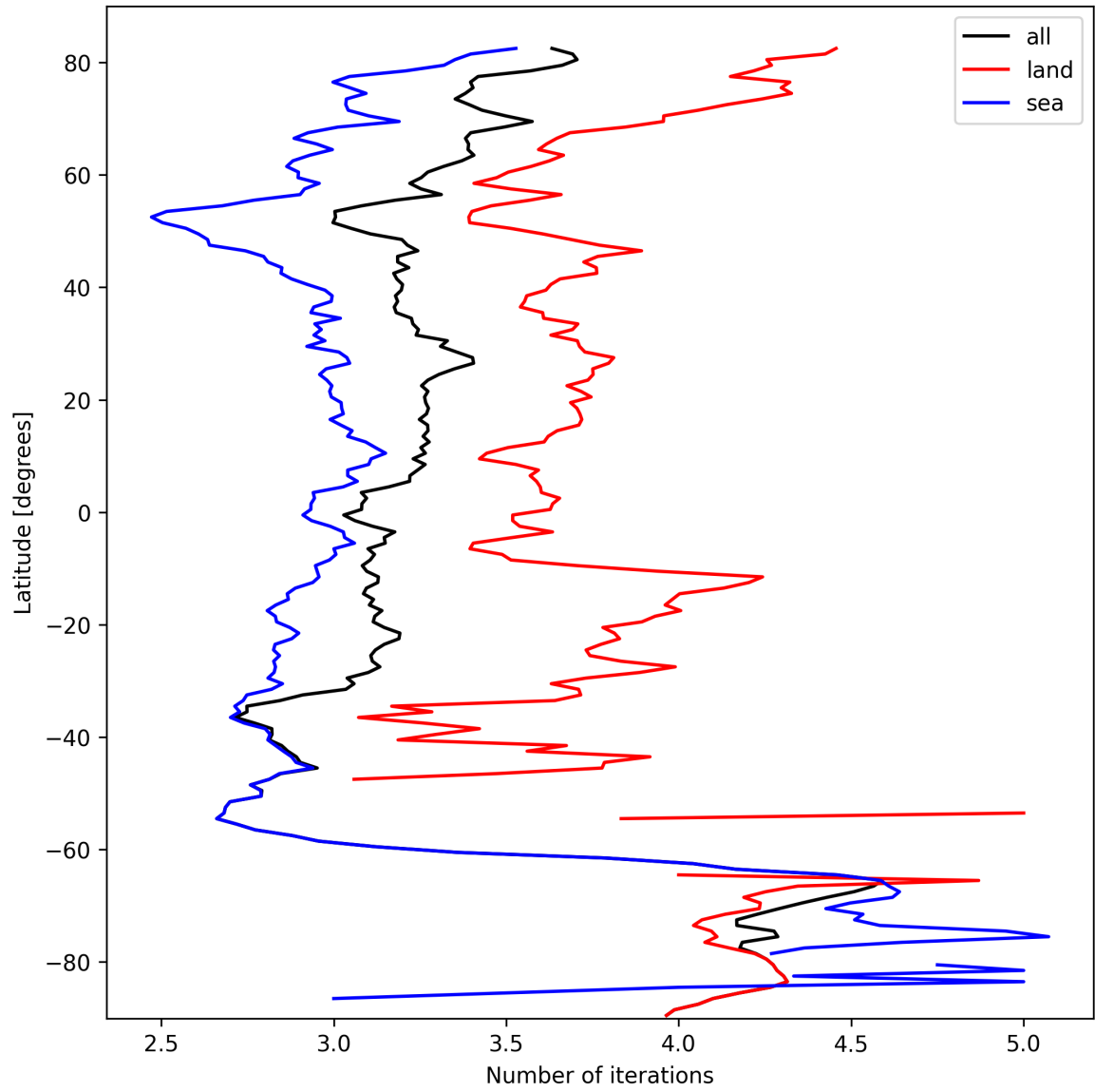
Figure 20: Zonal average of “Number of iterations” for 2025-10-07 to 2025-10-07.
