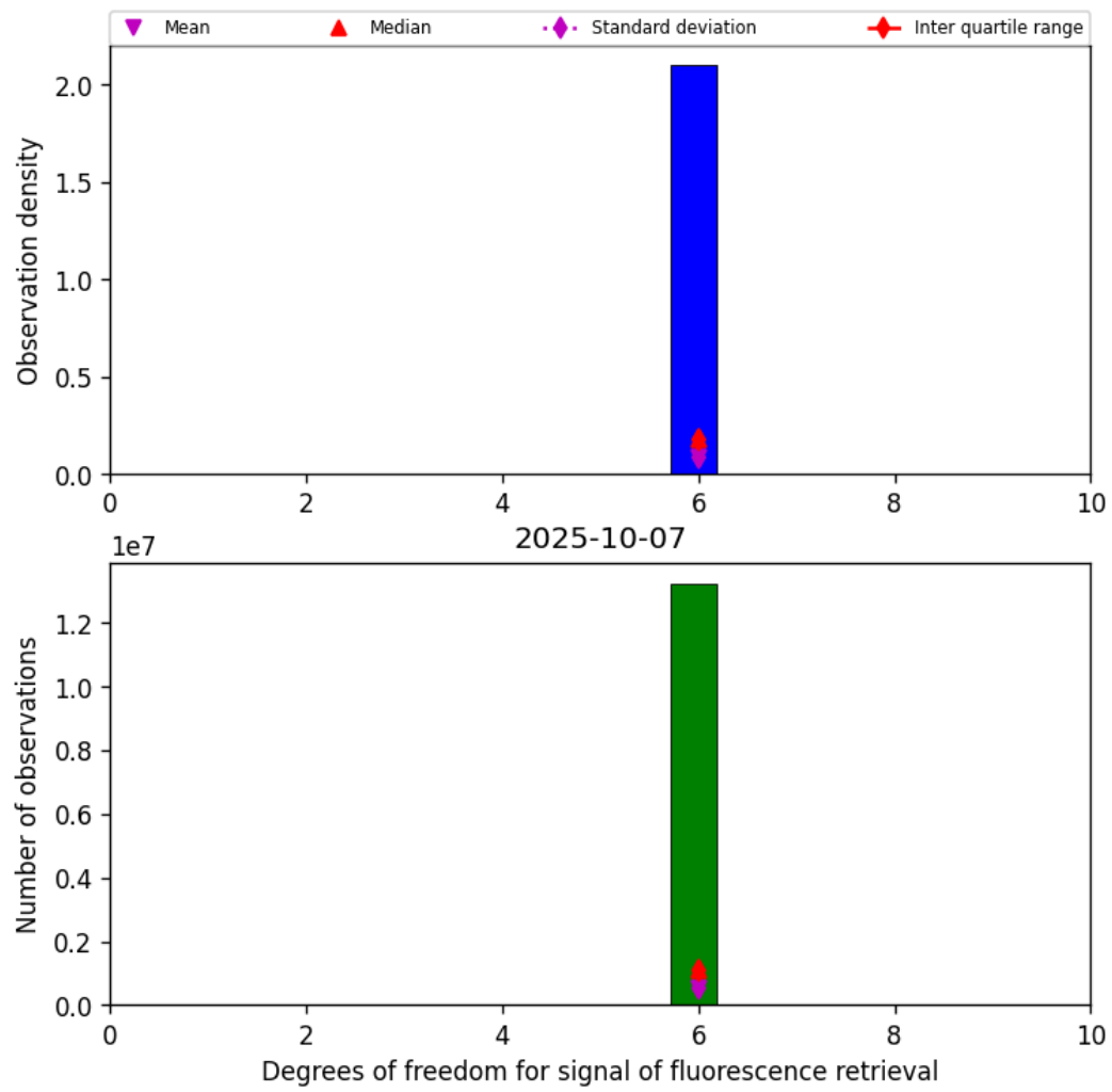
Figure 41: Histogram of “Degrees of freedom for signal of fluorescence retrieval” for 2025-10-07 to 2025-10-07
