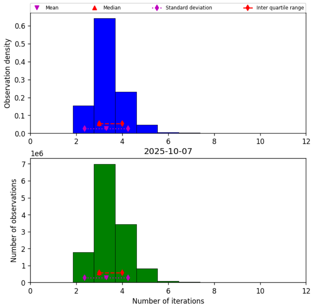
Figure 37: Histogram of “Number of iterations” for 2025-10-07 to 2025-10-07
