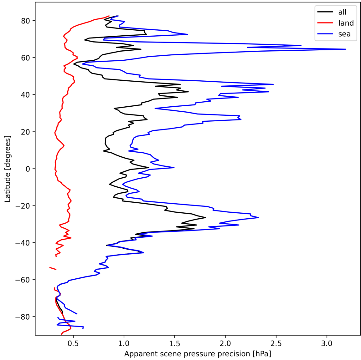
Figure 18: Zonal average of “Apparent scene pressure precision” for 2025-10-07 to 2025-10-07.
