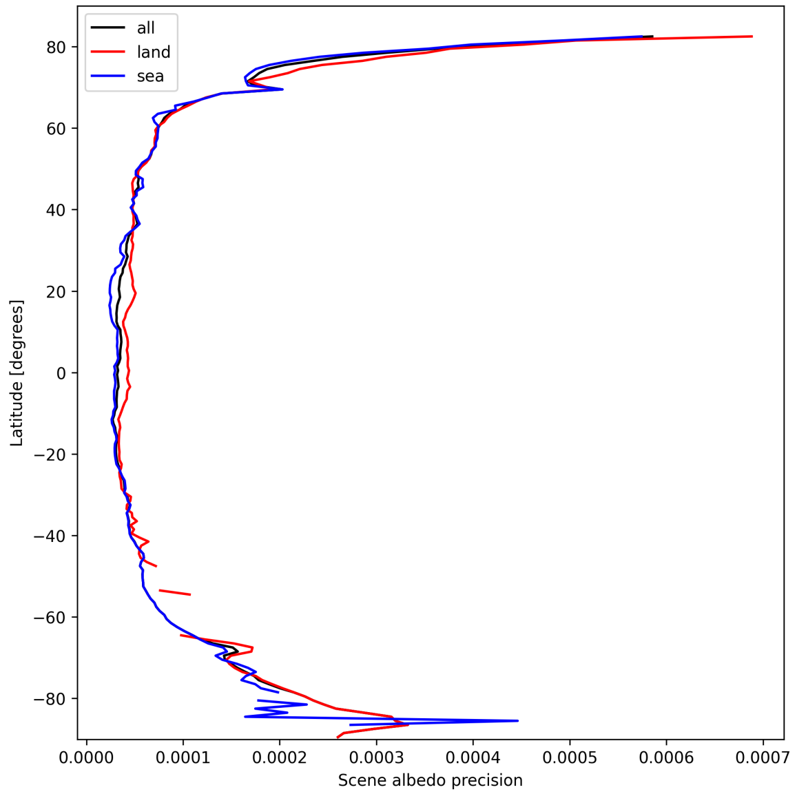
Figure 16: Zonal average of “Scene albedo precision” for 2025-10-07 to 2025-10-07.
