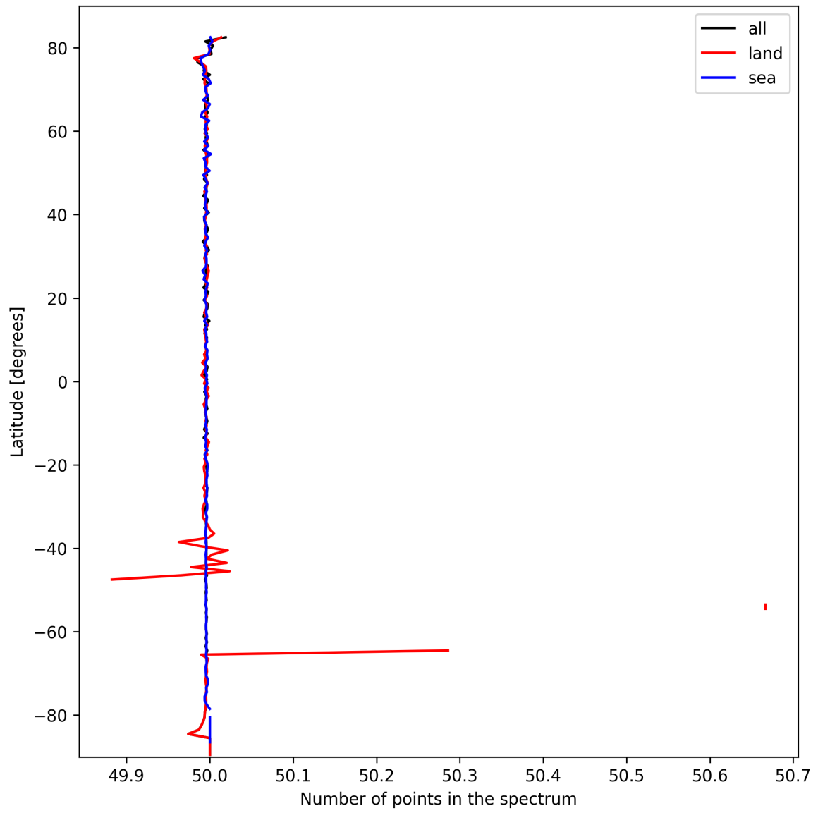
Figure 25: Zonal average of “Number of points in the spectrum” for 2025-10-07 to 2025-10-07.
