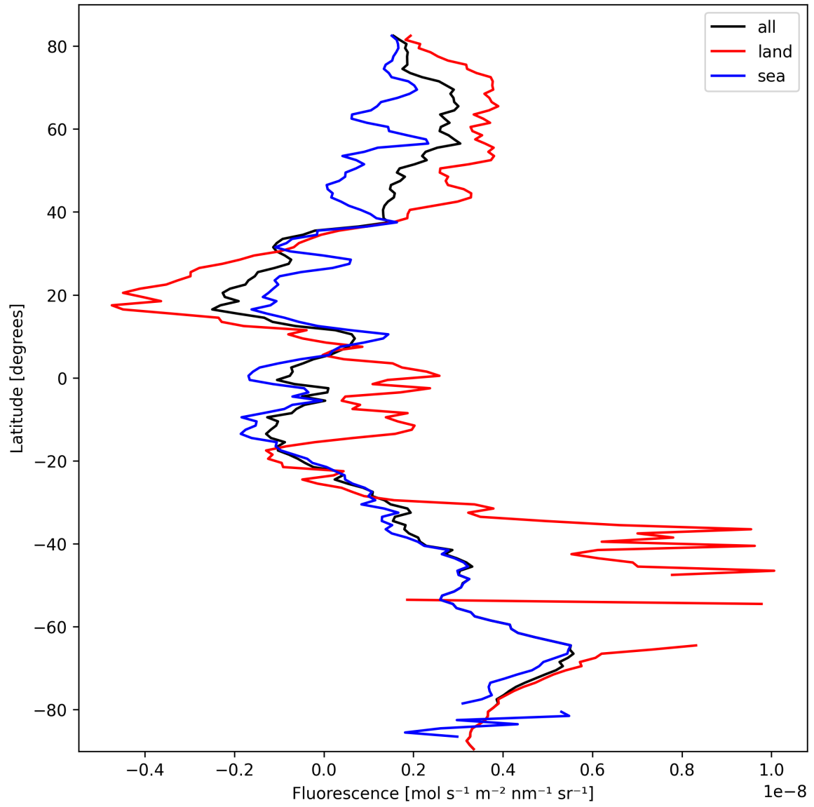
Figure 21: Zonal average of “Fluorescence” for 2025-10-07 to 2025-10-07.
