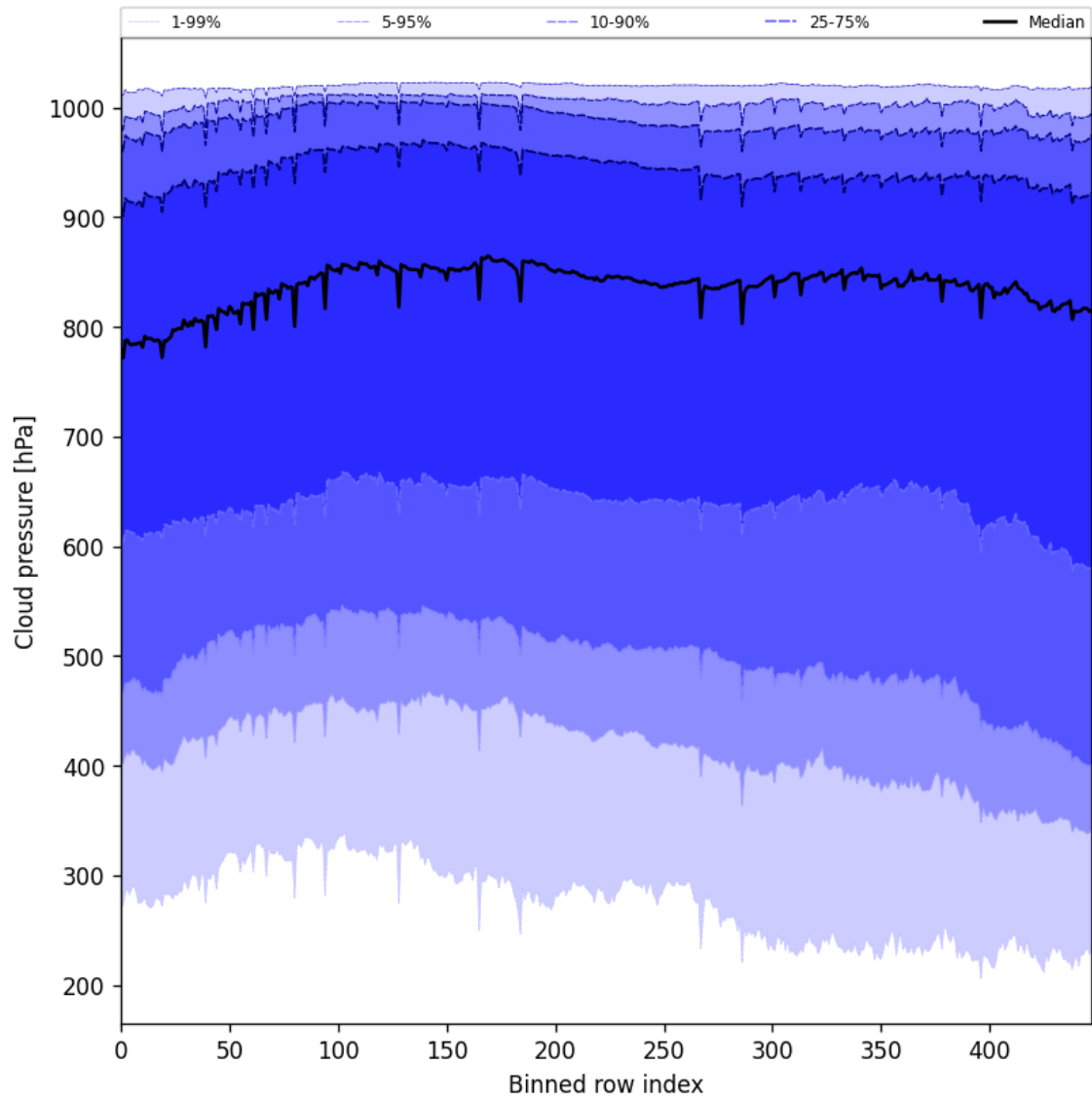
Figure 45: Along track statistics of “Cloud pressure” for 2025-10-07 to 2025-10-07
