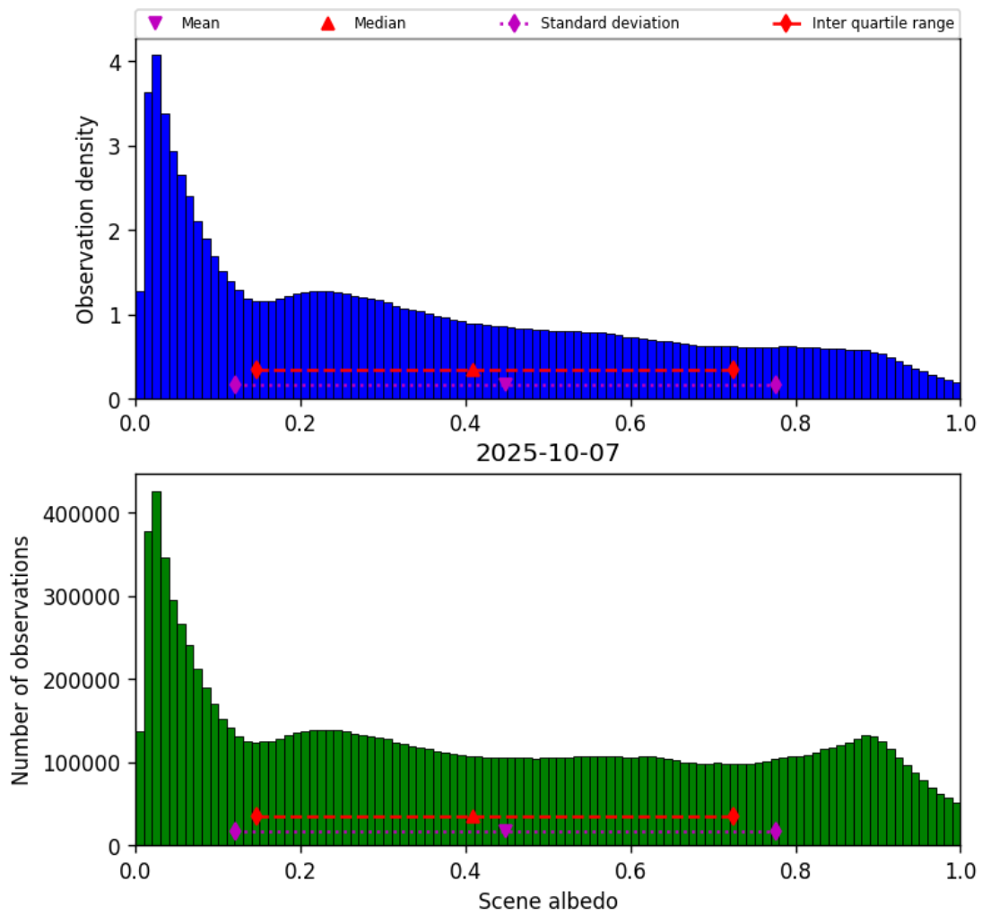
Figure 32: Histogram of “Scene albedo” for 2025-10-07 to 2025-10-07
