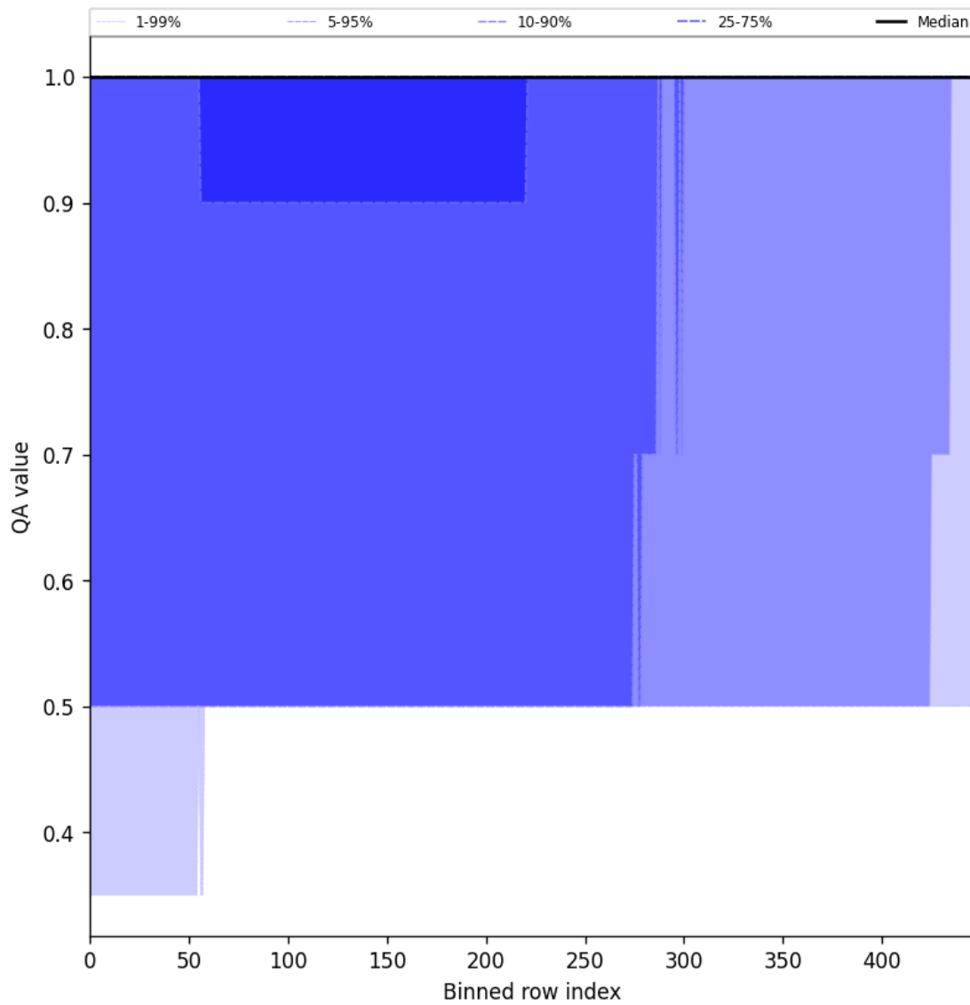
Figure 44: Along track statistics of “QA value” for 2025-10-07 to 2025-10-07
