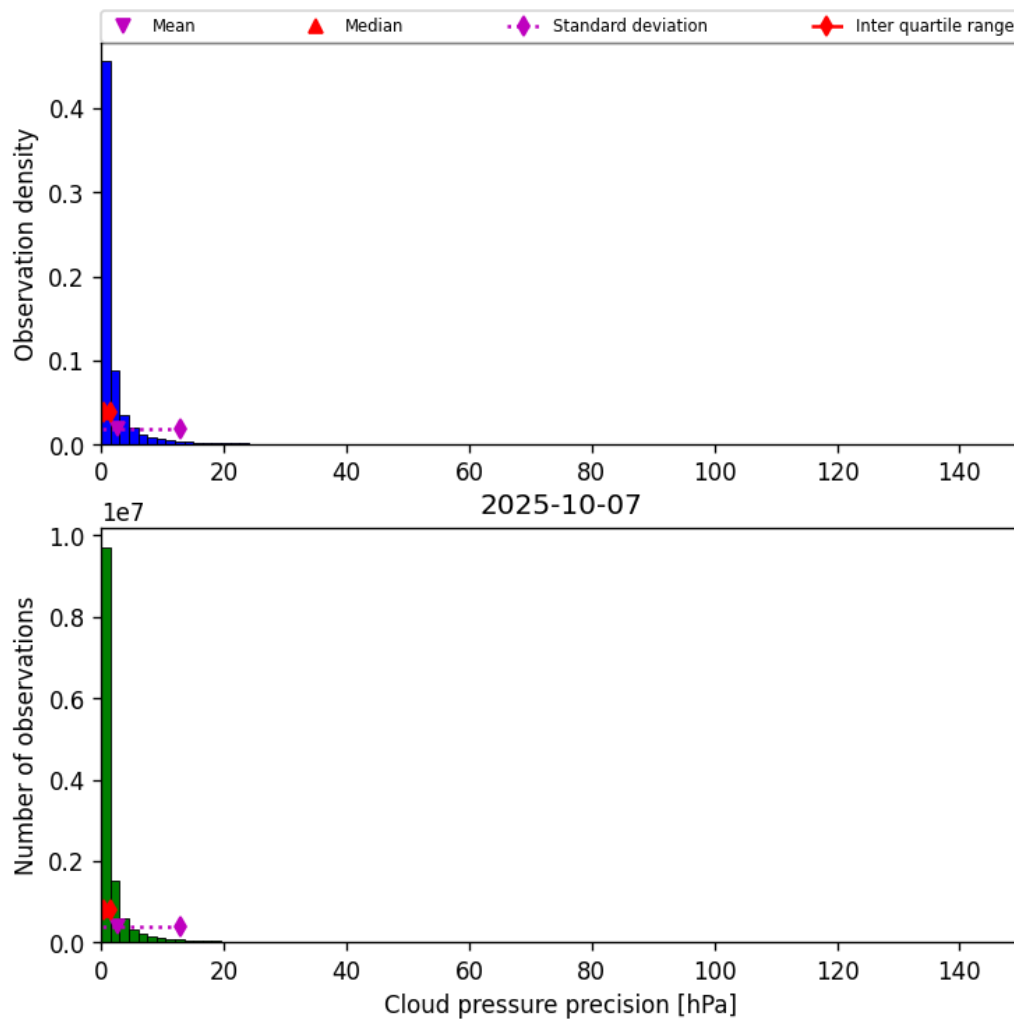
Figure 29: Histogram of “Cloud pressure precision” for 2025-10-07 to 2025-10-07
