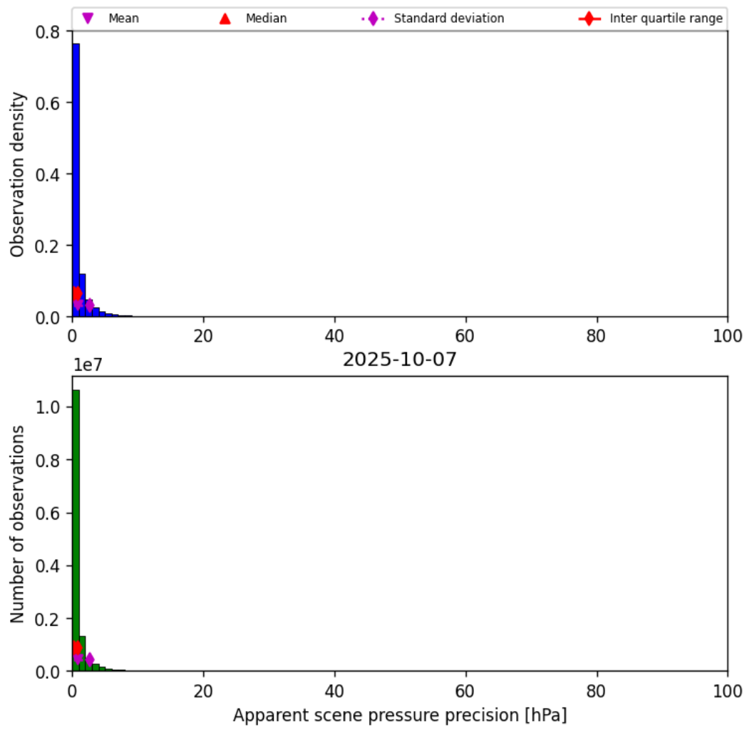
Figure 35: Histogram of “Apparent scene pressure precision” for 2025-10-07 to 2025-10-07
