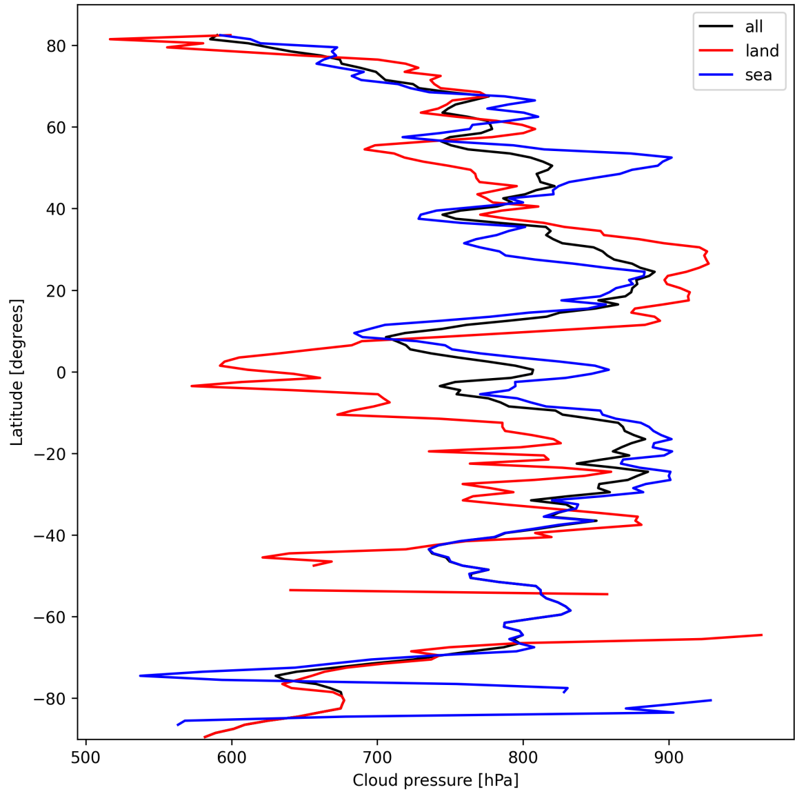
Figure 11: Zonal average of “Cloud pressure” for 2025-10-07 to 2025-10-07.
