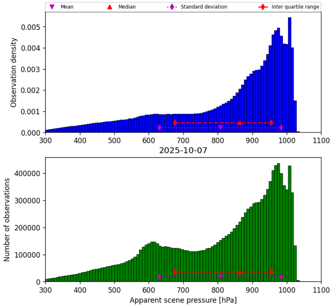
Figure 34: Histogram of “Apparent scene pressure” for 2025-10-07 to 2025-10-07
