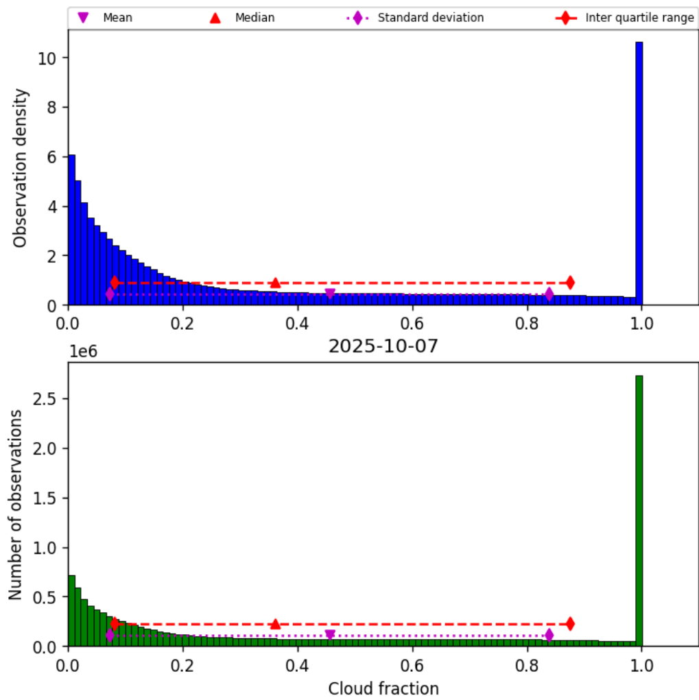
Figure 30: Histogram of “Cloud fraction” for 2025-10-07 to 2025-10-07
