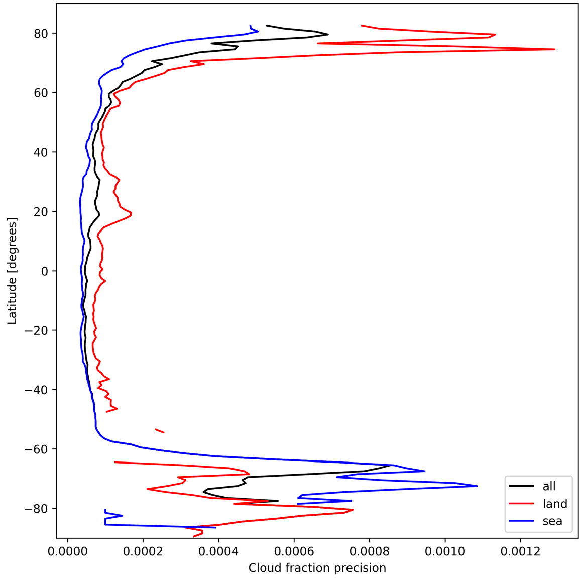
Figure 14: Zonal average of “Cloud fraction precision” for 2025-10-07 to 2025-10-07.
