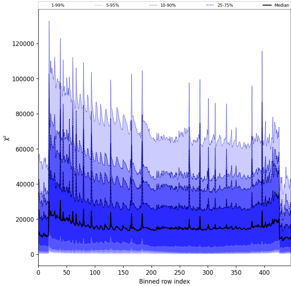
Figure 53: Along track statistics of “ \chi^2 ” for 2025-10-07 to 2025-10-07
