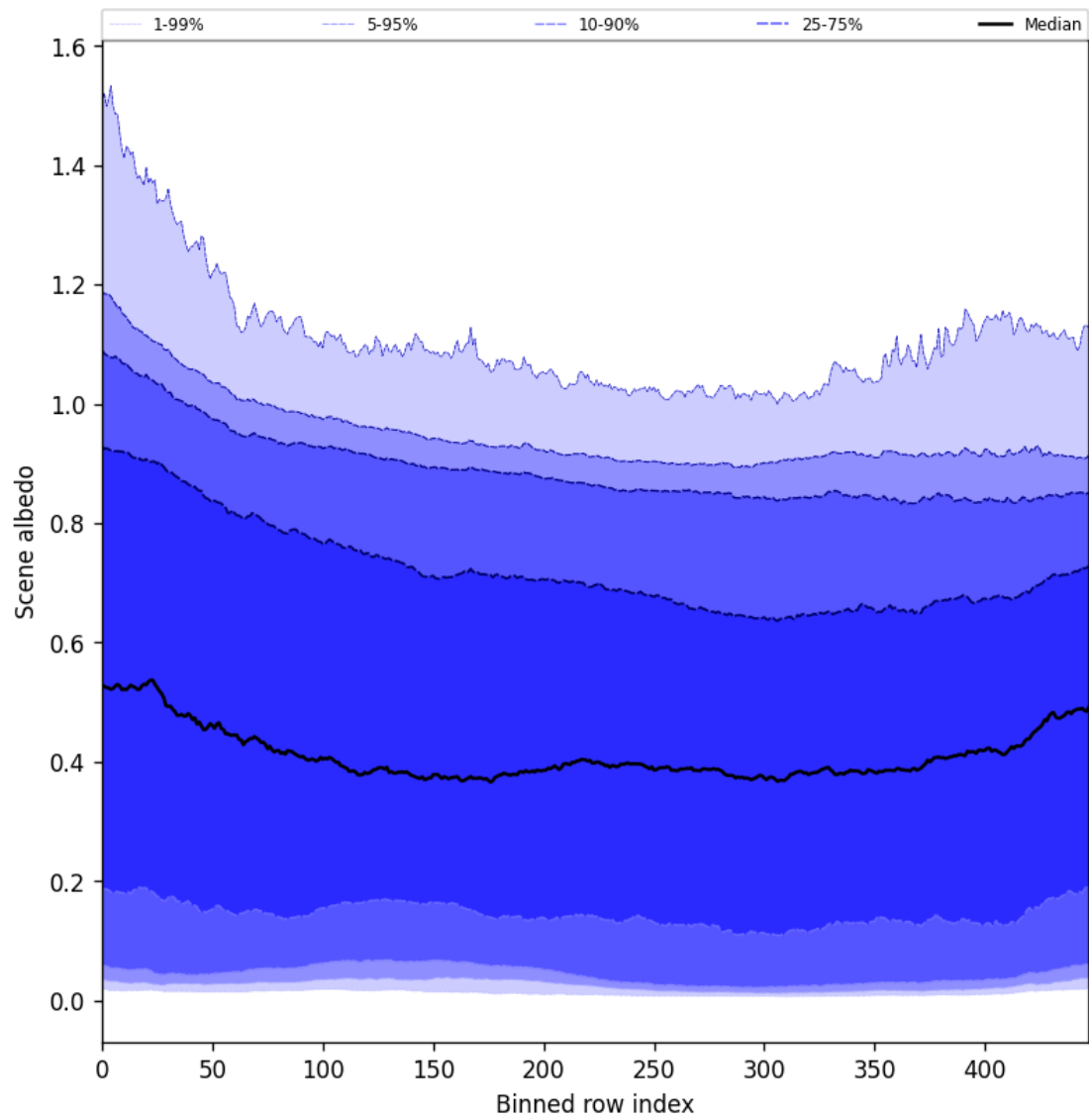
Figure 49: Along track statistics of “Scene albedo” for 2025-10-07 to 2025-10-07
