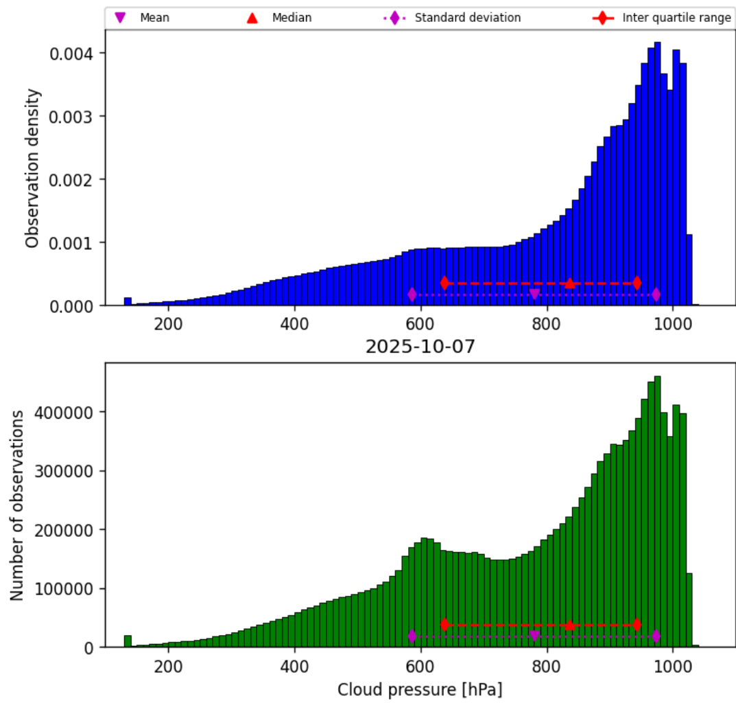
Figure 28: Histogram of “Cloud pressure” for 2025-10-07 to 2025-10-07
