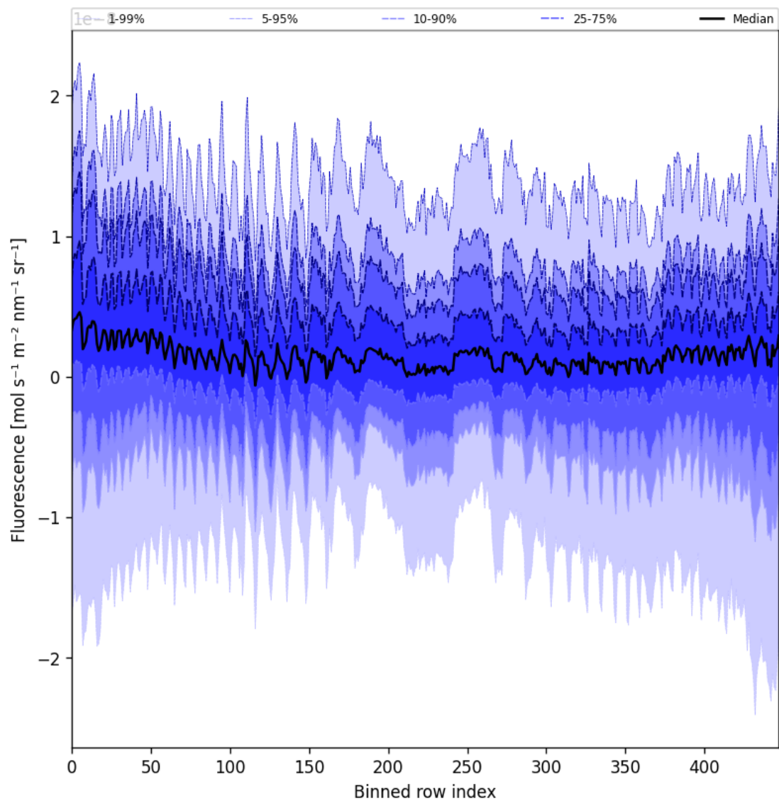
Figure 55: Along track statistics of “Fluorescence” for 2025-10-07 to 2025-10-07
