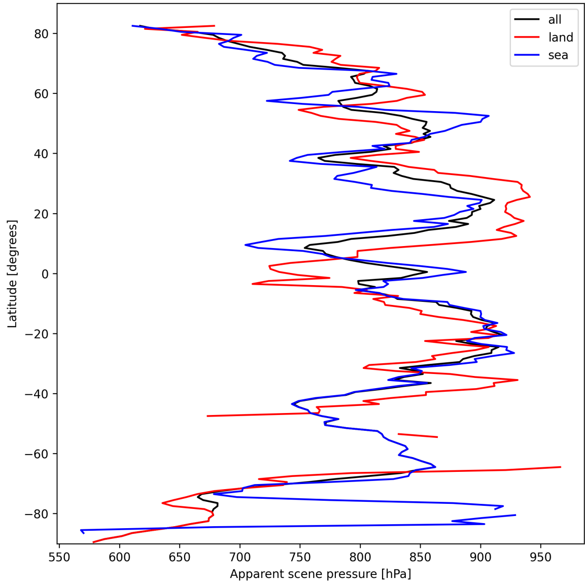
Figure 17: Zonal average of “Apparent scene pressure” for 2025-10-07 to 2025-10-07.
