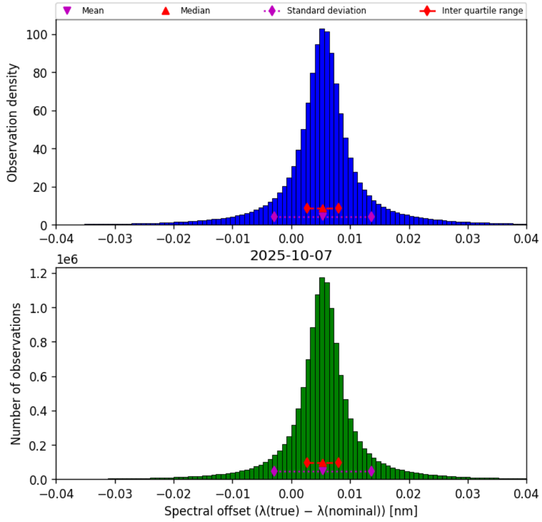
Figure 43: Histogram of “Spectral offset ( \lambda_{\text{true}} - \lambda_{\text{nominal}} )” for 2025-10-07 to 2025-10-07
