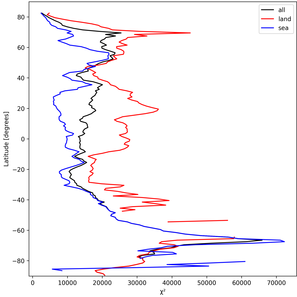
Figure 19: Zonal average of “ \chi^2 ” for 2025-10-07 to 2025-10-07.
