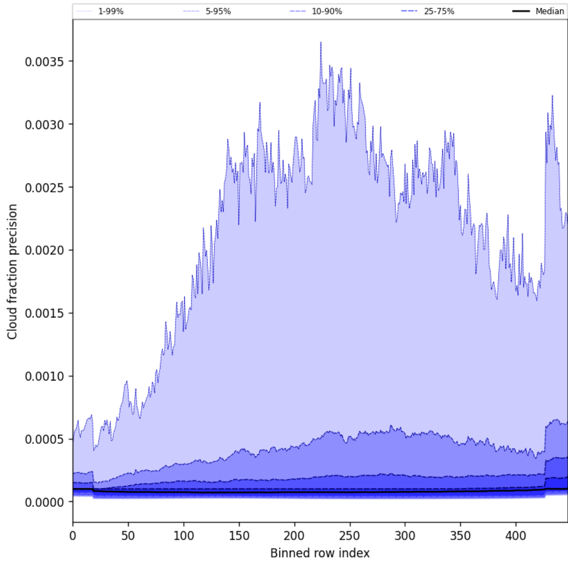
Figure 48: Along track statistics of “Cloud fraction precision” for 2025-10-07 to 2025-10-07
