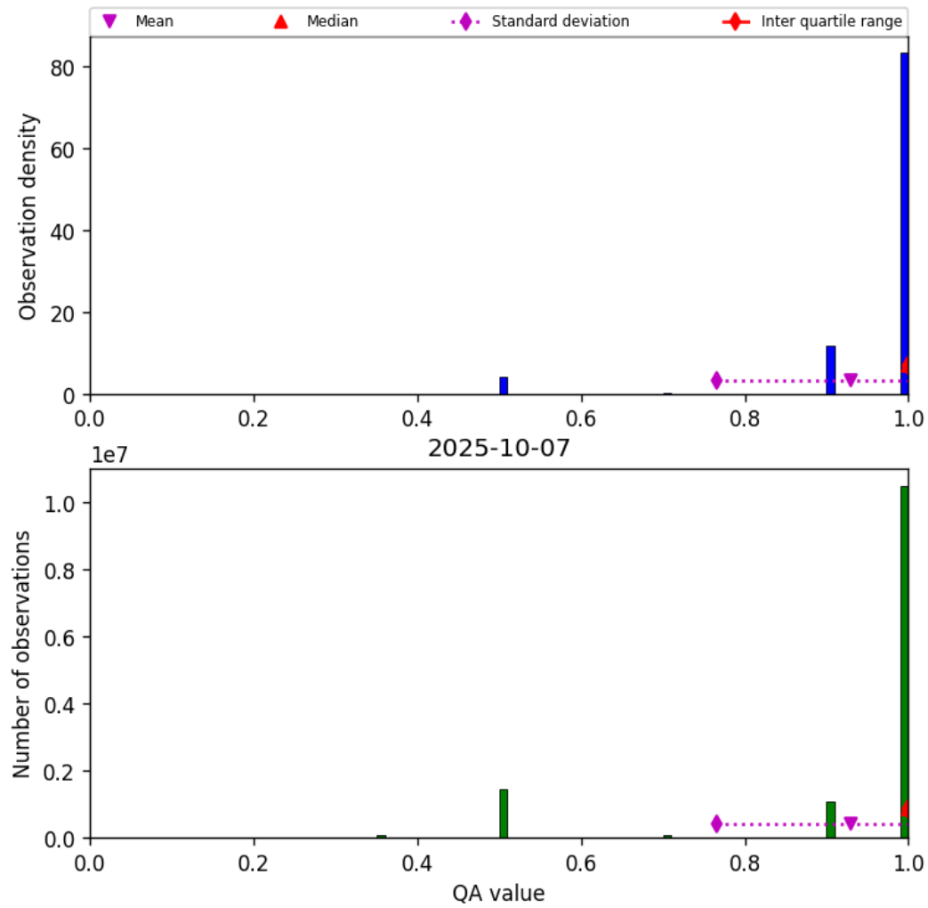
Figure 27: Histogram of “QA value” for 2025-10-07 to 2025-10-07
