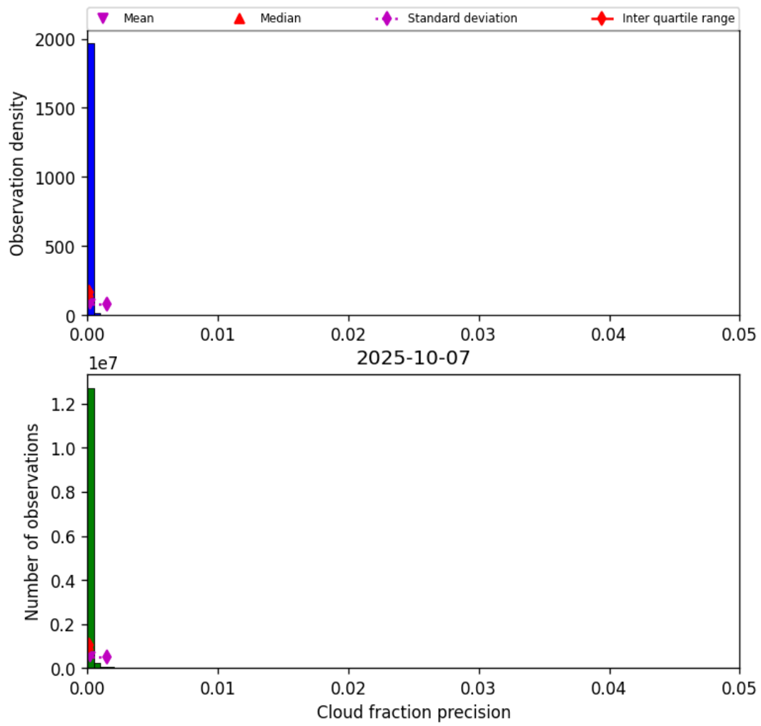
Figure 31: Histogram of “Cloud fraction precision” for 2025-10-07 to 2025-10-07
