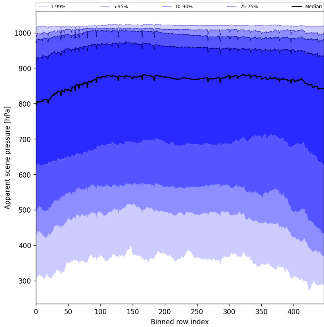
Figure 51: Along track statistics of “Apparent scene pressure” for 2025-10-07 to 2025-10-07
