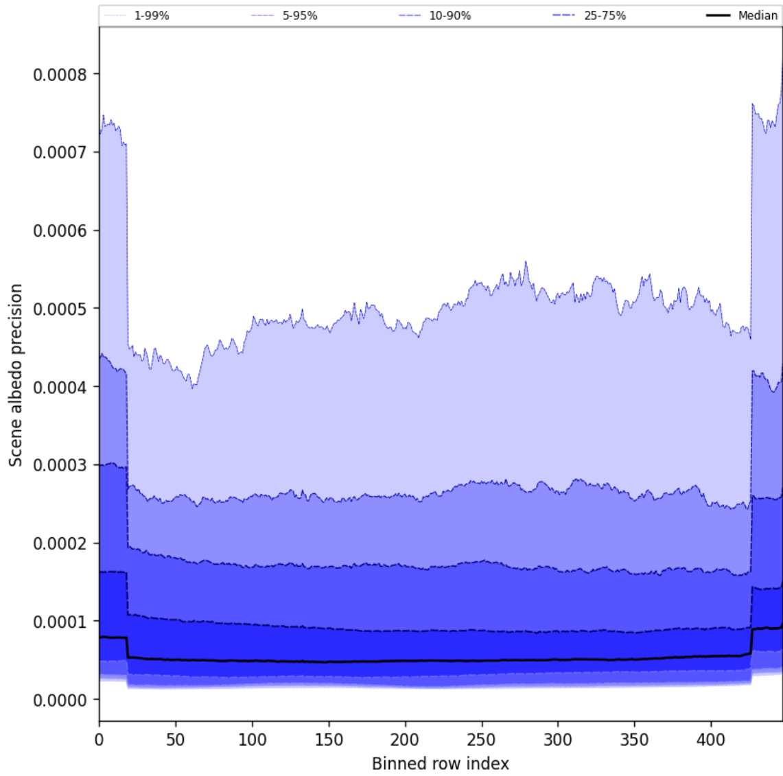
Figure 50: Along track statistics of “Scene albedo precision” for 2025-10-07 to 2025-10-07
