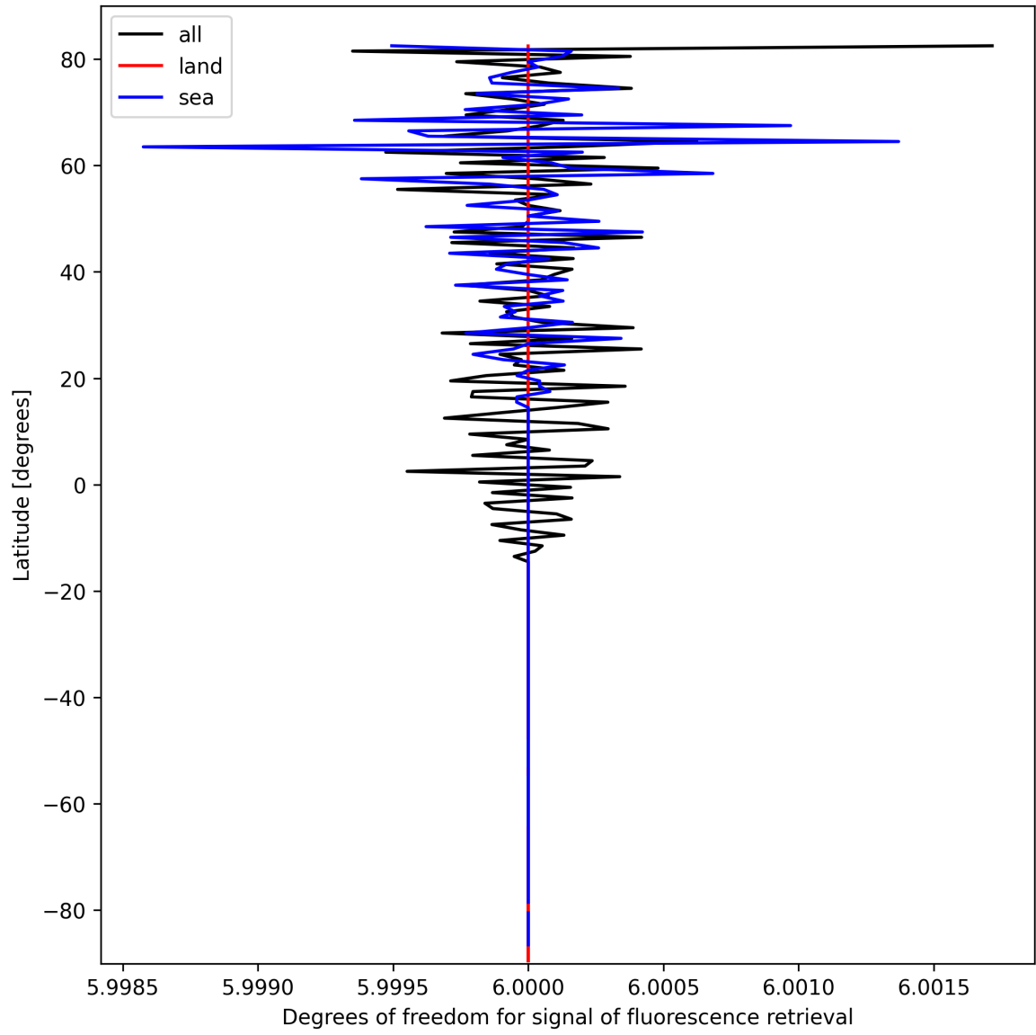
Figure 24: Zonal average of “Degrees of freedom for signal of fluorescence retrieval” for 2025-10-07 to 2025-10-07.
