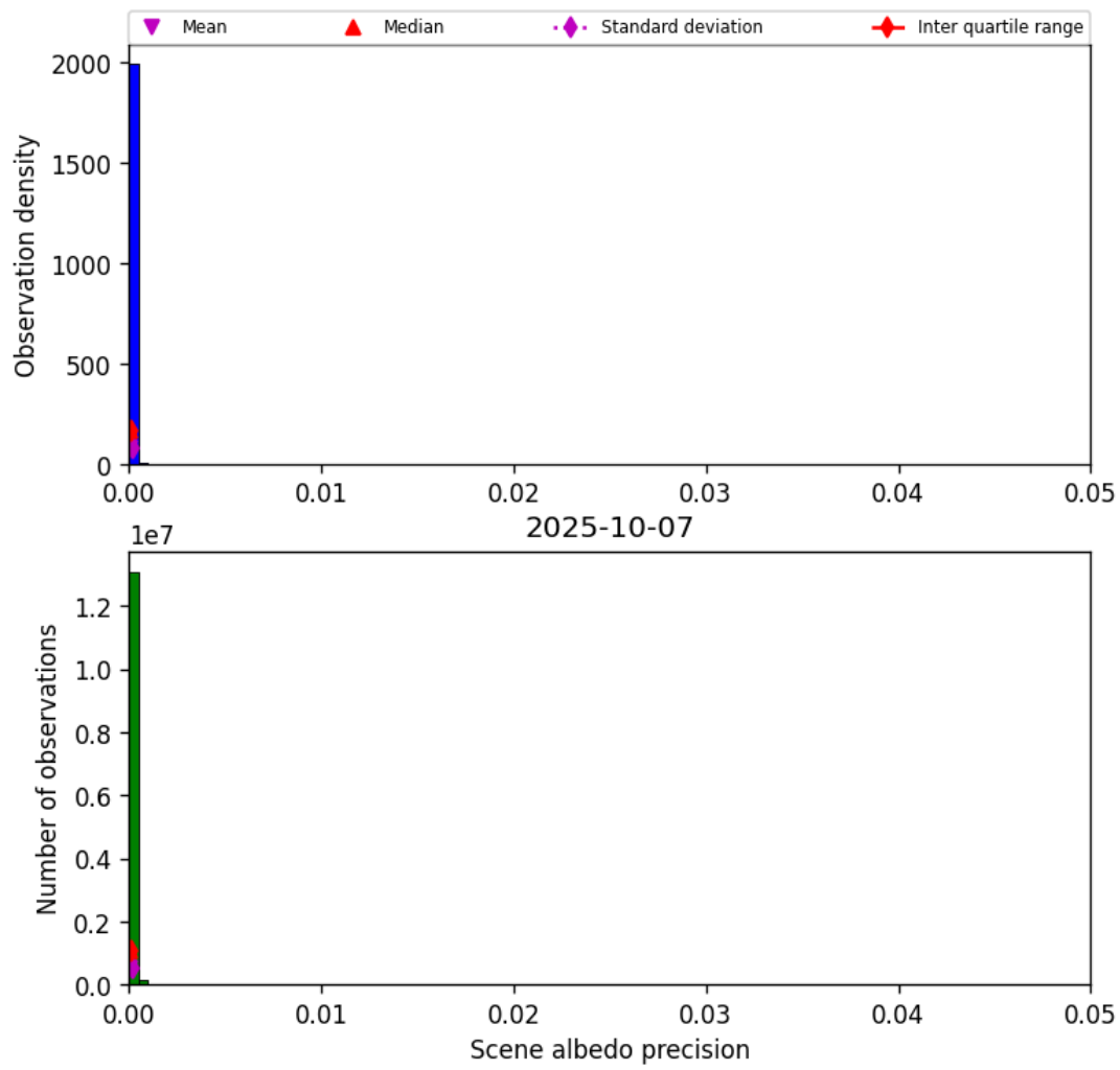
Figure 33: Histogram of “Scene albedo precision” for 2025-10-07 to 2025-10-07
