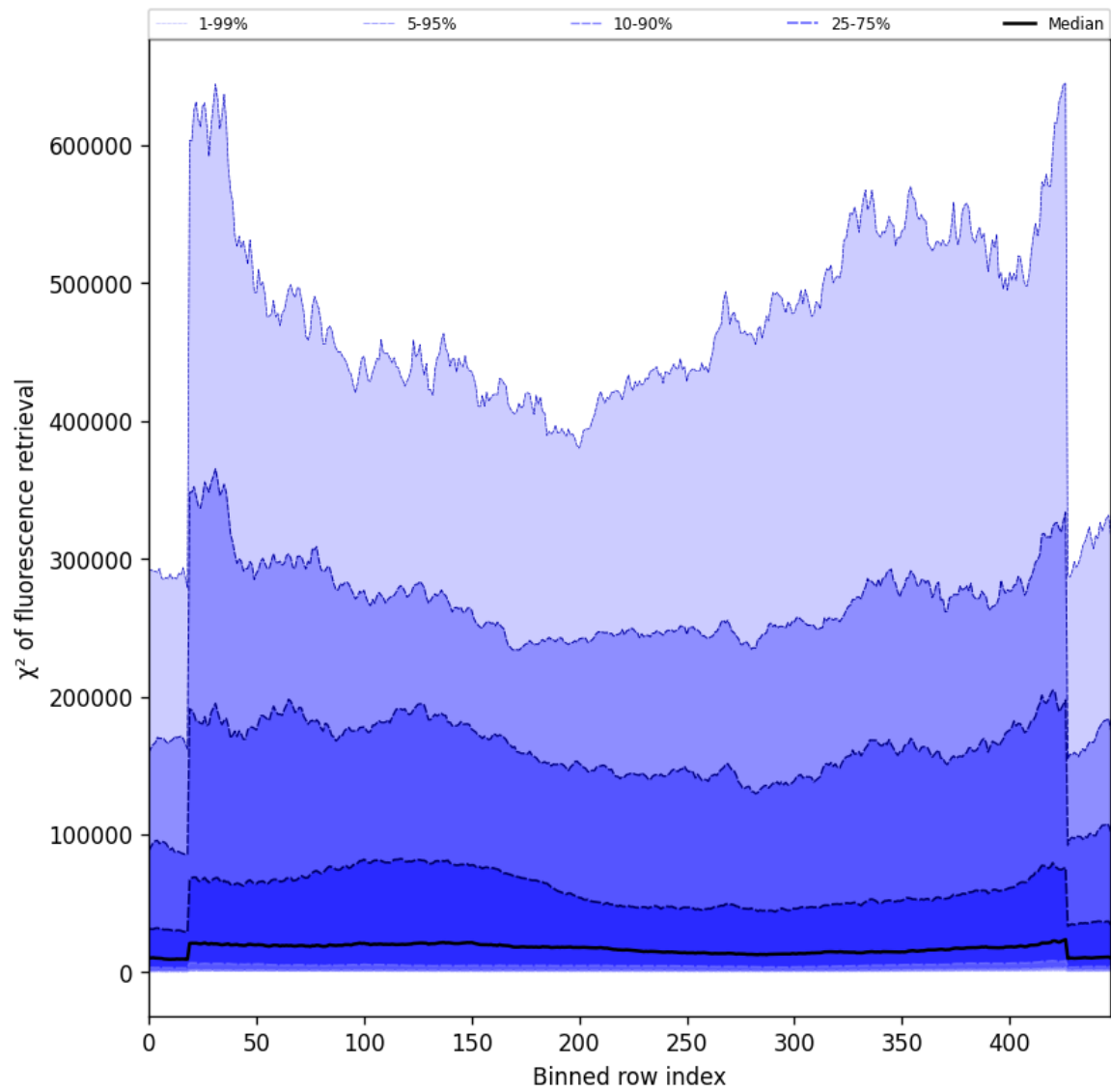
Figure 57: Along track statistics of “ \chi^2 of fluorescence retrieval” for 2025-10-07 to 2025-10-07
