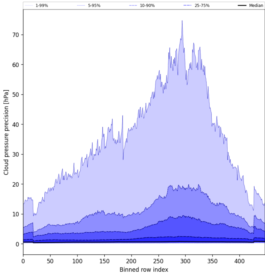
Figure 46: Along track statistics of “Cloud pressure precision” for 2025-10-07 to 2025-10-07
