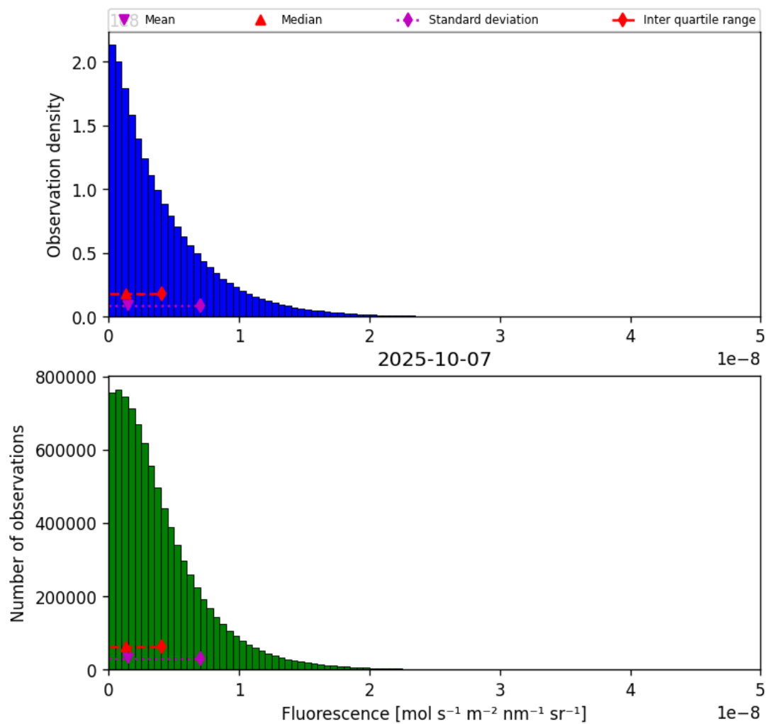
Figure 38: Histogram of “Fluorescence” for 2025-10-07 to 2025-10-07
