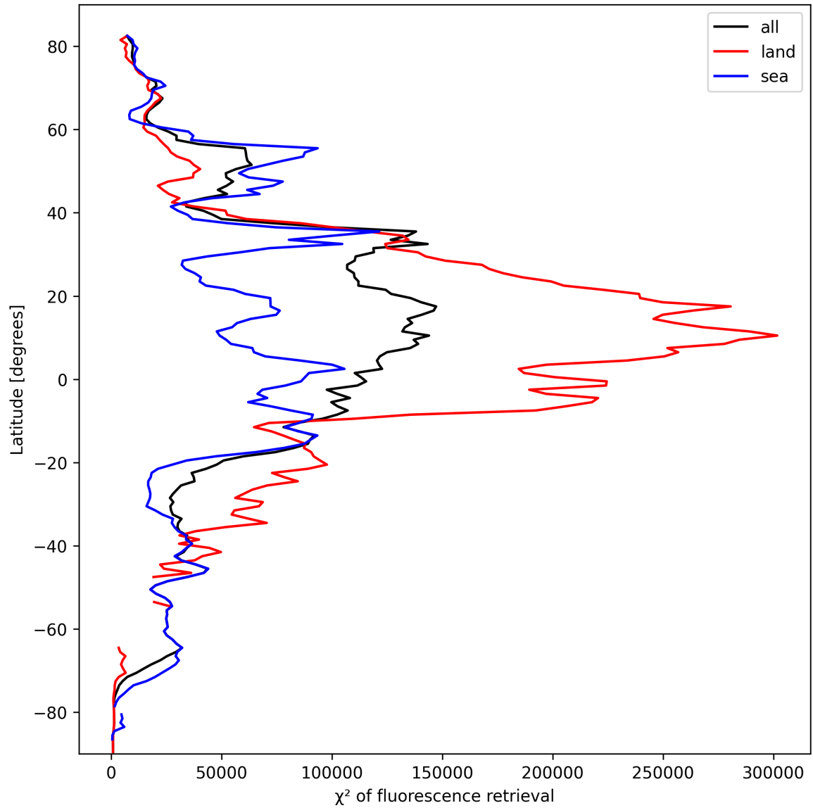
Figure 23: Zonal average of “ \chi^2 of fluorescence retrieval” for 2025-10-07 to 2025-10-07.
