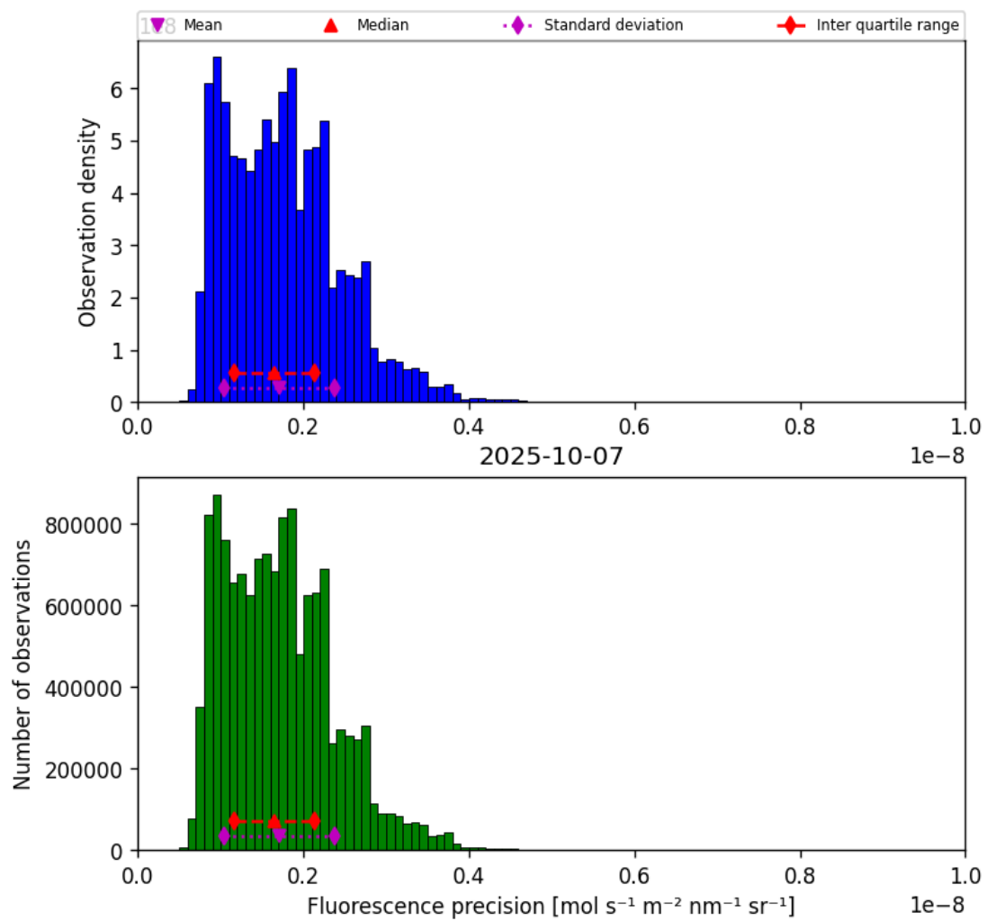
Figure 39: Histogram of “Fluorescence precision” for 2025-10-07 to 2025-10-07
