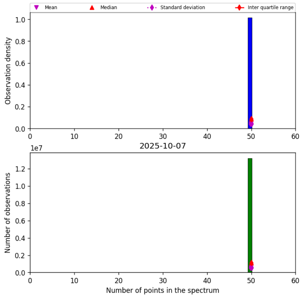
Figure 42: Histogram of “Number of points in the spectrum” for 2025-10-07 to 2025-10-07
