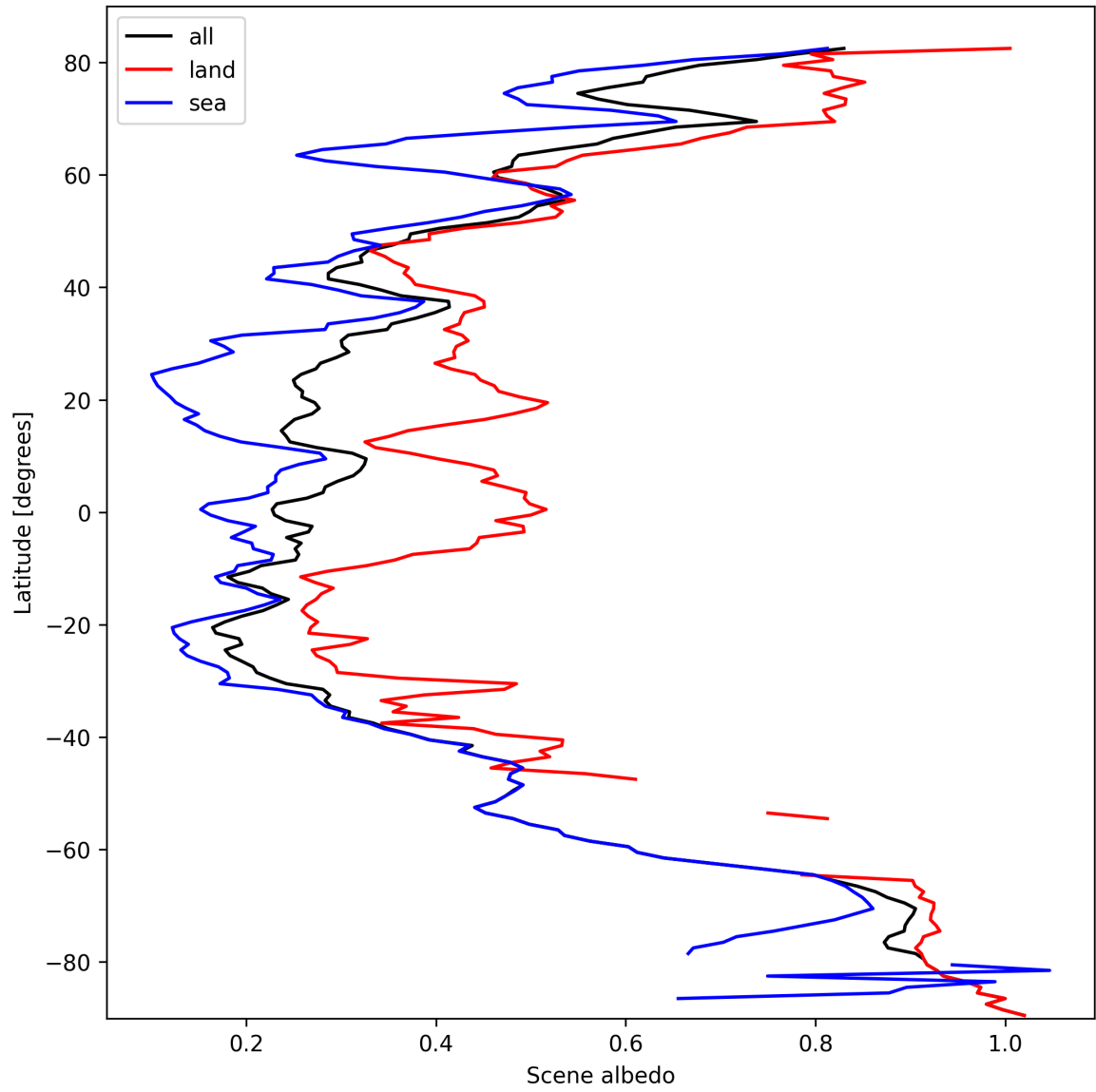
Figure 15: Zonal average of “Scene albedo” for 2025-10-07 to 2025-10-07.
