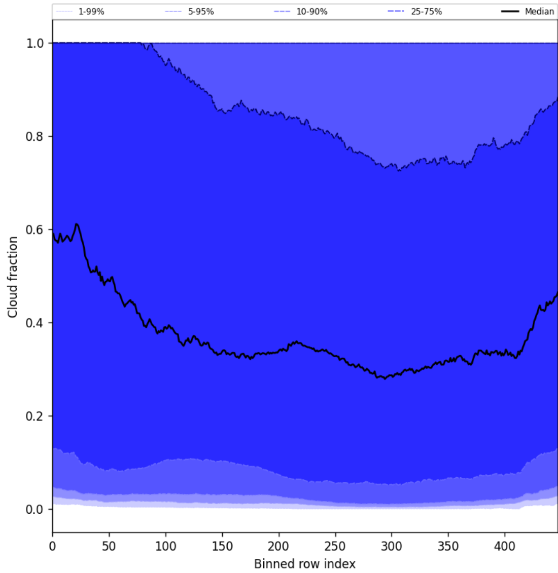
Figure 47: Along track statistics of “Cloud fraction” for 2025-10-07 to 2025-10-07
