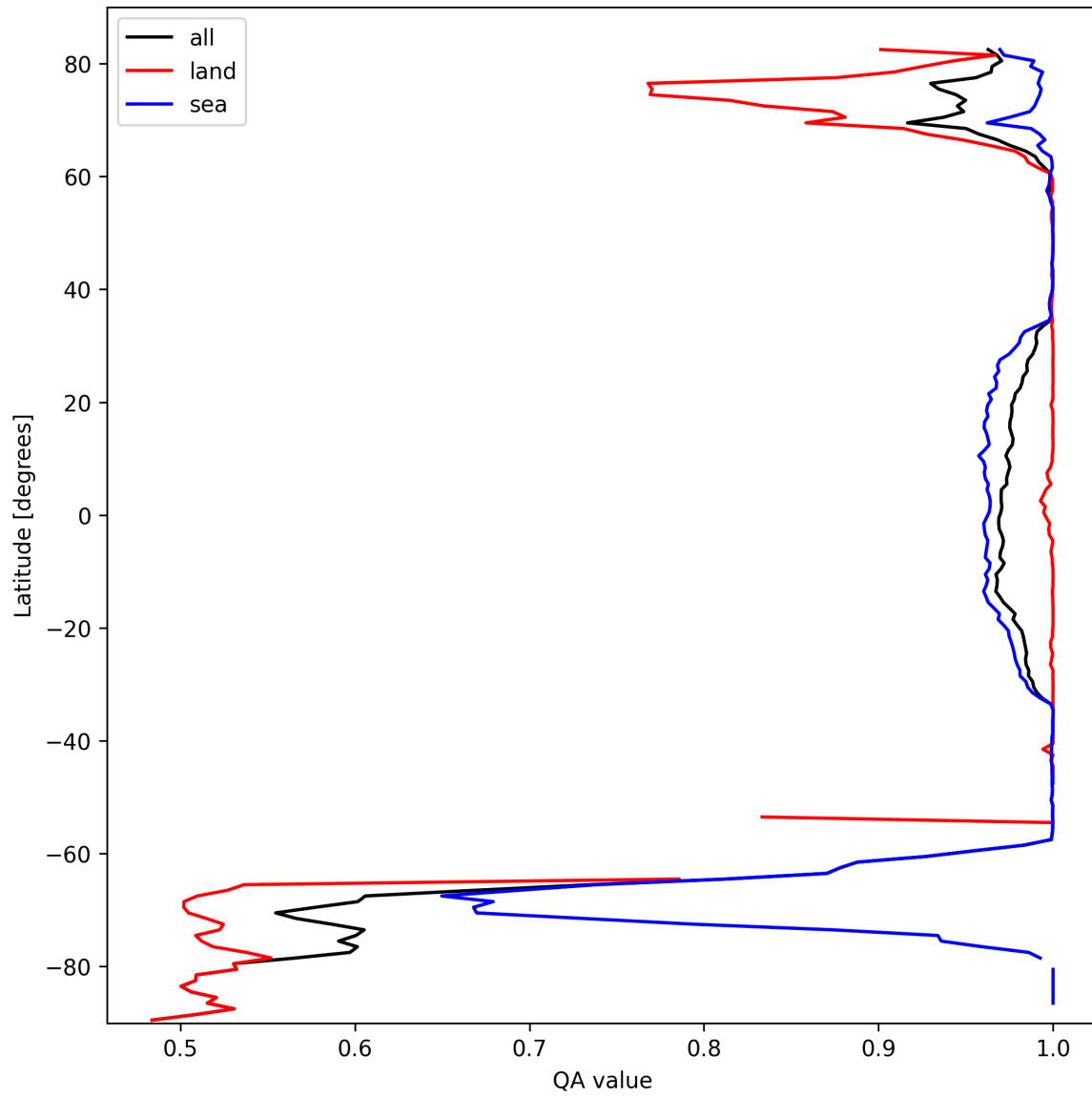
Figure 10: Zonal average of “QA value” for 2025-10-07 to 2025-10-07.
