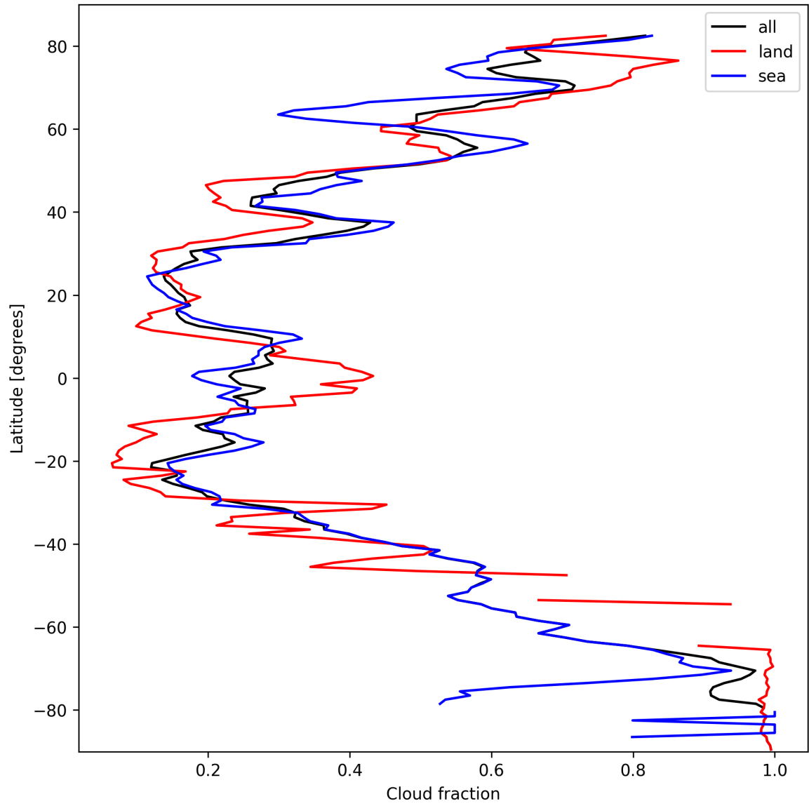
Figure 13: Zonal average of “Cloud fraction” for 2025-10-07 to 2025-10-07.
