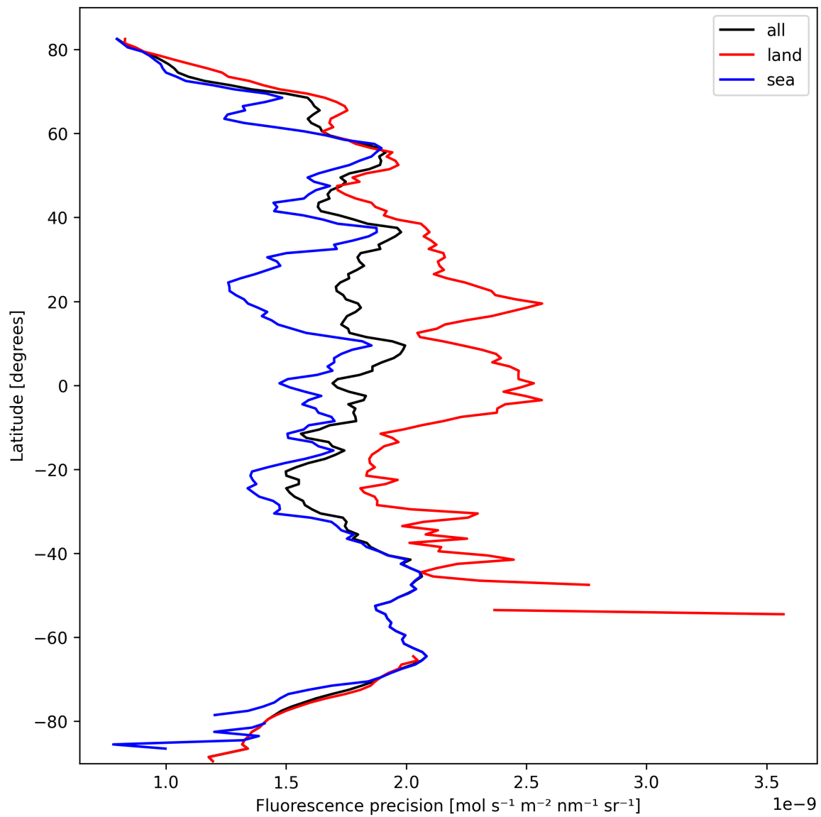
Figure 22: Zonal average of “Fluorescence precision” for 2025-10-07 to 2025-10-07.
