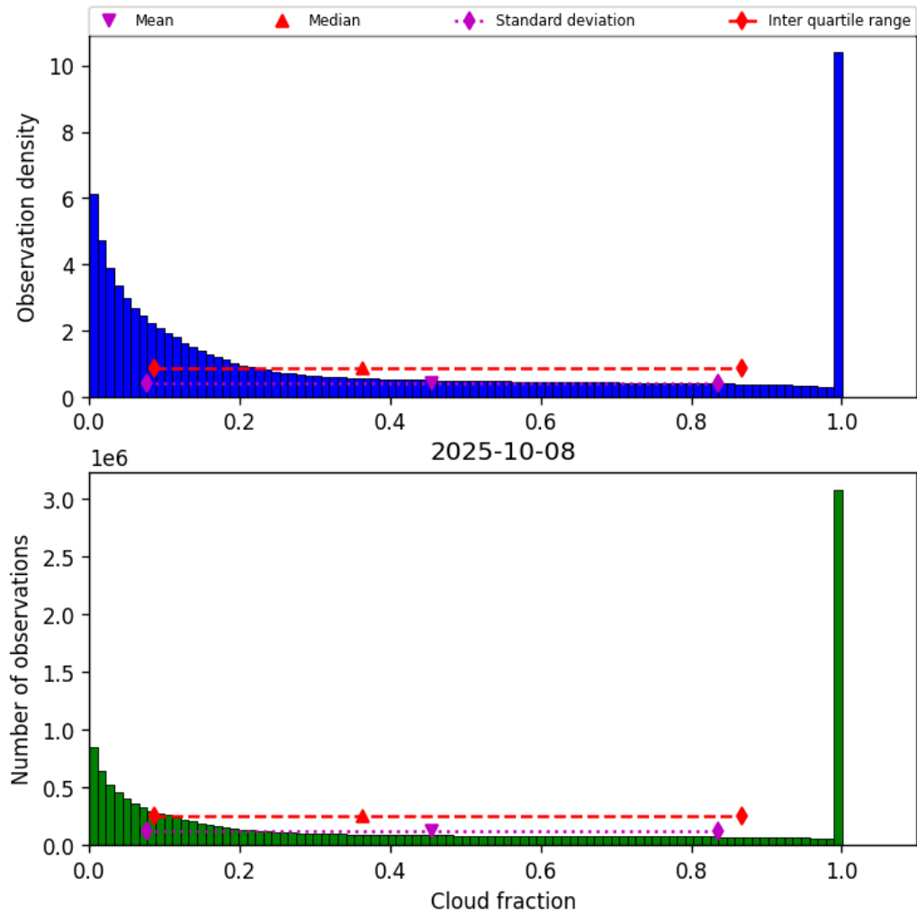
Figure 30: Histogram of “Cloud fraction” for 2025-10-08 to 2025-10-09
