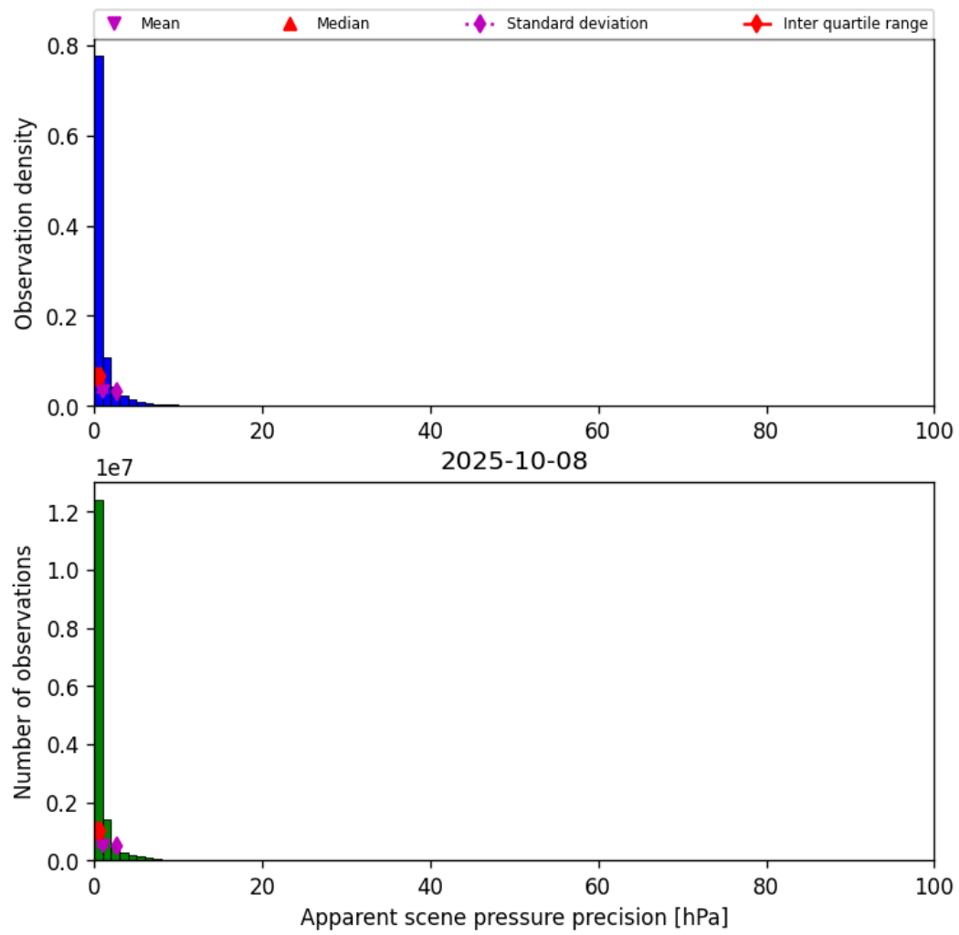
Figure 35: Histogram of “Apparent scene pressure precision” for 2025-10-08 to 2025-10-09
