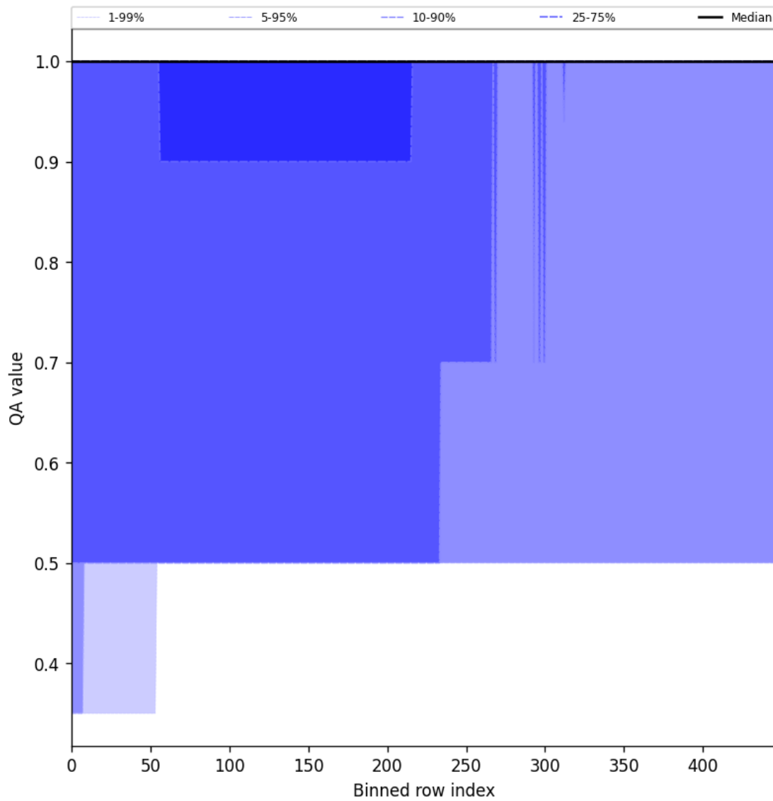
Figure 44: Along track statistics of “QA value” for 2025-10-08 to 2025-10-09
