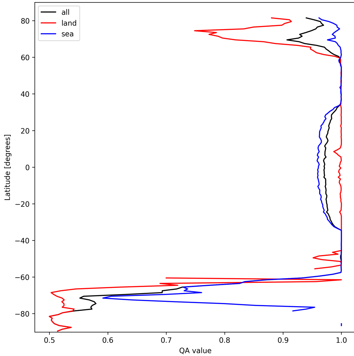
Figure 10: Zonal average of “QA value” for 2025-10-08 to 2025-10-09.
