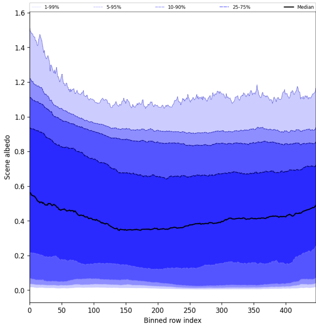
Figure 49: Along track statistics of “Scene albedo” for 2025-10-08 to 2025-10-09
