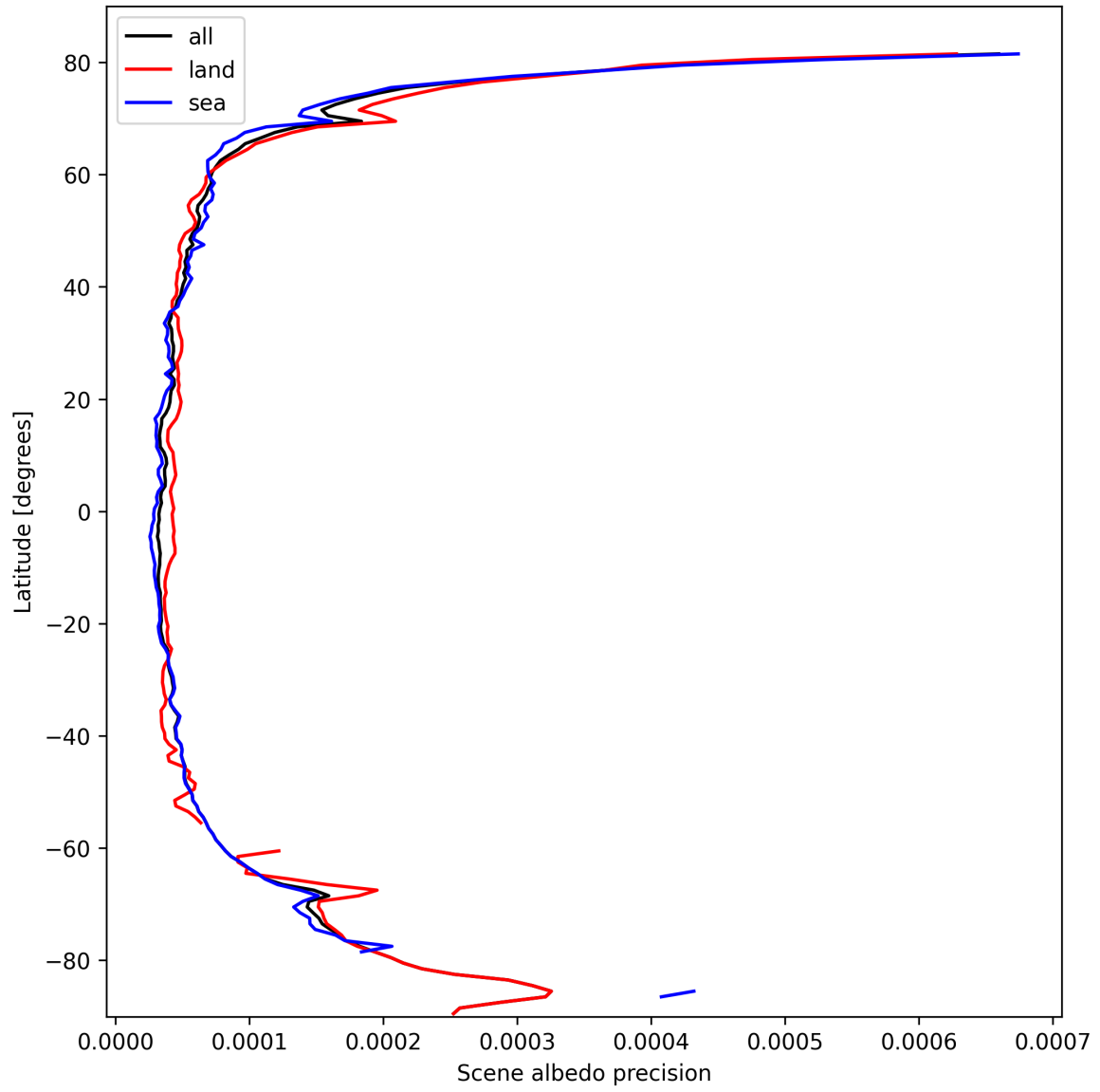
Figure 16: Zonal average of “Scene albedo precision” for 2025-10-08 to 2025-10-09.
