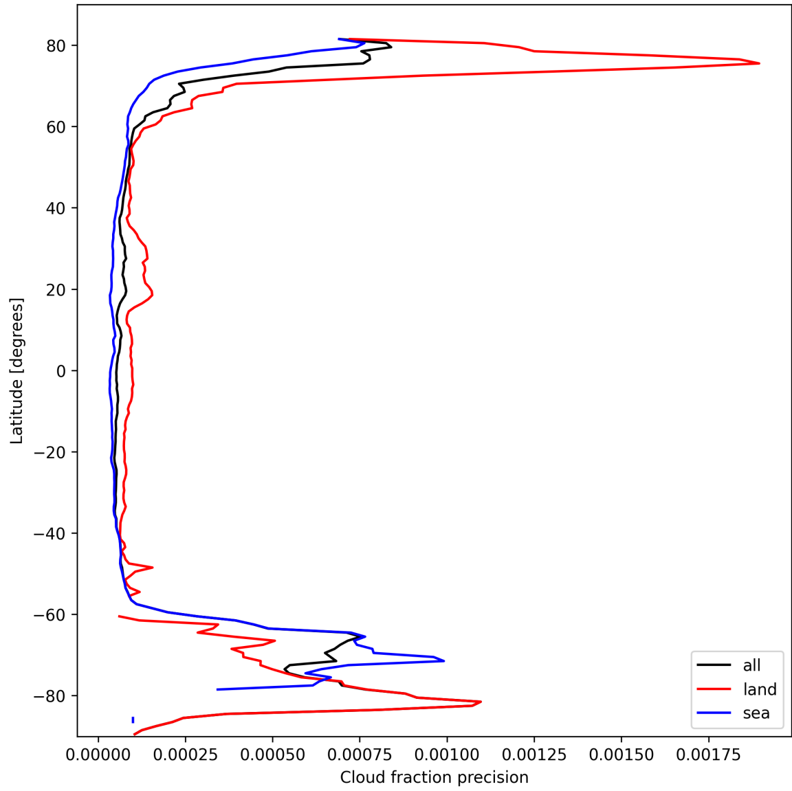
Figure 14: Zonal average of “Cloud fraction precision” for 2025-10-08 to 2025-10-09.
