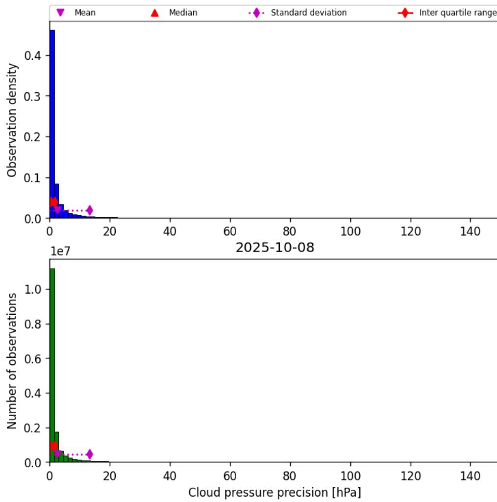
Figure 29: Histogram of “Cloud pressure precision” for 2025-10-08 to 2025-10-09
