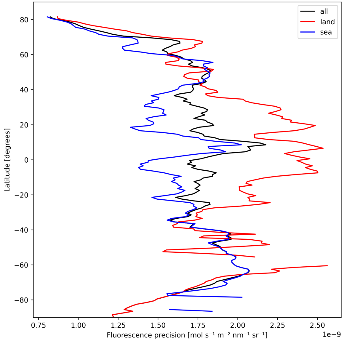
Figure 22: Zonal average of “Fluorescence precision” for 2025-10-08 to 2025-10-09.
