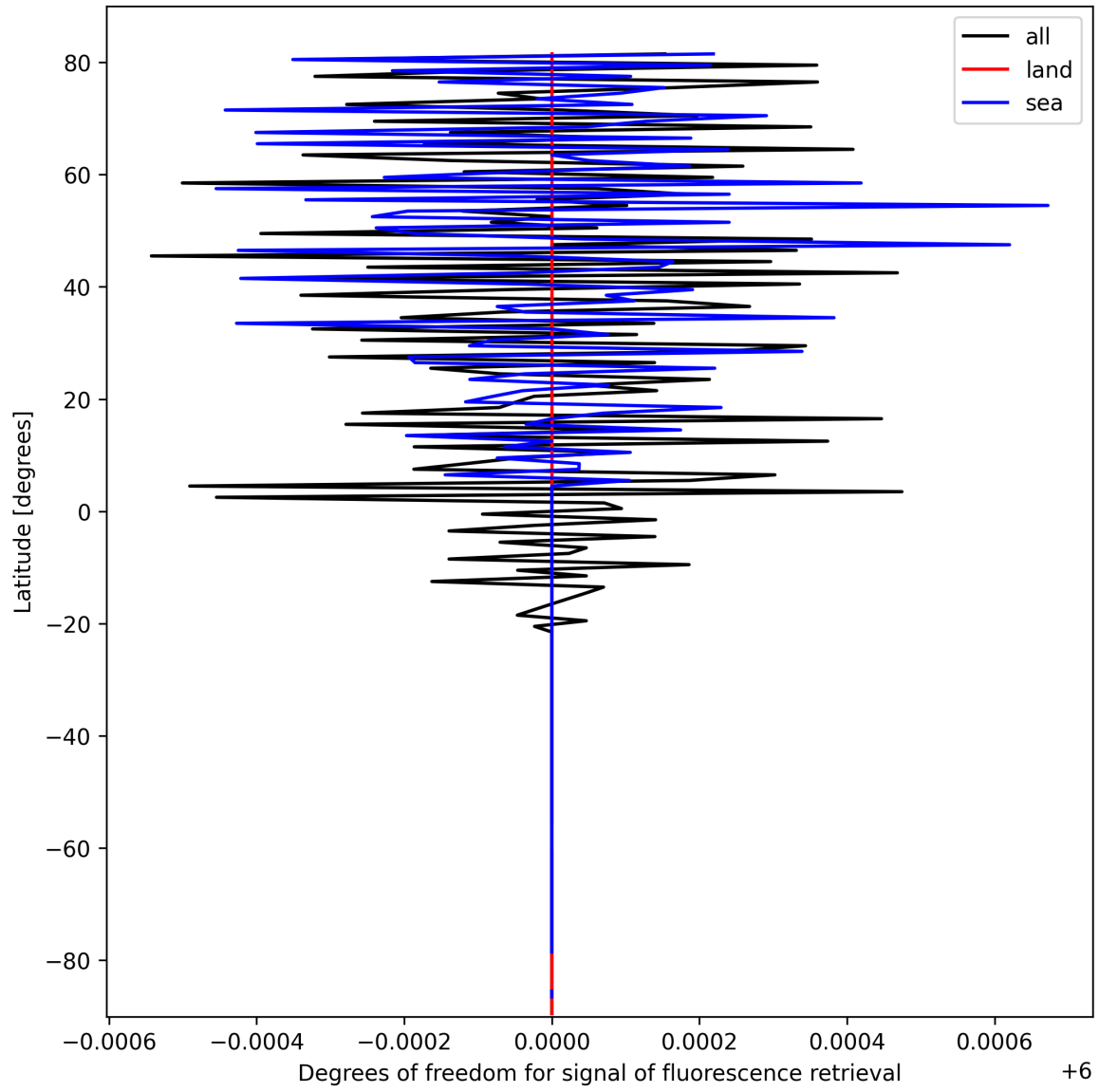
Figure 24: Zonal average of “Degrees of freedom for signal of fluorescence retrieval” for 2025-10-08 to 2025-10-09.
