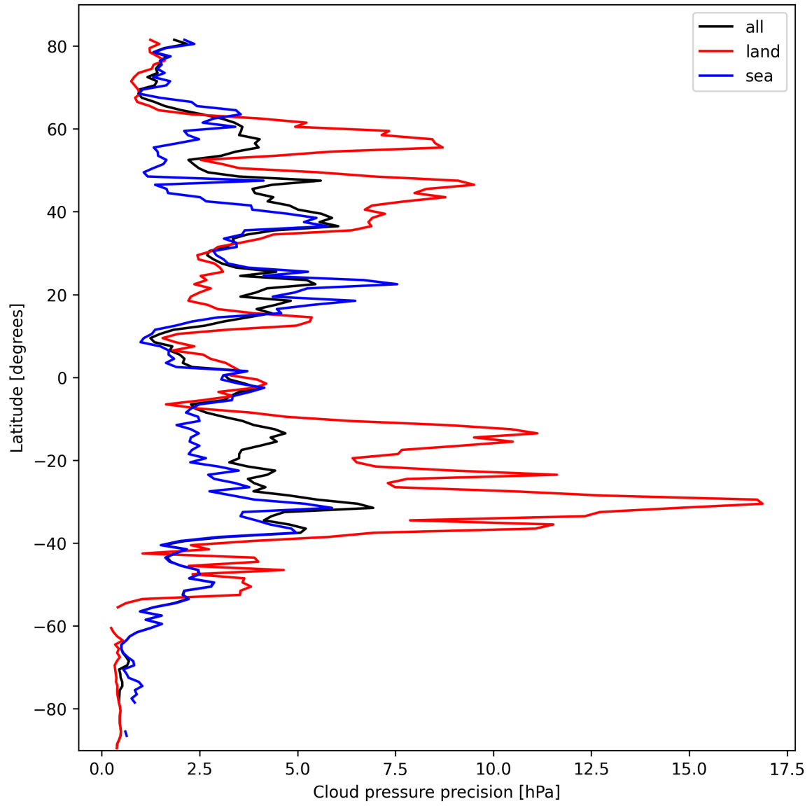
Figure 12: Zonal average of “Cloud pressure precision” for 2025-10-08 to 2025-10-09.
