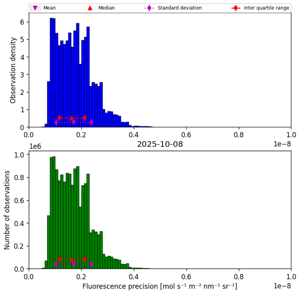
Figure 39: Histogram of “Fluorescence precision” for 2025-10-08 to 2025-10-09
