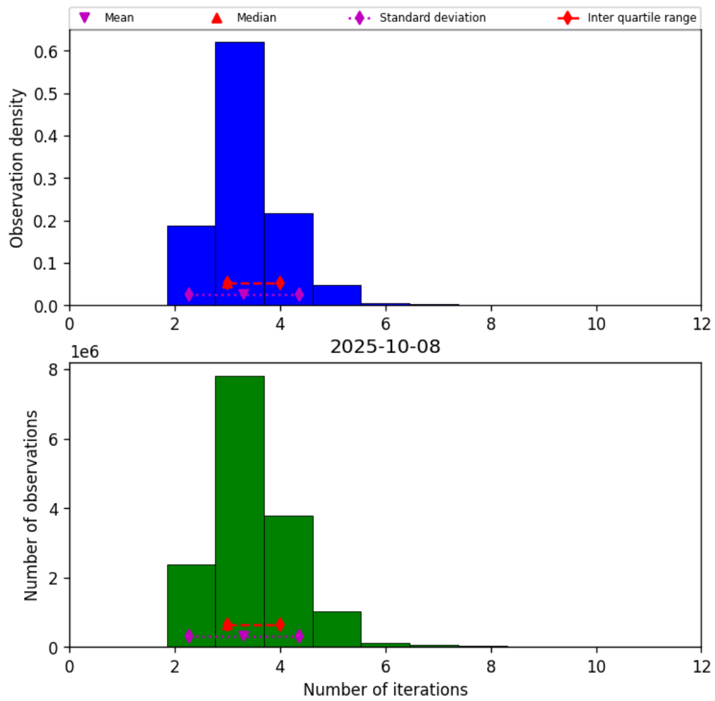
Figure 37: Histogram of “Number of iterations” for 2025-10-08 to 2025-10-09
