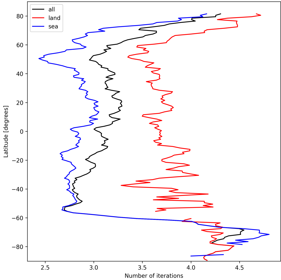
Figure 20: Zonal average of “Number of iterations” for 2025-10-08 to 2025-10-09.
