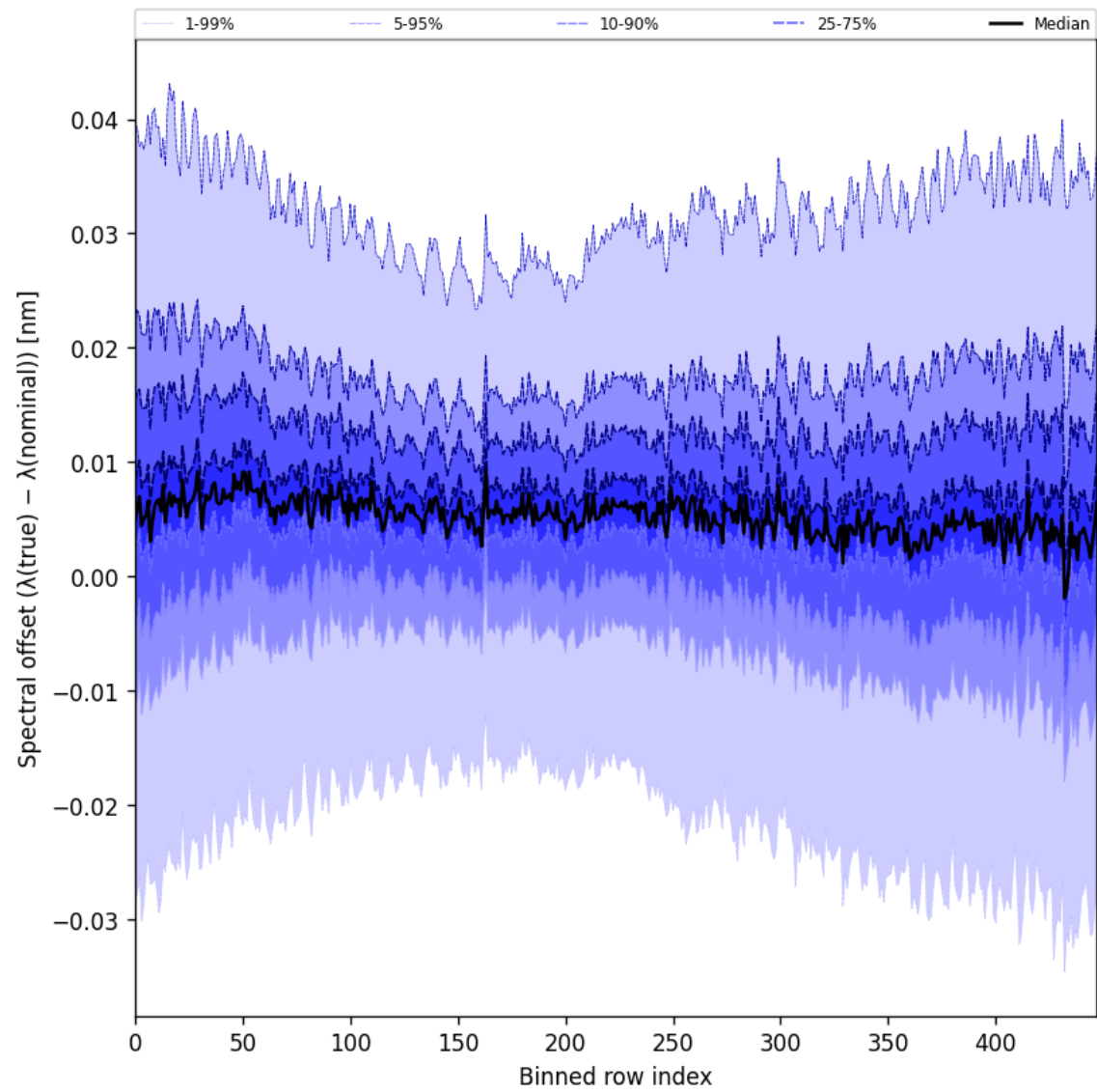
Figure 60: Along track statistics of “Spectral offset ( \lambda_{\text{true}} - \lambda_{\text{nominal}} )” for 2025-10-08 to 2025-10-09
