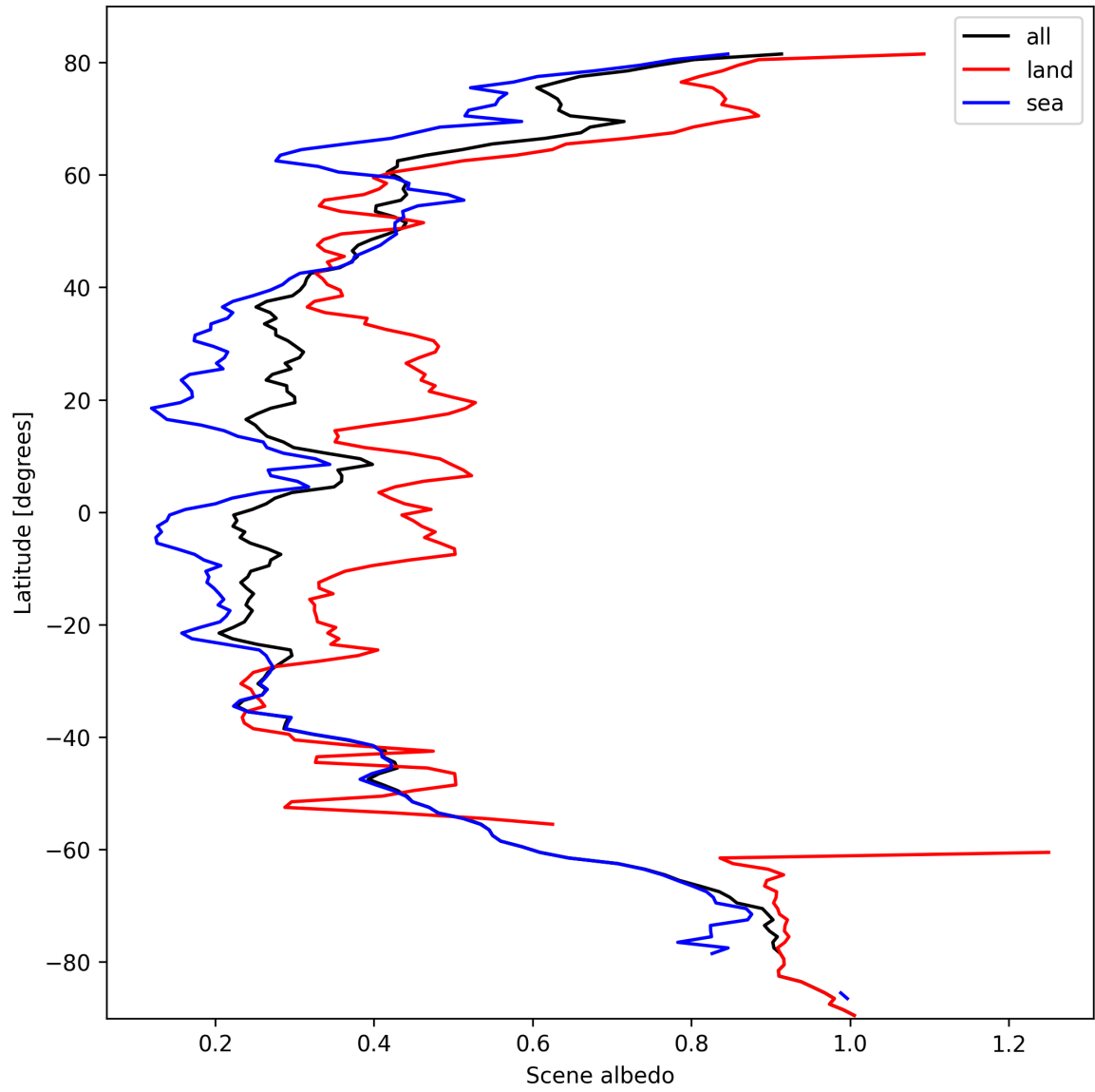
Figure 15: Zonal average of “Scene albedo” for 2025-10-08 to 2025-10-09.
