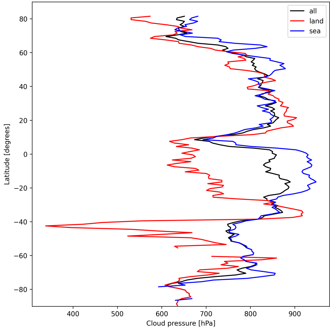
Figure 11: Zonal average of “Cloud pressure” for 2025-10-08 to 2025-10-09.
