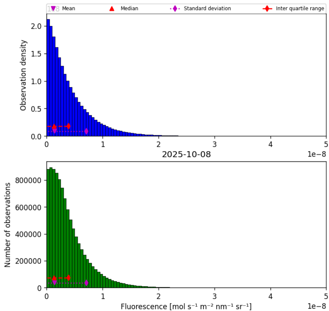
Figure 38: Histogram of “Fluorescence” for 2025-10-08 to 2025-10-09
