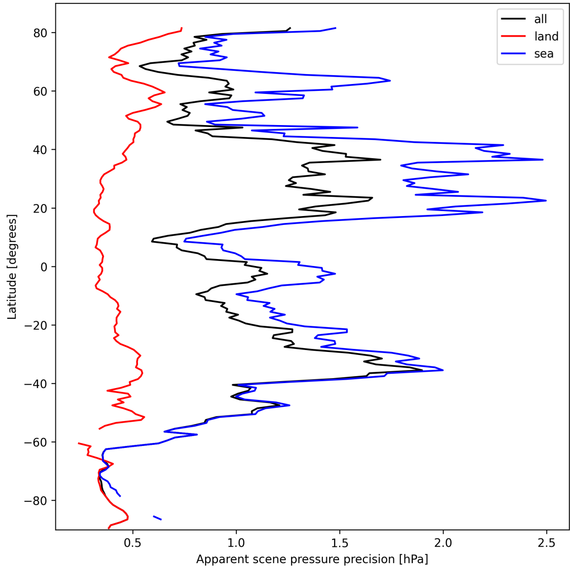
Figure 18: Zonal average of “Apparent scene pressure precision” for 2025-10-08 to 2025-10-09.
