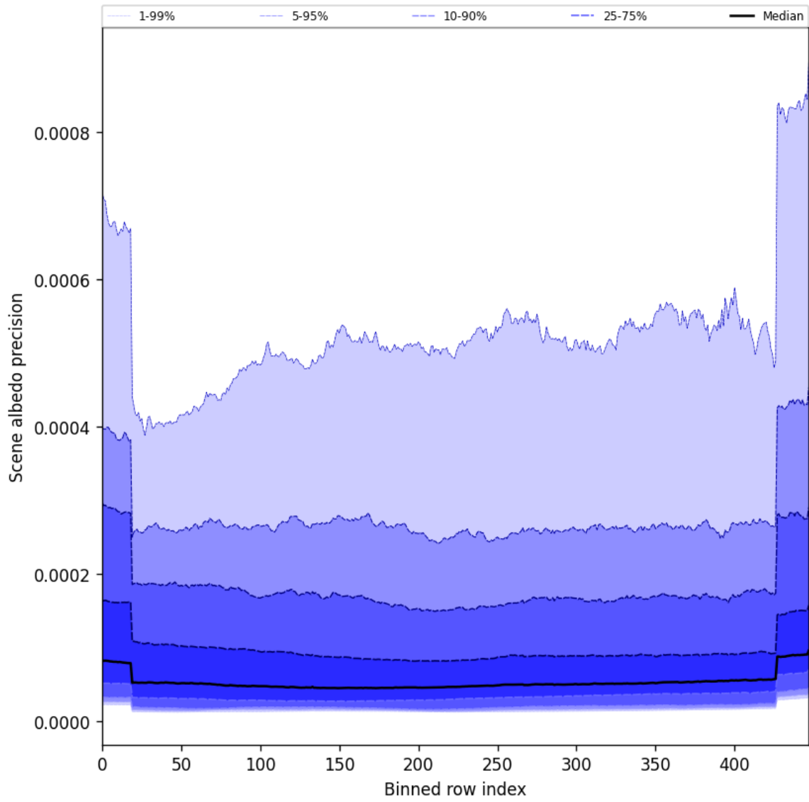
Figure 50: Along track statistics of “Scene albedo precision” for 2025-10-08 to 2025-10-09
