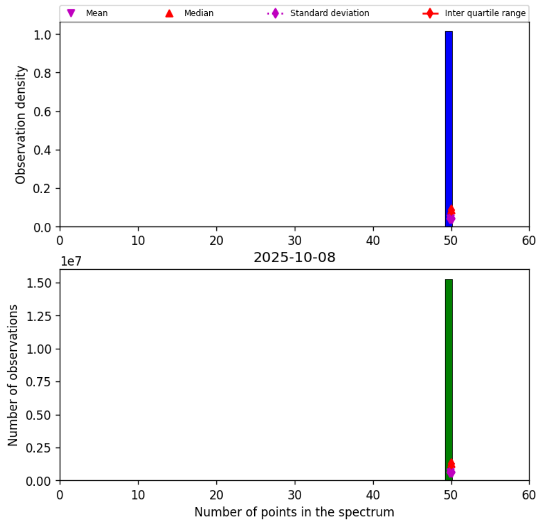
Figure 42: Histogram of “Number of points in the spectrum” for 2025-10-08 to 2025-10-09
