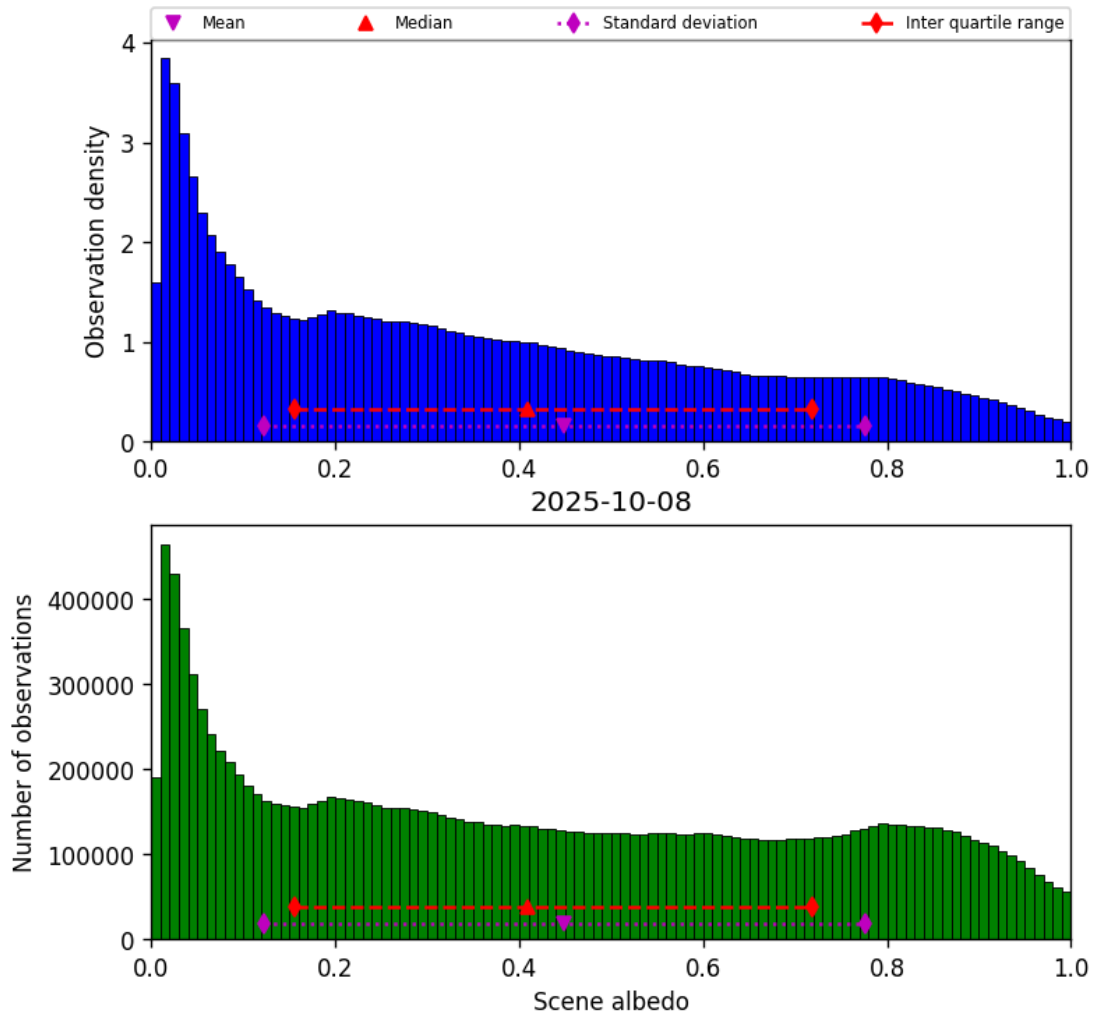
Figure 32: Histogram of “Scene albedo” for 2025-10-08 to 2025-10-09
