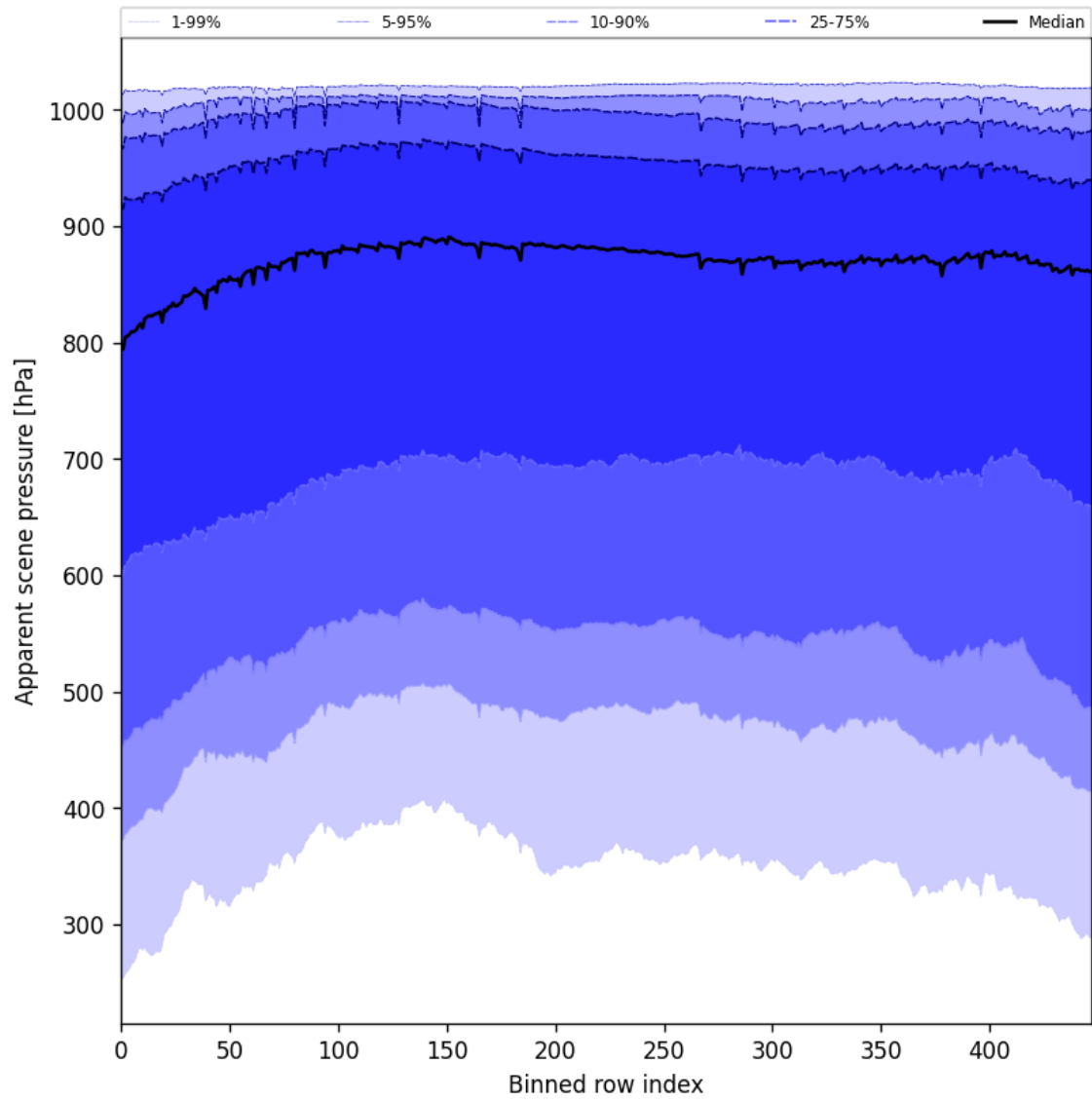
Figure 51: Along track statistics of “Apparent scene pressure” for 2025-10-08 to 2025-10-09
