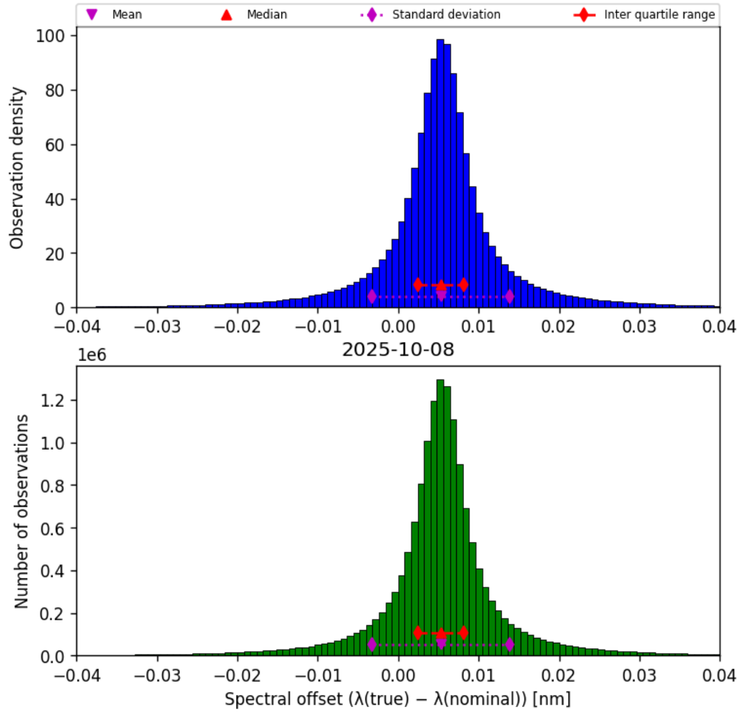
Figure 43: Histogram of “Spectral offset ( \lambda_{\text{true}} - \lambda_{\text{nominal}} )” for 2025-10-08 to 2025-10-09
