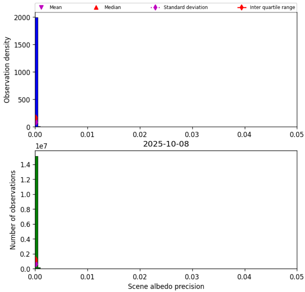
Figure 33: Histogram of “Scene albedo precision” for 2025-10-08 to 2025-10-09
