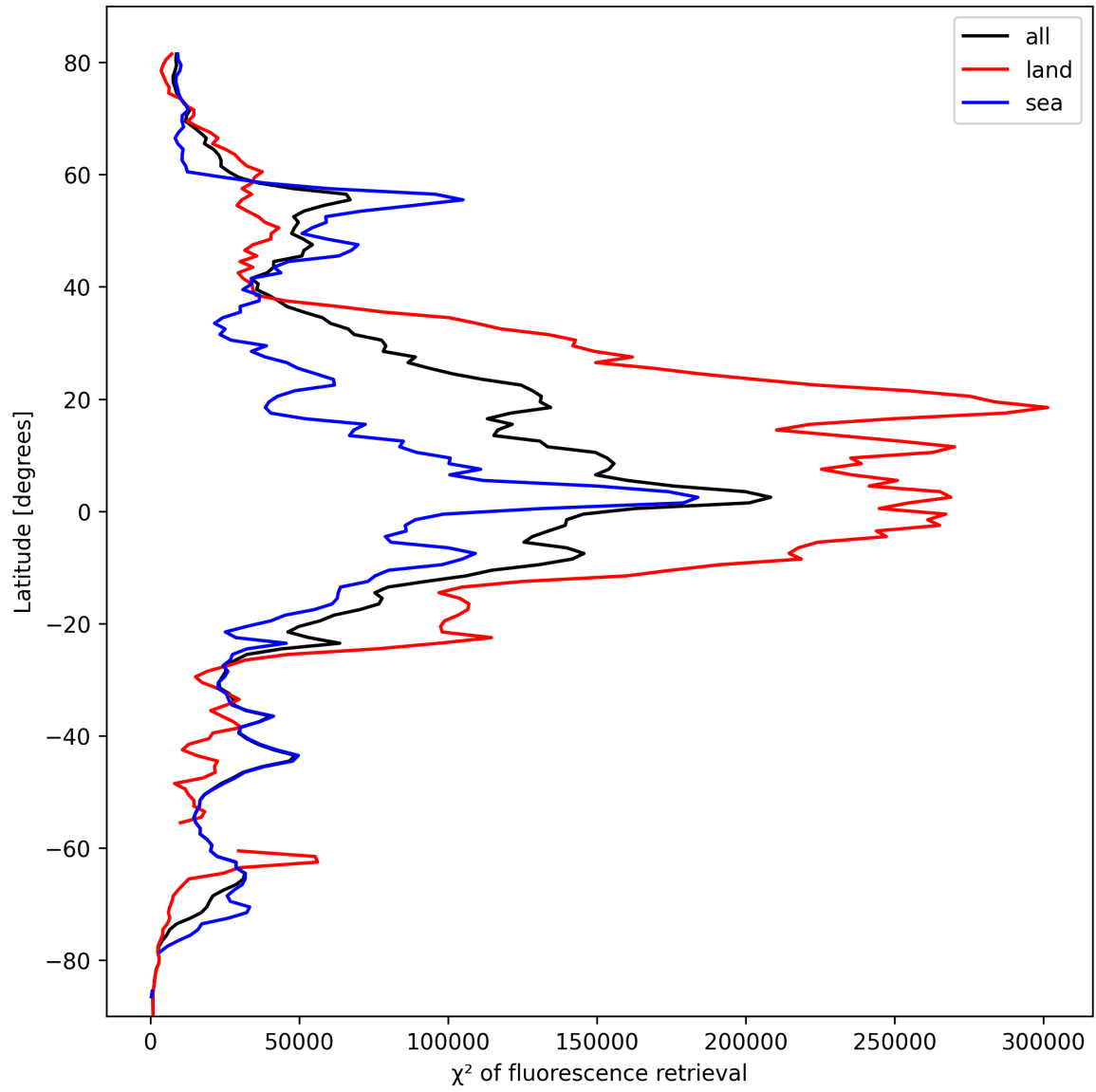
Figure 23: Zonal average of “ \chi^2 of fluorescence retrieval” for 2025-10-08 to 2025-10-09.
