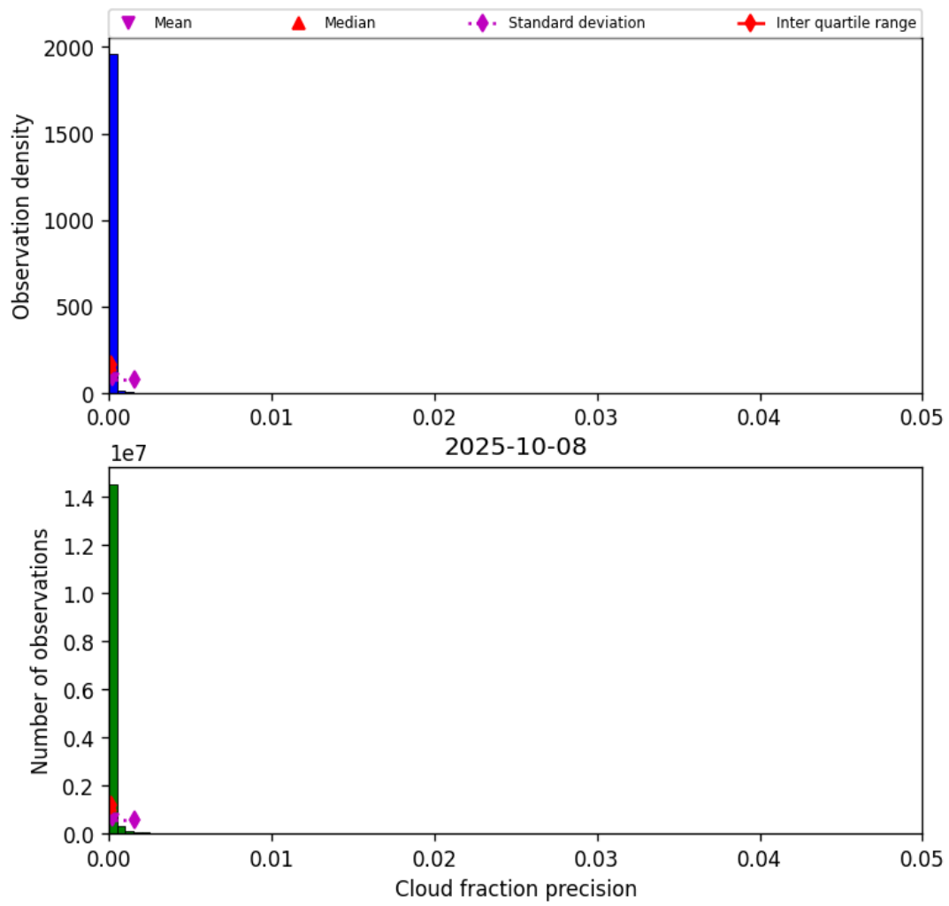
Figure 31: Histogram of “Cloud fraction precision” for 2025-10-08 to 2025-10-09
