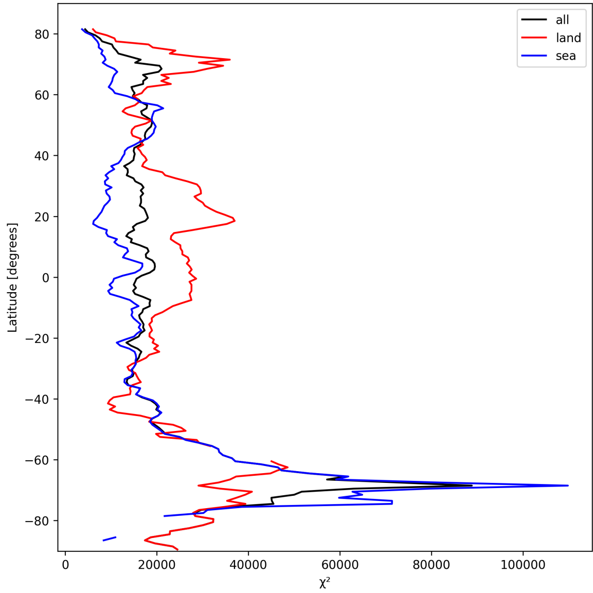
Figure 19: Zonal average of “ \chi^2 ” for 2025-10-08 to 2025-10-09.
