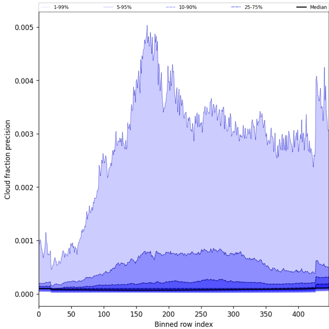
Figure 48: Along track statistics of “Cloud fraction precision” for 2025-10-08 to 2025-10-09
