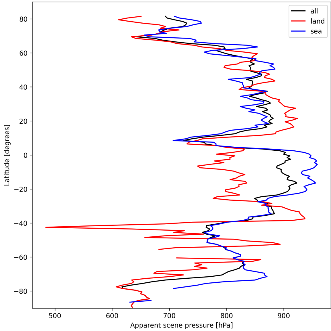
Figure 17: Zonal average of “Apparent scene pressure” for 2025-10-08 to 2025-10-09.
