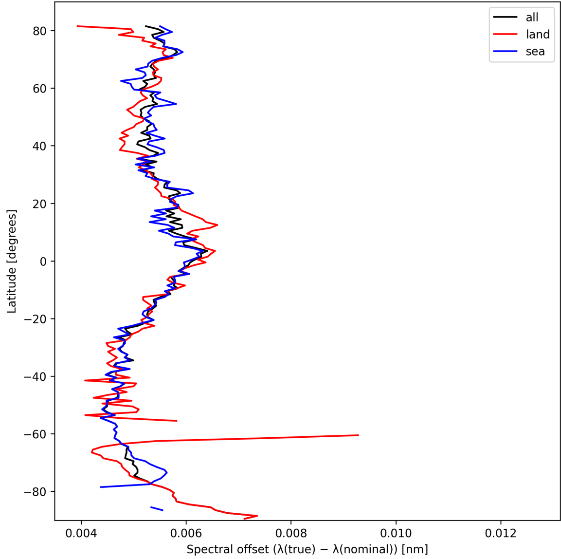
Figure 26: Zonal average of “Spectral offset ( \lambda_{\text{true}} - \lambda_{\text{nominal}} )” for 2025-10-08 to 2025-10-09.
