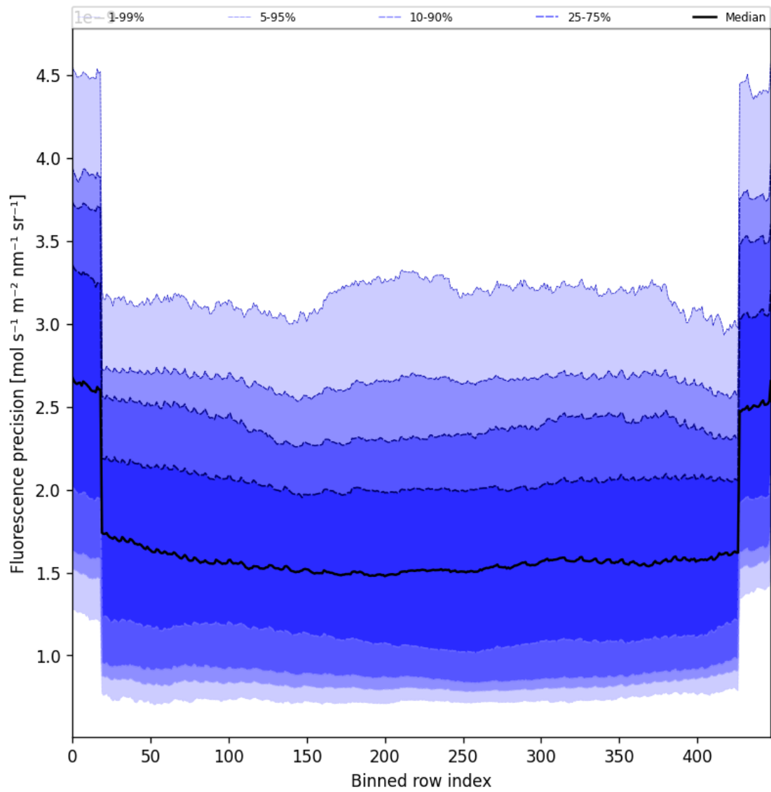
Figure 56: Along track statistics of “Fluorescence precision” for 2025-10-08 to 2025-10-09
