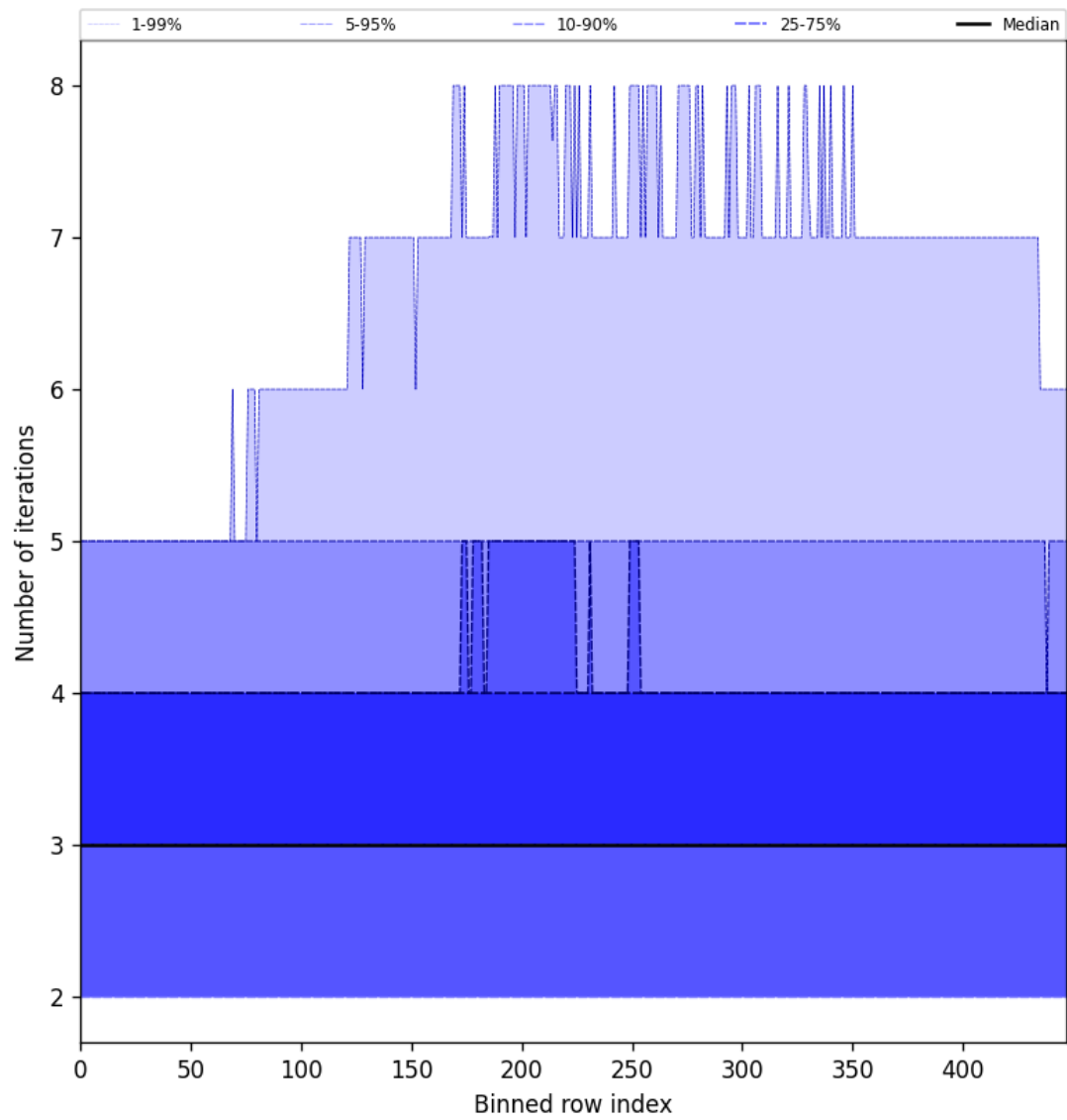
Figure 54: Along track statistics of “Number of iterations” for 2025-10-08 to 2025-10-09
