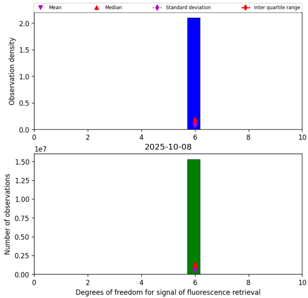
Figure 41: Histogram of "Degrees of freedom for signal of fluorescence retrieval" for 2025-10-08 to 2025-10-09
