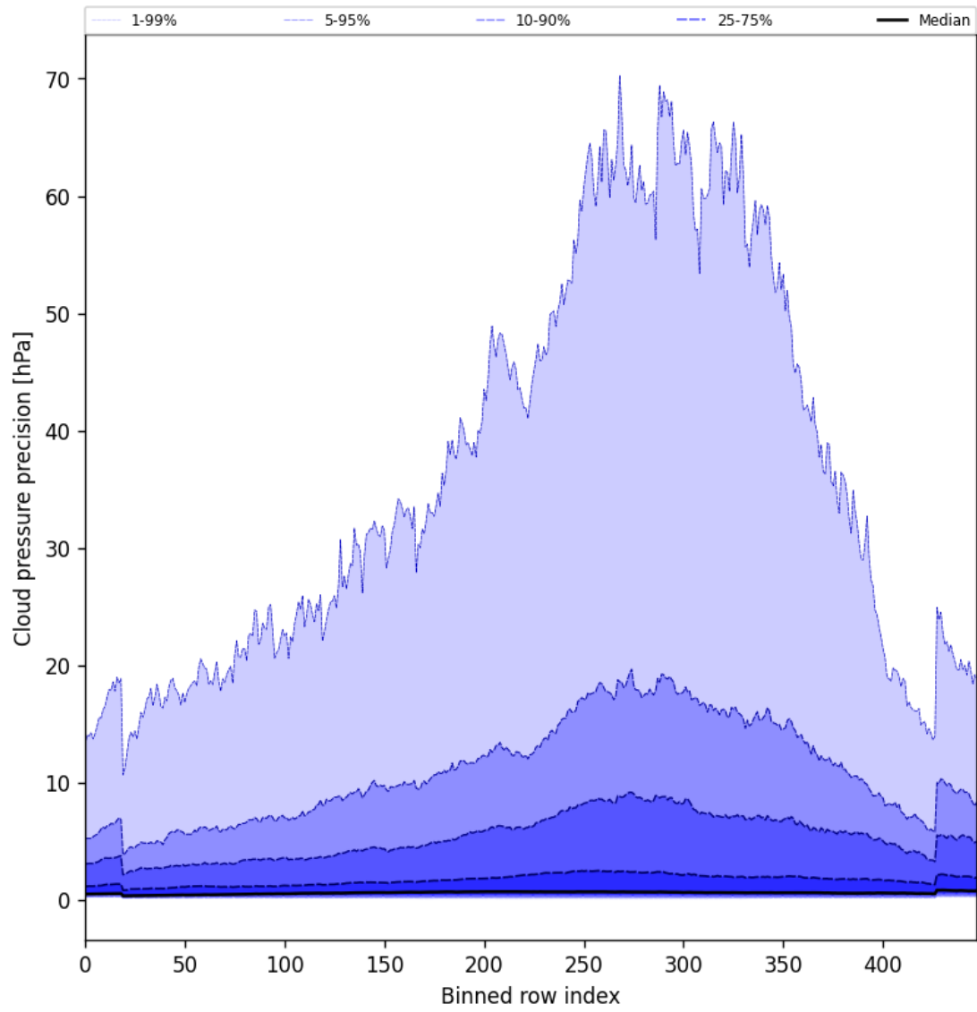
Figure 46: Along track statistics of “Cloud pressure precision” for 2025-10-08 to 2025-10-09
