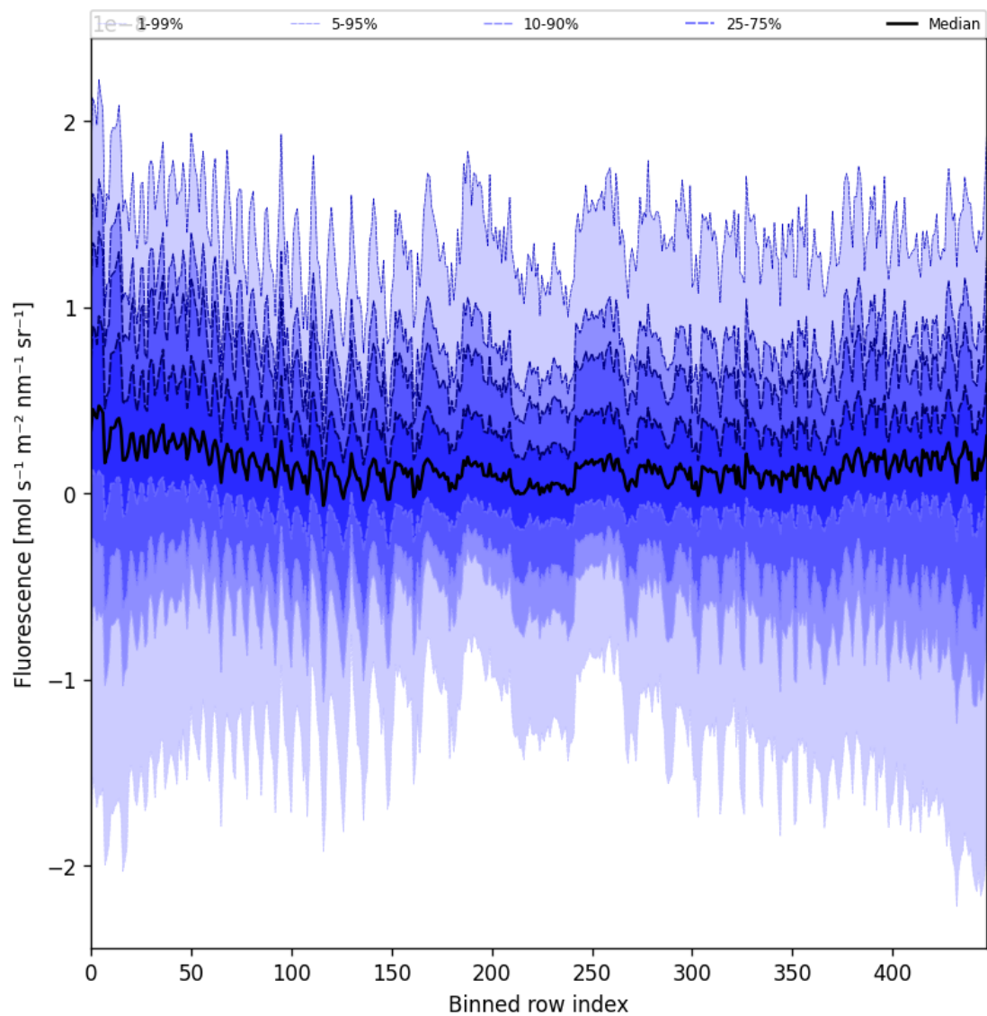
Figure 55: Along track statistics of “Fluorescence” for 2025-10-08 to 2025-10-09
