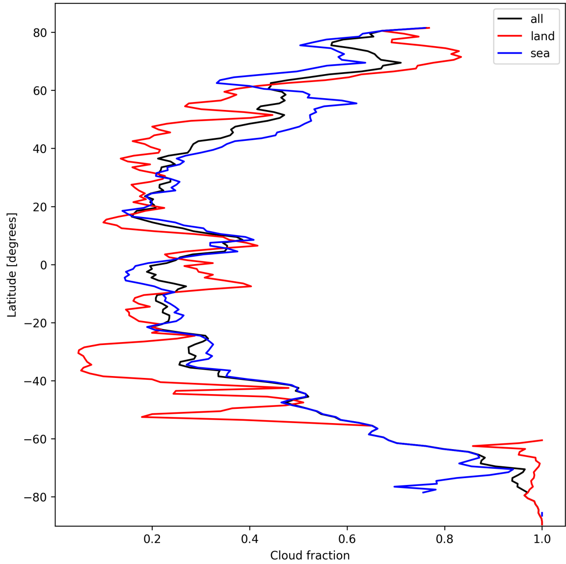
Figure 13: Zonal average of “Cloud fraction” for 2025-10-08 to 2025-10-09.
