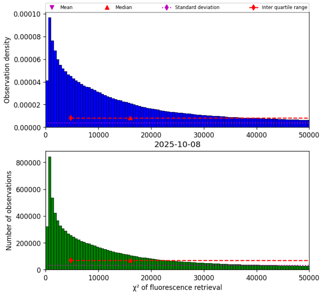
Figure 40: Histogram of “ \chi^2 of fluorescence retrieval” for 2025-10-08 to 2025-10-09
