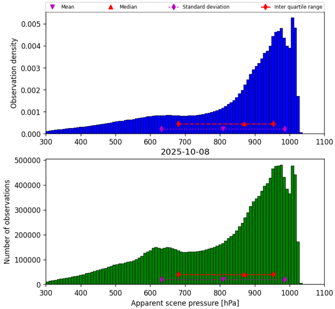
Figure 34: Histogram of “Apparent scene pressure” for 2025-10-08 to 2025-10-09
