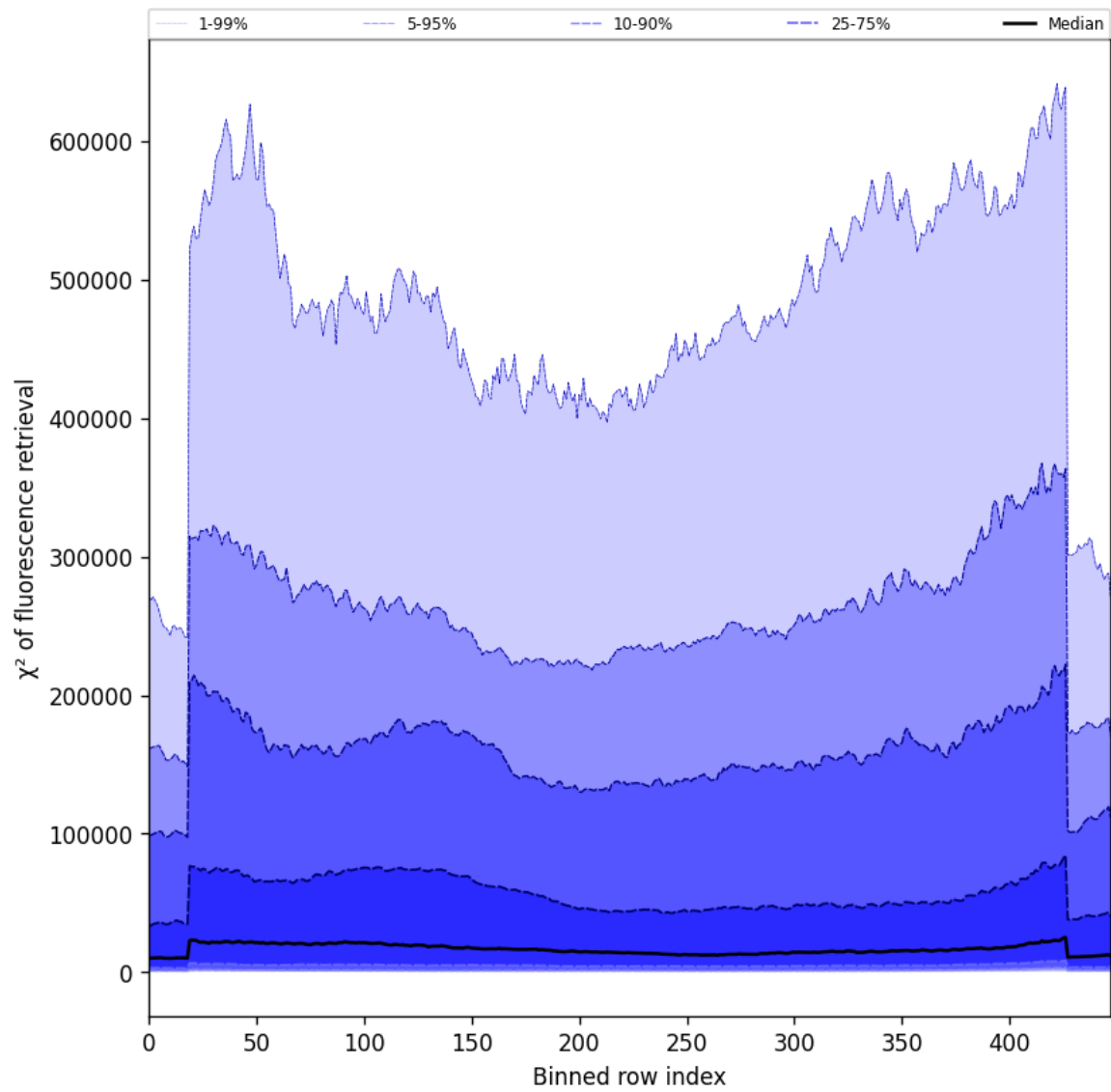
Figure 57: Along track statistics of “ \chi^2 of fluorescence retrieval” for 2025-10-08 to 2025-10-09
