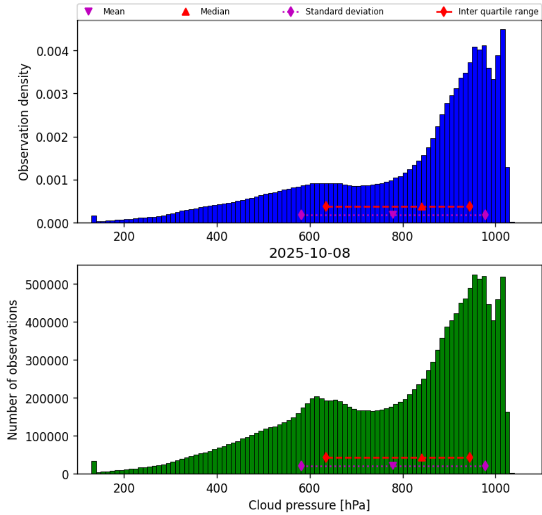
Figure 28: Histogram of “Cloud pressure” for 2025-10-08 to 2025-10-09
