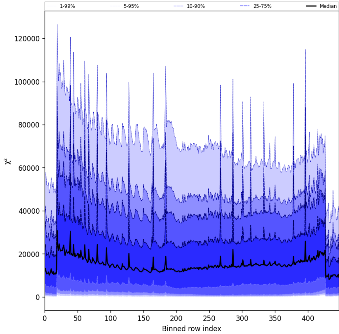
Figure 53: Along track statistics of “ \chi^2 ” for 2025-10-08 to 2025-10-09
