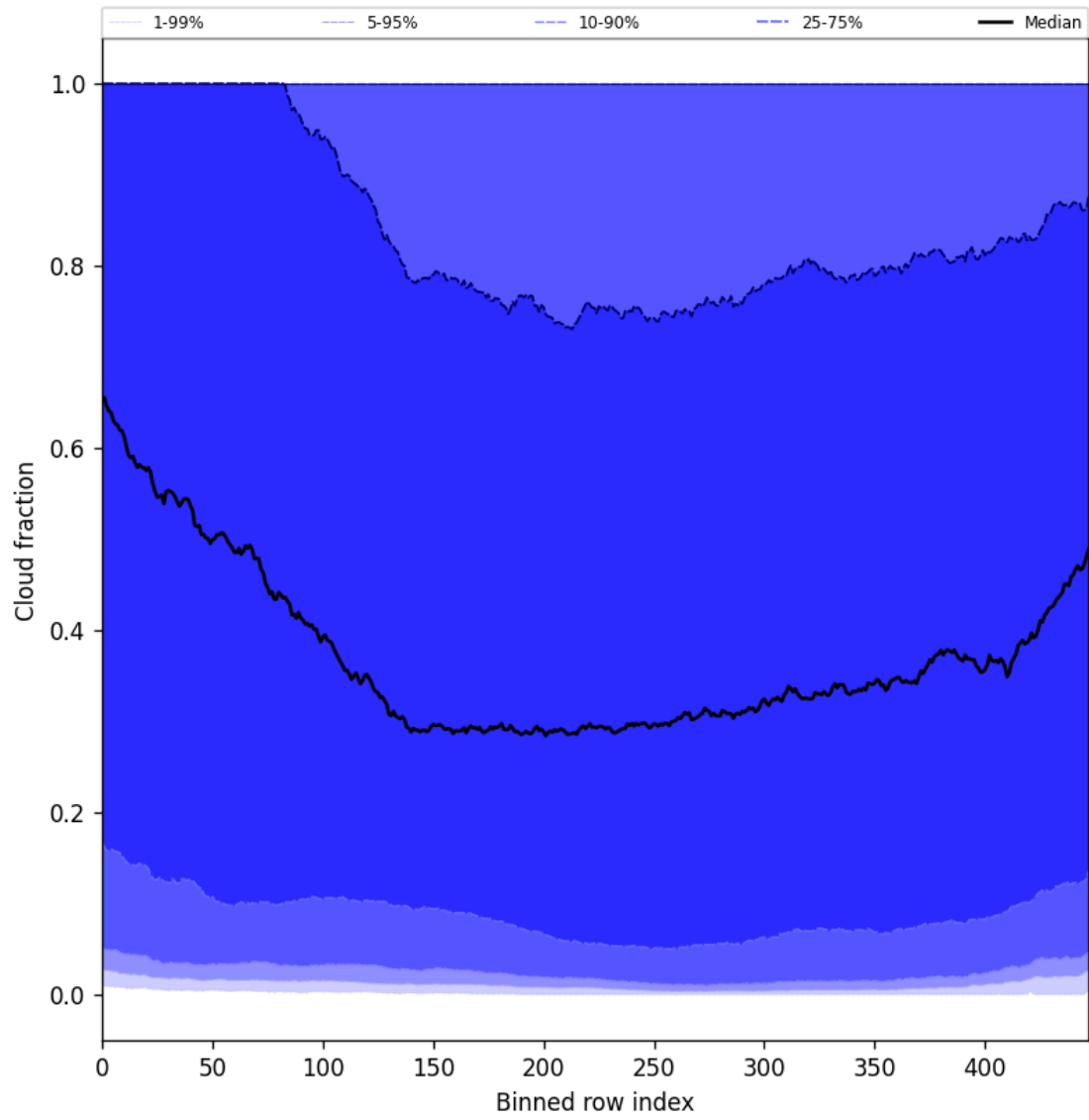
Figure 47: Along track statistics of “Cloud fraction” for 2025-10-08 to 2025-10-09
