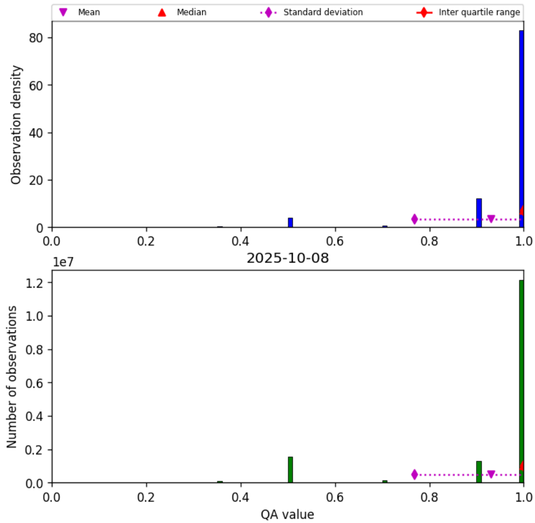
Figure 27: Histogram of “QA value” for 2025-10-08 to 2025-10-09
