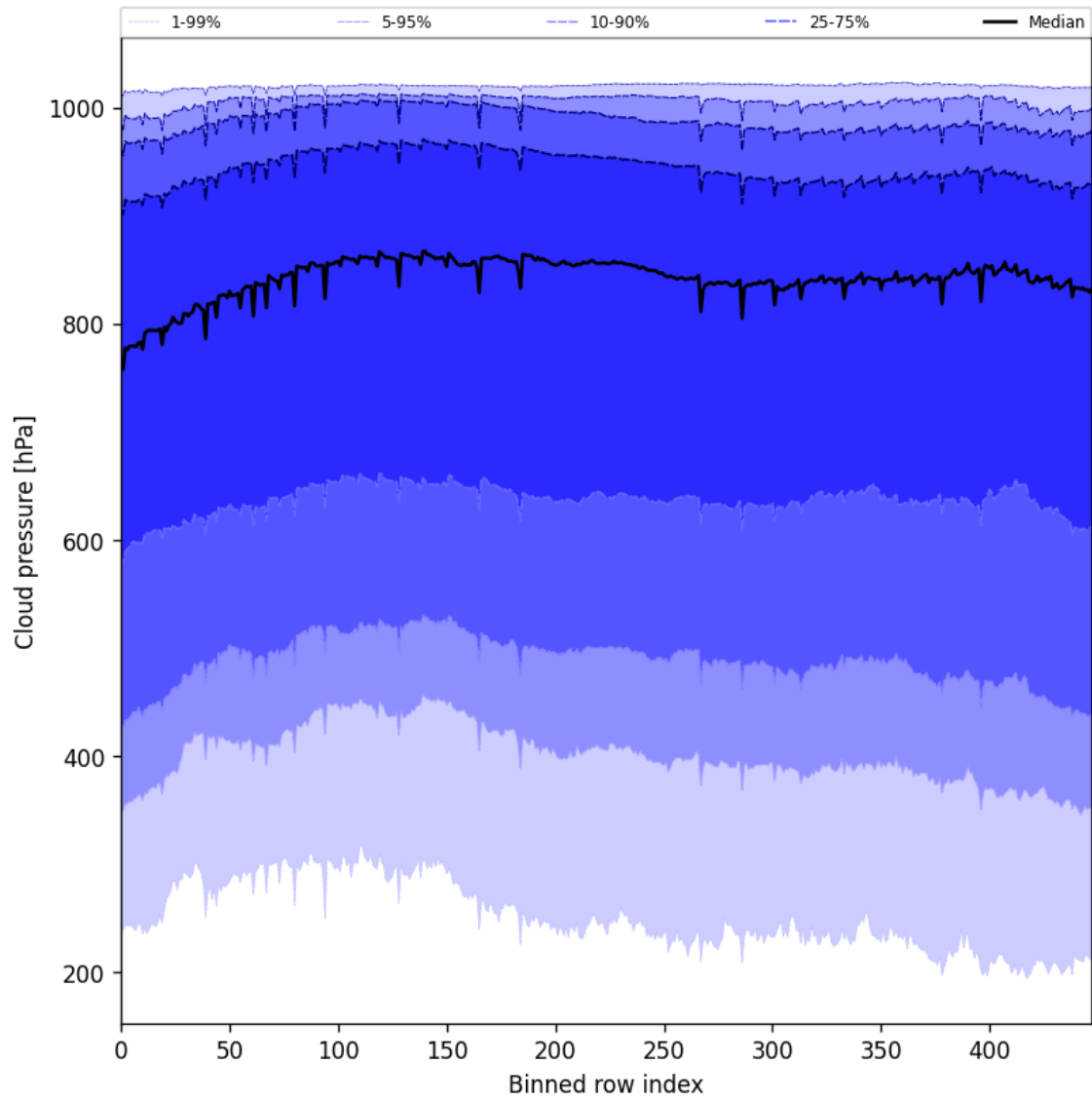
Figure 45: Along track statistics of “Cloud pressure” for 2025-10-08 to 2025-10-09
