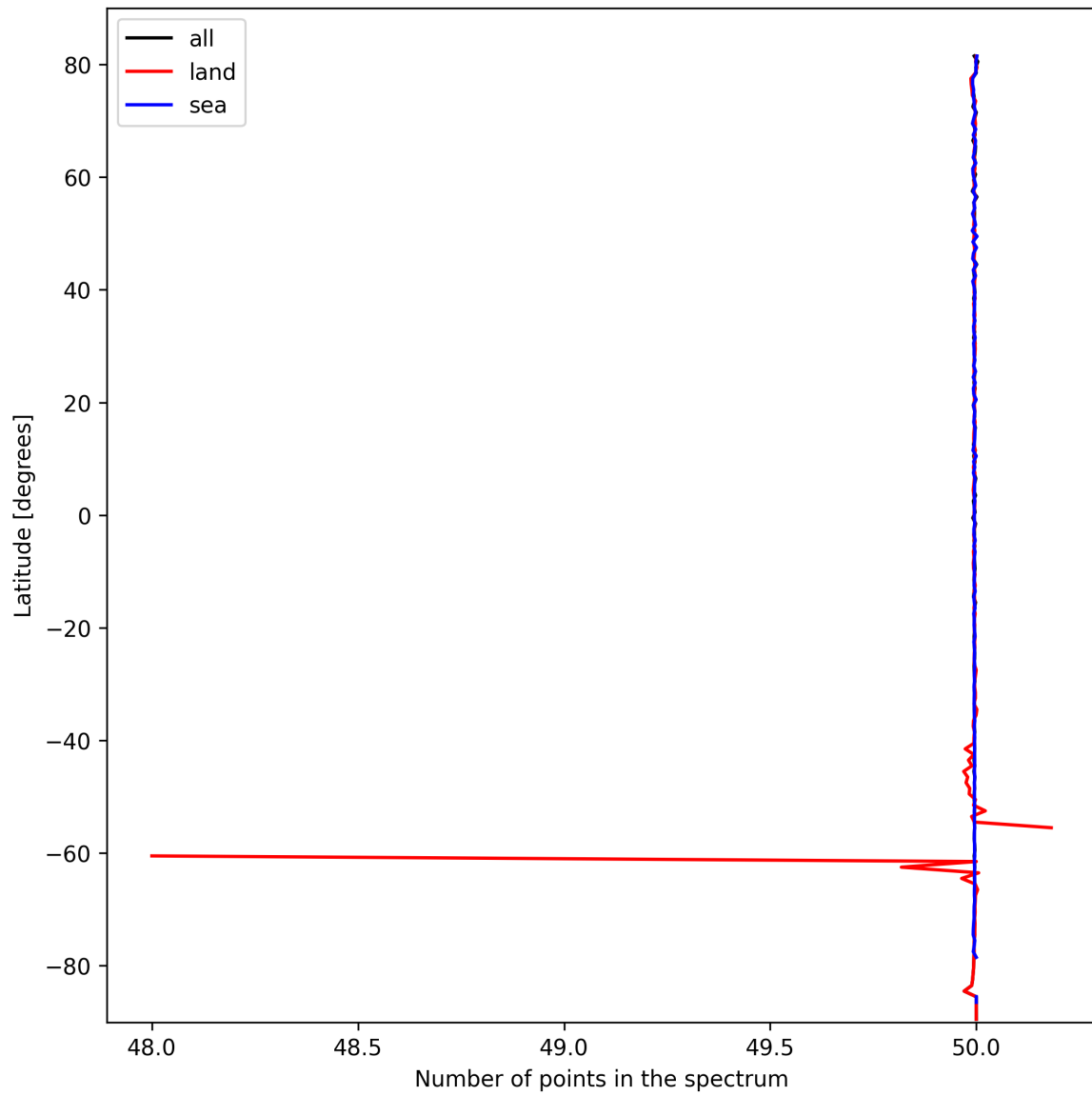
Figure 25: Zonal average of “Number of points in the spectrum” for 2025-10-08 to 2025-10-09.
