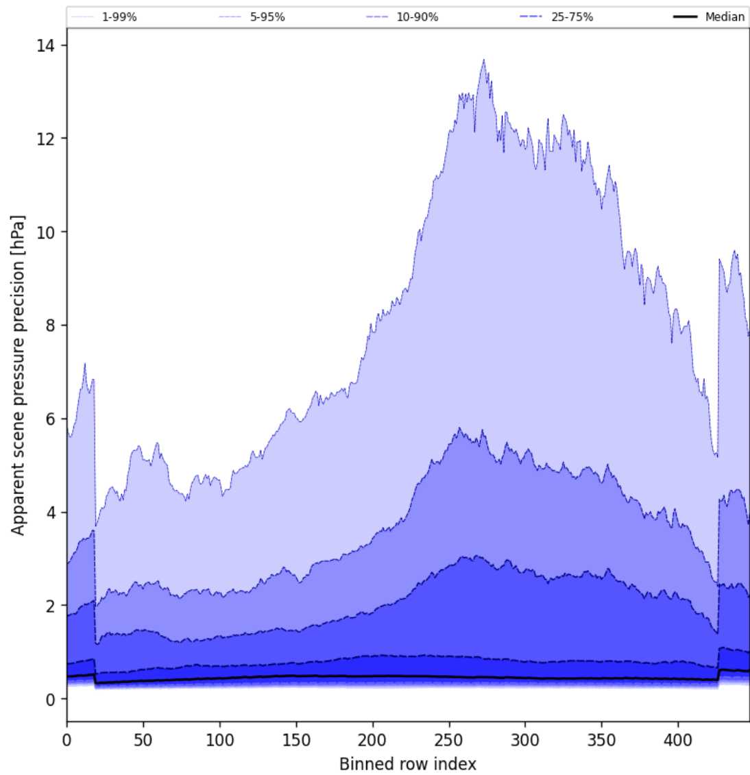
Figure 52: Along track statistics of “Apparent scene pressure precision” for 2025-10-08 to 2025-10-09
