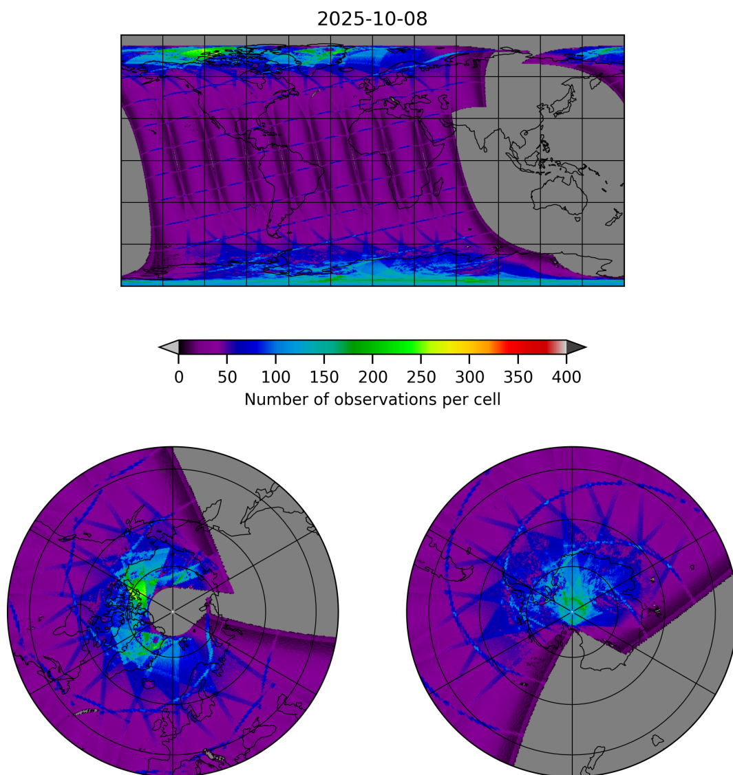
Figure 9: Map of the number of observations for 2025-10-08 to 2025-10-09
