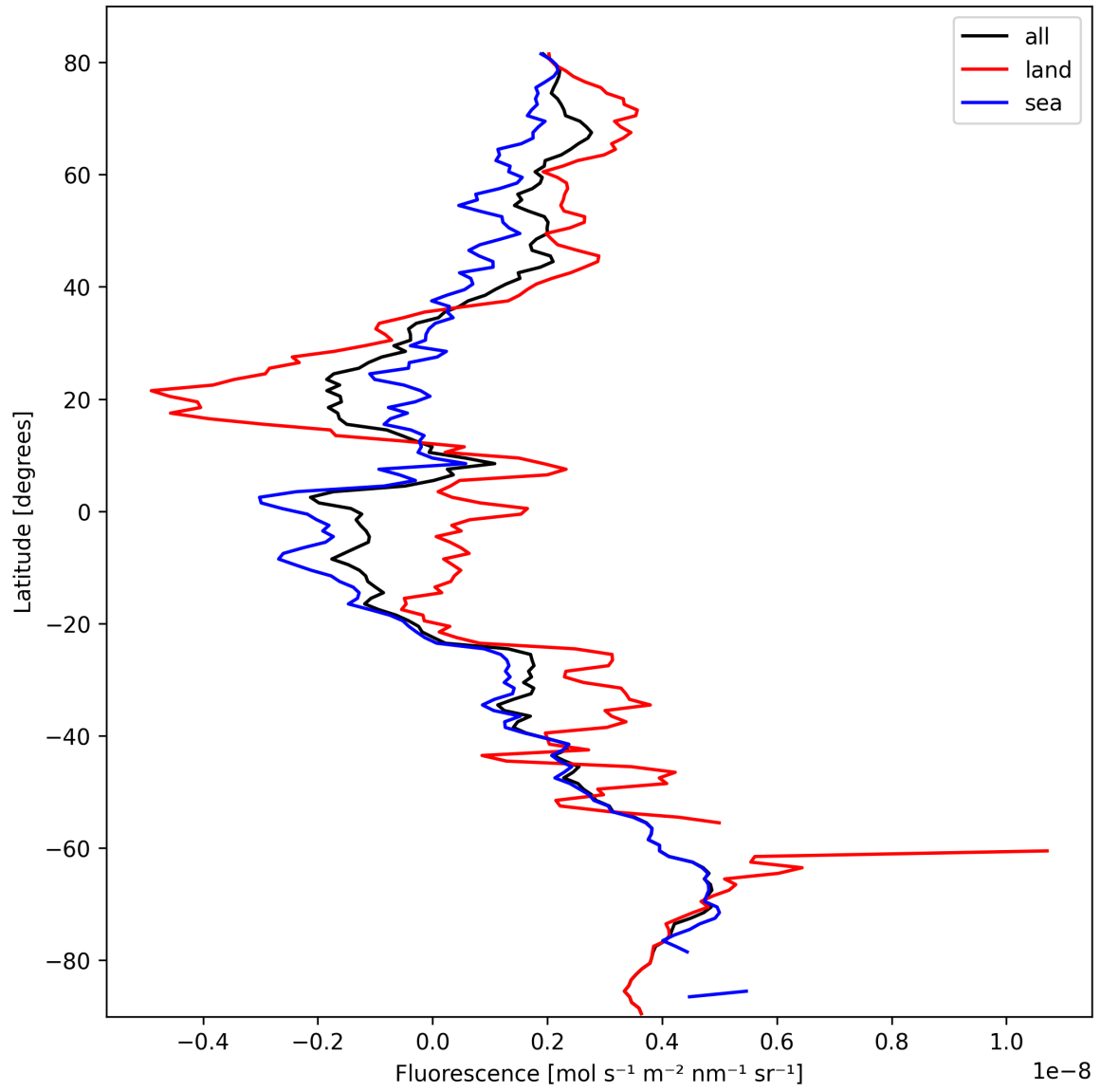
Figure 21: Zonal average of “Fluorescence” for 2025-10-08 to 2025-10-09.
