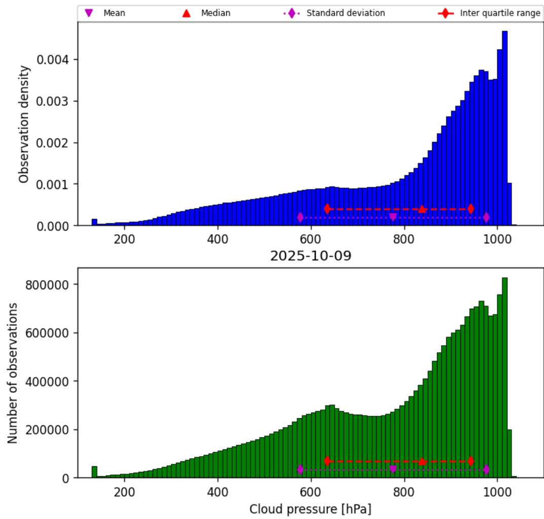
Figure 28: Histogram of “Cloud pressure” for 2025-10-09 to 2025-10-09
