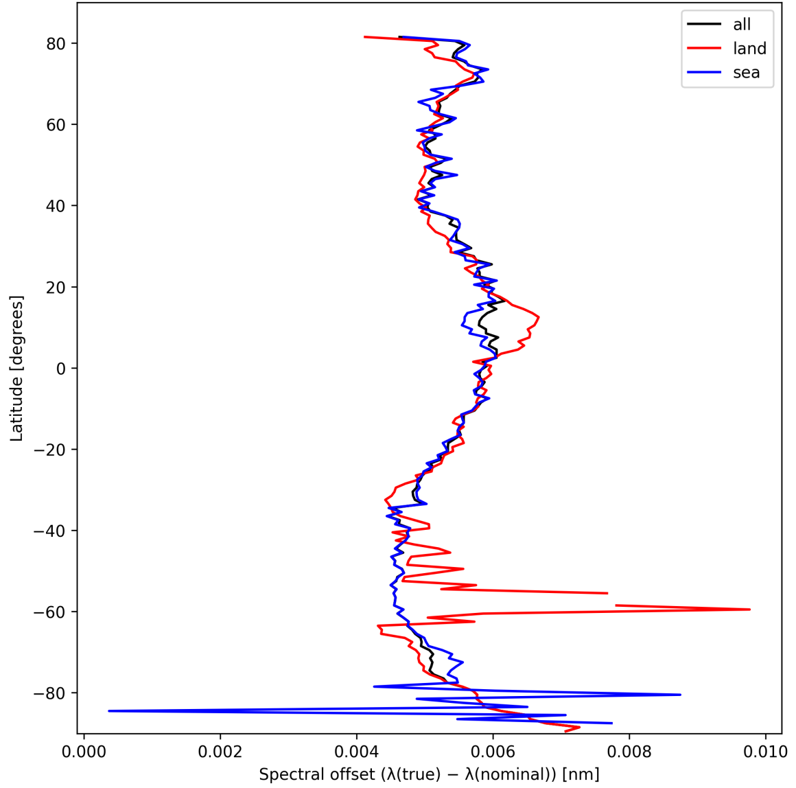
Figure 26: Zonal average of “Spectral offset ( \lambda_{\text{true}} - \lambda_{\text{nominal}} )” for 2025-10-09 to 2025-10-09.
