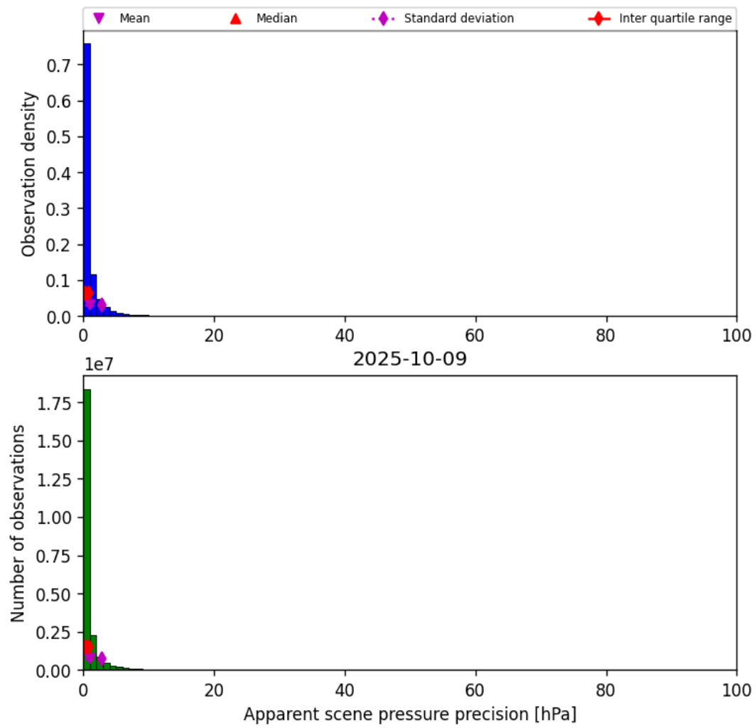
Figure 35: Histogram of “Apparent scene pressure precision” for 2025-10-09 to 2025-10-09
