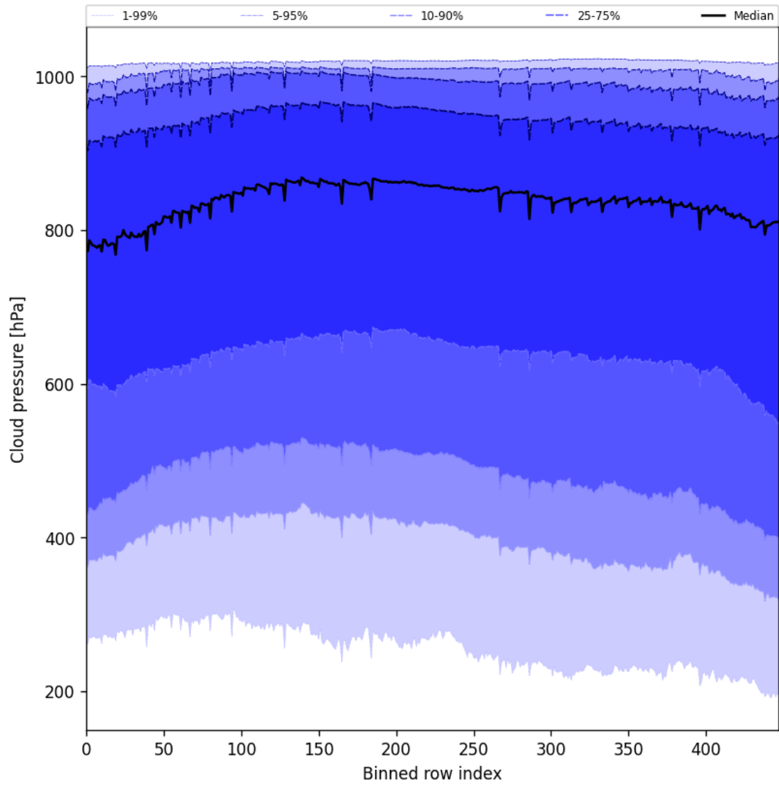
Figure 45: Along track statistics of “Cloud pressure” for 2025-10-09 to 2025-10-09
