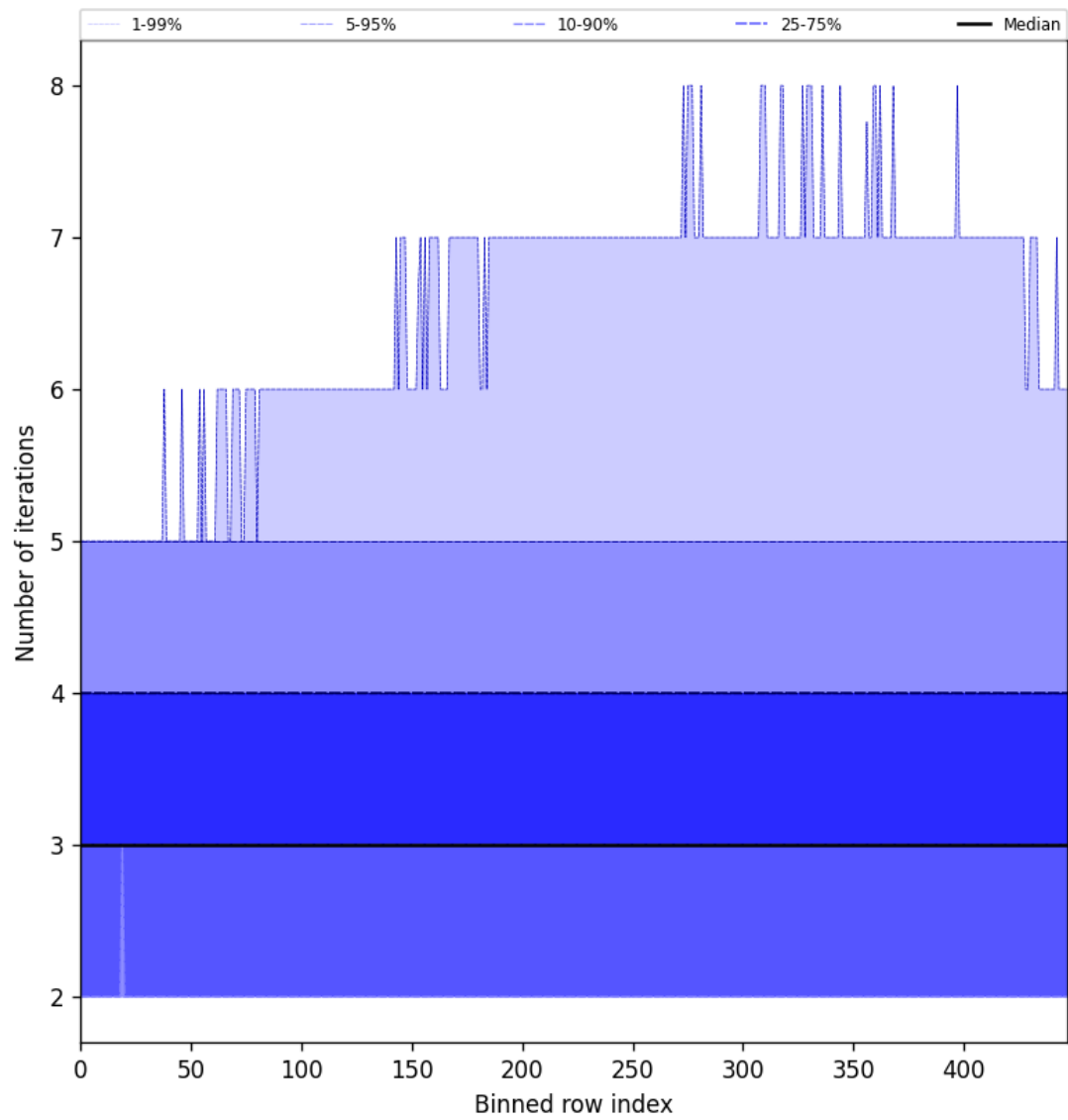
Figure 54: Along track statistics of “Number of iterations” for 2025-10-09 to 2025-10-09
