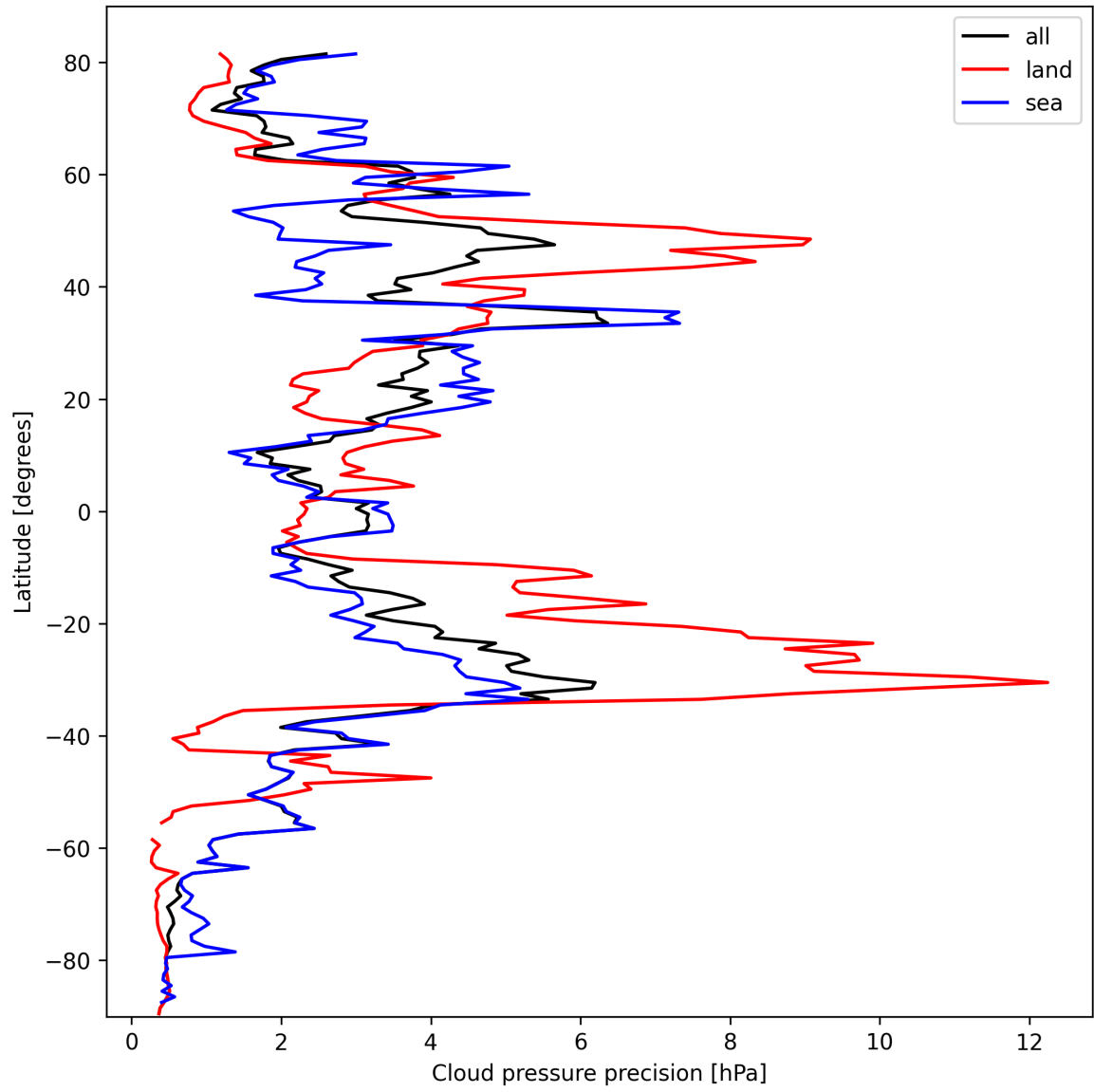
Figure 12: Zonal average of “Cloud pressure precision” for 2025-10-09 to 2025-10-09.
