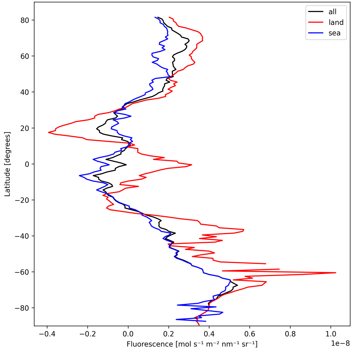
Figure 21: Zonal average of “Fluorescence” for 2025-10-09 to 2025-10-09.
