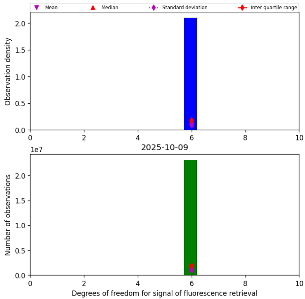
Figure 41: Histogram of “Degrees of freedom for signal of fluorescence retrieval” for 2025-10-09 to 2025-10-09
