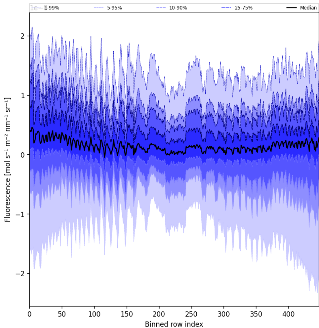
Figure 55: Along track statistics of “Fluorescence” for 2025-10-09 to 2025-10-09
