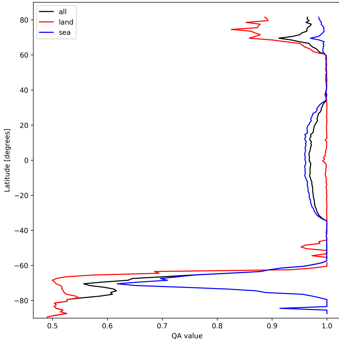
Figure 10: Zonal average of “QA value” for 2025-10-09 to 2025-10-09.
