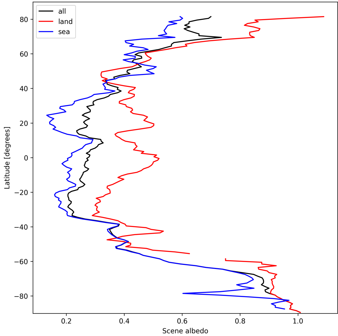
Figure 15: Zonal average of “Scene albedo” for 2025-10-09 to 2025-10-09.
