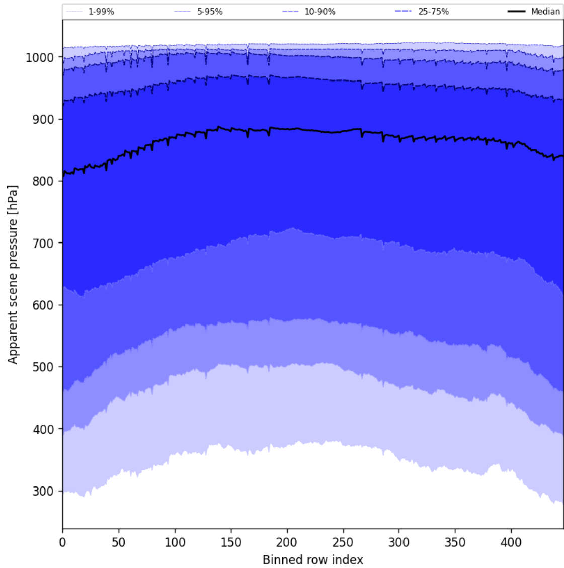
Figure 51: Along track statistics of “Apparent scene pressure” for 2025-10-09 to 2025-10-09
