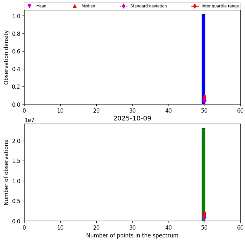
Figure 42: Histogram of “Number of points in the spectrum” for 2025-10-09 to 2025-10-09
