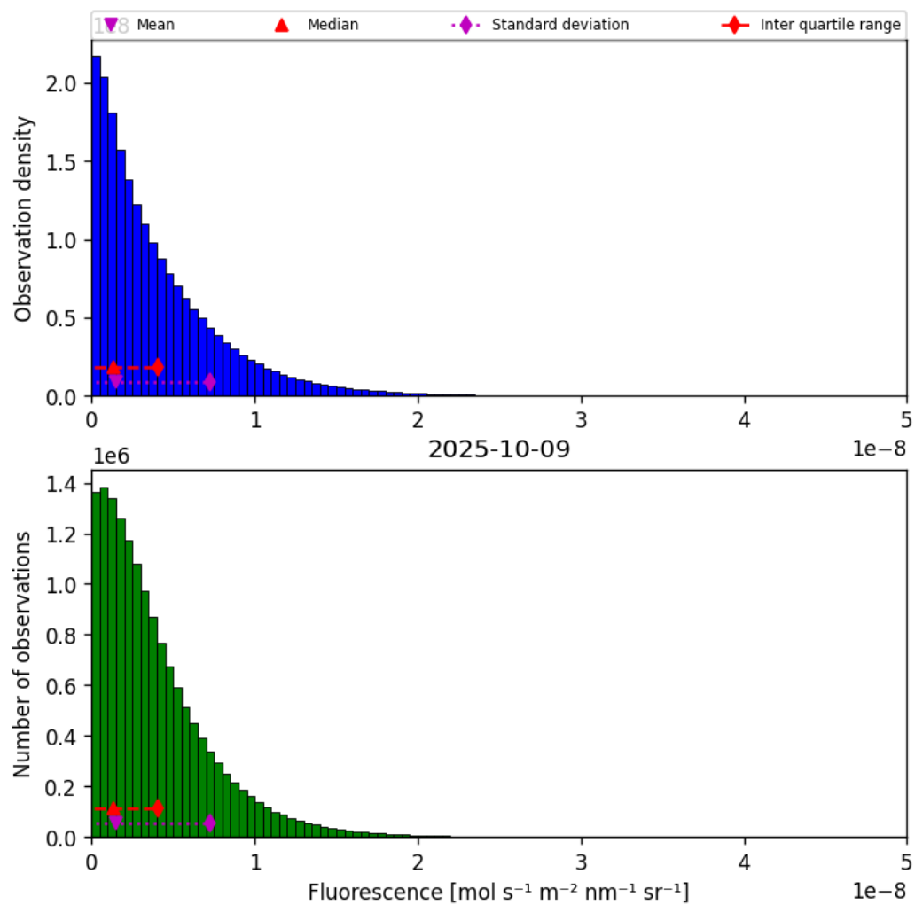
Figure 38: Histogram of “Fluorescence” for 2025-10-09 to 2025-10-09
