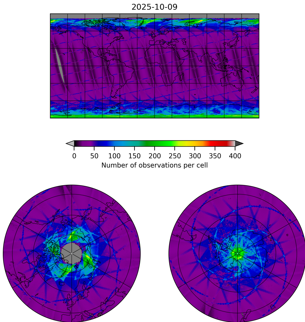
Figure 9: Map of the number of observations for 2025-10-09 to 2025-10-09
