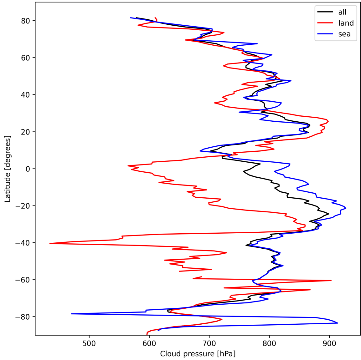
Figure 11: Zonal average of “Cloud pressure” for 2025-10-09 to 2025-10-09.
