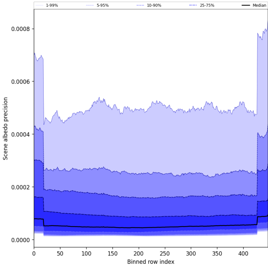
Figure 50: Along track statistics of “Scene albedo precision” for 2025-10-09 to 2025-10-09
