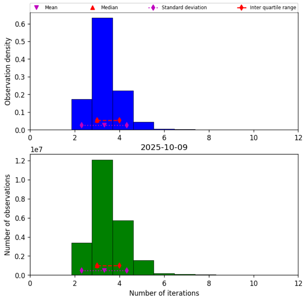
Figure 37: Histogram of “Number of iterations” for 2025-10-09 to 2025-10-09
