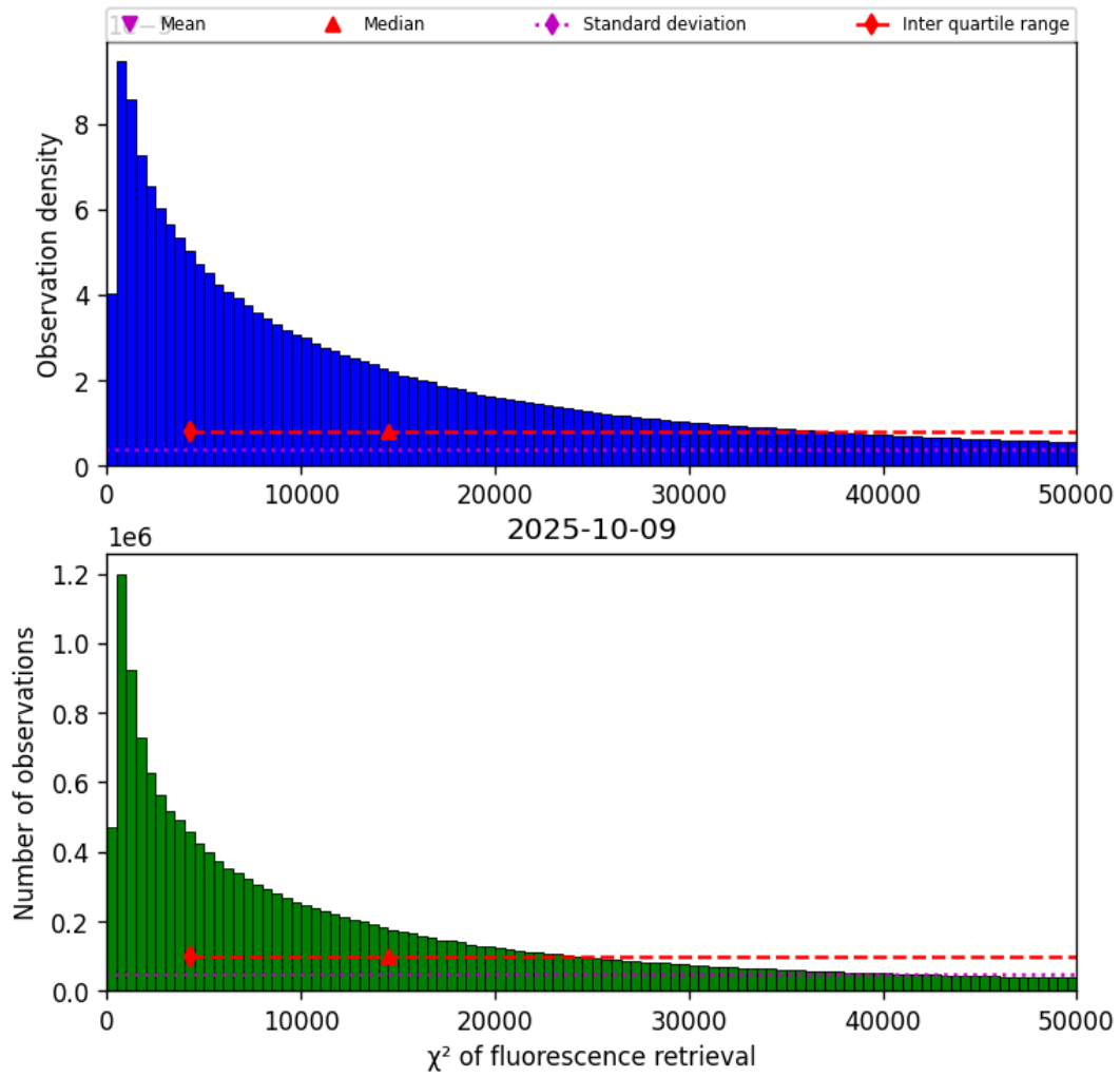
Figure 40: Histogram of “ \chi^2 of fluorescence retrieval” for 2025-10-09 to 2025-10-09
