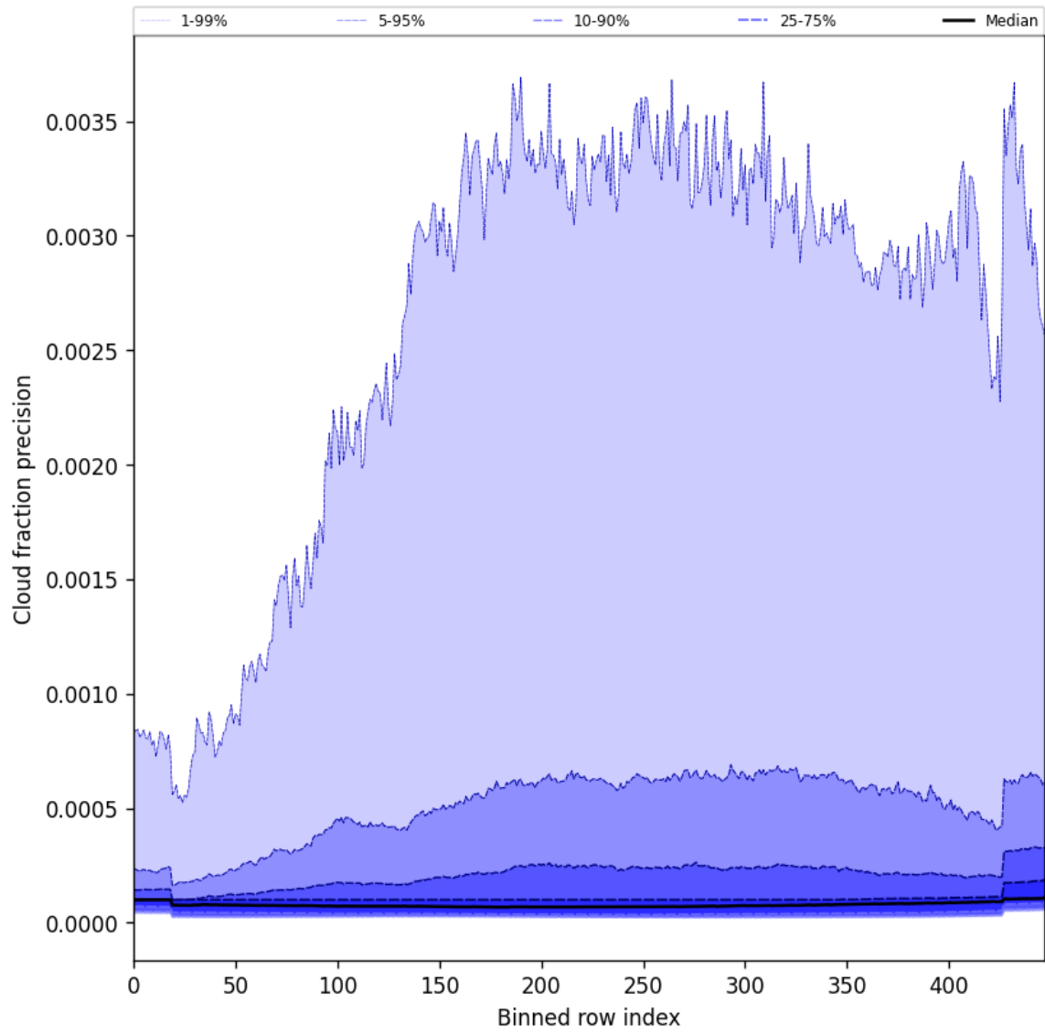
Figure 48: Along track statistics of “Cloud fraction precision” for 2025-10-09 to 2025-10-09
