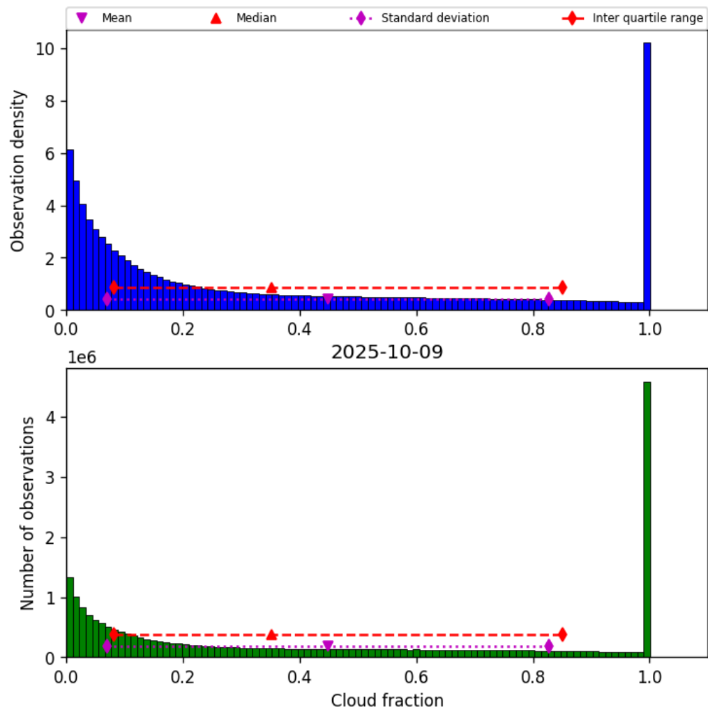
Figure 30: Histogram of “Cloud fraction” for 2025-10-09 to 2025-10-09
