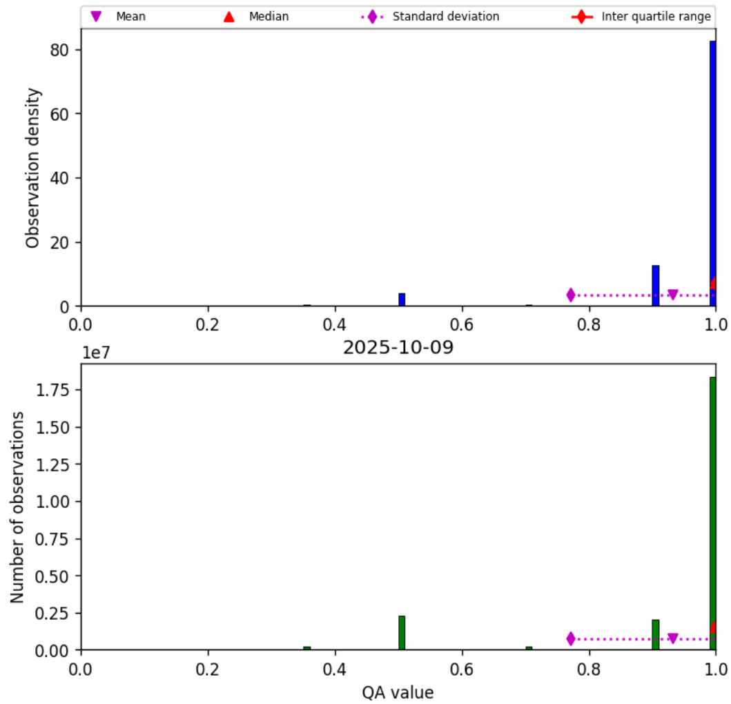
Figure 27: Histogram of “QA value” for 2025-10-09 to 2025-10-09
