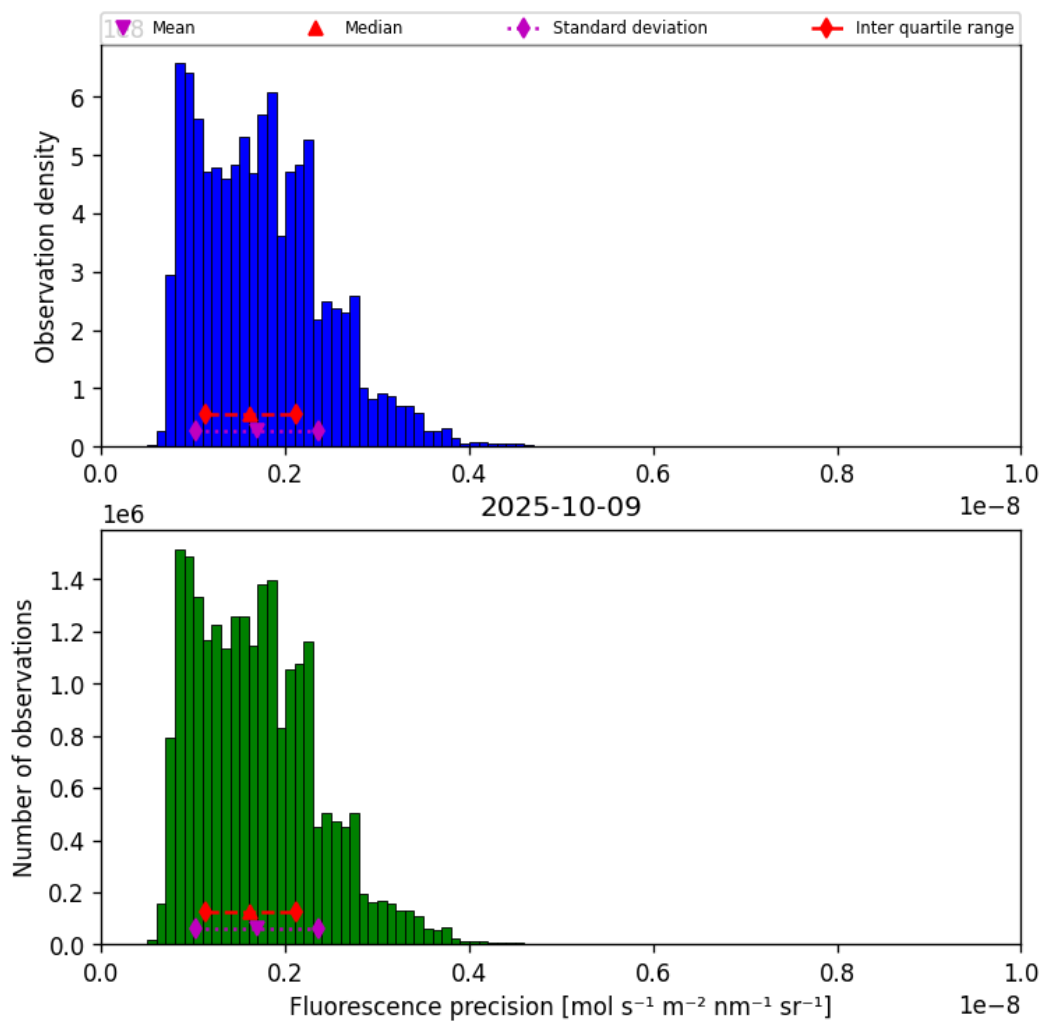
Figure 39: Histogram of “Fluorescence precision” for 2025-10-09 to 2025-10-09
