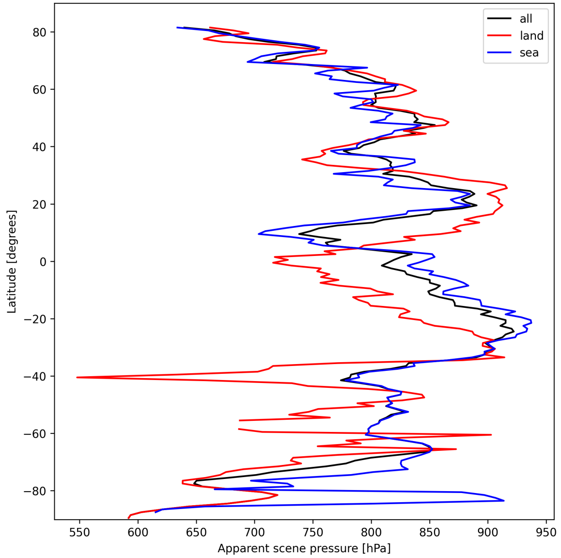
Figure 17: Zonal average of “Apparent scene pressure” for 2025-10-09 to 2025-10-09.
