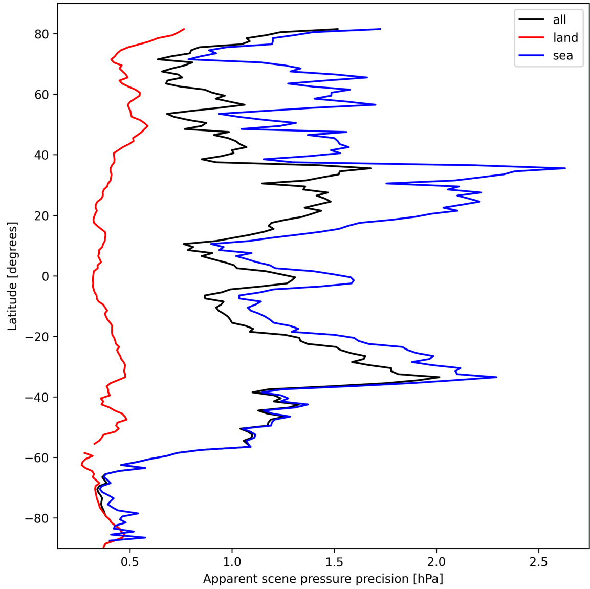
Figure 18: Zonal average of “Apparent scene pressure precision” for 2025-10-09 to 2025-10-09.
