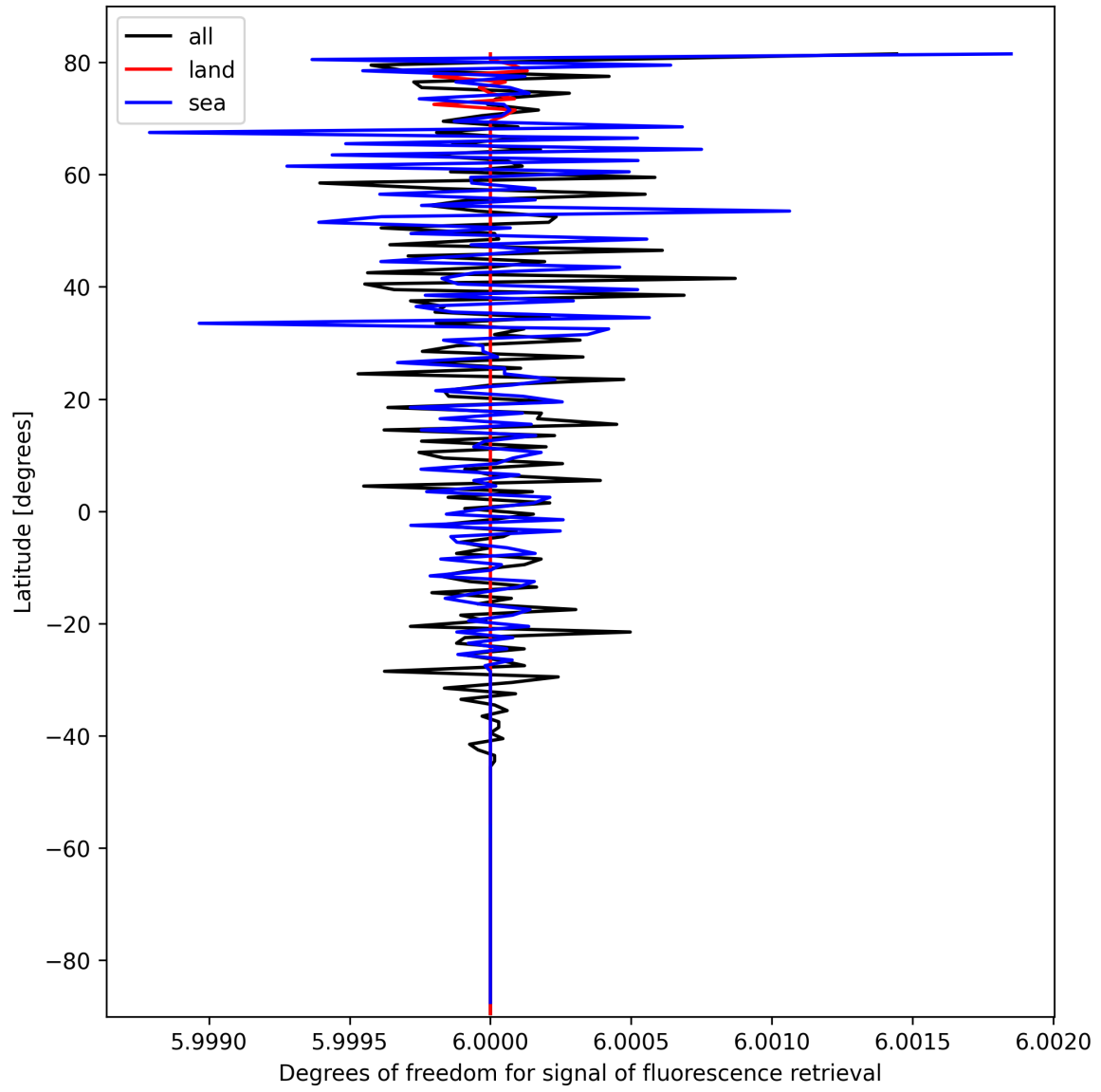
Figure 24: Zonal average of “Degrees of freedom for signal of fluorescence retrieval” for 2025-10-09 to 2025-10-09.
