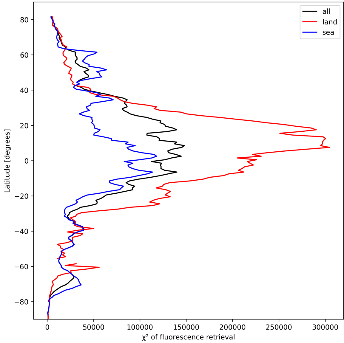
Figure 23: Zonal average of “ \chi^2 of fluorescence retrieval” for 2025-10-09 to 2025-10-09.
