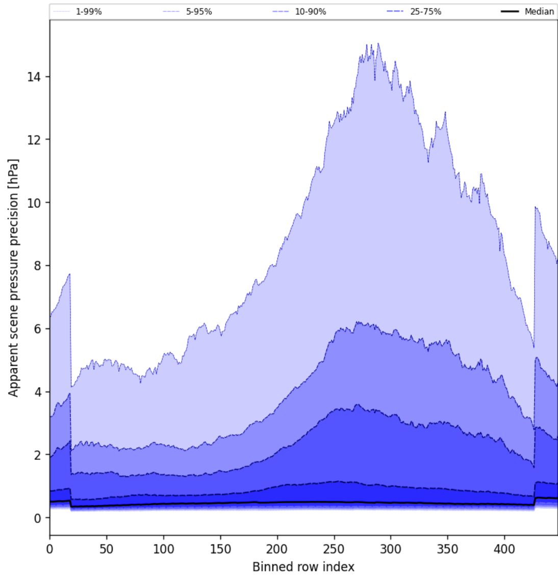
Figure 52: Along track statistics of “Apparent scene pressure precision” for 2025-10-09 to 2025-10-09
