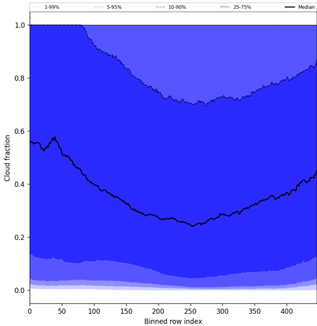
Figure 47: Along track statistics of “Cloud fraction” for 2025-10-09 to 2025-10-09
