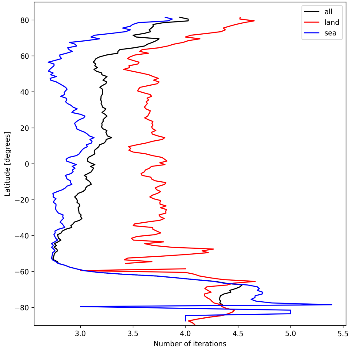
Figure 20: Zonal average of “Number of iterations” for 2025-10-09 to 2025-10-09.
