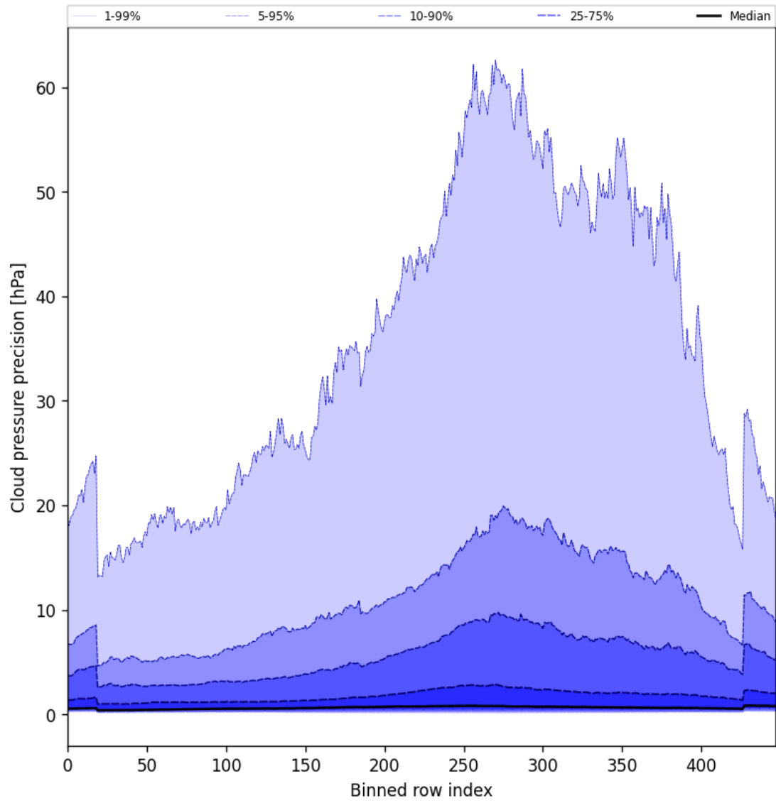
Figure 46: Along track statistics of “Cloud pressure precision” for 2025-10-09 to 2025-10-09
