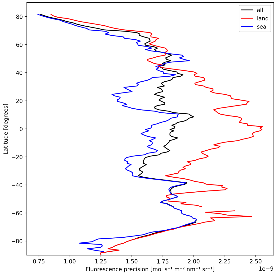
Figure 22: Zonal average of “Fluorescence precision” for 2025-10-09 to 2025-10-09.
