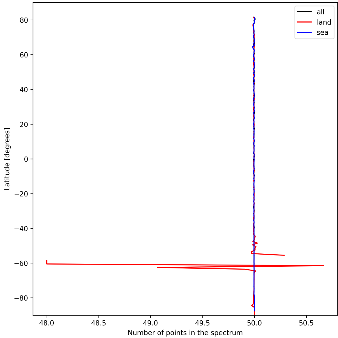
Figure 25: Zonal average of “Number of points in the spectrum” for 2025-10-09 to 2025-10-09.
