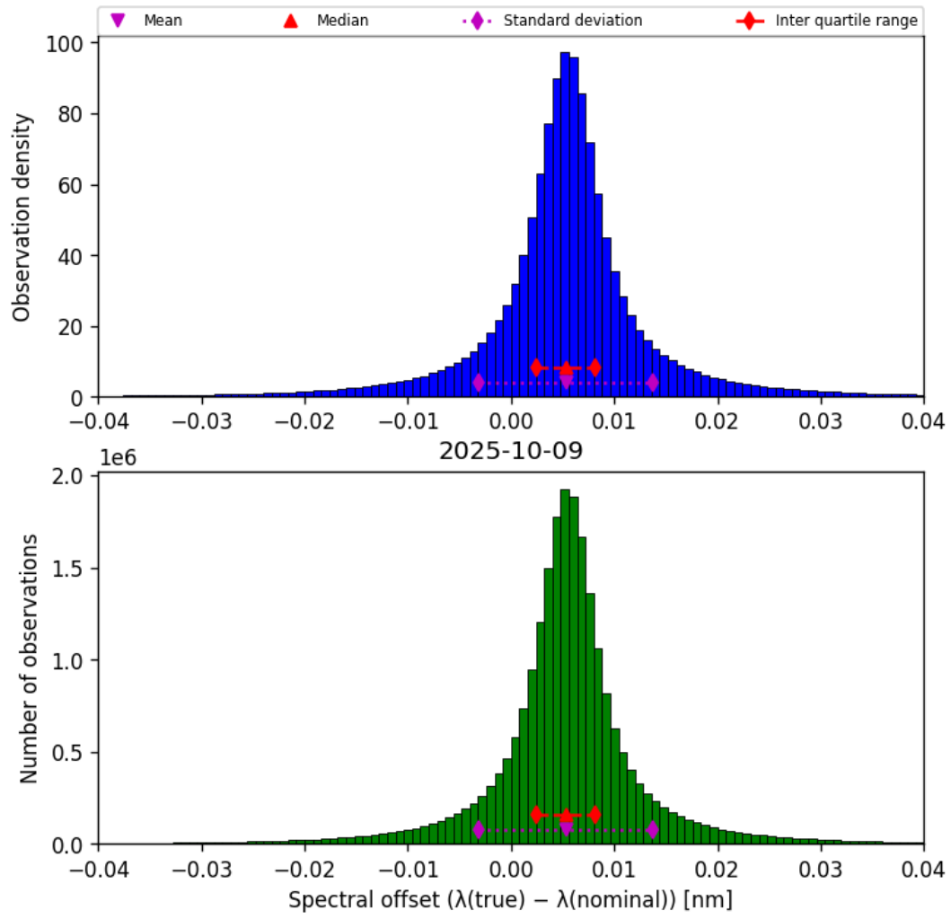
Figure 43: Histogram of “Spectral offset ( \lambda_{\text{true}} - \lambda_{\text{nominal}} )” for 2025-10-09 to 2025-10-09
