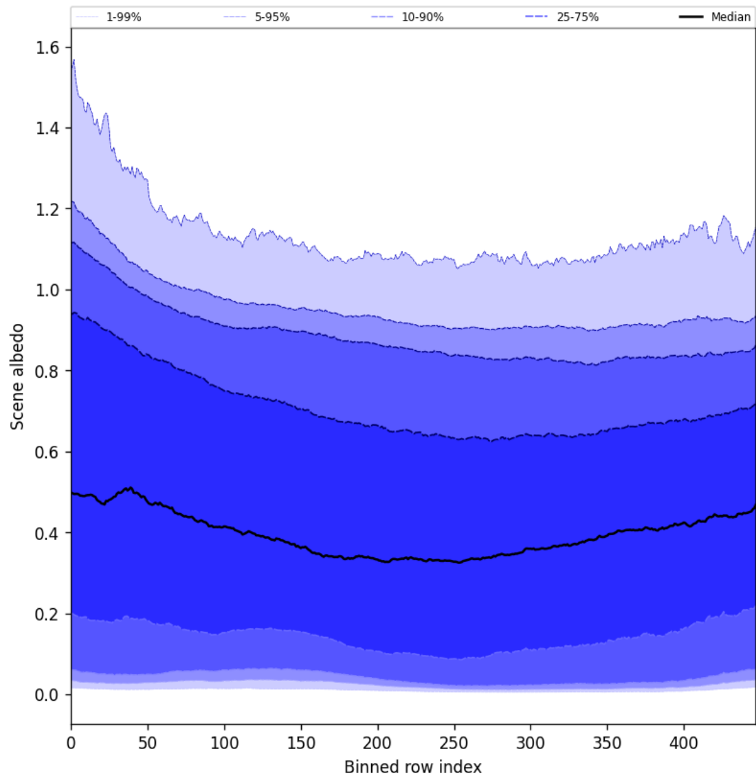
Figure 49: Along track statistics of “Scene albedo” for 2025-10-09 to 2025-10-09
