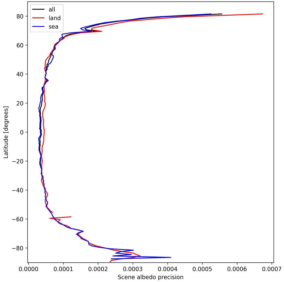
Figure 16: Zonal average of “Scene albedo precision” for 2025-10-09 to 2025-10-09.
