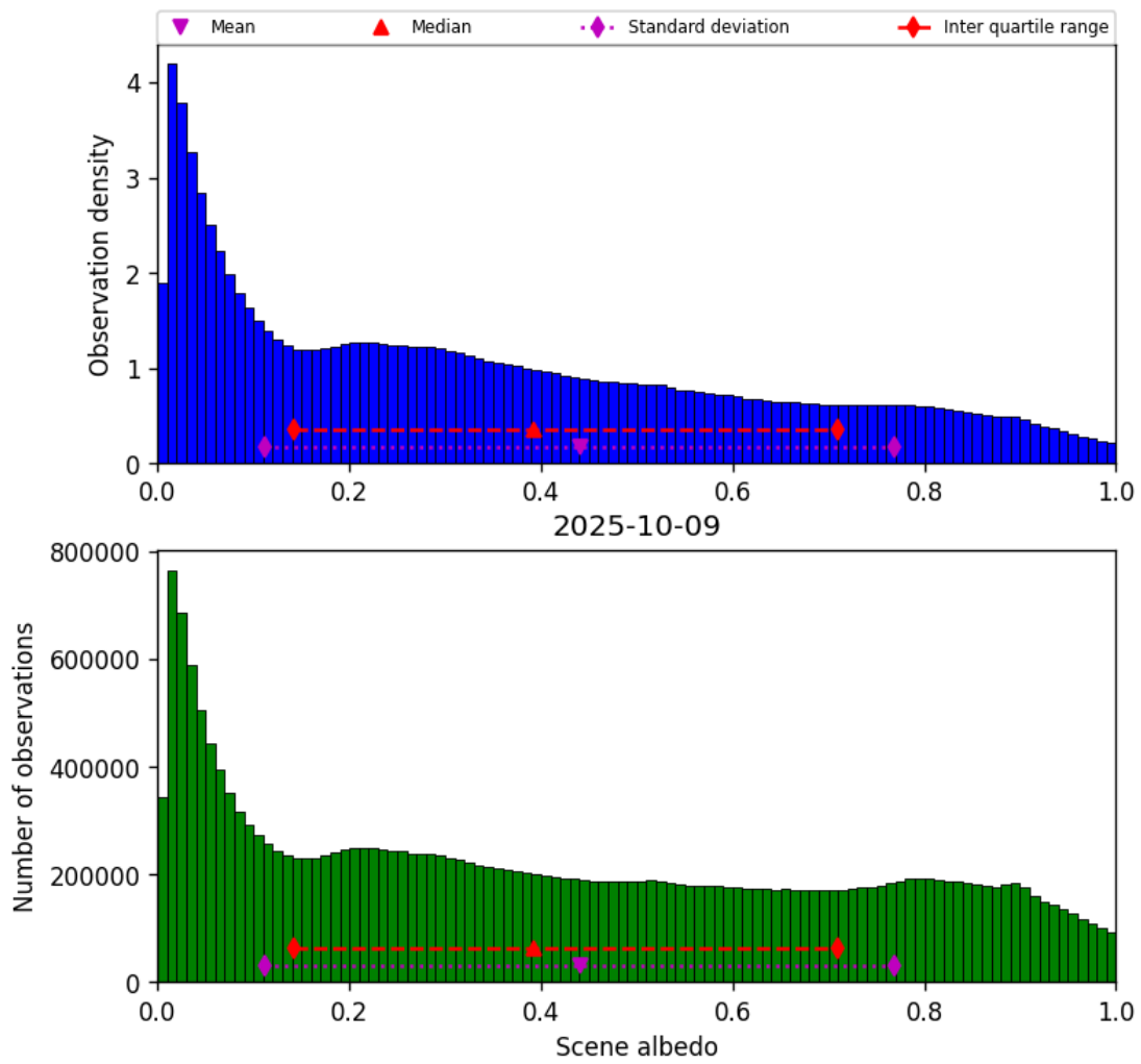
Figure 32: Histogram of “Scene albedo” for 2025-10-09 to 2025-10-09
