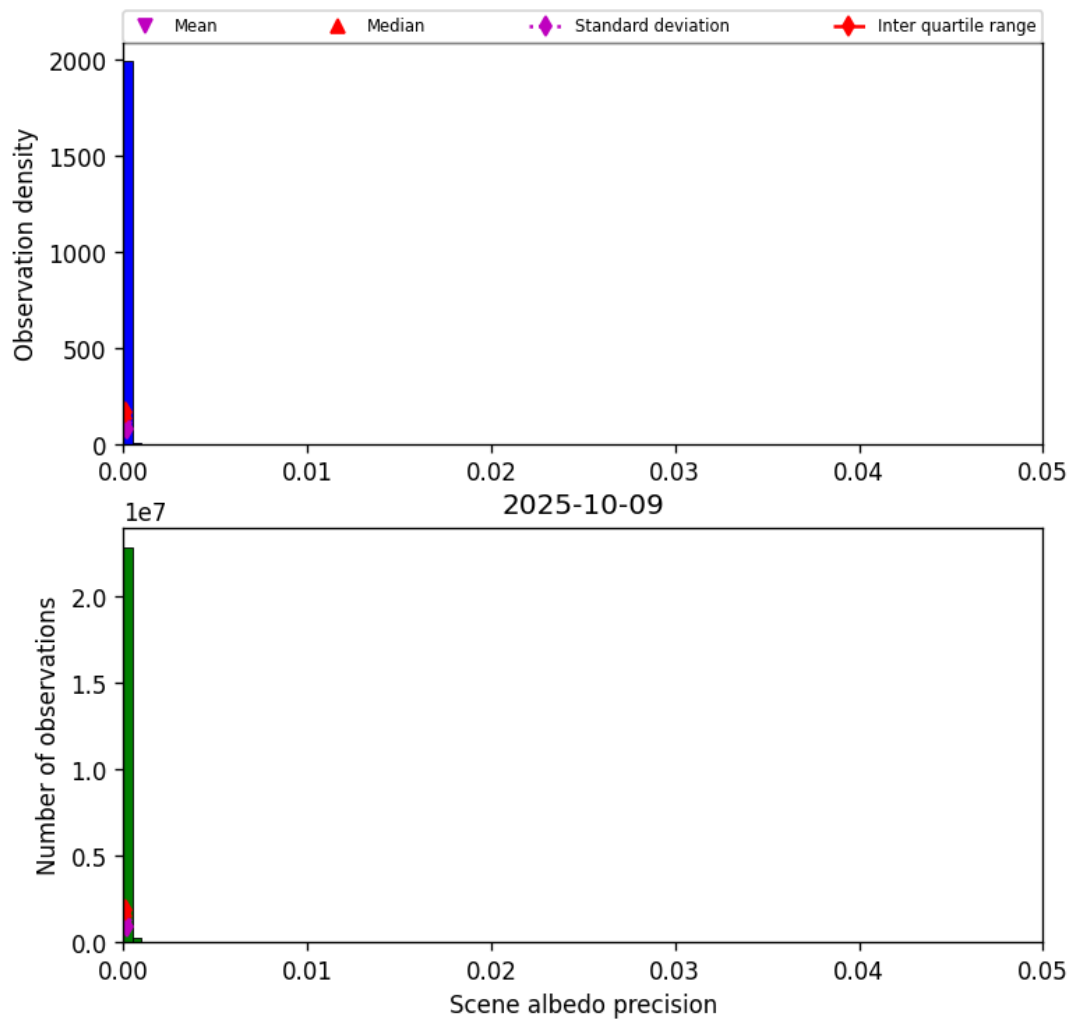
Figure 33: Histogram of “Scene albedo precision” for 2025-10-09 to 2025-10-09
