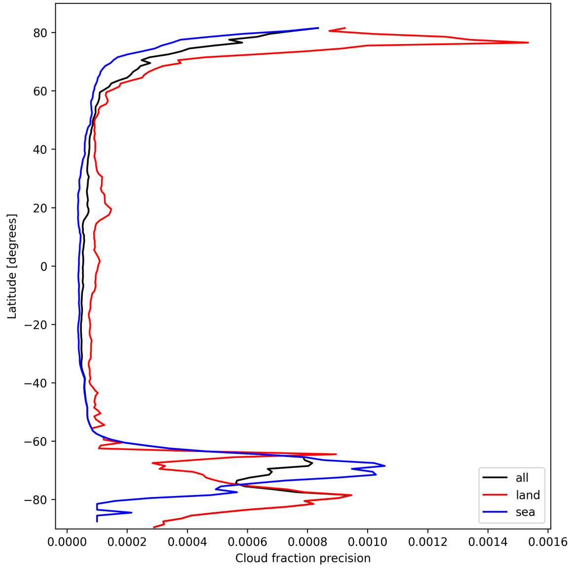
Figure 14: Zonal average of “Cloud fraction precision” for 2025-10-09 to 2025-10-09.
