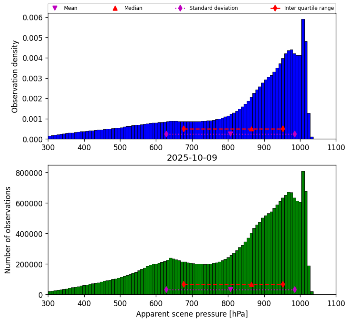
Figure 34: Histogram of “Apparent scene pressure” for 2025-10-09 to 2025-10-09
