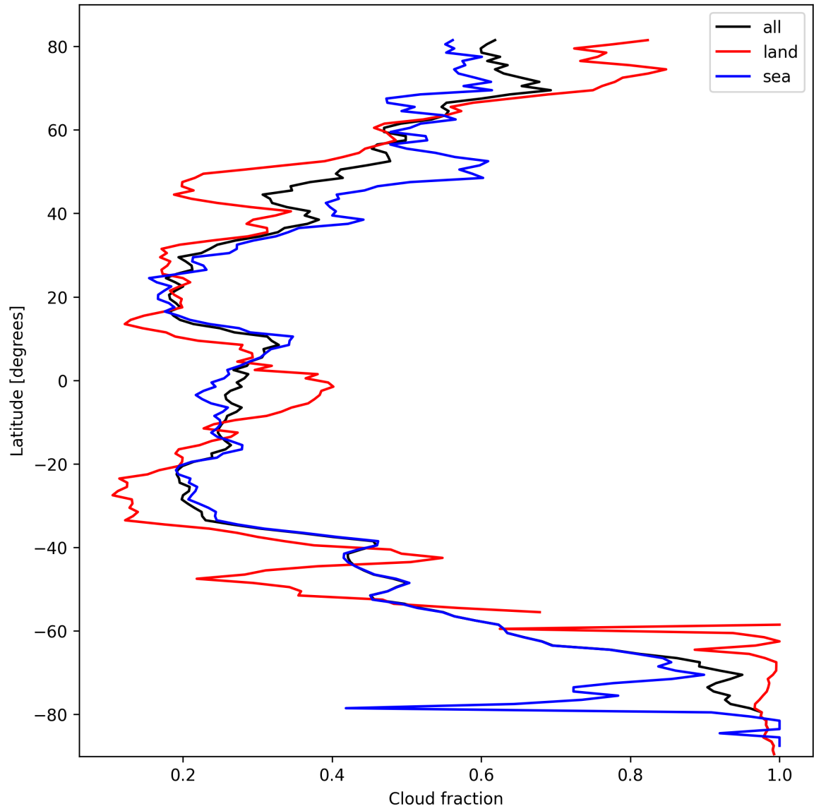
Figure 13: Zonal average of “Cloud fraction” for 2025-10-09 to 2025-10-09.
