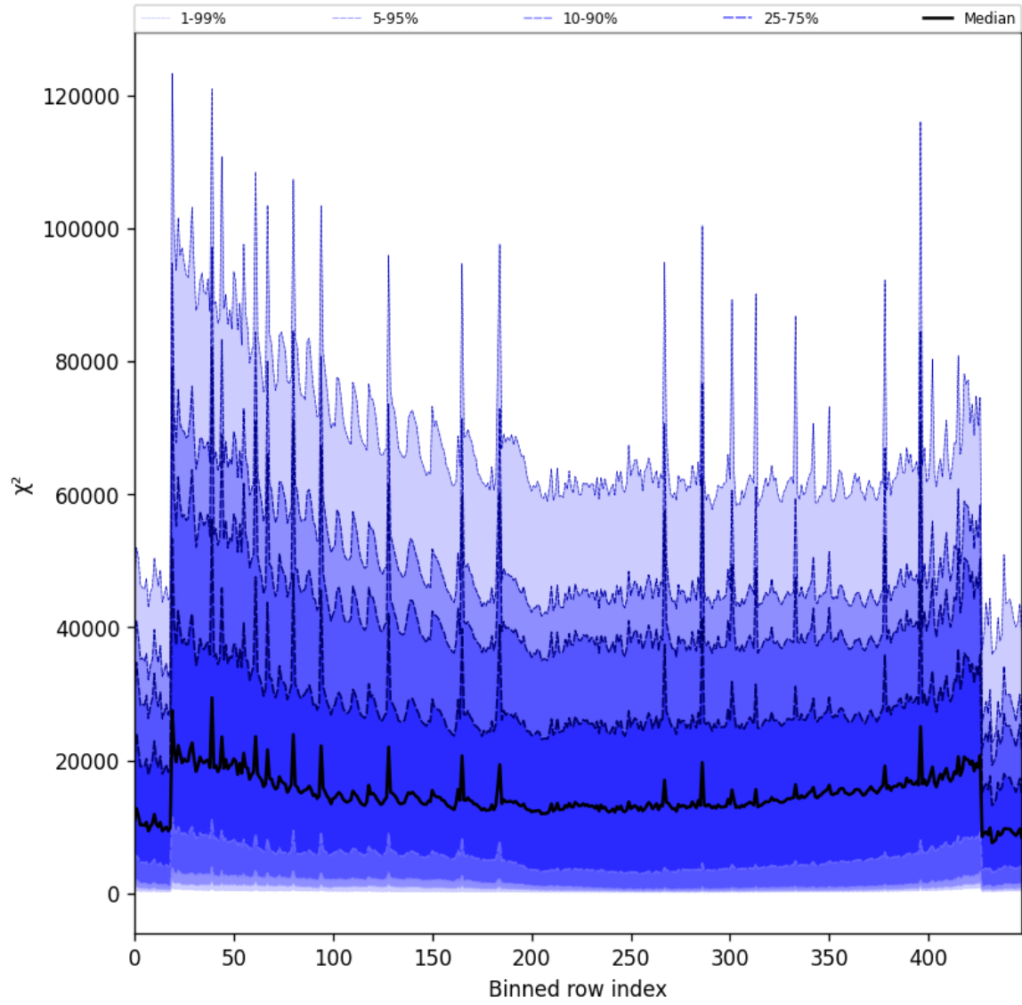
Figure 53: Along track statistics of “ \chi^2 ” for 2025-10-09 to 2025-10-09
