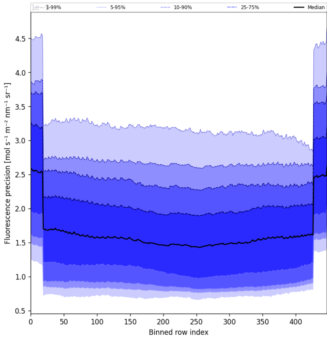
Figure 56: Along track statistics of “Fluorescence precision” for 2025-10-09 to 2025-10-09
