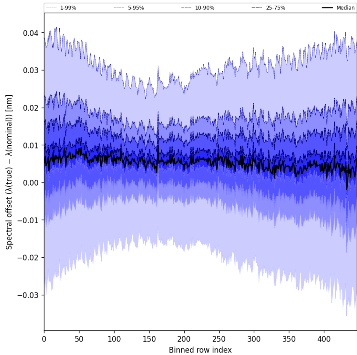
Figure 60: Along track statistics of “Spectral offset ( \lambda_{\text{true}} - \lambda_{\text{nominal}} )” for 2025-10-09 to 2025-10-09
