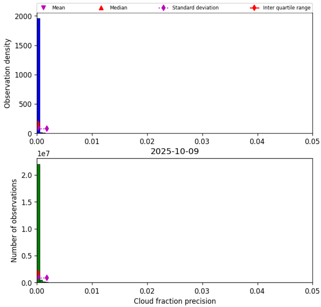
Figure 31: Histogram of “Cloud fraction precision” for 2025-10-09 to 2025-10-09
