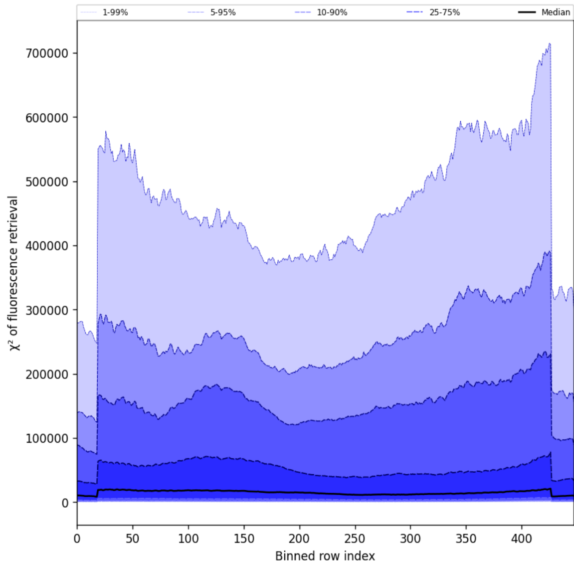
Figure 57: Along track statistics of “ \chi^2 of fluorescence retrieval” for 2025-10-09 to 2025-10-09
