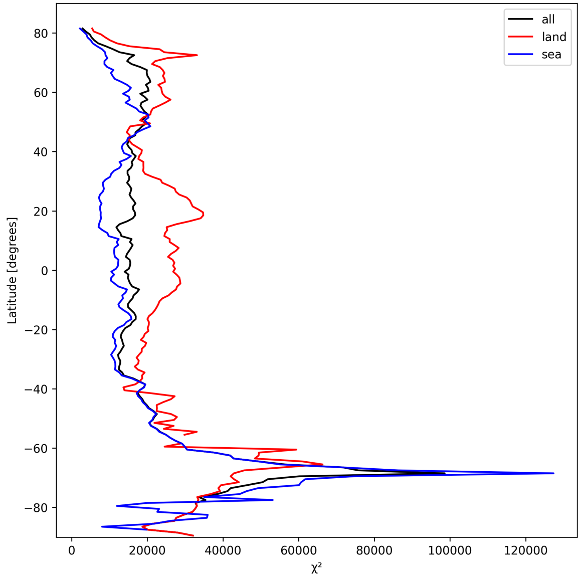
Figure 19: Zonal average of “ \chi^2 ” for 2025-10-09 to 2025-10-09.
