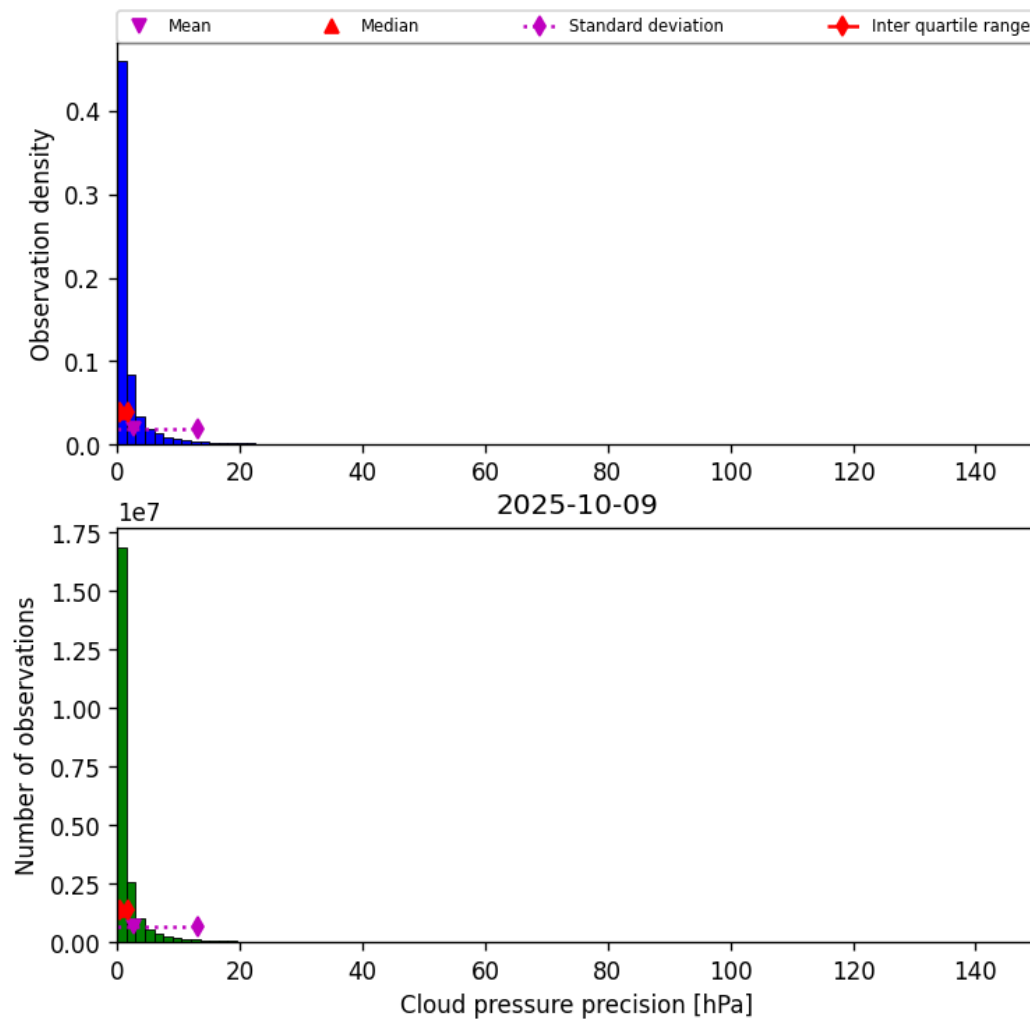
Figure 29: Histogram of “Cloud pressure precision” for 2025-10-09 to 2025-10-09
