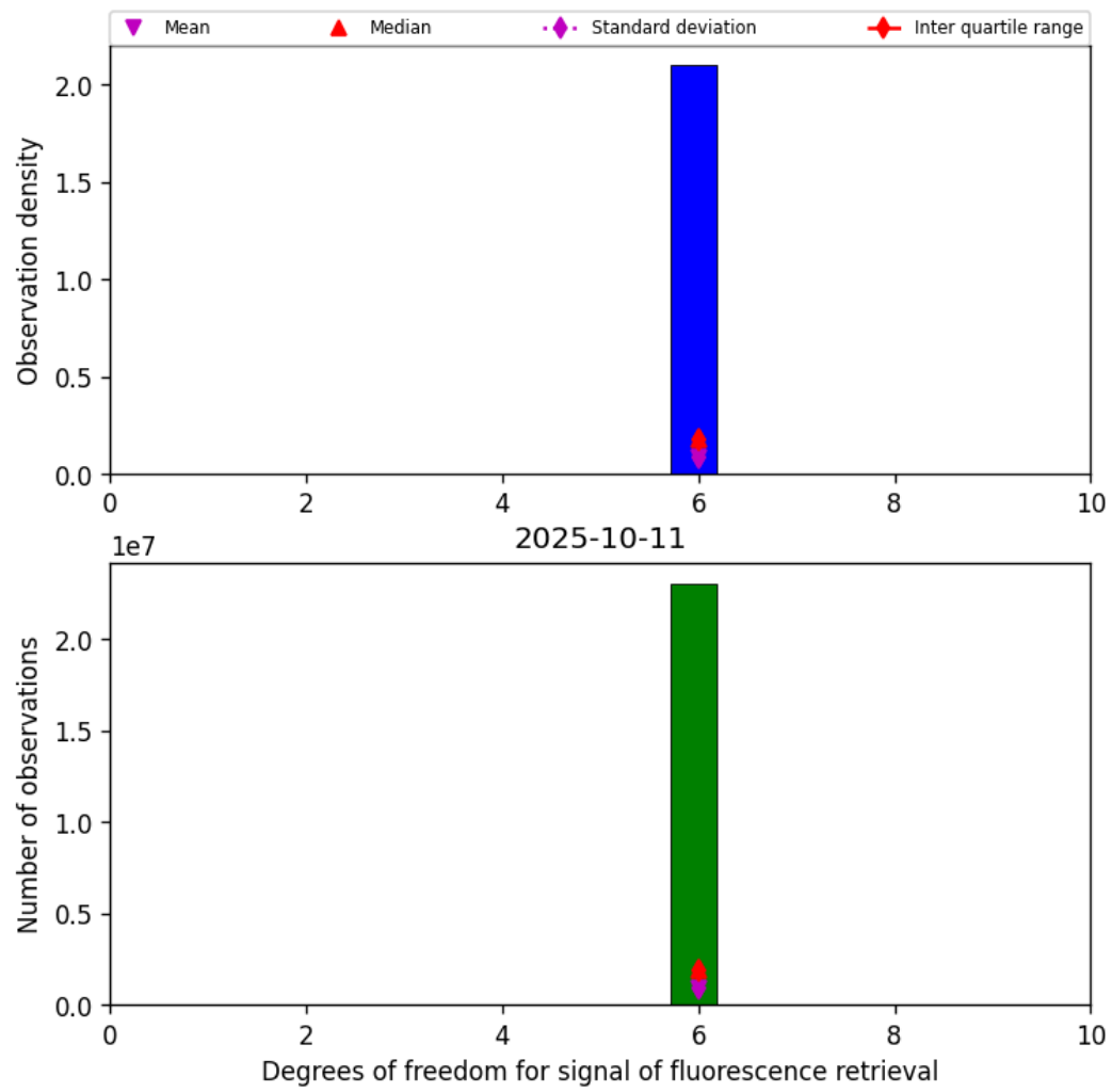
Figure 41: Histogram of “Degrees of freedom for signal of fluorescence retrieval” for 2025-10-11 to 2025-10-12
