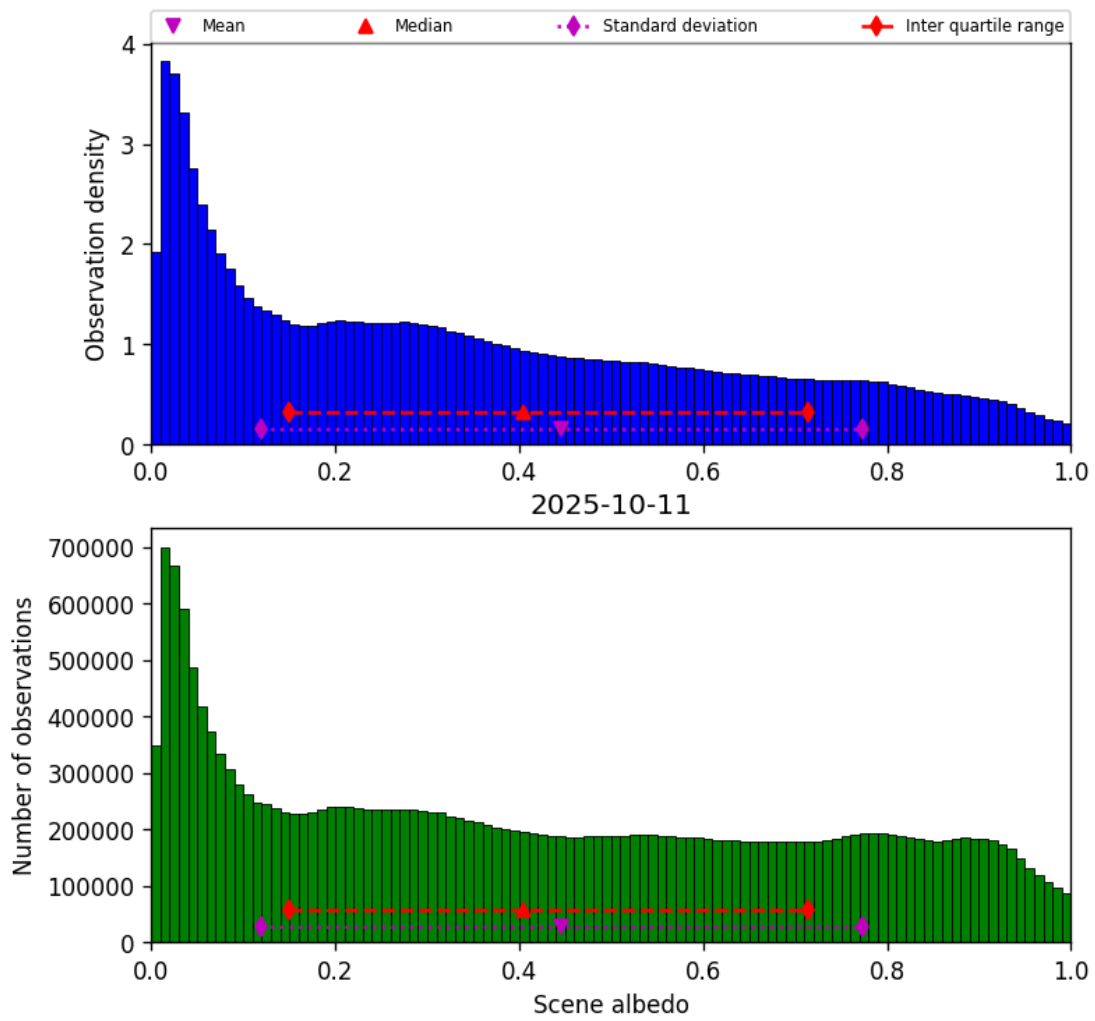
Figure 32: Histogram of “Scene albedo” for 2025-10-11 to 2025-10-12
