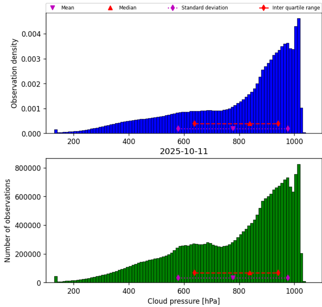
Figure 28: Histogram of “Cloud pressure” for 2025-10-11 to 2025-10-12
