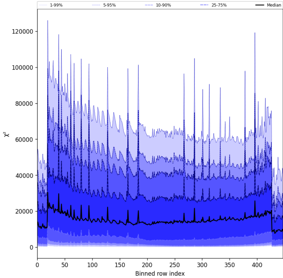
Figure 53: Along track statistics of “ \chi^2 ” for 2025-10-11 to 2025-10-12
