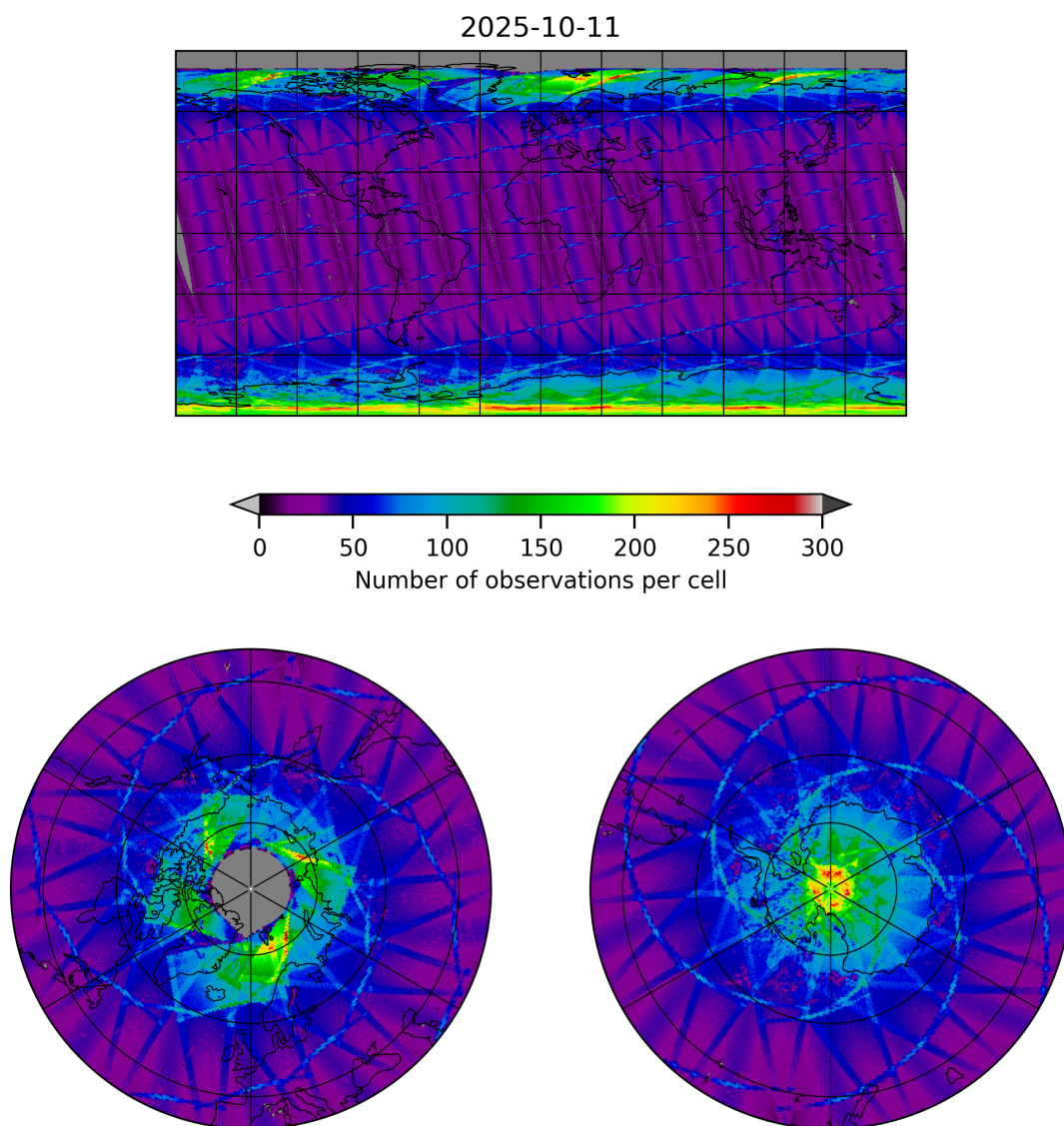
Figure 9: Map of the number of observations for 2025-10-11 to 2025-10-12
