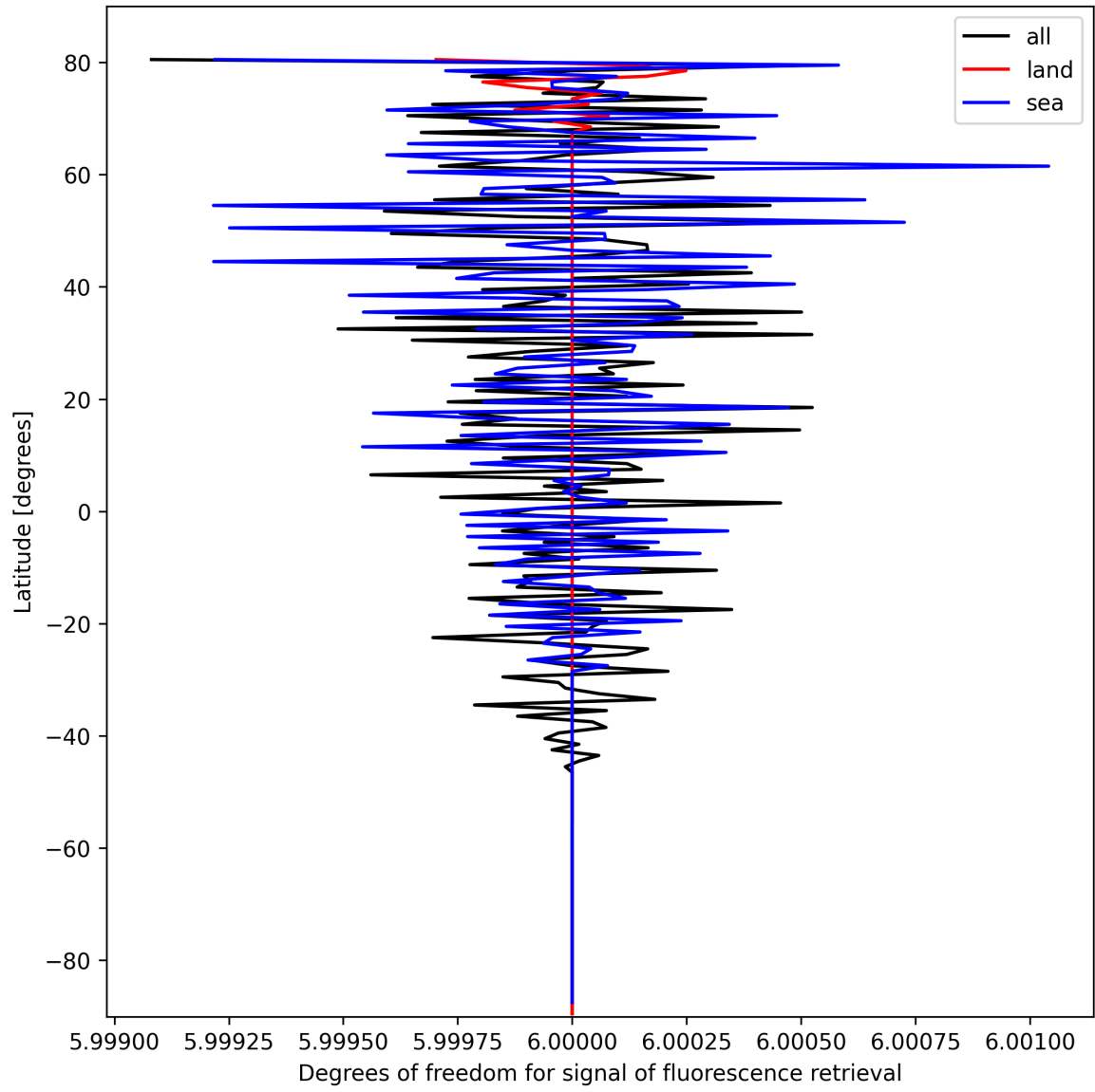
Figure 24: Zonal average of “Degrees of freedom for signal of fluorescence retrieval” for 2025-10-11 to 2025-10-12.
