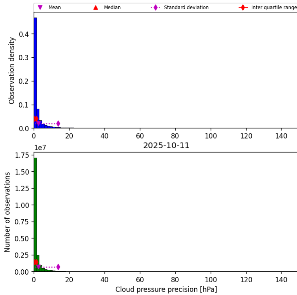
Figure 29: Histogram of “Cloud pressure precision” for 2025-10-11 to 2025-10-12
