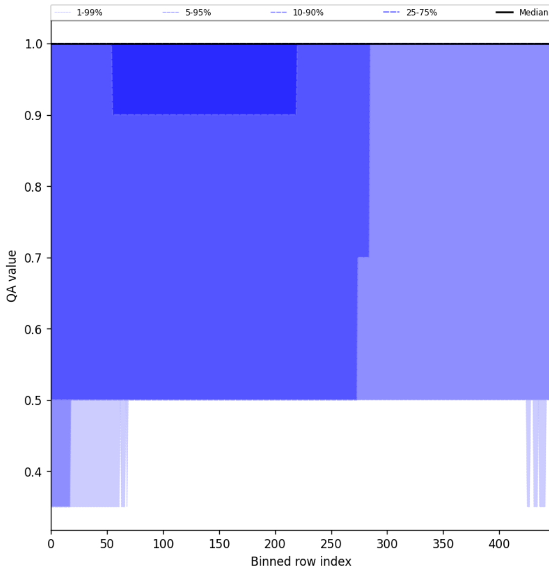
Figure 44: Along track statistics of “QA value” for 2025-10-11 to 2025-10-12
