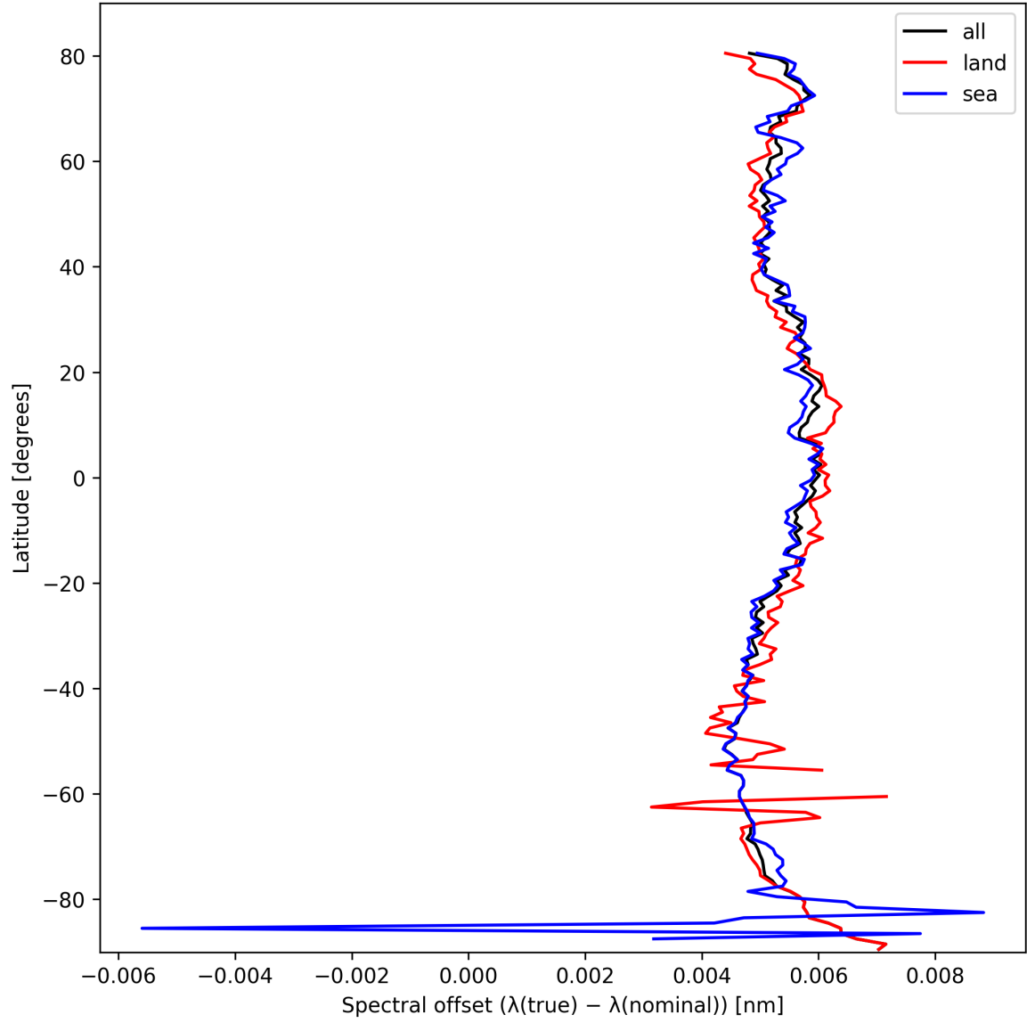
Figure 26: Zonal average of “Spectral offset ( \lambda_{\text{true}} - \lambda_{\text{nominal}} )” for 2025-10-11 to 2025-10-12.
