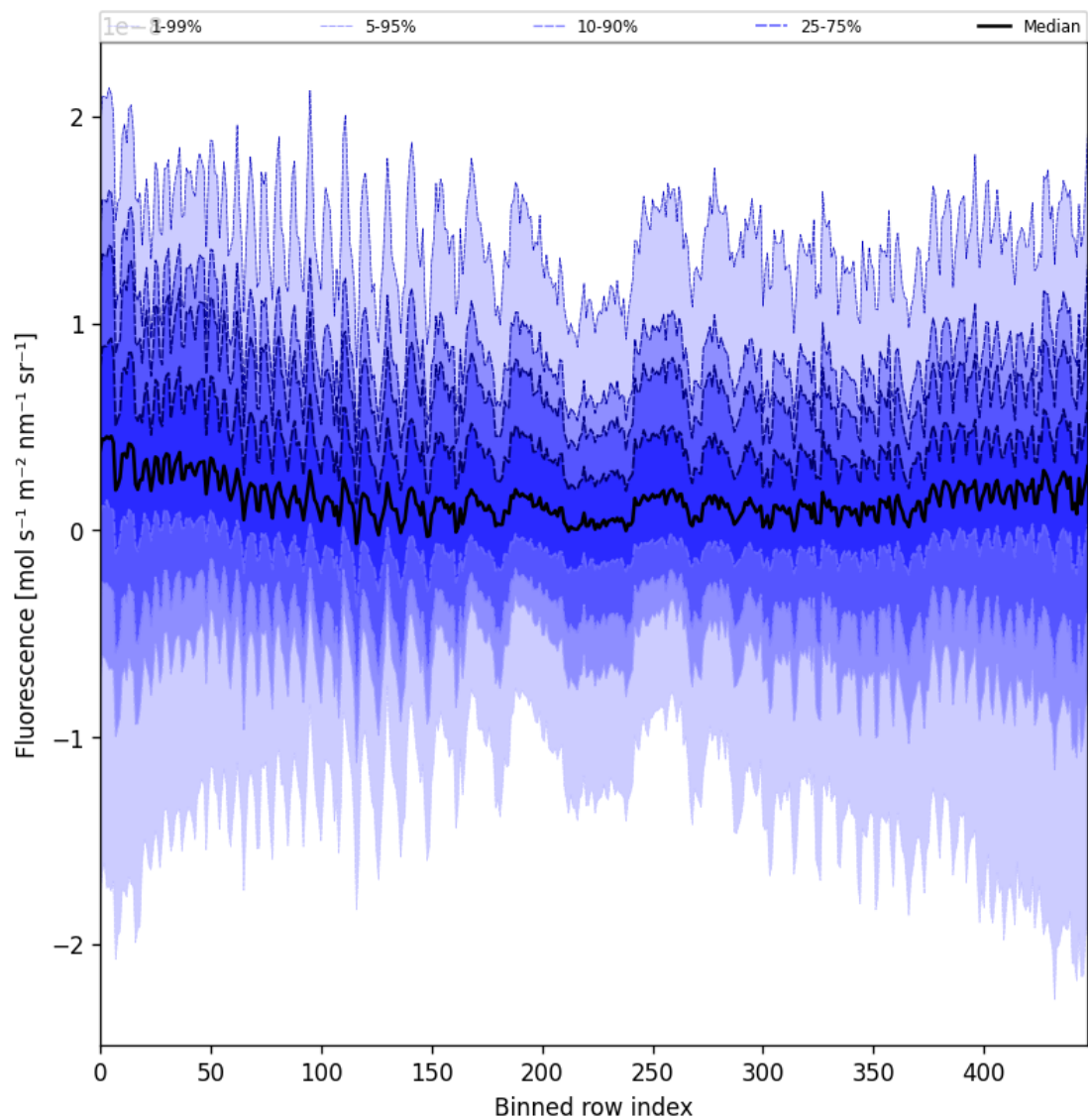
Figure 55: Along track statistics of “Fluorescence” for 2025-10-11 to 2025-10-12
