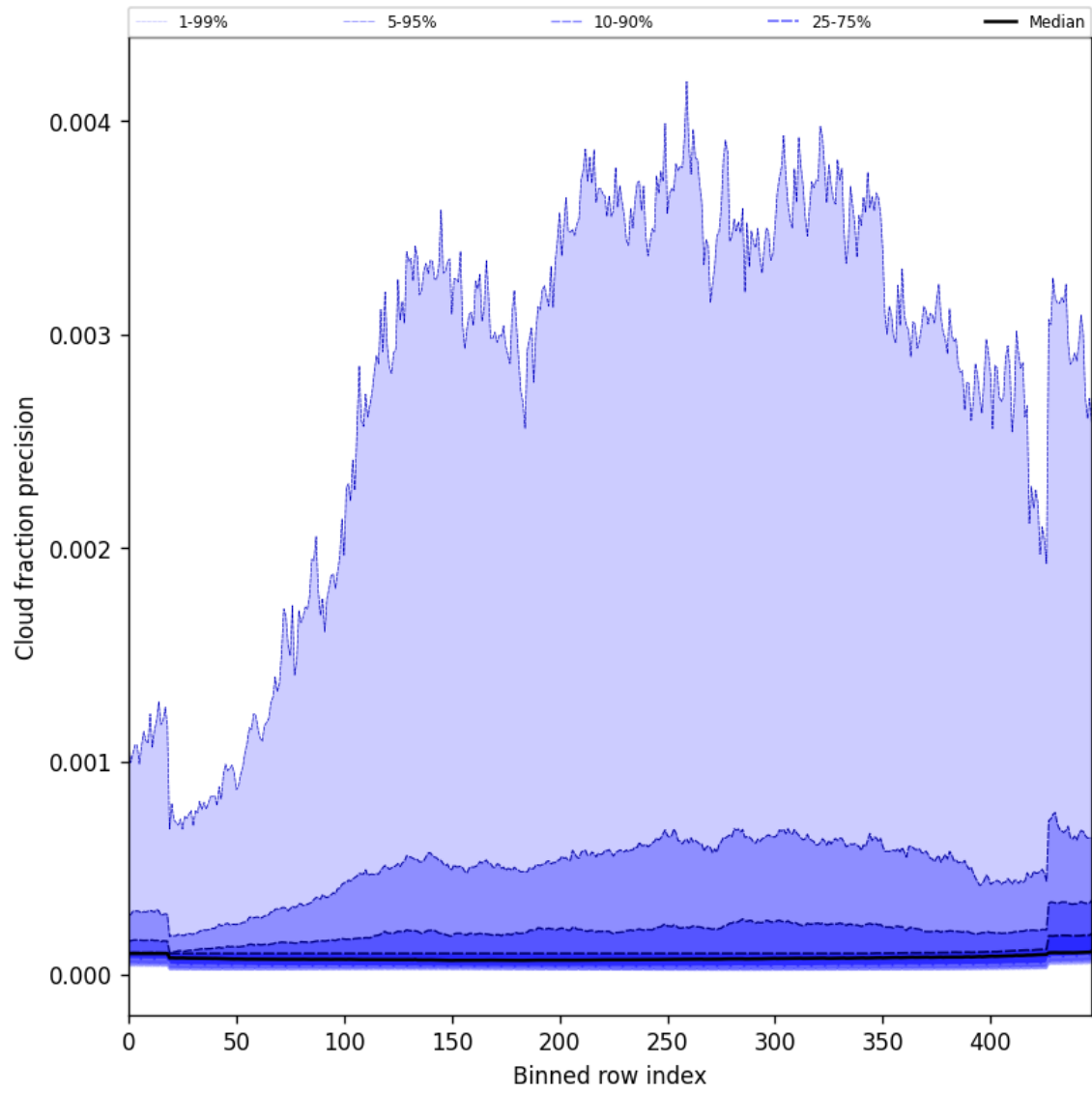
Figure 48: Along track statistics of “Cloud fraction precision” for 2025-10-11 to 2025-10-12
