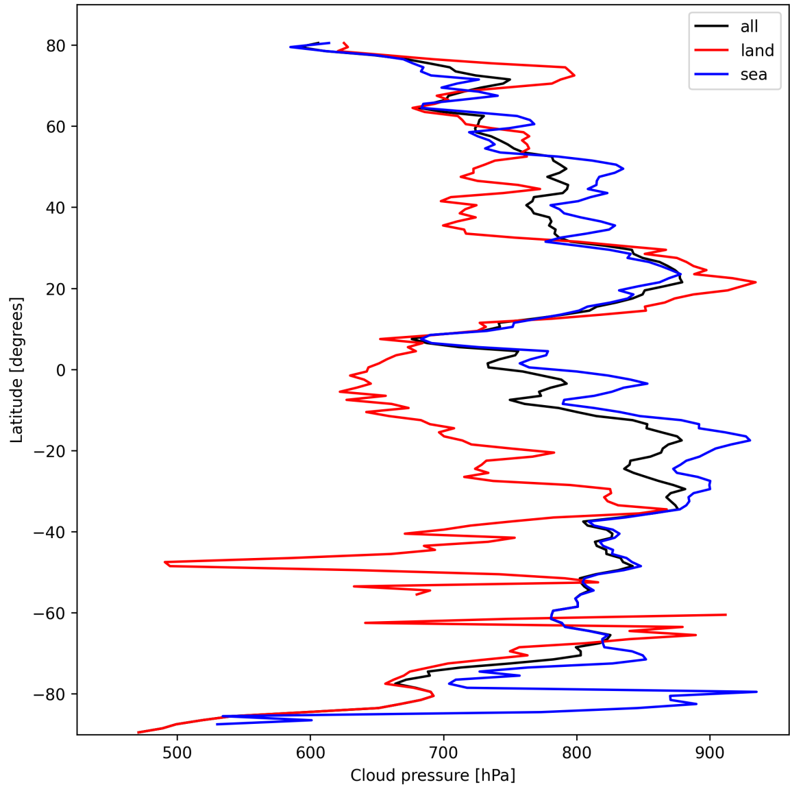
Figure 11: Zonal average of “Cloud pressure” for 2025-10-11 to 2025-10-12.
