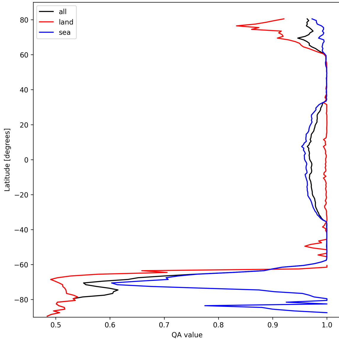
Figure 10: Zonal average of “QA value” for 2025-10-11 to 2025-10-12.
