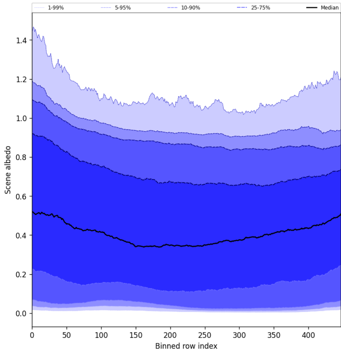
Figure 49: Along track statistics of “Scene albedo” for 2025-10-11 to 2025-10-12
