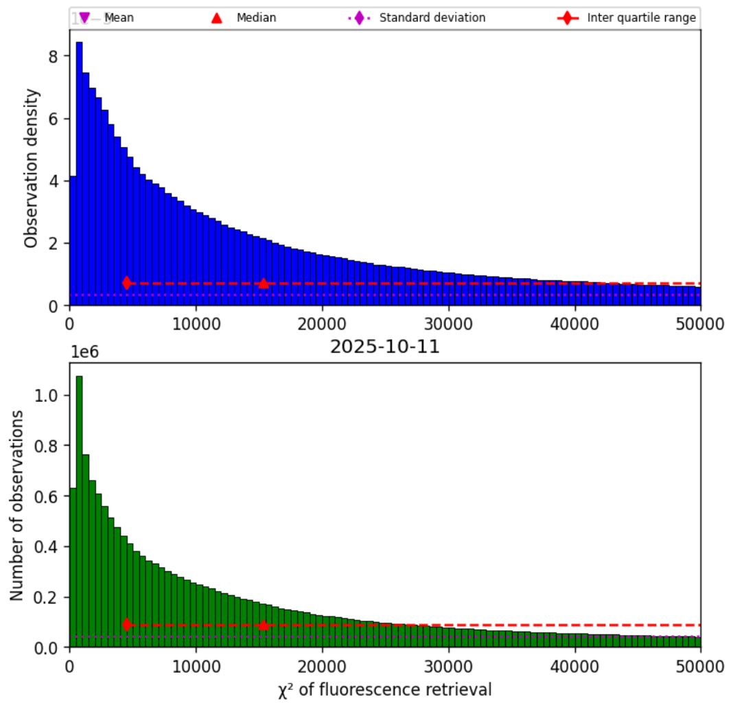
Figure 40: Histogram of “ \chi^2 of fluorescence retrieval” for 2025-10-11 to 2025-10-12
