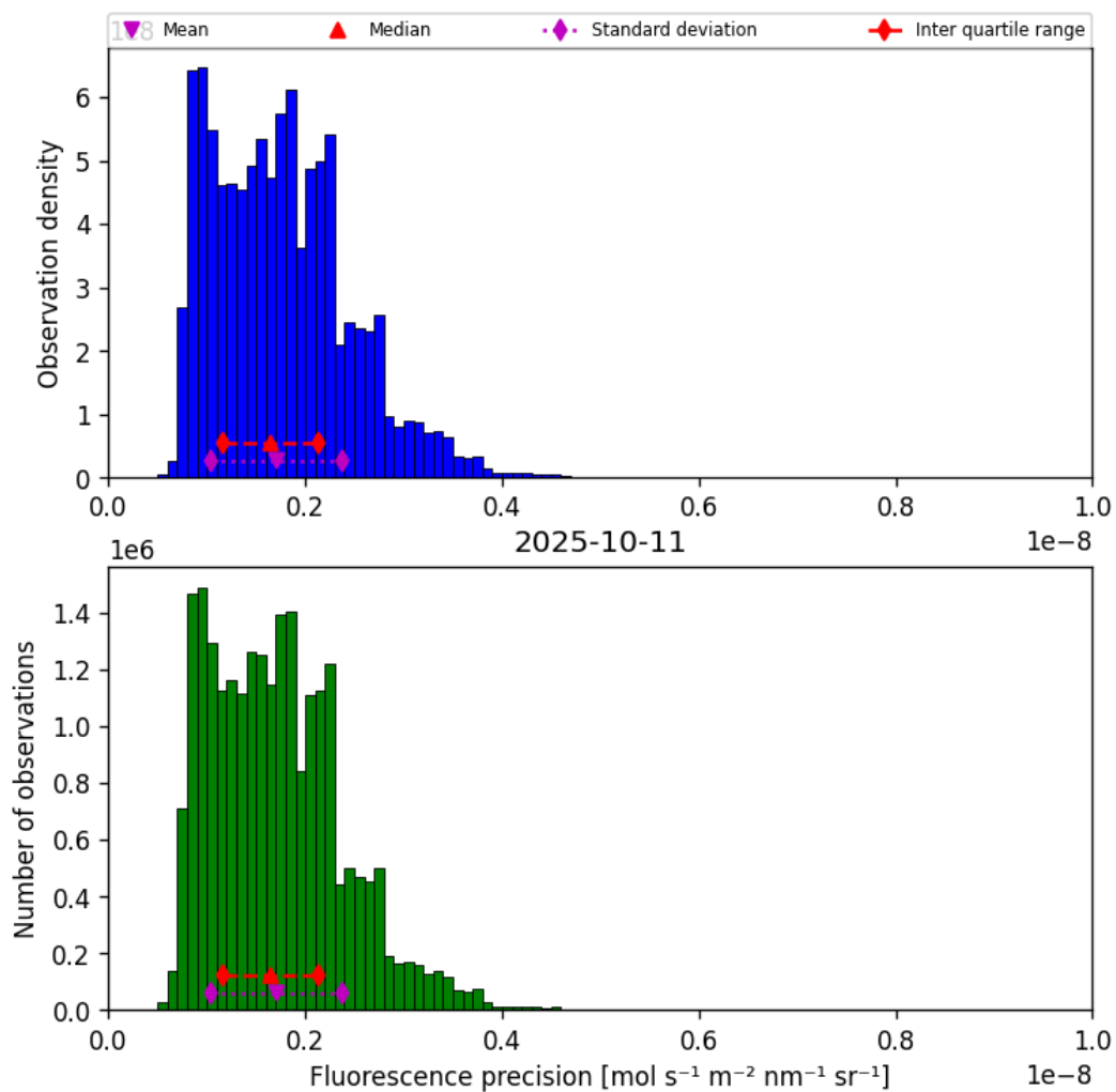
Figure 39: Histogram of “Fluorescence precision” for 2025-10-11 to 2025-10-12
