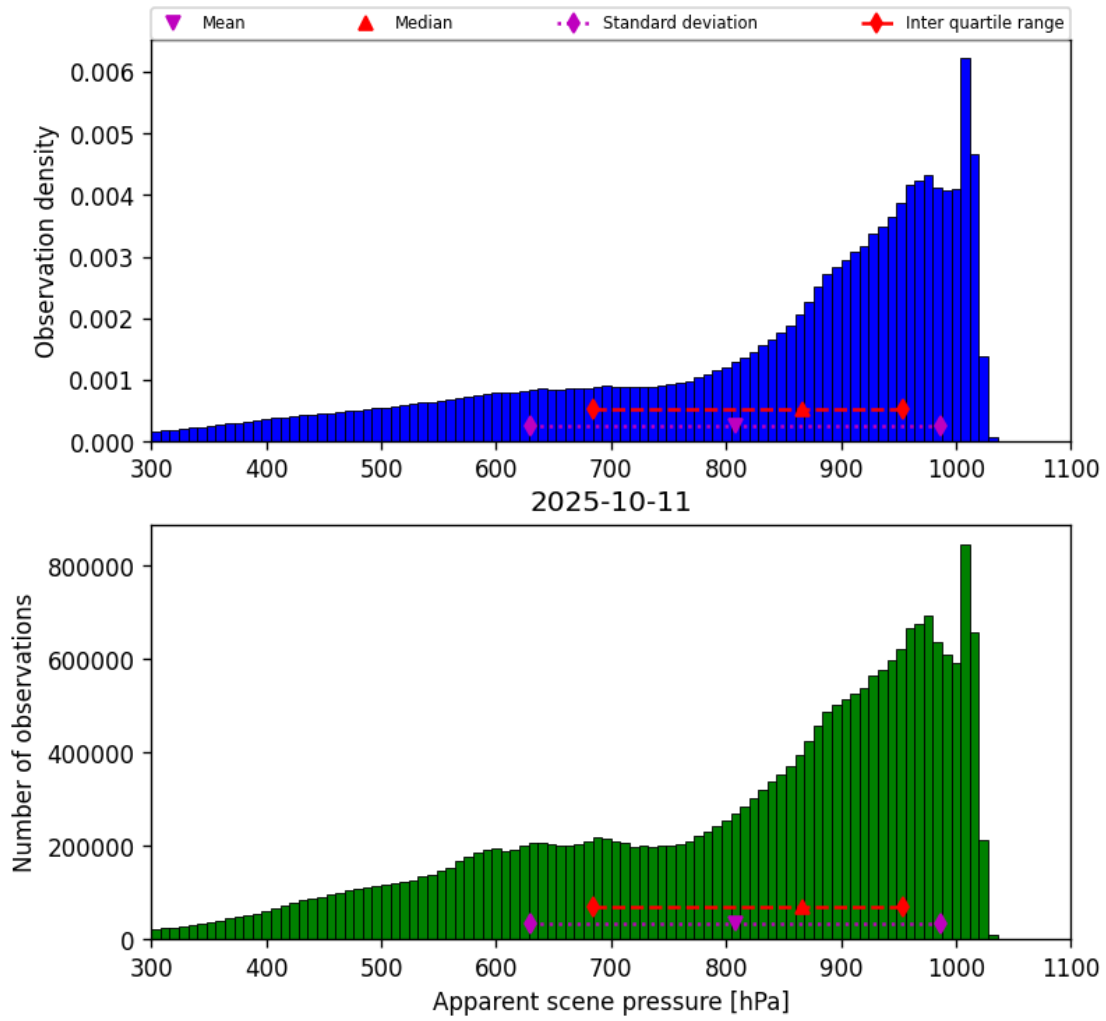
Figure 34: Histogram of “Apparent scene pressure” for 2025-10-11 to 2025-10-12
