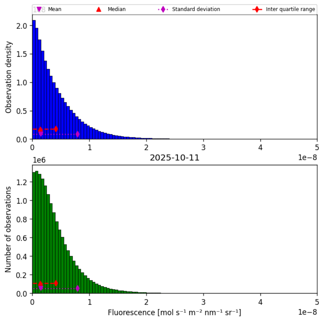
Figure 38: Histogram of “Fluorescence” for 2025-10-11 to 2025-10-12
