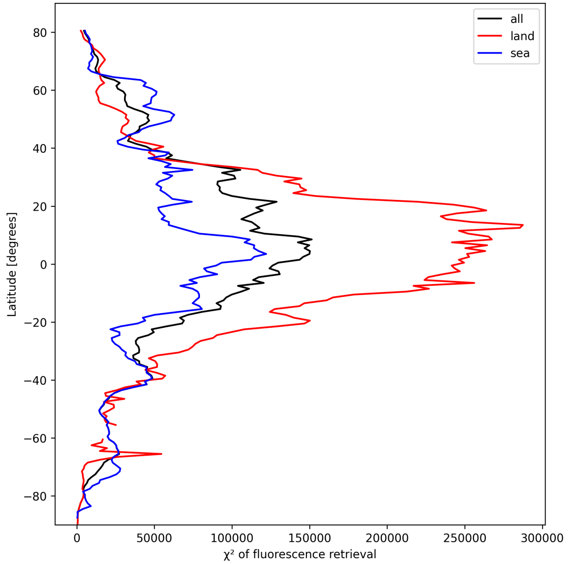
Figure 23: Zonal average of “ \chi^2 of fluorescence retrieval” for 2025-10-11 to 2025-10-12.
