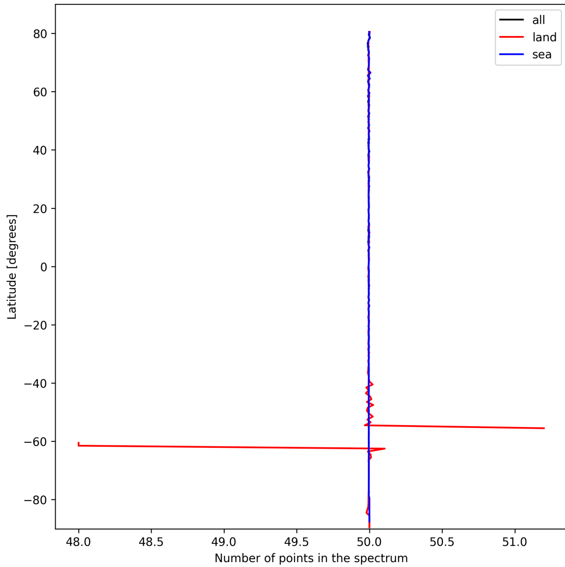
Figure 25: Zonal average of “Number of points in the spectrum” for 2025-10-11 to 2025-10-12.
