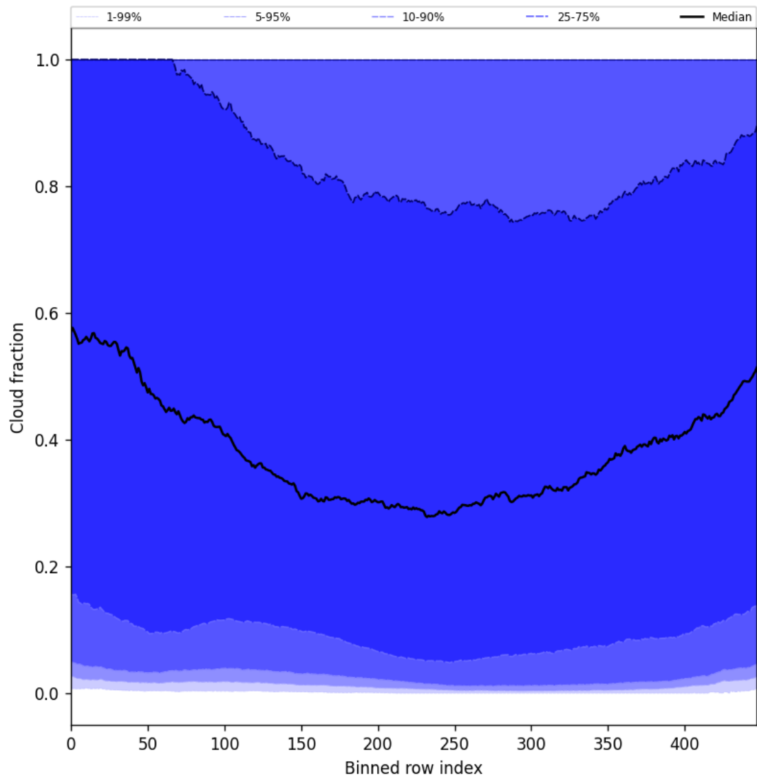
Figure 47: Along track statistics of “Cloud fraction” for 2025-10-11 to 2025-10-12
