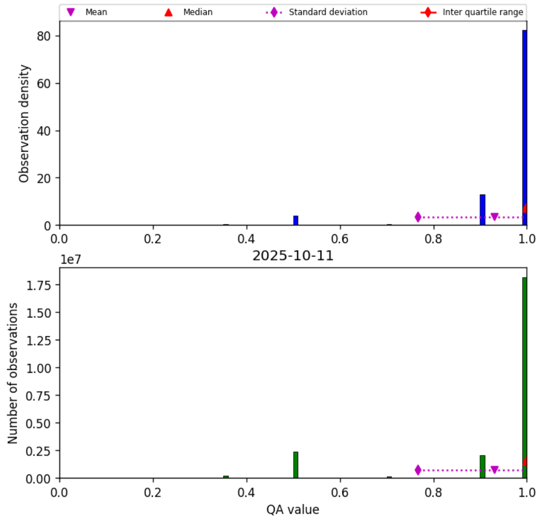
Figure 27: Histogram of “QA value” for 2025-10-11 to 2025-10-12
