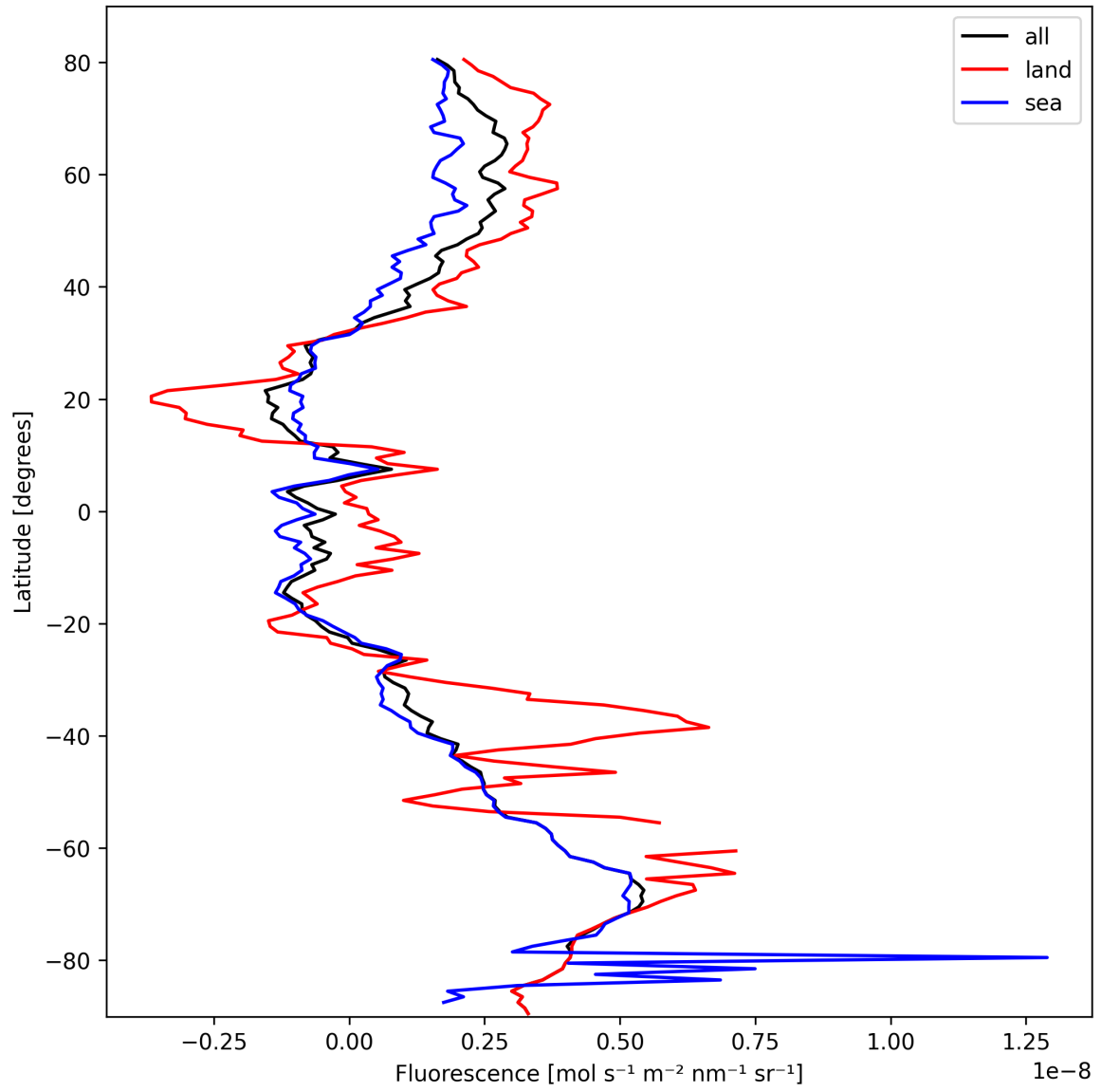
Figure 21: Zonal average of “Fluorescence” for 2025-10-11 to 2025-10-12.
