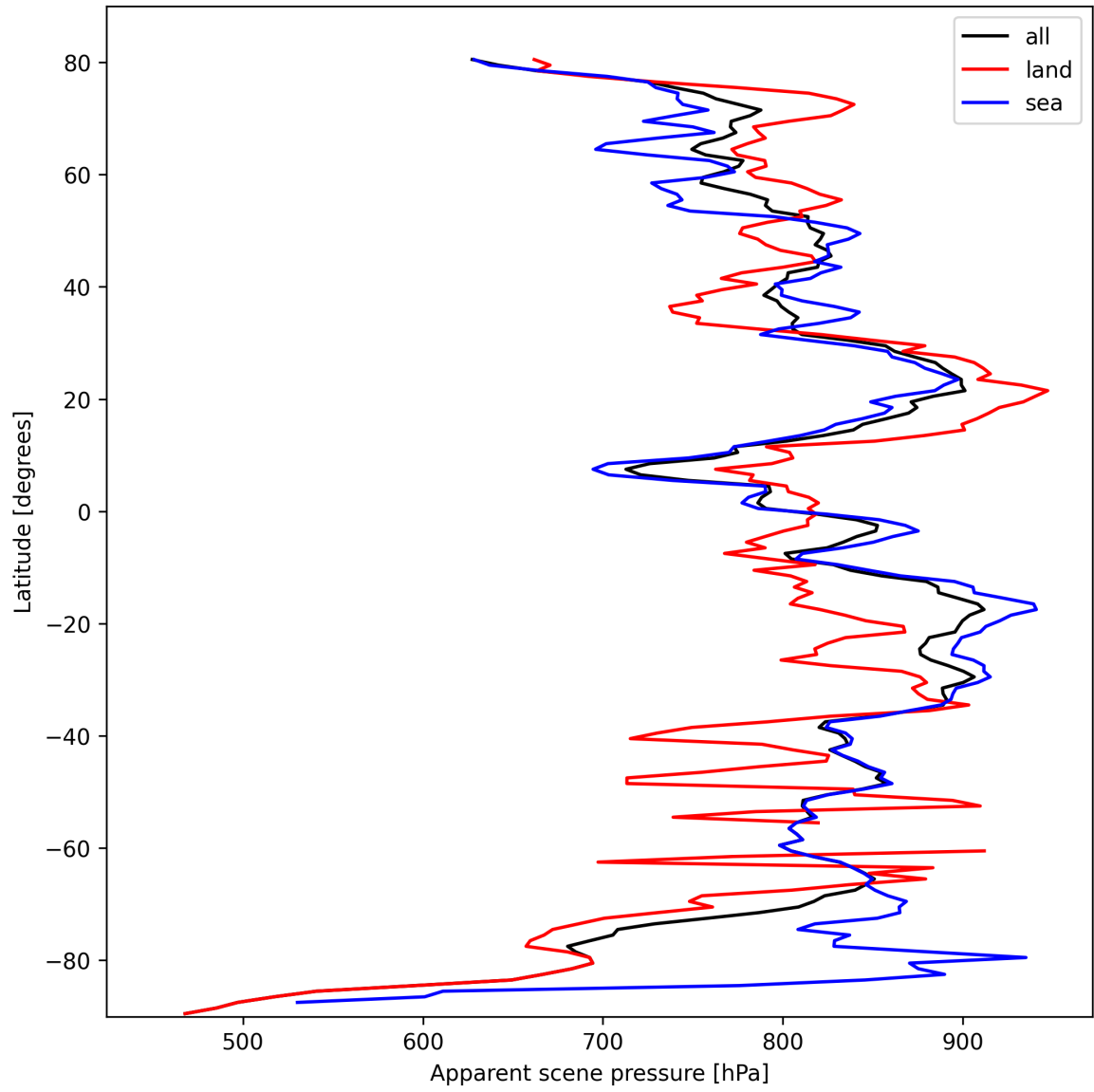
Figure 17: Zonal average of “Apparent scene pressure” for 2025-10-11 to 2025-10-12.
