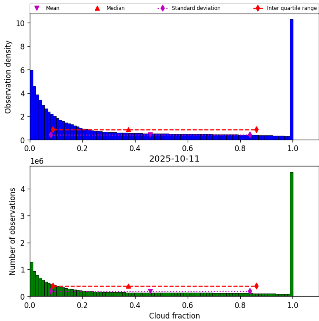
Figure 30: Histogram of “Cloud fraction” for 2025-10-11 to 2025-10-12
