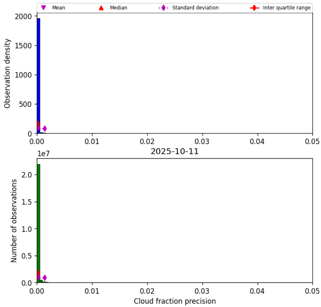
Figure 31: Histogram of “Cloud fraction precision” for 2025-10-11 to 2025-10-12
