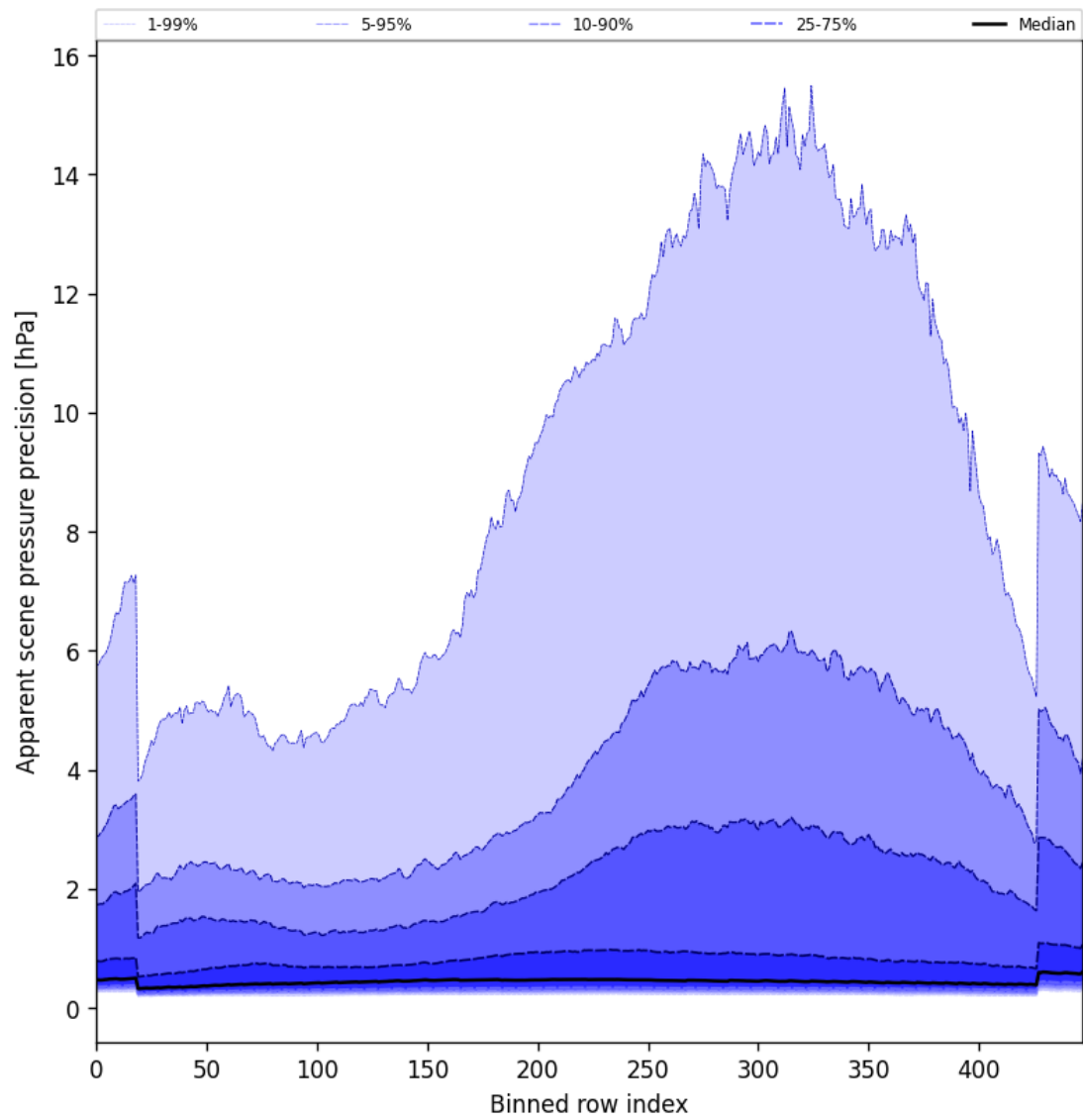
Figure 52: Along track statistics of “Apparent scene pressure precision” for 2025-10-11 to 2025-10-12
