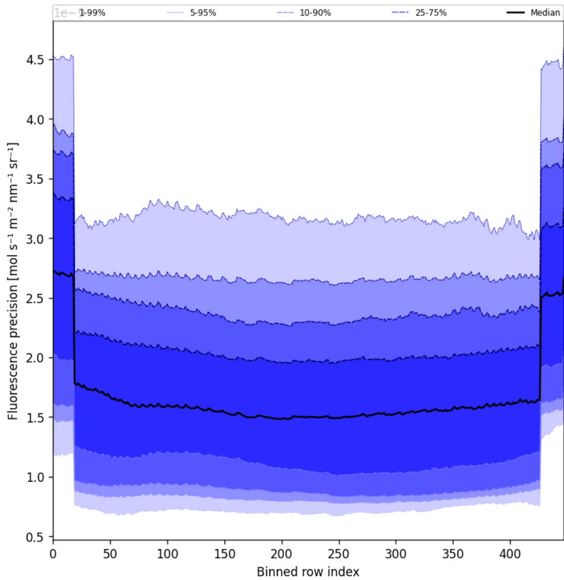
Figure 56: Along track statistics of “Fluorescence precision” for 2025-10-11 to 2025-10-12
