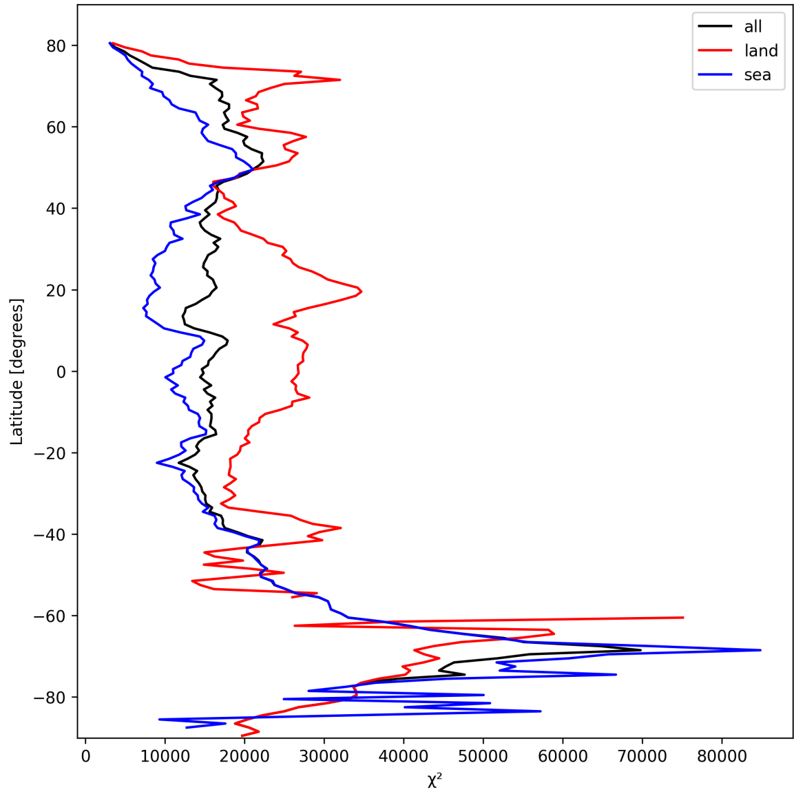
Figure 19: Zonal average of “ \chi^2 ” for 2025-10-11 to 2025-10-12.
