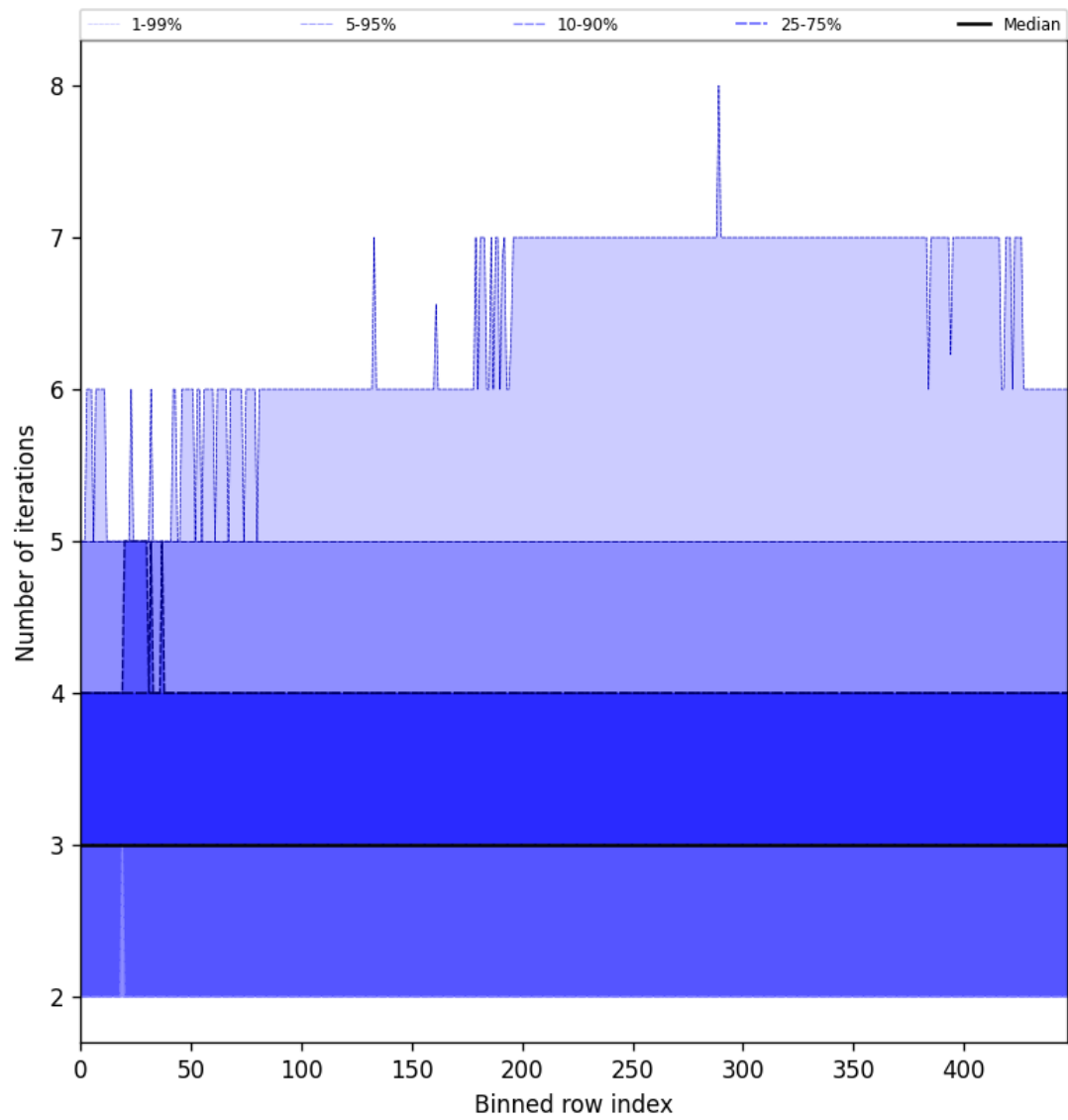
Figure 54: Along track statistics of “Number of iterations” for 2025-10-11 to 2025-10-12
