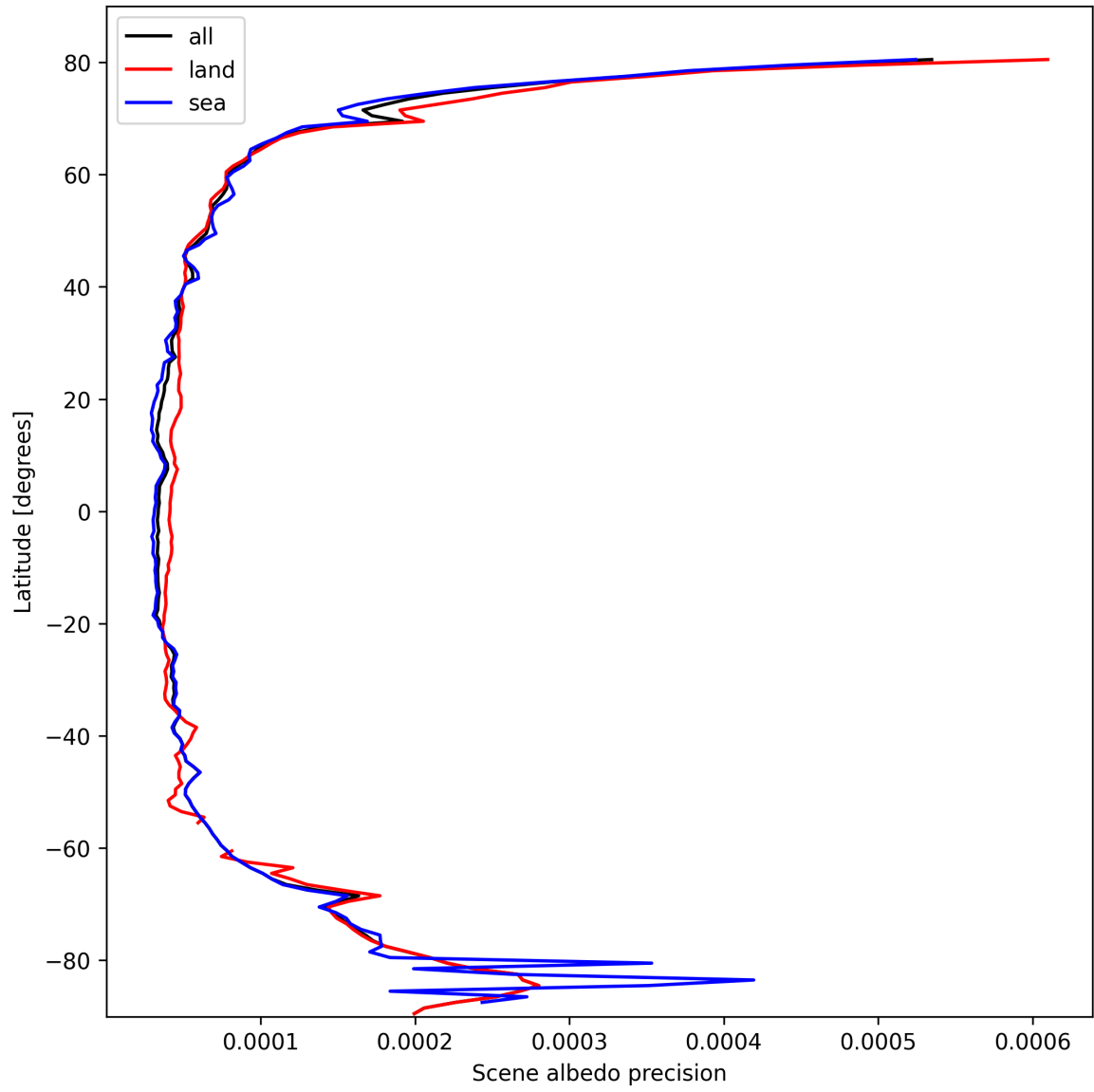
Figure 16: Zonal average of “Scene albedo precision” for 2025-10-11 to 2025-10-12.
