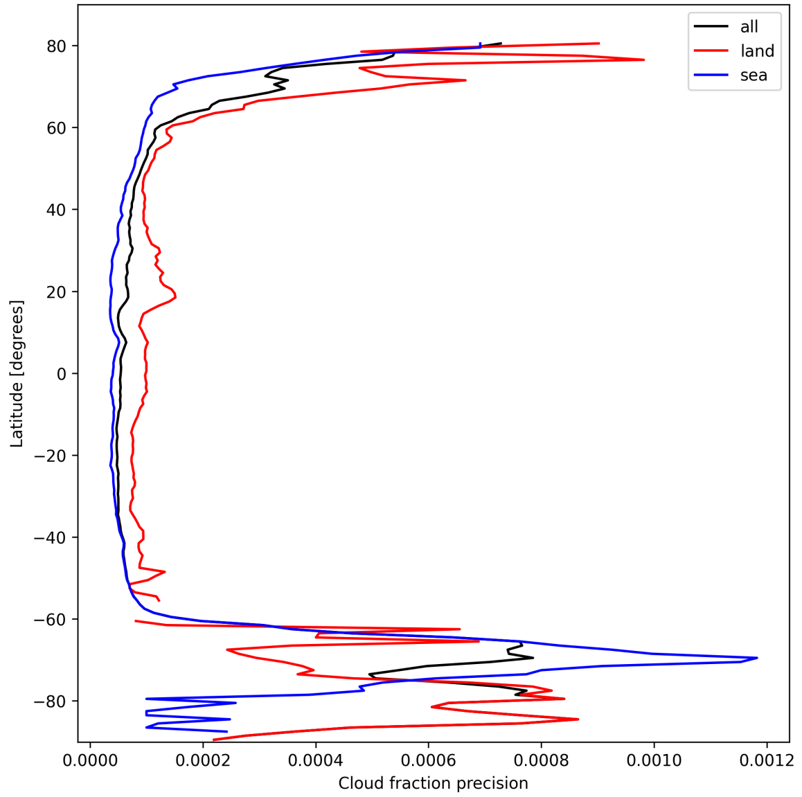
Figure 14: Zonal average of “Cloud fraction precision” for 2025-10-11 to 2025-10-12.
