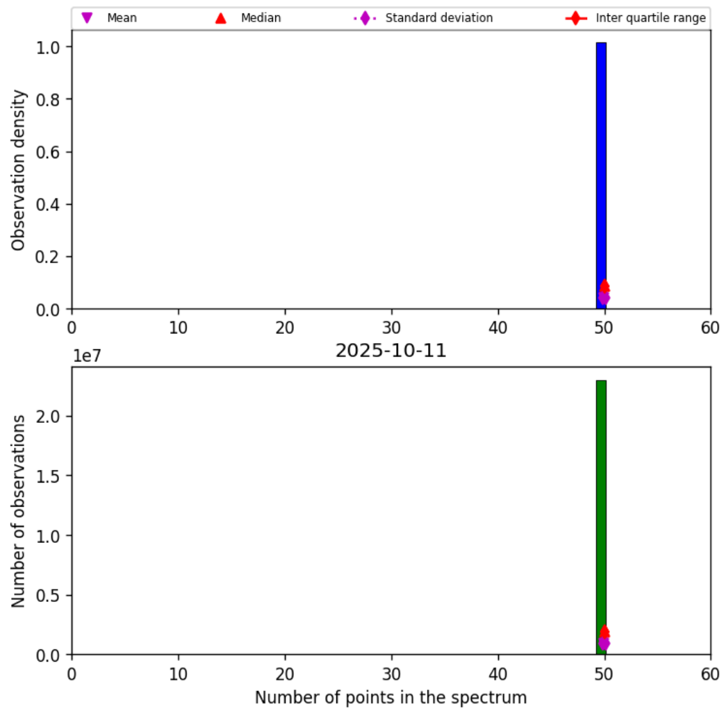
Figure 42: Histogram of “Number of points in the spectrum” for 2025-10-11 to 2025-10-12
