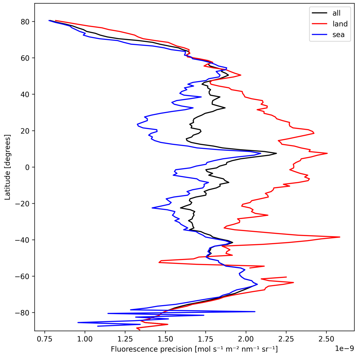
Figure 22: Zonal average of “Fluorescence precision” for 2025-10-11 to 2025-10-12.
