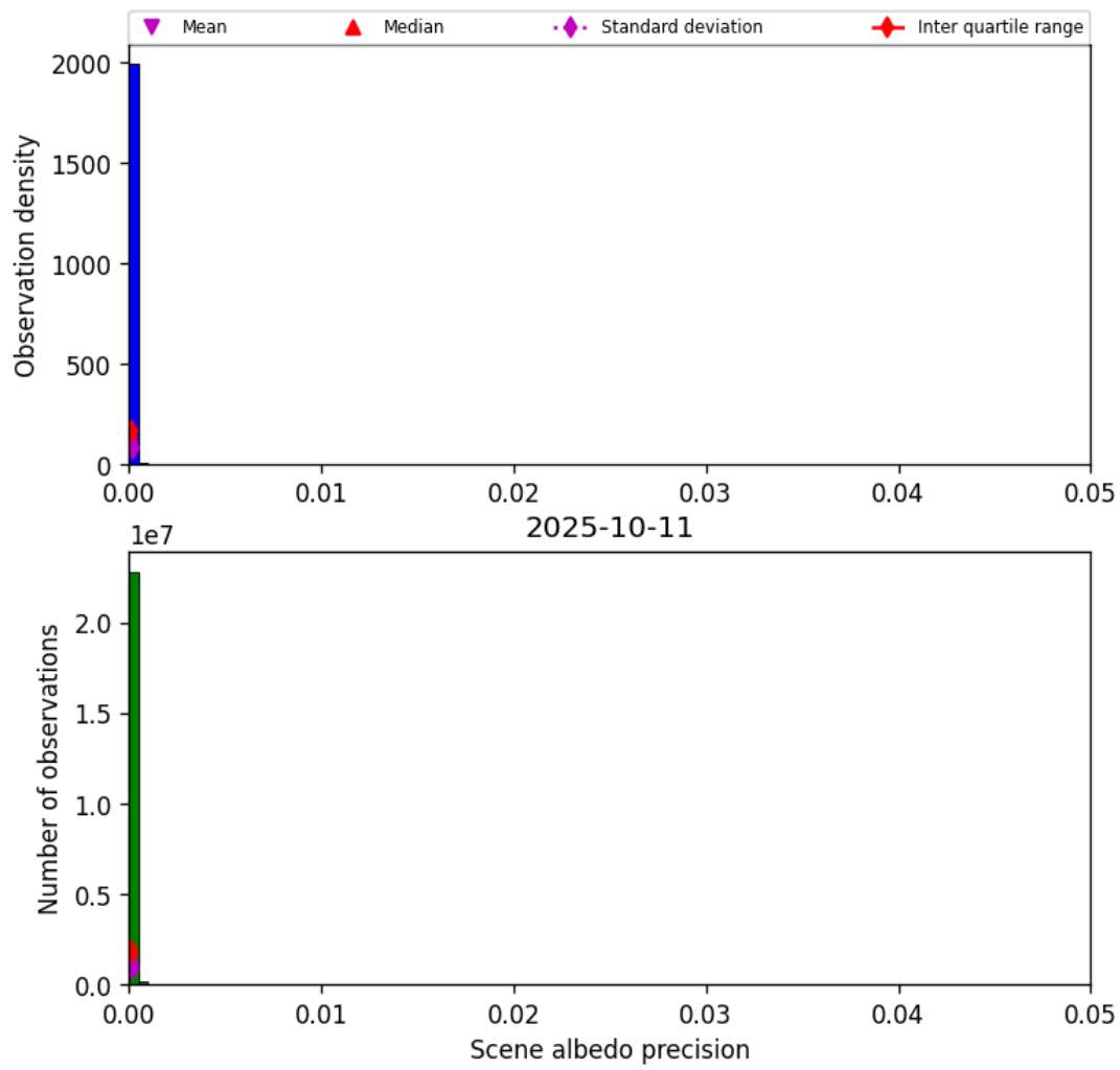
Figure 33: Histogram of “Scene albedo precision” for 2025-10-11 to 2025-10-12
