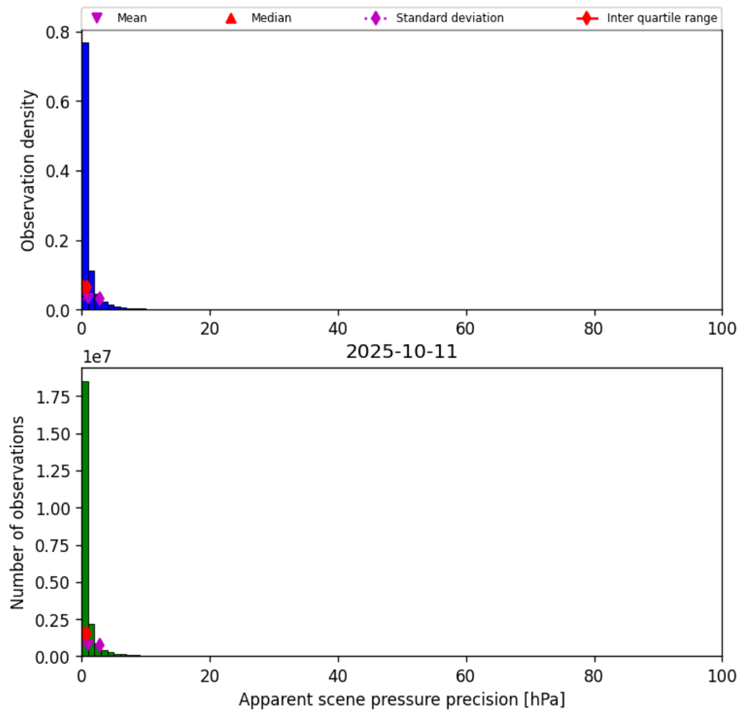
Figure 35: Histogram of “Apparent scene pressure precision” for 2025-10-11 to 2025-10-12
