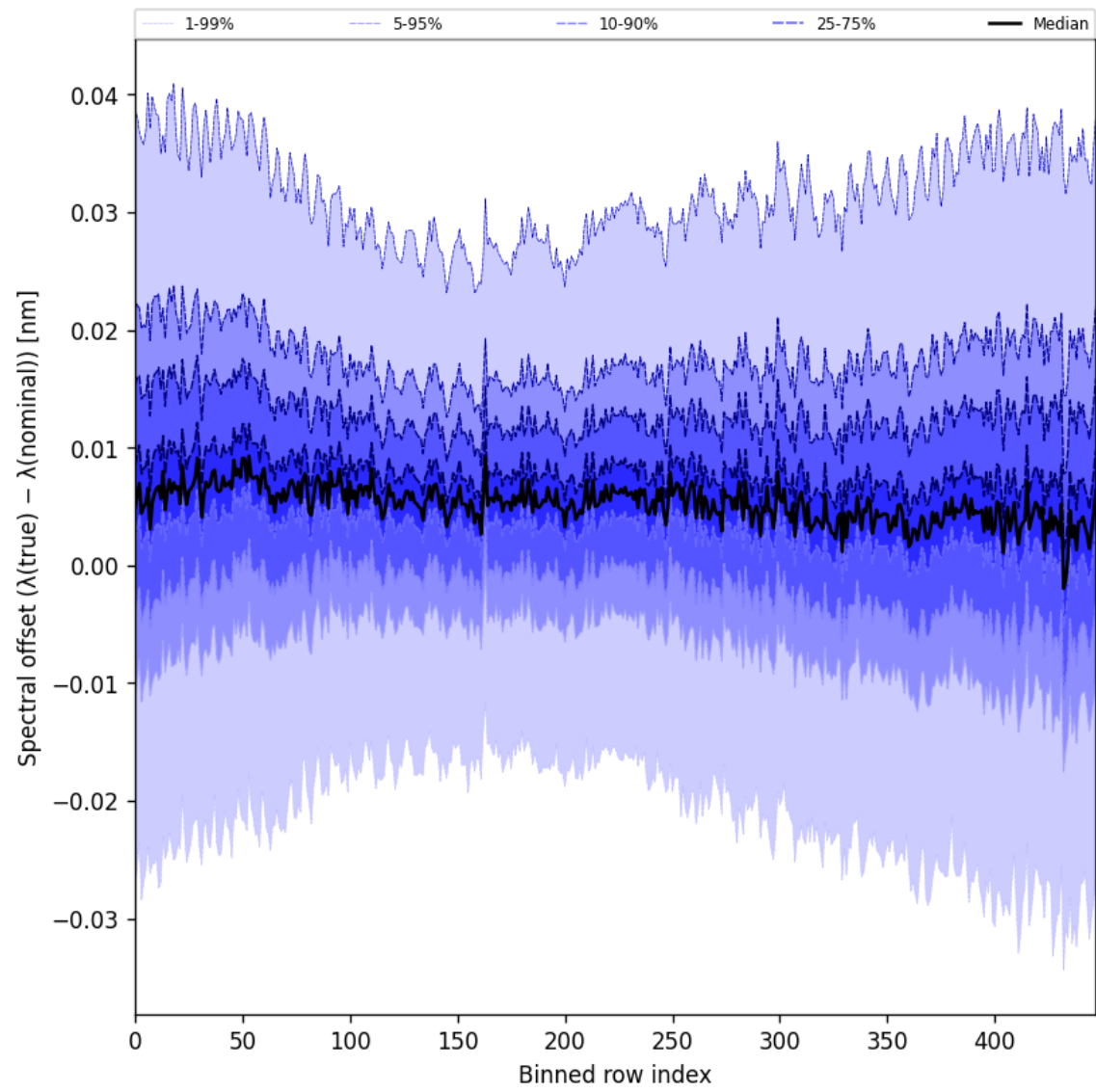
Figure 60: Along track statistics of “Spectral offset ( \lambda_{\text{true}} - \lambda_{\text{nominal}} )” for 2025-10-11 to 2025-10-12
