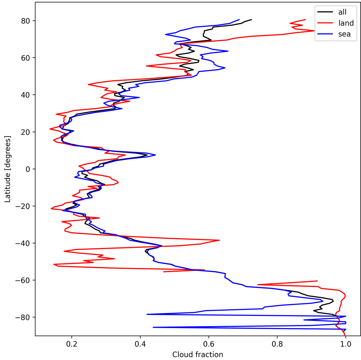
Figure 13: Zonal average of “Cloud fraction” for 2025-10-11 to 2025-10-12.
