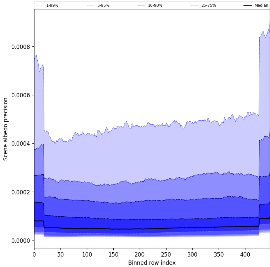
Figure 50: Along track statistics of “Scene albedo precision” for 2025-10-11 to 2025-10-12
