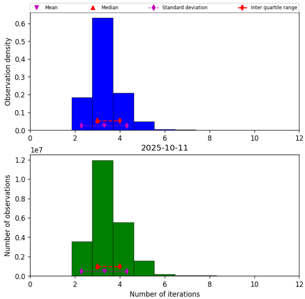
Figure 37: Histogram of “Number of iterations” for 2025-10-11 to 2025-10-12
