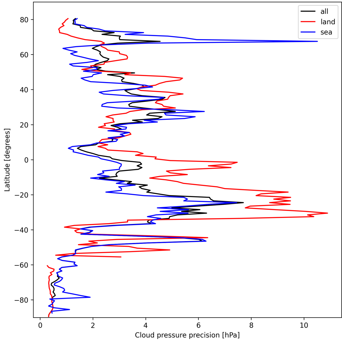
Figure 12: Zonal average of “Cloud pressure precision” for 2025-10-11 to 2025-10-12.
