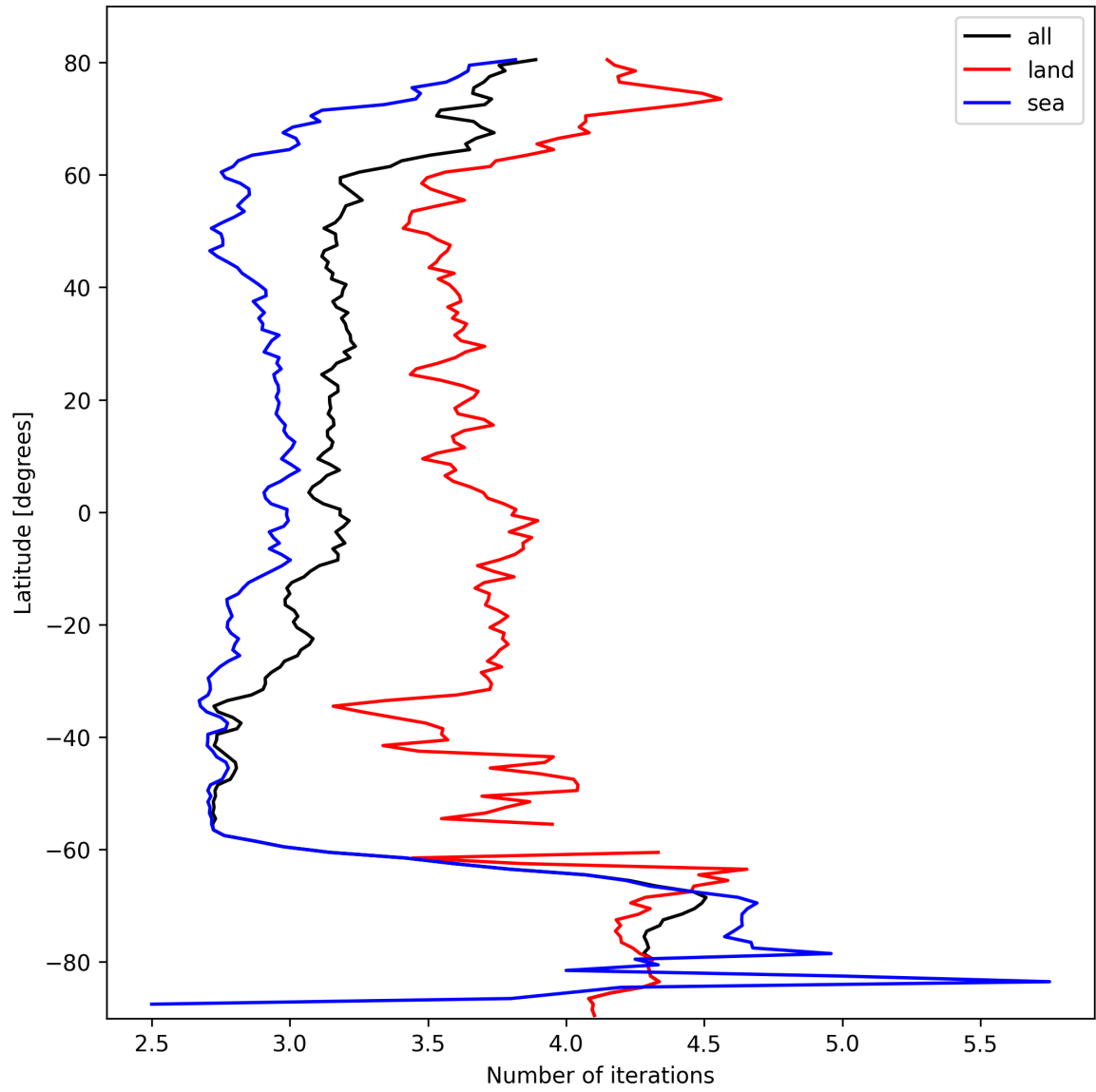
Figure 20: Zonal average of “Number of iterations” for 2025-10-11 to 2025-10-12.
