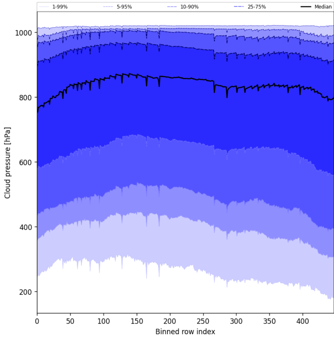
Figure 45: Along track statistics of “Cloud pressure” for 2025-10-11 to 2025-10-12
