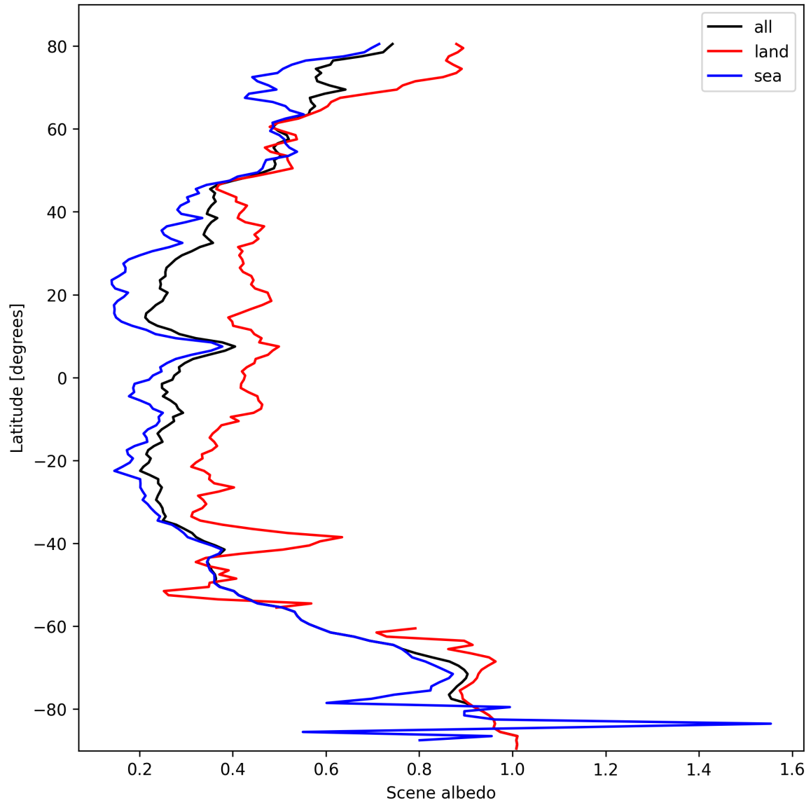
Figure 15: Zonal average of “Scene albedo” for 2025-10-11 to 2025-10-12.
