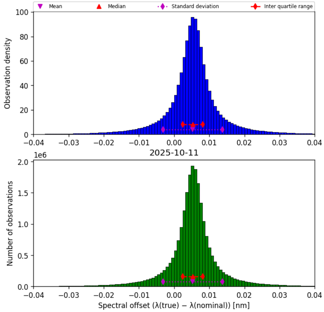
Figure 43: Histogram of “Spectral offset ( \lambda_{\text{true}} - \lambda_{\text{nominal}} )” for 2025-10-11 to 2025-10-12
