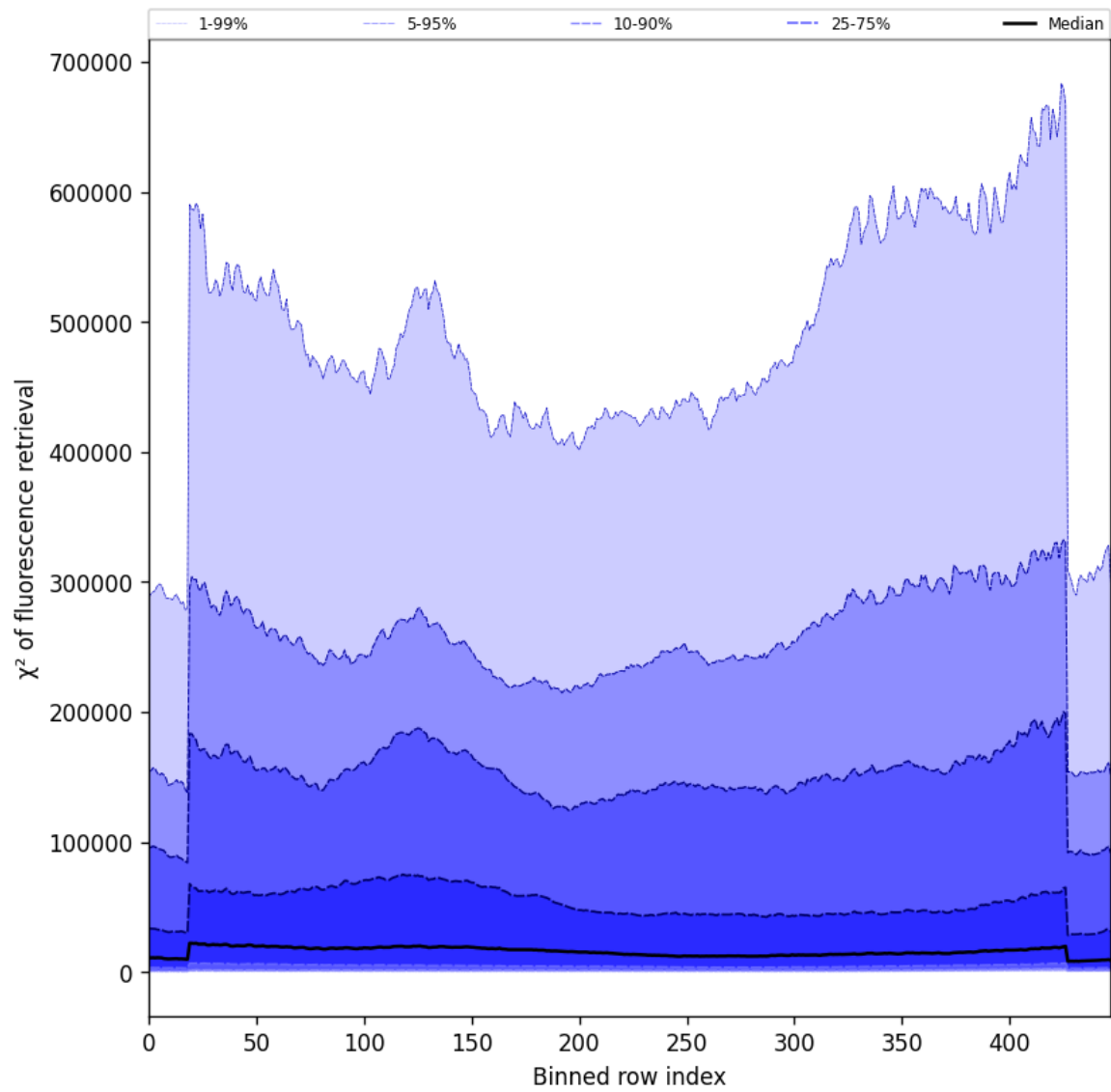
Figure 57: Along track statistics of “ \chi^2 of fluorescence retrieval” for 2025-10-11 to 2025-10-12
