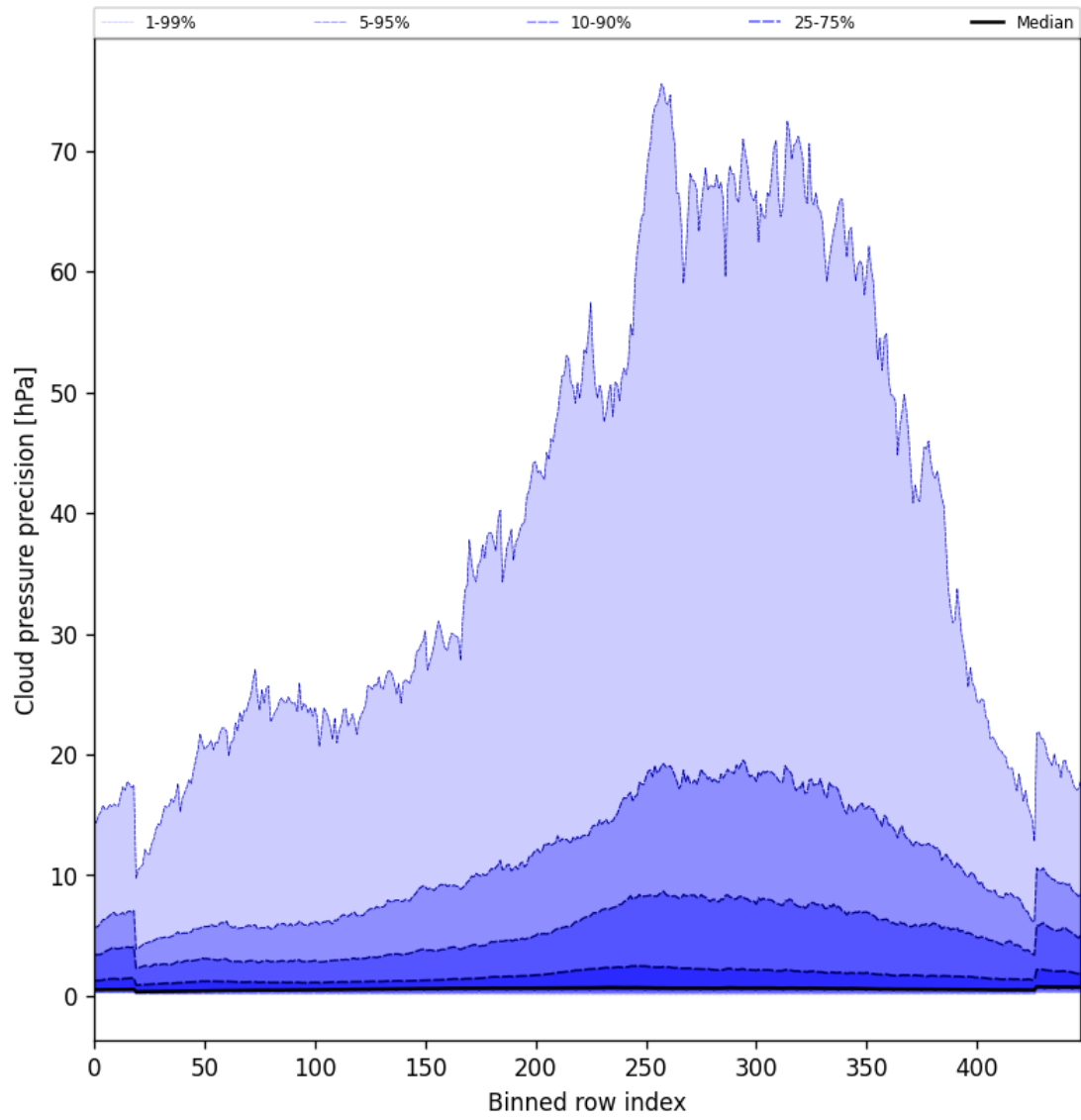
Figure 46: Along track statistics of “Cloud pressure precision” for 2025-10-11 to 2025-10-12
