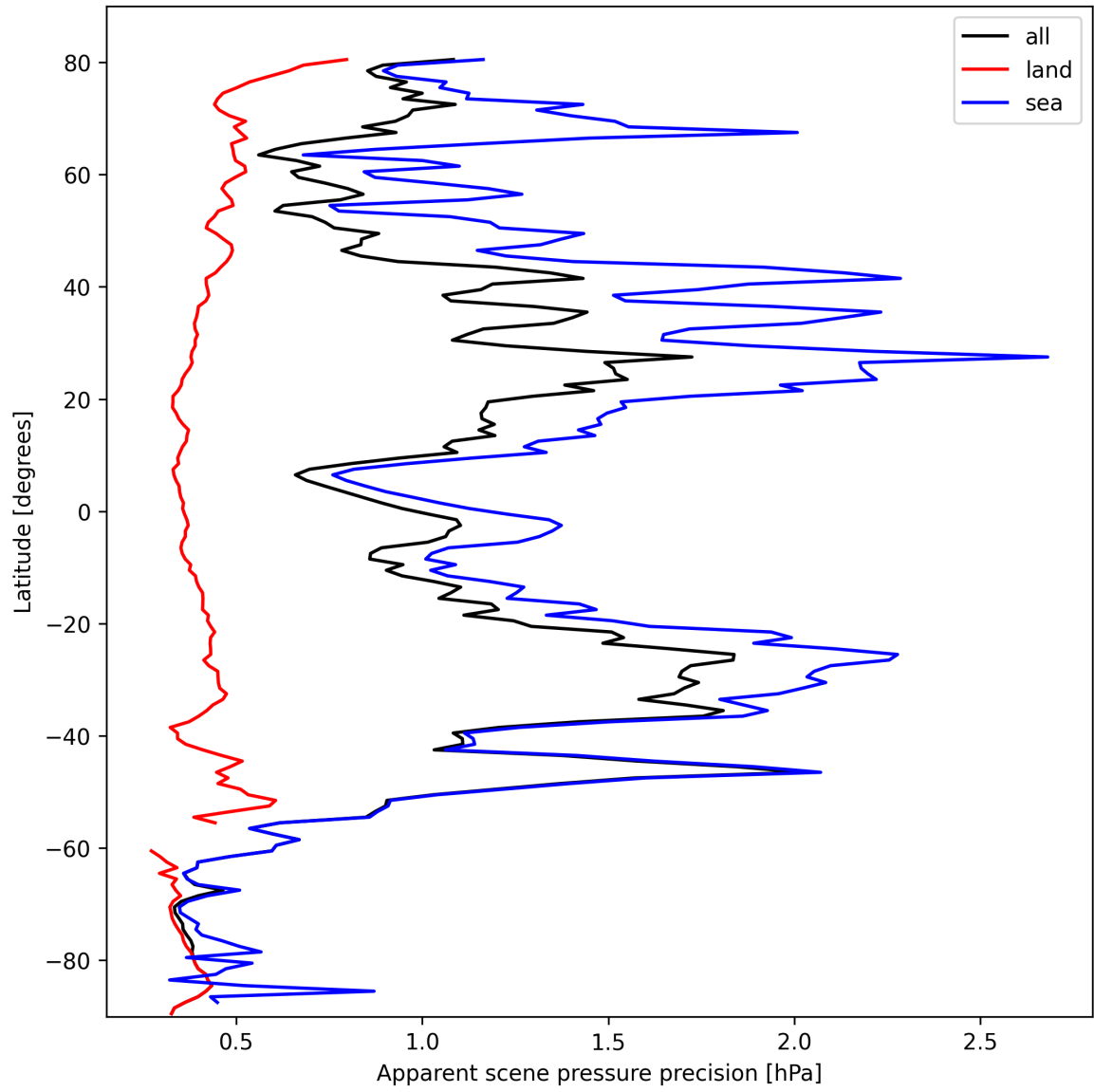
Figure 18: Zonal average of “Apparent scene pressure precision” for 2025-10-11 to 2025-10-12.
