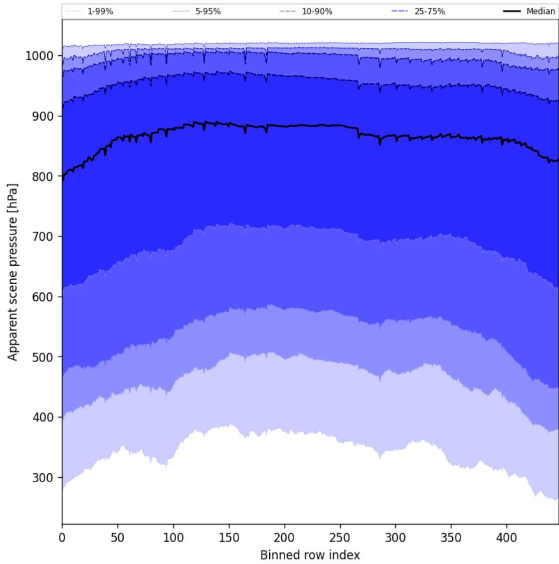
Figure 51: Along track statistics of “Apparent scene pressure” for 2025-10-11 to 2025-10-12
