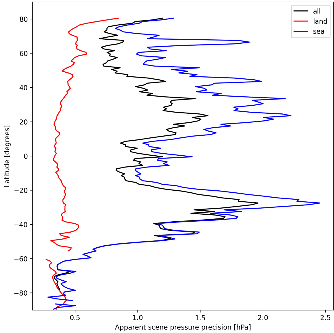
Figure 18: Zonal average of “Apparent scene pressure precision” for 2025-10-12 to 2025-10-13.
