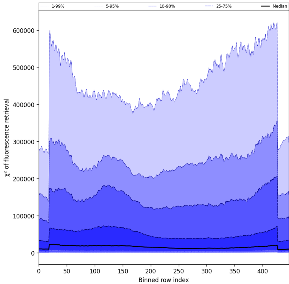
Figure 57: Along track statistics of “ \chi^2 of fluorescence retrieval” for 2025-10-12 to 2025-10-13
