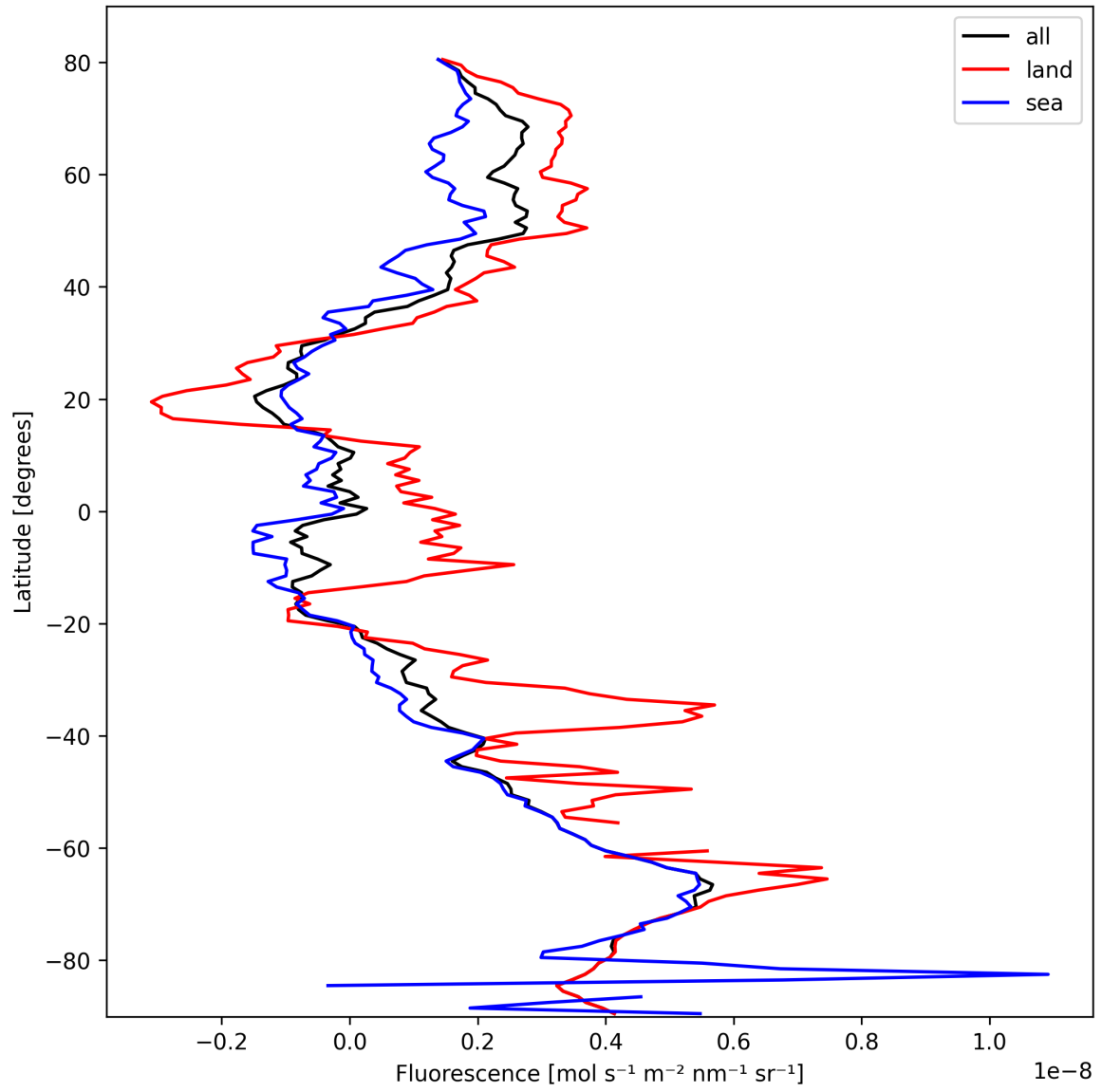
Figure 21: Zonal average of “Fluorescence” for 2025-10-12 to 2025-10-13.
