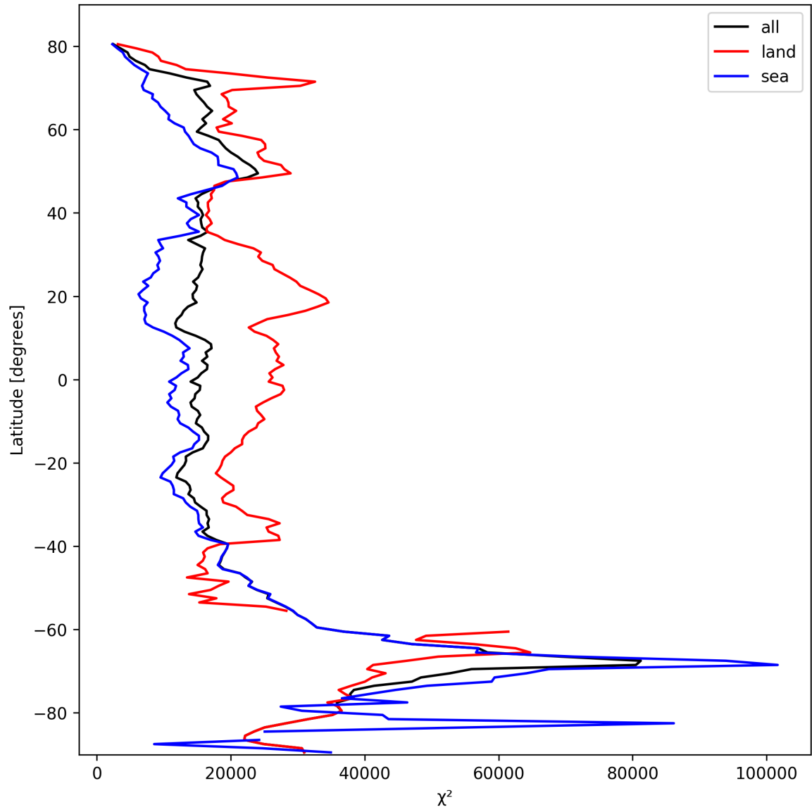
Figure 19: Zonal average of “ \chi^2 ” for 2025-10-12 to 2025-10-13.
