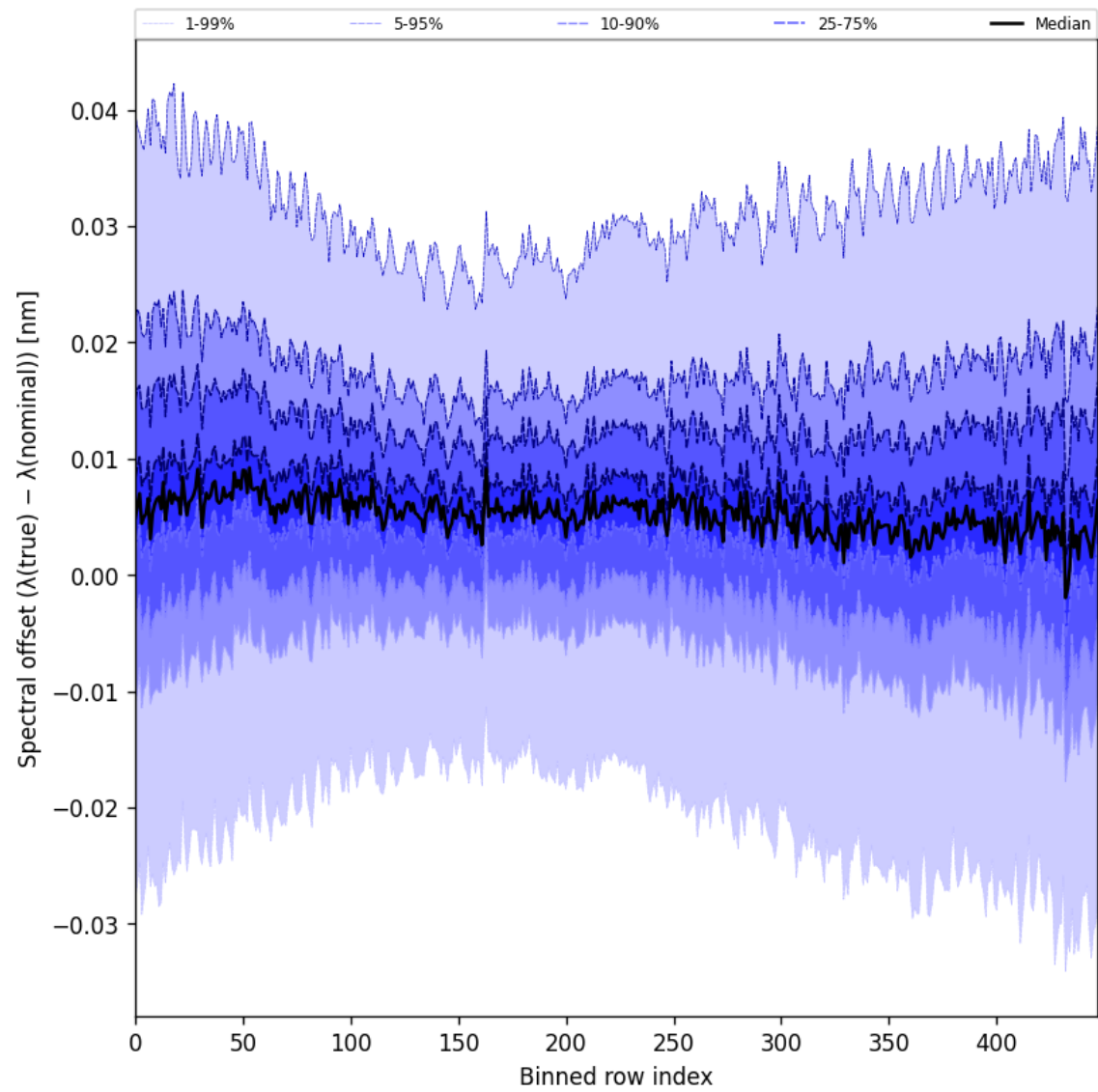
Figure 60: Along track statistics of “Spectral offset ( \lambda_{\text{true}} - \lambda_{\text{nominal}} )” for 2025-10-12 to 2025-10-13
