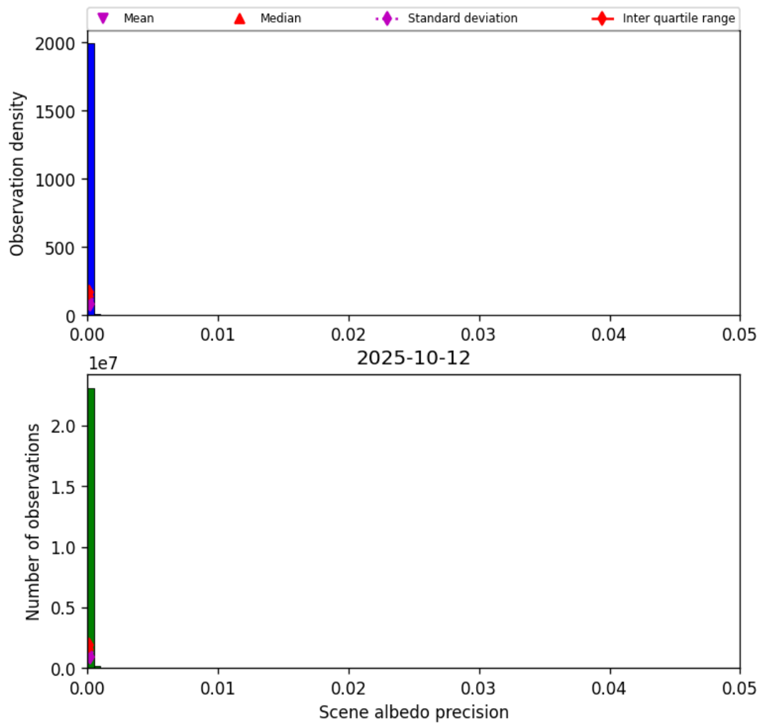
Figure 33: Histogram of “Scene albedo precision” for 2025-10-12 to 2025-10-13
