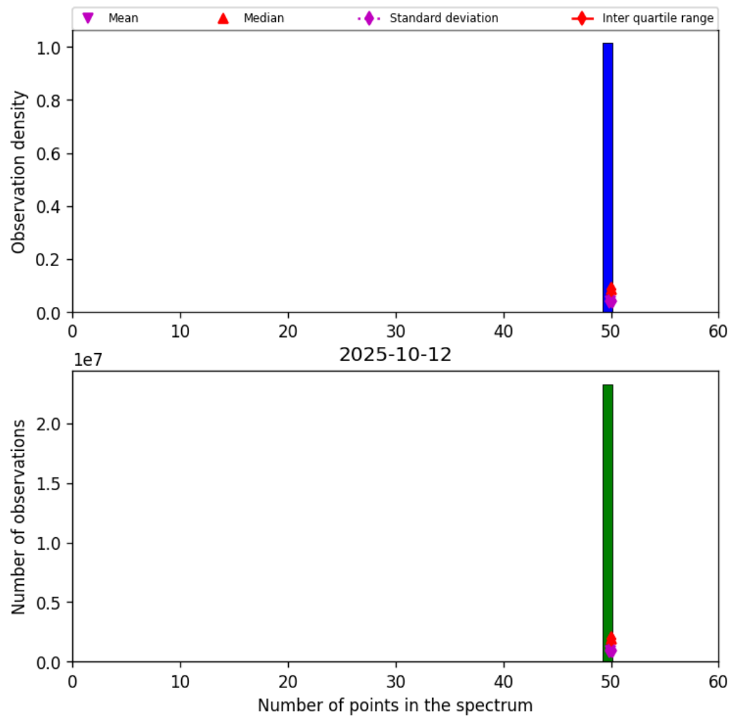
Figure 42: Histogram of “Number of points in the spectrum” for 2025-10-12 to 2025-10-13
