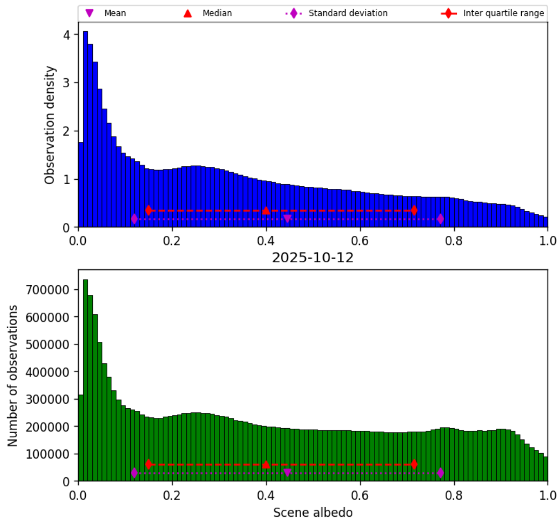
Figure 32: Histogram of “Scene albedo” for 2025-10-12 to 2025-10-13
