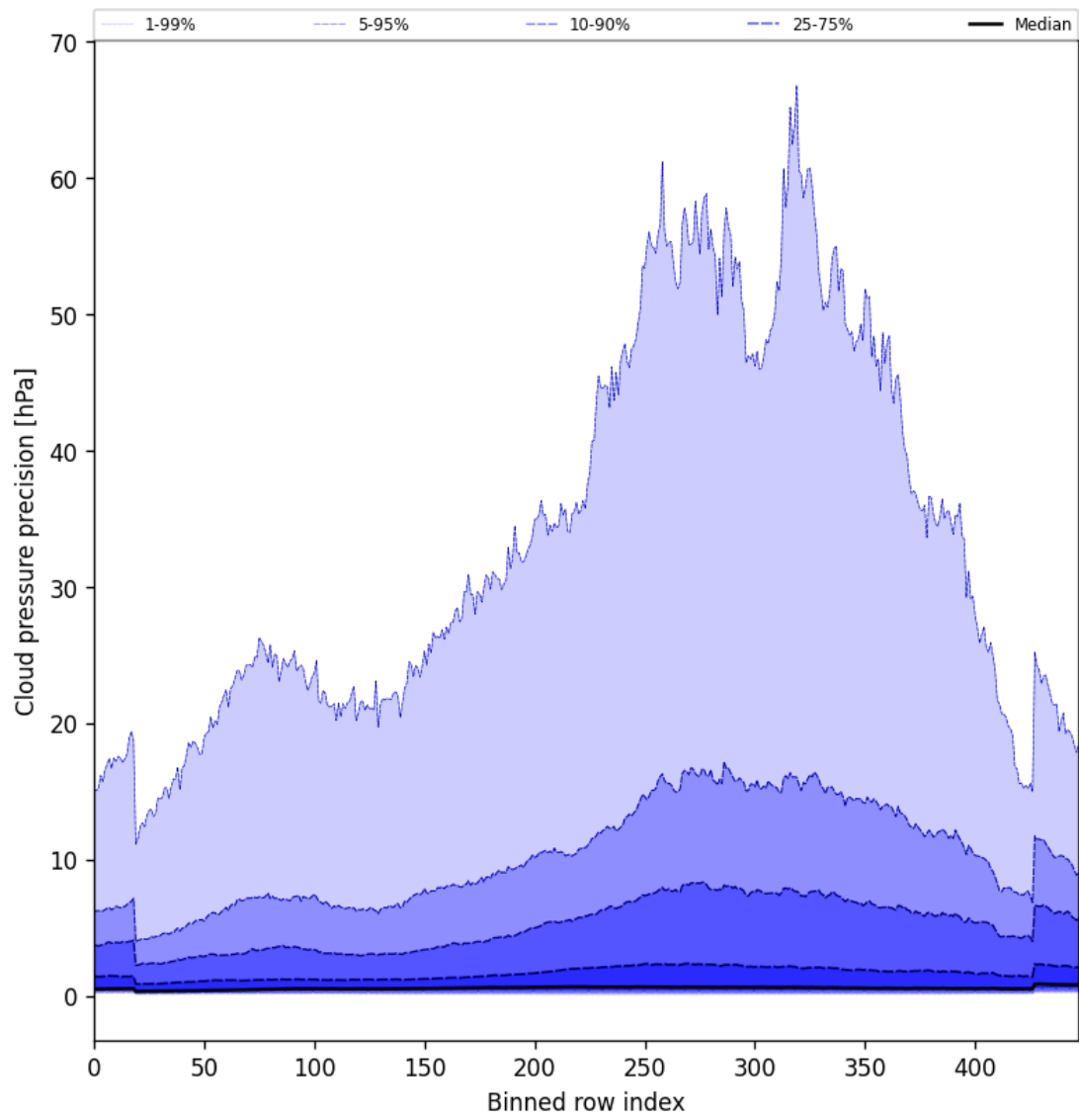
Figure 46: Along track statistics of “Cloud pressure precision” for 2025-10-12 to 2025-10-13
