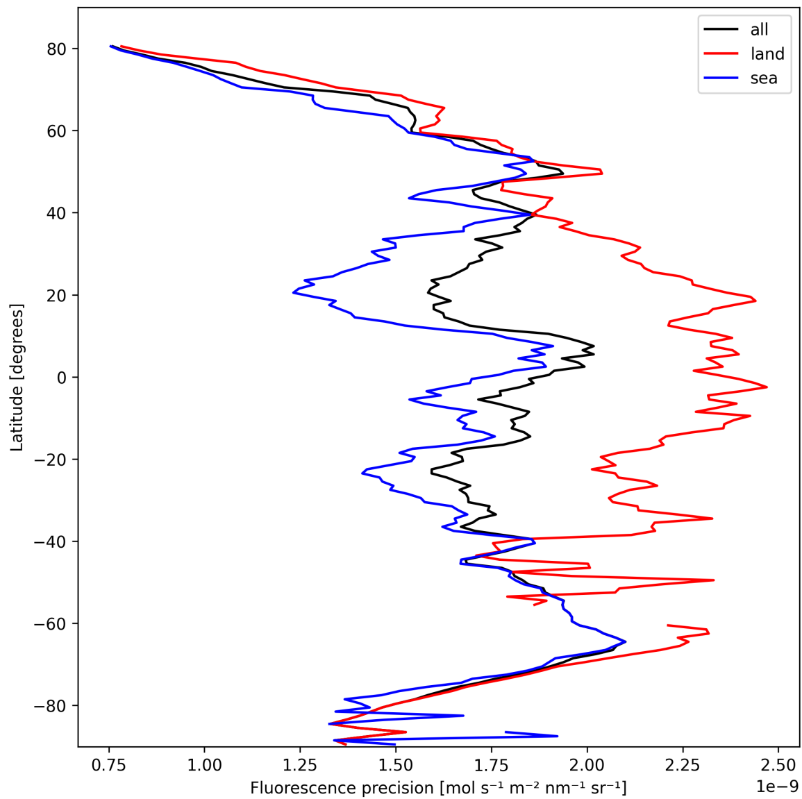
Figure 22: Zonal average of “Fluorescence precision” for 2025-10-12 to 2025-10-13.
