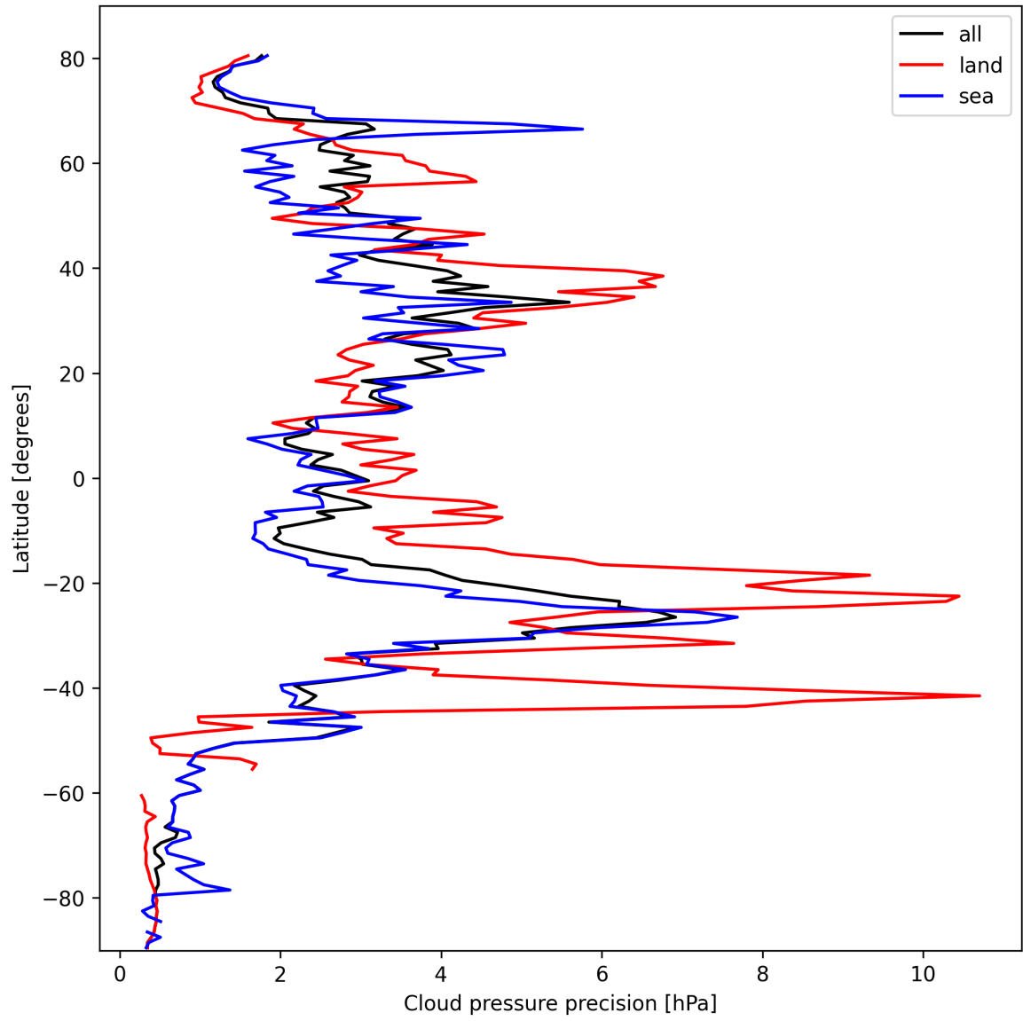
Figure 12: Zonal average of “Cloud pressure precision” for 2025-10-12 to 2025-10-13.
