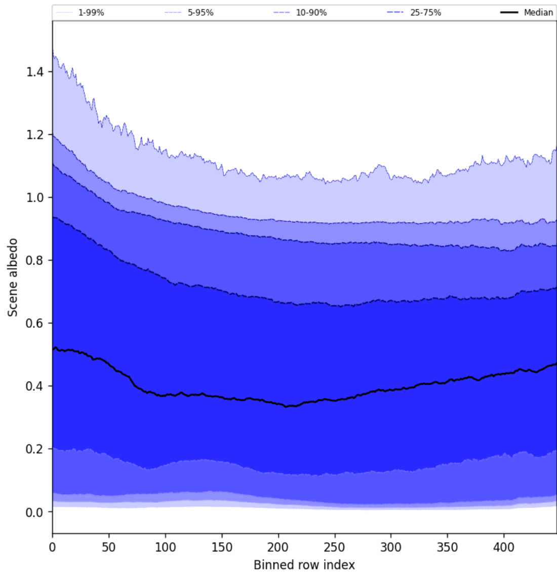
Figure 49: Along track statistics of “Scene albedo” for 2025-10-12 to 2025-10-13
