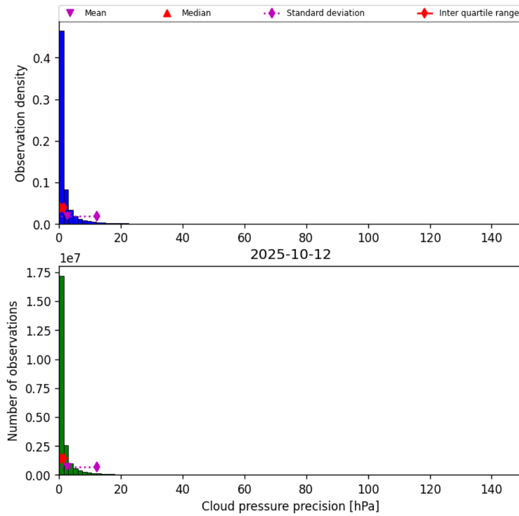
Figure 29: Histogram of “Cloud pressure precision” for 2025-10-12 to 2025-10-13
