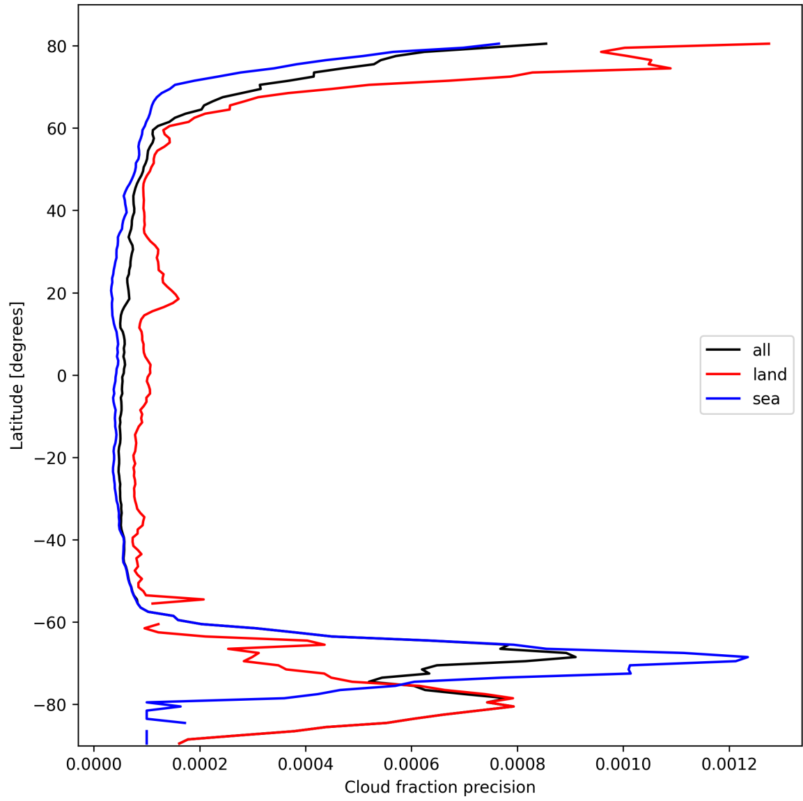
Figure 14: Zonal average of “Cloud fraction precision” for 2025-10-12 to 2025-10-13.
