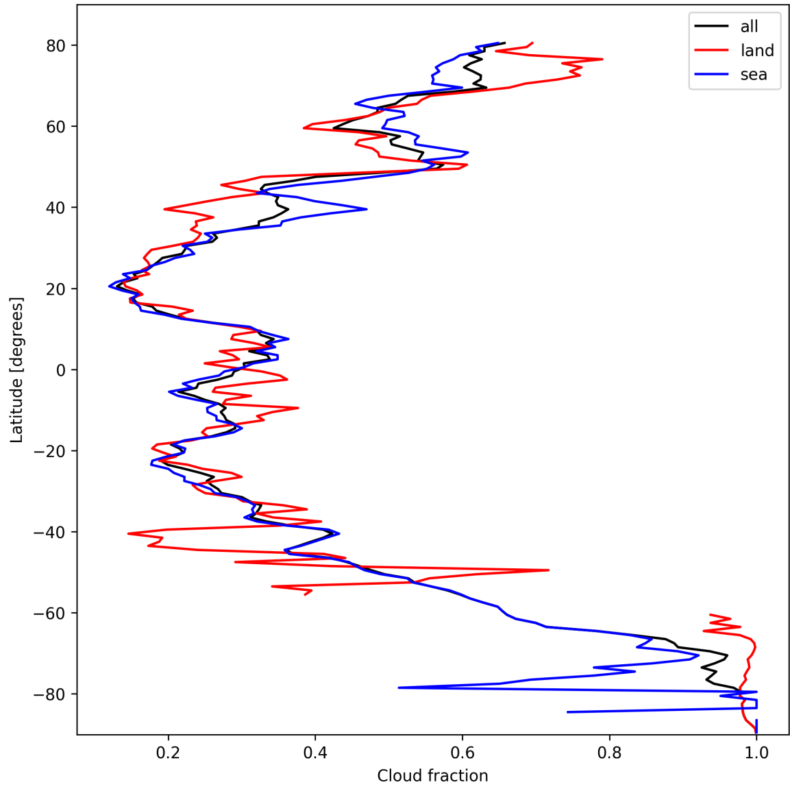
Figure 13: Zonal average of “Cloud fraction” for 2025-10-12 to 2025-10-13.
