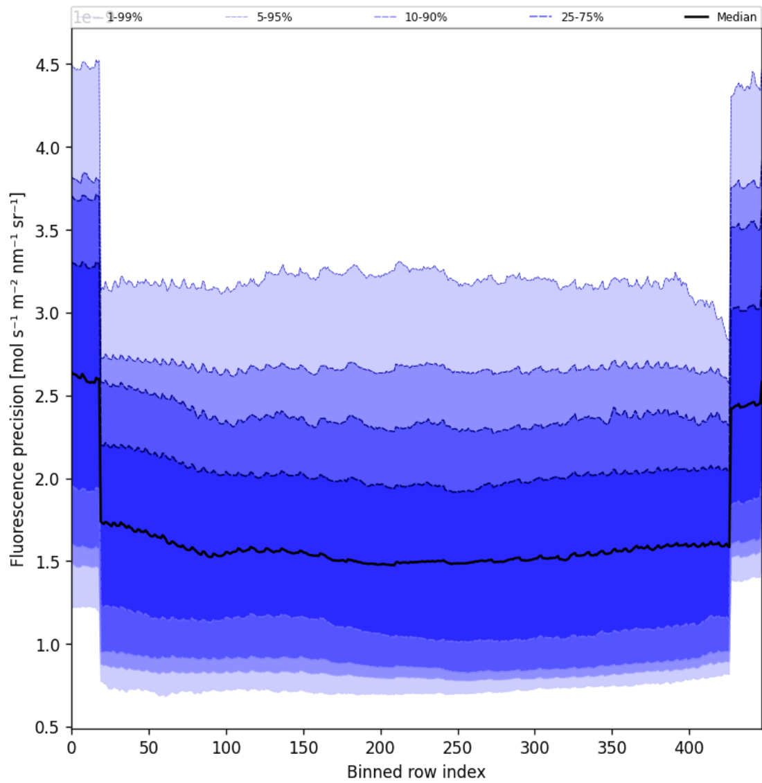
Figure 56: Along track statistics of “Fluorescence precision” for 2025-10-12 to 2025-10-13
