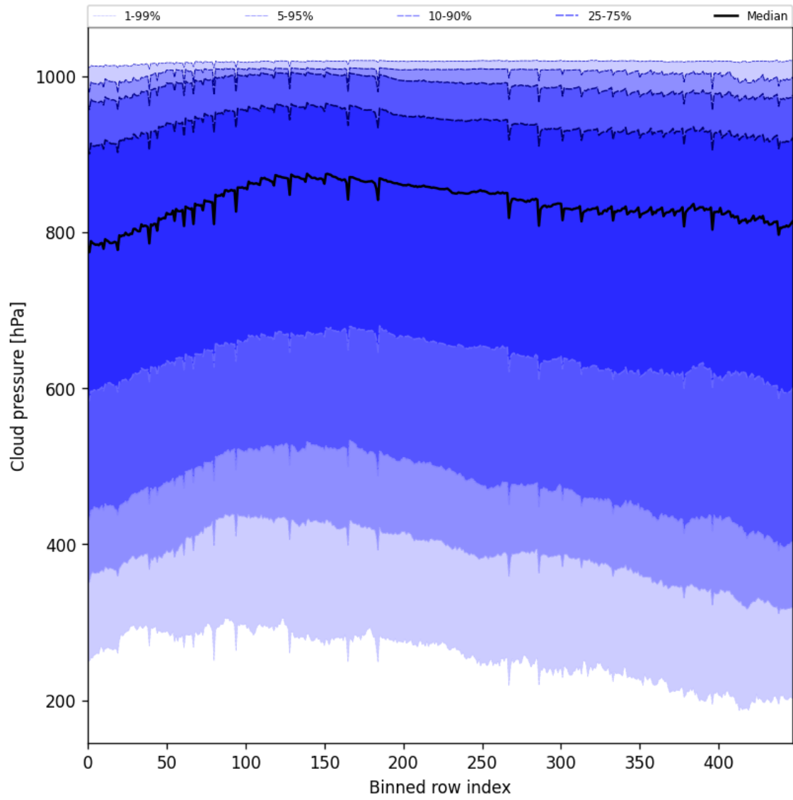
Figure 45: Along track statistics of “Cloud pressure” for 2025-10-12 to 2025-10-13
