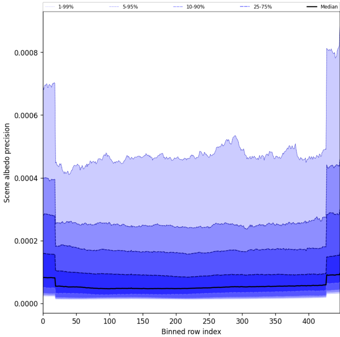
Figure 50: Along track statistics of “Scene albedo precision” for 2025-10-12 to 2025-10-13
