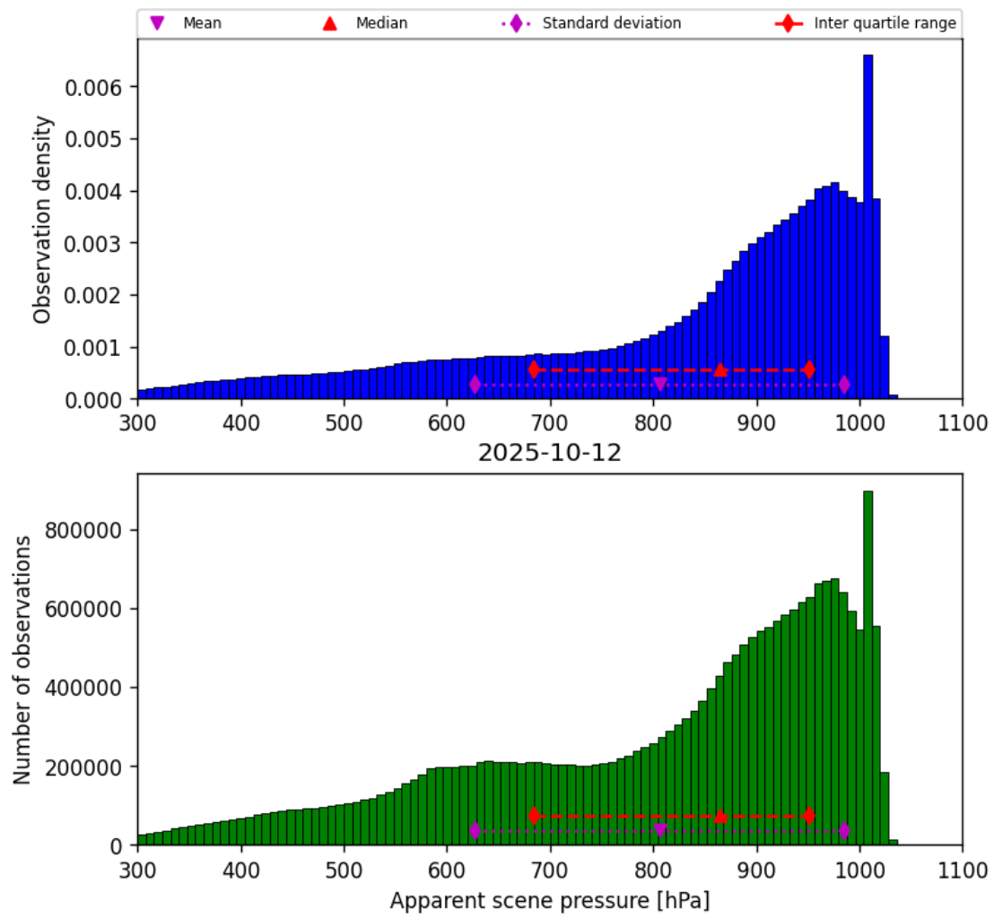
Figure 34: Histogram of “Apparent scene pressure” for 2025-10-12 to 2025-10-13
