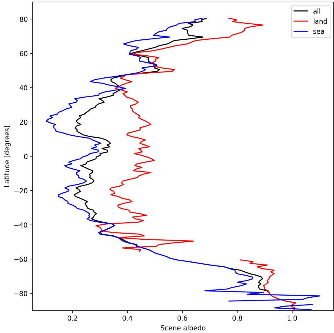
Figure 15: Zonal average of “Scene albedo” for 2025-10-12 to 2025-10-13.
