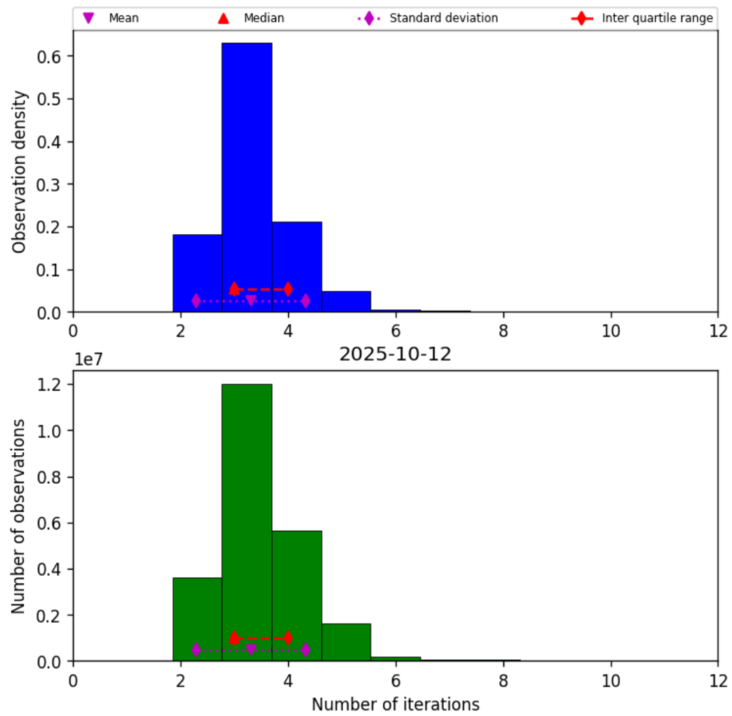
Figure 37: Histogram of “Number of iterations” for 2025-10-12 to 2025-10-13
