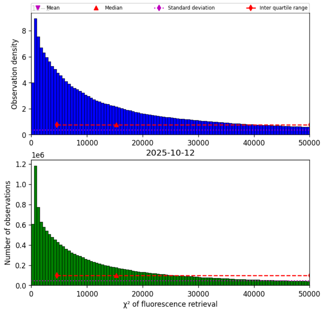
Figure 40: Histogram of “ \chi^2 of fluorescence retrieval” for 2025-10-12 to 2025-10-13
