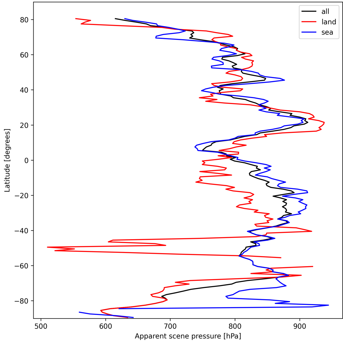
Figure 17: Zonal average of “Apparent scene pressure” for 2025-10-12 to 2025-10-13.
