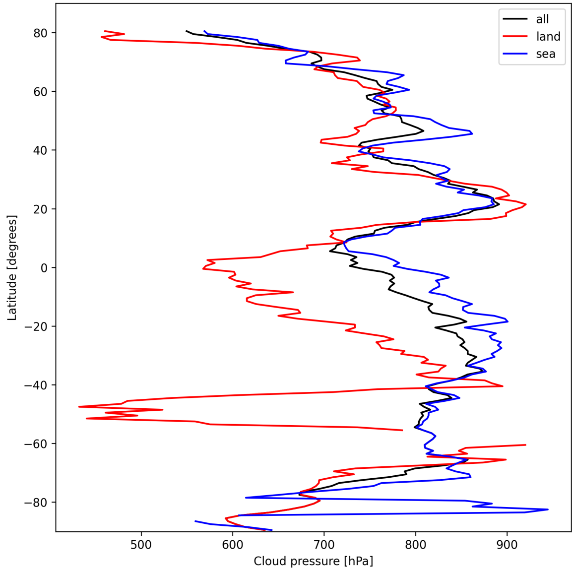
Figure 11: Zonal average of “Cloud pressure” for 2025-10-12 to 2025-10-13.
