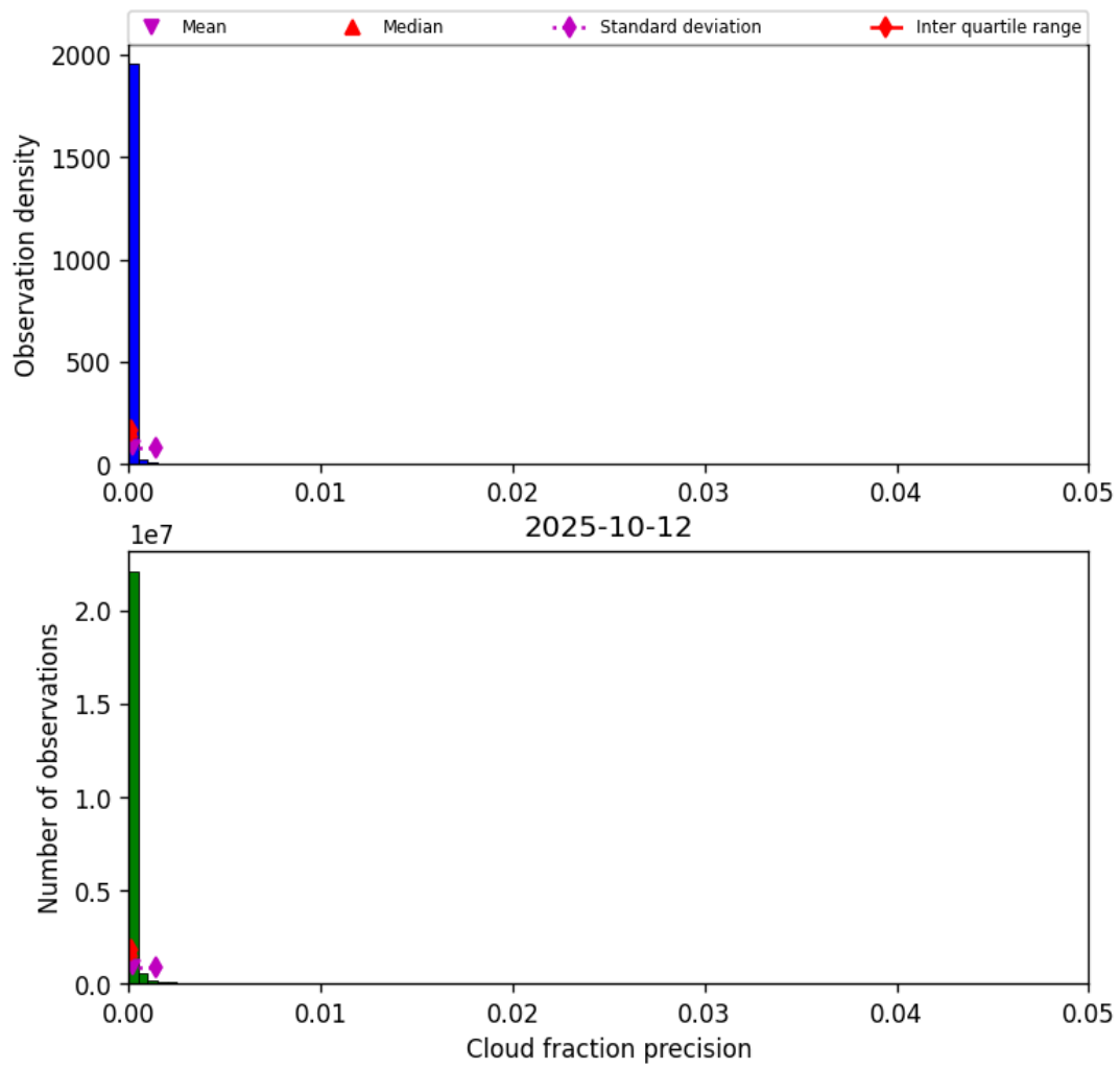
Figure 31: Histogram of “Cloud fraction precision” for 2025-10-12 to 2025-10-13
