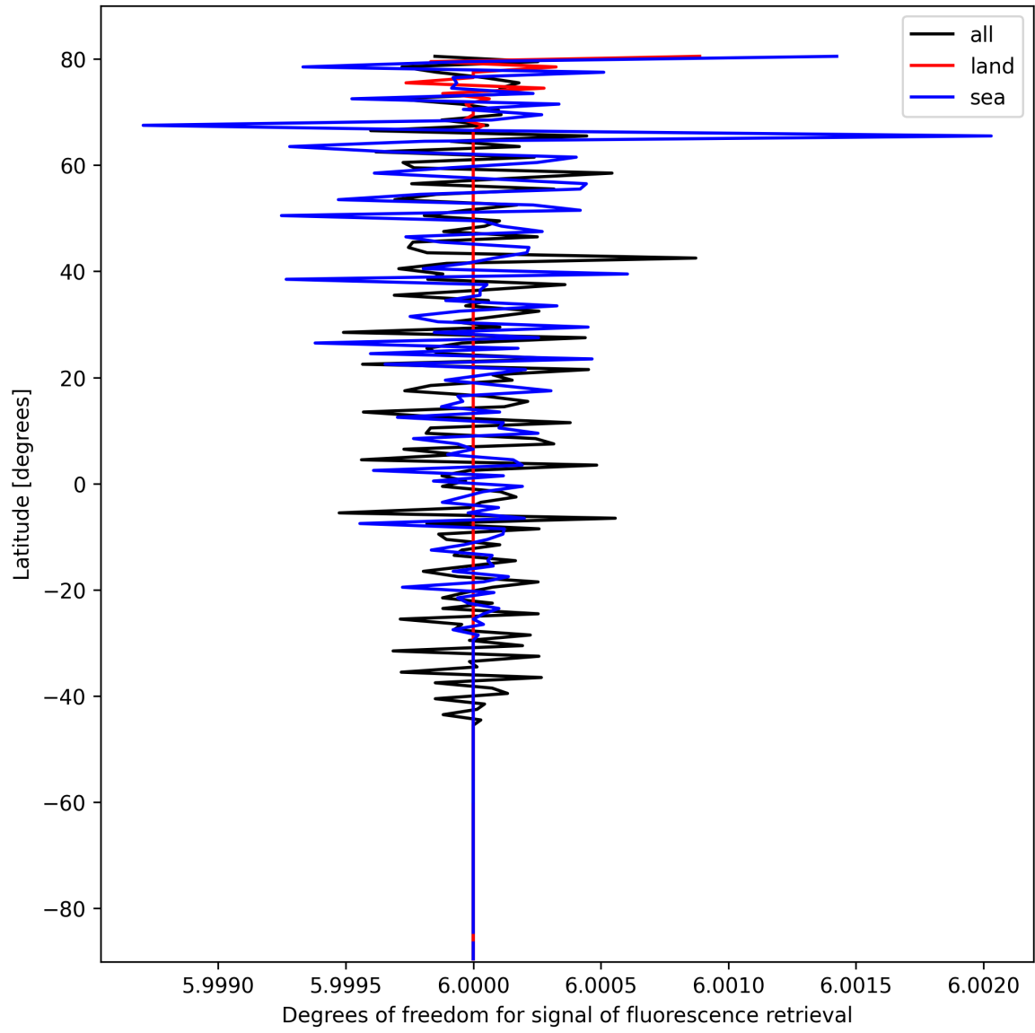
Figure 24: Zonal average of “Degrees of freedom for signal of fluorescence retrieval” for 2025-10-12 to 2025-10-13.
