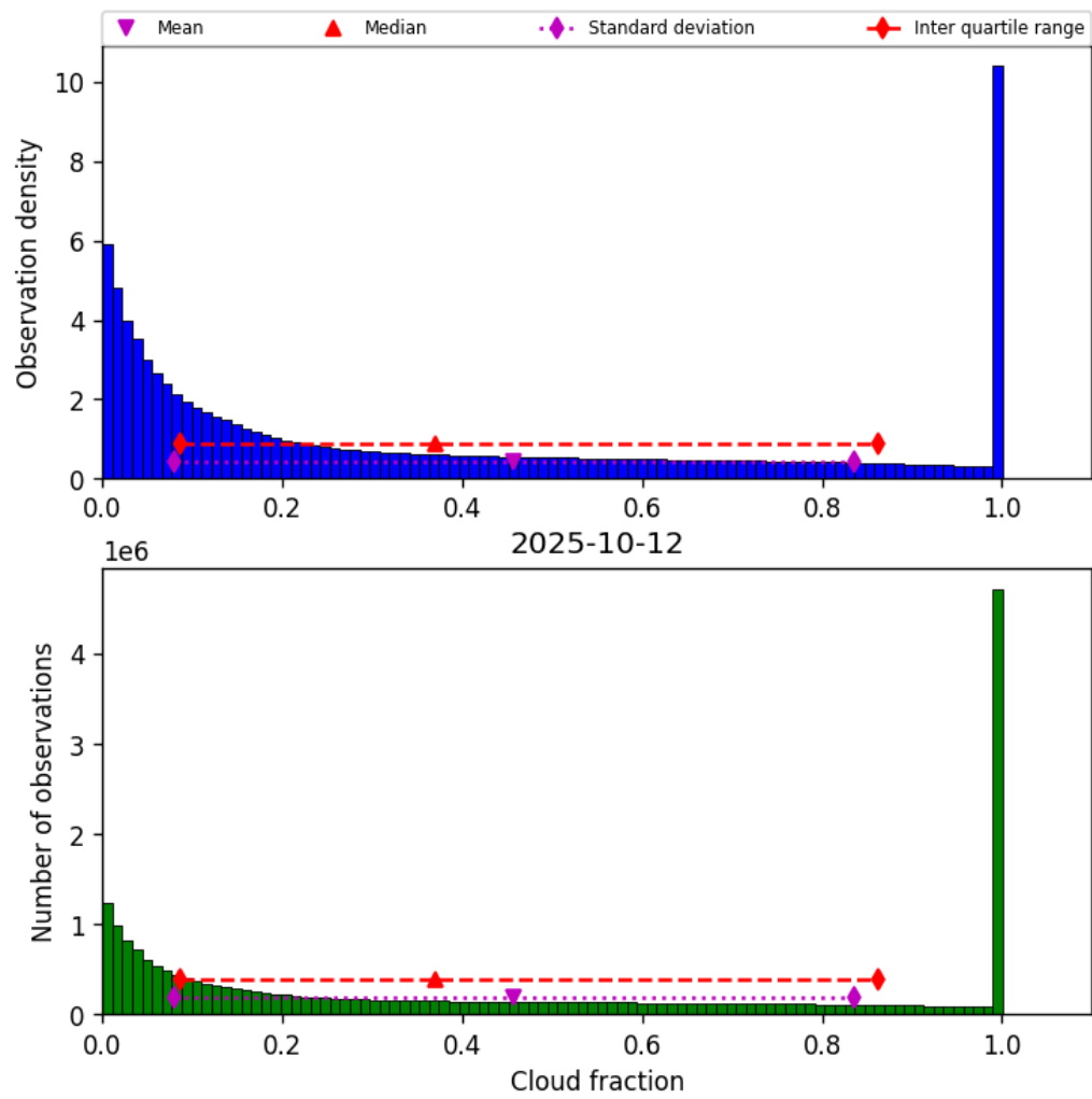
Figure 30: Histogram of “Cloud fraction” for 2025-10-12 to 2025-10-13
