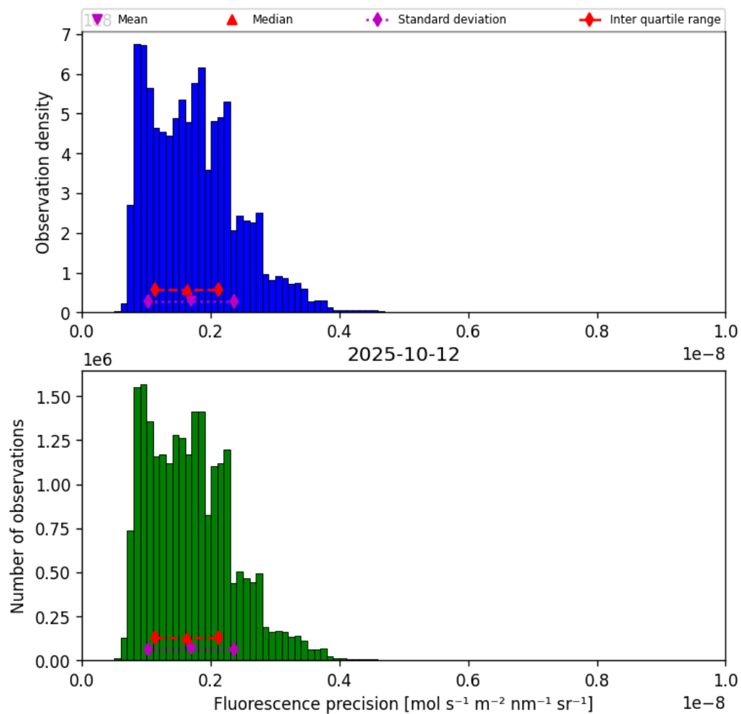
Figure 39: Histogram of “Fluorescence precision” for 2025-10-12 to 2025-10-13
