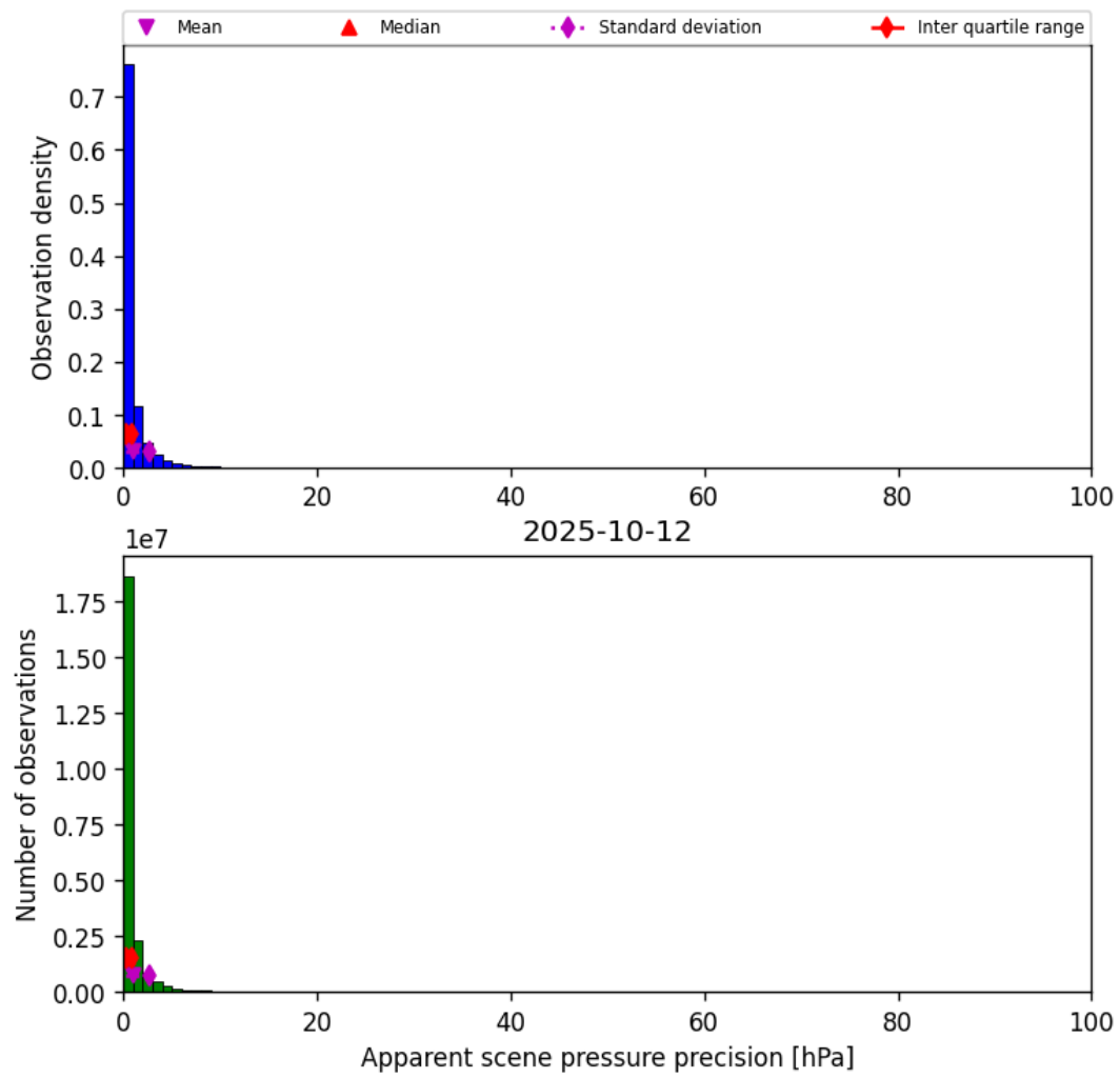
Figure 35: Histogram of “Apparent scene pressure precision” for 2025-10-12 to 2025-10-13
