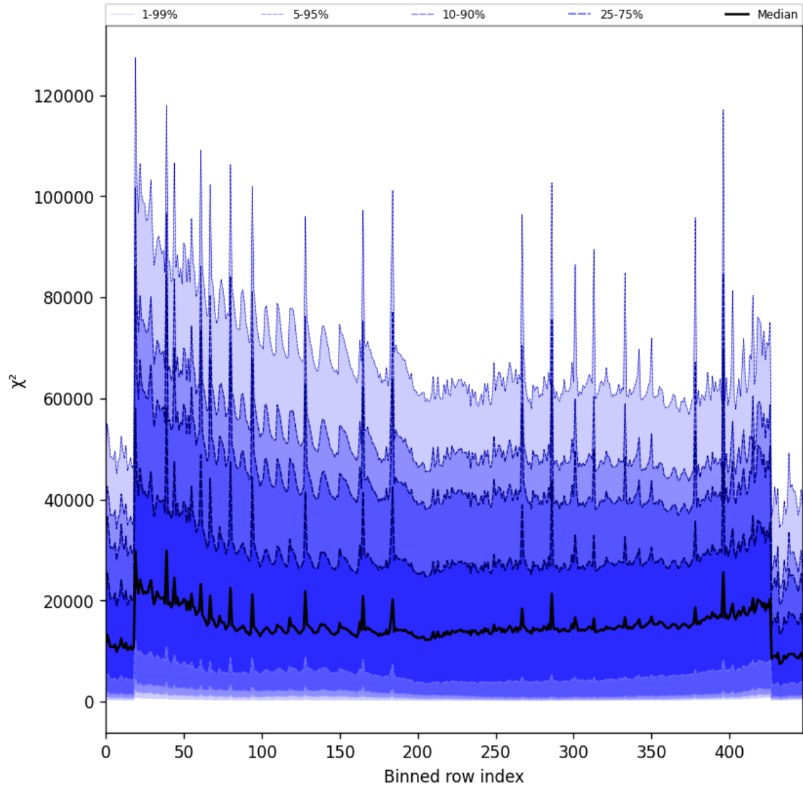
Figure 53: Along track statistics of “ \chi^2 ” for 2025-10-12 to 2025-10-13
