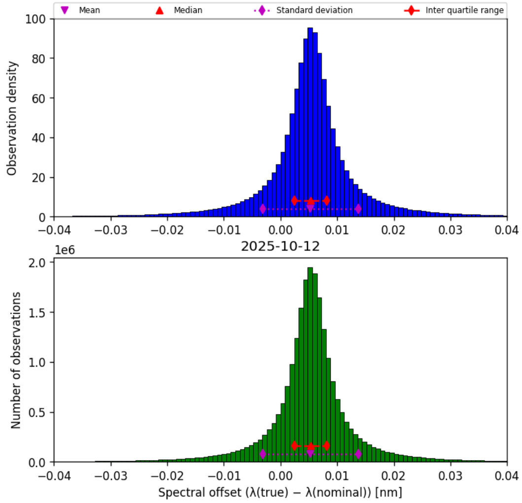
Figure 43: Histogram of “Spectral offset ( \lambda_{\text{true}} - \lambda_{\text{nominal}} )” for 2025-10-12 to 2025-10-13
