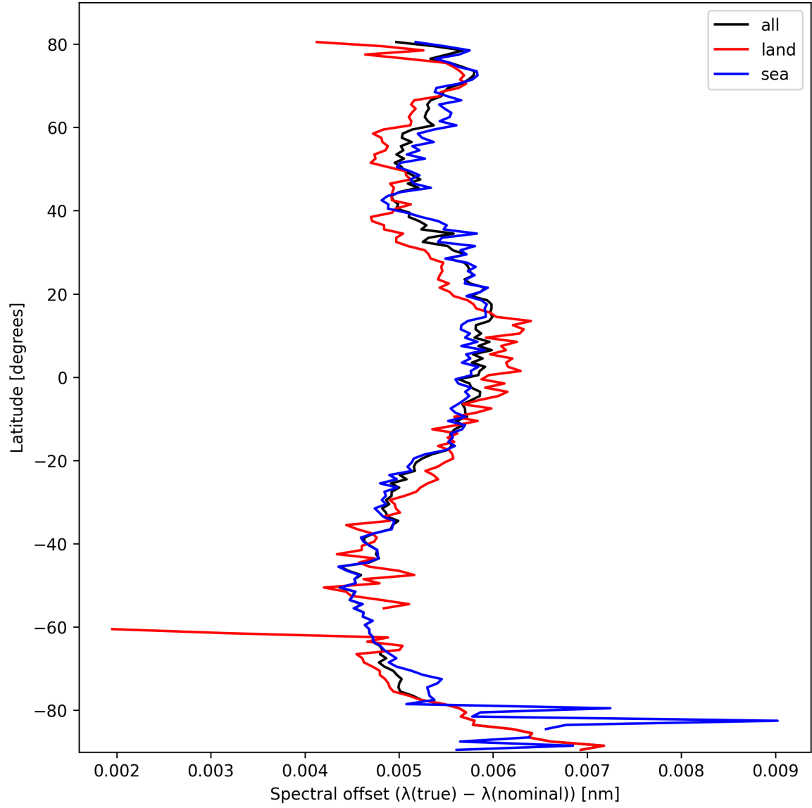
Figure 26: Zonal average of “Spectral offset ( \lambda_{\text{true}} - \lambda_{\text{nominal}} )” for 2025-10-12 to 2025-10-13.
