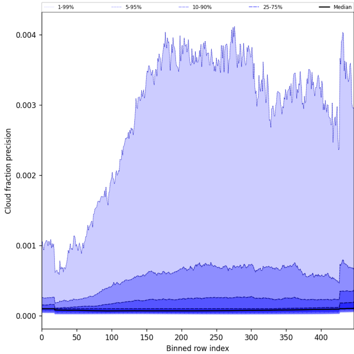
Figure 48: Along track statistics of “Cloud fraction precision” for 2025-10-12 to 2025-10-13
