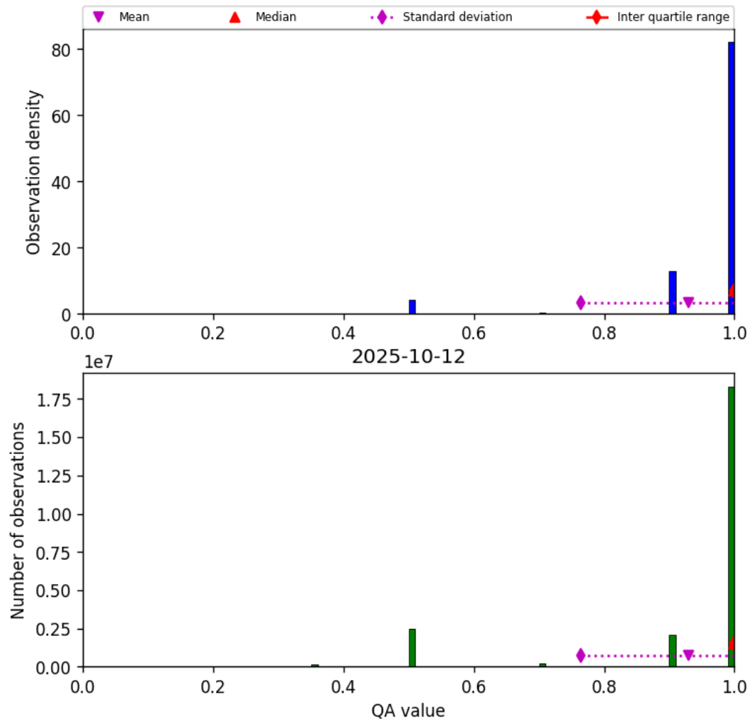
Figure 27: Histogram of “QA value” for 2025-10-12 to 2025-10-13
