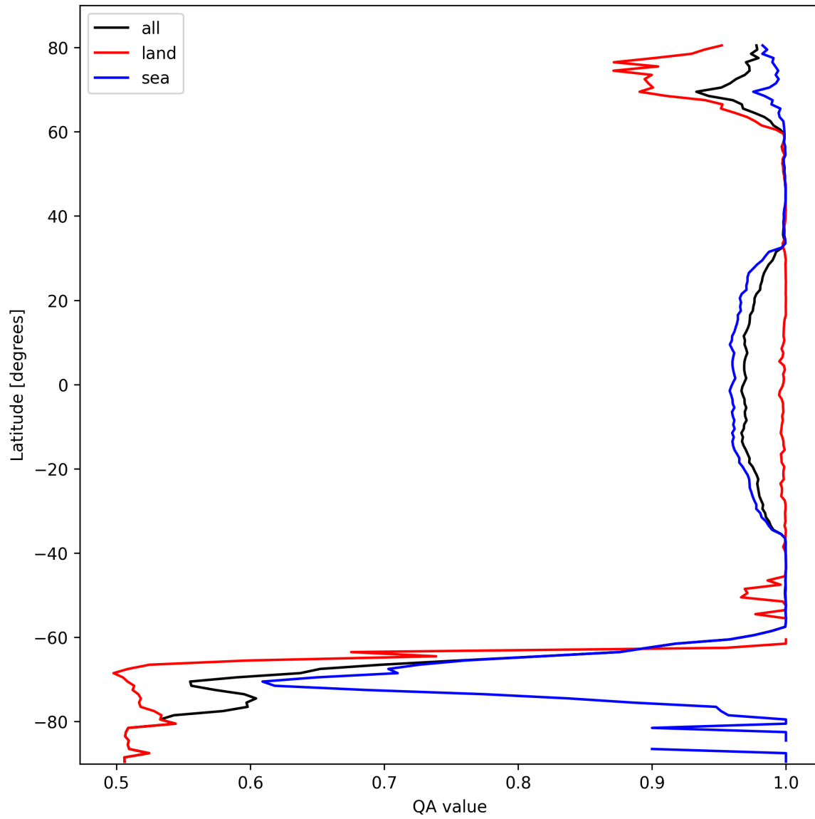
Figure 10: Zonal average of “QA value” for 2025-10-12 to 2025-10-13.
