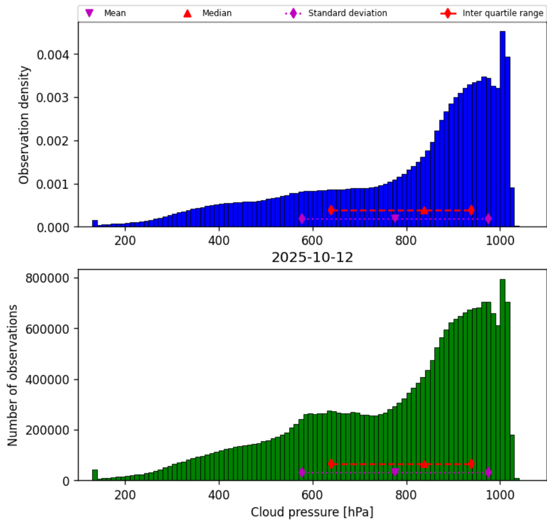
Figure 28: Histogram of “Cloud pressure” for 2025-10-12 to 2025-10-13
