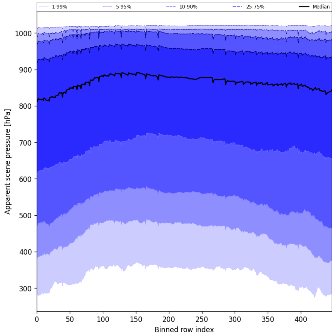
Figure 51: Along track statistics of “Apparent scene pressure” for 2025-10-12 to 2025-10-13
