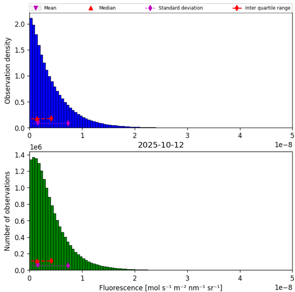
Figure 38: Histogram of “Fluorescence” for 2025-10-12 to 2025-10-13
