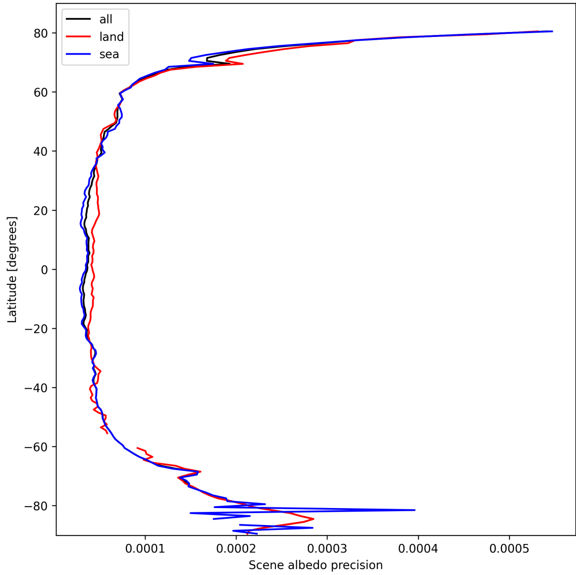
Figure 16: Zonal average of “Scene albedo precision” for 2025-10-12 to 2025-10-13.
