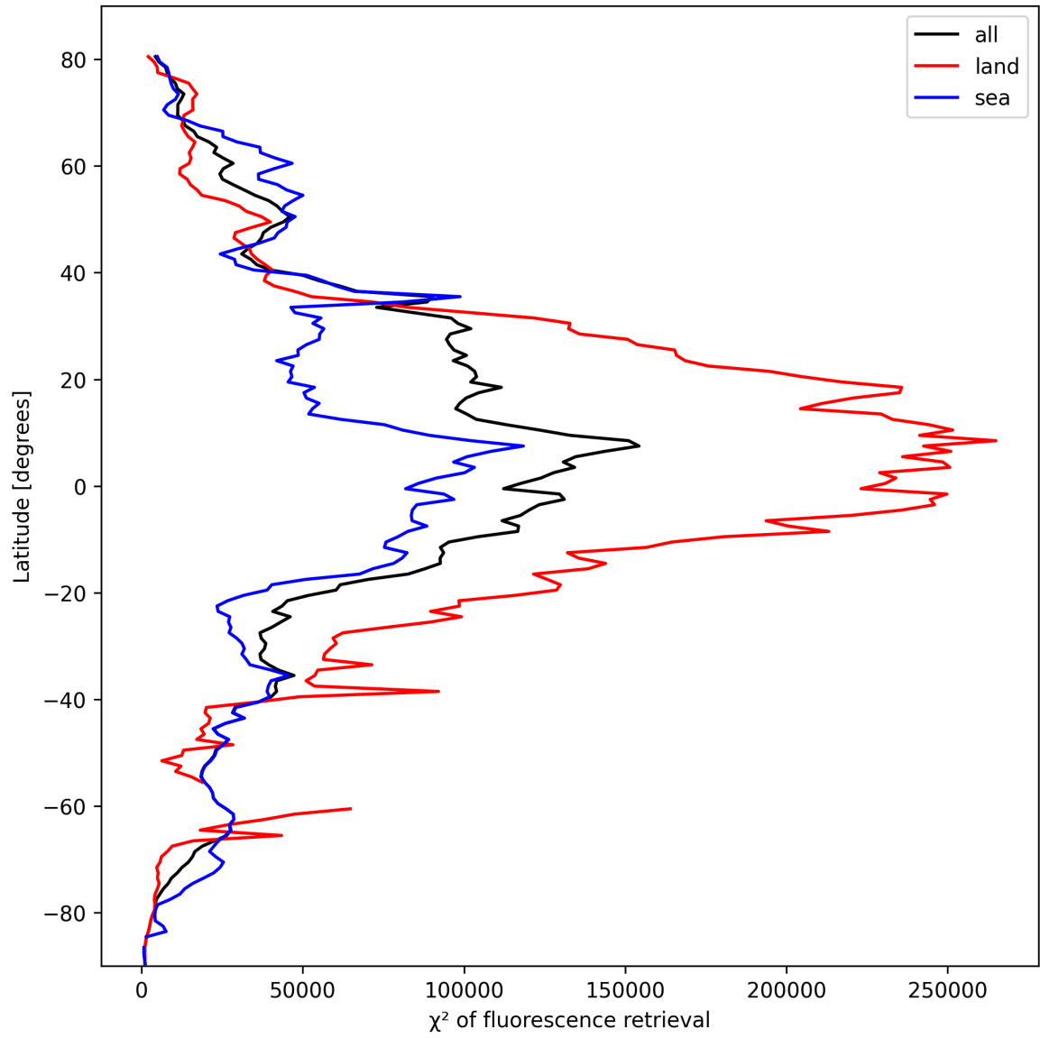
Figure 23: Zonal average of “ \chi^2 of fluorescence retrieval” for 2025-10-12 to 2025-10-13.
