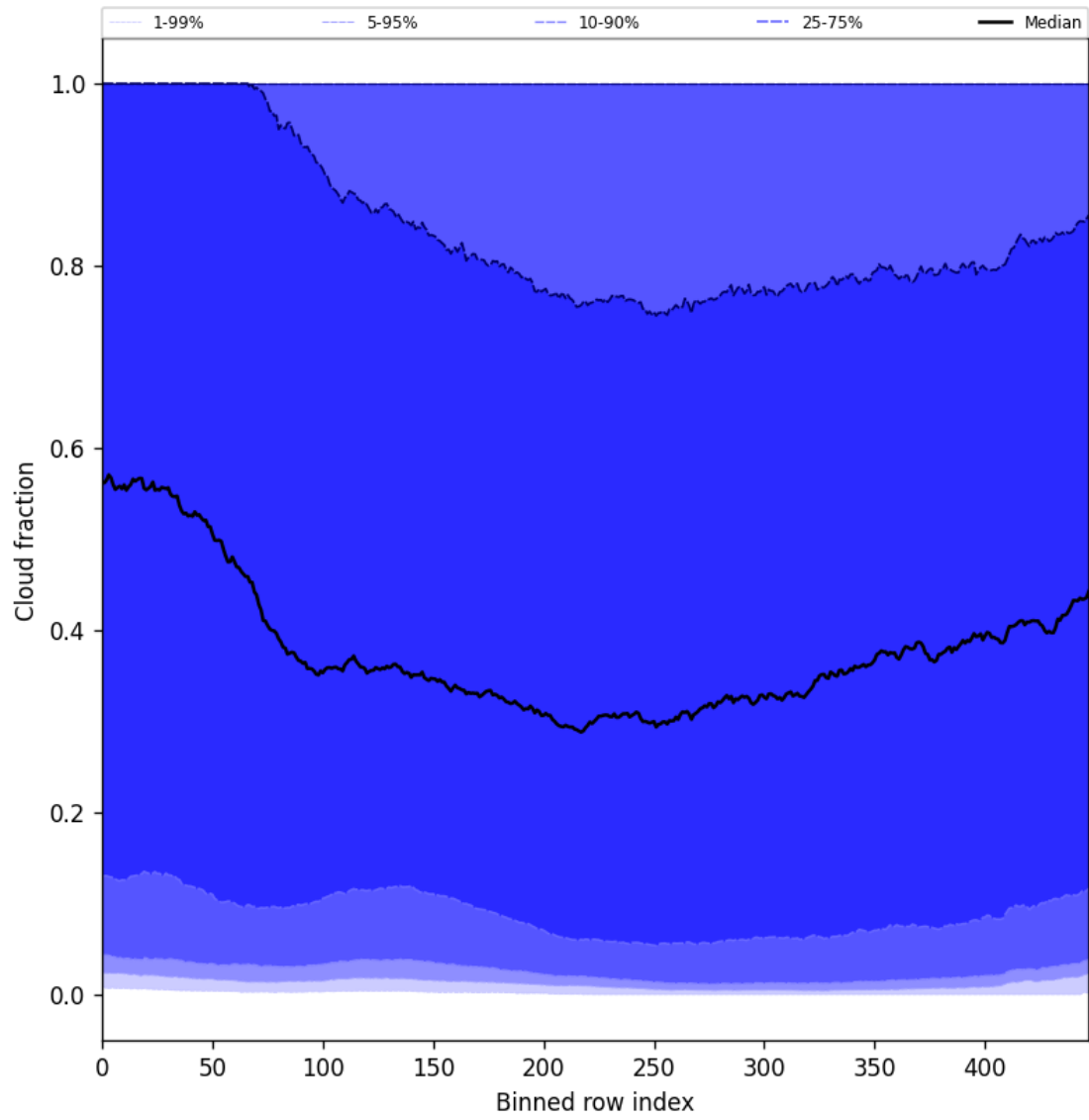
Figure 47: Along track statistics of “Cloud fraction” for 2025-10-12 to 2025-10-13
