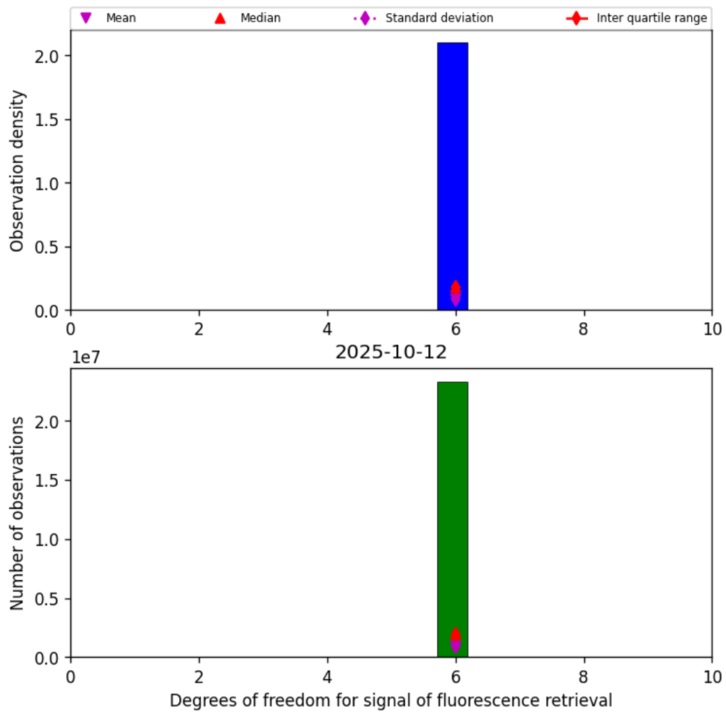
Figure 41: Histogram of “Degrees of freedom for signal of fluorescence retrieval” for 2025-10-12 to 2025-10-13
