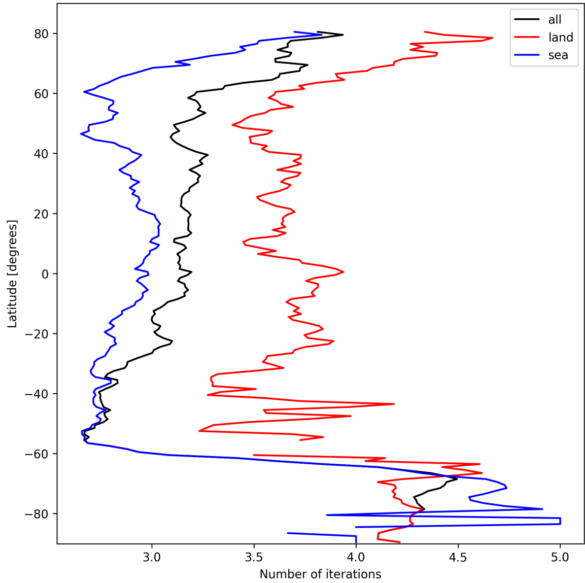
Figure 20: Zonal average of “Number of iterations” for 2025-10-12 to 2025-10-13.
