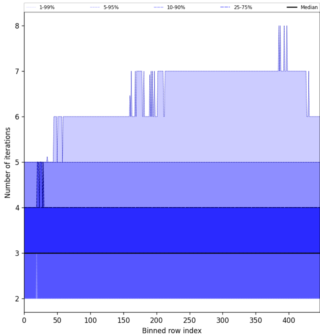
Figure 54: Along track statistics of “Number of iterations” for 2025-10-12 to 2025-10-13
