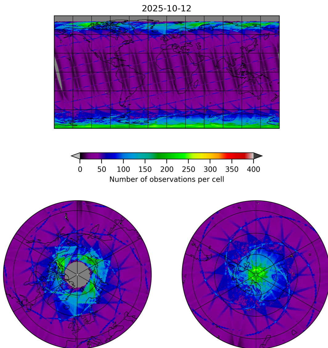
Figure 9: Map of the number of observations for 2025-10-12 to 2025-10-13
