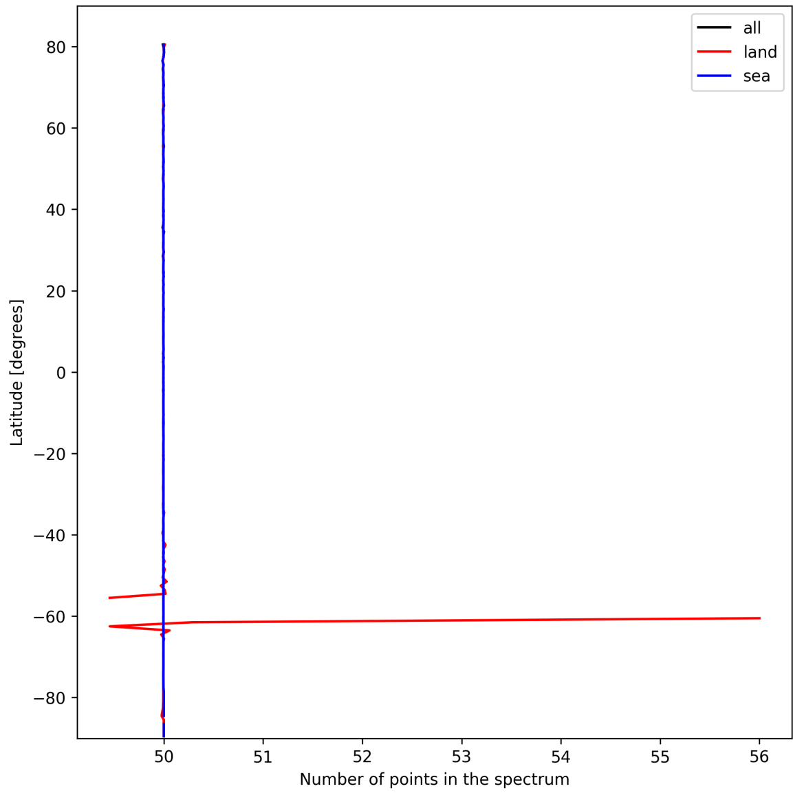
Figure 25: Zonal average of “Number of points in the spectrum” for 2025-10-12 to 2025-10-13.
