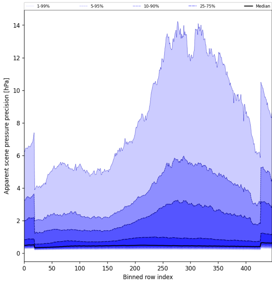
Figure 52: Along track statistics of “Apparent scene pressure precision” for 2025-10-12 to 2025-10-13
