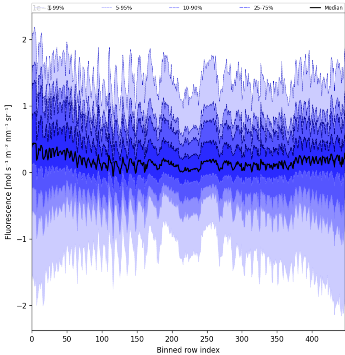
Figure 55: Along track statistics of "Fluorescence" for 2025-10-12 to 2025-10-13
