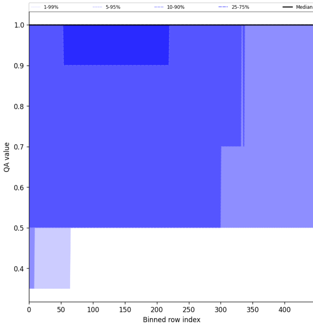
Figure 44: Along track statistics of “QA value” for 2025-10-12 to 2025-10-13
