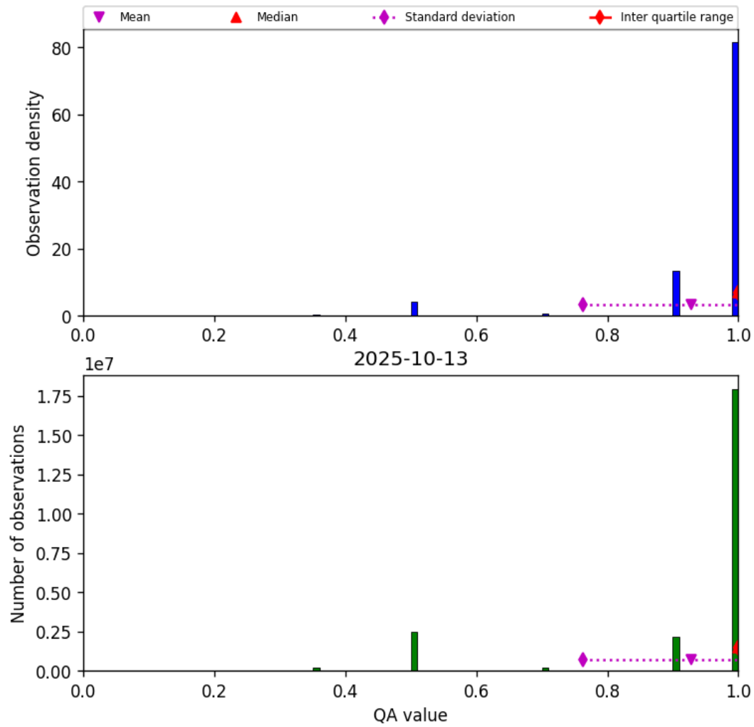
Figure 27: Histogram of “QA value” for 2025-10-13 to 2025-10-14
