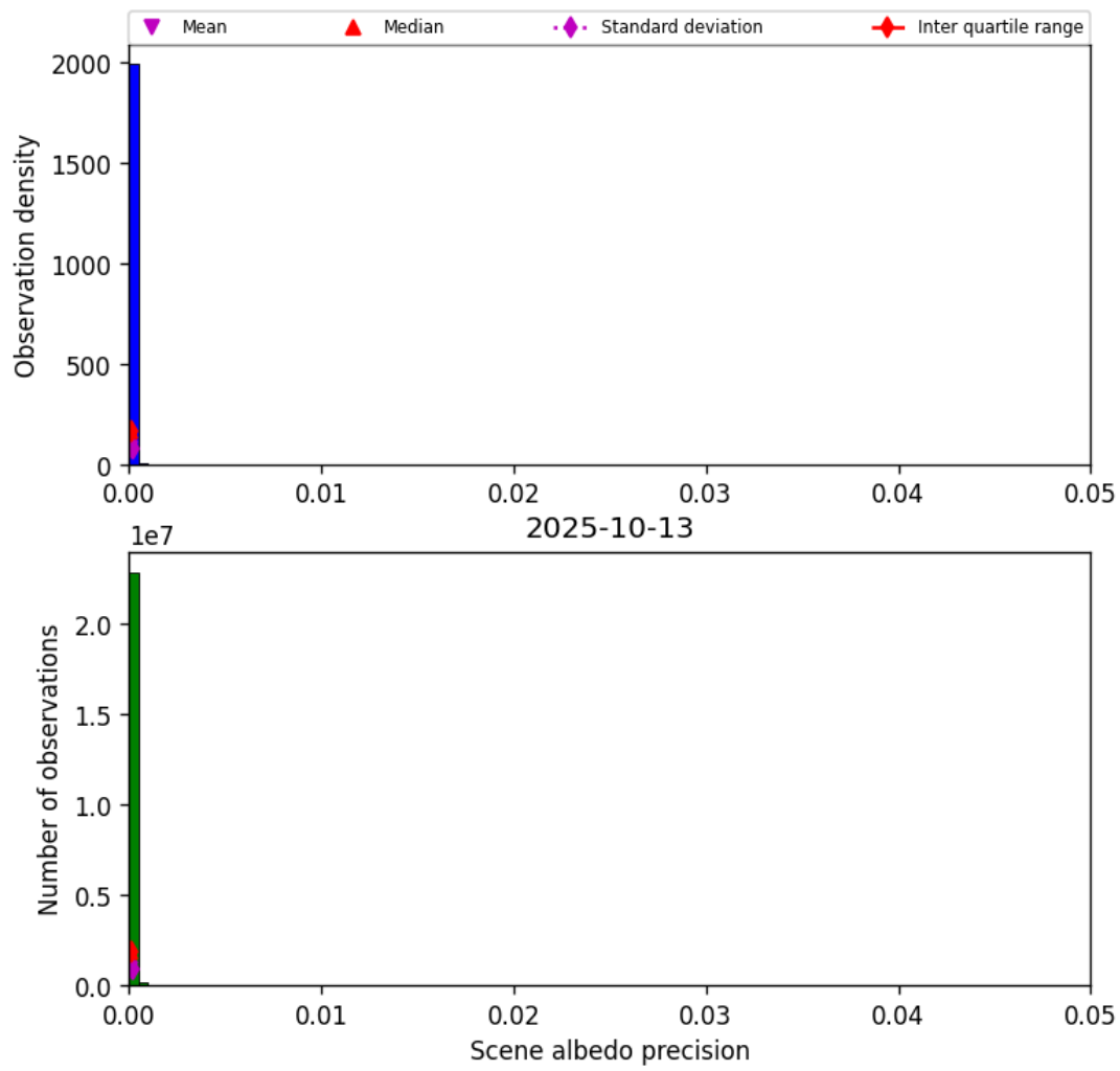
Figure 33: Histogram of “Scene albedo precision” for 2025-10-13 to 2025-10-14
