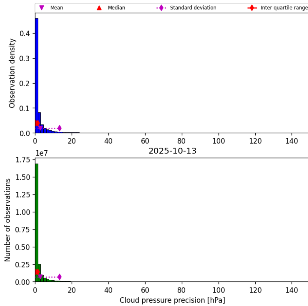
Figure 29: Histogram of “Cloud pressure precision” for 2025-10-13 to 2025-10-14
