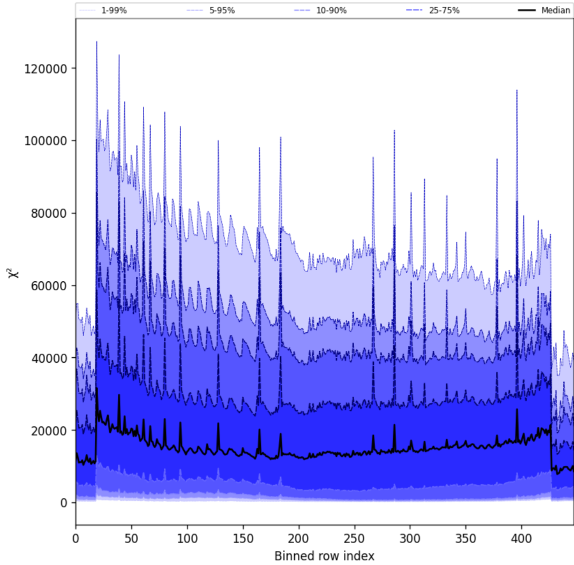
Figure 53: Along track statistics of “ \chi^2 ” for 2025-10-13 to 2025-10-14
