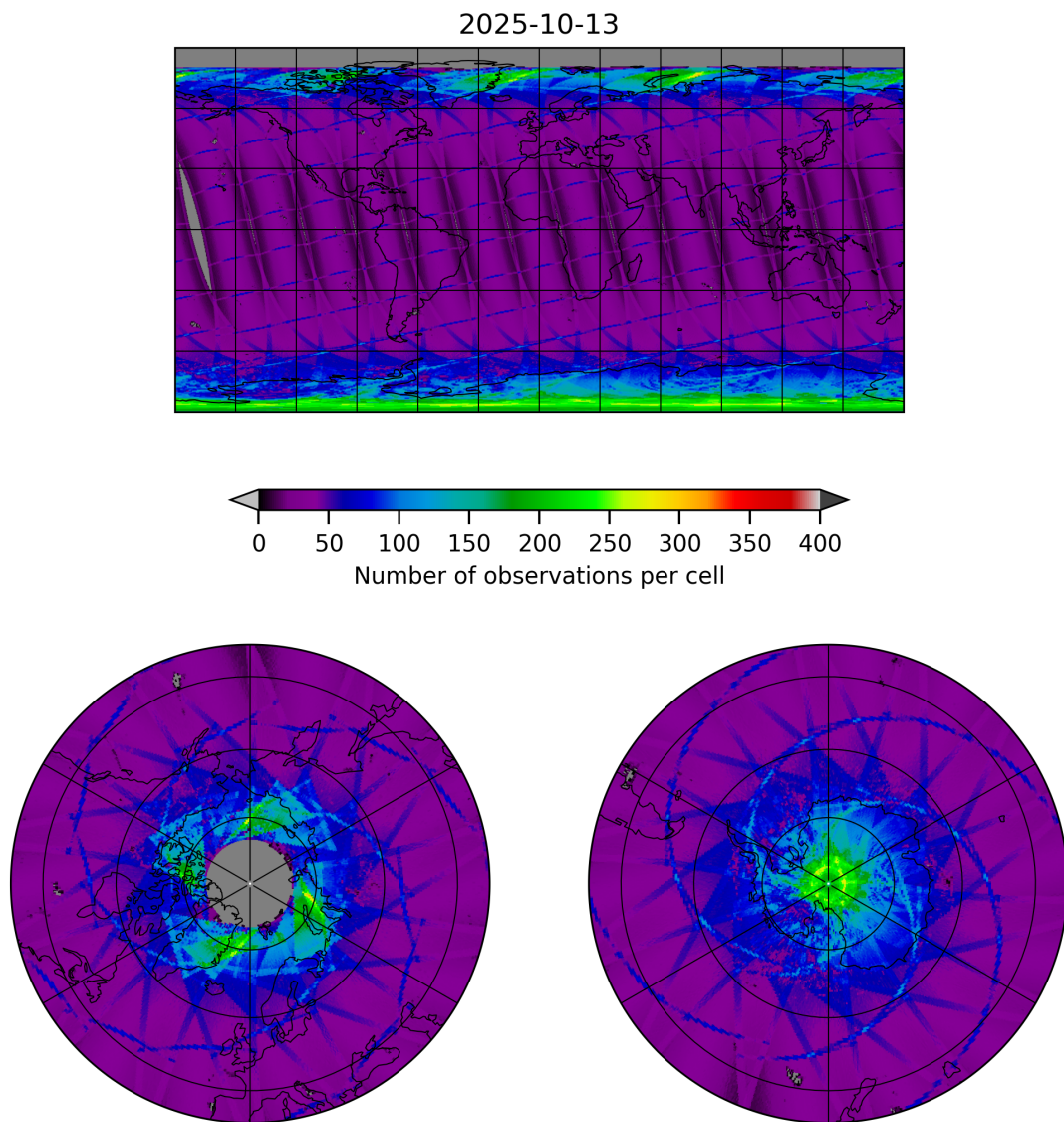
Figure 9: Map of the number of observations for 2025-10-13 to 2025-10-14
