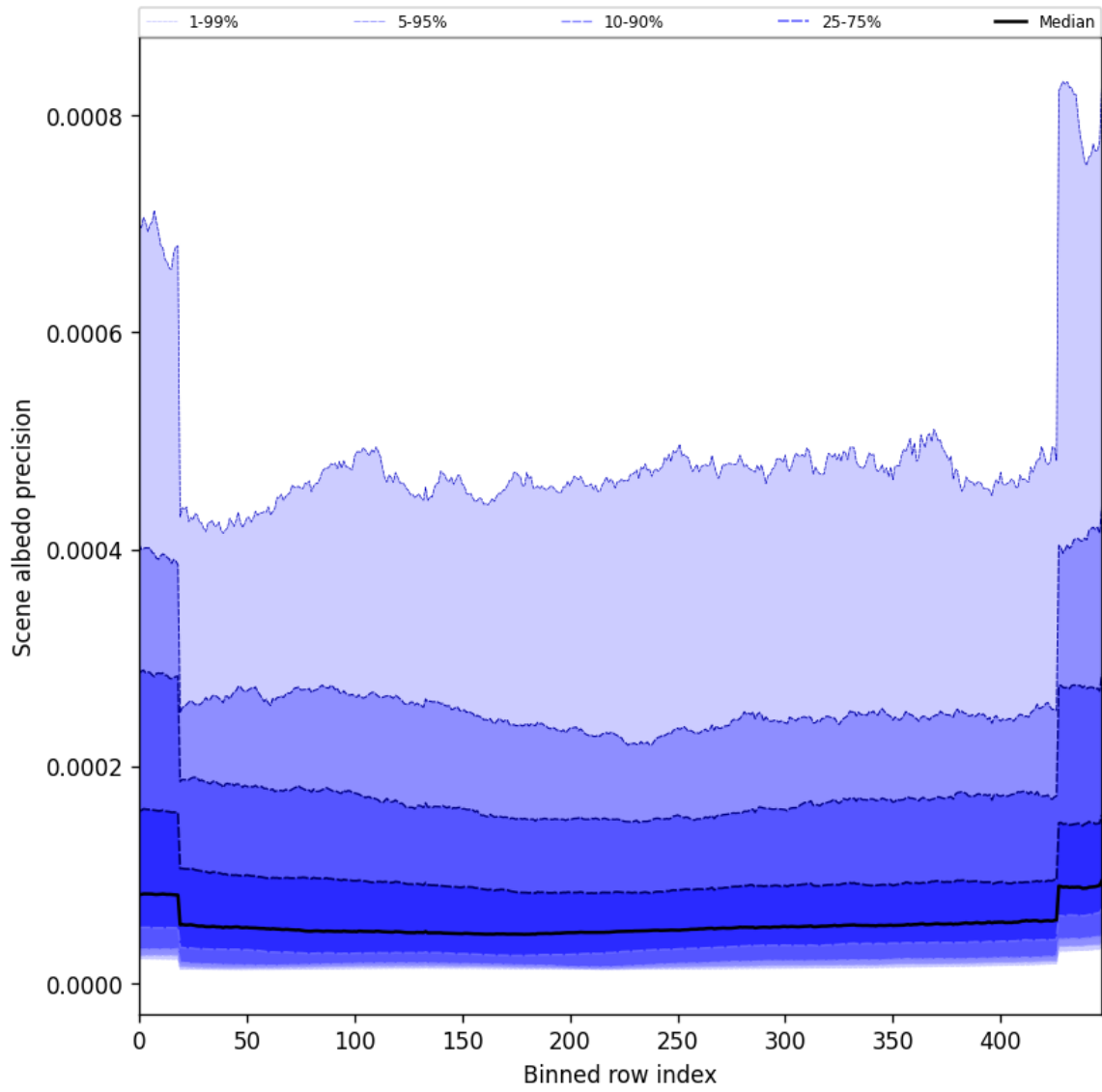
Figure 50: Along track statistics of “Scene albedo precision” for 2025-10-13 to 2025-10-14
