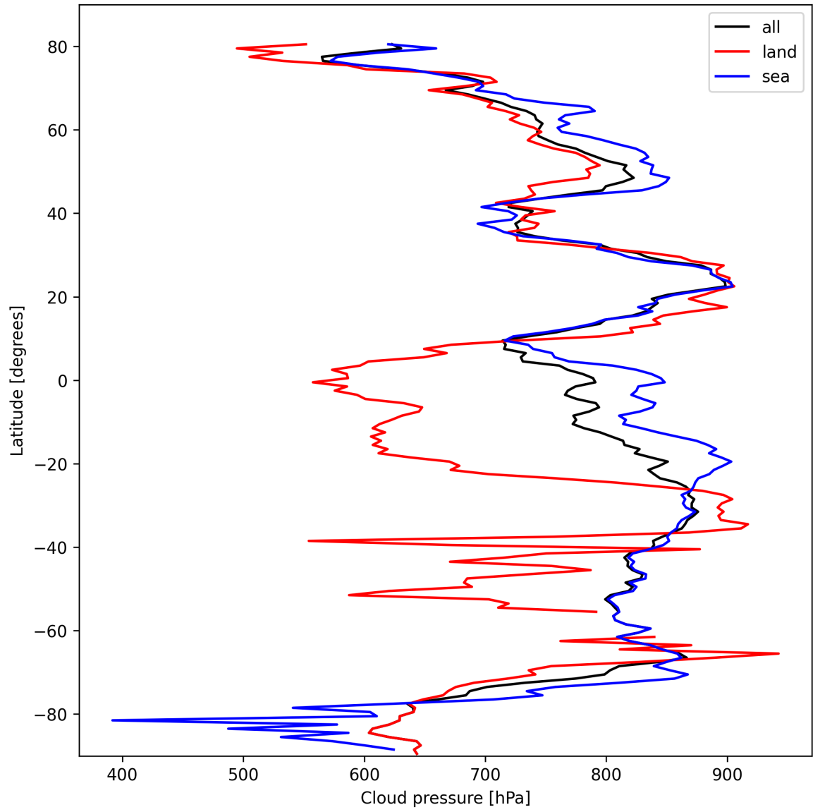
Figure 11: Zonal average of “Cloud pressure” for 2025-10-13 to 2025-10-14.
