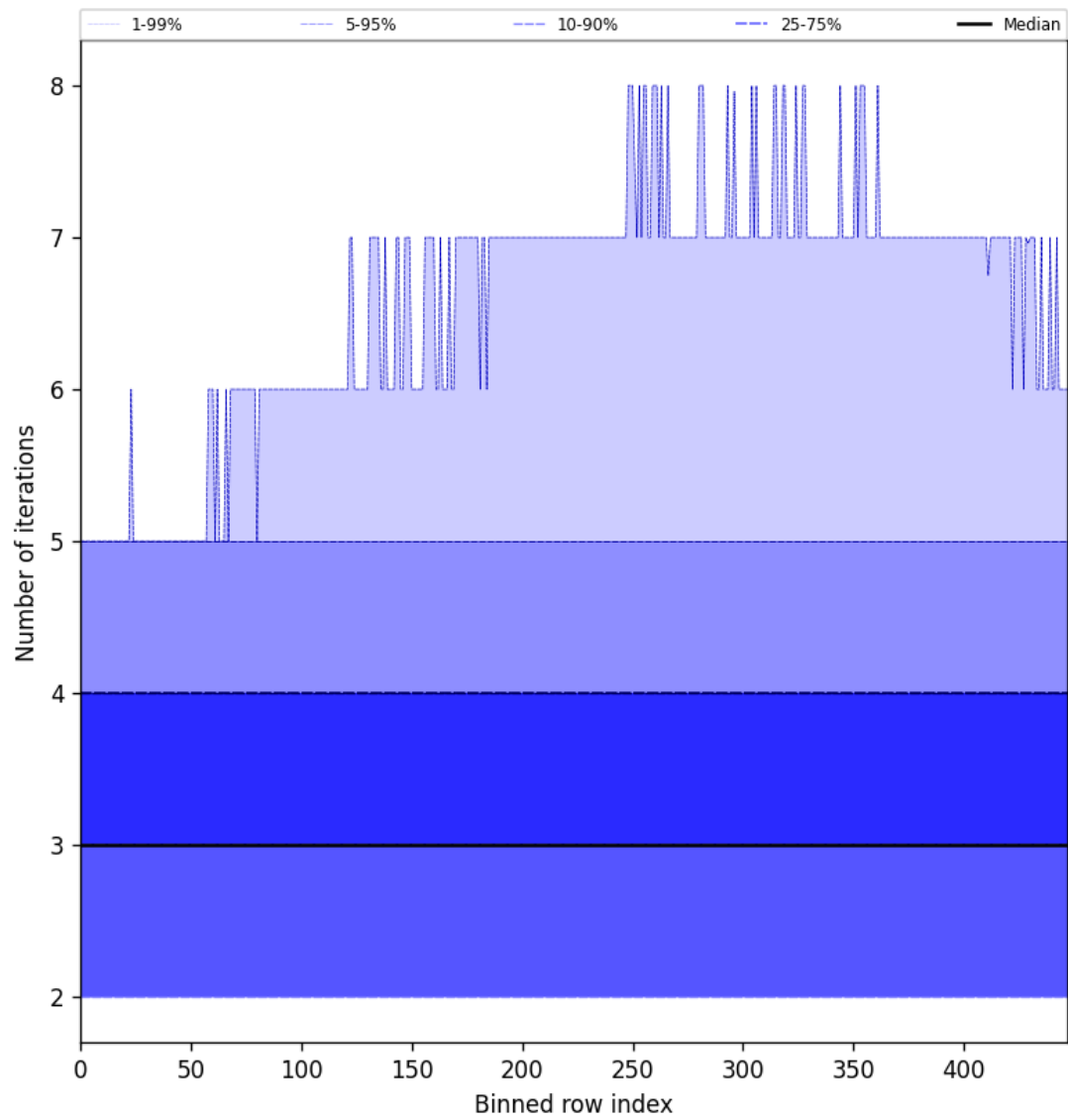
Figure 54: Along track statistics of “Number of iterations” for 2025-10-13 to 2025-10-14
