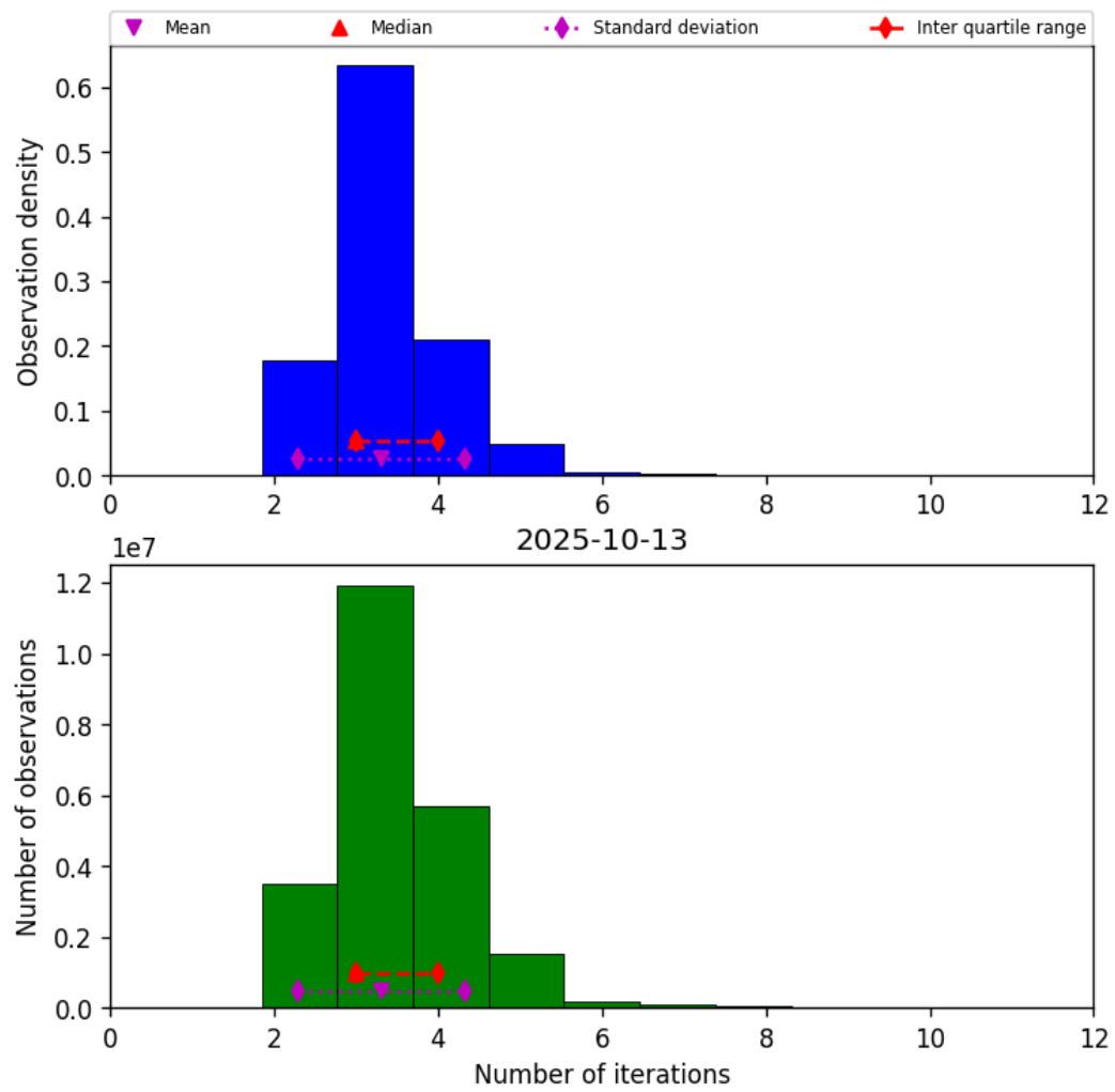
Figure 37: Histogram of “Number of iterations” for 2025-10-13 to 2025-10-14
