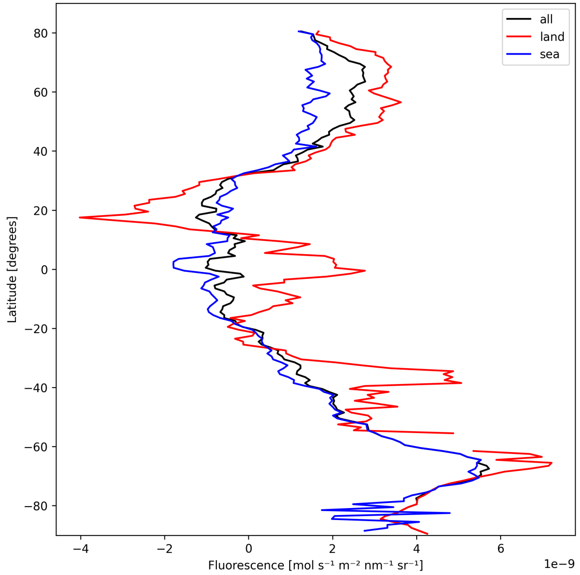
Figure 21: Zonal average of “Fluorescence” for 2025-10-13 to 2025-10-14.
