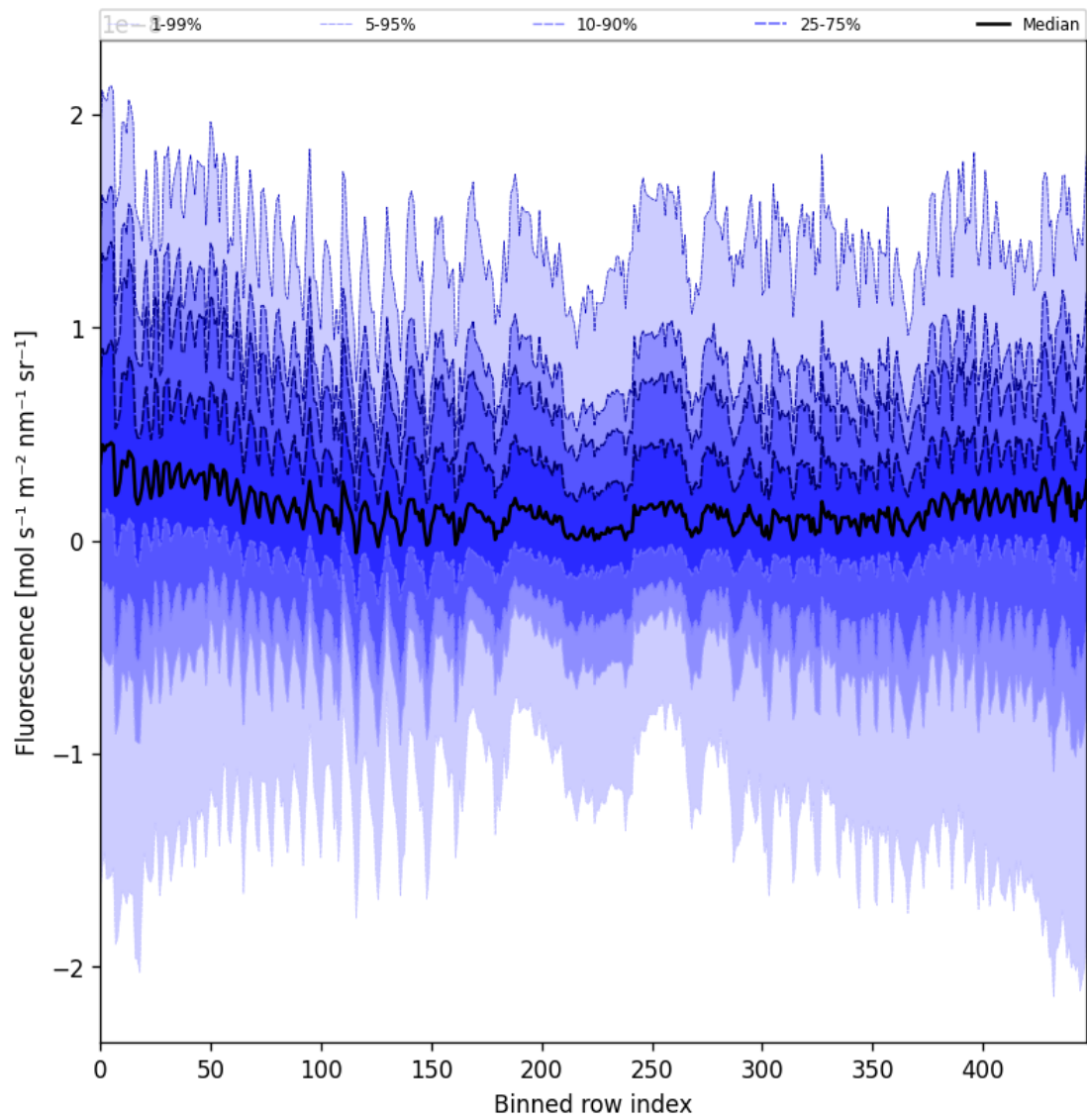
Figure 55: Along track statistics of “Fluorescence” for 2025-10-13 to 2025-10-14
