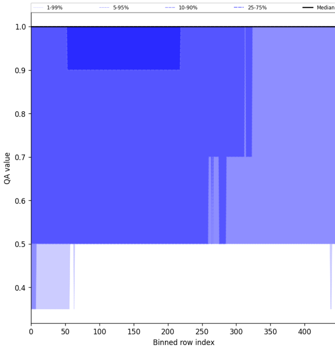
Figure 44: Along track statistics of “QA value” for 2025-10-13 to 2025-10-14
