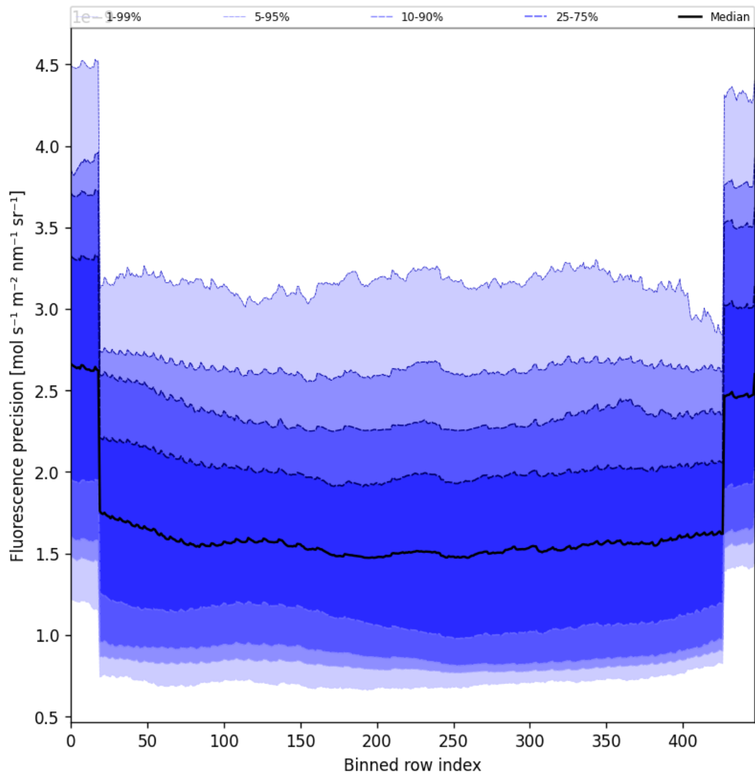
Figure 56: Along track statistics of “Fluorescence precision” for 2025-10-13 to 2025-10-14
