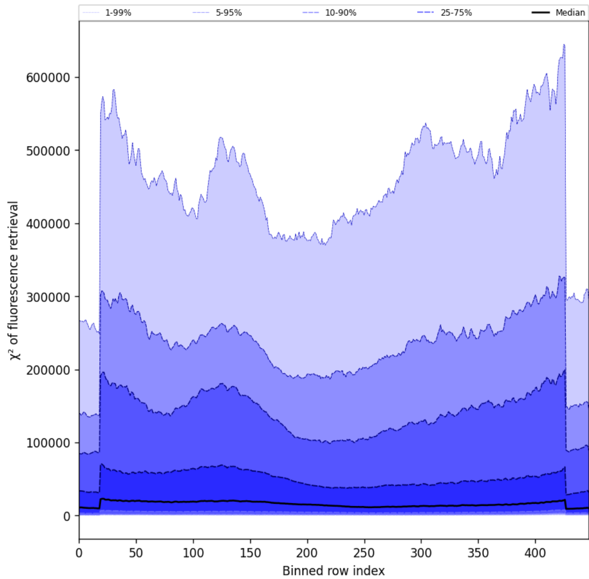
Figure 57: Along track statistics of “ \chi^2 of fluorescence retrieval” for 2025-10-13 to 2025-10-14
