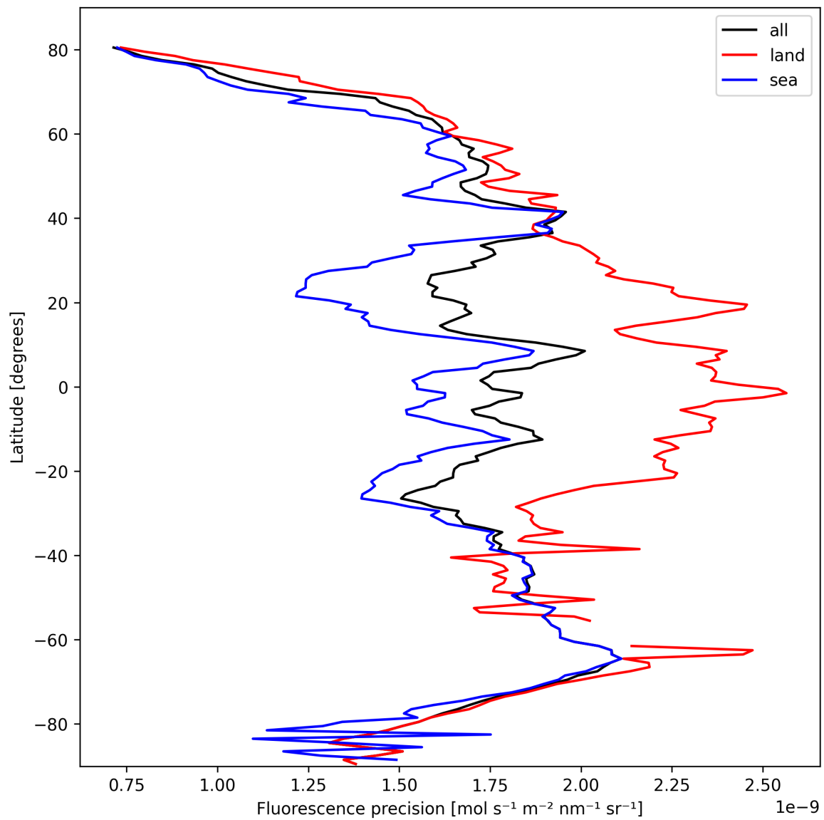
Figure 22: Zonal average of “Fluorescence precision” for 2025-10-13 to 2025-10-14.
