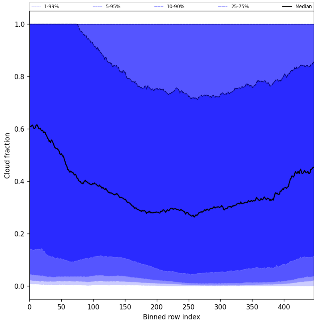
Figure 47: Along track statistics of “Cloud fraction” for 2025-10-13 to 2025-10-14
