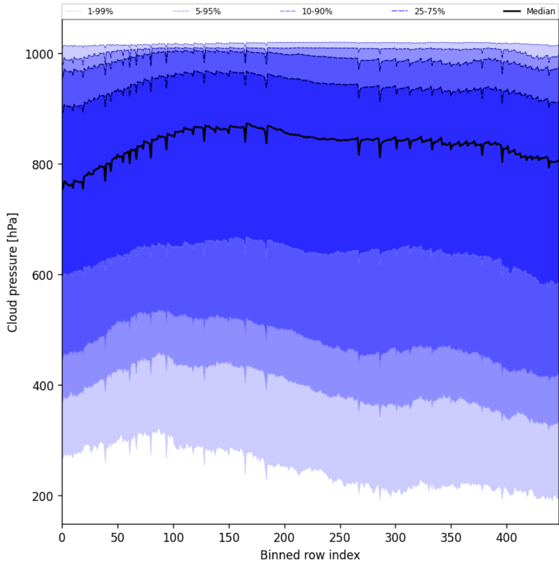
Figure 45: Along track statistics of “Cloud pressure” for 2025-10-13 to 2025-10-14
