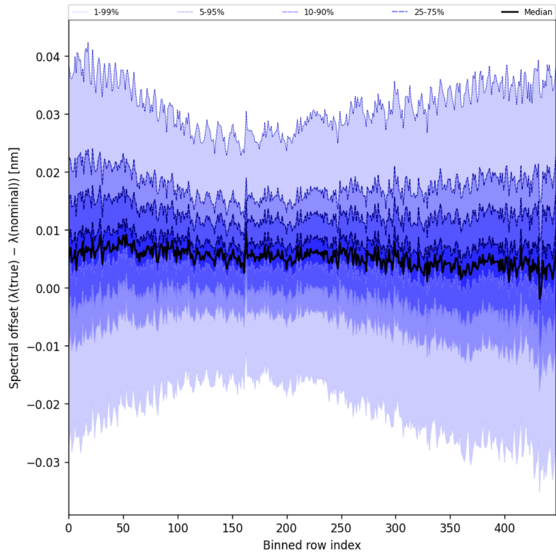
Figure 60: Along track statistics of “Spectral offset ( \lambda_{\text{true}} - \lambda_{\text{nominal}} )” for 2025-10-13 to 2025-10-14
