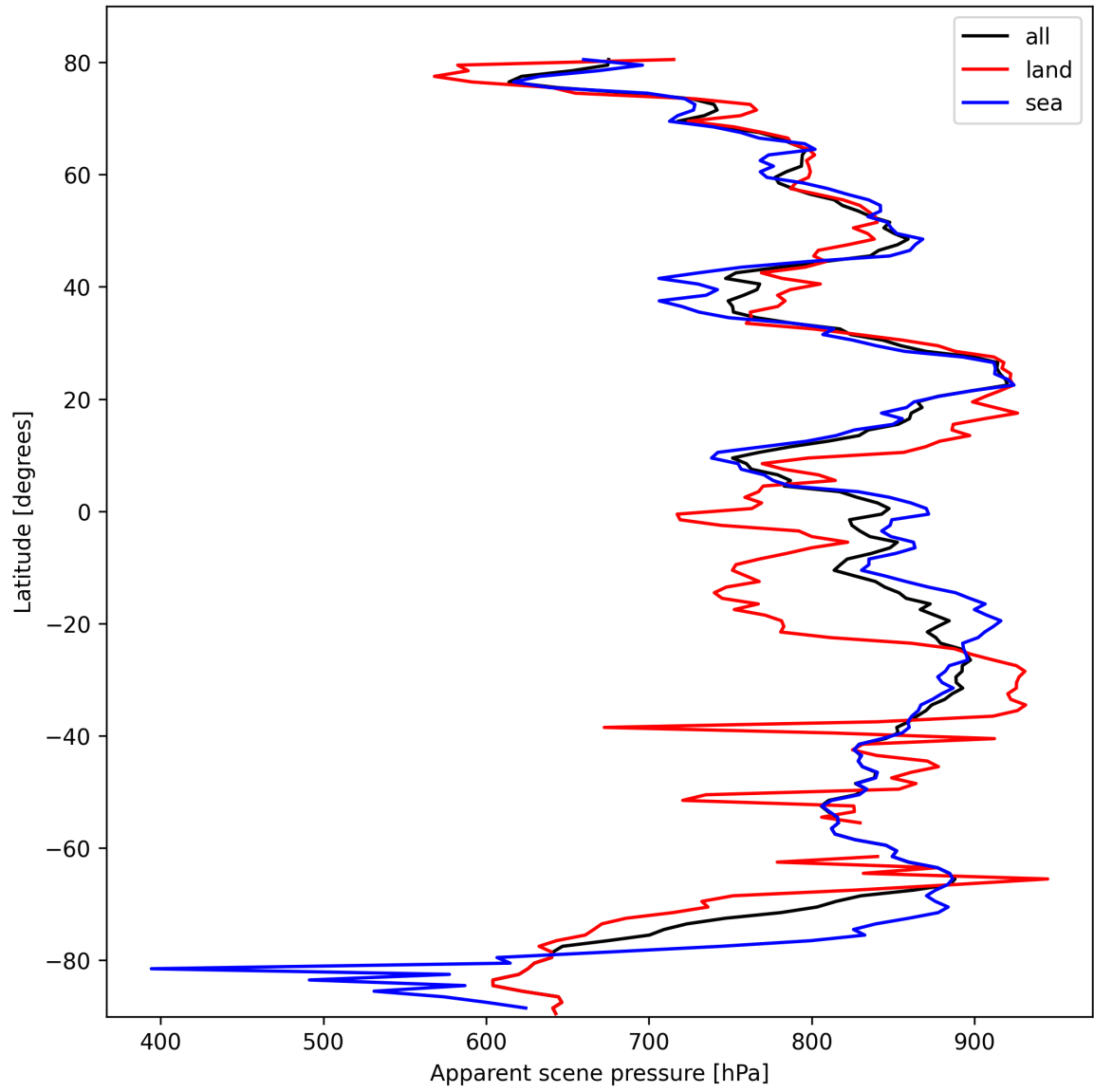
Figure 17: Zonal average of “Apparent scene pressure” for 2025-10-13 to 2025-10-14.
