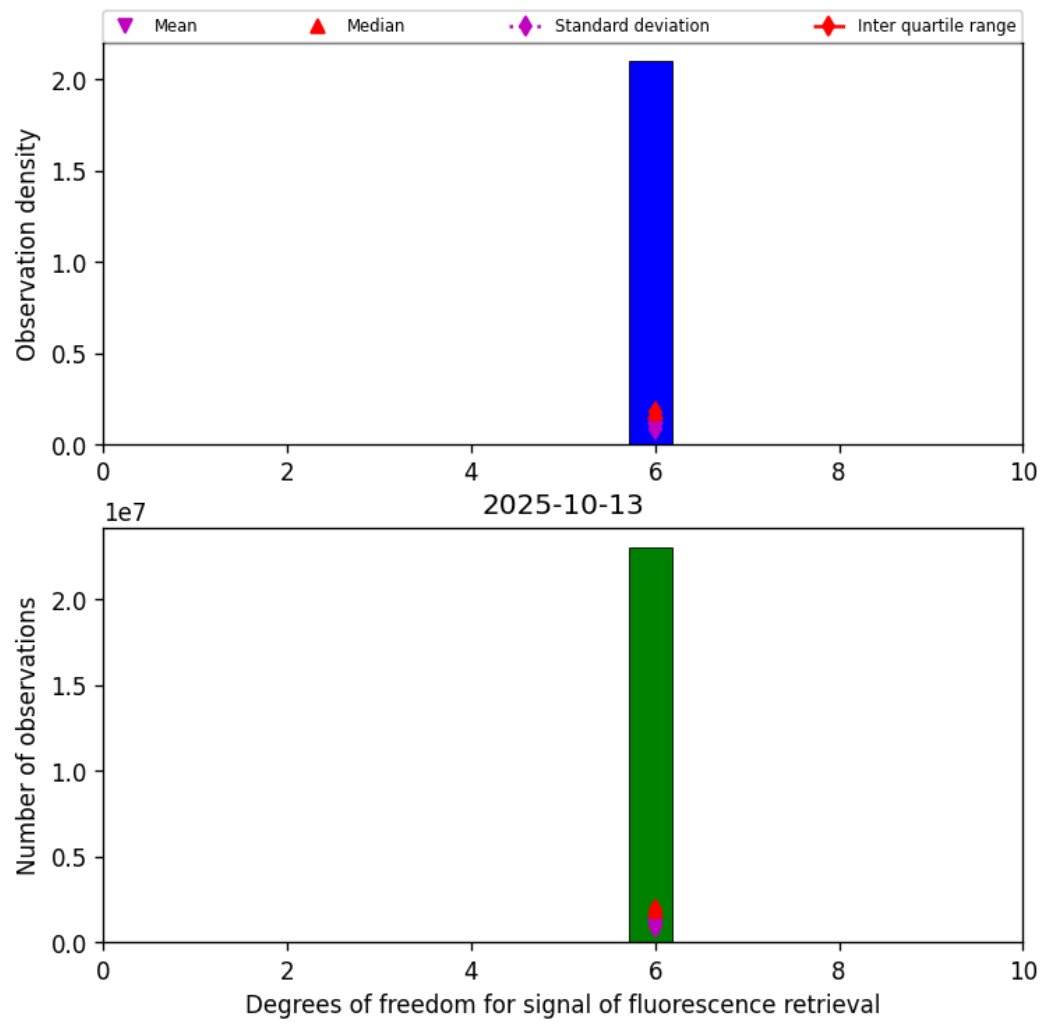
Figure 41: Histogram of “Degrees of freedom for signal of fluorescence retrieval” for 2025-10-13 to 2025-10-14
