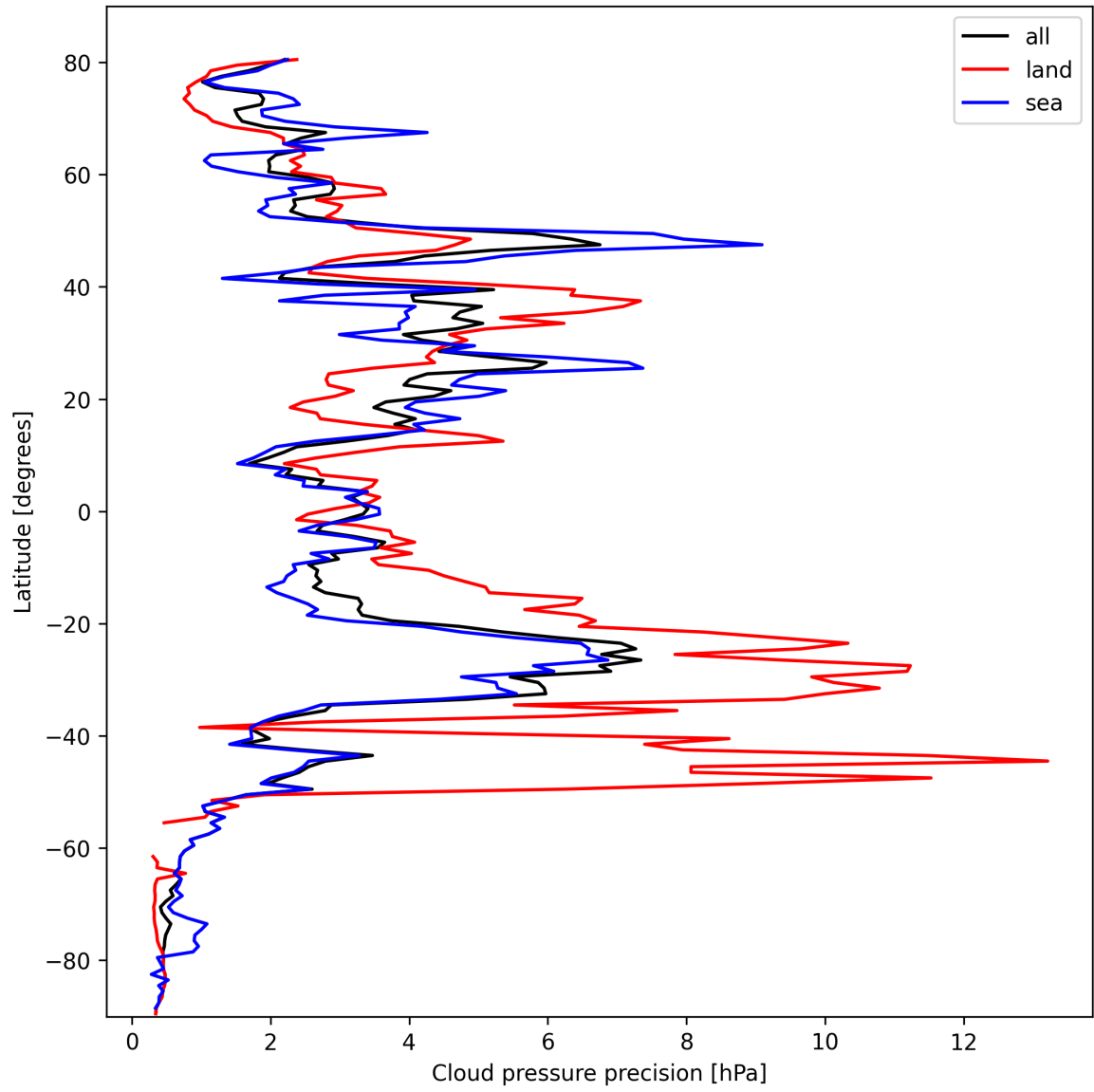
Figure 12: Zonal average of “Cloud pressure precision” for 2025-10-13 to 2025-10-14.
