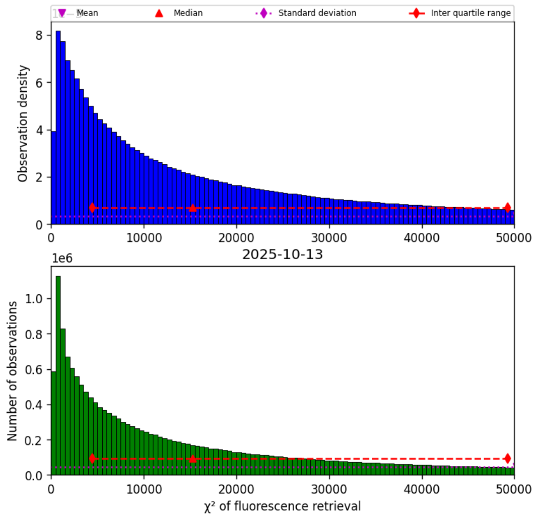
Figure 40: Histogram of “ \chi^2 of fluorescence retrieval” for 2025-10-13 to 2025-10-14
