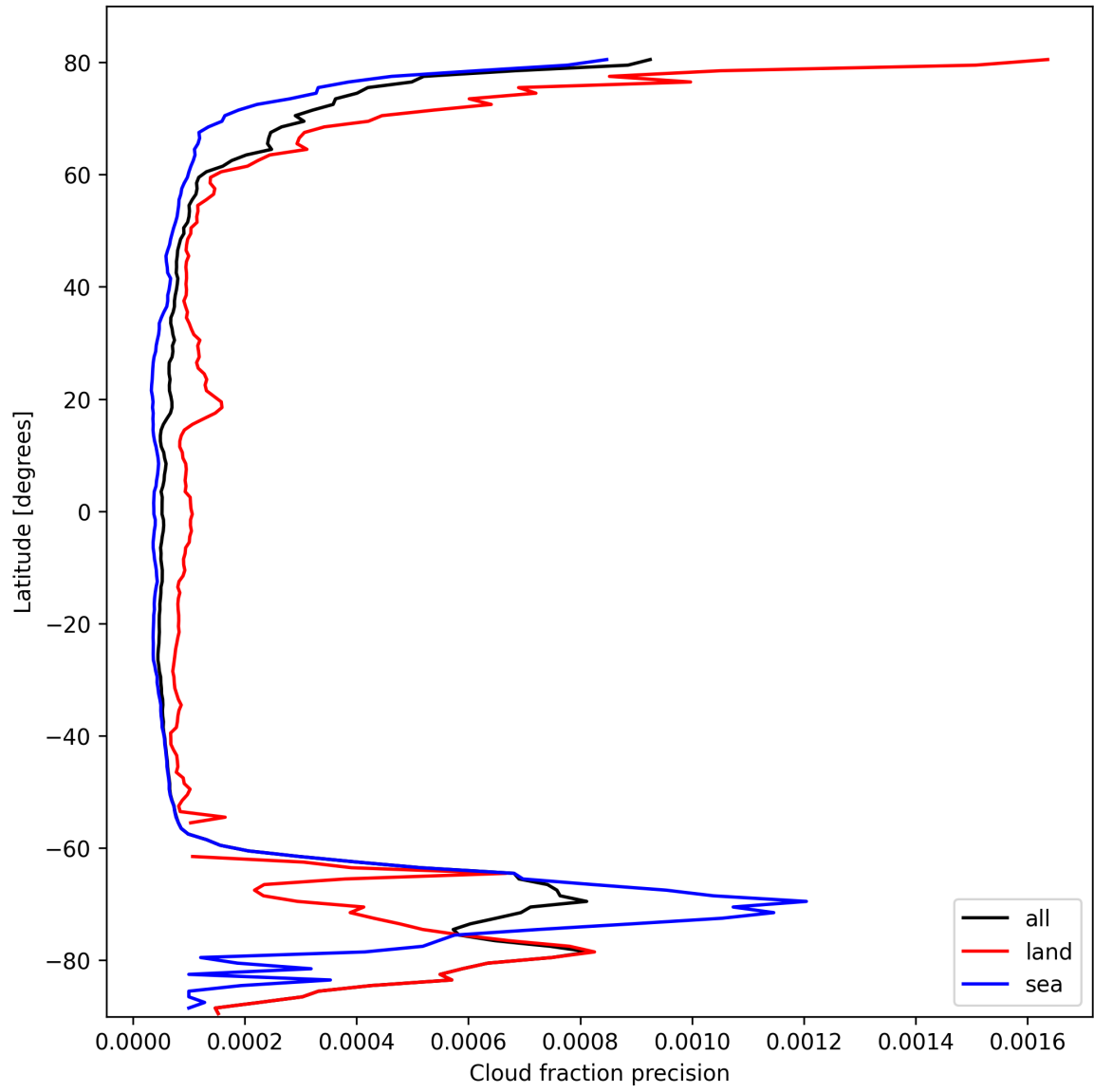
Figure 14: Zonal average of “Cloud fraction precision” for 2025-10-13 to 2025-10-14.
