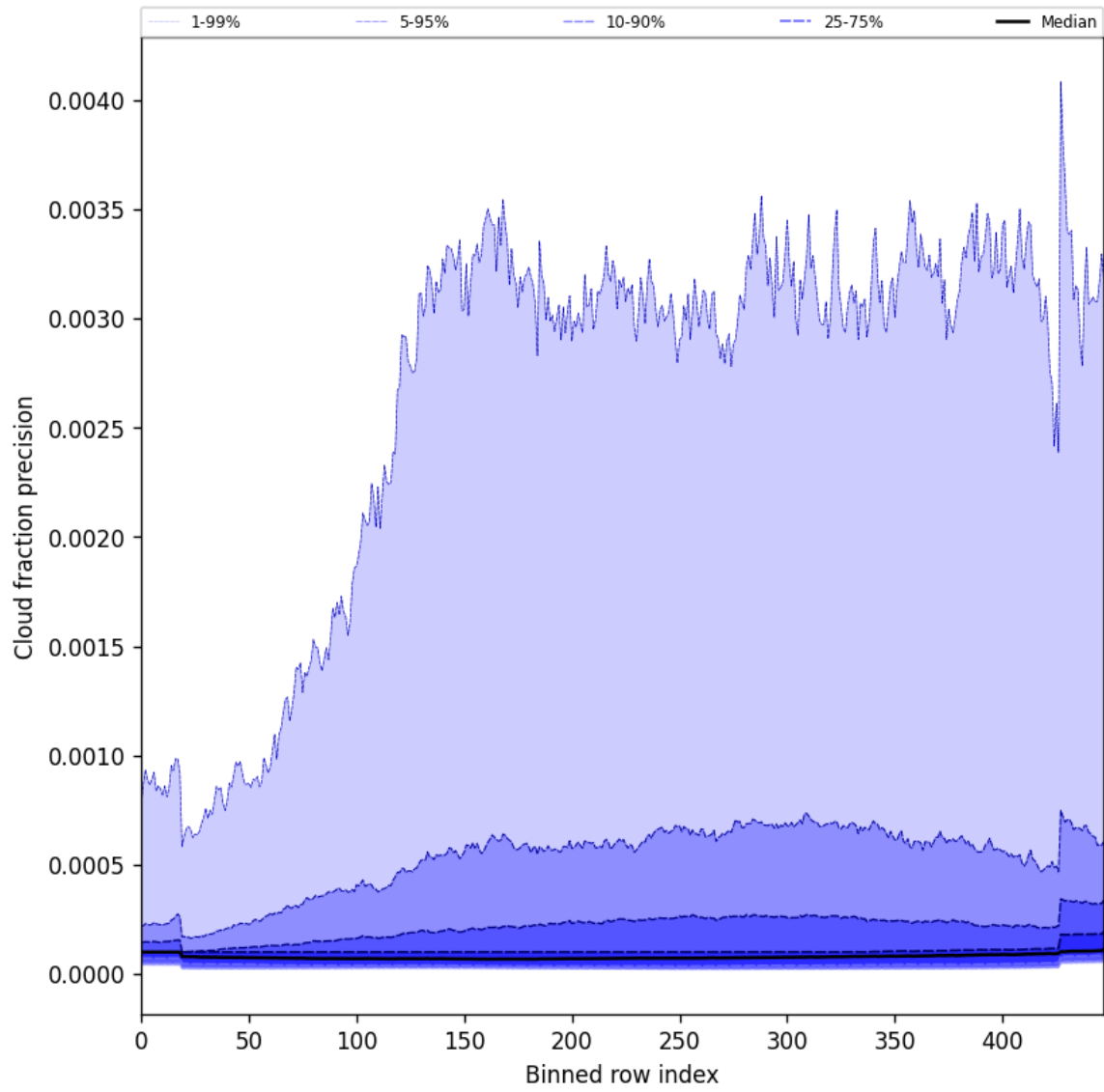
Figure 48: Along track statistics of “Cloud fraction precision” for 2025-10-13 to 2025-10-14
