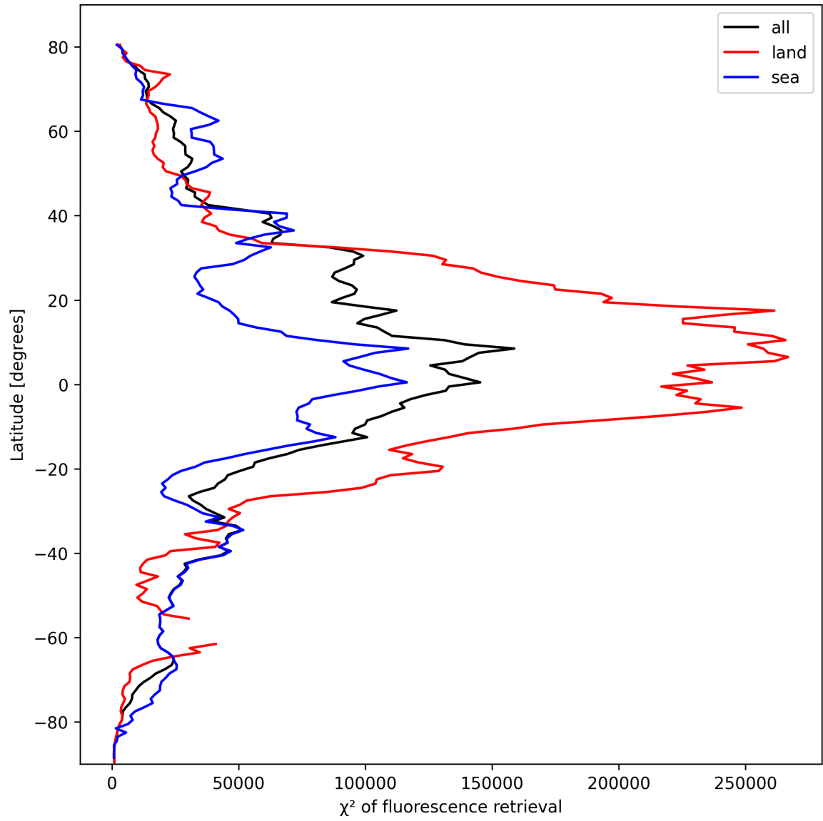
Figure 23: Zonal average of “ \chi^2 of fluorescence retrieval” for 2025-10-13 to 2025-10-14.
