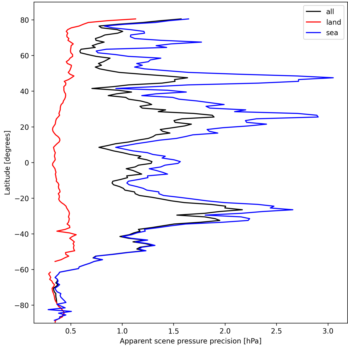
Figure 18: Zonal average of “Apparent scene pressure precision” for 2025-10-13 to 2025-10-14.
