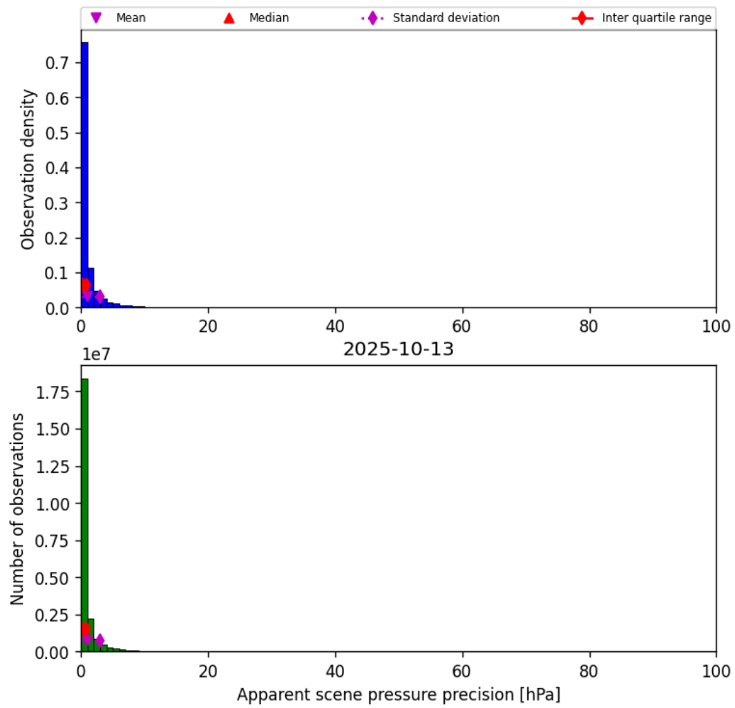
Figure 35: Histogram of “Apparent scene pressure precision” for 2025-10-13 to 2025-10-14
