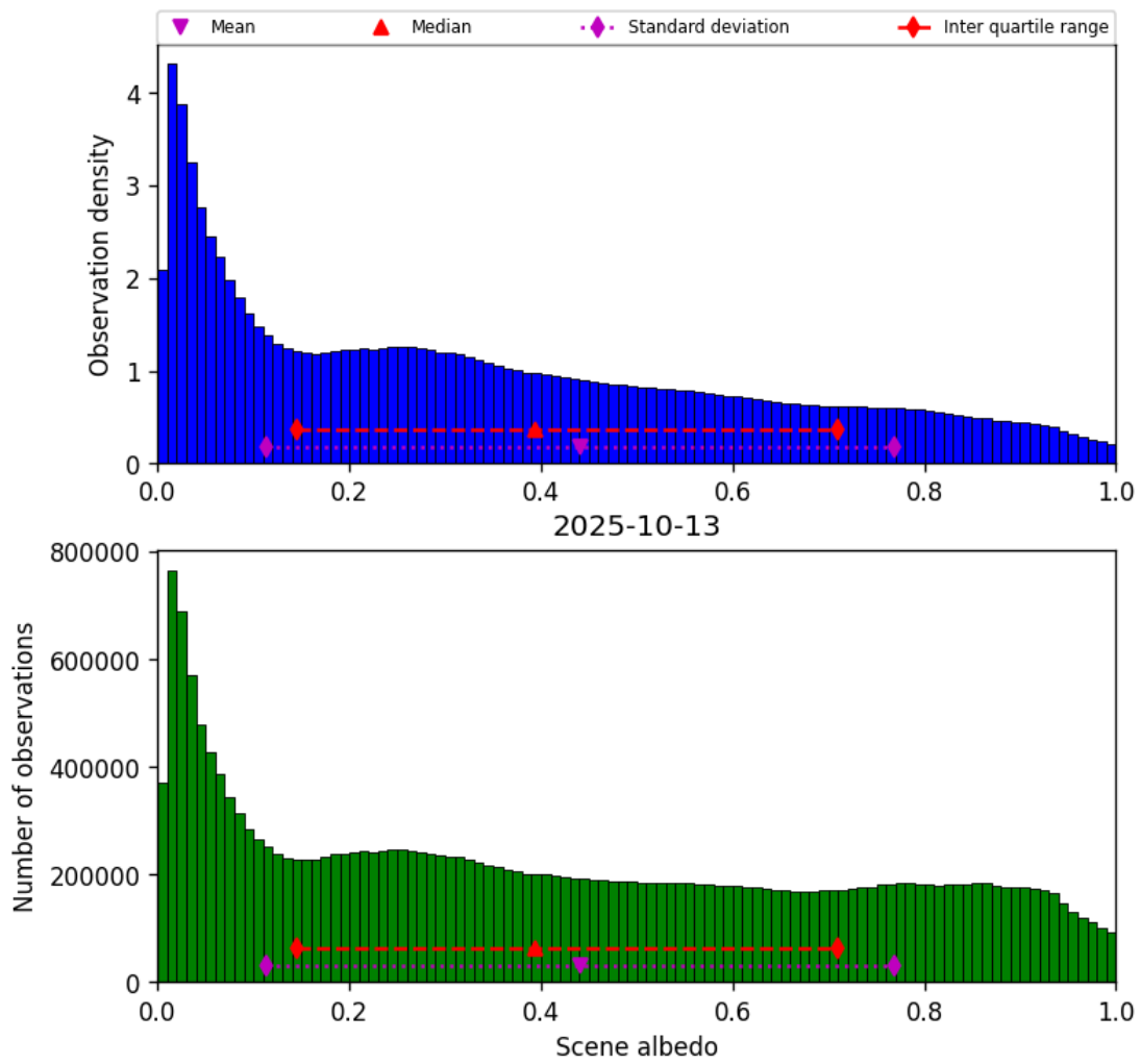
Figure 32: Histogram of “Scene albedo” for 2025-10-13 to 2025-10-14
