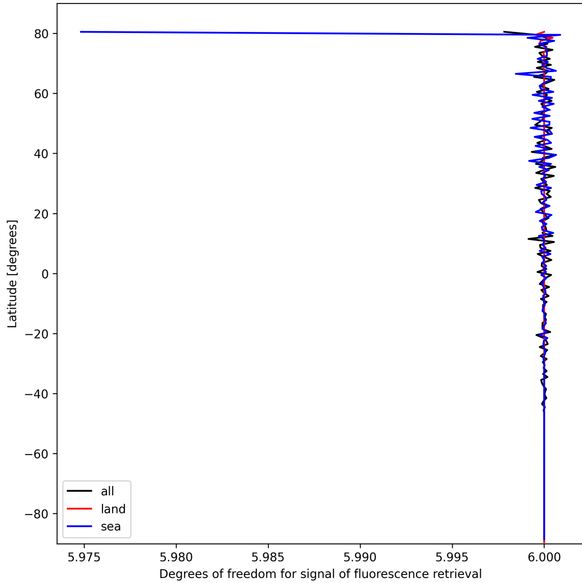
Figure 24: Zonal average of “Degrees of freedom for signal of fluorescence retrieval” for 2025-10-13 to 2025-10-14.
