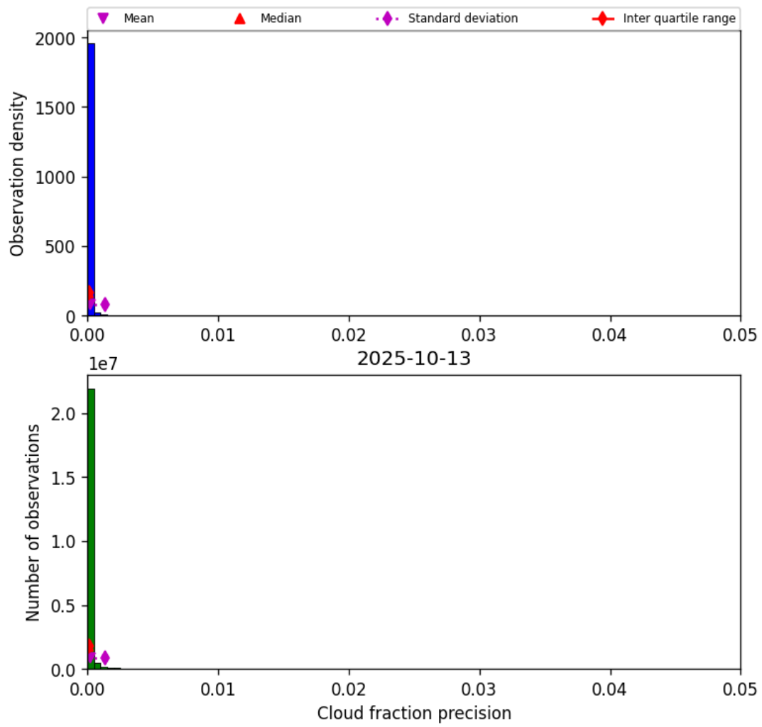
Figure 31: Histogram of “Cloud fraction precision” for 2025-10-13 to 2025-10-14
