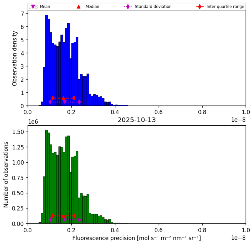
Figure 39: Histogram of “Fluorescence precision” for 2025-10-13 to 2025-10-14
