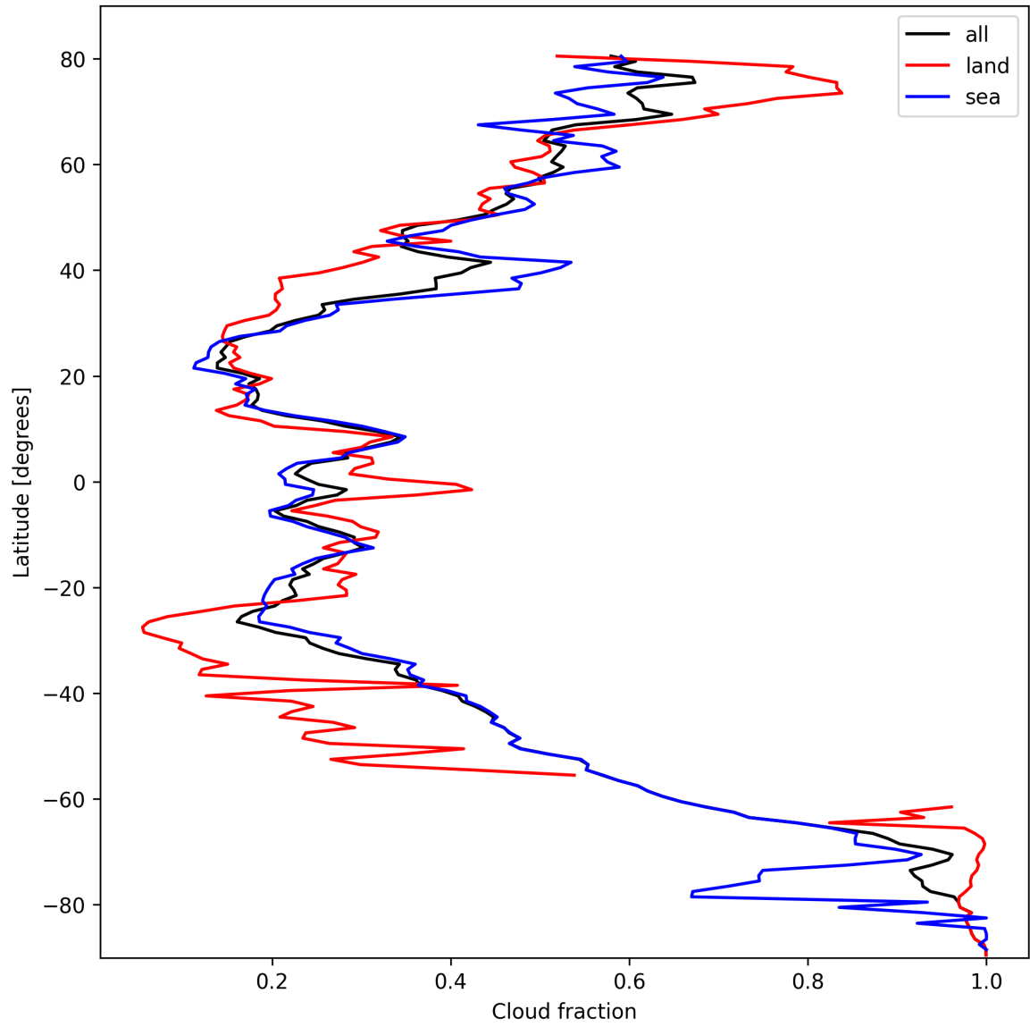
Figure 13: Zonal average of “Cloud fraction” for 2025-10-13 to 2025-10-14.
