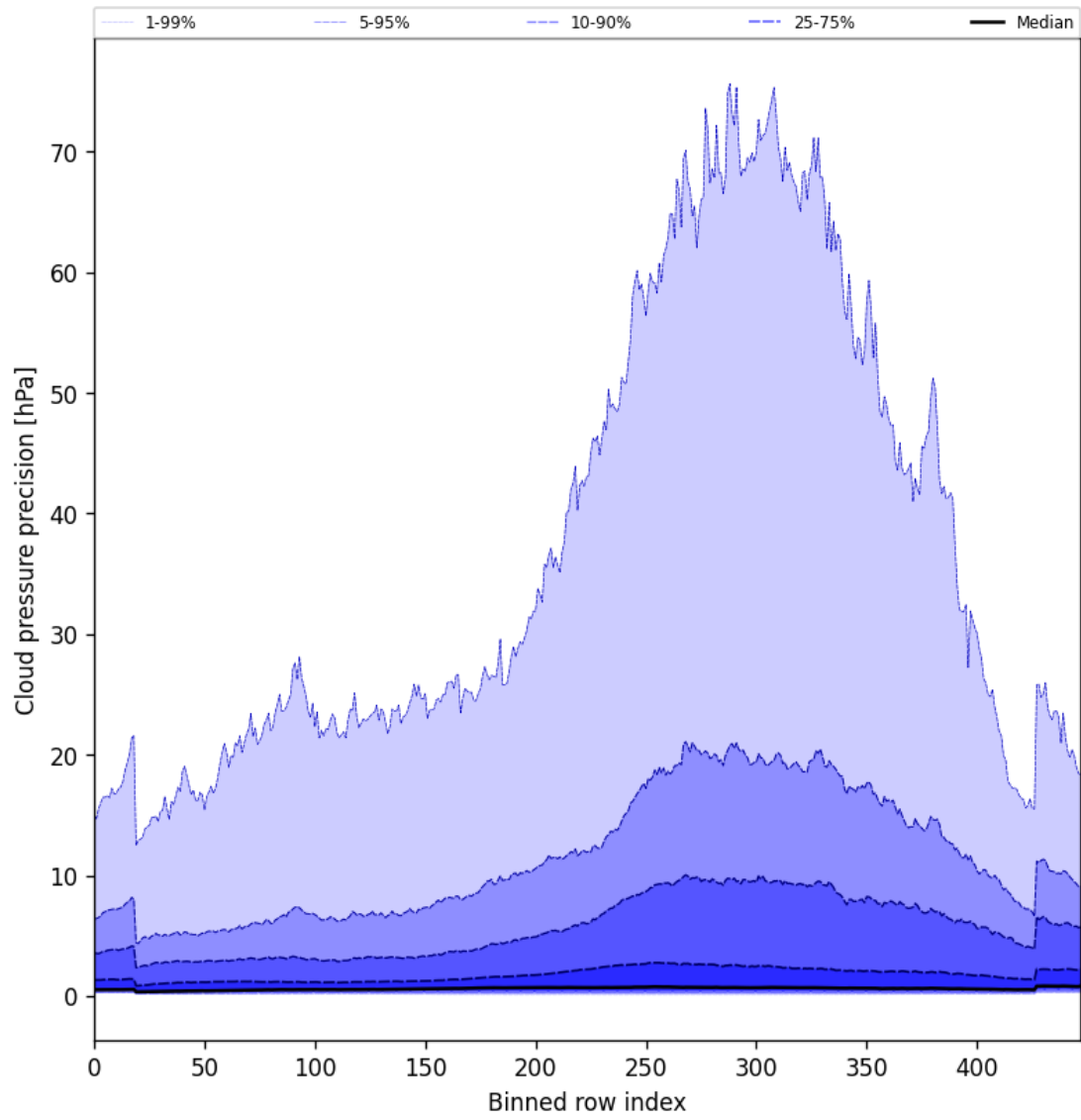
Figure 46: Along track statistics of “Cloud pressure precision” for 2025-10-13 to 2025-10-14
