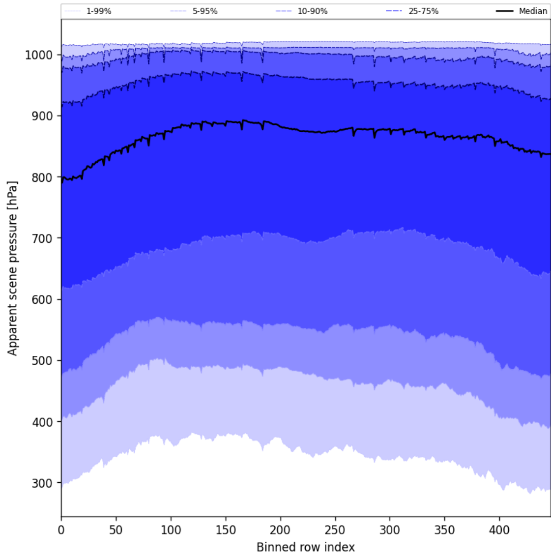
Figure 51: Along track statistics of “Apparent scene pressure” for 2025-10-13 to 2025-10-14
