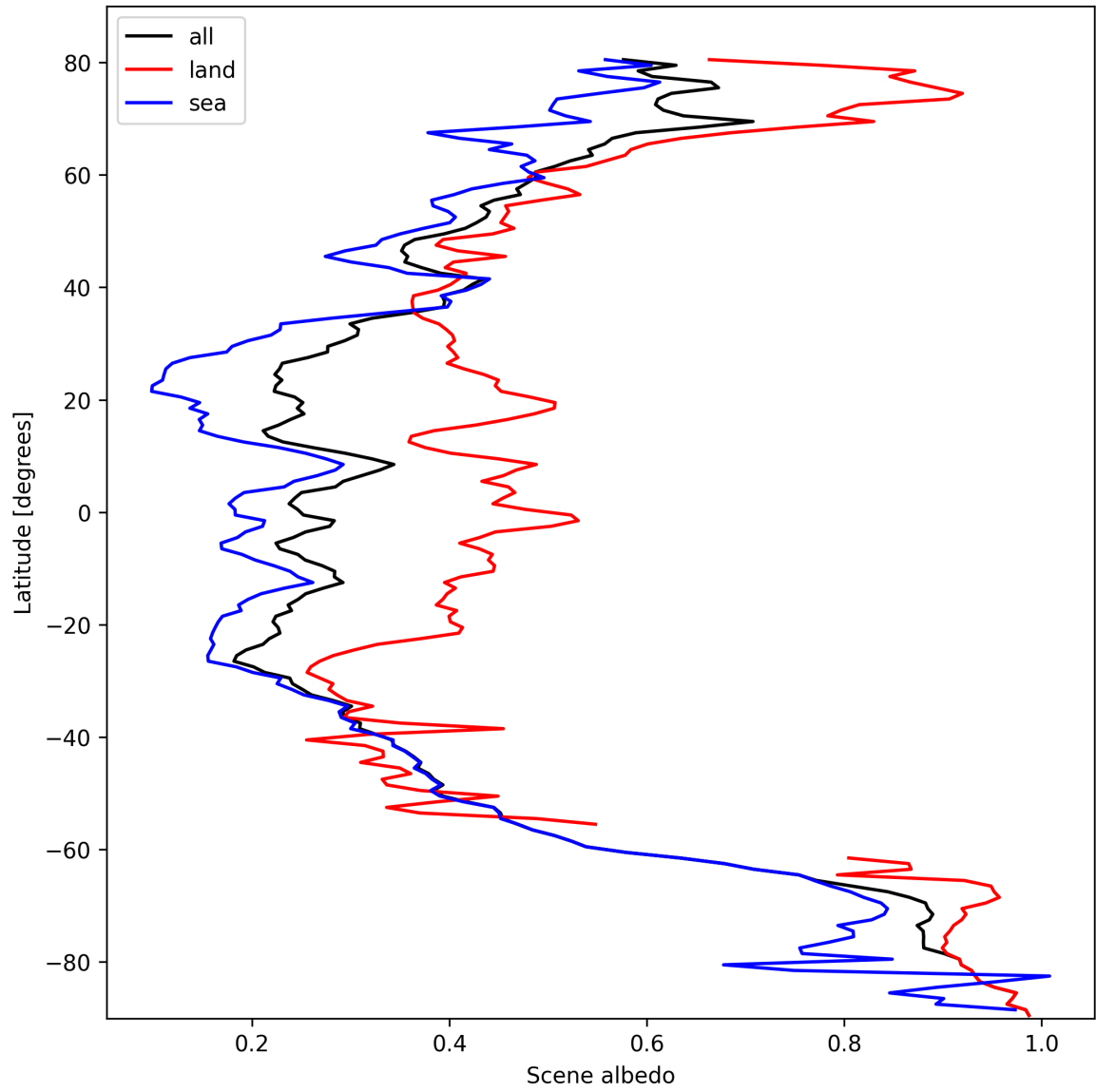
Figure 15: Zonal average of “Scene albedo” for 2025-10-13 to 2025-10-14.
