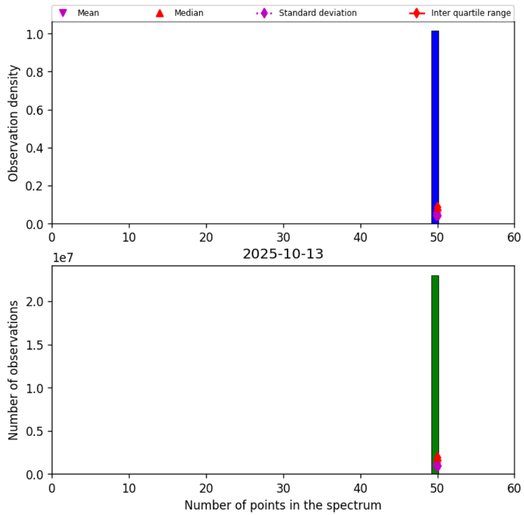
Figure 42: Histogram of “Number of points in the spectrum” for 2025-10-13 to 2025-10-14
