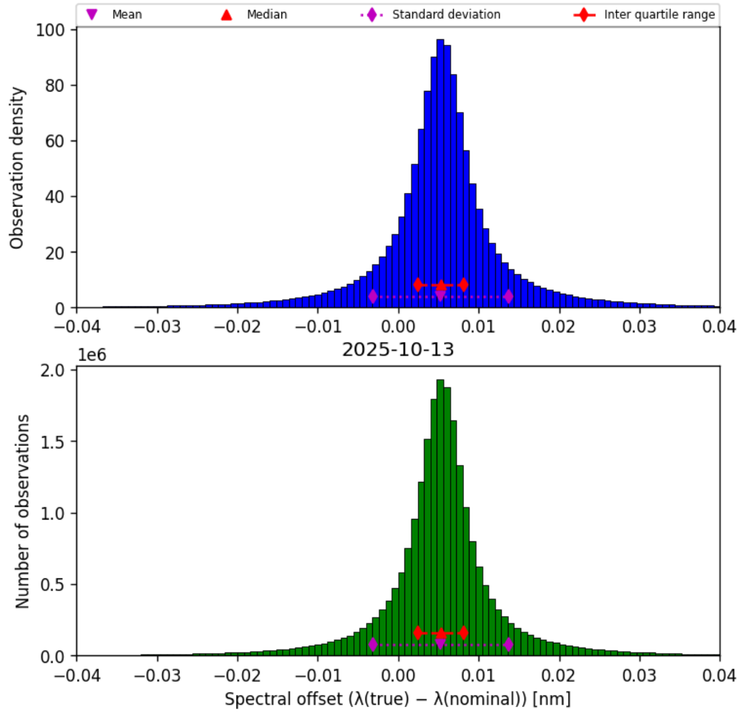
Figure 43: Histogram of “Spectral offset ( \lambda_{\text{true}} - \lambda_{\text{nominal}} )” for 2025-10-13 to 2025-10-14
