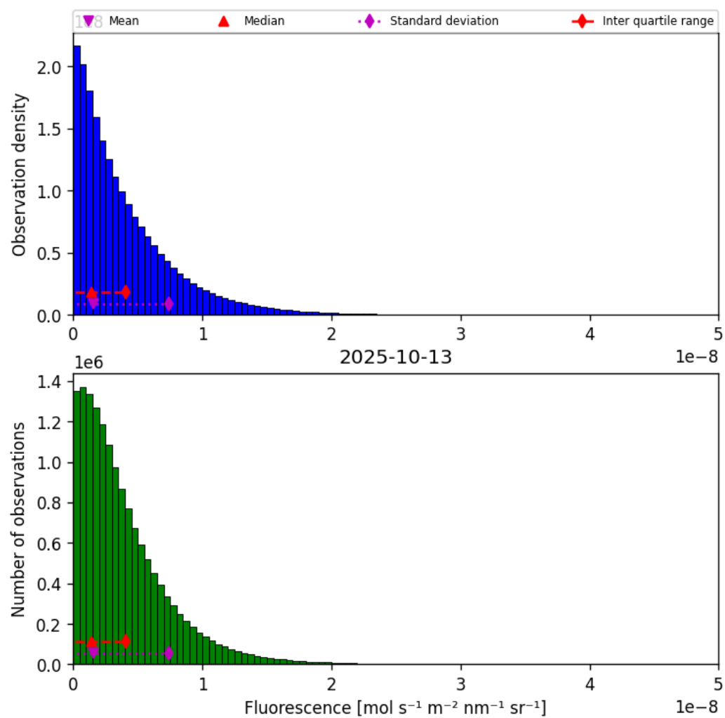
Figure 38: Histogram of “Fluorescence” for 2025-10-13 to 2025-10-14
