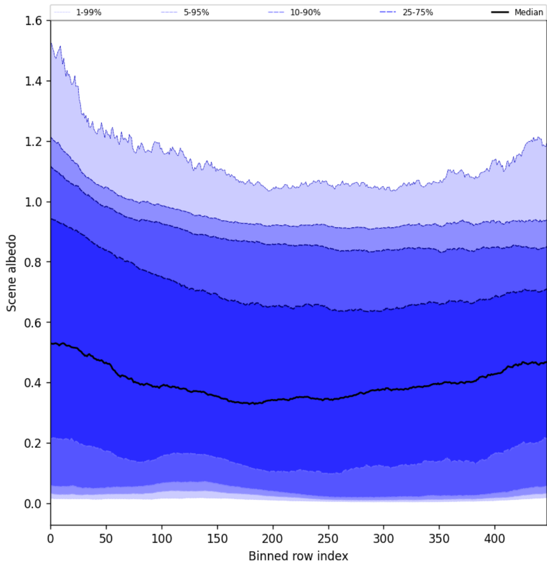
Figure 49: Along track statistics of “Scene albedo” for 2025-10-13 to 2025-10-14
