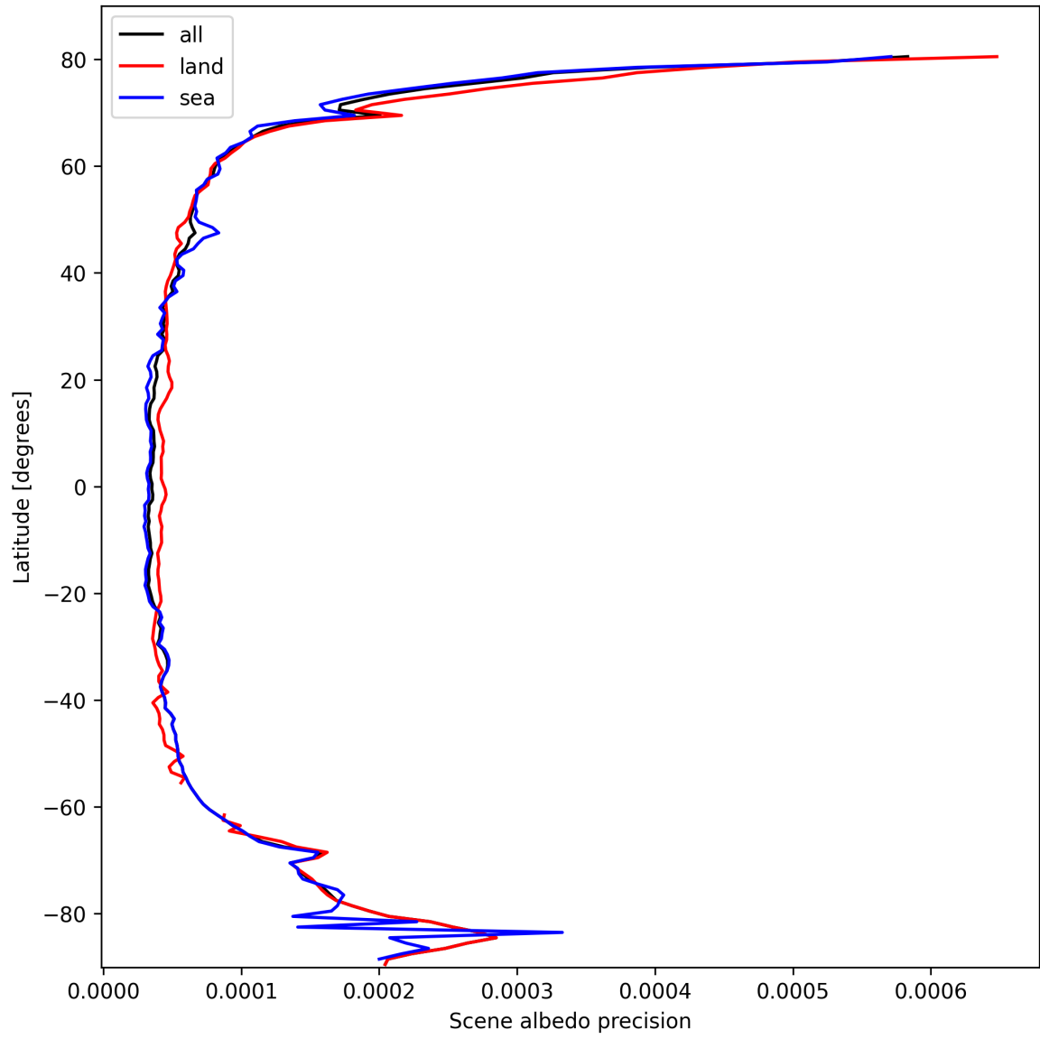
Figure 16: Zonal average of “Scene albedo precision” for 2025-10-13 to 2025-10-14.
