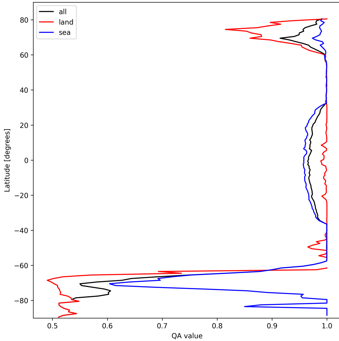
Figure 10: Zonal average of “QA value” for 2025-10-13 to 2025-10-14.
