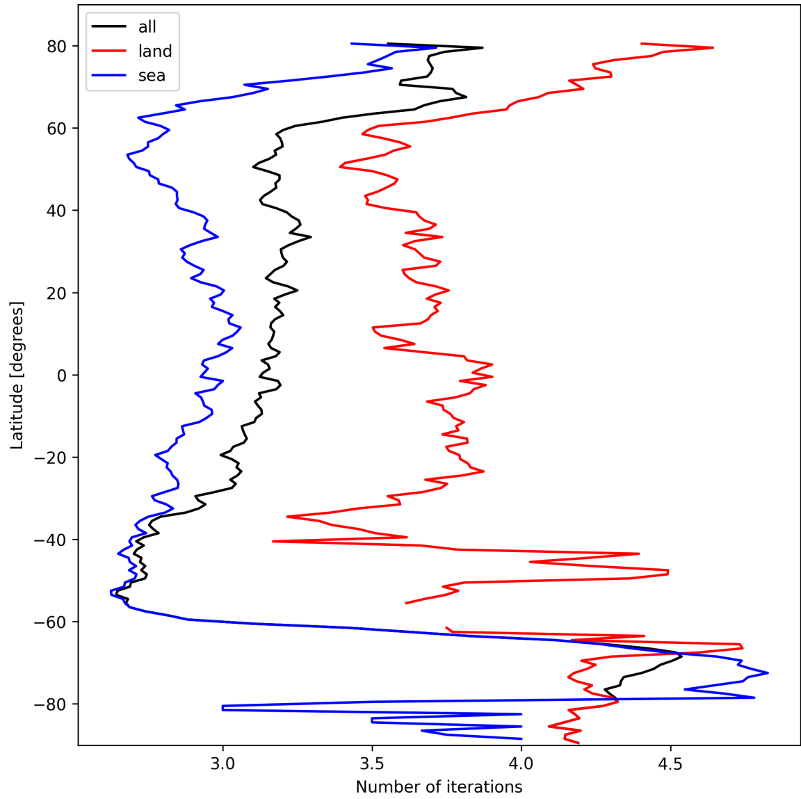
Figure 20: Zonal average of “Number of iterations” for 2025-10-13 to 2025-10-14.
