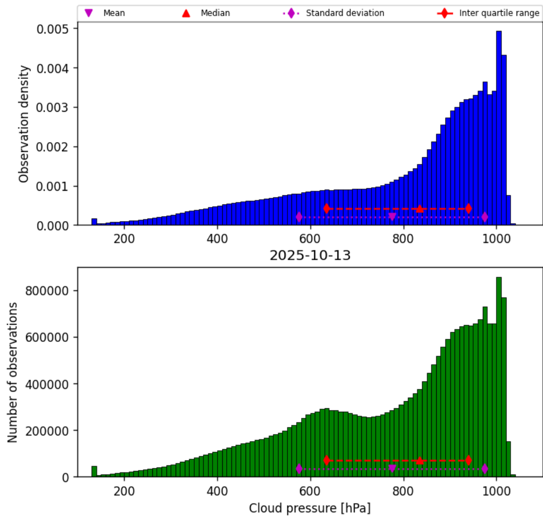
Figure 28: Histogram of “Cloud pressure” for 2025-10-13 to 2025-10-14
