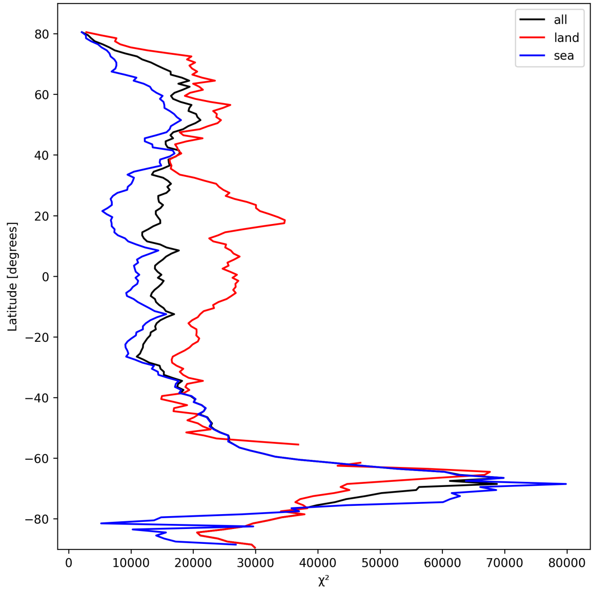
Figure 19: Zonal average of “ \chi^2 ” for 2025-10-13 to 2025-10-14.
