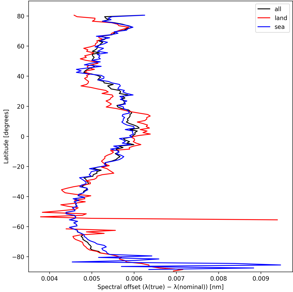
Figure 26: Zonal average of “Spectral offset ( \lambda_{\text{true}} - \lambda_{\text{nominal}} )” for 2025-10-13 to 2025-10-14.
