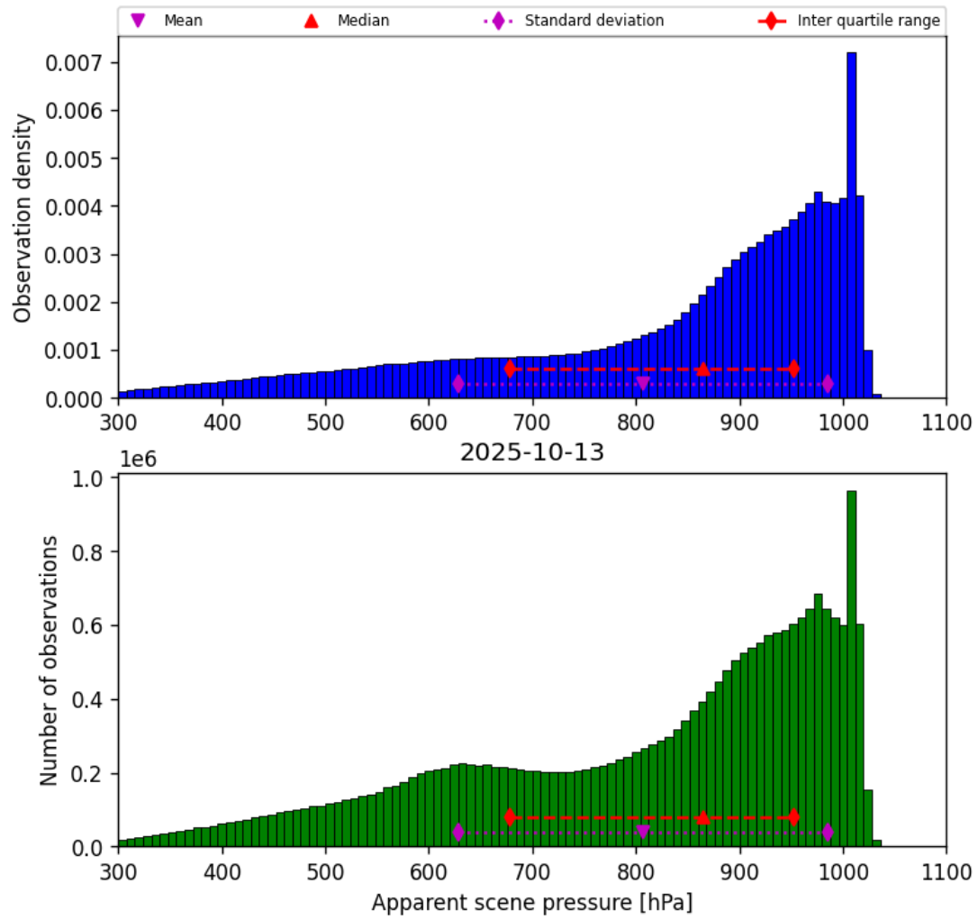
Figure 34: Histogram of “Apparent scene pressure” for 2025-10-13 to 2025-10-14
