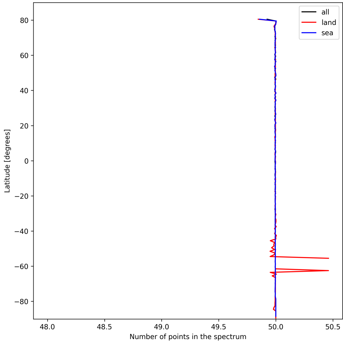
Figure 25: Zonal average of “Number of points in the spectrum” for 2025-10-13 to 2025-10-14.
