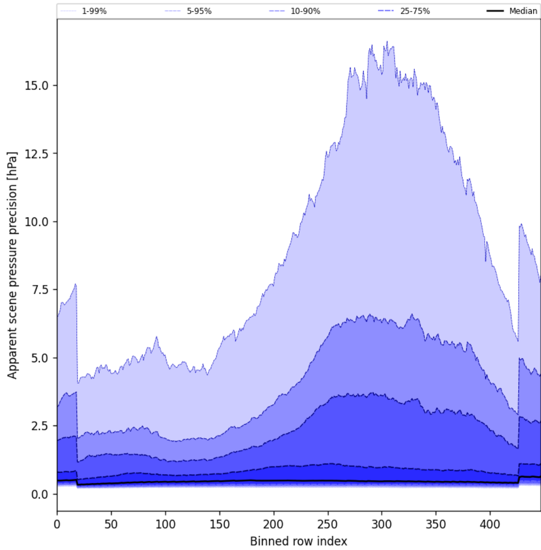
Figure 52: Along track statistics of “Apparent scene pressure precision” for 2025-10-13 to 2025-10-14
