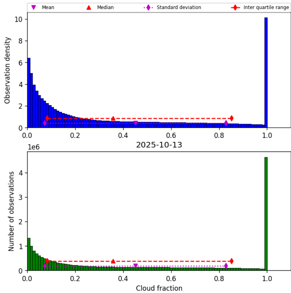
Figure 30: Histogram of “Cloud fraction” for 2025-10-13 to 2025-10-14
