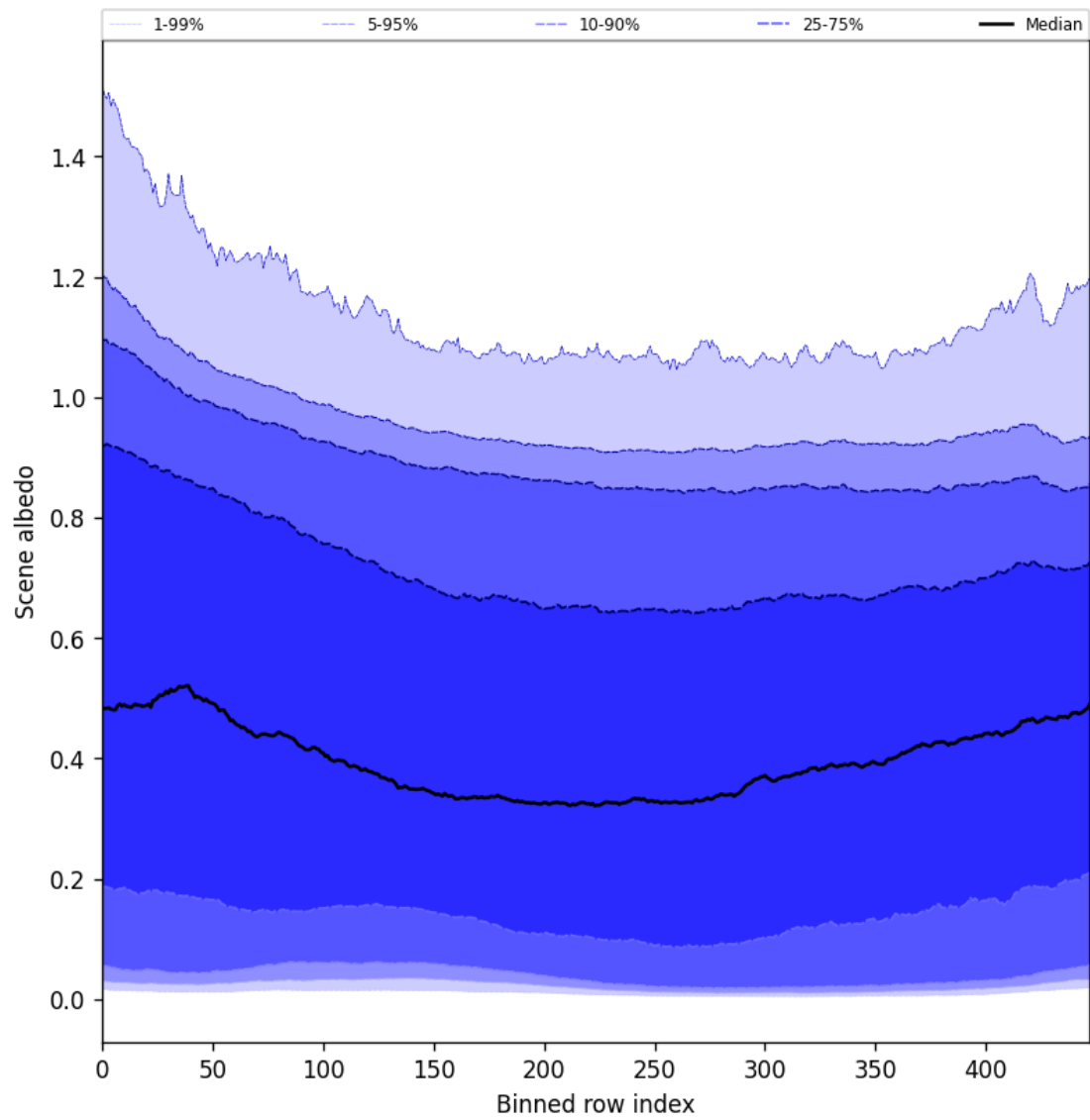
Figure 49: Along track statistics of “Scene albedo” for 2025-10-14 to 2025-10-15
