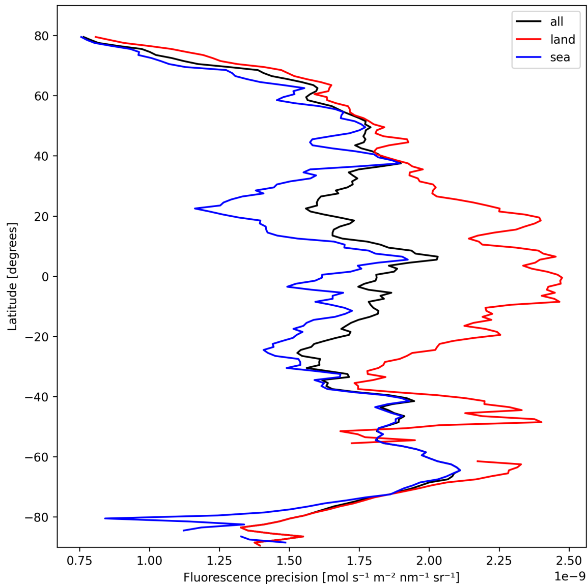
Figure 22: Zonal average of “Fluorescence precision” for 2025-10-14 to 2025-10-15.
