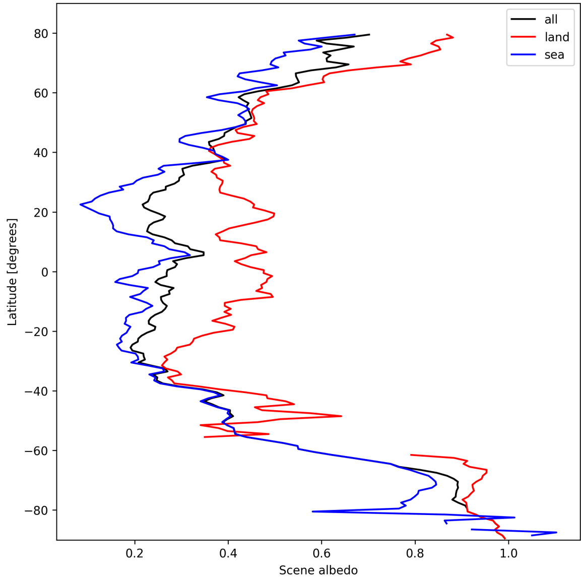
Figure 15: Zonal average of "Scene albedo" for 2025-10-14 to 2025-10-15.
