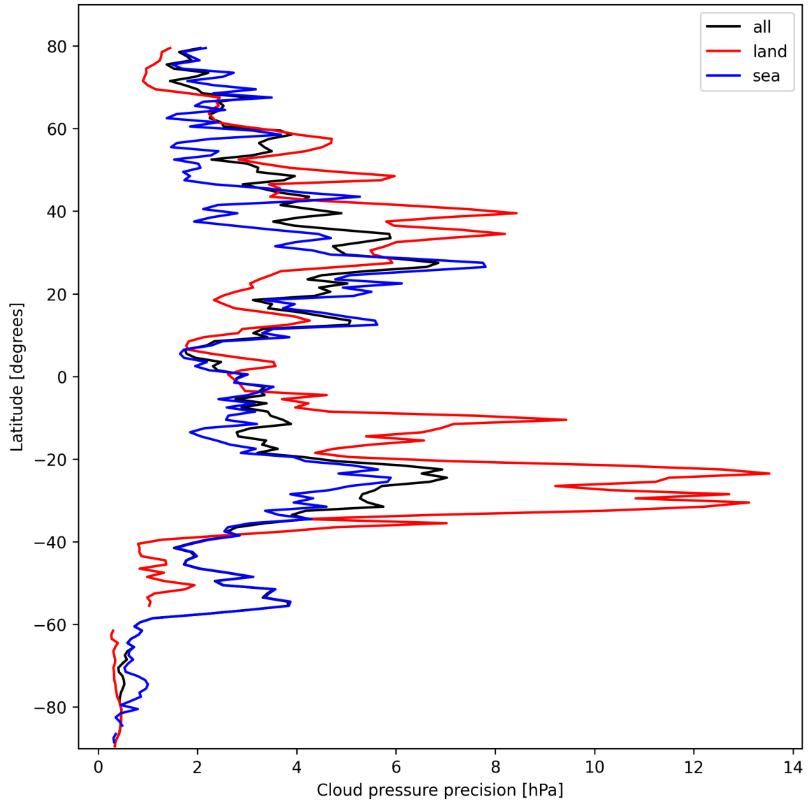
Figure 12: Zonal average of “Cloud pressure precision” for 2025-10-14 to 2025-10-15.
