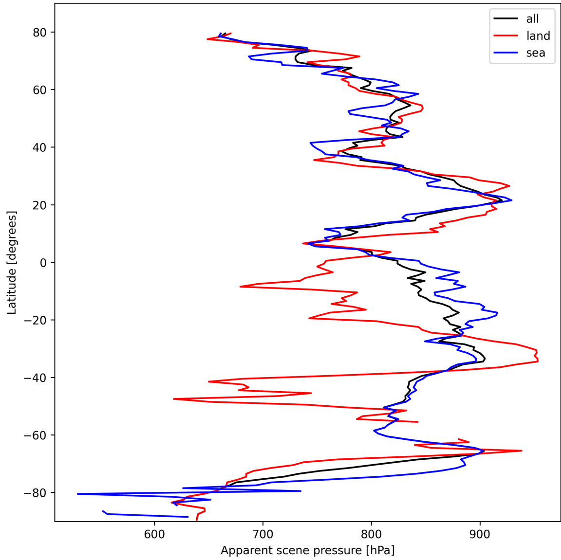
Figure 17: Zonal average of “Apparent scene pressure” for 2025-10-14 to 2025-10-15.
