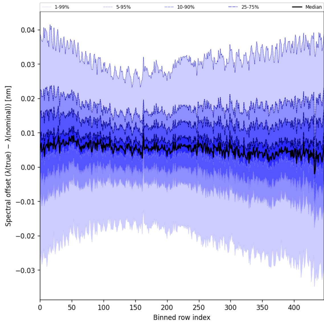
Figure 60: Along track statistics of “Spectral offset ( \lambda_{\text{true}} - \lambda_{\text{nominal}} )” for 2025-10-14 to 2025-10-15
