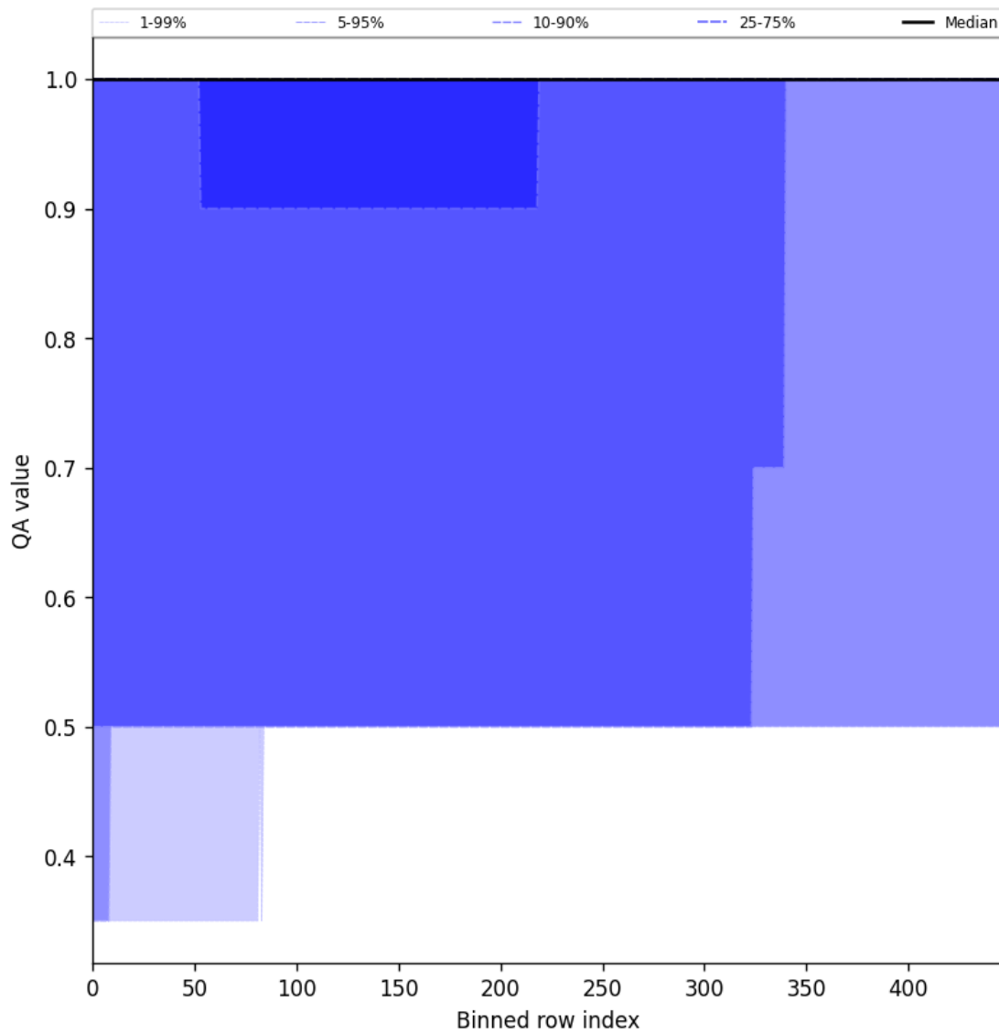
Figure 44: Along track statistics of “QA value” for 2025-10-14 to 2025-10-15
