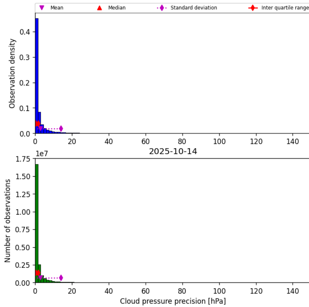
Figure 29: Histogram of “Cloud pressure precision” for 2025-10-14 to 2025-10-15
