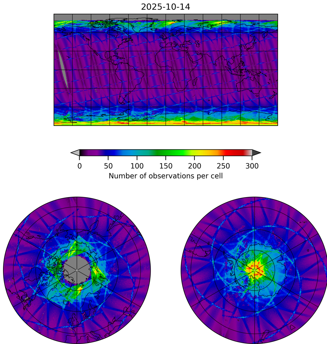
Figure 9: Map of the number of observations for 2025-10-14 to 2025-10-15
