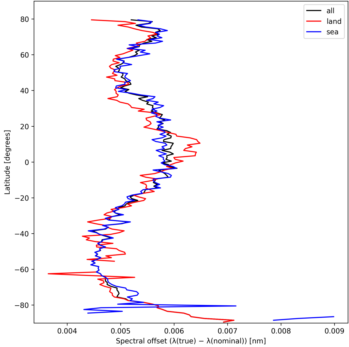
Figure 26: Zonal average of “Spectral offset ( \lambda_{\text{true}} - \lambda_{\text{nominal}} )” for 2025-10-14 to 2025-10-15.
