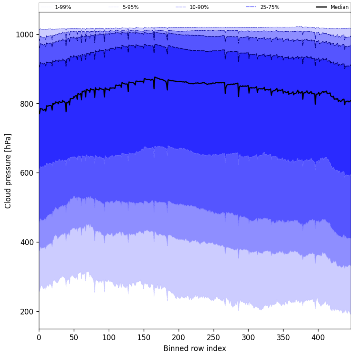
Figure 45: Along track statistics of “Cloud pressure” for 2025-10-14 to 2025-10-15
