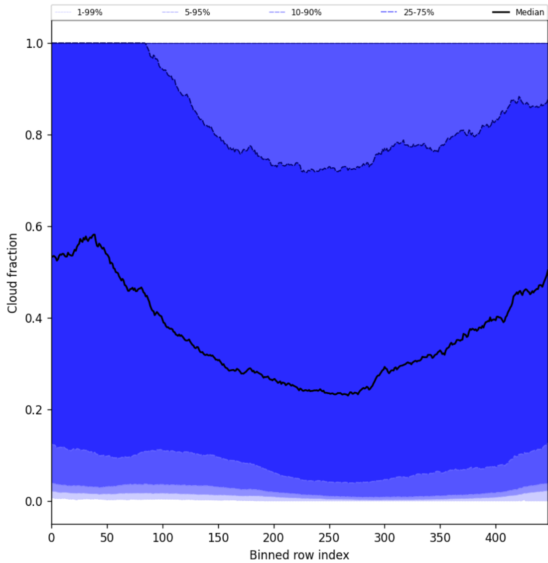
Figure 47: Along track statistics of “Cloud fraction” for 2025-10-14 to 2025-10-15
