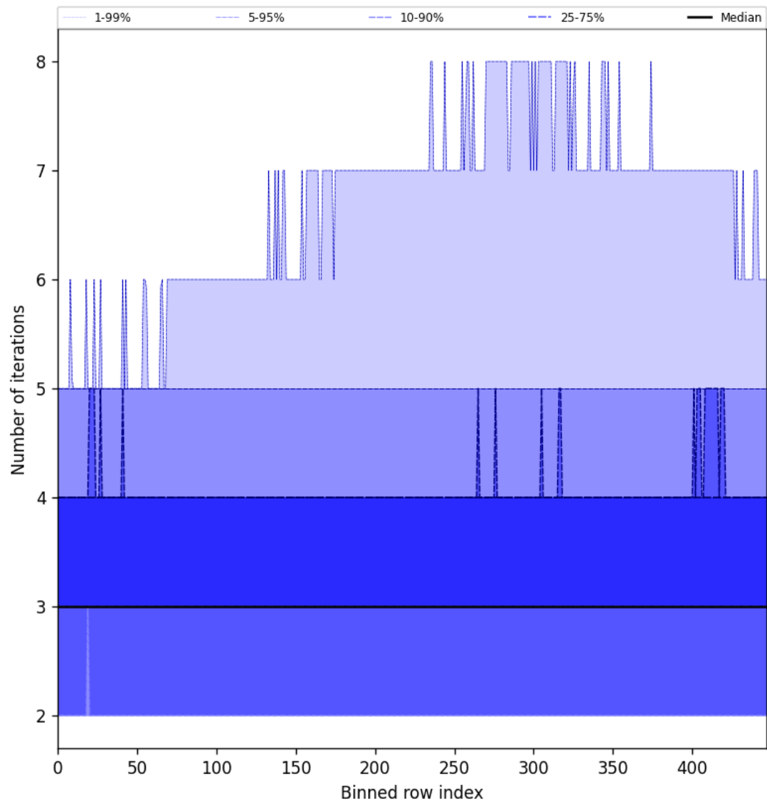
Figure 54: Along track statistics of “Number of iterations” for 2025-10-14 to 2025-10-15
