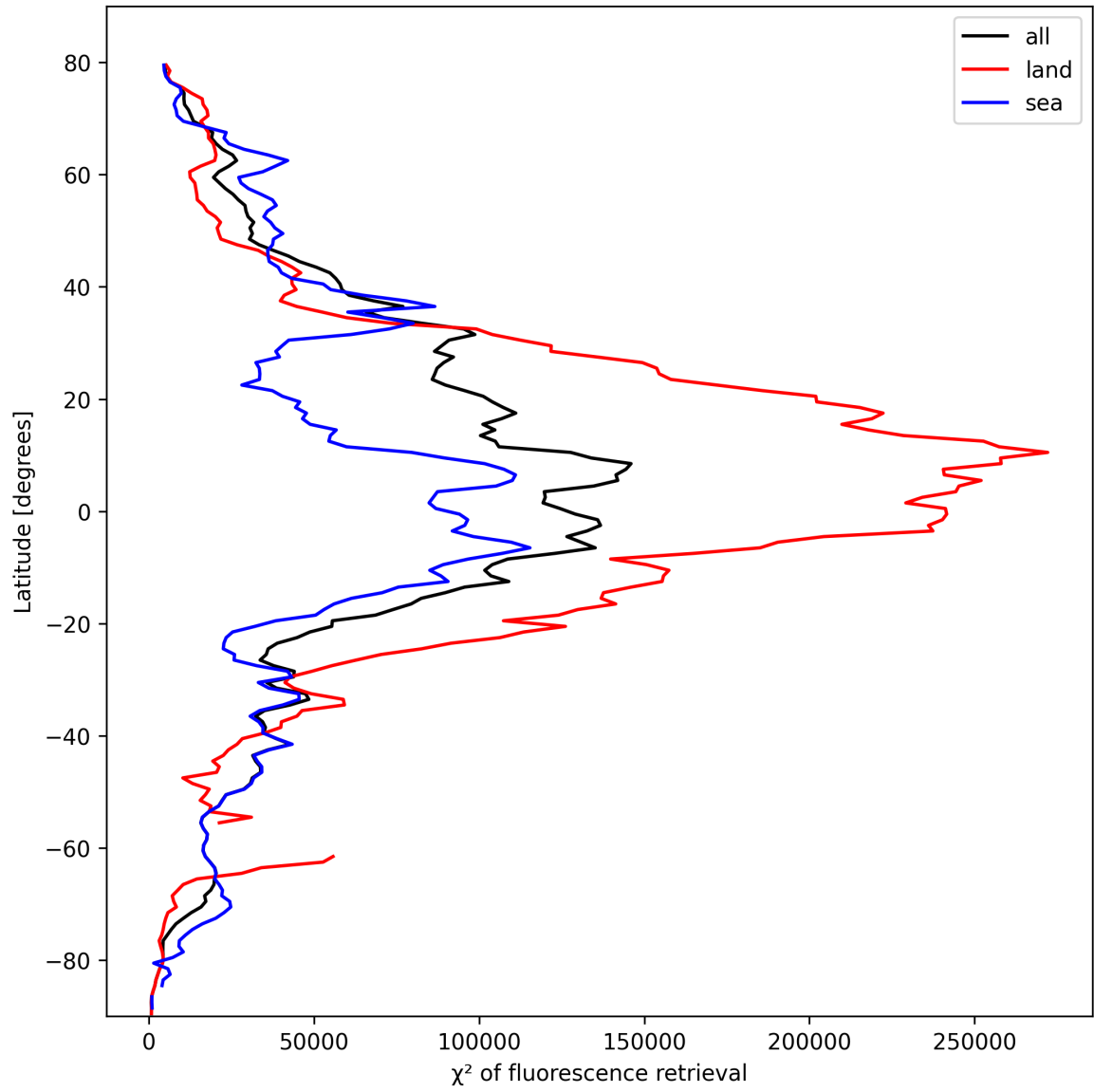
Figure 23: Zonal average of “ \chi^2 of fluorescence retrieval” for 2025-10-14 to 2025-10-15.
