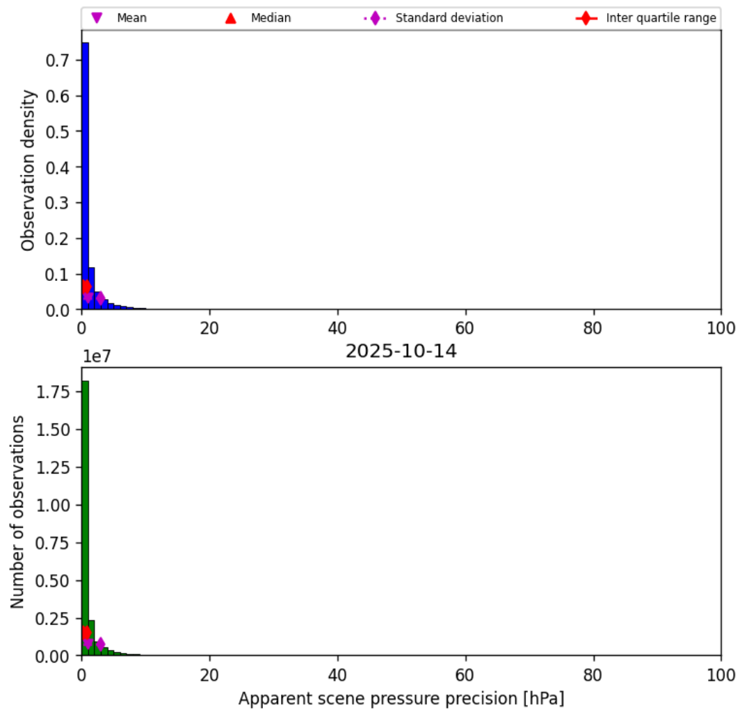
Figure 35: Histogram of “Apparent scene pressure precision” for 2025-10-14 to 2025-10-15
