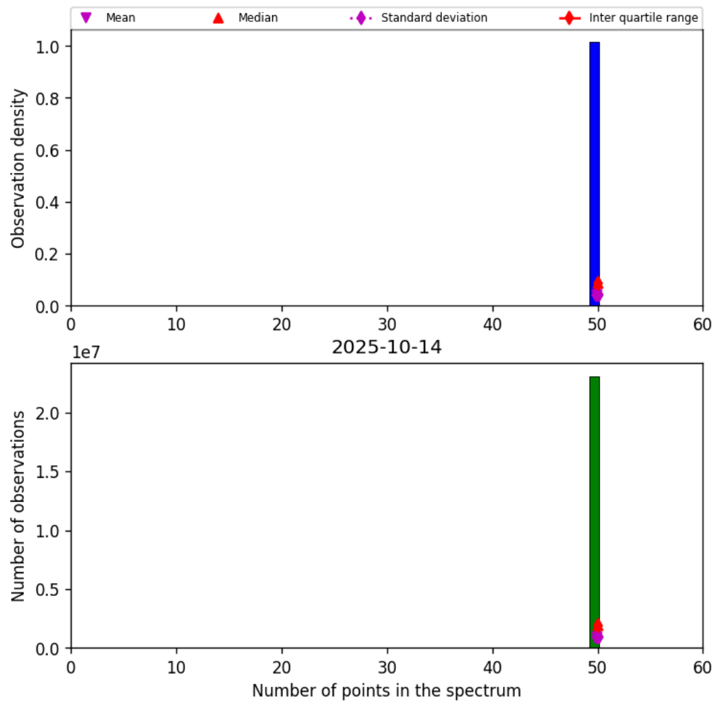
Figure 42: Histogram of “Number of points in the spectrum” for 2025-10-14 to 2025-10-15
