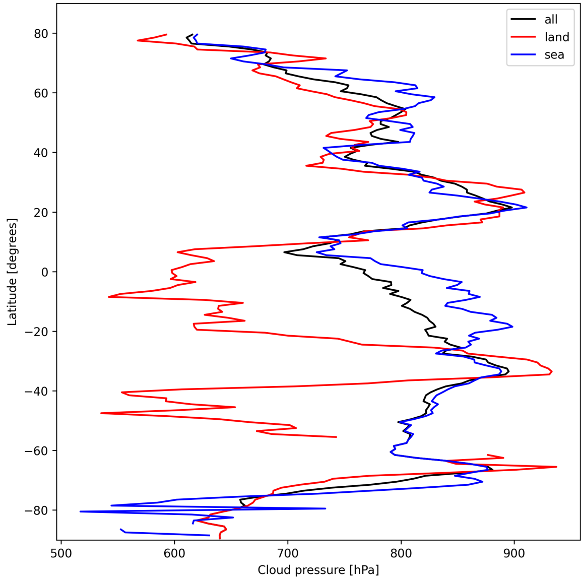
Figure 11: Zonal average of “Cloud pressure” for 2025-10-14 to 2025-10-15.
