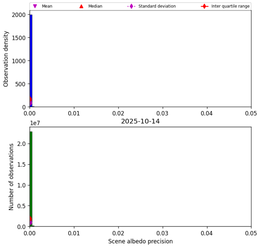
Figure 33: Histogram of “Scene albedo precision” for 2025-10-14 to 2025-10-15
