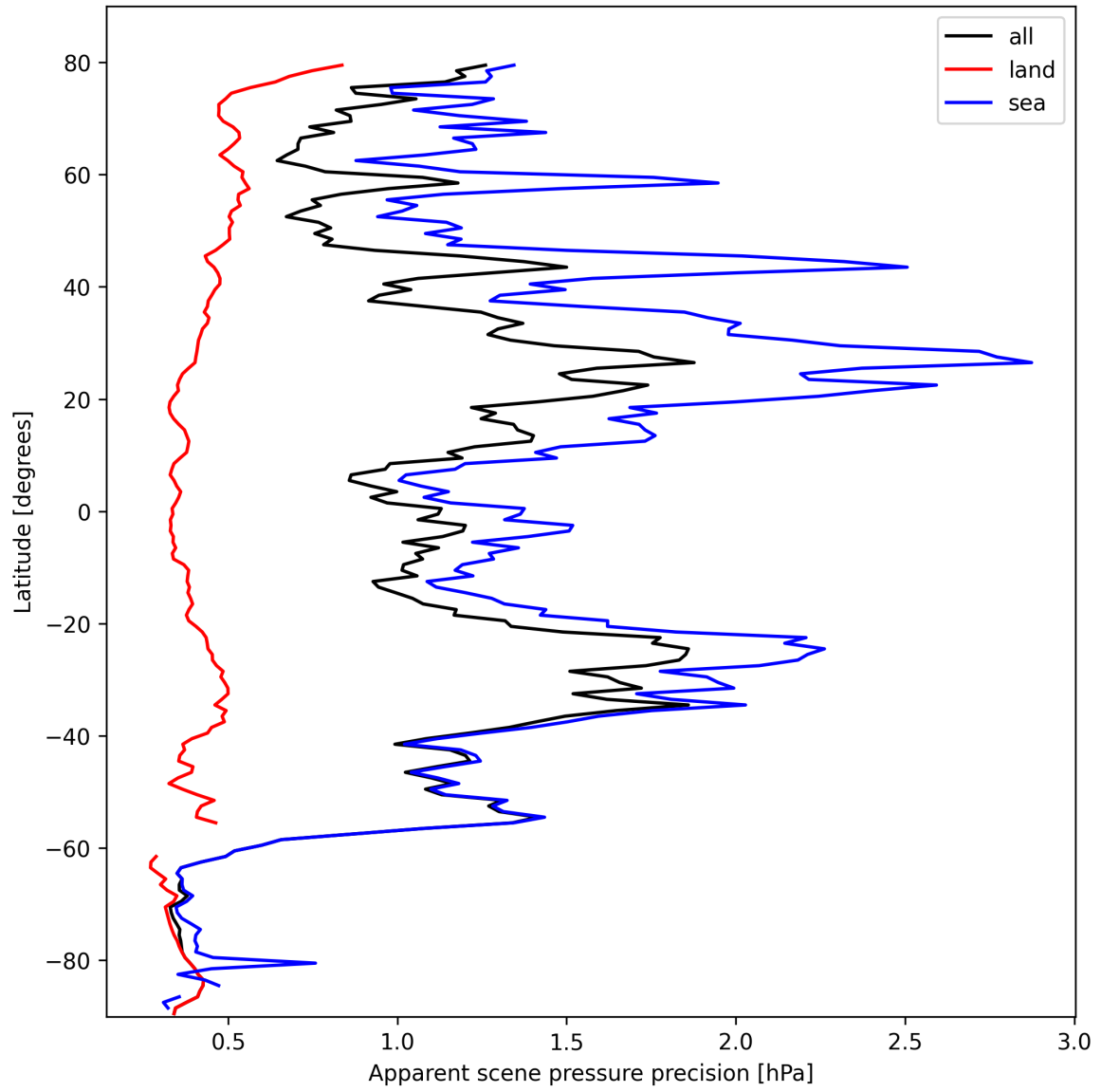
Figure 18: Zonal average of “Apparent scene pressure precision” for 2025-10-14 to 2025-10-15.
