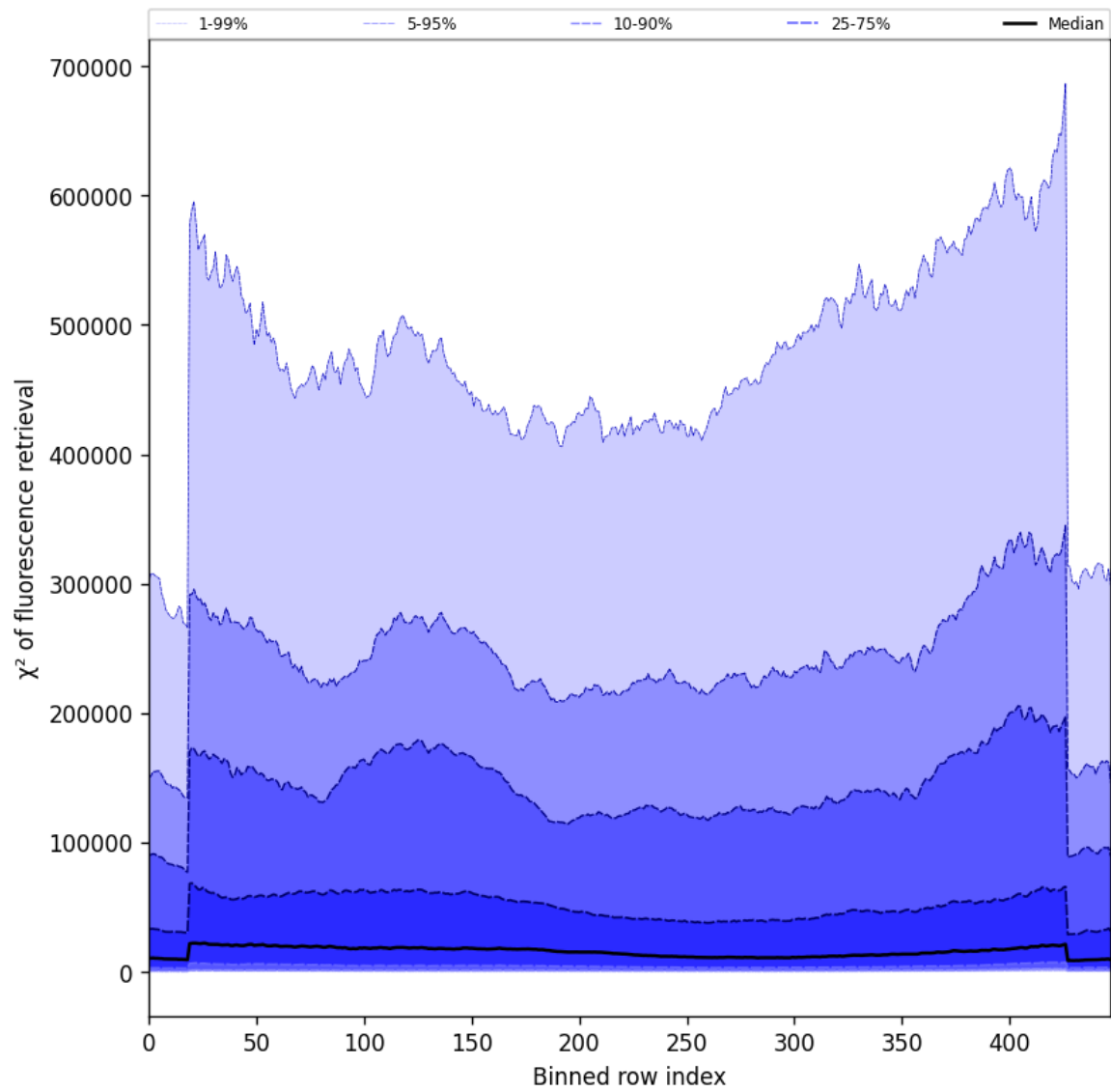
Figure 57: Along track statistics of “ \chi^2 of fluorescence retrieval” for 2025-10-14 to 2025-10-15
