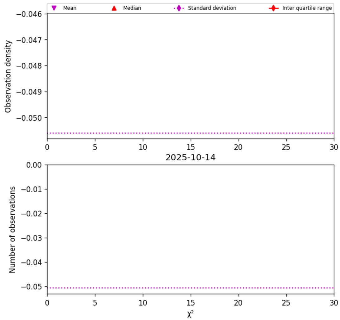
Figure 36: Histogram of " \chi^2 " for 2025-10-14 to 2025-10-15
