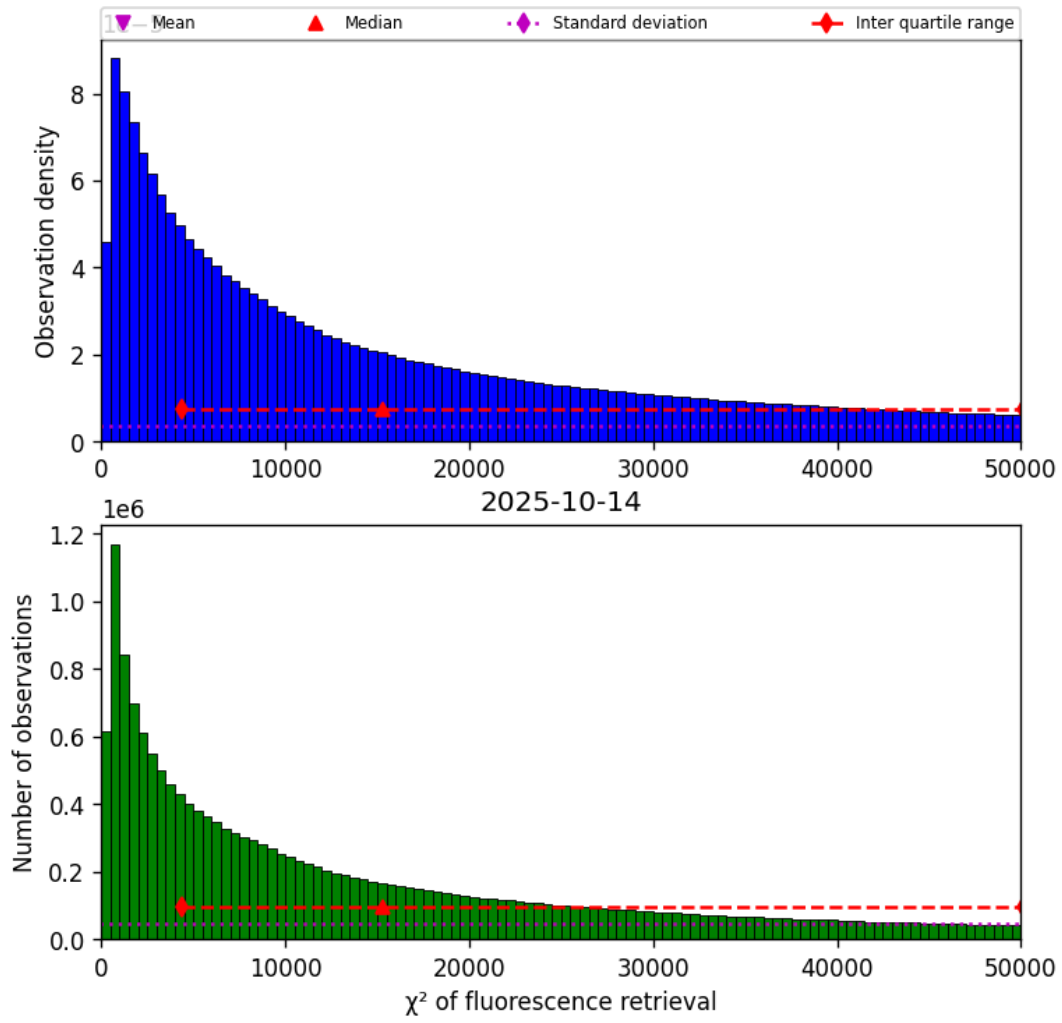
Figure 40: Histogram of “ \chi^2 of fluorescence retrieval” for 2025-10-14 to 2025-10-15
