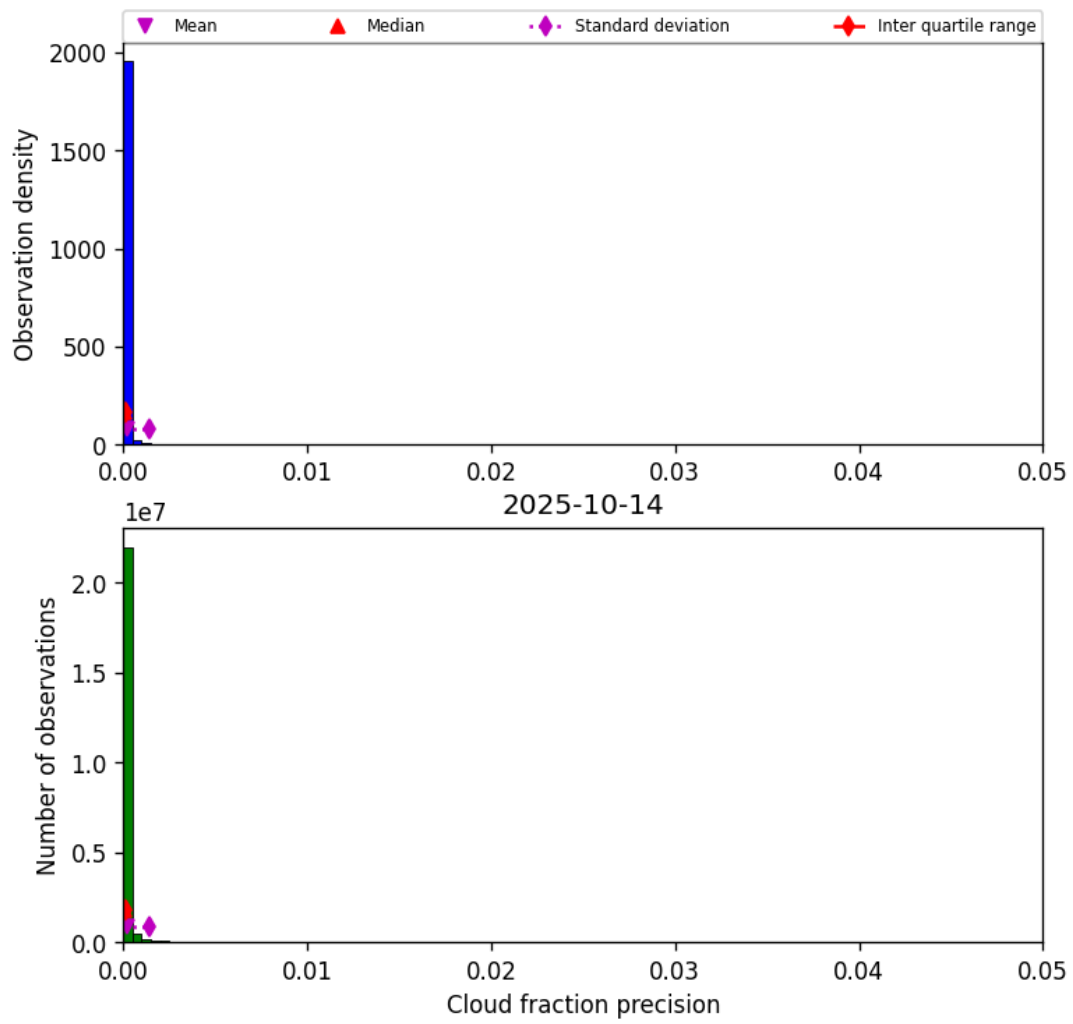
Figure 31: Histogram of “Cloud fraction precision” for 2025-10-14 to 2025-10-15
