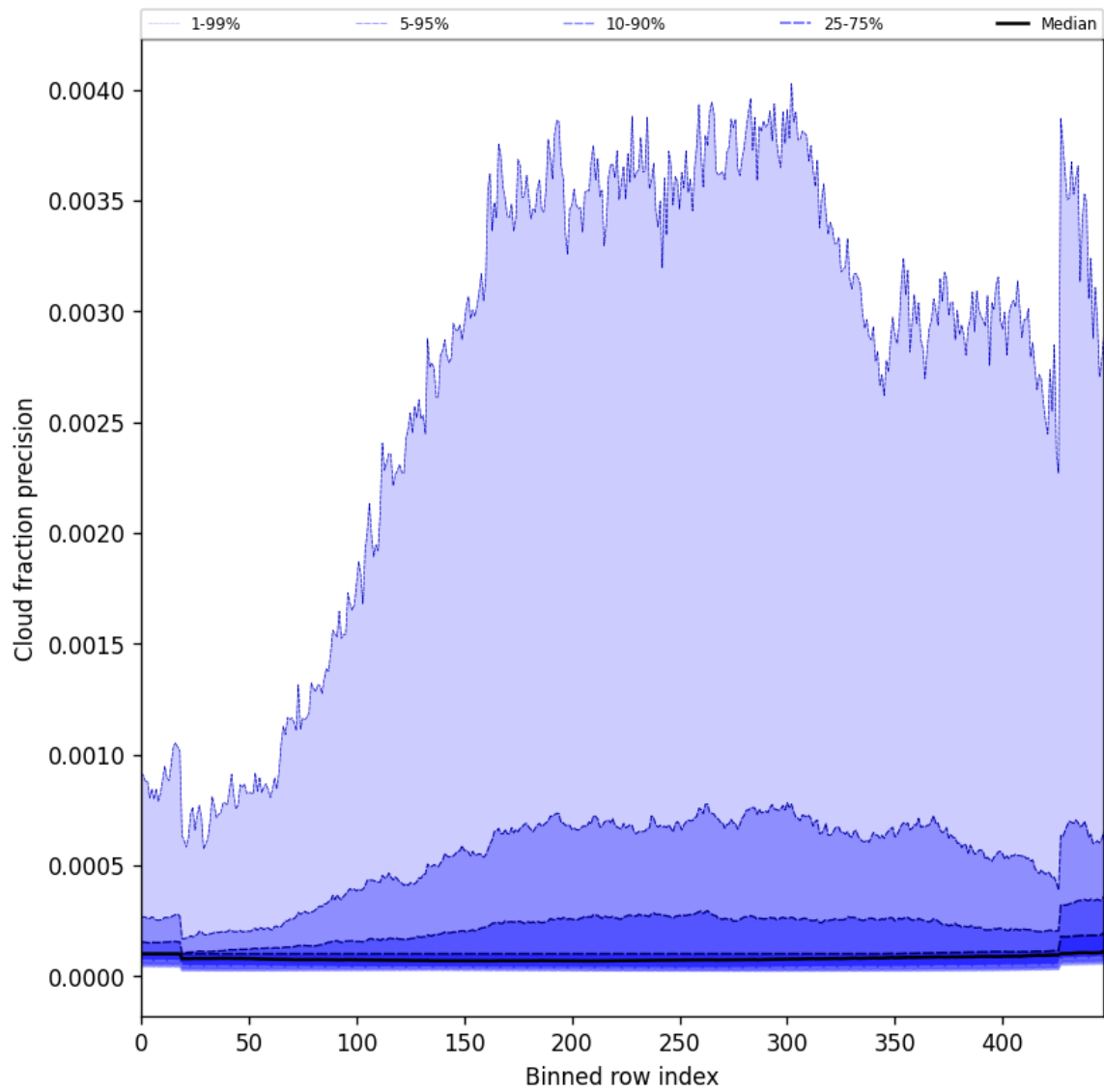
Figure 48: Along track statistics of “Cloud fraction precision” for 2025-10-14 to 2025-10-15
