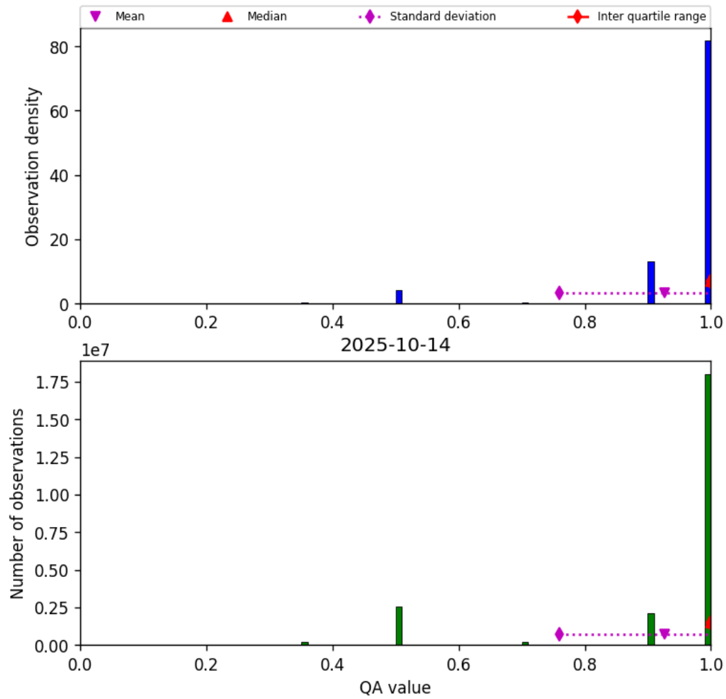
Figure 27: Histogram of “QA value” for 2025-10-14 to 2025-10-15
