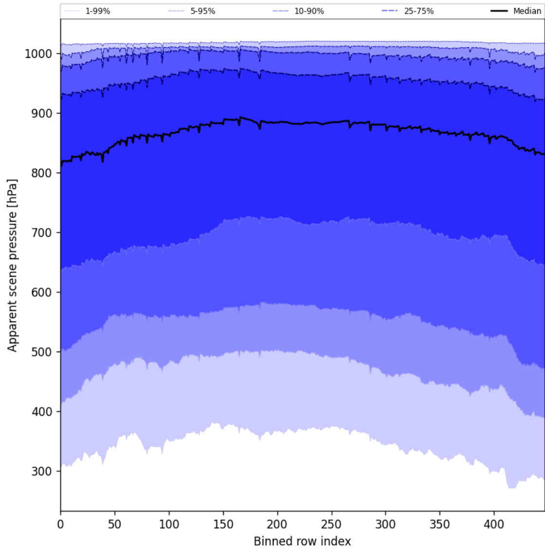
Figure 51: Along track statistics of “Apparent scene pressure” for 2025-10-14 to 2025-10-15
