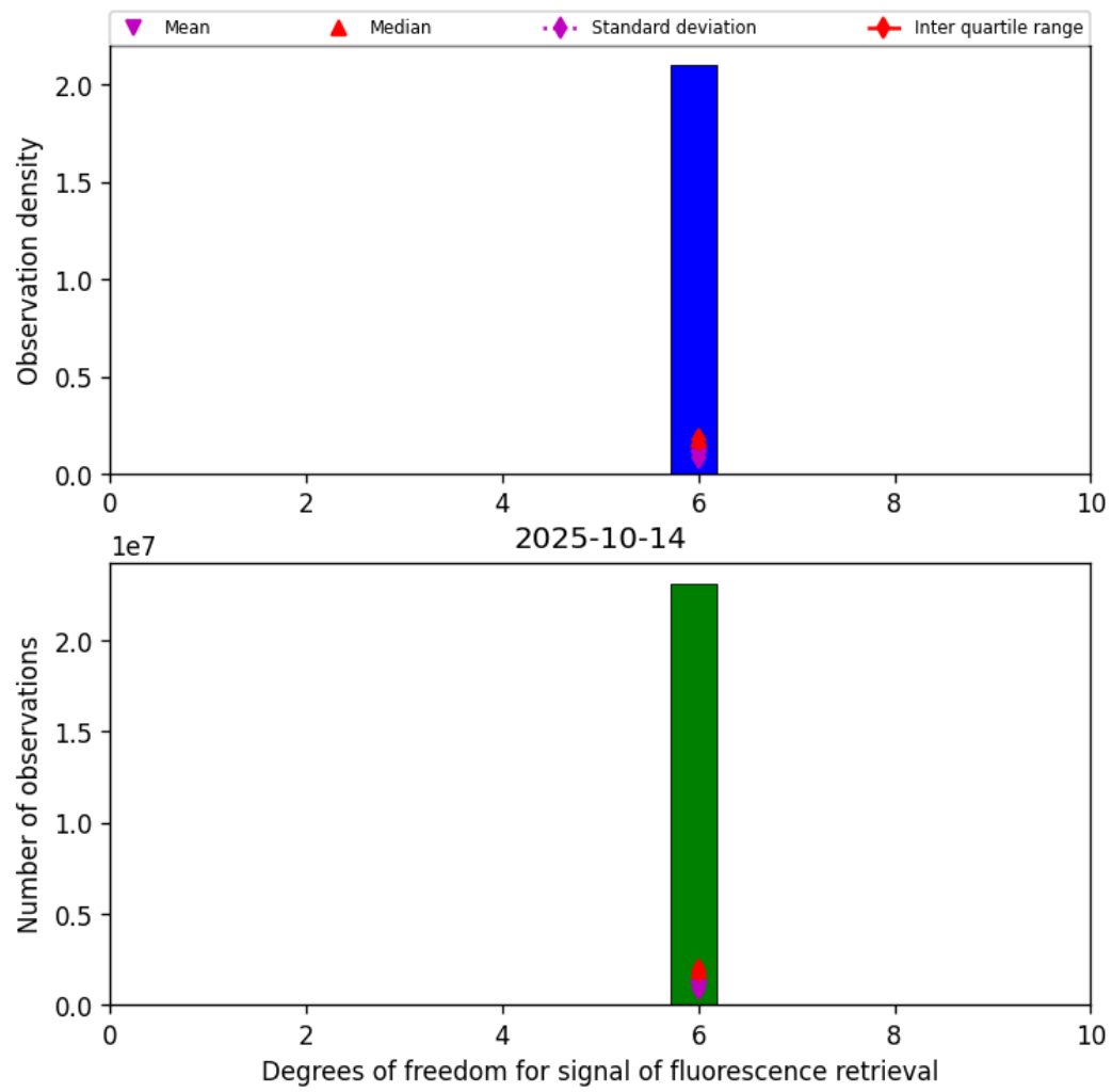
Figure 41: Histogram of “Degrees of freedom for signal of fluorescence retrieval” for 2025-10-14 to 2025-10-15
