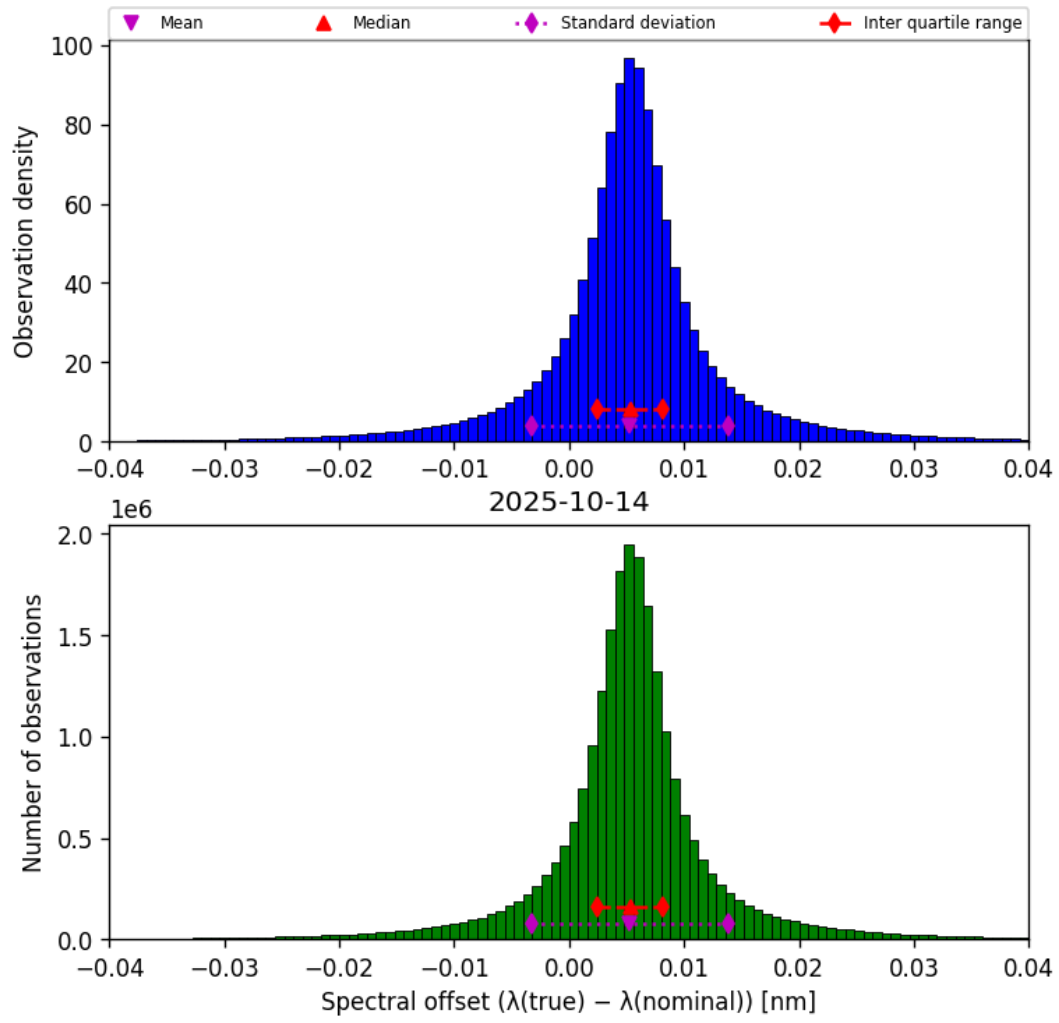
Figure 43: Histogram of “Spectral offset ( \lambda_{\text{true}} - \lambda_{\text{nominal}} )” for 2025-10-14 to 2025-10-15
