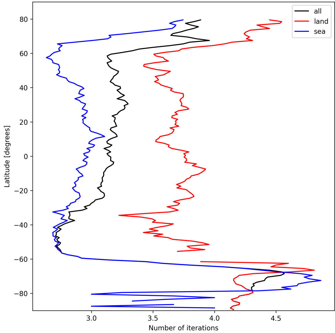
Figure 20: Zonal average of “Number of iterations” for 2025-10-14 to 2025-10-15.
