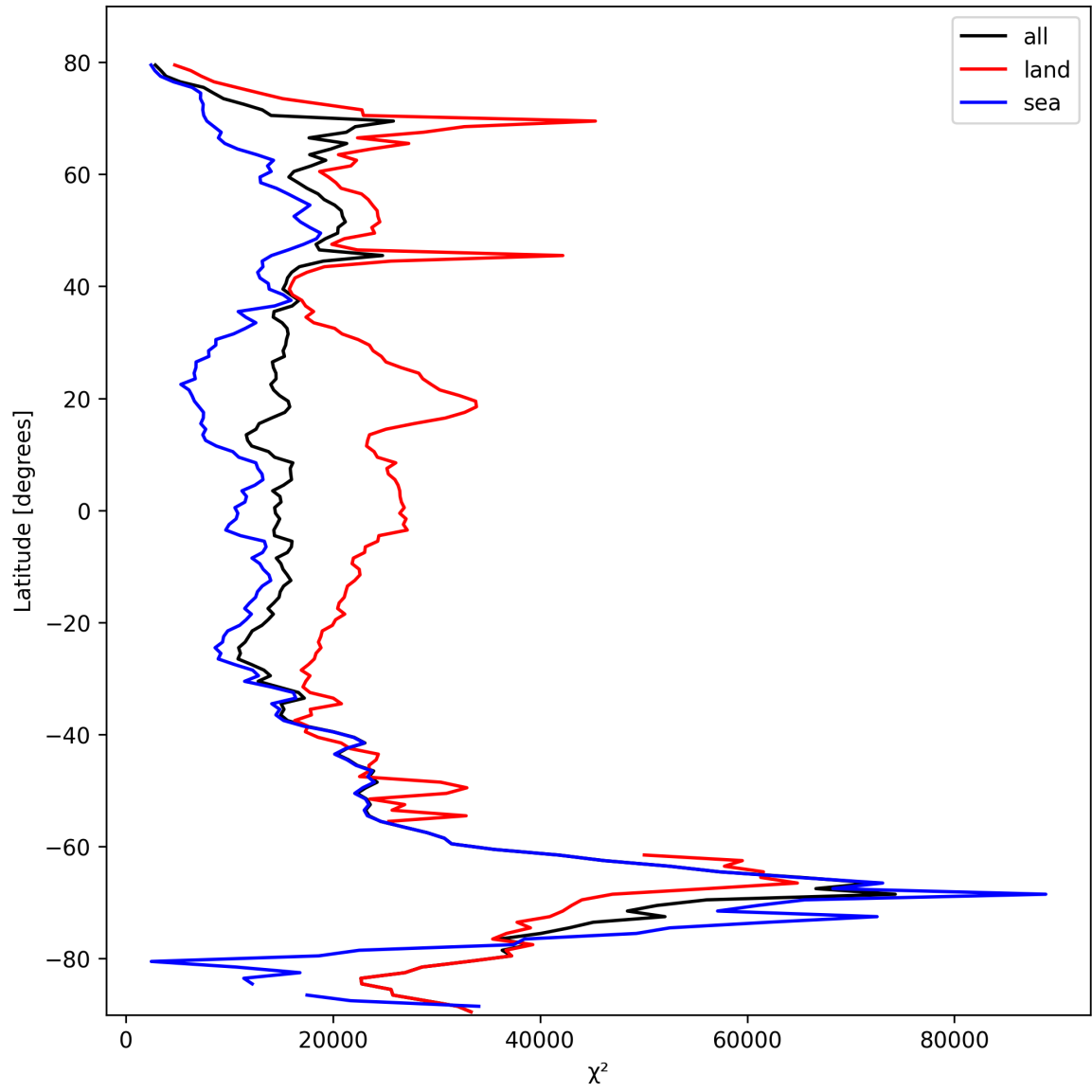
Figure 19: Zonal average of “ \chi^2 ” for 2025-10-14 to 2025-10-15.
