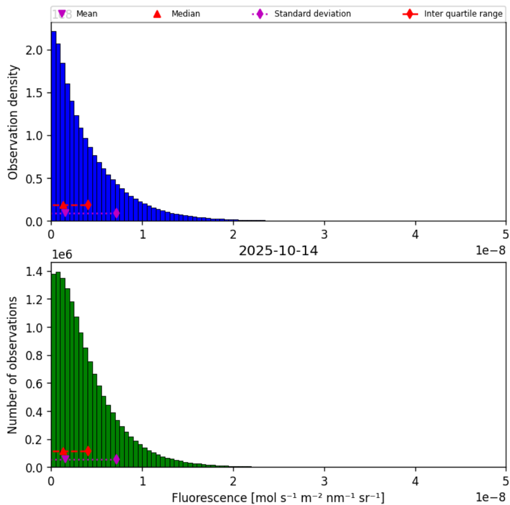
Figure 38: Histogram of “Fluorescence” for 2025-10-14 to 2025-10-15
