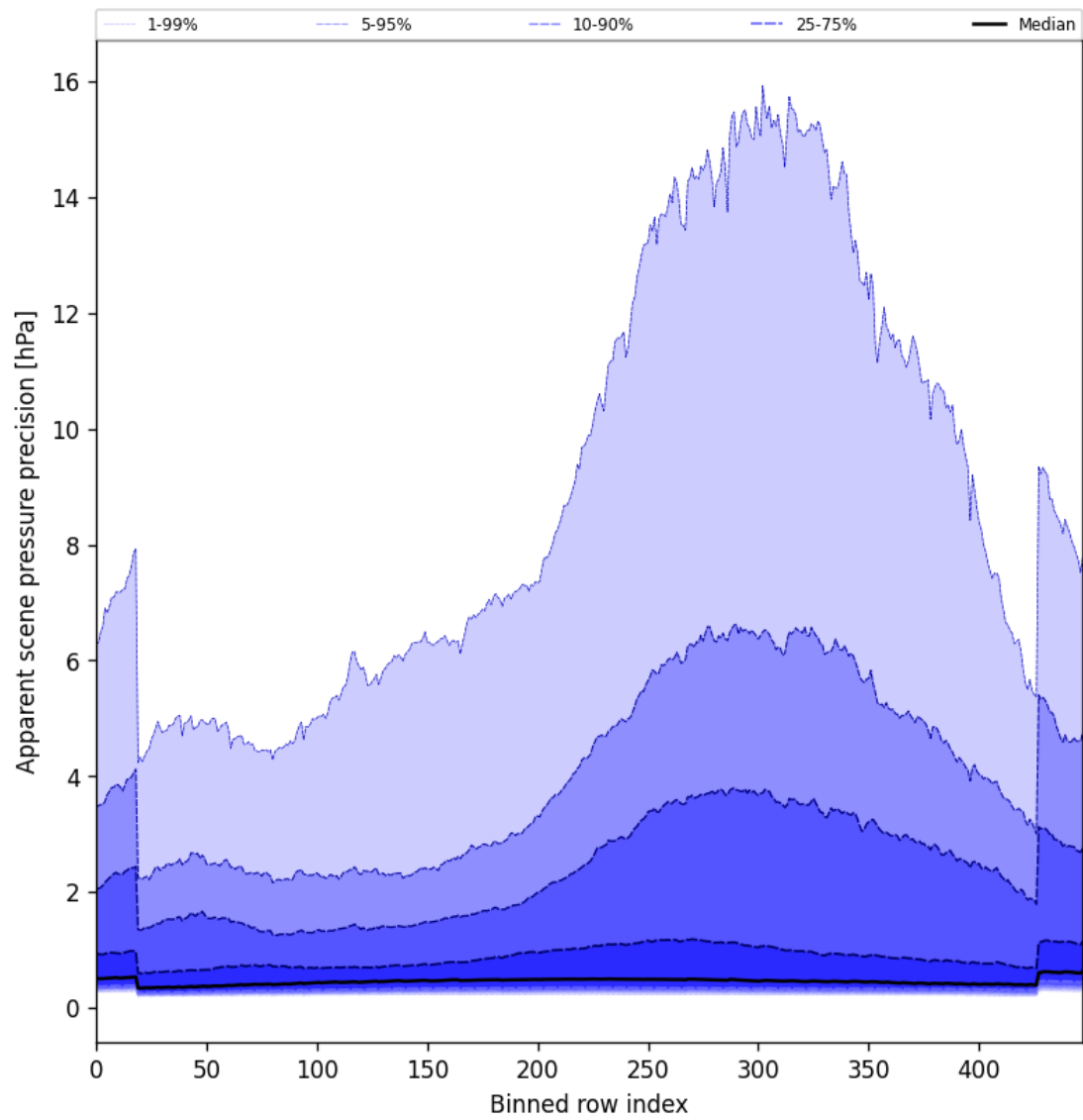
Figure 52: Along track statistics of “Apparent scene pressure precision” for 2025-10-14 to 2025-10-15
