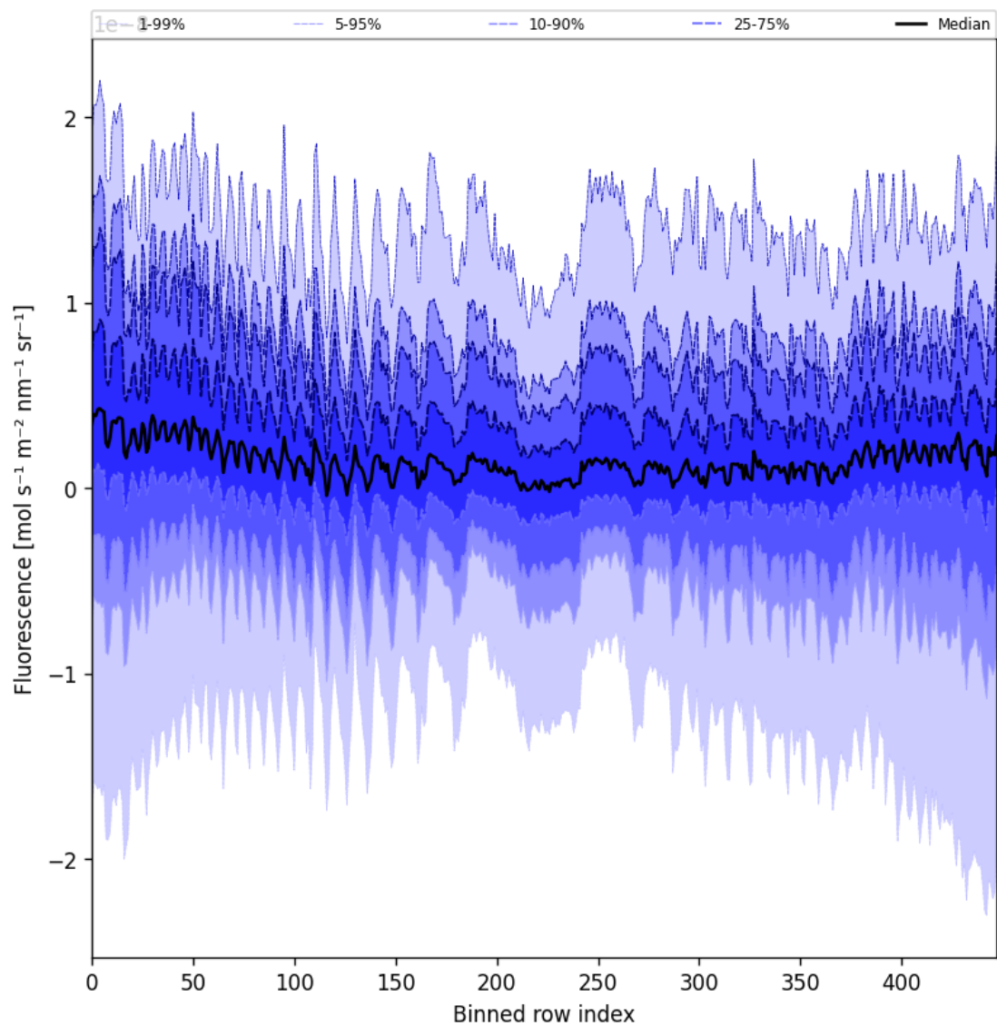
Figure 55: Along track statistics of “Fluorescence” for 2025-10-14 to 2025-10-15
