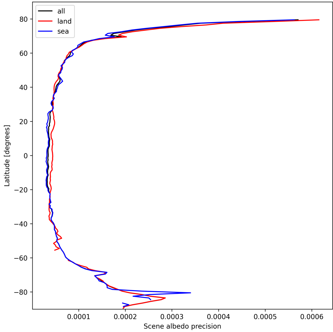
Figure 16: Zonal average of “Scene albedo precision” for 2025-10-14 to 2025-10-15.
