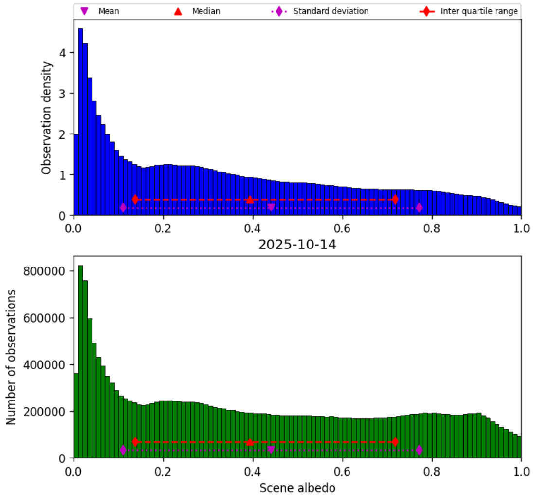
Figure 32: Histogram of “Scene albedo” for 2025-10-14 to 2025-10-15
