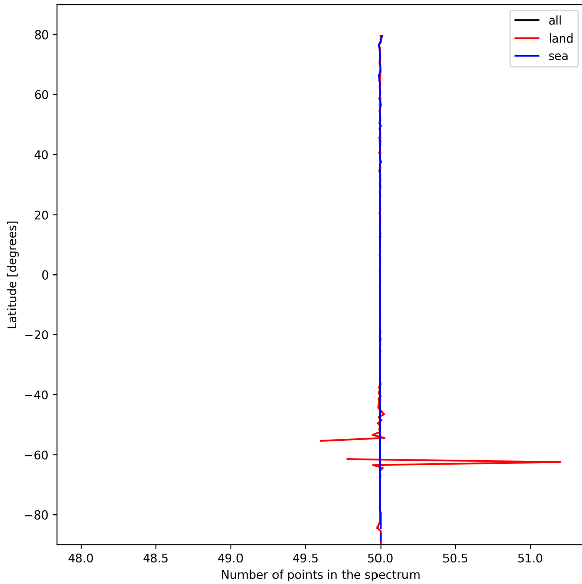
Figure 25: Zonal average of “Number of points in the spectrum” for 2025-10-14 to 2025-10-15.
