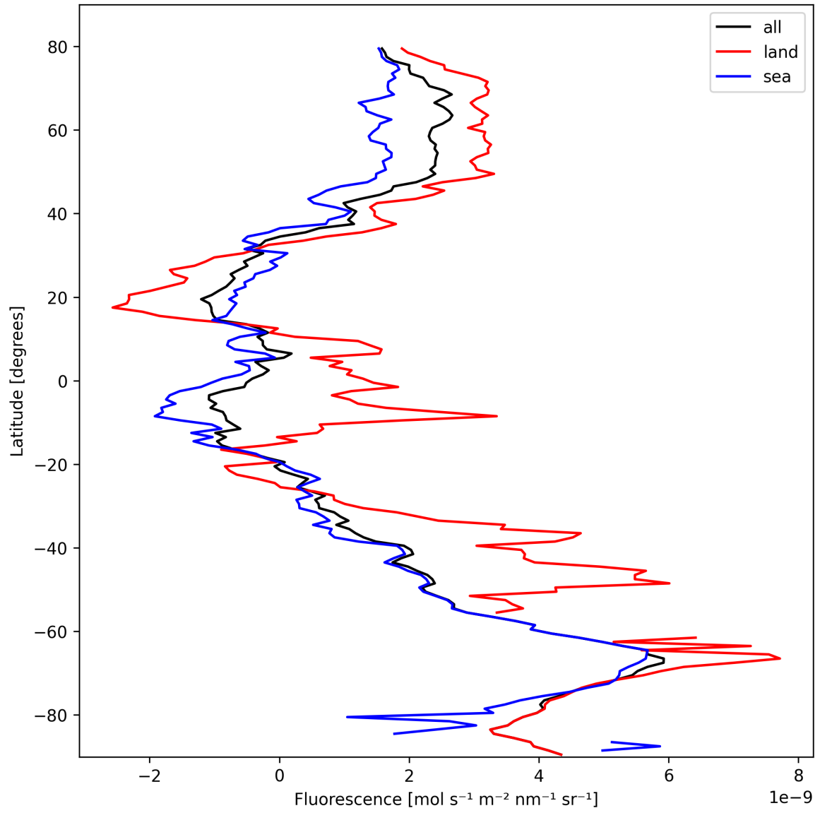
Figure 21: Zonal average of “Fluorescence” for 2025-10-14 to 2025-10-15.
