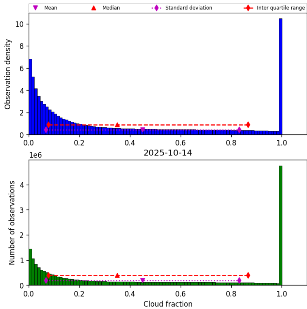
Figure 30: Histogram of “Cloud fraction” for 2025-10-14 to 2025-10-15
