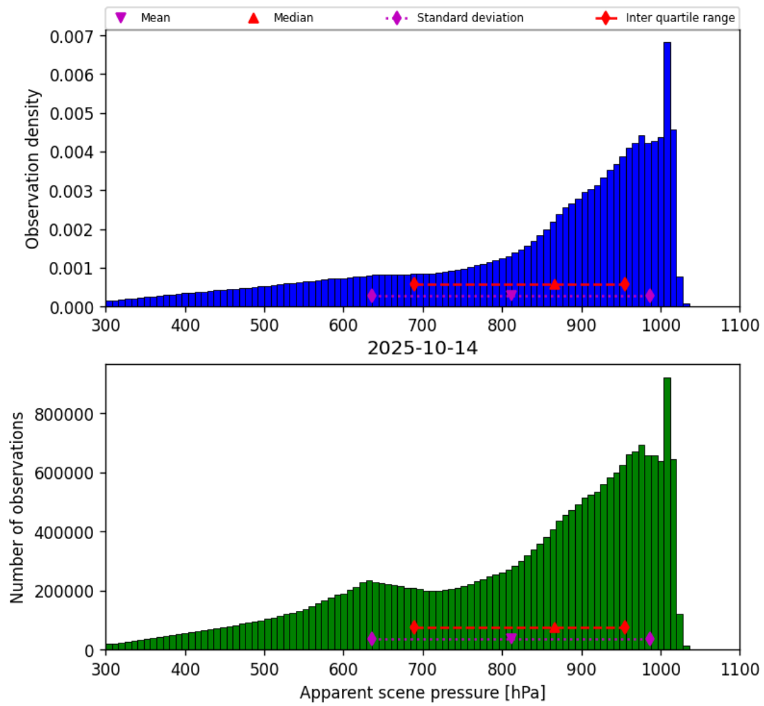
Figure 34: Histogram of “Apparent scene pressure” for 2025-10-14 to 2025-10-15
