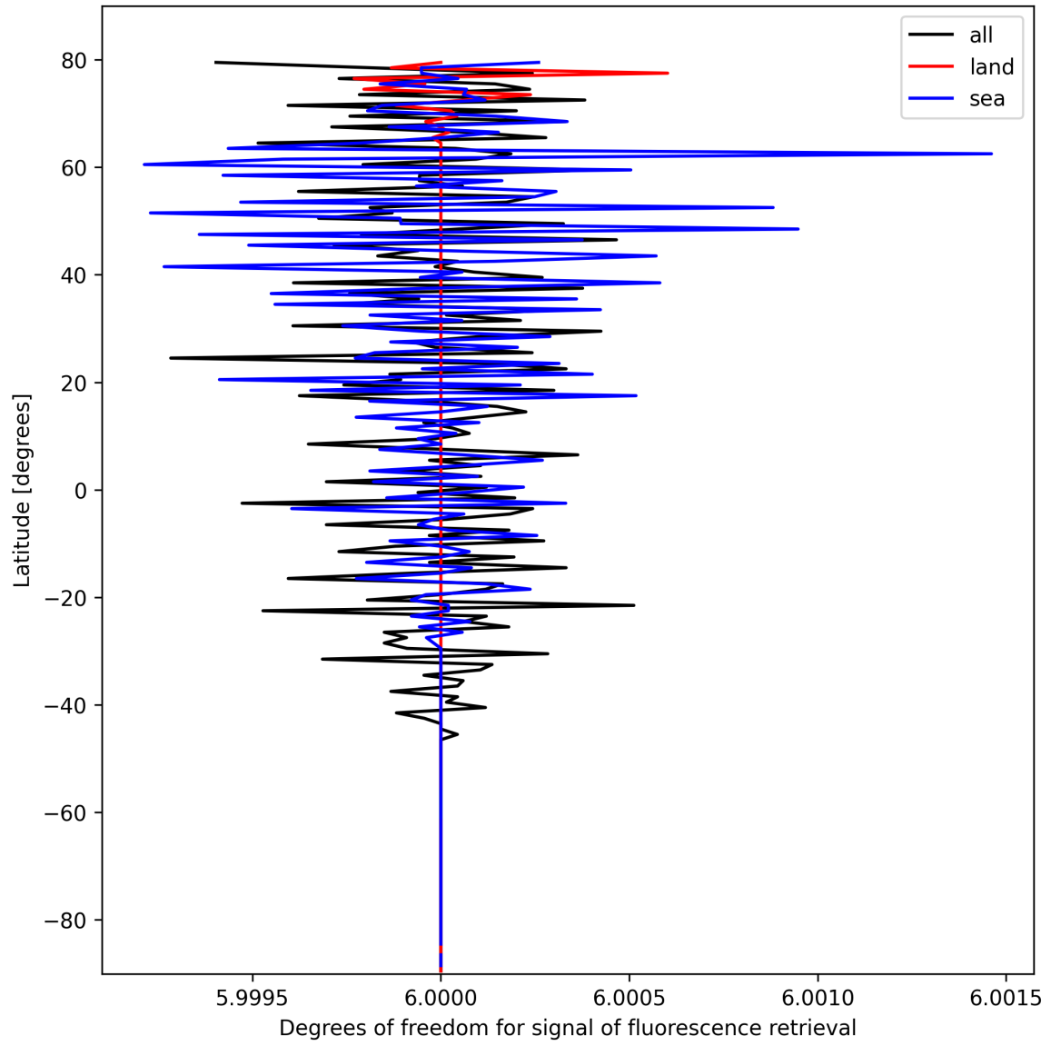
Figure 24: Zonal average of “Degrees of freedom for signal of fluorescence retrieval” for 2025-10-14 to 2025-10-15.
