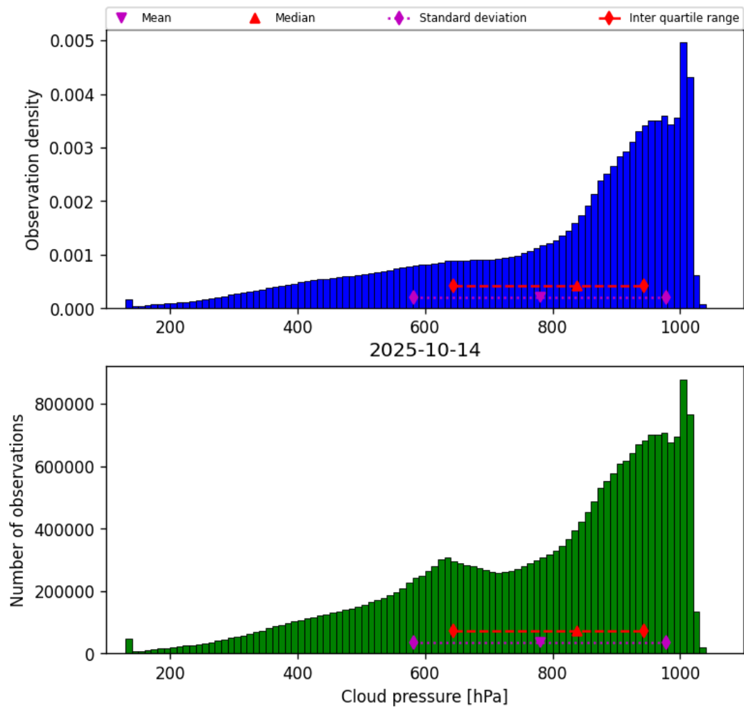
Figure 28: Histogram of “Cloud pressure” for 2025-10-14 to 2025-10-15
