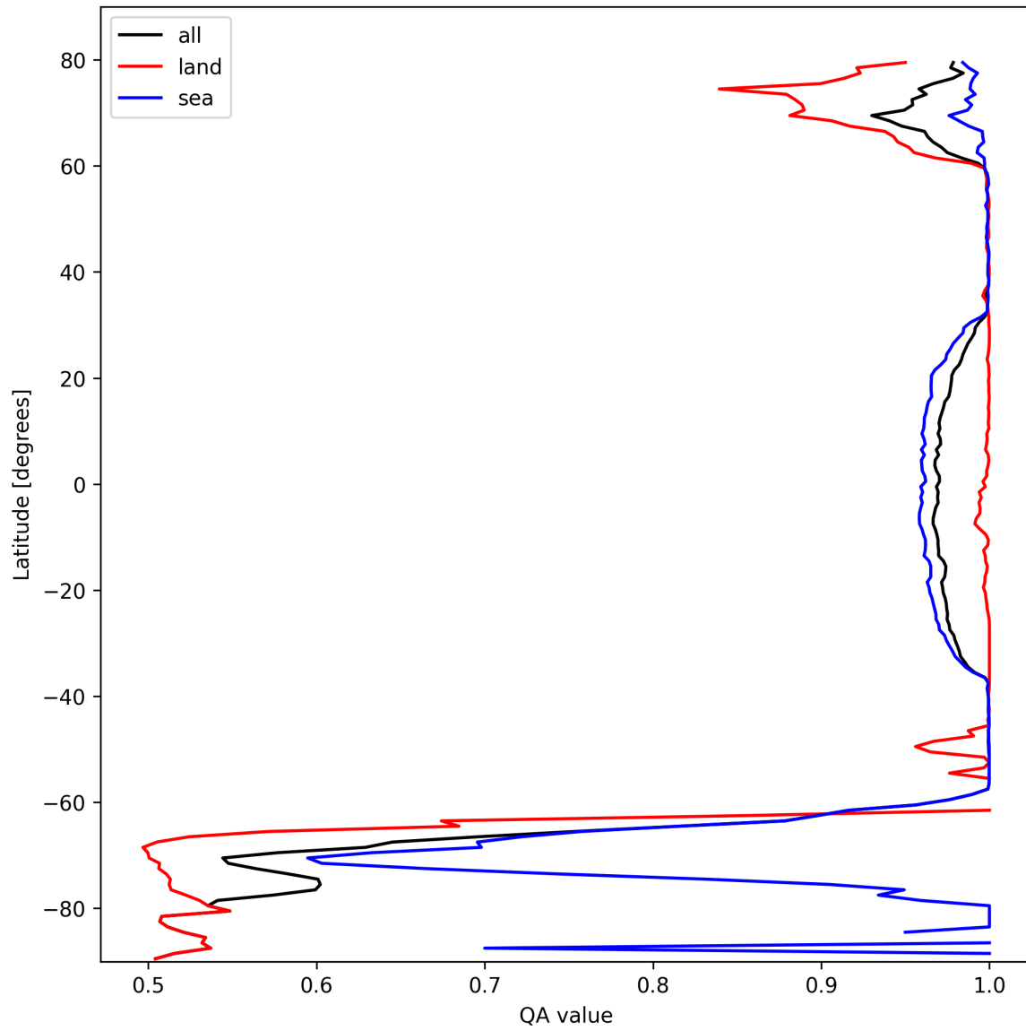
Figure 10: Zonal average of “QA value” for 2025-10-14 to 2025-10-15.
