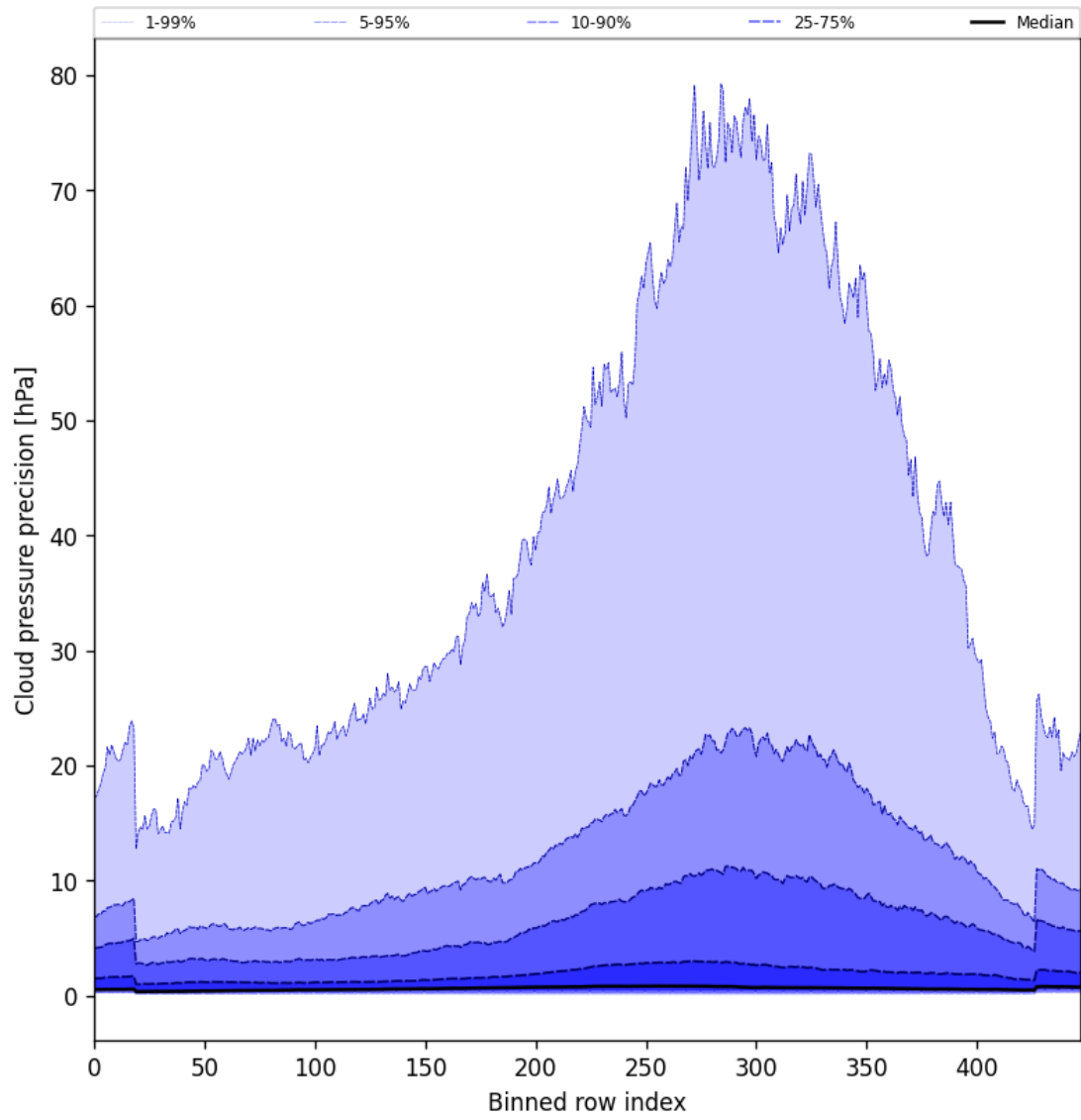
Figure 46: Along track statistics of “Cloud pressure precision” for 2025-10-14 to 2025-10-15
