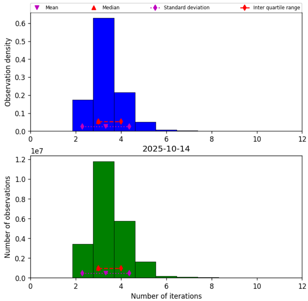
Figure 37: Histogram of “Number of iterations” for 2025-10-14 to 2025-10-15
