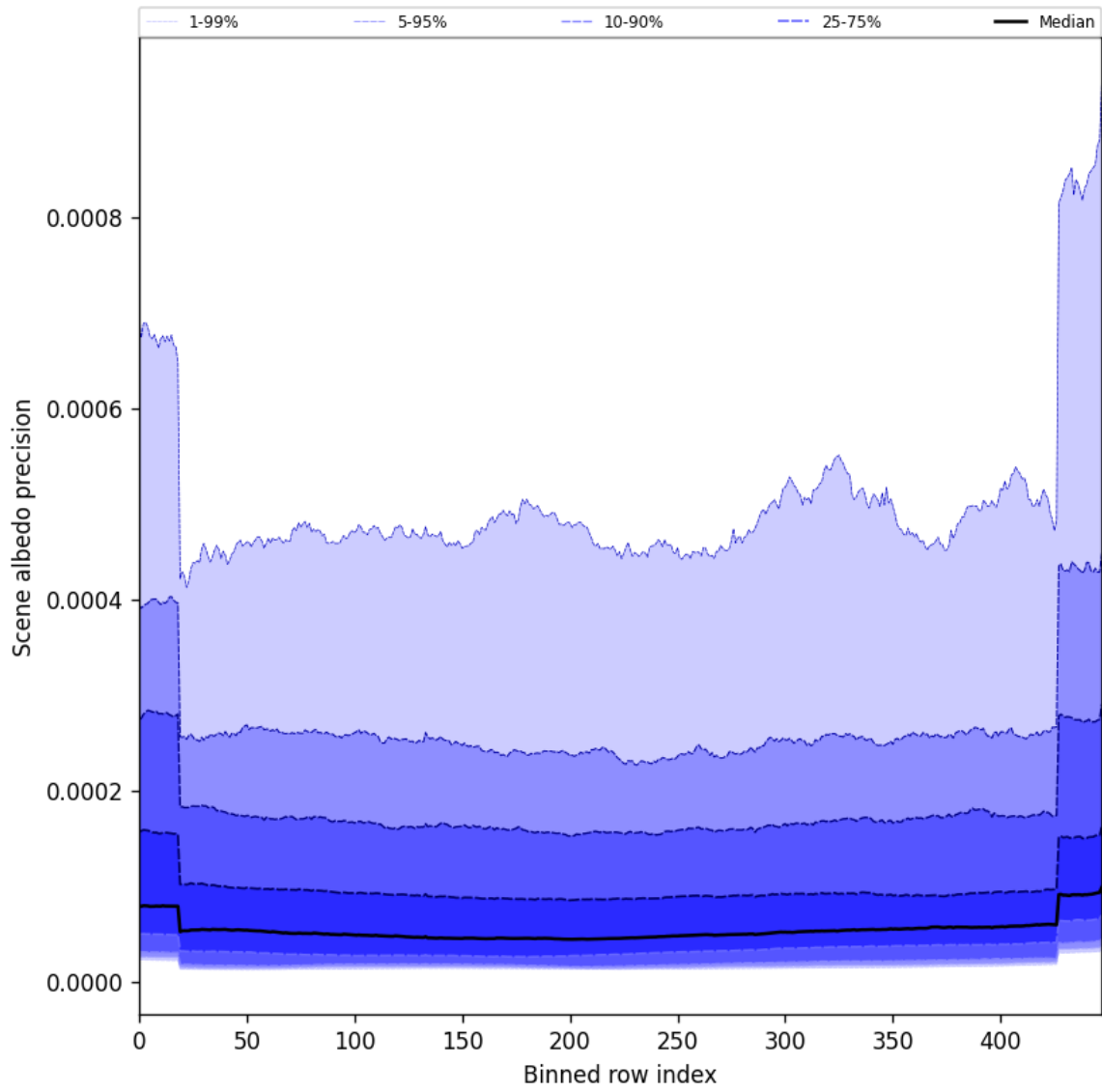
Figure 50: Along track statistics of “Scene albedo precision” for 2025-10-14 to 2025-10-15
