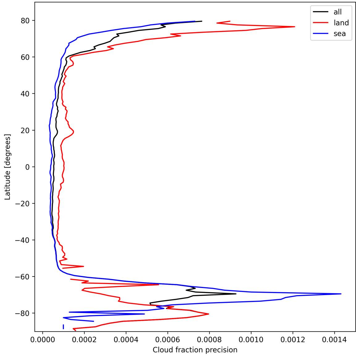
Figure 14: Zonal average of “Cloud fraction precision” for 2025-10-14 to 2025-10-15.
