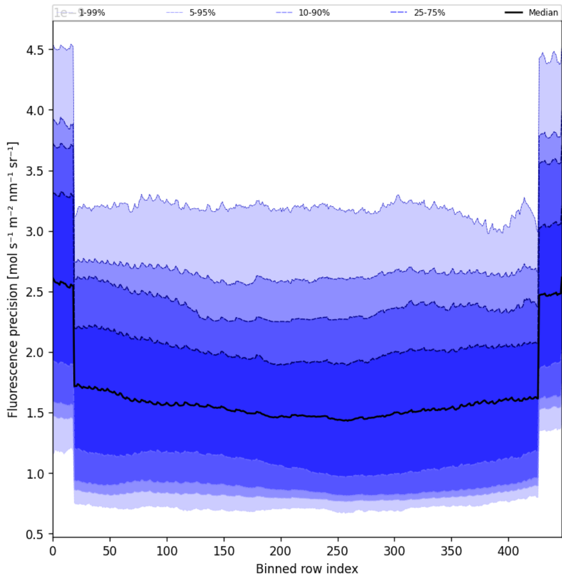
Figure 56: Along track statistics of “Fluorescence precision” for 2025-10-14 to 2025-10-15
