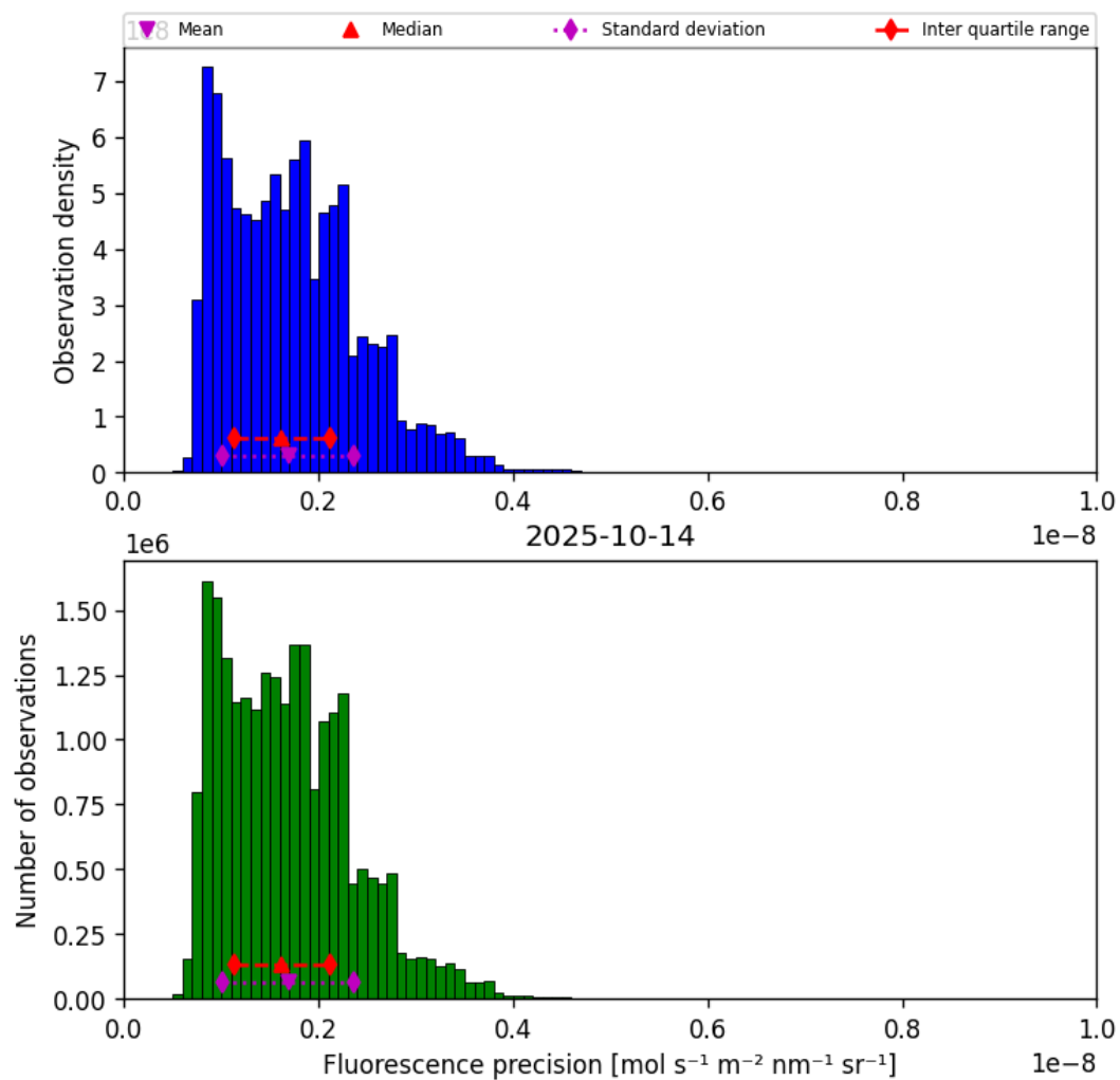
Figure 39: Histogram of “Fluorescence precision” for 2025-10-14 to 2025-10-15
