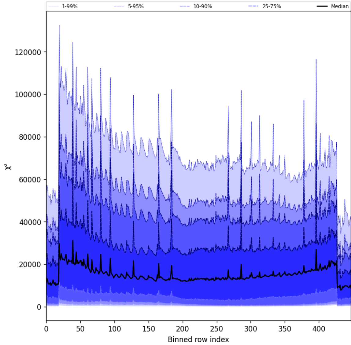
Figure 53: Along track statistics of “ \chi^2 ” for 2025-10-14 to 2025-10-15
