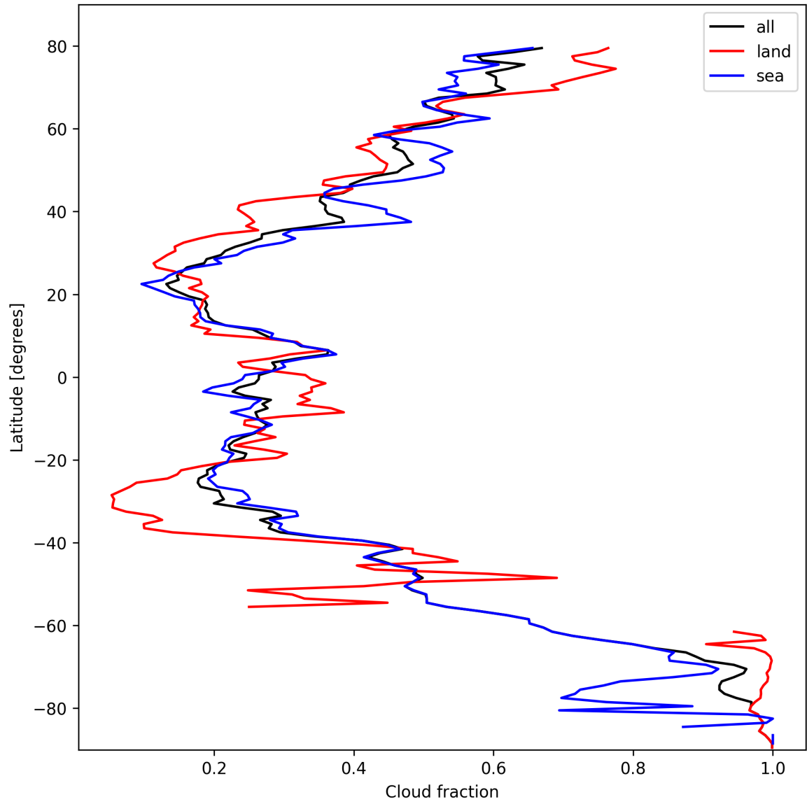
Figure 13: Zonal average of “Cloud fraction” for 2025-10-14 to 2025-10-15.
