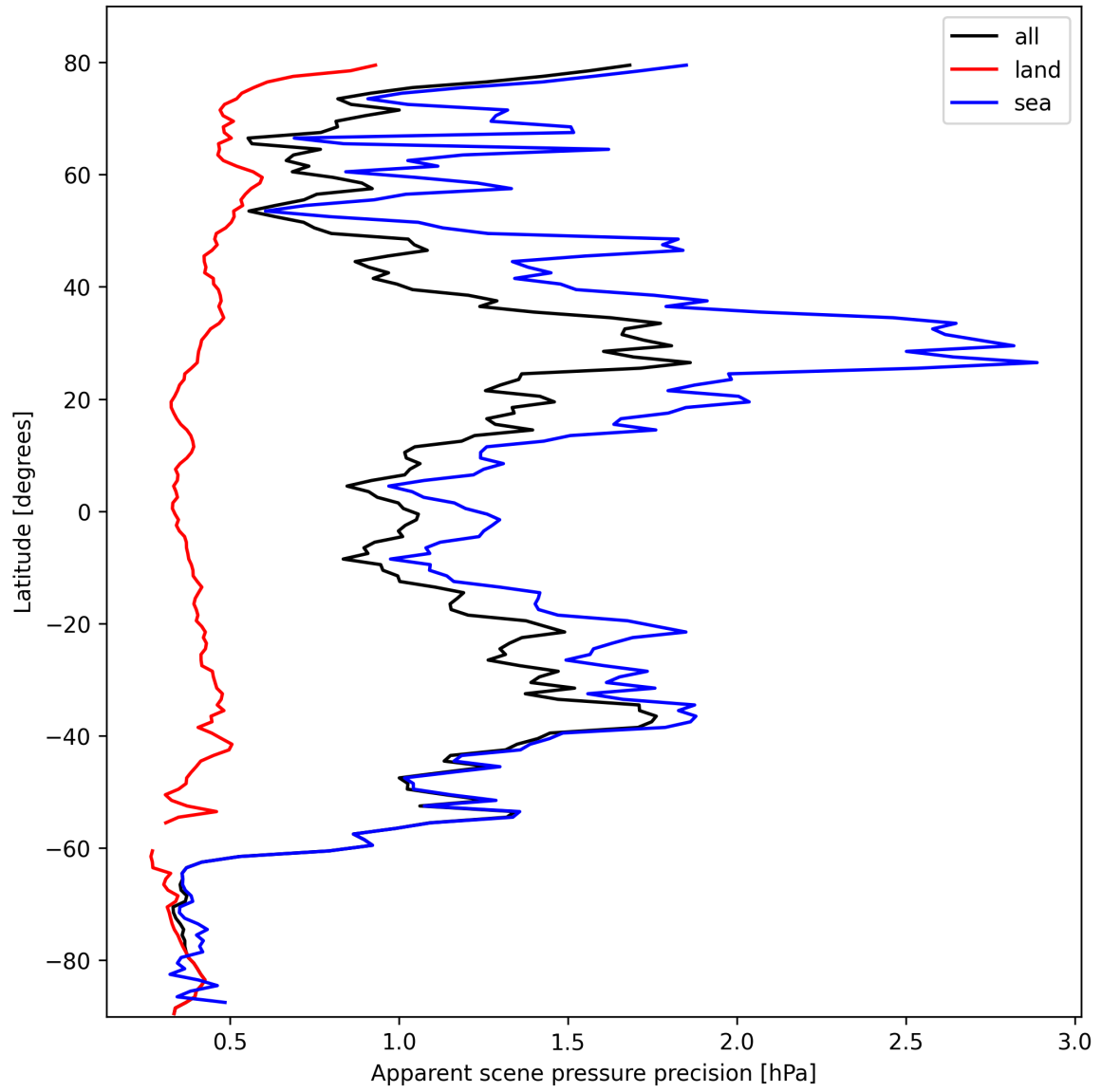
Figure 18: Zonal average of “Apparent scene pressure precision” for 2025-10-15 to 2025-10-15.
