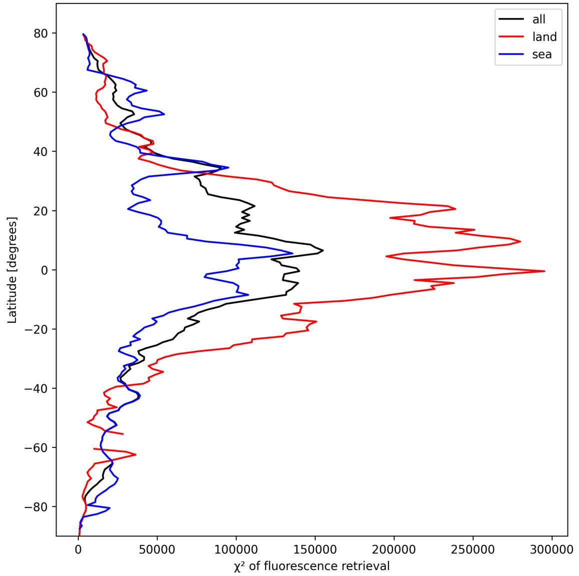
Figure 23: Zonal average of “ \chi^2 of fluorescence retrieval” for 2025-10-15 to 2025-10-15.
