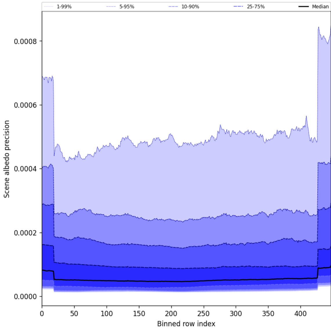
Figure 50: Along track statistics of “Scene albedo precision” for 2025-10-15 to 2025-10-15
