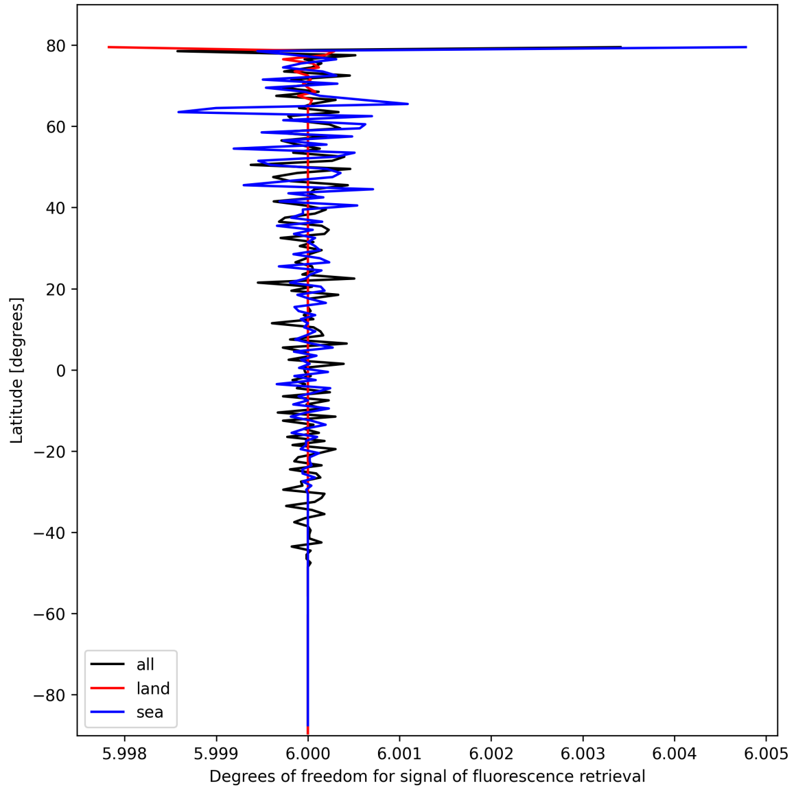
Figure 24: Zonal average of “Degrees of freedom for signal of fluorescence retrieval” for 2025-10-15 to 2025-10-15.
