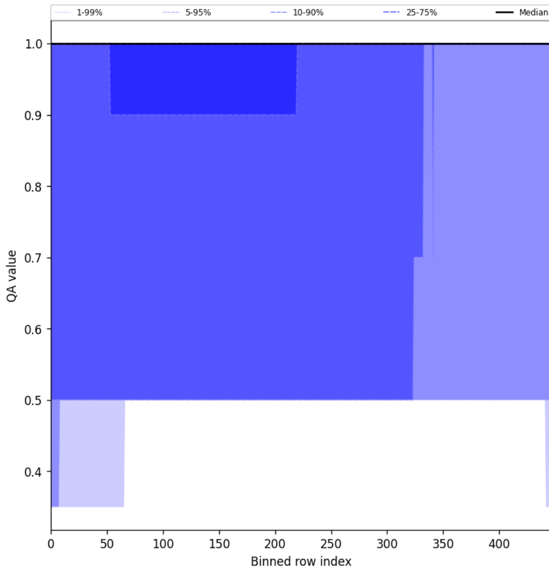
Figure 44: Along track statistics of “QA value” for 2025-10-15 to 2025-10-15
