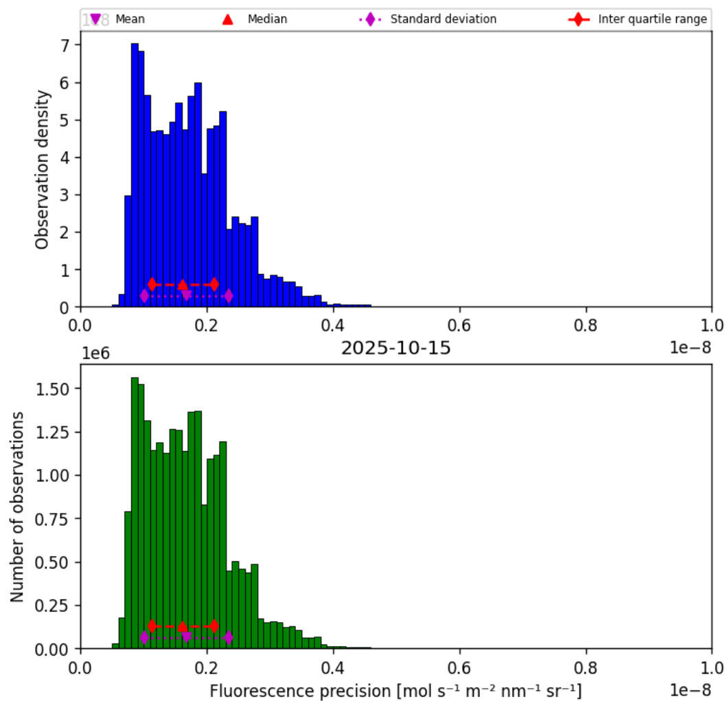
Figure 39: Histogram of “Fluorescence precision” for 2025-10-15 to 2025-10-15
