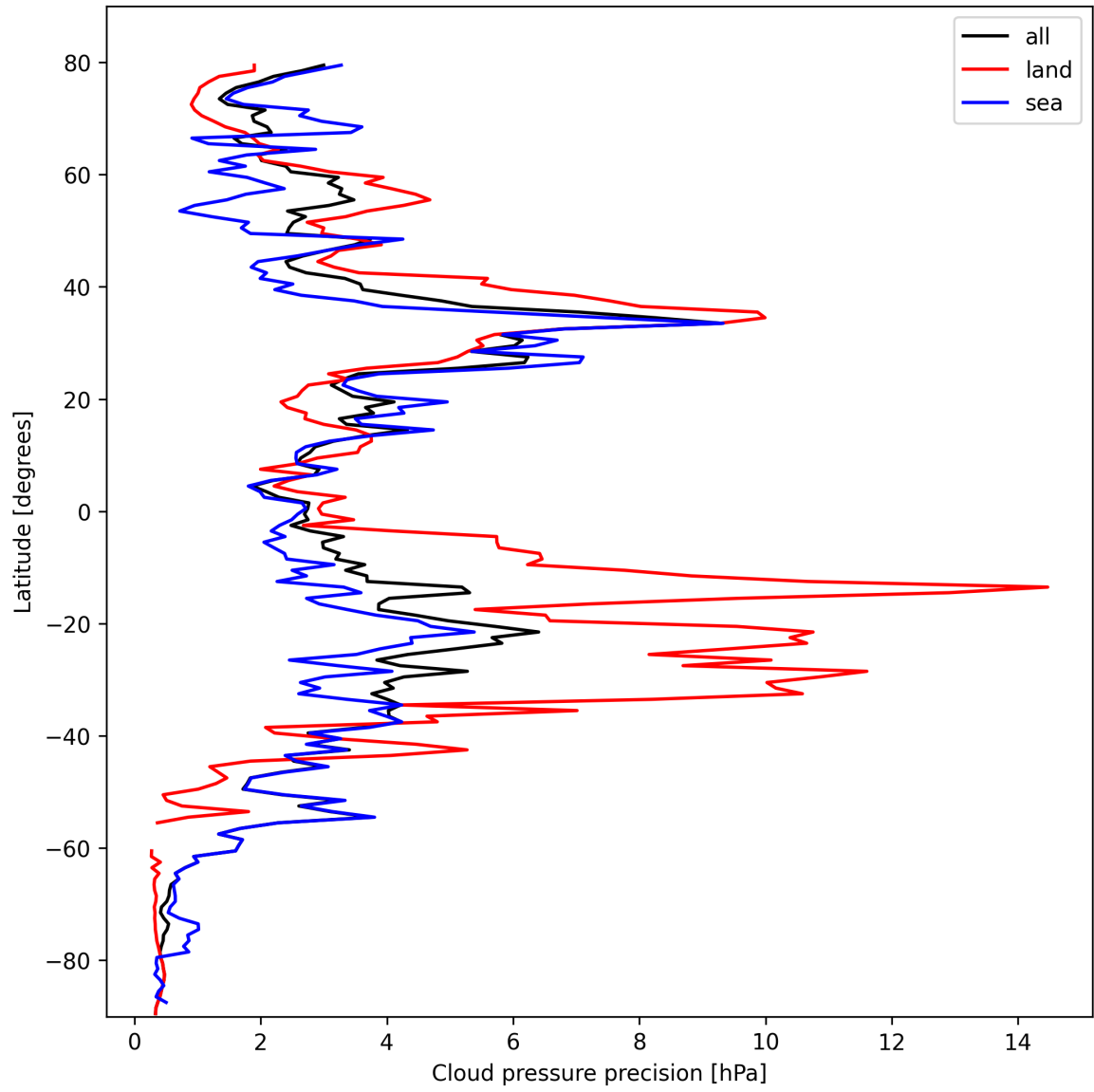
Figure 12: Zonal average of “Cloud pressure precision” for 2025-10-15 to 2025-10-15.
