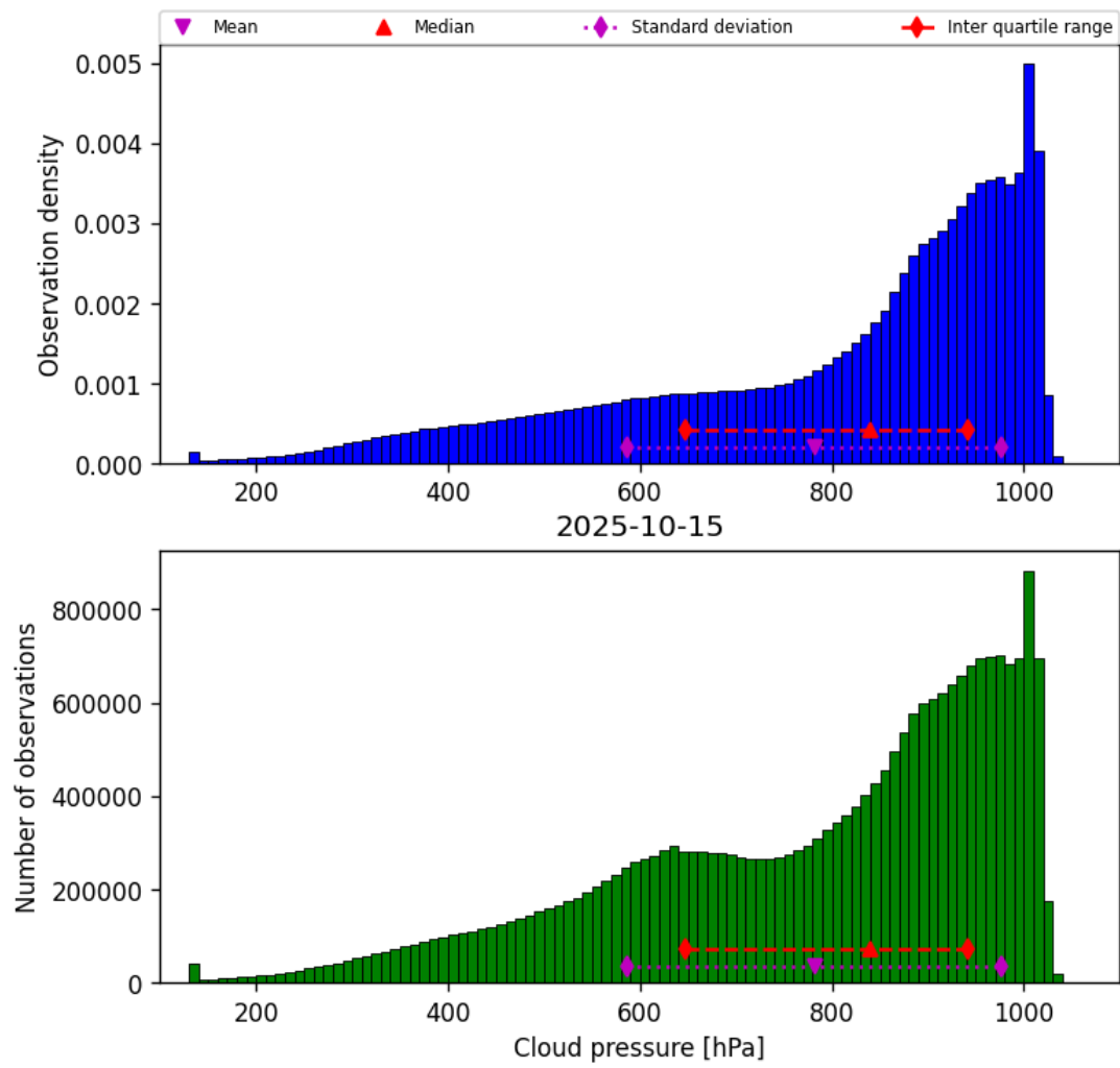
Figure 28: Histogram of “Cloud pressure” for 2025-10-15 to 2025-10-15
