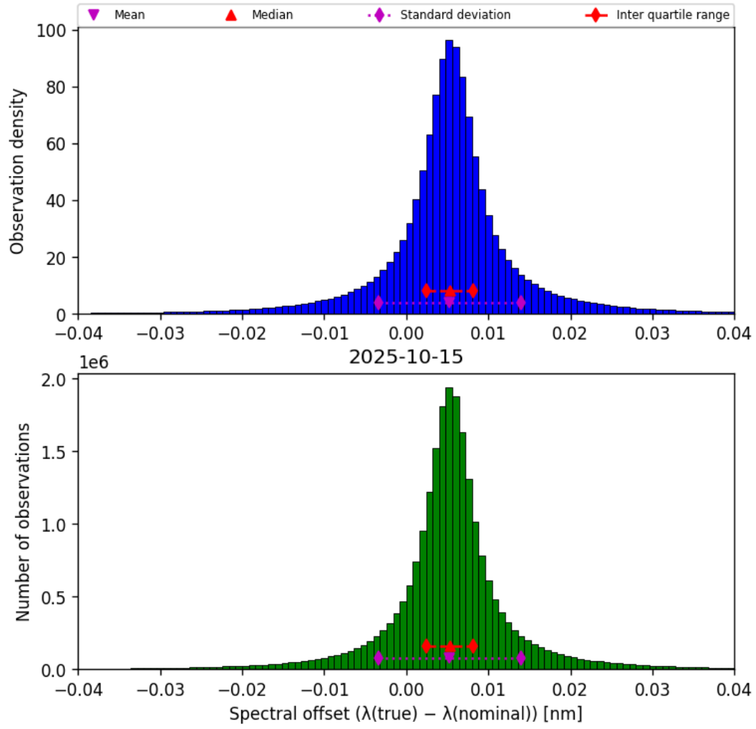
Figure 43: Histogram of “Spectral offset ( \lambda_{\text{true}} - \lambda_{\text{nominal}} )” for 2025-10-15 to 2025-10-15
