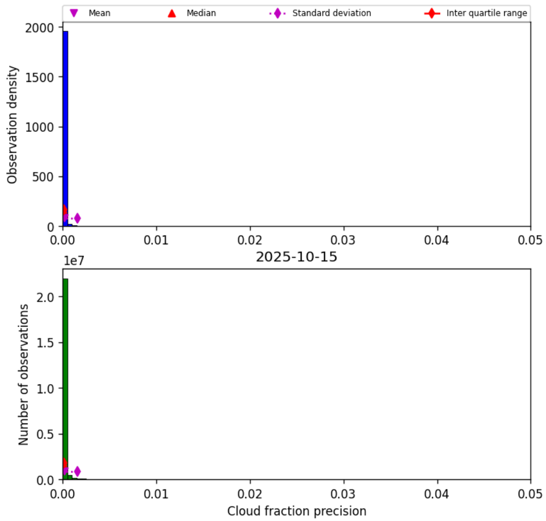
Figure 31: Histogram of “Cloud fraction precision” for 2025-10-15 to 2025-10-15
