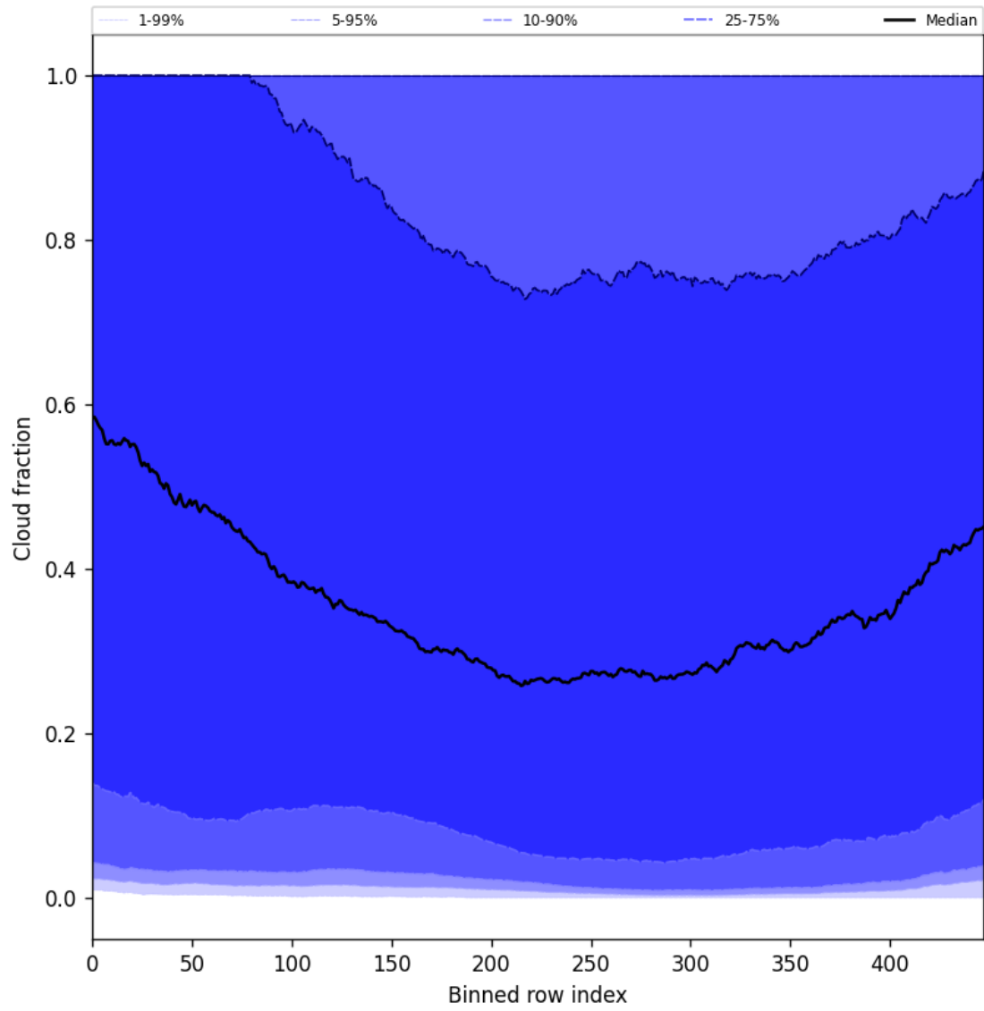
Figure 47: Along track statistics of “Cloud fraction” for 2025-10-15 to 2025-10-15
