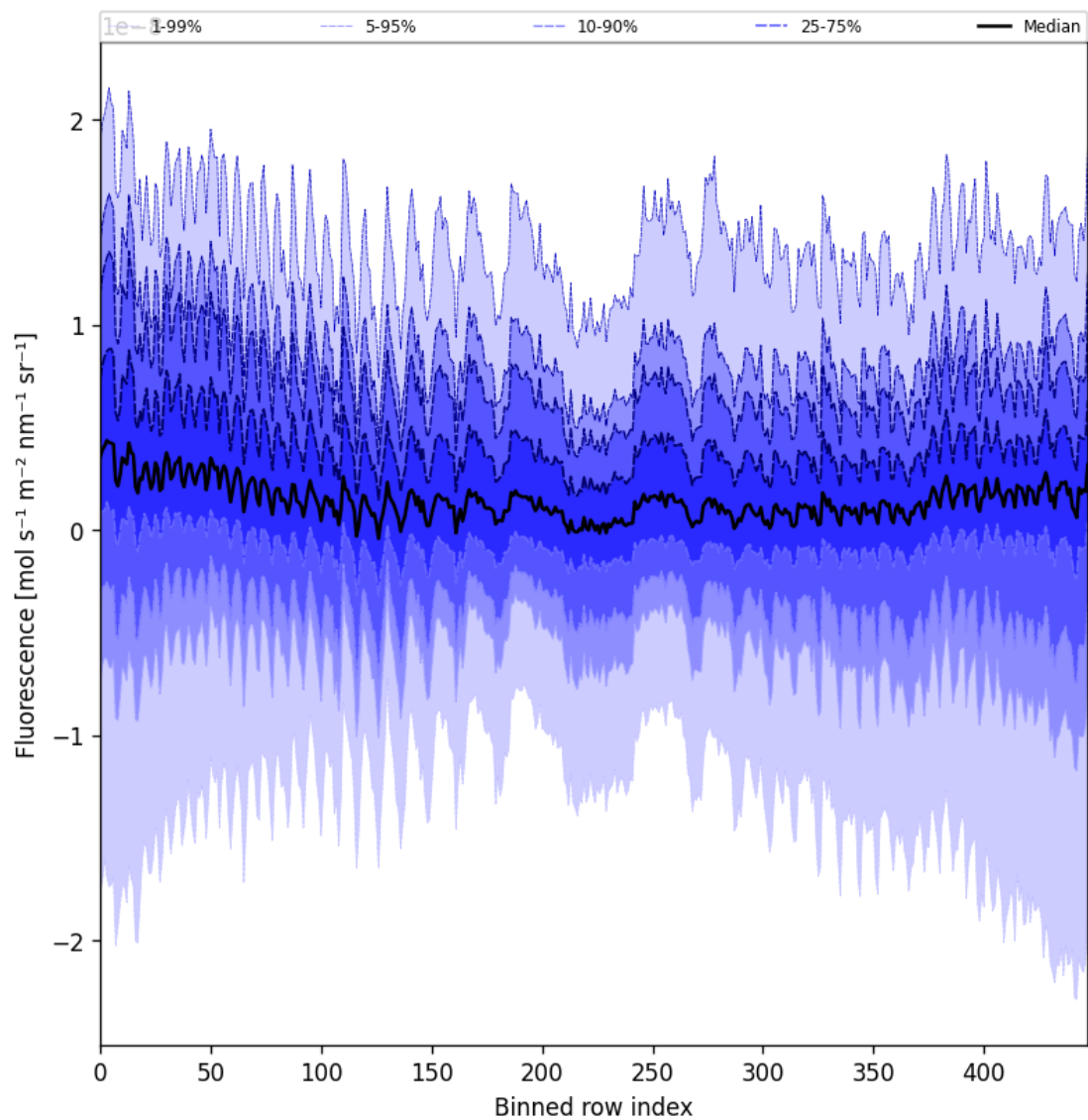
Figure 55: Along track statistics of “Fluorescence” for 2025-10-15 to 2025-10-15
