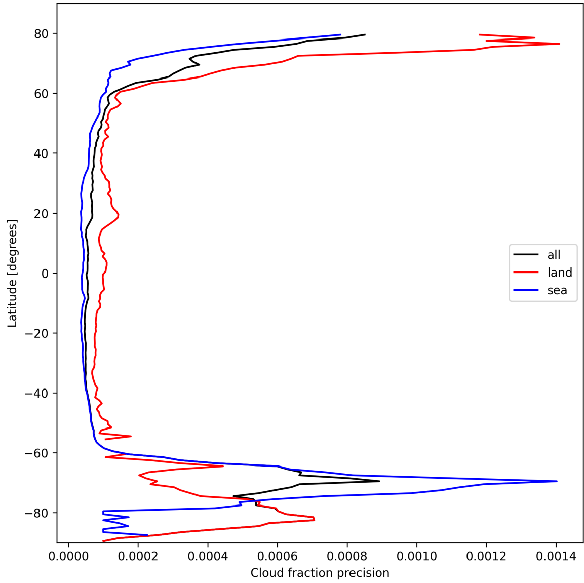
Figure 14: Zonal average of “Cloud fraction precision” for 2025-10-15 to 2025-10-15.
