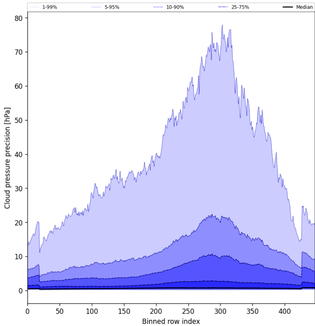
Figure 46: Along track statistics of “Cloud pressure precision” for 2025-10-15 to 2025-10-15
