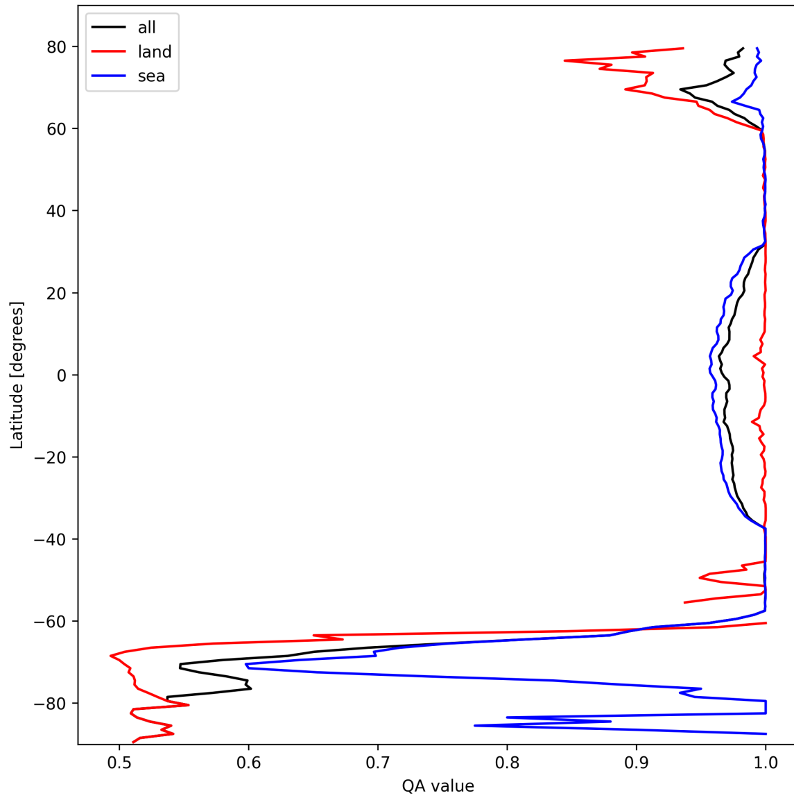
Figure 10: Zonal average of “QA value” for 2025-10-15 to 2025-10-15.
