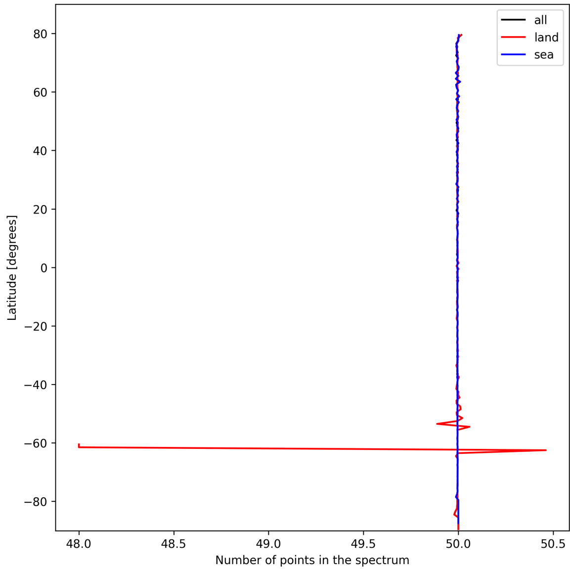
Figure 25: Zonal average of “Number of points in the spectrum” for 2025-10-15 to 2025-10-15.
