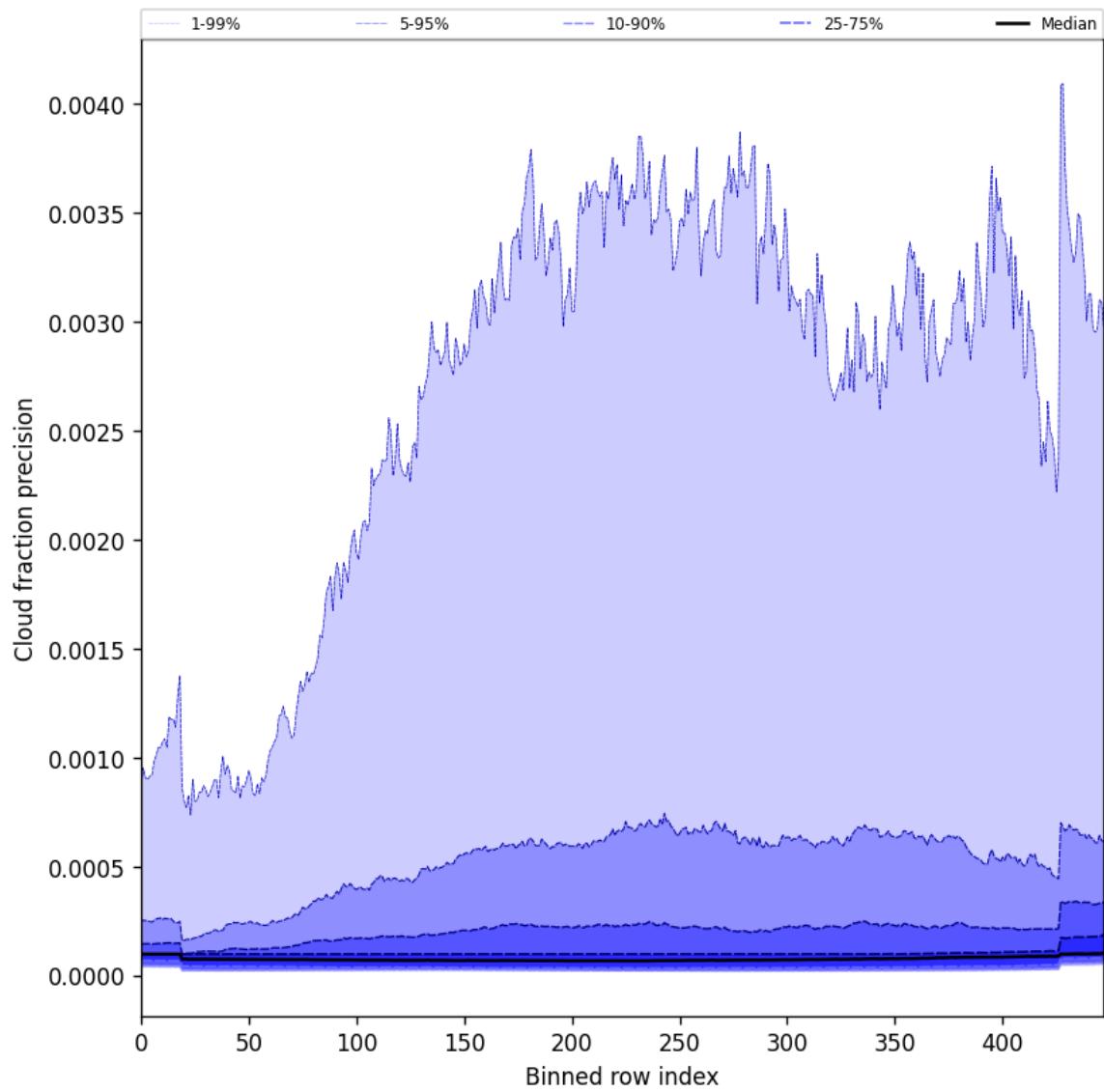
Figure 48: Along track statistics of “Cloud fraction precision” for 2025-10-15 to 2025-10-15
