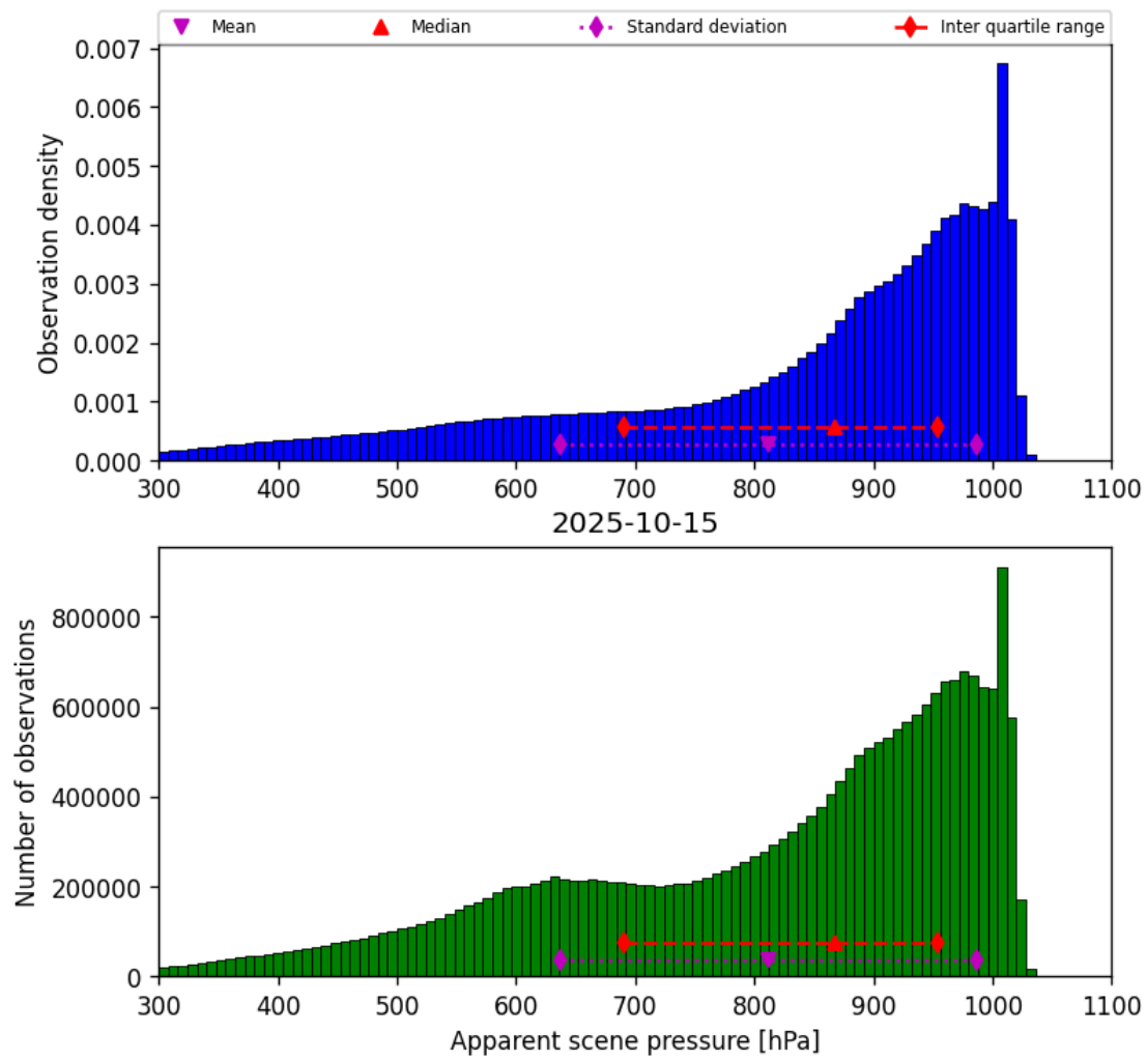
Figure 34: Histogram of “Apparent scene pressure” for 2025-10-15 to 2025-10-15
