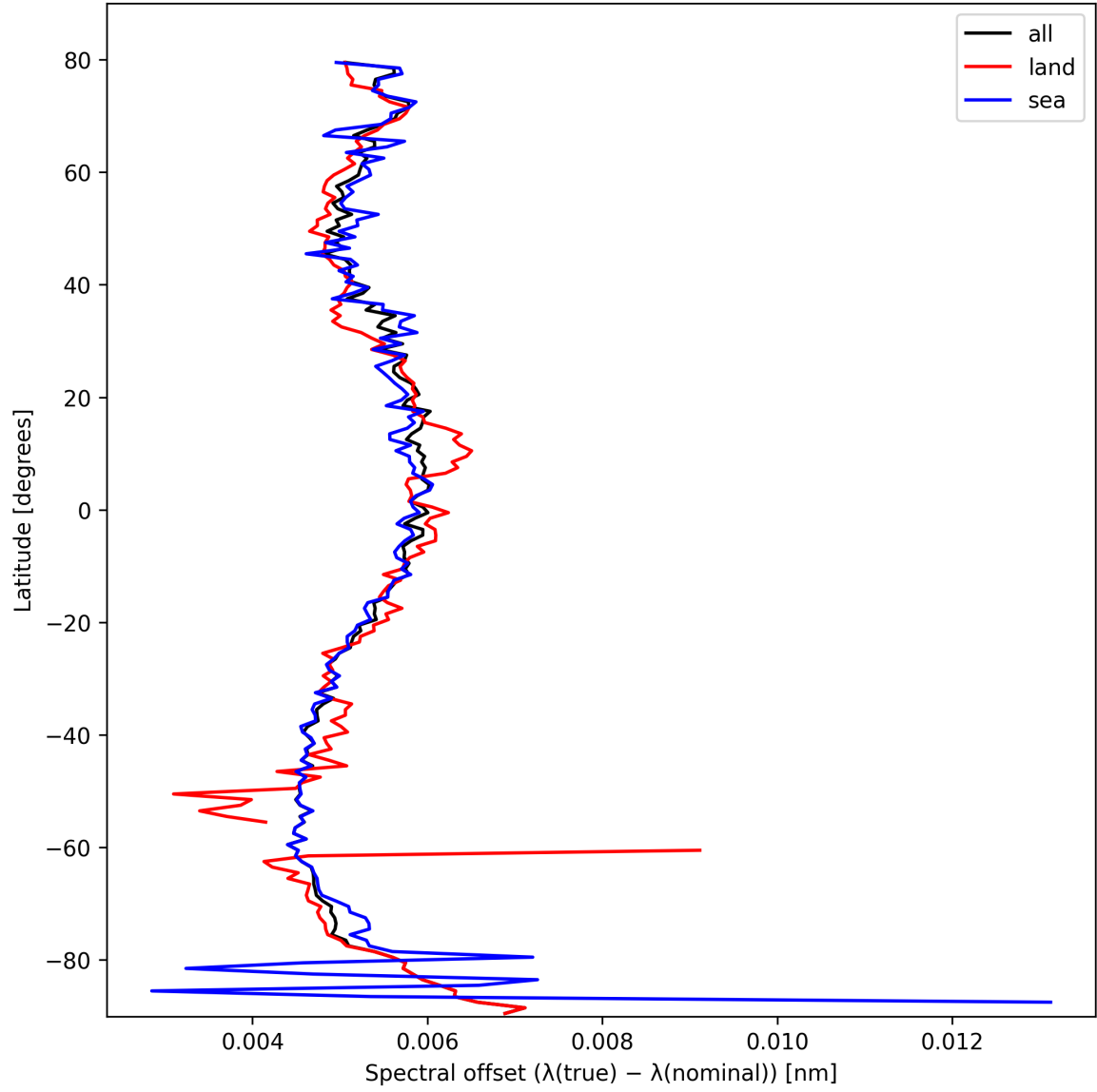
Figure 26: Zonal average of “Spectral offset ( \lambda_{\text{true}} - \lambda_{\text{nominal}} )” for 2025-10-15 to 2025-10-15.
