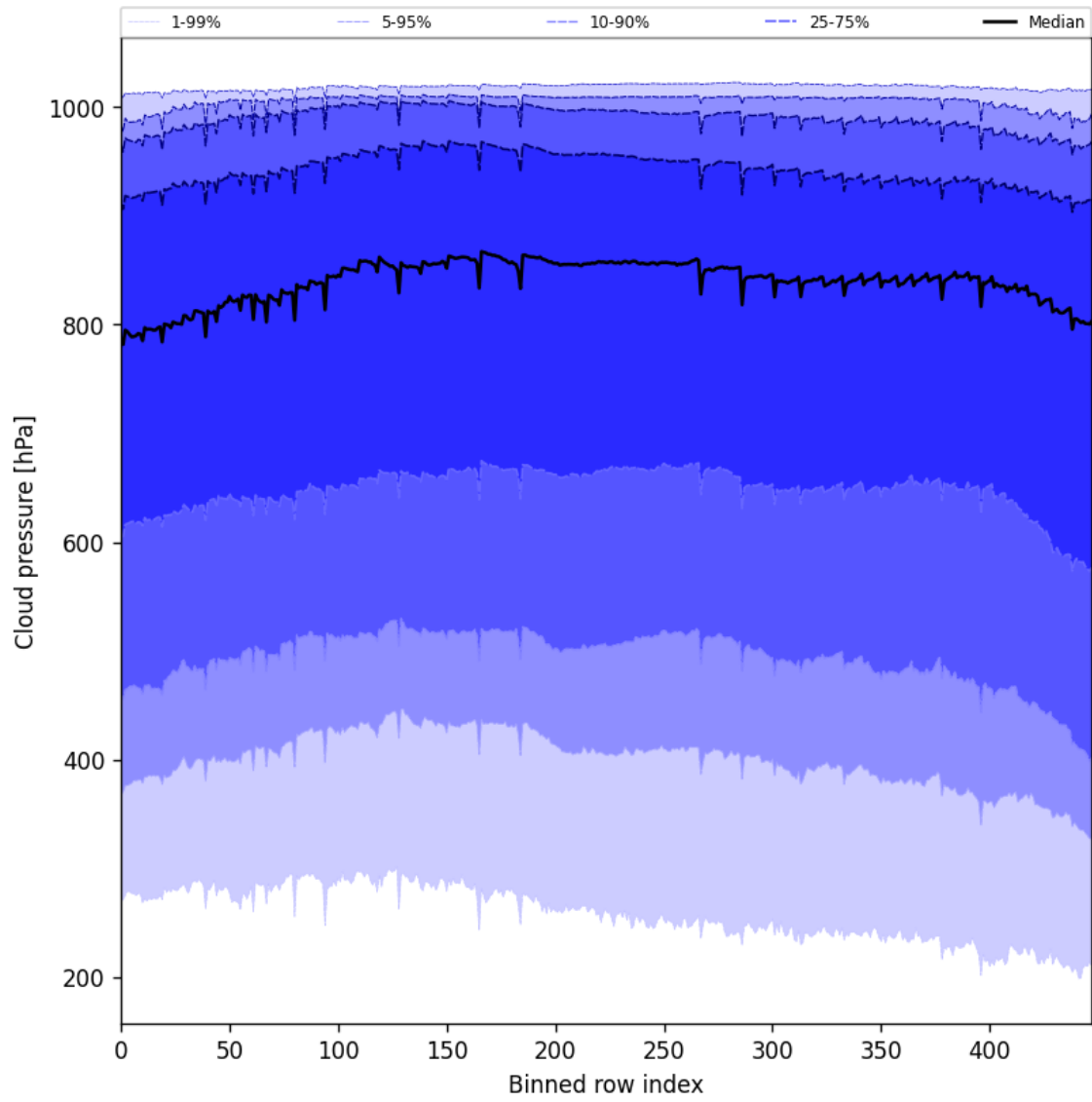
Figure 45: Along track statistics of “Cloud pressure” for 2025-10-15 to 2025-10-15
