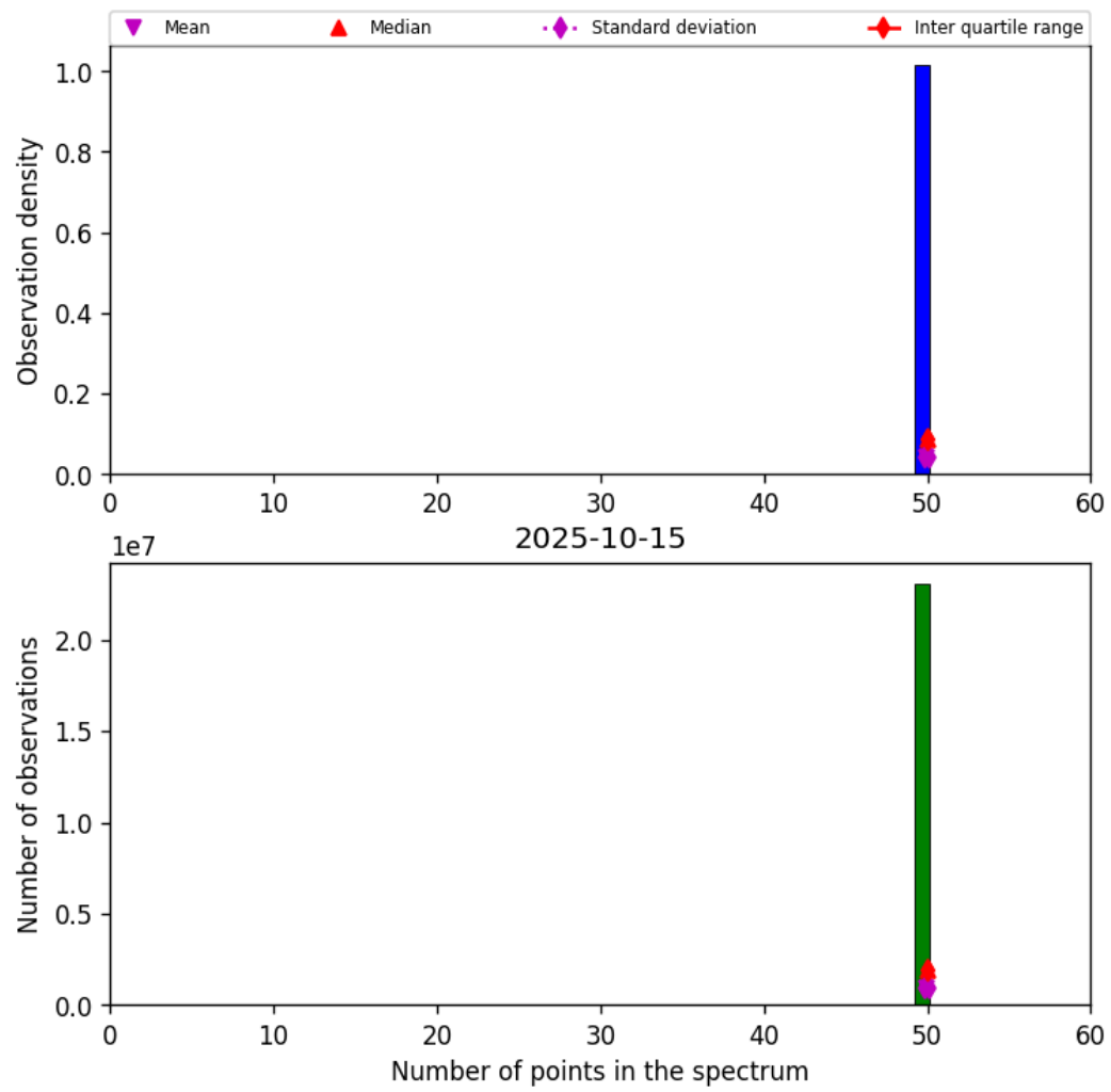
Figure 42: Histogram of “Number of points in the spectrum” for 2025-10-15 to 2025-10-15
