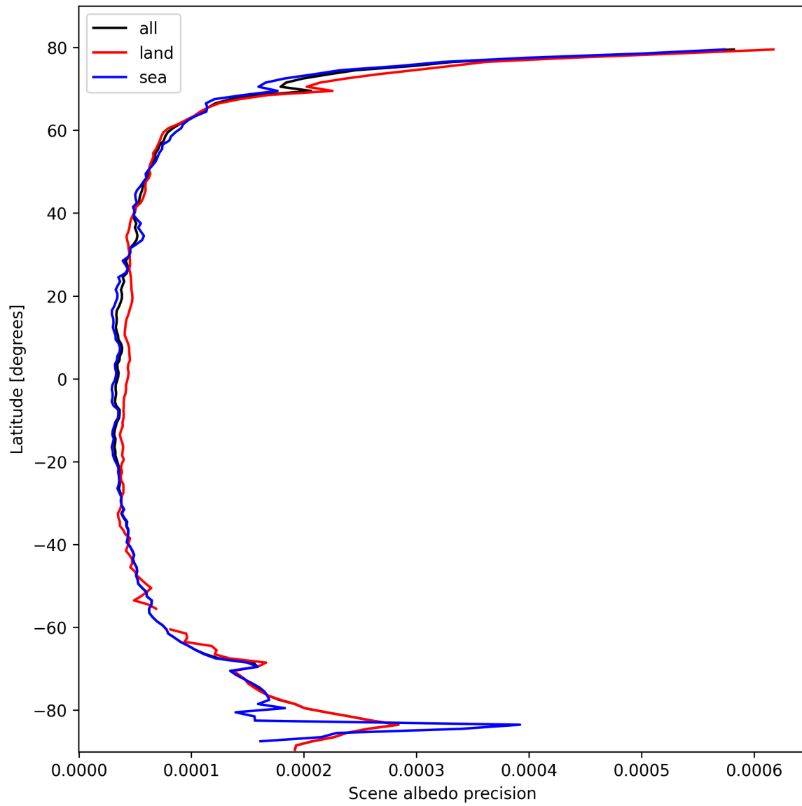
Figure 16: Zonal average of “Scene albedo precision” for 2025-10-15 to 2025-10-15.
