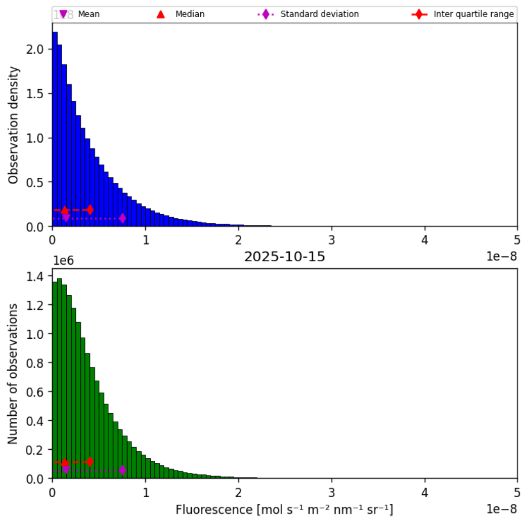
Figure 38: Histogram of “Fluorescence” for 2025-10-15 to 2025-10-15
