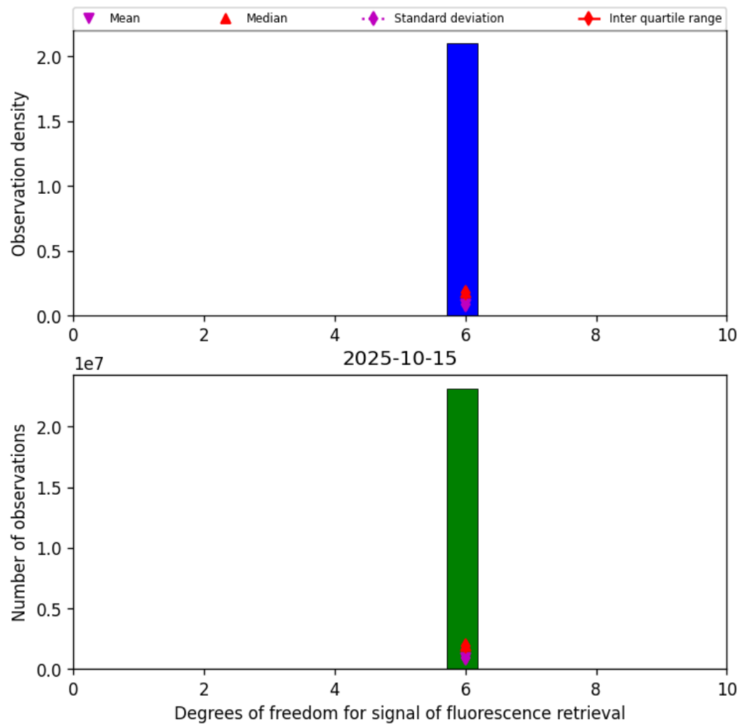
Figure 41: Histogram of “Degrees of freedom for signal of fluorescence retrieval” for 2025-10-15 to 2025-10-15
