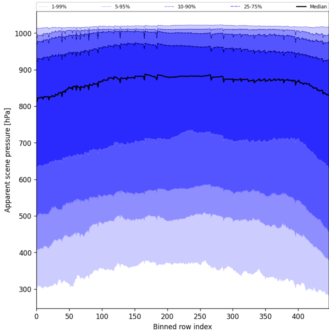
Figure 51: Along track statistics of “Apparent scene pressure” for 2025-10-15 to 2025-10-15
