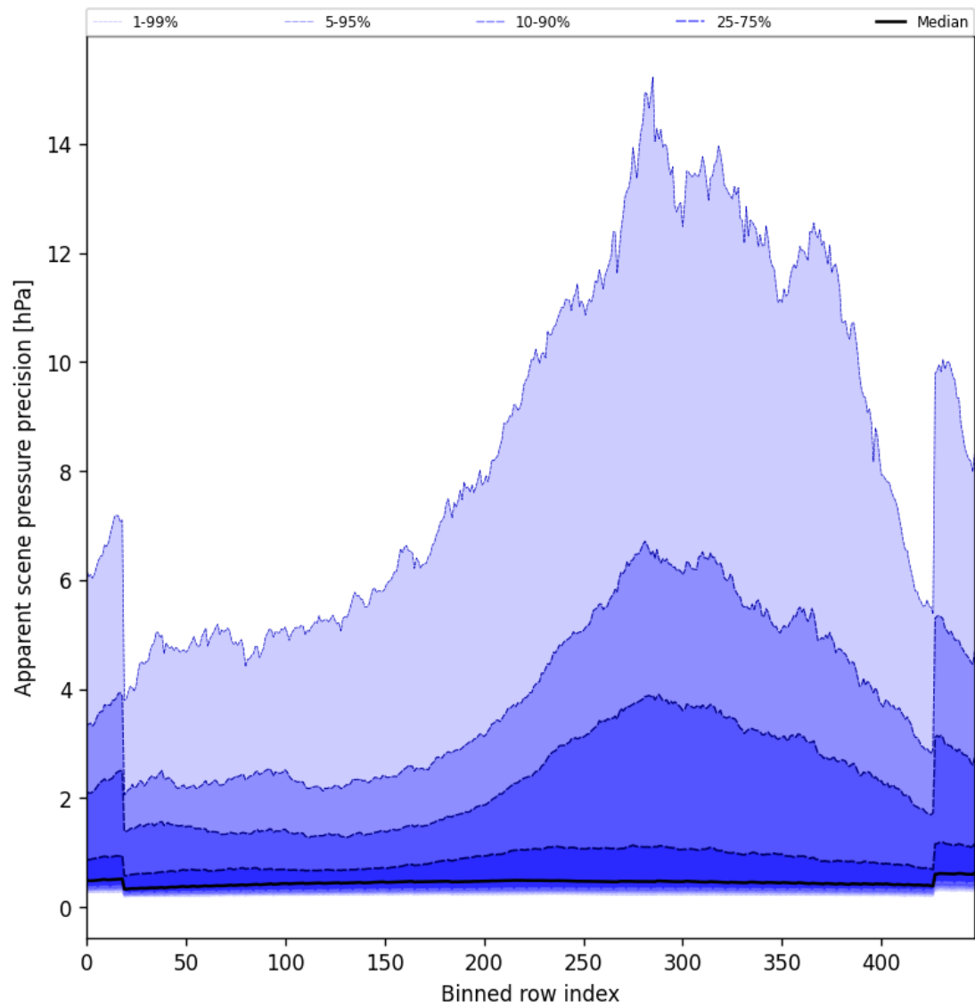
Figure 52: Along track statistics of “Apparent scene pressure precision” for 2025-10-15 to 2025-10-15
