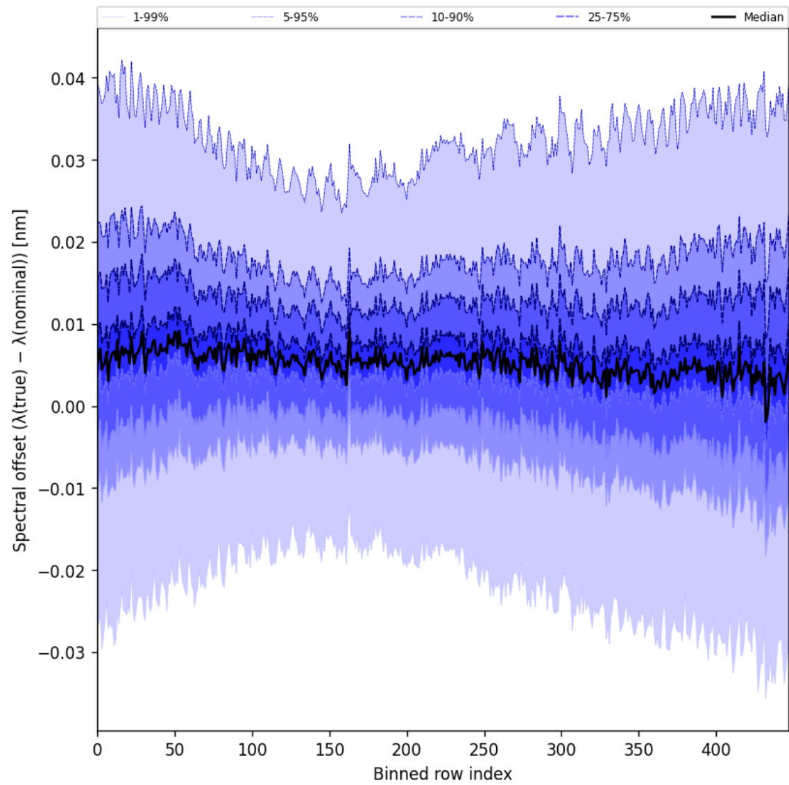
Figure 60: Along track statistics of “Spectral offset ( \lambda_{\text{true}} - \lambda_{\text{nominal}} )” for 2025-10-15 to 2025-10-15
