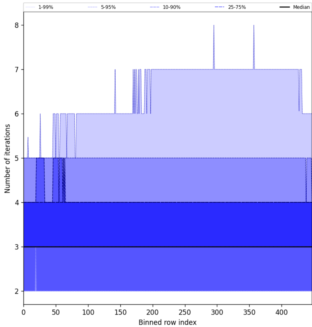
Figure 54: Along track statistics of “Number of iterations” for 2025-10-15 to 2025-10-15
