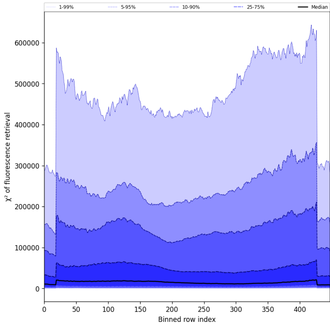
Figure 57: Along track statistics of “ \chi^2 of fluorescence retrieval” for 2025-10-15 to 2025-10-15
