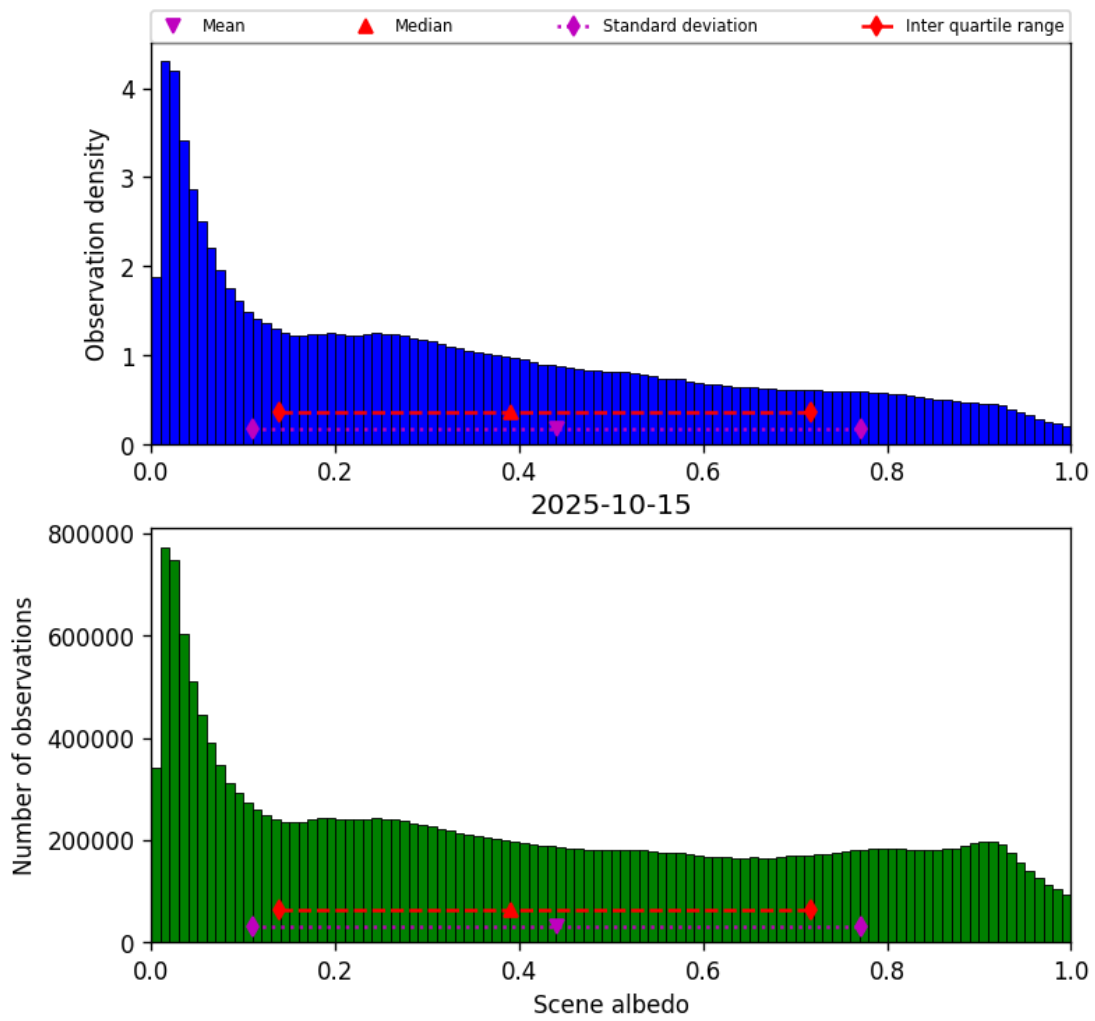
Figure 32: Histogram of “Scene albedo” for 2025-10-15 to 2025-10-15
