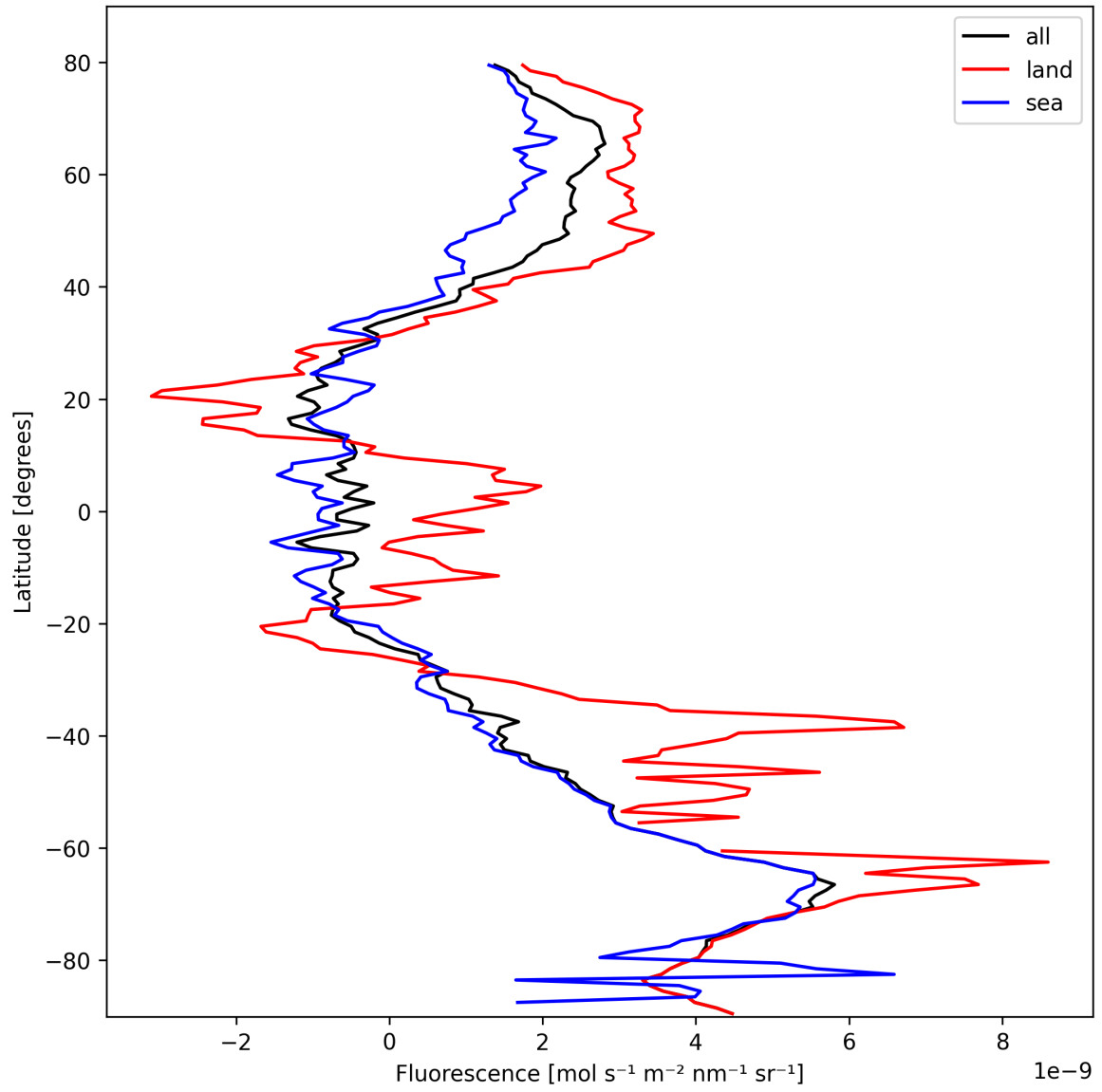
Figure 21: Zonal average of “Fluorescence” for 2025-10-15 to 2025-10-15.
