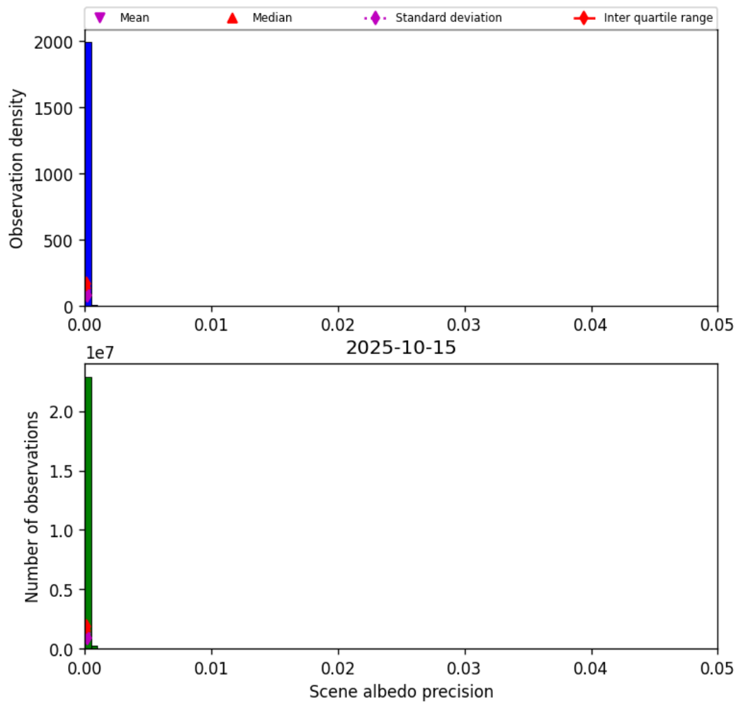
Figure 33: Histogram of “Scene albedo precision” for 2025-10-15 to 2025-10-15
