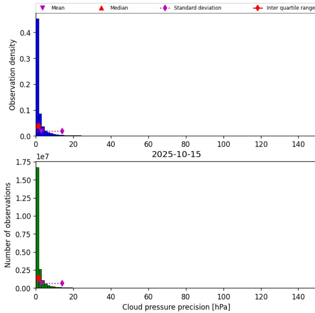
Figure 29: Histogram of “Cloud pressure precision” for 2025-10-15 to 2025-10-15
