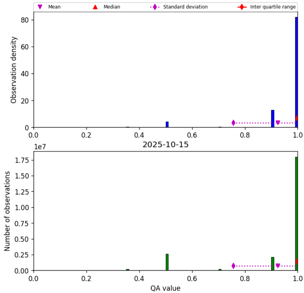
Figure 27: Histogram of “QA value” for 2025-10-15 to 2025-10-15
