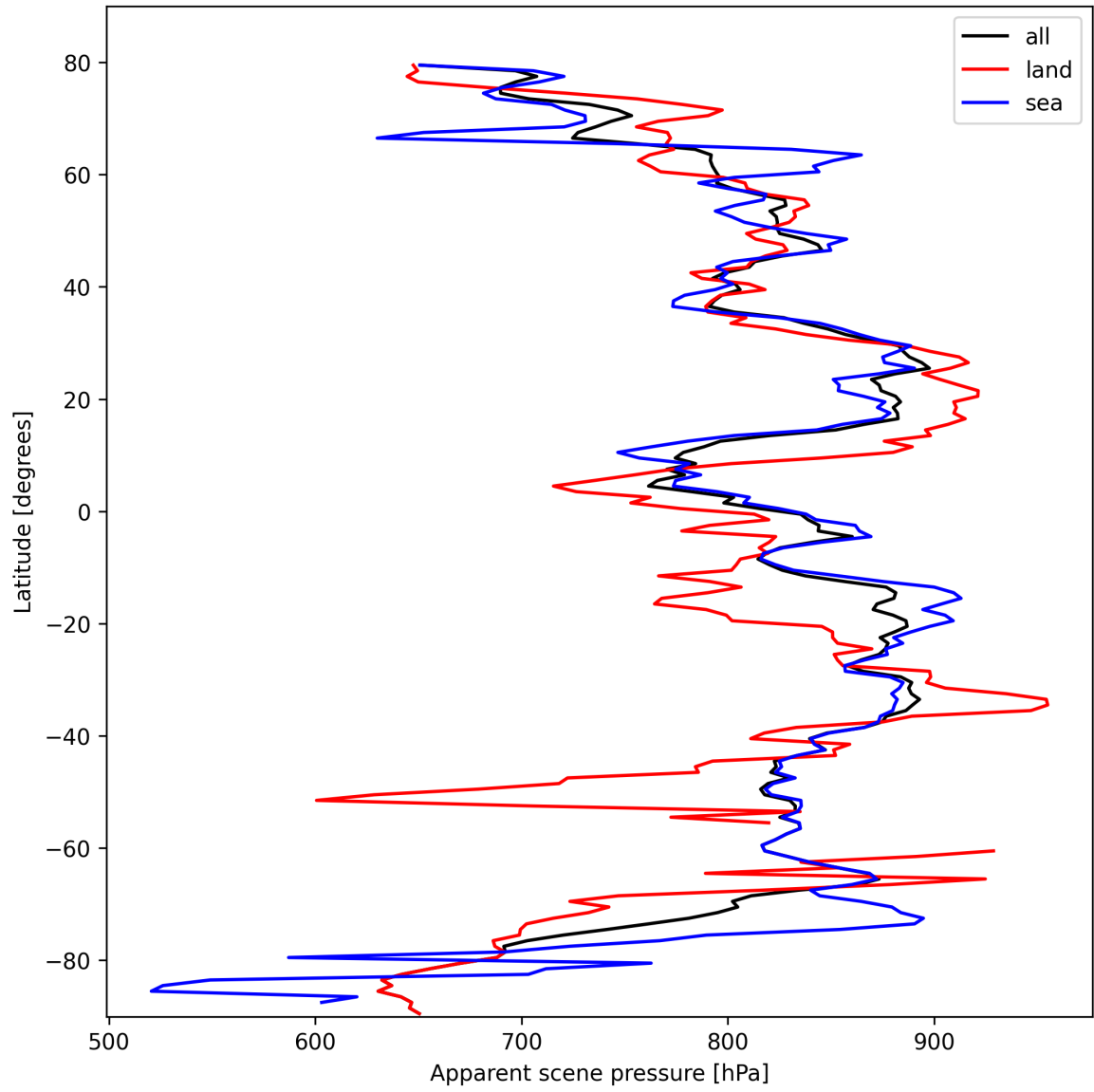
Figure 17: Zonal average of “Apparent scene pressure” for 2025-10-15 to 2025-10-15.
