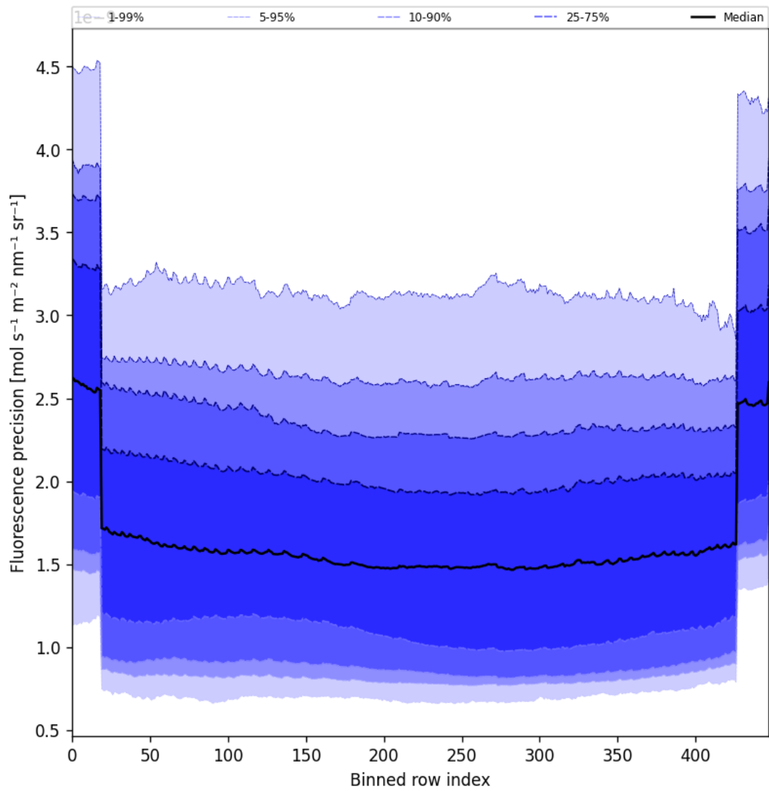
Figure 56: Along track statistics of “Fluorescence precision” for 2025-10-15 to 2025-10-15
