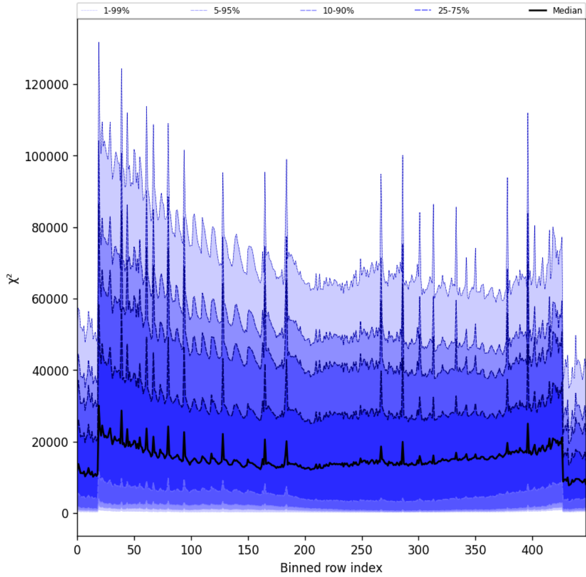
Figure 53: Along track statistics of “ \chi^2 ” for 2025-10-15 to 2025-10-15
