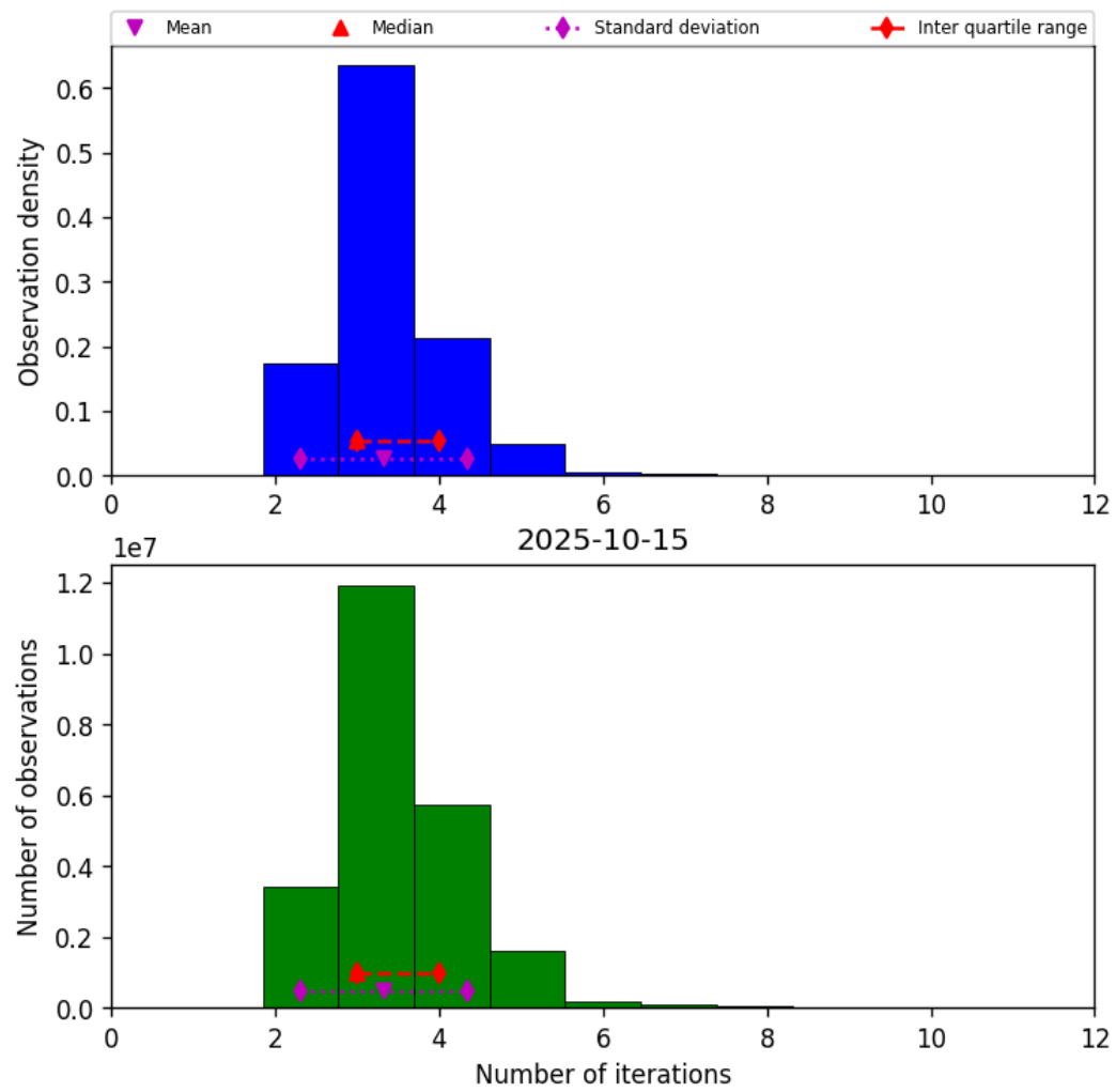
Figure 37: Histogram of “Number of iterations” for 2025-10-15 to 2025-10-15
