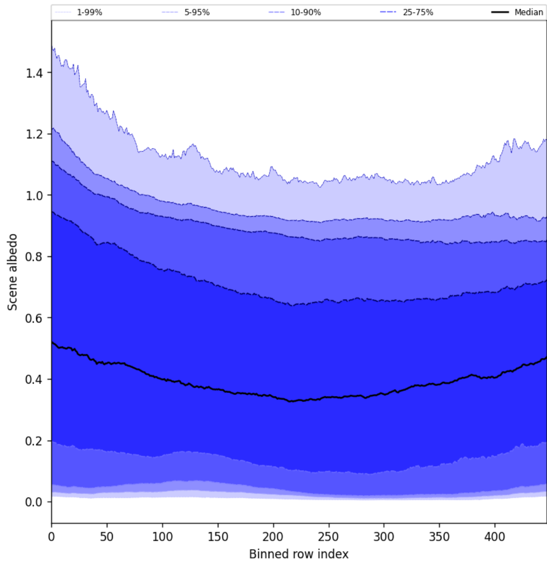
Figure 49: Along track statistics of “Scene albedo” for 2025-10-15 to 2025-10-15
