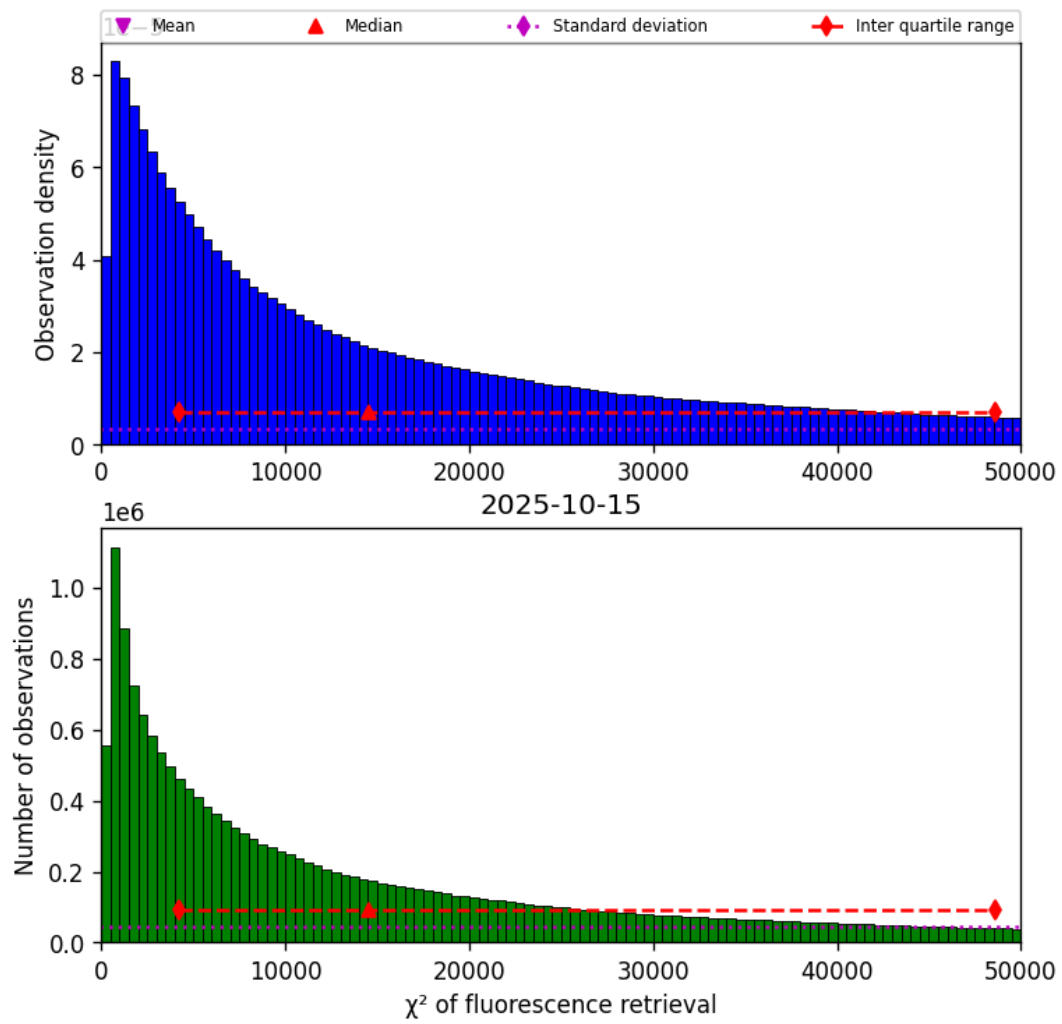
Figure 40: Histogram of “ \chi^2 of fluorescence retrieval” for 2025-10-15 to 2025-10-15
