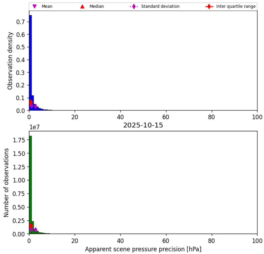
Figure 35: Histogram of “Apparent scene pressure precision” for 2025-10-15 to 2025-10-15
