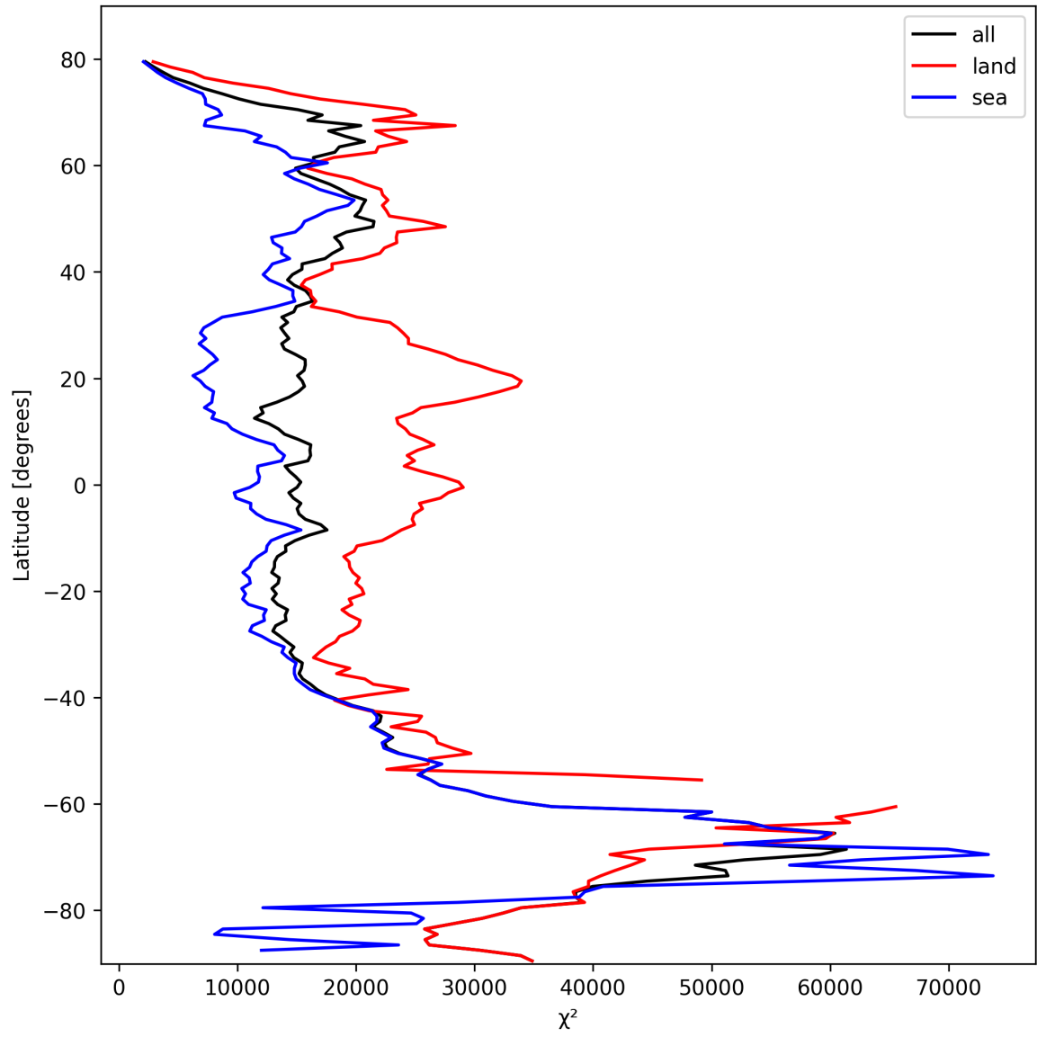
Figure 19: Zonal average of “ \chi^2 ” for 2025-10-15 to 2025-10-15.
