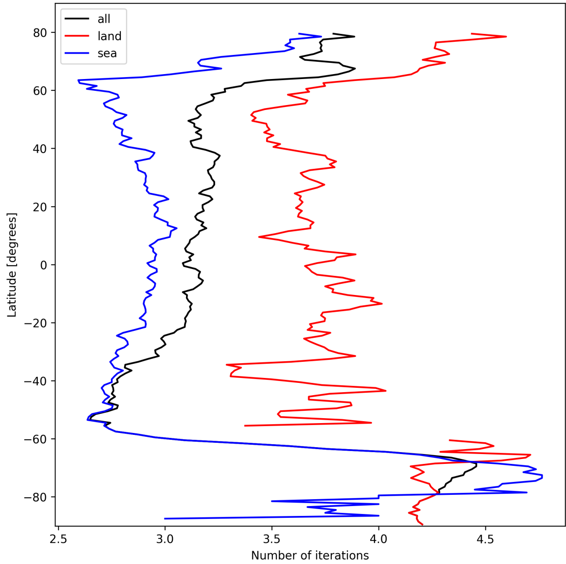
Figure 20: Zonal average of “Number of iterations” for 2025-10-15 to 2025-10-15.
