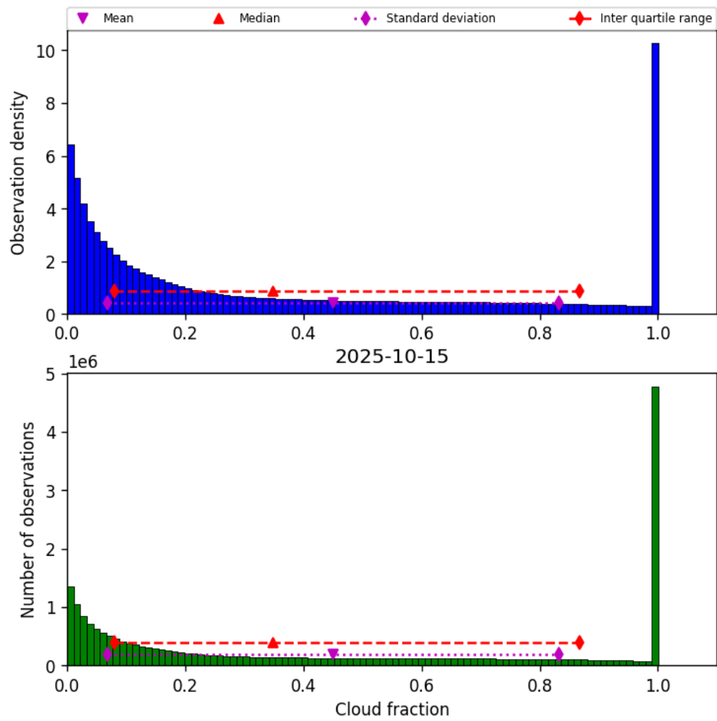
Figure 30: Histogram of “Cloud fraction” for 2025-10-15 to 2025-10-15
