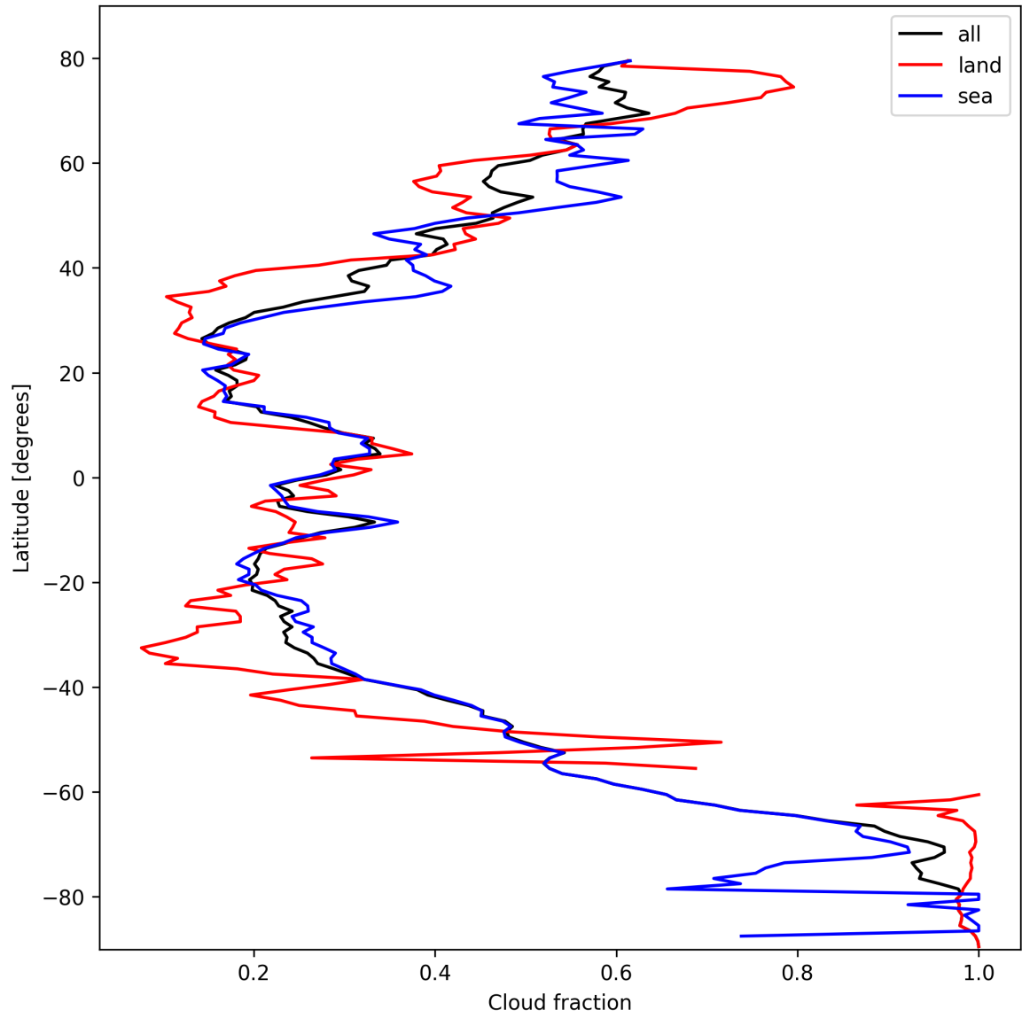
Figure 13: Zonal average of “Cloud fraction” for 2025-10-15 to 2025-10-15.
