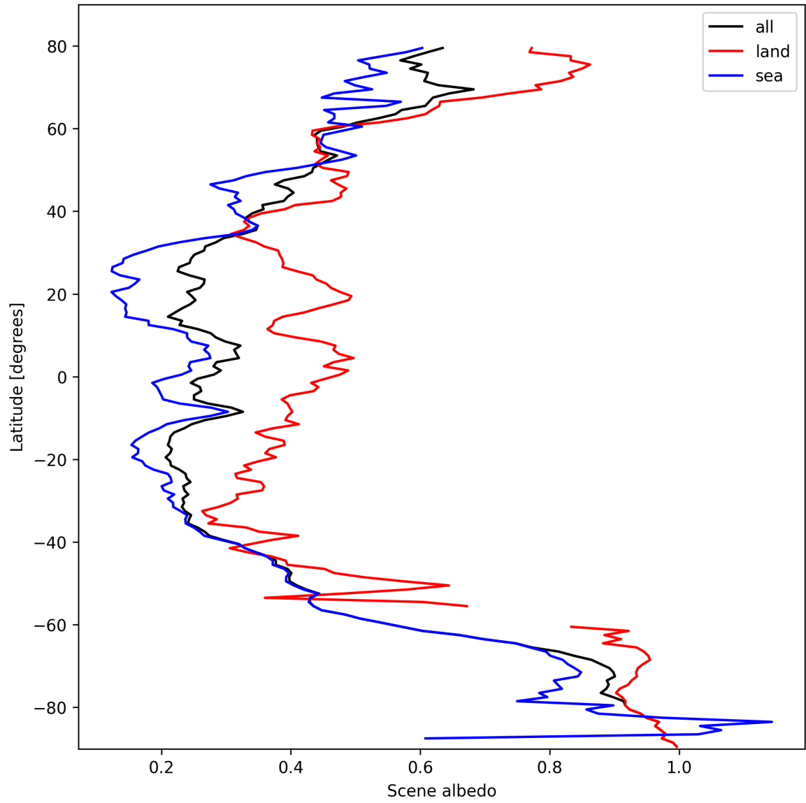
Figure 15: Zonal average of “Scene albedo” for 2025-10-15 to 2025-10-15.
