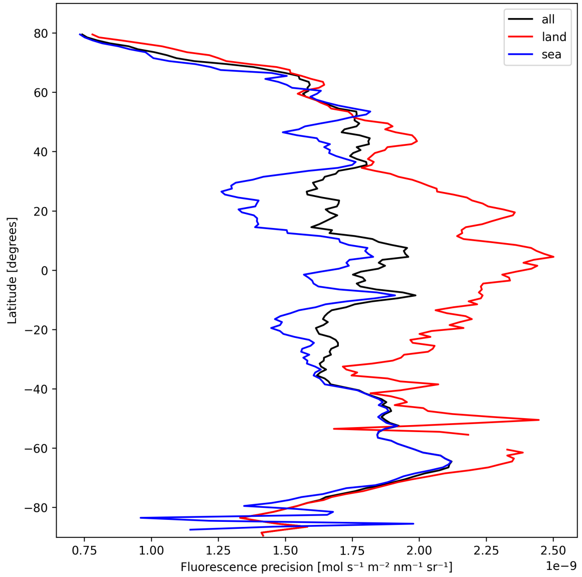
Figure 22: Zonal average of “Fluorescence precision” for 2025-10-15 to 2025-10-15.
