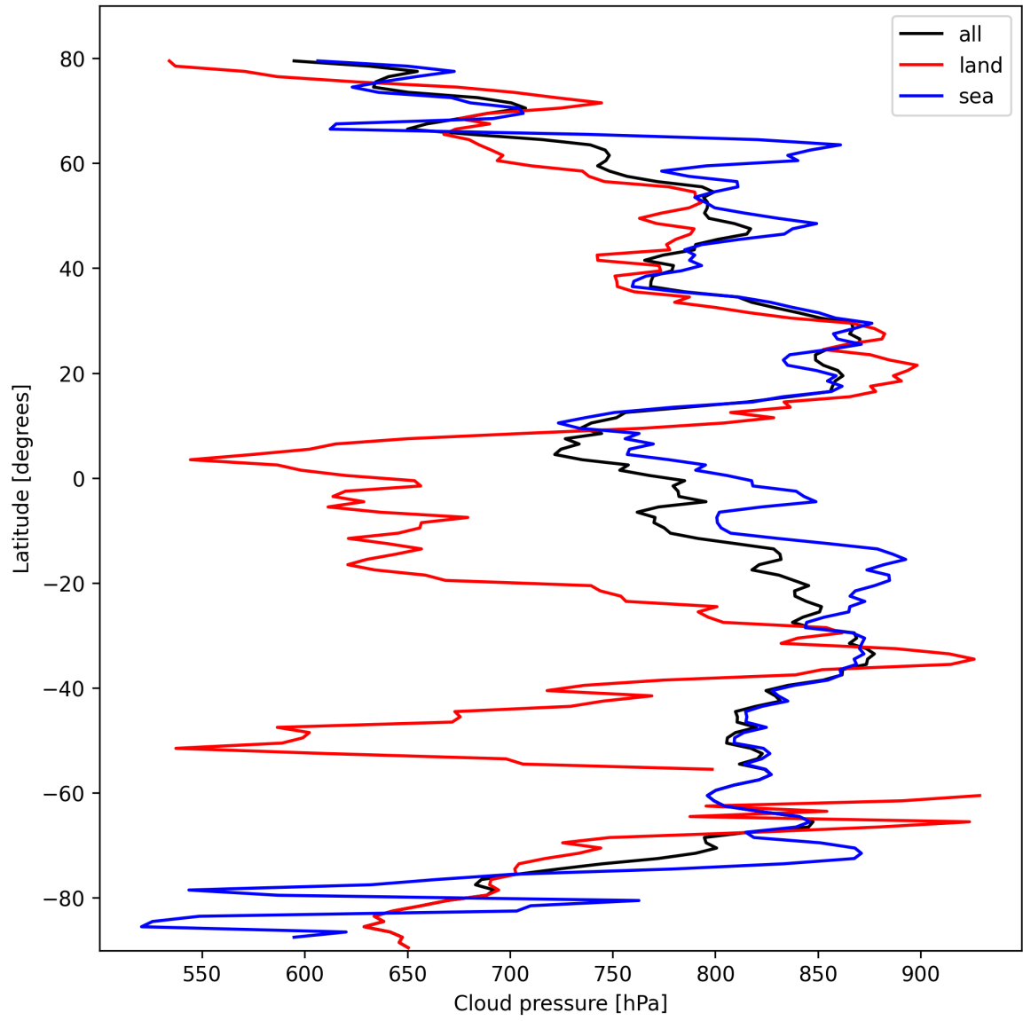
Figure 11: Zonal average of “Cloud pressure” for 2025-10-15 to 2025-10-15.
