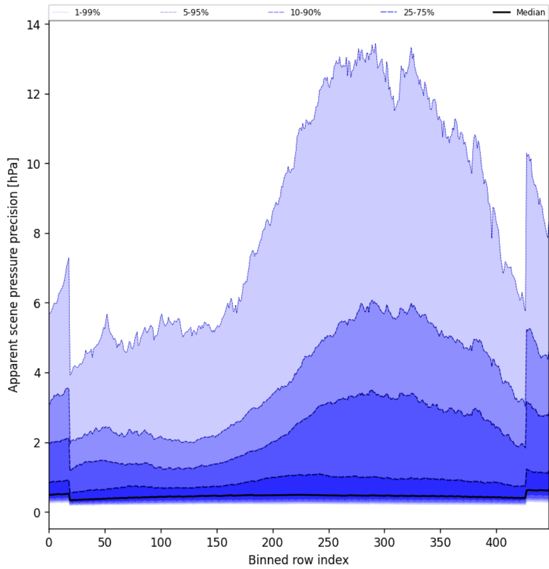
Figure 52: Along track statistics of “Apparent scene pressure precision” for 2025-10-16 to 2025-10-17
