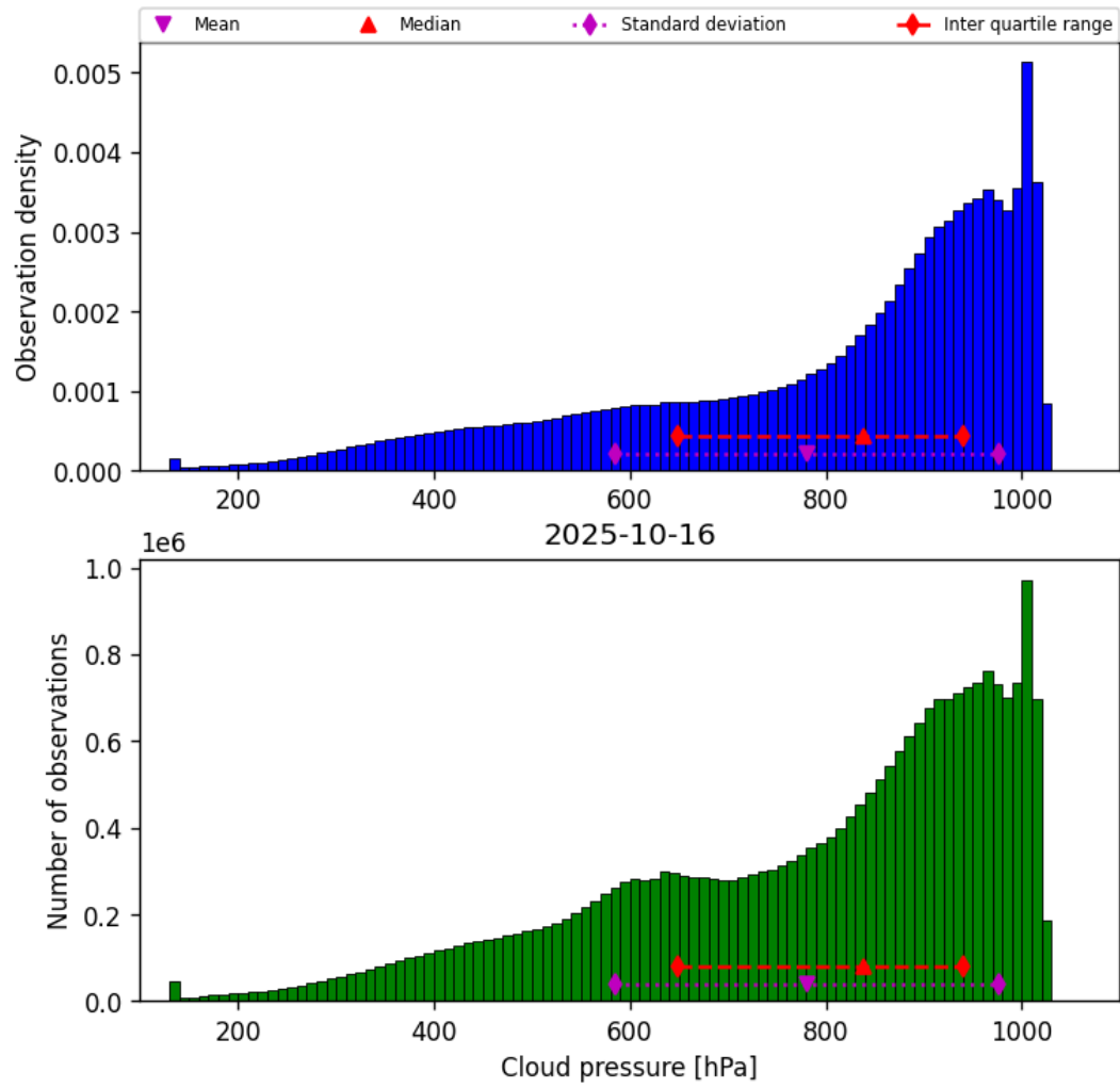
Figure 28: Histogram of “Cloud pressure” for 2025-10-16 to 2025-10-17
