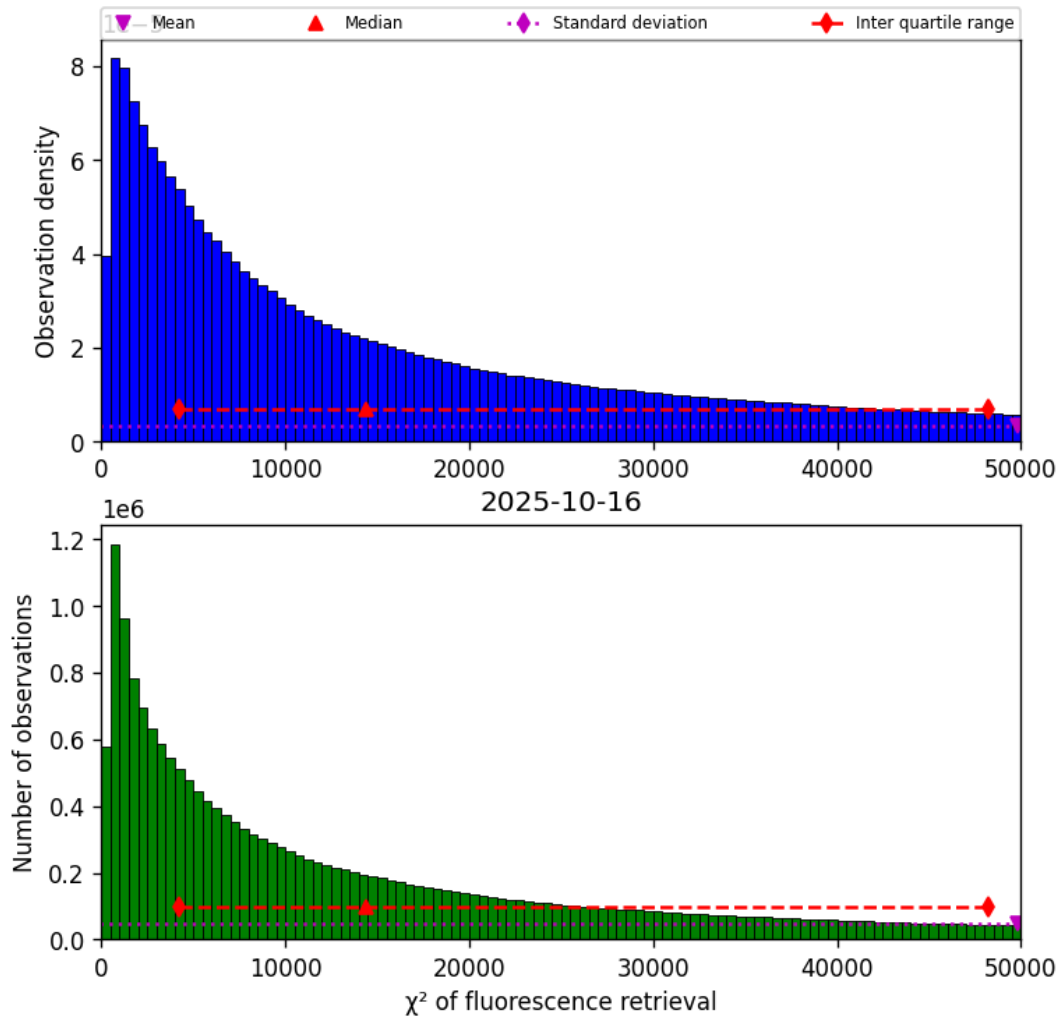
Figure 40: Histogram of “ \chi^2 of fluorescence retrieval” for 2025-10-16 to 2025-10-17
