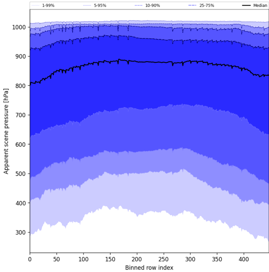
Figure 51: Along track statistics of “Apparent scene pressure” for 2025-10-16 to 2025-10-17
