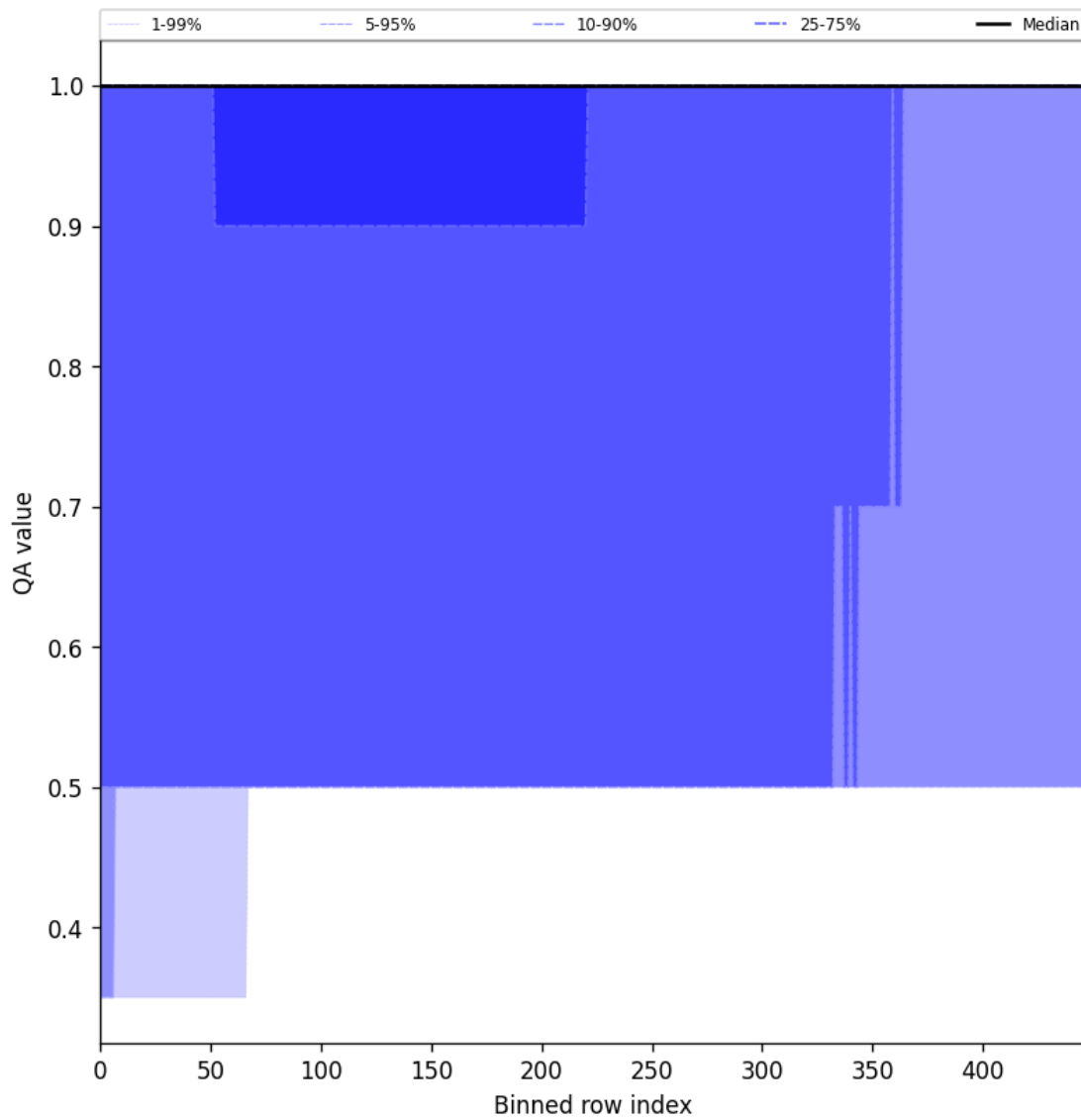
Figure 44: Along track statistics of “QA value” for 2025-10-16 to 2025-10-17
