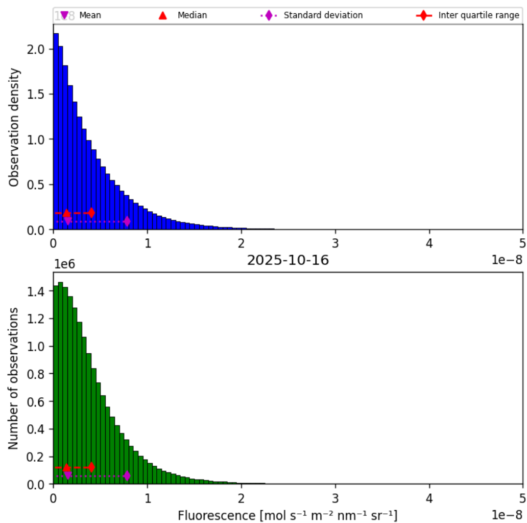
Figure 38: Histogram of “Fluorescence” for 2025-10-16 to 2025-10-17
