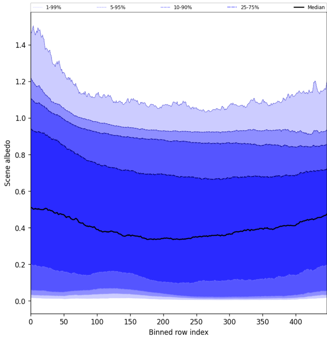
Figure 49: Along track statistics of “Scene albedo” for 2025-10-16 to 2025-10-17
