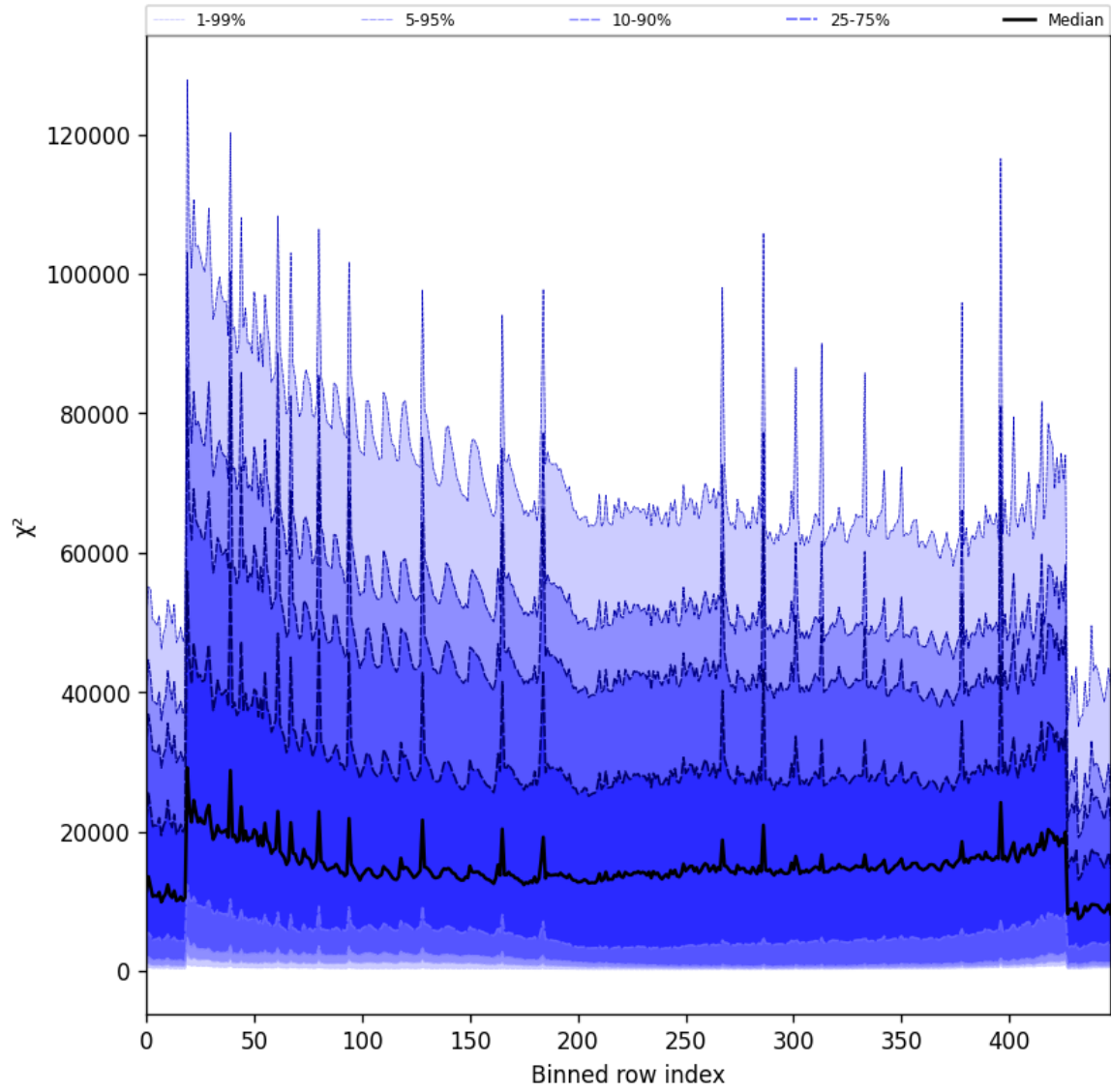
Figure 53: Along track statistics of “ \chi^2 ” for 2025-10-16 to 2025-10-17
