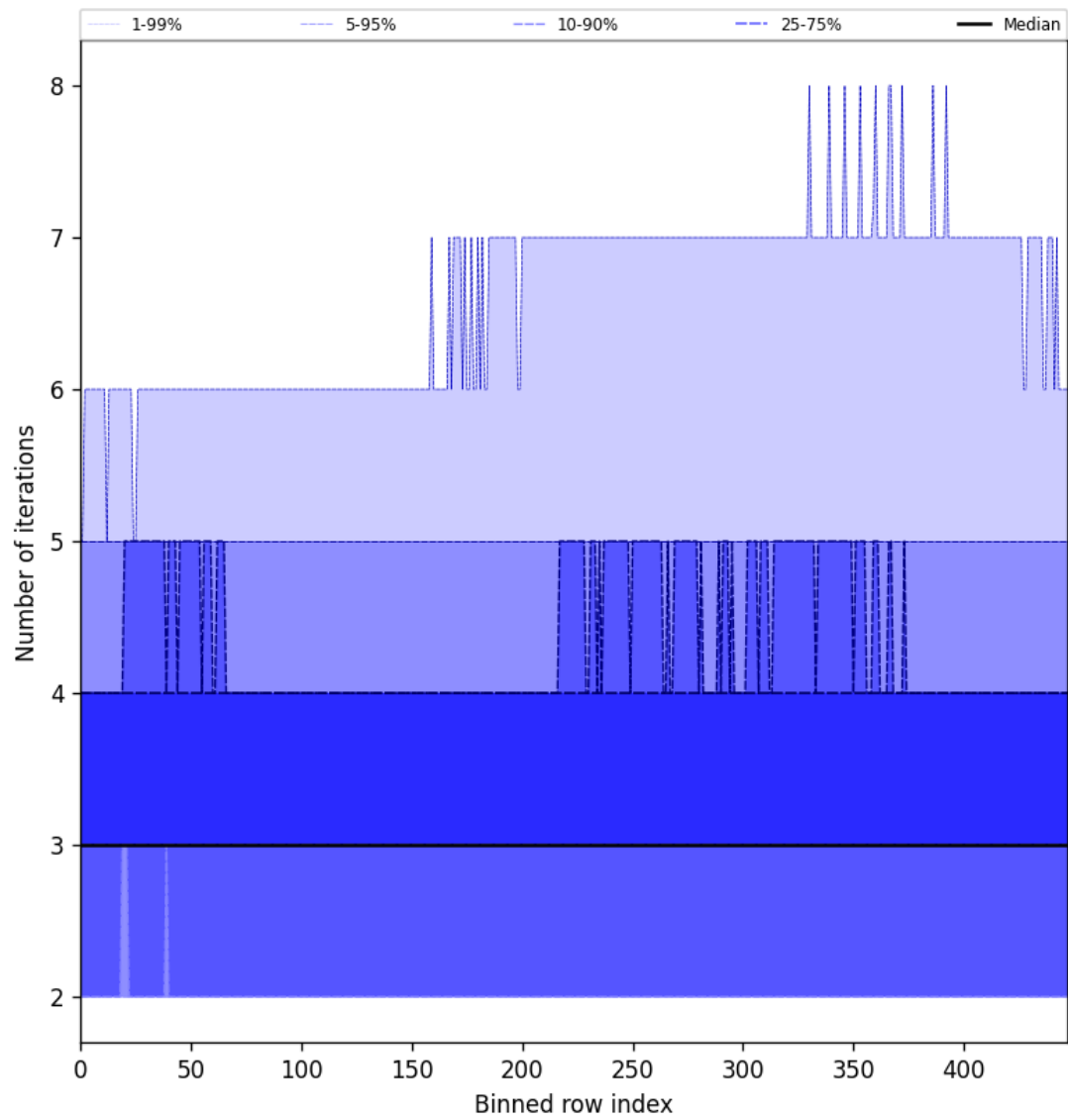
Figure 54: Along track statistics of “Number of iterations” for 2025-10-16 to 2025-10-17
