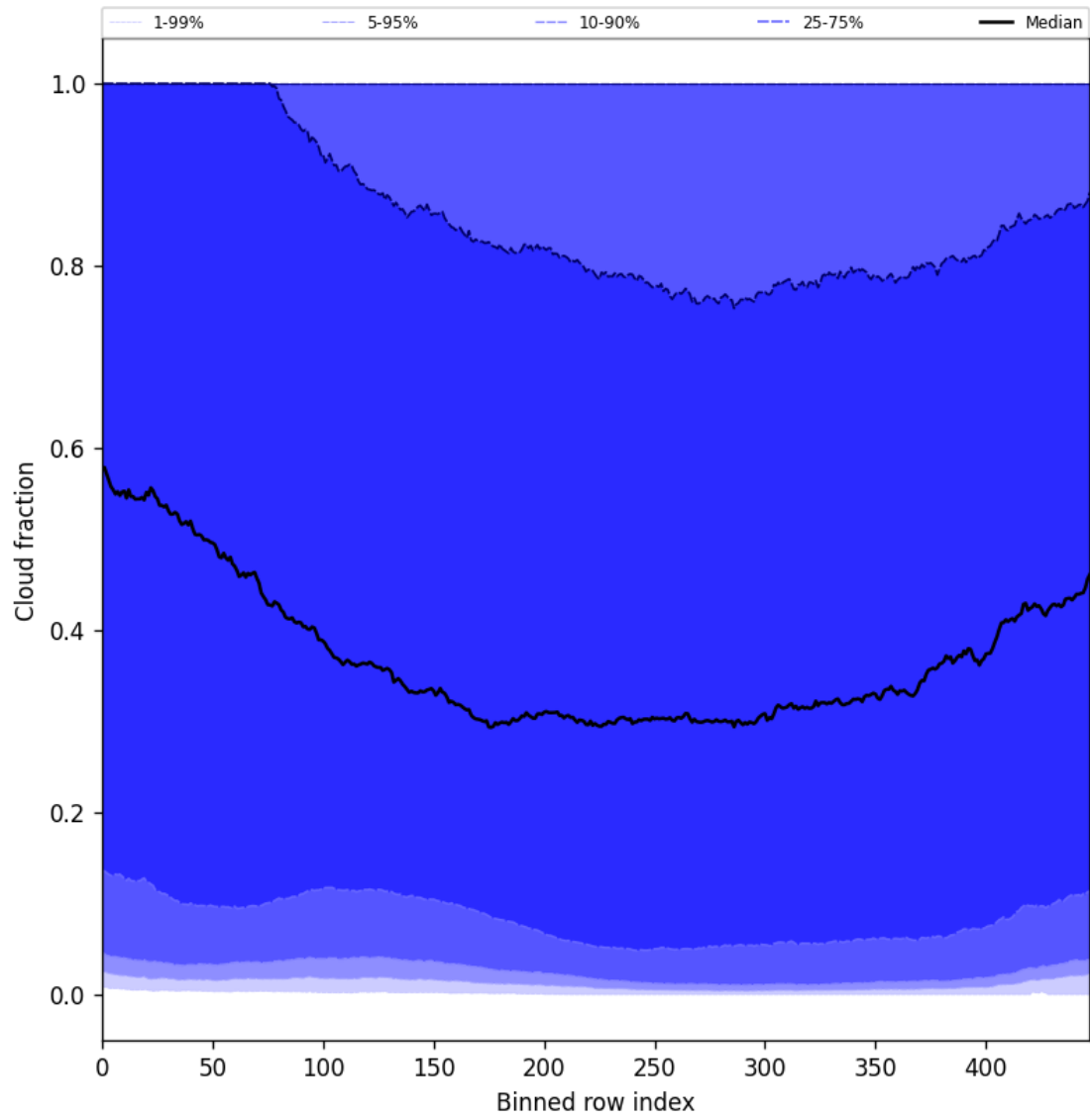
Figure 47: Along track statistics of “Cloud fraction” for 2025-10-16 to 2025-10-17
