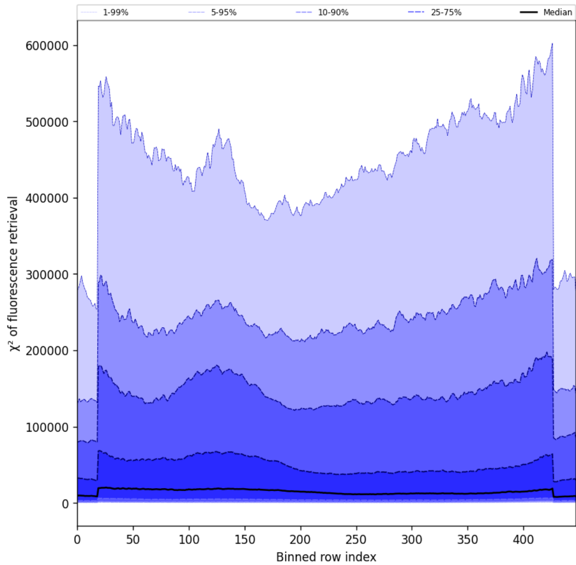
Figure 57: Along track statistics of “ \chi^2 of fluorescence retrieval” for 2025-10-16 to 2025-10-17
