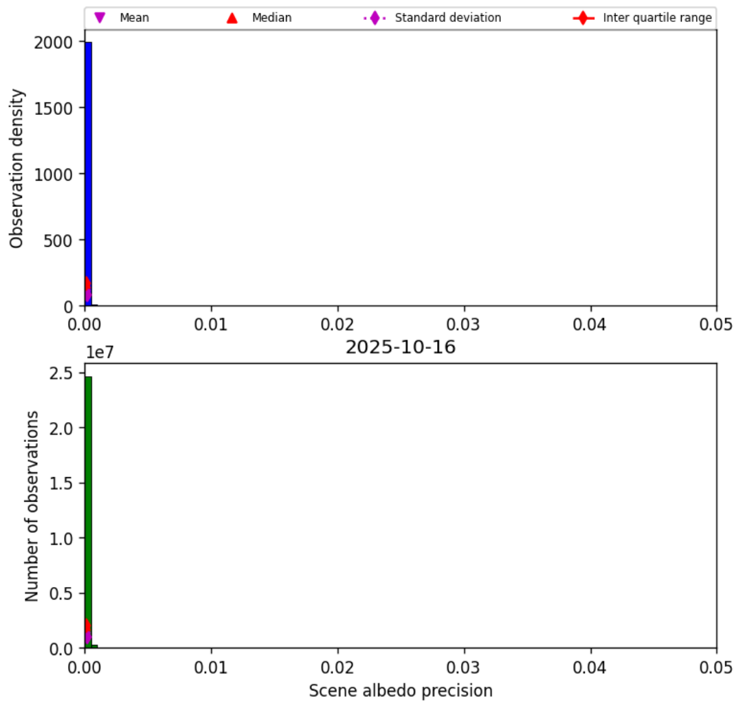
Figure 33: Histogram of “Scene albedo precision” for 2025-10-16 to 2025-10-17
