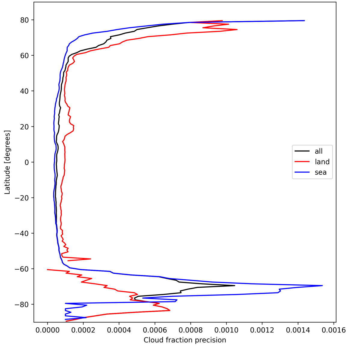
Figure 14: Zonal average of “Cloud fraction precision” for 2025-10-16 to 2025-10-17.
