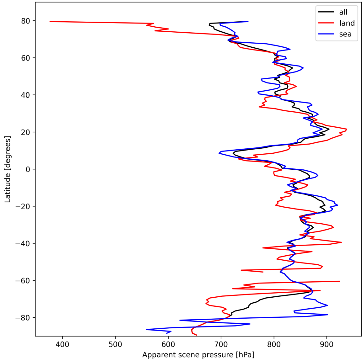
Figure 17: Zonal average of “Apparent scene pressure” for 2025-10-16 to 2025-10-17.
