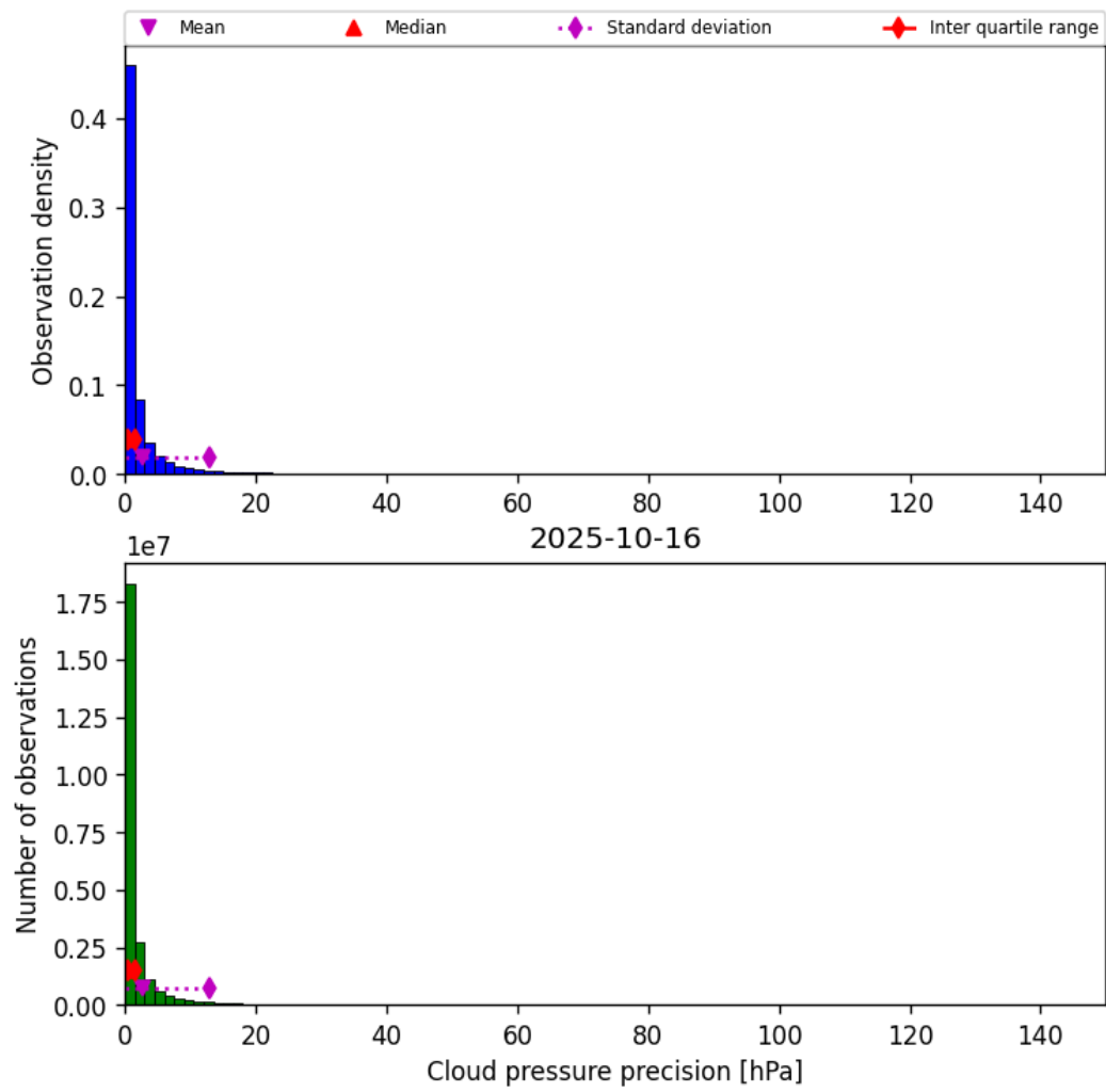
Figure 29: Histogram of “Cloud pressure precision” for 2025-10-16 to 2025-10-17
