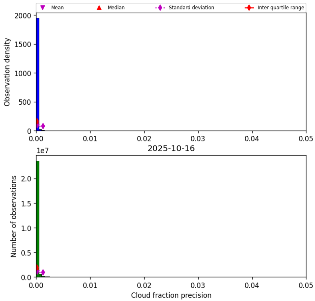
Figure 31: Histogram of “Cloud fraction precision” for 2025-10-16 to 2025-10-17
