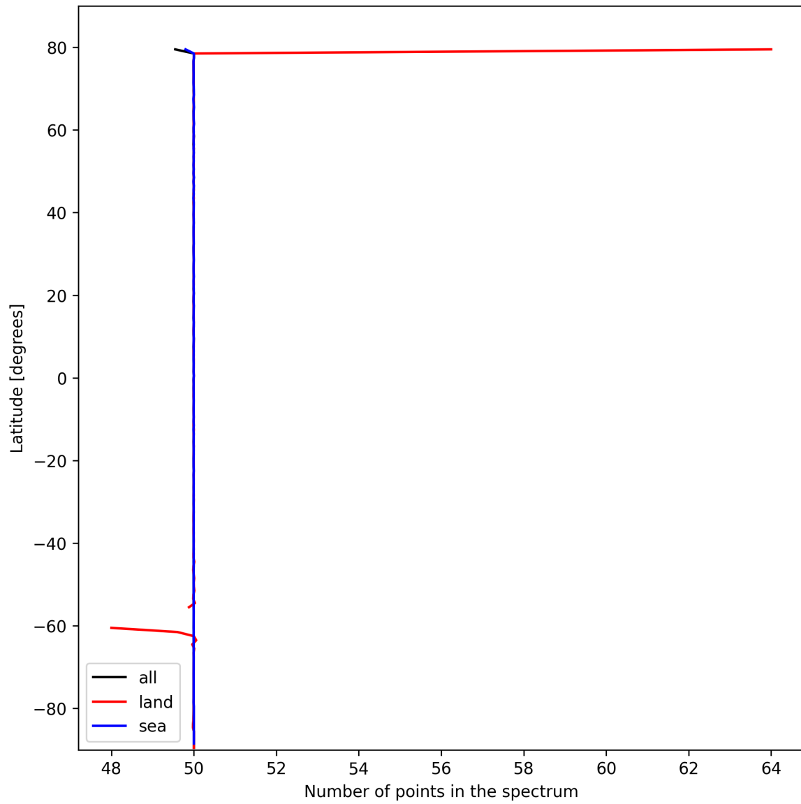
Figure 25: Zonal average of “Number of points in the spectrum” for 2025-10-16 to 2025-10-17.
