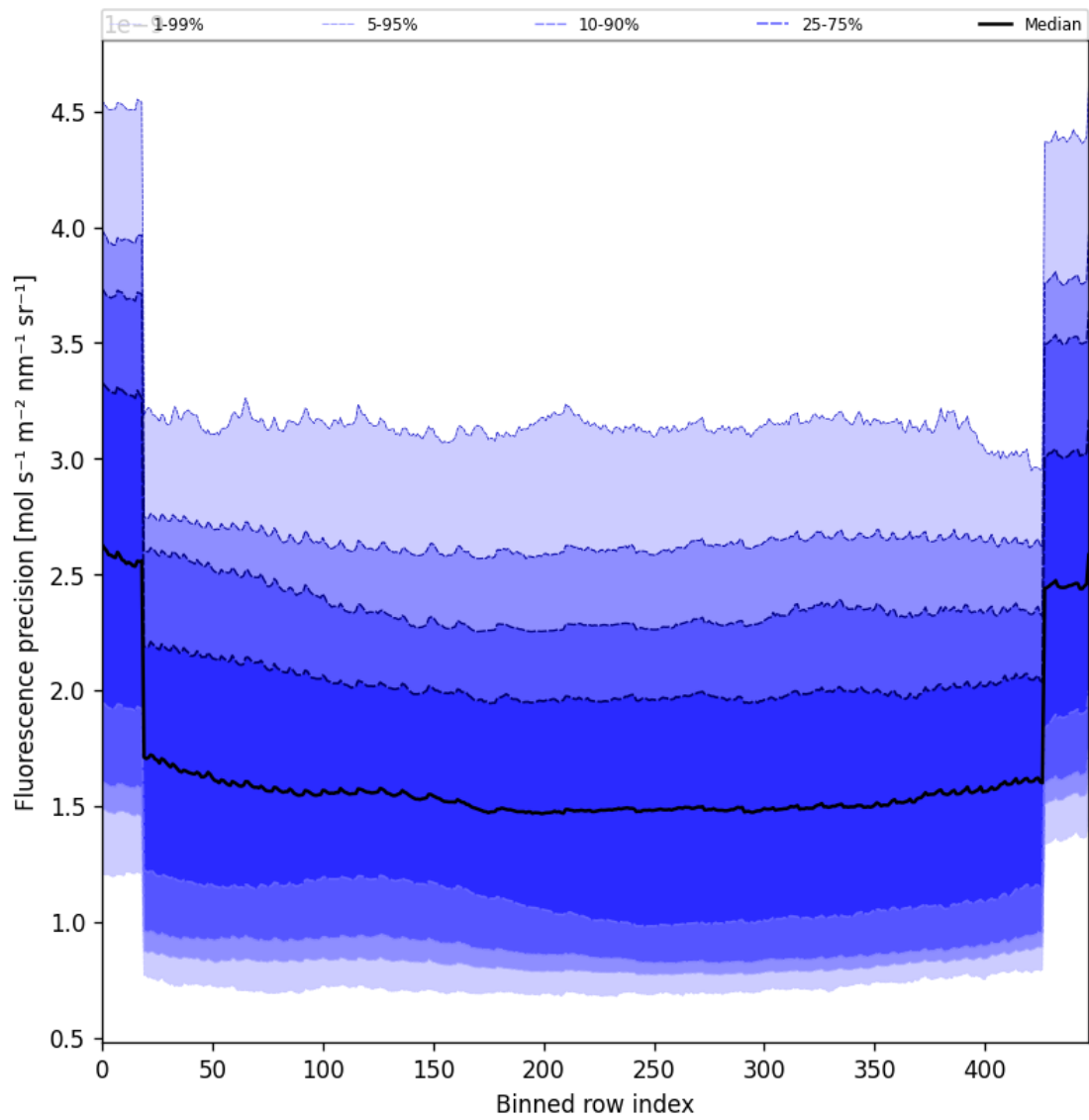
Figure 56: Along track statistics of “Fluorescence precision” for 2025-10-16 to 2025-10-17
