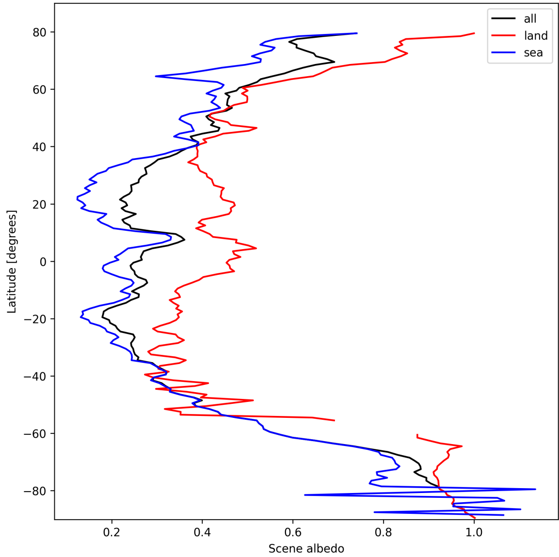
Figure 15: Zonal average of “Scene albedo” for 2025-10-16 to 2025-10-17.
