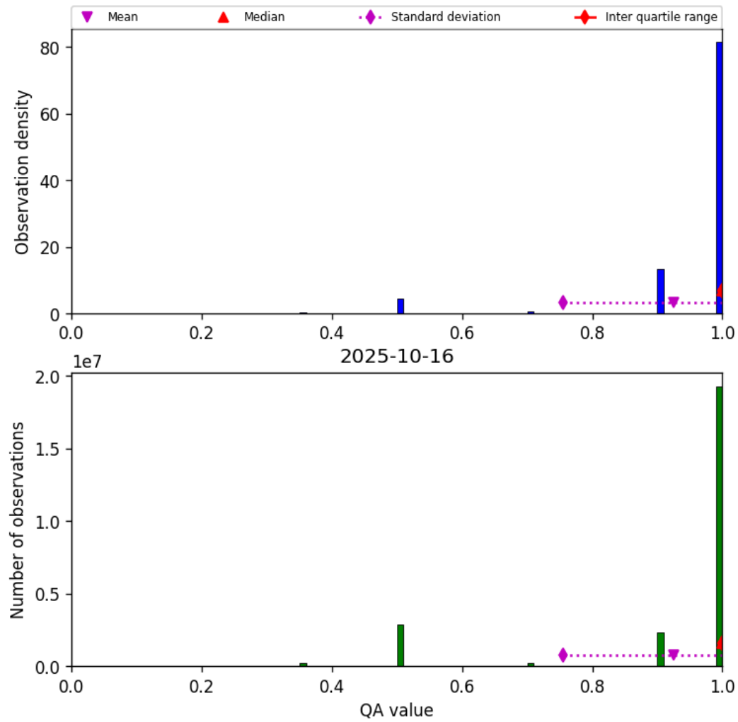
Figure 27: Histogram of “QA value” for 2025-10-16 to 2025-10-17
