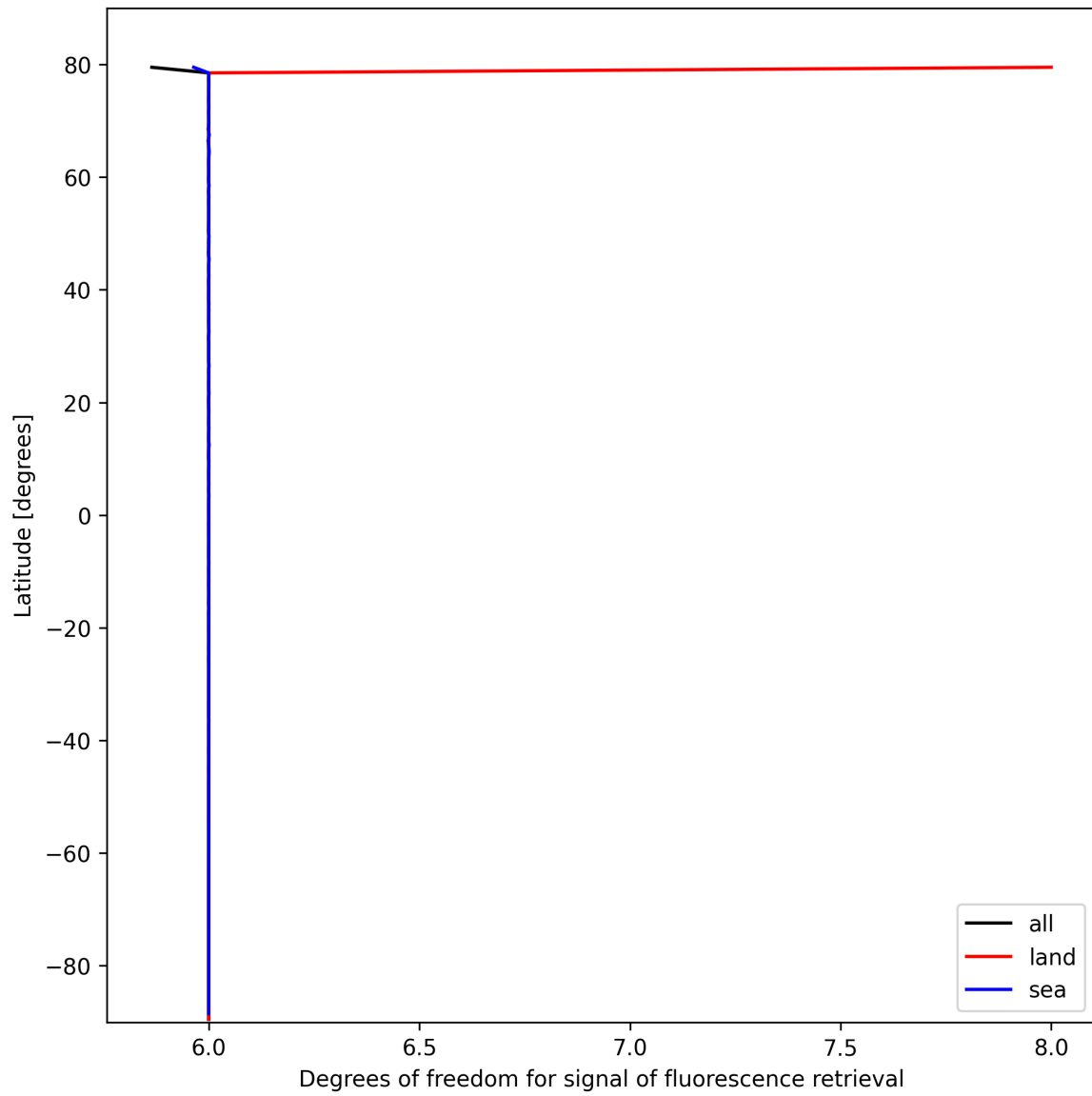
Figure 24: Zonal average of “Degrees of freedom for signal of fluorescence retrieval” for 2025-10-16 to 2025-10-17.
