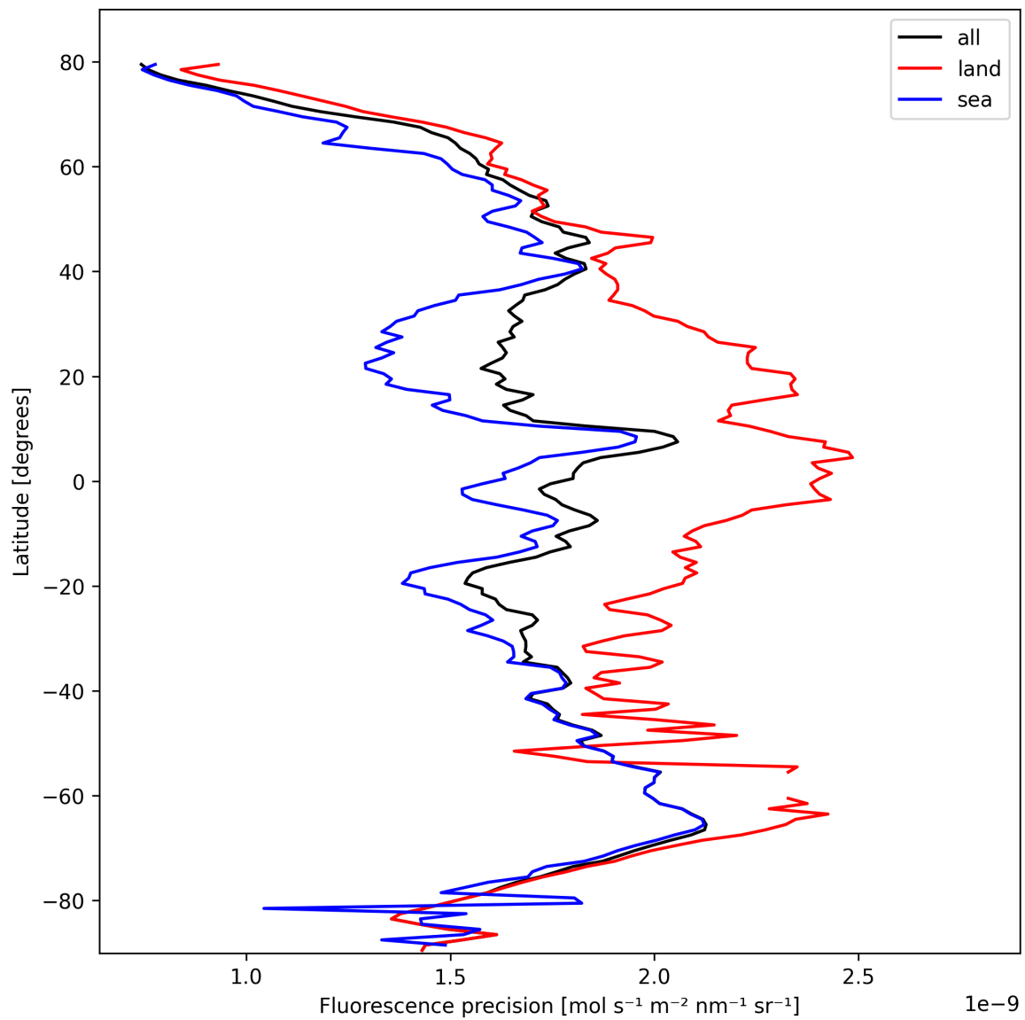
Figure 22: Zonal average of “Fluorescence precision” for 2025-10-16 to 2025-10-17.
