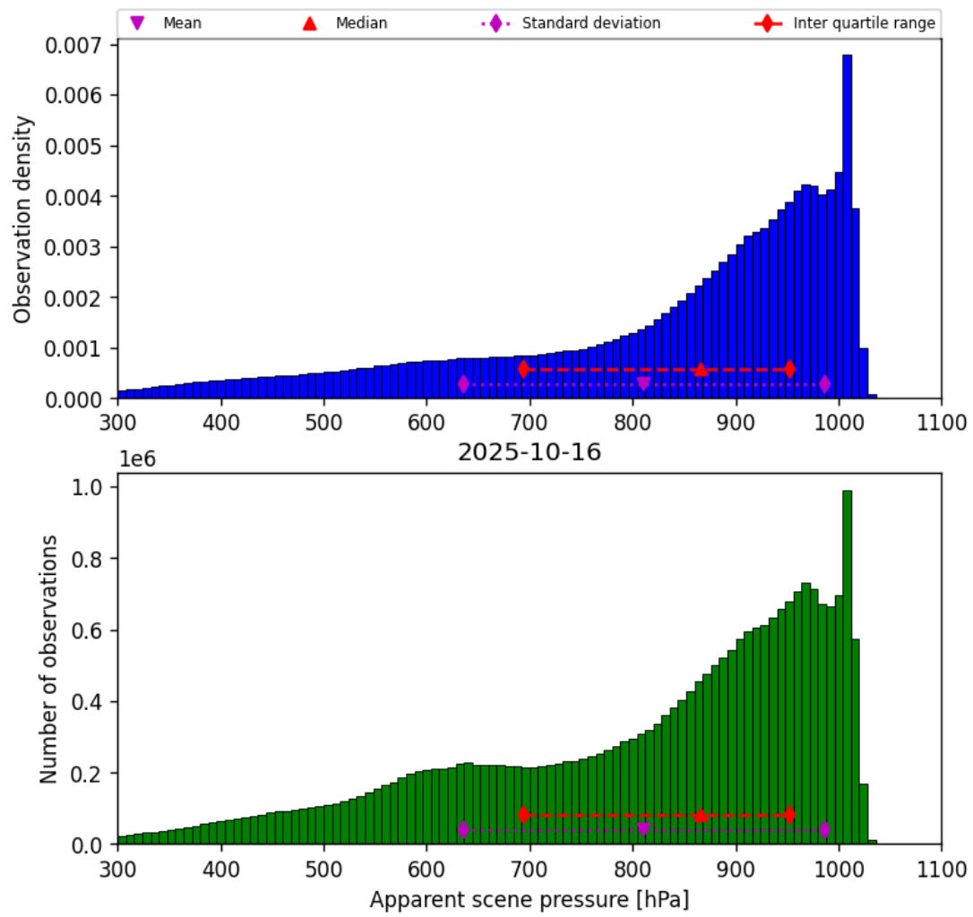
Figure 34: Histogram of “Apparent scene pressure” for 2025-10-16 to 2025-10-17
