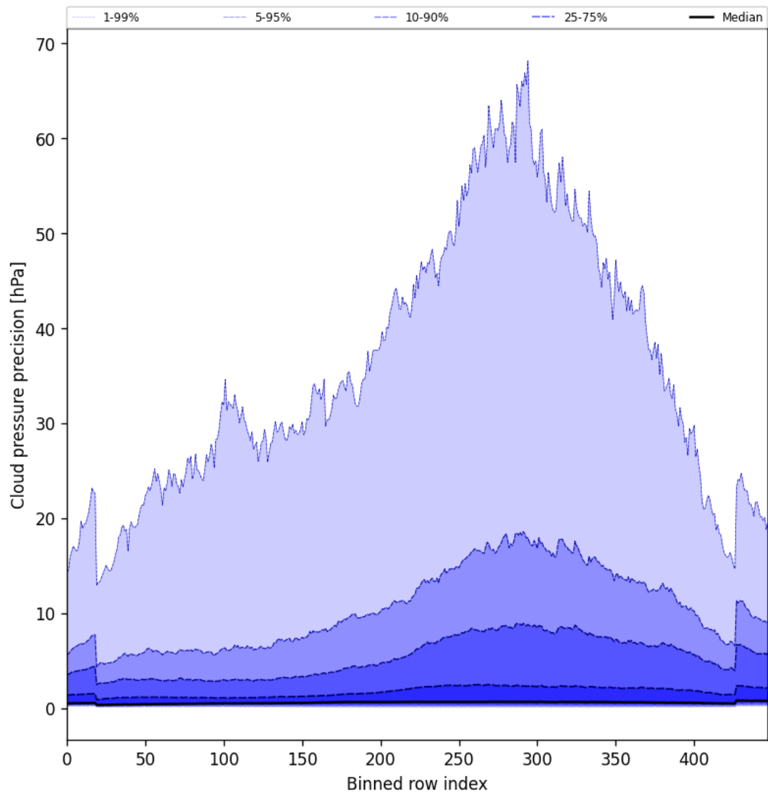
Figure 46: Along track statistics of “Cloud pressure precision” for 2025-10-16 to 2025-10-17
