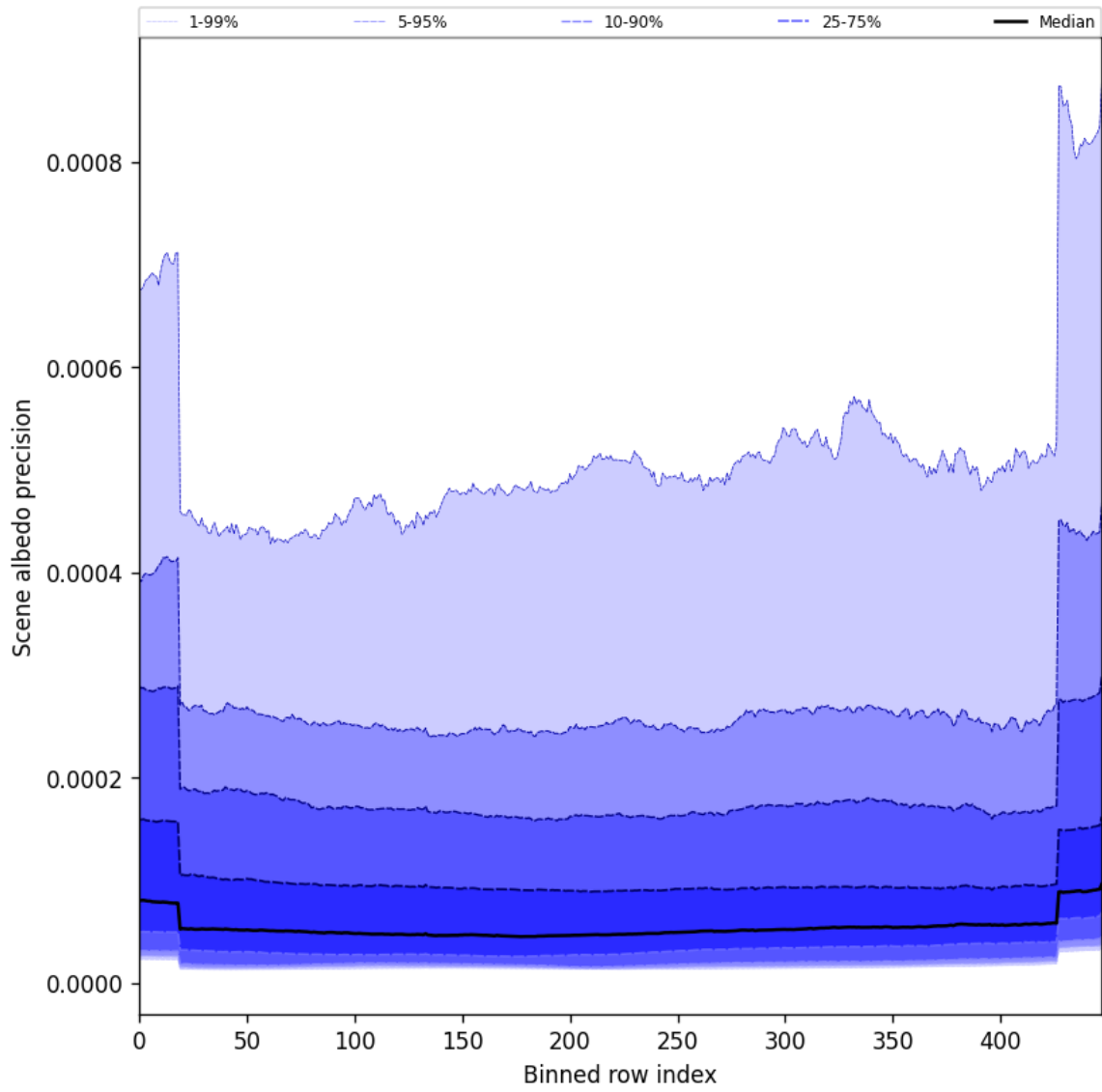
Figure 50: Along track statistics of “Scene albedo precision” for 2025-10-16 to 2025-10-17
