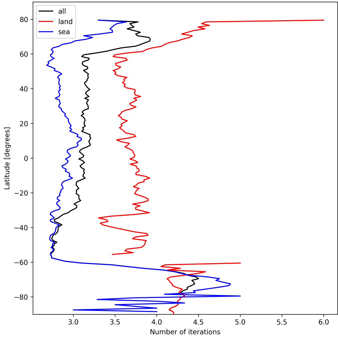
Figure 20: Zonal average of “Number of iterations” for 2025-10-16 to 2025-10-17.
