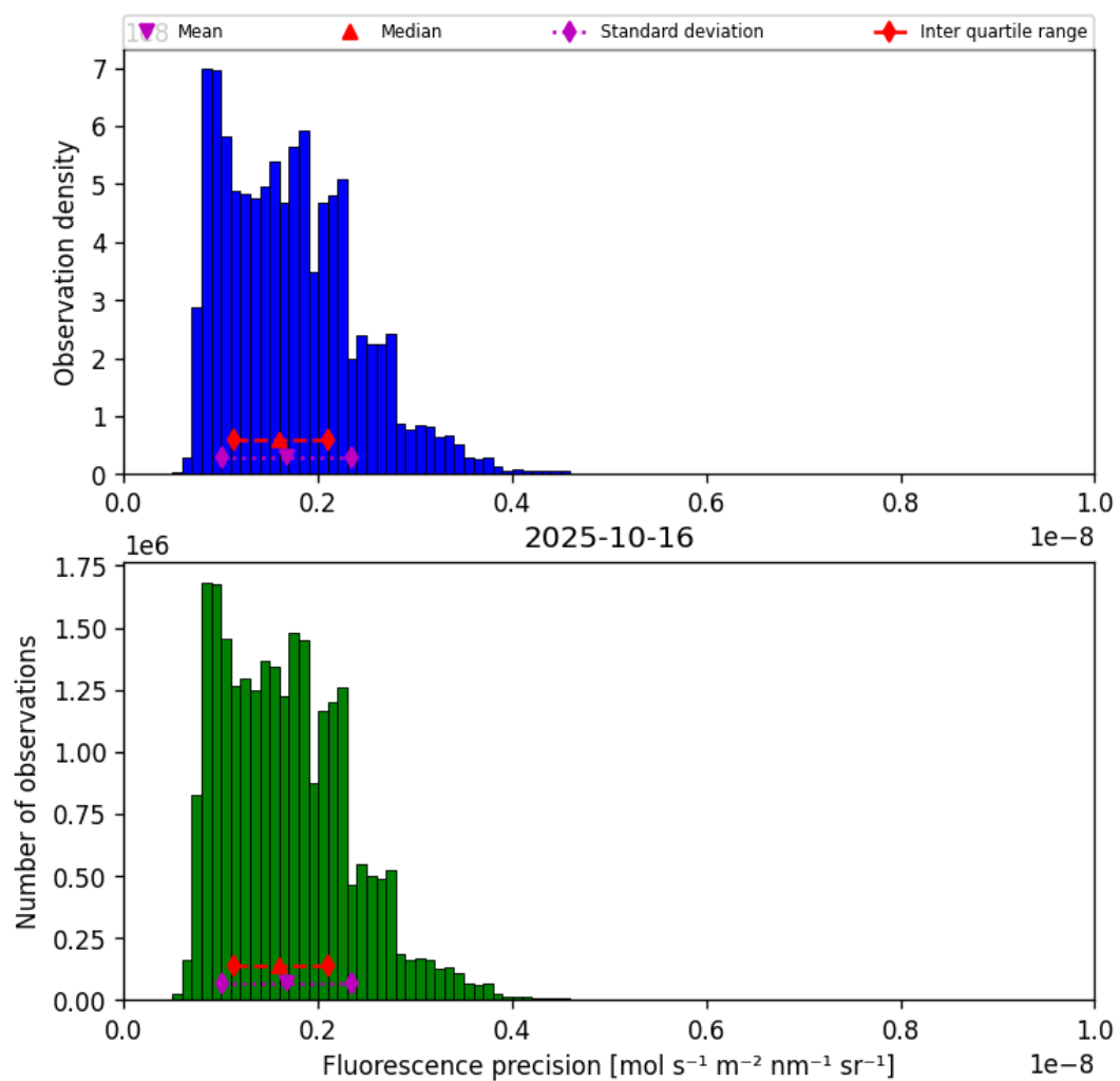
Figure 39: Histogram of “Fluorescence precision” for 2025-10-16 to 2025-10-17
