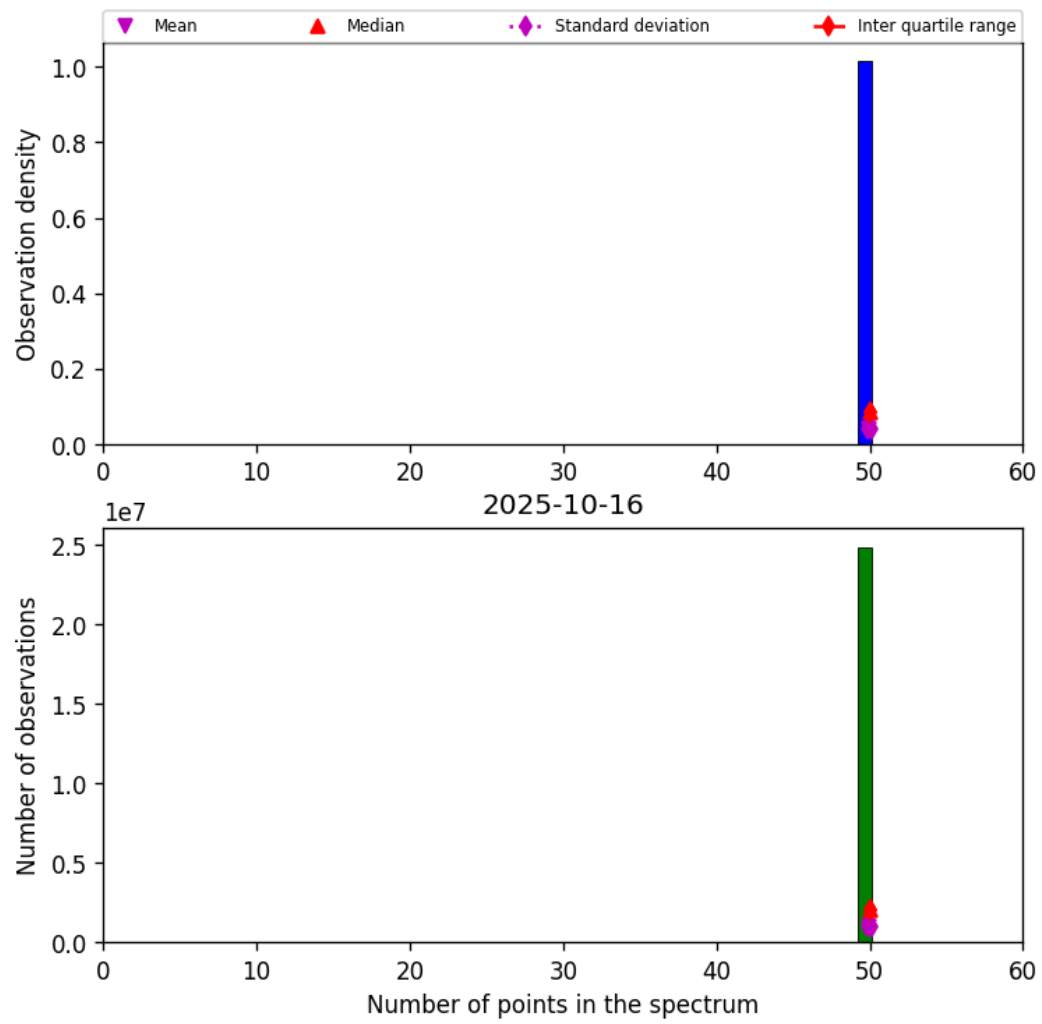
Figure 42: Histogram of “Number of points in the spectrum” for 2025-10-16 to 2025-10-17
