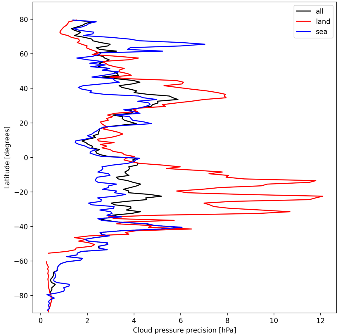
Figure 12: Zonal average of “Cloud pressure precision” for 2025-10-16 to 2025-10-17.
