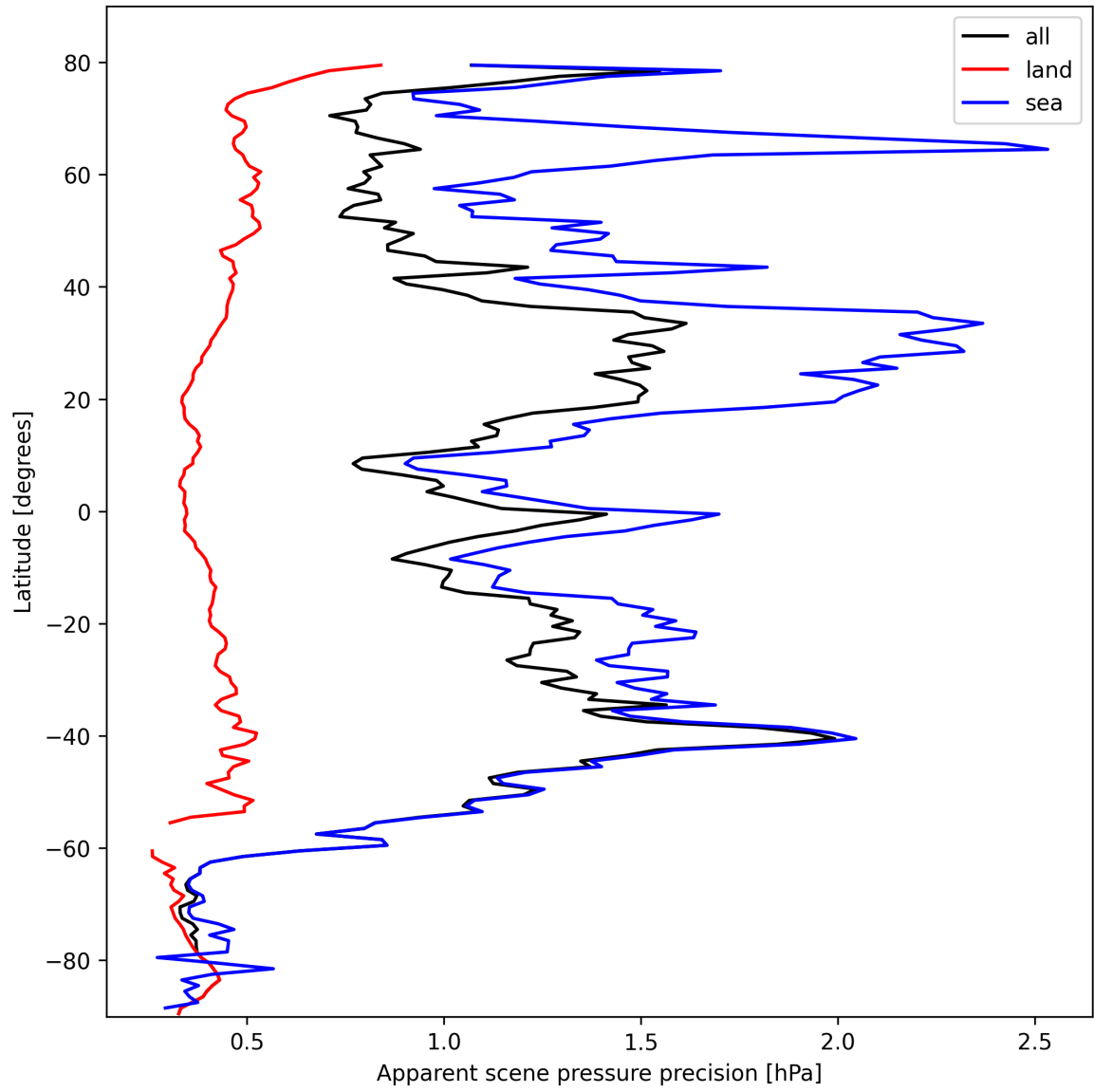
Figure 18: Zonal average of “Apparent scene pressure precision” for 2025-10-16 to 2025-10-17.
