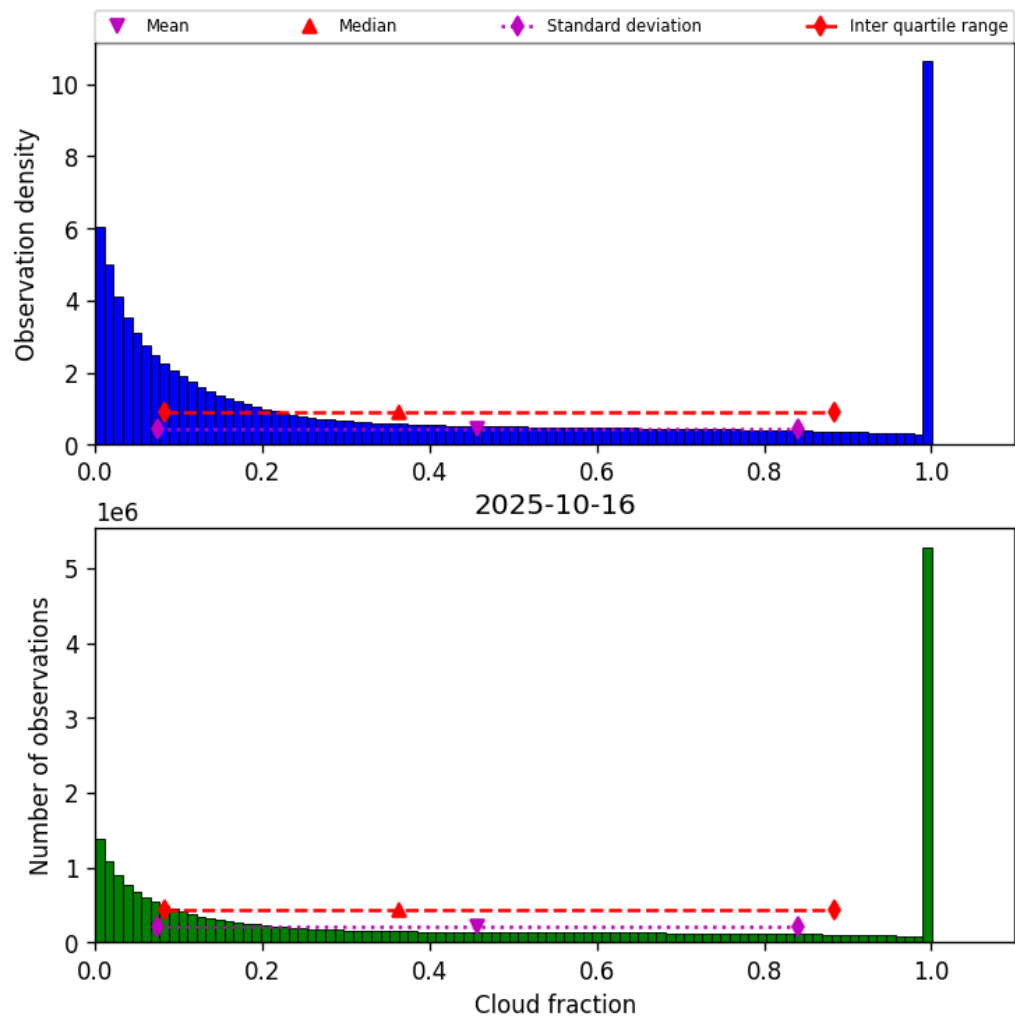
Figure 30: Histogram of “Cloud fraction” for 2025-10-16 to 2025-10-17
