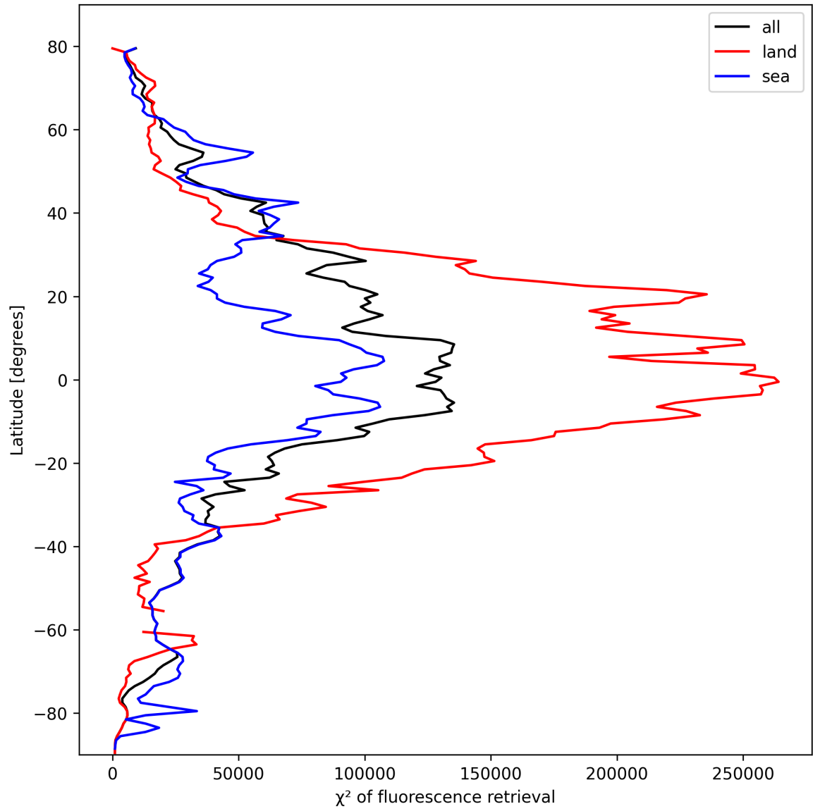
Figure 23: Zonal average of “ \chi^2 of fluorescence retrieval” for 2025-10-16 to 2025-10-17.
