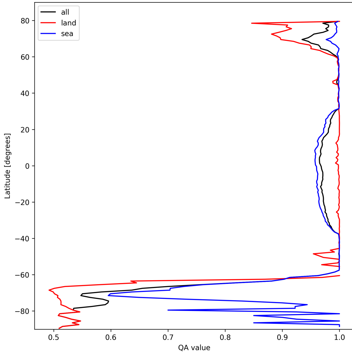
Figure 10: Zonal average of “QA value” for 2025-10-16 to 2025-10-17.
