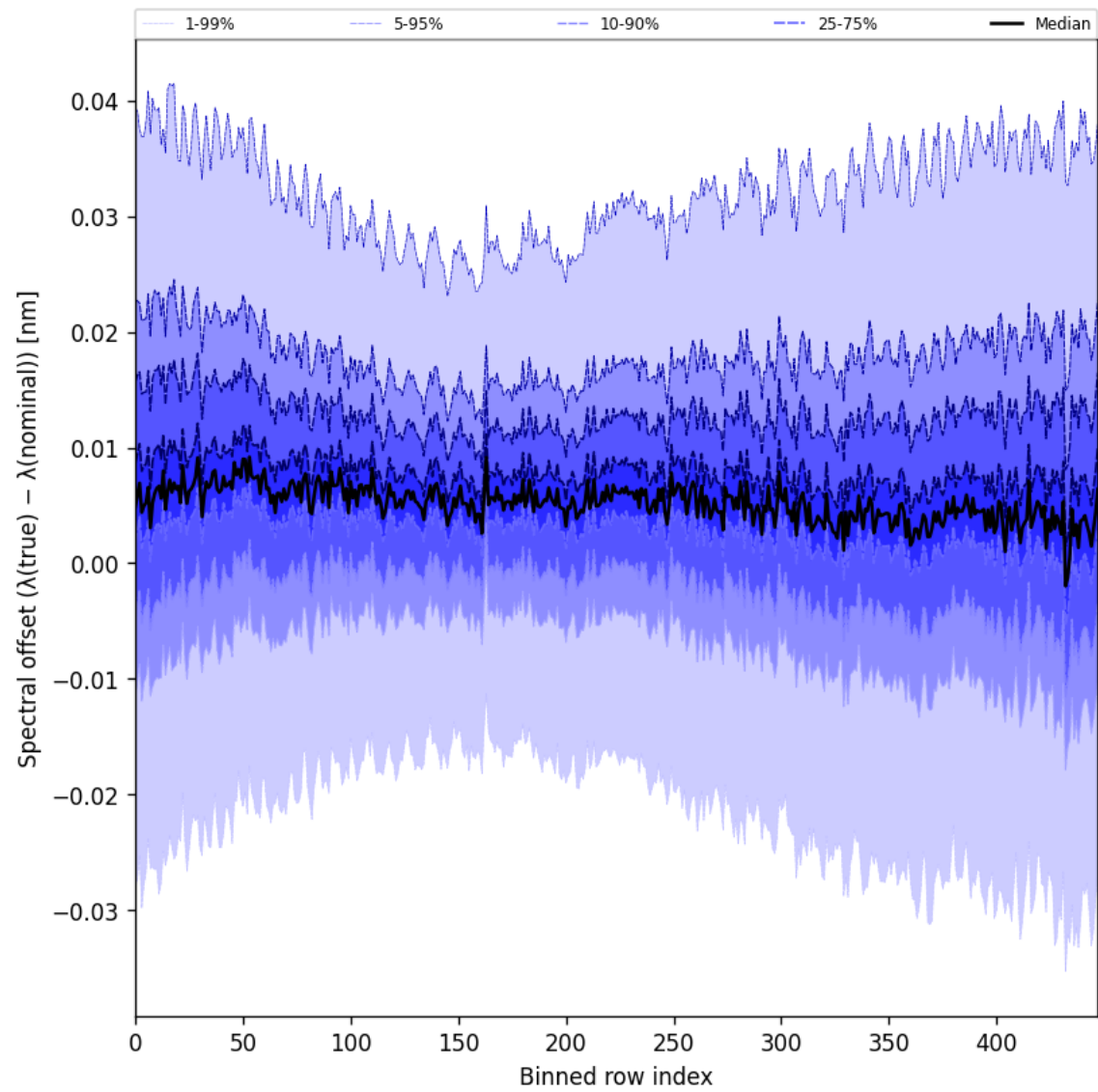
Figure 60: Along track statistics of “Spectral offset ( \lambda_{\text{true}} - \lambda_{\text{nominal}} )” for 2025-10-16 to 2025-10-17
