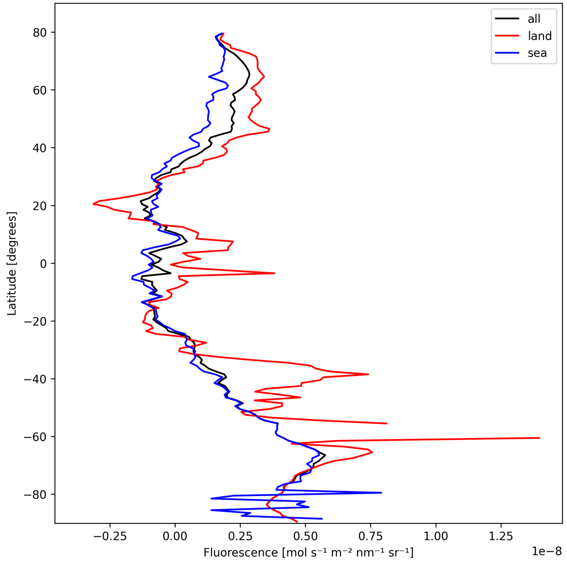
Figure 21: Zonal average of “Fluorescence” for 2025-10-16 to 2025-10-17.
