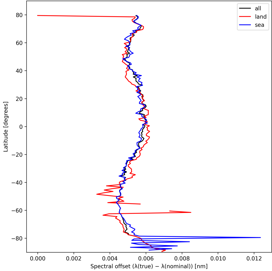
Figure 26: Zonal average of “Spectral offset ( \lambda_{\text{true}} - \lambda_{\text{nominal}} )” for 2025-10-16 to 2025-10-17.
