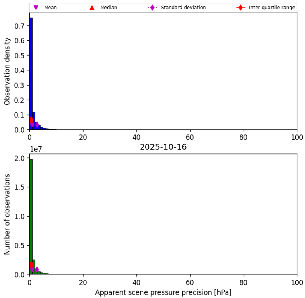
Figure 35: Histogram of “Apparent scene pressure precision” for 2025-10-16 to 2025-10-17
