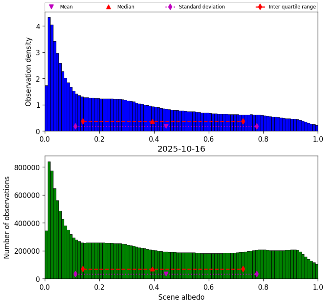
Figure 32: Histogram of “Scene albedo” for 2025-10-16 to 2025-10-17
