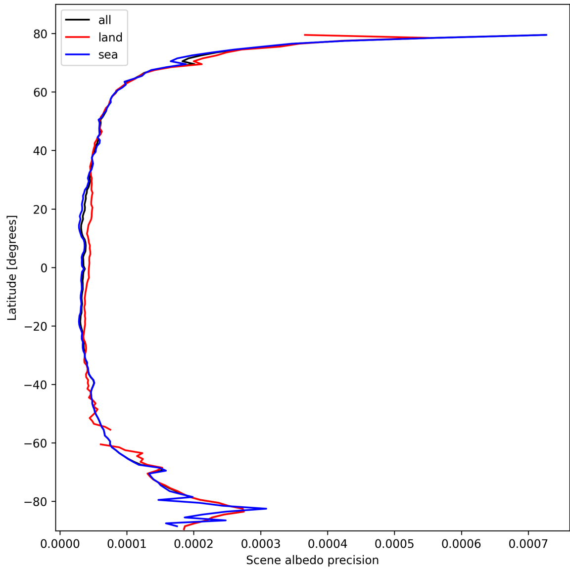
Figure 16: Zonal average of “Scene albedo precision” for 2025-10-16 to 2025-10-17.
