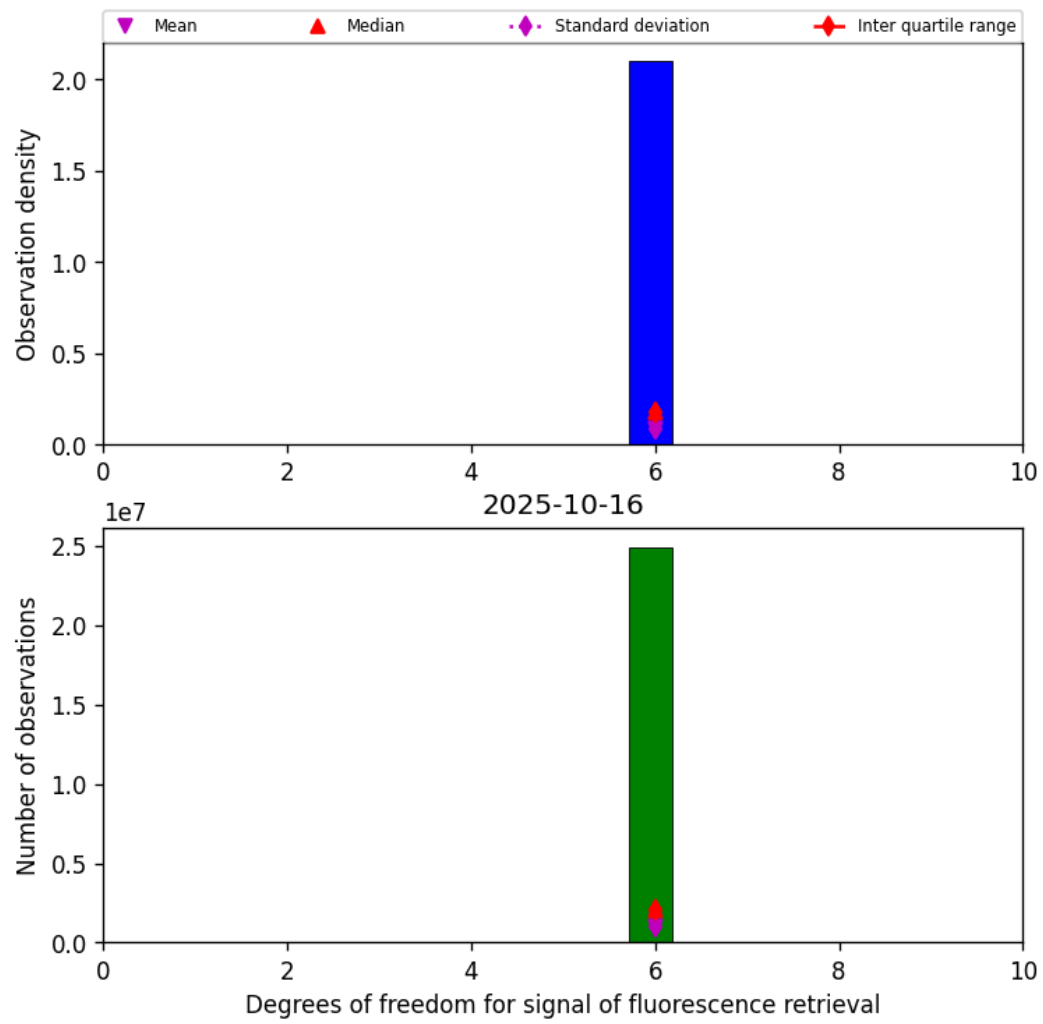
Figure 41: Histogram of “Degrees of freedom for signal of fluorescence retrieval” for 2025-10-16 to 2025-10-17
