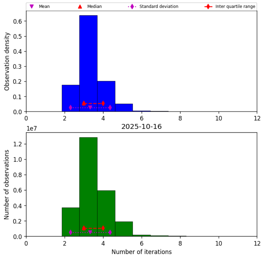
Figure 37: Histogram of “Number of iterations” for 2025-10-16 to 2025-10-17
