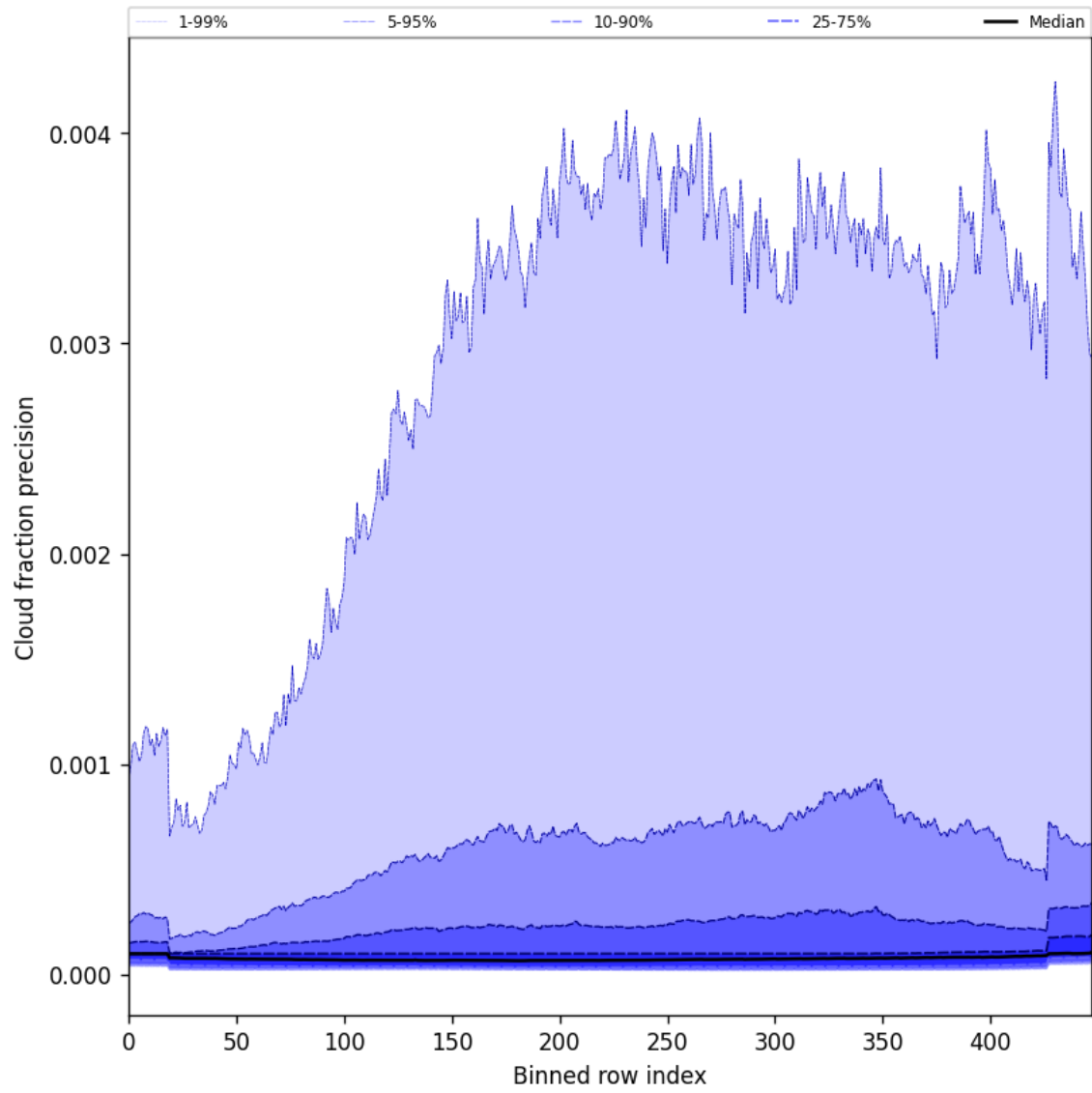
Figure 48: Along track statistics of “Cloud fraction precision” for 2025-10-16 to 2025-10-17
