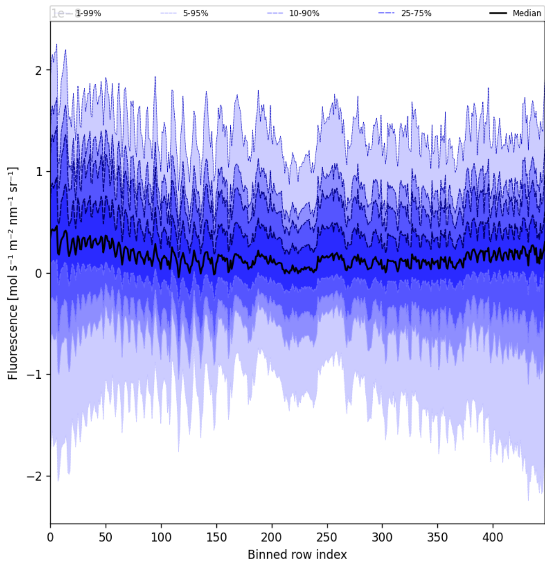
Figure 55: Along track statistics of “Fluorescence” for 2025-10-16 to 2025-10-17
