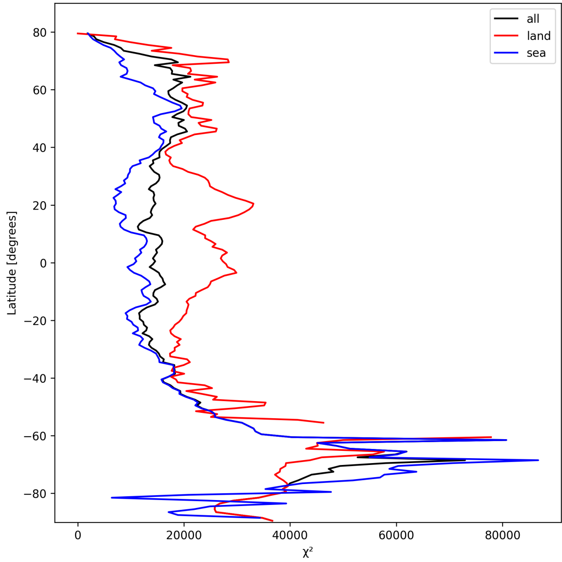
Figure 19: Zonal average of “ \chi^2 ” for 2025-10-16 to 2025-10-17.
