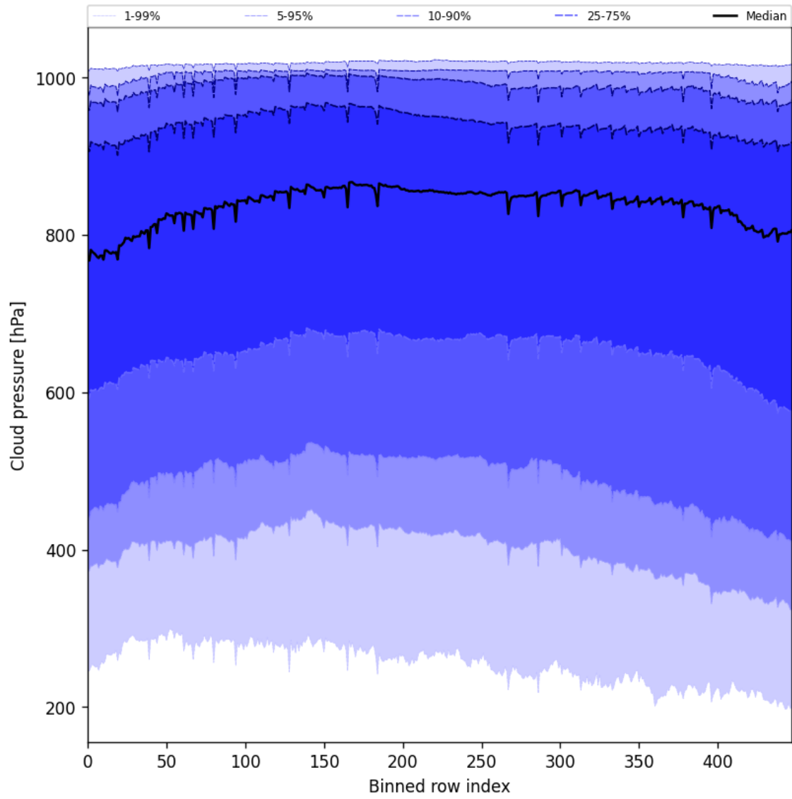
Figure 45: Along track statistics of “Cloud pressure” for 2025-10-16 to 2025-10-17
