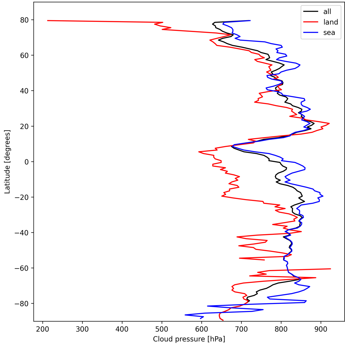
Figure 11: Zonal average of “Cloud pressure” for 2025-10-16 to 2025-10-17.
