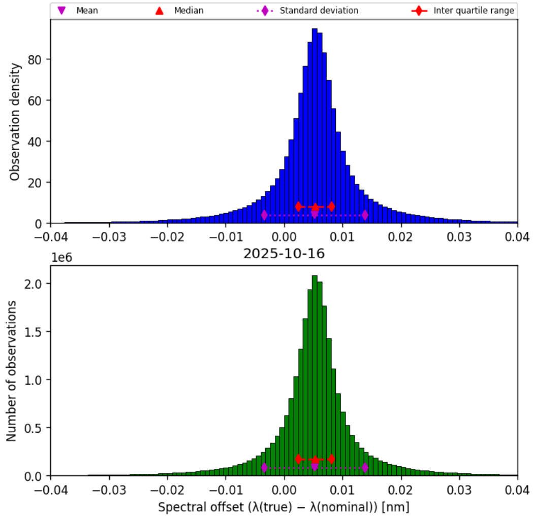
Figure 43: Histogram of “Spectral offset ( \lambda_{\text{true}} - \lambda_{\text{nominal}} )” for 2025-10-16 to 2025-10-17
