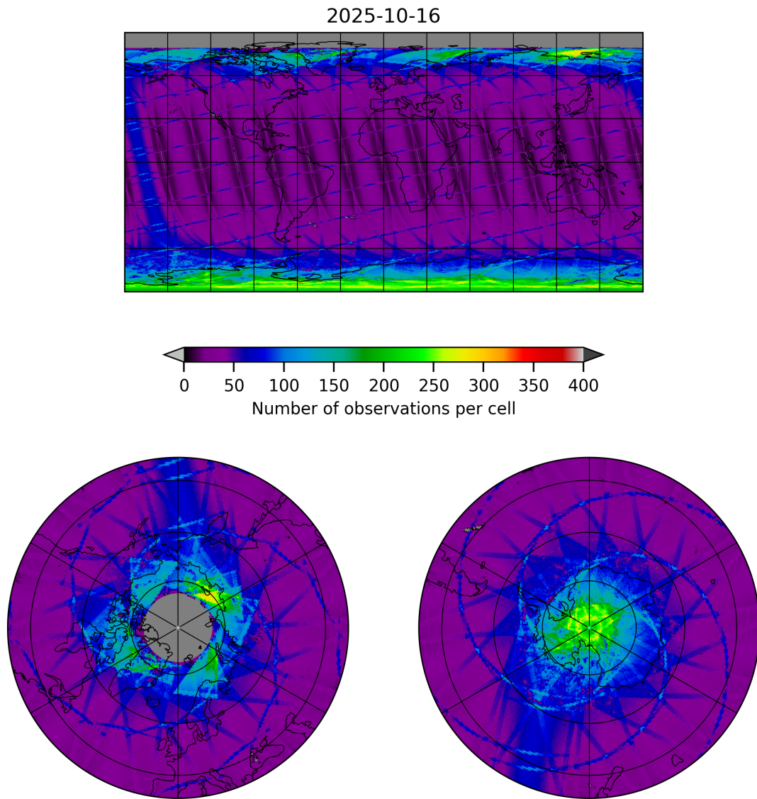
Figure 9: Map of the number of observations for 2025-10-16 to 2025-10-17
