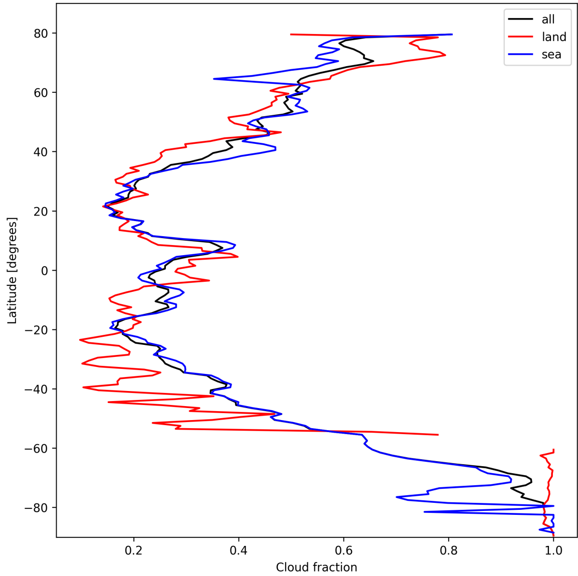
Figure 13: Zonal average of “Cloud fraction” for 2025-10-16 to 2025-10-17.
