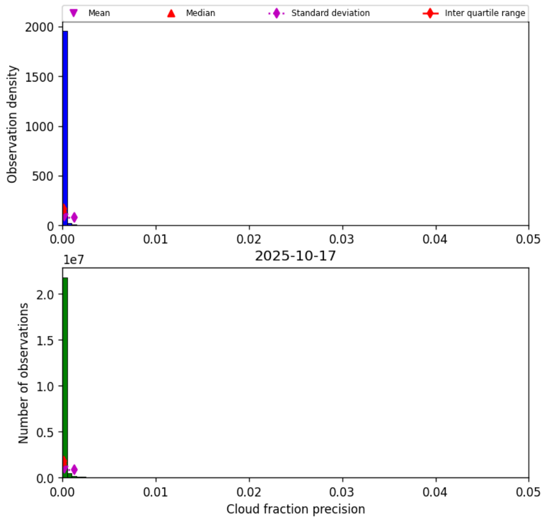
Figure 31: Histogram of “Cloud fraction precision” for 2025-10-17 to 2025-10-18
