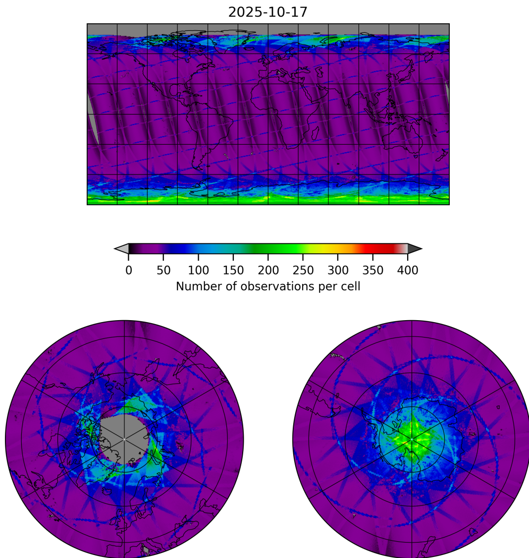
Figure 9: Map of the number of observations for 2025-10-17 to 2025-10-18
