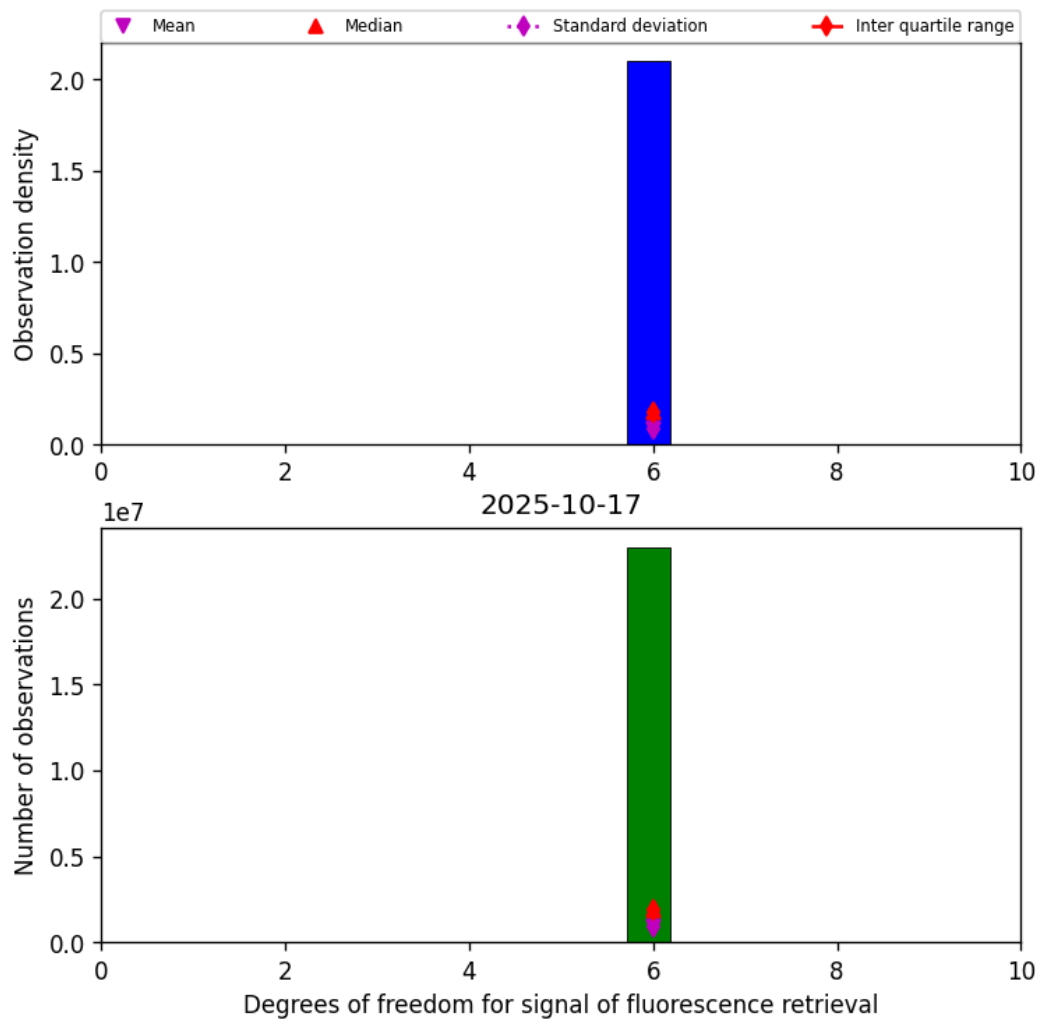
Figure 41: Histogram of “Degrees of freedom for signal of fluorescence retrieval” for 2025-10-17 to 2025-10-18
