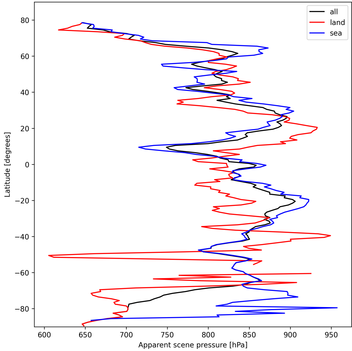
Figure 17: Zonal average of “Apparent scene pressure” for 2025-10-17 to 2025-10-18.
