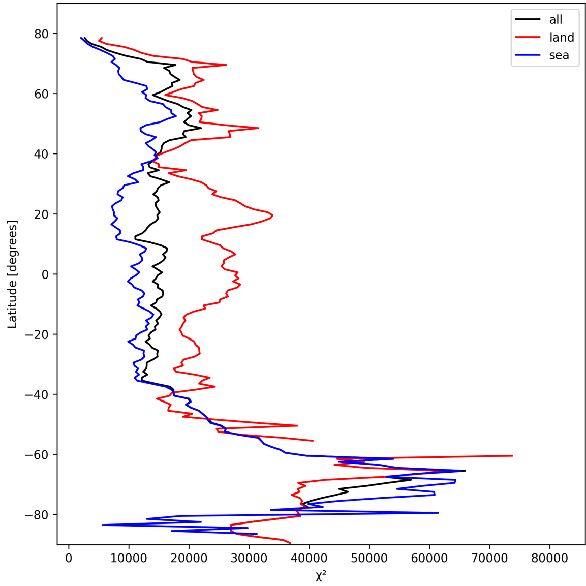
Figure 19: Zonal average of “ \chi^2 ” for 2025-10-17 to 2025-10-18.
