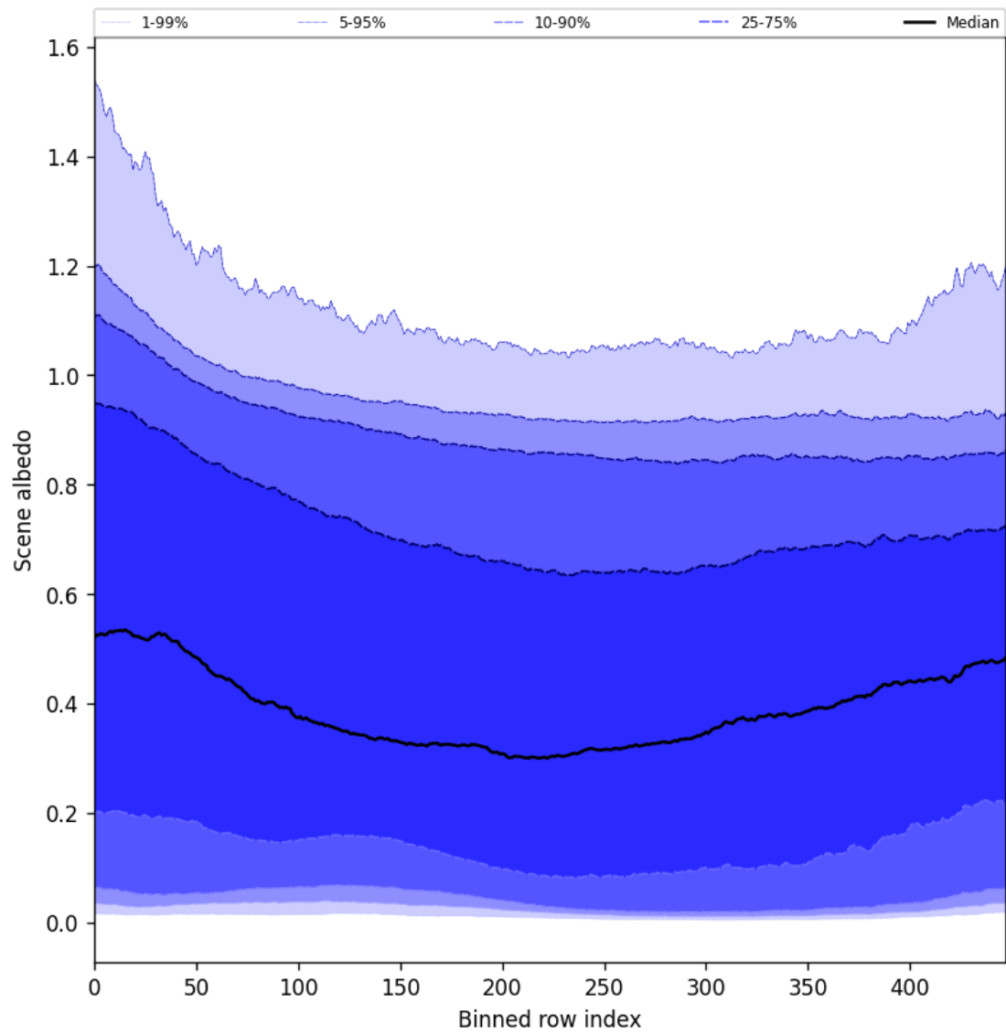
Figure 49: Along track statistics of “Scene albedo” for 2025-10-17 to 2025-10-18
