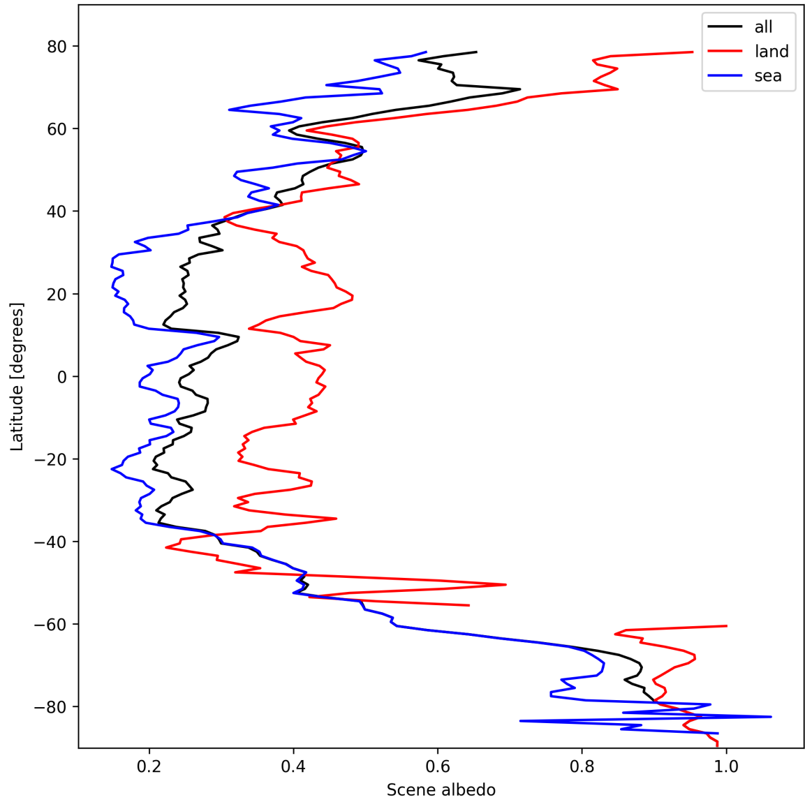
Figure 15: Zonal average of “Scene albedo” for 2025-10-17 to 2025-10-18.
