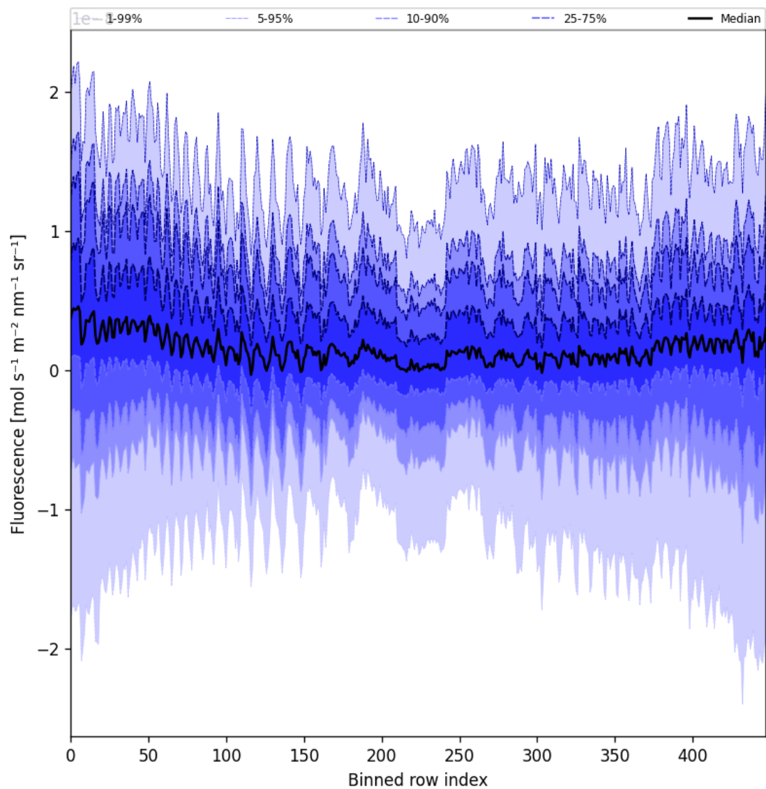
Figure 55: Along track statistics of “Fluorescence” for 2025-10-17 to 2025-10-18
