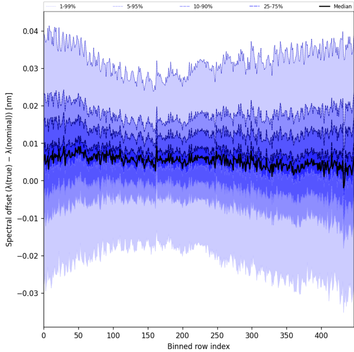
Figure 60: Along track statistics of “Spectral offset ( \lambda_{\text{true}} - \lambda_{\text{nominal}} )” for 2025-10-17 to 2025-10-18
