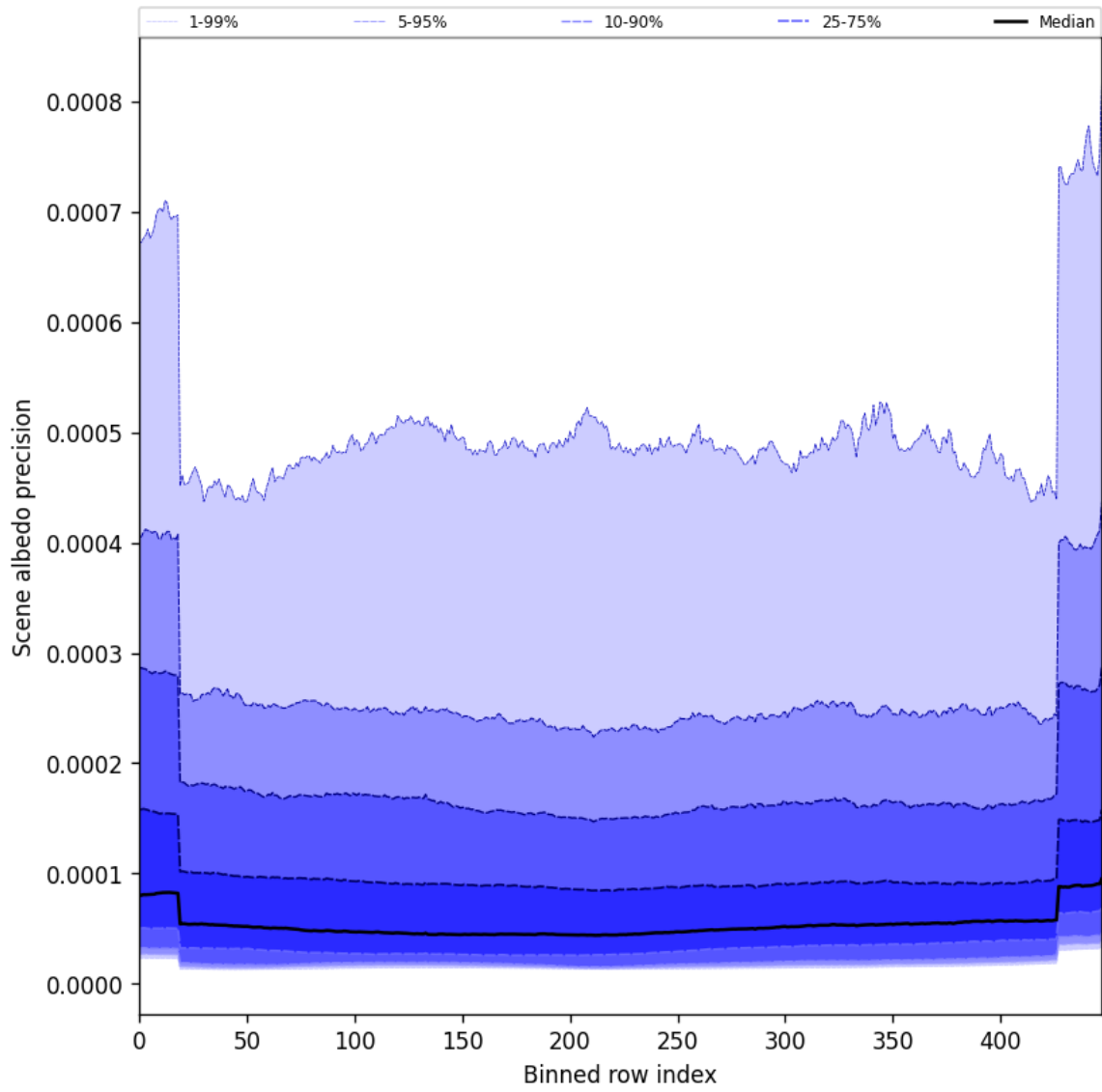
Figure 50: Along track statistics of “Scene albedo precision” for 2025-10-17 to 2025-10-18
