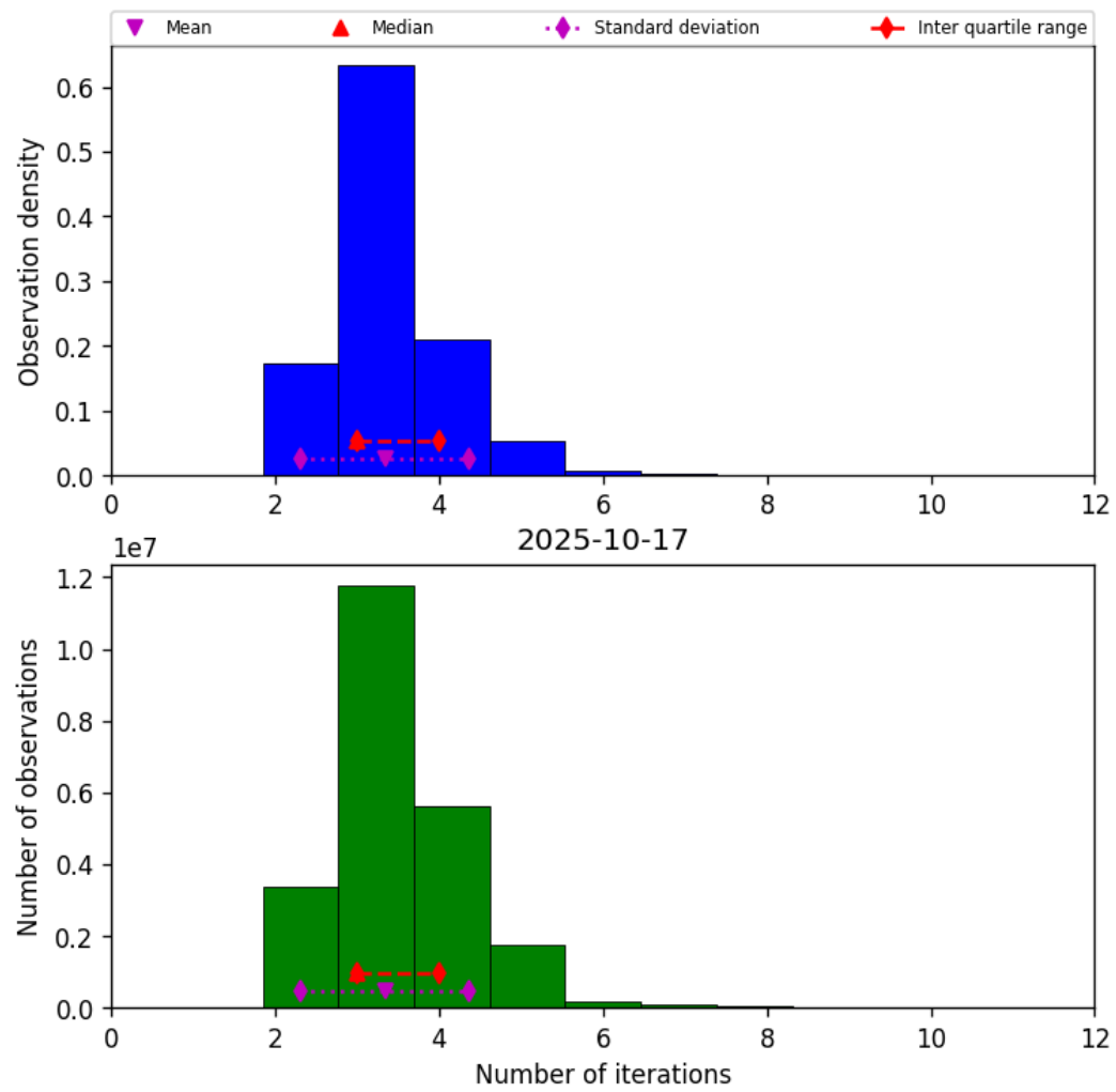
Figure 37: Histogram of “Number of iterations” for 2025-10-17 to 2025-10-18
