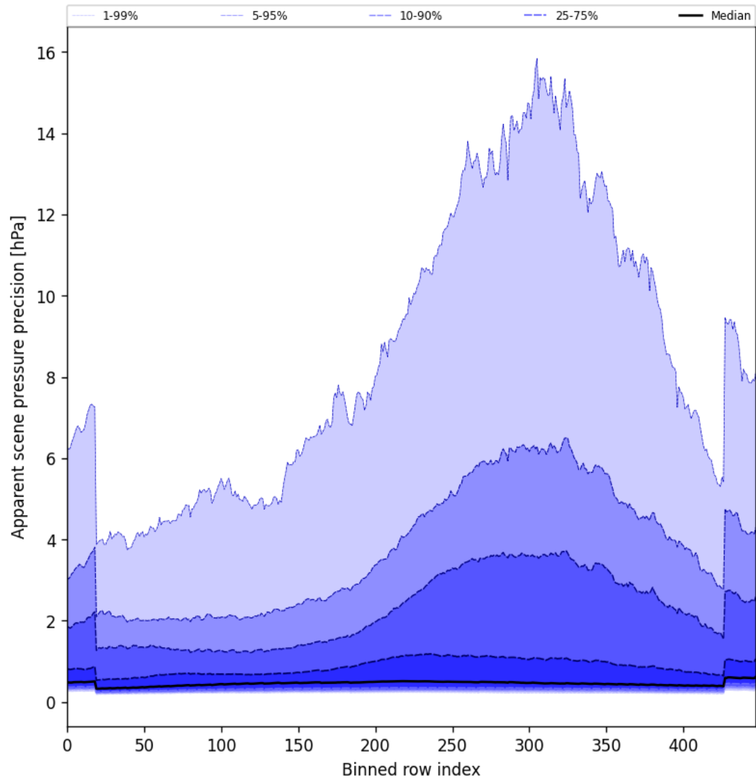
Figure 52: Along track statistics of “Apparent scene pressure precision” for 2025-10-17 to 2025-10-18
