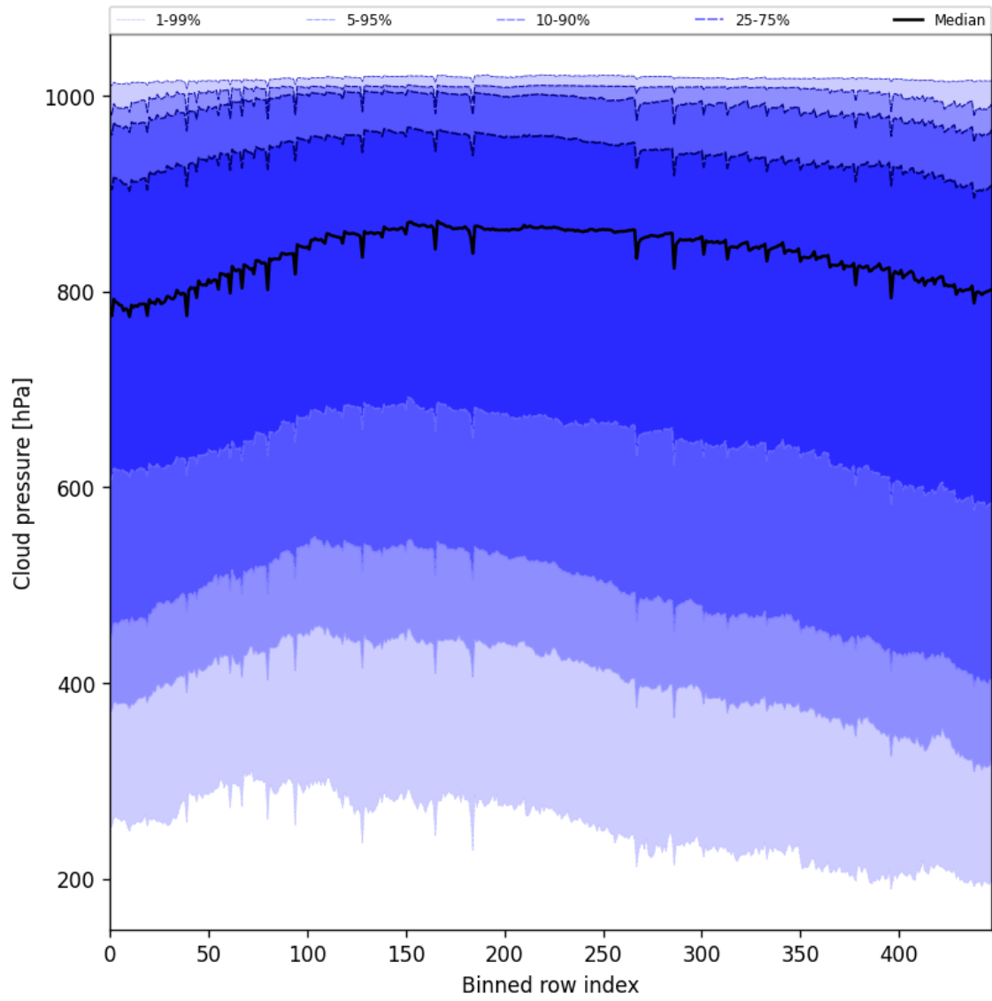
Figure 45: Along track statistics of “Cloud pressure” for 2025-10-17 to 2025-10-18
