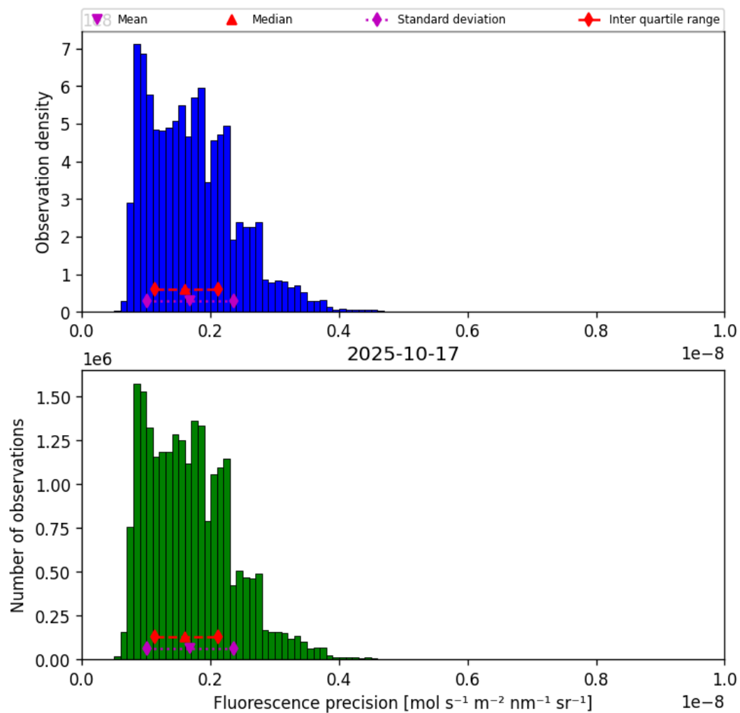
Figure 39: Histogram of “Fluorescence precision” for 2025-10-17 to 2025-10-18
