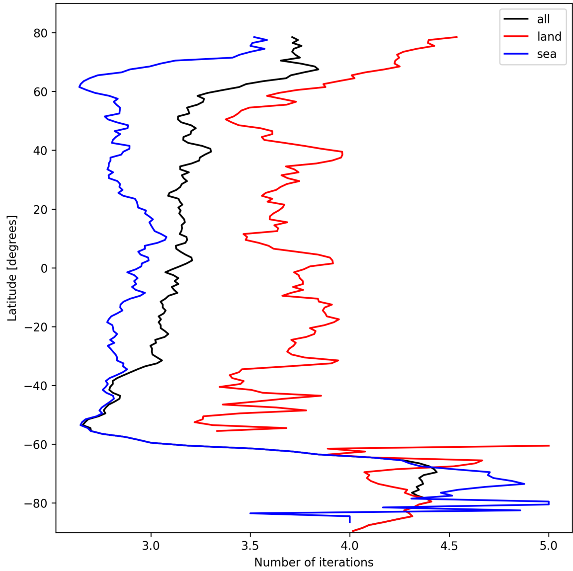
Figure 20: Zonal average of “Number of iterations” for 2025-10-17 to 2025-10-18.
