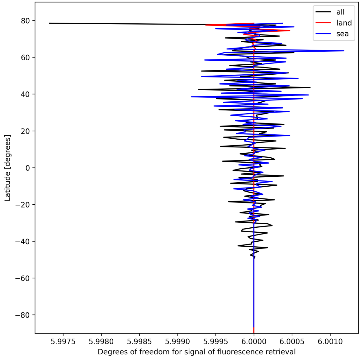
Figure 24: Zonal average of “Degrees of freedom for signal of fluorescence retrieval” for 2025-10-17 to 2025-10-18.
