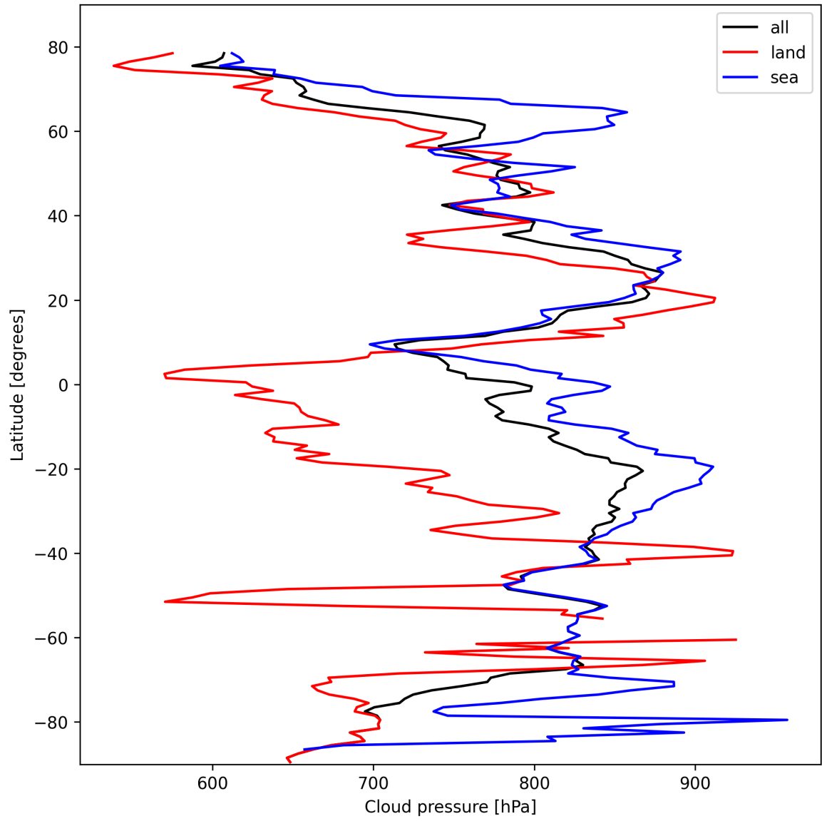
Figure 11: Zonal average of “Cloud pressure” for 2025-10-17 to 2025-10-18.
