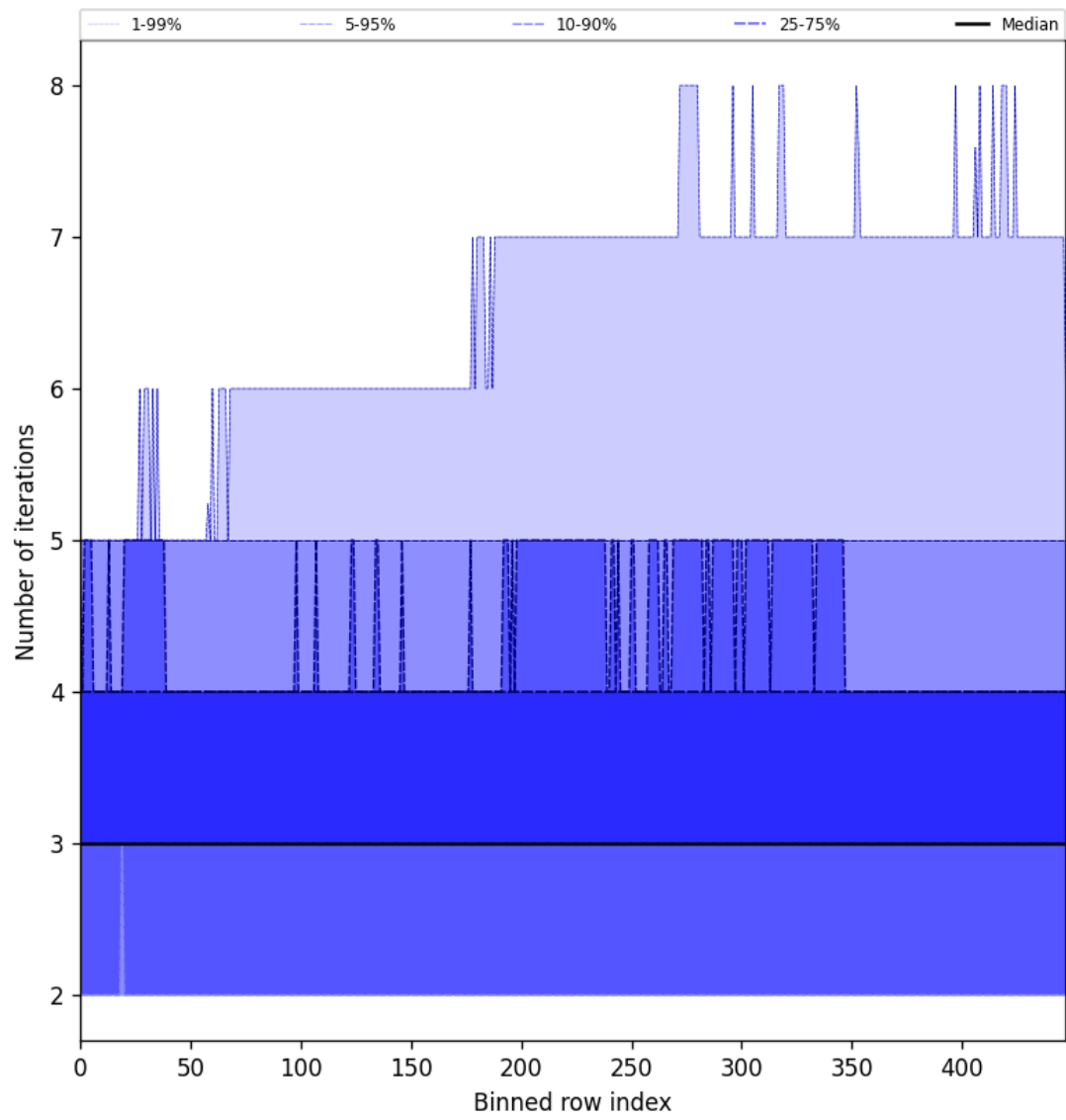
Figure 54: Along track statistics of “Number of iterations” for 2025-10-17 to 2025-10-18
