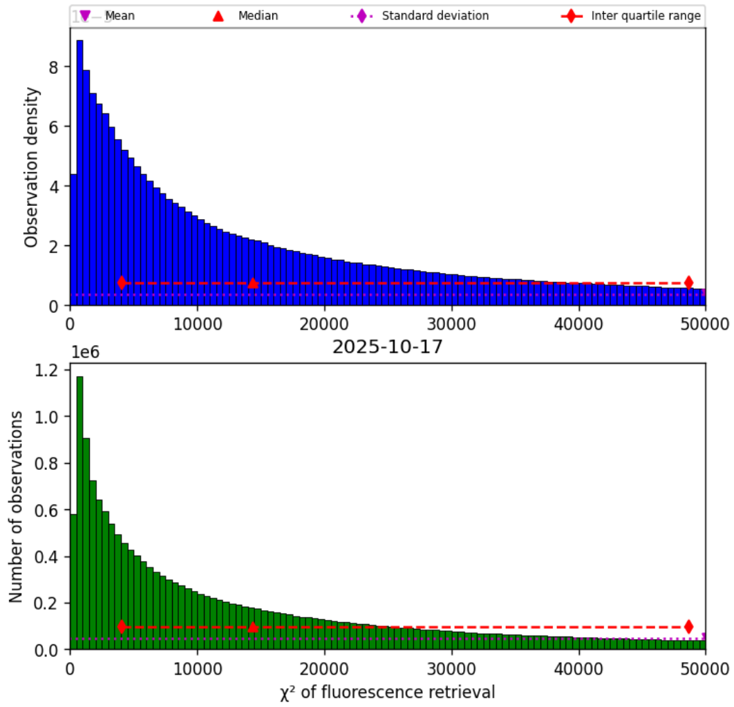
Figure 40: Histogram of “ \chi^2 of fluorescence retrieval” for 2025-10-17 to 2025-10-18
