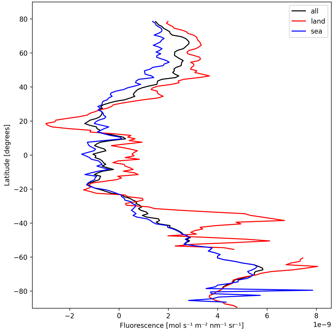
Figure 21: Zonal average of “Fluorescence” for 2025-10-17 to 2025-10-18.
