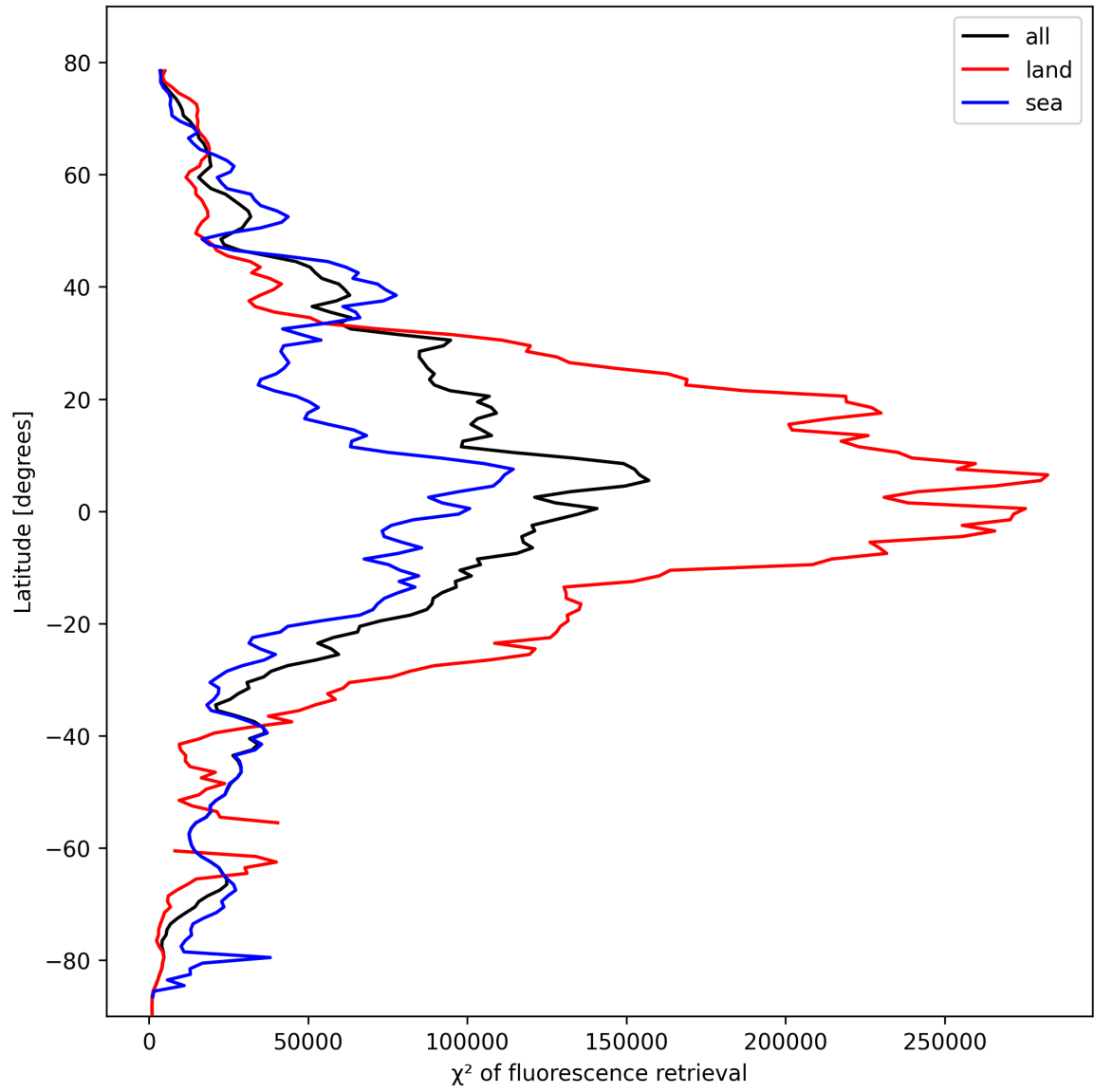
Figure 23: Zonal average of “ \chi^2 of fluorescence retrieval” for 2025-10-17 to 2025-10-18.
