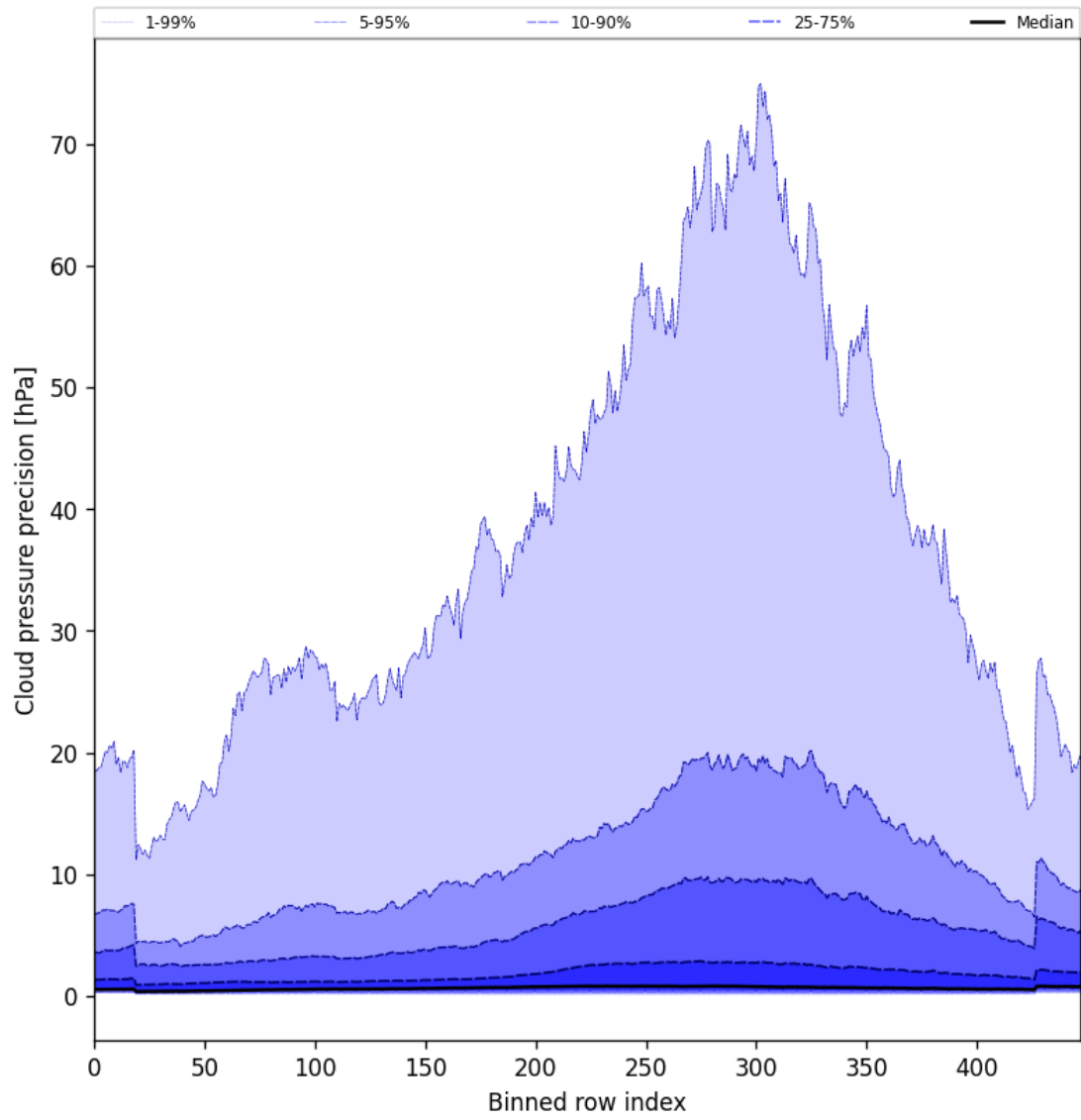
Figure 46: Along track statistics of “Cloud pressure precision” for 2025-10-17 to 2025-10-18
