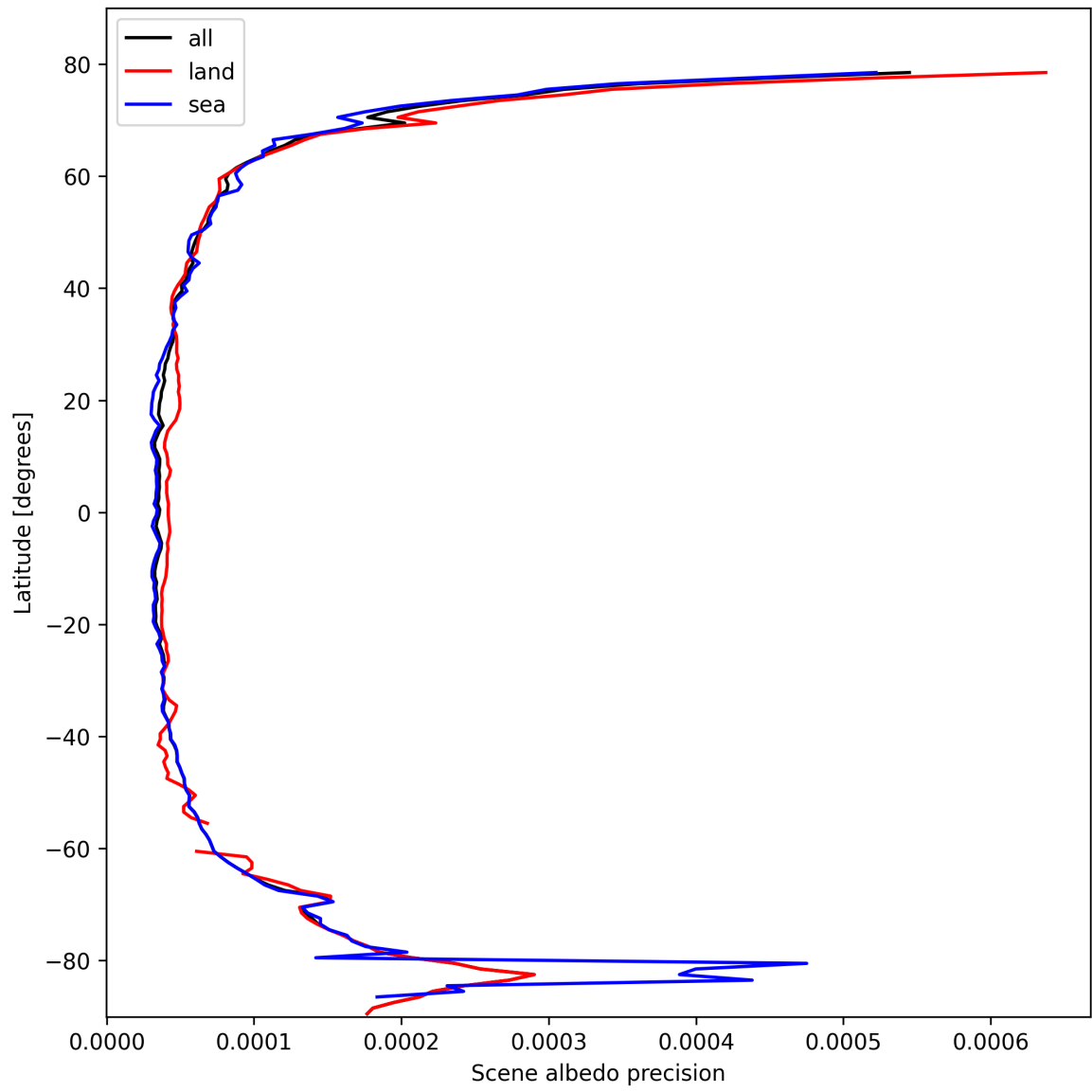
Figure 16: Zonal average of “Scene albedo precision” for 2025-10-17 to 2025-10-18.
