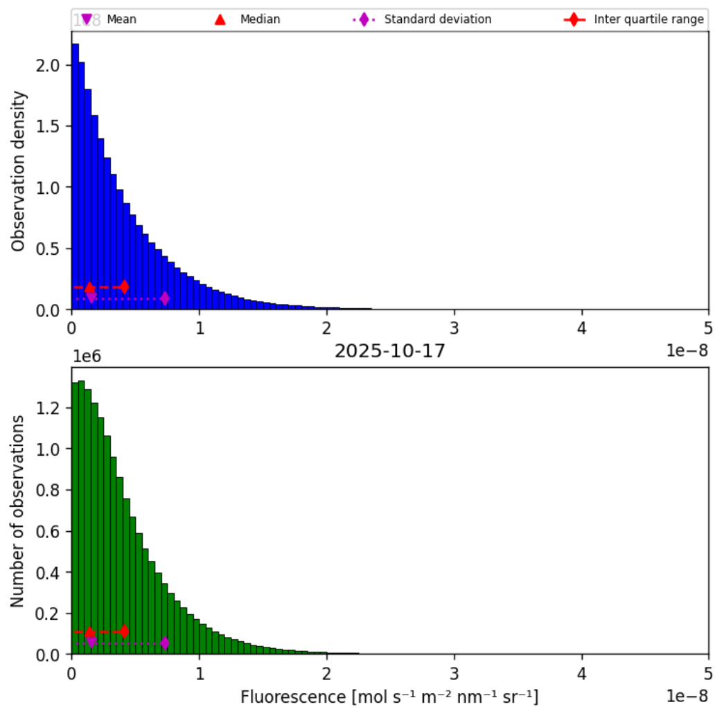
Figure 38: Histogram of “Fluorescence” for 2025-10-17 to 2025-10-18
