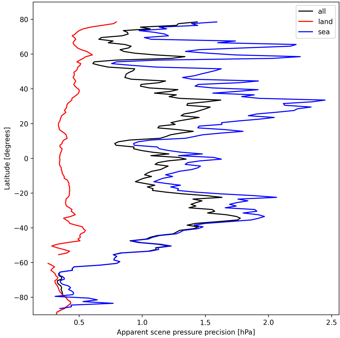
Figure 18: Zonal average of “Apparent scene pressure precision” for 2025-10-17 to 2025-10-18.
