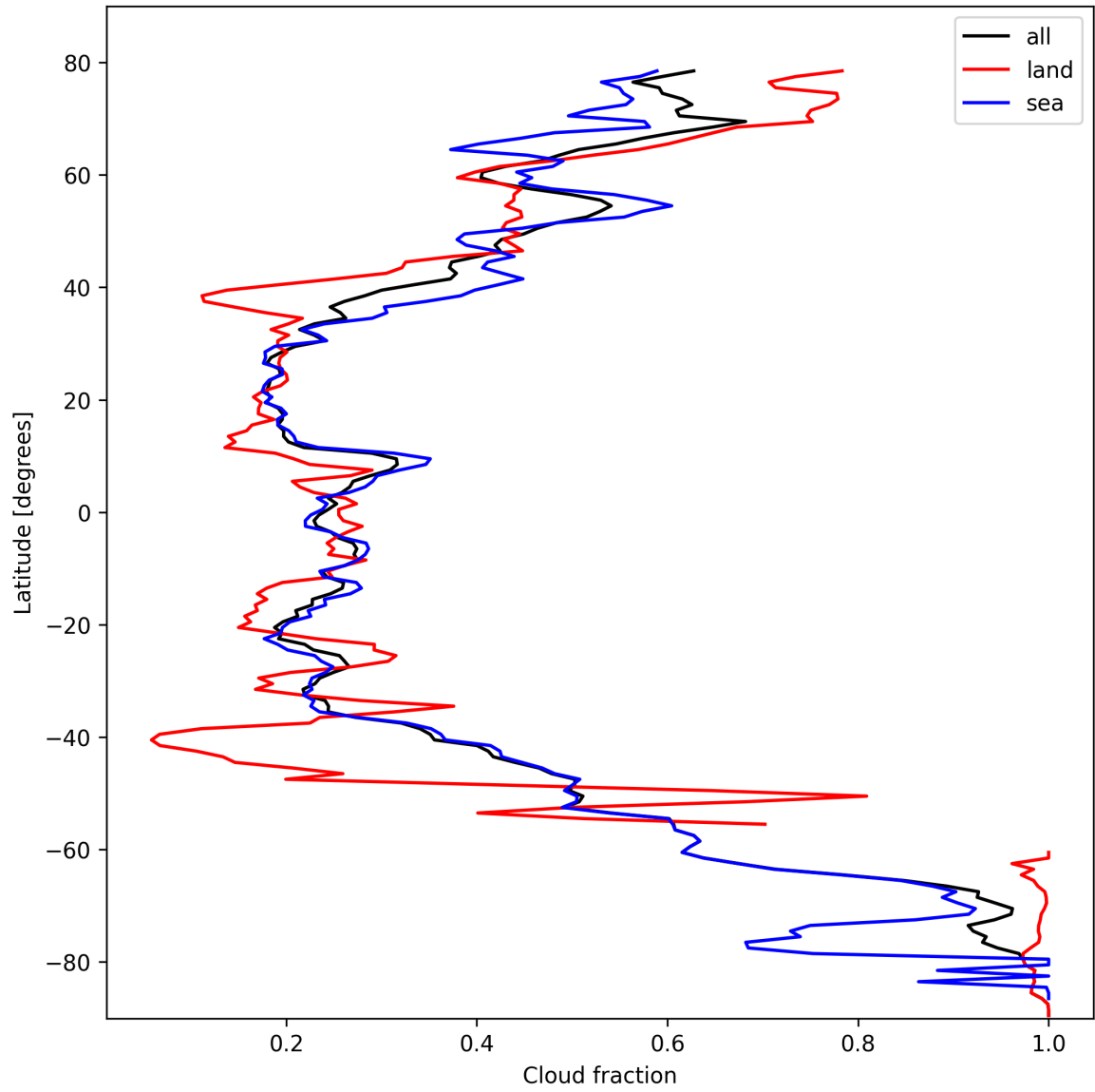
Figure 13: Zonal average of “Cloud fraction” for 2025-10-17 to 2025-10-18.
