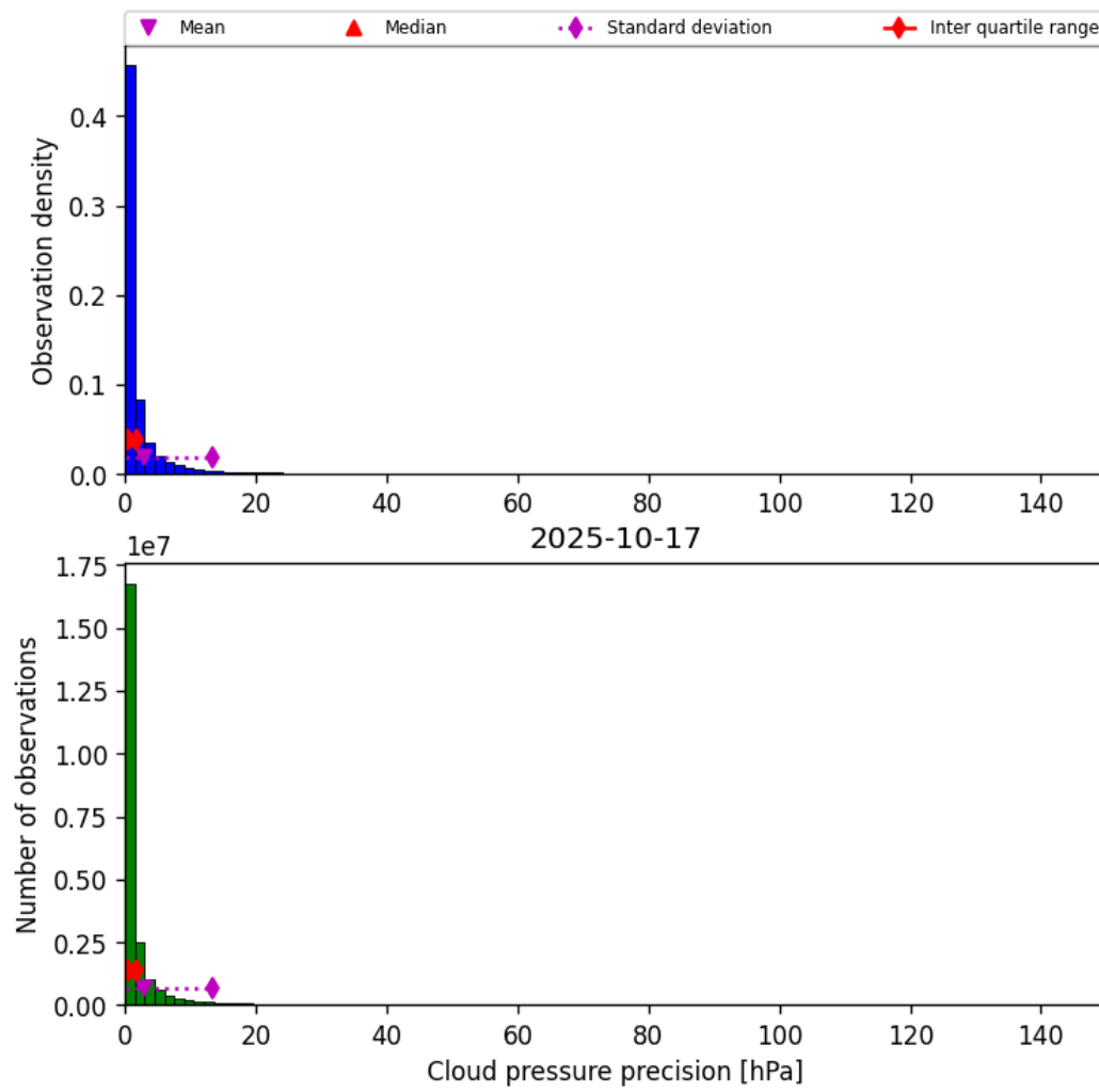
Figure 29: Histogram of “Cloud pressure precision” for 2025-10-17 to 2025-10-18
