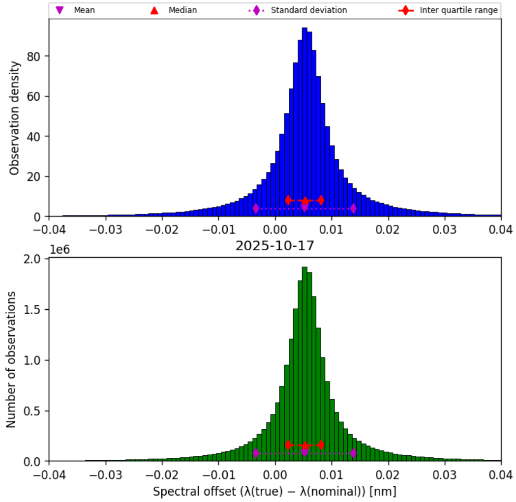
Figure 43: Histogram of “Spectral offset ( \lambda_{\text{true}} - \lambda_{\text{nominal}} )” for 2025-10-17 to 2025-10-18
