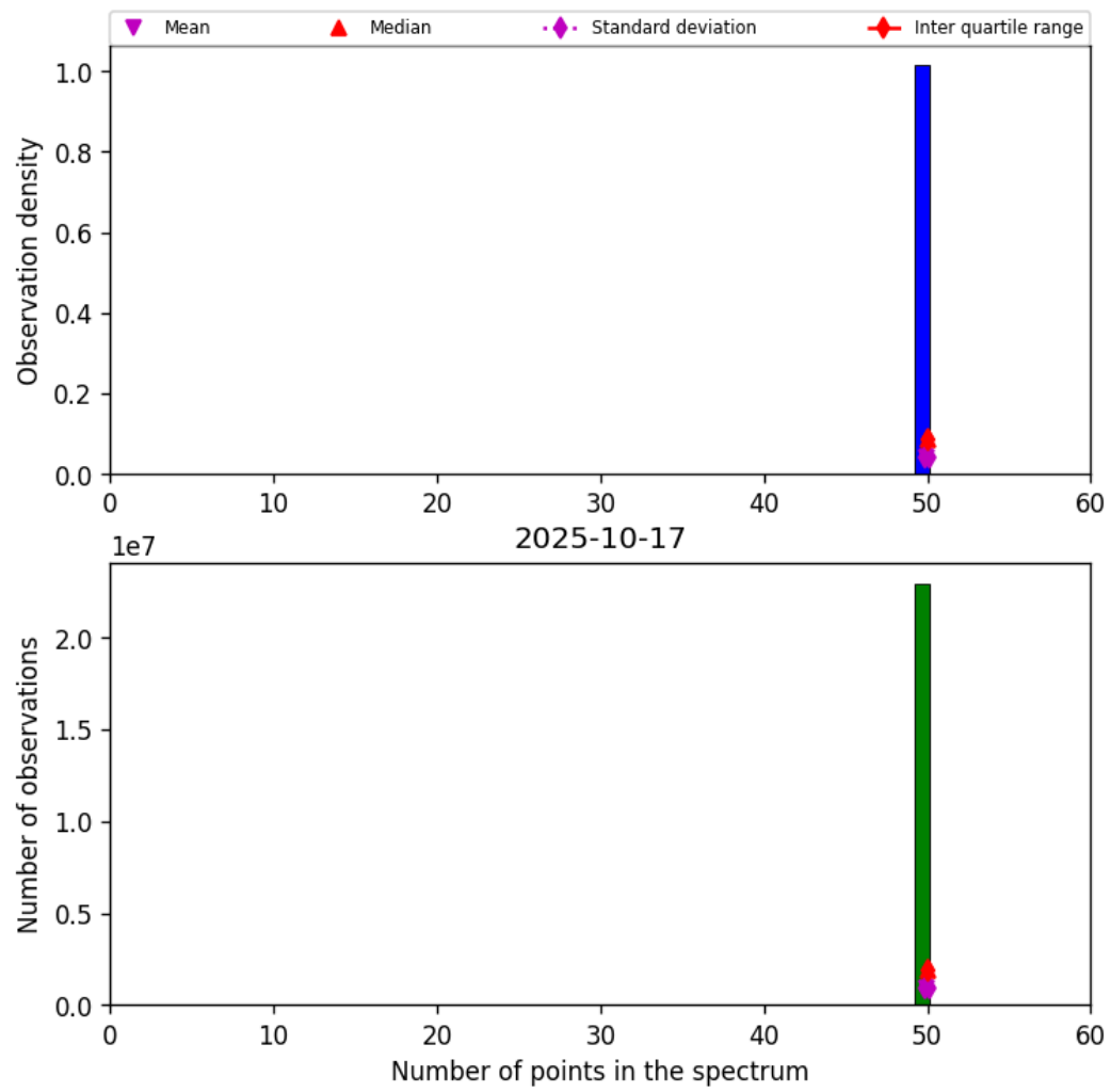
Figure 42: Histogram of “Number of points in the spectrum” for 2025-10-17 to 2025-10-18
