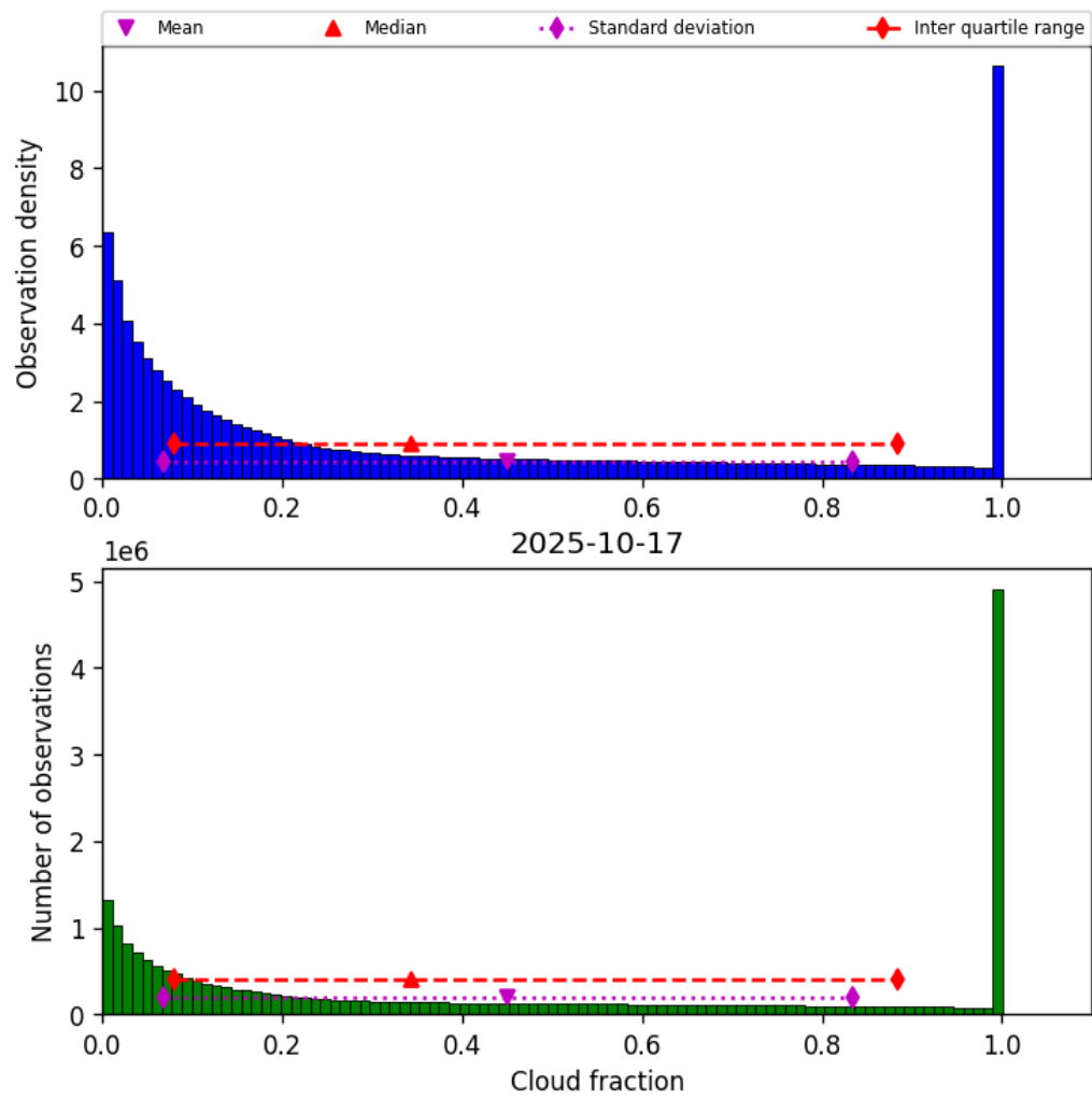
Figure 30: Histogram of “Cloud fraction” for 2025-10-17 to 2025-10-18
