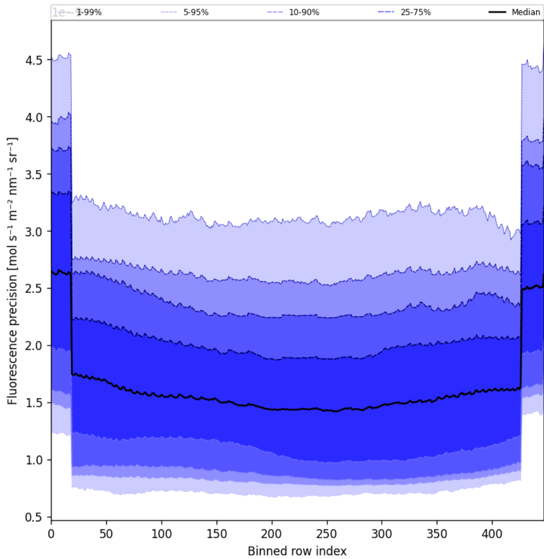
Figure 56: Along track statistics of “Fluorescence precision” for 2025-10-17 to 2025-10-18
