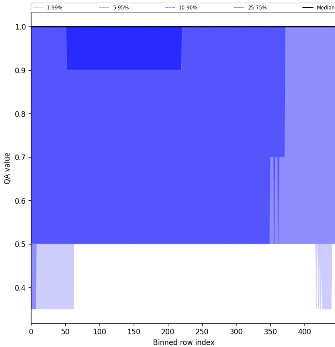
Figure 44: Along track statistics of “QA value” for 2025-10-17 to 2025-10-18
