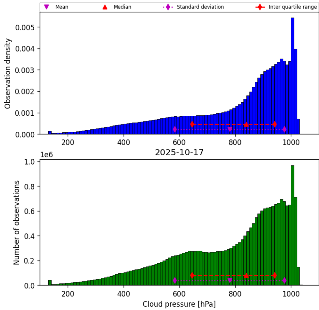
Figure 28: Histogram of “Cloud pressure” for 2025-10-17 to 2025-10-18
