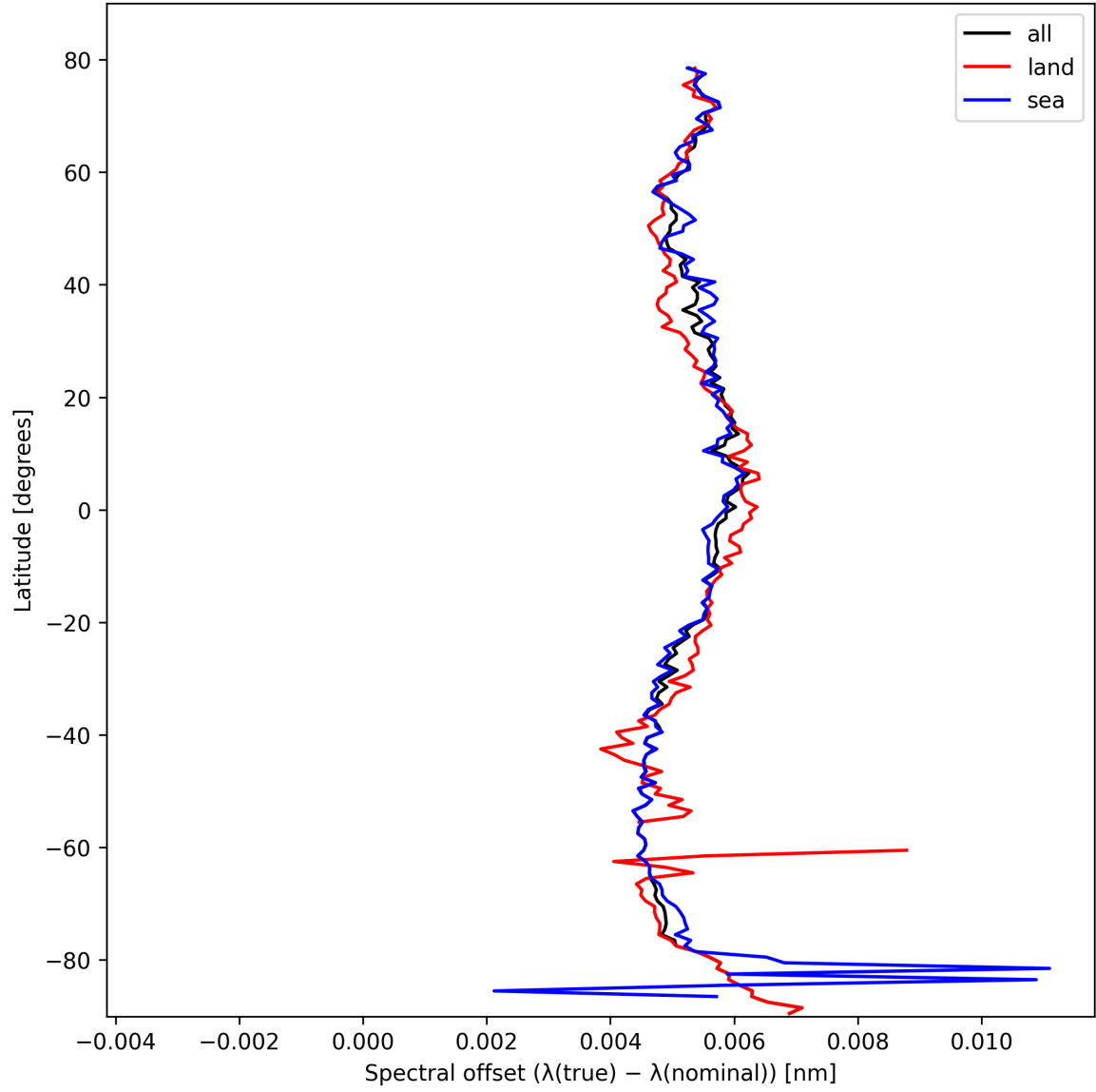
Figure 26: Zonal average of “Spectral offset ( \lambda_{\text{true}} - \lambda_{\text{nominal}} )” for 2025-10-17 to 2025-10-18.
