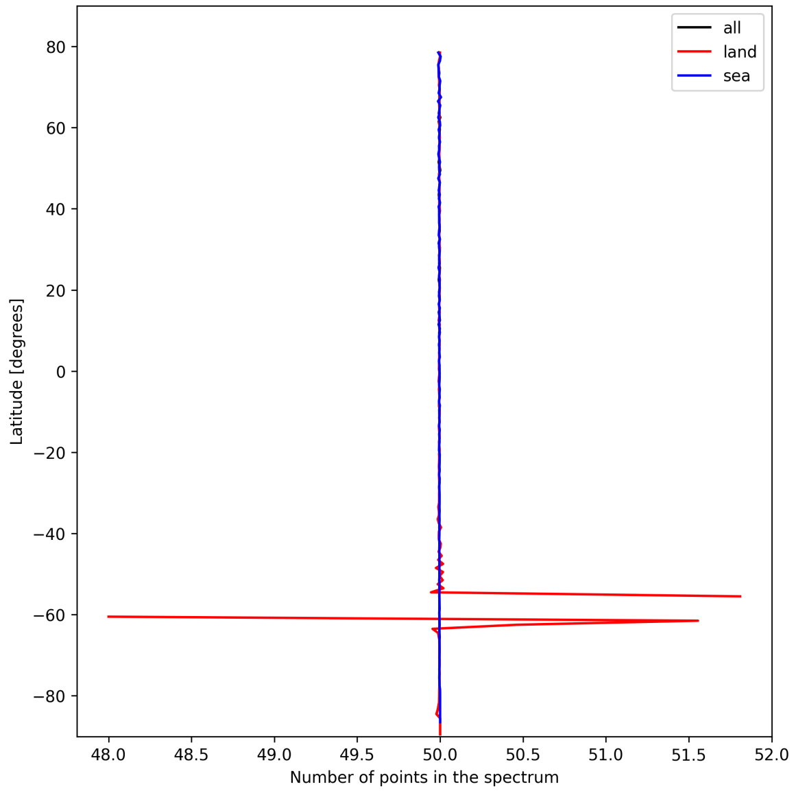
Figure 25: Zonal average of “Number of points in the spectrum” for 2025-10-17 to 2025-10-18.
