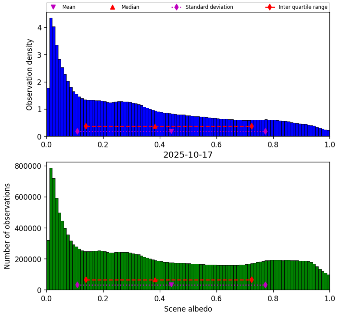
Figure 32: Histogram of “Scene albedo” for 2025-10-17 to 2025-10-18
