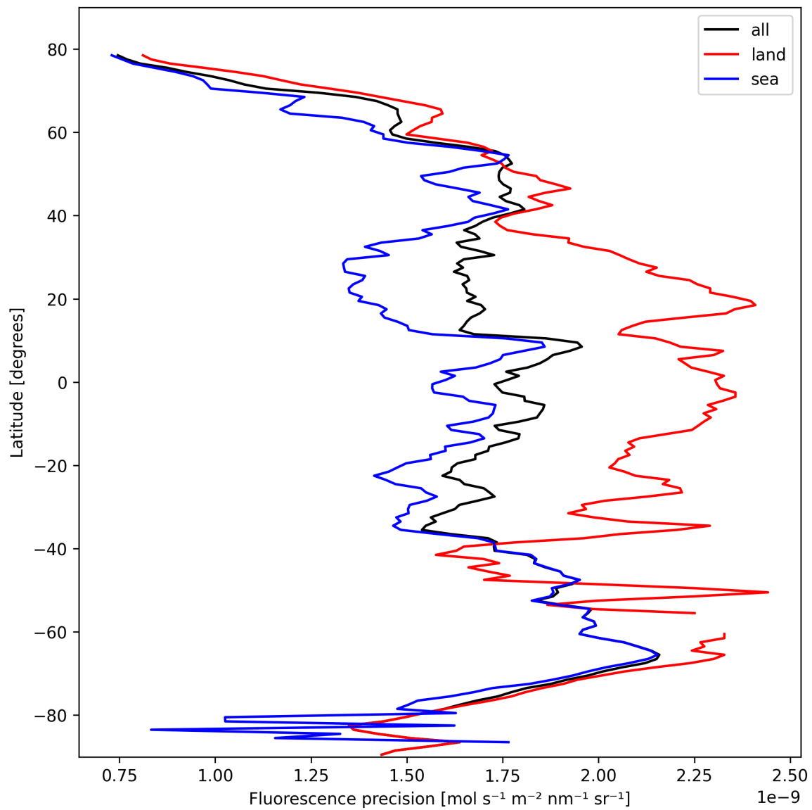
Figure 22: Zonal average of “Fluorescence precision” for 2025-10-17 to 2025-10-18.
