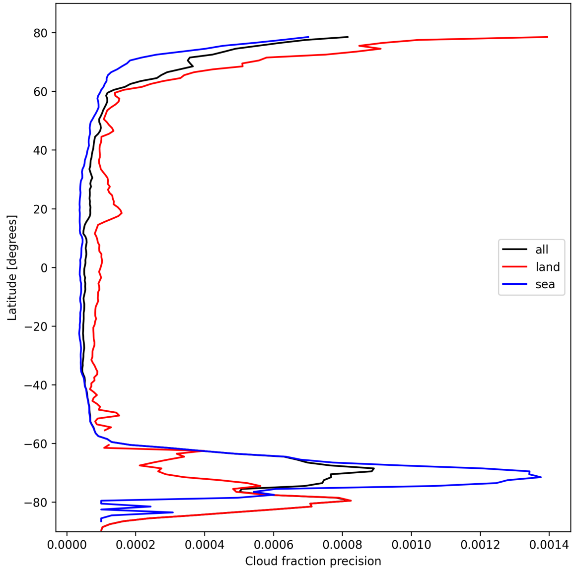
Figure 14: Zonal average of “Cloud fraction precision” for 2025-10-17 to 2025-10-18.
