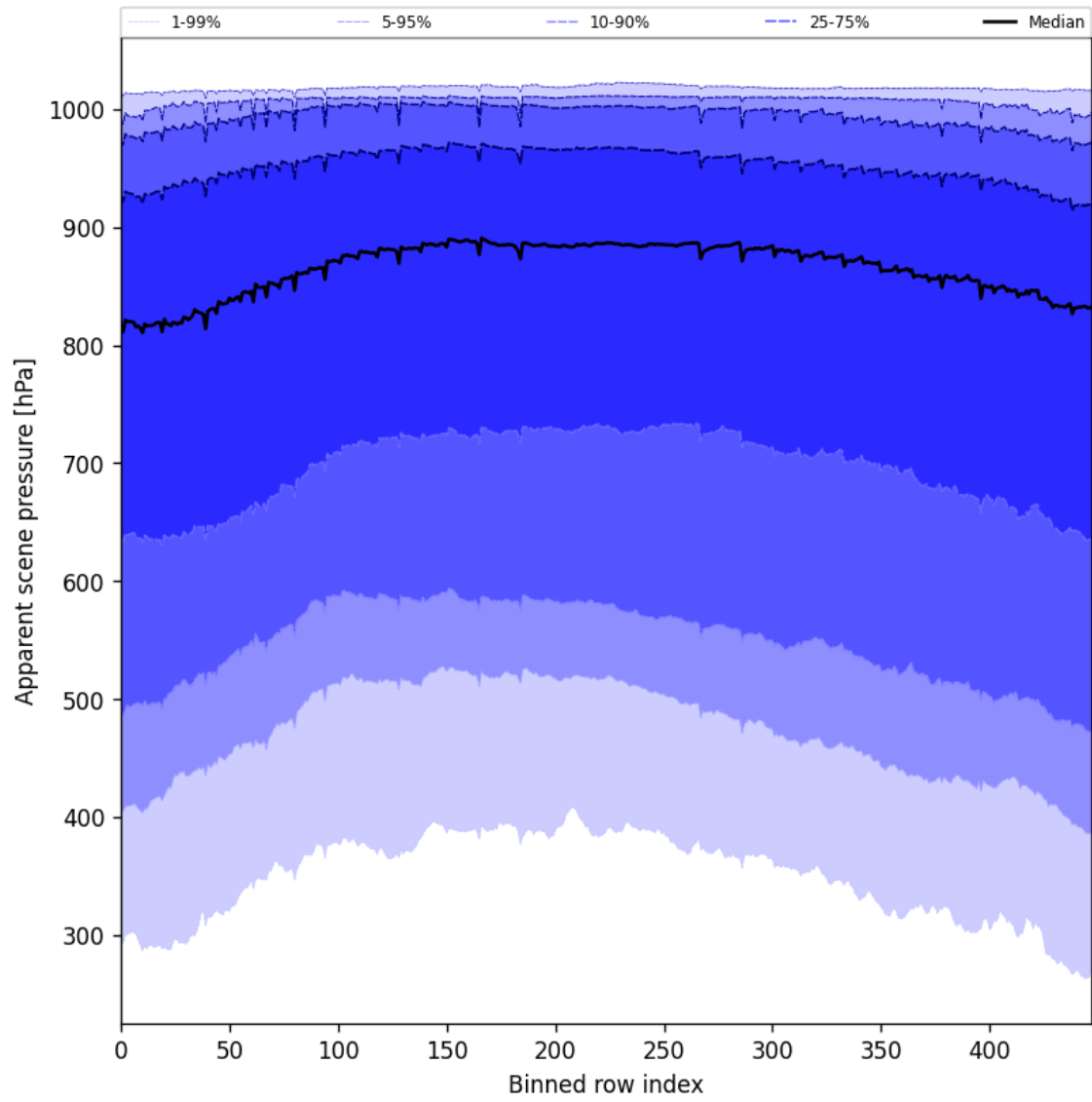
Figure 51: Along track statistics of “Apparent scene pressure” for 2025-10-17 to 2025-10-18
