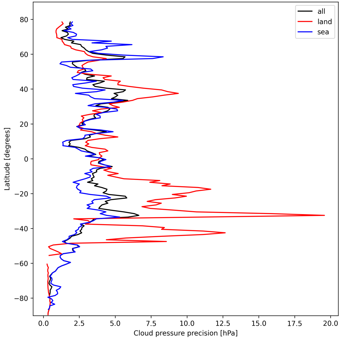
Figure 12: Zonal average of “Cloud pressure precision” for 2025-10-17 to 2025-10-18.
