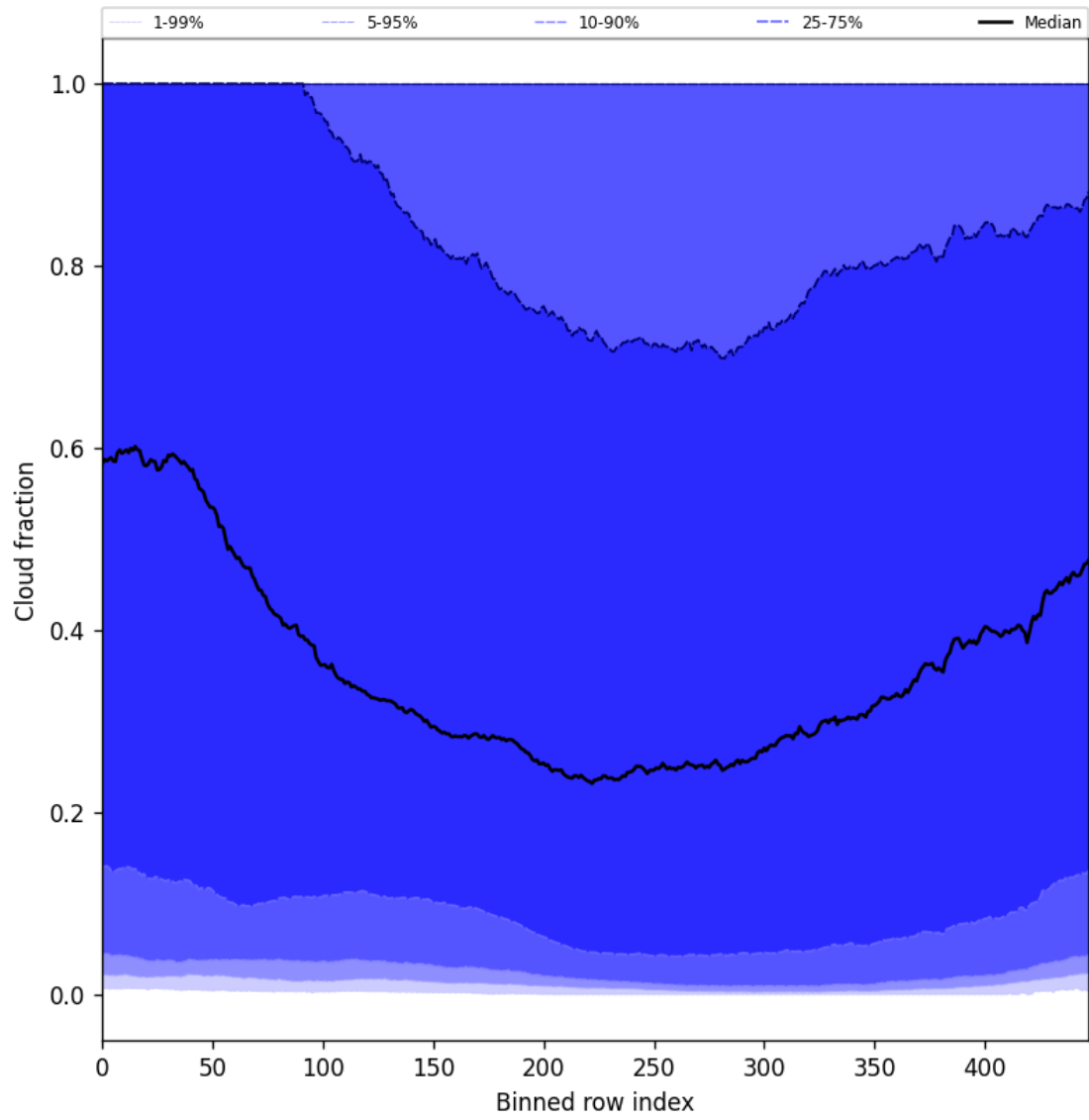
Figure 47: Along track statistics of “Cloud fraction” for 2025-10-17 to 2025-10-18
