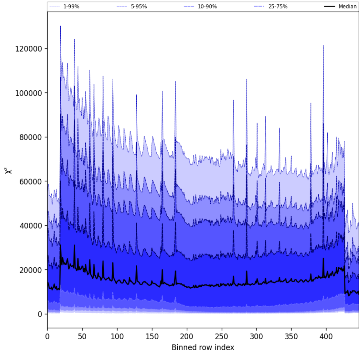
Figure 53: Along track statistics of “ \chi^2 ” for 2025-10-17 to 2025-10-18
