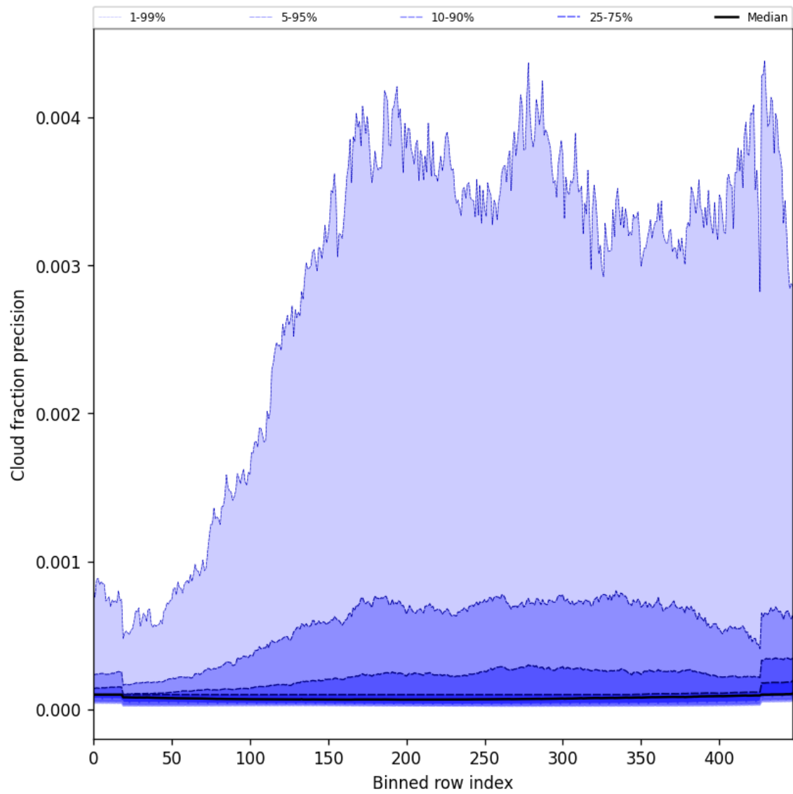
Figure 48: Along track statistics of “Cloud fraction precision” for 2025-10-17 to 2025-10-18
