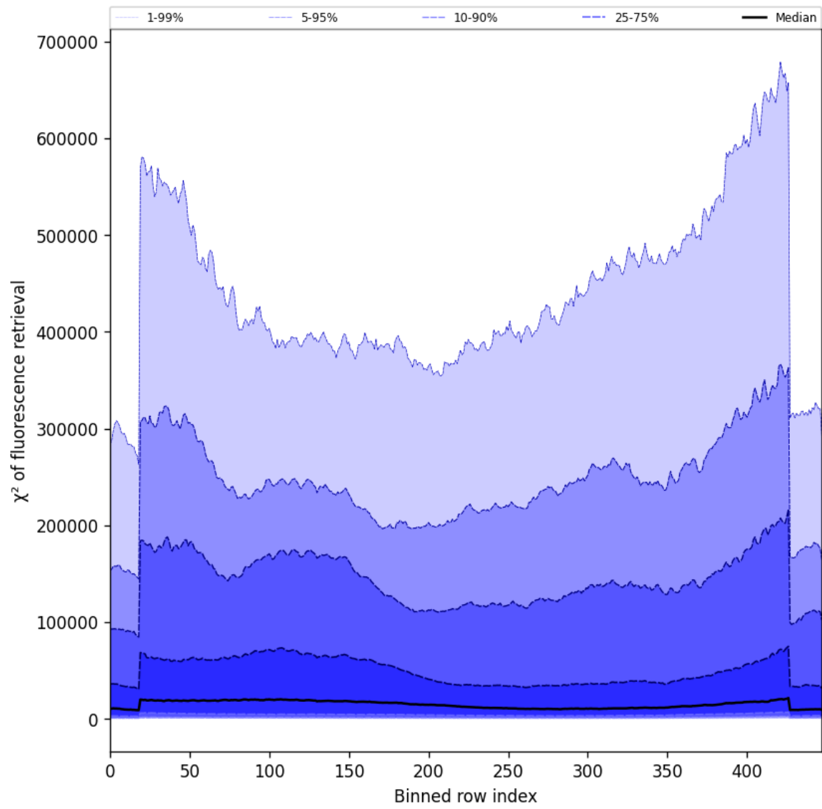
Figure 57: Along track statistics of “ \chi^2 of fluorescence retrieval” for 2025-10-17 to 2025-10-18
