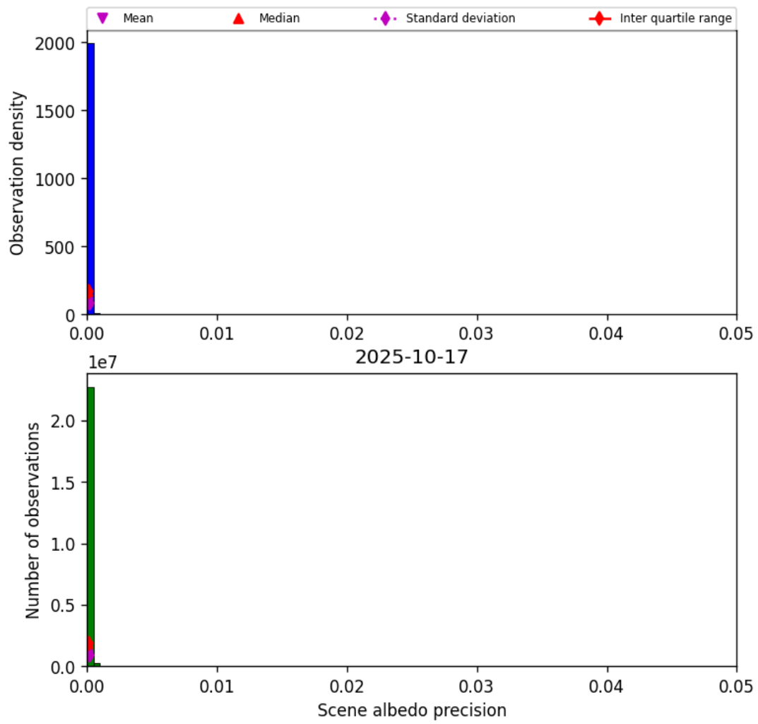
Figure 33: Histogram of “Scene albedo precision” for 2025-10-17 to 2025-10-18
