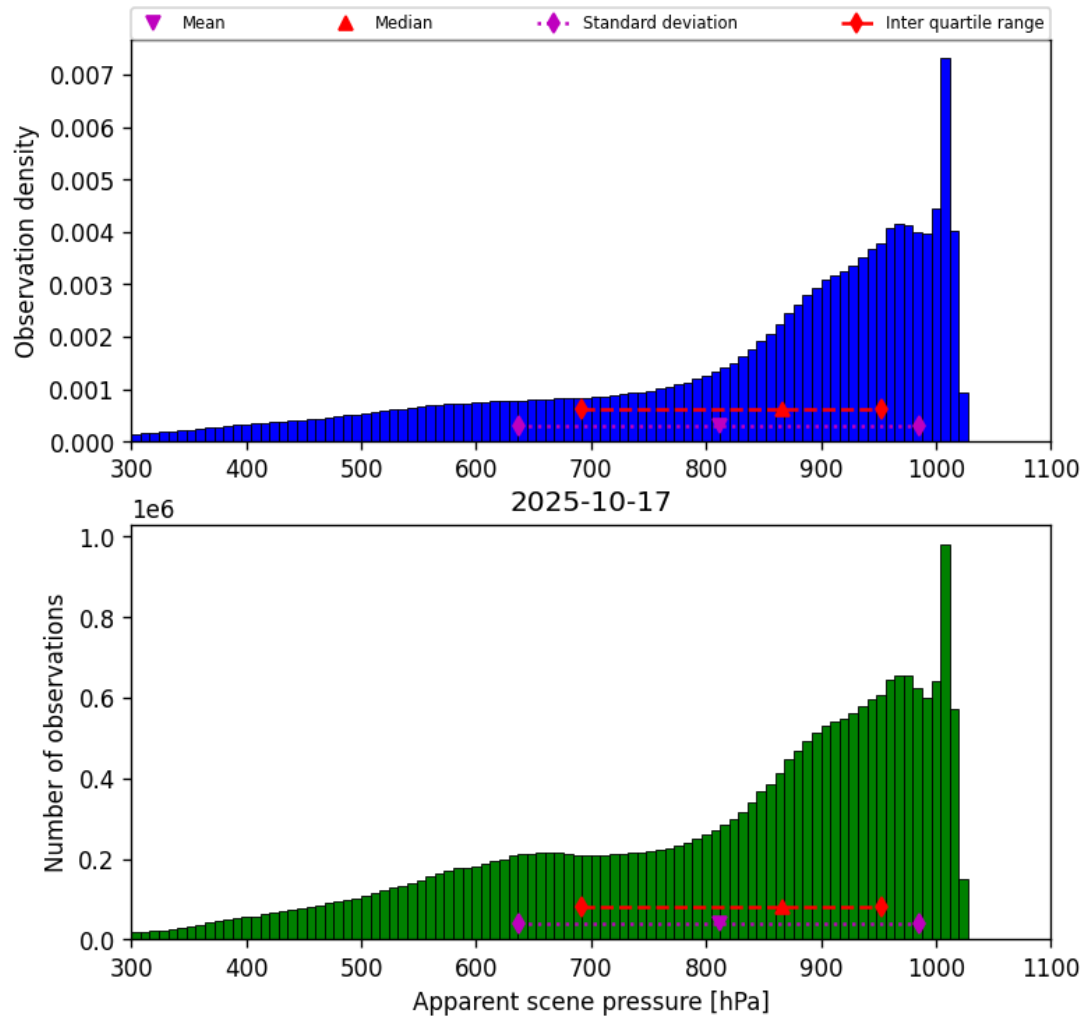
Figure 34: Histogram of “Apparent scene pressure” for 2025-10-17 to 2025-10-18
