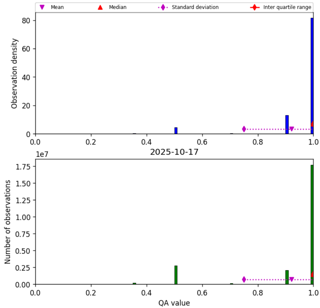
Figure 27: Histogram of “QA value” for 2025-10-17 to 2025-10-18
