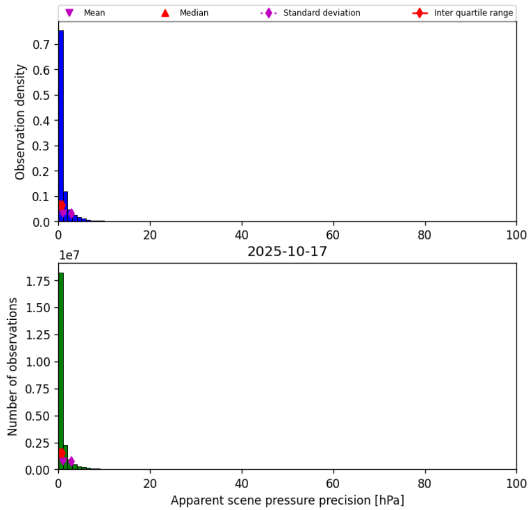
Figure 35: Histogram of “Apparent scene pressure precision” for 2025-10-17 to 2025-10-18
