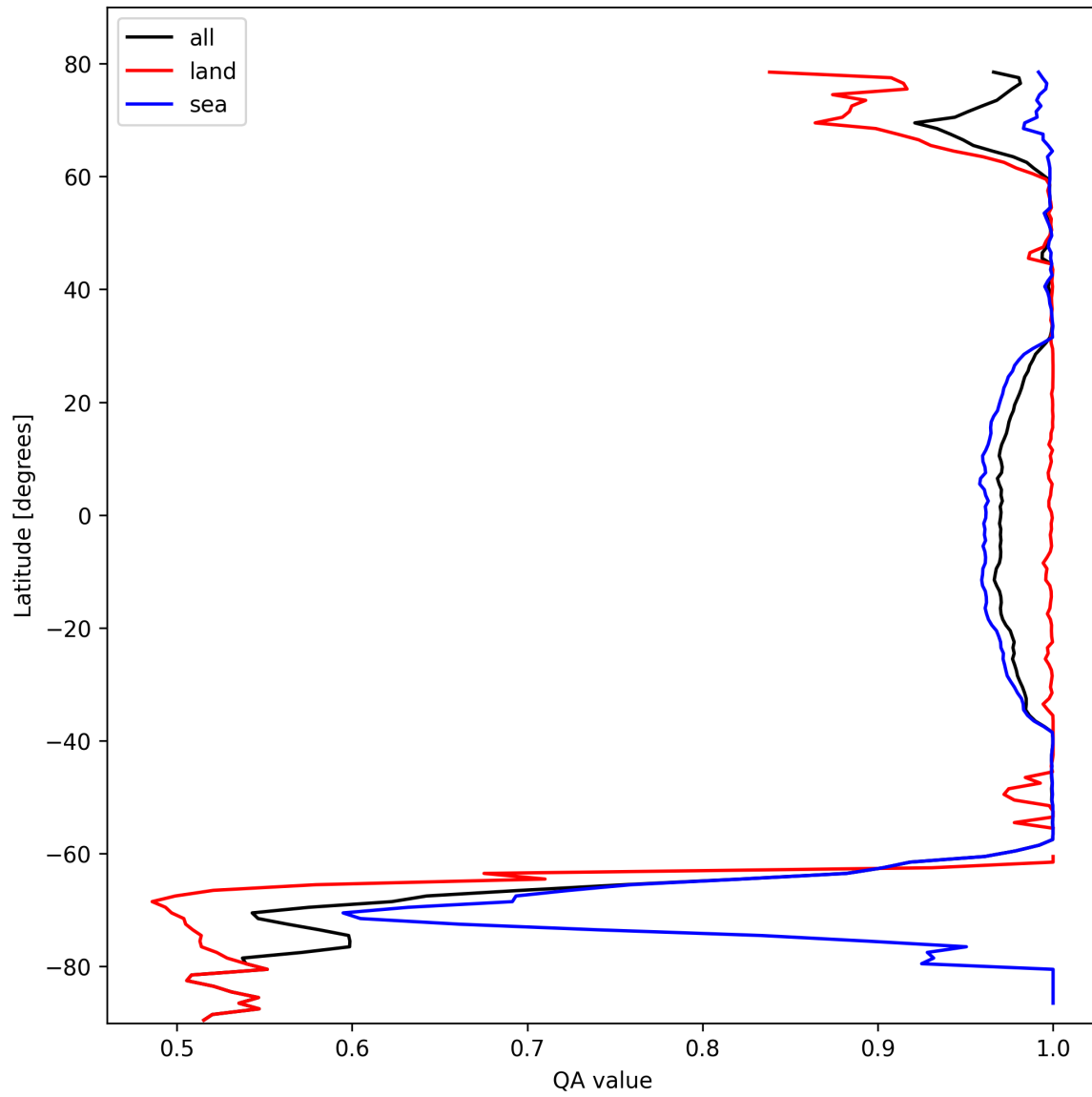
Figure 10: Zonal average of “QA value” for 2025-10-17 to 2025-10-18.
