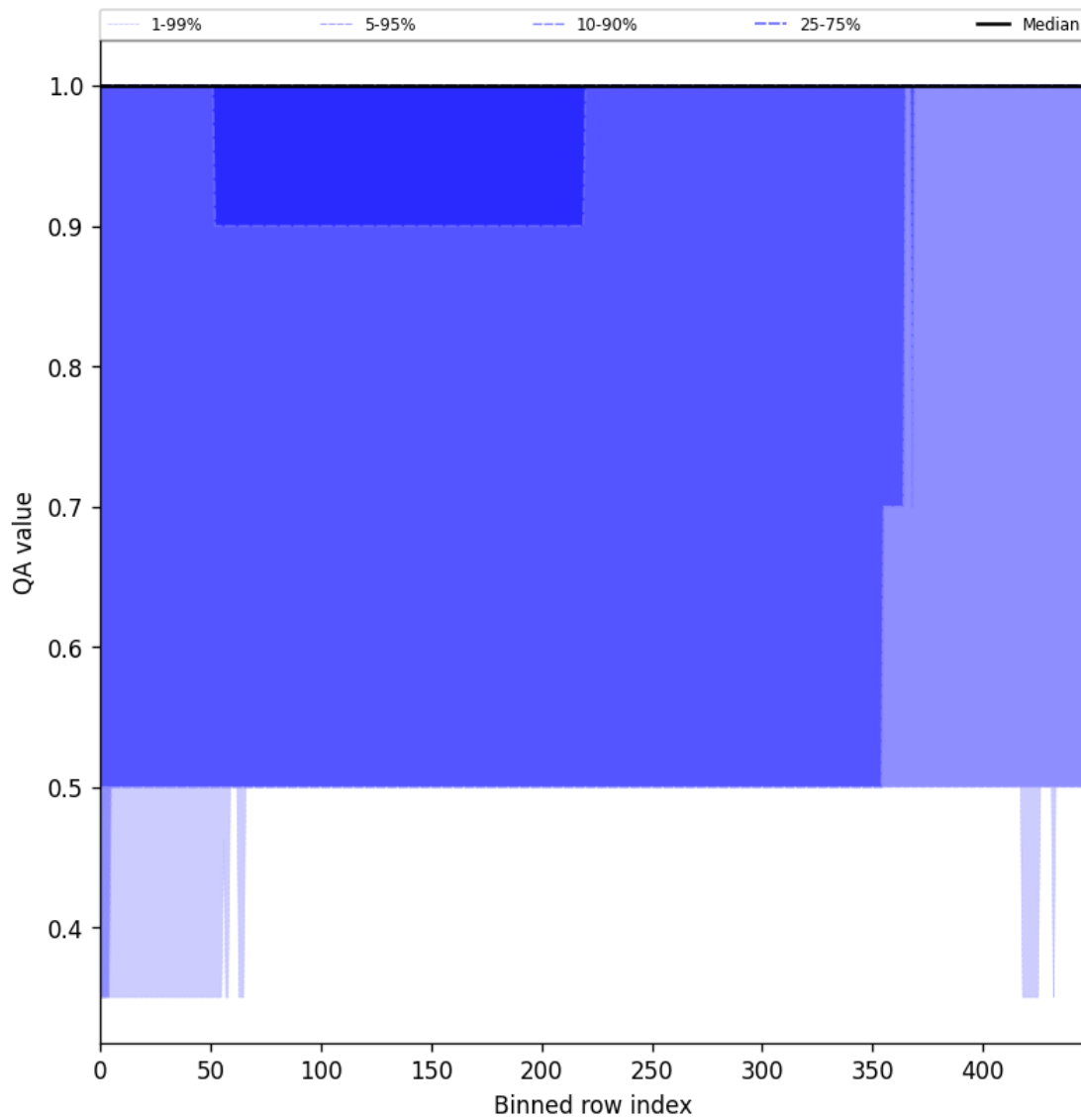
Figure 44: Along track statistics of “QA value” for 2025-10-18 to 2025-10-19
