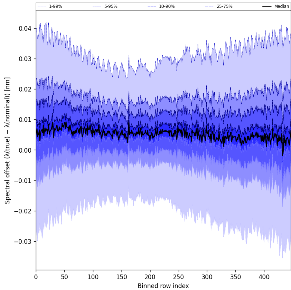
Figure 60: Along track statistics of “Spectral offset ( \lambda_{\text{true}} - \lambda_{\text{nominal}} )” for 2025-10-18 to 2025-10-19
