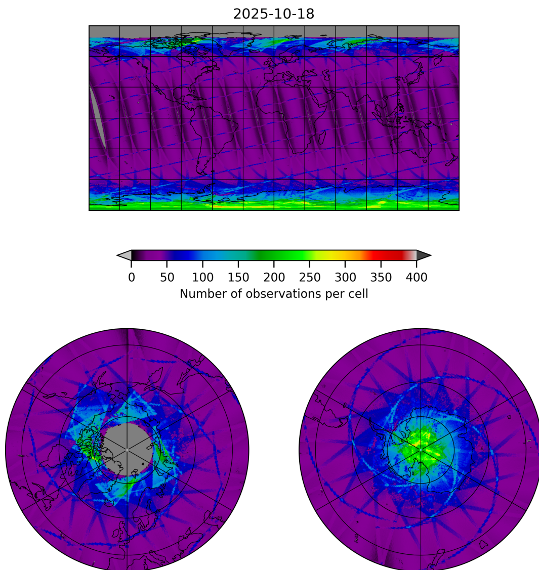
Figure 9: Map of the number of observations for 2025-10-18 to 2025-10-19
