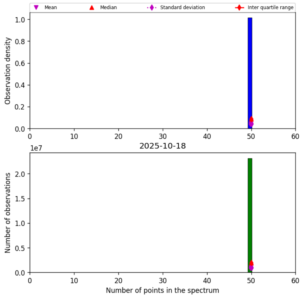
Figure 42: Histogram of “Number of points in the spectrum” for 2025-10-18 to 2025-10-19
