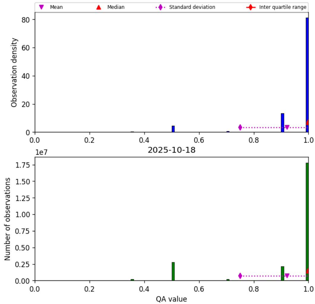
Figure 27: Histogram of “QA value” for 2025-10-18 to 2025-10-19
