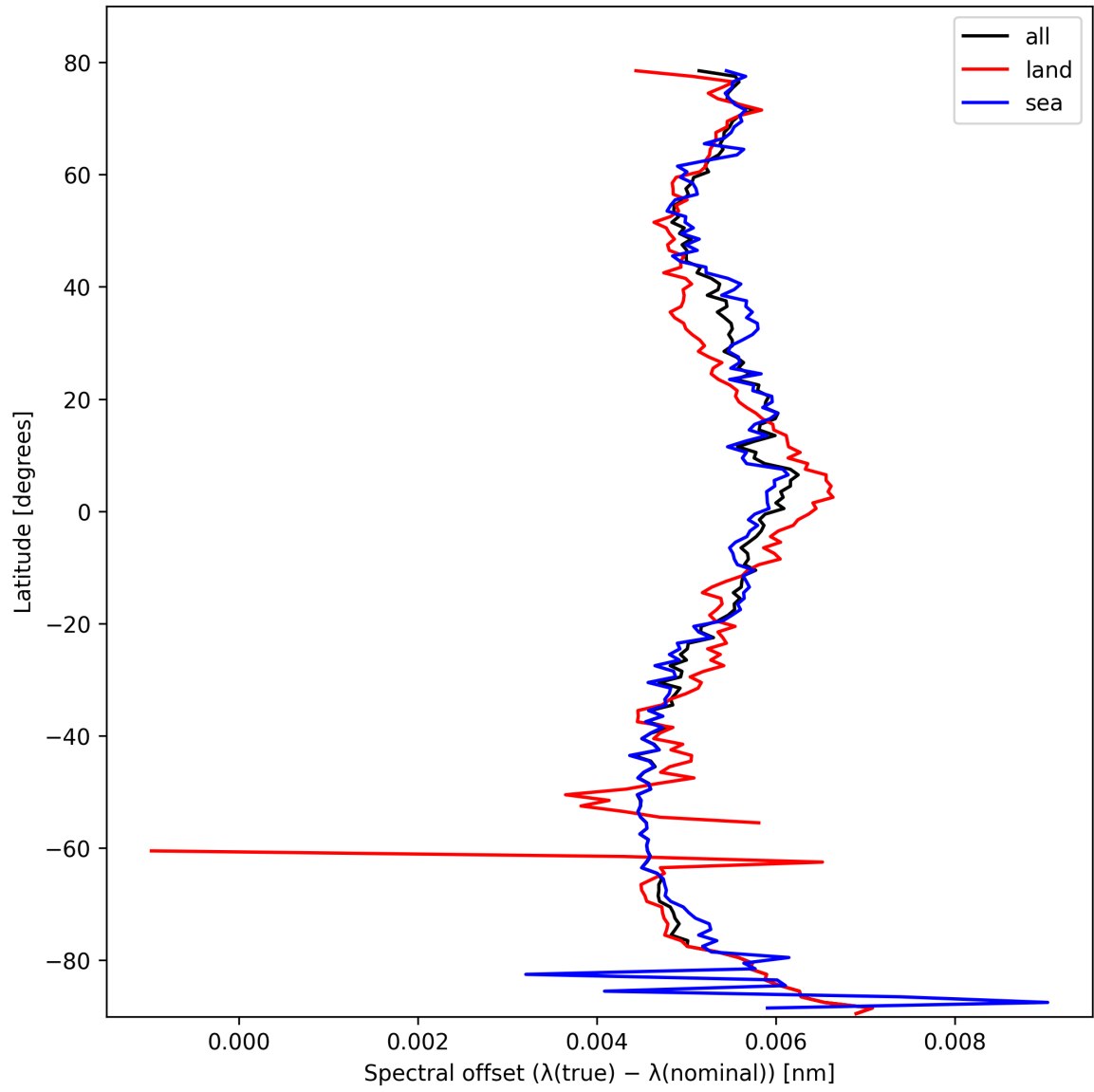
Figure 26: Zonal average of “Spectral offset ( \lambda_{\text{true}} - \lambda_{\text{nominal}} )” for 2025-10-18 to 2025-10-19.
