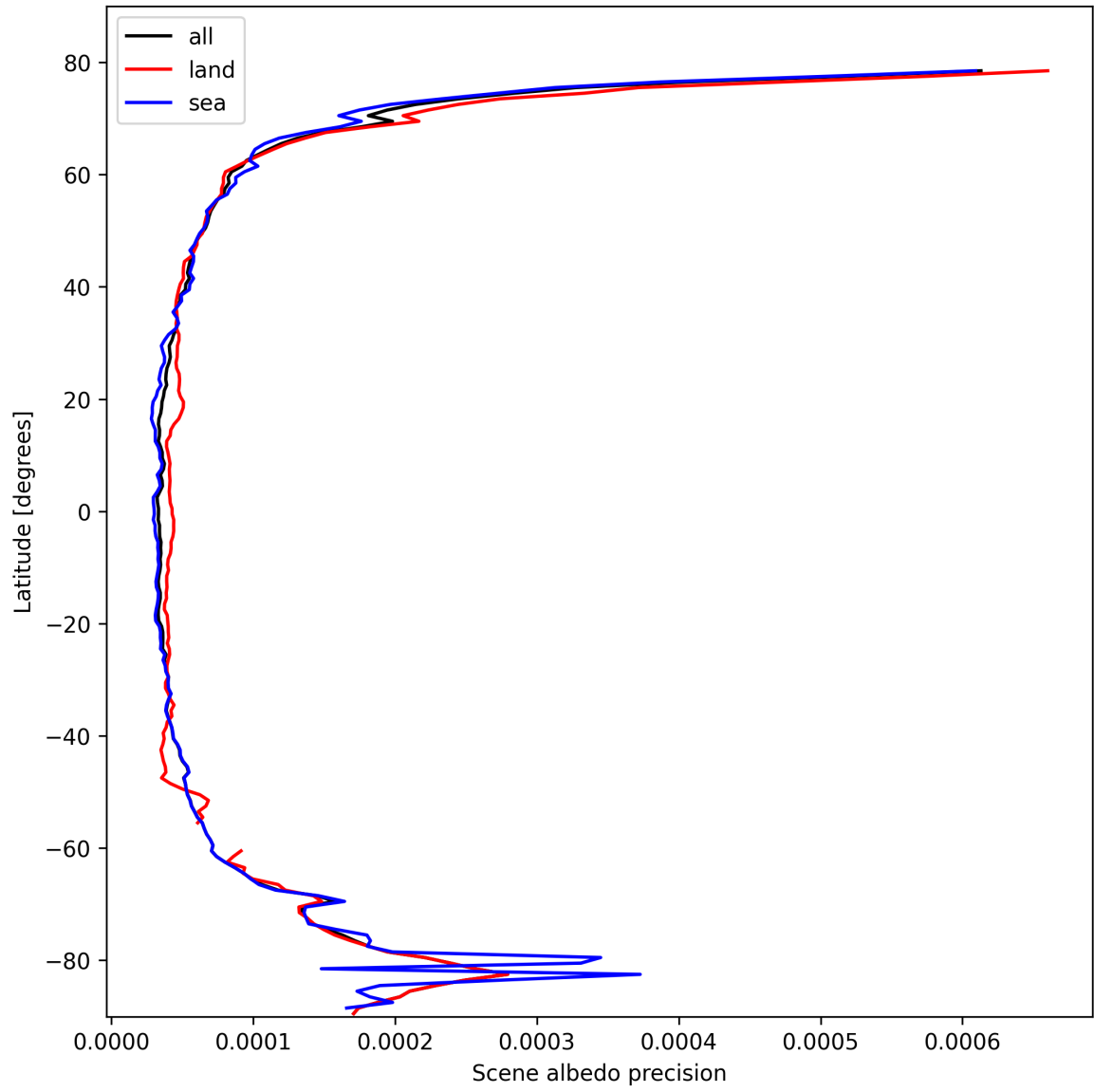
Figure 16: Zonal average of “Scene albedo precision” for 2025-10-18 to 2025-10-19.
