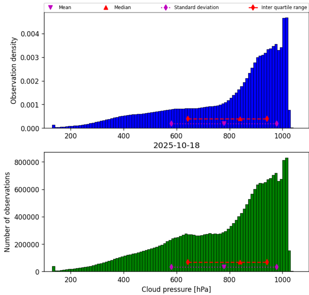
Figure 28: Histogram of “Cloud pressure” for 2025-10-18 to 2025-10-19
