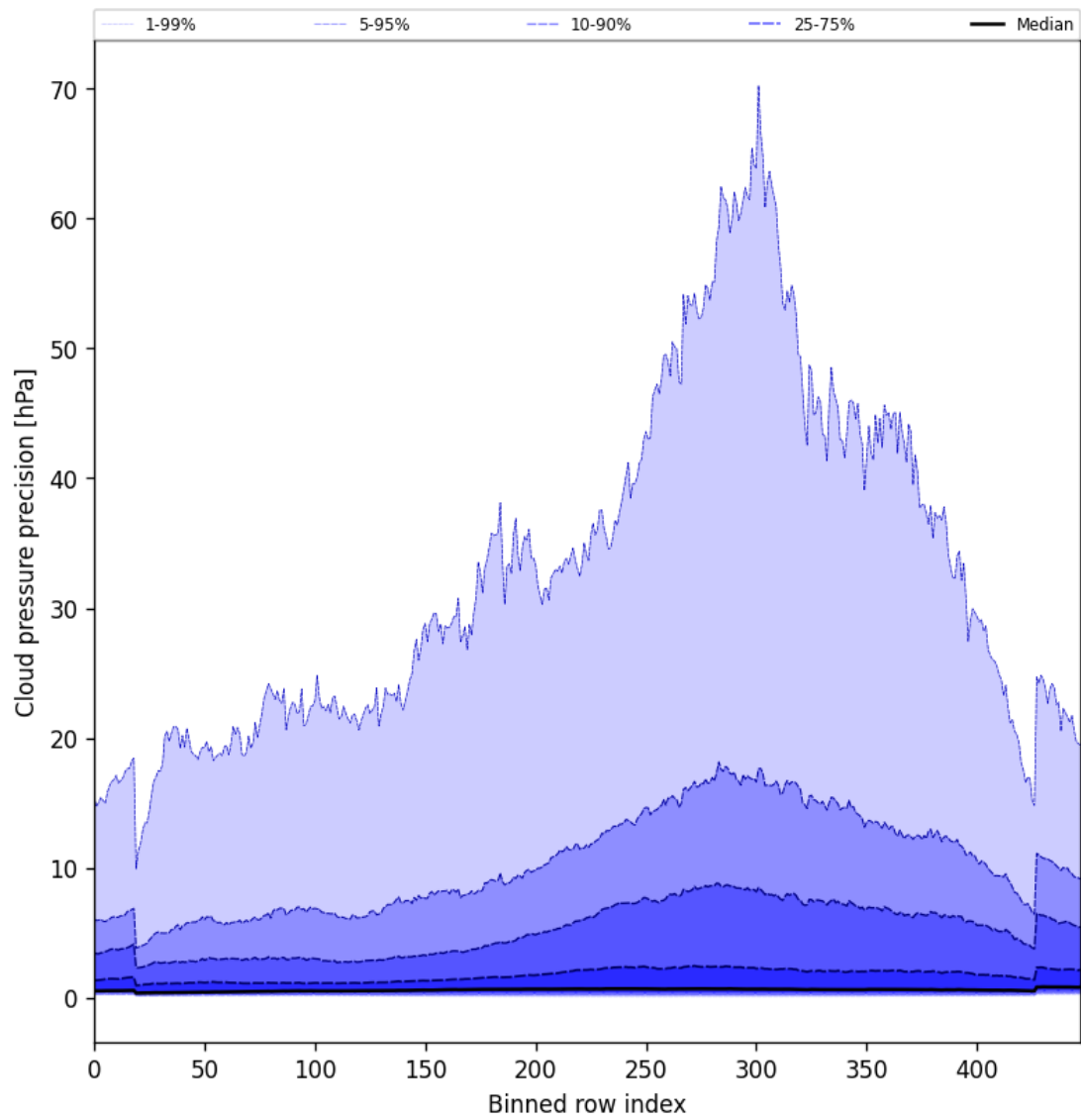
Figure 46: Along track statistics of “Cloud pressure precision” for 2025-10-18 to 2025-10-19
