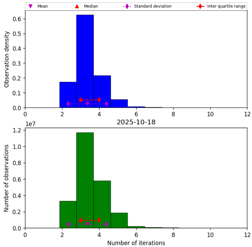
Figure 37: Histogram of “Number of iterations” for 2025-10-18 to 2025-10-19
