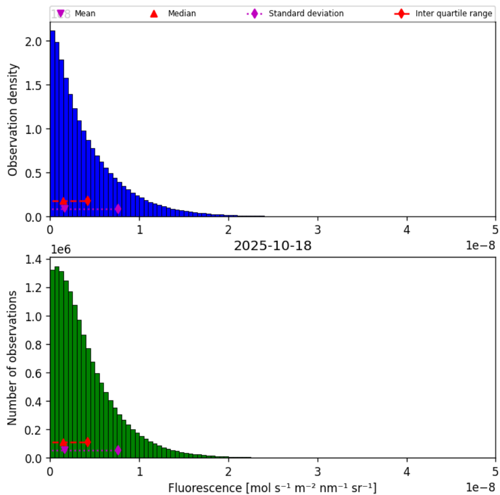
Figure 38: Histogram of “Fluorescence” for 2025-10-18 to 2025-10-19
