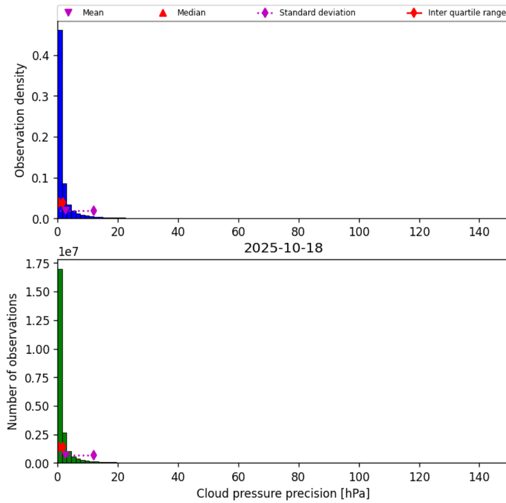
Figure 29: Histogram of "Cloud pressure precision" for 2025-10-18 to 2025-10-19
