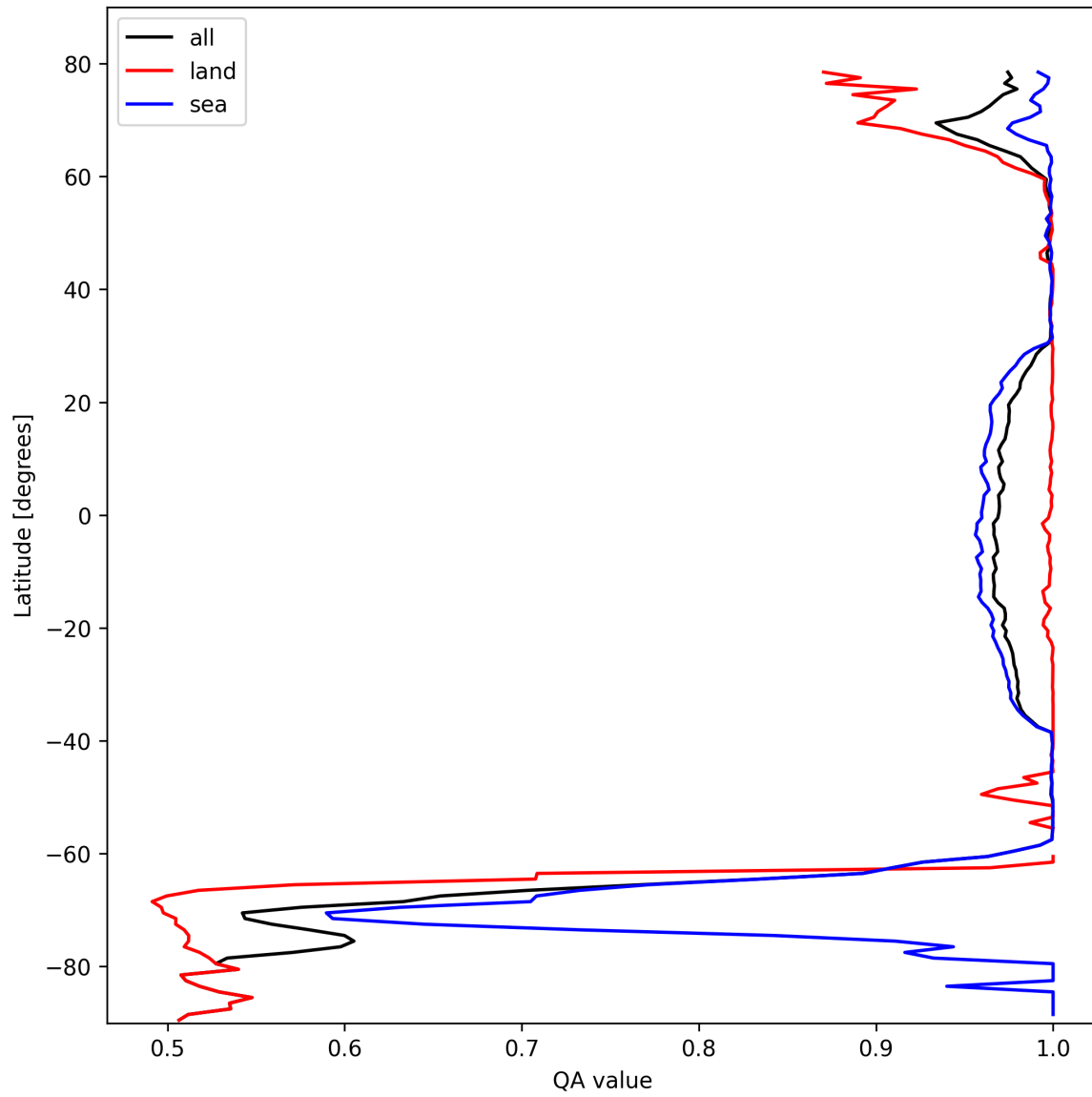
Figure 10: Zonal average of “QA value” for 2025-10-18 to 2025-10-19.
