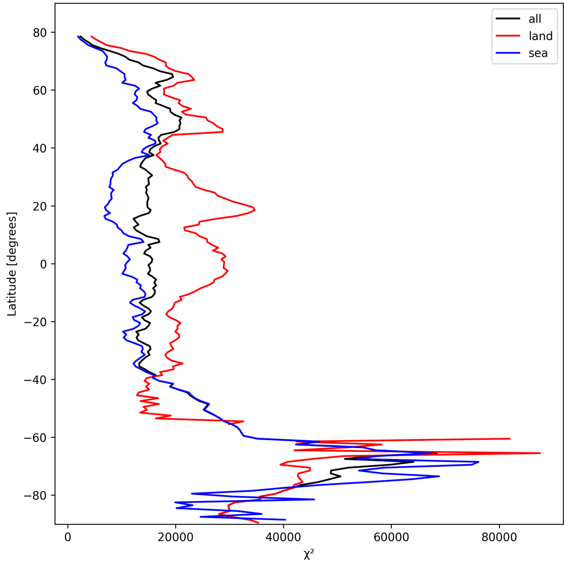
Figure 19: Zonal average of “ \chi^2 ” for 2025-10-18 to 2025-10-19.
