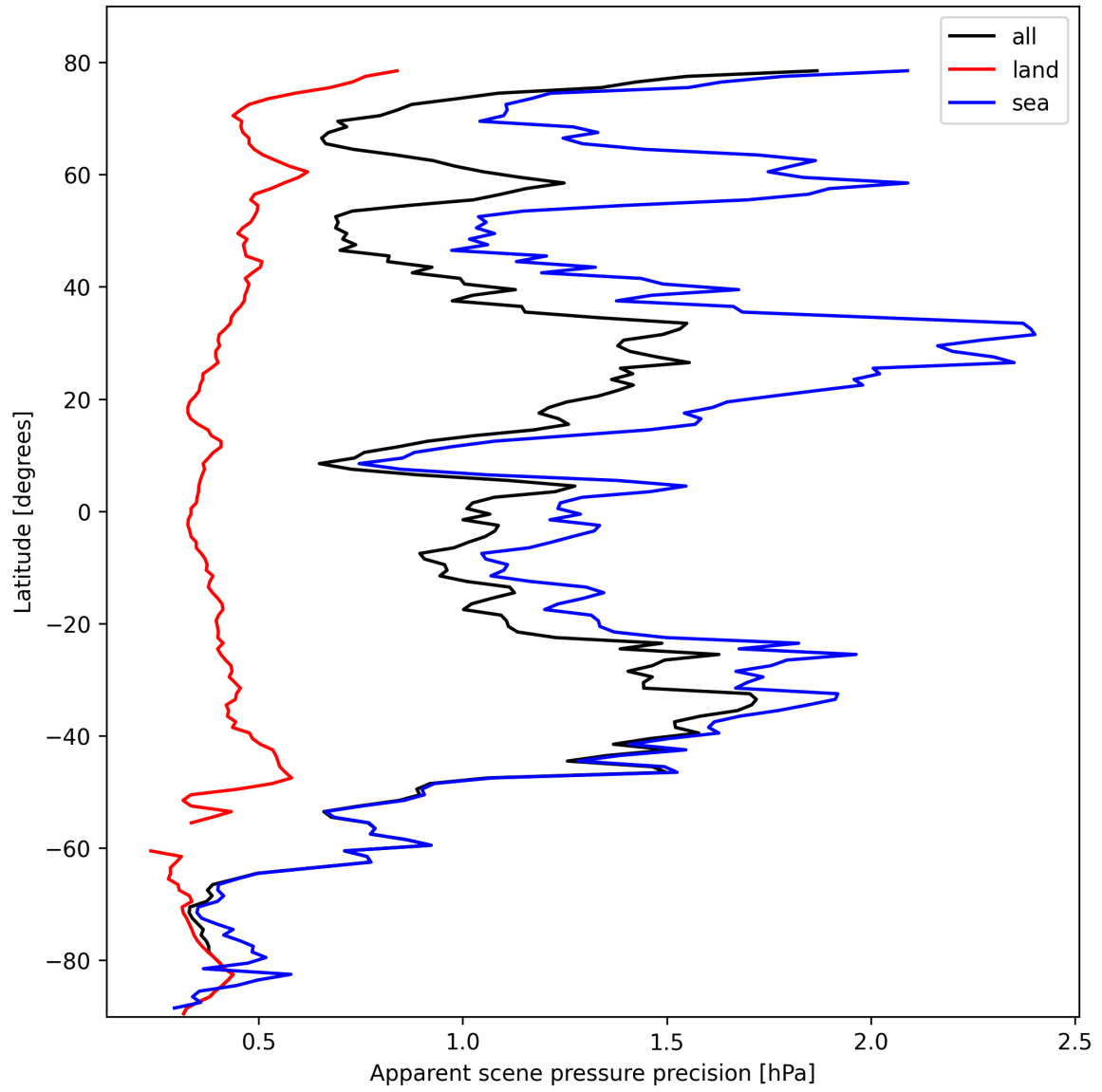
Figure 18: Zonal average of “Apparent scene pressure precision” for 2025-10-18 to 2025-10-19.
