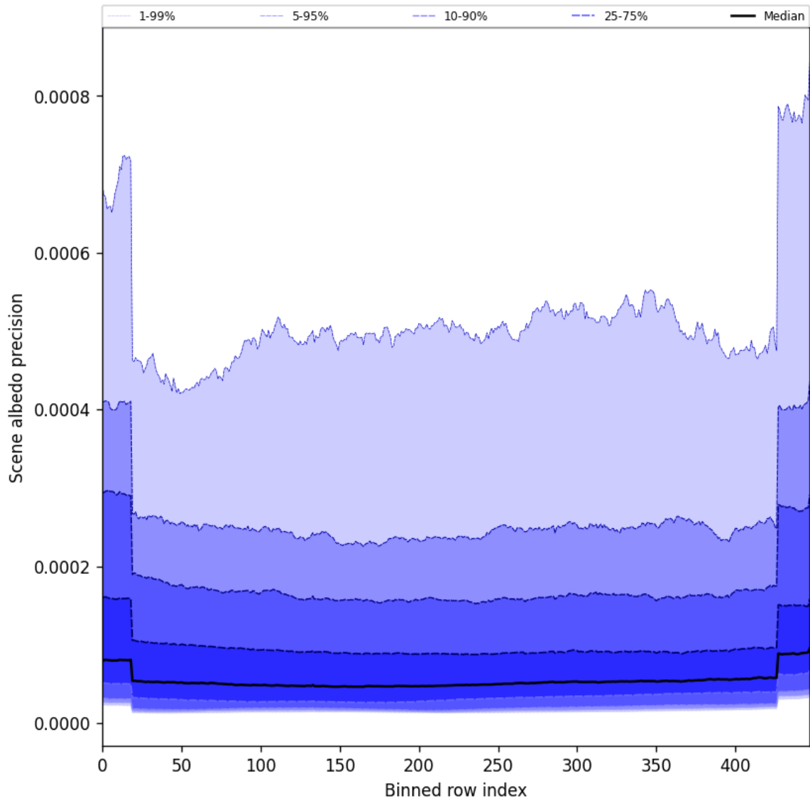
Figure 50: Along track statistics of “Scene albedo precision” for 2025-10-18 to 2025-10-19
