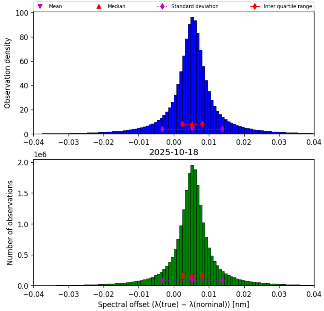
Figure 43: Histogram of “Spectral offset ( \lambda_{\text{true}} - \lambda_{\text{nominal}} )” for 2025-10-18 to 2025-10-19
