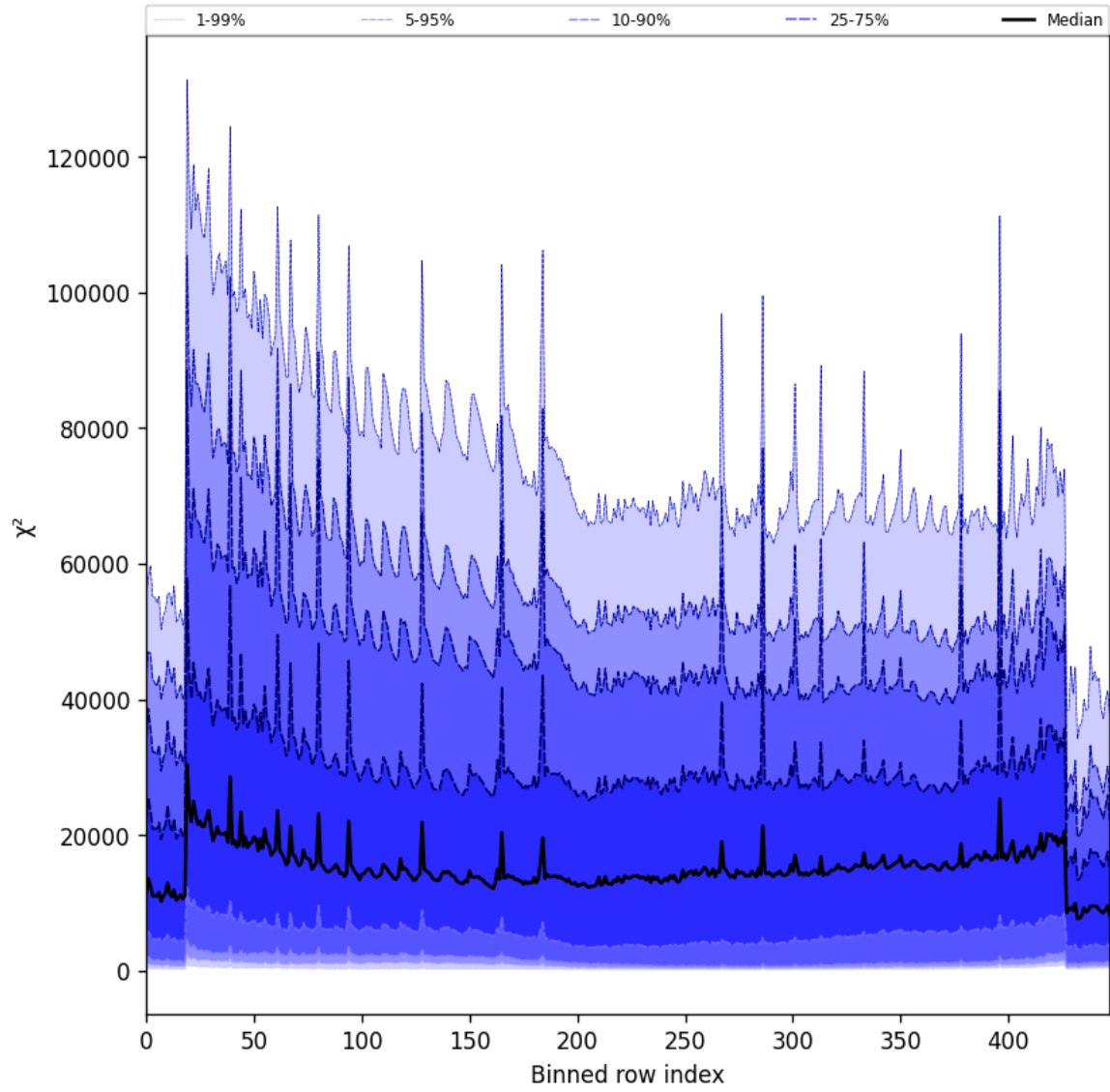
Figure 53: Along track statistics of “ \chi^2 ” for 2025-10-18 to 2025-10-19
