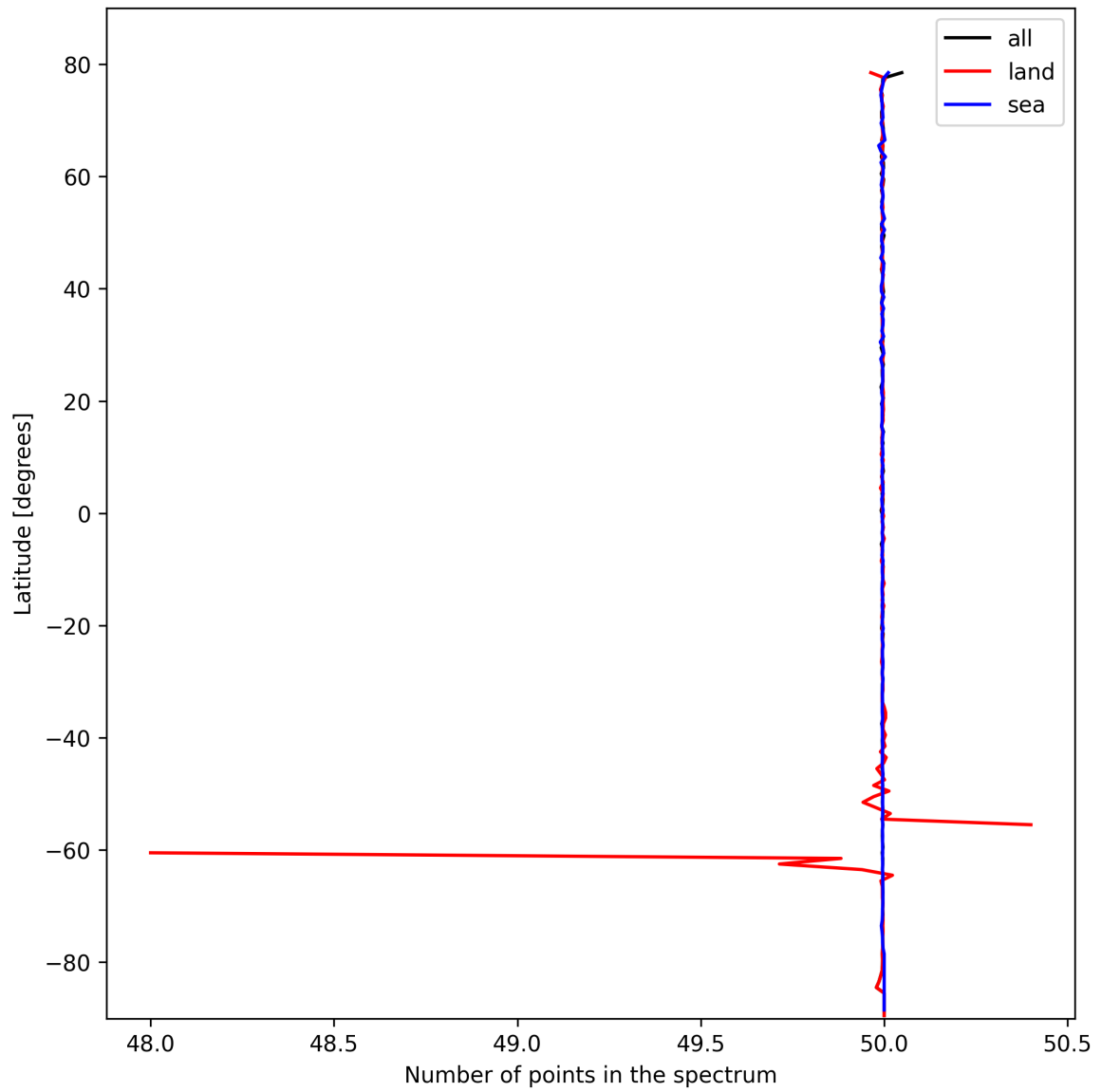
Figure 25: Zonal average of “Number of points in the spectrum” for 2025-10-18 to 2025-10-19.
