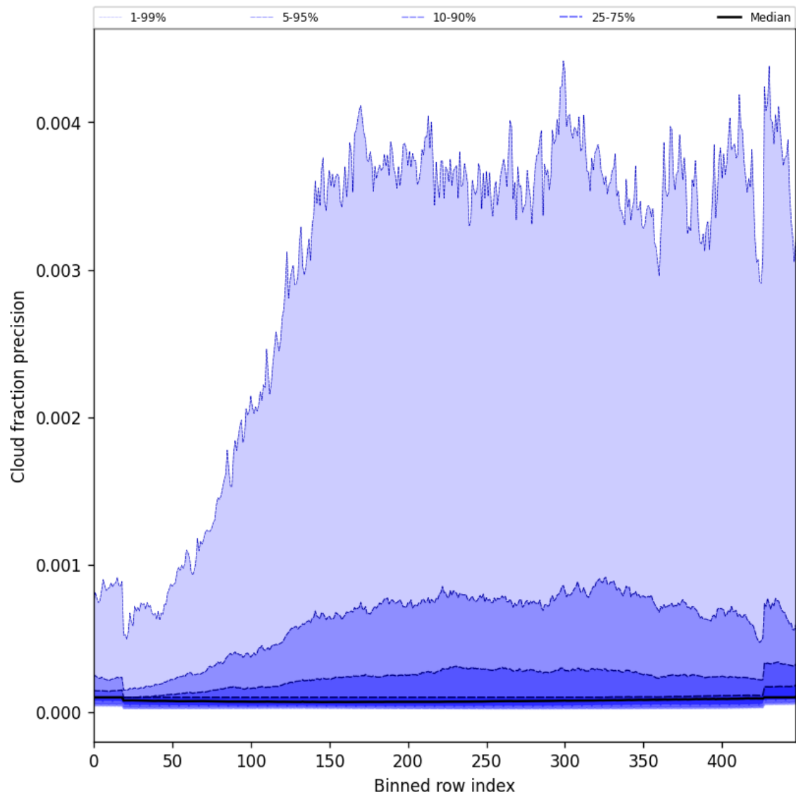
Figure 48: Along track statistics of “Cloud fraction precision” for 2025-10-18 to 2025-10-19
