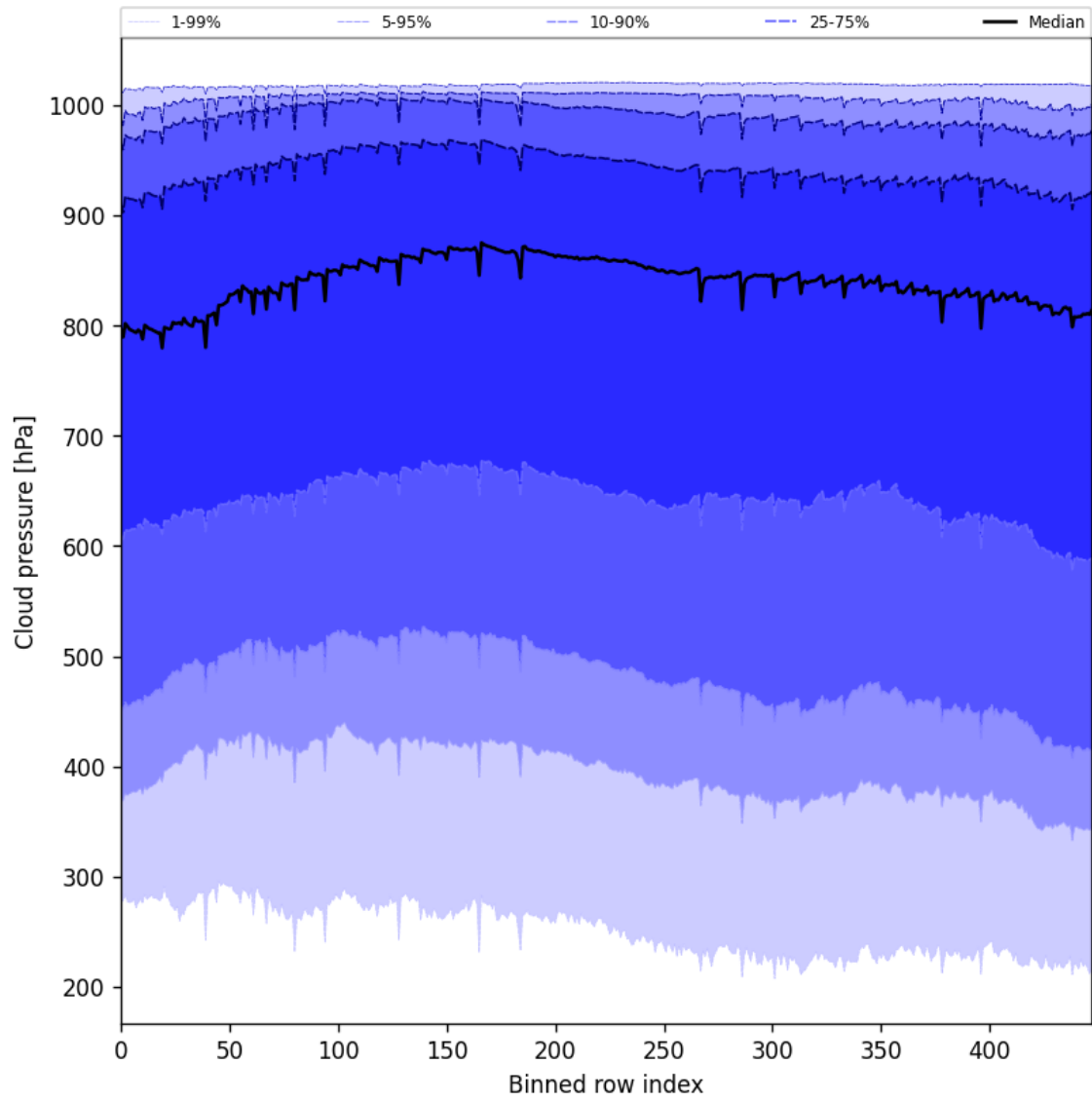
Figure 45: Along track statistics of “Cloud pressure” for 2025-10-18 to 2025-10-19
