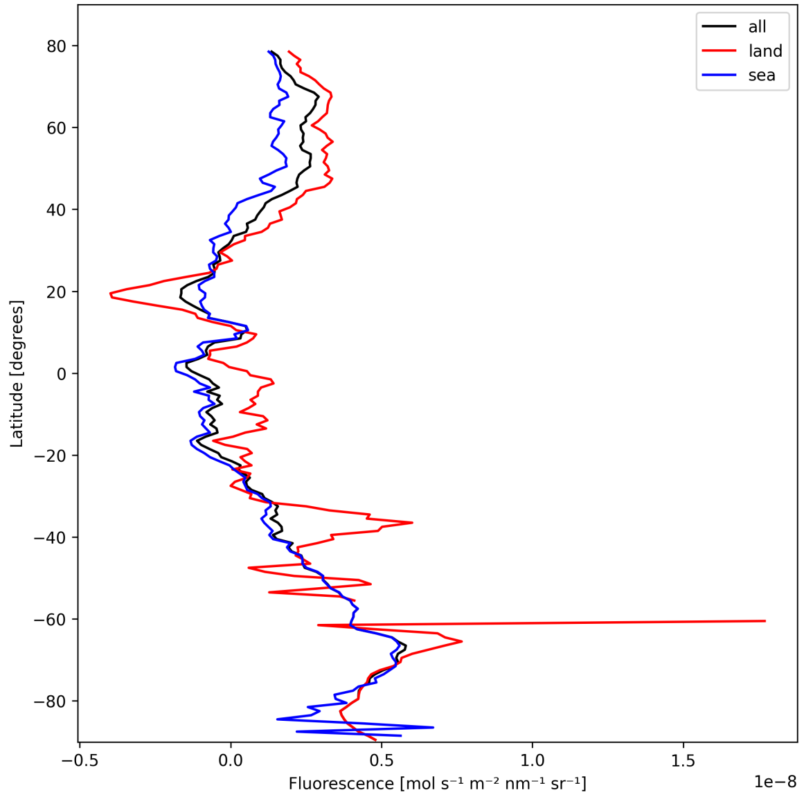
Figure 21: Zonal average of “Fluorescence” for 2025-10-18 to 2025-10-19.
