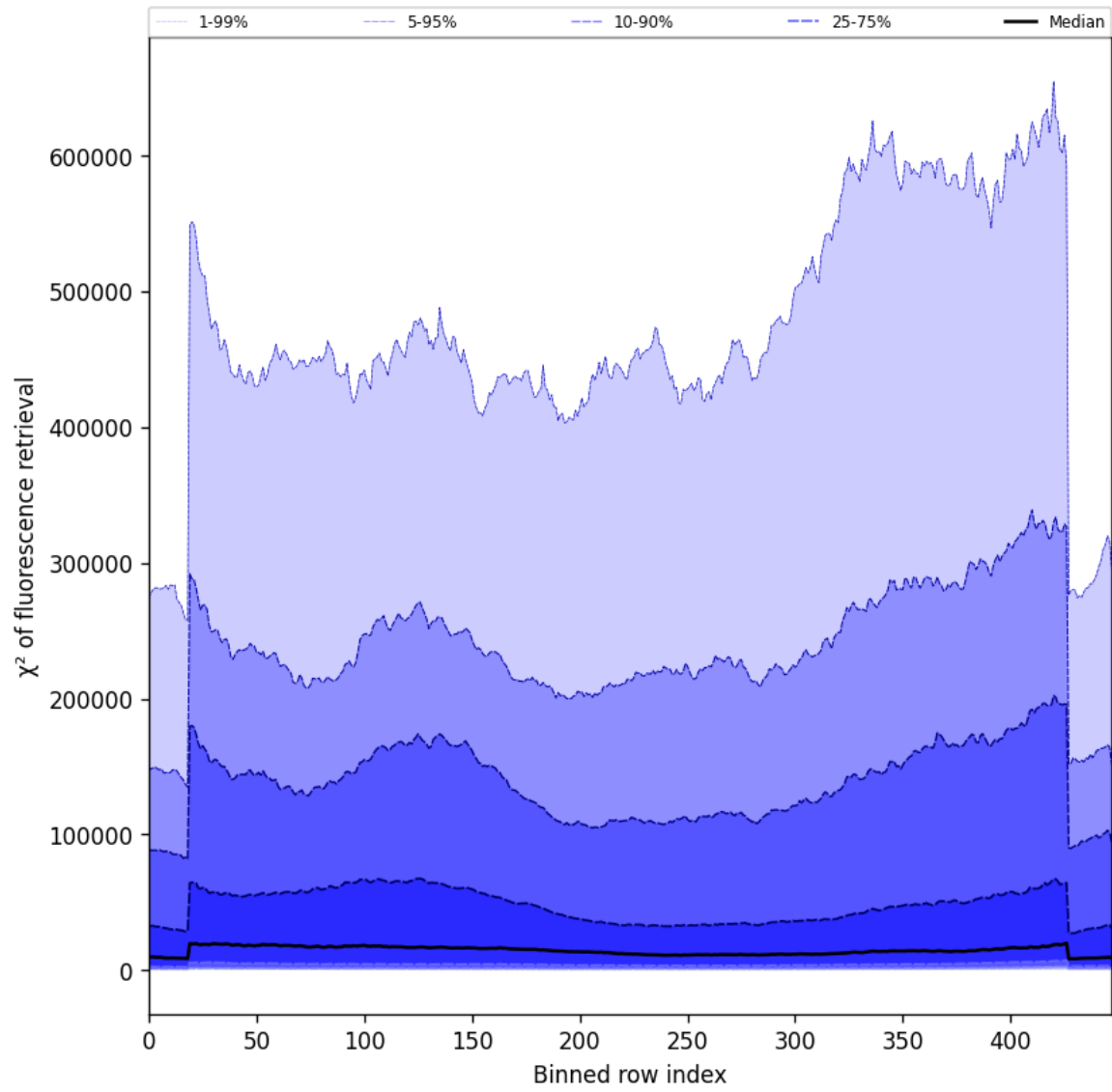
Figure 57: Along track statistics of “ \chi^2 of fluorescence retrieval” for 2025-10-18 to 2025-10-19
