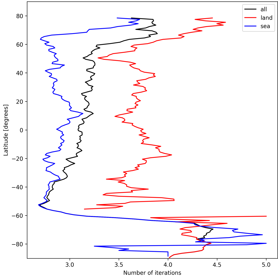
Figure 20: Zonal average of “Number of iterations” for 2025-10-18 to 2025-10-19.
