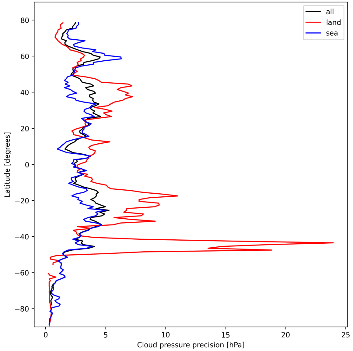
Figure 12: Zonal average of "Cloud pressure precision" for 2025-10-18 to 2025-10-19.
