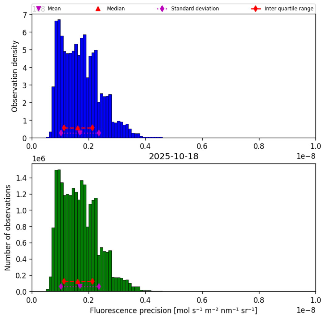
Figure 39: Histogram of “Fluorescence precision” for 2025-10-18 to 2025-10-19
