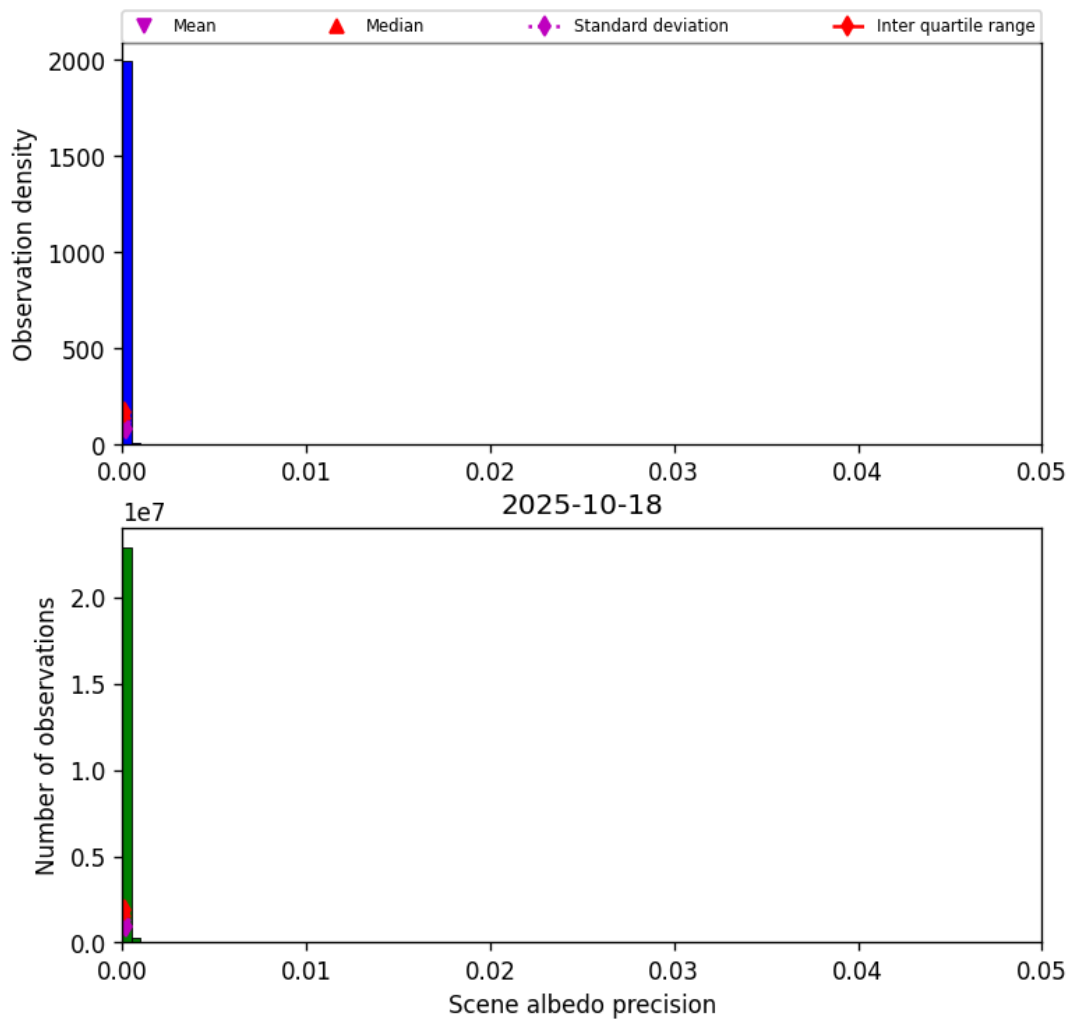
Figure 33: Histogram of “Scene albedo precision” for 2025-10-18 to 2025-10-19
