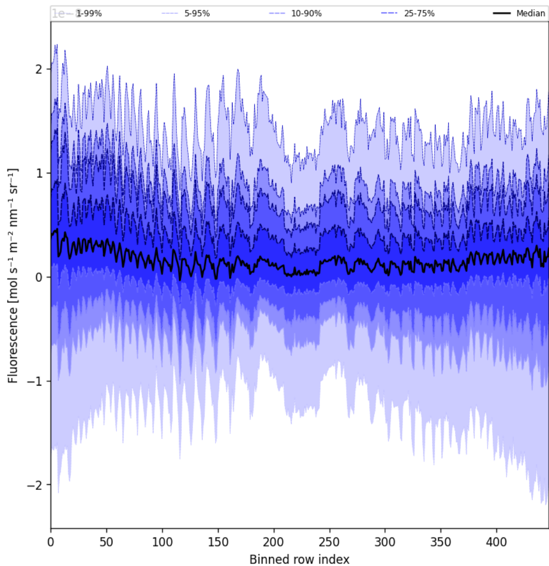
Figure 55: Along track statistics of "Fluorescence" for 2025-10-18 to 2025-10-19
