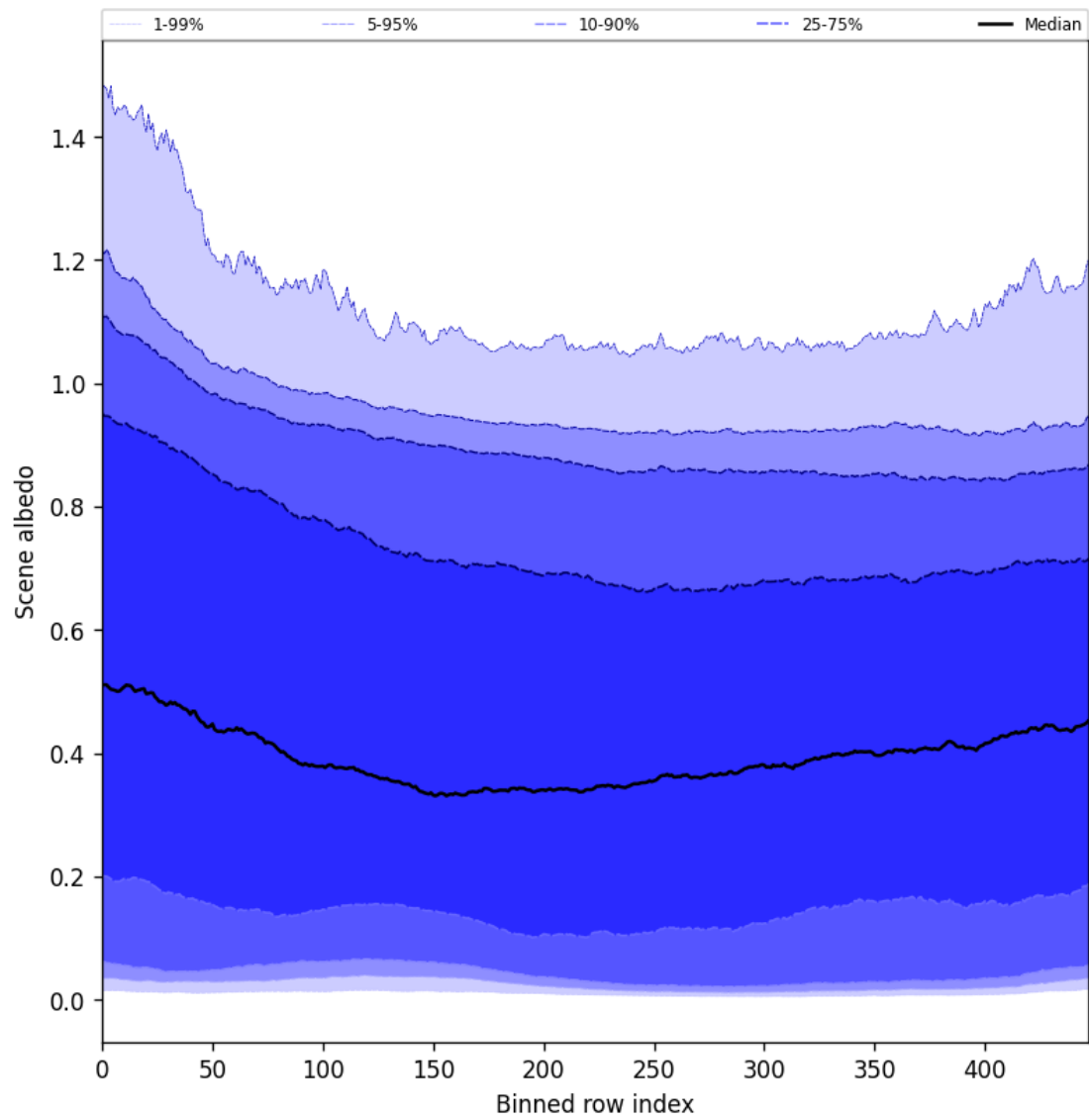
Figure 49: Along track statistics of “Scene albedo” for 2025-10-18 to 2025-10-19
