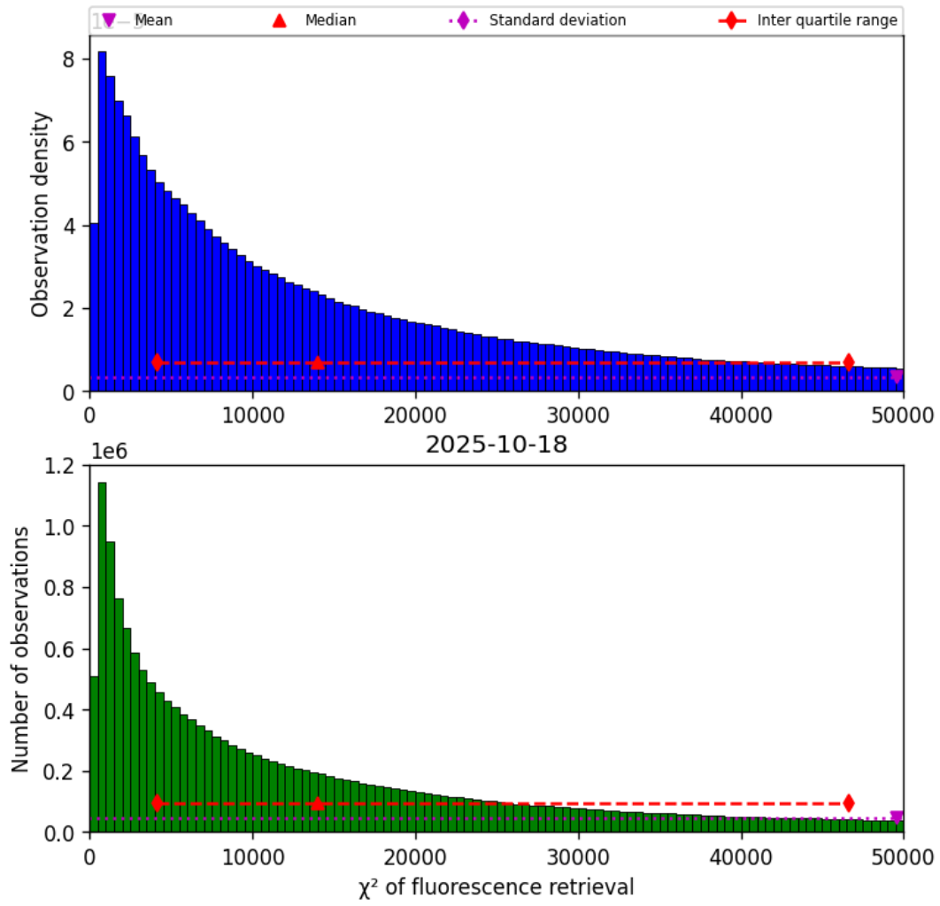
Figure 40: Histogram of “ \chi^2 of fluorescence retrieval” for 2025-10-18 to 2025-10-19
