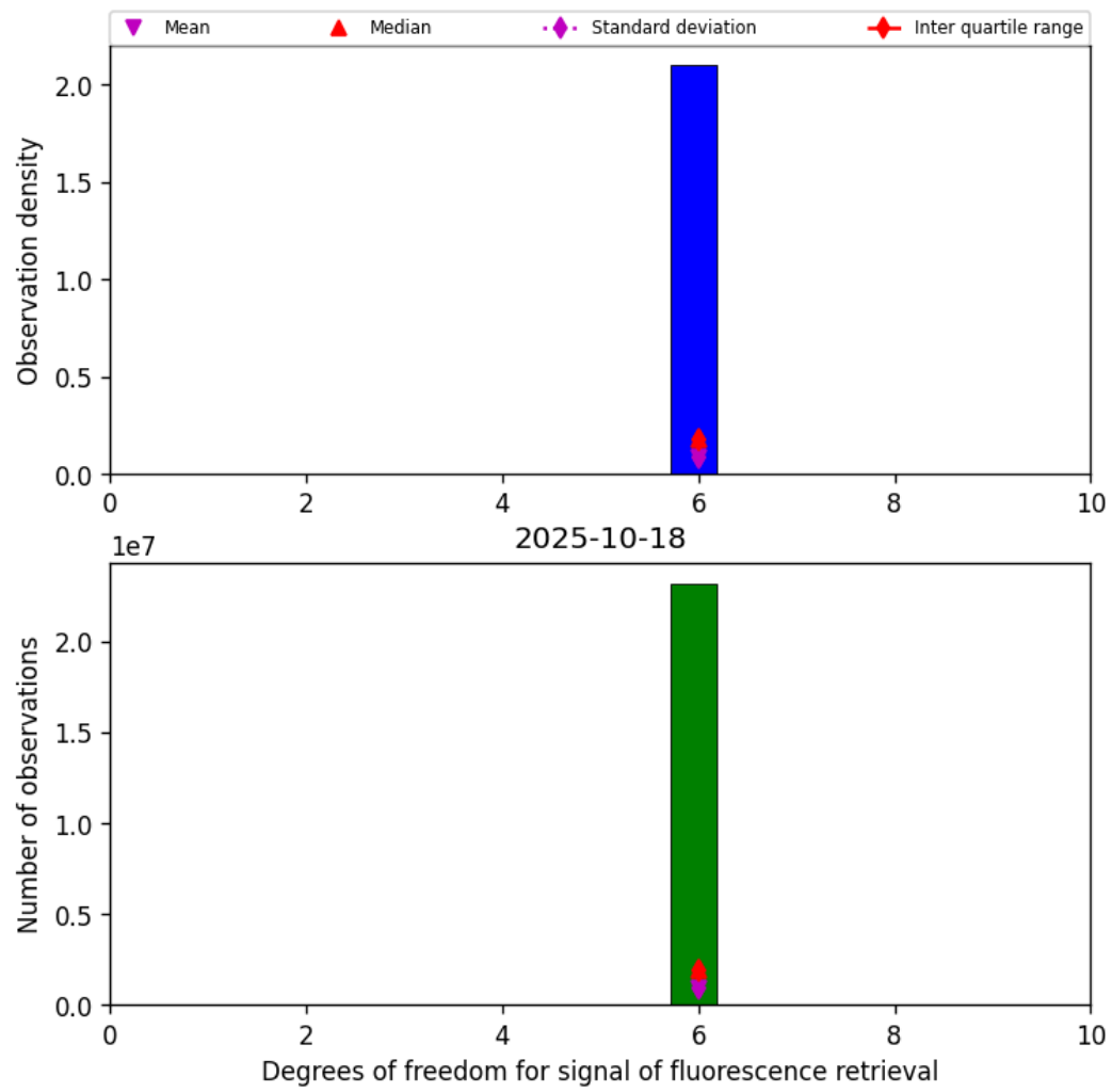
Figure 41: Histogram of “Degrees of freedom for signal of fluorescence retrieval” for 2025-10-18 to 2025-10-19
