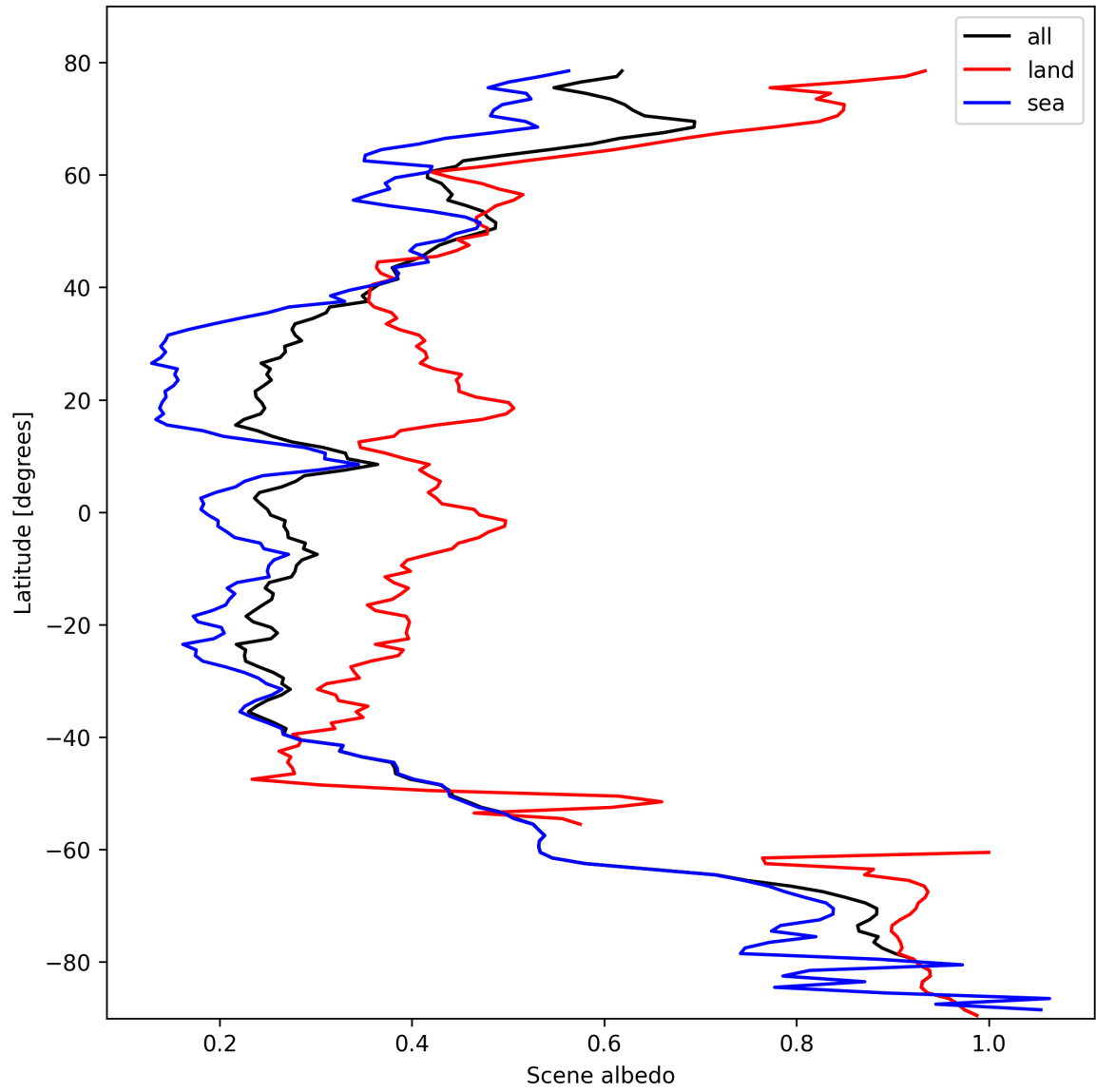
Figure 15: Zonal average of "Scene albedo" for 2025-10-18 to 2025-10-19.
