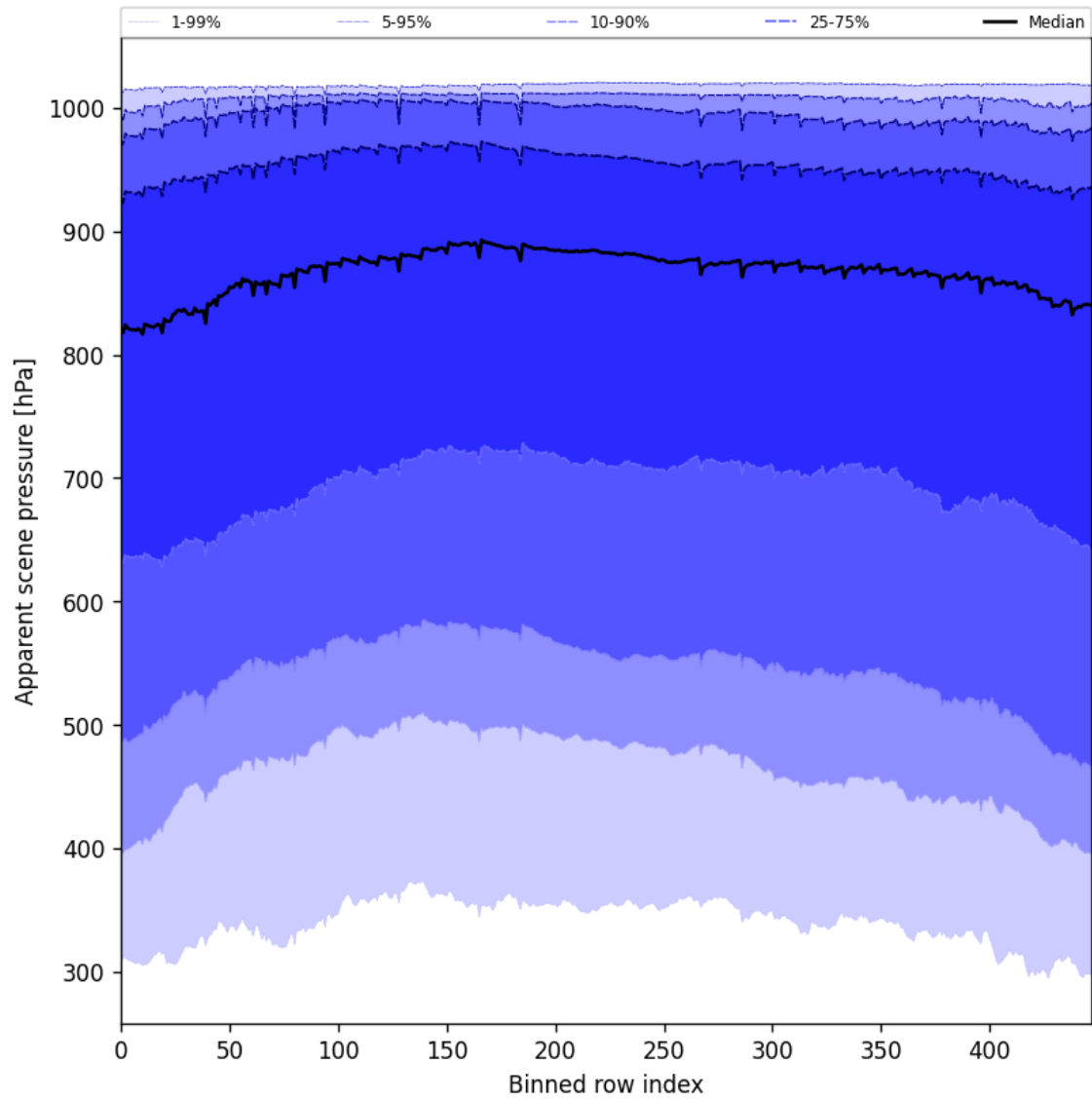
Figure 51: Along track statistics of “Apparent scene pressure” for 2025-10-18 to 2025-10-19
