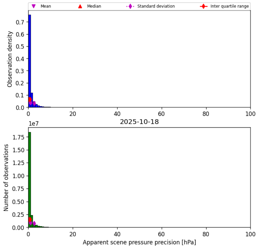
Figure 35: Histogram of “Apparent scene pressure precision” for 2025-10-18 to 2025-10-19
