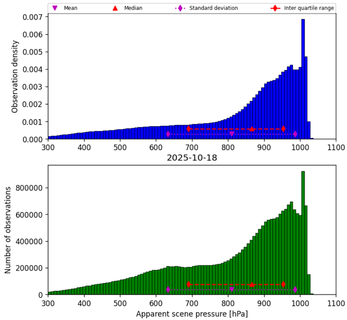
Figure 34: Histogram of “Apparent scene pressure” for 2025-10-18 to 2025-10-19
