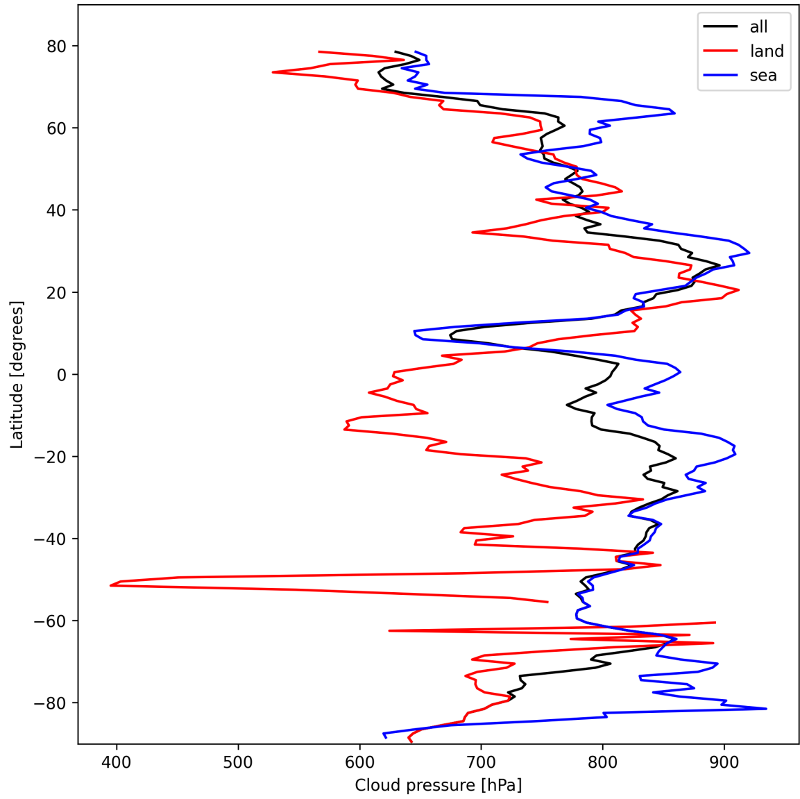
Figure 11: Zonal average of “Cloud pressure” for 2025-10-18 to 2025-10-19.
