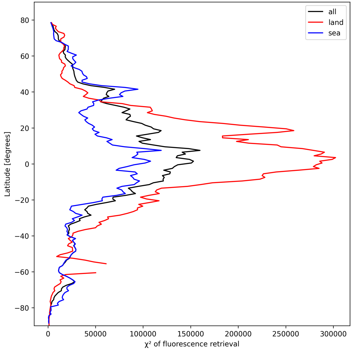
Figure 23: Zonal average of “ \chi^2 of fluorescence retrieval” for 2025-10-18 to 2025-10-19.
