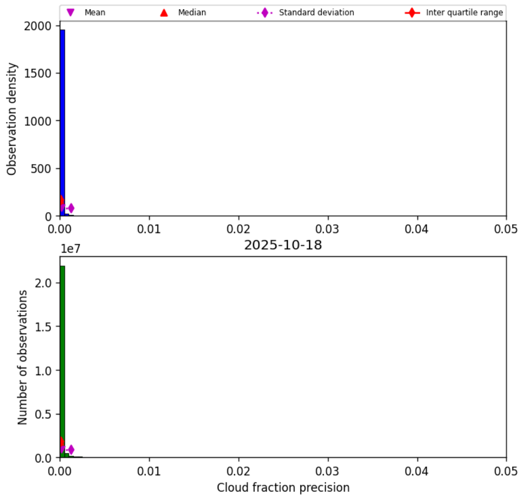
Figure 31: Histogram of “Cloud fraction precision” for 2025-10-18 to 2025-10-19
