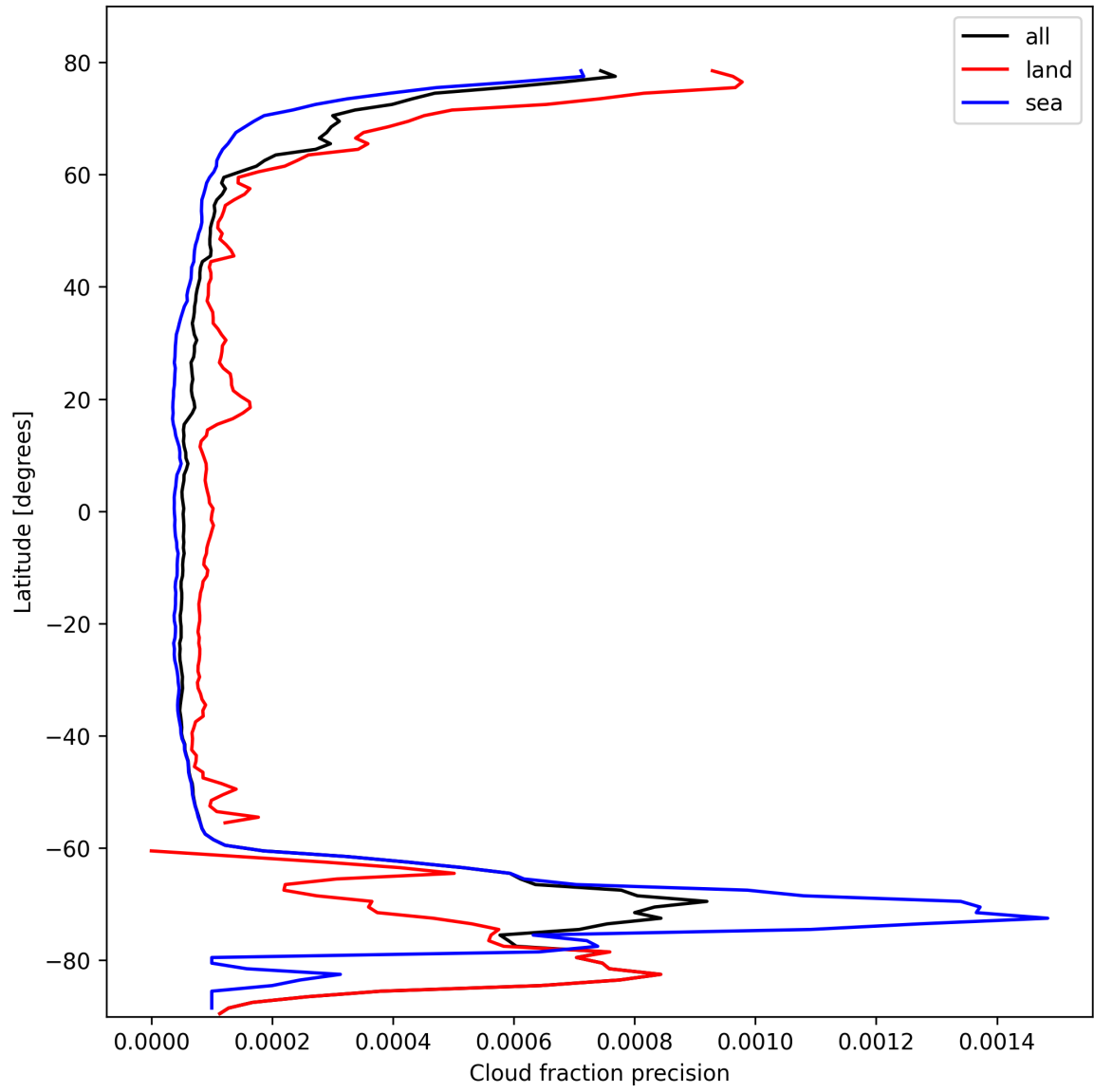
Figure 14: Zonal average of “Cloud fraction precision” for 2025-10-18 to 2025-10-19.
