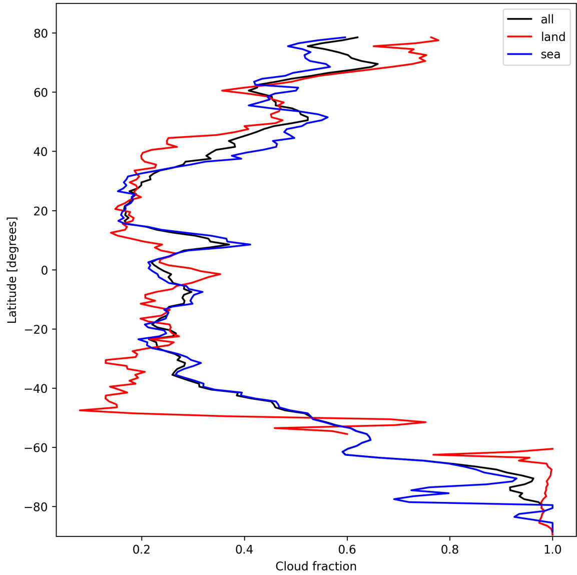
Figure 13: Zonal average of “Cloud fraction” for 2025-10-18 to 2025-10-19.
