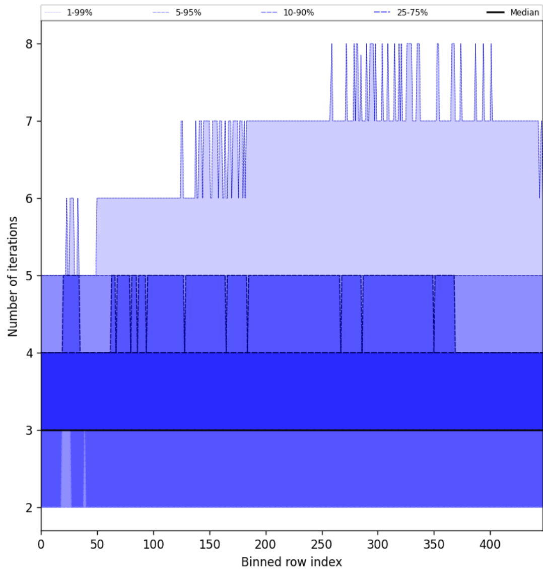
Figure 54: Along track statistics of “Number of iterations” for 2025-10-18 to 2025-10-19
