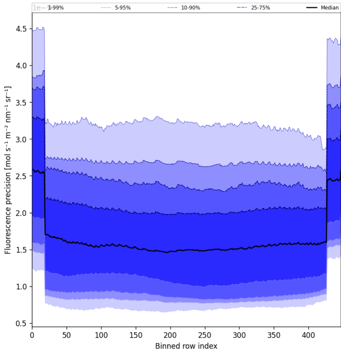
Figure 56: Along track statistics of “Fluorescence precision” for 2025-10-18 to 2025-10-19
