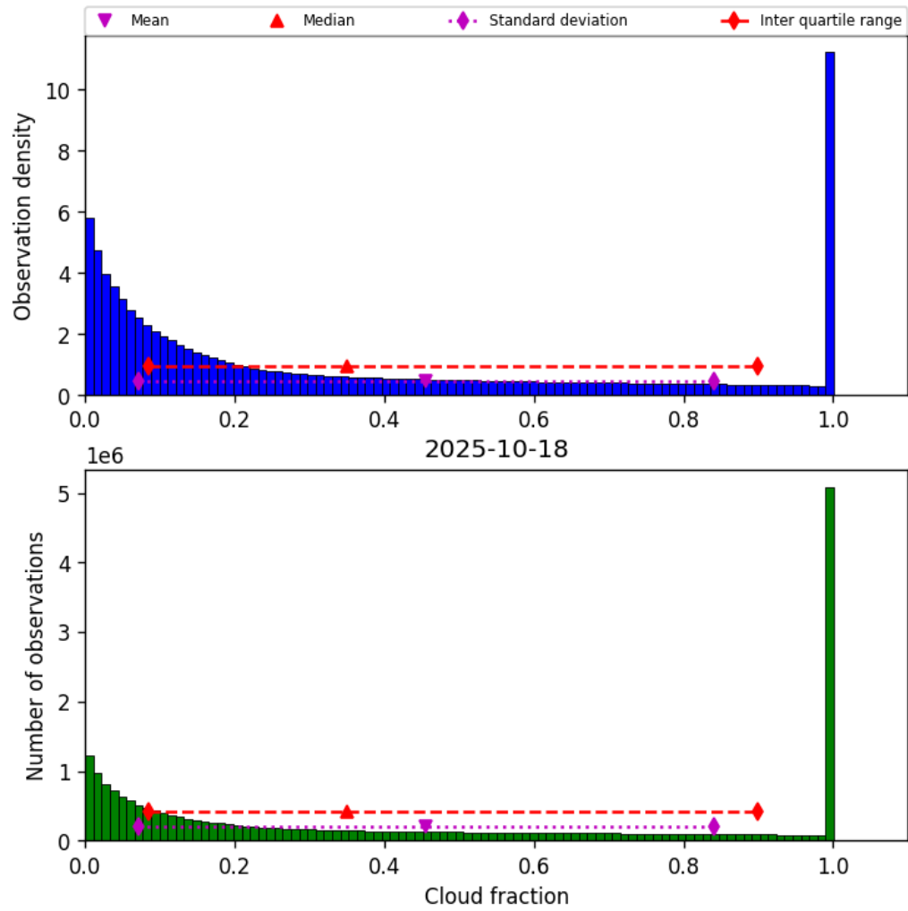
Figure 30: Histogram of “Cloud fraction” for 2025-10-18 to 2025-10-19
