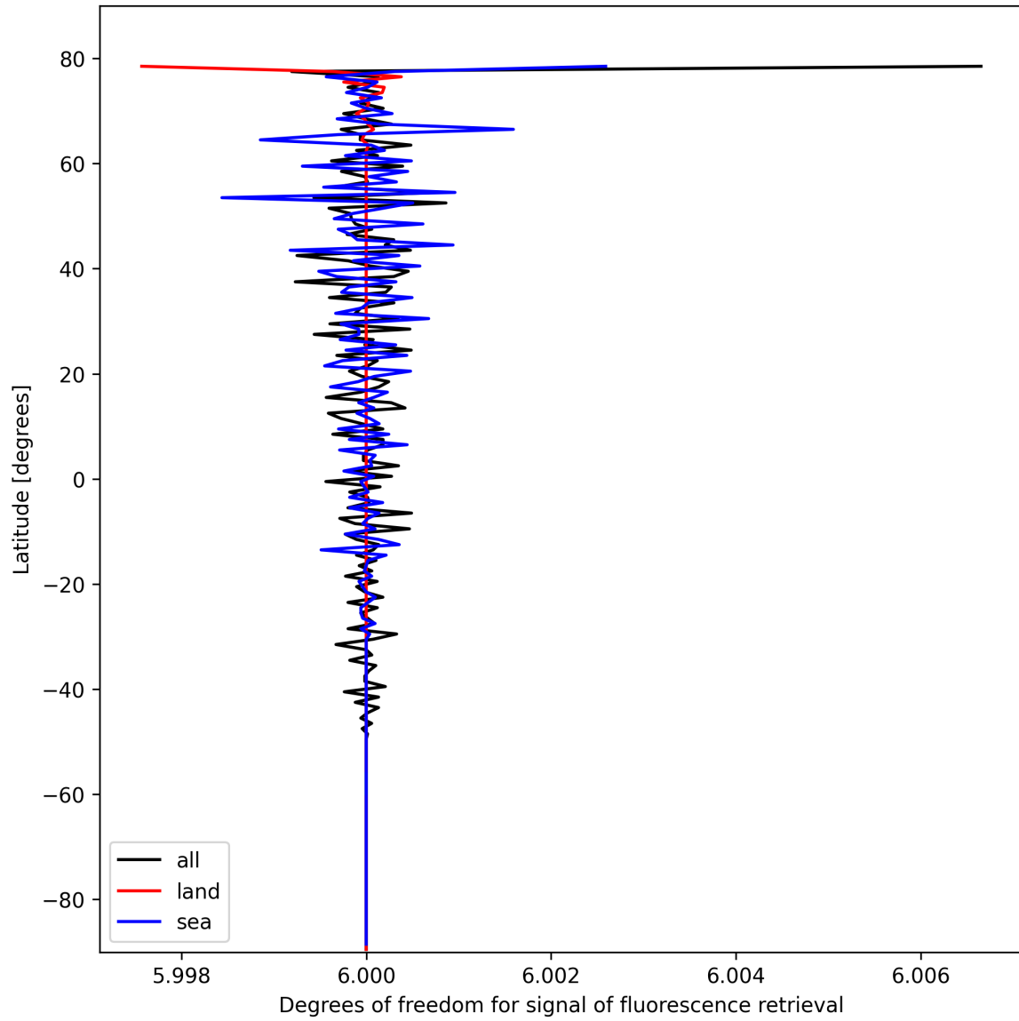
Figure 24: Zonal average of “Degrees of freedom for signal of fluorescence retrieval” for 2025-10-18 to 2025-10-19.
