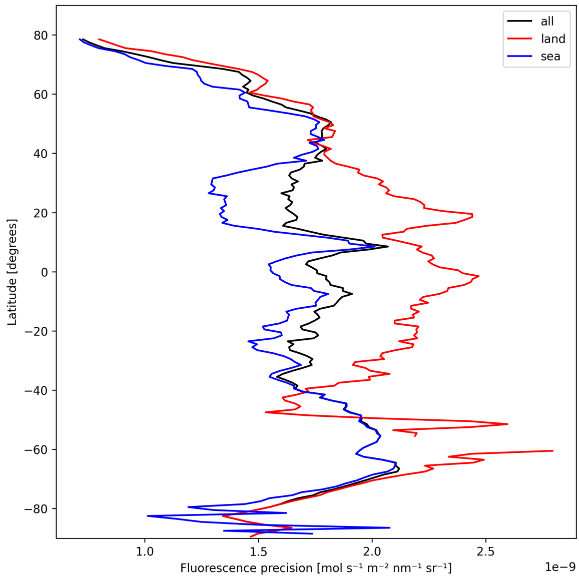
Figure 22: Zonal average of “Fluorescence precision” for 2025-10-18 to 2025-10-19.
