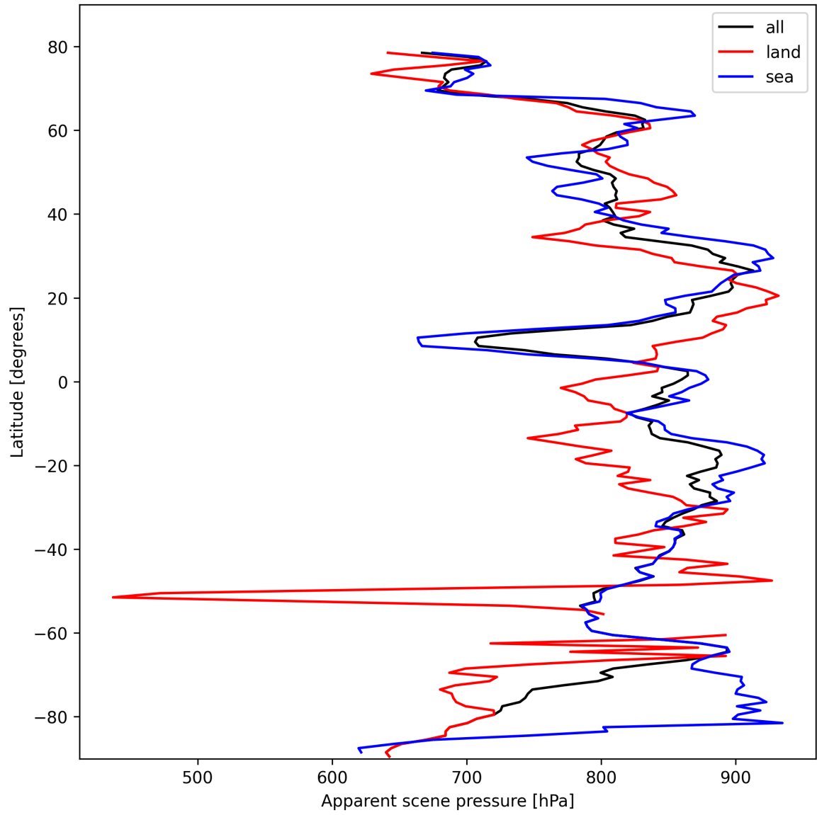
Figure 17: Zonal average of “Apparent scene pressure” for 2025-10-18 to 2025-10-19.
