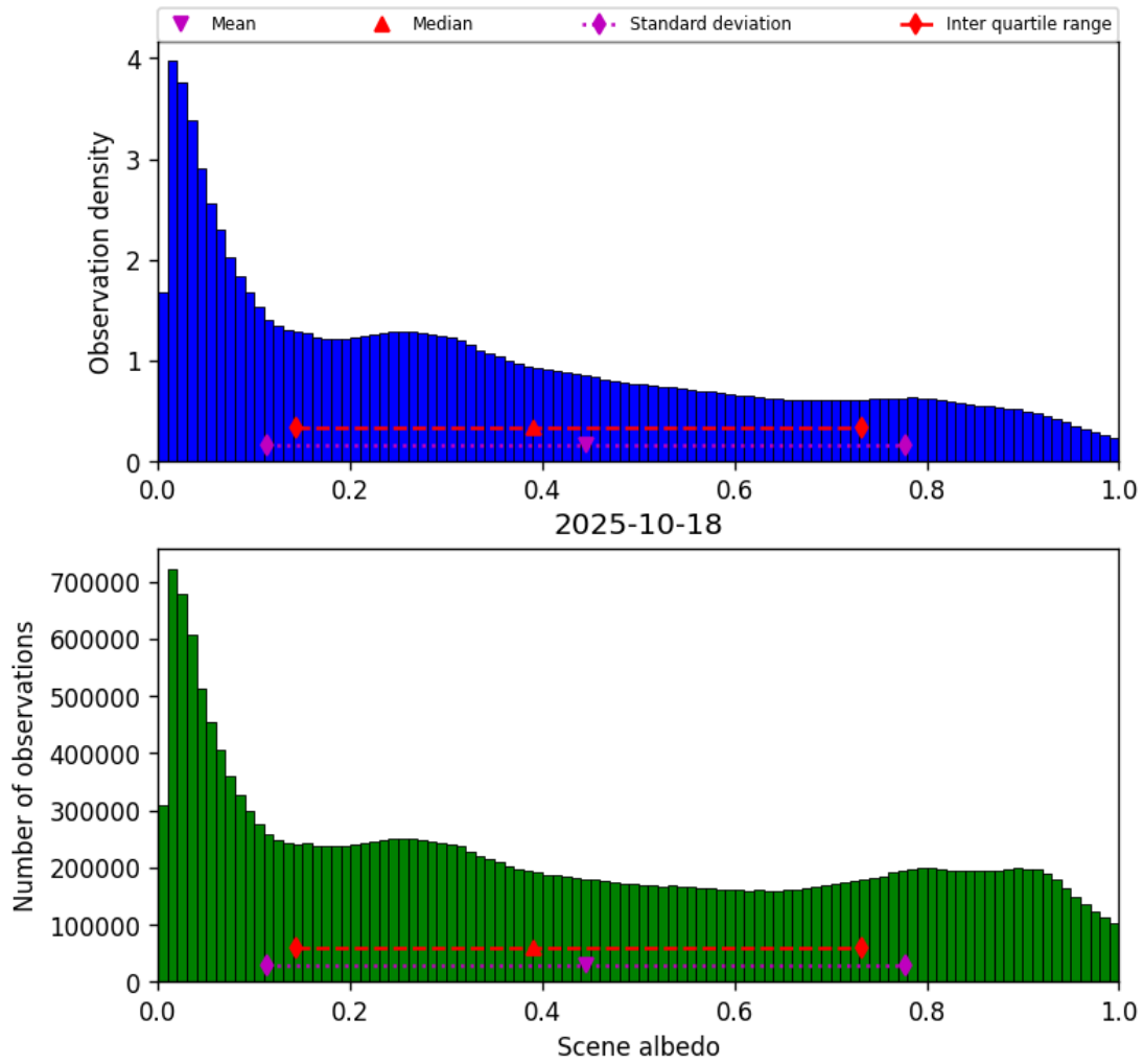
Figure 32: Histogram of “Scene albedo” for 2025-10-18 to 2025-10-19
