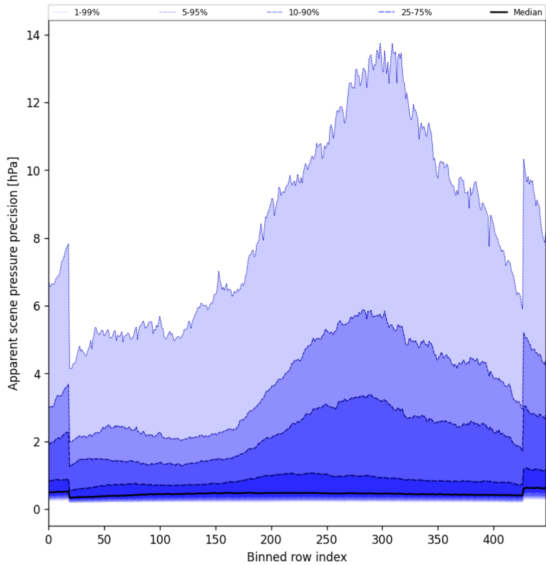
Figure 52: Along track statistics of “Apparent scene pressure precision” for 2025-10-18 to 2025-10-19
