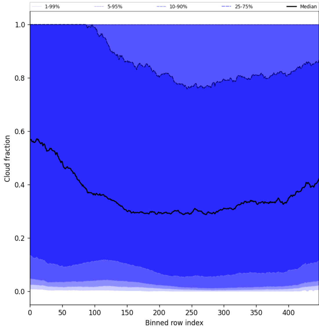
Figure 47: Along track statistics of “Cloud fraction” for 2025-10-18 to 2025-10-19
