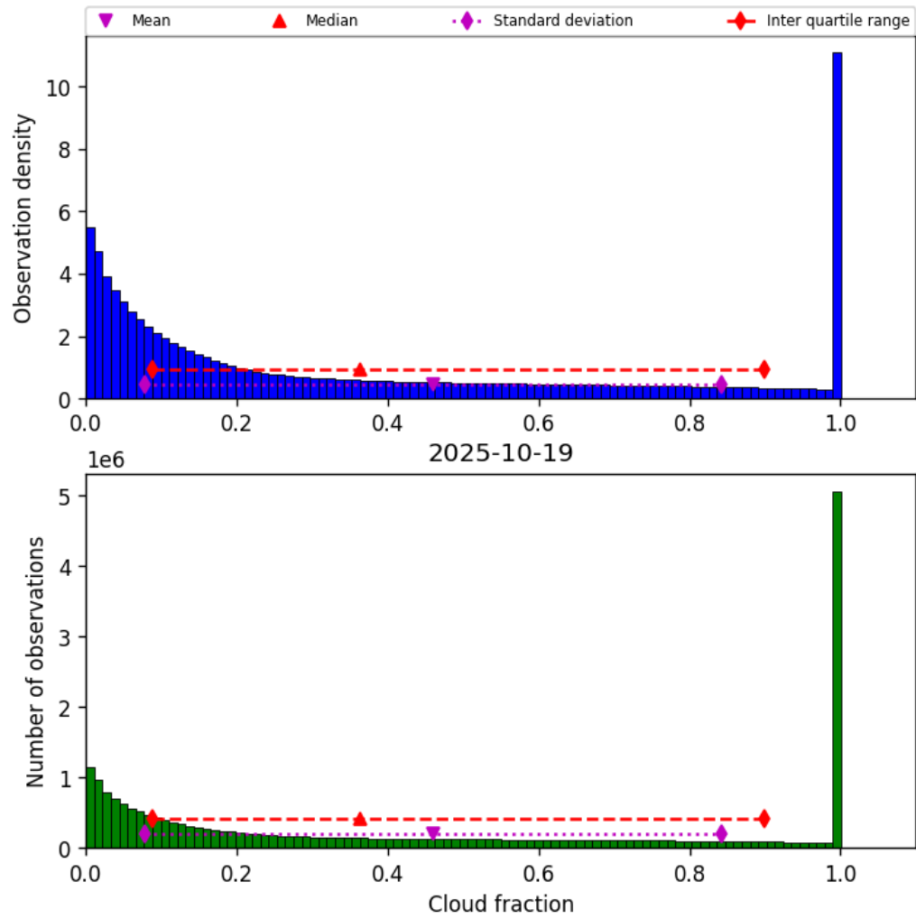
Figure 30: Histogram of “Cloud fraction” for 2025-10-19 to 2025-10-20
