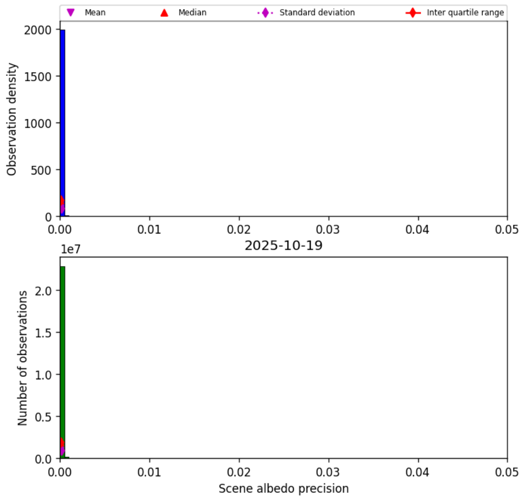
Figure 33: Histogram of “Scene albedo precision” for 2025-10-19 to 2025-10-20
