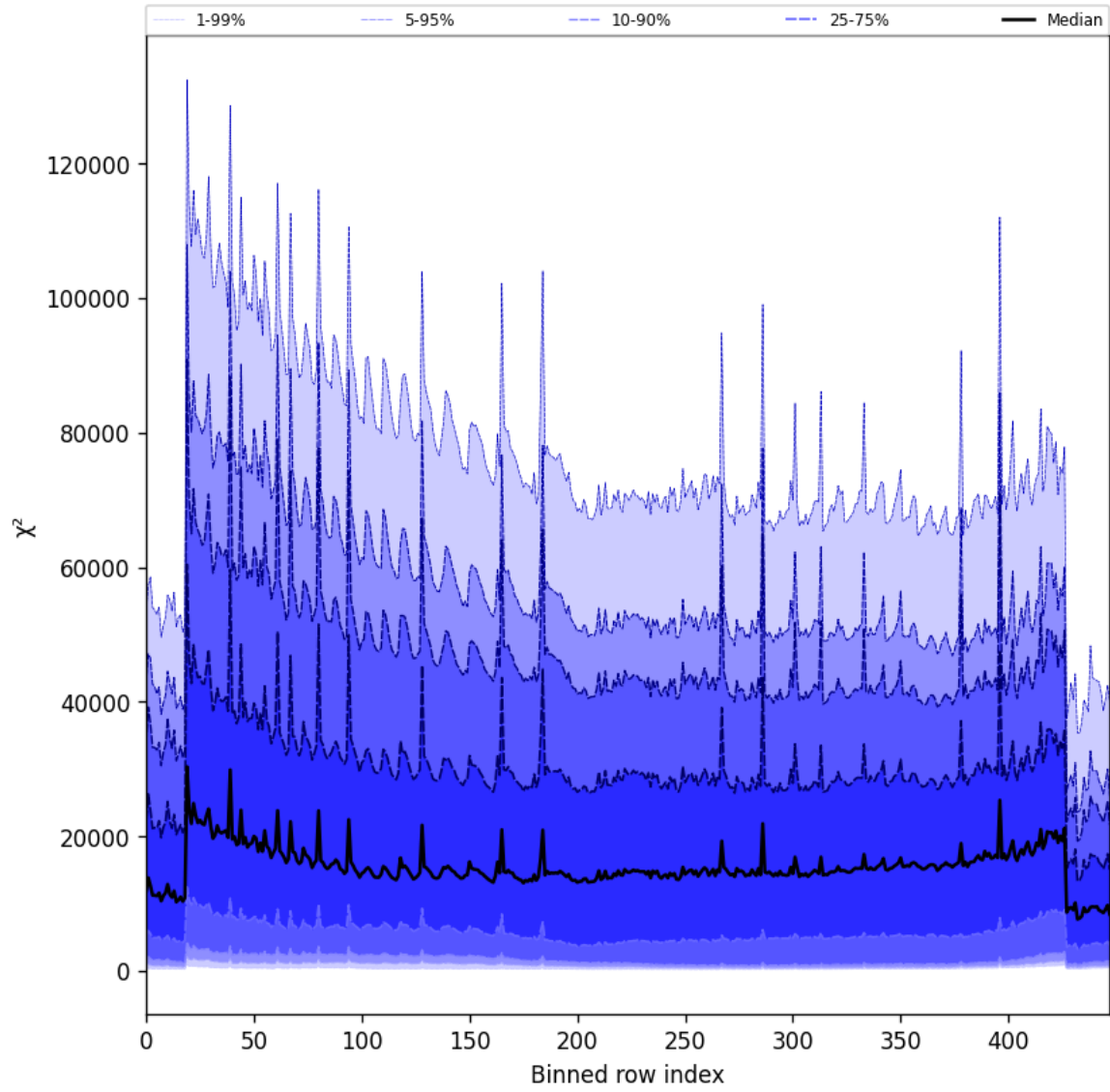
Figure 53: Along track statistics of “ \chi^2 ” for 2025-10-19 to 2025-10-20
