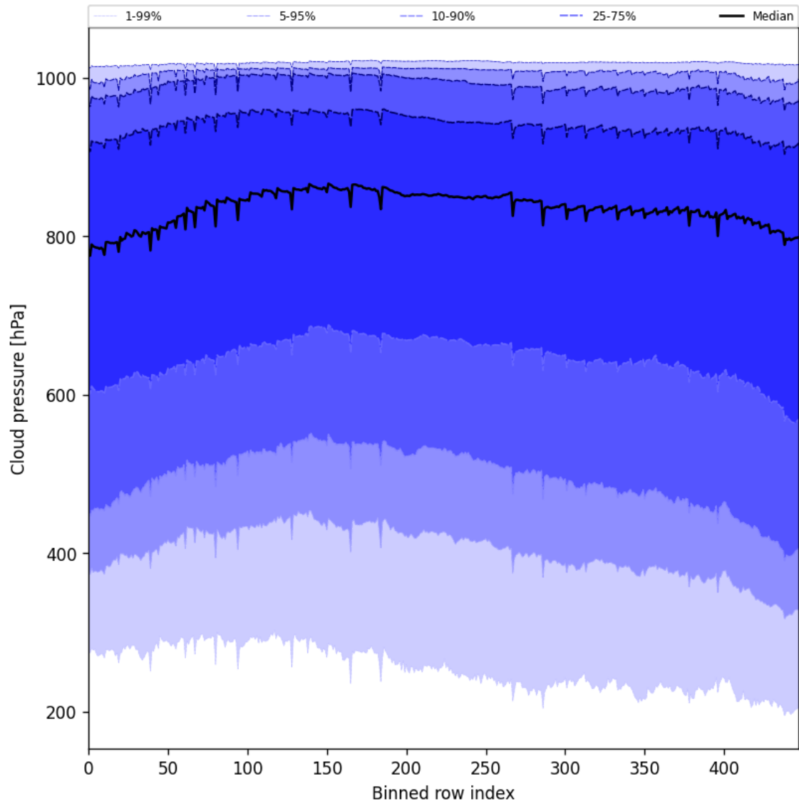
Figure 45: Along track statistics of “Cloud pressure” for 2025-10-19 to 2025-10-20
