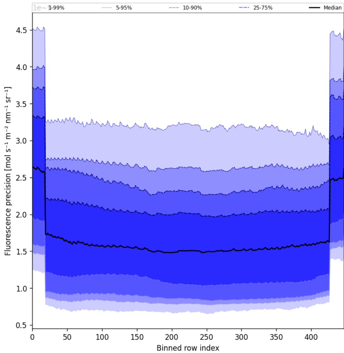
Figure 56: Along track statistics of “Fluorescence precision” for 2025-10-19 to 2025-10-20
