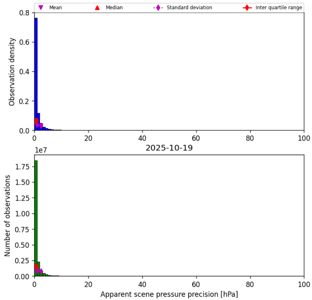
Figure 35: Histogram of “Apparent scene pressure precision” for 2025-10-19 to 2025-10-20
