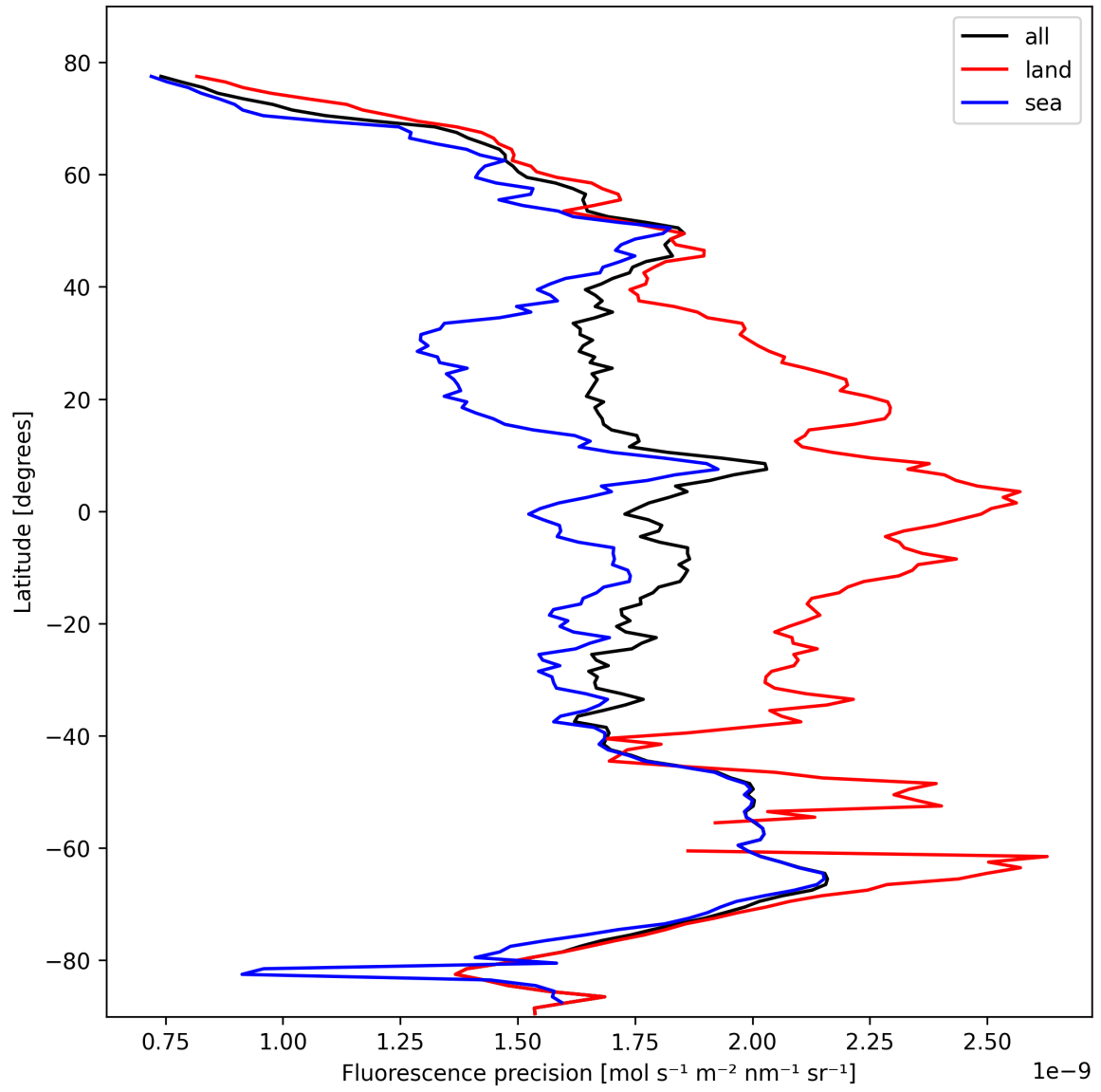
Figure 22: Zonal average of “Fluorescence precision” for 2025-10-19 to 2025-10-20.
