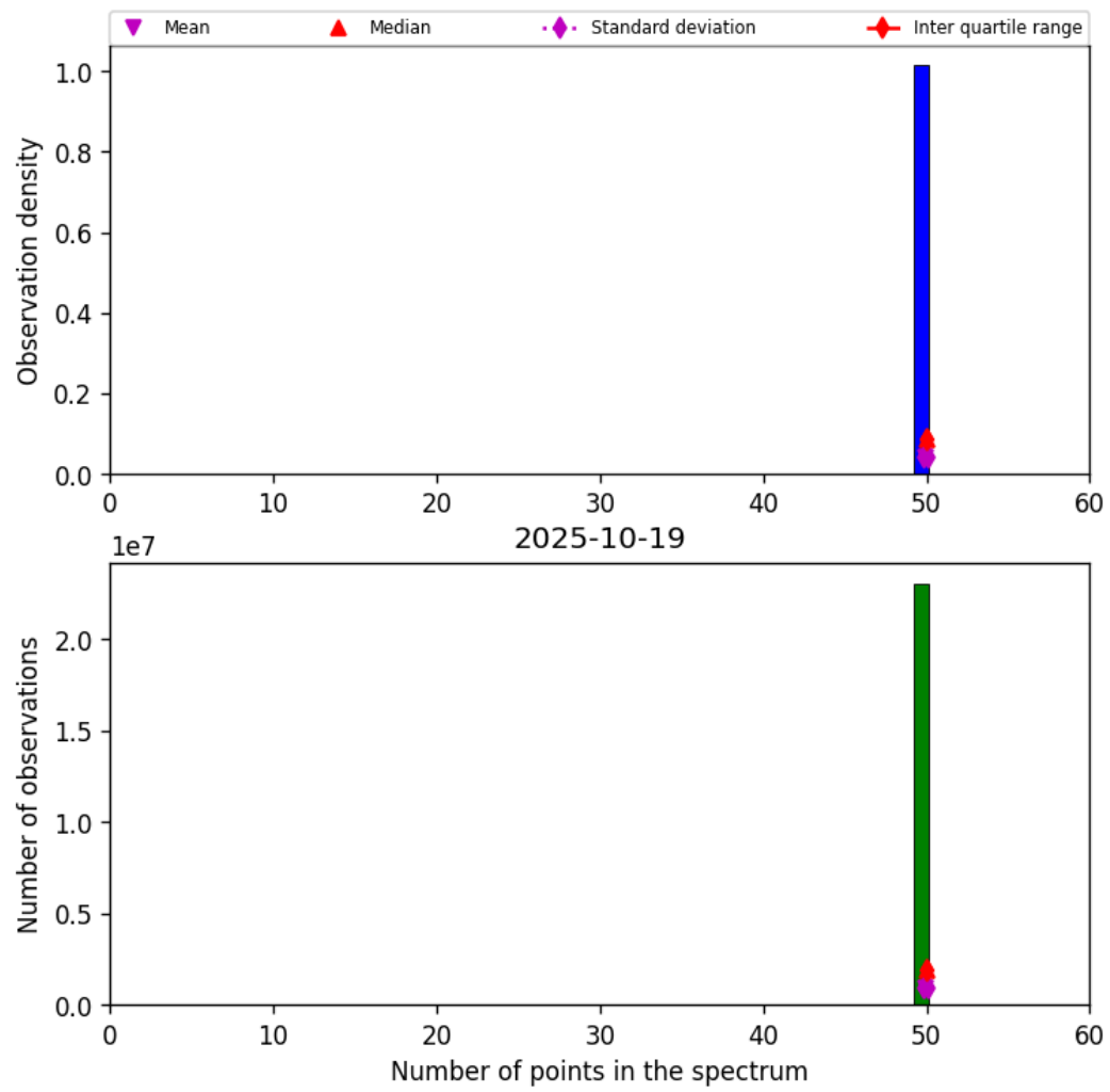
Figure 42: Histogram of “Number of points in the spectrum” for 2025-10-19 to 2025-10-20
