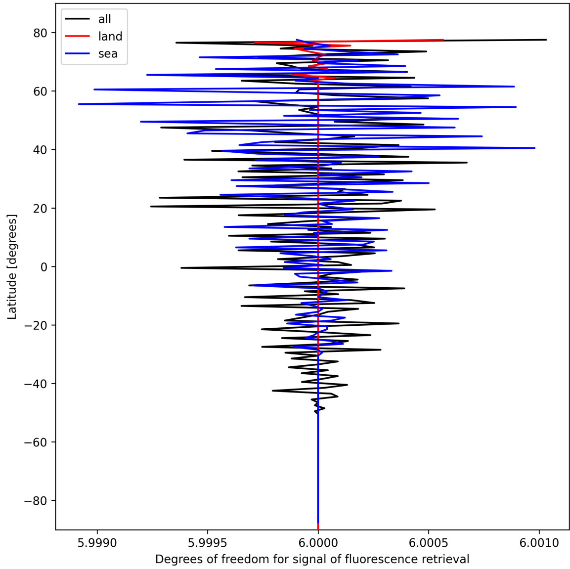
Figure 24: Zonal average of “Degrees of freedom for signal of fluorescence retrieval” for 2025-10-19 to 2025-10-20.
