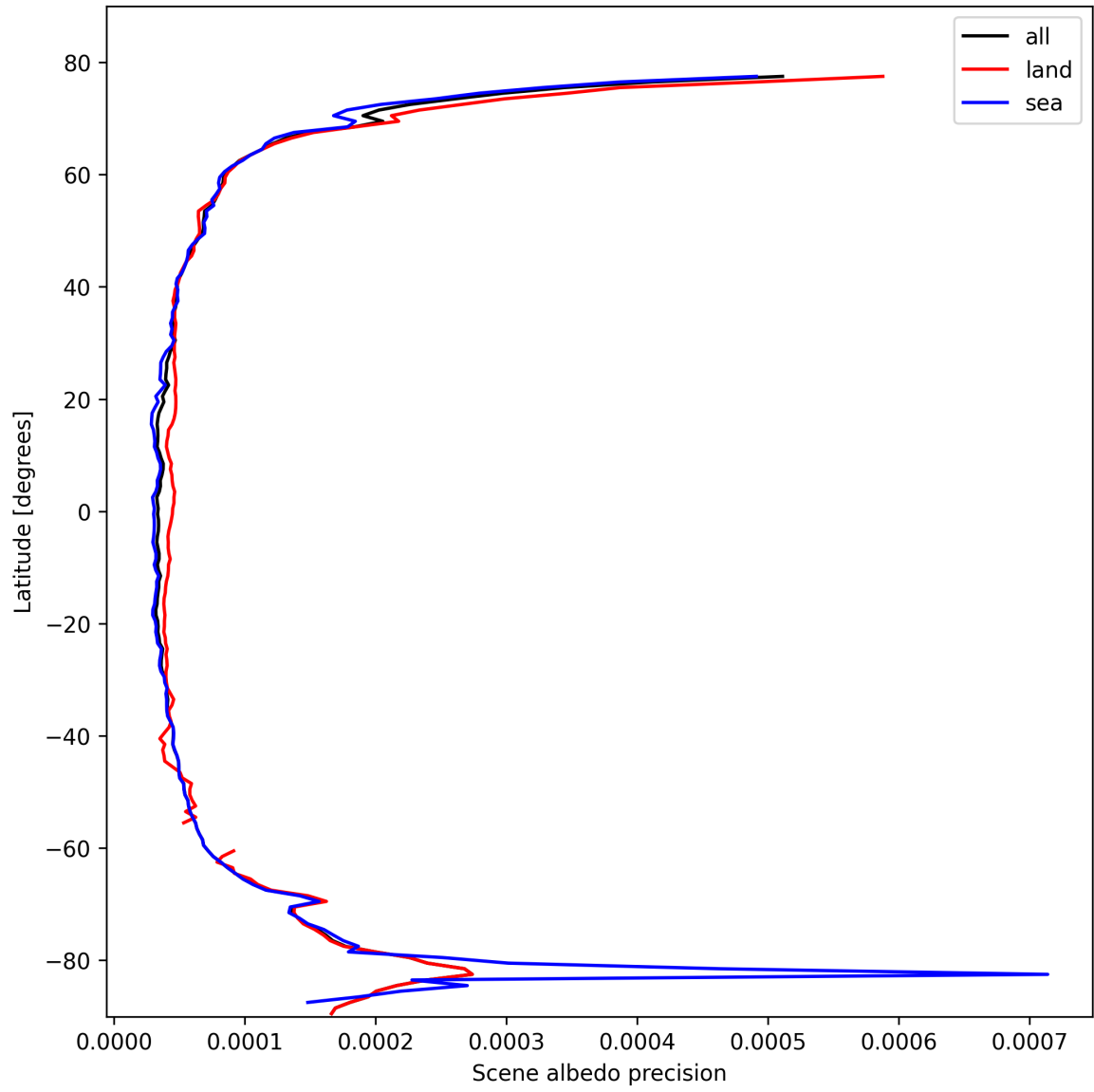
Figure 16: Zonal average of “Scene albedo precision” for 2025-10-19 to 2025-10-20.
