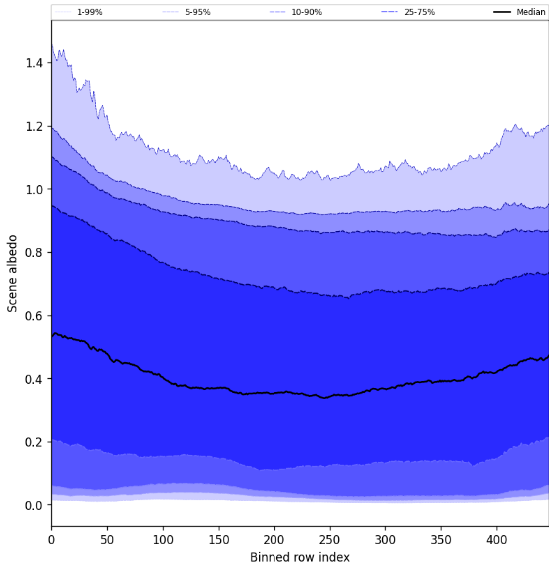
Figure 49: Along track statistics of “Scene albedo” for 2025-10-19 to 2025-10-20
