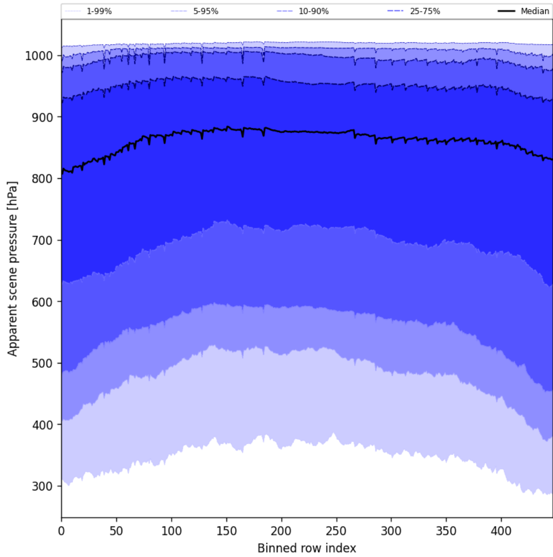
Figure 51: Along track statistics of “Apparent scene pressure” for 2025-10-19 to 2025-10-20
