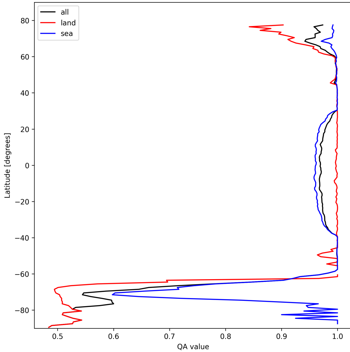
Figure 10: Zonal average of “QA value” for 2025-10-19 to 2025-10-20.
