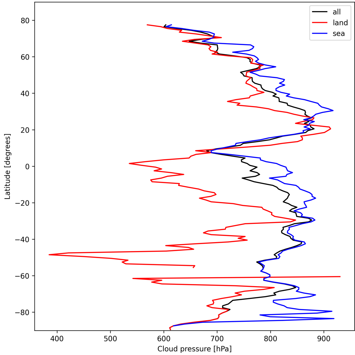
Figure 11: Zonal average of “Cloud pressure” for 2025-10-19 to 2025-10-20.
