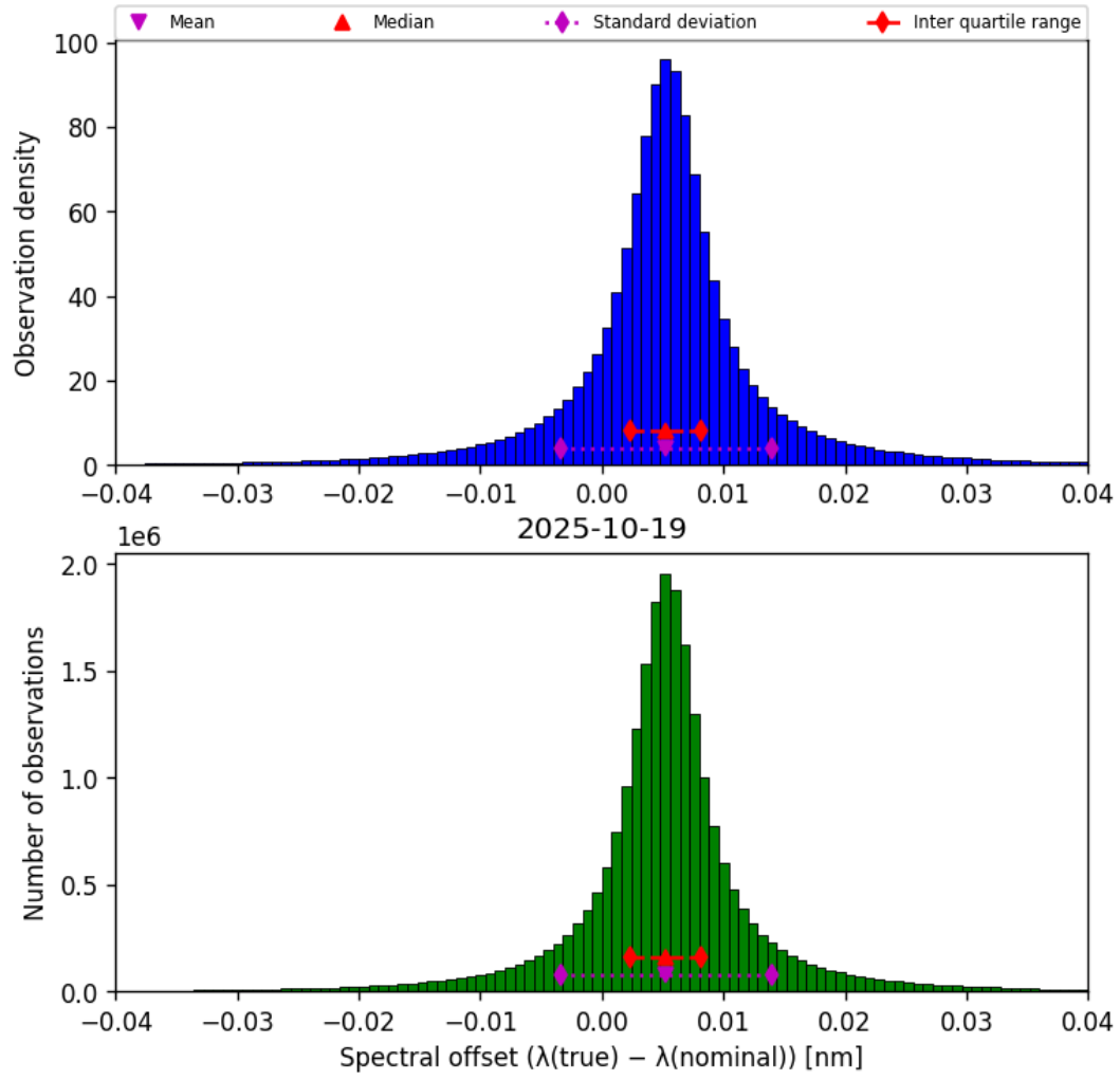
Figure 43: Histogram of “Spectral offset ( \lambda_{\text{true}} - \lambda_{\text{nominal}} )” for 2025-10-19 to 2025-10-20
