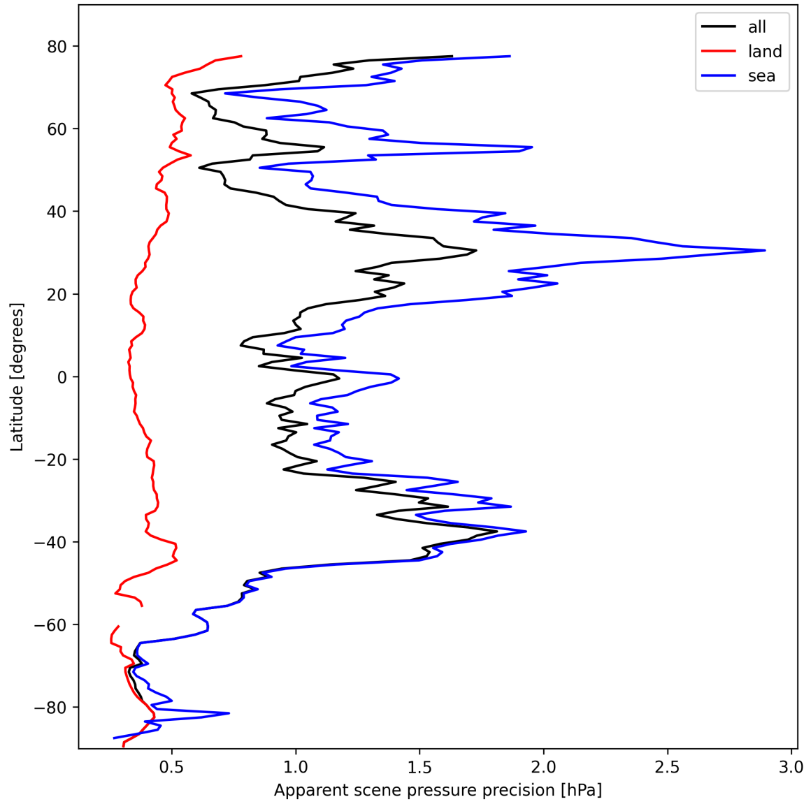
Figure 18: Zonal average of “Apparent scene pressure precision” for 2025-10-19 to 2025-10-20.
