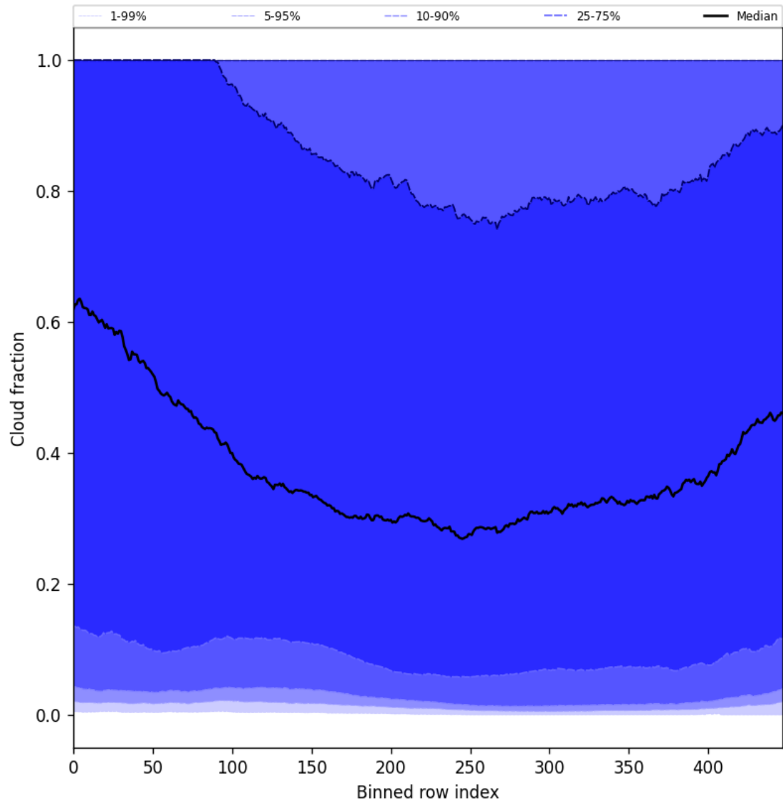
Figure 47: Along track statistics of “Cloud fraction” for 2025-10-19 to 2025-10-20
