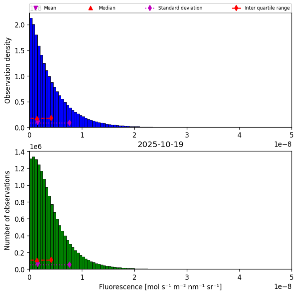
Figure 38: Histogram of “Fluorescence” for 2025-10-19 to 2025-10-20
