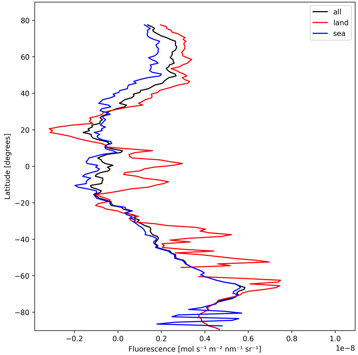
Figure 21: Zonal average of “Fluorescence” for 2025-10-19 to 2025-10-20.
