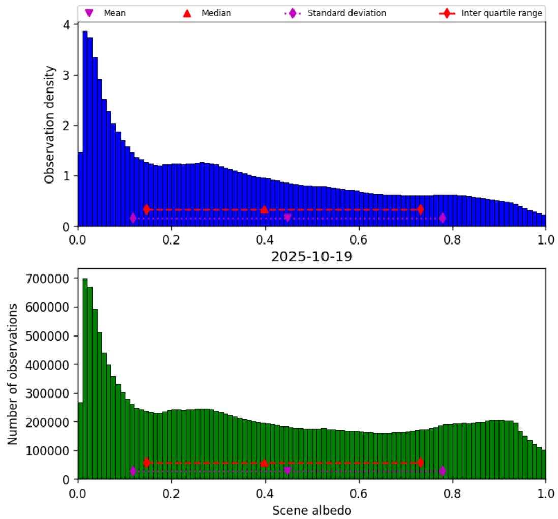
Figure 32: Histogram of “Scene albedo” for 2025-10-19 to 2025-10-20
