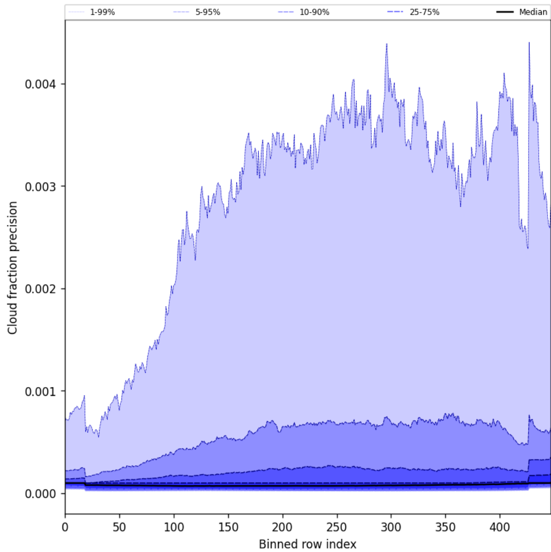
Figure 48: Along track statistics of “Cloud fraction precision” for 2025-10-19 to 2025-10-20
