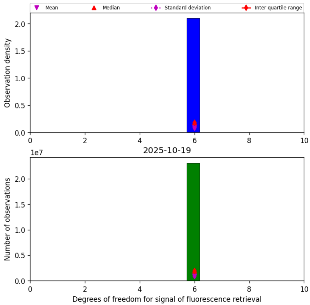
Figure 41: Histogram of “Degrees of freedom for signal of fluorescence retrieval” for 2025-10-19 to 2025-10-20
