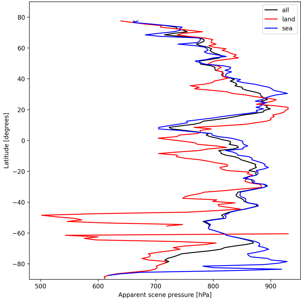
Figure 17: Zonal average of “Apparent scene pressure” for 2025-10-19 to 2025-10-20.
