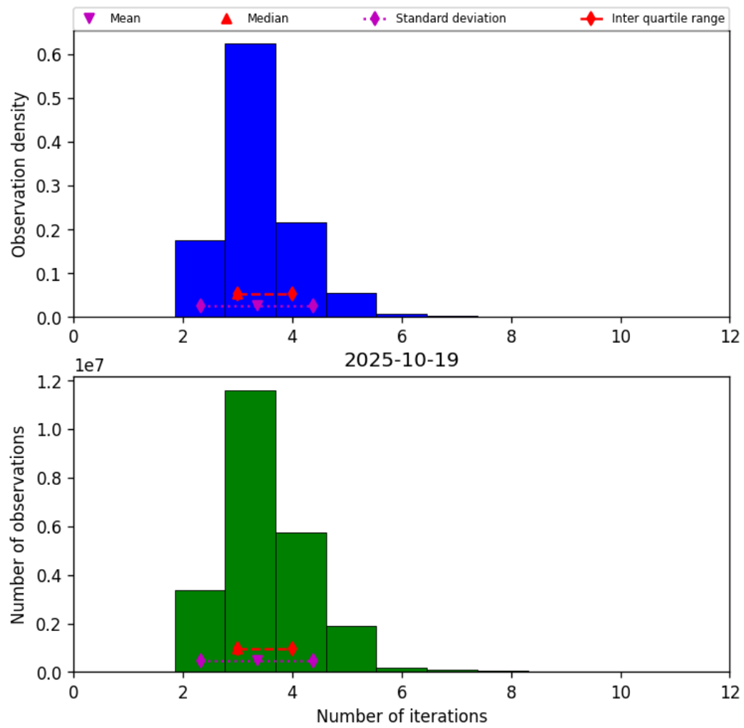
Figure 37: Histogram of “Number of iterations” for 2025-10-19 to 2025-10-20
