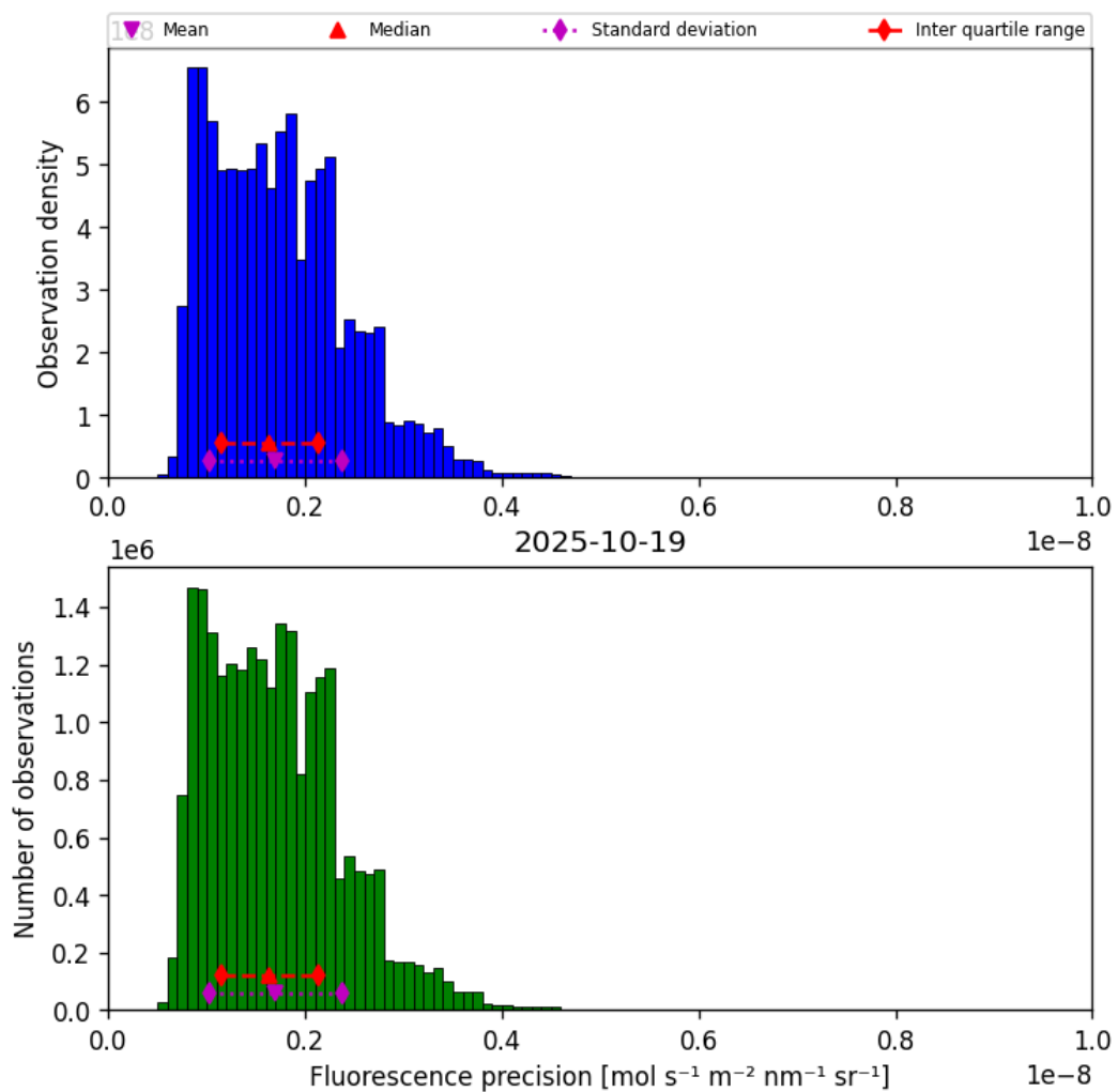
Figure 39: Histogram of “Fluorescence precision” for 2025-10-19 to 2025-10-20
