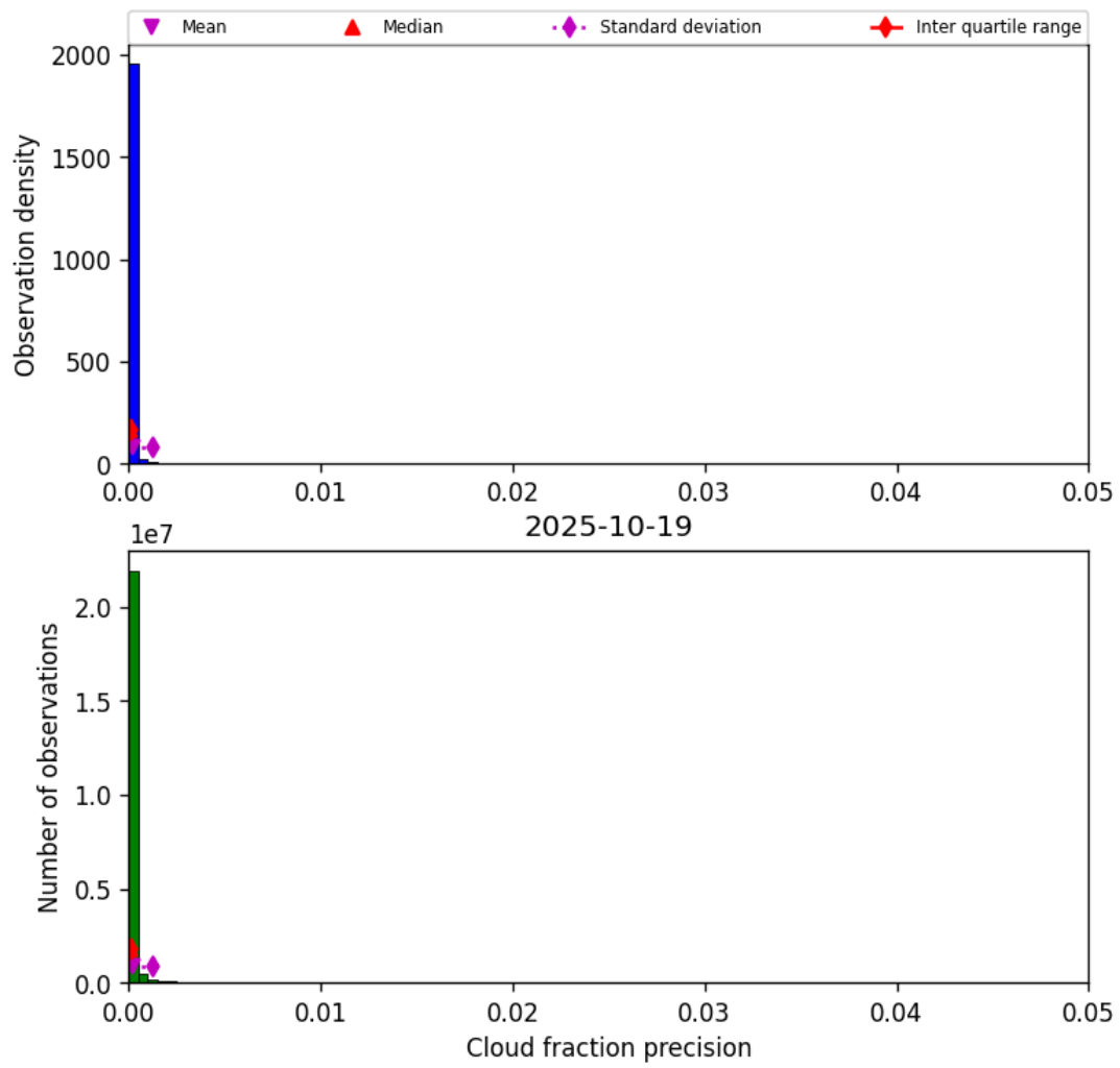
Figure 31: Histogram of “Cloud fraction precision” for 2025-10-19 to 2025-10-20
