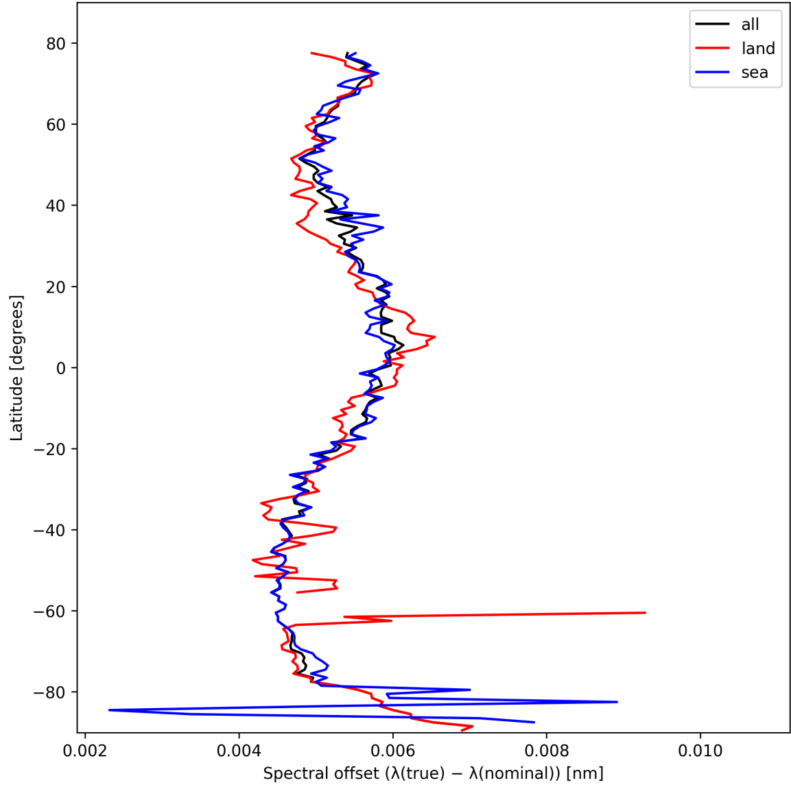
Figure 26: Zonal average of “Spectral offset ( \lambda_{\text{true}} - \lambda_{\text{nominal}} )” for 2025-10-19 to 2025-10-20.
