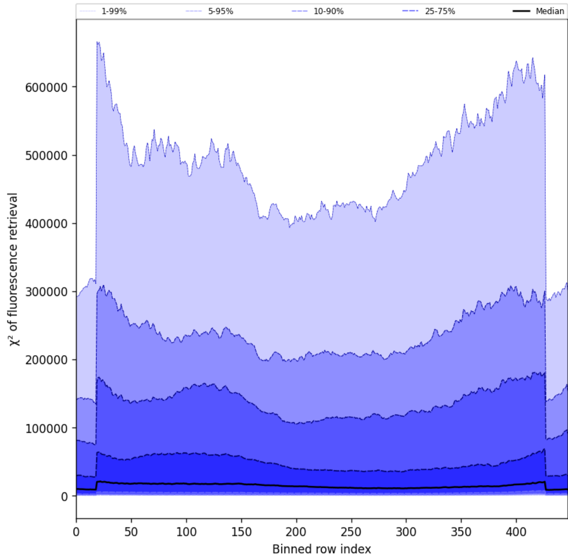
Figure 57: Along track statistics of “ \chi^2 of fluorescence retrieval” for 2025-10-19 to 2025-10-20
