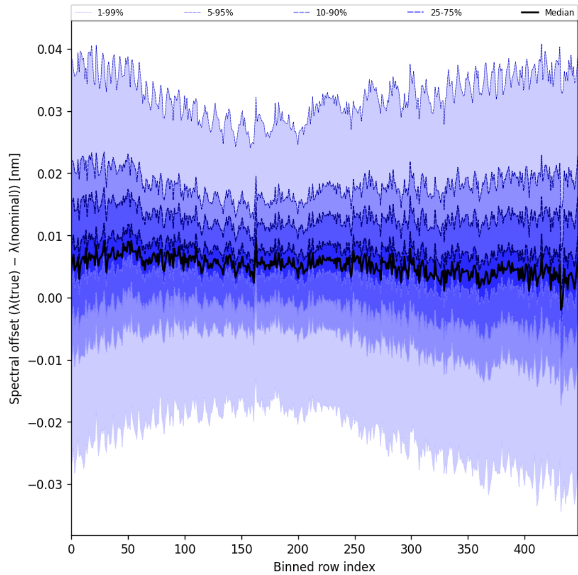
Figure 60: Along track statistics of “Spectral offset ( \lambda_{\text{true}} - \lambda_{\text{nominal}} )” for 2025-10-19 to 2025-10-20
