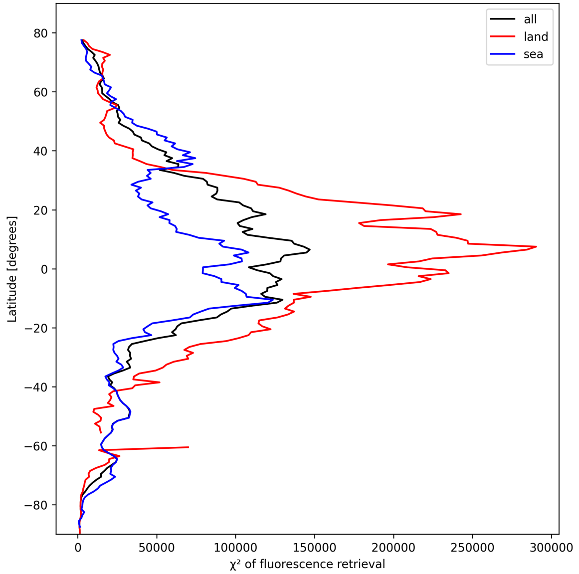
Figure 23: Zonal average of “ \chi^2 of fluorescence retrieval” for 2025-10-19 to 2025-10-20.
