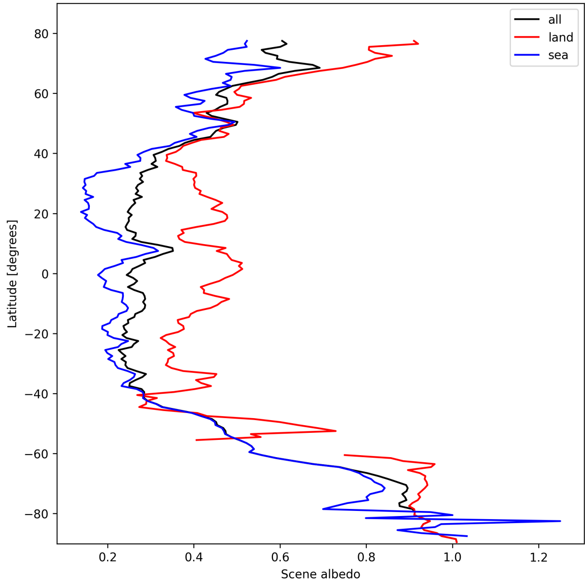
Figure 15: Zonal average of “Scene albedo” for 2025-10-19 to 2025-10-20.
