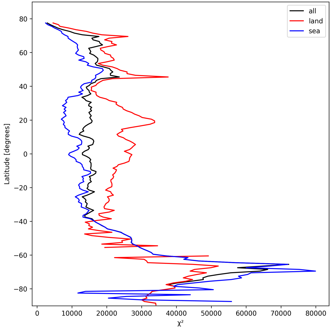
Figure 19: Zonal average of “ \chi^2 ” for 2025-10-19 to 2025-10-20.
