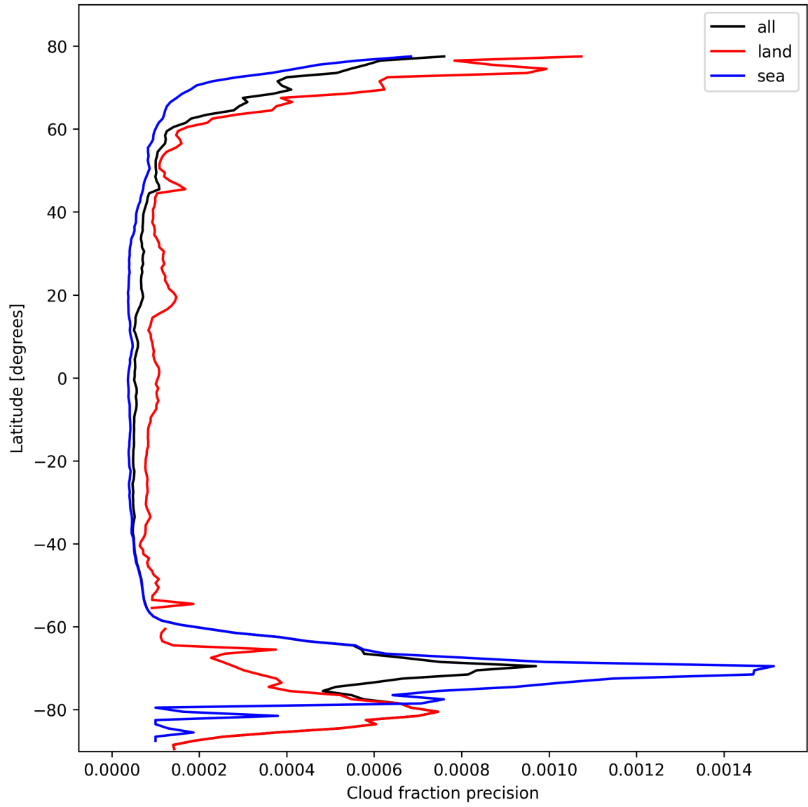
Figure 14: Zonal average of “Cloud fraction precision” for 2025-10-19 to 2025-10-20.
