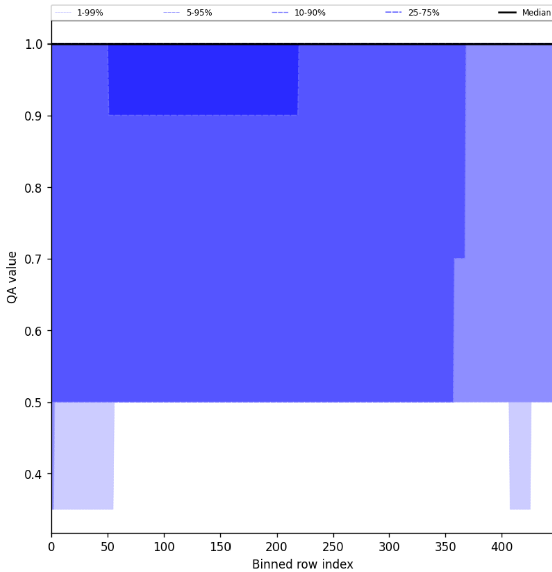
Figure 44: Along track statistics of “QA value” for 2025-10-19 to 2025-10-20
