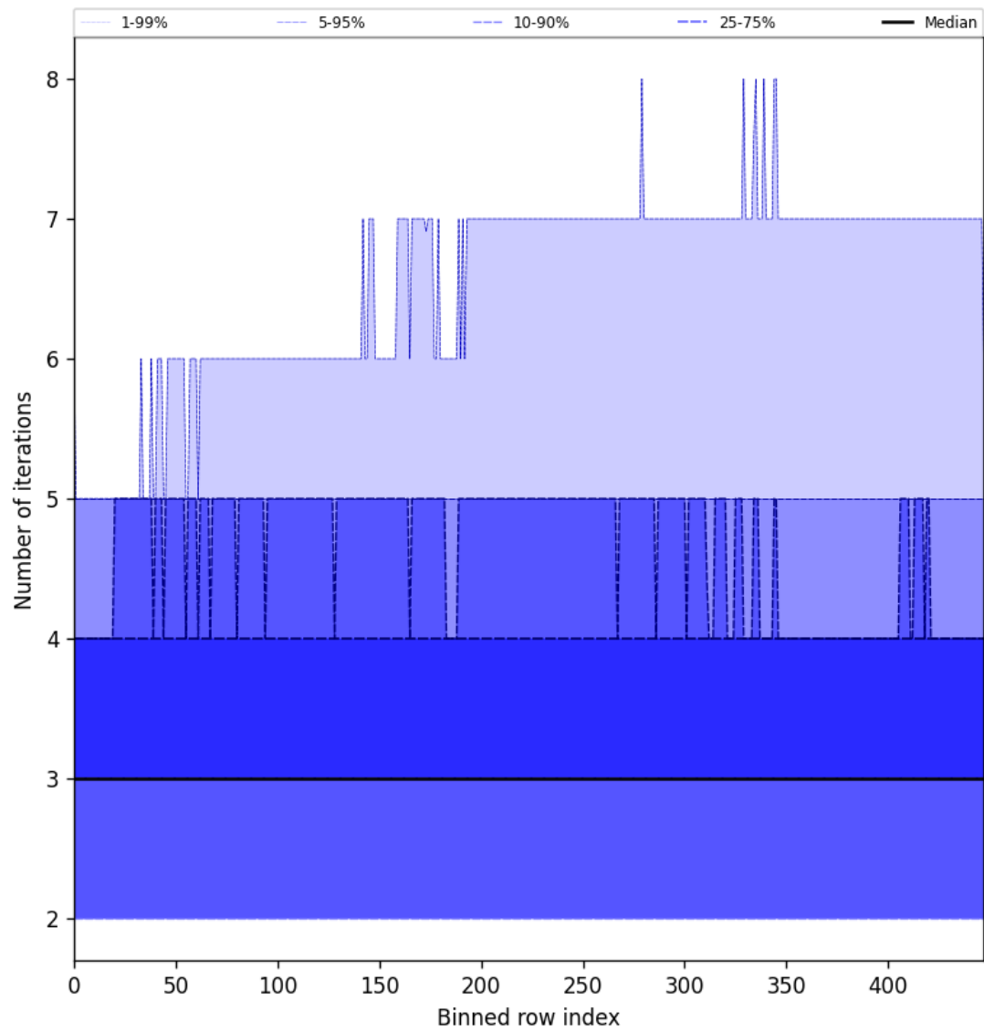
Figure 54: Along track statistics of “Number of iterations” for 2025-10-19 to 2025-10-20
