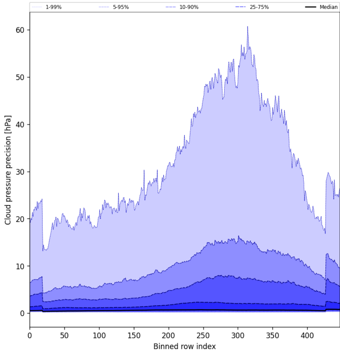
Figure 46: Along track statistics of “Cloud pressure precision” for 2025-10-19 to 2025-10-20
