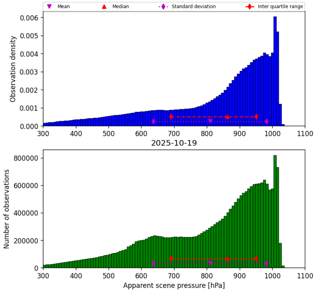
Figure 34: Histogram of “Apparent scene pressure” for 2025-10-19 to 2025-10-20
