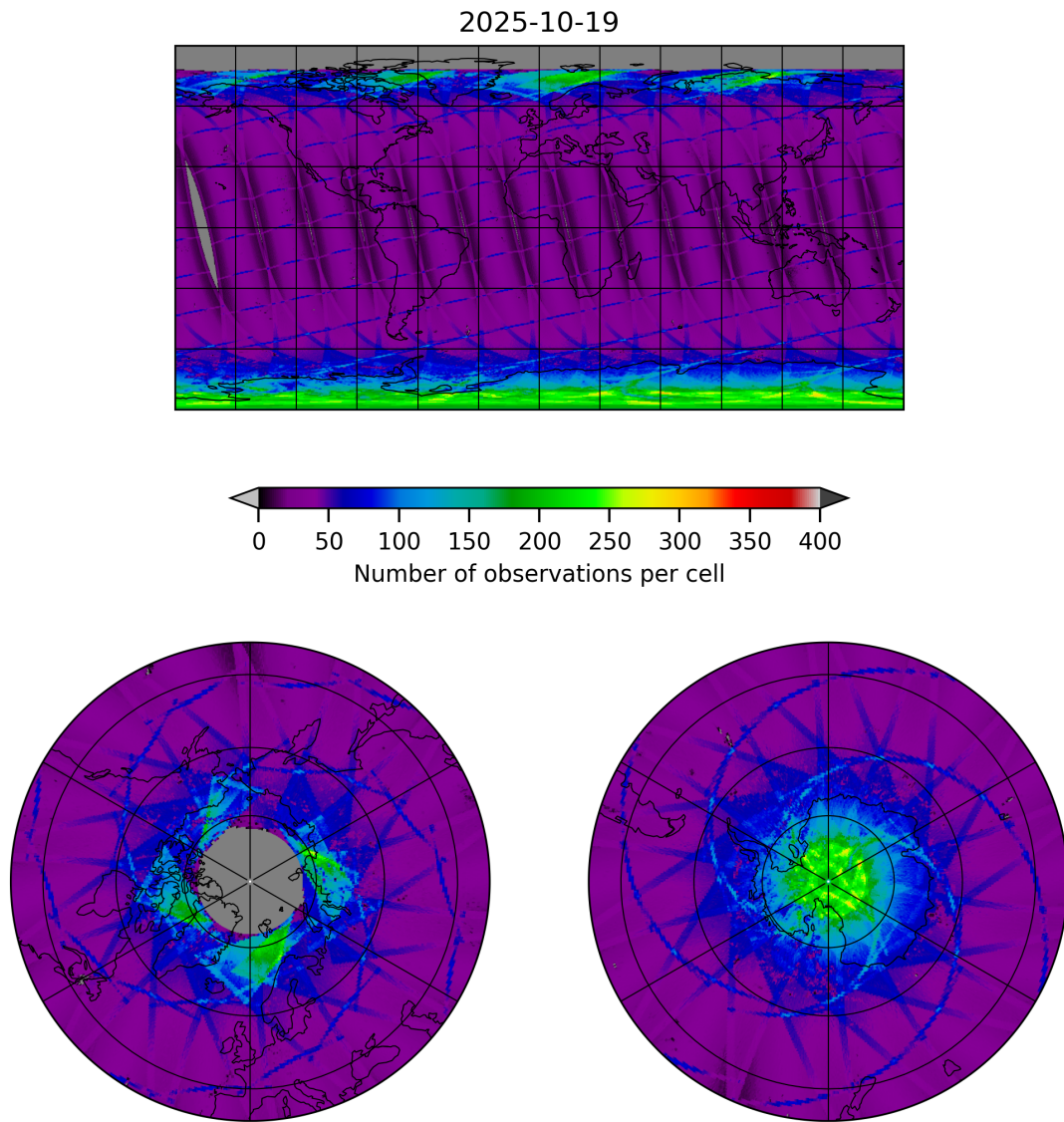
Figure 9: Map of the number of observations for 2025-10-19 to 2025-10-20
