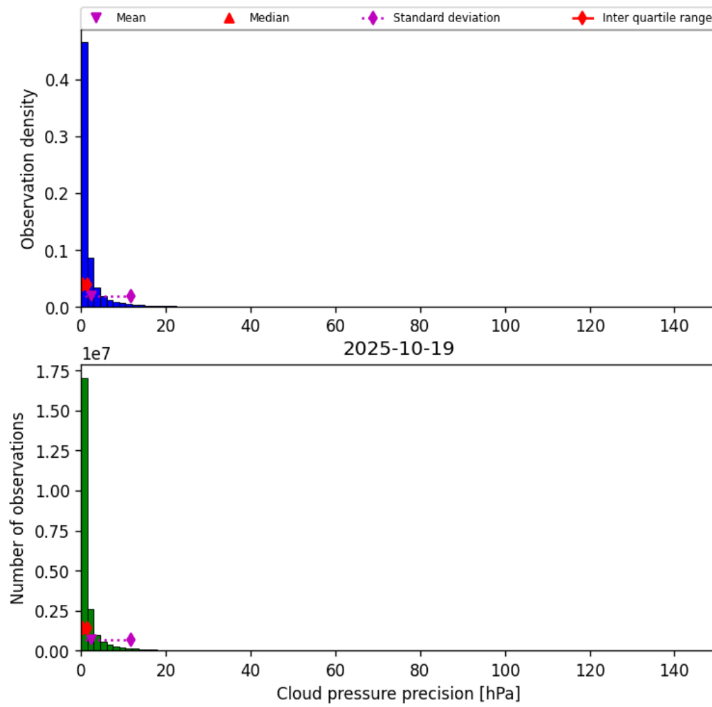
Figure 29: Histogram of “Cloud pressure precision” for 2025-10-19 to 2025-10-20
