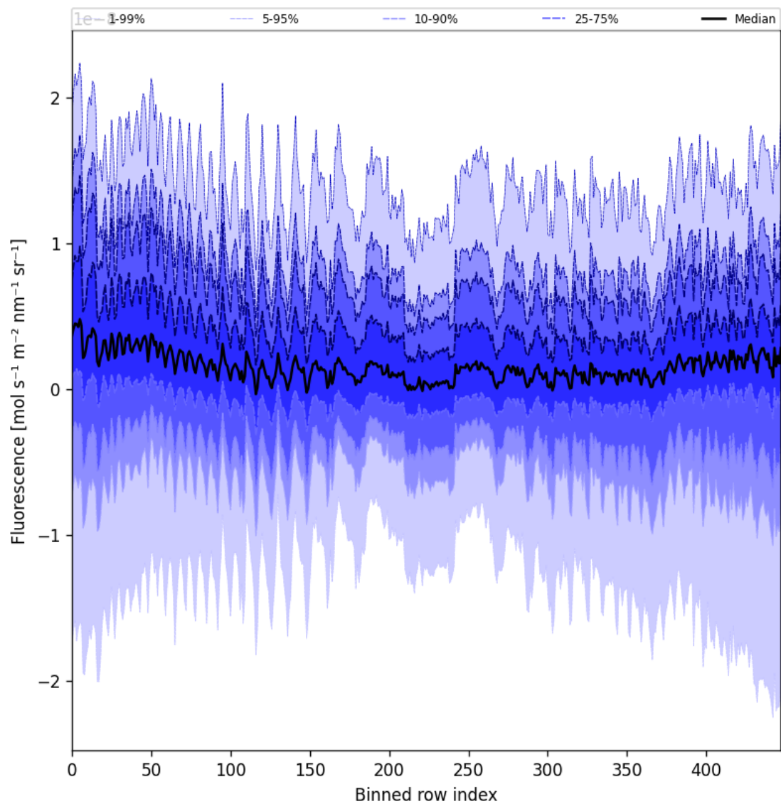
Figure 55: Along track statistics of “Fluorescence” for 2025-10-19 to 2025-10-20
