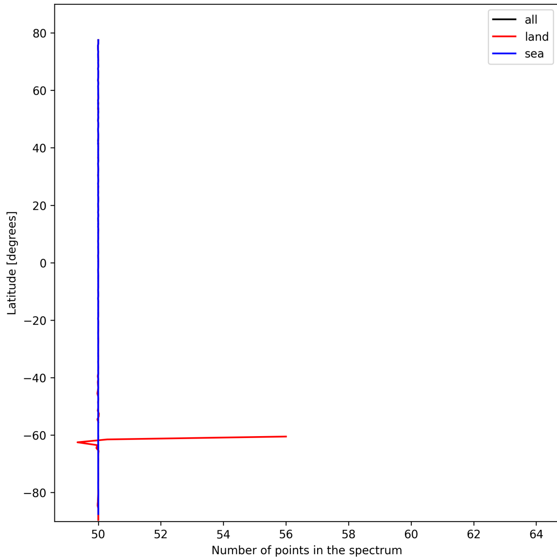
Figure 25: Zonal average of “Number of points in the spectrum” for 2025-10-19 to 2025-10-20.
