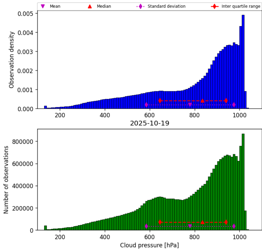
Figure 28: Histogram of “Cloud pressure” for 2025-10-19 to 2025-10-20
