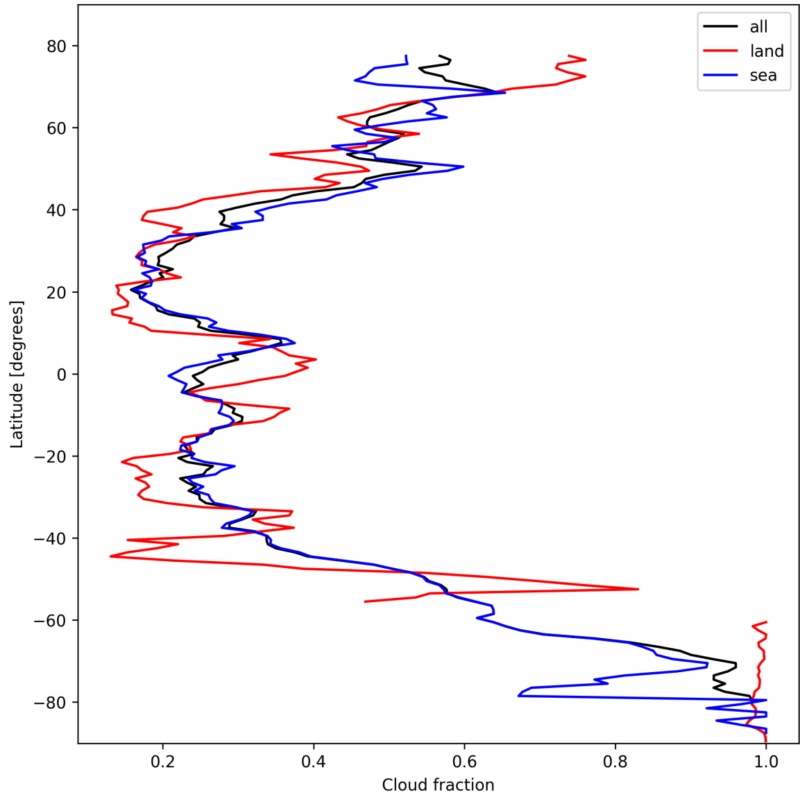
Figure 13: Zonal average of “Cloud fraction” for 2025-10-19 to 2025-10-20.
