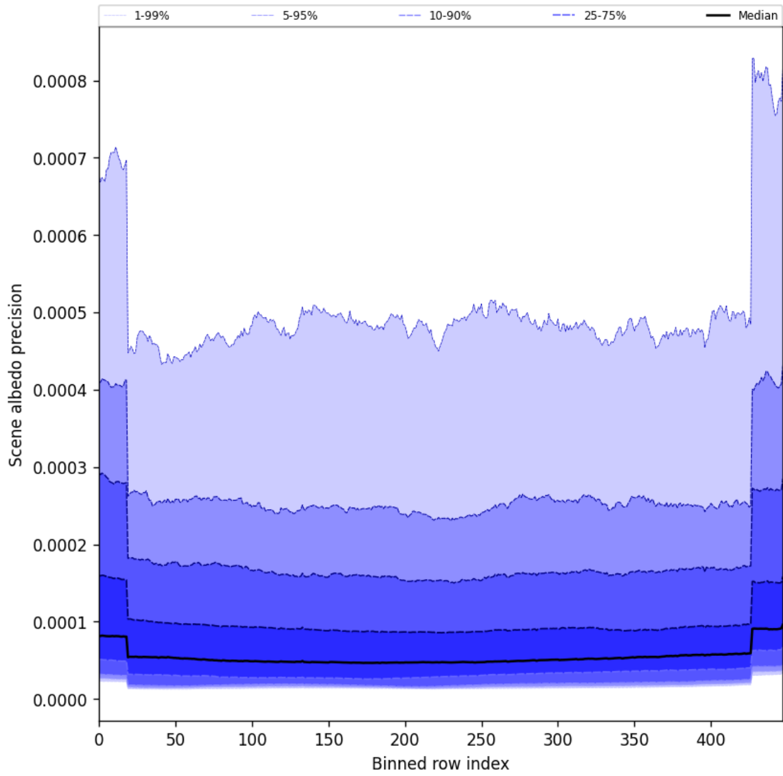
Figure 50: Along track statistics of “Scene albedo precision” for 2025-10-19 to 2025-10-20
