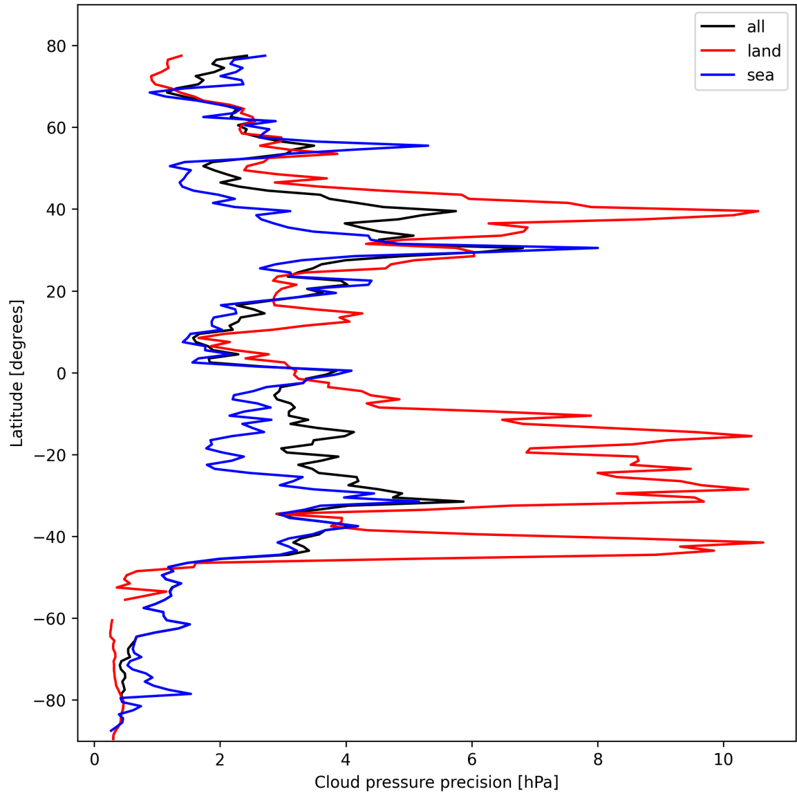
Figure 12: Zonal average of “Cloud pressure precision” for 2025-10-19 to 2025-10-20.
