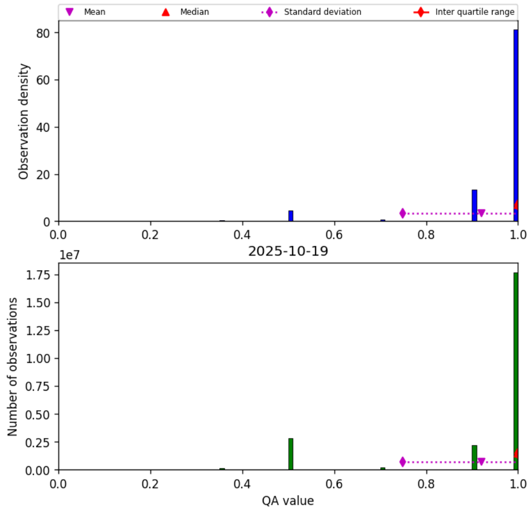
Figure 27: Histogram of “QA value” for 2025-10-19 to 2025-10-20
