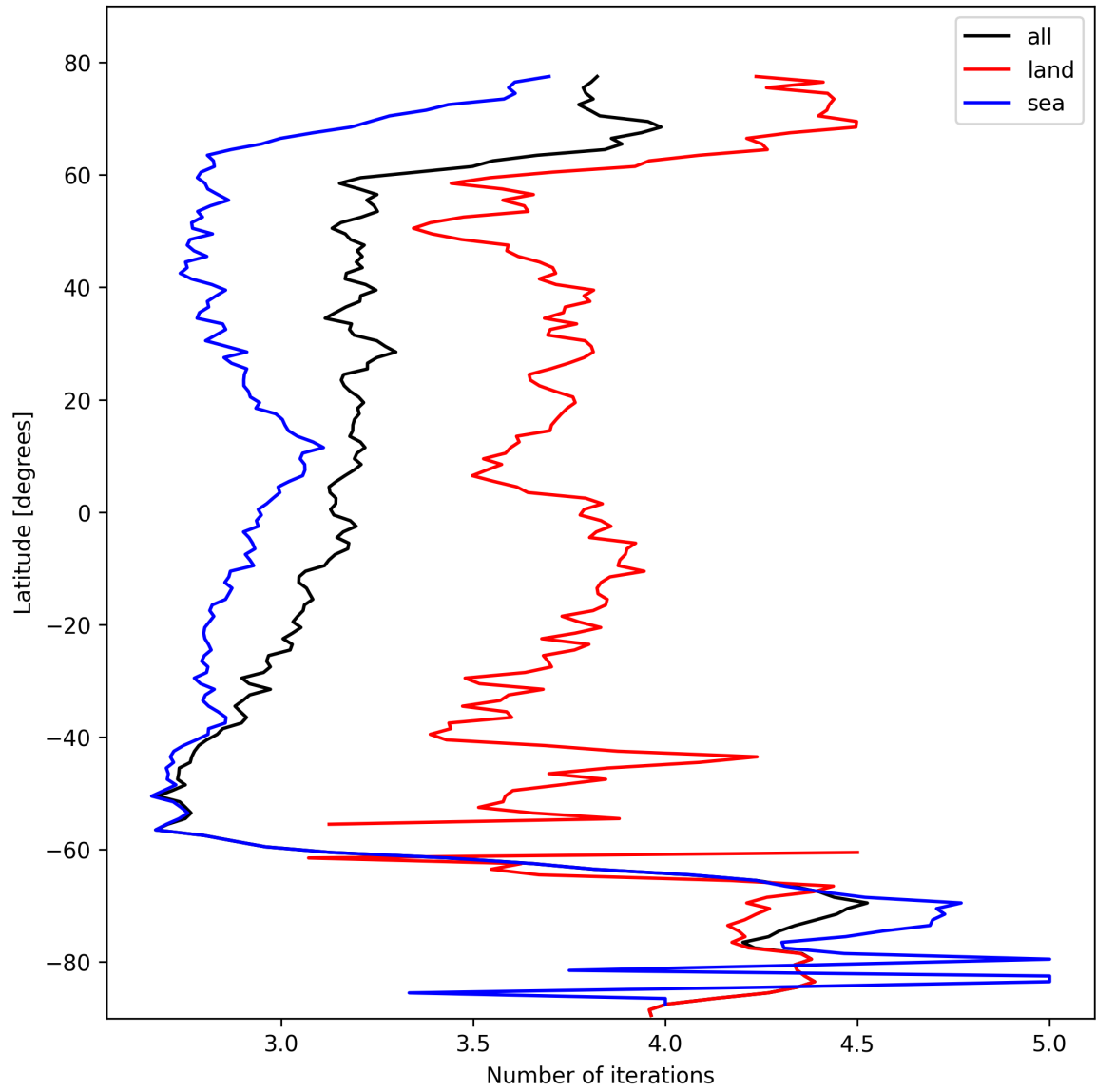
Figure 20: Zonal average of “Number of iterations” for 2025-10-19 to 2025-10-20.
