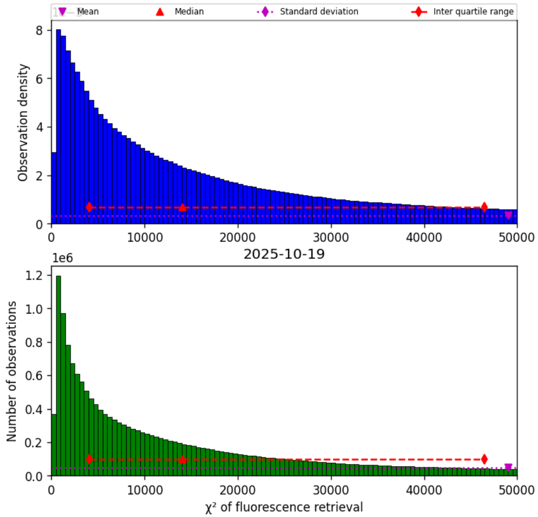
Figure 40: Histogram of “ \chi^2 of fluorescence retrieval” for 2025-10-19 to 2025-10-20
