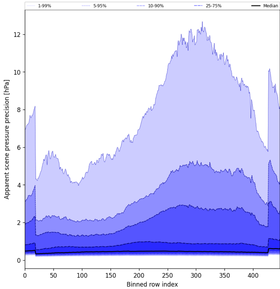
Figure 52: Along track statistics of “Apparent scene pressure precision” for 2025-10-19 to 2025-10-20
