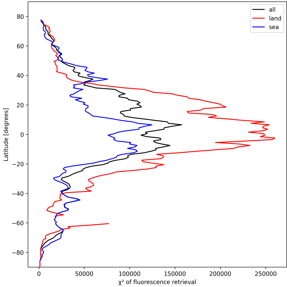
Figure 23: Zonal average of “ \chi^2 of fluorescence retrieval” for 2025-10-20 to 2025-10-20.
