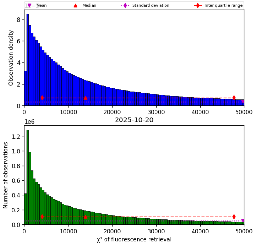
Figure 40: Histogram of “ \chi^2 of fluorescence retrieval” for 2025-10-20 to 2025-10-20
