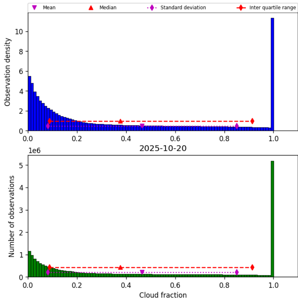
Figure 30: Histogram of “Cloud fraction” for 2025-10-20 to 2025-10-20
