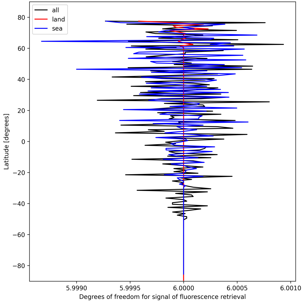
Figure 24: Zonal average of “Degrees of freedom for signal of fluorescence retrieval” for 2025-10-20 to 2025-10-20.
