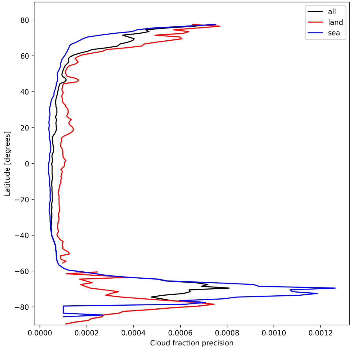
Figure 14: Zonal average of “Cloud fraction precision” for 2025-10-20 to 2025-10-20.
