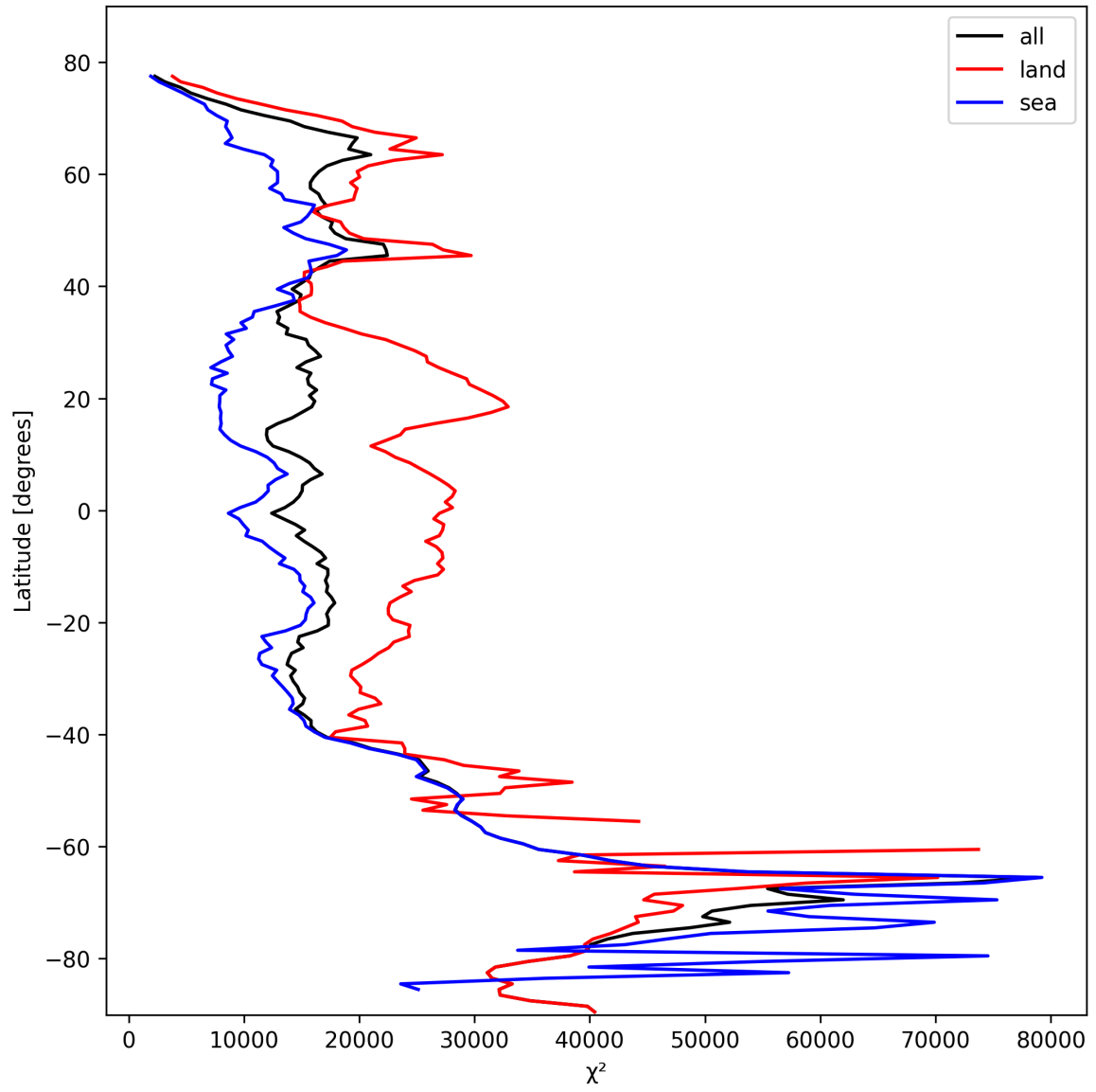
Figure 19: Zonal average of “ \chi^2 ” for 2025-10-20 to 2025-10-20.
