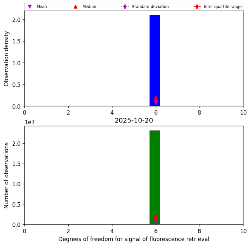
Figure 41: Histogram of “Degrees of freedom for signal of fluorescence retrieval” for 2025-10-20 to 2025-10-20
