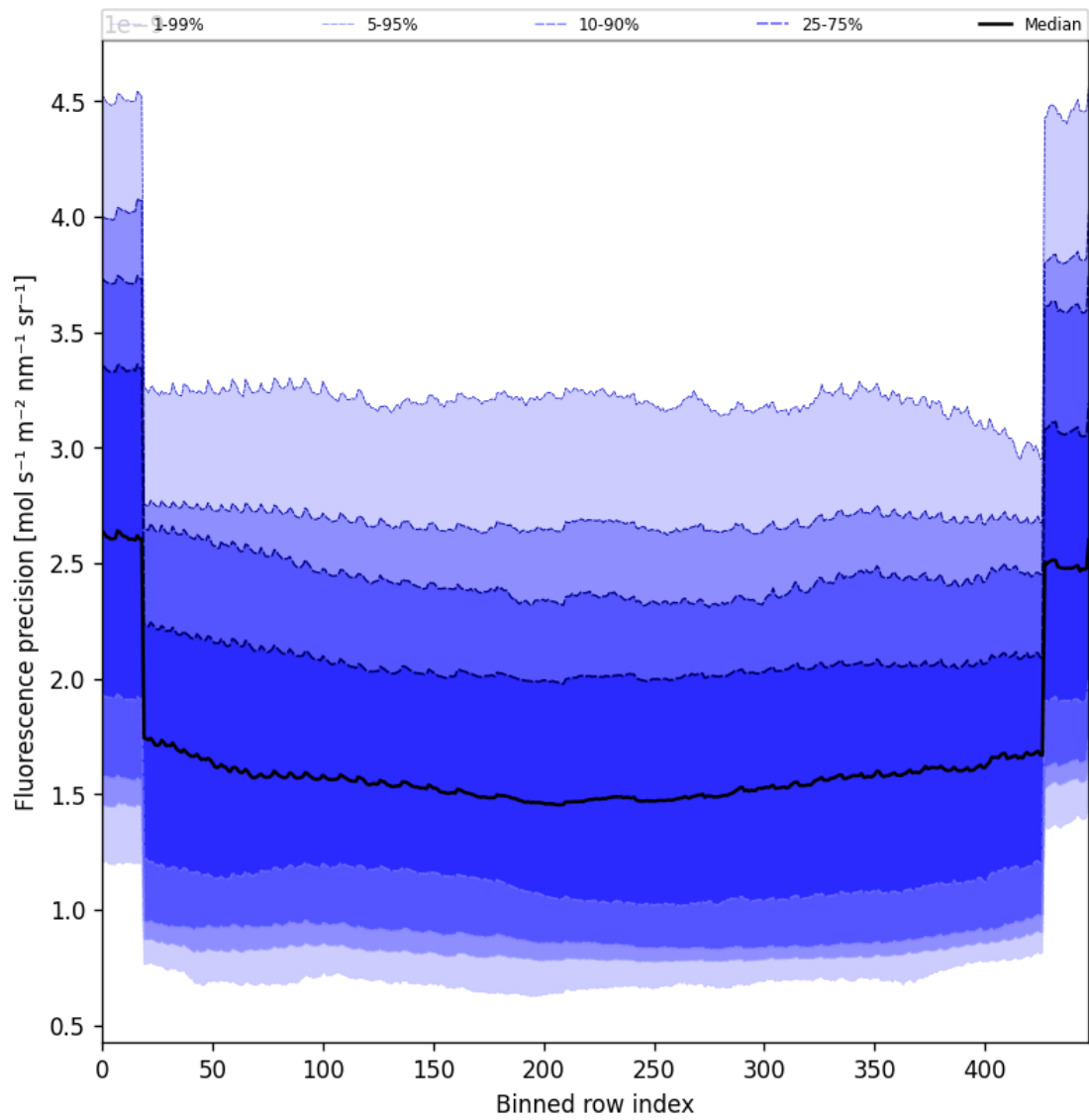
Figure 56: Along track statistics of “Fluorescence precision” for 2025-10-20 to 2025-10-20
