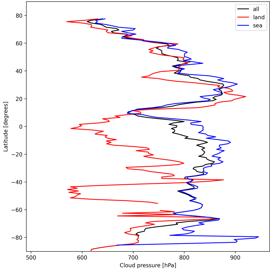
Figure 11: Zonal average of “Cloud pressure” for 2025-10-20 to 2025-10-20.
