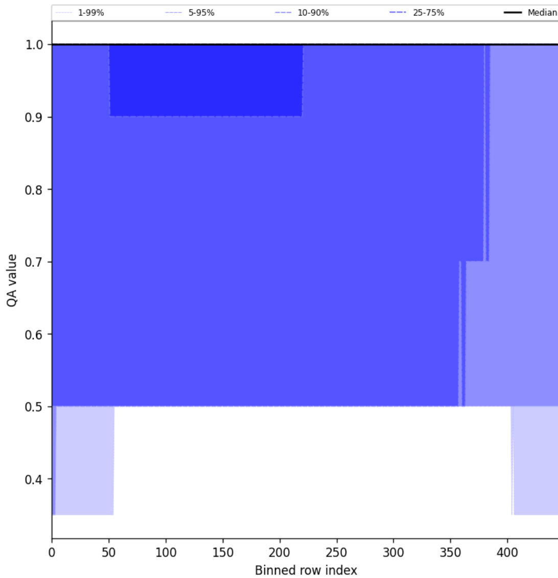
Figure 44: Along track statistics of “QA value” for 2025-10-20 to 2025-10-20
