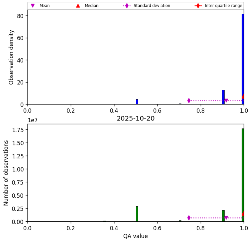
Figure 27: Histogram of “QA value” for 2025-10-20 to 2025-10-20
