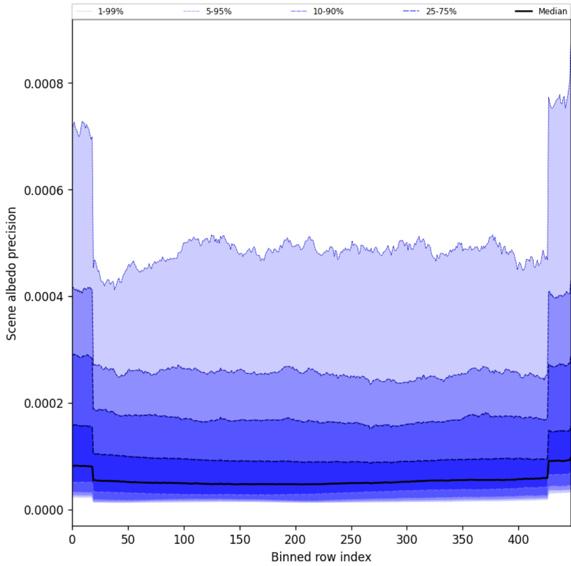
Figure 50: Along track statistics of “Scene albedo precision” for 2025-10-20 to 2025-10-20
