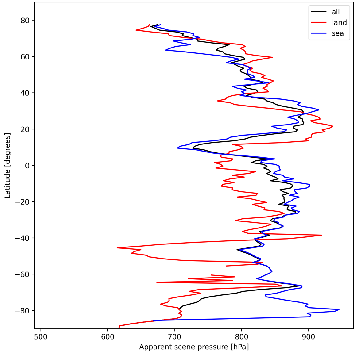
Figure 17: Zonal average of “Apparent scene pressure” for 2025-10-20 to 2025-10-20.
