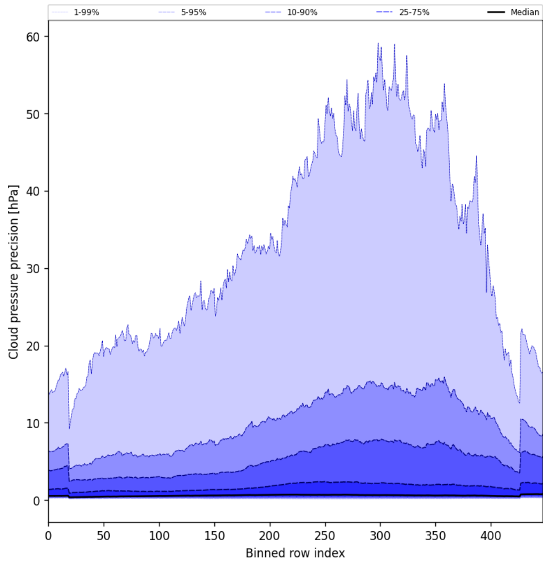
Figure 46: Along track statistics of “Cloud pressure precision” for 2025-10-20 to 2025-10-20
