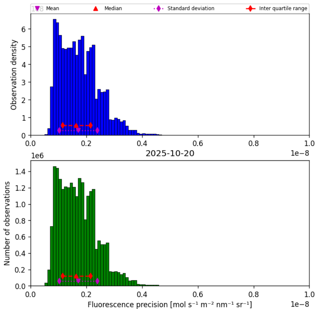
Figure 39: Histogram of “Fluorescence precision” for 2025-10-20 to 2025-10-20
