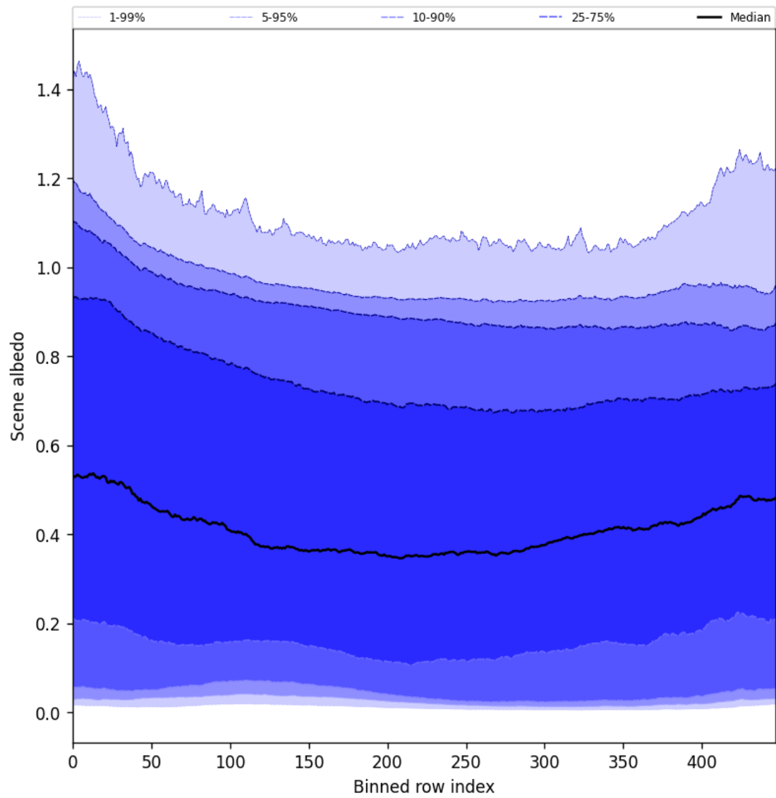
Figure 49: Along track statistics of “Scene albedo” for 2025-10-20 to 2025-10-20
