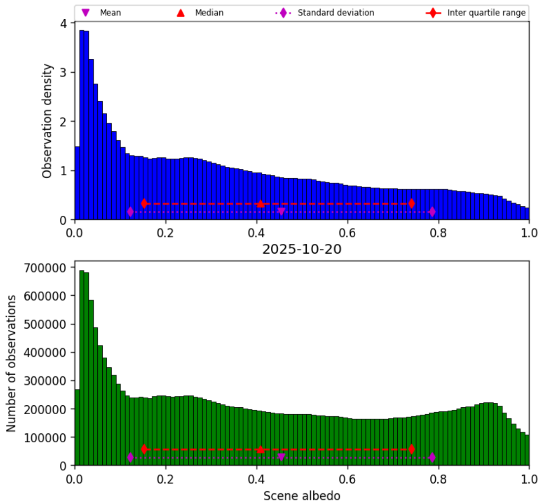
Figure 32: Histogram of “Scene albedo” for 2025-10-20 to 2025-10-20
