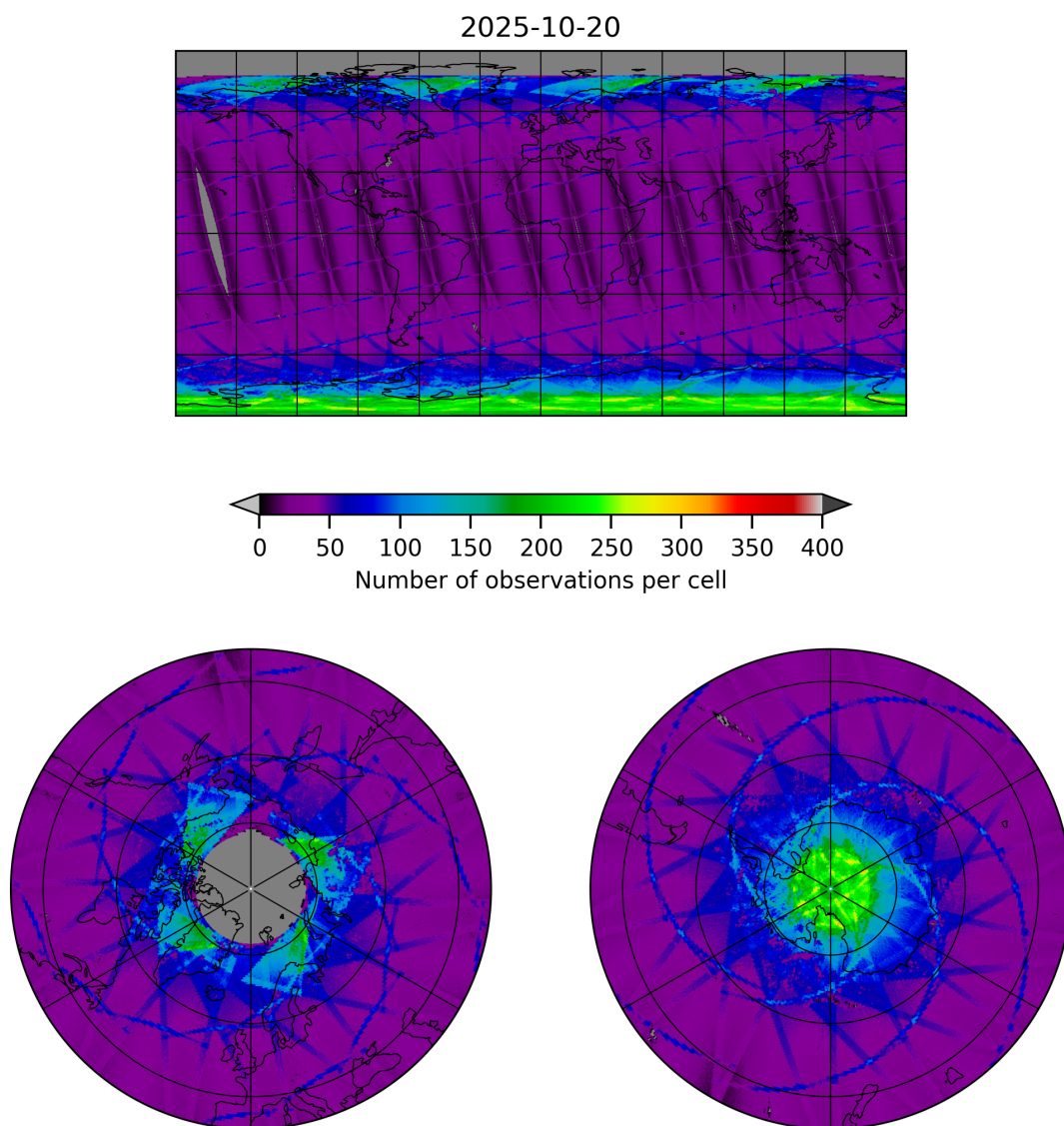
Figure 9: Map of the number of observations for 2025-10-20 to 2025-10-20
