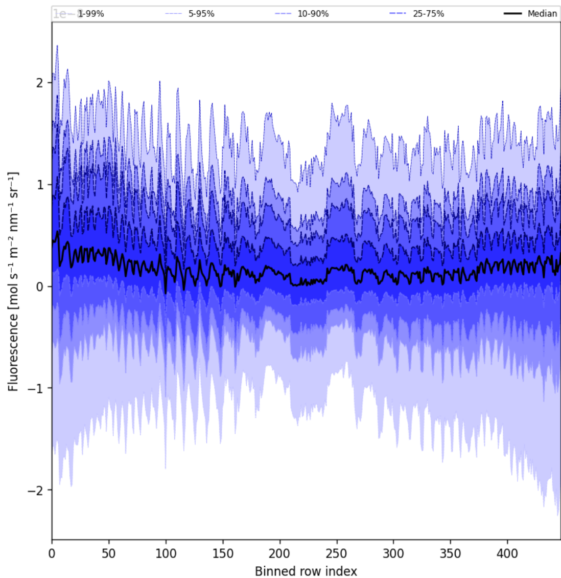
Figure 55: Along track statistics of “Fluorescence” for 2025-10-20 to 2025-10-20
