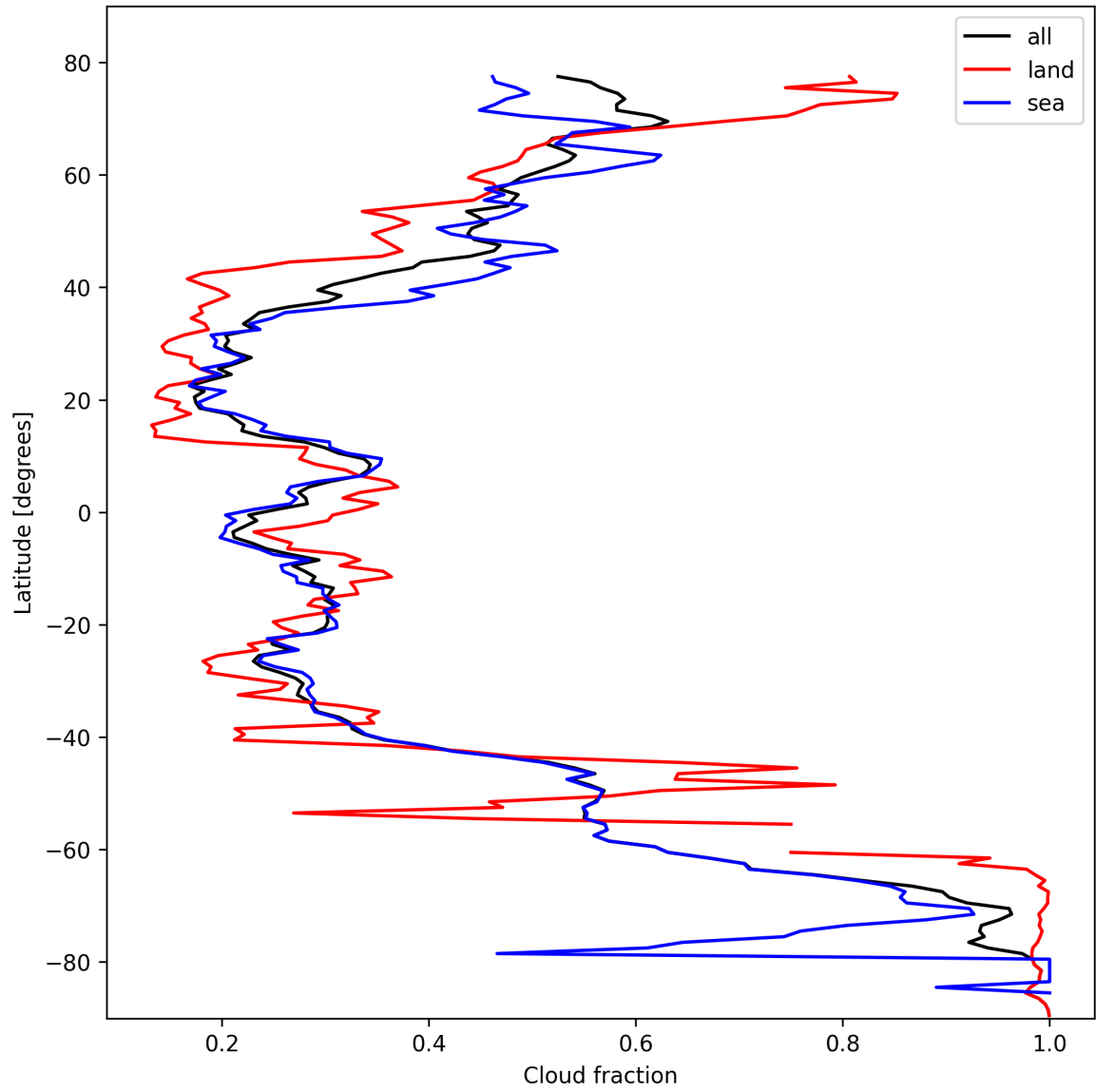
Figure 13: Zonal average of “Cloud fraction” for 2025-10-20 to 2025-10-20.
