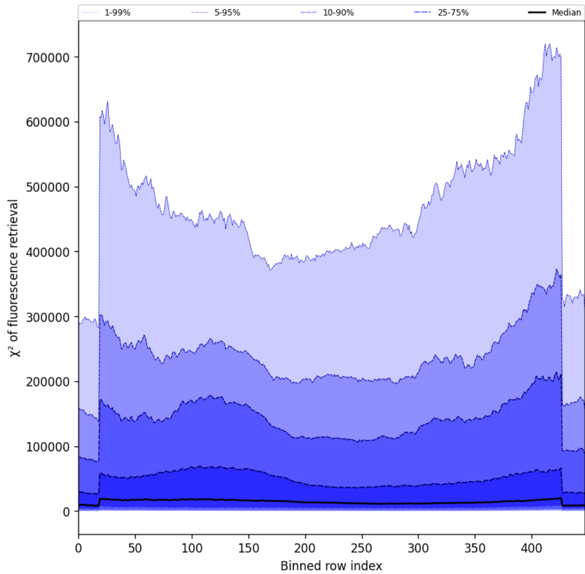
Figure 57: Along track statistics of “ \chi^2 of fluorescence retrieval” for 2025-10-20 to 2025-10-20
