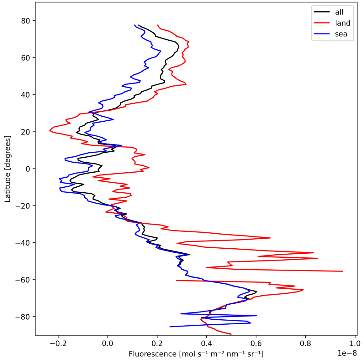
Figure 21: Zonal average of “Fluorescence” for 2025-10-20 to 2025-10-20.
