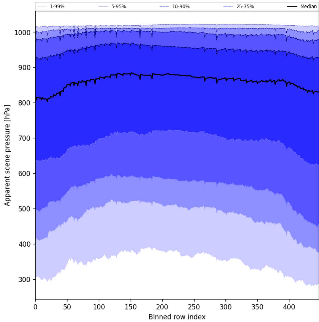
Figure 51: Along track statistics of “Apparent scene pressure” for 2025-10-20 to 2025-10-20
