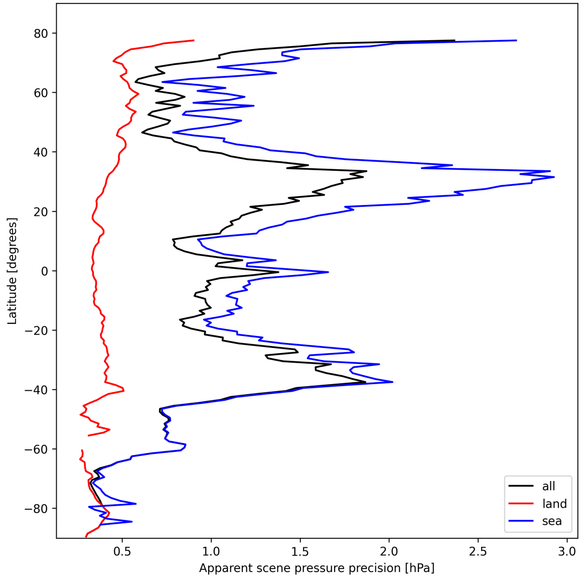
Figure 18: Zonal average of “Apparent scene pressure precision” for 2025-10-20 to 2025-10-20.
