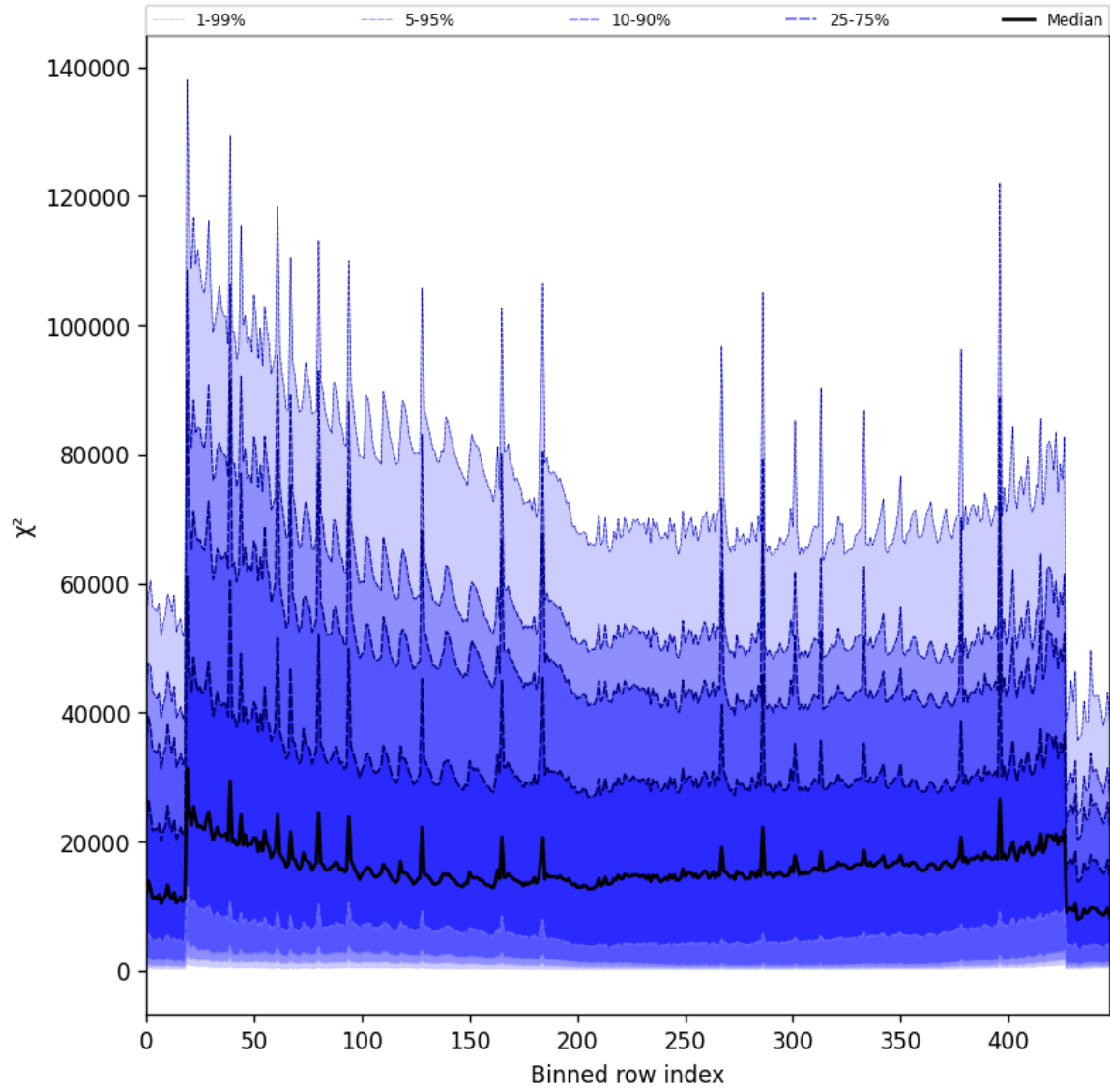
Figure 53: Along track statistics of “ \chi^2 ” for 2025-10-20 to 2025-10-20
