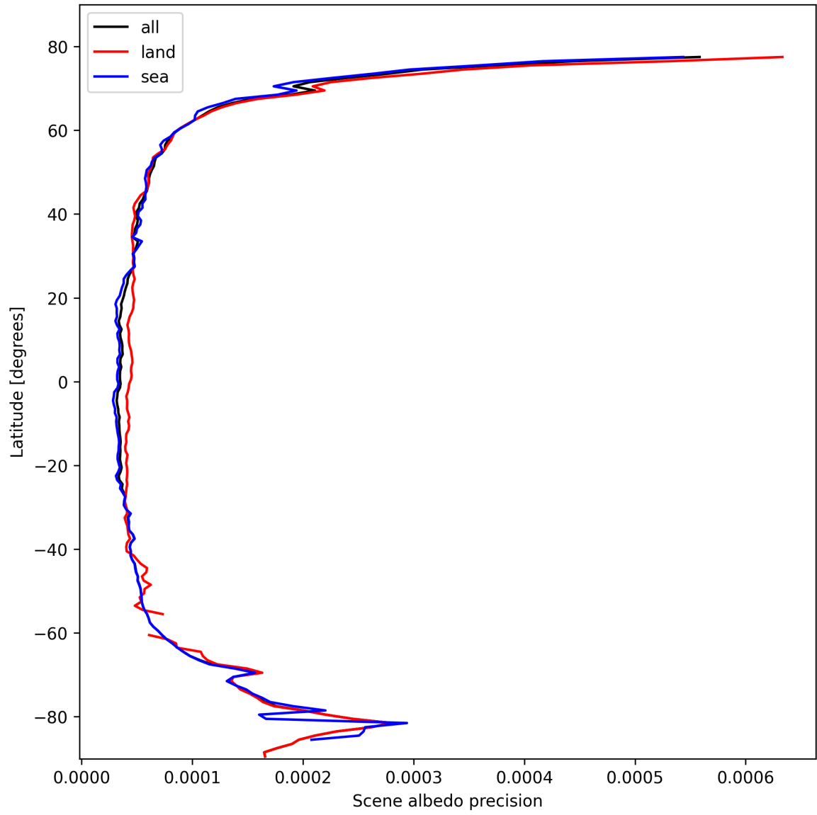
Figure 16: Zonal average of “Scene albedo precision” for 2025-10-20 to 2025-10-20.
