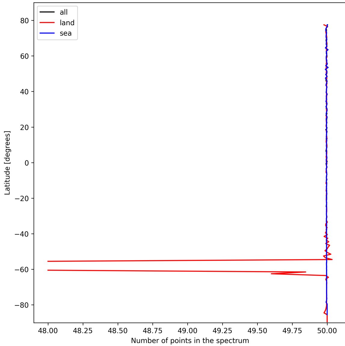
Figure 25: Zonal average of “Number of points in the spectrum” for 2025-10-20 to 2025-10-20.
