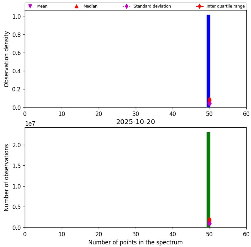
Figure 42: Histogram of “Number of points in the spectrum” for 2025-10-20 to 2025-10-20
