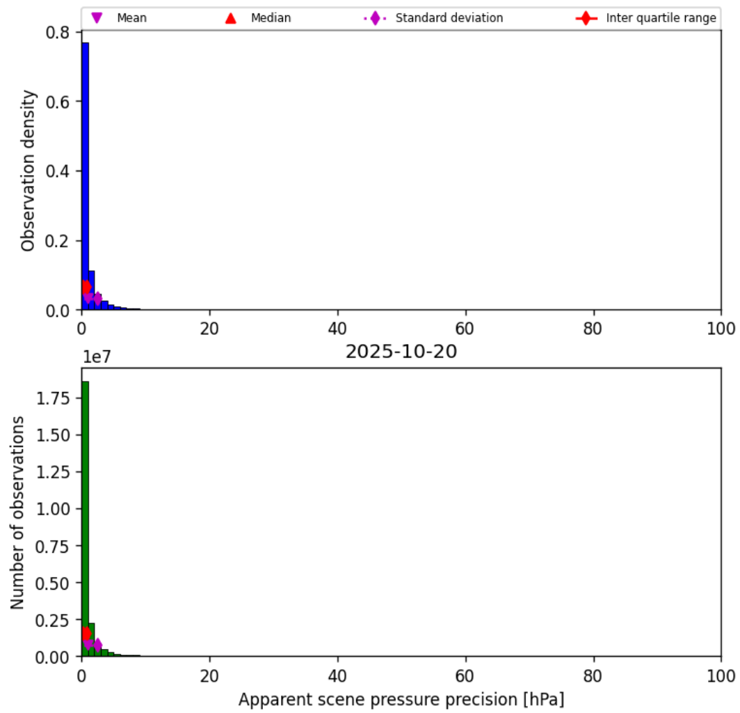
Figure 35: Histogram of “Apparent scene pressure precision” for 2025-10-20 to 2025-10-20
