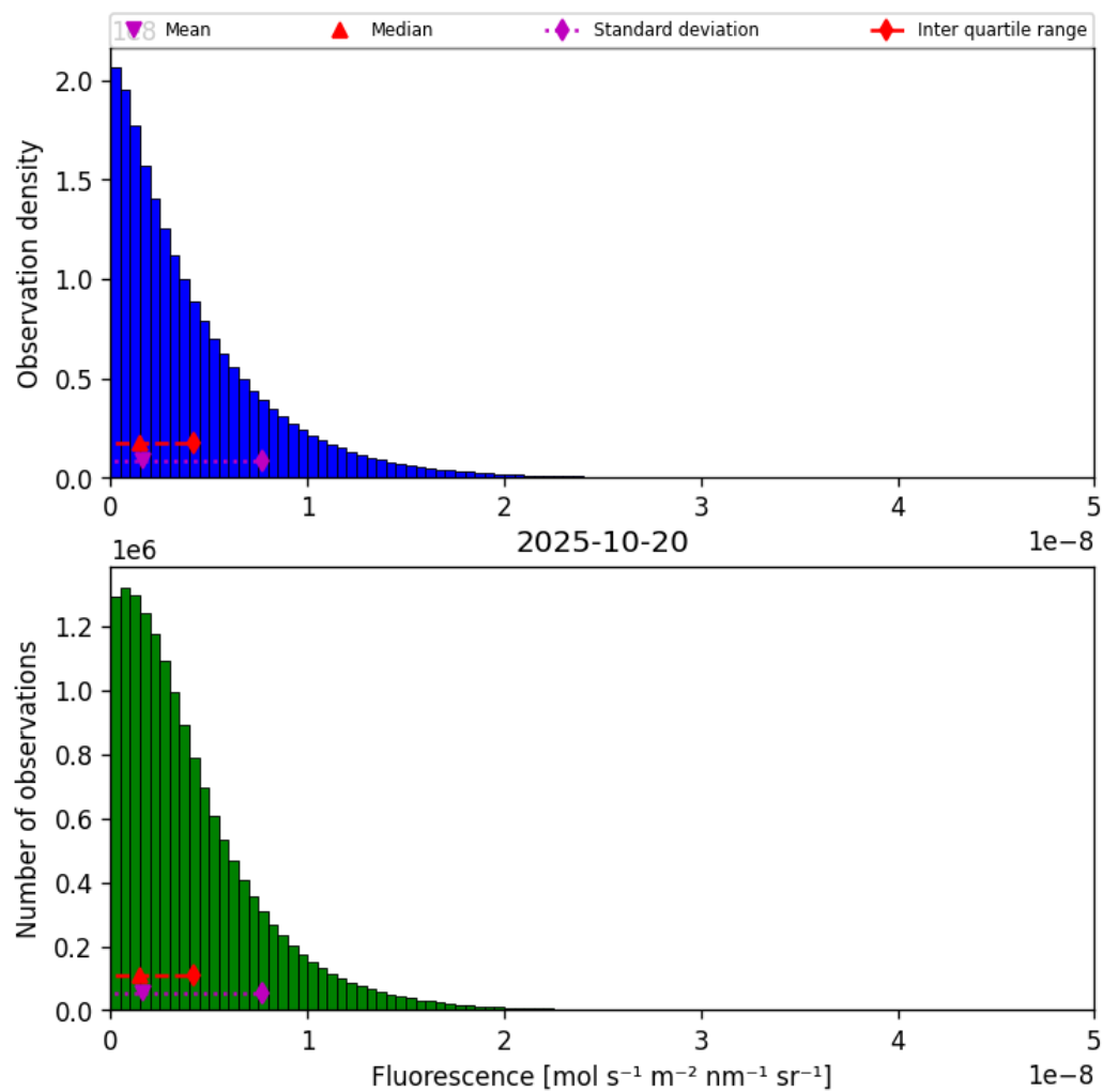
Figure 38: Histogram of “Fluorescence” for 2025-10-20 to 2025-10-20
