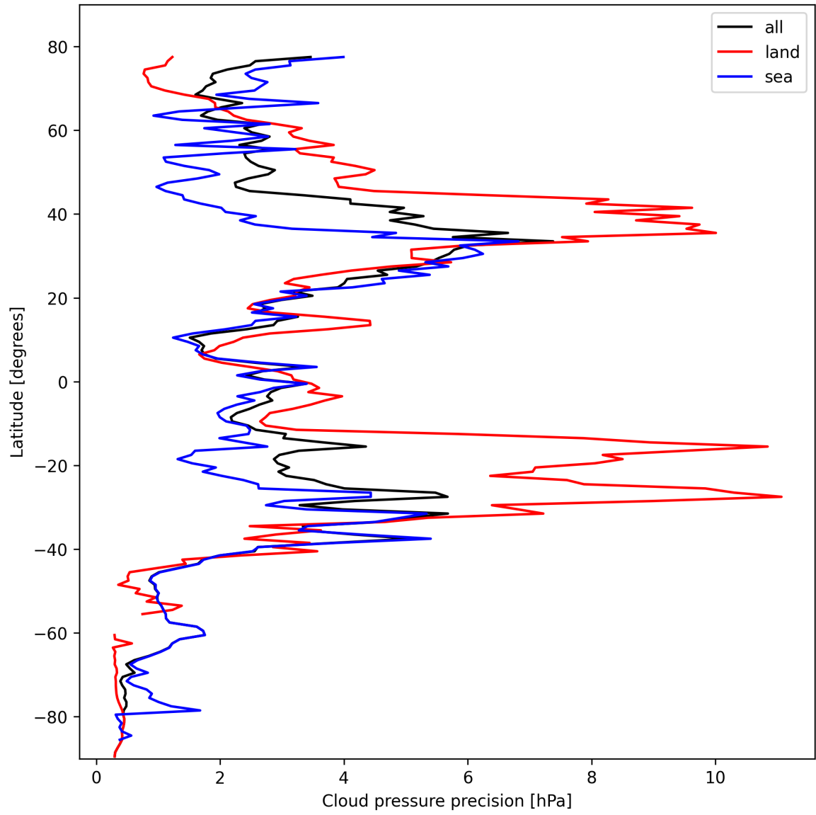
Figure 12: Zonal average of “Cloud pressure precision” for 2025-10-20 to 2025-10-20.
