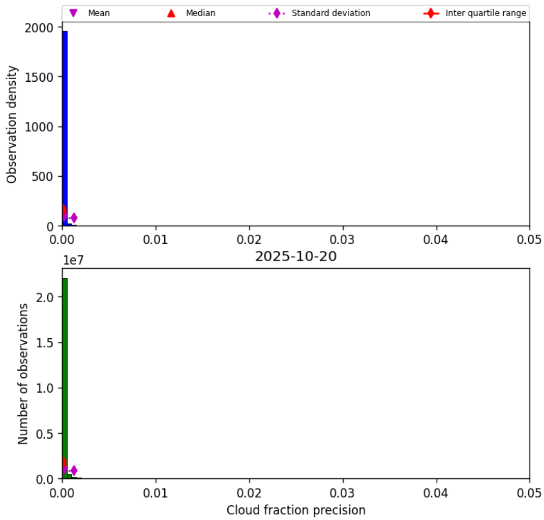
Figure 31: Histogram of “Cloud fraction precision” for 2025-10-20 to 2025-10-20
