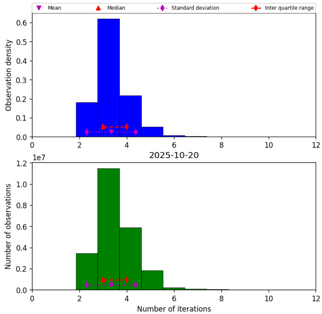
Figure 37: Histogram of “Number of iterations” for 2025-10-20 to 2025-10-20
