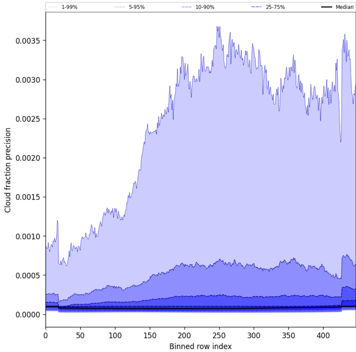
Figure 48: Along track statistics of “Cloud fraction precision” for 2025-10-20 to 2025-10-20
