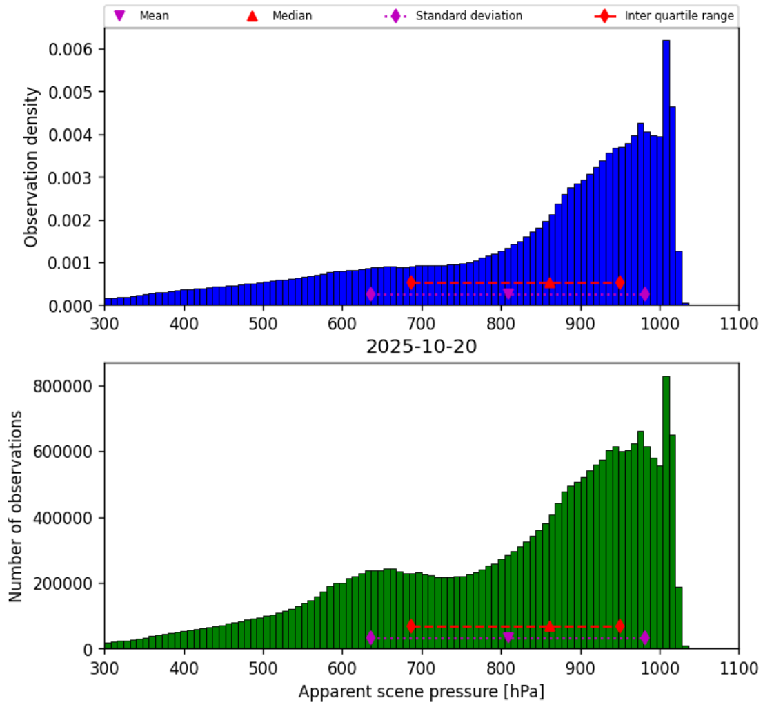
Figure 34: Histogram of “Apparent scene pressure” for 2025-10-20 to 2025-10-20
