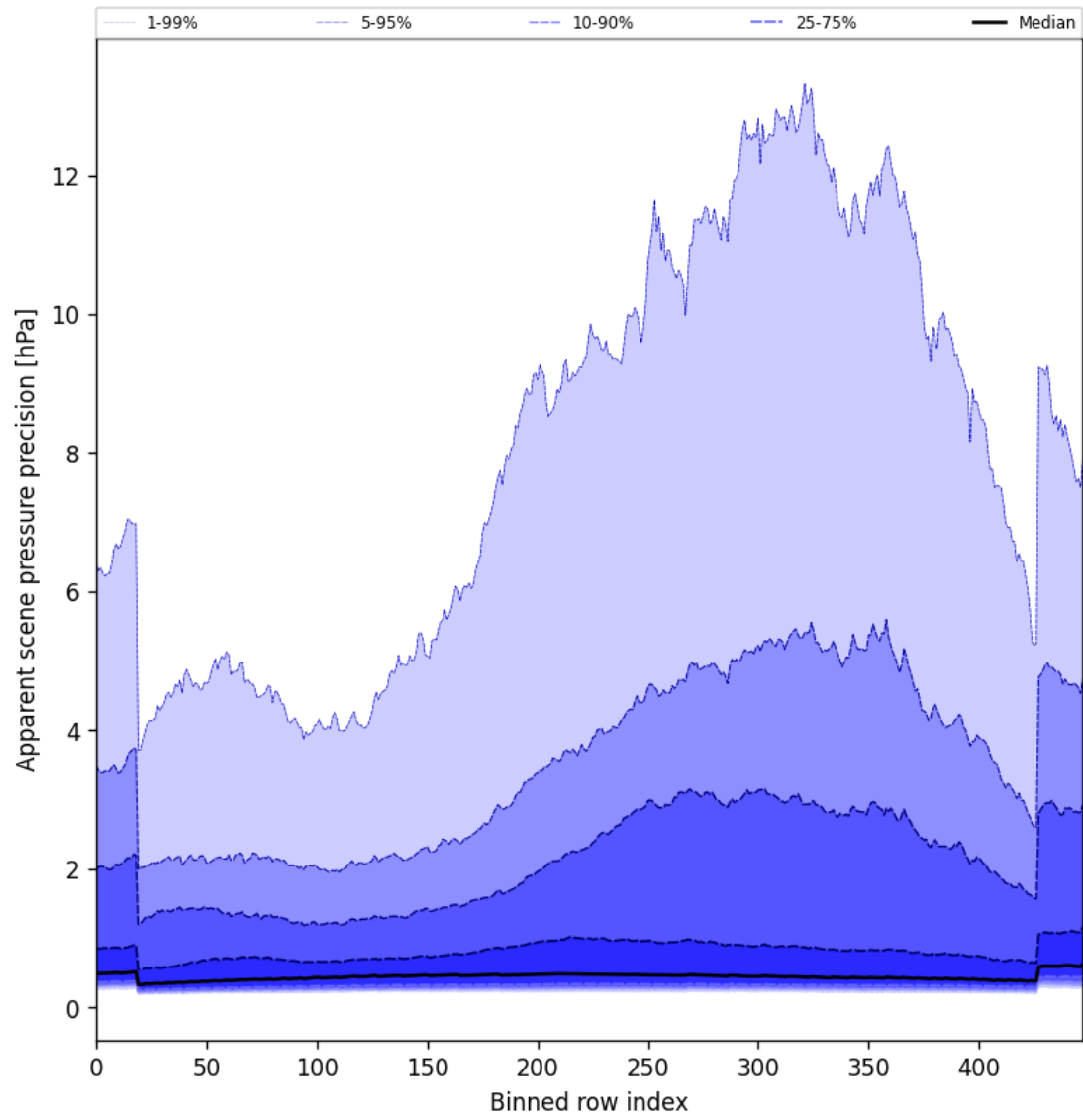
Figure 52: Along track statistics of “Apparent scene pressure precision” for 2025-10-20 to 2025-10-20
