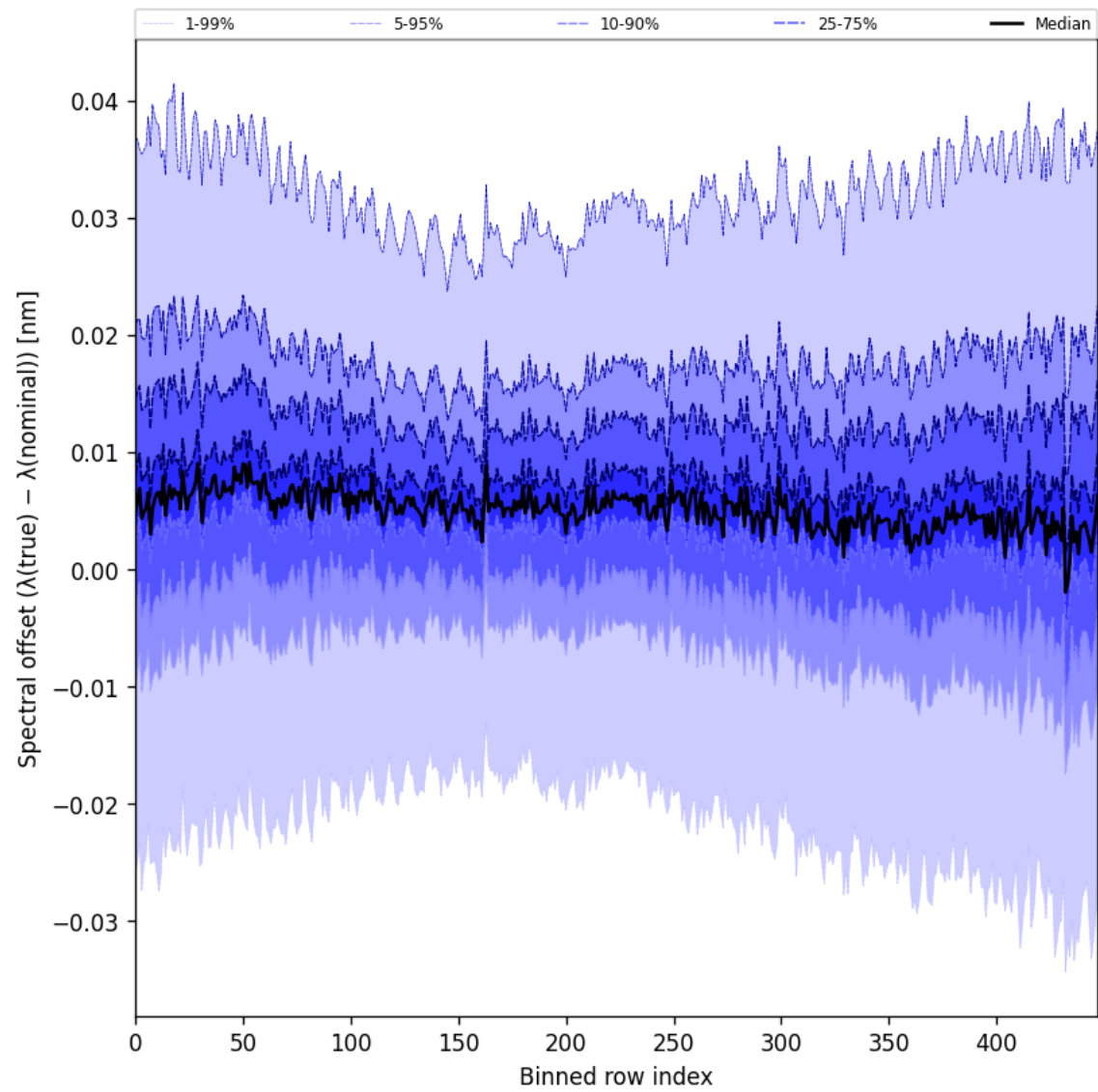
Figure 60: Along track statistics of “Spectral offset ( \lambda_{\text{true}} - \lambda_{\text{nominal}} )” for 2025-10-20 to 2025-10-20
