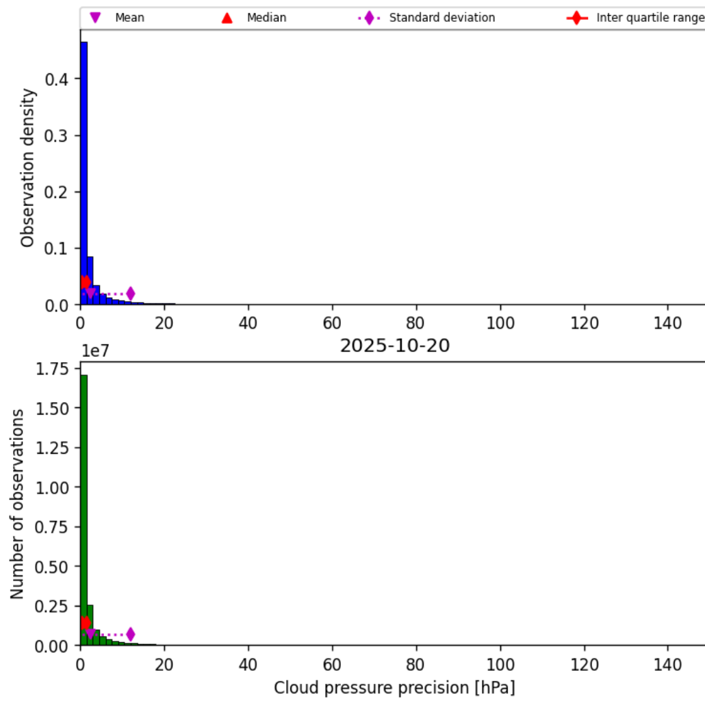
Figure 29: Histogram of “Cloud pressure precision” for 2025-10-20 to 2025-10-20
