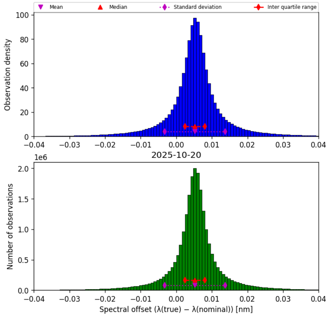
Figure 43: Histogram of “Spectral offset ( \lambda_{\text{true}} - \lambda_{\text{nominal}} )” for 2025-10-20 to 2025-10-20
