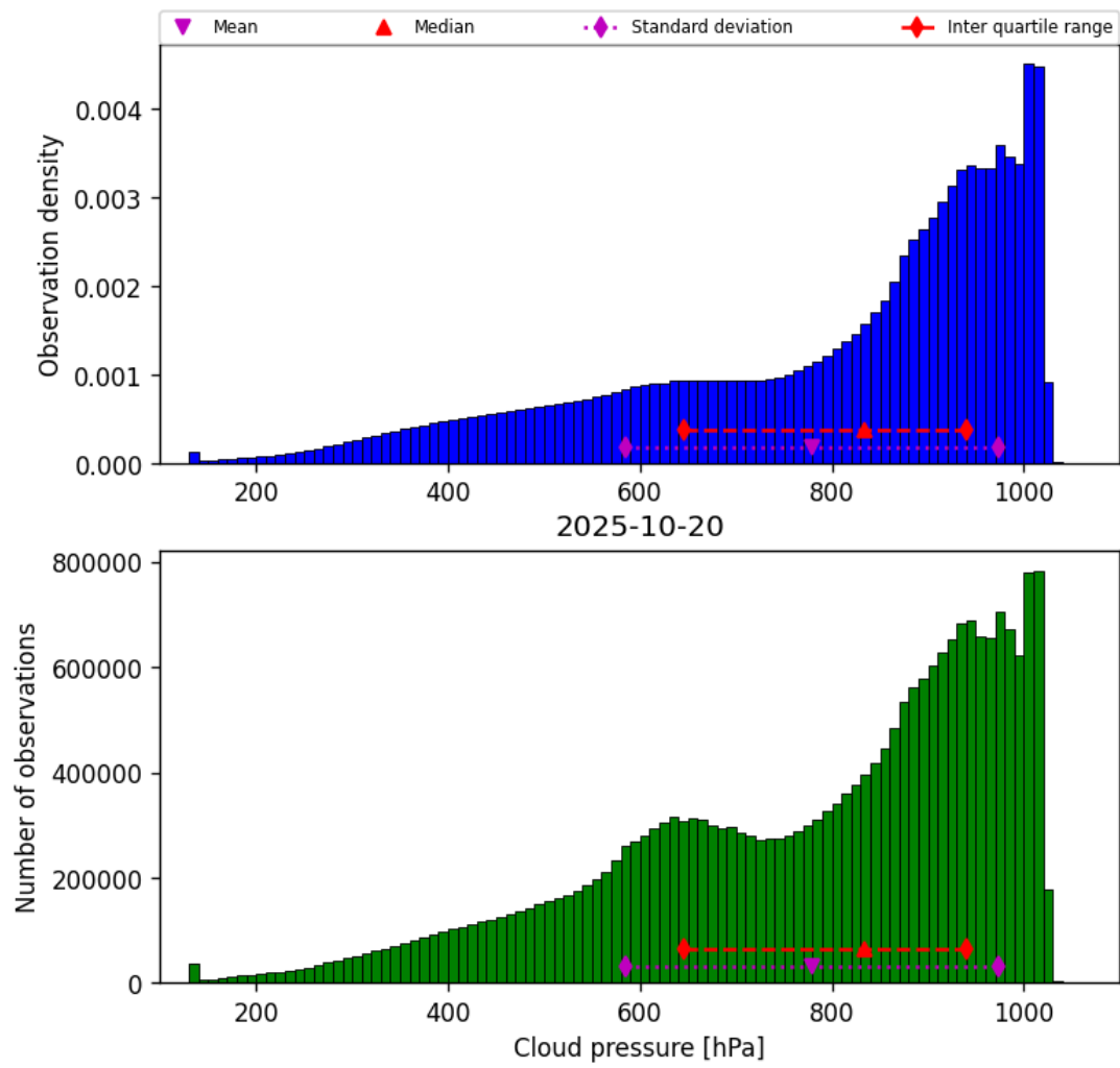
Figure 28: Histogram of “Cloud pressure” for 2025-10-20 to 2025-10-20
