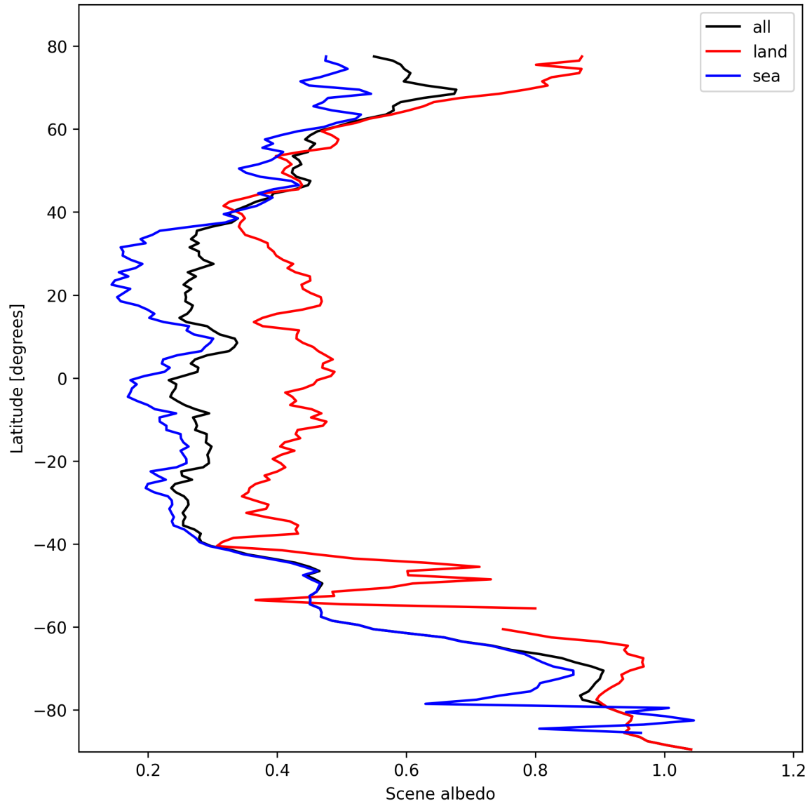
Figure 15: Zonal average of “Scene albedo” for 2025-10-20 to 2025-10-20.
