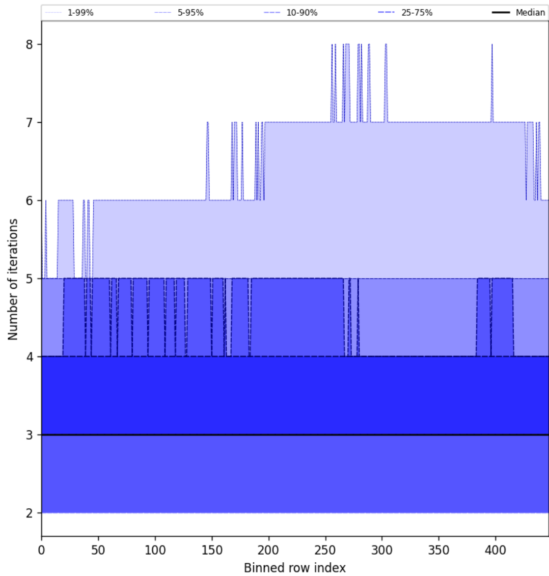
Figure 54: Along track statistics of “Number of iterations” for 2025-10-20 to 2025-10-20
