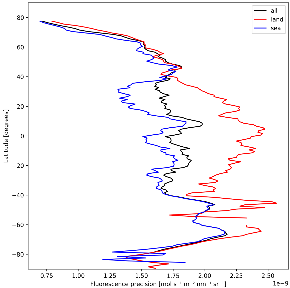
Figure 22: Zonal average of “Fluorescence precision” for 2025-10-20 to 2025-10-20.
