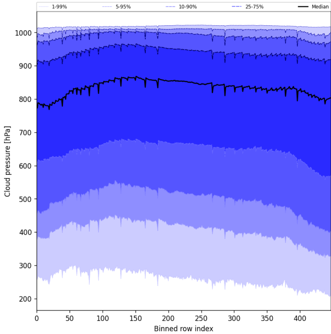
Figure 45: Along track statistics of “Cloud pressure” for 2025-10-20 to 2025-10-20
