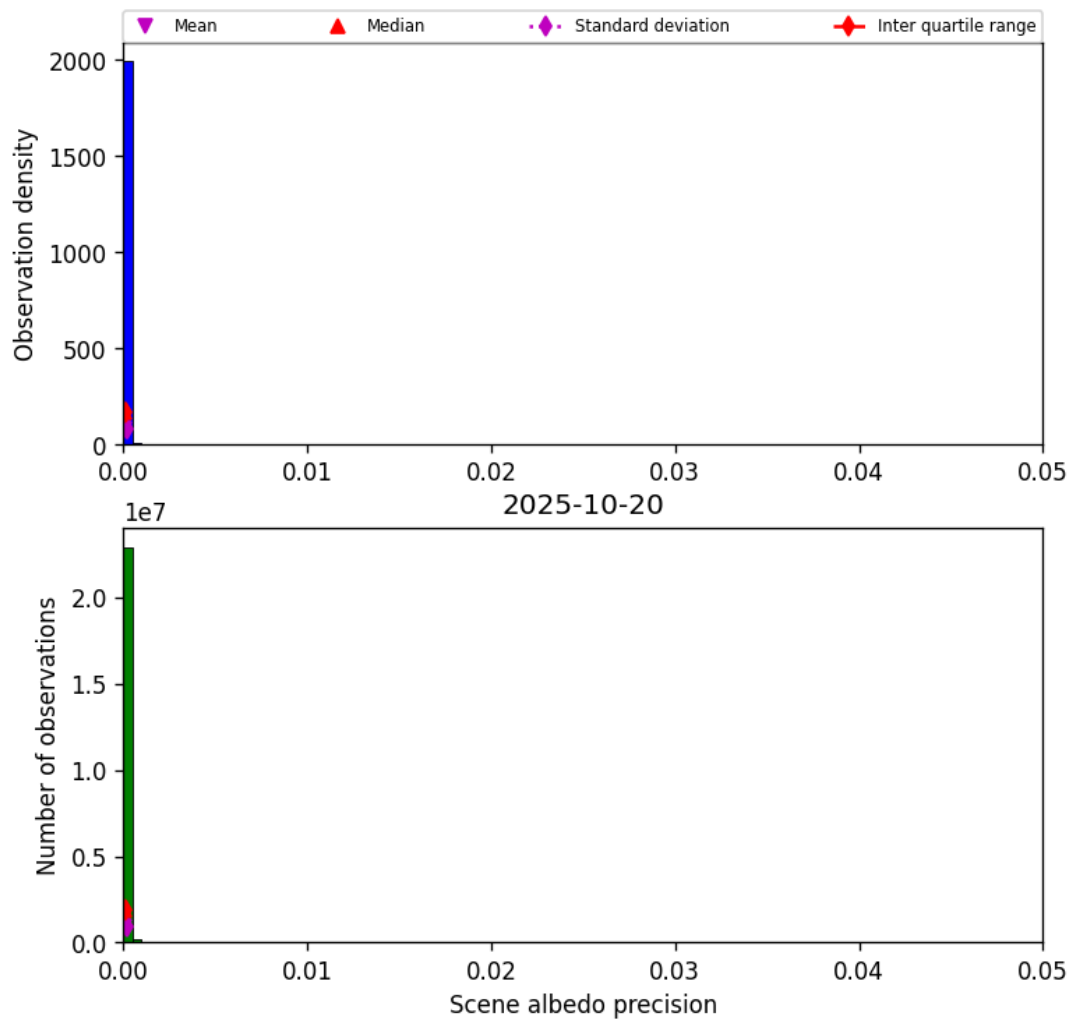
Figure 33: Histogram of “Scene albedo precision” for 2025-10-20 to 2025-10-20
