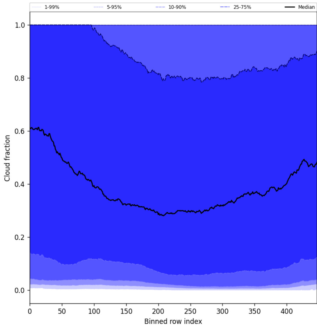
Figure 47: Along track statistics of “Cloud fraction” for 2025-10-20 to 2025-10-20
