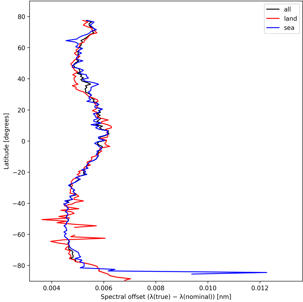
Figure 26: Zonal average of “Spectral offset ( \lambda_{\text{true}} - \lambda_{\text{nominal}} )” for 2025-10-20 to 2025-10-20.
