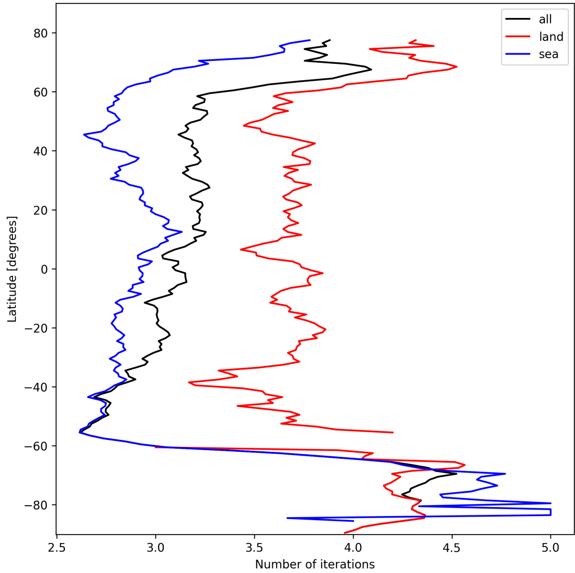
Figure 20: Zonal average of “Number of iterations” for 2025-10-20 to 2025-10-20.
