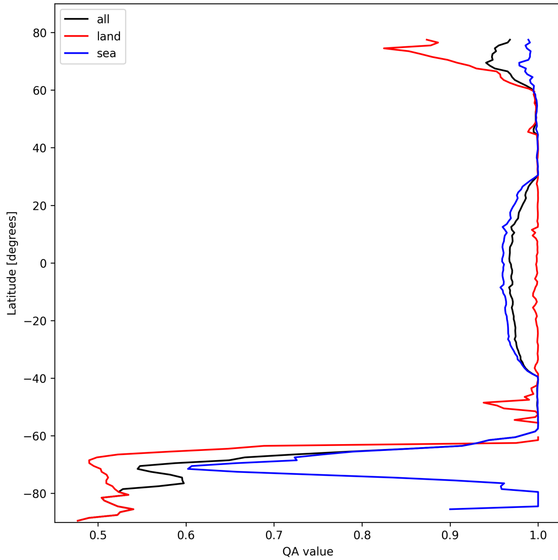
Figure 10: Zonal average of “QA value” for 2025-10-20 to 2025-10-20.
