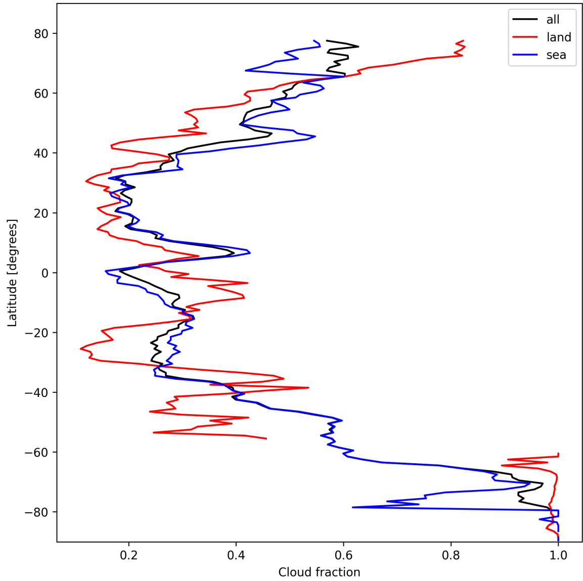
Figure 13: Zonal average of “Cloud fraction” for 2025-10-21 to 2025-10-22.
