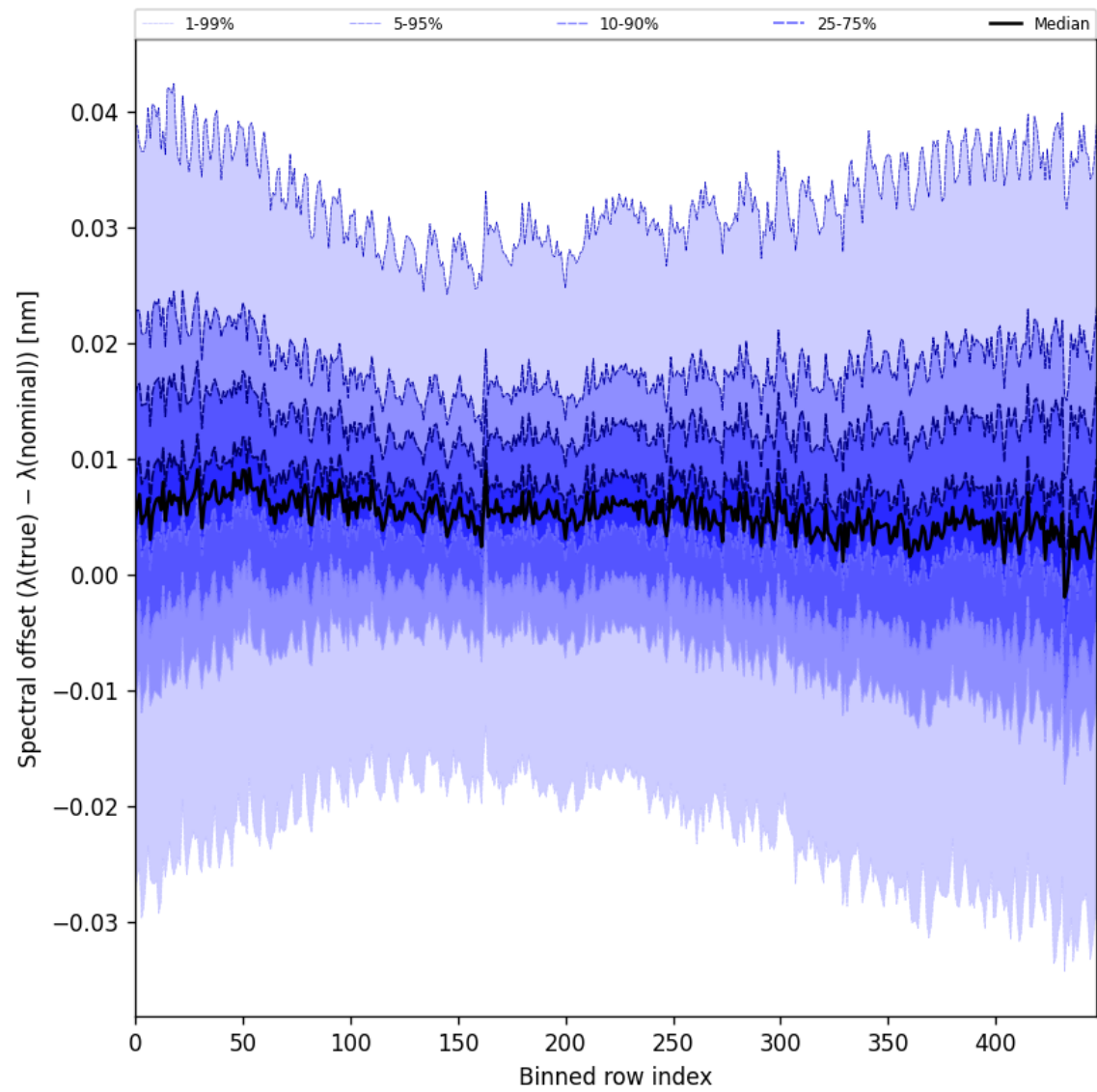
Figure 60: Along track statistics of “Spectral offset ( \lambda_{\text{true}} - \lambda_{\text{nominal}} )” for 2025-10-21 to 2025-10-22
