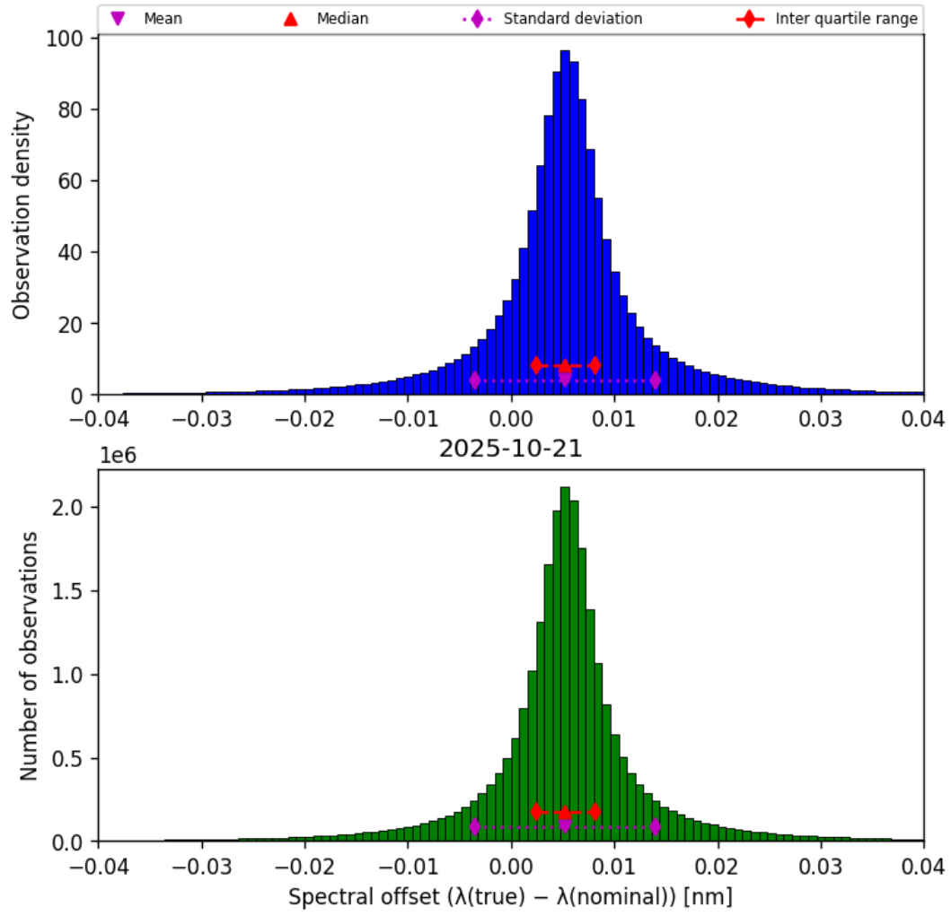
Figure 43: Histogram of “Spectral offset ( \lambda_{\text{true}} - \lambda_{\text{nominal}} )” for 2025-10-21 to 2025-10-22
