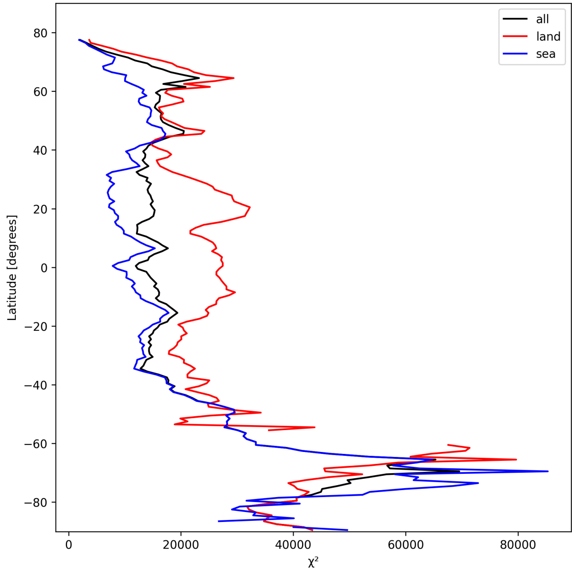
Figure 19: Zonal average of “ \chi^2 ” for 2025-10-21 to 2025-10-22.
