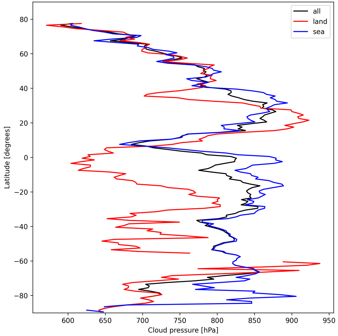
Figure 11: Zonal average of “Cloud pressure” for 2025-10-21 to 2025-10-22.
