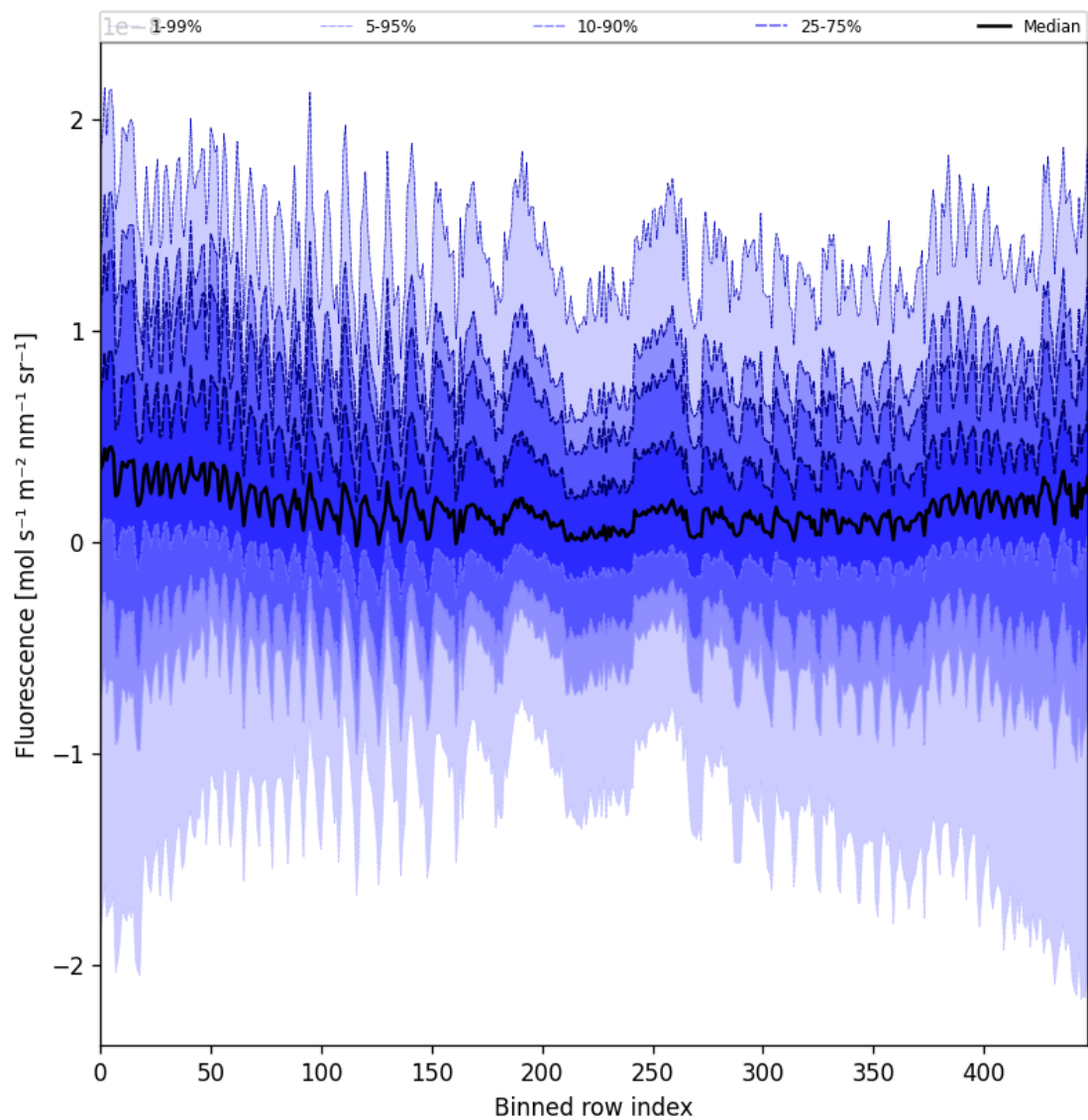
Figure 55: Along track statistics of “Fluorescence” for 2025-10-21 to 2025-10-22
