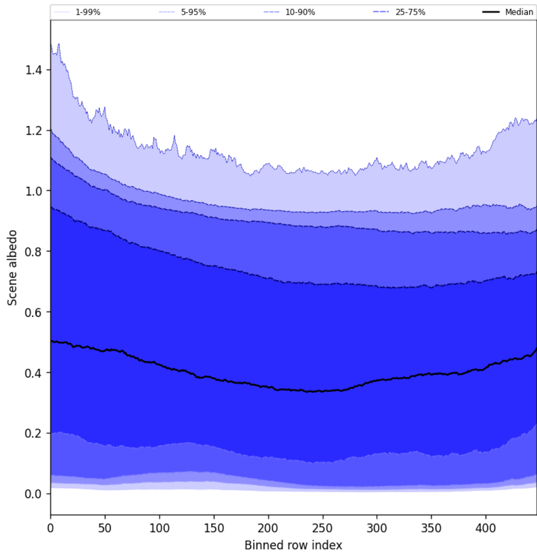
Figure 49: Along track statistics of “Scene albedo” for 2025-10-21 to 2025-10-22
