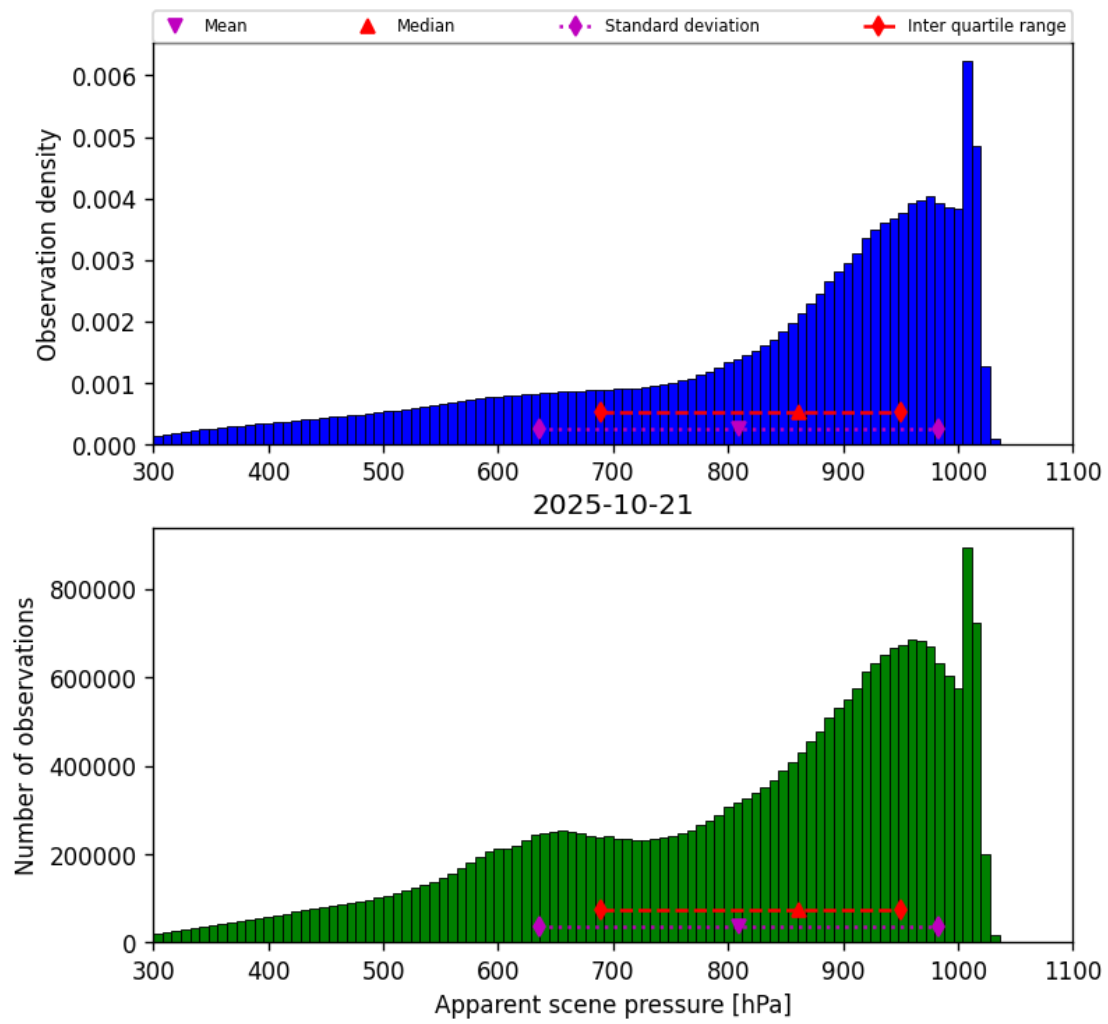
Figure 34: Histogram of “Apparent scene pressure” for 2025-10-21 to 2025-10-22
