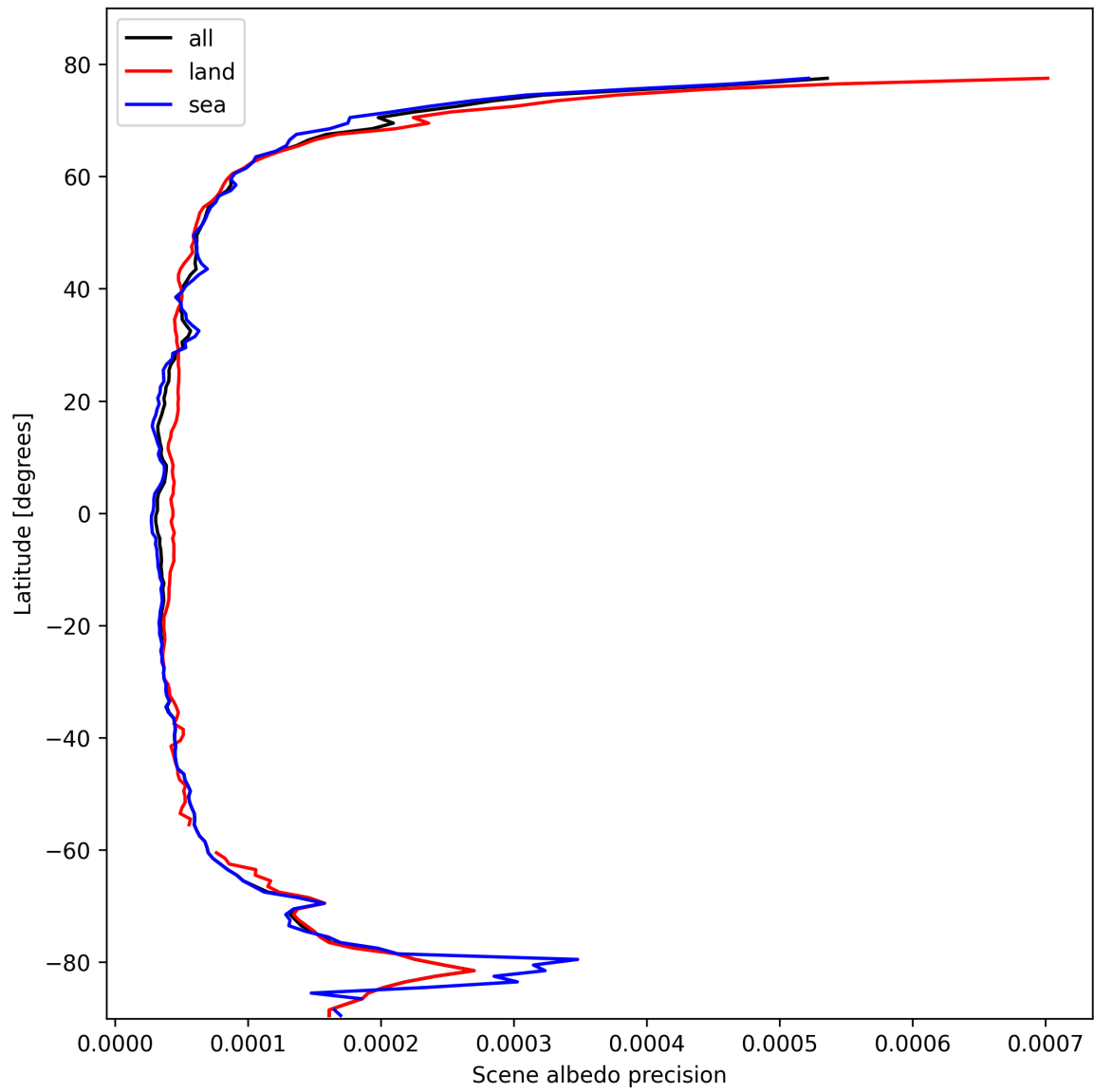
Figure 16: Zonal average of “Scene albedo precision” for 2025-10-21 to 2025-10-22.
