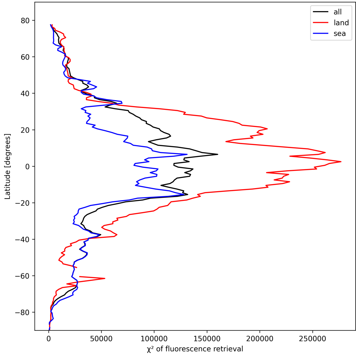
Figure 23: Zonal average of “ \chi^2 of fluorescence retrieval” for 2025-10-21 to 2025-10-22.
