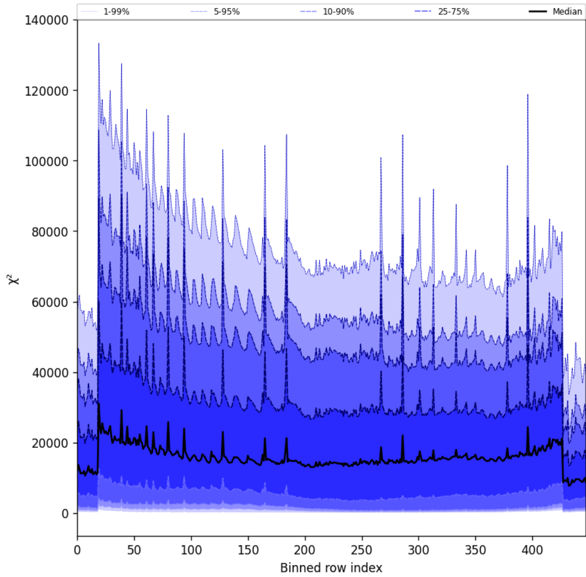
Figure 53: Along track statistics of “ \chi^2 ” for 2025-10-21 to 2025-10-22
