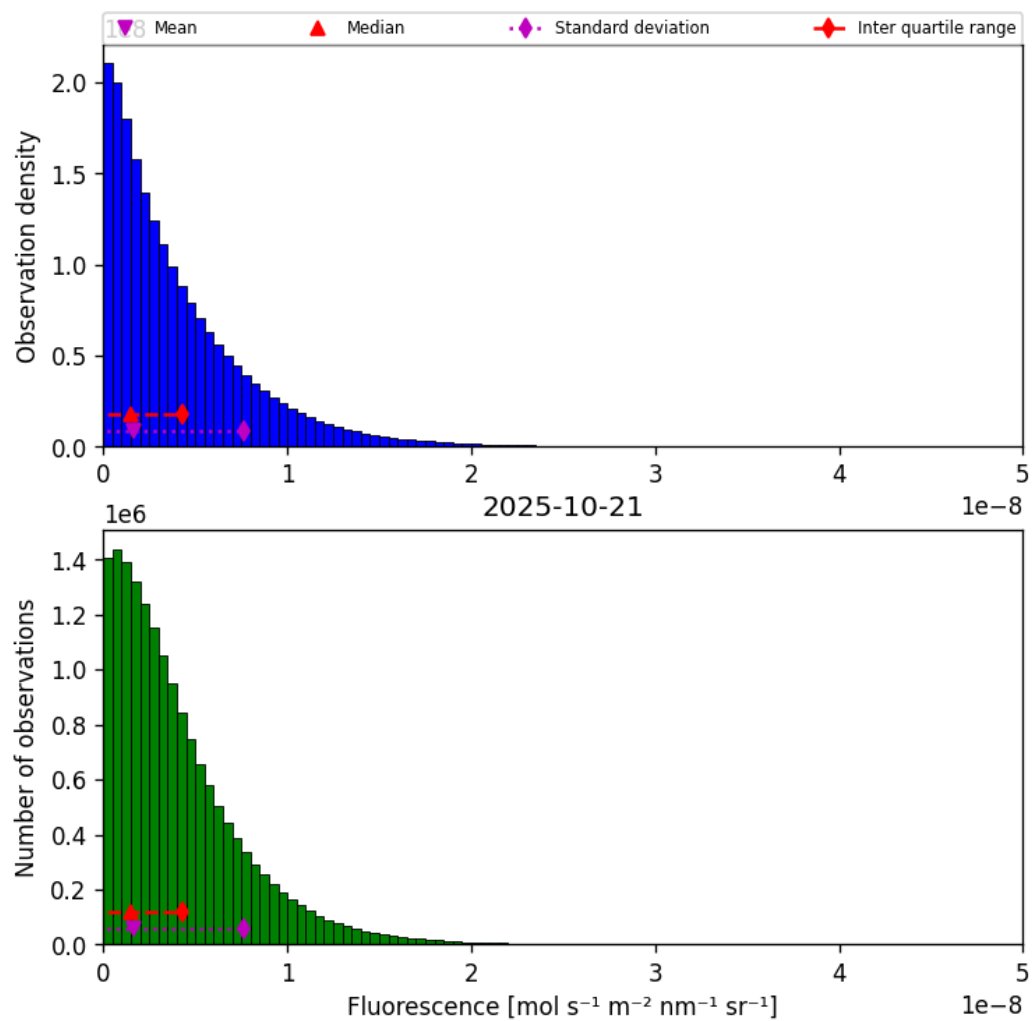
Figure 38: Histogram of “Fluorescence” for 2025-10-21 to 2025-10-22
