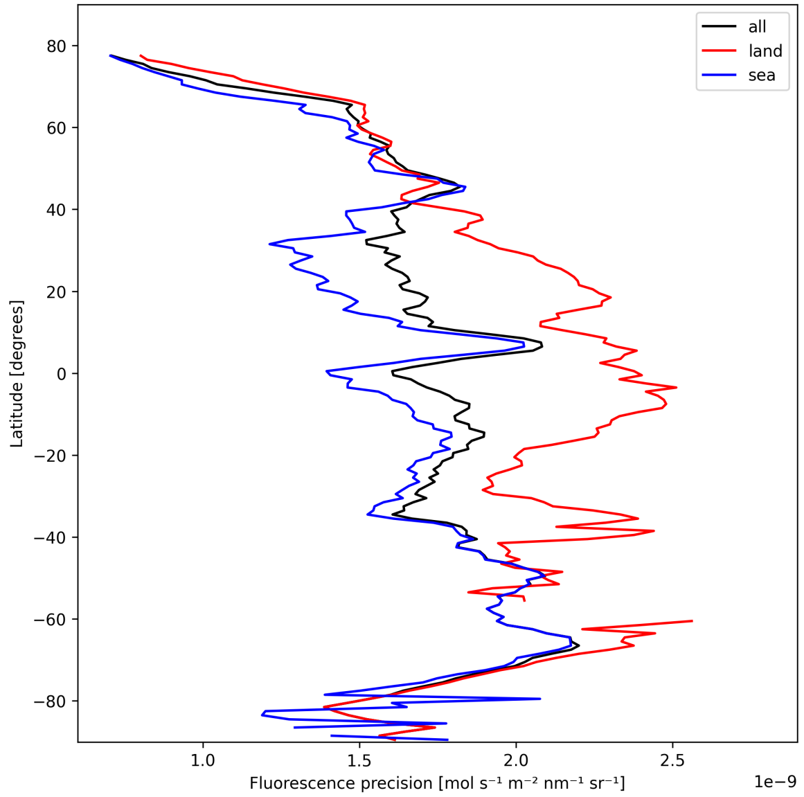
Figure 22: Zonal average of “Fluorescence precision” for 2025-10-21 to 2025-10-22.
