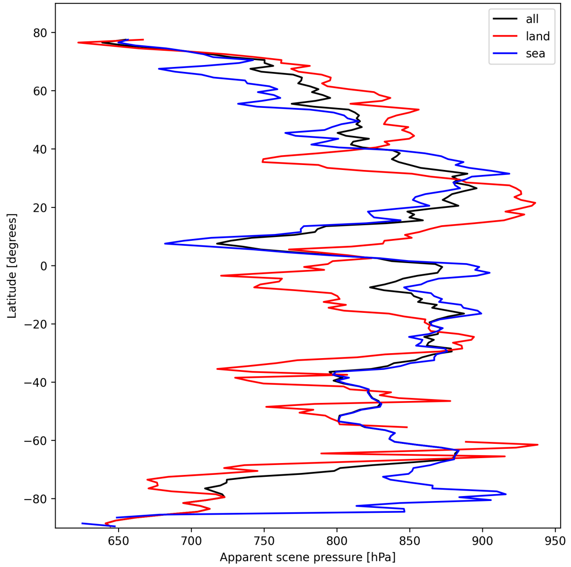
Figure 17: Zonal average of “Apparent scene pressure” for 2025-10-21 to 2025-10-22.
