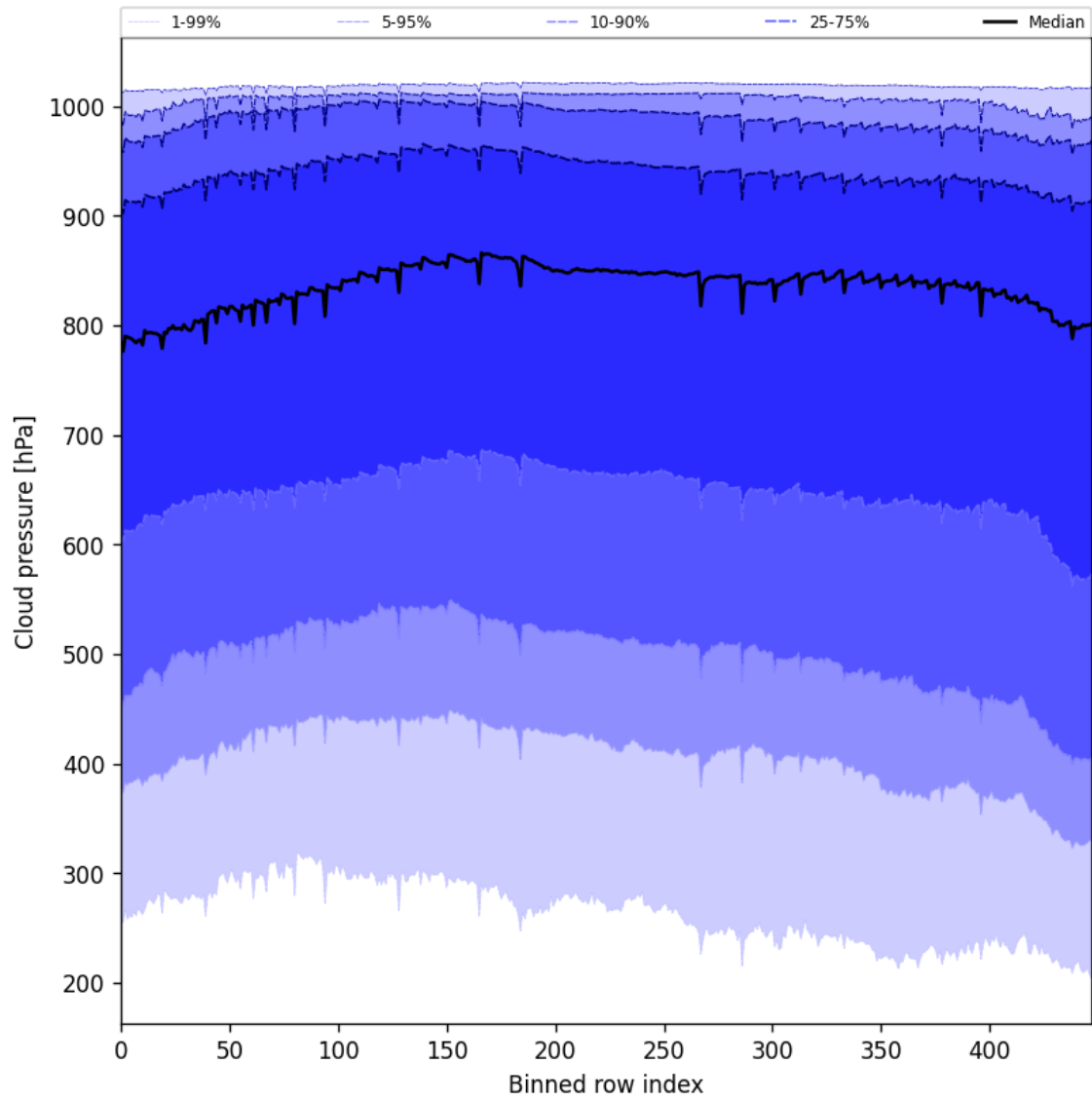
Figure 45: Along track statistics of “Cloud pressure” for 2025-10-21 to 2025-10-22
