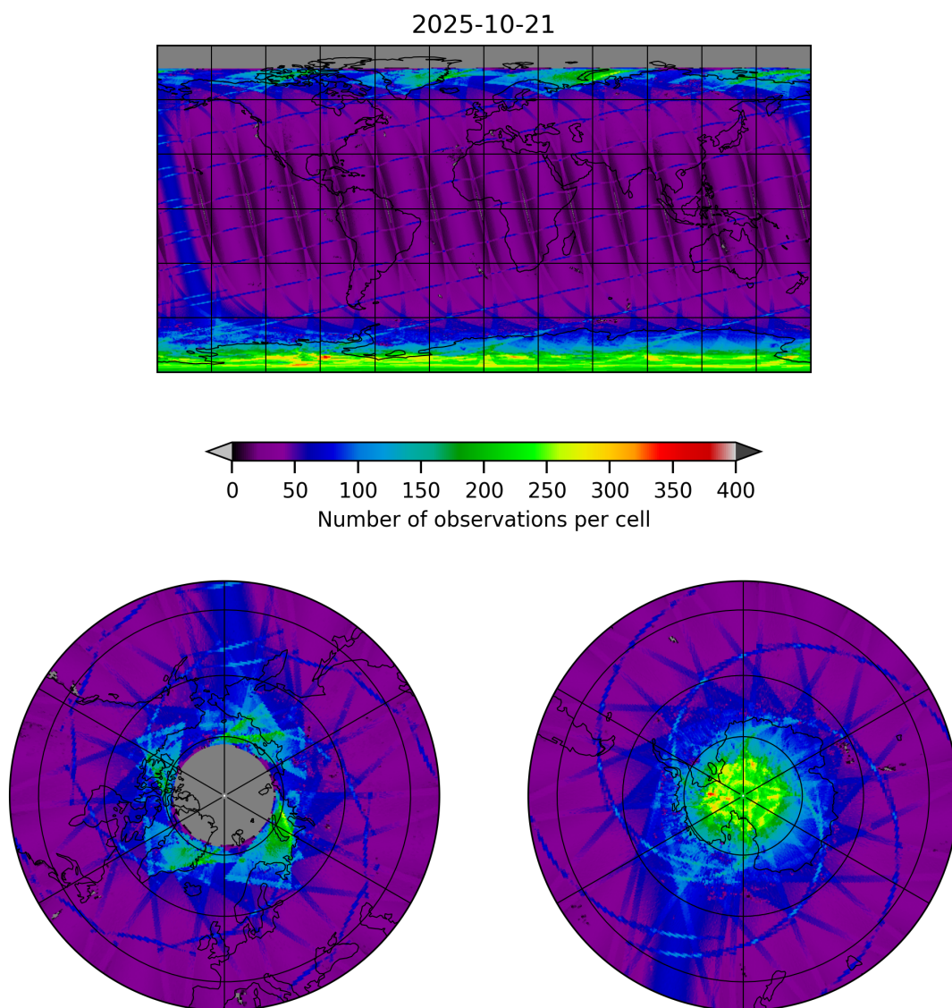
Figure 9: Map of the number of observations for 2025-10-21 to 2025-10-22
