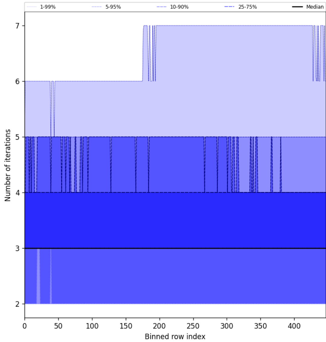
Figure 54: Along track statistics of “Number of iterations” for 2025-10-21 to 2025-10-22
