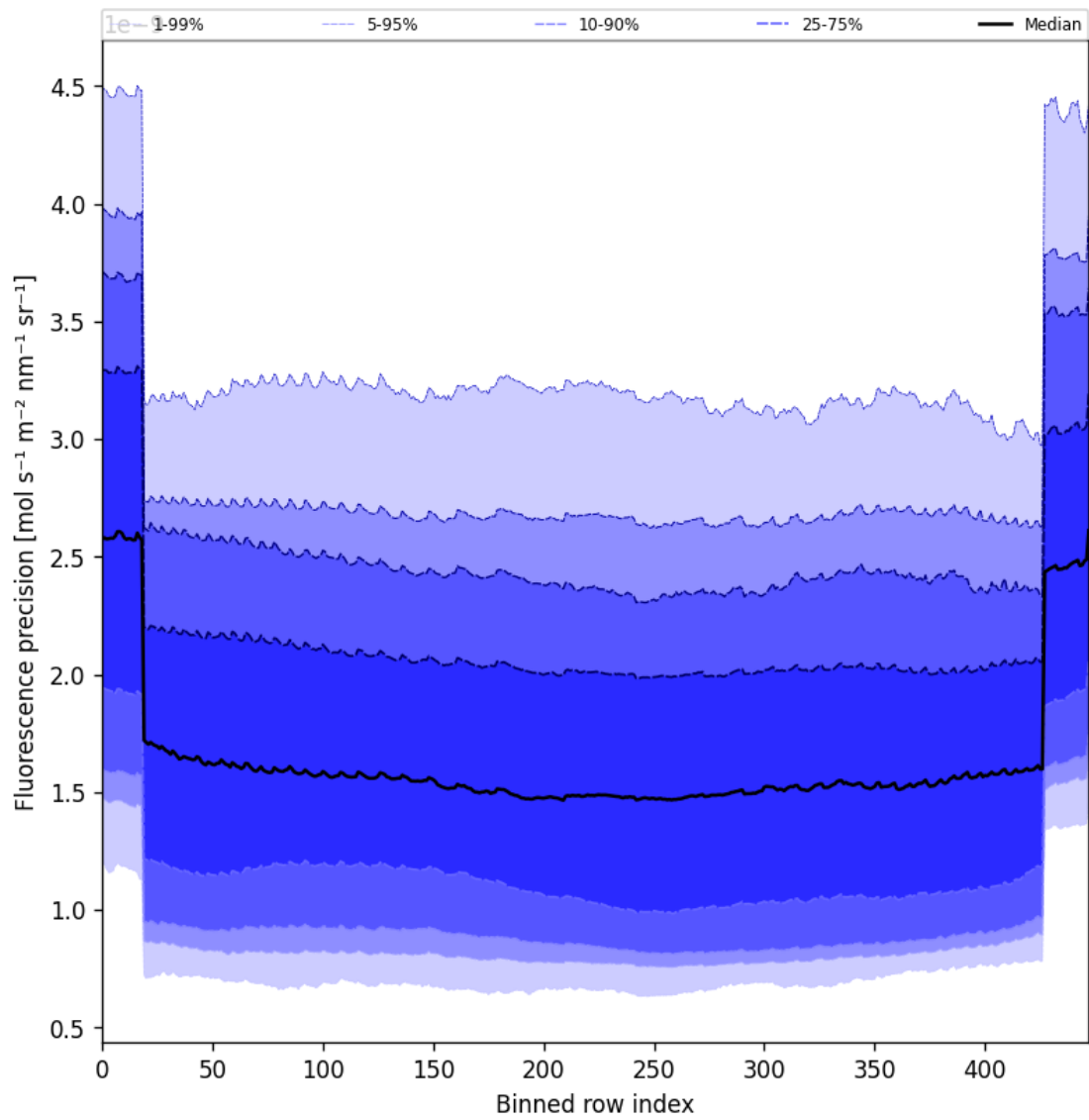
Figure 56: Along track statistics of “Fluorescence precision” for 2025-10-21 to 2025-10-22
