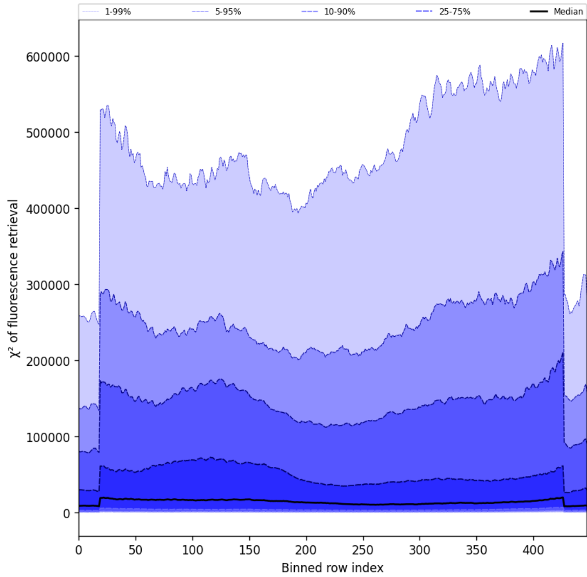
Figure 57: Along track statistics of “ \chi^2 of fluorescence retrieval” for 2025-10-21 to 2025-10-22
