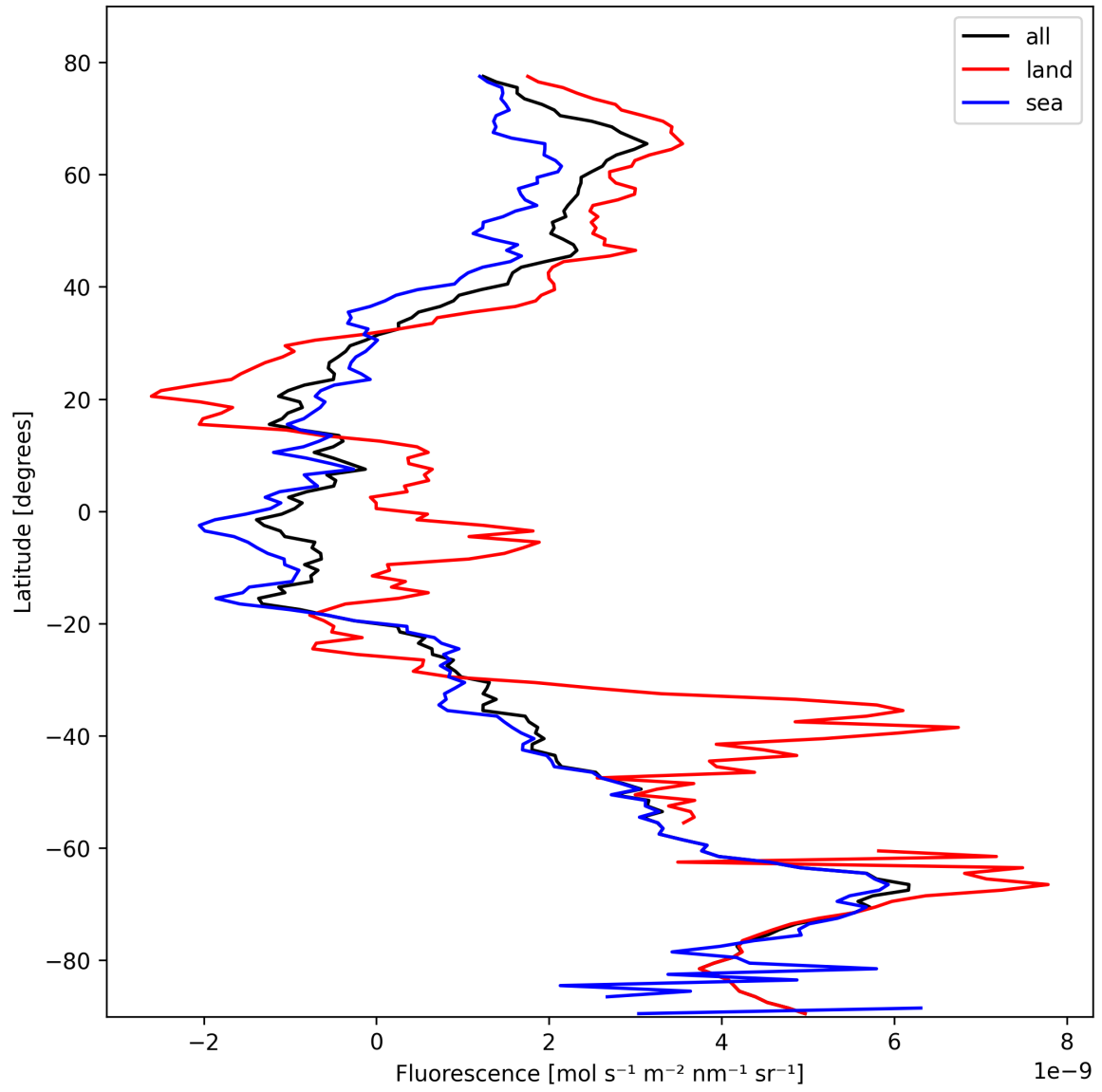
Figure 21: Zonal average of “Fluorescence” for 2025-10-21 to 2025-10-22.
