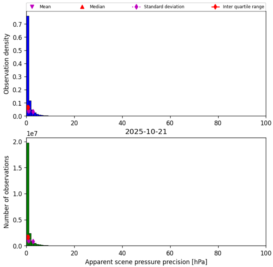
Figure 35: Histogram of “Apparent scene pressure precision” for 2025-10-21 to 2025-10-22
