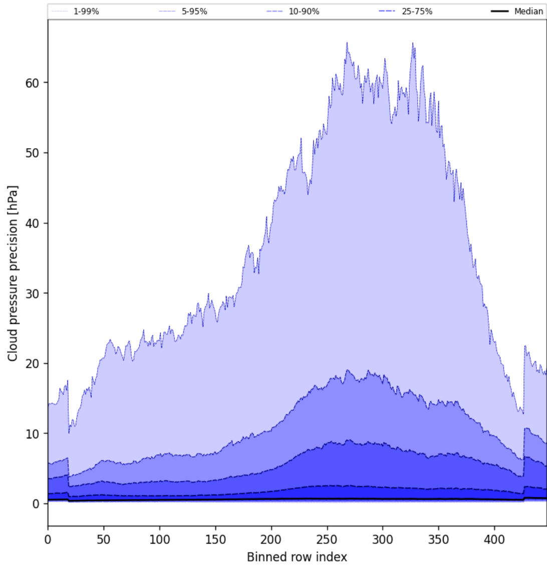
Figure 46: Along track statistics of “Cloud pressure precision” for 2025-10-21 to 2025-10-22
