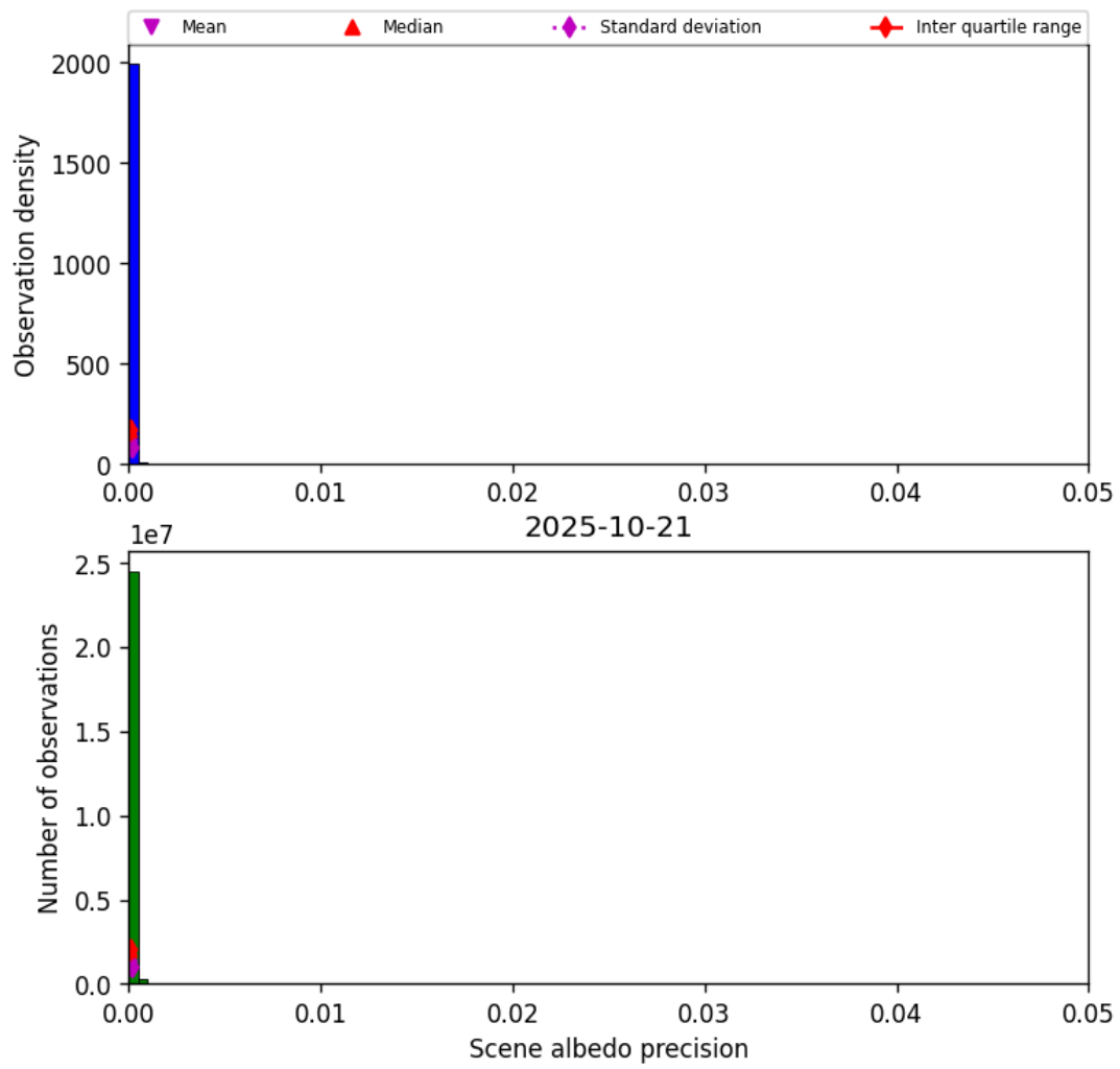
Figure 33: Histogram of “Scene albedo precision” for 2025-10-21 to 2025-10-22
