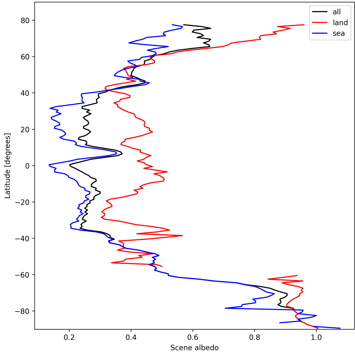
Figure 15: Zonal average of “Scene albedo” for 2025-10-21 to 2025-10-22.
