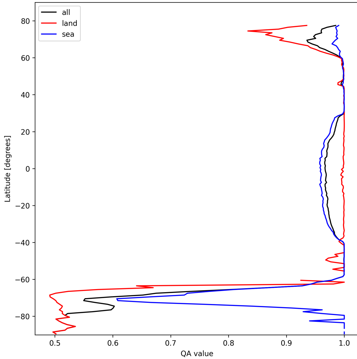
Figure 10: Zonal average of “QA value” for 2025-10-21 to 2025-10-22.
