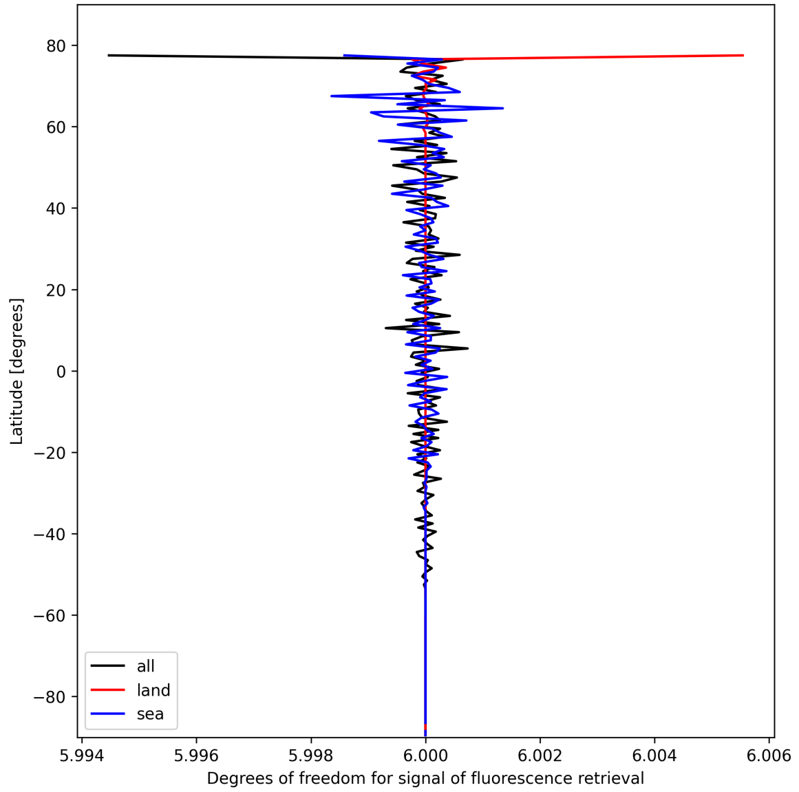
Figure 24: Zonal average of “Degrees of freedom for signal of fluorescence retrieval” for 2025-10-21 to 2025-10-22.
