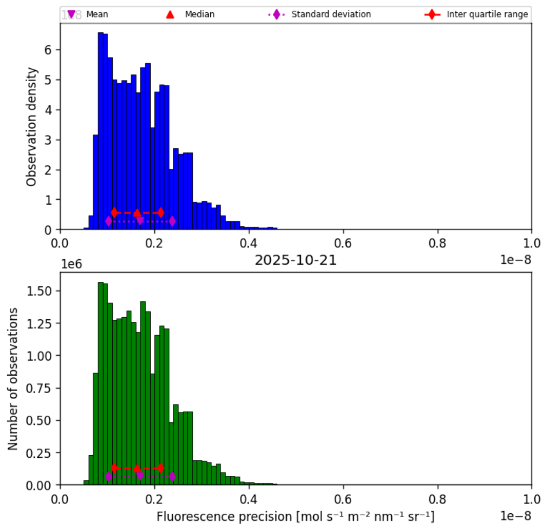
Figure 39: Histogram of “Fluorescence precision” for 2025-10-21 to 2025-10-22
