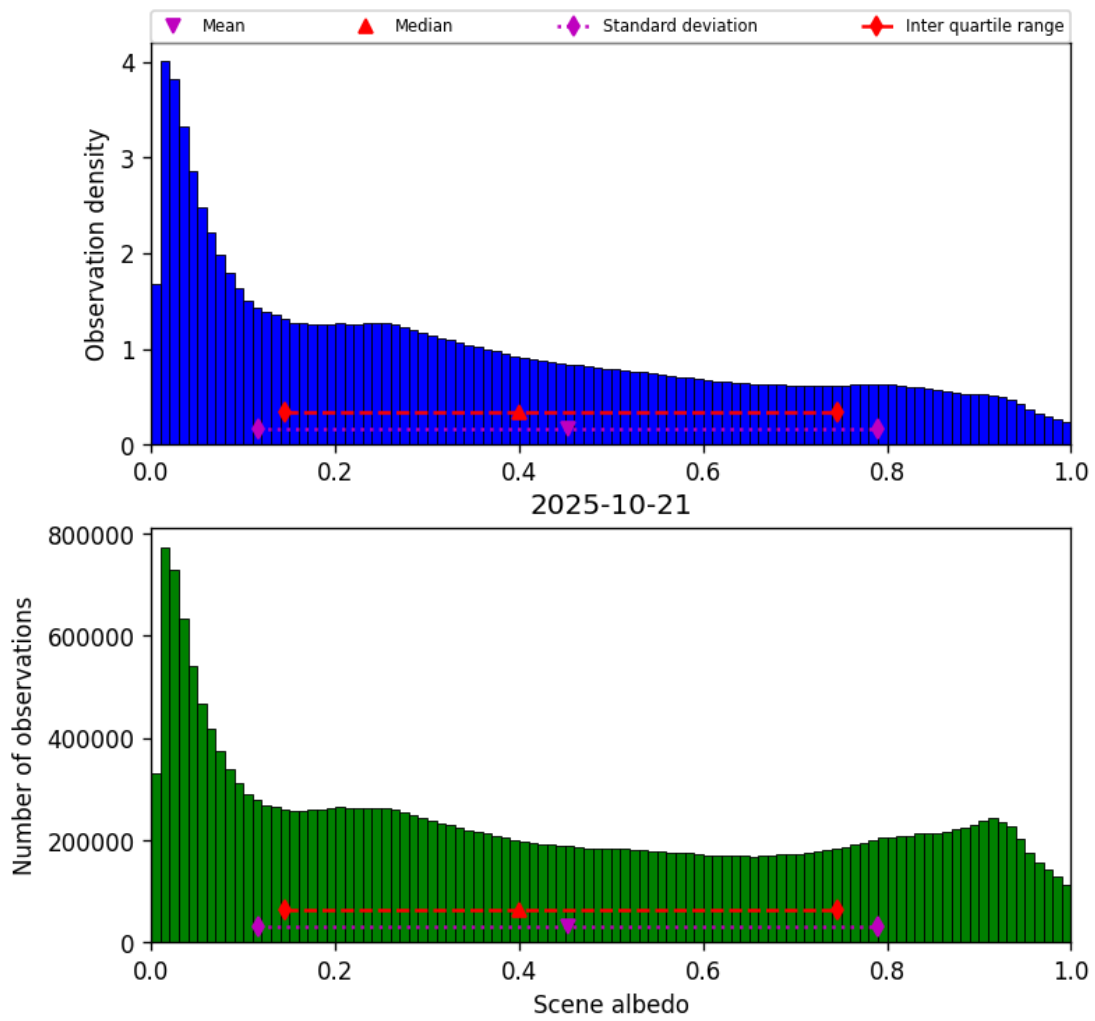
Figure 32: Histogram of “Scene albedo” for 2025-10-21 to 2025-10-22
