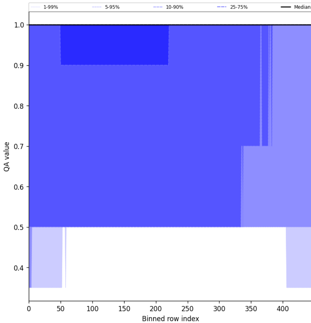
Figure 44: Along track statistics of “QA value” for 2025-10-21 to 2025-10-22
