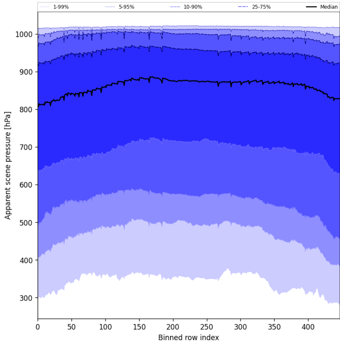
Figure 51: Along track statistics of “Apparent scene pressure” for 2025-10-21 to 2025-10-22
