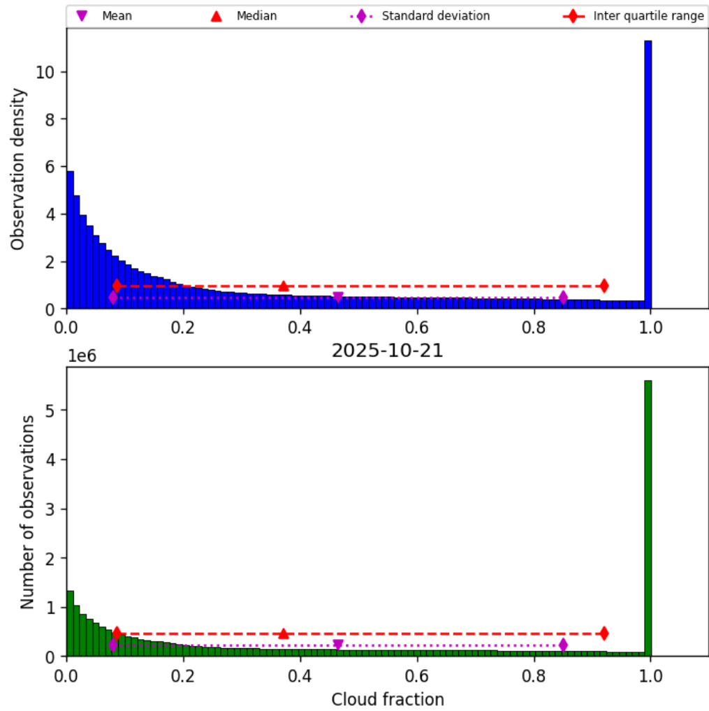
Figure 30: Histogram of “Cloud fraction” for 2025-10-21 to 2025-10-22
