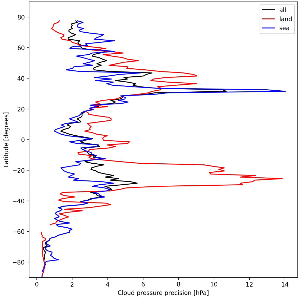
Figure 12: Zonal average of “Cloud pressure precision” for 2025-10-21 to 2025-10-22.
