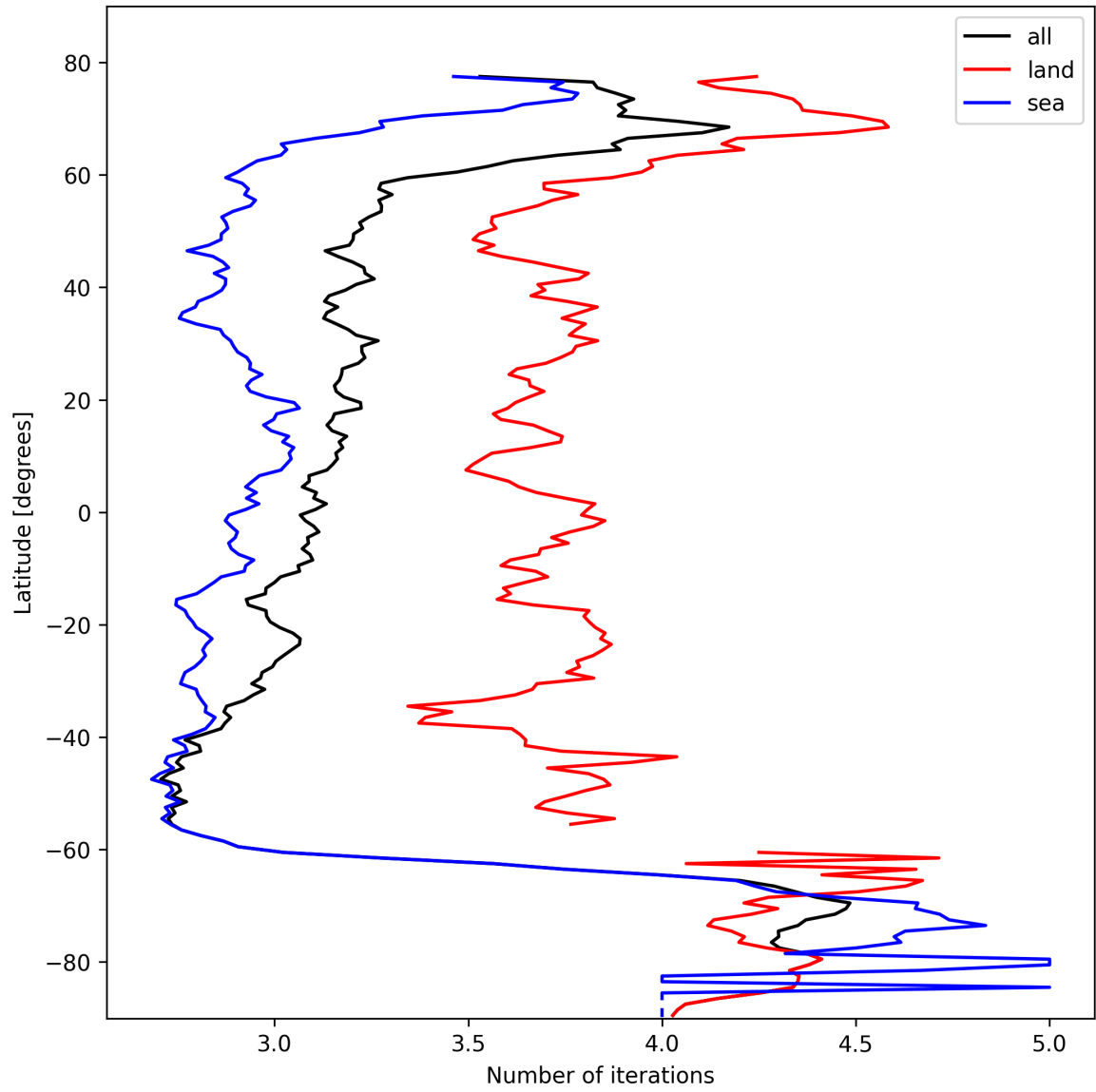
Figure 20: Zonal average of “Number of iterations” for 2025-10-21 to 2025-10-22.
