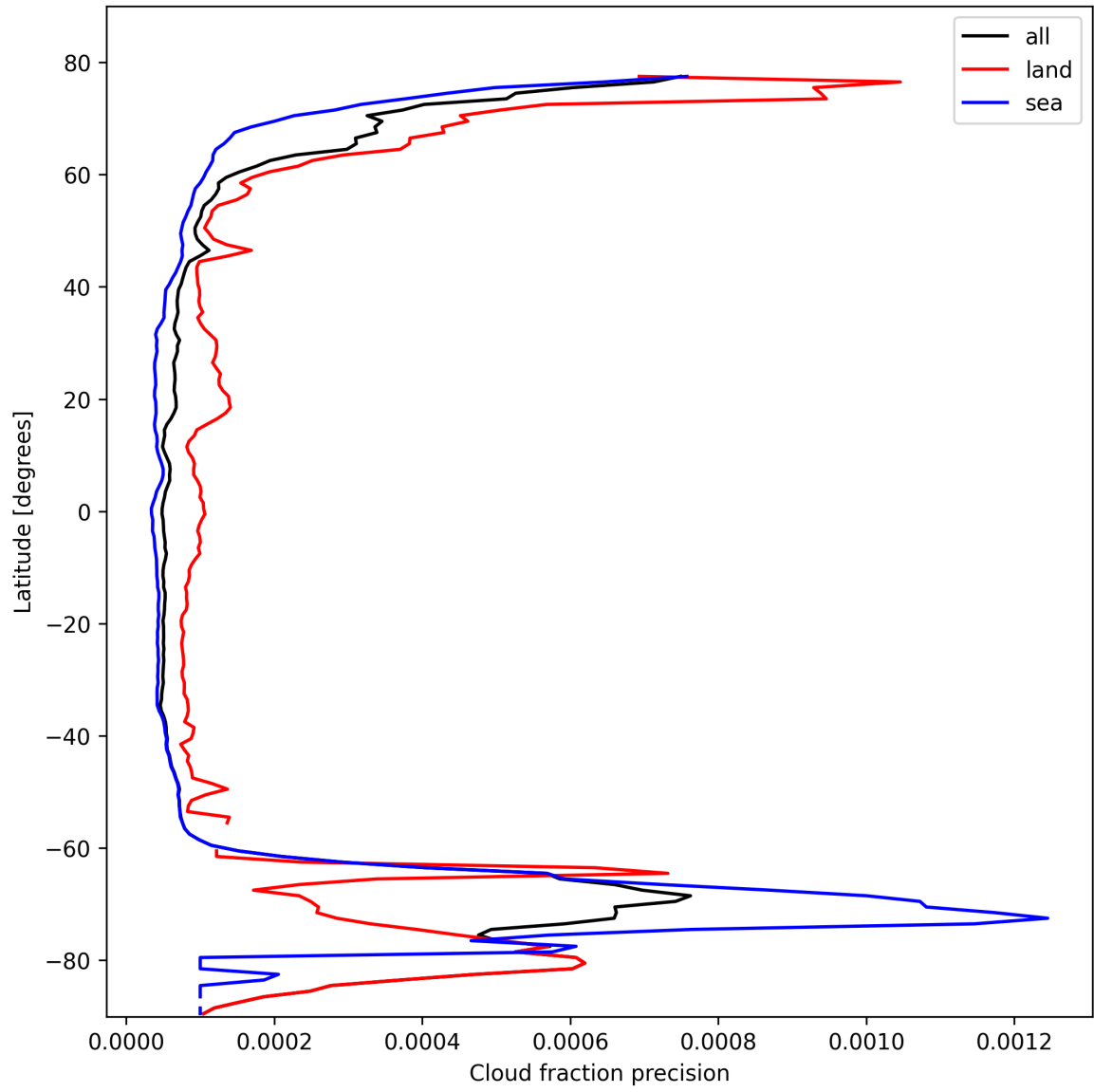
Figure 14: Zonal average of “Cloud fraction precision” for 2025-10-21 to 2025-10-22.
