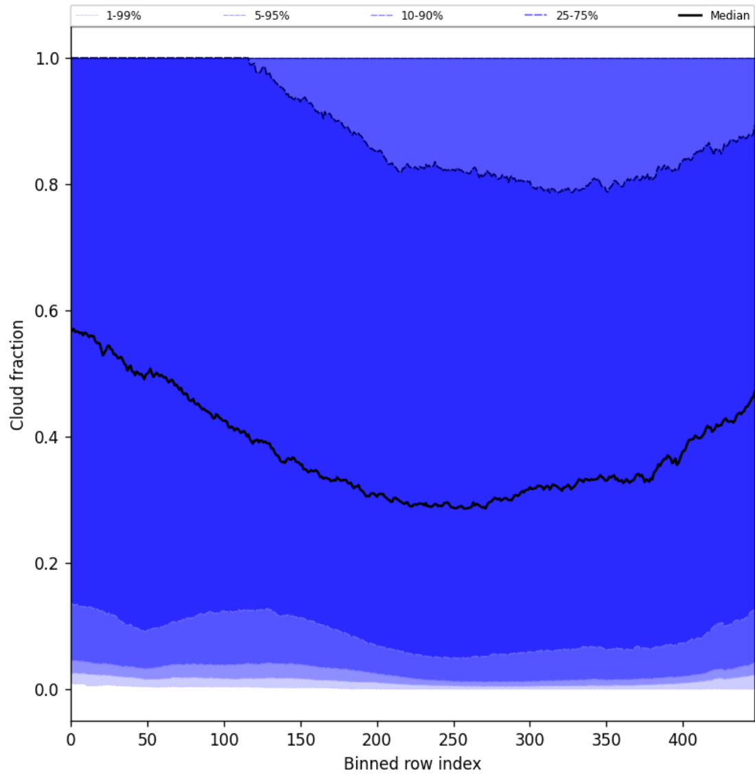
Figure 47: Along track statistics of “Cloud fraction” for 2025-10-21 to 2025-10-22
