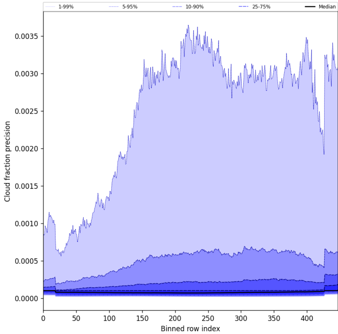
Figure 48: Along track statistics of “Cloud fraction precision” for 2025-10-21 to 2025-10-22
