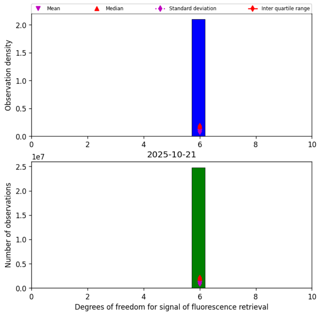
Figure 41: Histogram of “Degrees of freedom for signal of fluorescence retrieval” for 2025-10-21 to 2025-10-22
