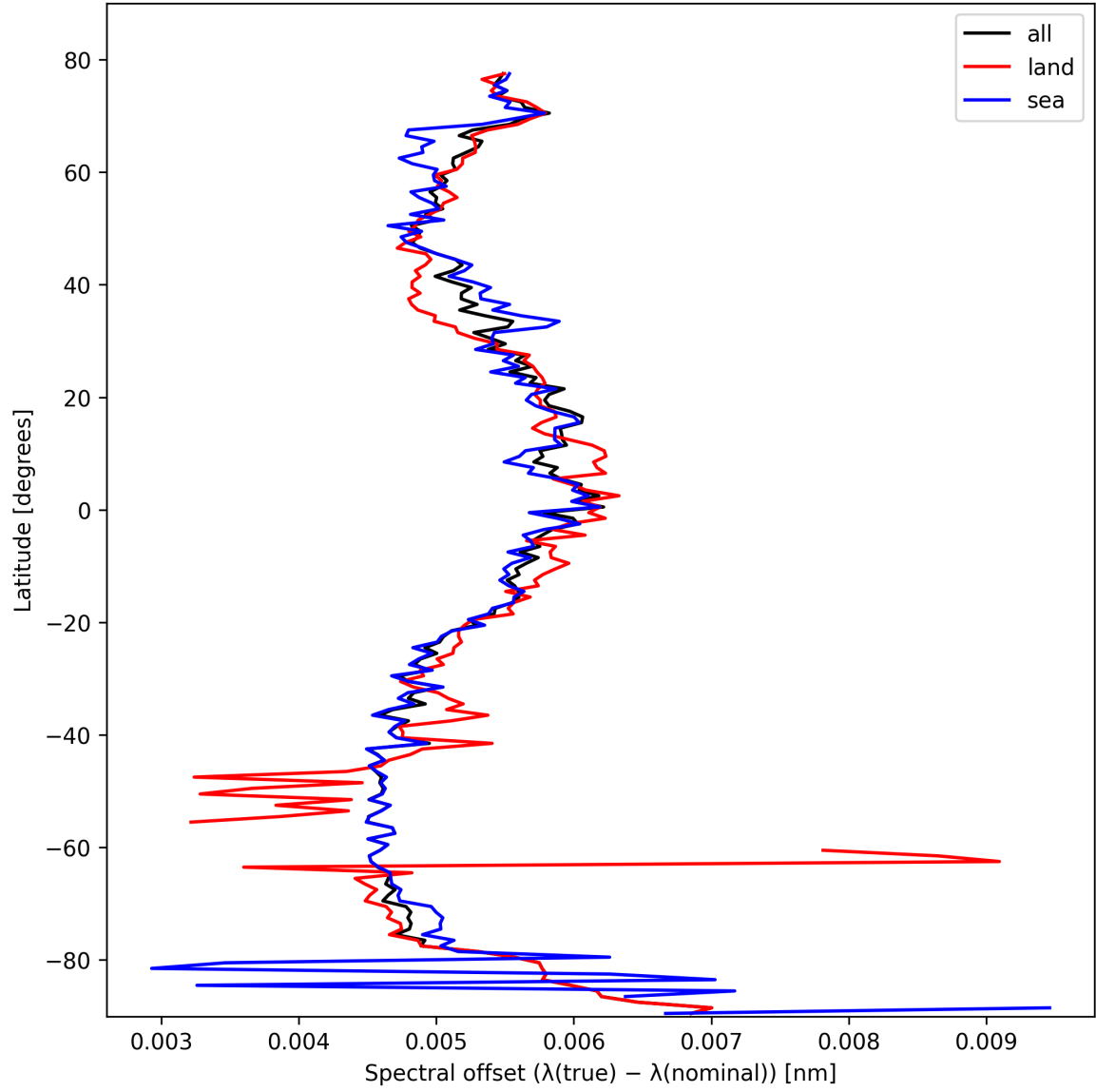
Figure 26: Zonal average of “Spectral offset ( \lambda_{\text{true}} - \lambda_{\text{nominal}} )” for 2025-10-21 to 2025-10-22.
