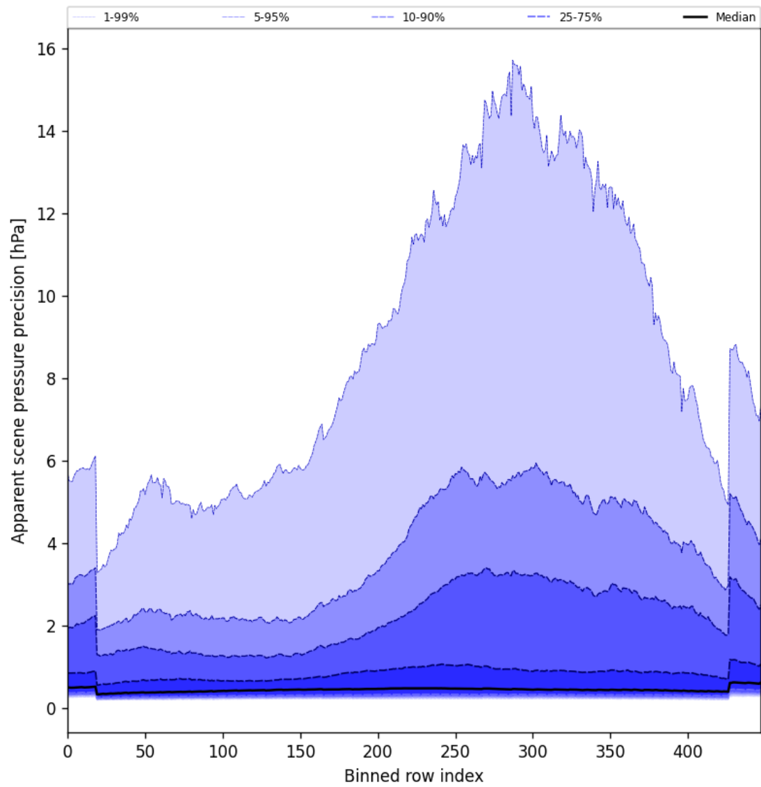
Figure 52: Along track statistics of “Apparent scene pressure precision” for 2025-10-21 to 2025-10-22
