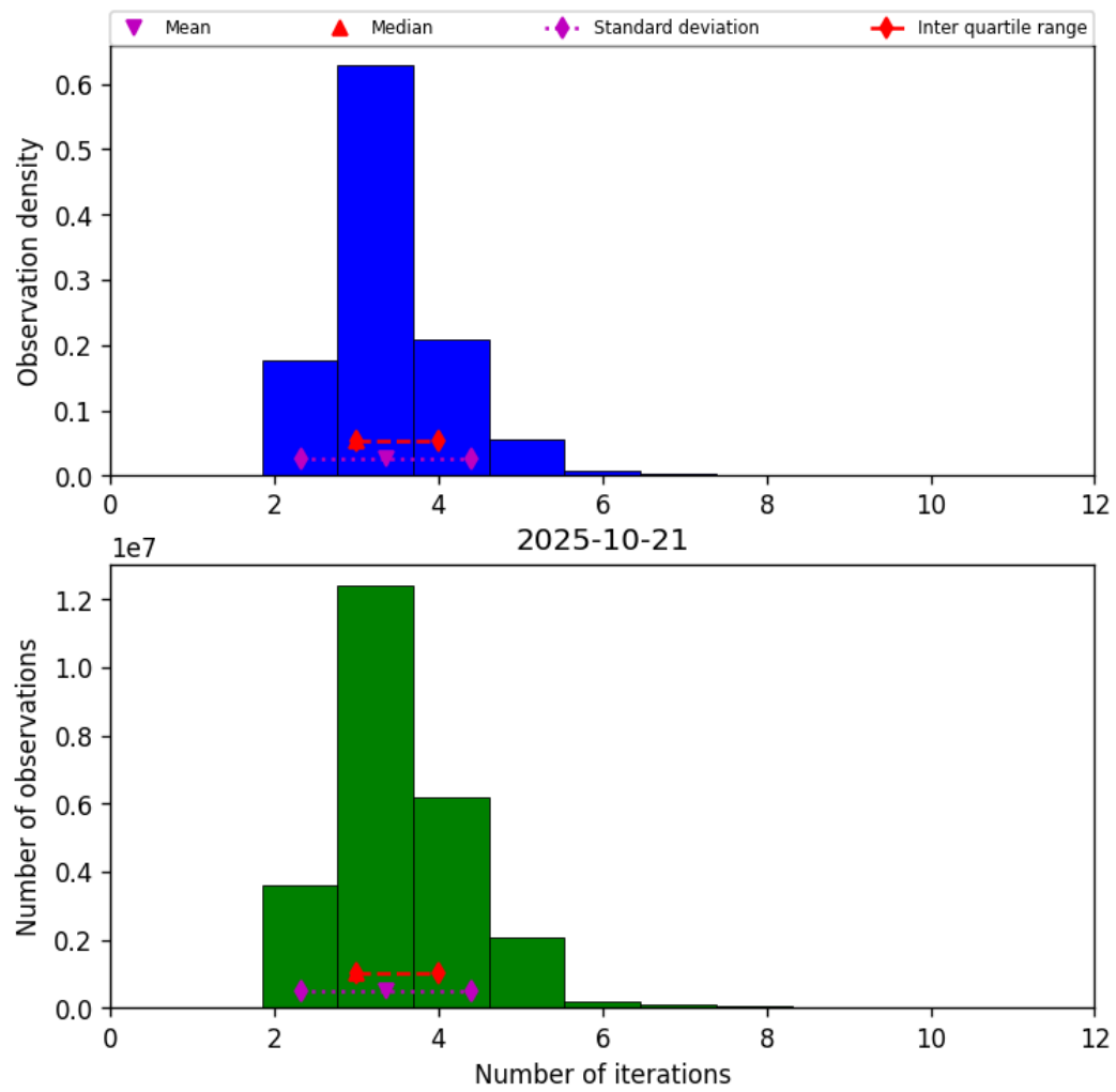
Figure 37: Histogram of “Number of iterations” for 2025-10-21 to 2025-10-22
