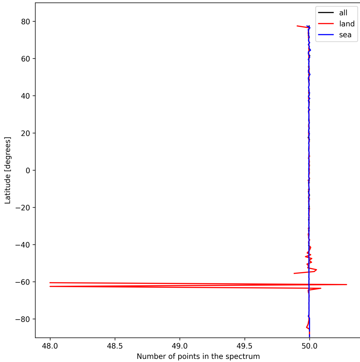
Figure 25: Zonal average of “Number of points in the spectrum” for 2025-10-21 to 2025-10-22.
