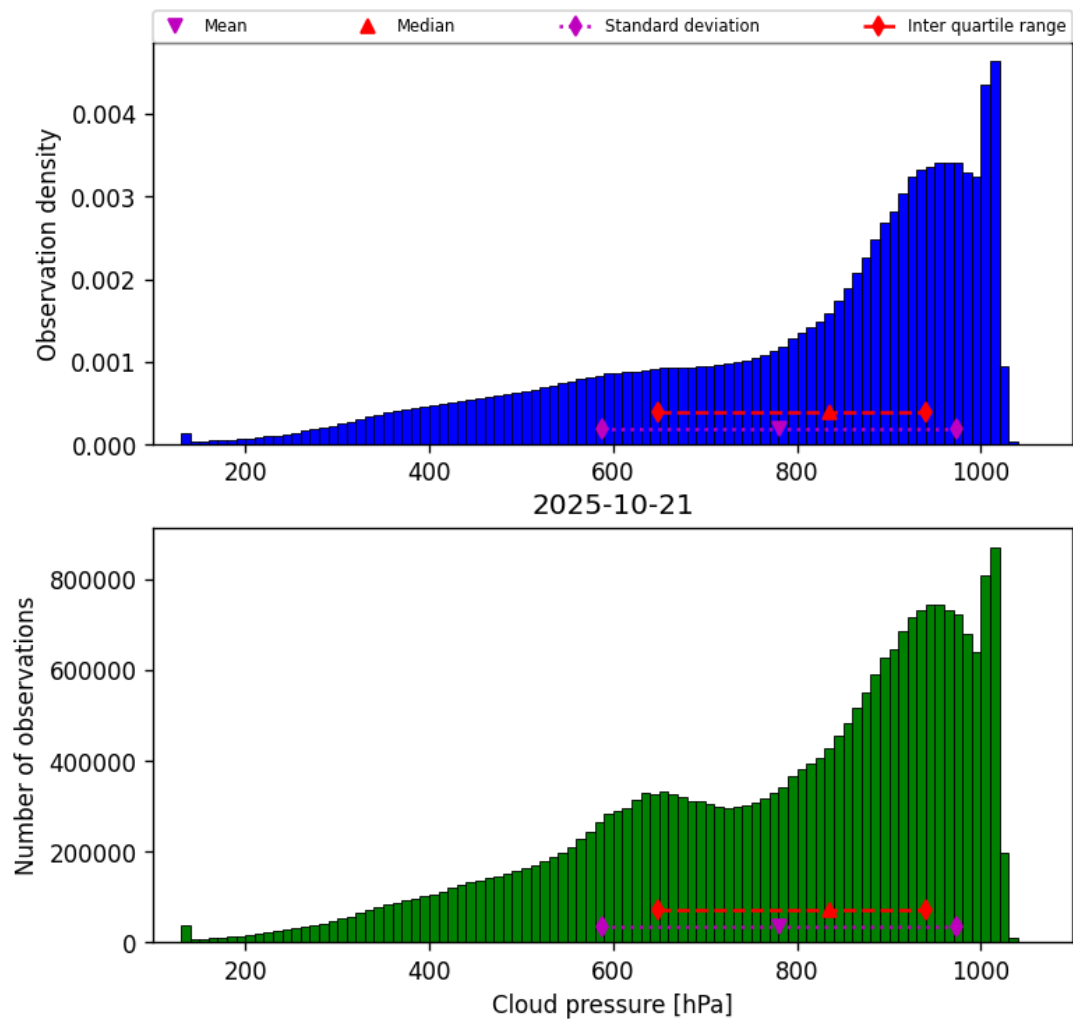
Figure 28: Histogram of “Cloud pressure” for 2025-10-21 to 2025-10-22
