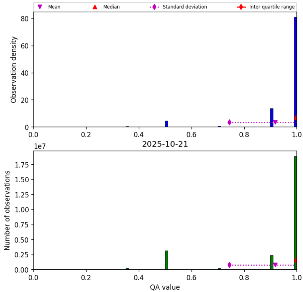
Figure 27: Histogram of “QA value” for 2025-10-21 to 2025-10-22
