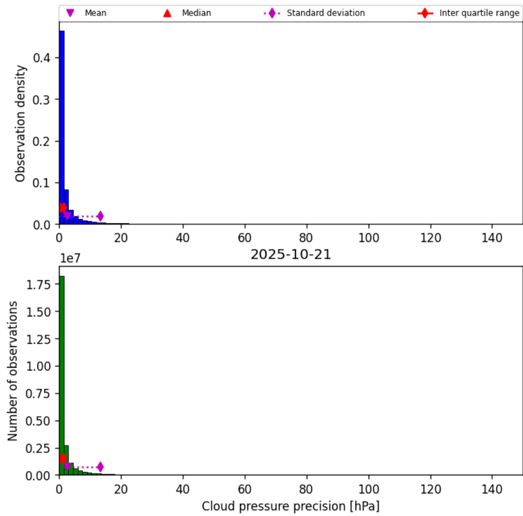
Figure 29: Histogram of “Cloud pressure precision” for 2025-10-21 to 2025-10-22
