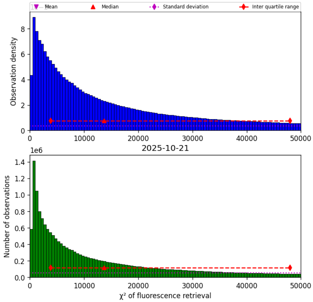
Figure 40: Histogram of “ \chi^2 of fluorescence retrieval” for 2025-10-21 to 2025-10-22
