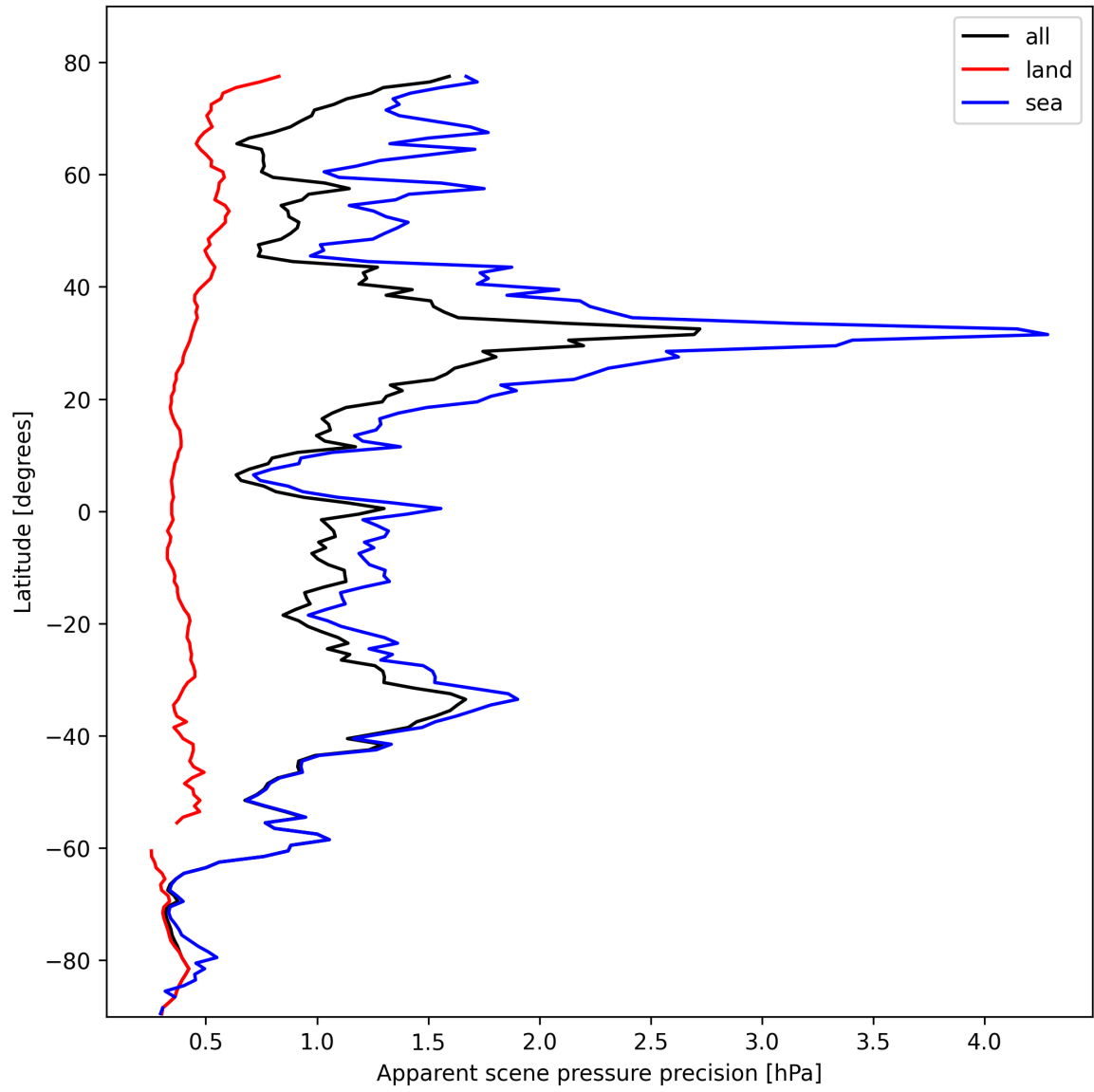
Figure 18: Zonal average of “Apparent scene pressure precision” for 2025-10-21 to 2025-10-22.
