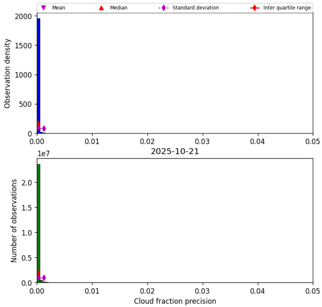
Figure 31: Histogram of “Cloud fraction precision” for 2025-10-21 to 2025-10-22
