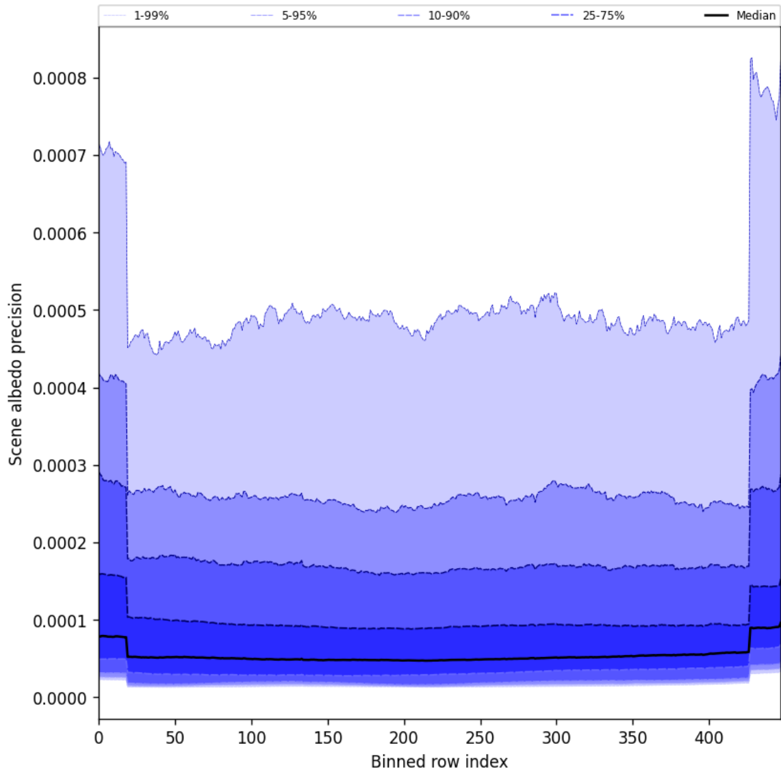
Figure 50: Along track statistics of “Scene albedo precision” for 2025-10-21 to 2025-10-22
