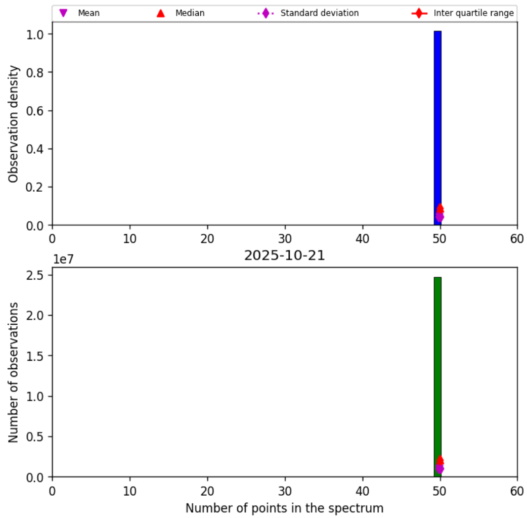
Figure 42: Histogram of “Number of points in the spectrum” for 2025-10-21 to 2025-10-22
