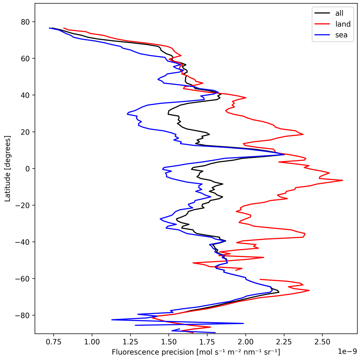
Figure 22: Zonal average of “Fluorescence precision” for 2025-10-22 to 2025-10-23.
