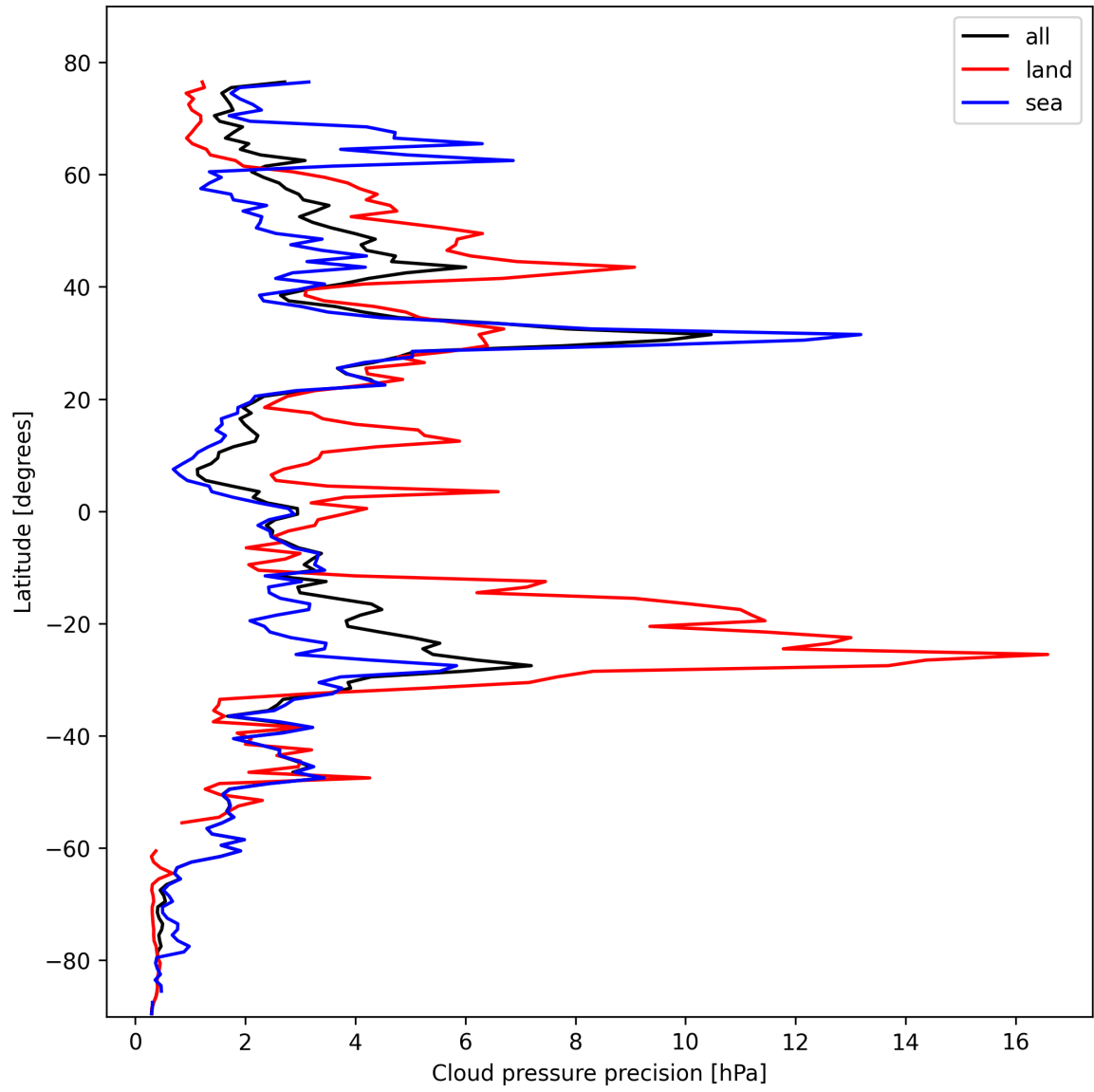
Figure 12: Zonal average of “Cloud pressure precision” for 2025-10-22 to 2025-10-23.
