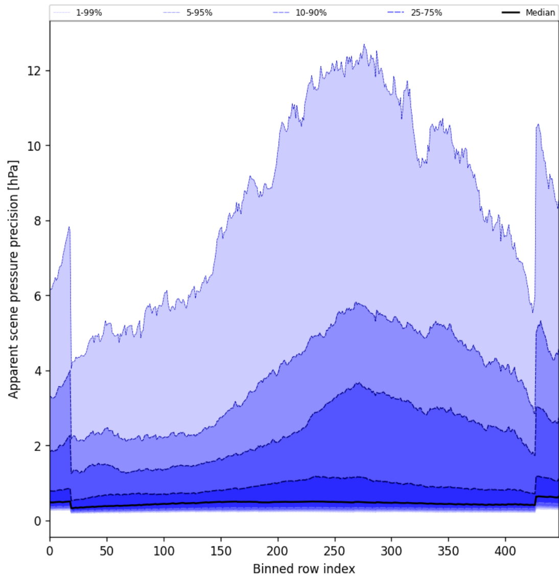
Figure 52: Along track statistics of “Apparent scene pressure precision” for 2025-10-22 to 2025-10-23
