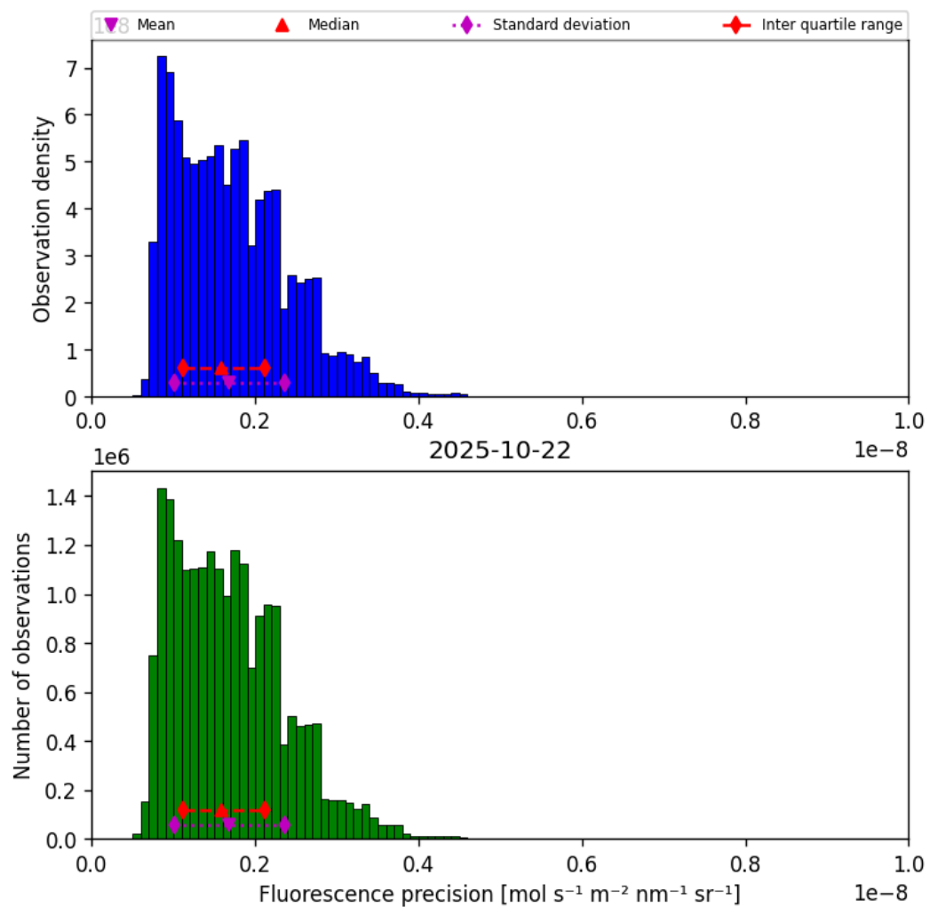
Figure 39: Histogram of “Fluorescence precision” for 2025-10-22 to 2025-10-23
