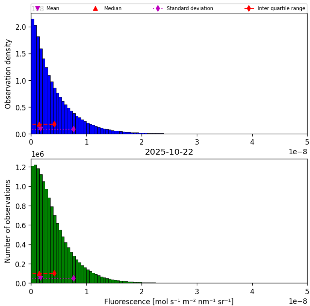
Figure 38: Histogram of “Fluorescence” for 2025-10-22 to 2025-10-23
