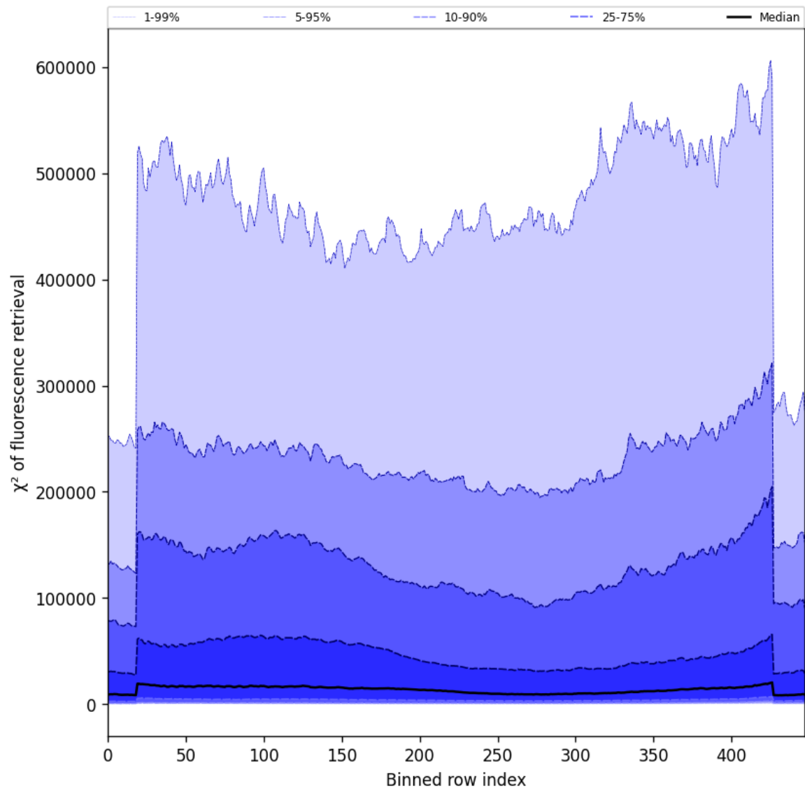
Figure 57: Along track statistics of “ \chi^2 of fluorescence retrieval” for 2025-10-22 to 2025-10-23
