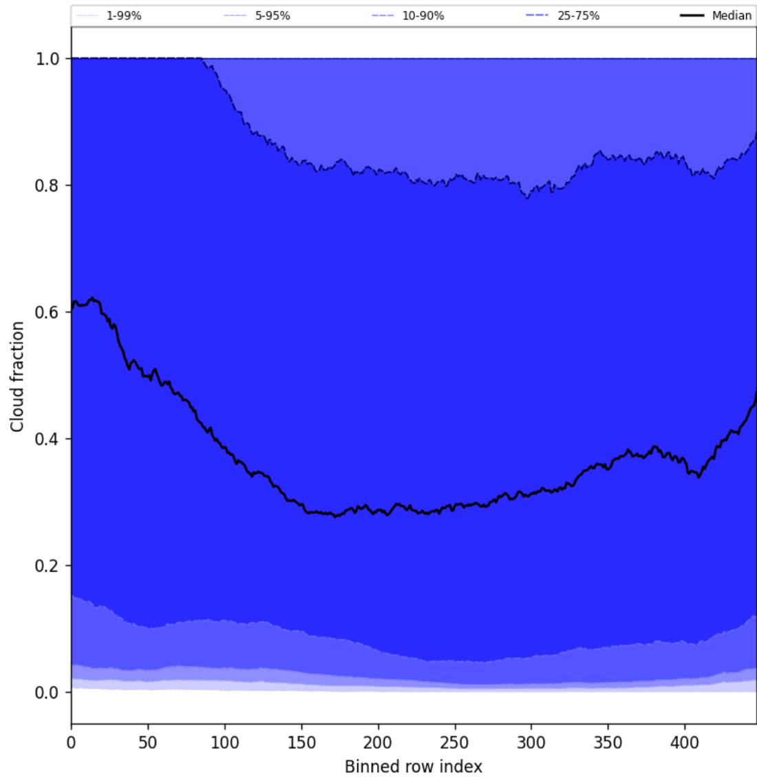
Figure 47: Along track statistics of “Cloud fraction” for 2025-10-22 to 2025-10-23
