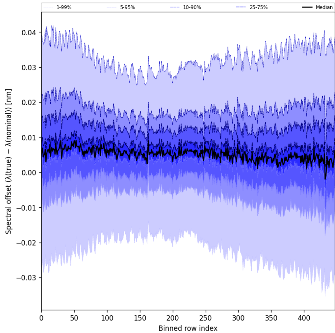
Figure 60: Along track statistics of “Spectral offset ( \lambda_{\text{true}} - \lambda_{\text{nominal}} )” for 2025-10-22 to 2025-10-23
