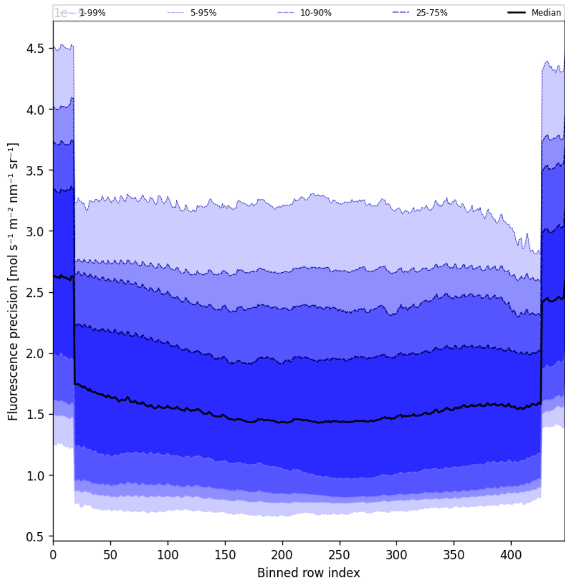
Figure 56: Along track statistics of “Fluorescence precision” for 2025-10-22 to 2025-10-23
