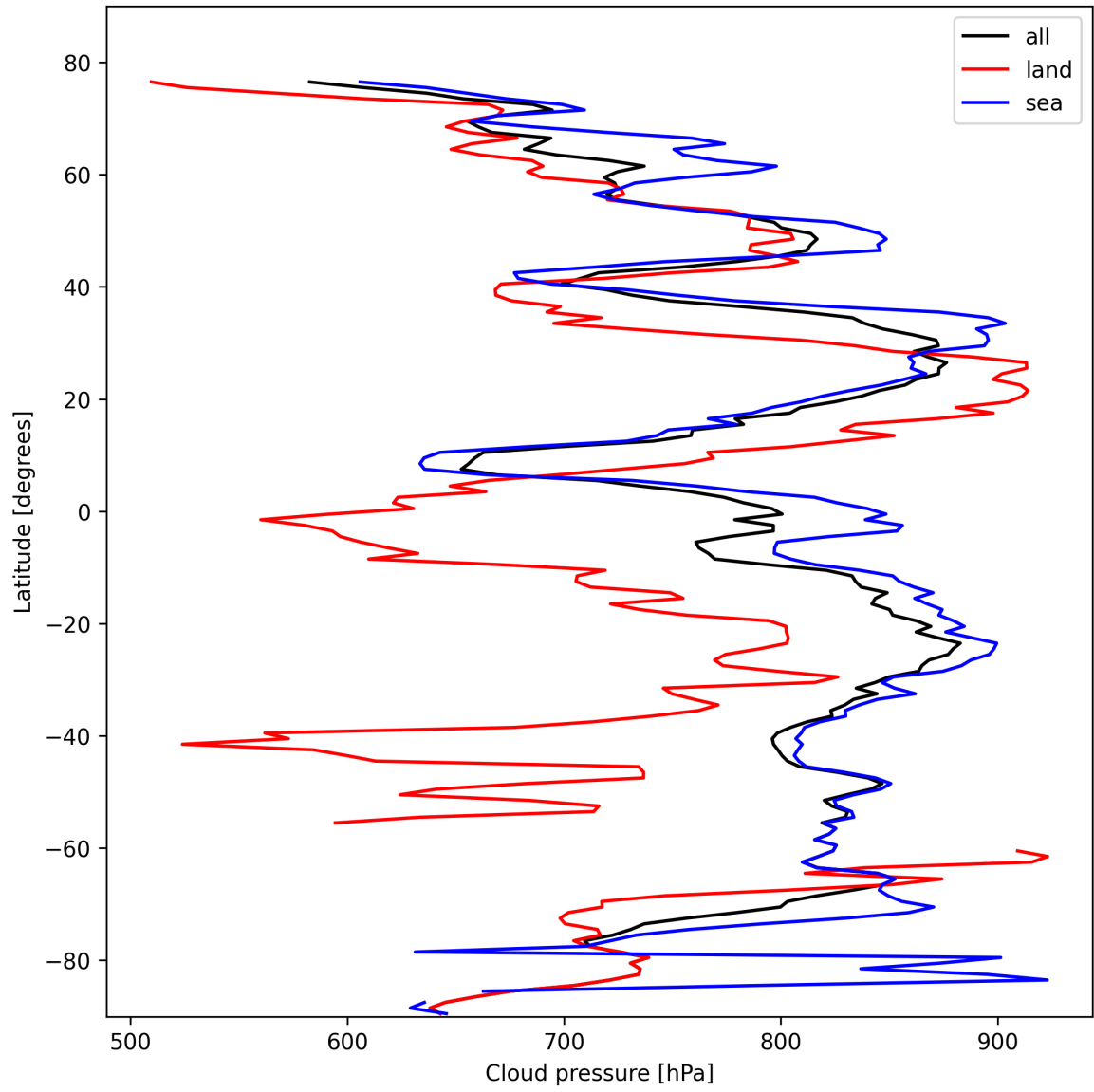
Figure 11: Zonal average of “Cloud pressure” for 2025-10-22 to 2025-10-23.
