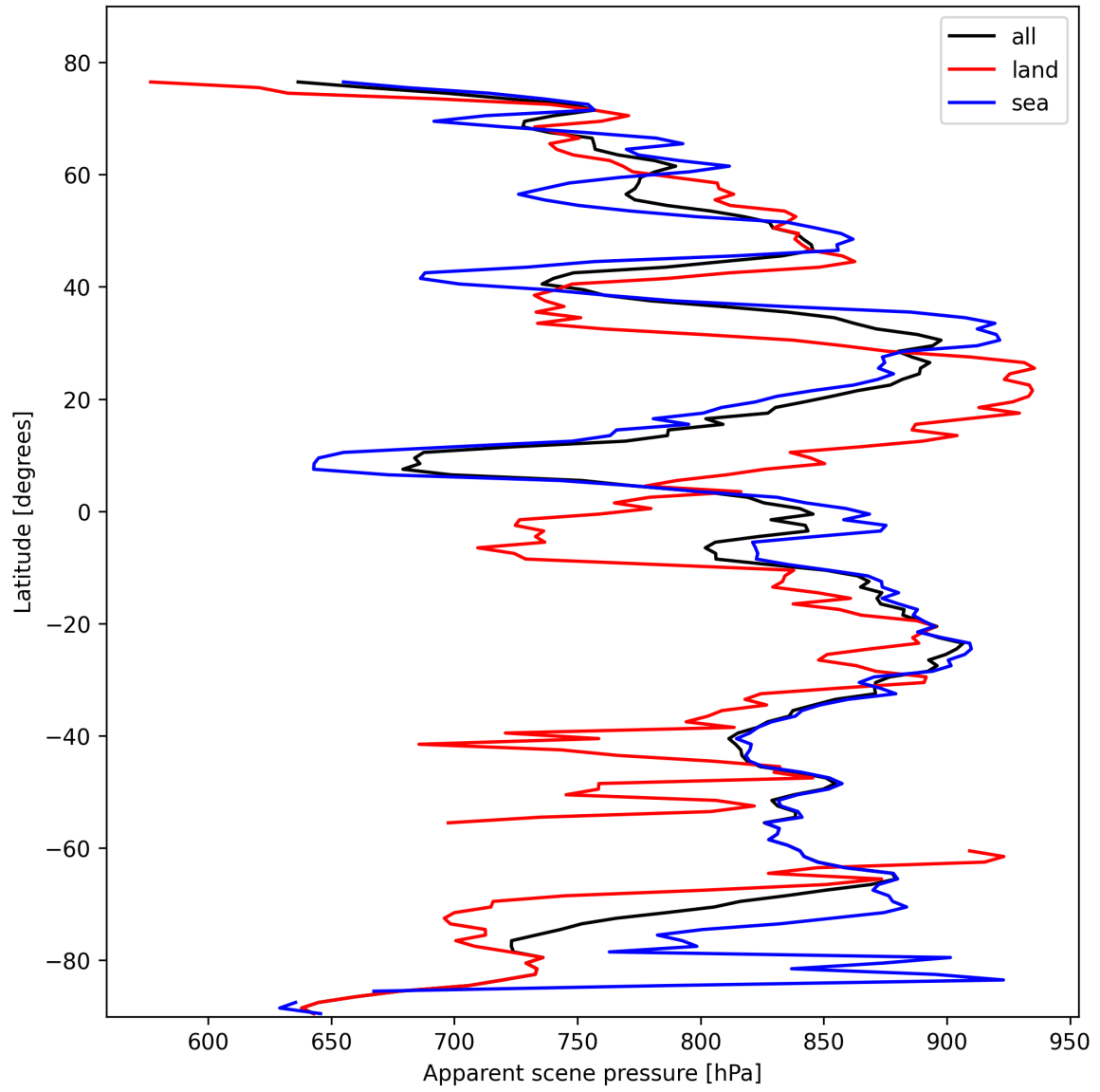
Figure 17: Zonal average of “Apparent scene pressure” for 2025-10-22 to 2025-10-23.
