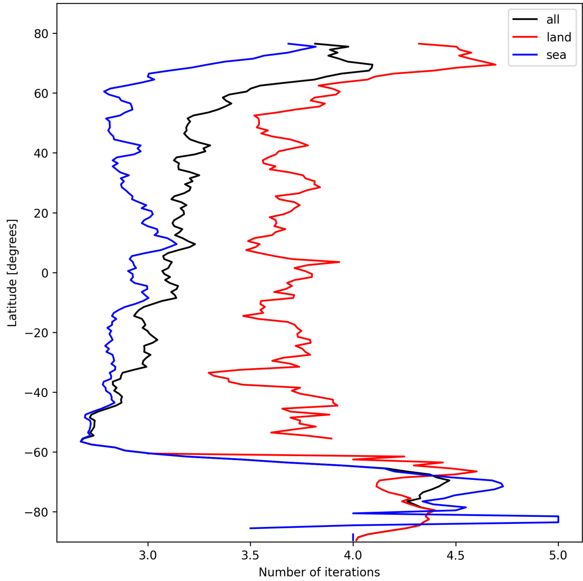
Figure 20: Zonal average of “Number of iterations” for 2025-10-22 to 2025-10-23.
