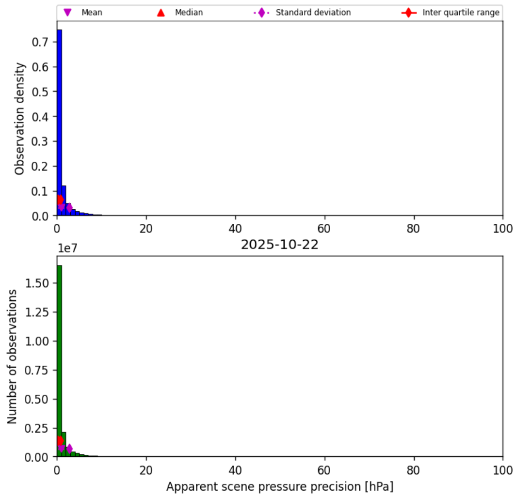
Figure 35: Histogram of “Apparent scene pressure precision” for 2025-10-22 to 2025-10-23
