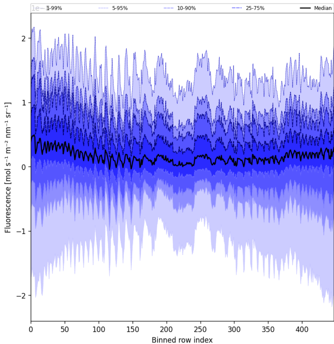
Figure 55: Along track statistics of "Fluorescence" for 2025-10-22 to 2025-10-23
