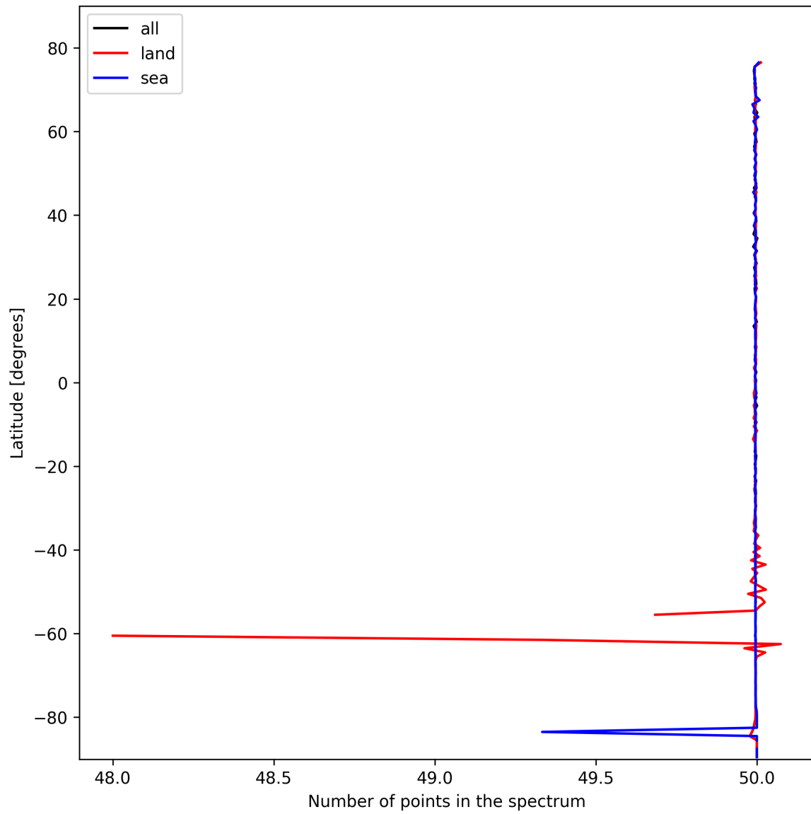
Figure 25: Zonal average of “Number of points in the spectrum” for 2025-10-22 to 2025-10-23.
