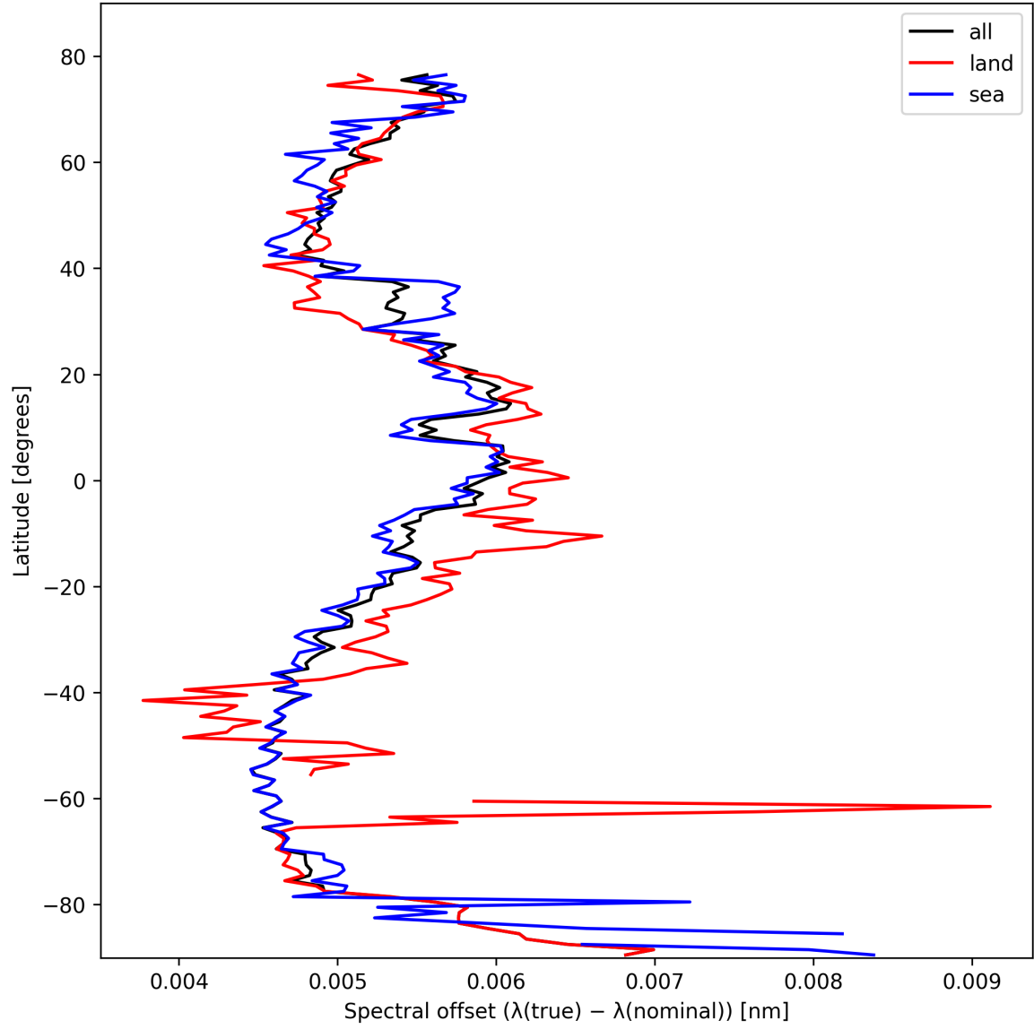
Figure 26: Zonal average of “Spectral offset ( \lambda_{\text{true}} - \lambda_{\text{nominal}} )” for 2025-10-22 to 2025-10-23.
