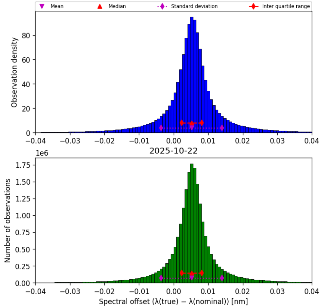
Figure 43: Histogram of “Spectral offset ( \lambda_{\text{true}} - \lambda_{\text{nominal}} )” for 2025-10-22 to 2025-10-23
