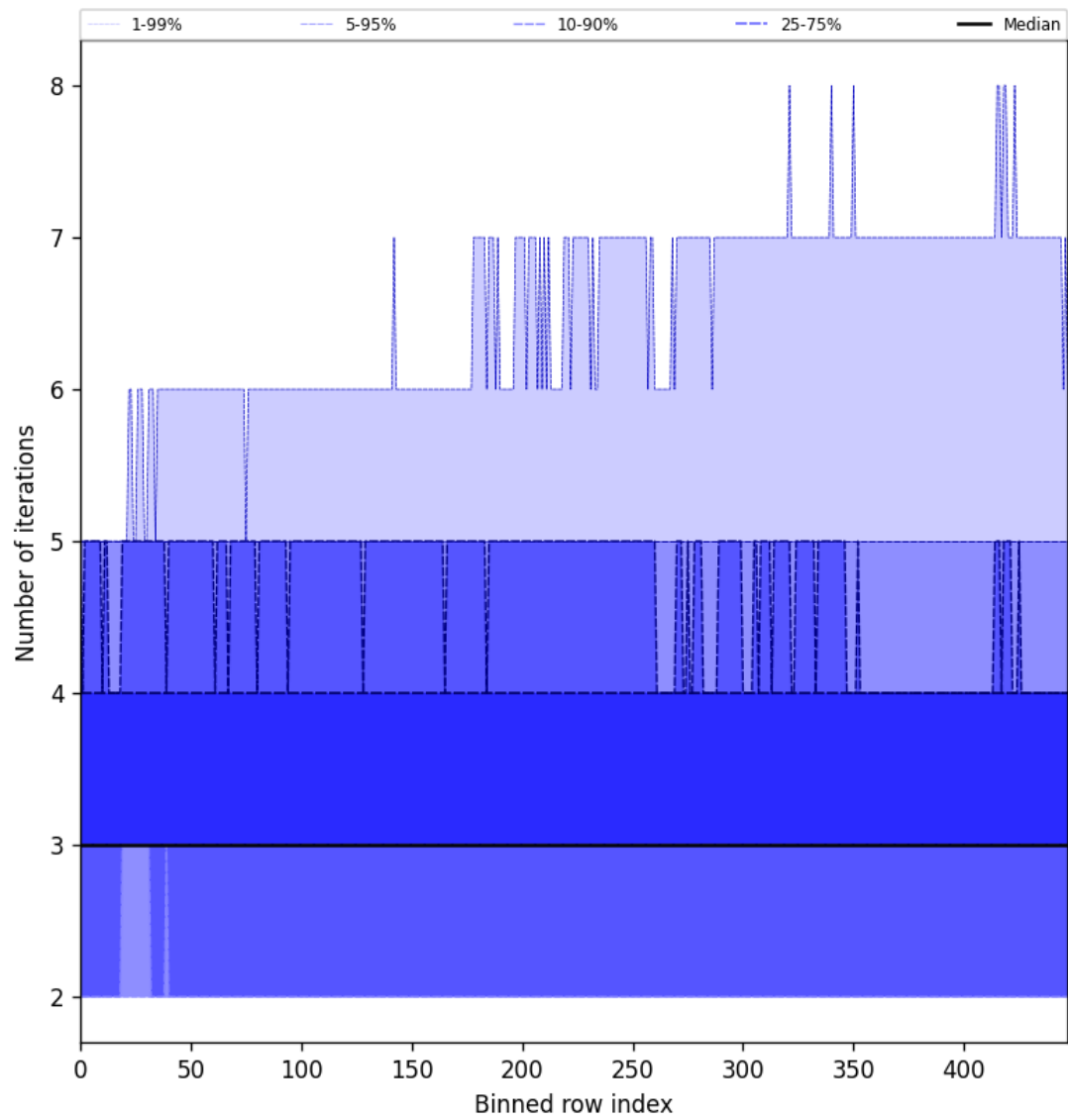
Figure 54: Along track statistics of “Number of iterations” for 2025-10-22 to 2025-10-23
