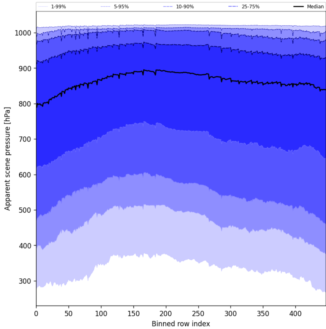
Figure 51: Along track statistics of “Apparent scene pressure” for 2025-10-22 to 2025-10-23
