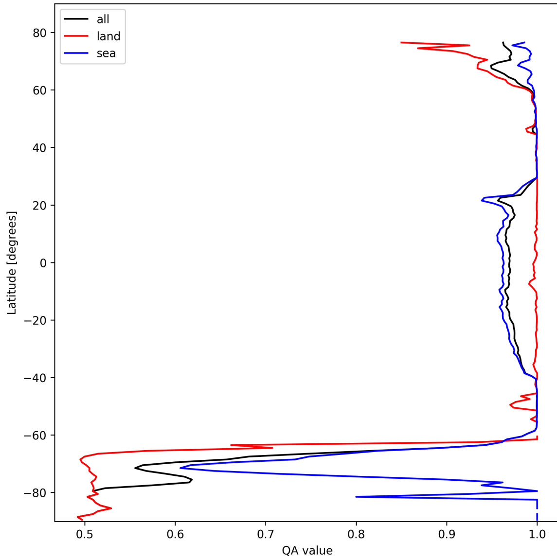
Figure 10: Zonal average of “QA value” for 2025-10-22 to 2025-10-23.
