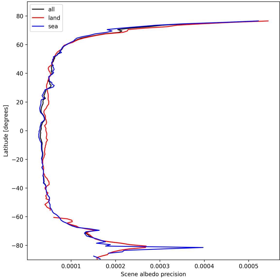
Figure 16: Zonal average of “Scene albedo precision” for 2025-10-22 to 2025-10-23.
