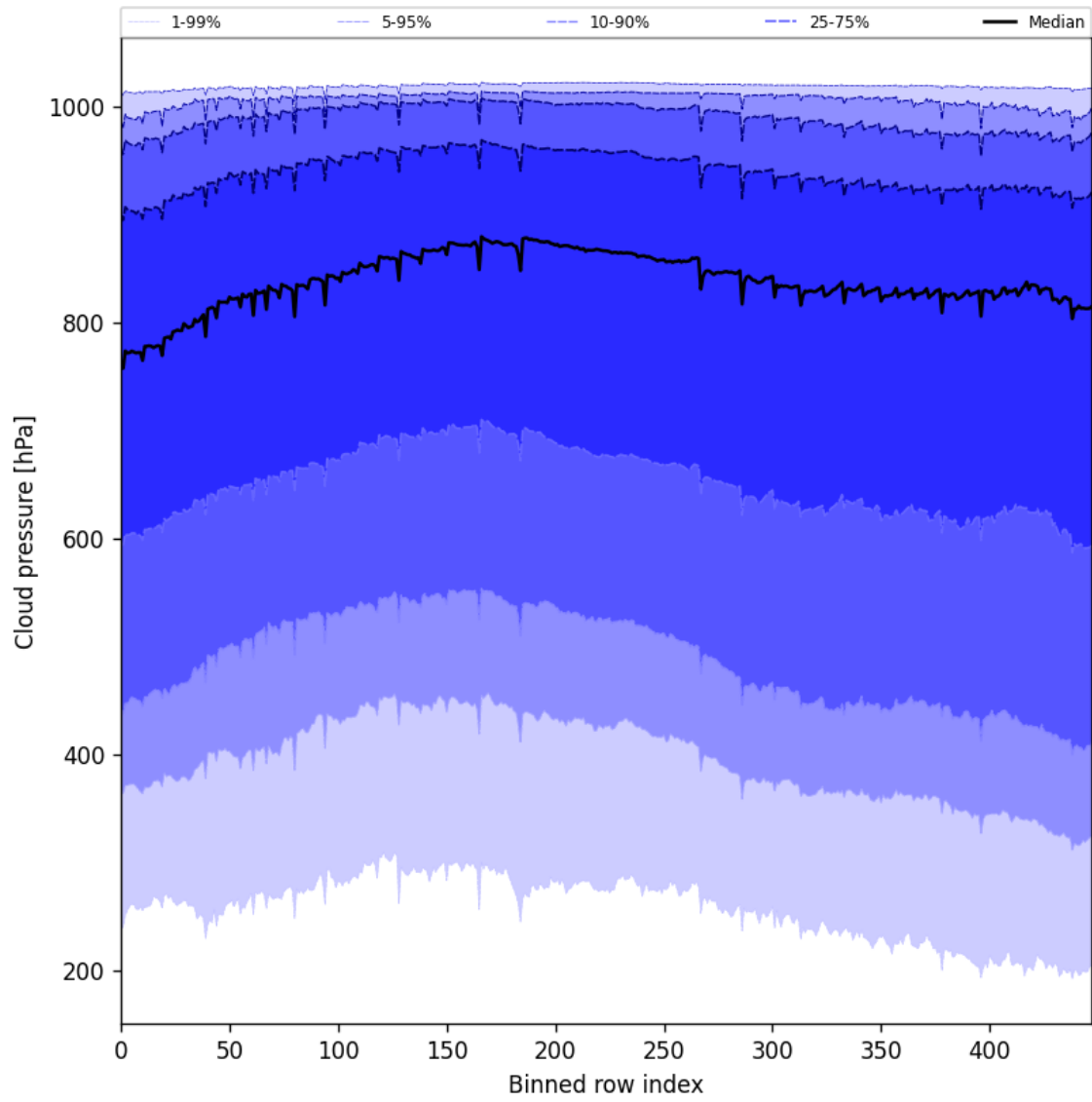
Figure 45: Along track statistics of “Cloud pressure” for 2025-10-22 to 2025-10-23
