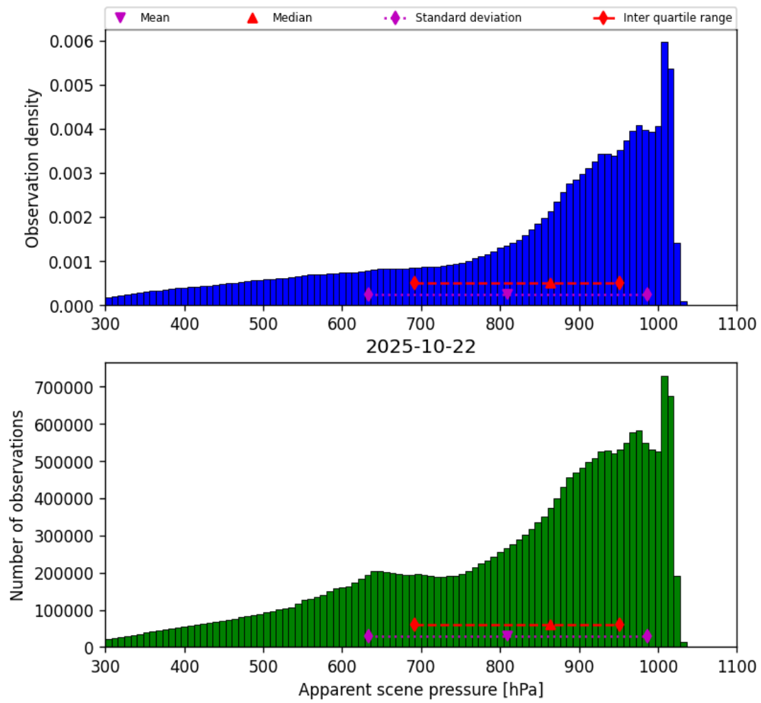
Figure 34: Histogram of “Apparent scene pressure” for 2025-10-22 to 2025-10-23
