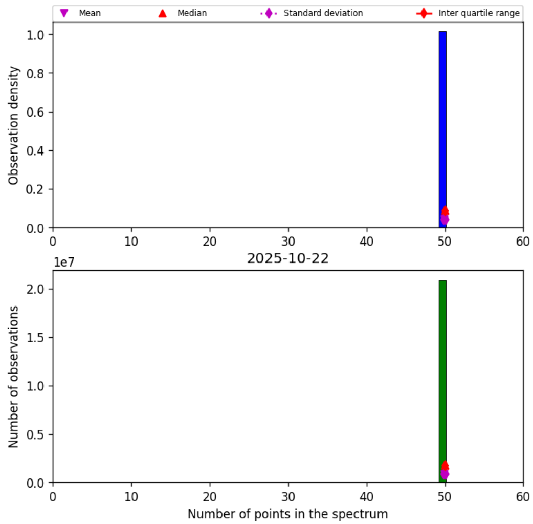
Figure 42: Histogram of “Number of points in the spectrum” for 2025-10-22 to 2025-10-23
