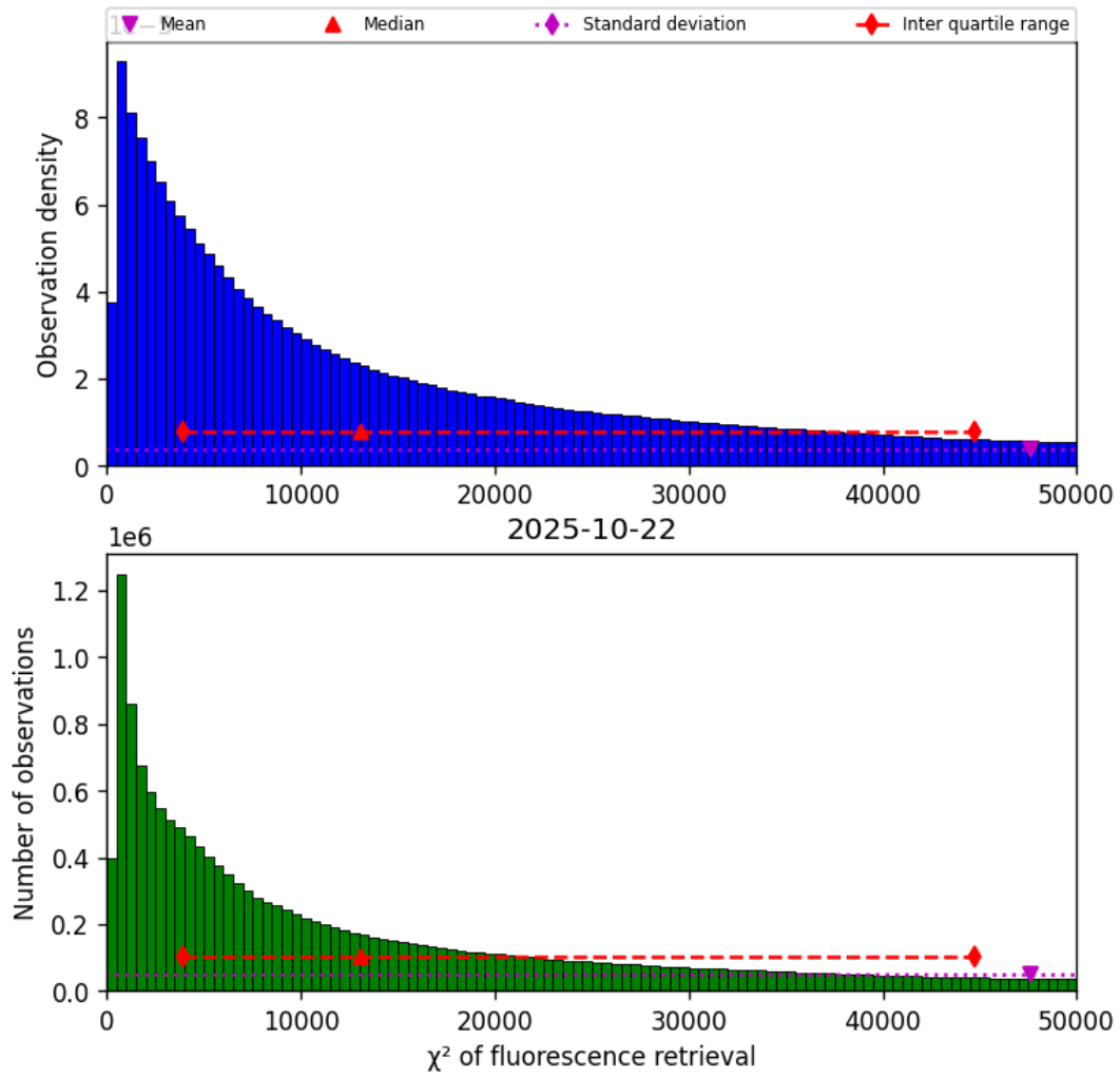
Figure 40: Histogram of “ \chi^2 of fluorescence retrieval” for 2025-10-22 to 2025-10-23
