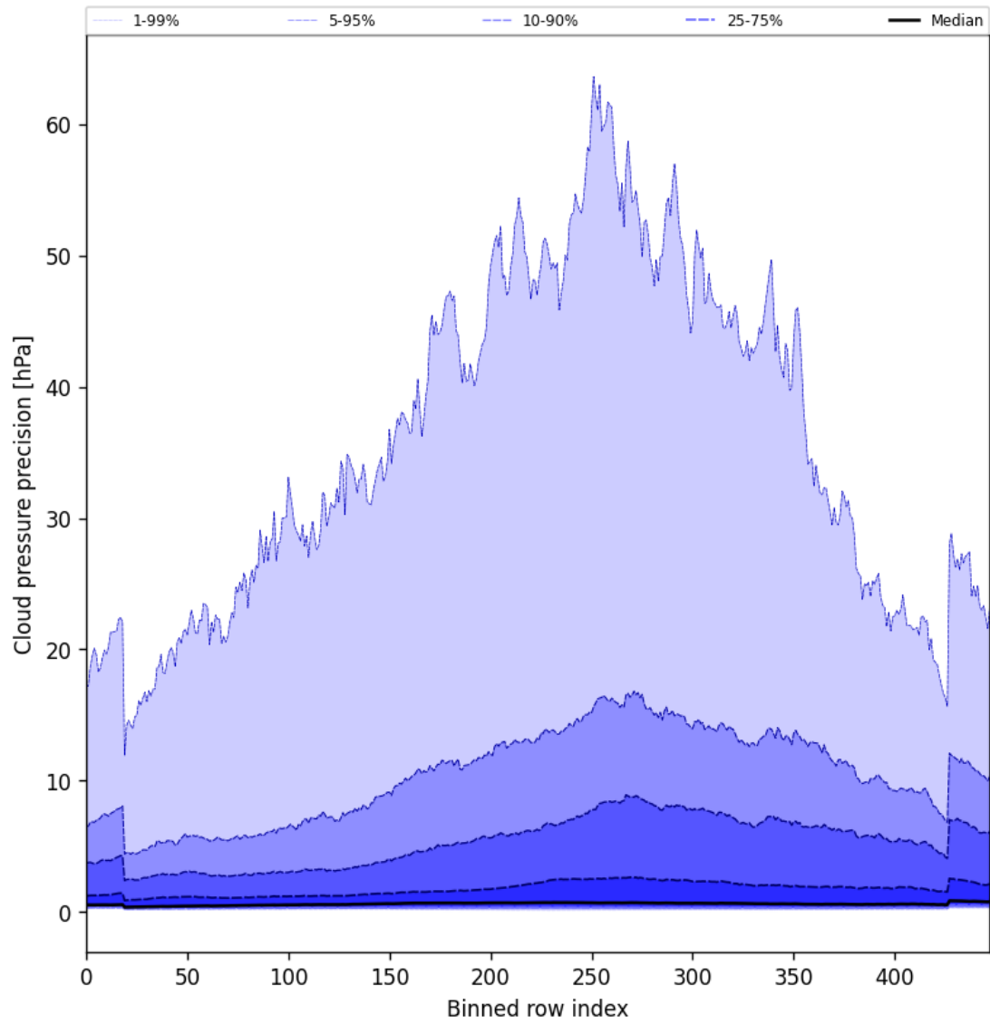
Figure 46: Along track statistics of “Cloud pressure precision” for 2025-10-22 to 2025-10-23
