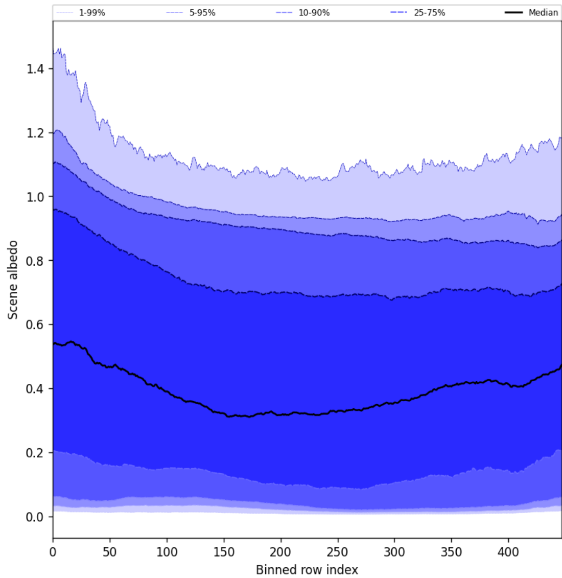
Figure 49: Along track statistics of “Scene albedo” for 2025-10-22 to 2025-10-23
