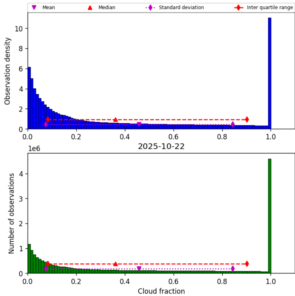
Figure 30: Histogram of “Cloud fraction” for 2025-10-22 to 2025-10-23
