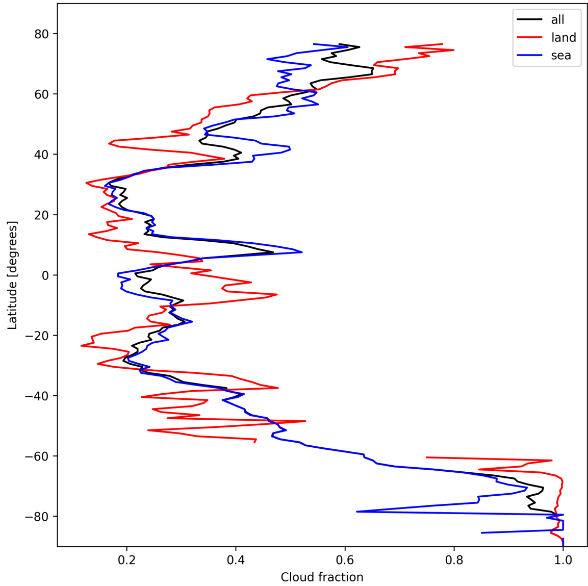
Figure 13: Zonal average of “Cloud fraction” for 2025-10-22 to 2025-10-23.
