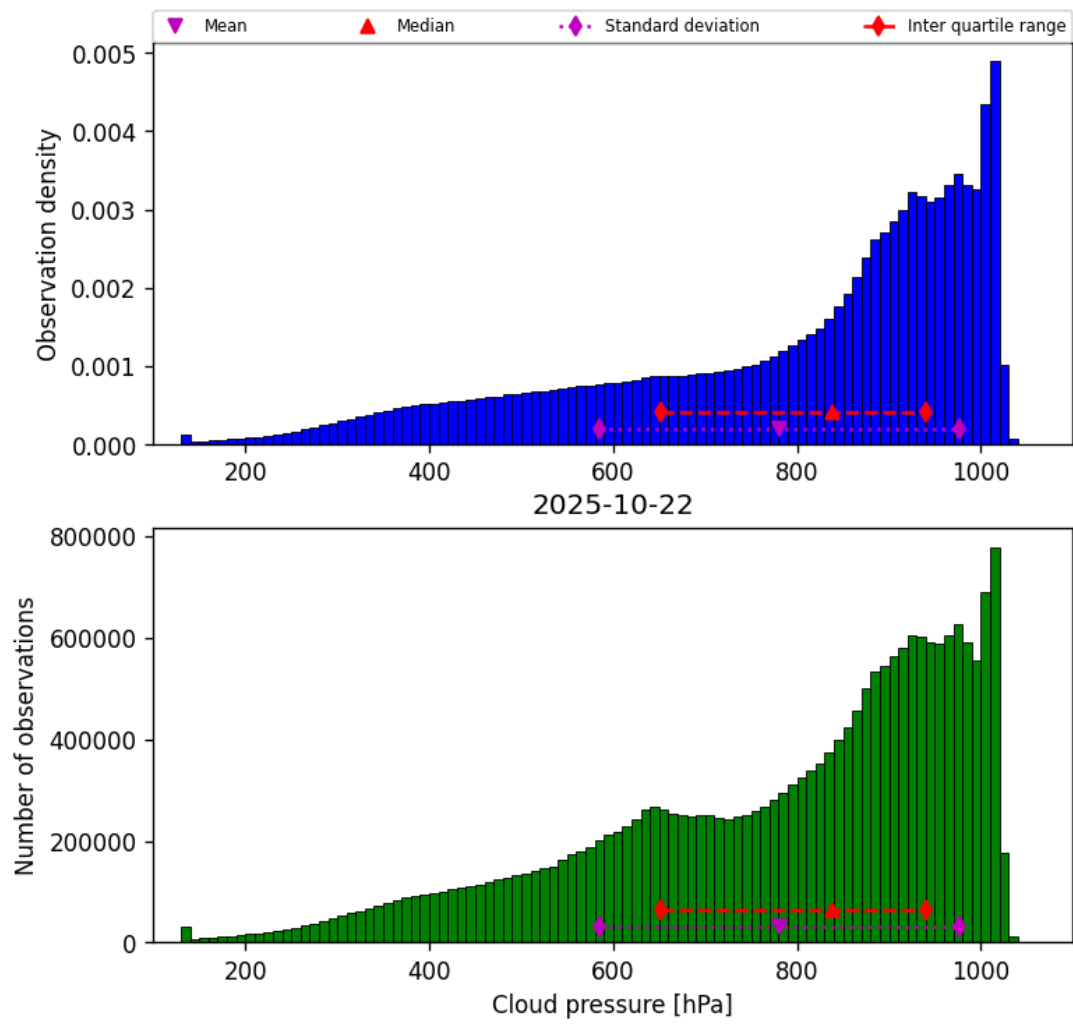
Figure 28: Histogram of “Cloud pressure” for 2025-10-22 to 2025-10-23
