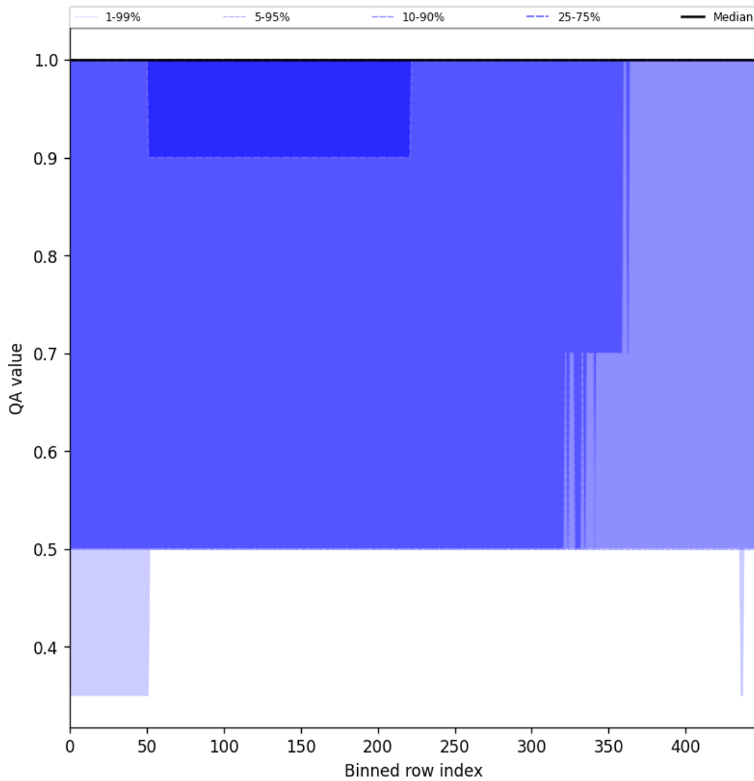
Figure 44: Along track statistics of “QA value” for 2025-10-22 to 2025-10-23
