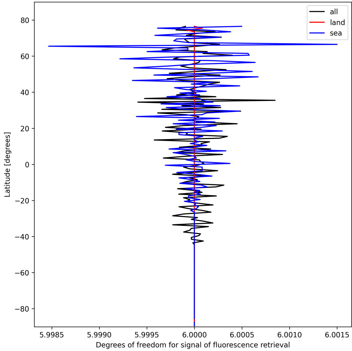
Figure 24: Zonal average of “Degrees of freedom for signal of fluorescence retrieval” for 2025-10-22 to 2025-10-23.
