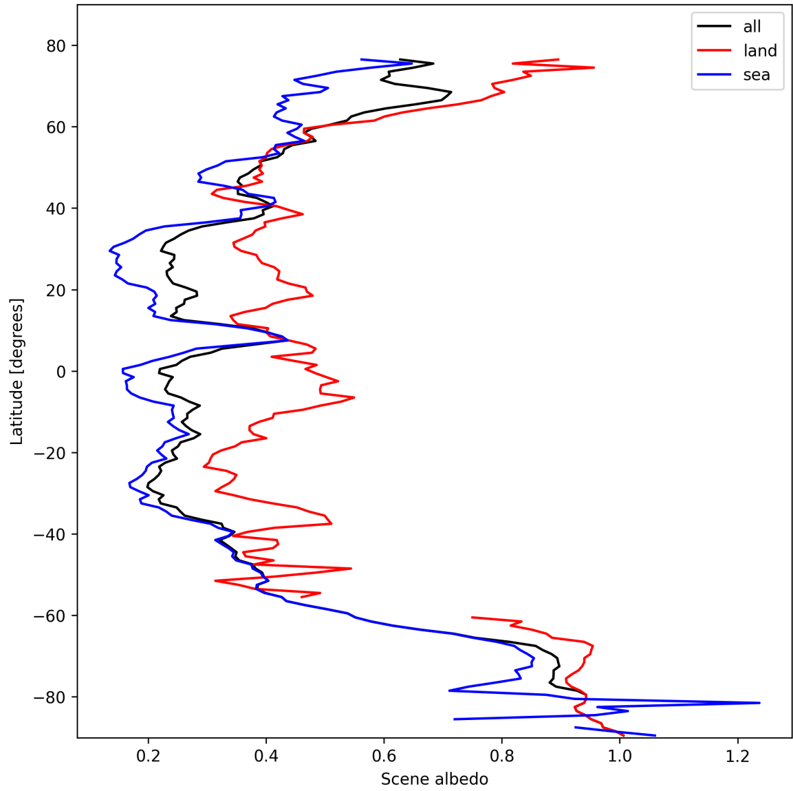
Figure 15: Zonal average of “Scene albedo” for 2025-10-22 to 2025-10-23.
