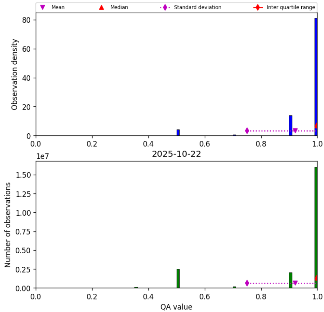
Figure 27: Histogram of “QA value” for 2025-10-22 to 2025-10-23
