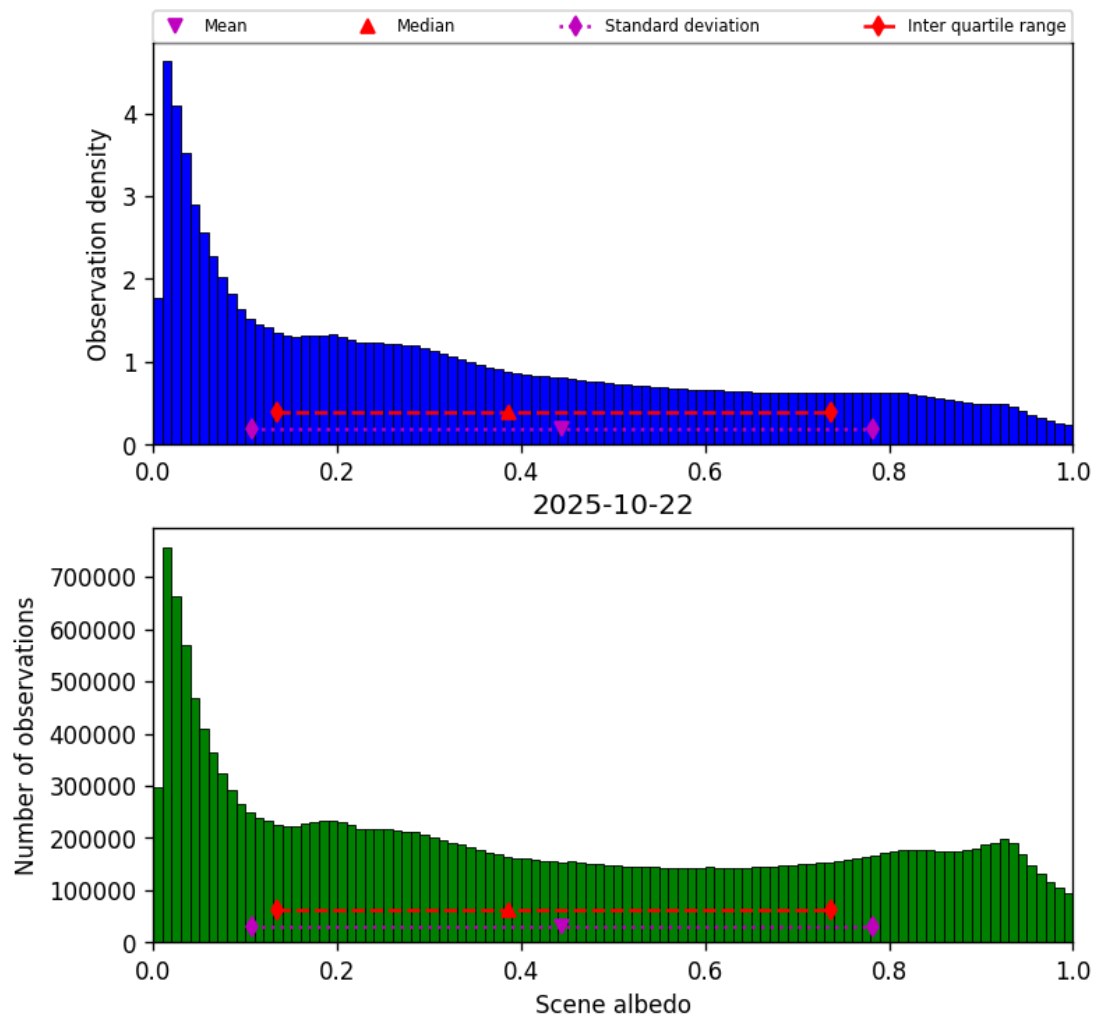
Figure 32: Histogram of “Scene albedo” for 2025-10-22 to 2025-10-23
