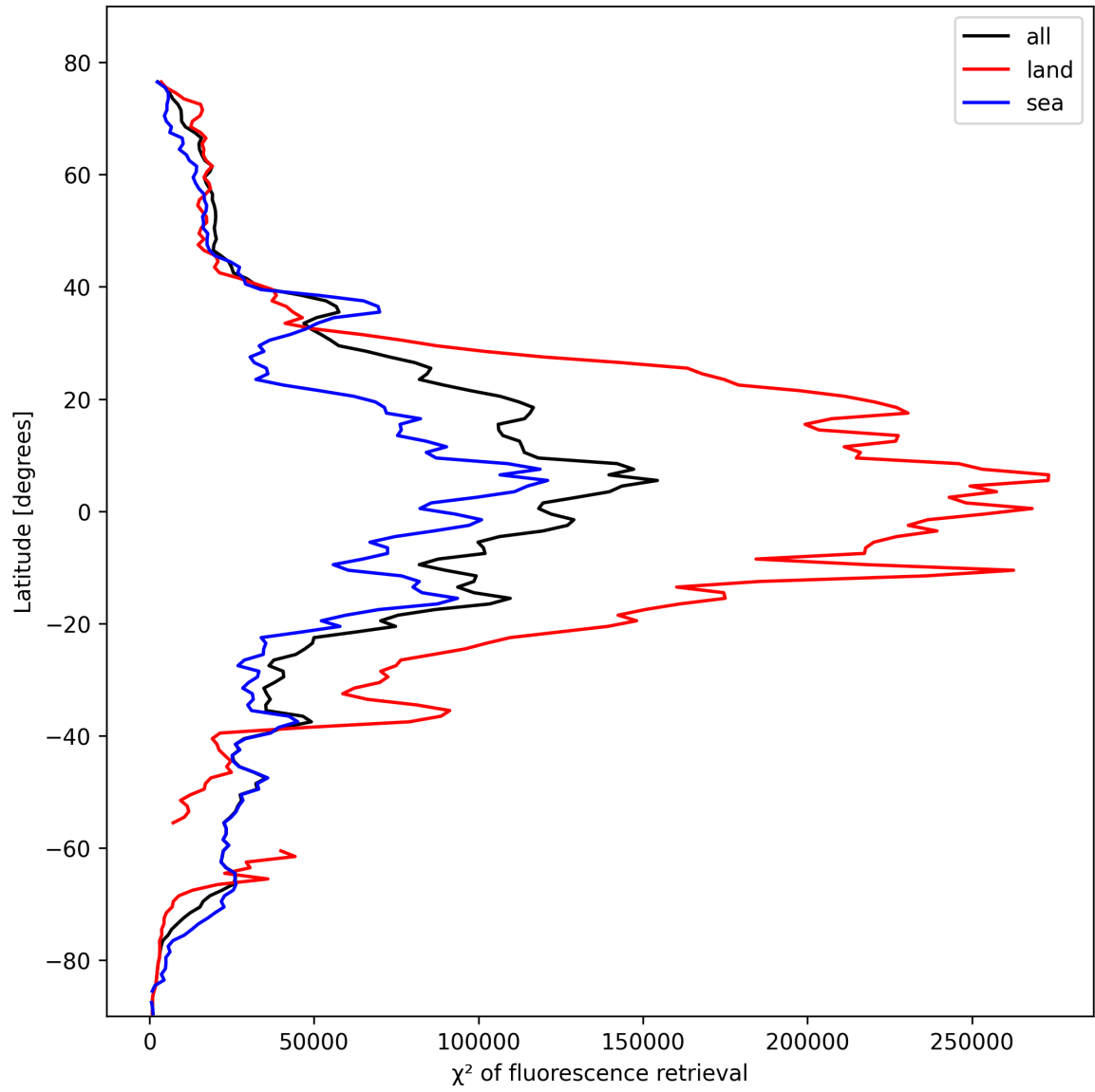
Figure 23: Zonal average of “ \chi^2 of fluorescence retrieval” for 2025-10-22 to 2025-10-23.
