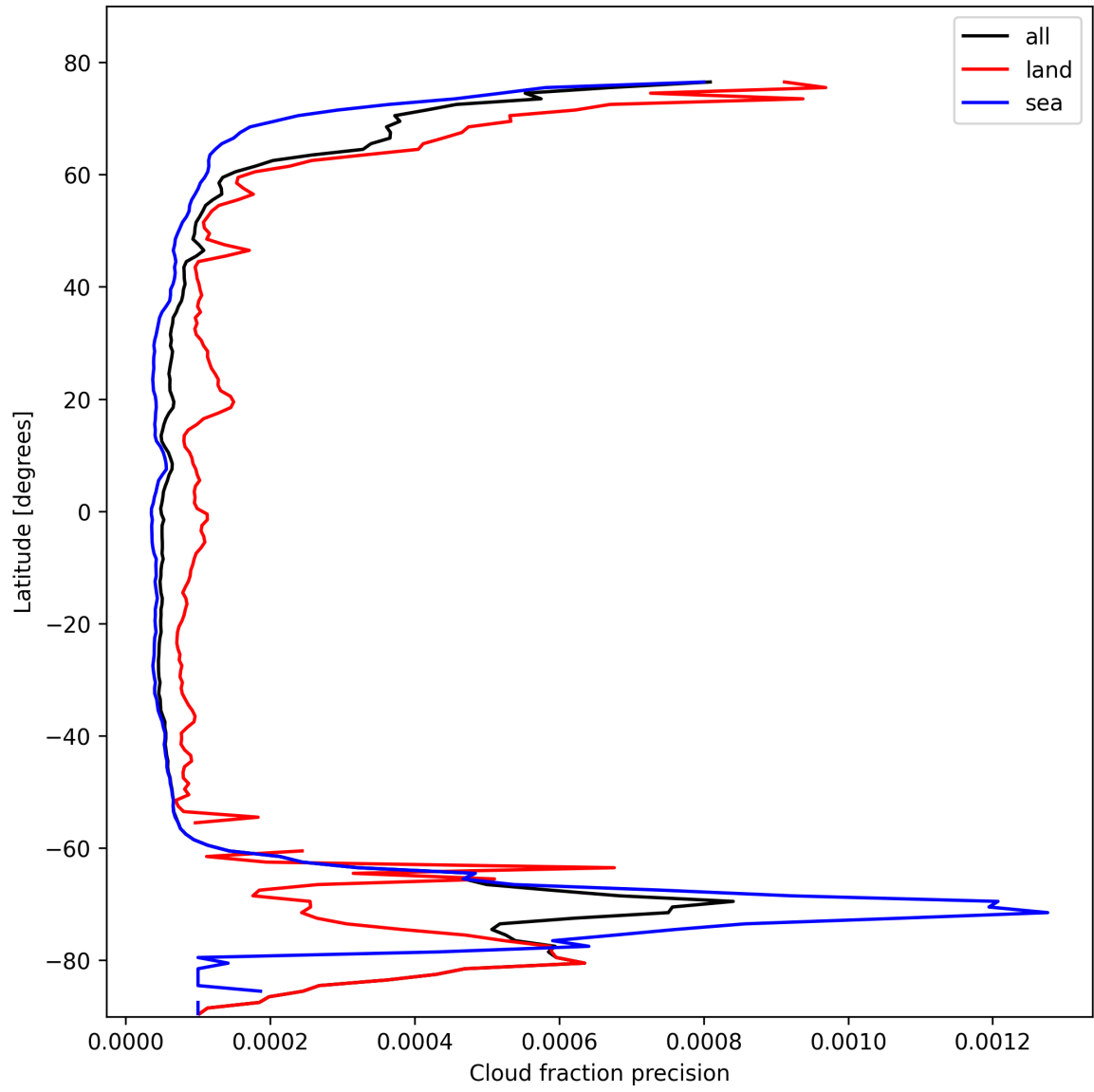
Figure 14: Zonal average of “Cloud fraction precision” for 2025-10-22 to 2025-10-23.
