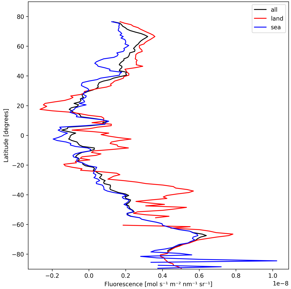
Figure 21: Zonal average of “Fluorescence” for 2025-10-22 to 2025-10-23.
