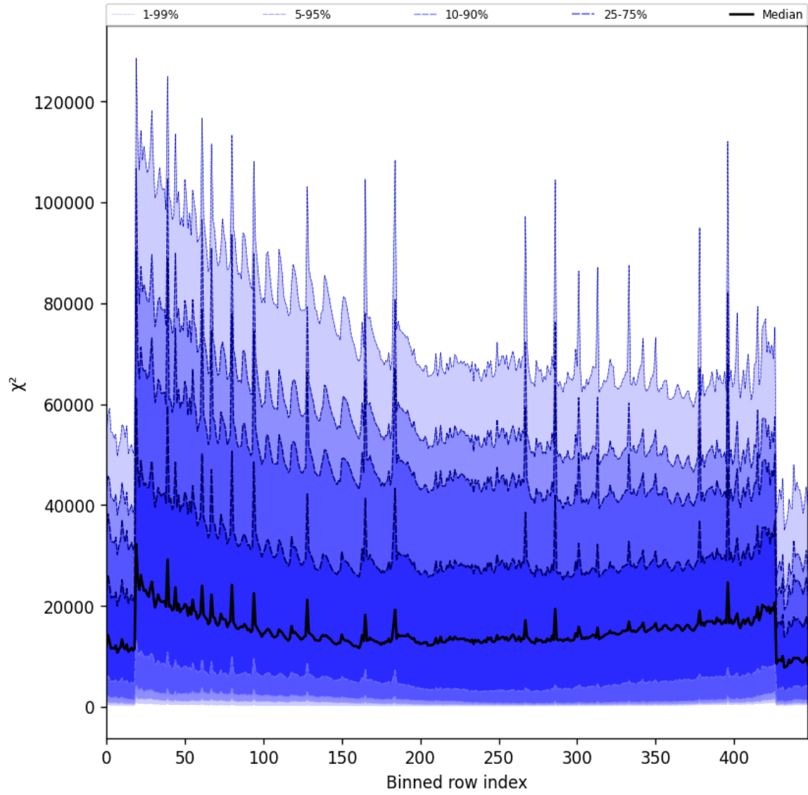
Figure 53: Along track statistics of “ \chi^2 ” for 2025-10-22 to 2025-10-23
