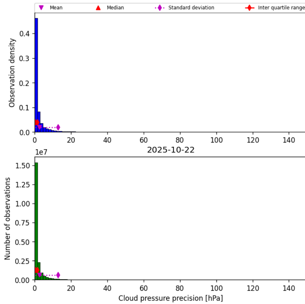
Figure 29: Histogram of “Cloud pressure precision” for 2025-10-22 to 2025-10-23
