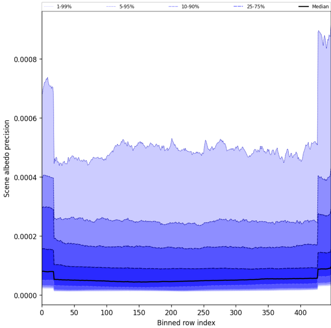
Figure 50: Along track statistics of “Scene albedo precision” for 2025-10-22 to 2025-10-23
