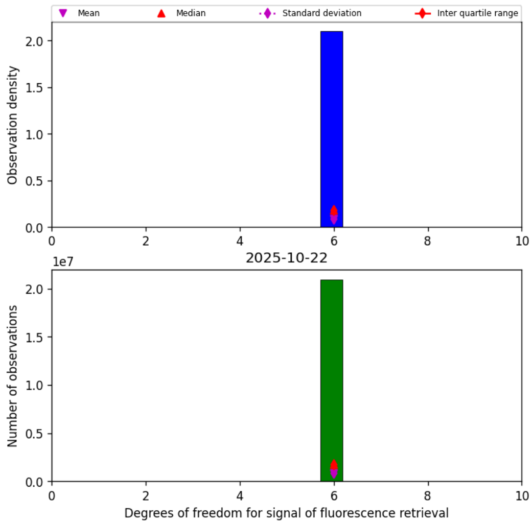
Figure 41: Histogram of “Degrees of freedom for signal of fluorescence retrieval” for 2025-10-22 to 2025-10-23
