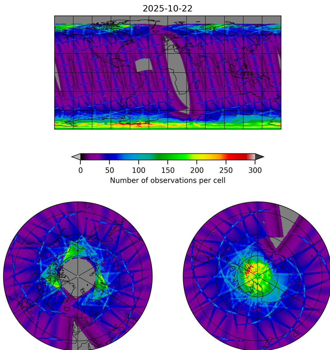
Figure 9: Map of the number of observations for 2025-10-22 to 2025-10-23
