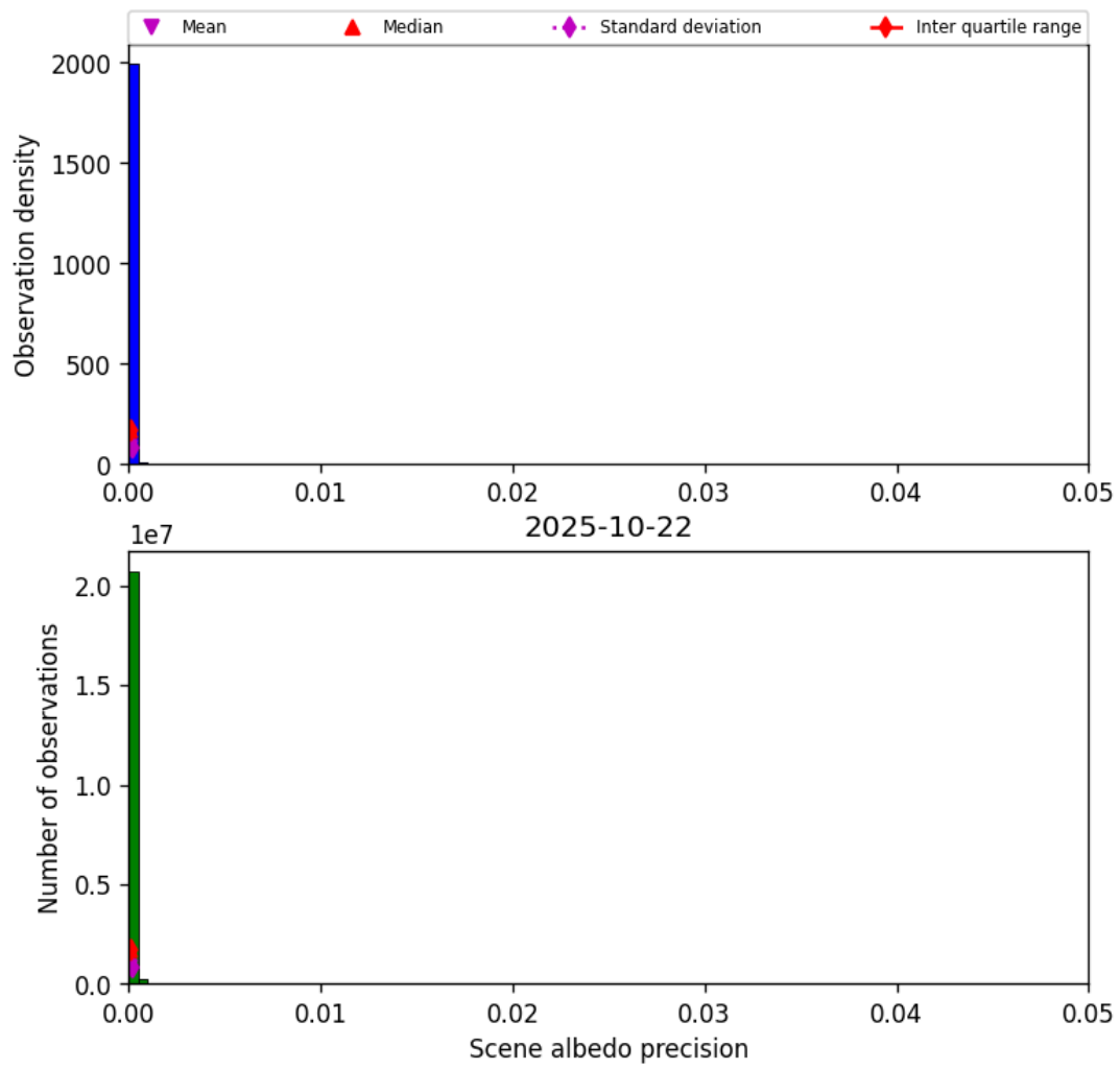
Figure 33: Histogram of “Scene albedo precision” for 2025-10-22 to 2025-10-23
