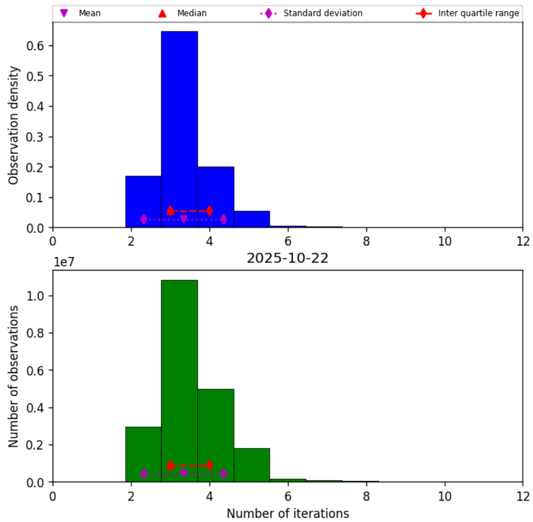
Figure 37: Histogram of “Number of iterations” for 2025-10-22 to 2025-10-23
