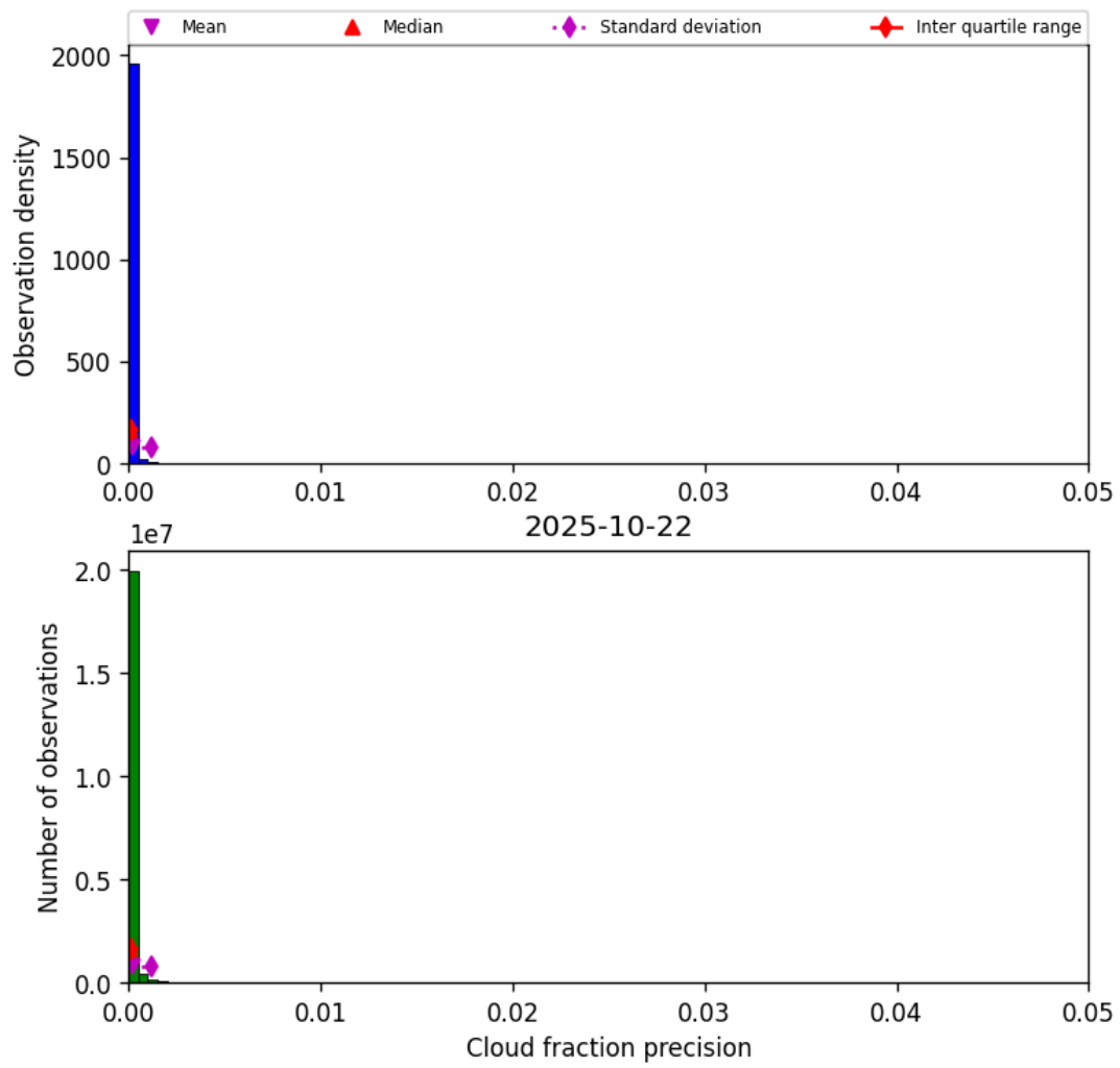
Figure 31: Histogram of “Cloud fraction precision” for 2025-10-22 to 2025-10-23
