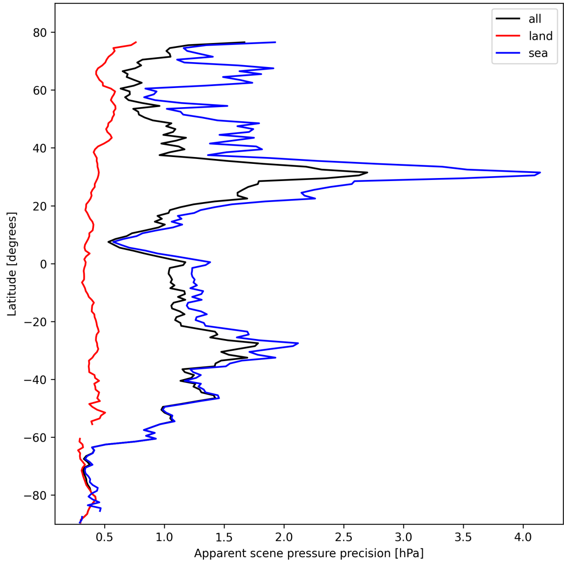
Figure 18: Zonal average of “Apparent scene pressure precision” for 2025-10-22 to 2025-10-23.
