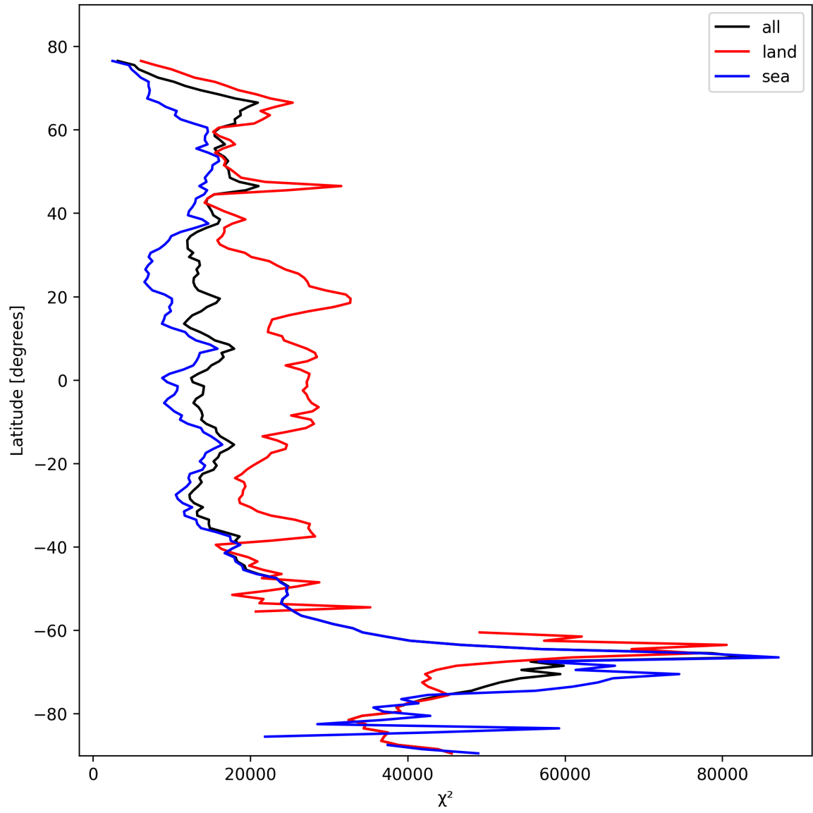
Figure 19: Zonal average of “ \chi^2 ” for 2025-10-22 to 2025-10-23.
