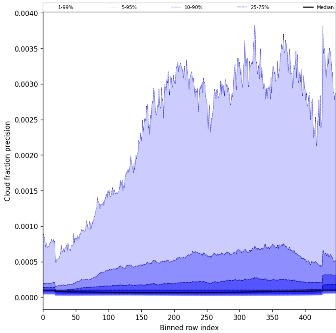
Figure 48: Along track statistics of “Cloud fraction precision” for 2025-10-22 to 2025-10-23
