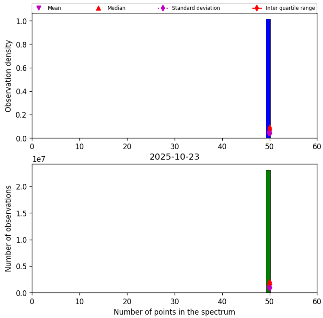
Figure 42: Histogram of “Number of points in the spectrum” for 2025-10-23 to 2025-10-24
