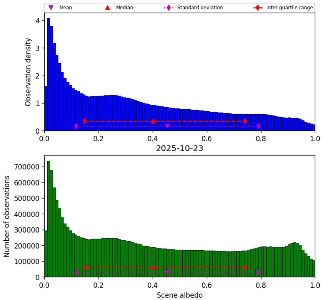
Figure 32: Histogram of “Scene albedo” for 2025-10-23 to 2025-10-24
