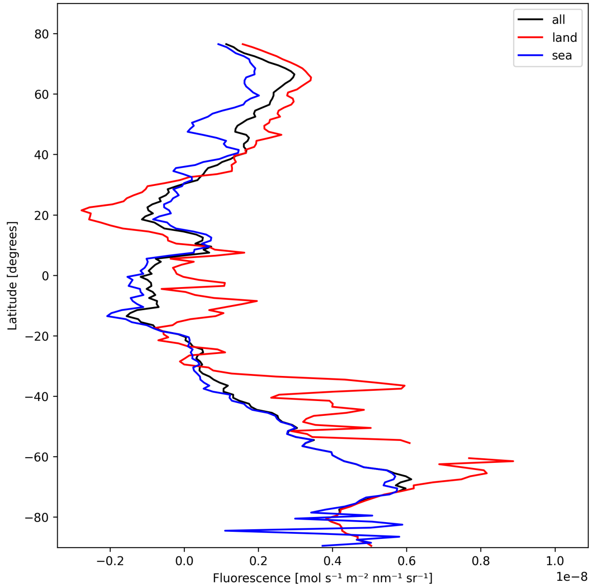
Figure 21: Zonal average of “Fluorescence” for 2025-10-23 to 2025-10-24.
