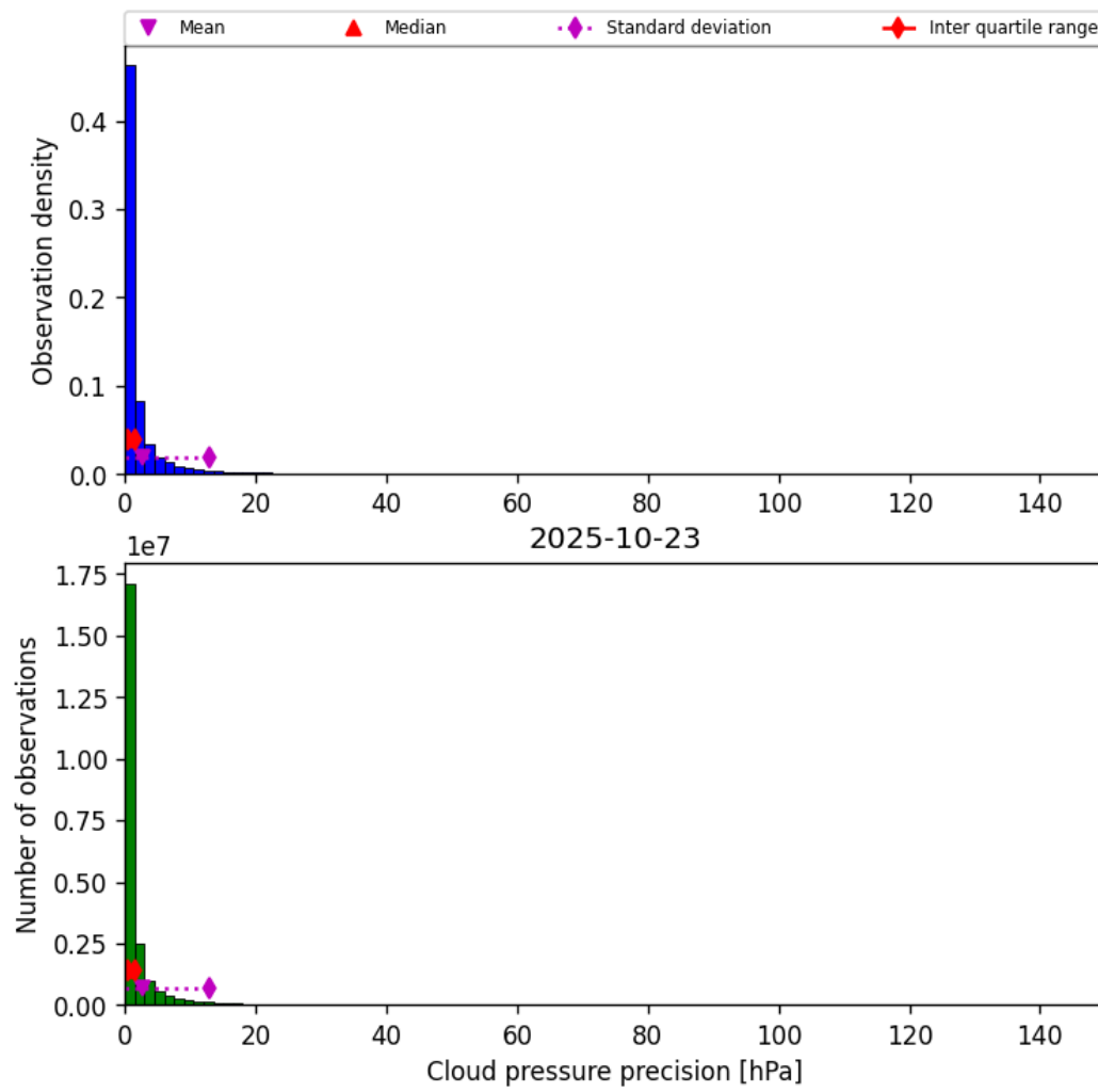
Figure 29: Histogram of “Cloud pressure precision” for 2025-10-23 to 2025-10-24
