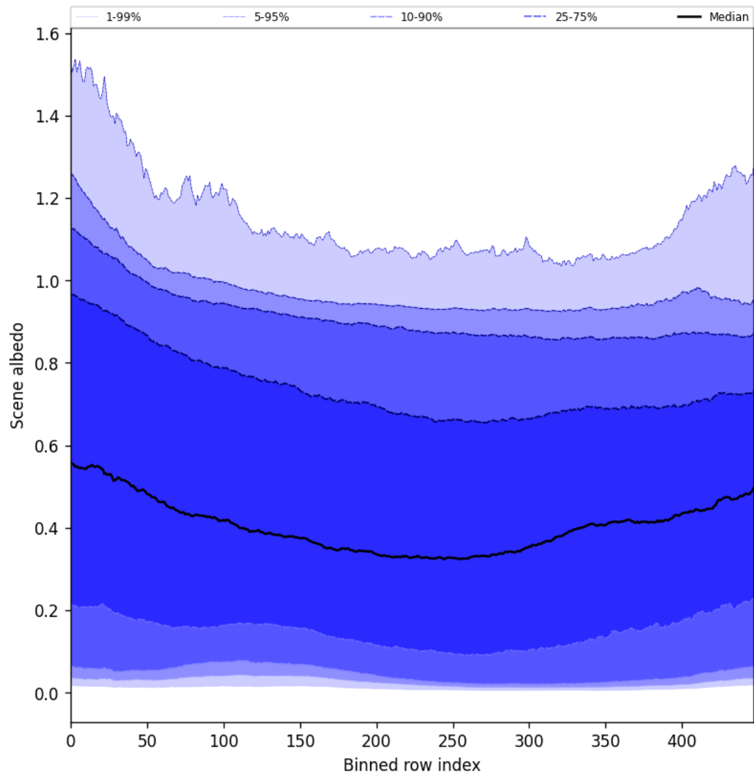
Figure 49: Along track statistics of “Scene albedo” for 2025-10-23 to 2025-10-24
