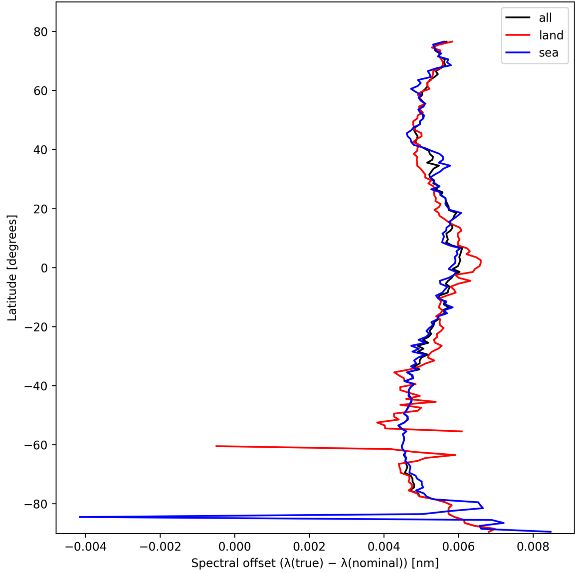
Figure 26: Zonal average of “Spectral offset ( \lambda_{\text{true}} - \lambda_{\text{nominal}} )” for 2025-10-23 to 2025-10-24.
