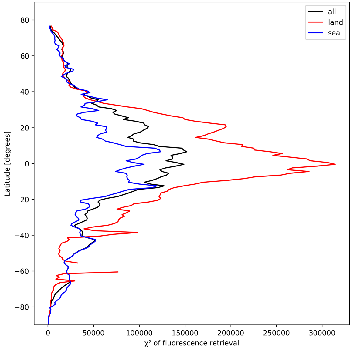
Figure 23: Zonal average of “ \chi^2 of fluorescence retrieval” for 2025-10-23 to 2025-10-24.
