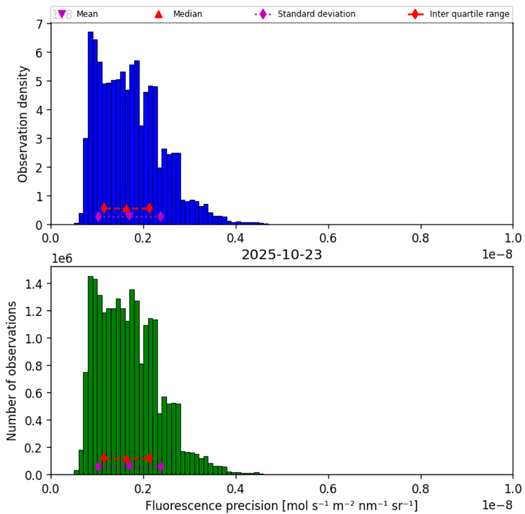
Figure 39: Histogram of “Fluorescence precision” for 2025-10-23 to 2025-10-24
