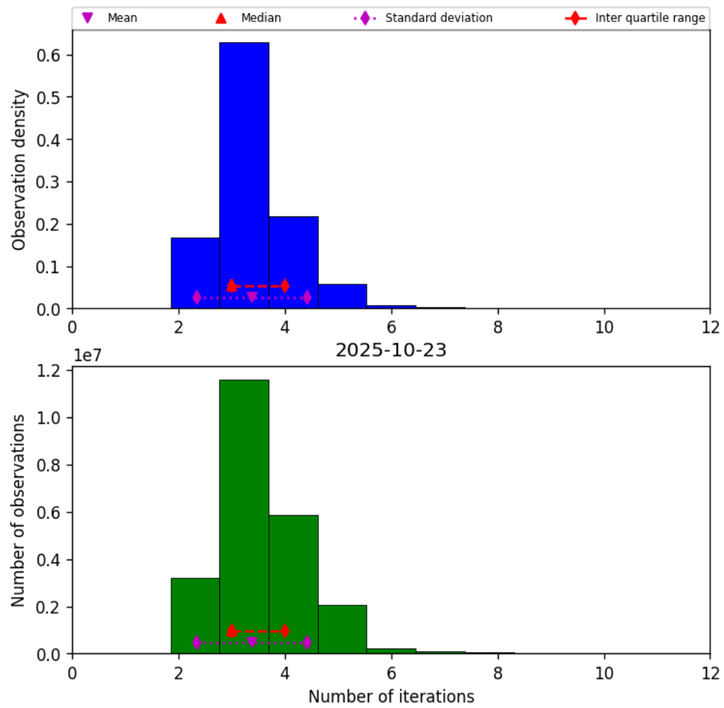
Figure 37: Histogram of “Number of iterations” for 2025-10-23 to 2025-10-24
