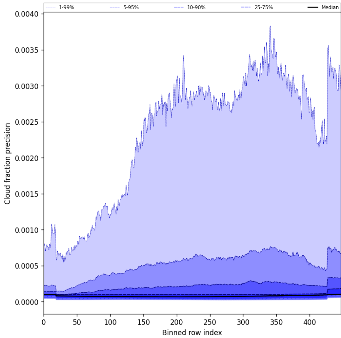
Figure 48: Along track statistics of “Cloud fraction precision” for 2025-10-23 to 2025-10-24
