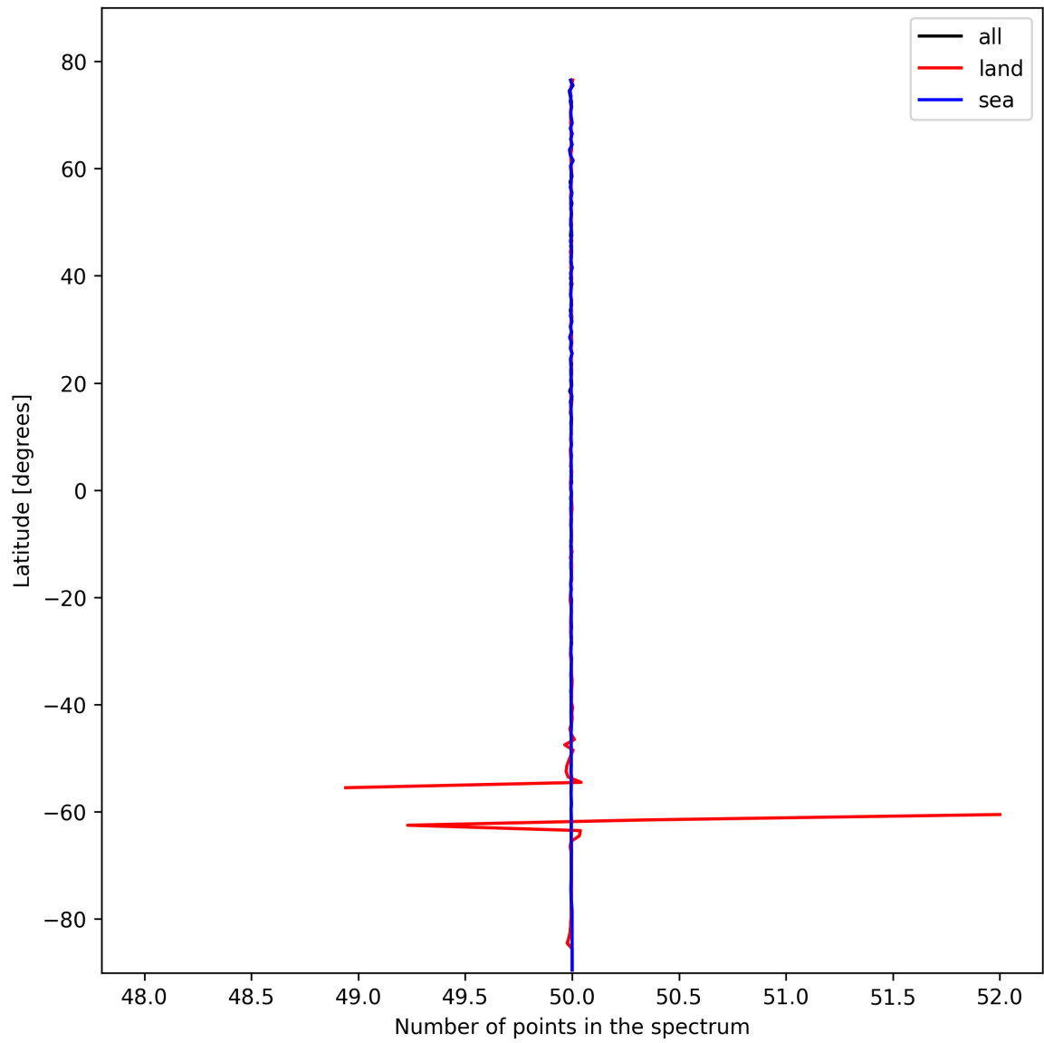
Figure 25: Zonal average of “Number of points in the spectrum” for 2025-10-23 to 2025-10-24.
