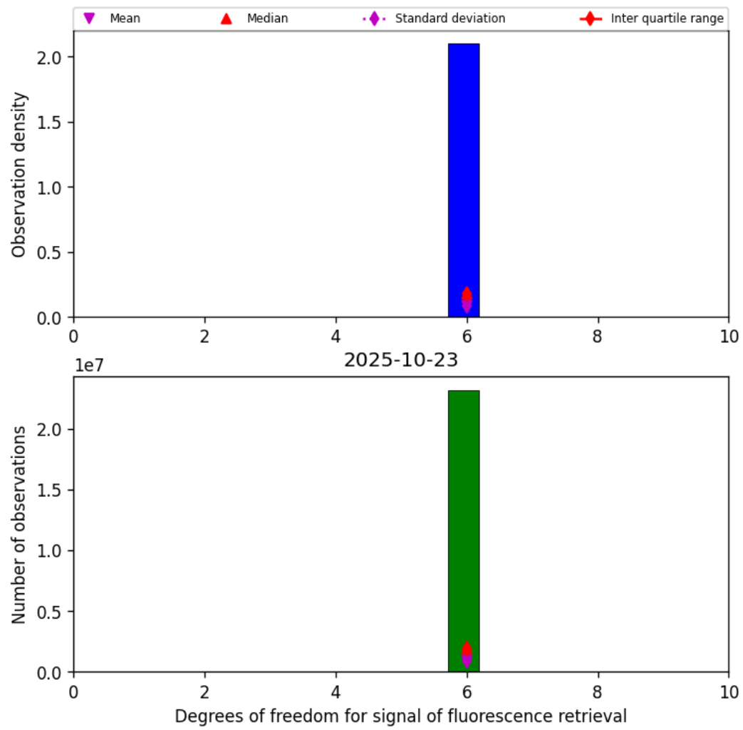
Figure 41: Histogram of “Degrees of freedom for signal of fluorescence retrieval” for 2025-10-23 to 2025-10-24
