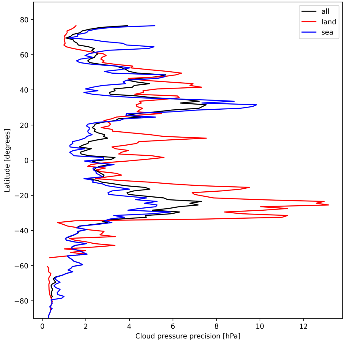
Figure 12: Zonal average of "Cloud pressure precision" for 2025-10-23 to 2025-10-24.
