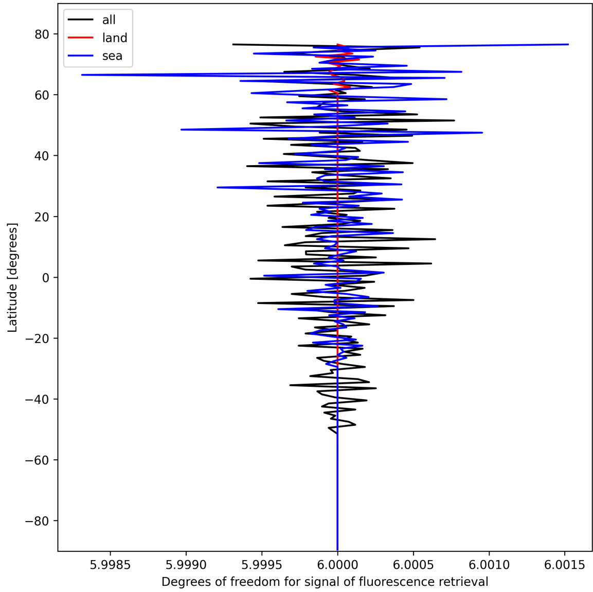
Figure 24: Zonal average of “Degrees of freedom for signal of fluorescence retrieval” for 2025-10-23 to 2025-10-24.
