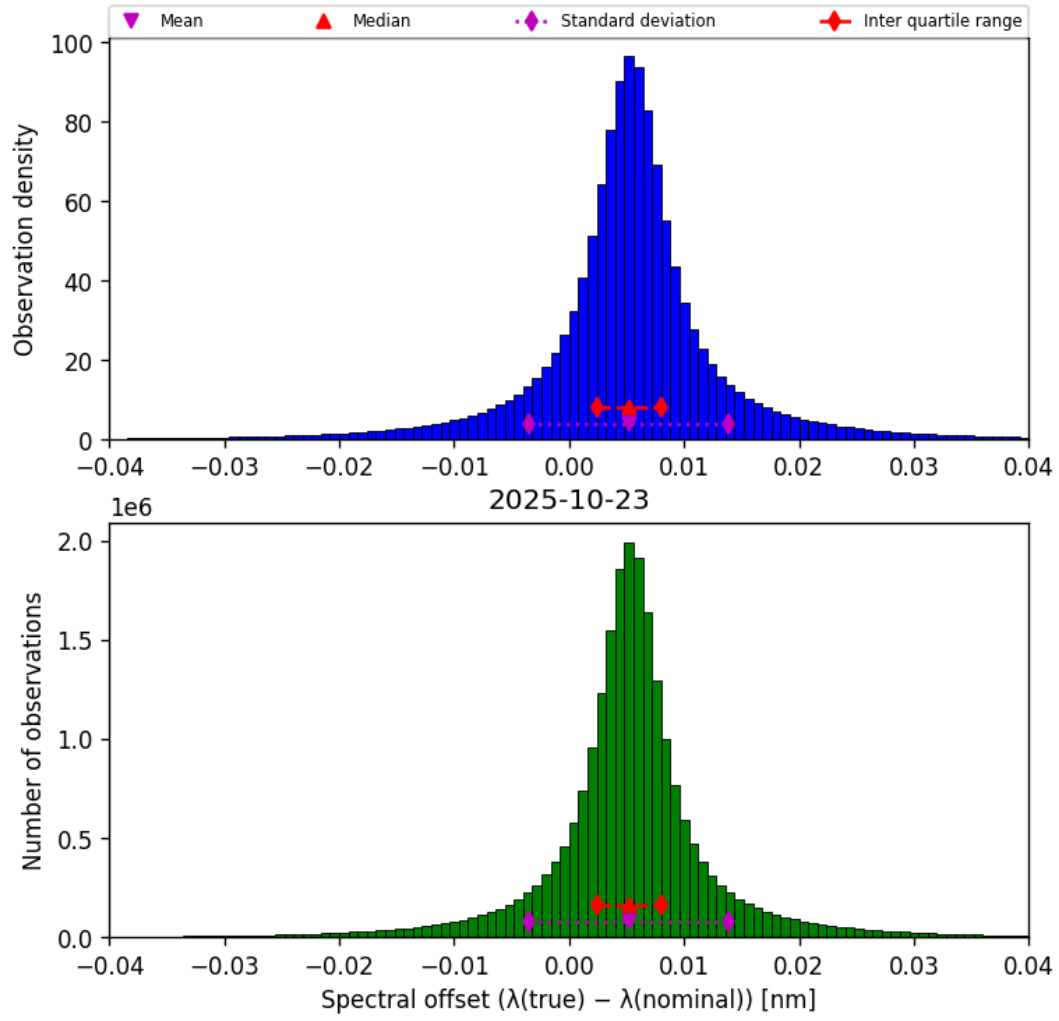
Figure 43: Histogram of “Spectral offset ( \lambda_{\text{true}} - \lambda_{\text{nominal}} )” for 2025-10-23 to 2025-10-24
