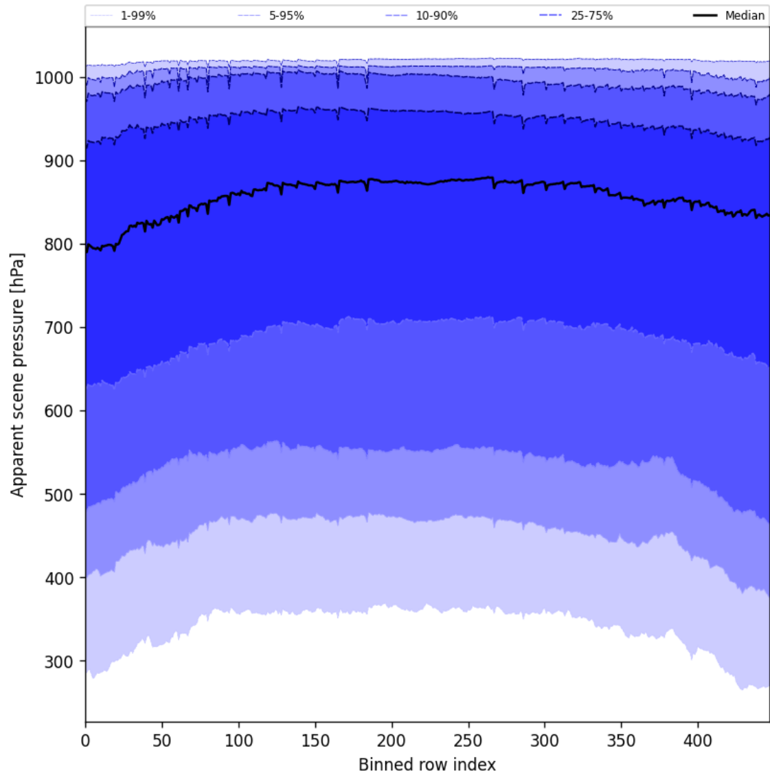
Figure 51: Along track statistics of “Apparent scene pressure” for 2025-10-23 to 2025-10-24
