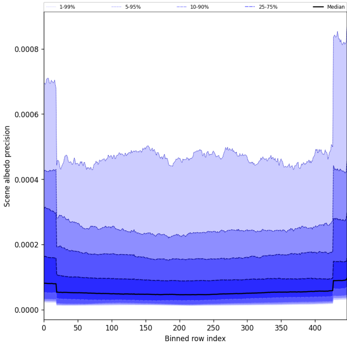
Figure 50: Along track statistics of “Scene albedo precision” for 2025-10-23 to 2025-10-24
