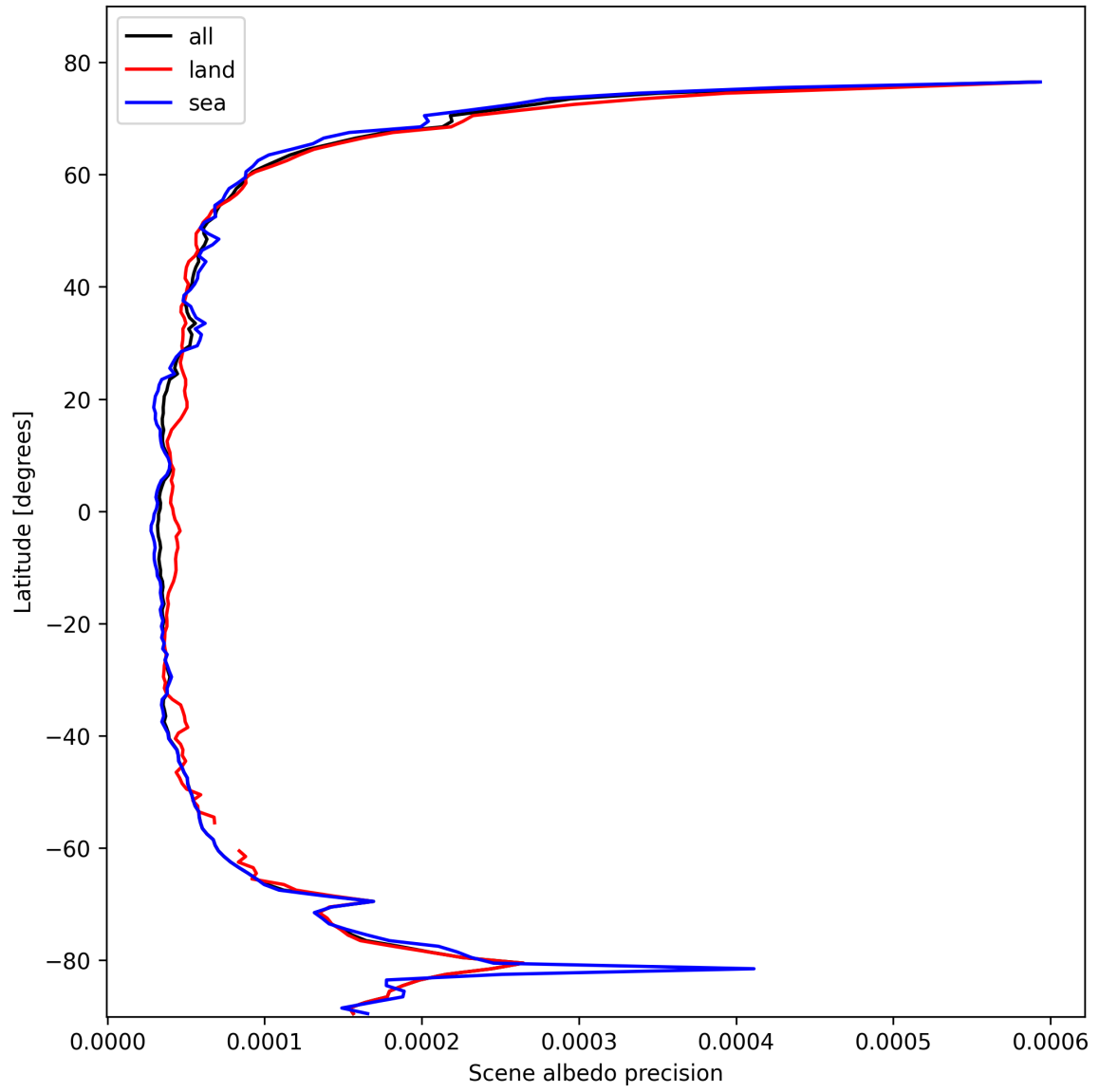
Figure 16: Zonal average of “Scene albedo precision” for 2025-10-23 to 2025-10-24.
