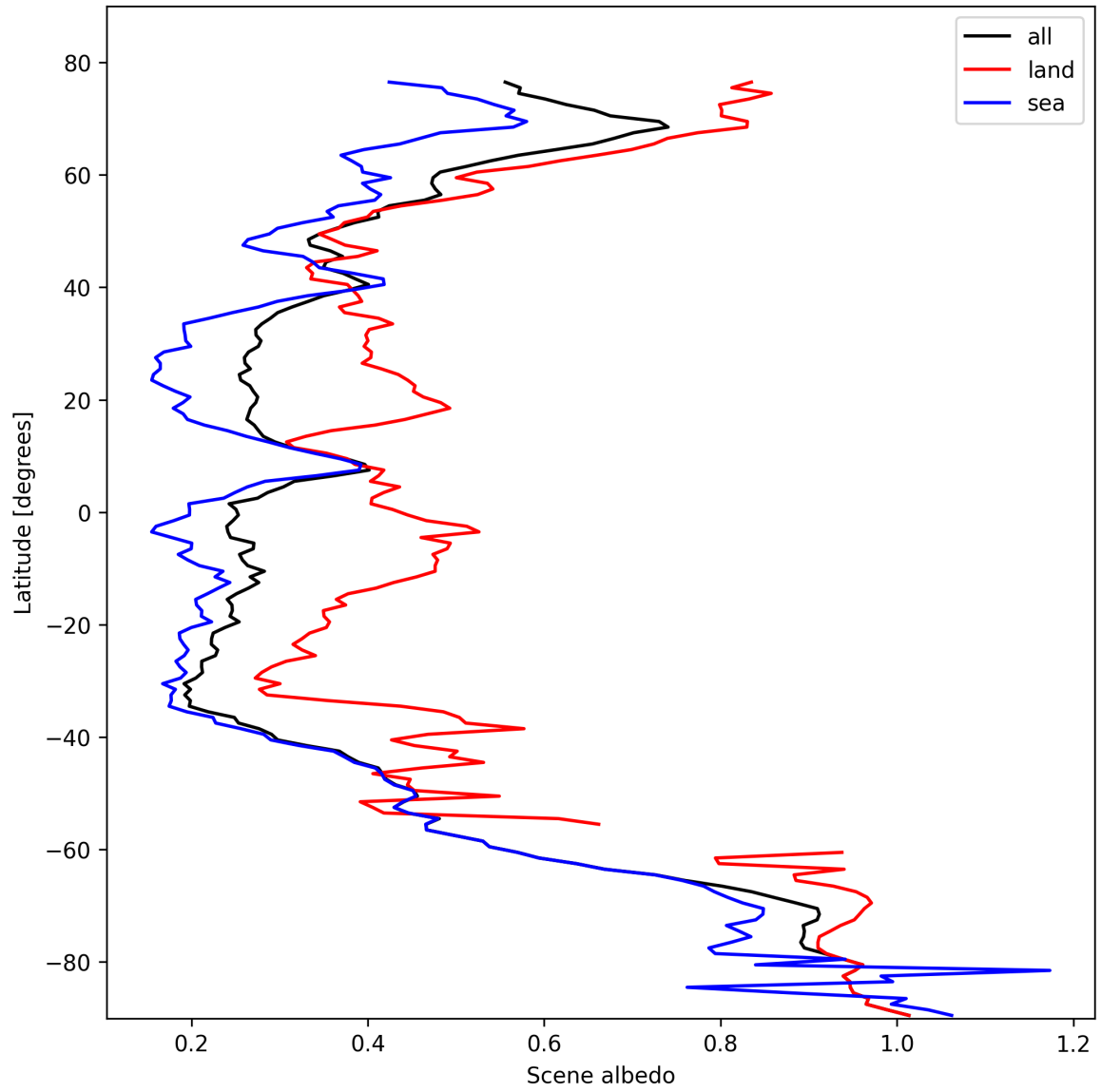
Figure 15: Zonal average of “Scene albedo” for 2025-10-23 to 2025-10-24.
