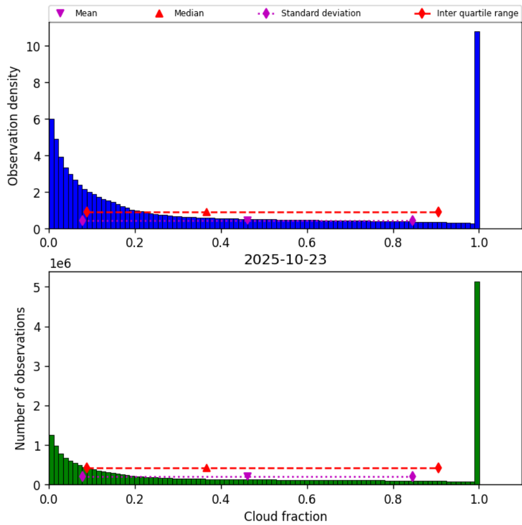
Figure 30: Histogram of “Cloud fraction” for 2025-10-23 to 2025-10-24
