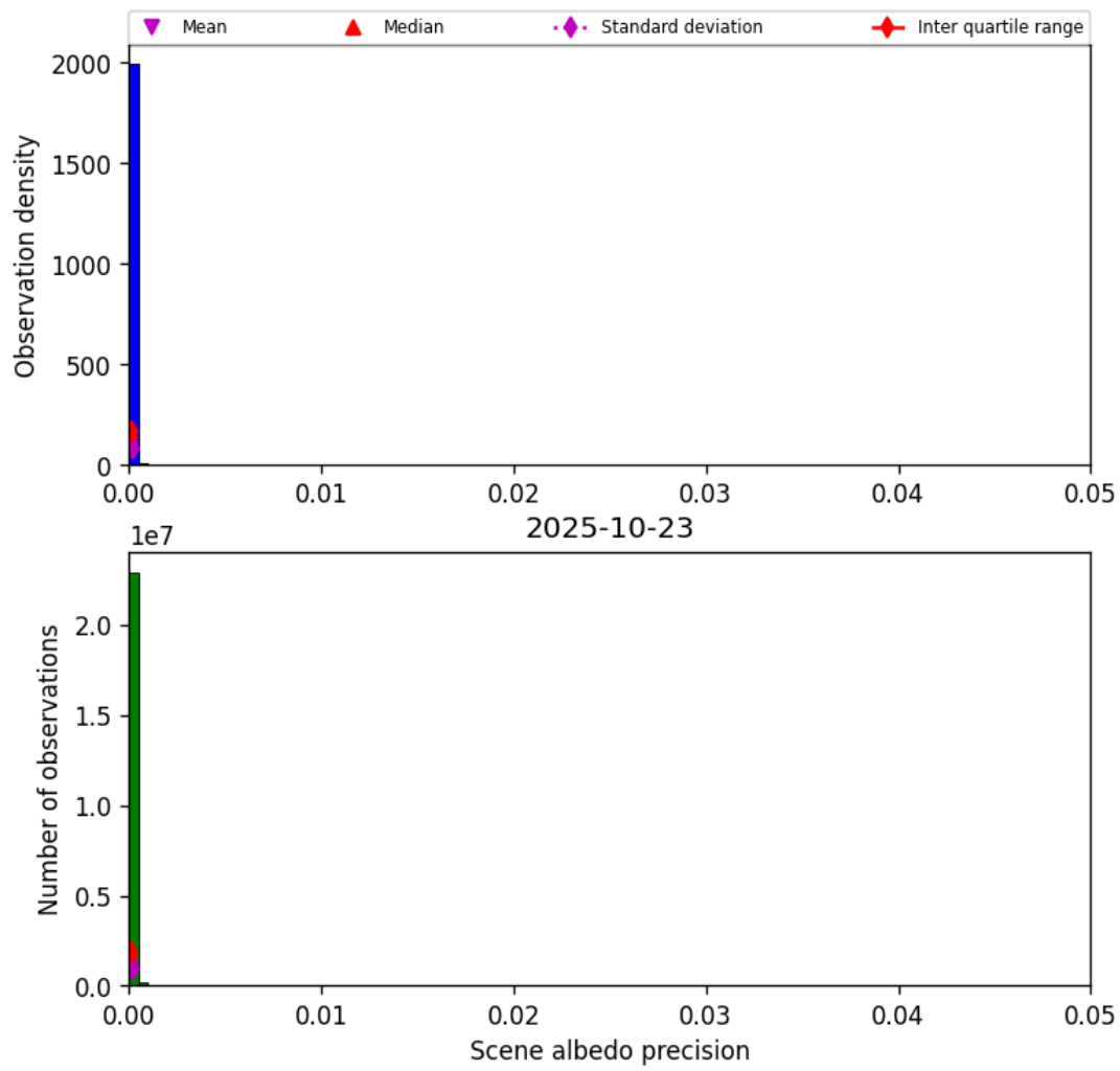
Figure 33: Histogram of “Scene albedo precision” for 2025-10-23 to 2025-10-24
