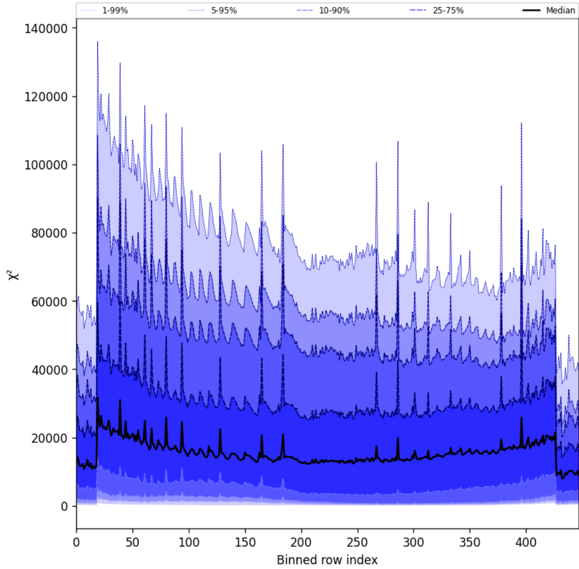
Figure 53: Along track statistics of “ \chi^2 ” for 2025-10-23 to 2025-10-24
