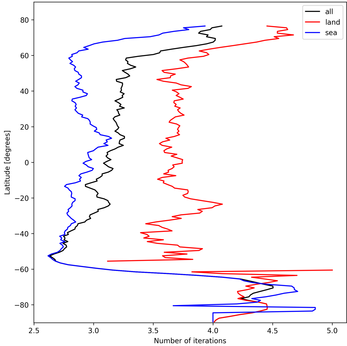
Figure 20: Zonal average of “Number of iterations” for 2025-10-23 to 2025-10-24.
