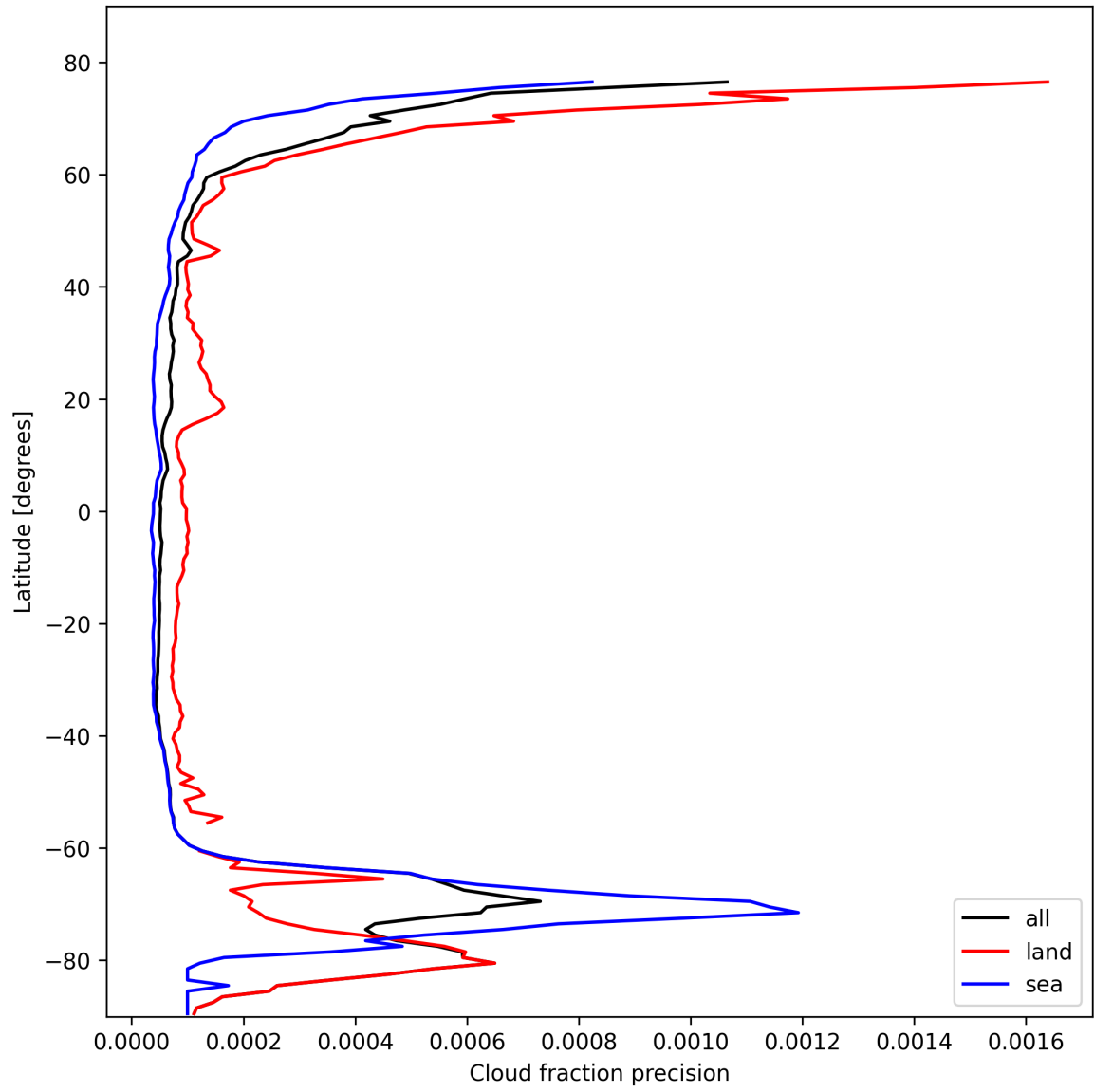
Figure 14: Zonal average of “Cloud fraction precision” for 2025-10-23 to 2025-10-24.
