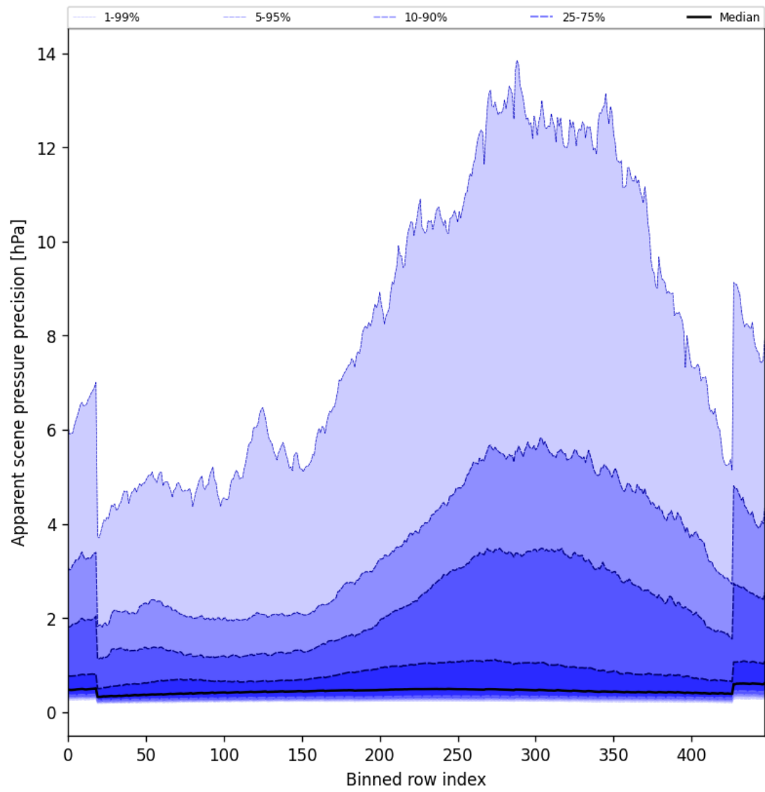
Figure 52: Along track statistics of “Apparent scene pressure precision” for 2025-10-23 to 2025-10-24
