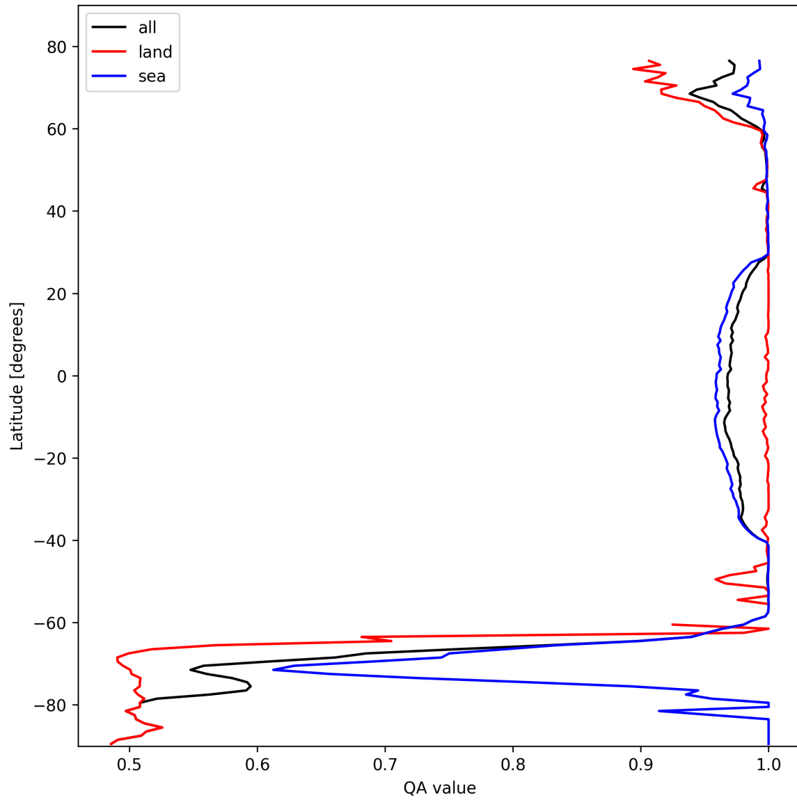
Figure 10: Zonal average of “QA value” for 2025-10-23 to 2025-10-24.
