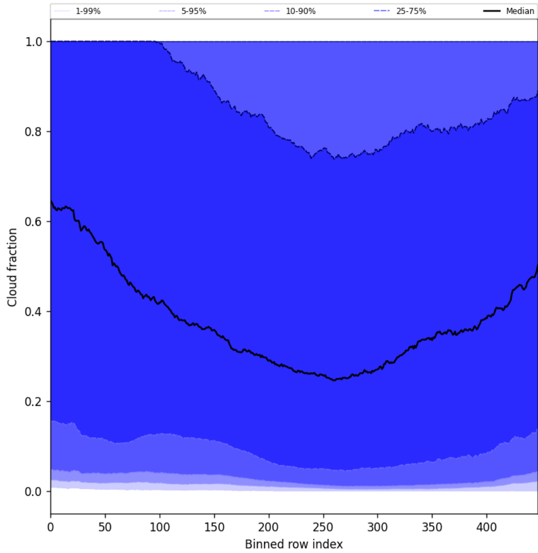
Figure 47: Along track statistics of “Cloud fraction” for 2025-10-23 to 2025-10-24
