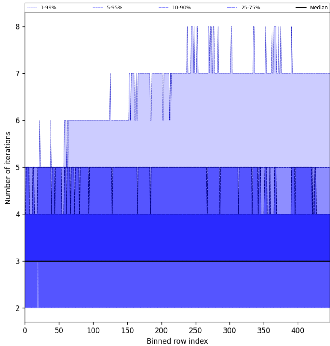
Figure 54: Along track statistics of “Number of iterations” for 2025-10-23 to 2025-10-24
