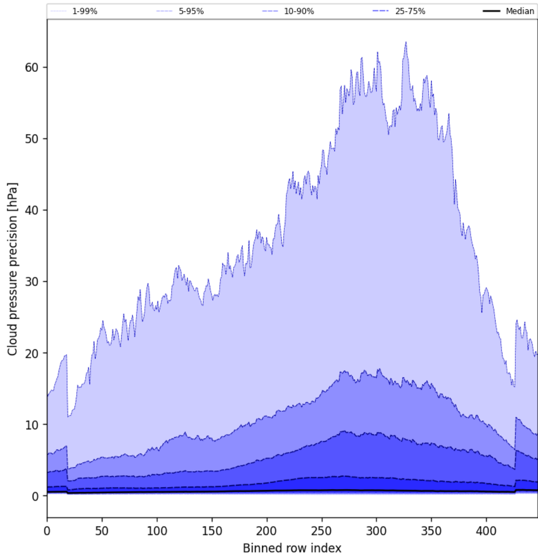
Figure 46: Along track statistics of “Cloud pressure precision” for 2025-10-23 to 2025-10-24
