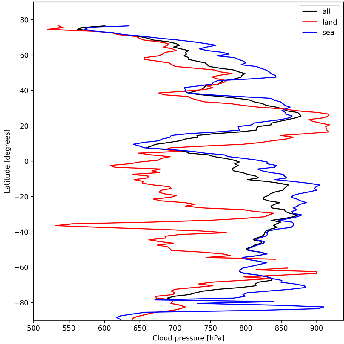
Figure 11: Zonal average of “Cloud pressure” for 2025-10-23 to 2025-10-24.
