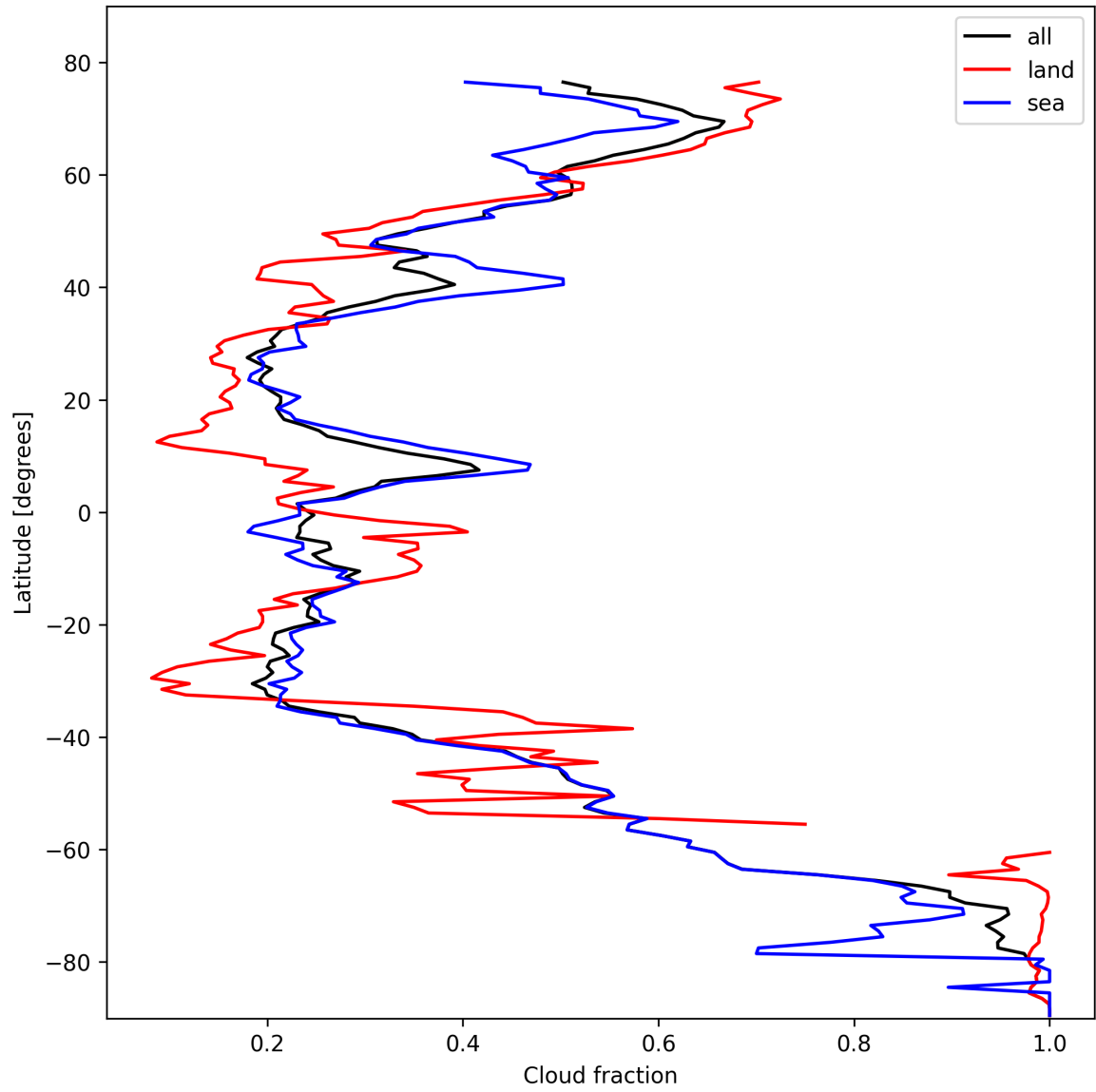
Figure 13: Zonal average of “Cloud fraction” for 2025-10-23 to 2025-10-24.
