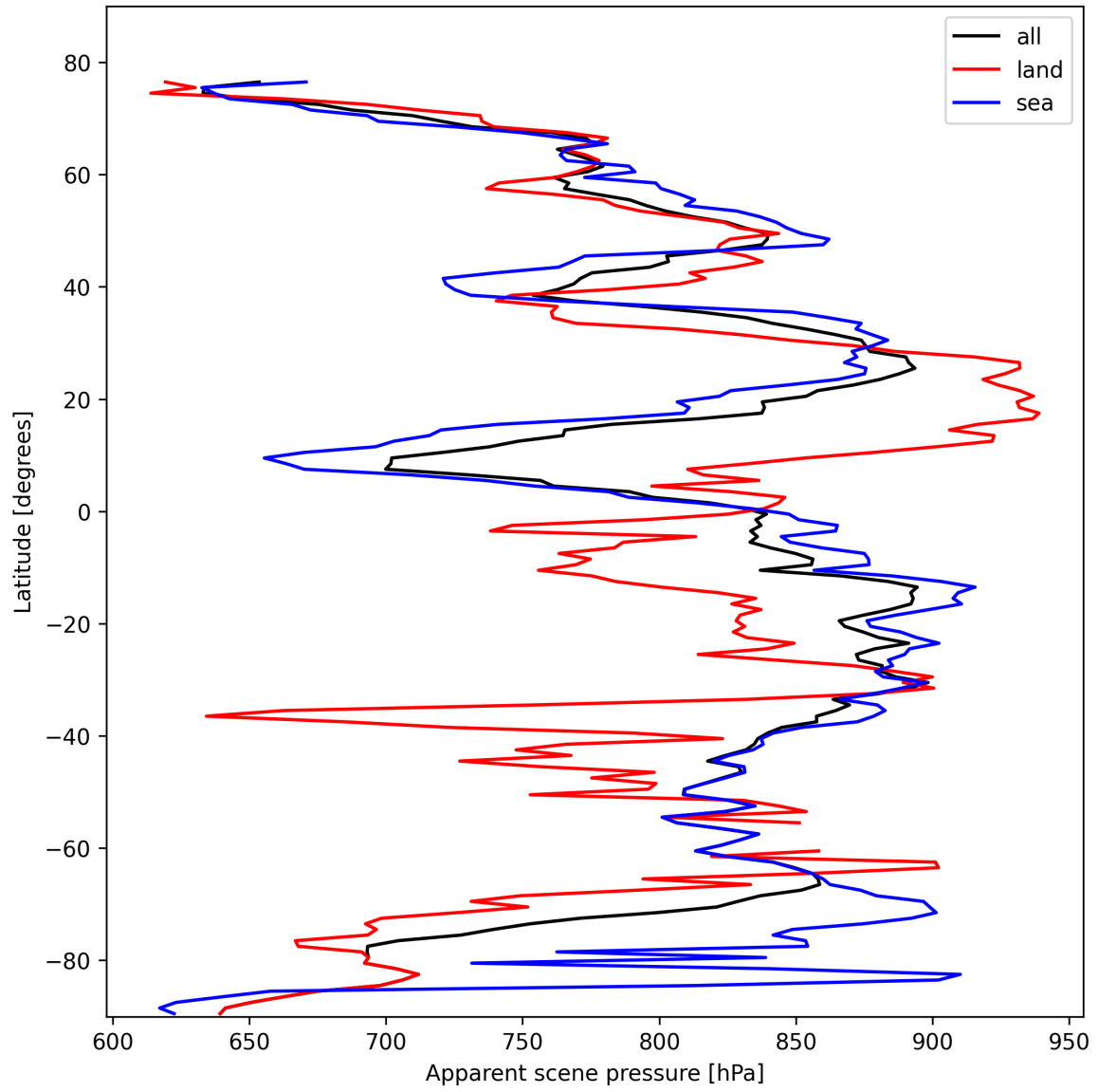
Figure 17: Zonal average of “Apparent scene pressure” for 2025-10-23 to 2025-10-24.
