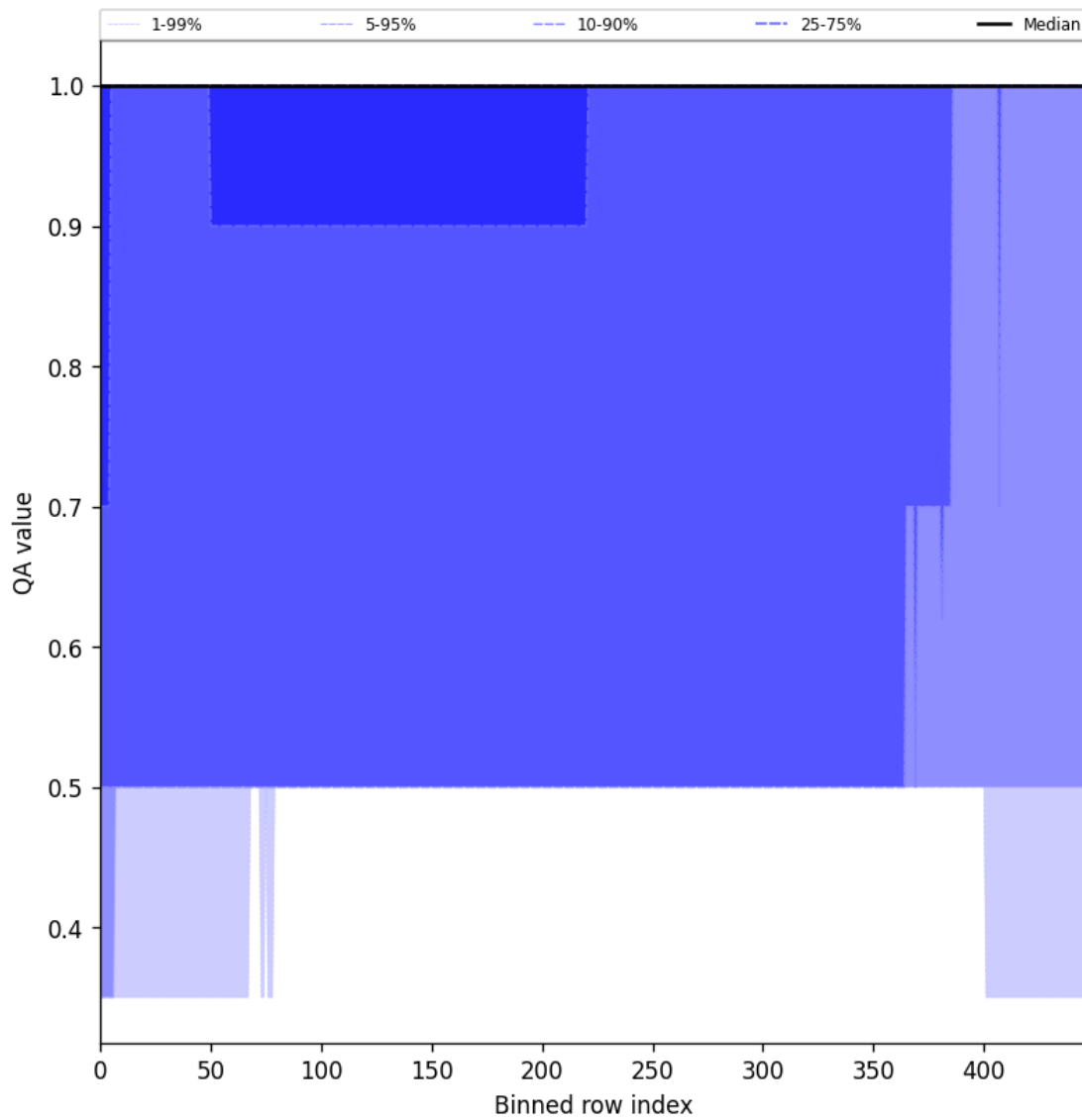
Figure 44: Along track statistics of “QA value” for 2025-10-23 to 2025-10-24
