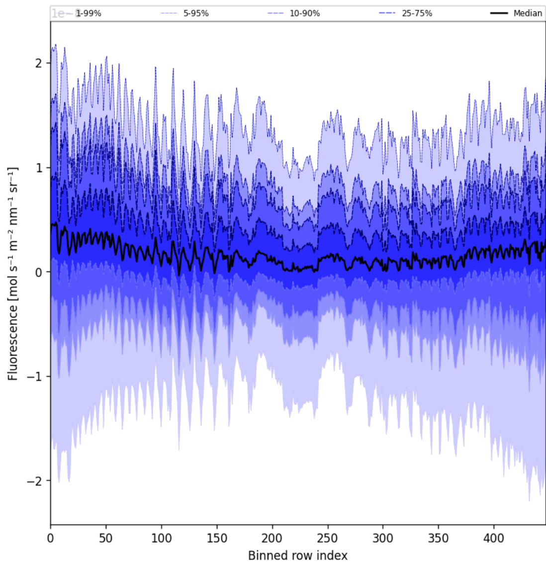
Figure 55: Along track statistics of “Fluorescence” for 2025-10-23 to 2025-10-24
