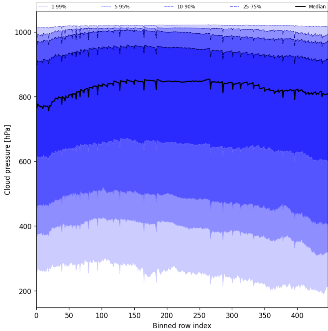
Figure 45: Along track statistics of “Cloud pressure” for 2025-10-23 to 2025-10-24
