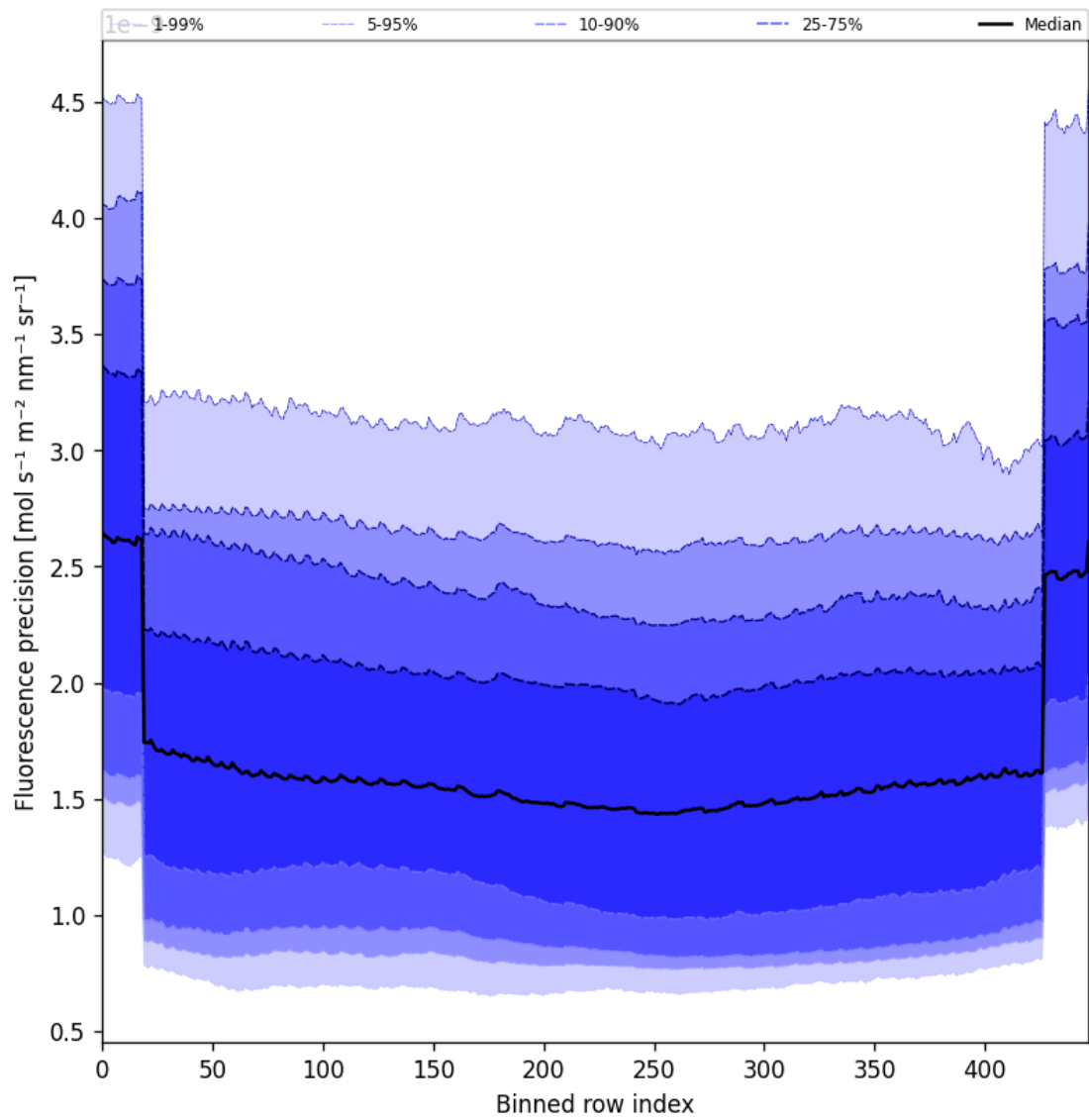
Figure 56: Along track statistics of “Fluorescence precision” for 2025-10-23 to 2025-10-24
