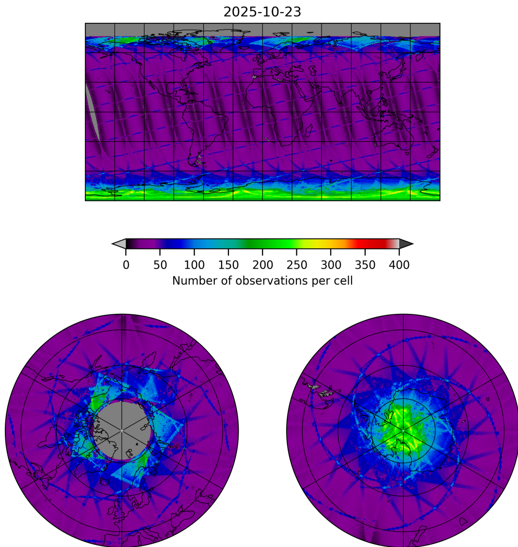
Figure 9: Map of the number of observations for 2025-10-23 to 2025-10-24
