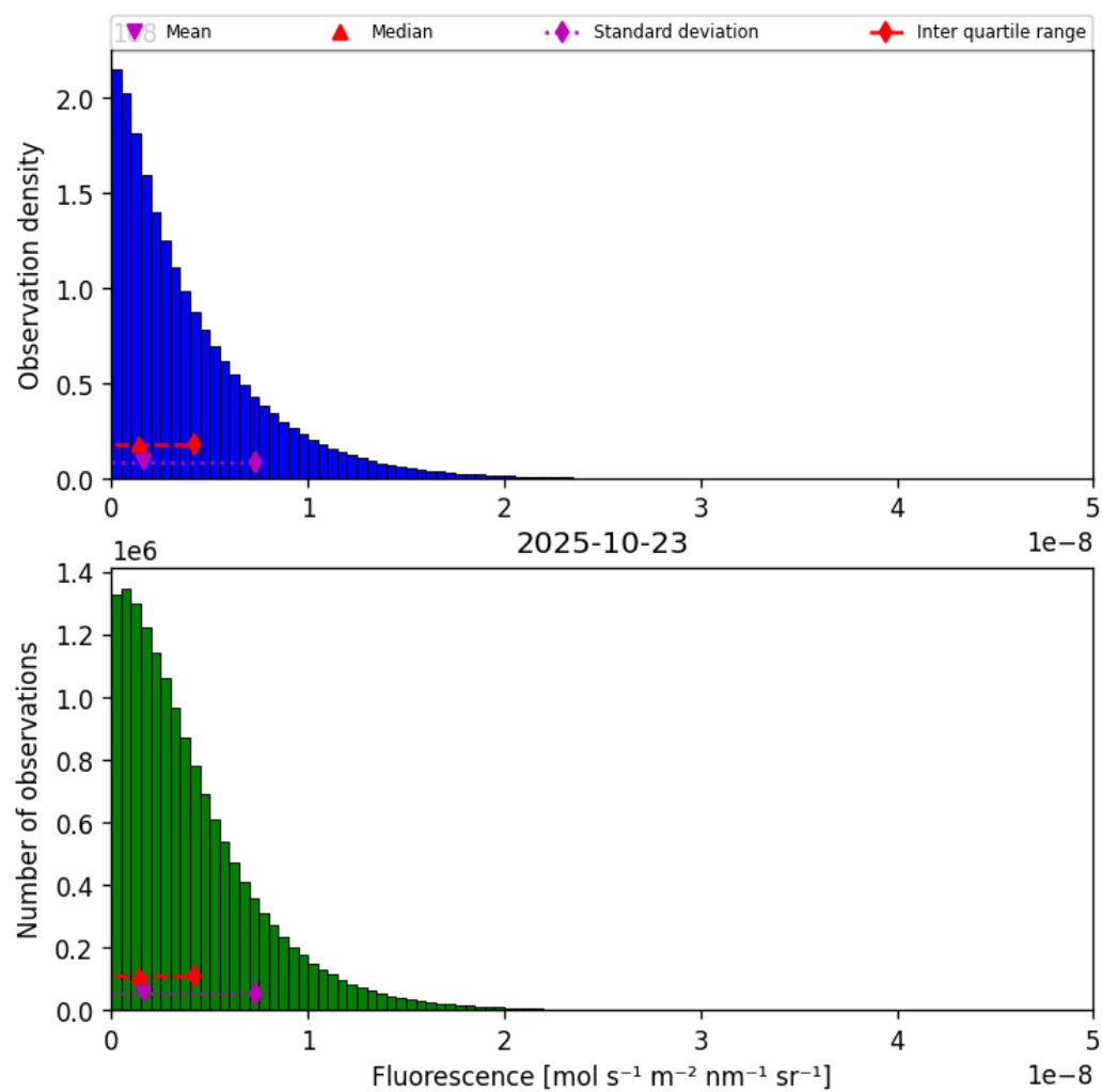
Figure 38: Histogram of “Fluorescence” for 2025-10-23 to 2025-10-24
