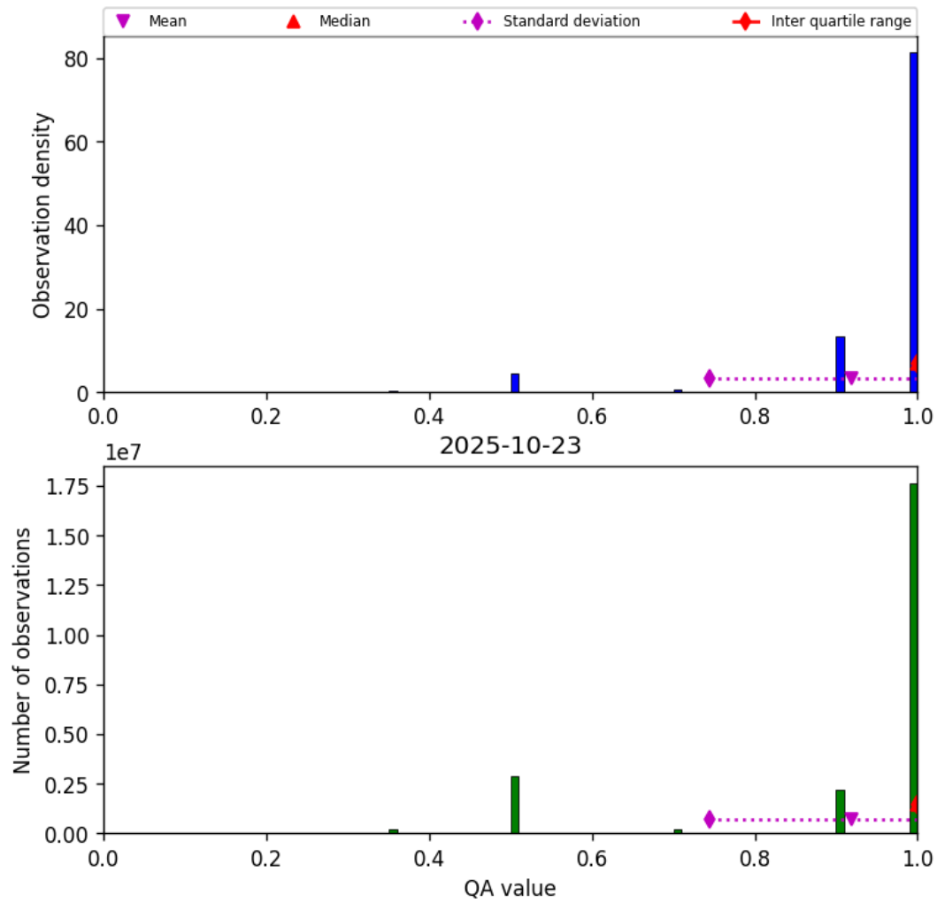
Figure 27: Histogram of “QA value” for 2025-10-23 to 2025-10-24
