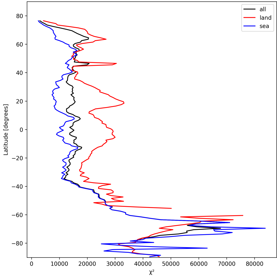
Figure 19: Zonal average of “ \chi^2 ” for 2025-10-23 to 2025-10-24.
