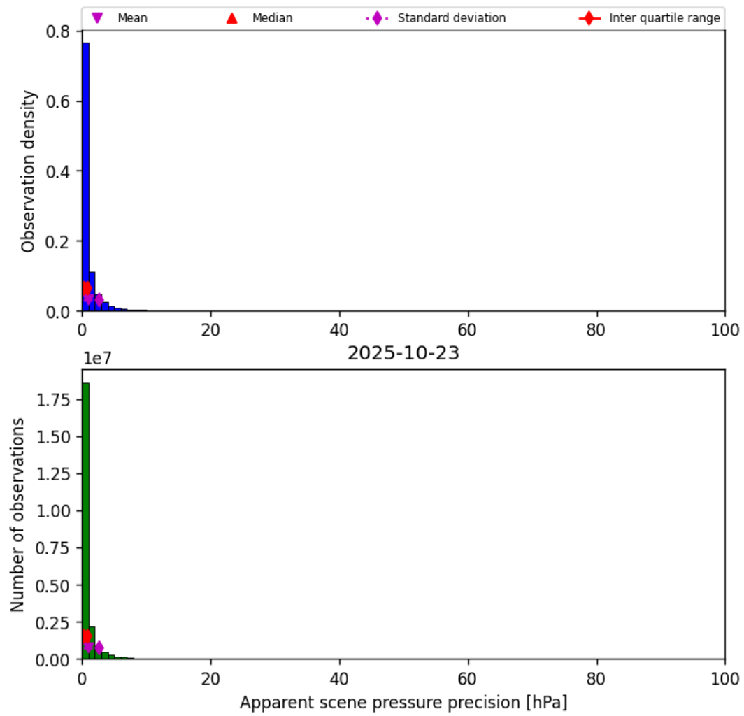
Figure 35: Histogram of “Apparent scene pressure precision” for 2025-10-23 to 2025-10-24
