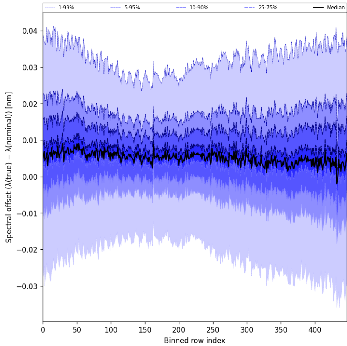
Figure 60: Along track statistics of “Spectral offset ( \lambda_{\text{true}} - \lambda_{\text{nominal}} )” for 2025-10-23 to 2025-10-24
