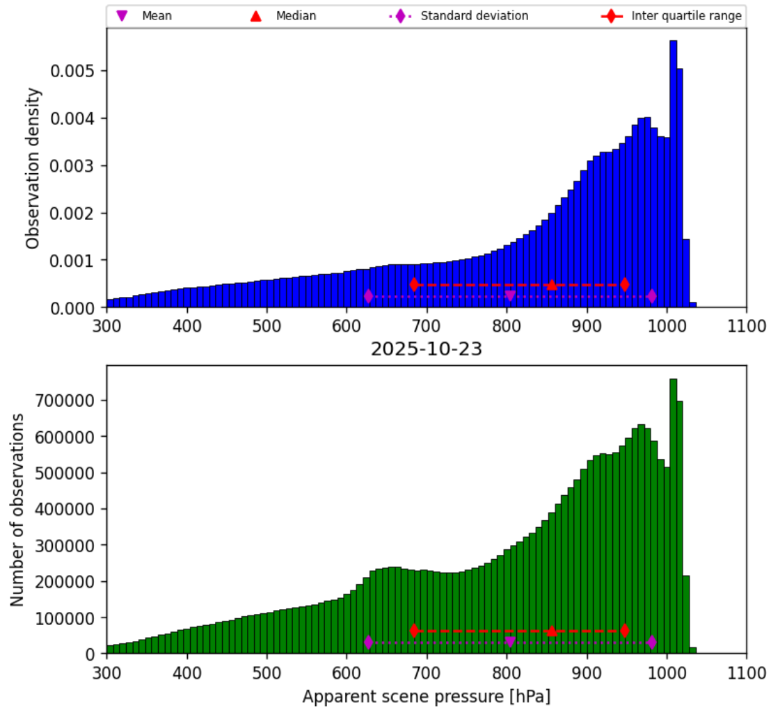
Figure 34: Histogram of “Apparent scene pressure” for 2025-10-23 to 2025-10-24
