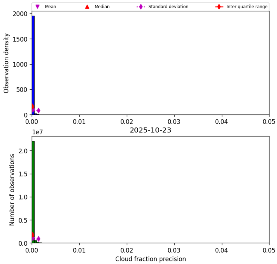
Figure 31: Histogram of “Cloud fraction precision” for 2025-10-23 to 2025-10-24
