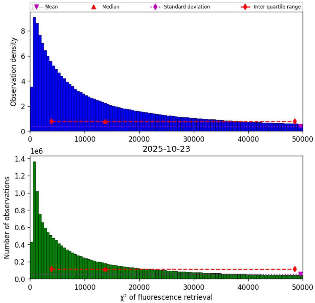
Figure 40: Histogram of “ \chi^2 of fluorescence retrieval” for 2025-10-23 to 2025-10-24
