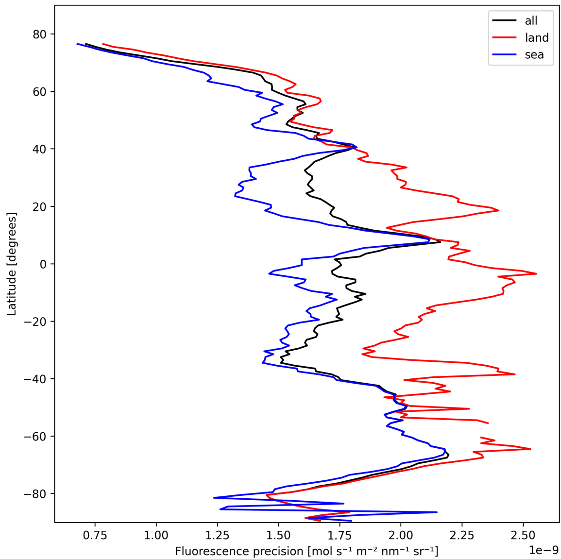
Figure 22: Zonal average of “Fluorescence precision” for 2025-10-23 to 2025-10-24.
