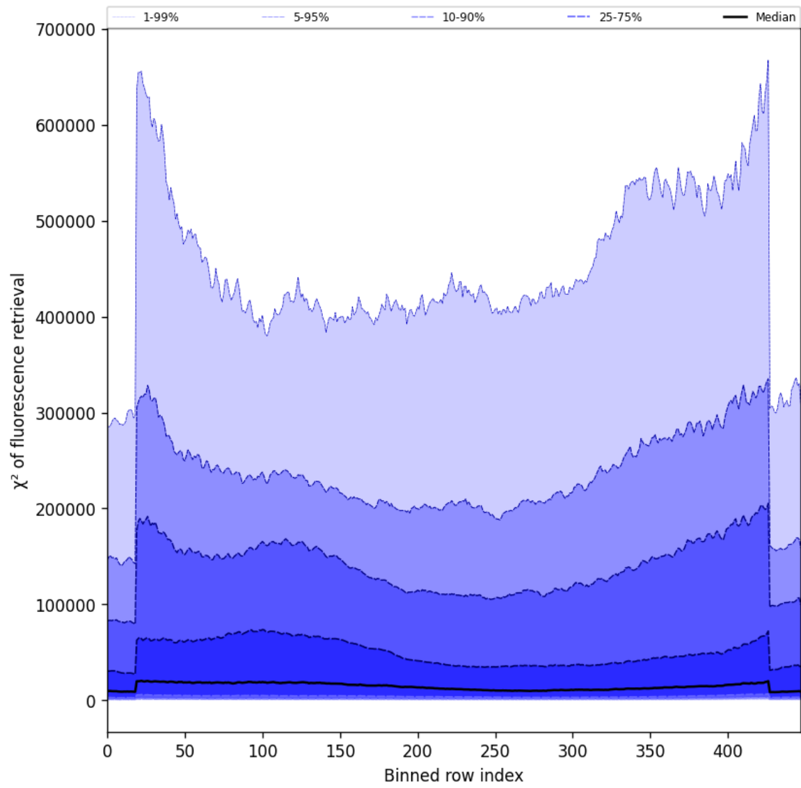
Figure 57: Along track statistics of “ \chi^2 of fluorescence retrieval” for 2025-10-23 to 2025-10-24
