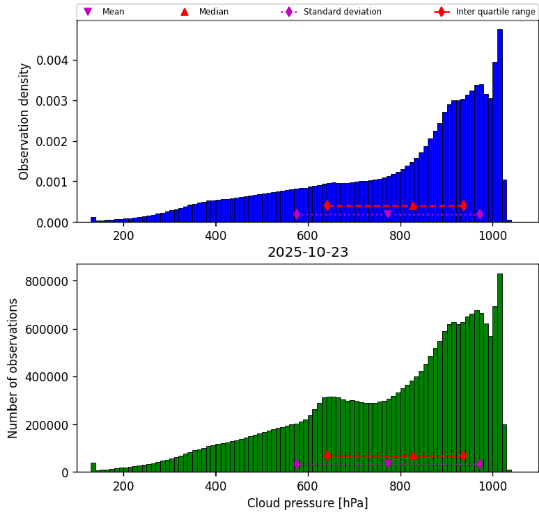
Figure 28: Histogram of “Cloud pressure” for 2025-10-23 to 2025-10-24
