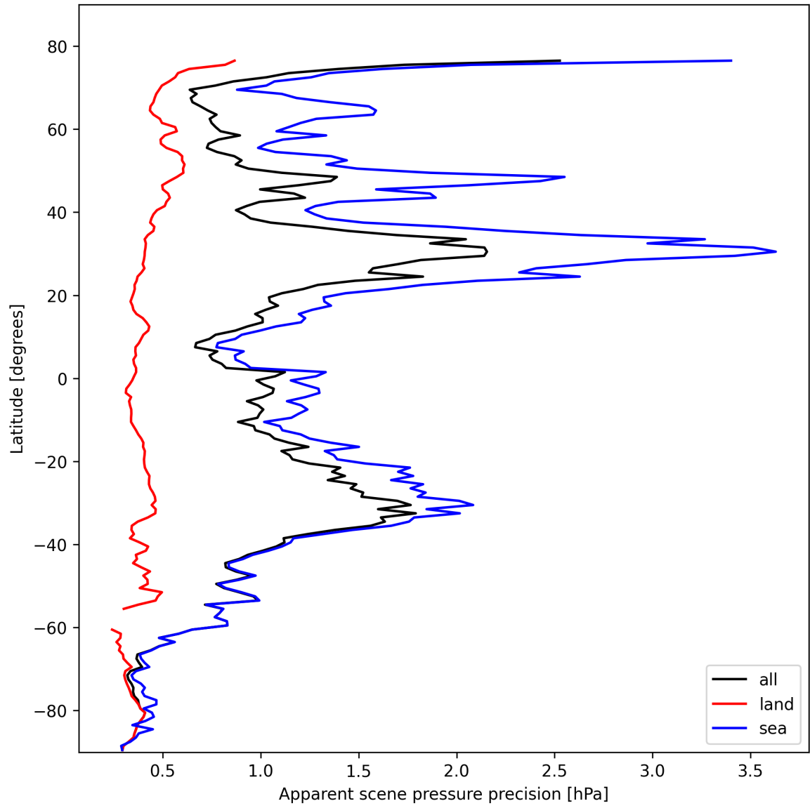
Figure 18: Zonal average of “Apparent scene pressure precision” for 2025-10-23 to 2025-10-24.
