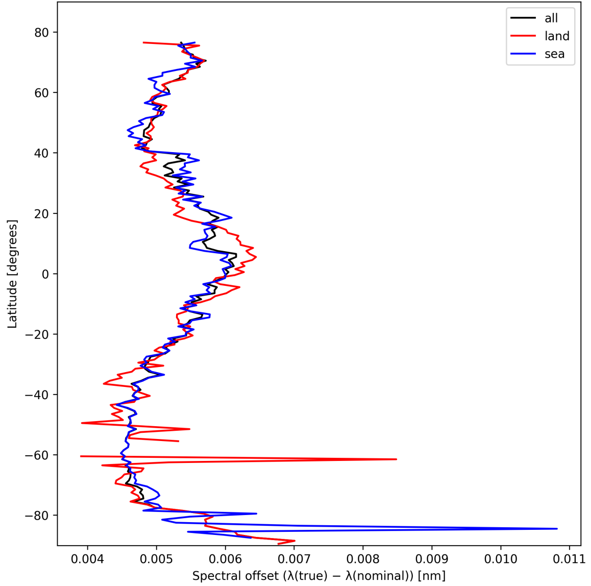
Figure 26: Zonal average of “Spectral offset ( \lambda_{\text{true}} - \lambda_{\text{nominal}} )” for 2025-10-24 to 2025-10-25.
