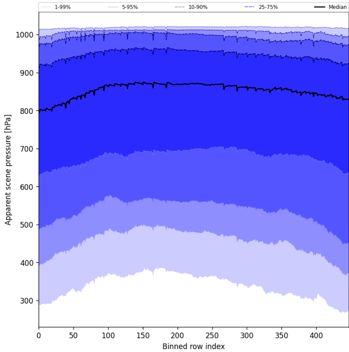
Figure 51: Along track statistics of “Apparent scene pressure” for 2025-10-24 to 2025-10-25
