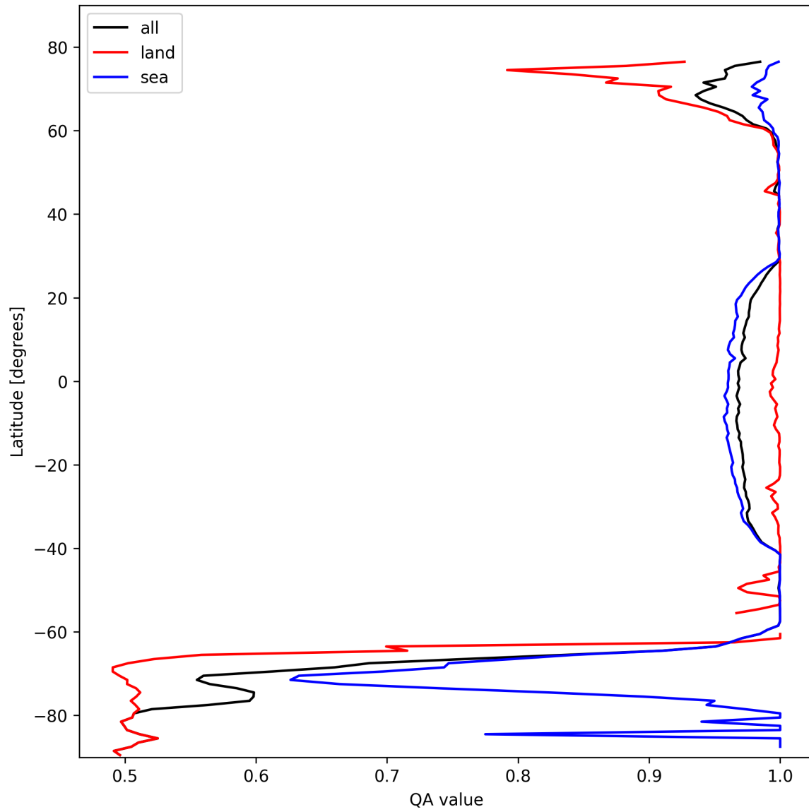
Figure 10: Zonal average of “QA value” for 2025-10-24 to 2025-10-25.
