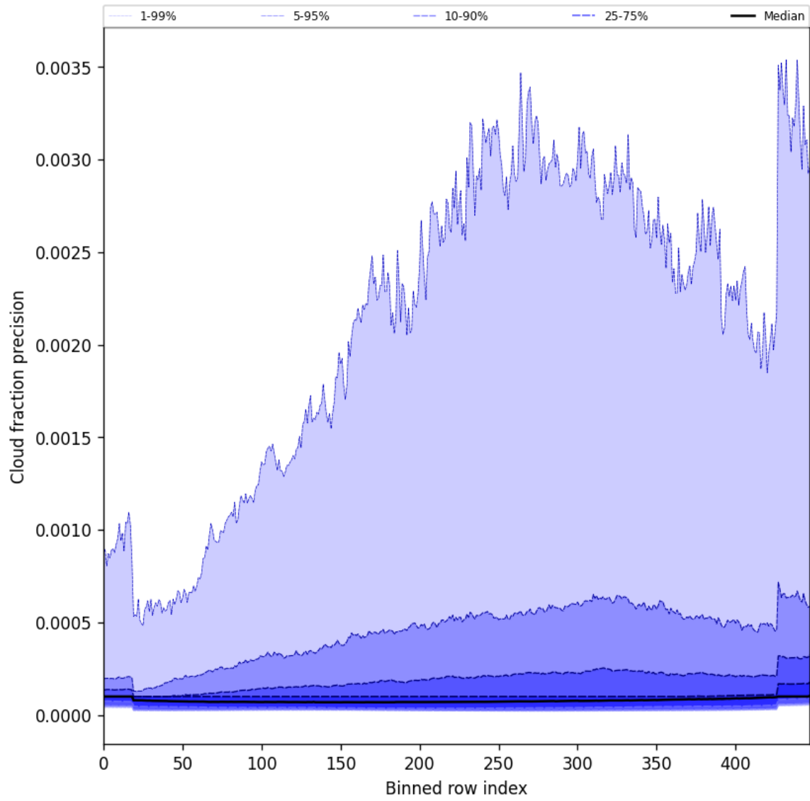
Figure 48: Along track statistics of “Cloud fraction precision” for 2025-10-24 to 2025-10-25
