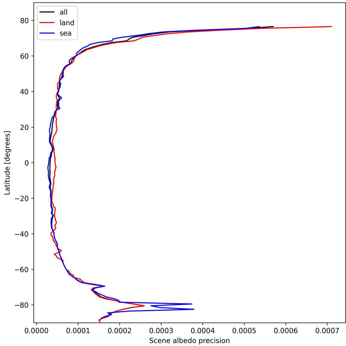
Figure 16: Zonal average of “Scene albedo precision” for 2025-10-24 to 2025-10-25.
