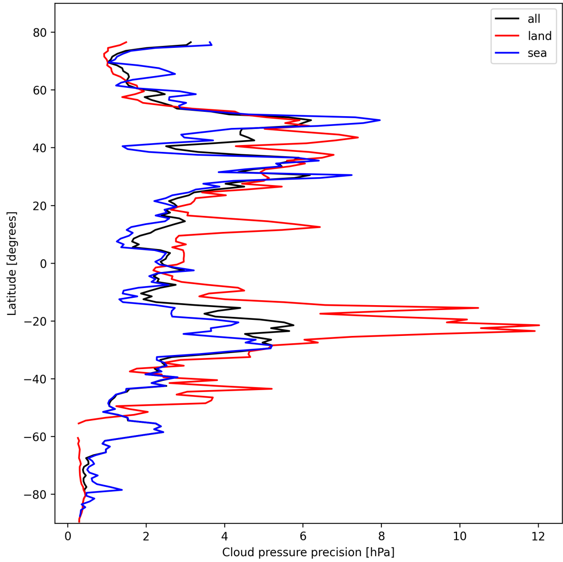
Figure 12: Zonal average of "Cloud pressure precision" for 2025-10-24 to 2025-10-25.
