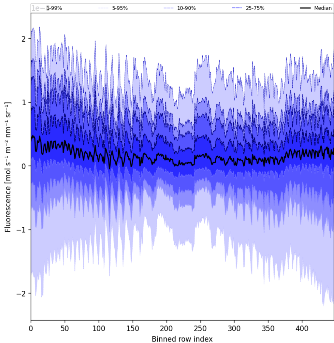
Figure 55: Along track statistics of “Fluorescence” for 2025-10-24 to 2025-10-25
