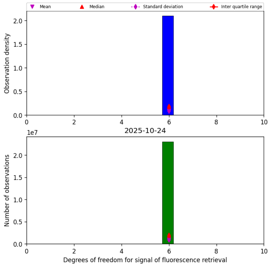
Figure 41: Histogram of “Degrees of freedom for signal of fluorescence retrieval” for 2025-10-24 to 2025-10-25
