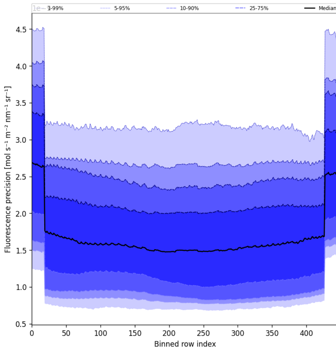
Figure 56: Along track statistics of “Fluorescence precision” for 2025-10-24 to 2025-10-25
