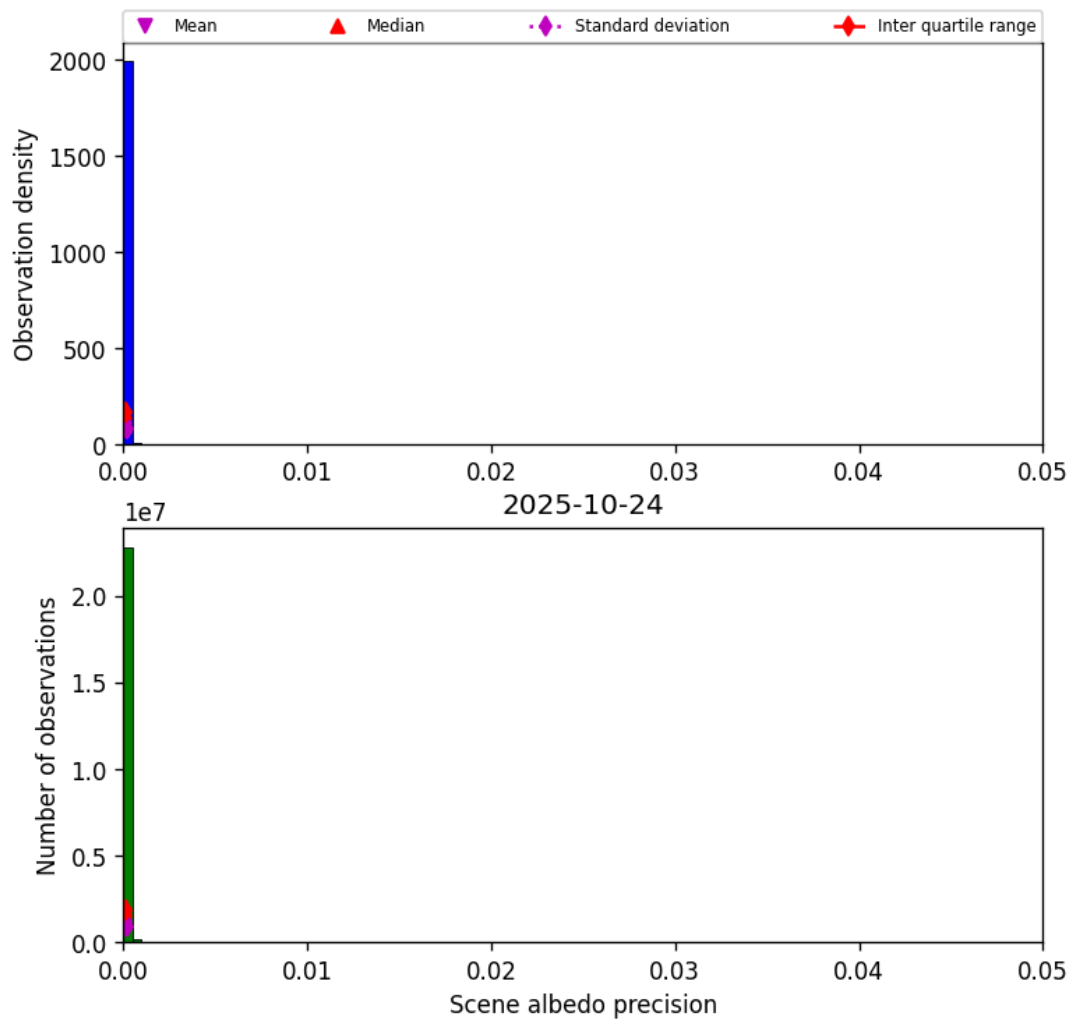
Figure 33: Histogram of “Scene albedo precision” for 2025-10-24 to 2025-10-25
