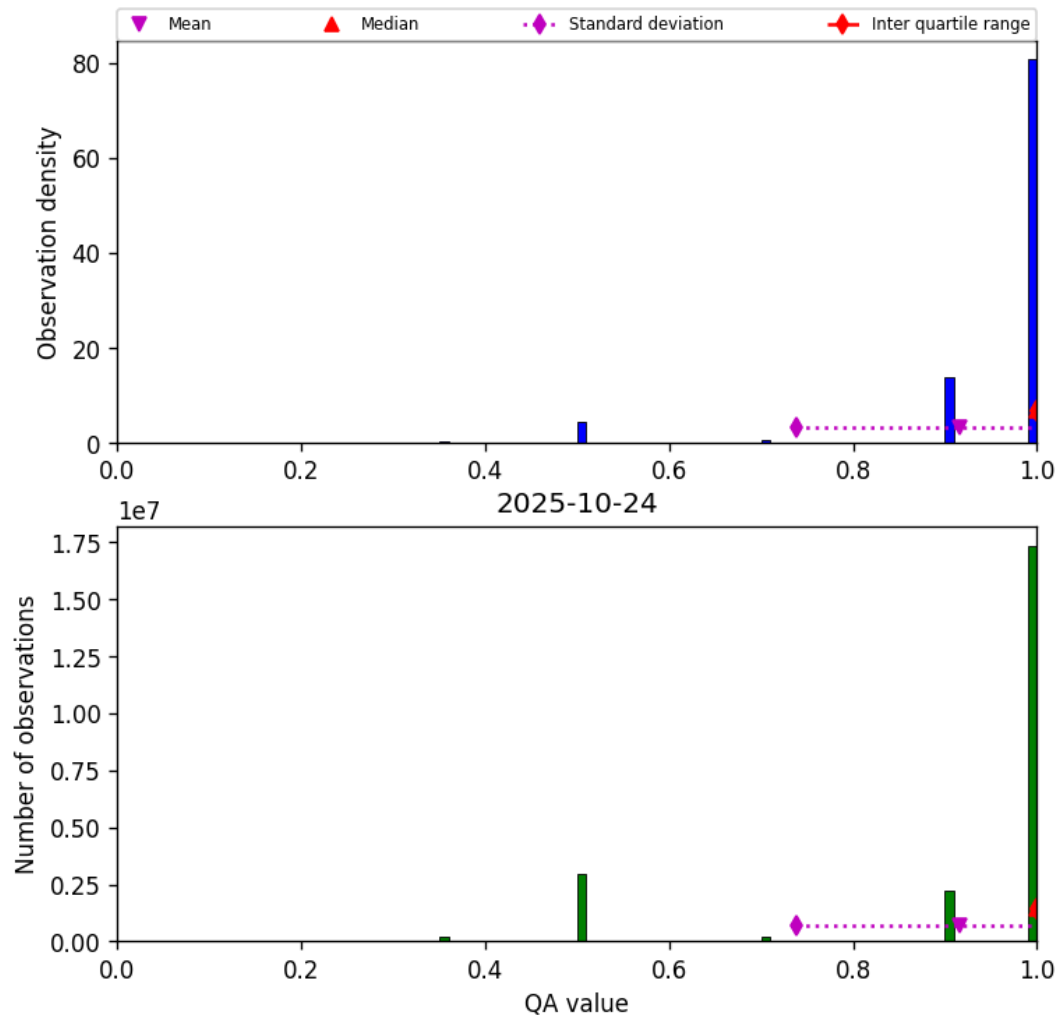
Figure 27: Histogram of “QA value” for 2025-10-24 to 2025-10-25
