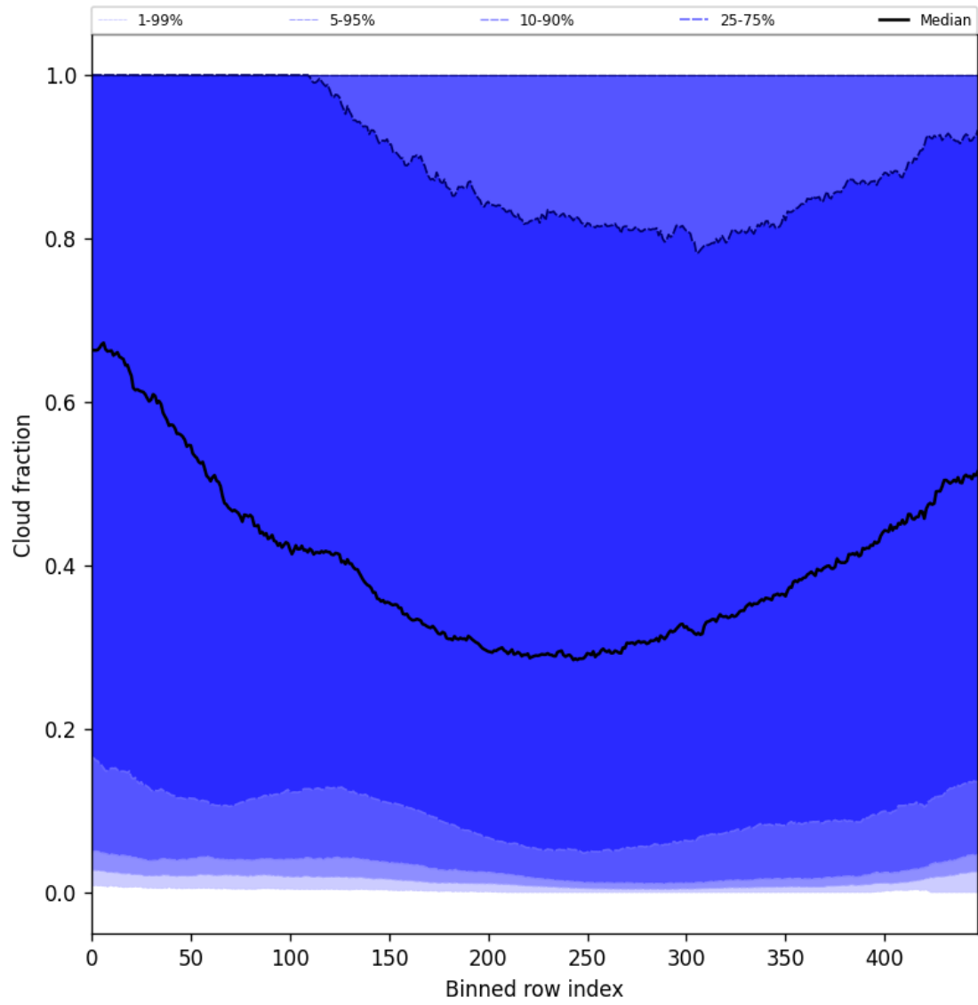
Figure 47: Along track statistics of “Cloud fraction” for 2025-10-24 to 2025-10-25
