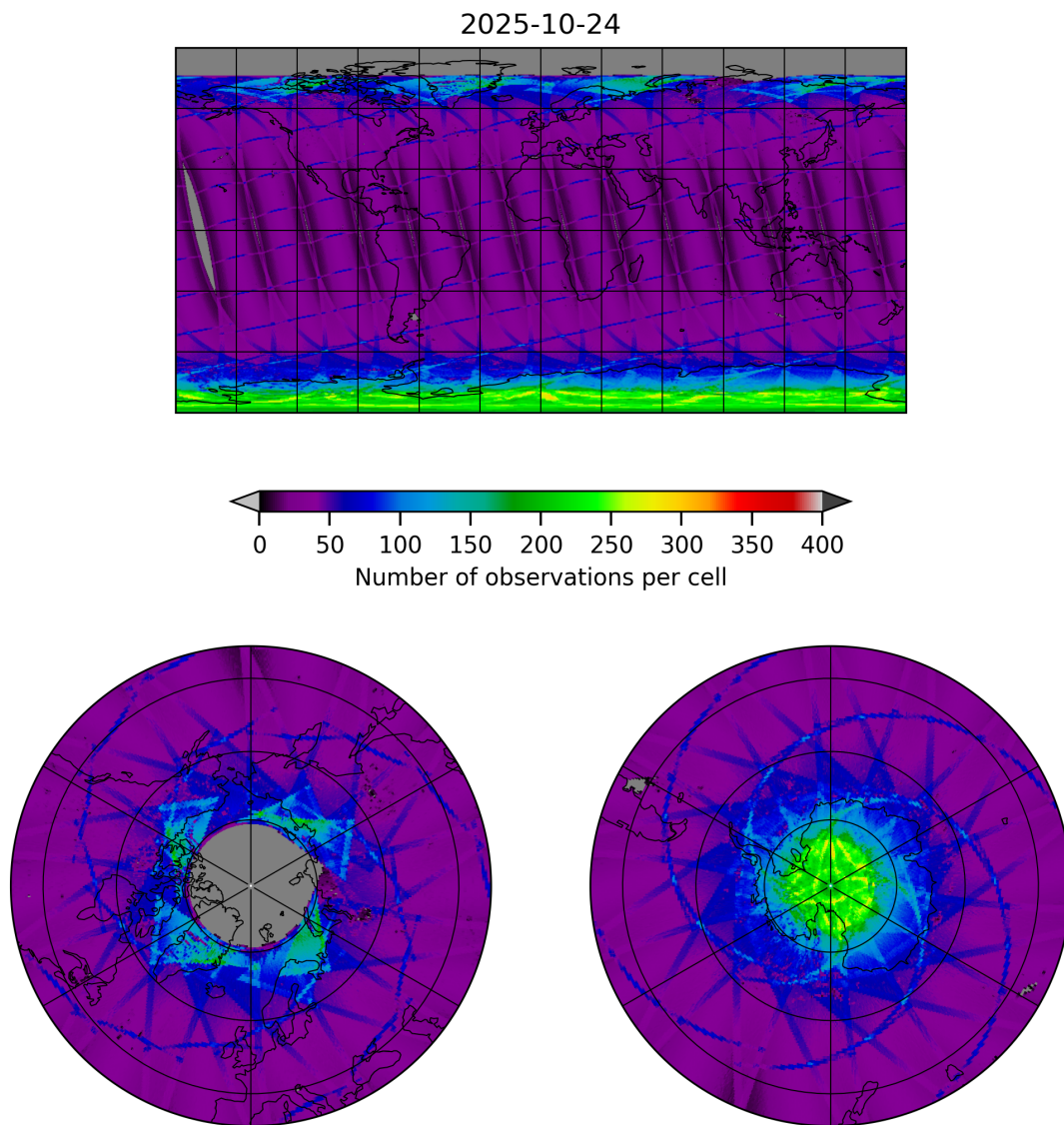
Figure 9: Map of the number of observations for 2025-10-24 to 2025-10-25
