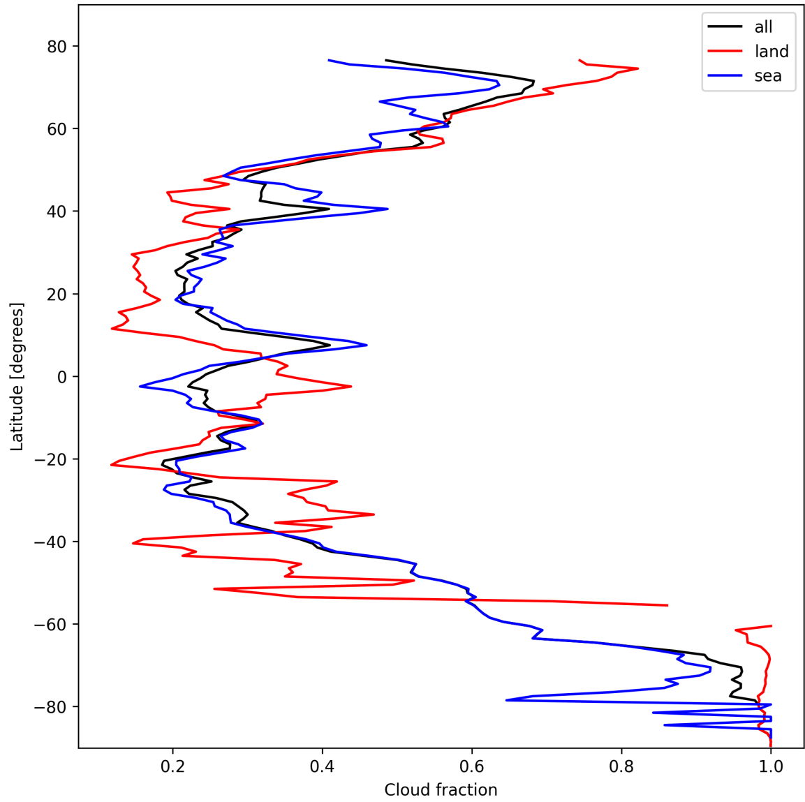
Figure 13: Zonal average of “Cloud fraction” for 2025-10-24 to 2025-10-25.
