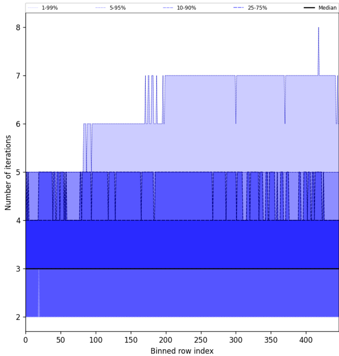
Figure 54: Along track statistics of “Number of iterations” for 2025-10-24 to 2025-10-25
