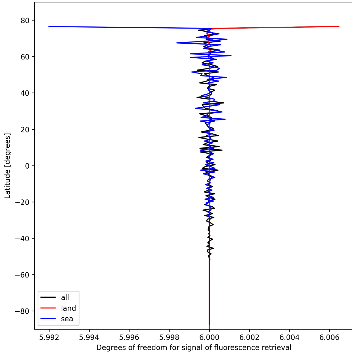
Figure 24: Zonal average of “Degrees of freedom for signal of fluorescence retrieval” for 2025-10-24 to 2025-10-25.
