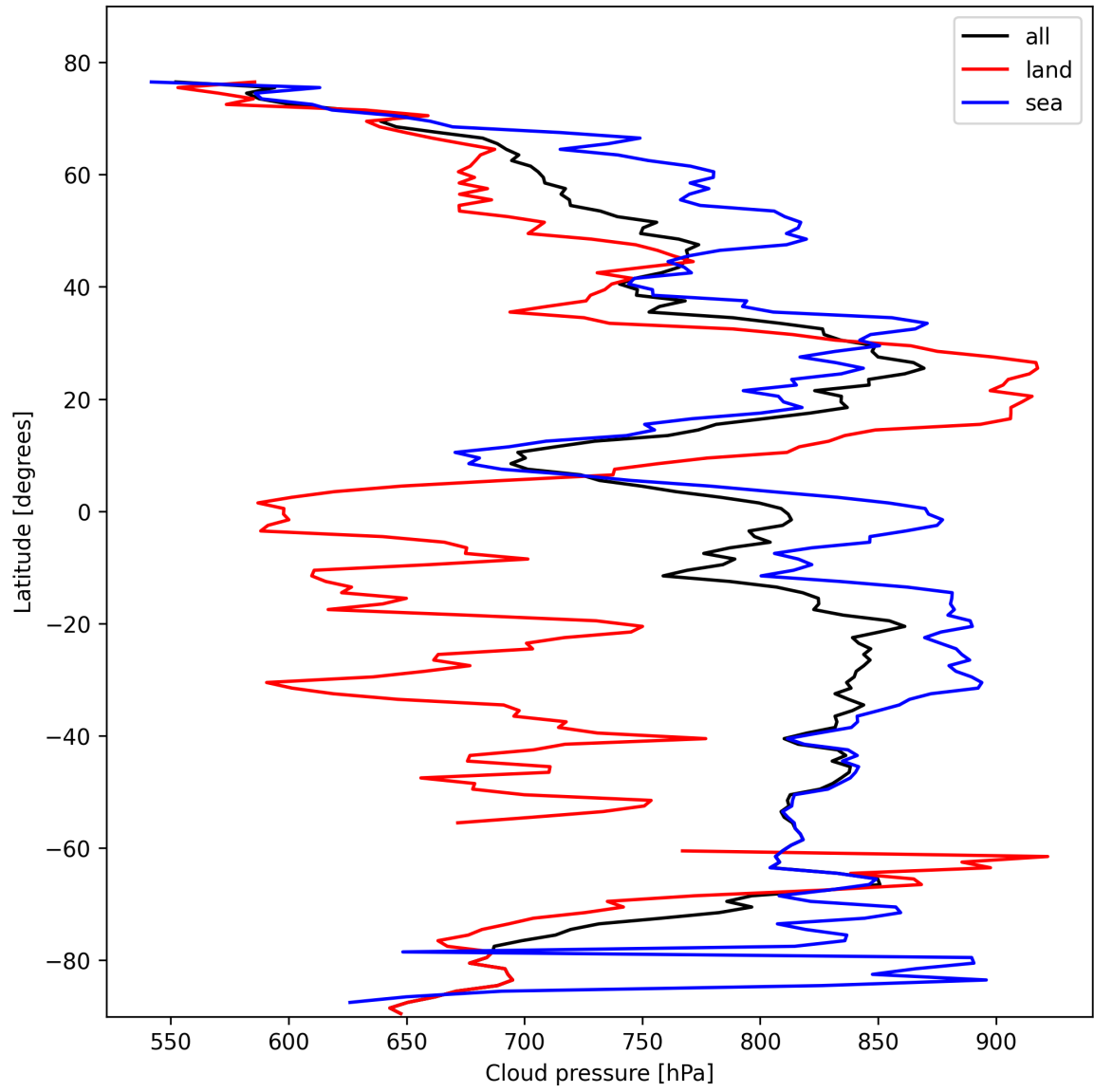
Figure 11: Zonal average of “Cloud pressure” for 2025-10-24 to 2025-10-25.
