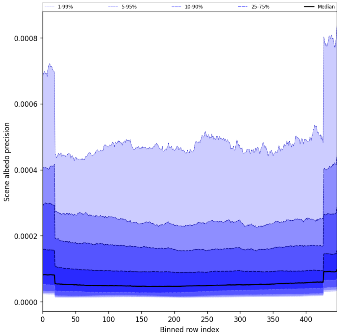
Figure 50: Along track statistics of “Scene albedo precision” for 2025-10-24 to 2025-10-25
