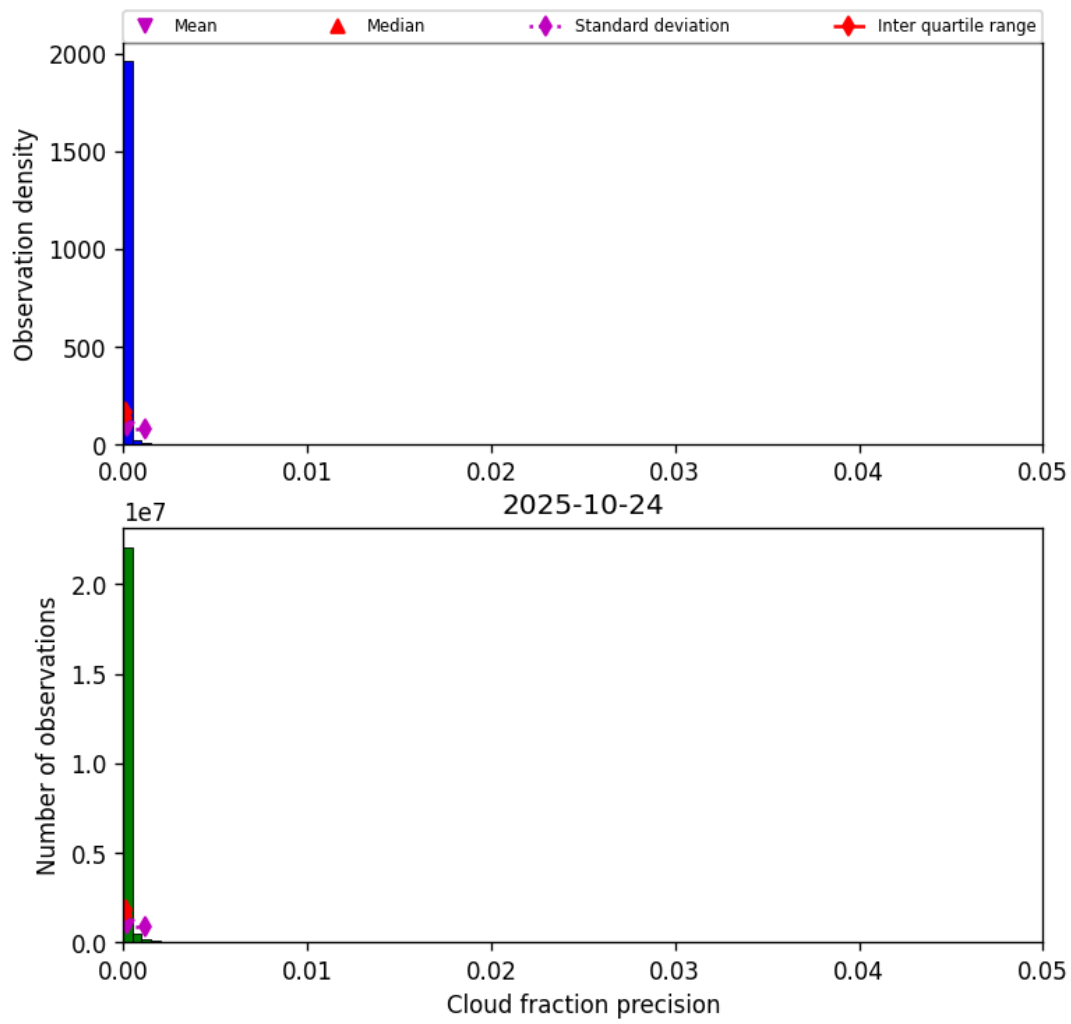
Figure 31: Histogram of “Cloud fraction precision” for 2025-10-24 to 2025-10-25
