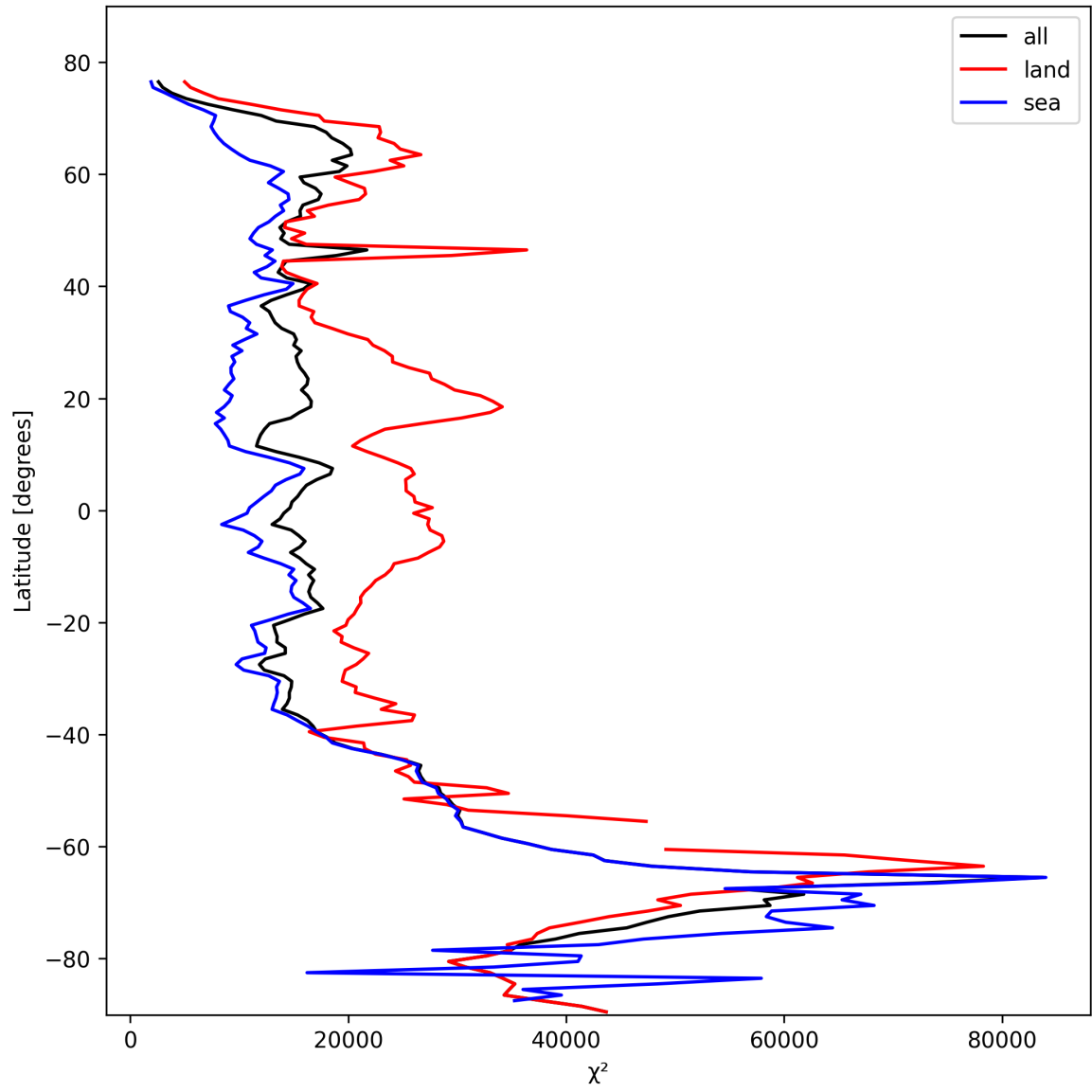
Figure 19: Zonal average of “ \chi^2 ” for 2025-10-24 to 2025-10-25.
