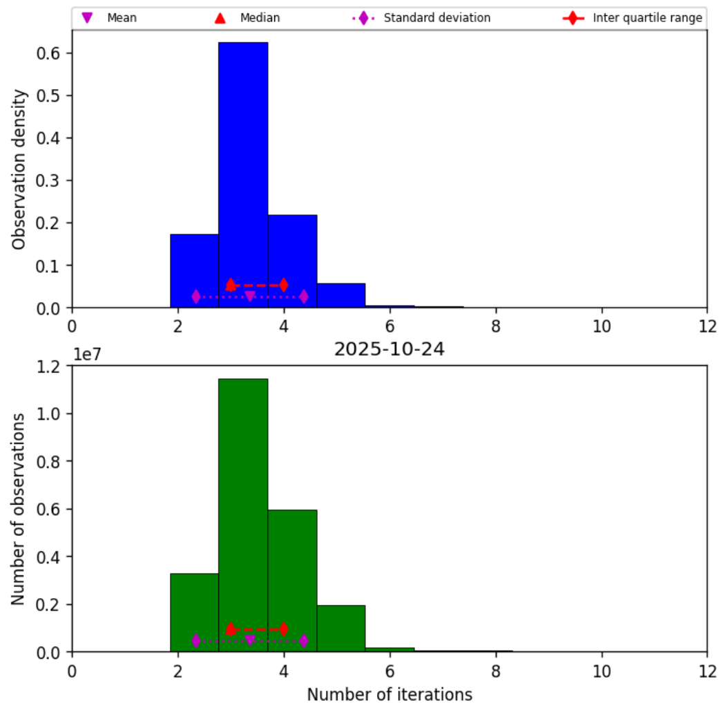
Figure 37: Histogram of “Number of iterations” for 2025-10-24 to 2025-10-25
