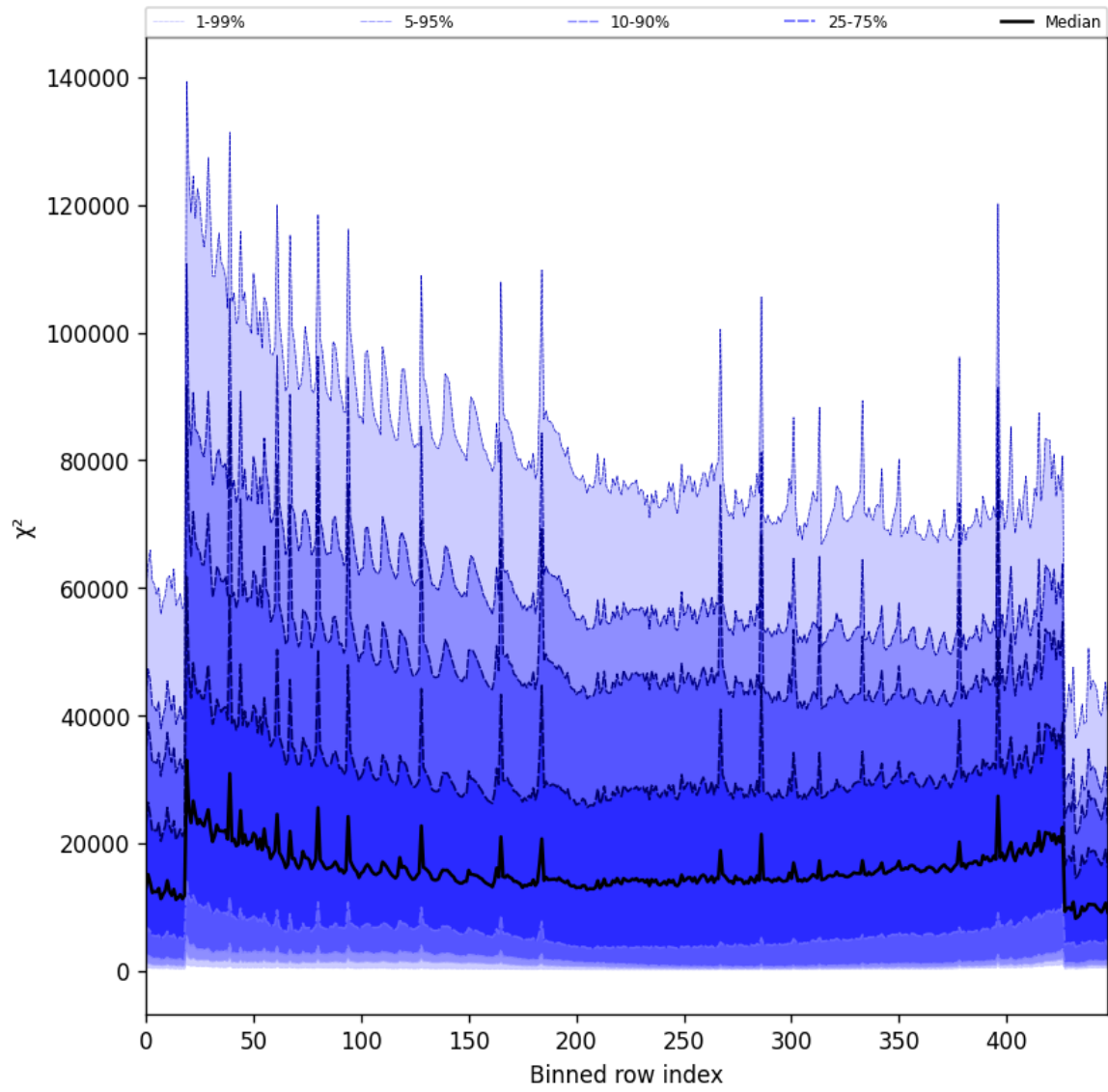
Figure 53: Along track statistics of “ \chi^2 ” for 2025-10-24 to 2025-10-25
