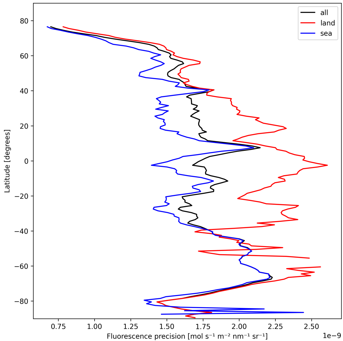
Figure 22: Zonal average of “Fluorescence precision” for 2025-10-24 to 2025-10-25.
