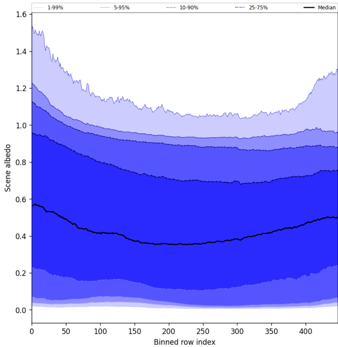
Figure 49: Along track statistics of “Scene albedo” for 2025-10-24 to 2025-10-25
