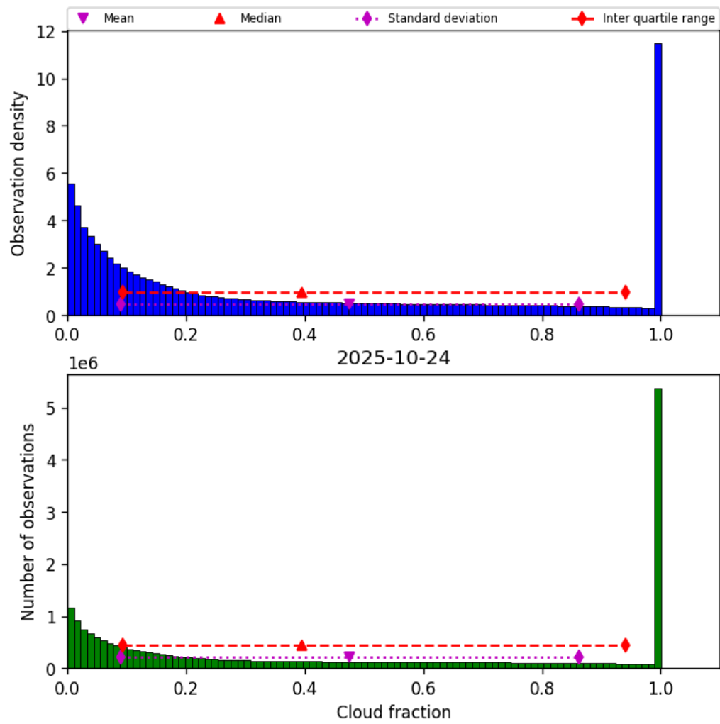
Figure 30: Histogram of “Cloud fraction” for 2025-10-24 to 2025-10-25
