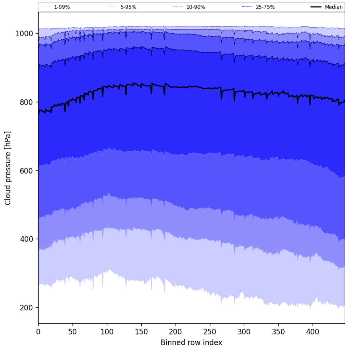
Figure 45: Along track statistics of “Cloud pressure” for 2025-10-24 to 2025-10-25
