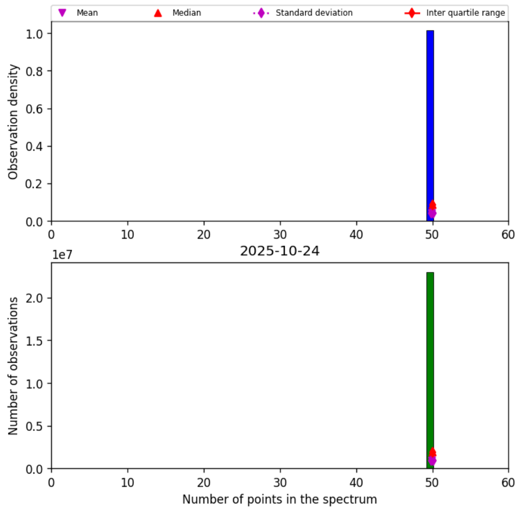
Figure 42: Histogram of “Number of points in the spectrum” for 2025-10-24 to 2025-10-25
