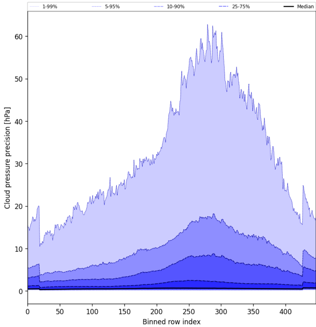
Figure 46: Along track statistics of “Cloud pressure precision” for 2025-10-24 to 2025-10-25
