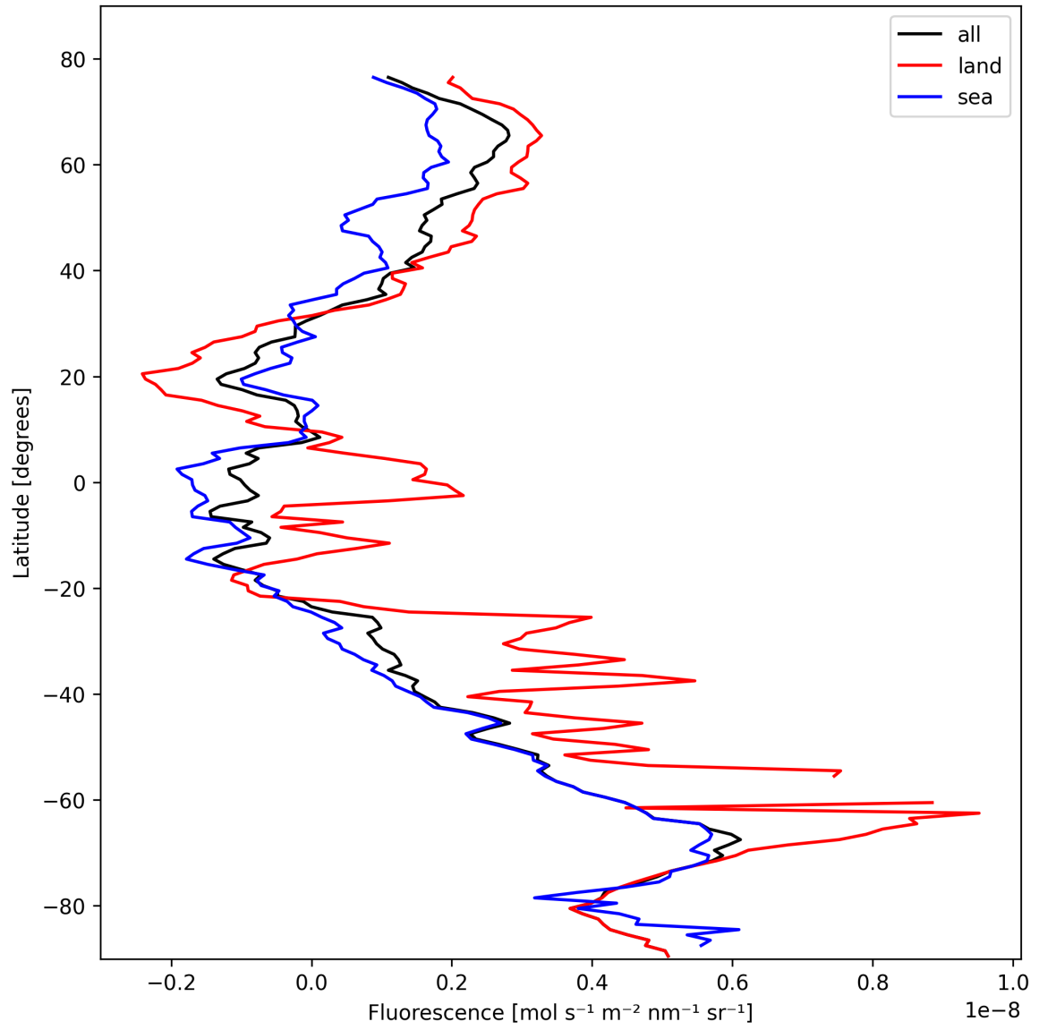
Figure 21: Zonal average of “Fluorescence” for 2025-10-24 to 2025-10-25.
