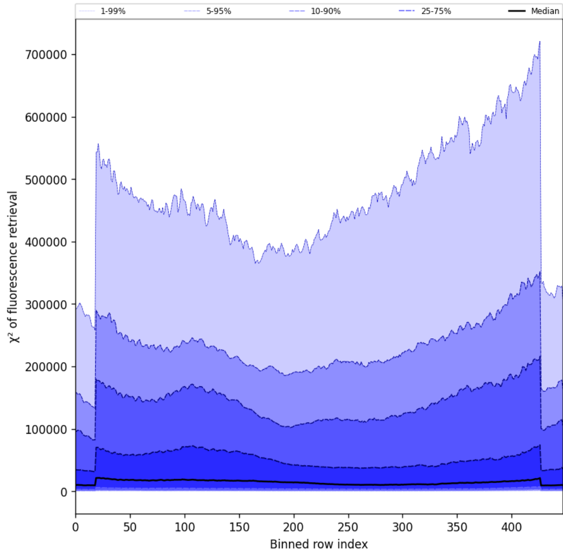
Figure 57: Along track statistics of “ \chi^2 of fluorescence retrieval” for 2025-10-24 to 2025-10-25
