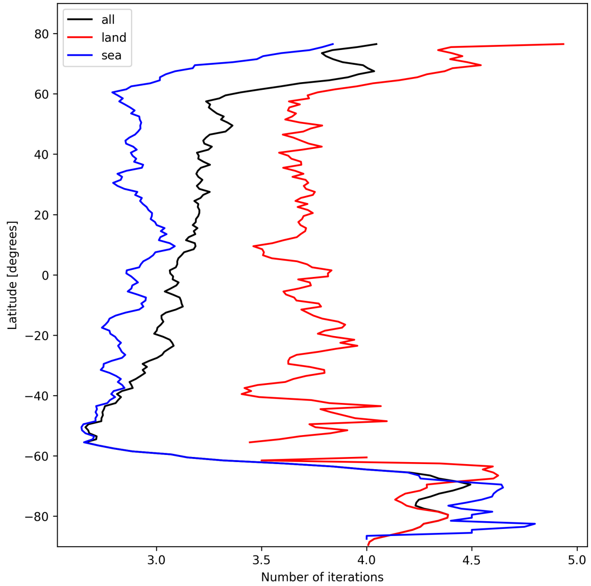
Figure 20: Zonal average of “Number of iterations” for 2025-10-24 to 2025-10-25.
