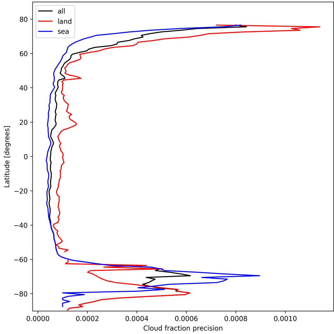
Figure 14: Zonal average of “Cloud fraction precision” for 2025-10-24 to 2025-10-25.
