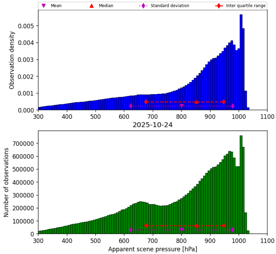
Figure 34: Histogram of “Apparent scene pressure” for 2025-10-24 to 2025-10-25
