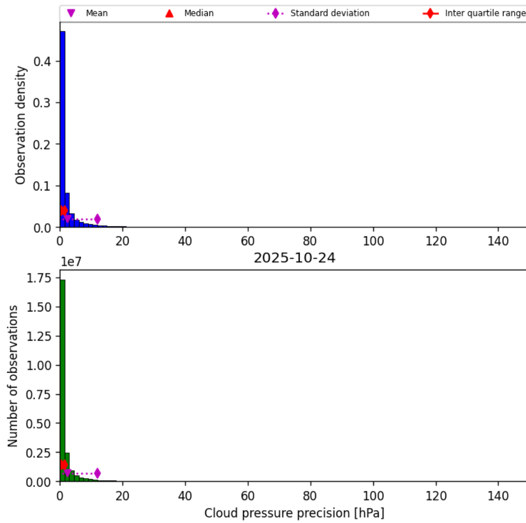
Figure 29: Histogram of “Cloud pressure precision” for 2025-10-24 to 2025-10-25
