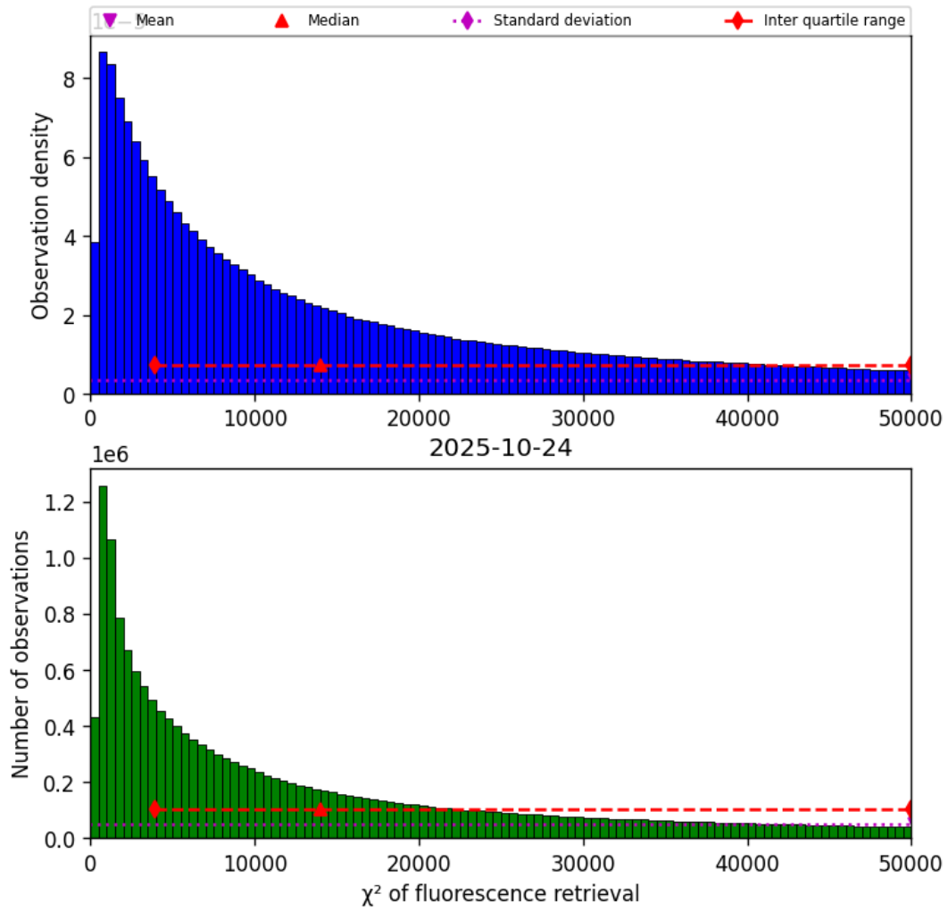
Figure 40: Histogram of “ \chi^2 of fluorescence retrieval” for 2025-10-24 to 2025-10-25
