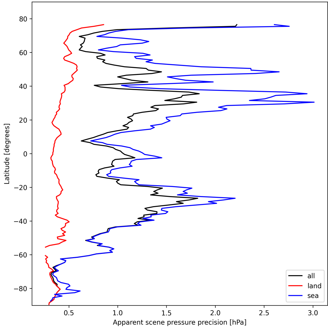
Figure 18: Zonal average of “Apparent scene pressure precision” for 2025-10-24 to 2025-10-25.
