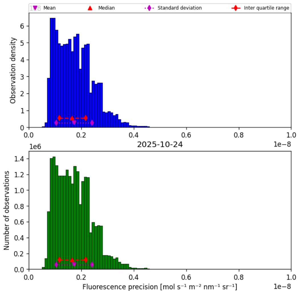
Figure 39: Histogram of “Fluorescence precision” for 2025-10-24 to 2025-10-25
