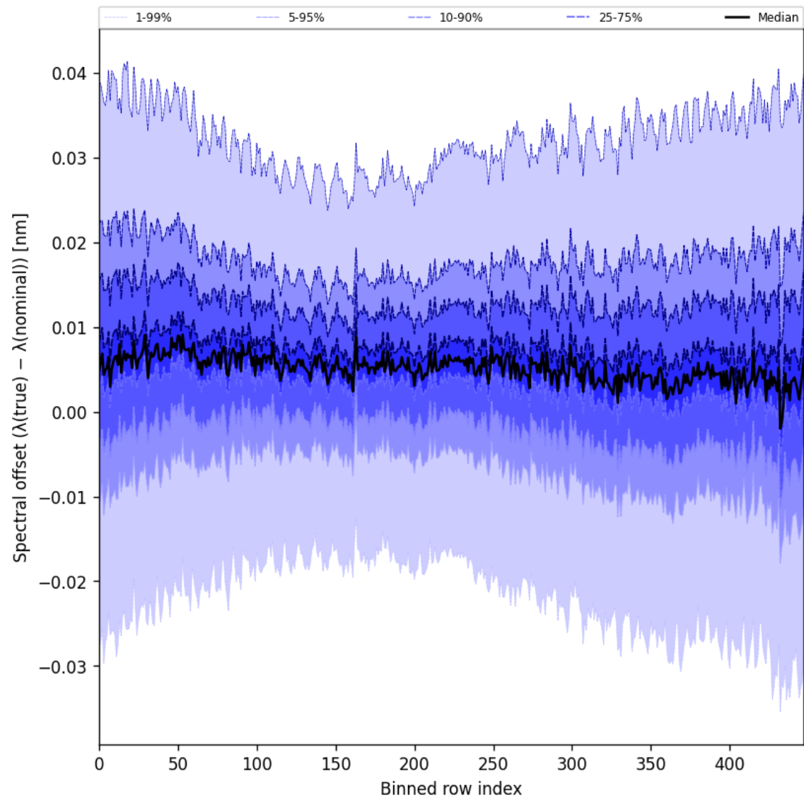
Figure 60: Along track statistics of “Spectral offset ( \lambda_{\text{true}} - \lambda_{\text{nominal}} )” for 2025-10-24 to 2025-10-25
