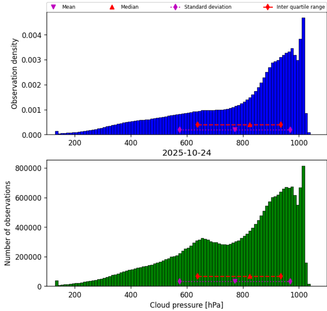
Figure 28: Histogram of “Cloud pressure” for 2025-10-24 to 2025-10-25
