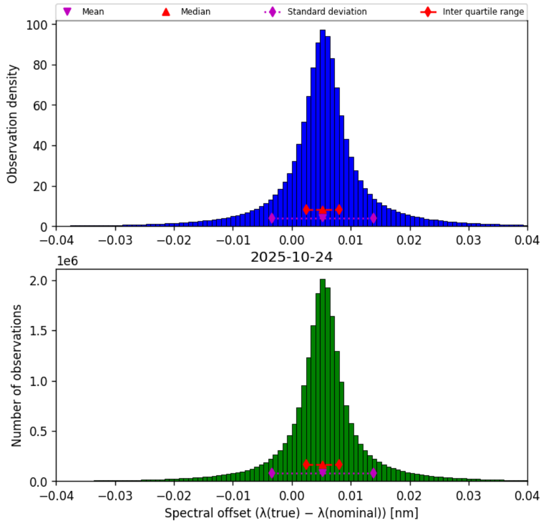
Figure 43: Histogram of “Spectral offset ( \lambda_{\text{true}} - \lambda_{\text{nominal}} )” for 2025-10-24 to 2025-10-25
