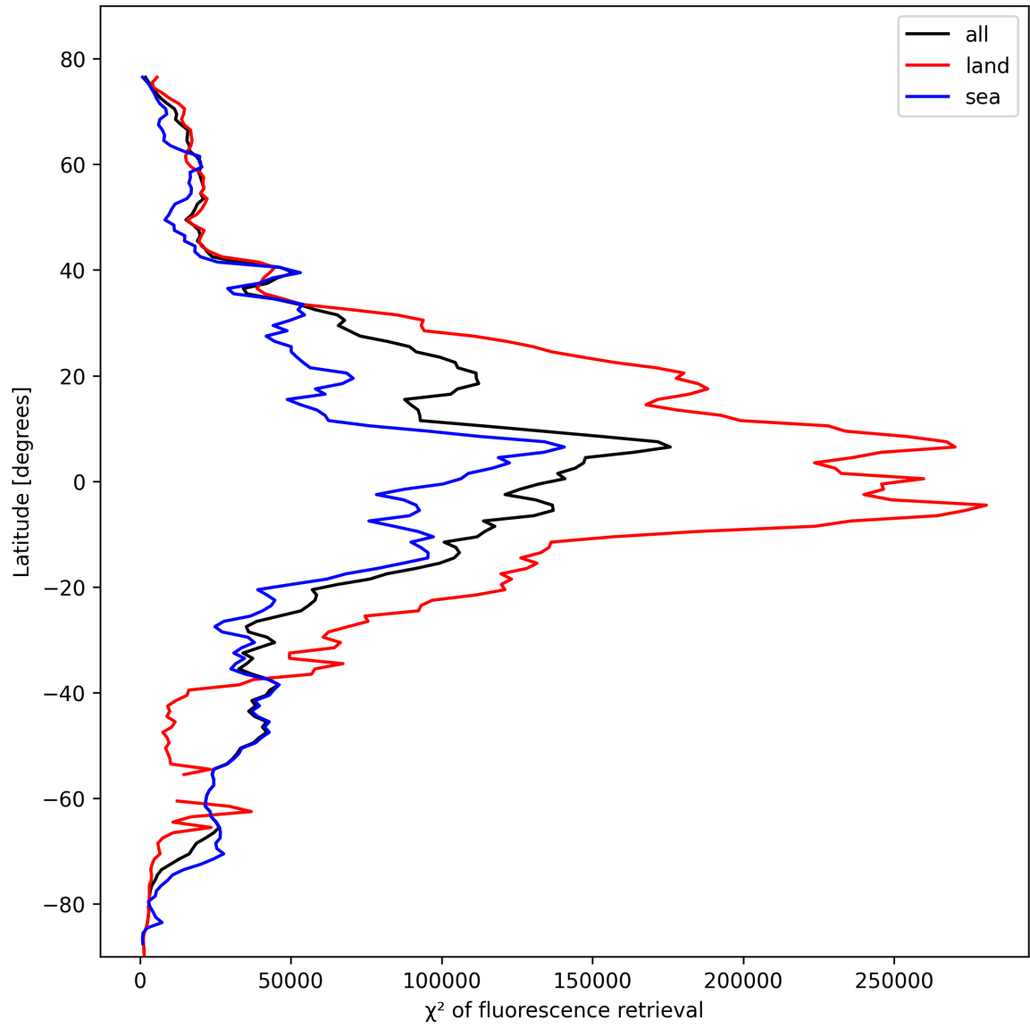
Figure 23: Zonal average of “ \chi^2 of fluorescence retrieval” for 2025-10-24 to 2025-10-25.
