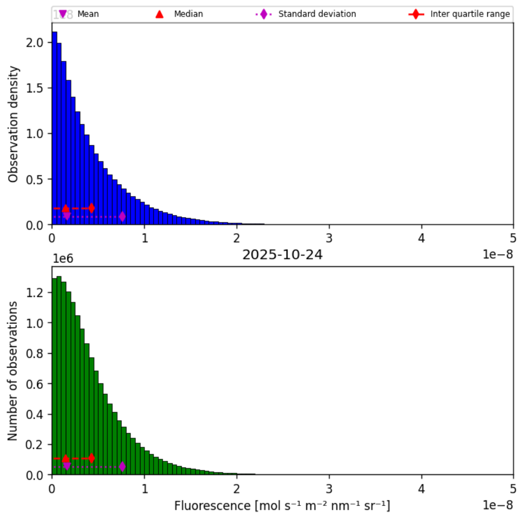
Figure 38: Histogram of “Fluorescence” for 2025-10-24 to 2025-10-25
