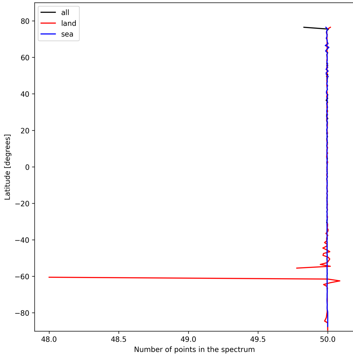
Figure 25: Zonal average of “Number of points in the spectrum” for 2025-10-24 to 2025-10-25.
