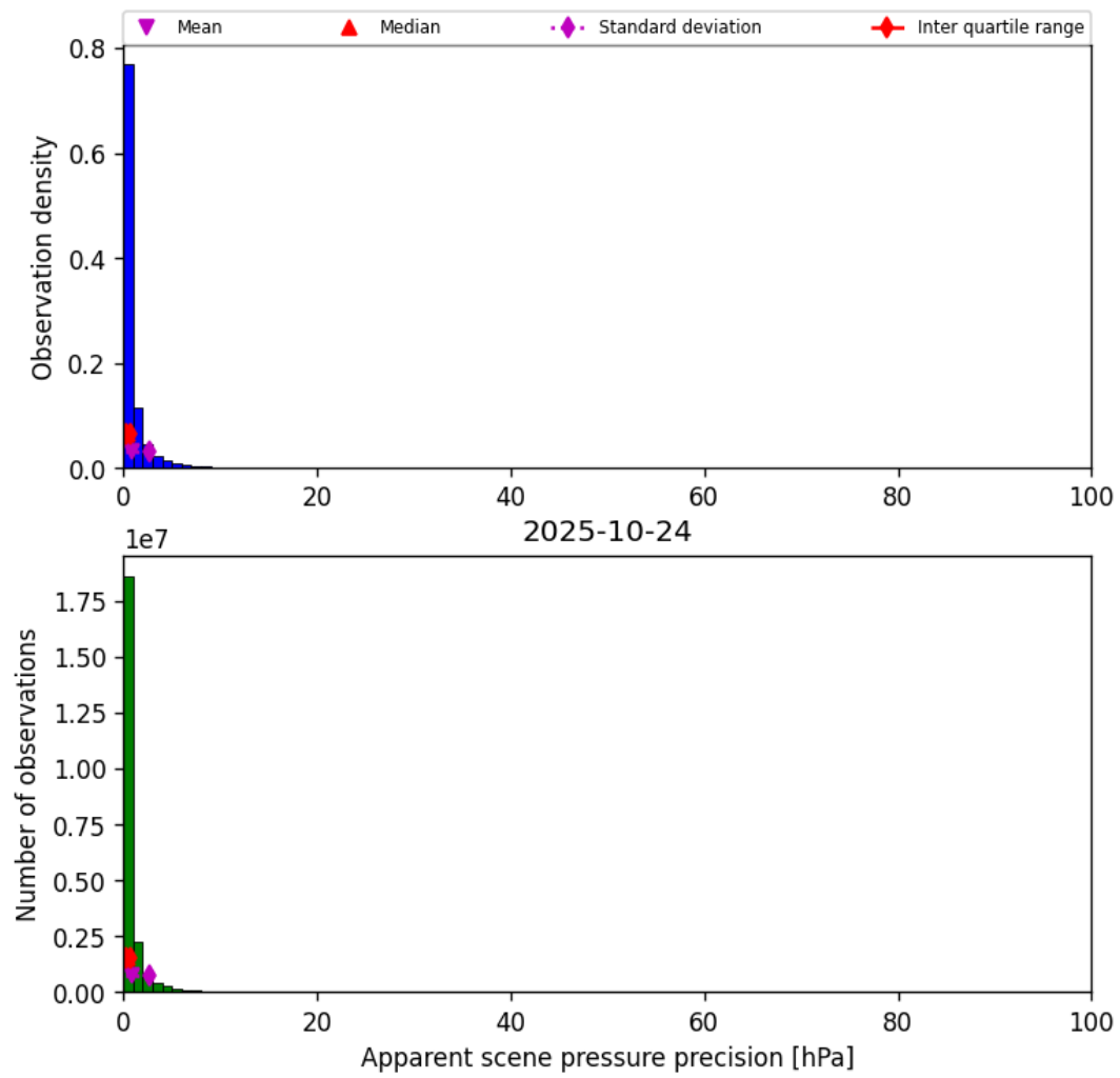
Figure 35: Histogram of “Apparent scene pressure precision” for 2025-10-24 to 2025-10-25
