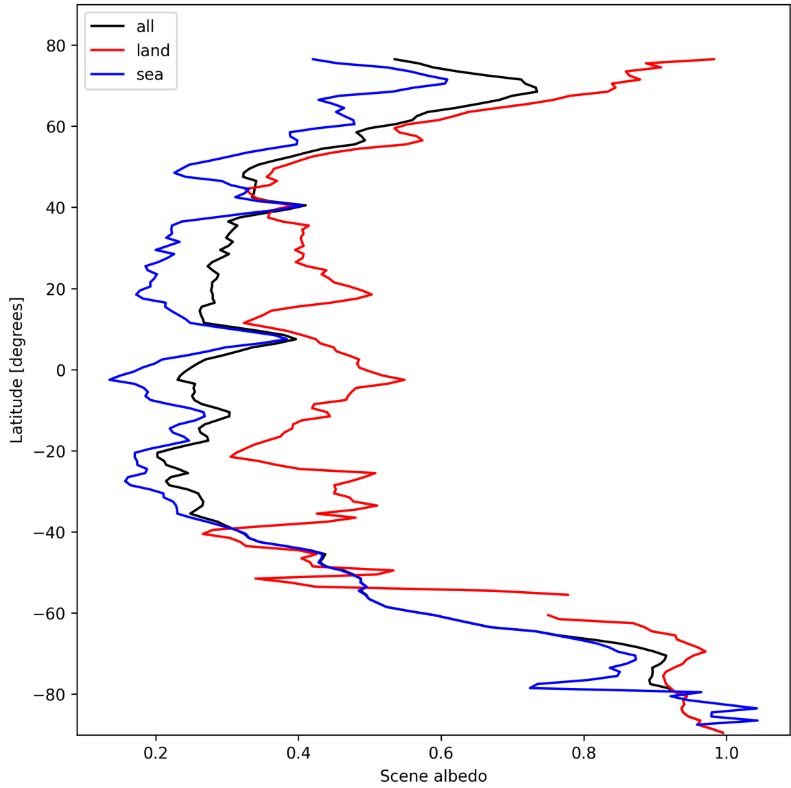
Figure 15: Zonal average of “Scene albedo” for 2025-10-24 to 2025-10-25.
