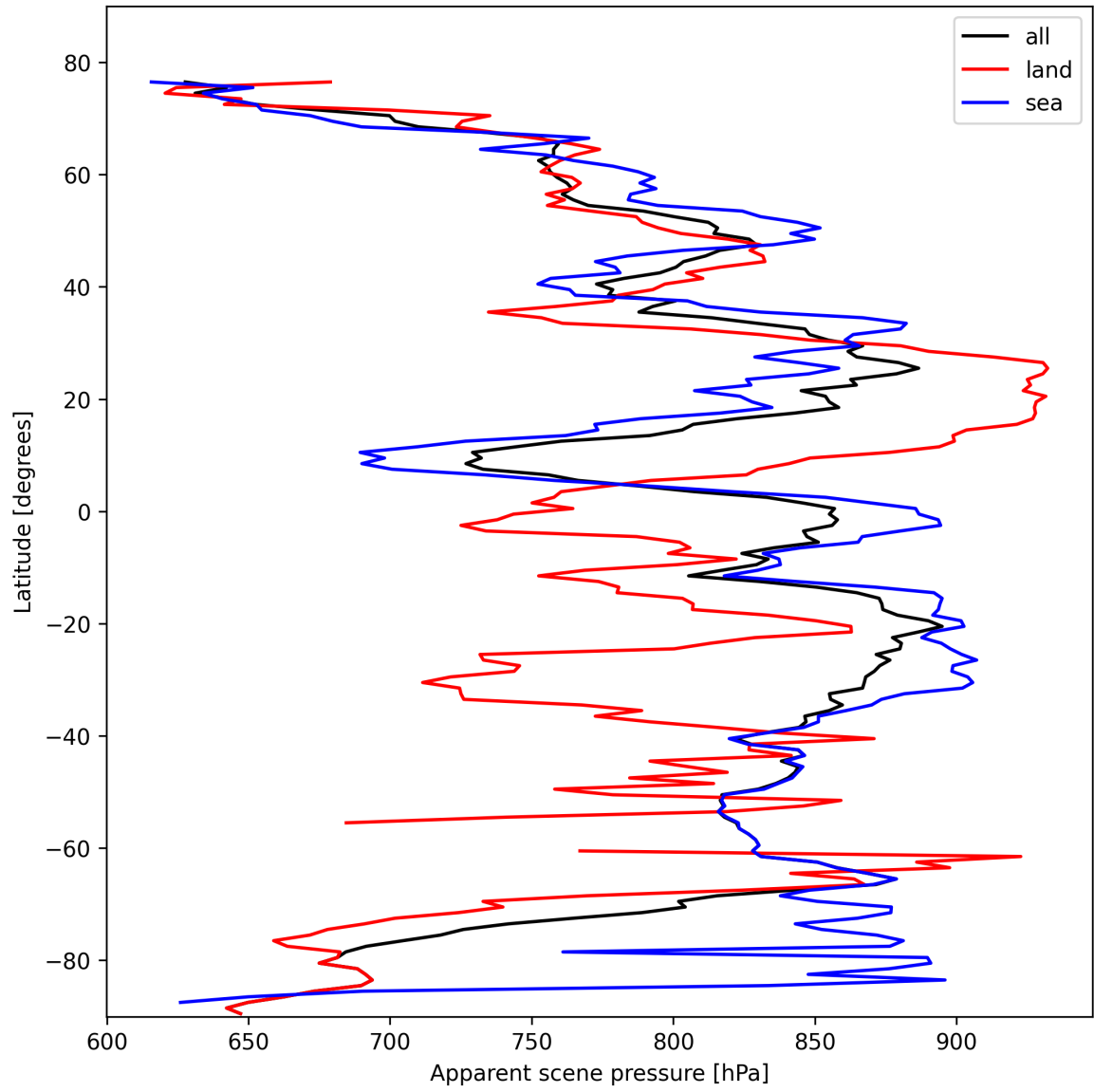
Figure 17: Zonal average of “Apparent scene pressure” for 2025-10-24 to 2025-10-25.
