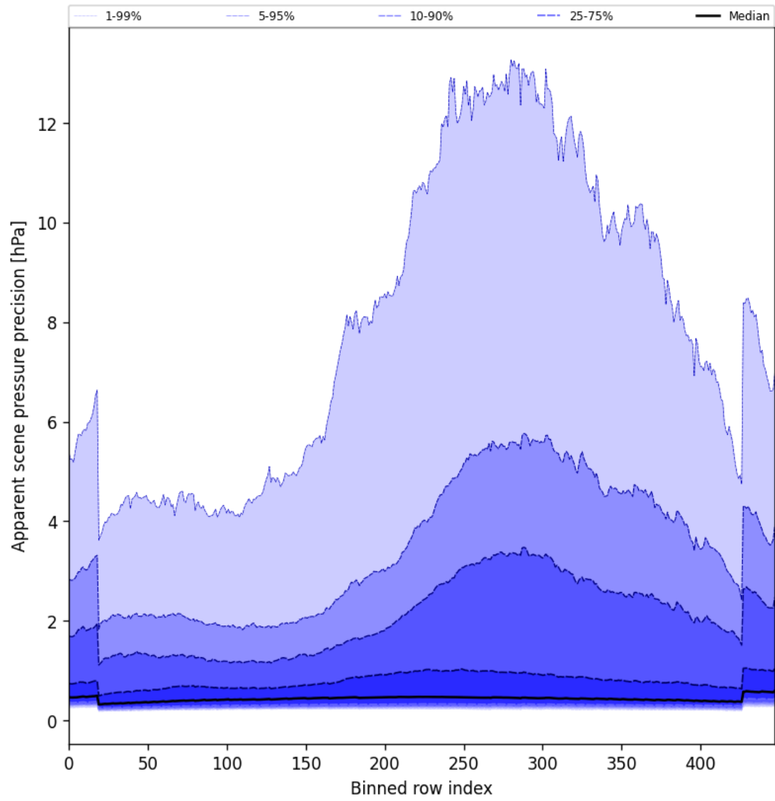
Figure 52: Along track statistics of “Apparent scene pressure precision” for 2025-10-24 to 2025-10-25
