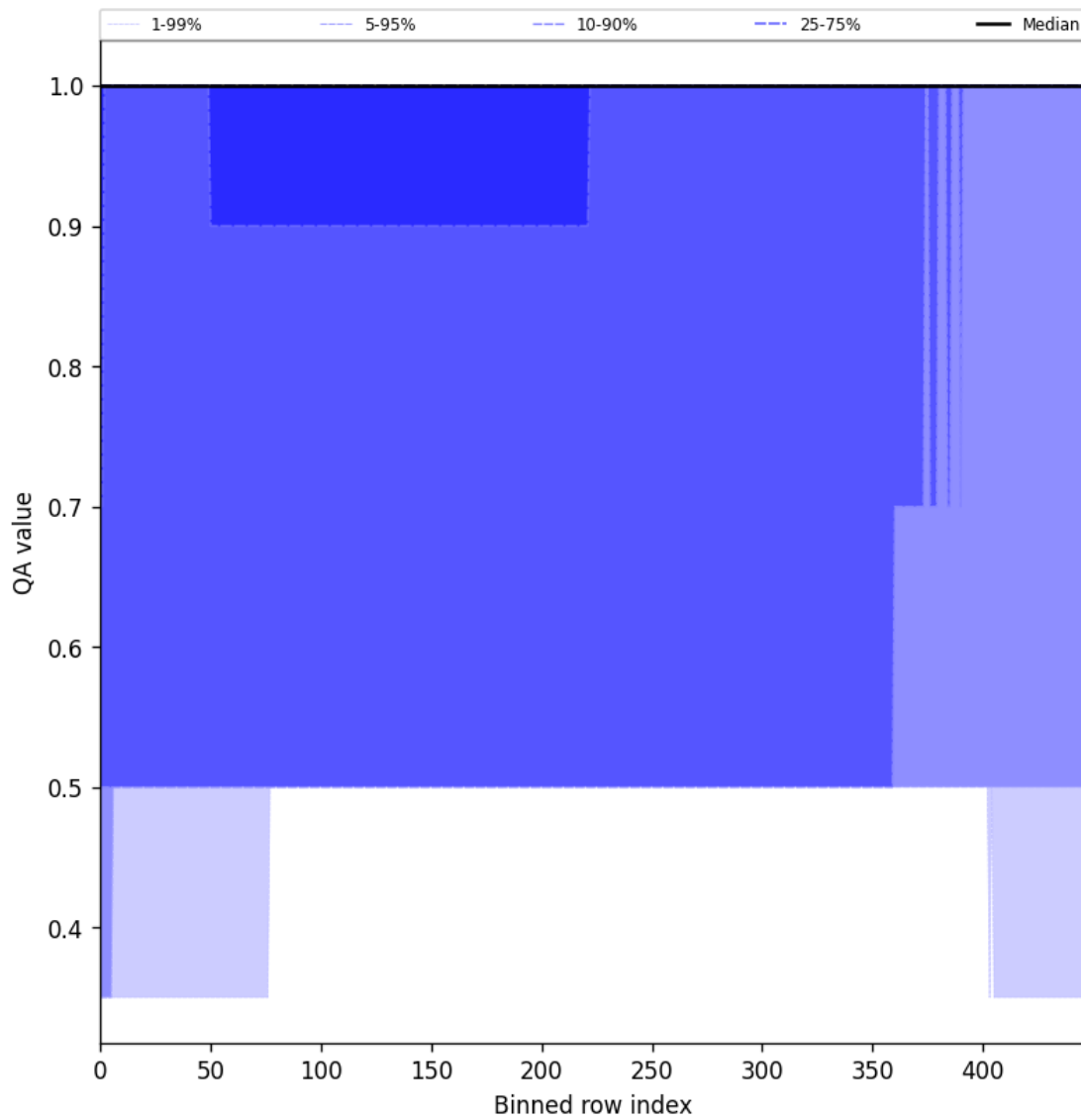
Figure 44: Along track statistics of “QA value” for 2025-10-24 to 2025-10-25
