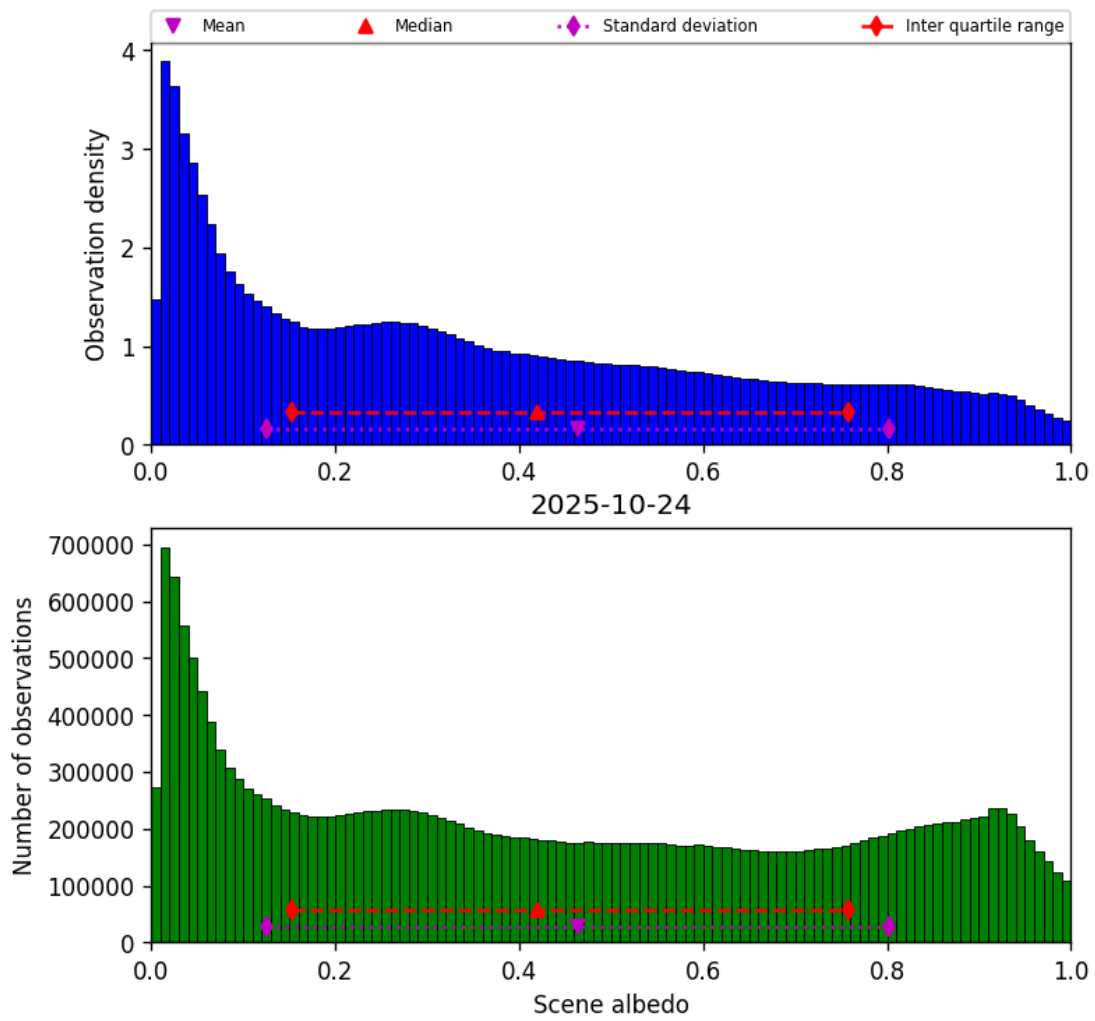
Figure 32: Histogram of “Scene albedo” for 2025-10-24 to 2025-10-25
