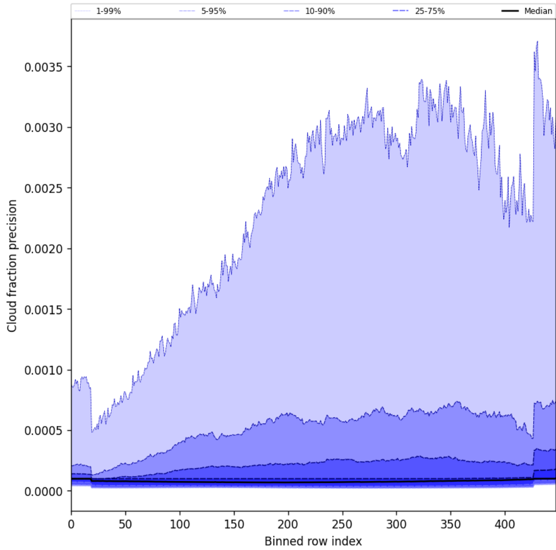
Figure 48: Along track statistics of “Cloud fraction precision” for 2025-10-25 to 2025-10-25
