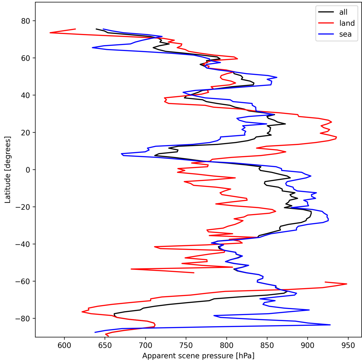
Figure 17: Zonal average of “Apparent scene pressure” for 2025-10-25 to 2025-10-25.
