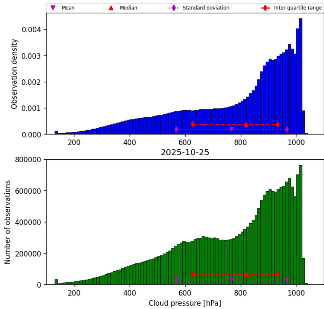
Figure 28: Histogram of “Cloud pressure” for 2025-10-25 to 2025-10-25
