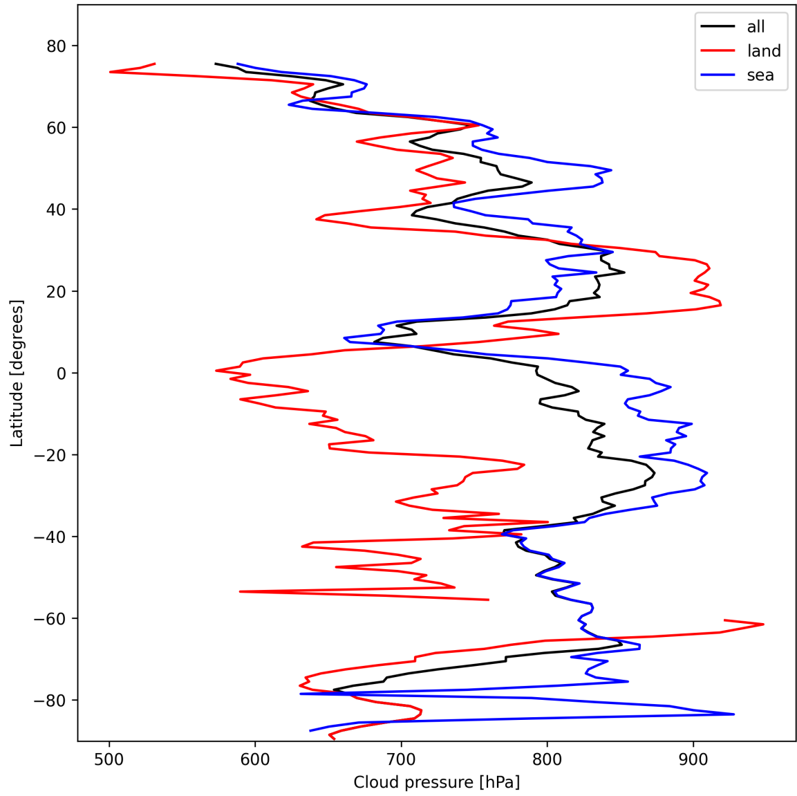
Figure 11: Zonal average of “Cloud pressure” for 2025-10-25 to 2025-10-25.
