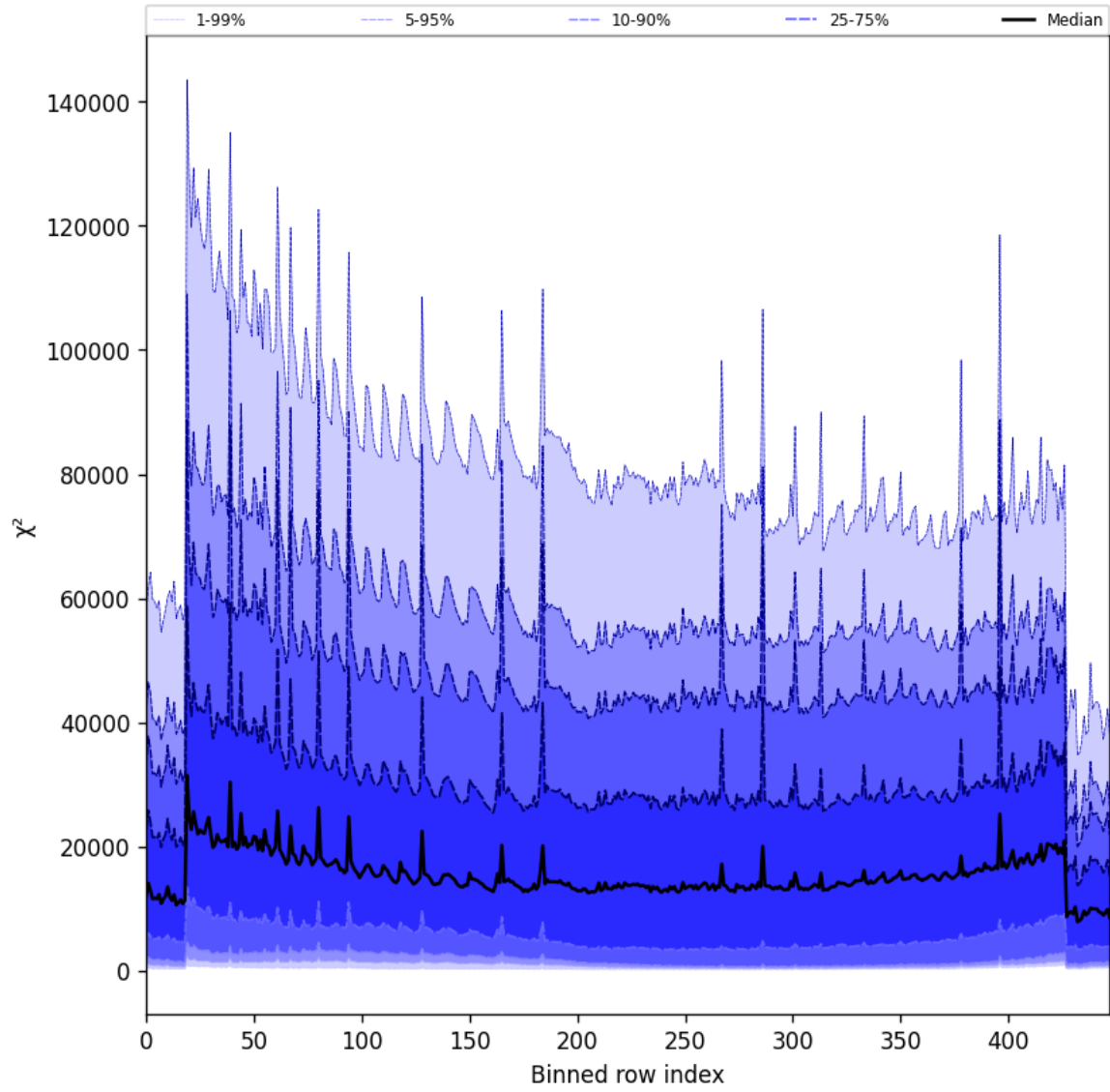
Figure 53: Along track statistics of “ \chi^2 ” for 2025-10-25 to 2025-10-25
