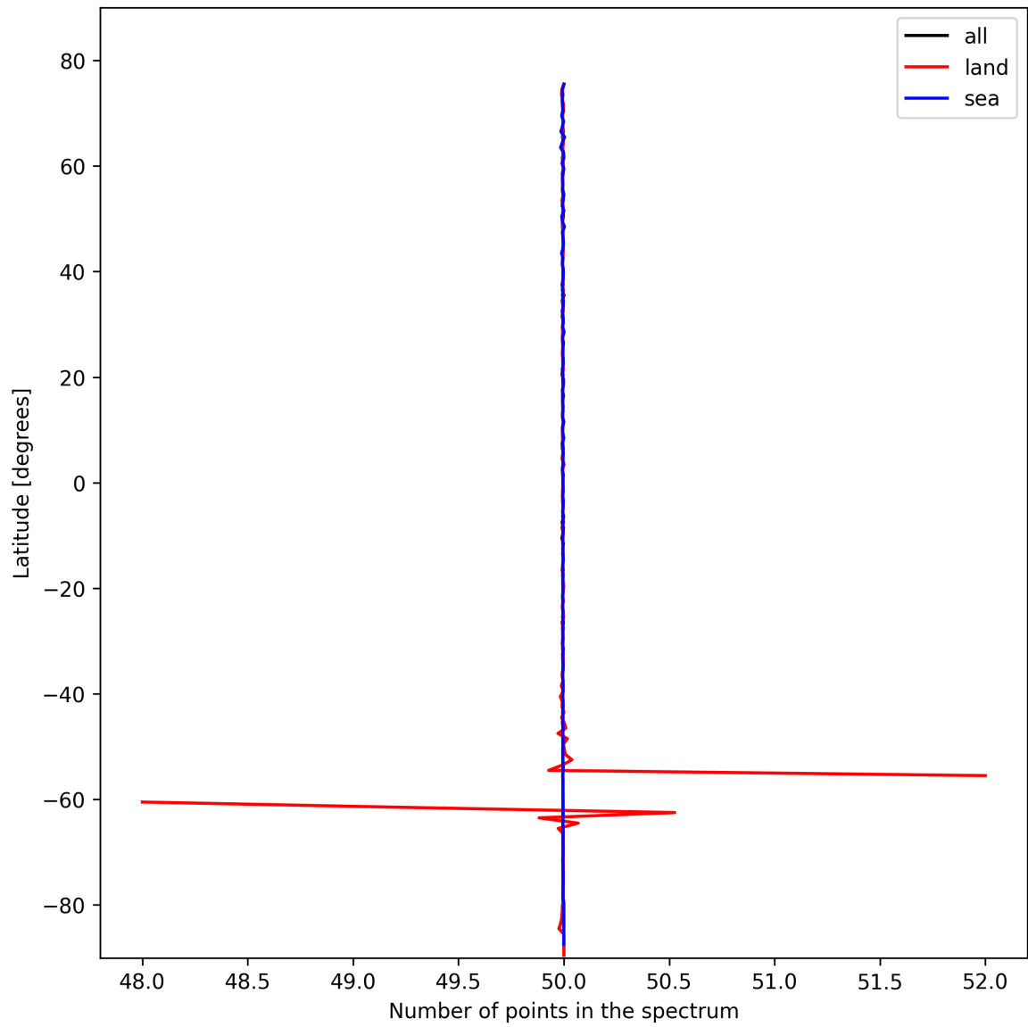
Figure 25: Zonal average of “Number of points in the spectrum” for 2025-10-25 to 2025-10-25.
