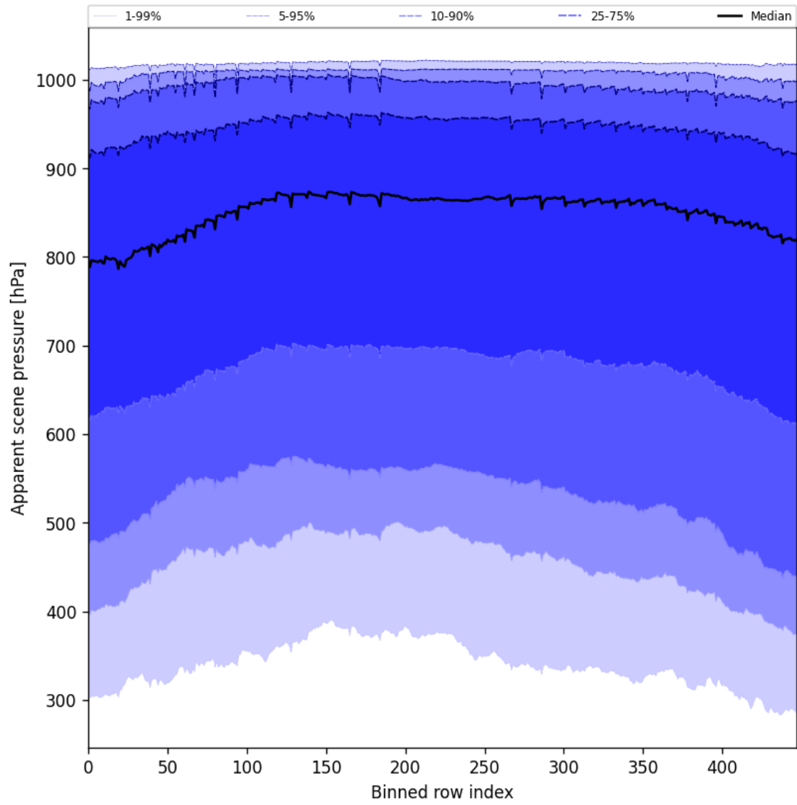
Figure 51: Along track statistics of “Apparent scene pressure” for 2025-10-25 to 2025-10-25
