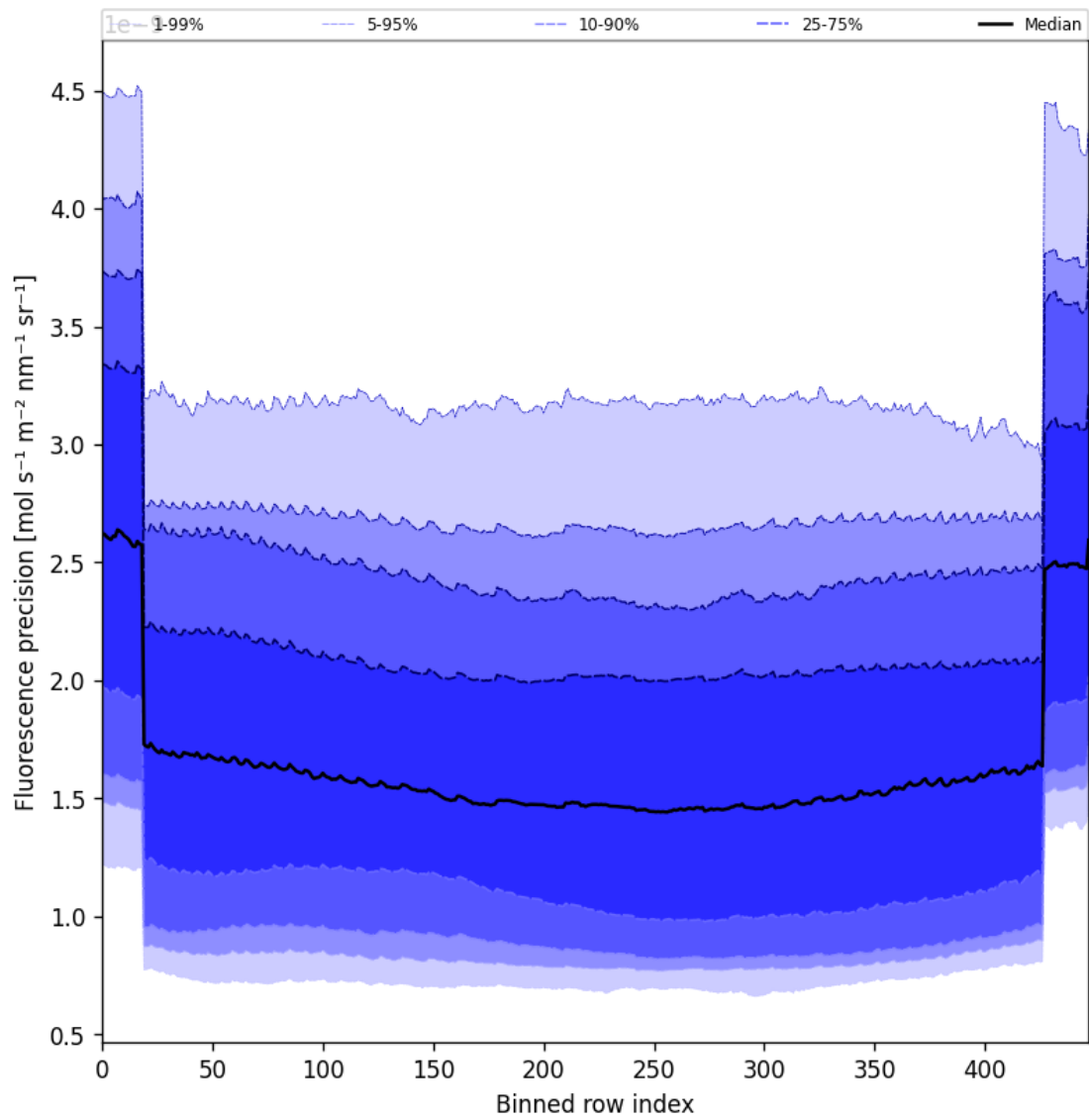
Figure 56: Along track statistics of “Fluorescence precision” for 2025-10-25 to 2025-10-25
