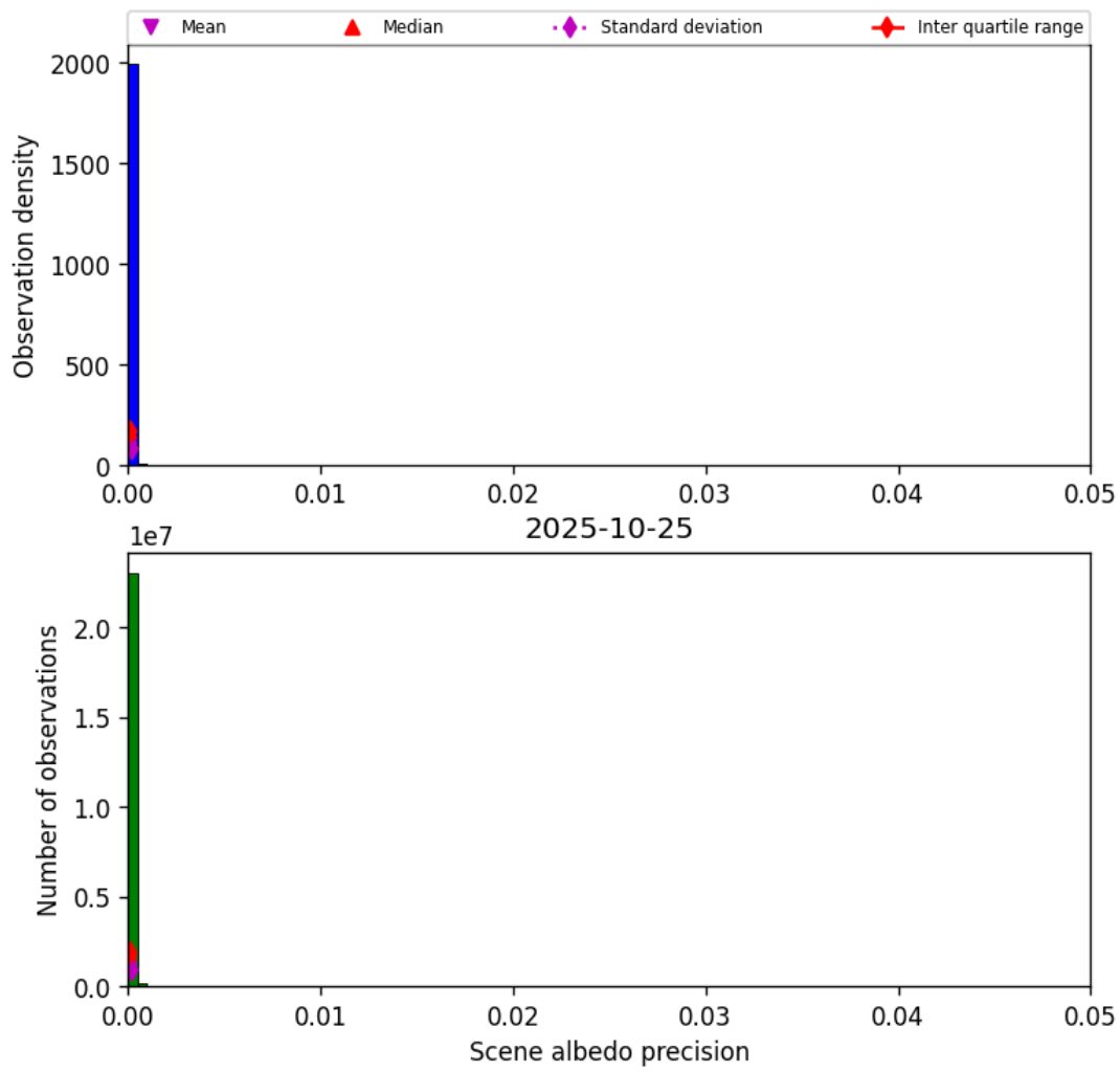
Figure 33: Histogram of “Scene albedo precision” for 2025-10-25 to 2025-10-25
