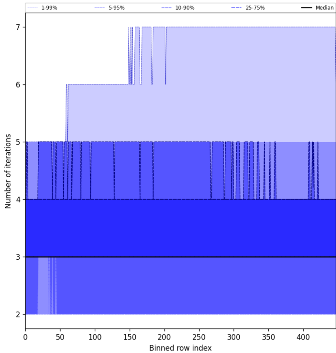
Figure 54: Along track statistics of “Number of iterations” for 2025-10-25 to 2025-10-25
