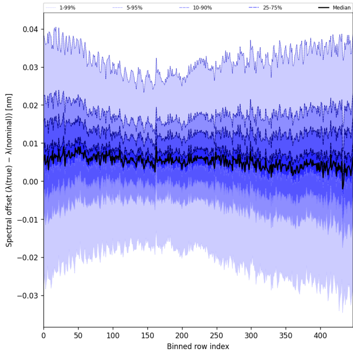
Figure 60: Along track statistics of “Spectral offset ( \lambda_{\text{true}} - \lambda_{\text{nominal}} )” for 2025-10-25 to 2025-10-25
