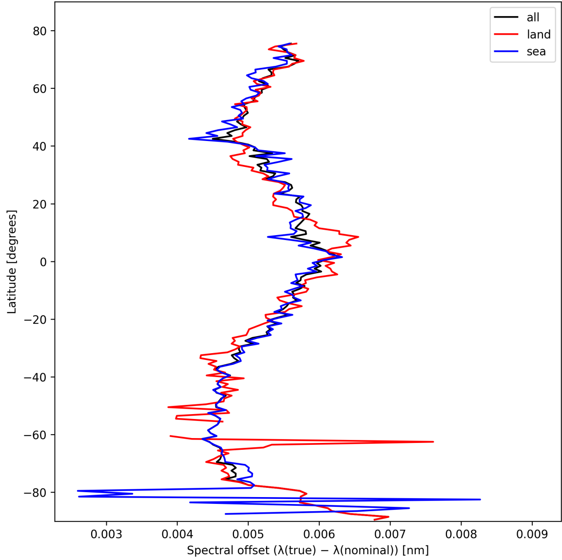
Figure 26: Zonal average of “Spectral offset ( \lambda_{\text{true}} - \lambda_{\text{nominal}} )” for 2025-10-25 to 2025-10-25.
