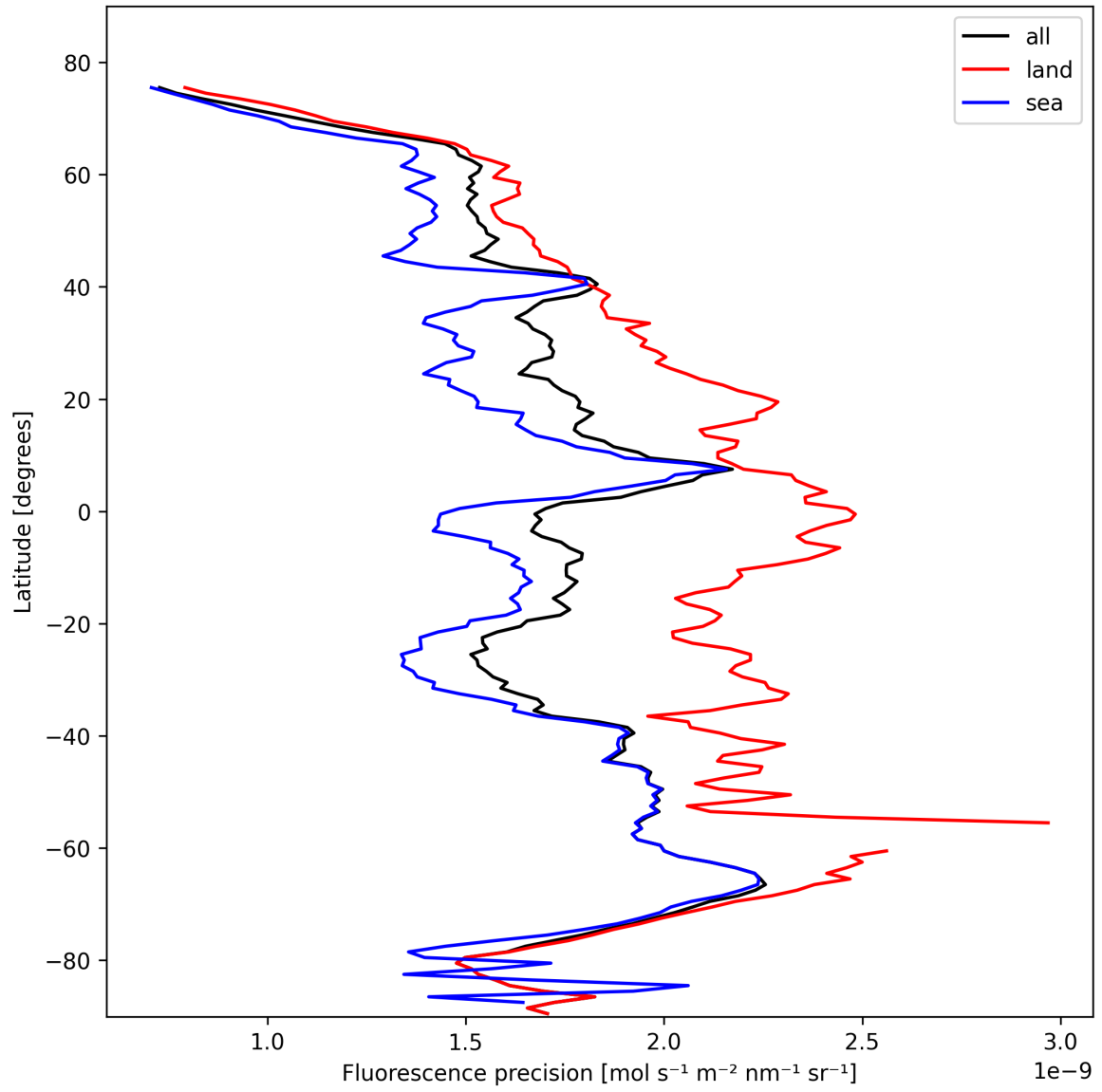
Figure 22: Zonal average of “Fluorescence precision” for 2025-10-25 to 2025-10-25.
