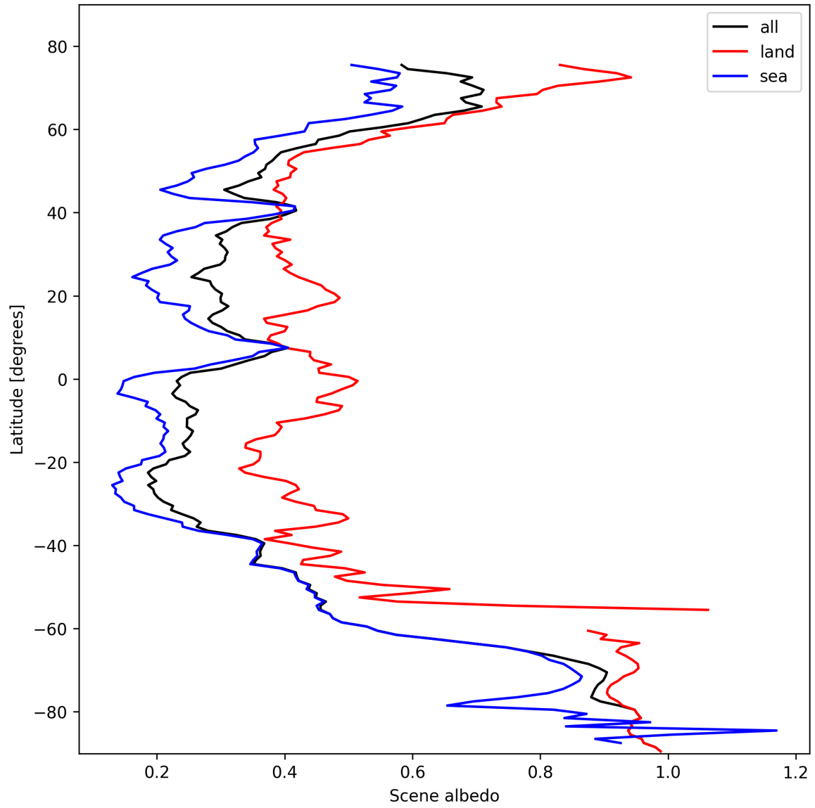
Figure 15: Zonal average of “Scene albedo” for 2025-10-25 to 2025-10-25.
