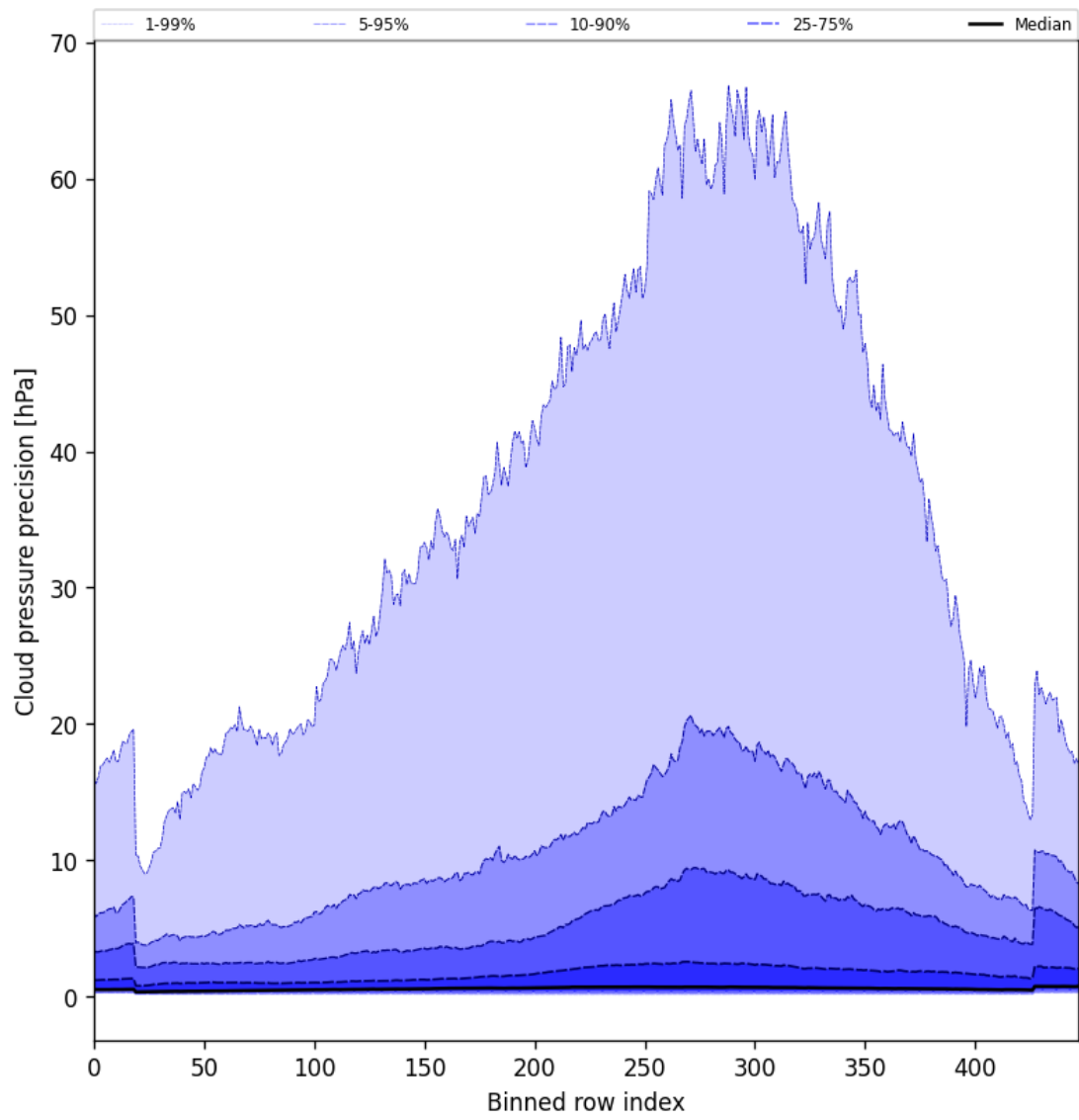
Figure 46: Along track statistics of “Cloud pressure precision” for 2025-10-25 to 2025-10-25
