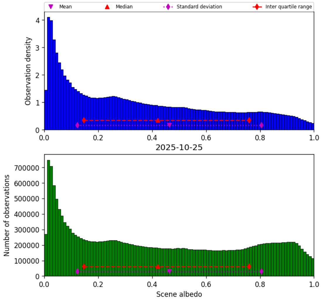
Figure 32: Histogram of “Scene albedo” for 2025-10-25 to 2025-10-25
