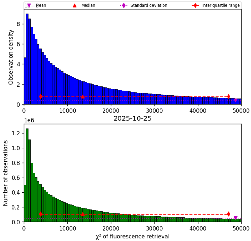
Figure 40: Histogram of “ \chi^2 of fluorescence retrieval” for 2025-10-25 to 2025-10-25
