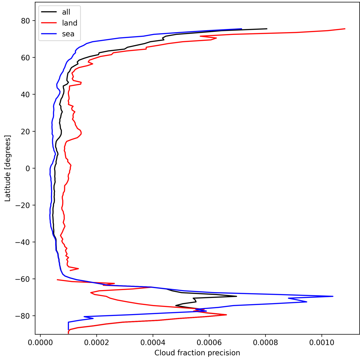
Figure 14: Zonal average of “Cloud fraction precision” for 2025-10-25 to 2025-10-25.
