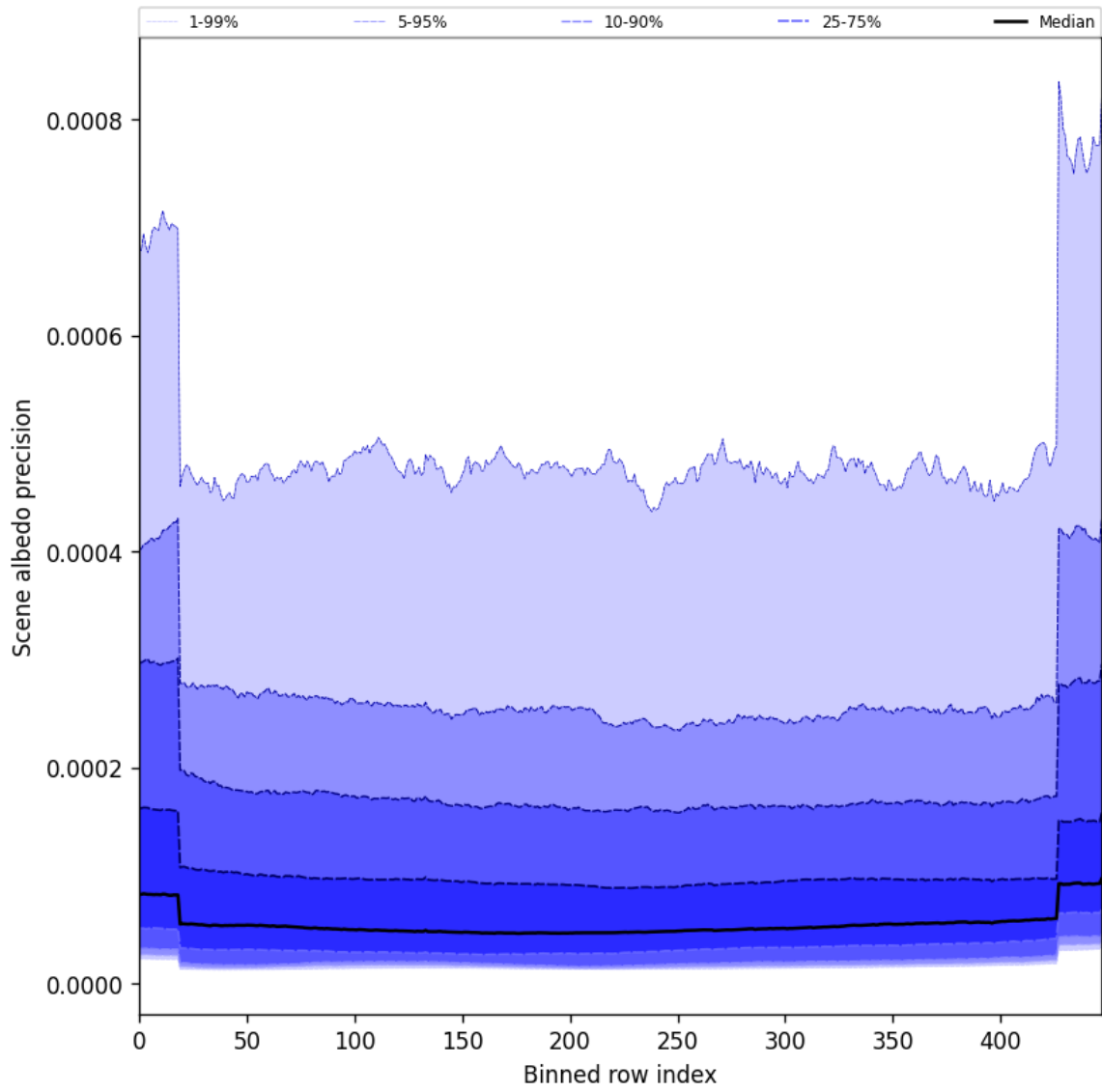
Figure 50: Along track statistics of “Scene albedo precision” for 2025-10-25 to 2025-10-25
