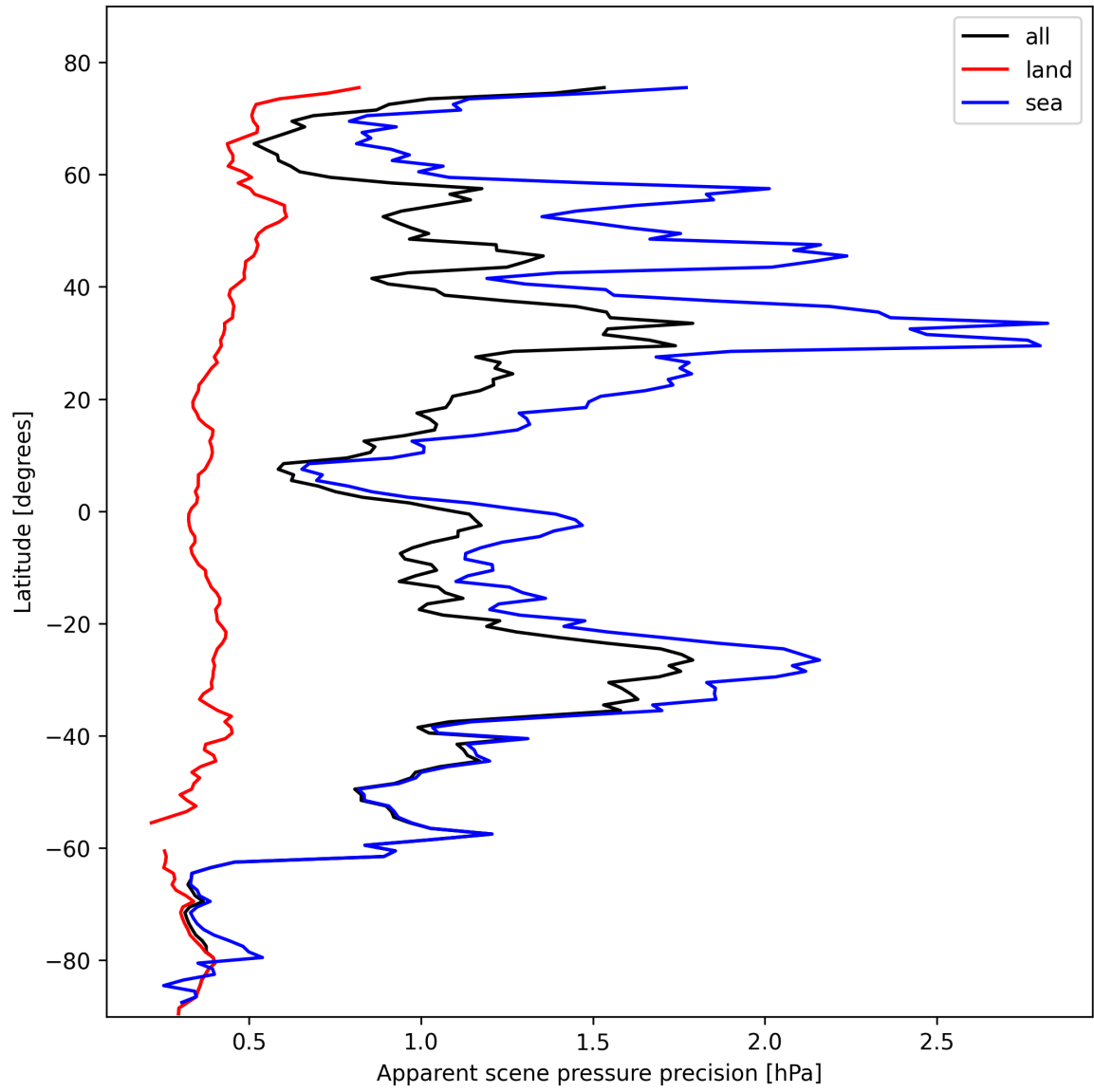
Figure 18: Zonal average of “Apparent scene pressure precision” for 2025-10-25 to 2025-10-25.
