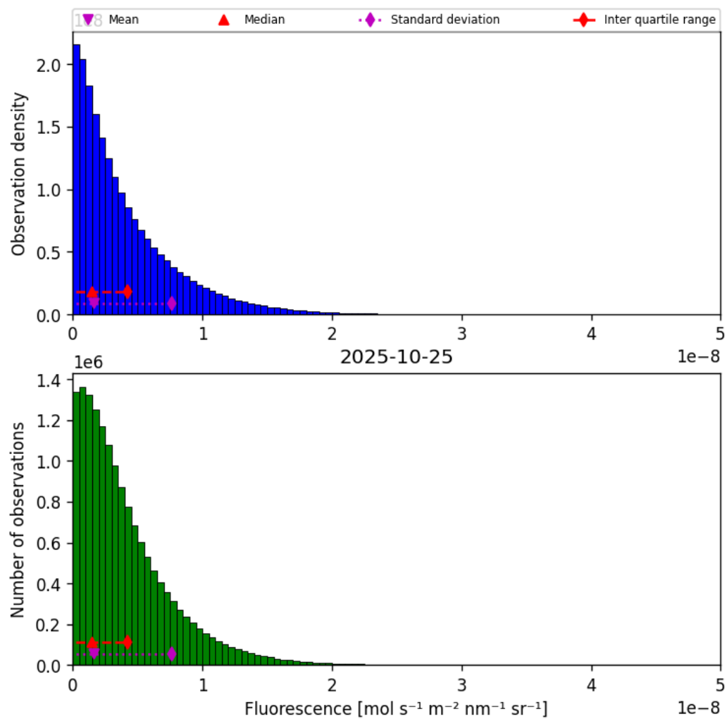
Figure 38: Histogram of “Fluorescence” for 2025-10-25 to 2025-10-25
