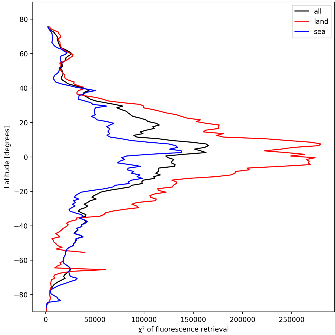
Figure 23: Zonal average of “ \chi^2 of fluorescence retrieval” for 2025-10-25 to 2025-10-25.
