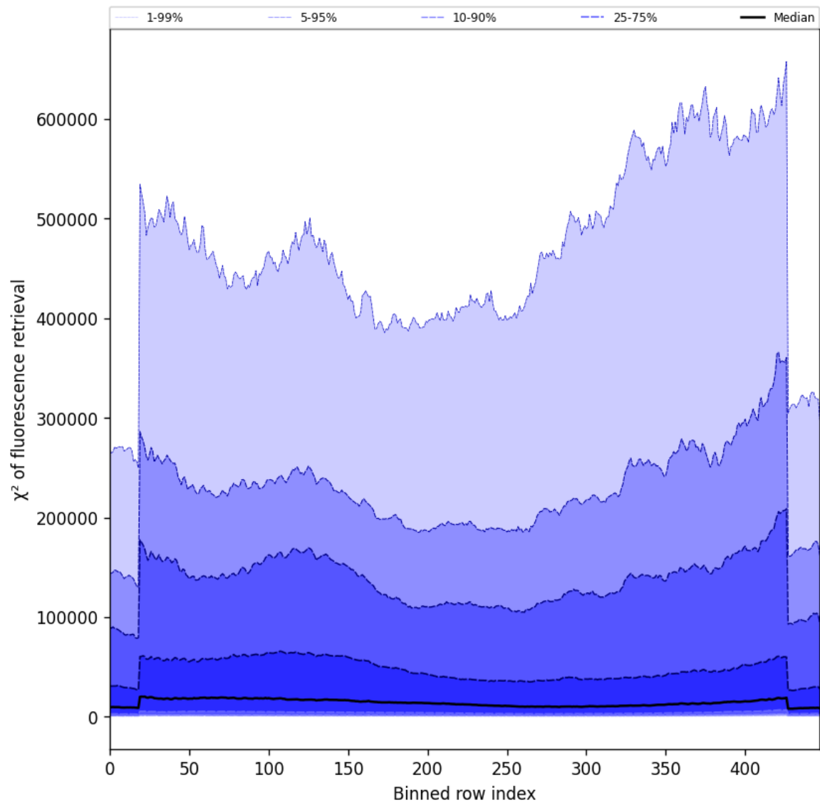
Figure 57: Along track statistics of “ \chi^2 of fluorescence retrieval” for 2025-10-25 to 2025-10-25
