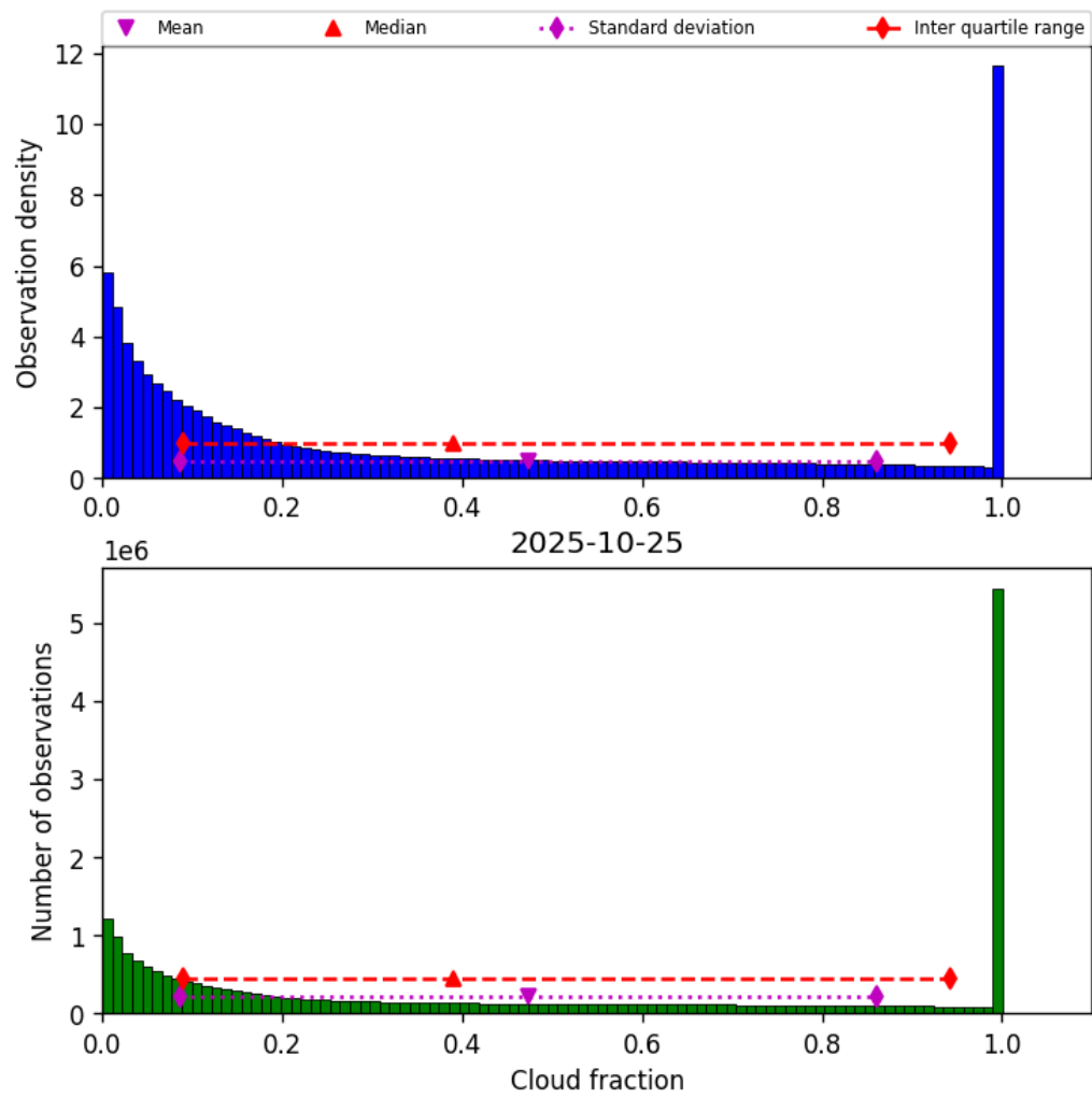
Figure 30: Histogram of “Cloud fraction” for 2025-10-25 to 2025-10-25
