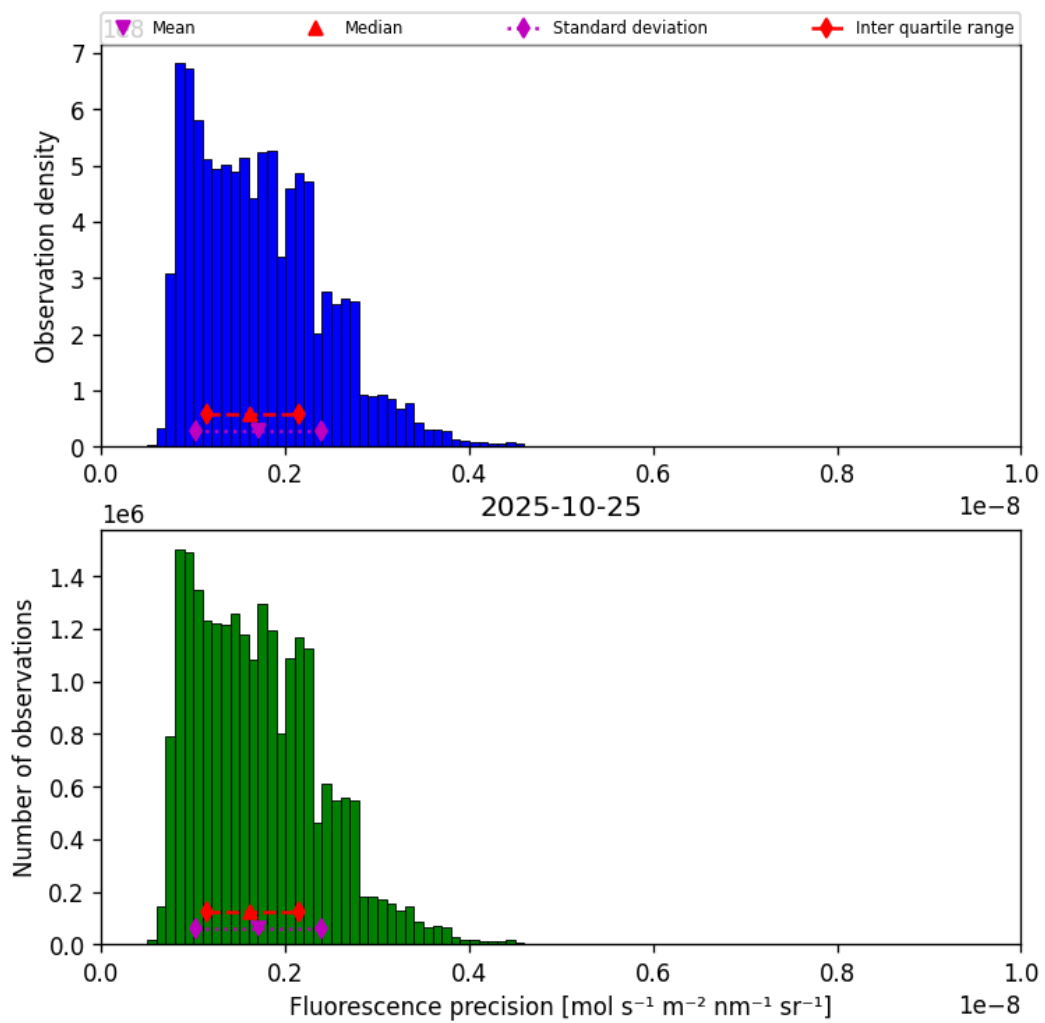
Figure 39: Histogram of “Fluorescence precision” for 2025-10-25 to 2025-10-25
