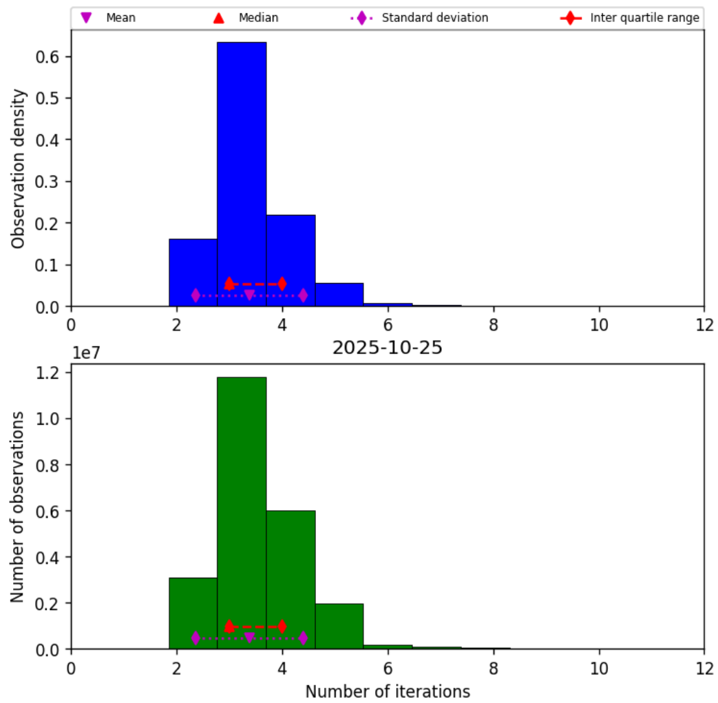
Figure 37: Histogram of “Number of iterations” for 2025-10-25 to 2025-10-25
