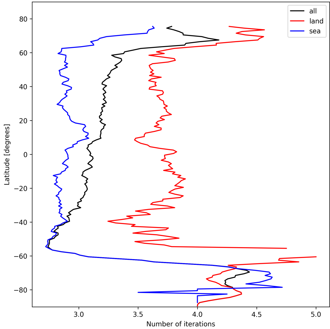
Figure 20: Zonal average of “Number of iterations” for 2025-10-25 to 2025-10-25.
