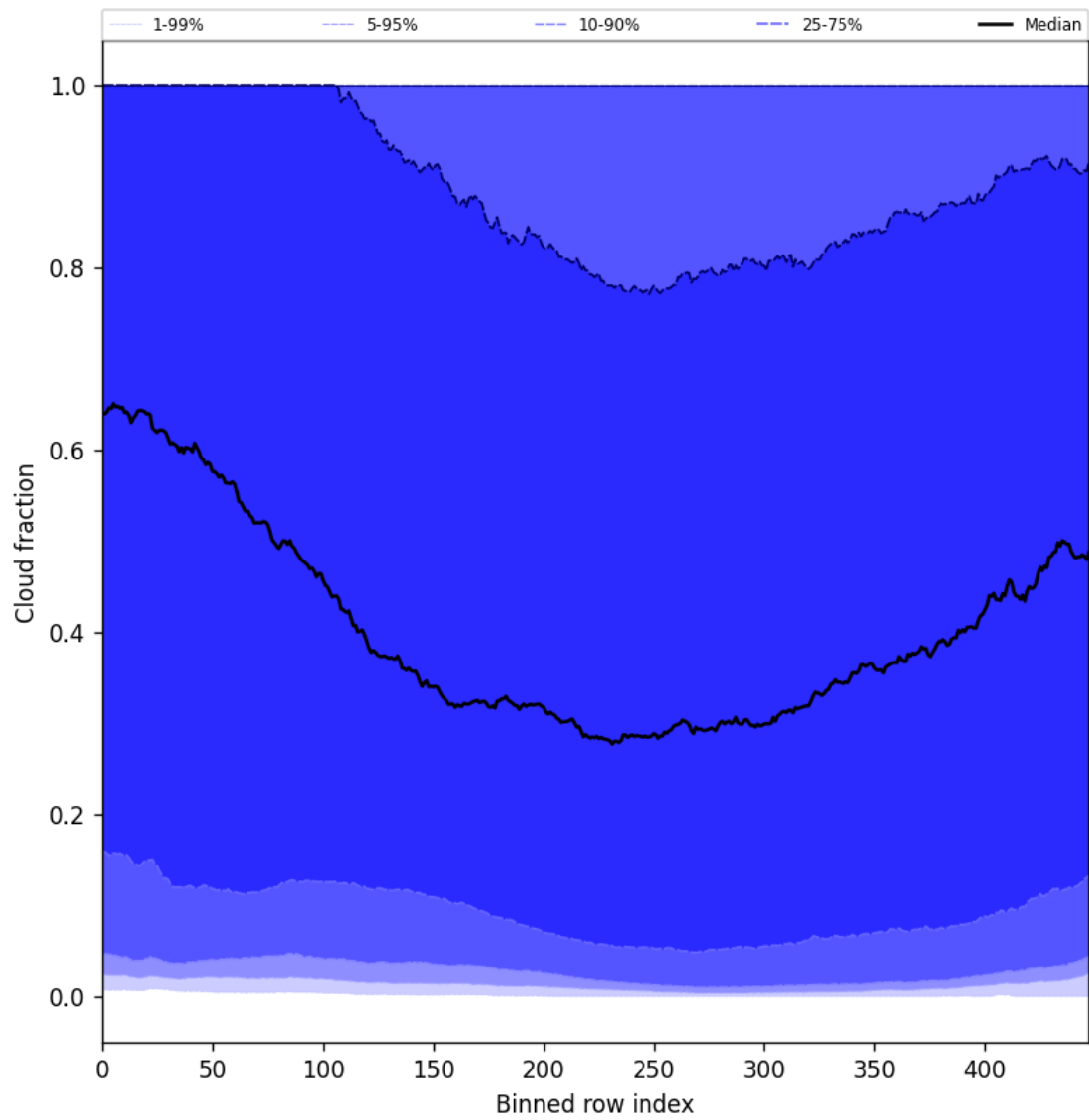
Figure 47: Along track statistics of “Cloud fraction” for 2025-10-25 to 2025-10-25
