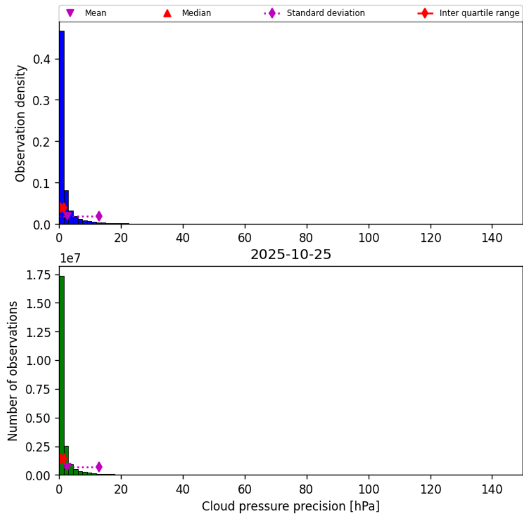
Figure 29: Histogram of “Cloud pressure precision” for 2025-10-25 to 2025-10-25
