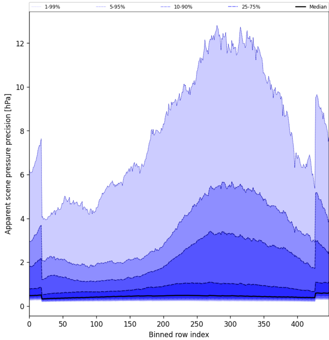
Figure 52: Along track statistics of “Apparent scene pressure precision” for 2025-10-25 to 2025-10-25
