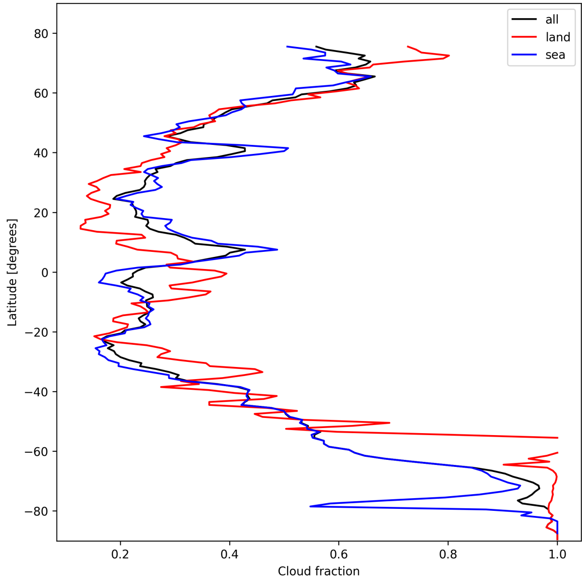
Figure 13: Zonal average of “Cloud fraction” for 2025-10-25 to 2025-10-25.
