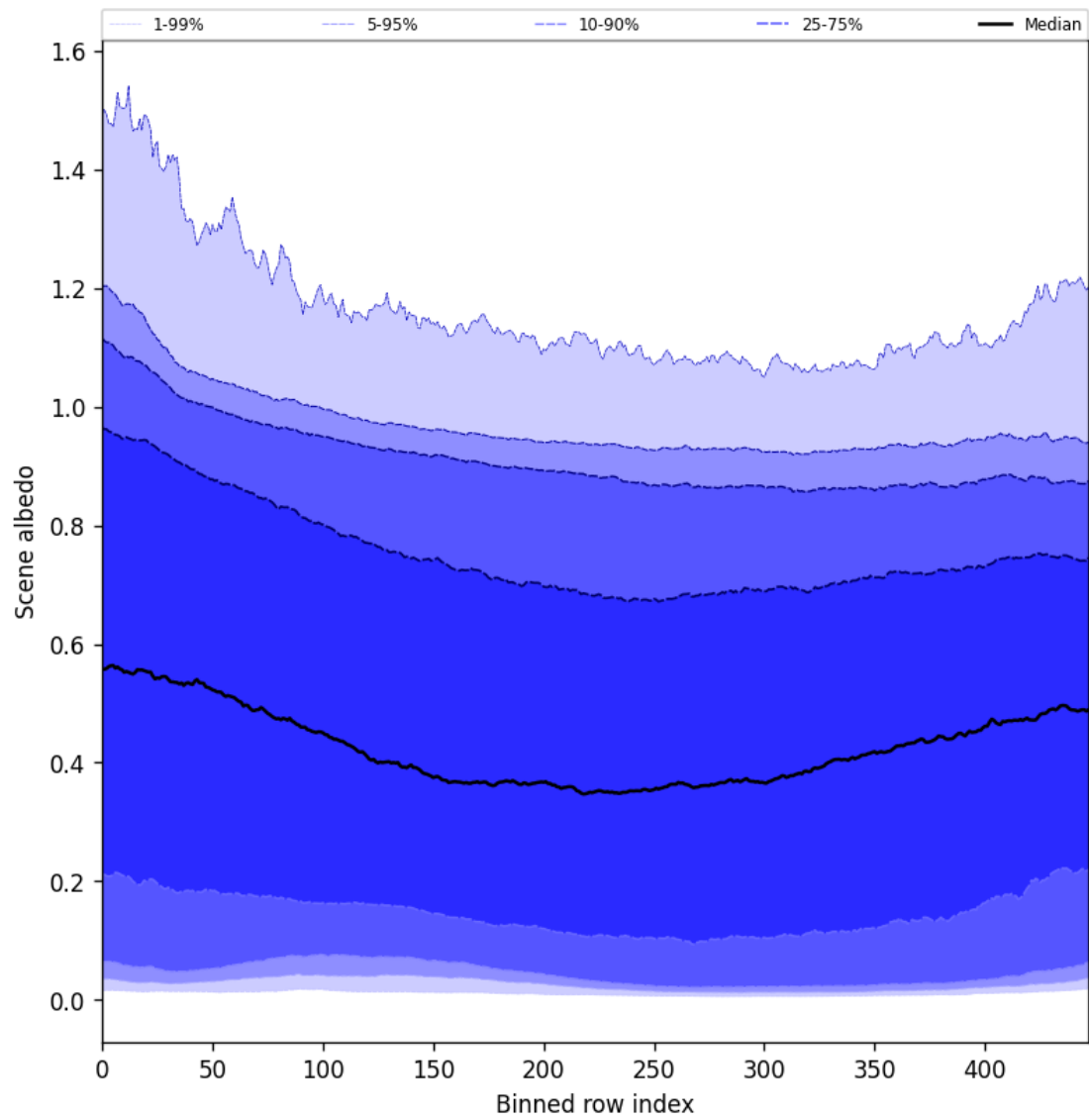
Figure 49: Along track statistics of “Scene albedo” for 2025-10-25 to 2025-10-25
