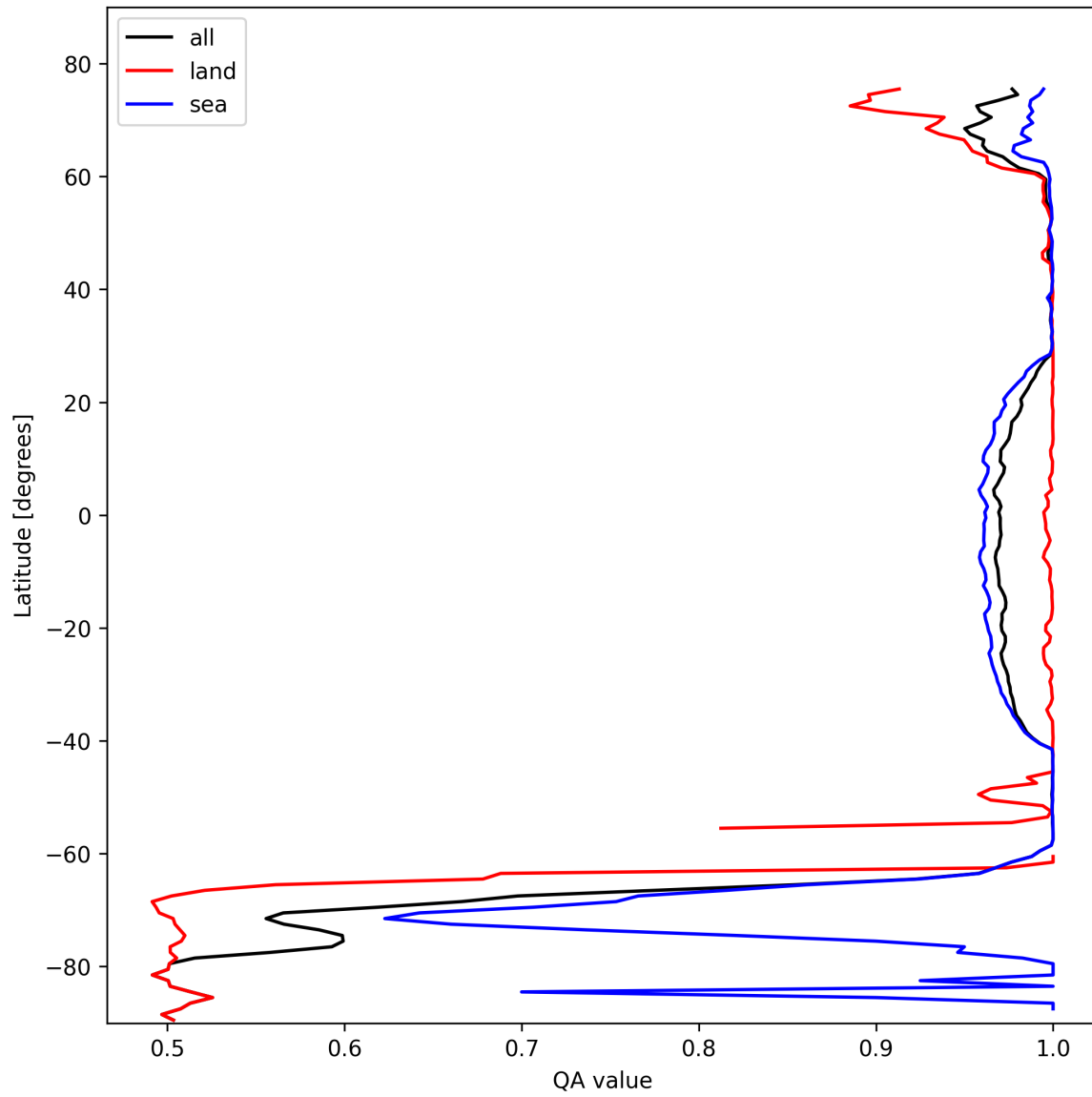
Figure 10: Zonal average of “QA value” for 2025-10-25 to 2025-10-25.
