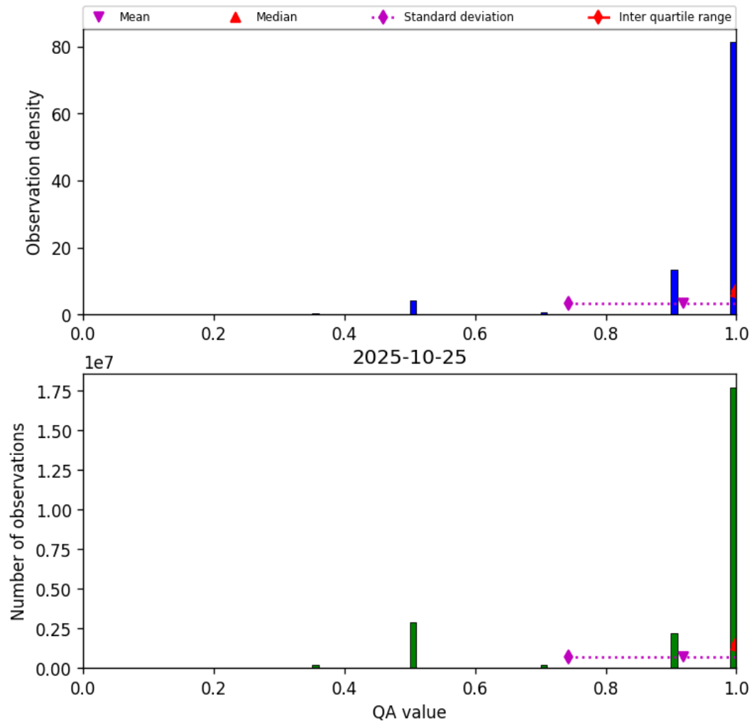
Figure 27: Histogram of “QA value” for 2025-10-25 to 2025-10-25
