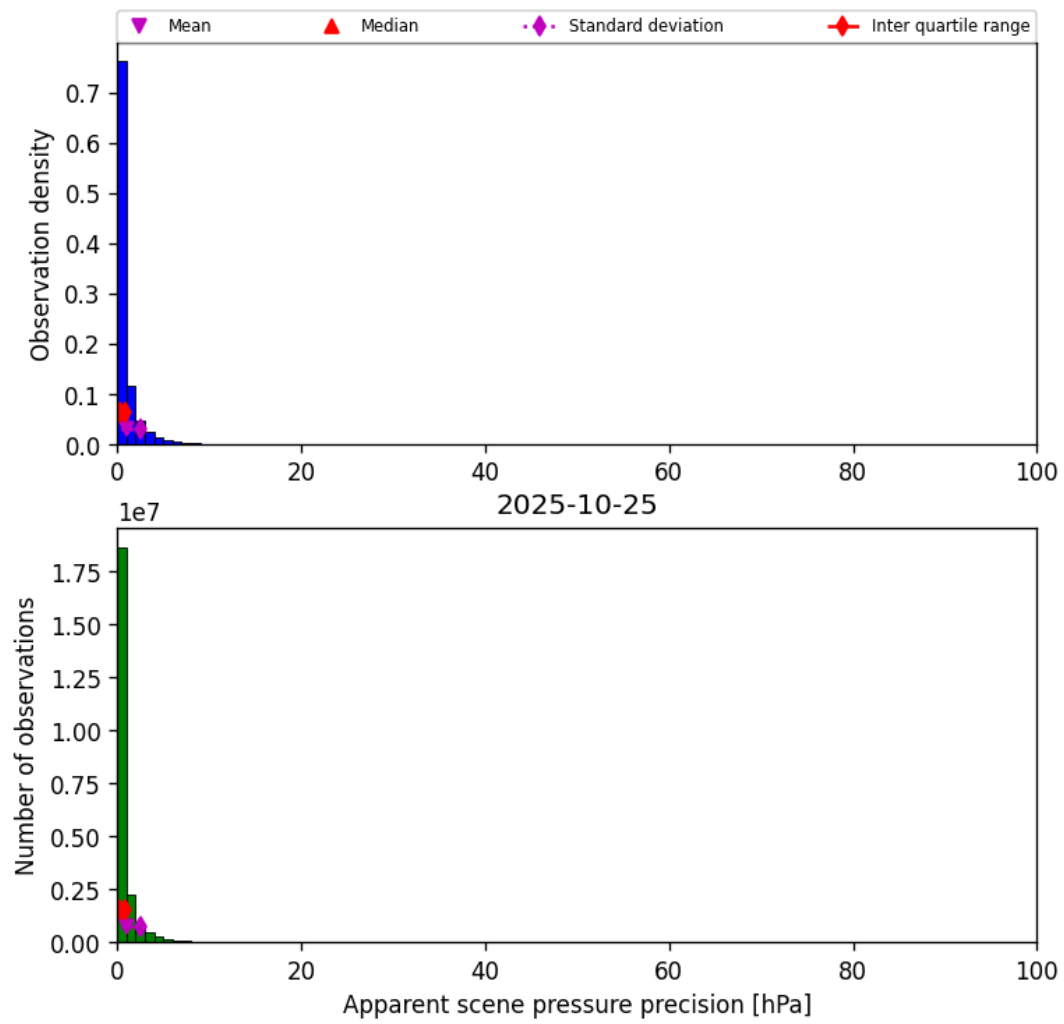
Figure 35: Histogram of “Apparent scene pressure precision” for 2025-10-25 to 2025-10-25
