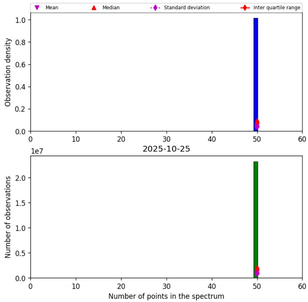
Figure 42: Histogram of “Number of points in the spectrum” for 2025-10-25 to 2025-10-25
