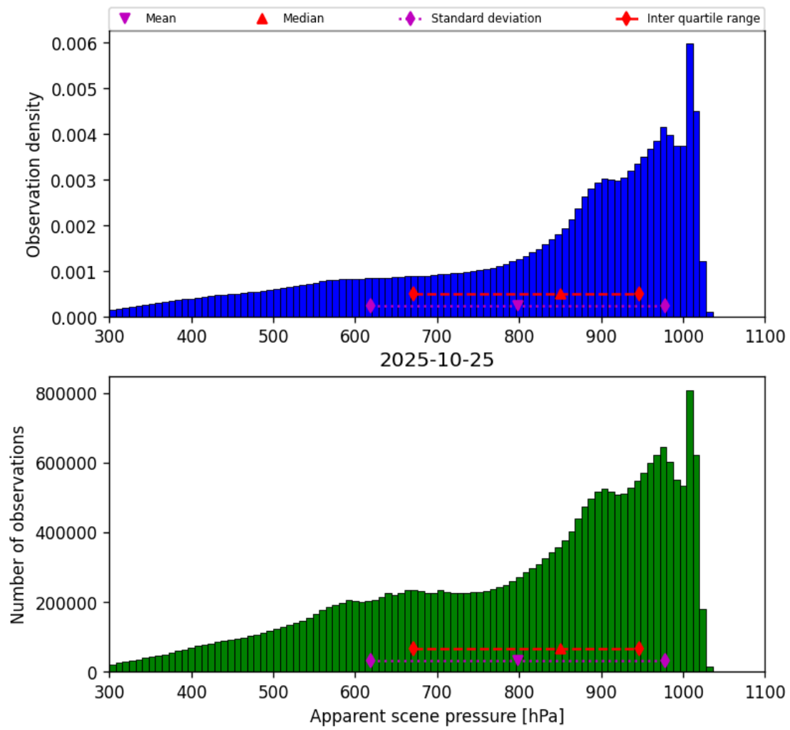
Figure 34: Histogram of “Apparent scene pressure” for 2025-10-25 to 2025-10-25
