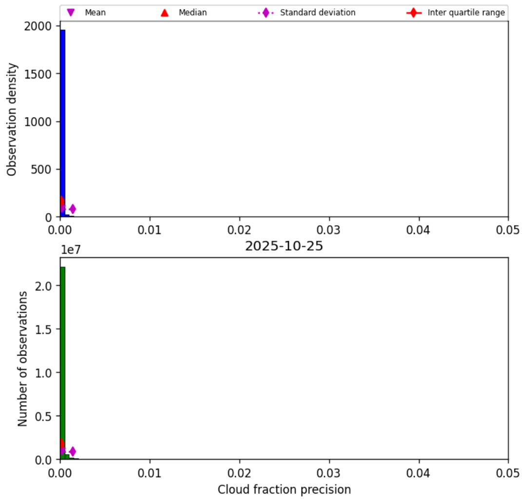
Figure 31: Histogram of “Cloud fraction precision” for 2025-10-25 to 2025-10-25
