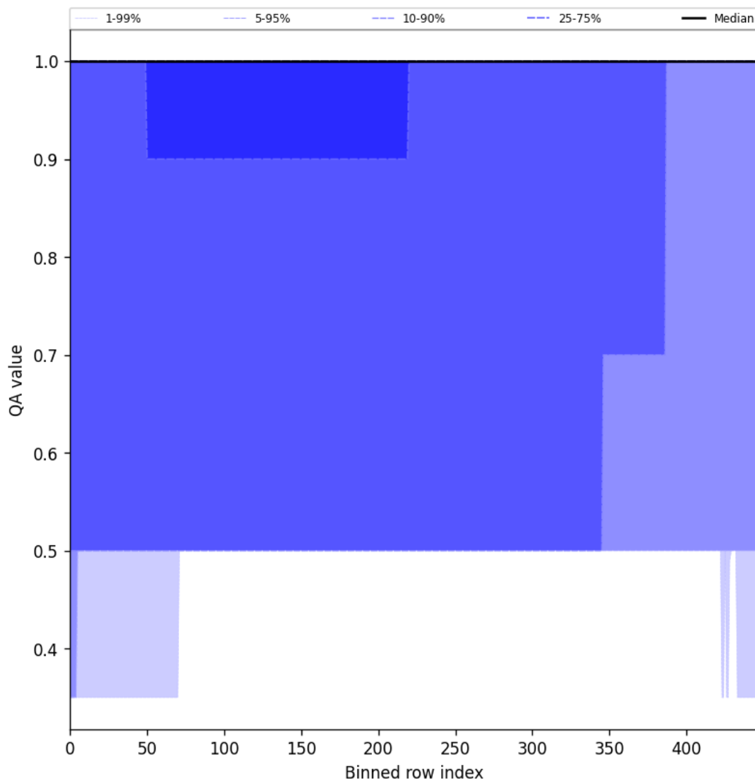
Figure 44: Along track statistics of “QA value” for 2025-10-25 to 2025-10-25
