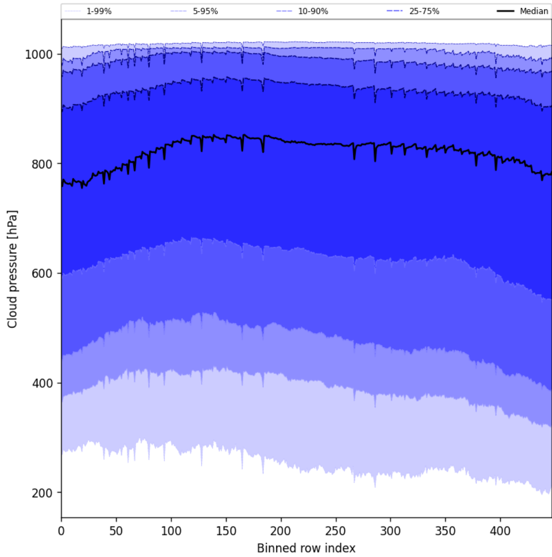
Figure 45: Along track statistics of “Cloud pressure” for 2025-10-25 to 2025-10-25
