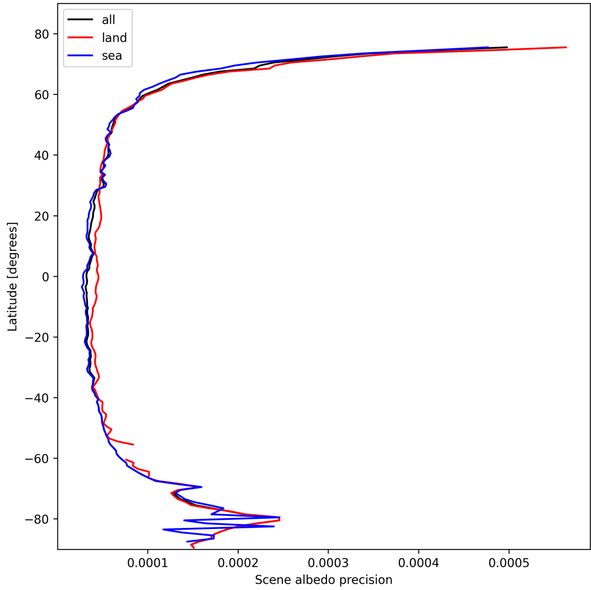
Figure 16: Zonal average of “Scene albedo precision” for 2025-10-25 to 2025-10-25.
