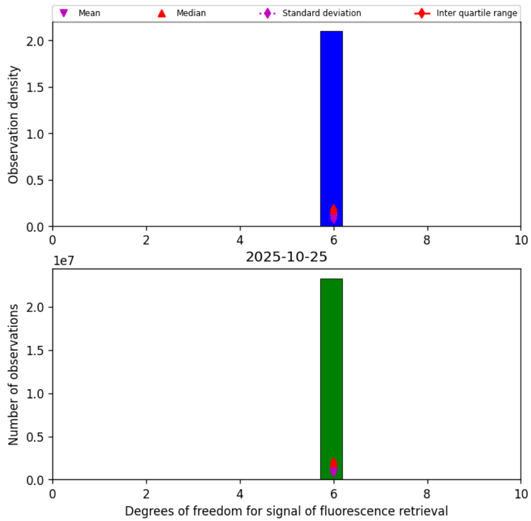
Figure 41: Histogram of “Degrees of freedom for signal of fluorescence retrieval” for 2025-10-25 to 2025-10-25
