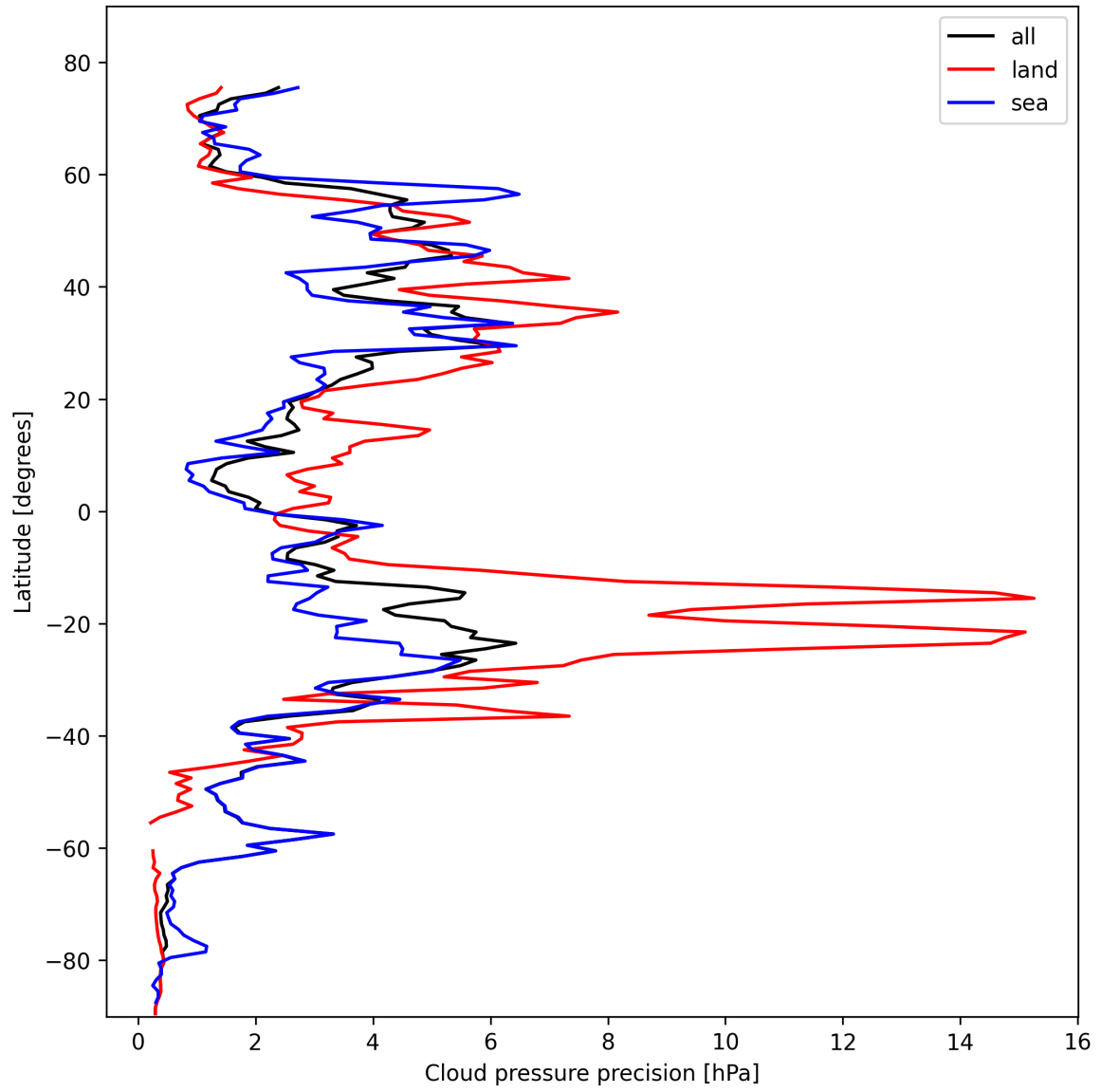
Figure 12: Zonal average of “Cloud pressure precision” for 2025-10-25 to 2025-10-25.
