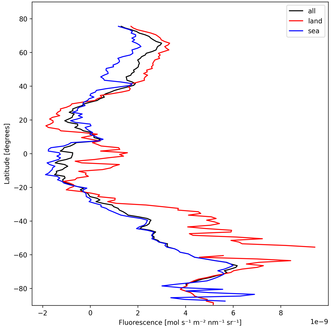
Figure 21: Zonal average of “Fluorescence” for 2025-10-25 to 2025-10-25.
