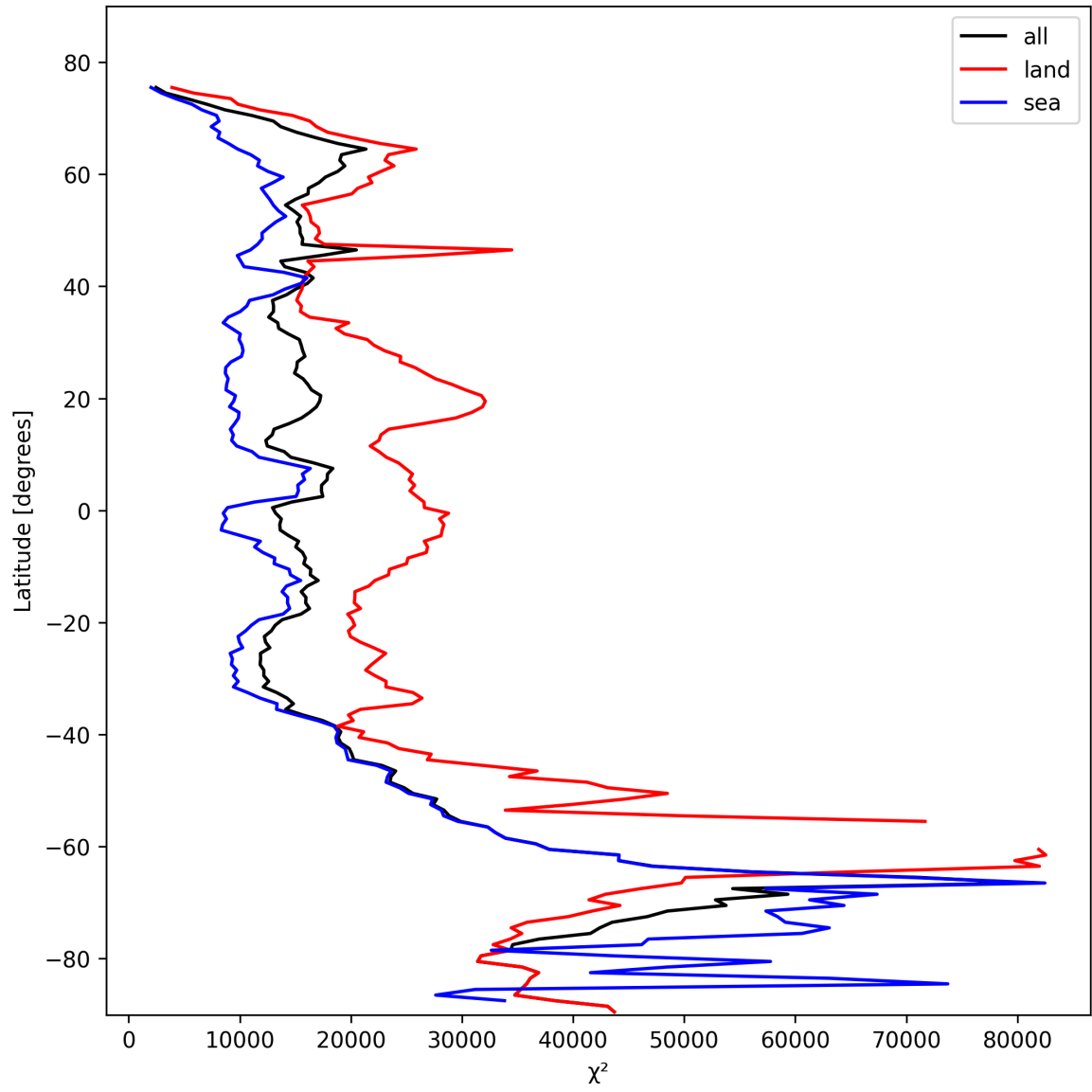
Figure 19: Zonal average of “ \chi^2 ” for 2025-10-25 to 2025-10-25.
