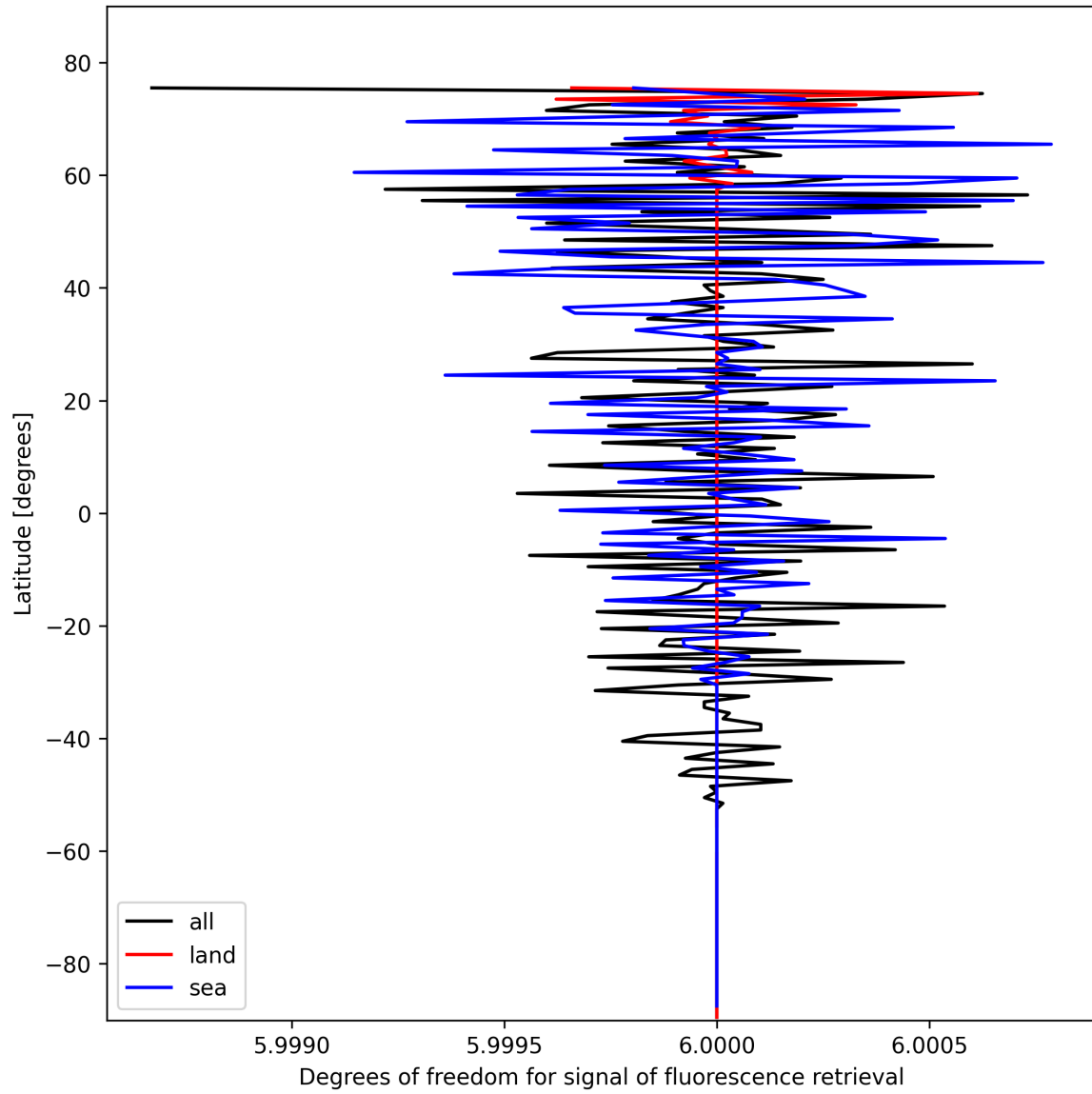
Figure 24: Zonal average of “Degrees of freedom for signal of fluorescence retrieval” for 2025-10-25 to 2025-10-25.
