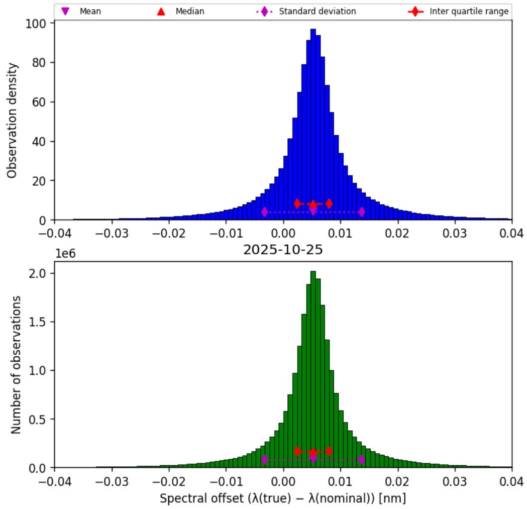
Figure 43: Histogram of “Spectral offset ( \lambda_{\text{true}} - \lambda_{\text{nominal}} )” for 2025-10-25 to 2025-10-25
