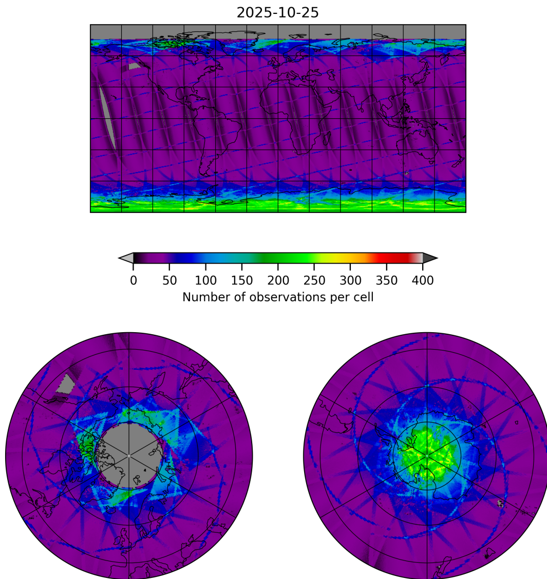
Figure 9: Map of the number of observations for 2025-10-25 to 2025-10-25
