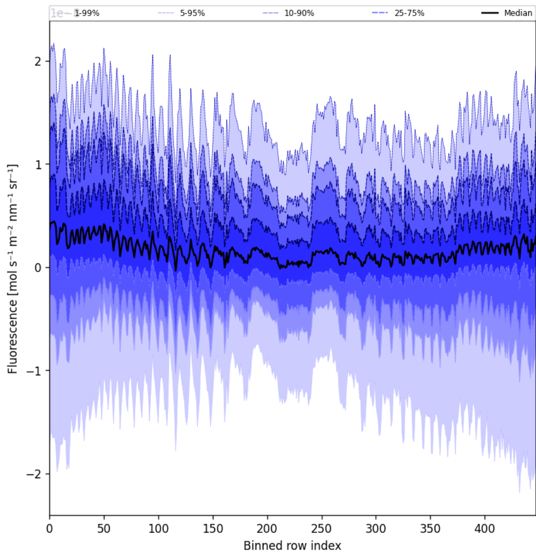
Figure 55: Along track statistics of “Fluorescence” for 2025-10-25 to 2025-10-25
