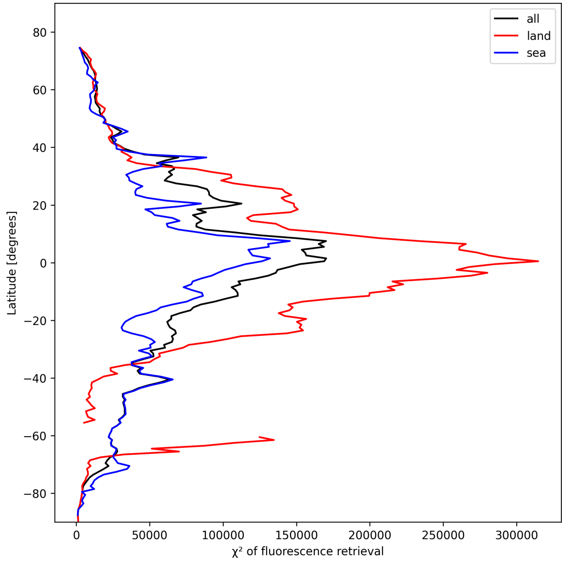
Figure 23: Zonal average of “ \chi^2 of fluorescence retrieval” for 2025-10-28 to 2025-10-29.
