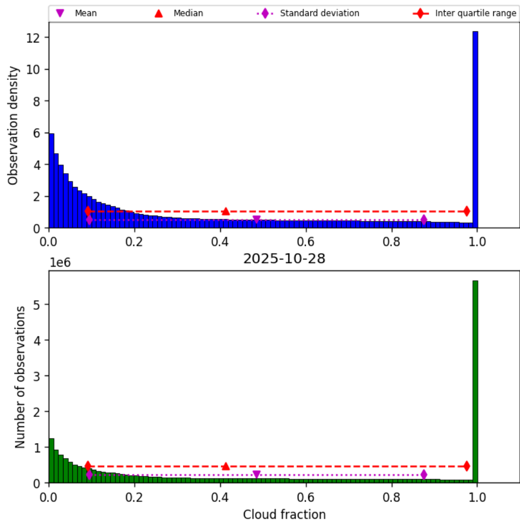
Figure 30: Histogram of “Cloud fraction” for 2025-10-28 to 2025-10-29
