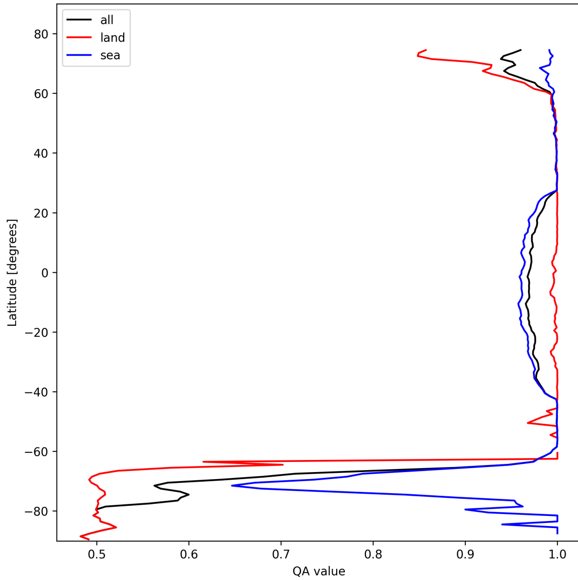
Figure 10: Zonal average of “QA value” for 2025-10-28 to 2025-10-29.
