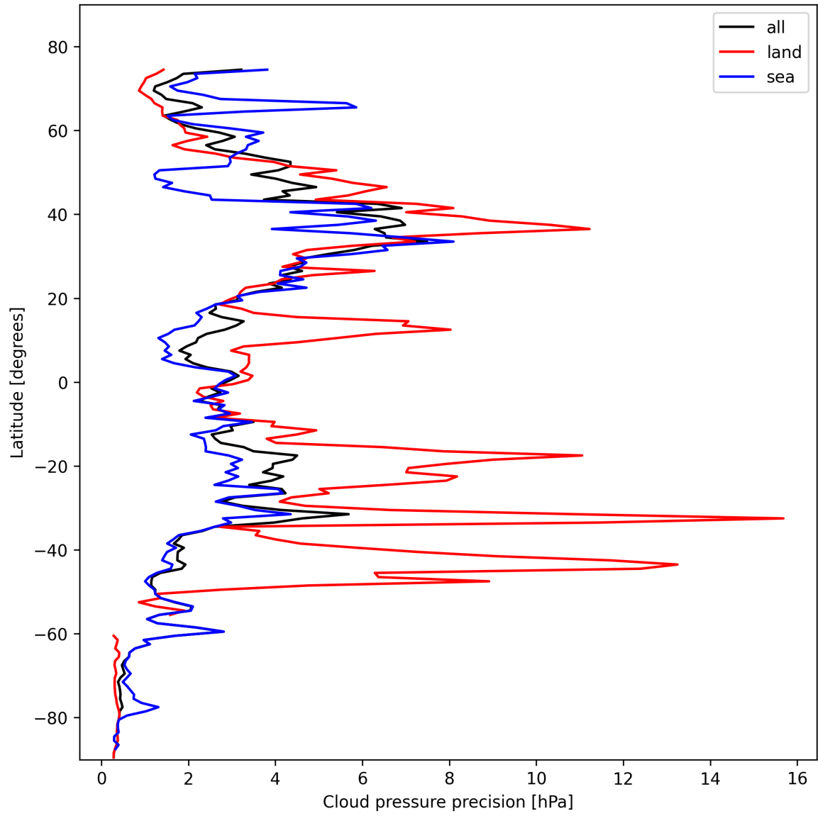
Figure 12: Zonal average of "Cloud pressure precision" for 2025-10-28 to 2025-10-29.
