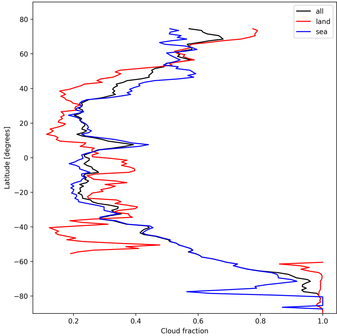
Figure 13: Zonal average of “Cloud fraction” for 2025-10-28 to 2025-10-29.
