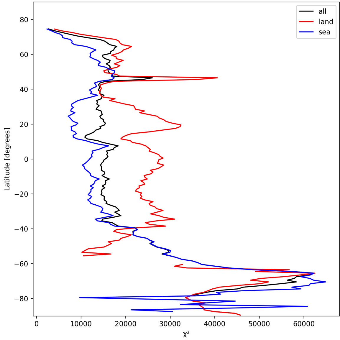
Figure 19: Zonal average of “ \chi^2 ” for 2025-10-28 to 2025-10-29.
