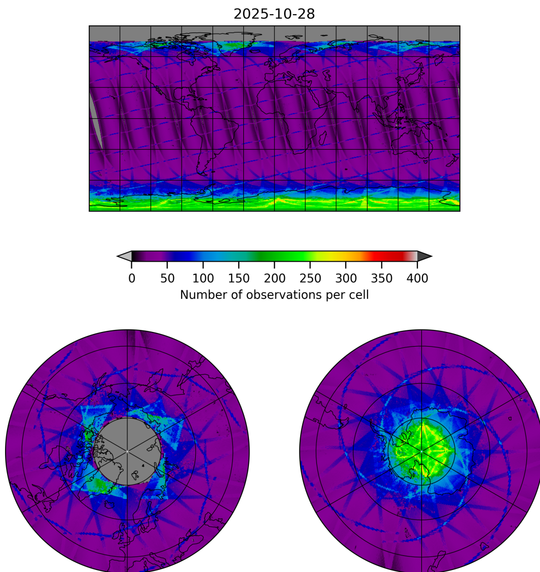
Figure 9: Map of the number of observations for 2025-10-28 to 2025-10-29
