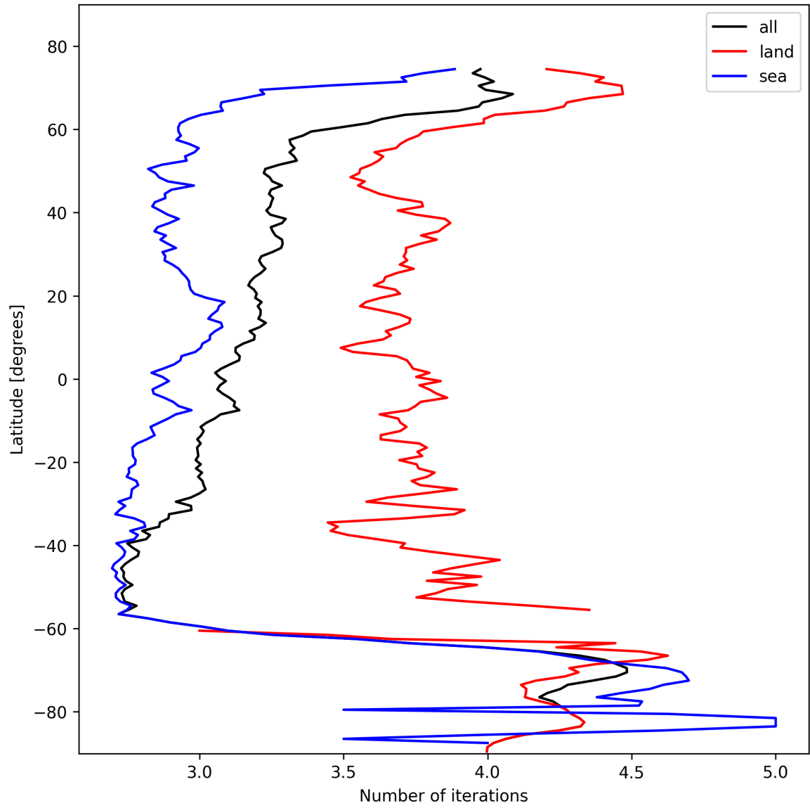
Figure 20: Zonal average of “Number of iterations” for 2025-10-28 to 2025-10-29.
