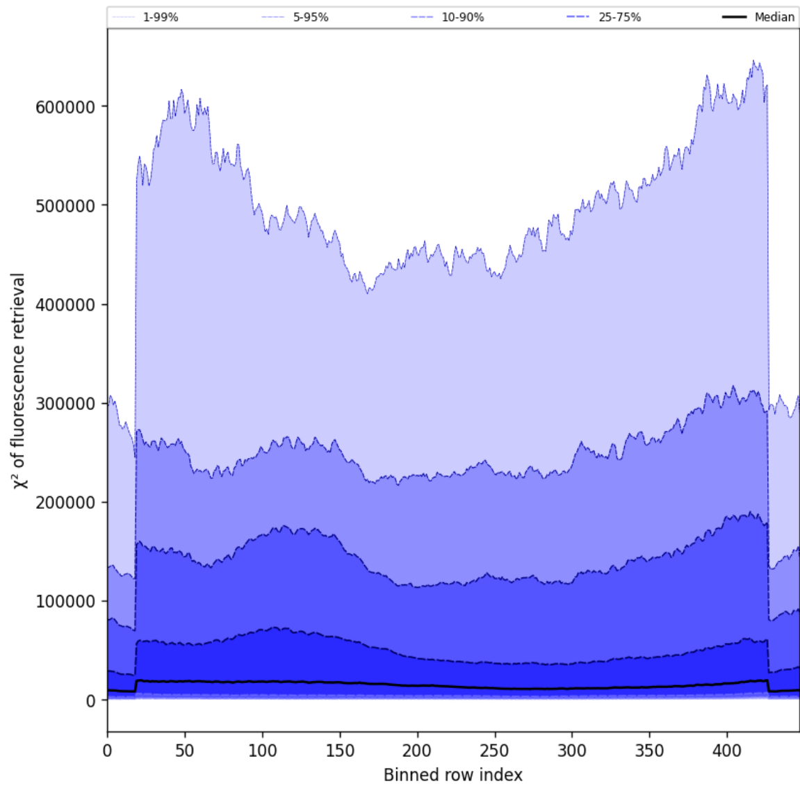
Figure 57: Along track statistics of “ \chi^2 of fluorescence retrieval” for 2025-10-28 to 2025-10-29
