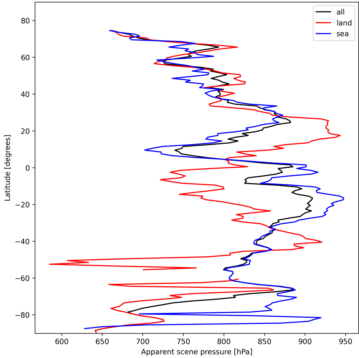
Figure 17: Zonal average of “Apparent scene pressure” for 2025-10-28 to 2025-10-29.
