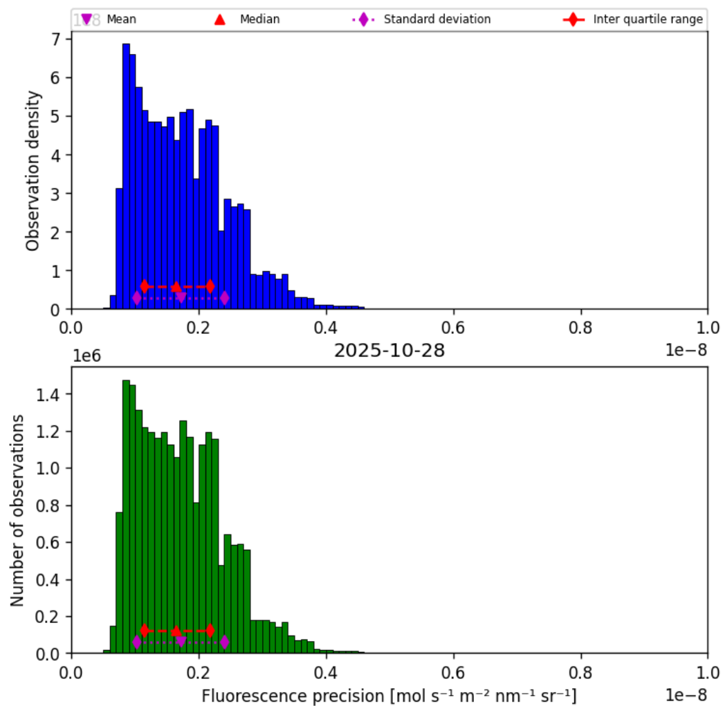
Figure 39: Histogram of “Fluorescence precision” for 2025-10-28 to 2025-10-29
