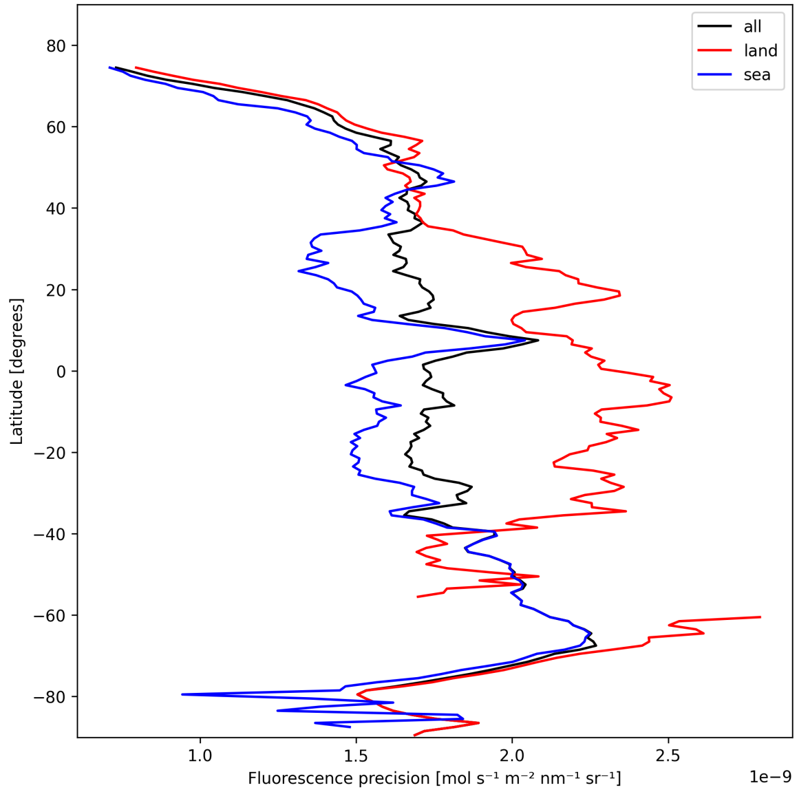
Figure 22: Zonal average of “Fluorescence precision” for 2025-10-28 to 2025-10-29.
