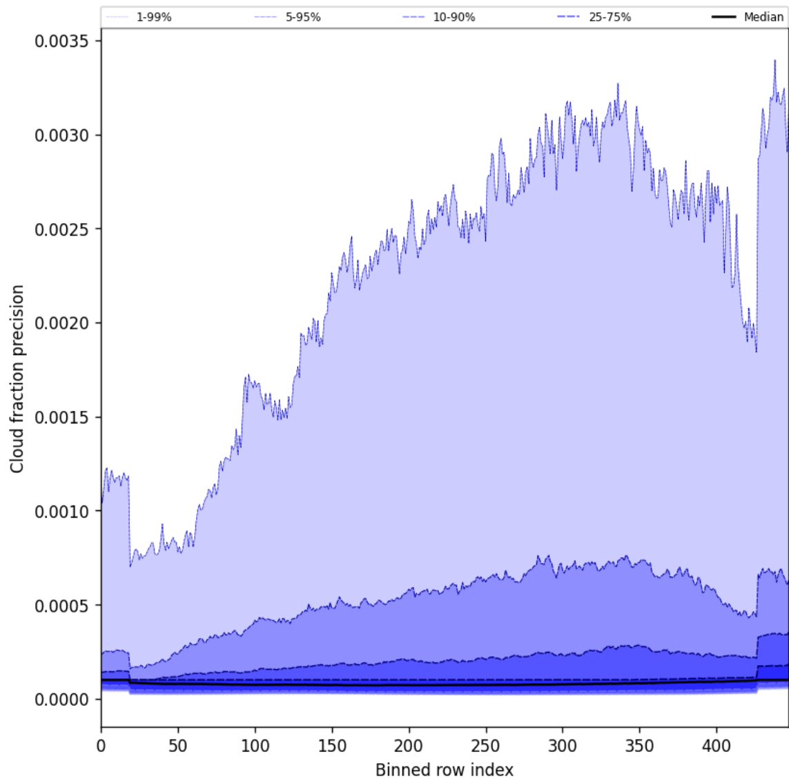
Figure 48: Along track statistics of “Cloud fraction precision” for 2025-10-28 to 2025-10-29
