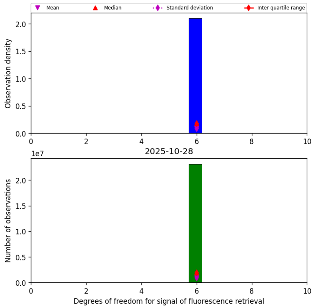
Figure 41: Histogram of “Degrees of freedom for signal of fluorescence retrieval” for 2025-10-28 to 2025-10-29
