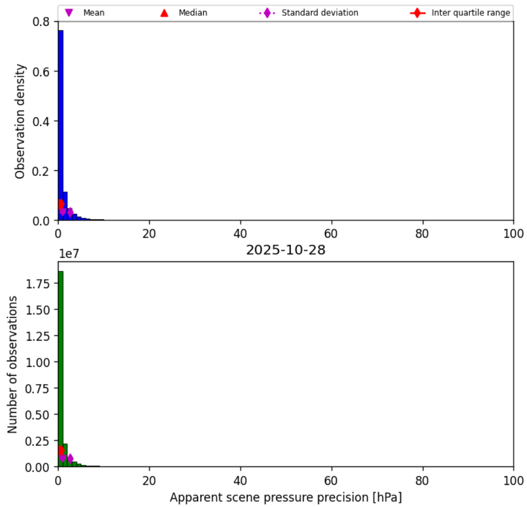
Figure 35: Histogram of “Apparent scene pressure precision” for 2025-10-28 to 2025-10-29
