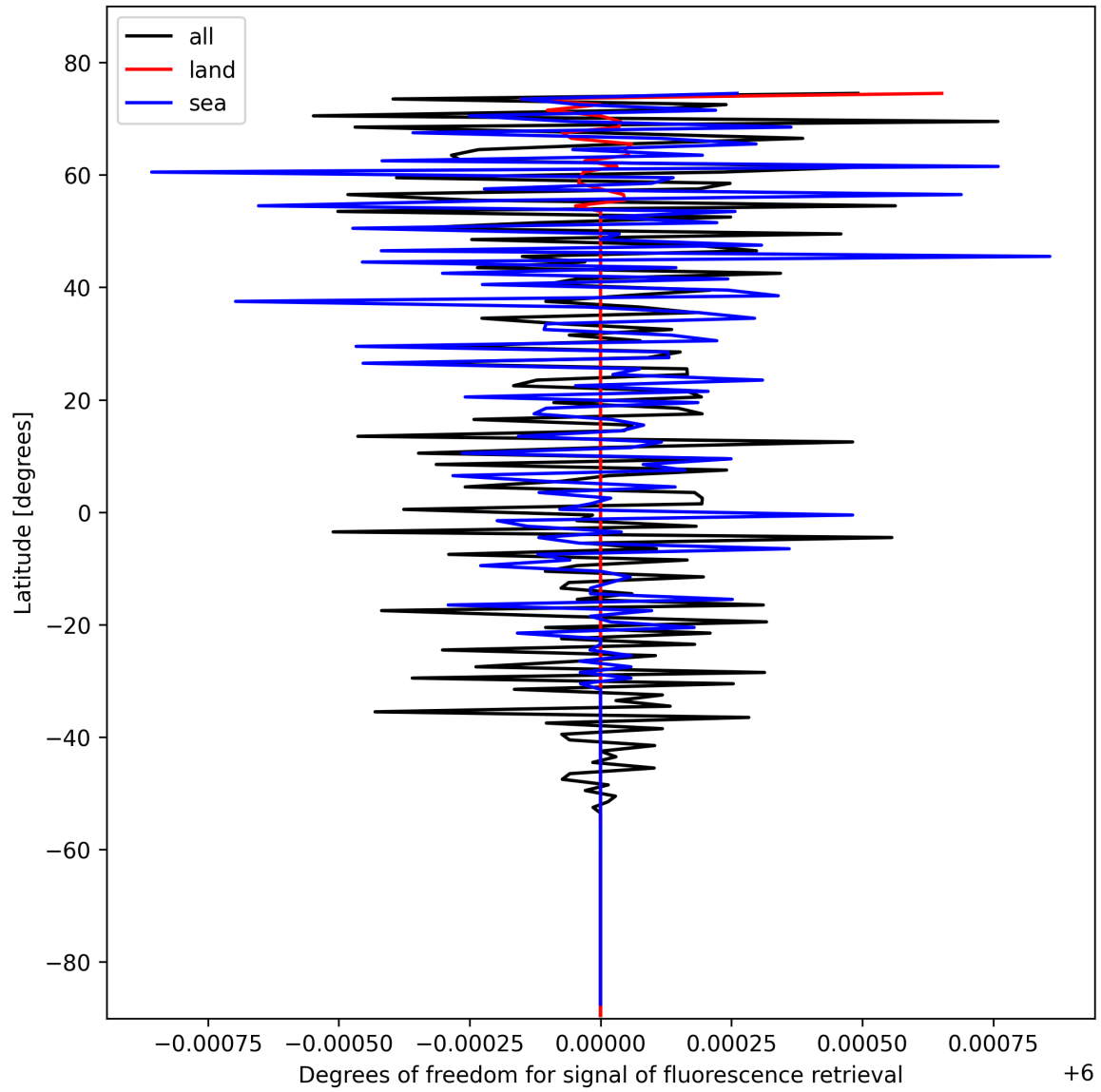
Figure 24: Zonal average of “Degrees of freedom for signal of fluorescence retrieval” for 2025-10-28 to 2025-10-29.
