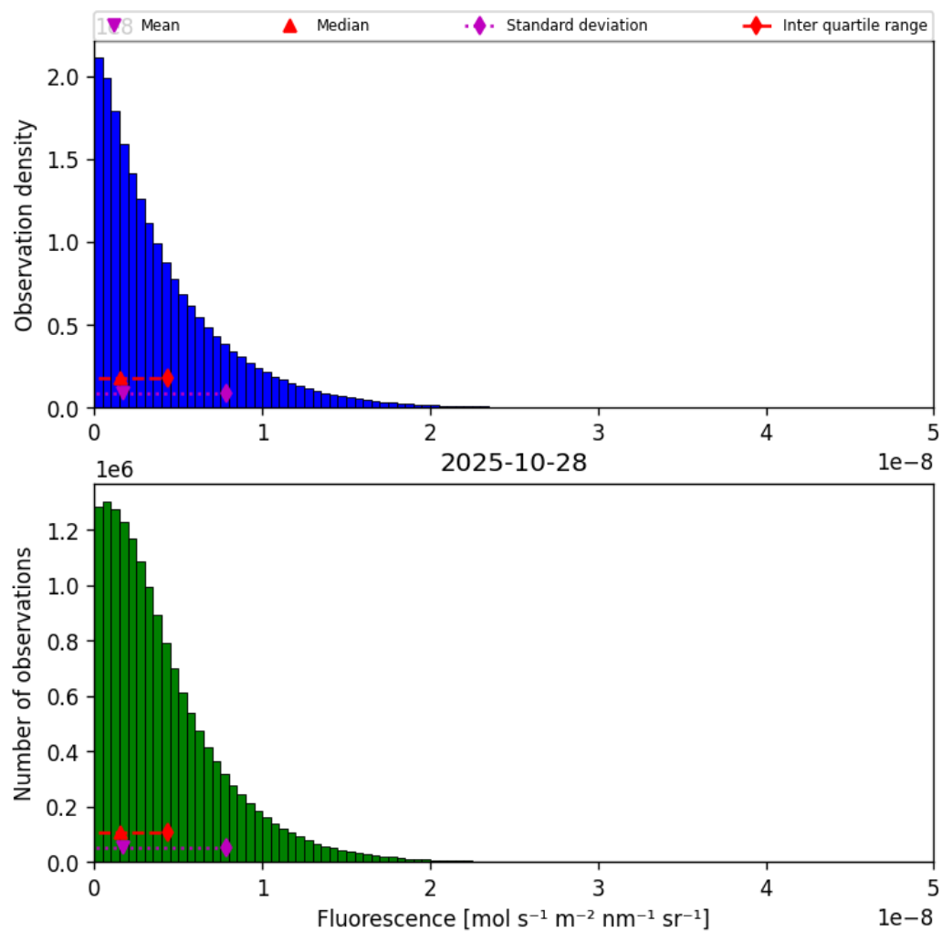
Figure 38: Histogram of “Fluorescence” for 2025-10-28 to 2025-10-29
