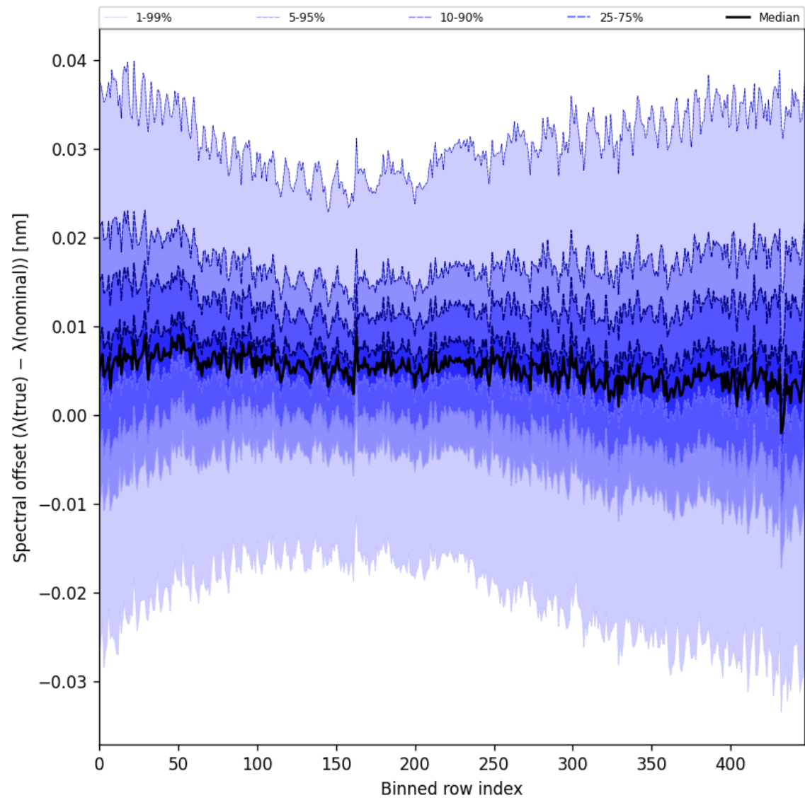
Figure 60: Along track statistics of “Spectral offset ( \lambda_{\text{true}} - \lambda_{\text{nominal}} )” for 2025-10-28 to 2025-10-29
