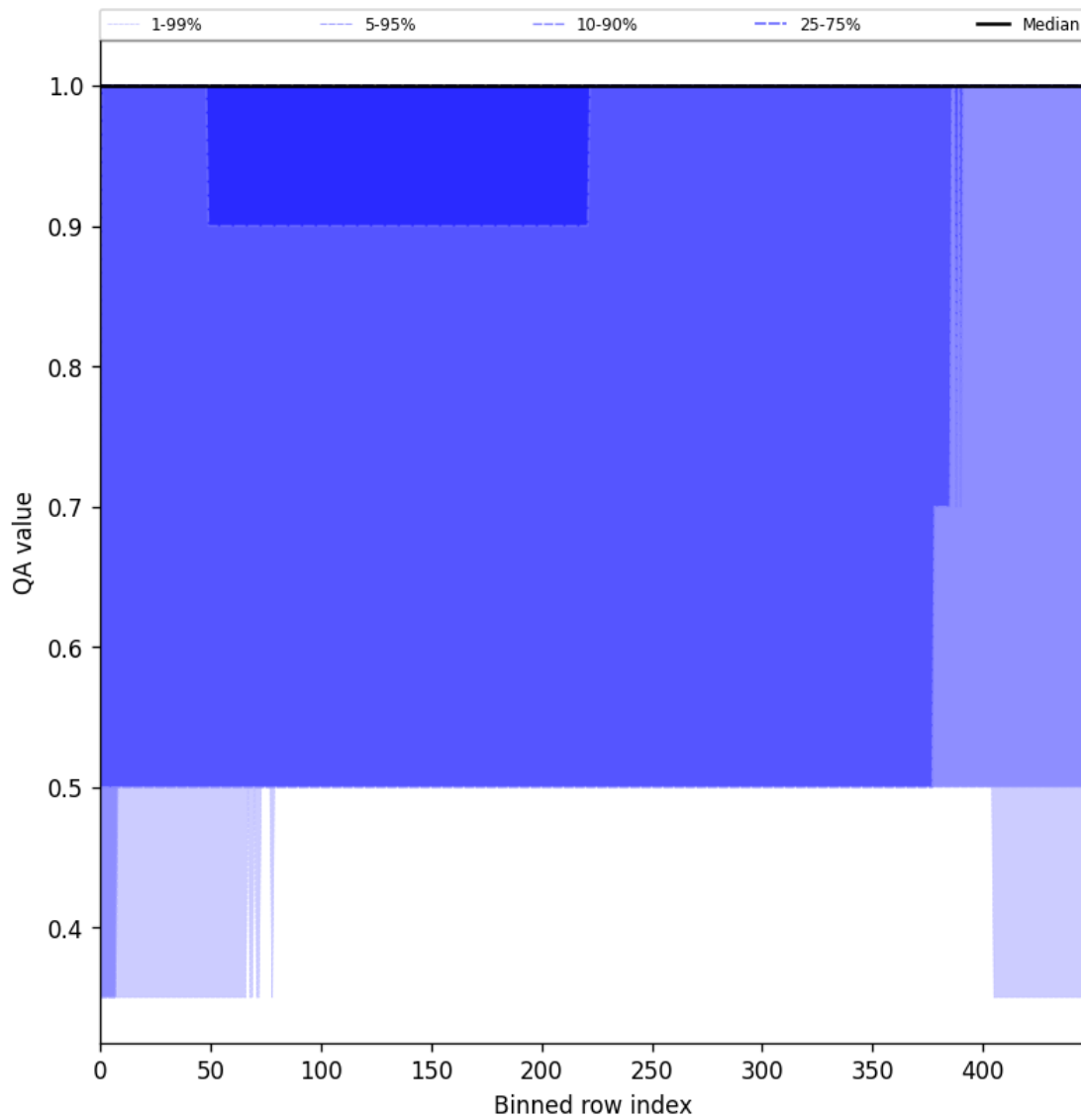
Figure 44: Along track statistics of “QA value” for 2025-10-28 to 2025-10-29
