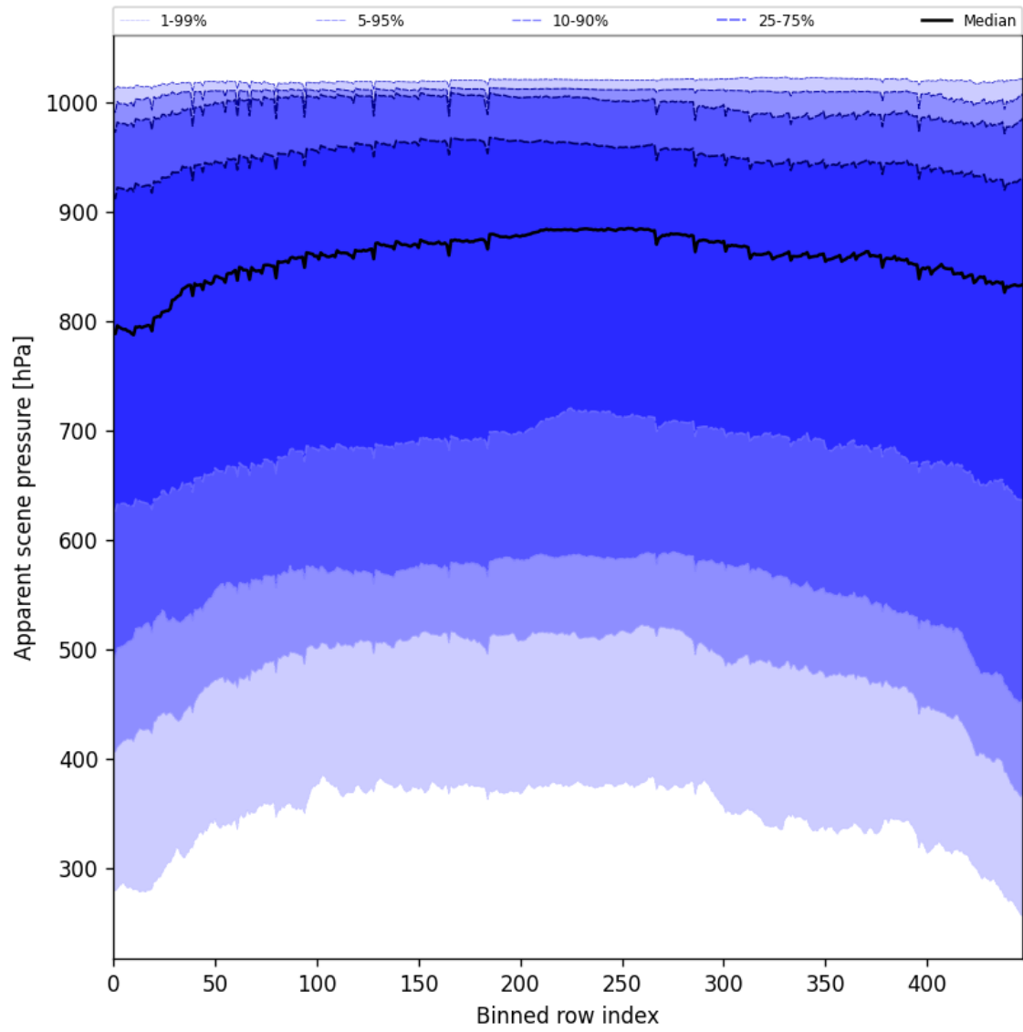
Figure 51: Along track statistics of “Apparent scene pressure” for 2025-10-28 to 2025-10-29
