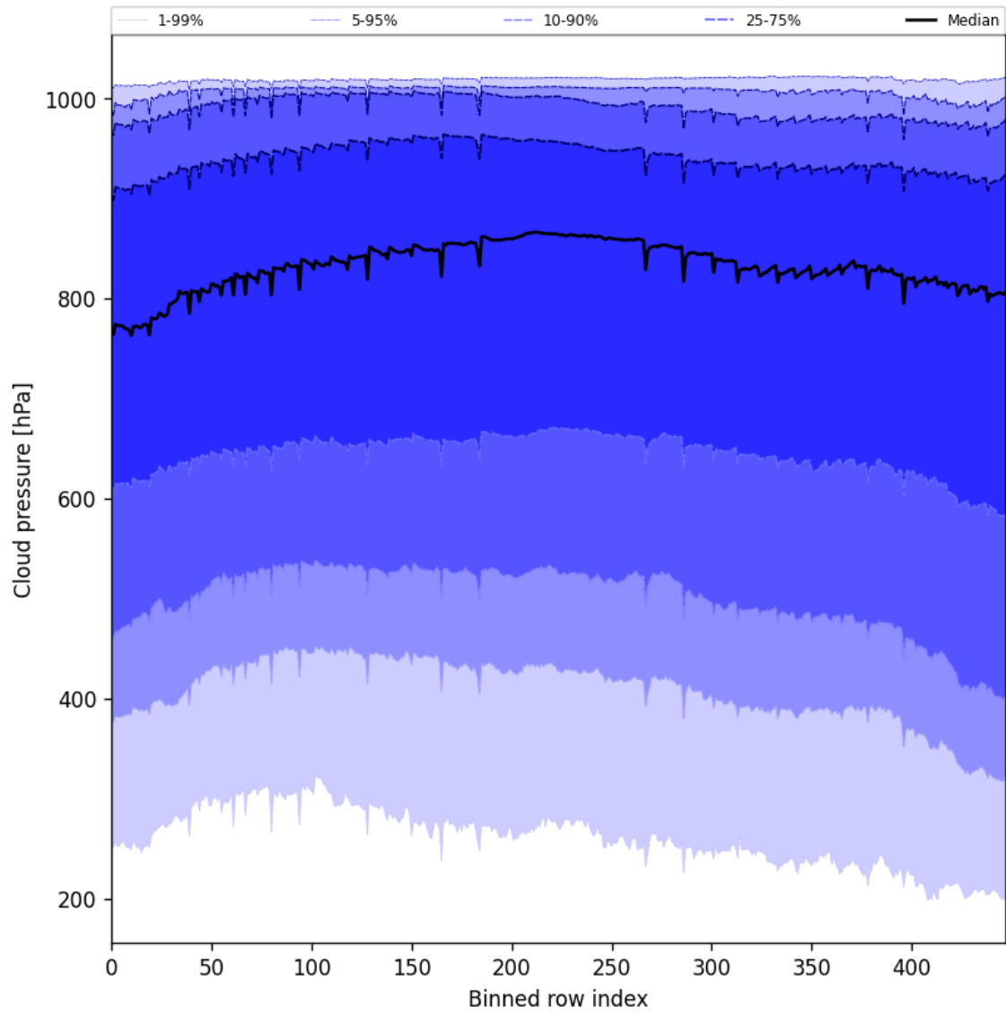
Figure 45: Along track statistics of “Cloud pressure” for 2025-10-28 to 2025-10-29
