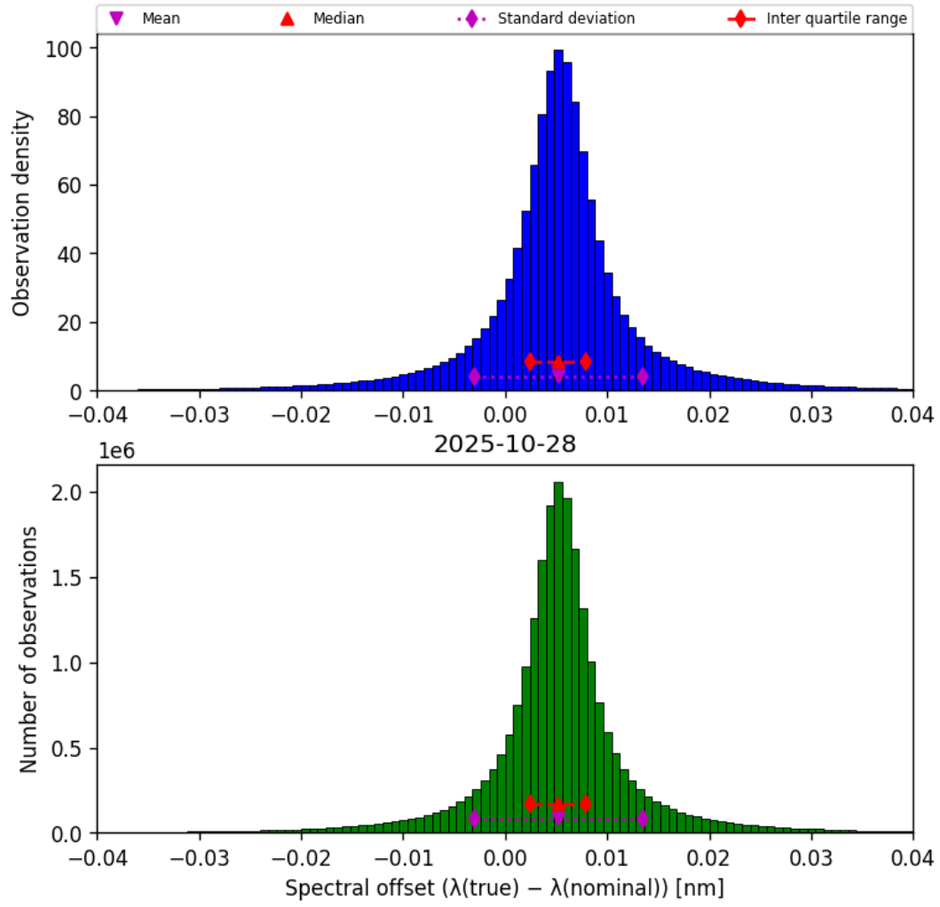
Figure 43: Histogram of “Spectral offset ( \lambda_{\text{true}} - \lambda_{\text{nominal}} )” for 2025-10-28 to 2025-10-29
