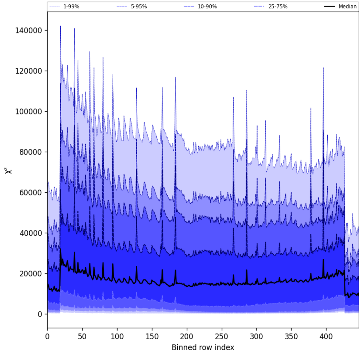
Figure 53: Along track statistics of “ \chi^2 ” for 2025-10-28 to 2025-10-29
