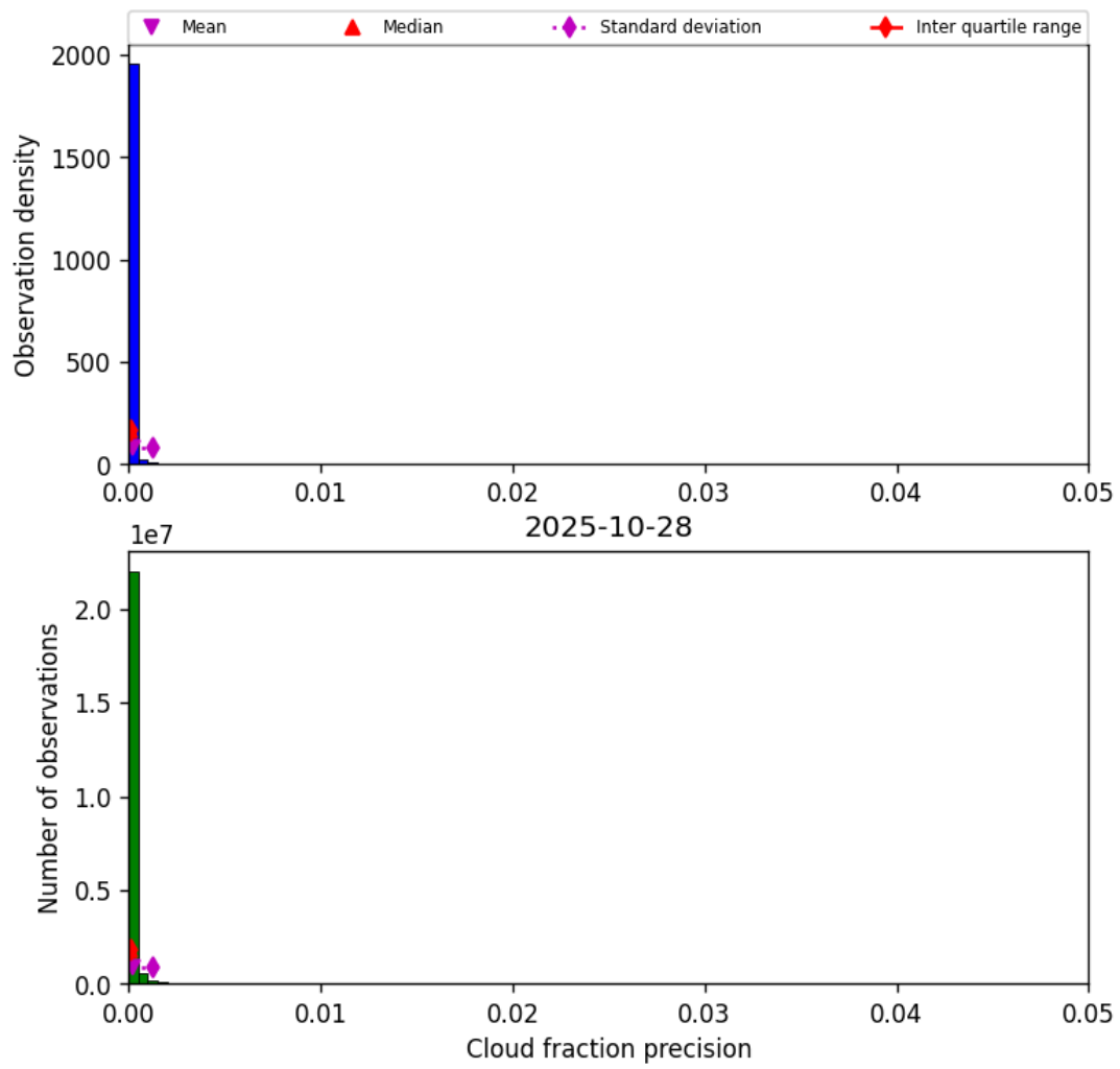
Figure 31: Histogram of “Cloud fraction precision” for 2025-10-28 to 2025-10-29
