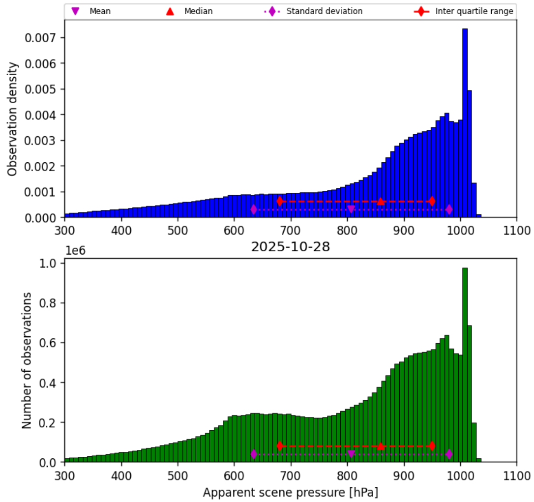
Figure 34: Histogram of “Apparent scene pressure” for 2025-10-28 to 2025-10-29
