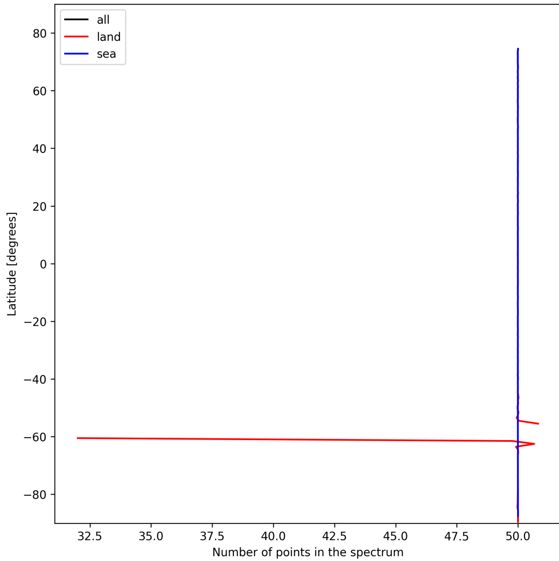
Figure 25: Zonal average of “Number of points in the spectrum” for 2025-10-28 to 2025-10-29.
