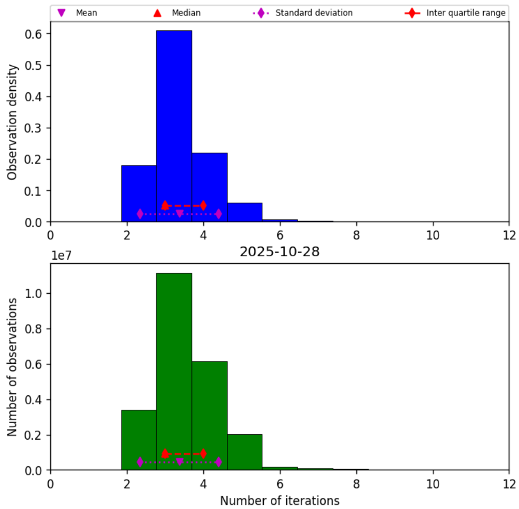
Figure 37: Histogram of “Number of iterations” for 2025-10-28 to 2025-10-29
