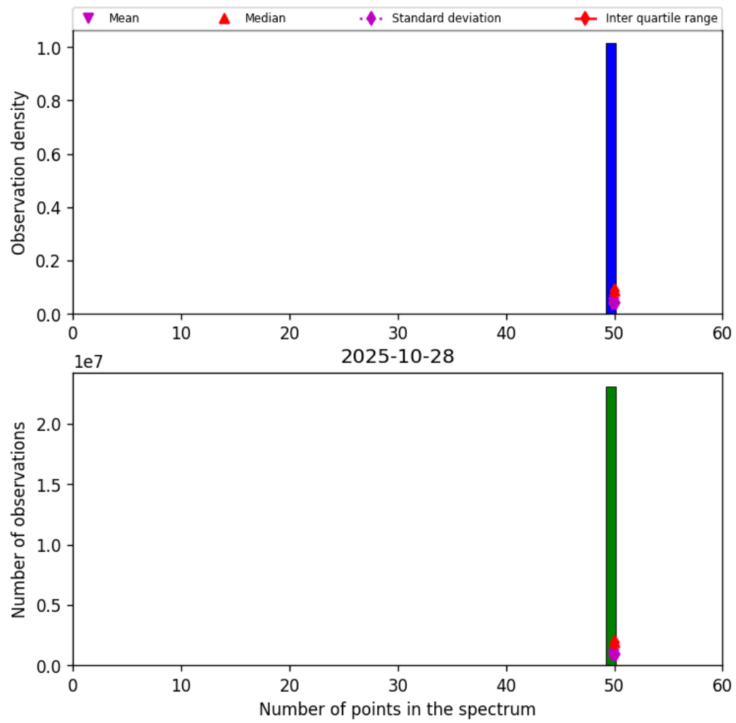
Figure 42: Histogram of “Number of points in the spectrum” for 2025-10-28 to 2025-10-29
