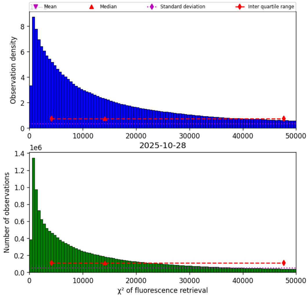
Figure 40: Histogram of “ \chi^2 of fluorescence retrieval” for 2025-10-28 to 2025-10-29
