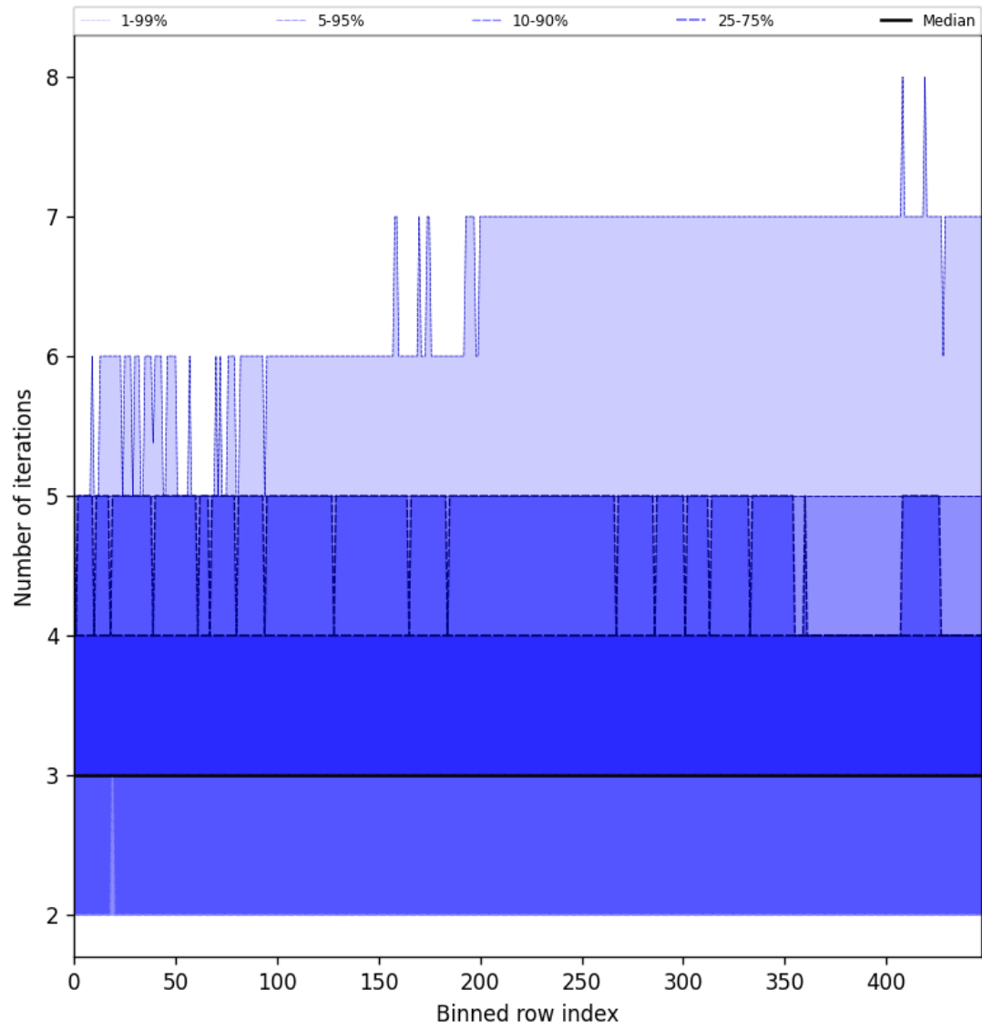
Figure 54: Along track statistics of “Number of iterations” for 2025-10-28 to 2025-10-29
