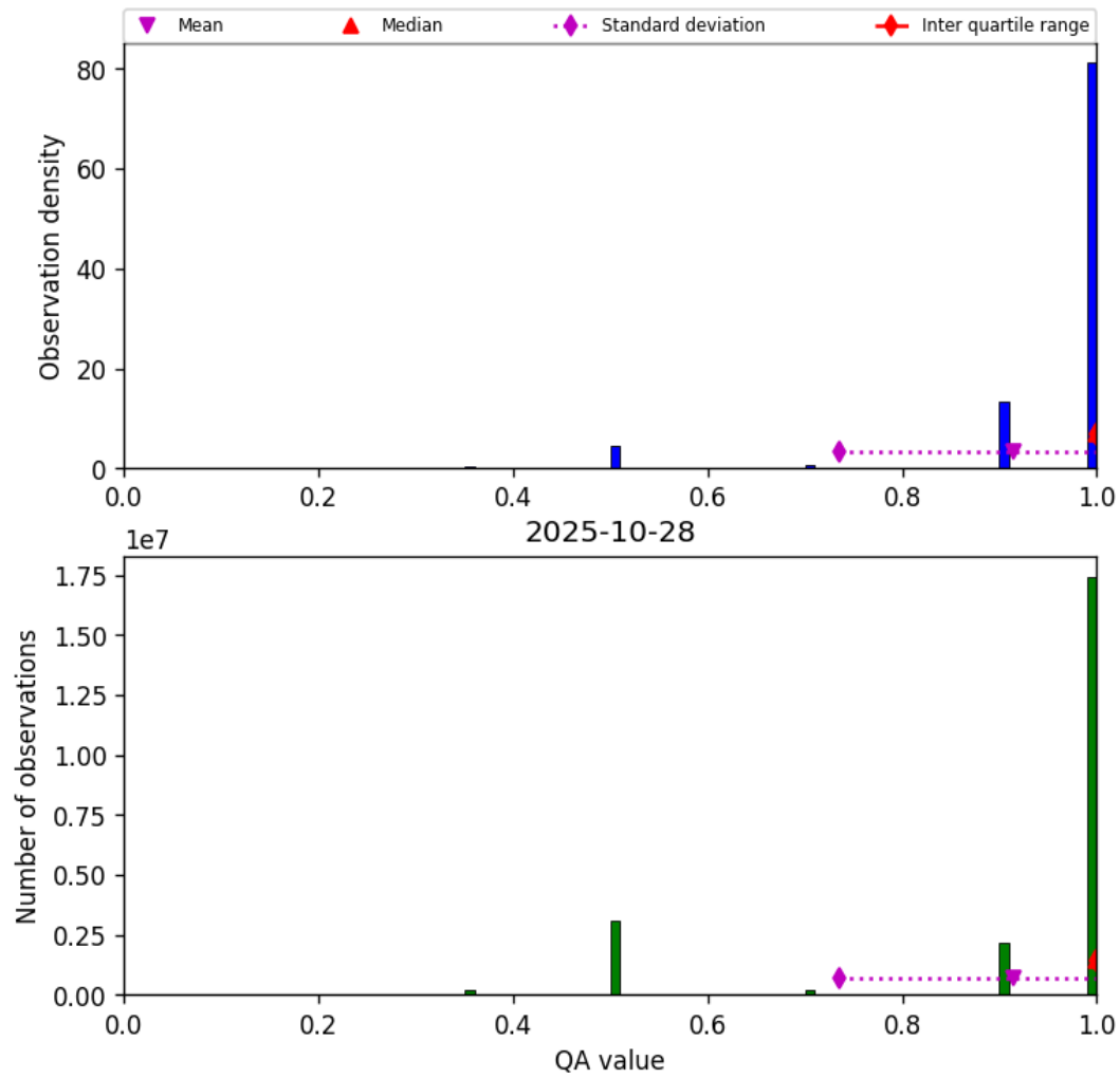
Figure 27: Histogram of “QA value” for 2025-10-28 to 2025-10-29
