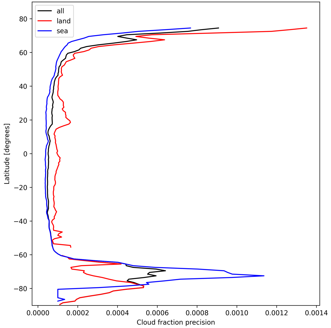
Figure 14: Zonal average of “Cloud fraction precision” for 2025-10-28 to 2025-10-29.
