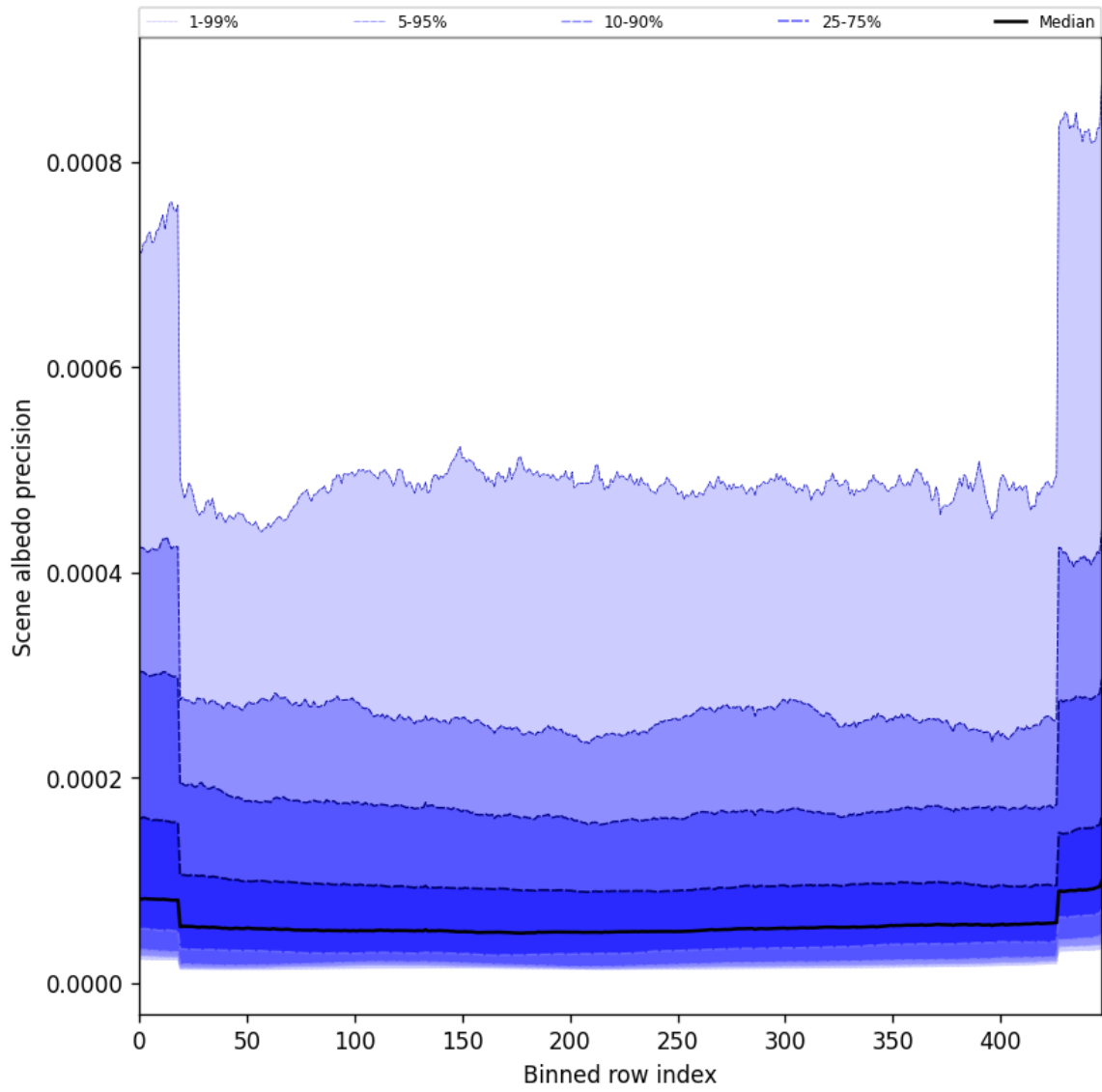
Figure 50: Along track statistics of “Scene albedo precision” for 2025-10-28 to 2025-10-29
