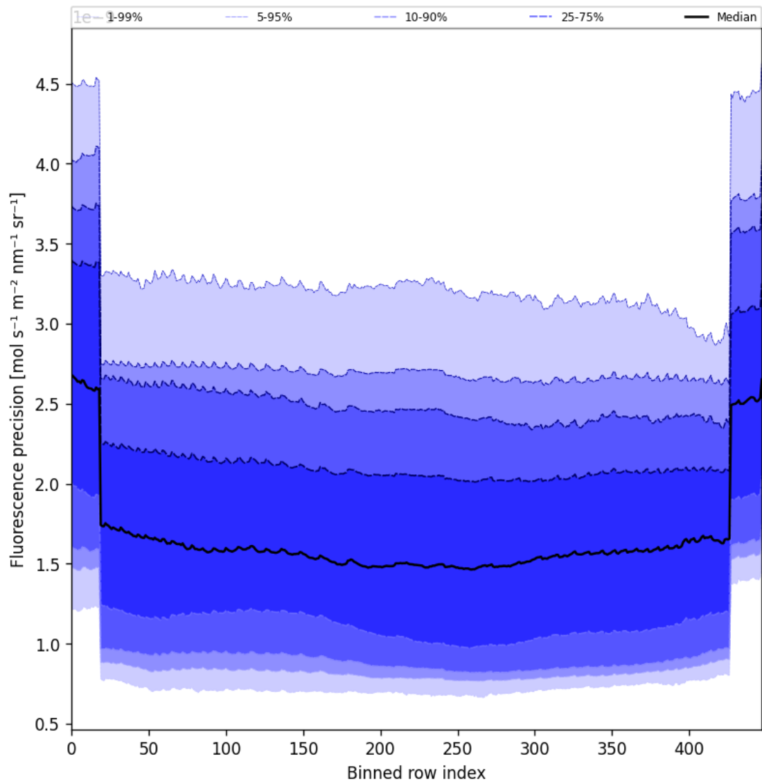
Figure 56: Along track statistics of “Fluorescence precision” for 2025-10-28 to 2025-10-29
