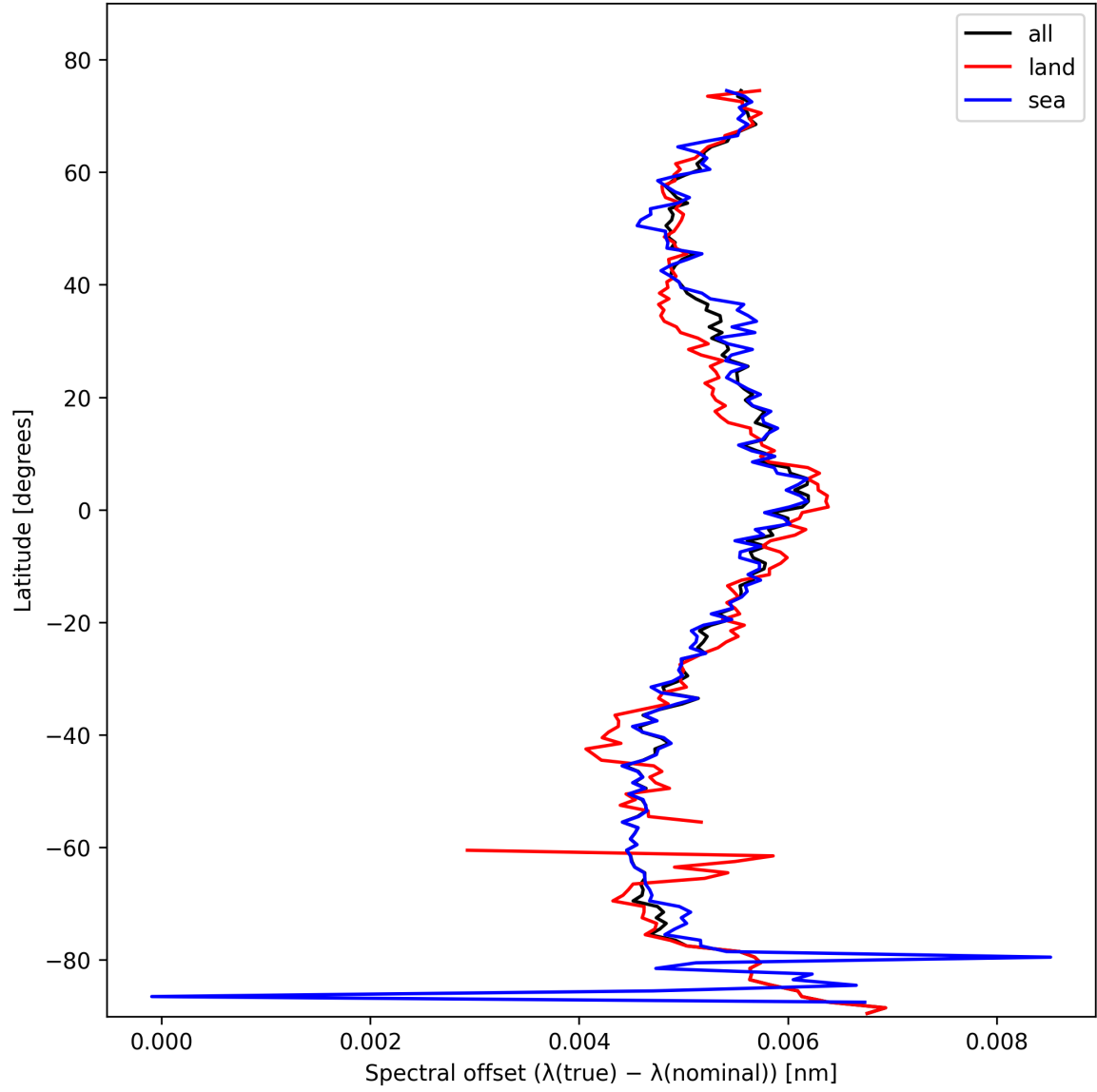
Figure 26: Zonal average of “Spectral offset ( \lambda_{\text{true}} - \lambda_{\text{nominal}} )” for 2025-10-28 to 2025-10-29.
