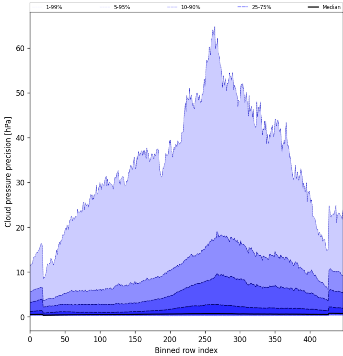
Figure 46: Along track statistics of “Cloud pressure precision” for 2025-10-28 to 2025-10-29
