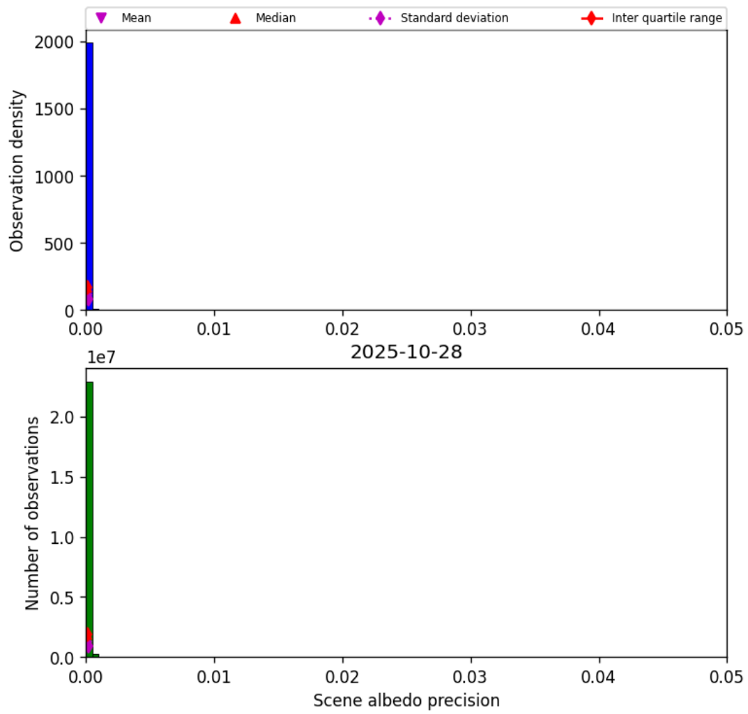
Figure 33: Histogram of “Scene albedo precision” for 2025-10-28 to 2025-10-29
