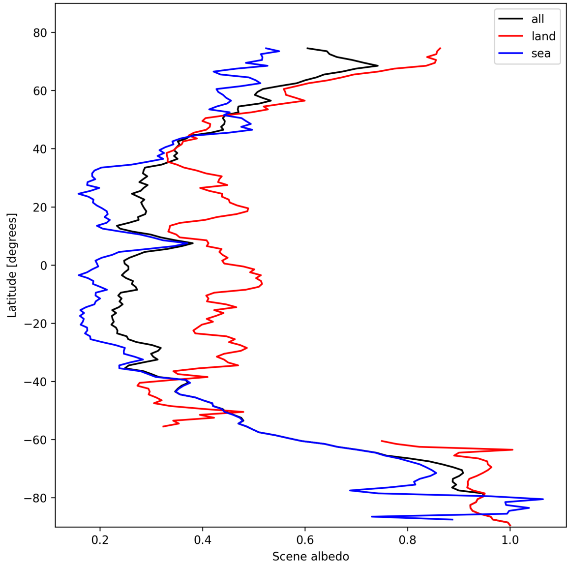
Figure 15: Zonal average of “Scene albedo” for 2025-10-28 to 2025-10-29.
