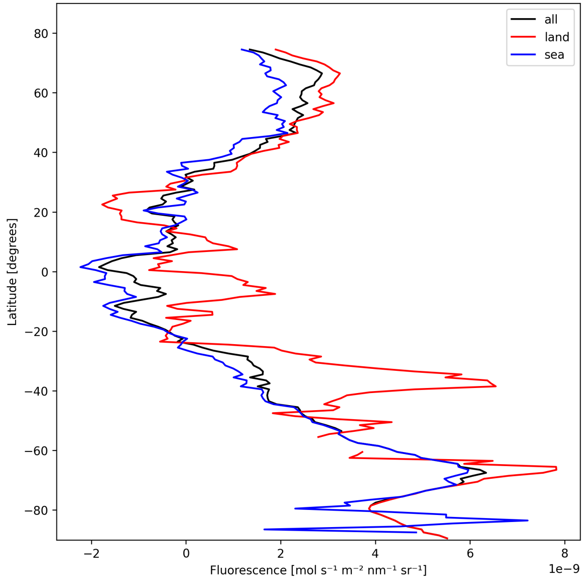
Figure 21: Zonal average of “Fluorescence” for 2025-10-28 to 2025-10-29.
