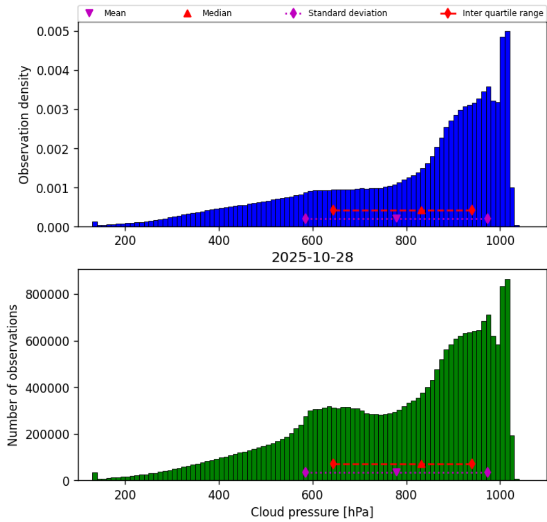
Figure 28: Histogram of “Cloud pressure” for 2025-10-28 to 2025-10-29
