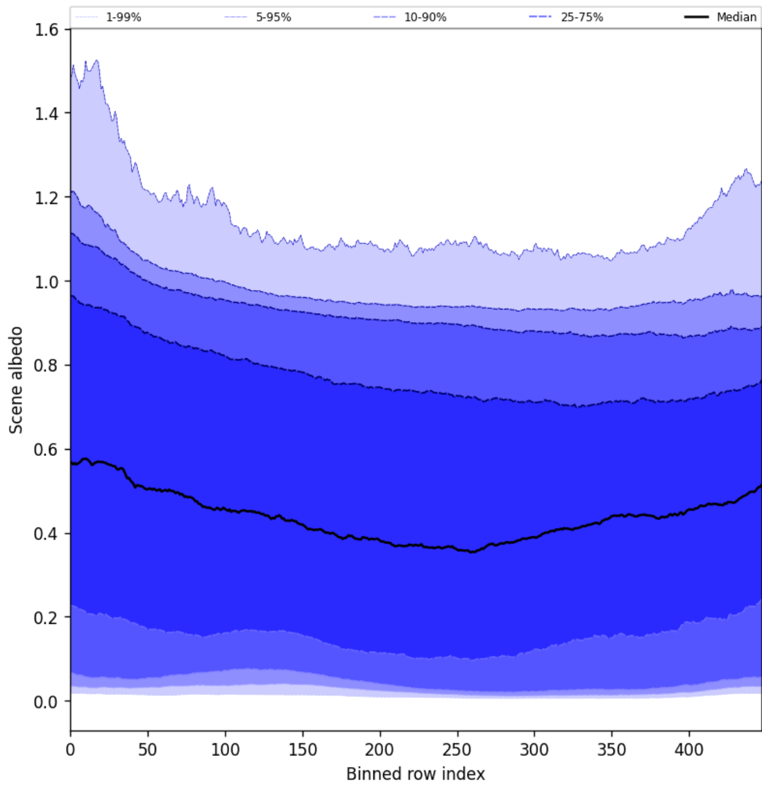
Figure 49: Along track statistics of “Scene albedo” for 2025-10-28 to 2025-10-29
