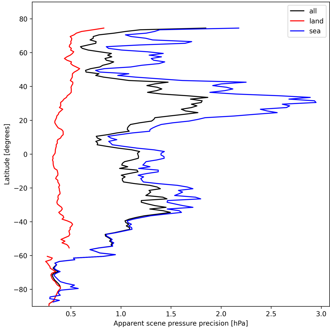
Figure 18: Zonal average of “Apparent scene pressure precision” for 2025-10-28 to 2025-10-29.
