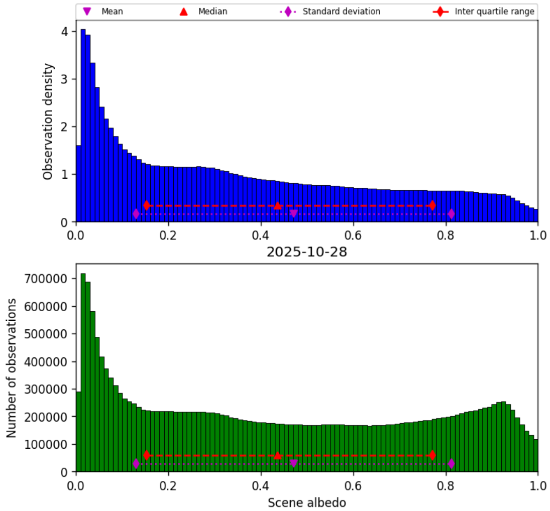
Figure 32: Histogram of “Scene albedo” for 2025-10-28 to 2025-10-29
