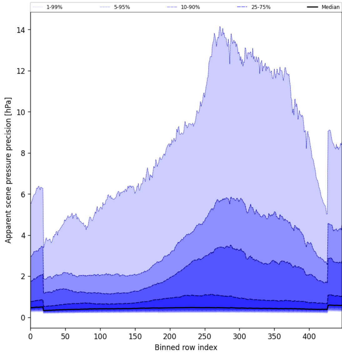
Figure 52: Along track statistics of “Apparent scene pressure precision” for 2025-10-28 to 2025-10-29
