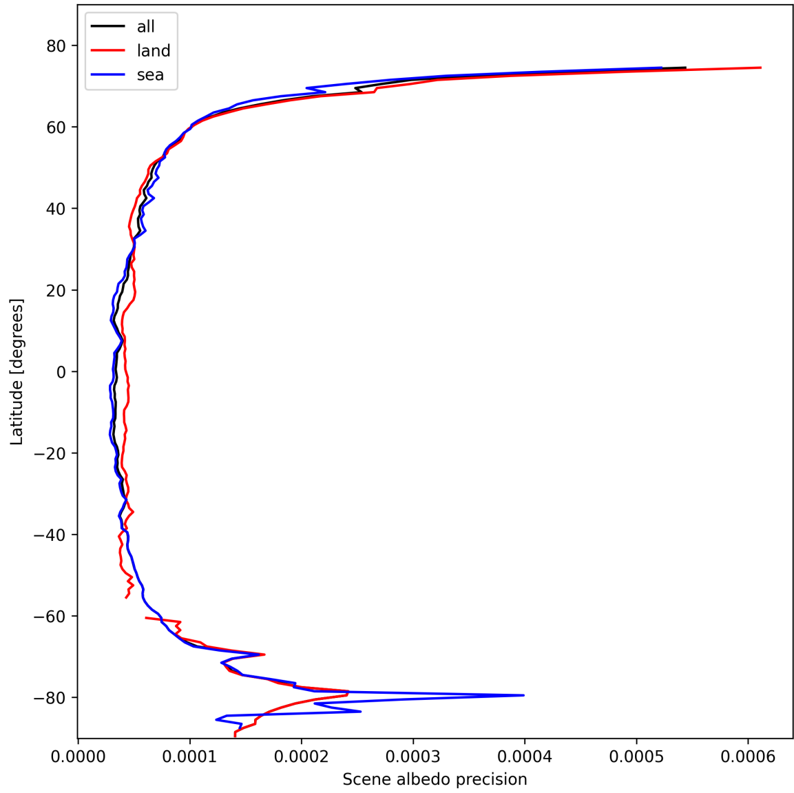
Figure 16: Zonal average of “Scene albedo precision” for 2025-10-28 to 2025-10-29.
