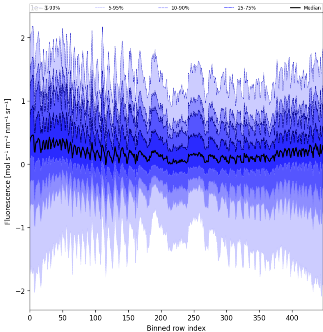
Figure 55: Along track statistics of “Fluorescence” for 2025-10-28 to 2025-10-29
