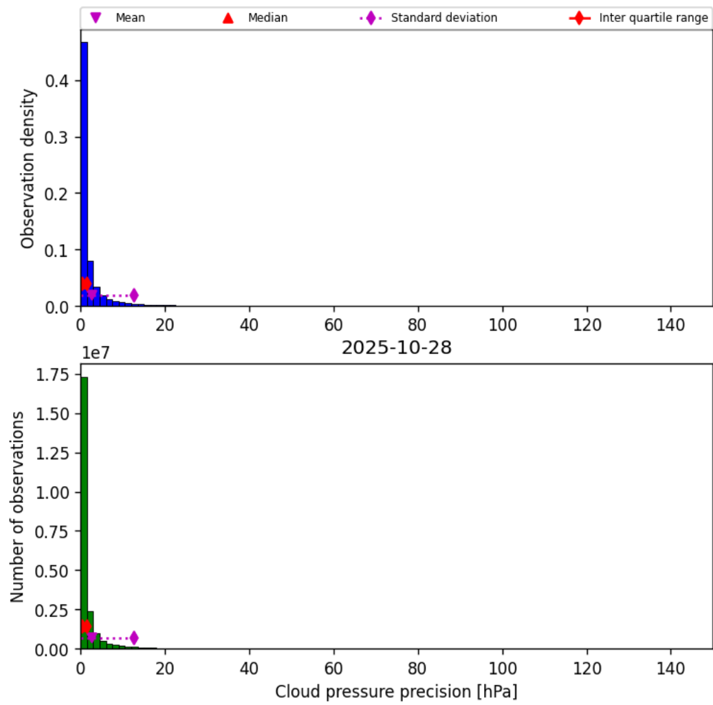
Figure 29: Histogram of “Cloud pressure precision” for 2025-10-28 to 2025-10-29
