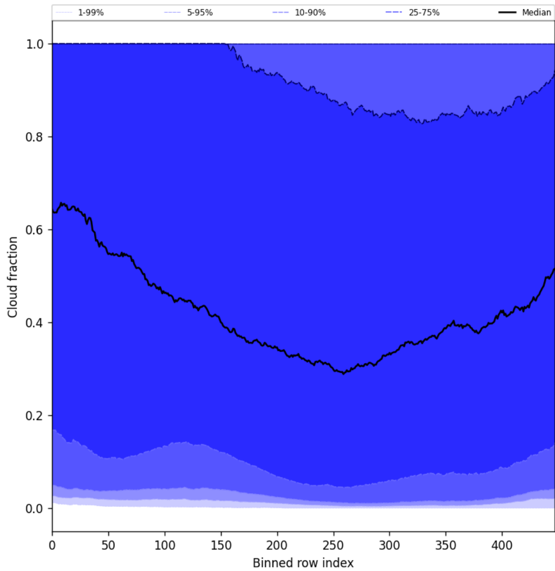
Figure 47: Along track statistics of “Cloud fraction” for 2025-10-28 to 2025-10-29
