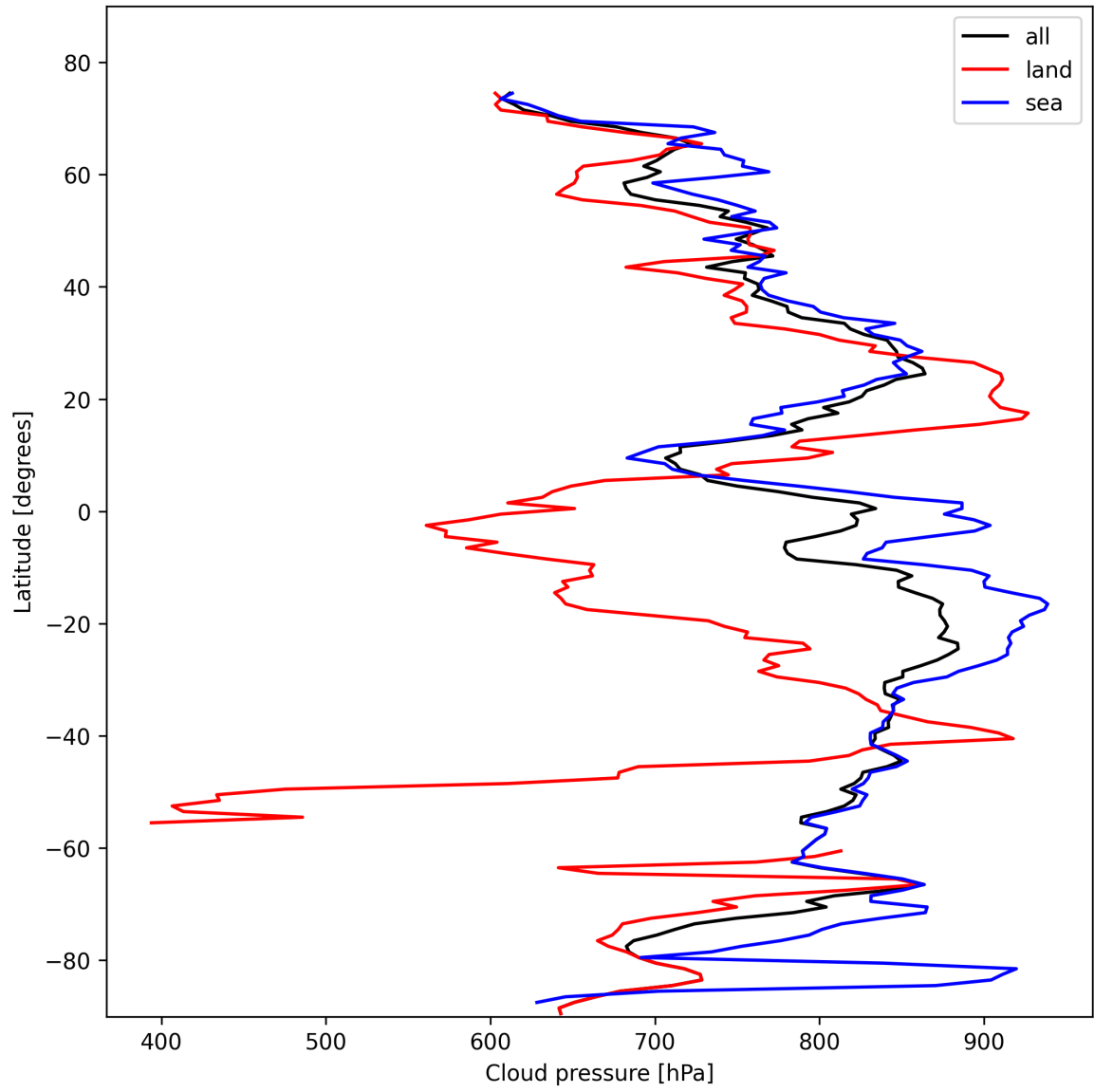
Figure 11: Zonal average of “Cloud pressure” for 2025-10-28 to 2025-10-29.
