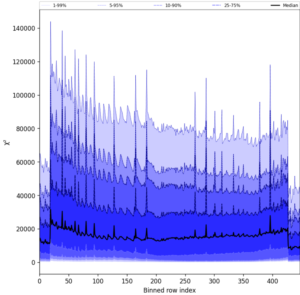
Figure 53: Along track statistics of “ \chi^2 ” for 2025-10-29 to 2025-10-30
