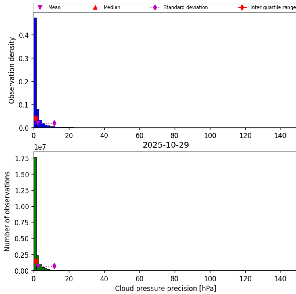
Figure 29: Histogram of “Cloud pressure precision” for 2025-10-29 to 2025-10-30
