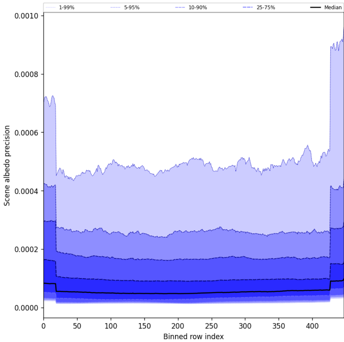
Figure 50: Along track statistics of “Scene albedo precision” for 2025-10-29 to 2025-10-30
