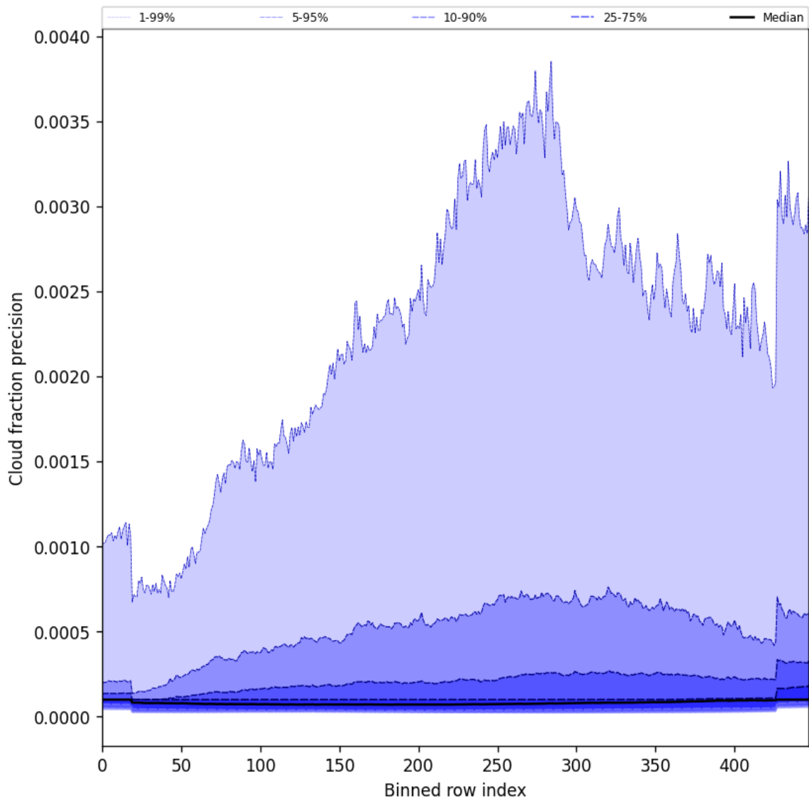
Figure 48: Along track statistics of “Cloud fraction precision” for 2025-10-29 to 2025-10-30
