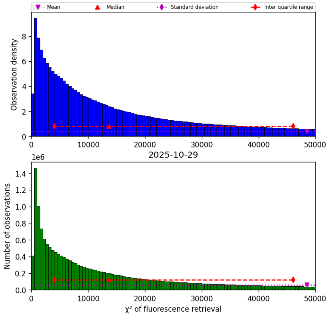
Figure 40: Histogram of “ \chi^2 of fluorescence retrieval” for 2025-10-29 to 2025-10-30
