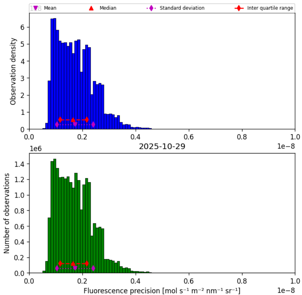
Figure 39: Histogram of “Fluorescence precision” for 2025-10-29 to 2025-10-30
