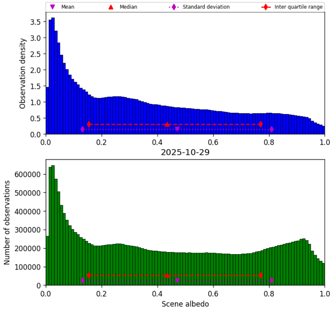
Figure 32: Histogram of “Scene albedo” for 2025-10-29 to 2025-10-30
