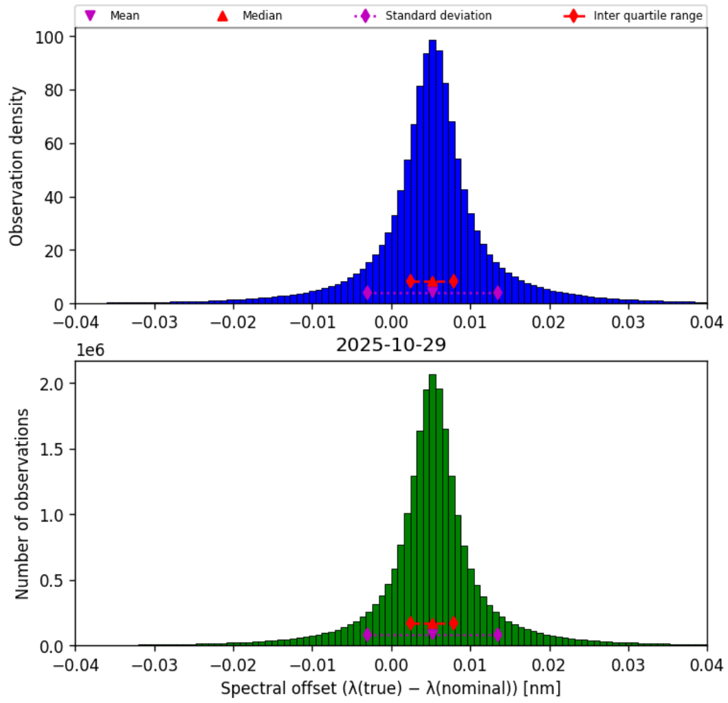
Figure 43: Histogram of “Spectral offset ( \lambda_{\text{true}} - \lambda_{\text{nominal}} )” for 2025-10-29 to 2025-10-30
