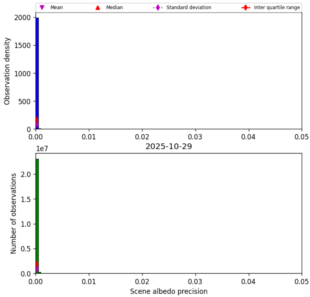
Figure 33: Histogram of “Scene albedo precision” for 2025-10-29 to 2025-10-30
