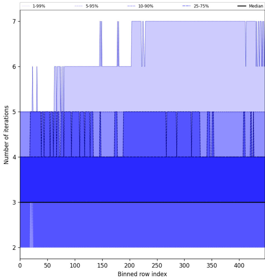
Figure 54: Along track statistics of “Number of iterations” for 2025-10-29 to 2025-10-30
