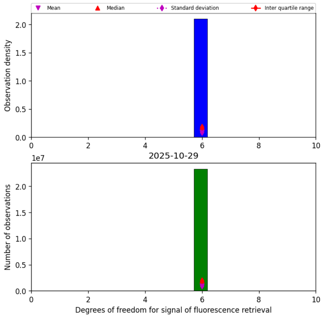
Figure 41: Histogram of “Degrees of freedom for signal of fluorescence retrieval” for 2025-10-29 to 2025-10-30
