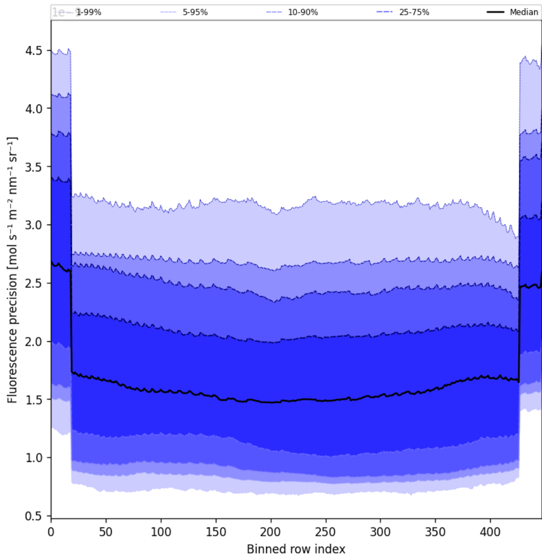
Figure 56: Along track statistics of “Fluorescence precision” for 2025-10-29 to 2025-10-30
