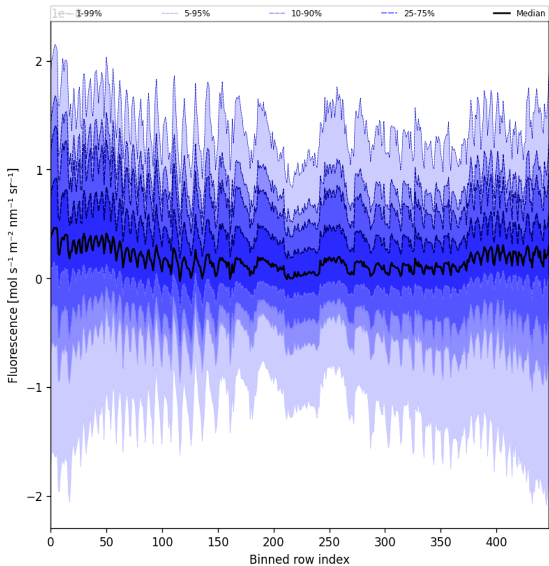
Figure 55: Along track statistics of “Fluorescence” for 2025-10-29 to 2025-10-30
