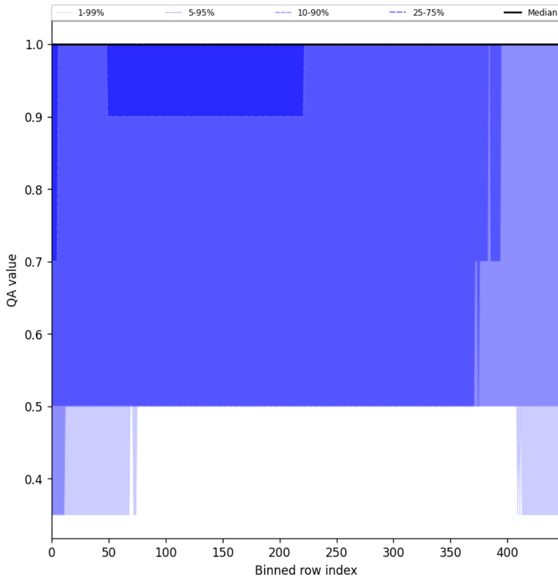
Figure 44: Along track statistics of “QA value” for 2025-10-29 to 2025-10-30
