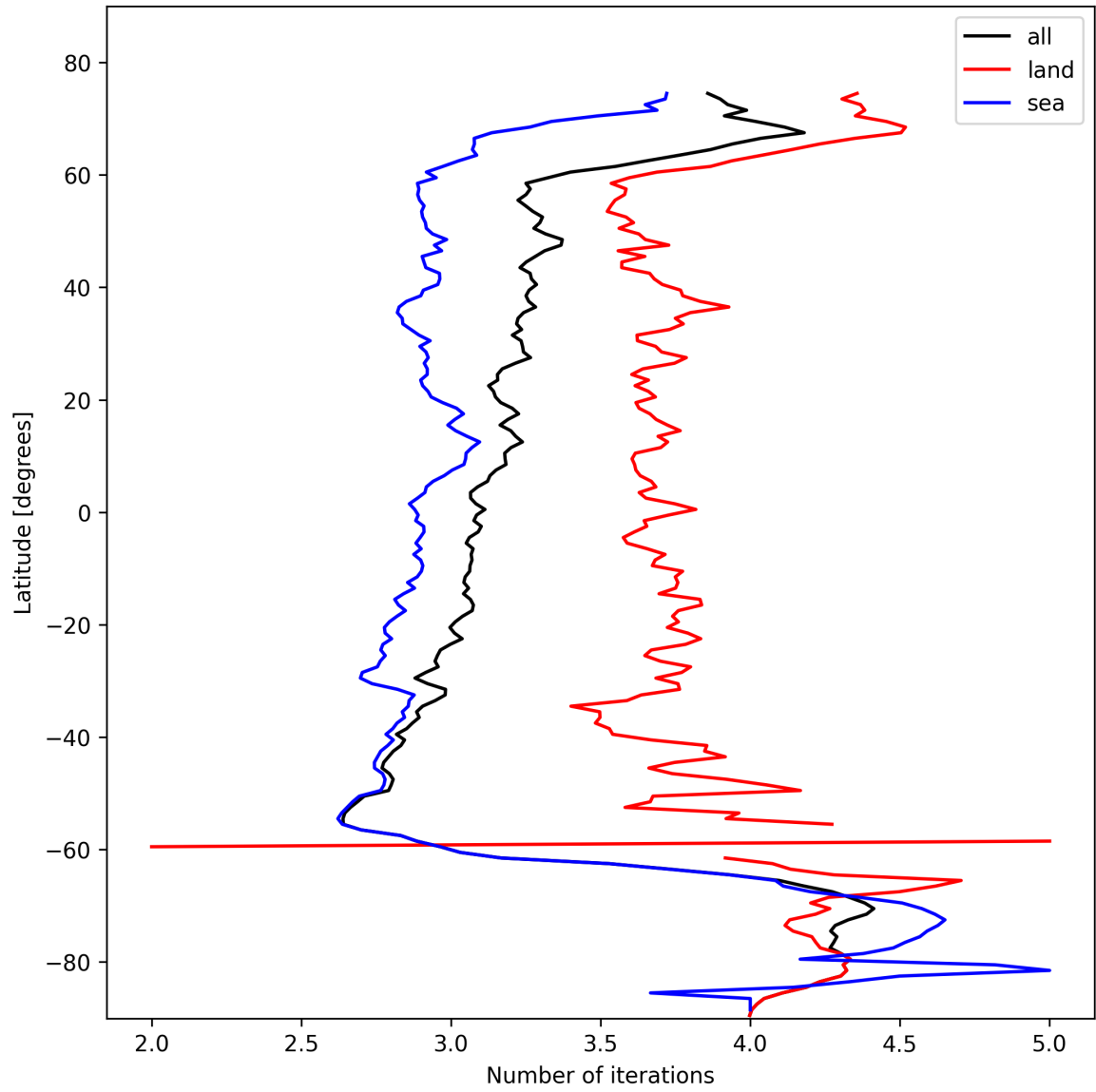
Figure 20: Zonal average of “Number of iterations” for 2025-10-29 to 2025-10-30.
