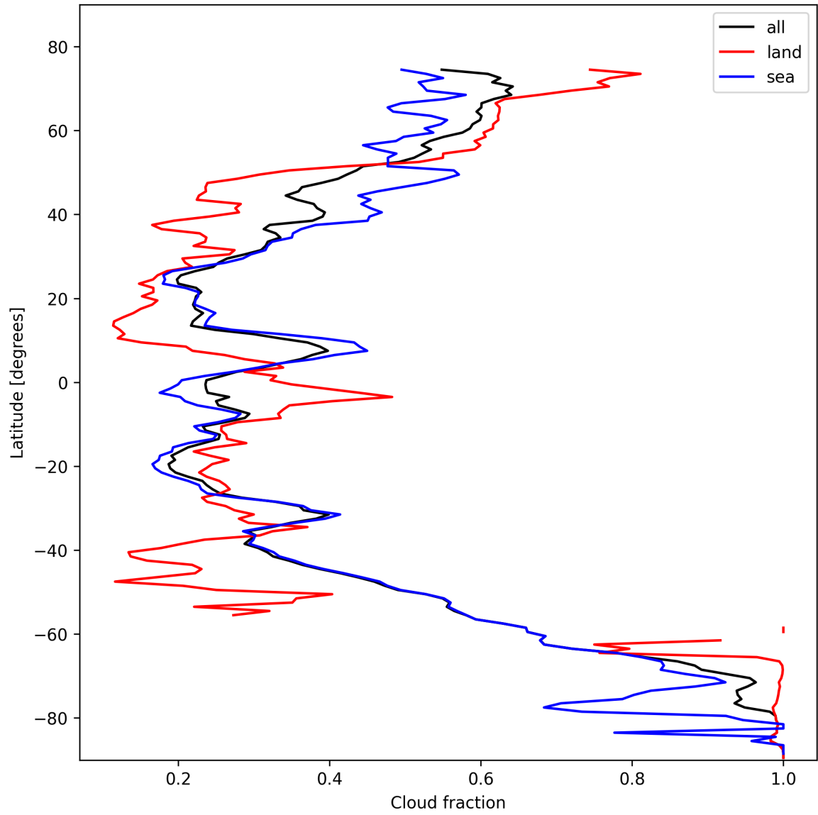
Figure 13: Zonal average of “Cloud fraction” for 2025-10-29 to 2025-10-30.
