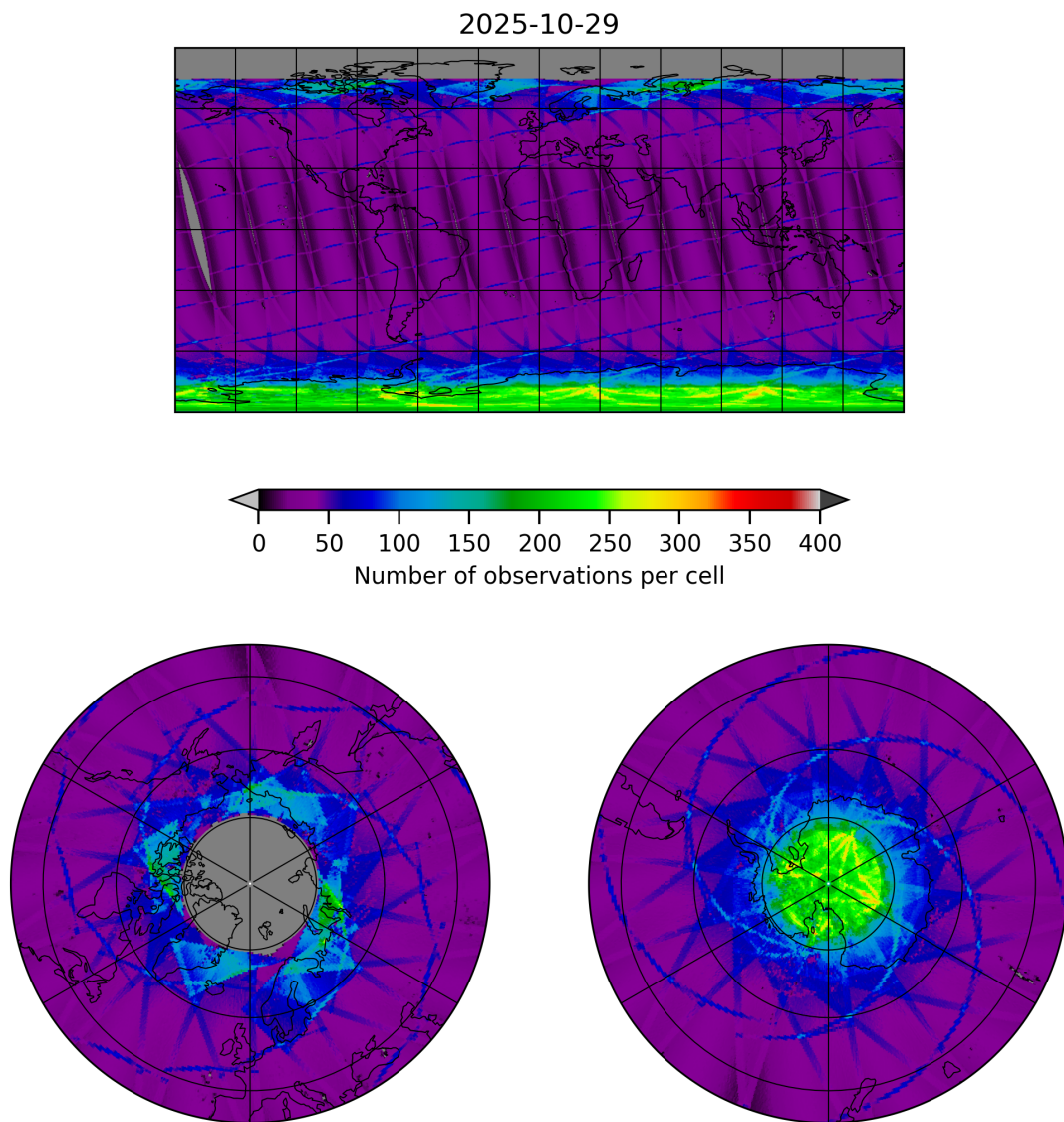
Figure 9: Map of the number of observations for 2025-10-29 to 2025-10-30
