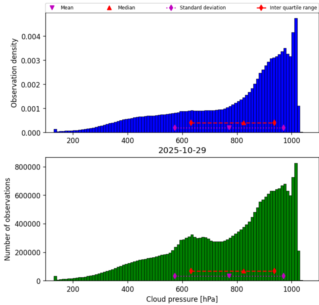
Figure 28: Histogram of “Cloud pressure” for 2025-10-29 to 2025-10-30
