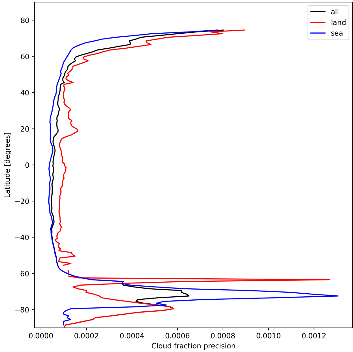
Figure 14: Zonal average of “Cloud fraction precision” for 2025-10-29 to 2025-10-30.
