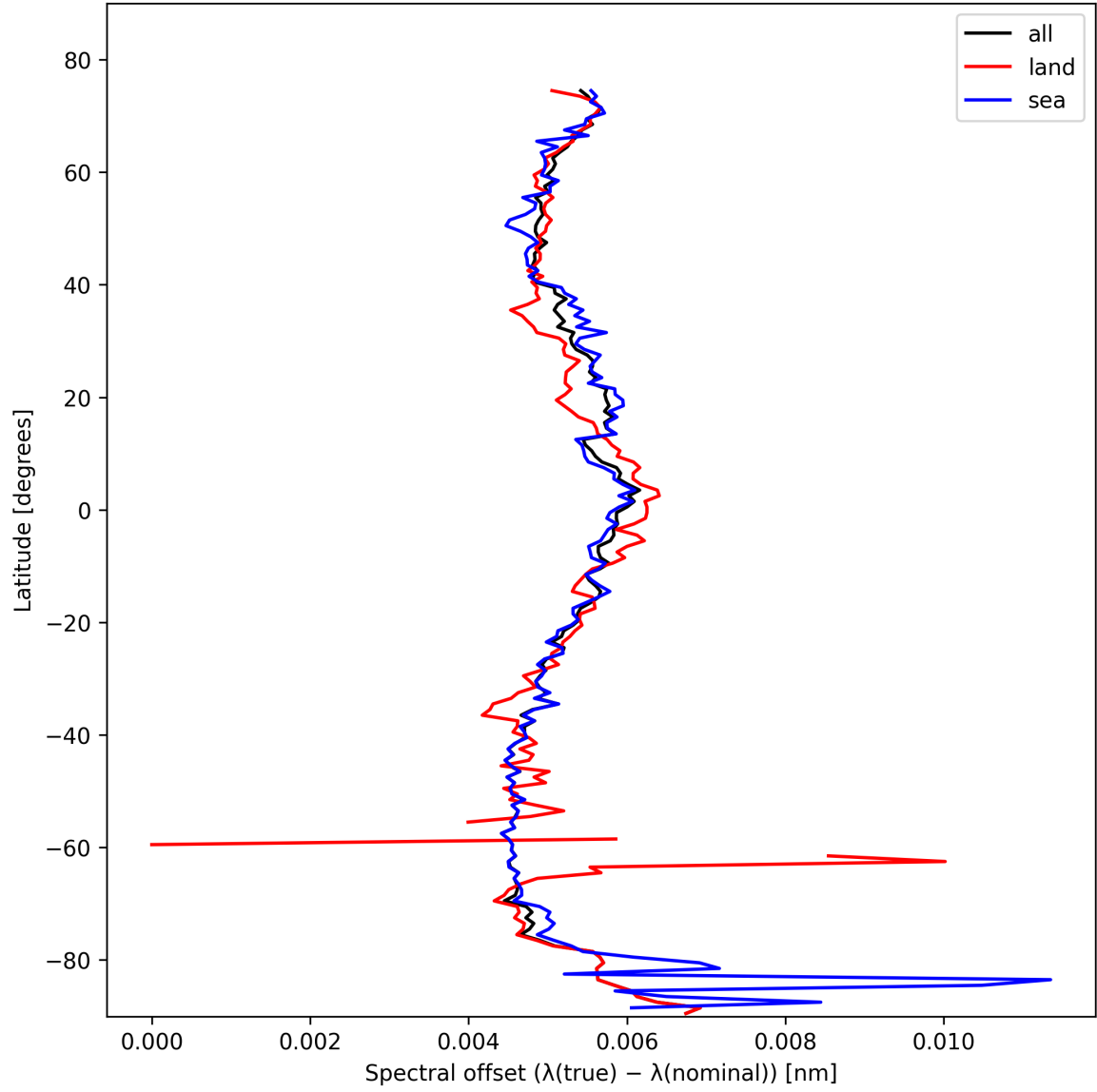
Figure 26: Zonal average of “Spectral offset ( \lambda_{\text{true}} - \lambda_{\text{nominal}} )” for 2025-10-29 to 2025-10-30.
