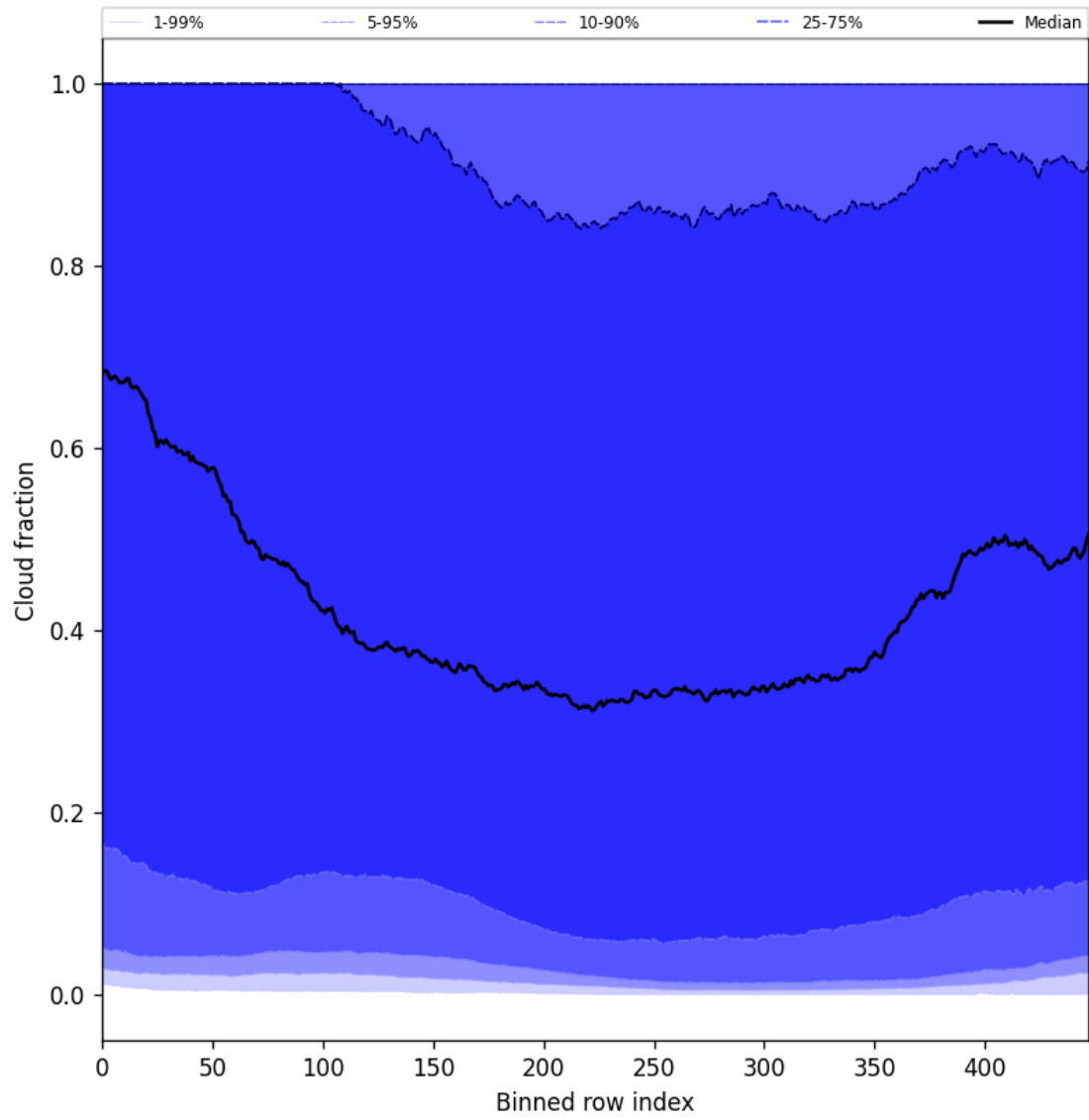
Figure 47: Along track statistics of “Cloud fraction” for 2025-10-29 to 2025-10-30
