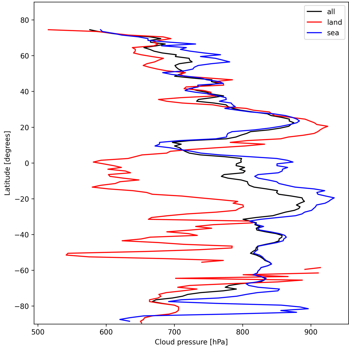
Figure 11: Zonal average of “Cloud pressure” for 2025-10-29 to 2025-10-30.
