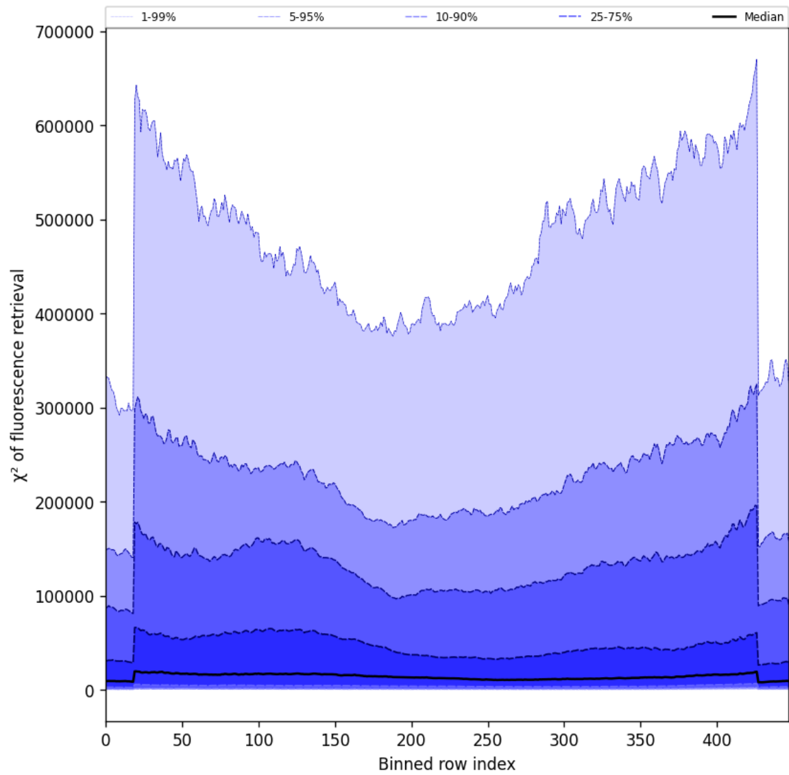
Figure 57: Along track statistics of “ \chi^2 of fluorescence retrieval” for 2025-10-29 to 2025-10-30
