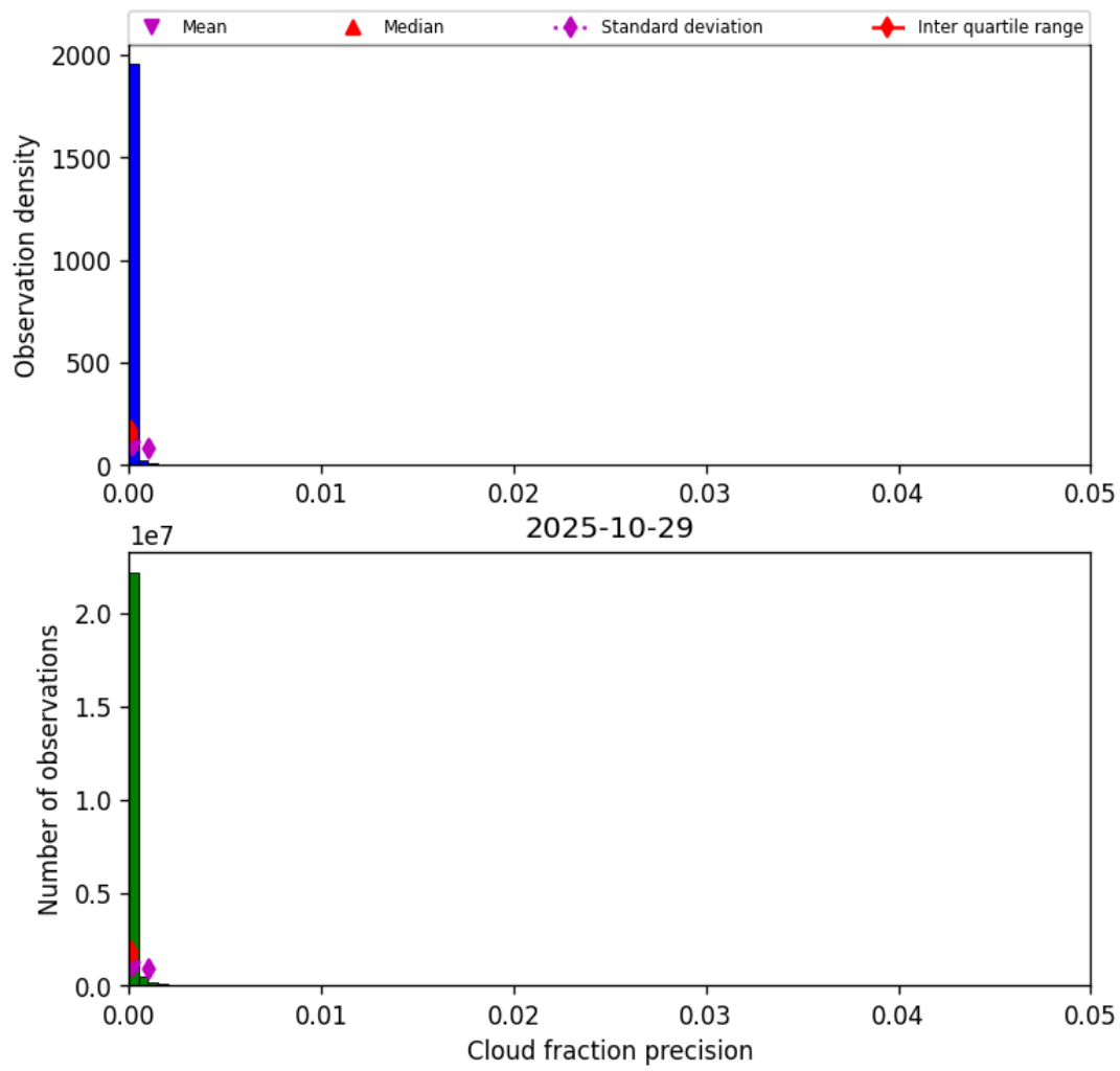
Figure 31: Histogram of “Cloud fraction precision” for 2025-10-29 to 2025-10-30
