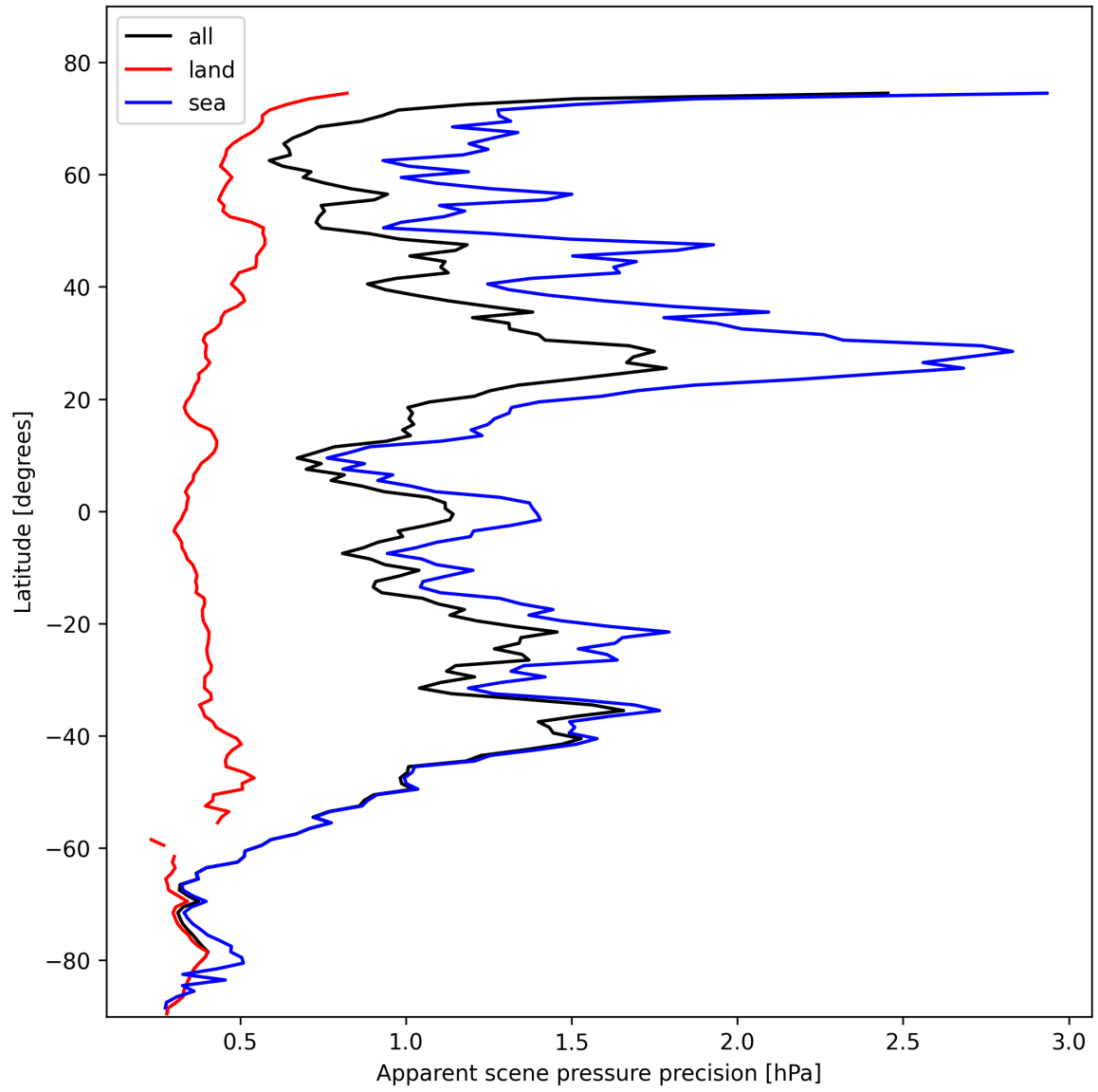
Figure 18: Zonal average of “Apparent scene pressure precision” for 2025-10-29 to 2025-10-30.
