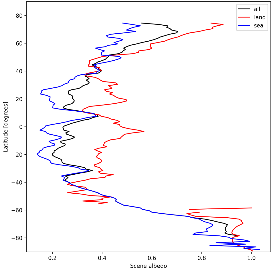
Figure 15: Zonal average of “Scene albedo” for 2025-10-29 to 2025-10-30.
