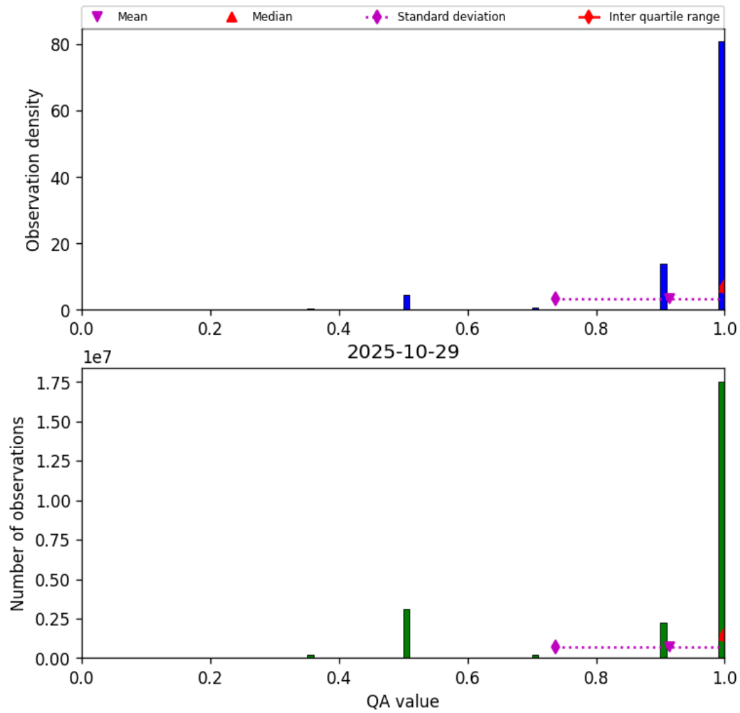
Figure 27: Histogram of “QA value” for 2025-10-29 to 2025-10-30
