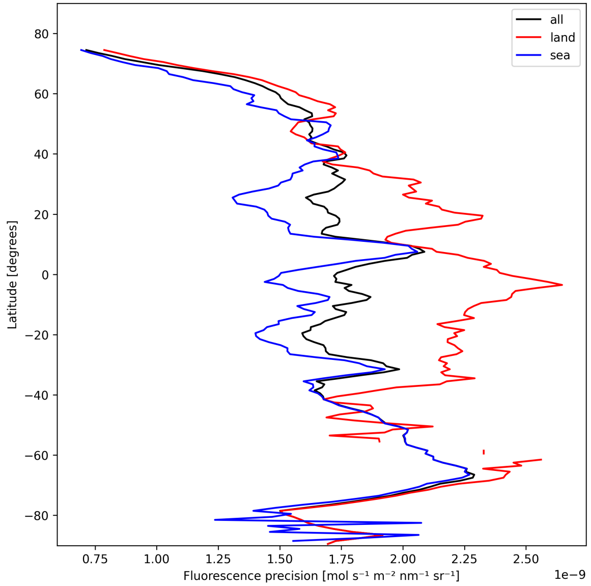
Figure 22: Zonal average of “Fluorescence precision” for 2025-10-29 to 2025-10-30.
