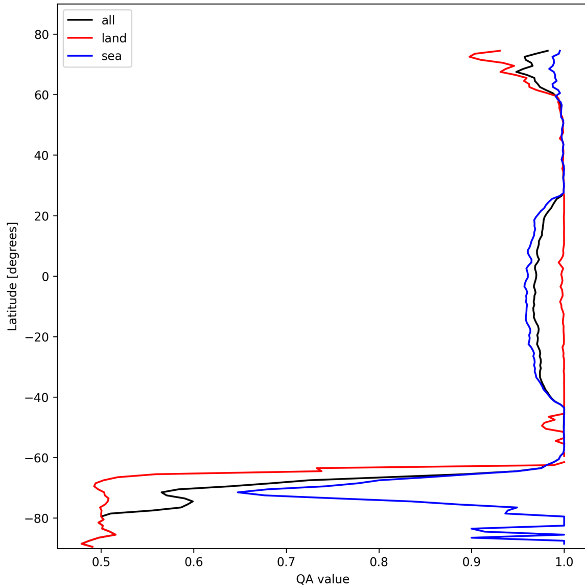
Figure 10: Zonal average of “QA value” for 2025-10-29 to 2025-10-30.
