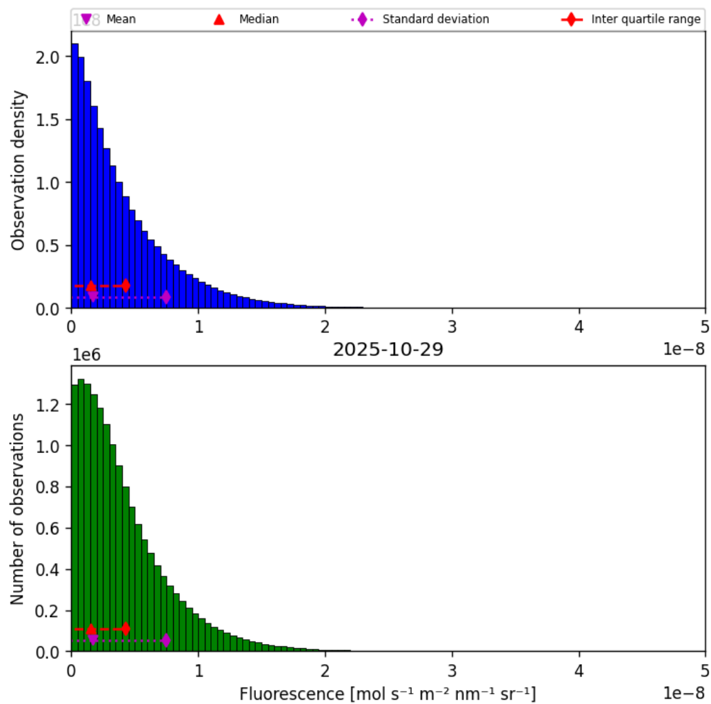
Figure 38: Histogram of “Fluorescence” for 2025-10-29 to 2025-10-30
