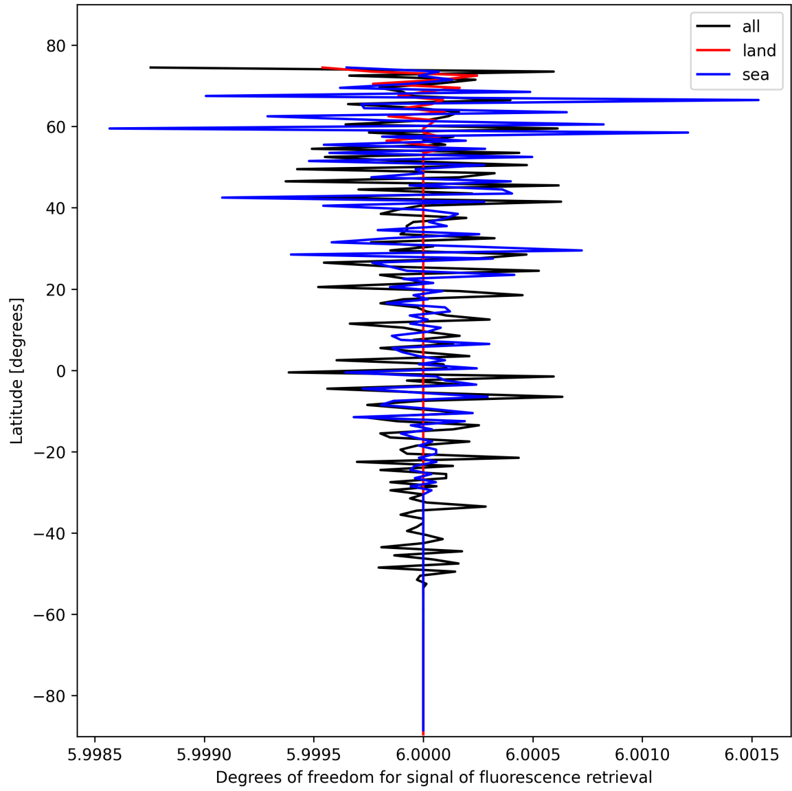
Figure 24: Zonal average of “Degrees of freedom for signal of fluorescence retrieval” for 2025-10-29 to 2025-10-30.
