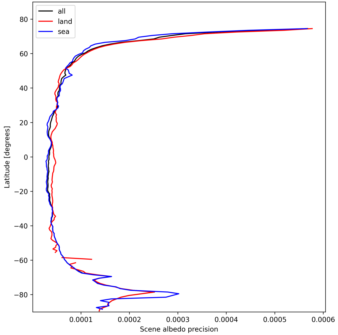
Figure 16: Zonal average of “Scene albedo precision” for 2025-10-29 to 2025-10-30.
