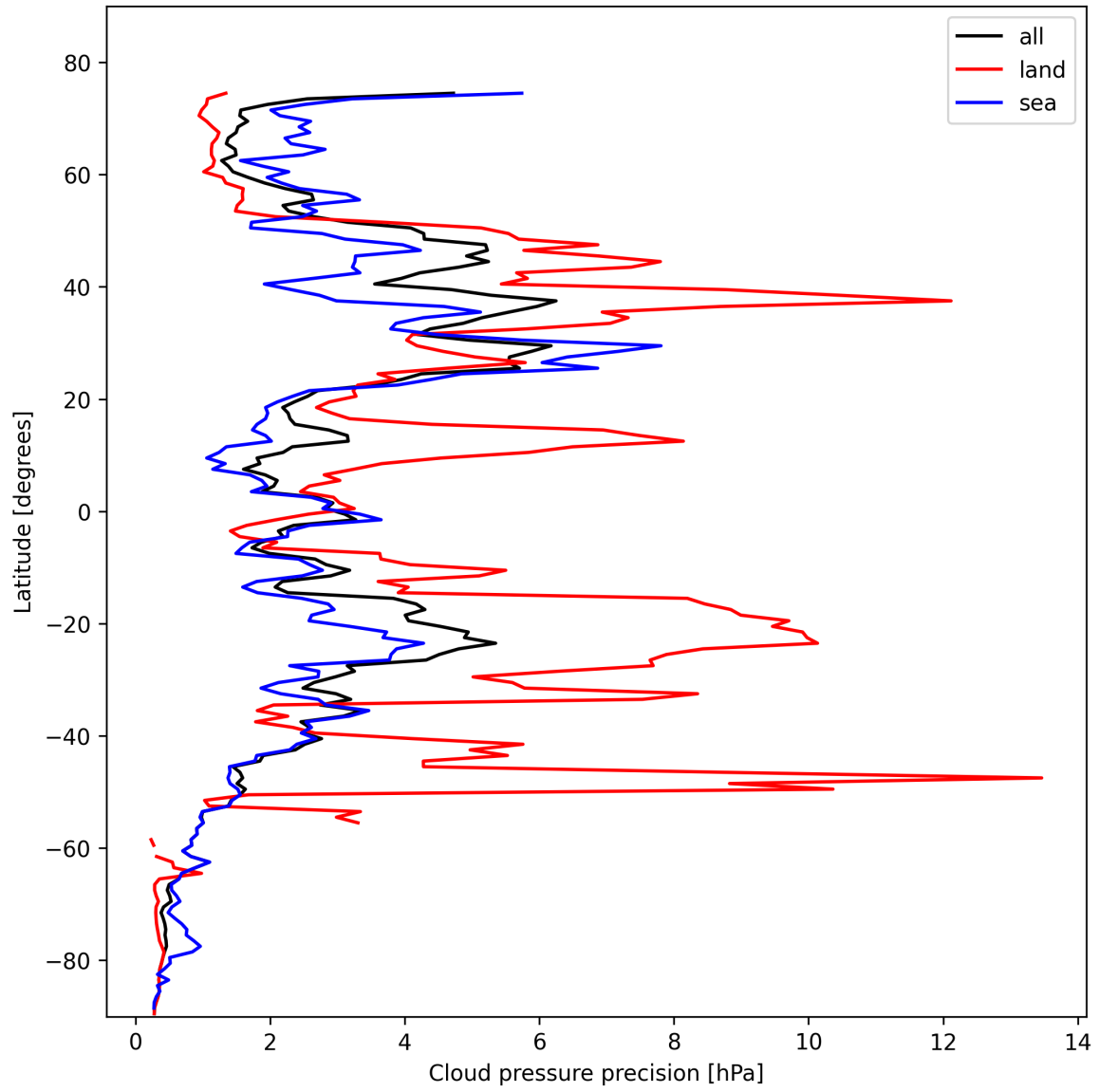
Figure 12: Zonal average of “Cloud pressure precision” for 2025-10-29 to 2025-10-30.
