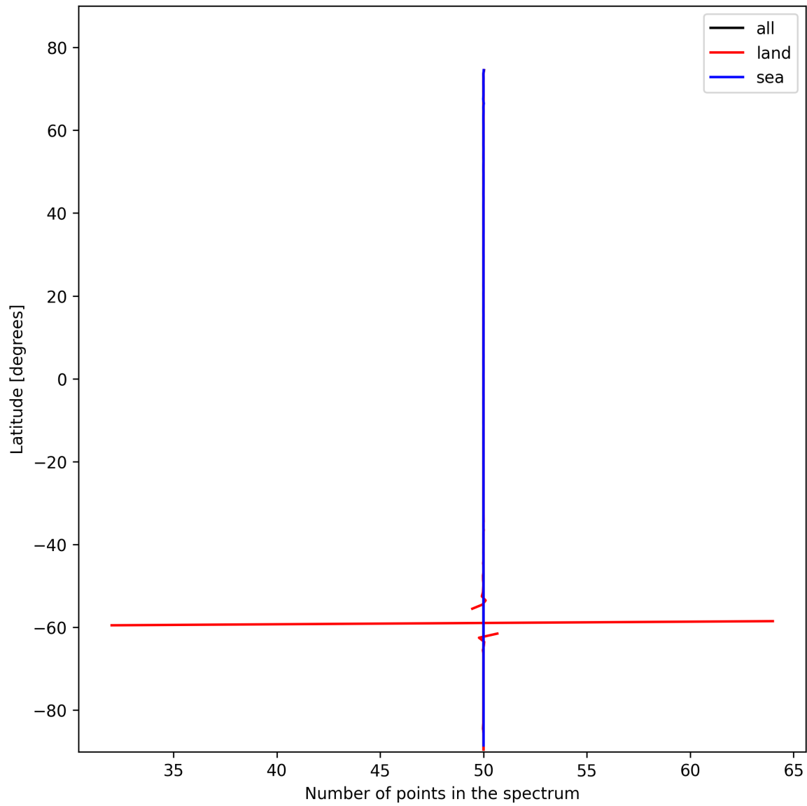
Figure 25: Zonal average of “Number of points in the spectrum” for 2025-10-29 to 2025-10-30.
