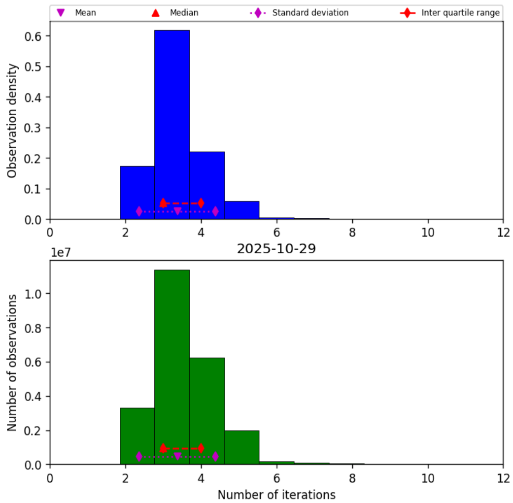
Figure 37: Histogram of “Number of iterations” for 2025-10-29 to 2025-10-30
