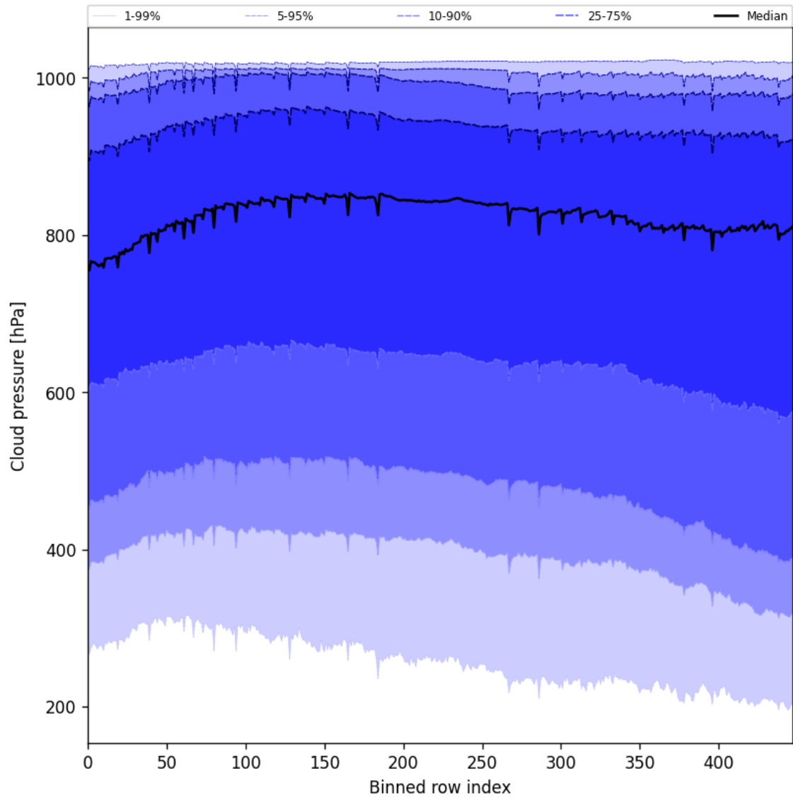
Figure 45: Along track statistics of “Cloud pressure” for 2025-10-29 to 2025-10-30
