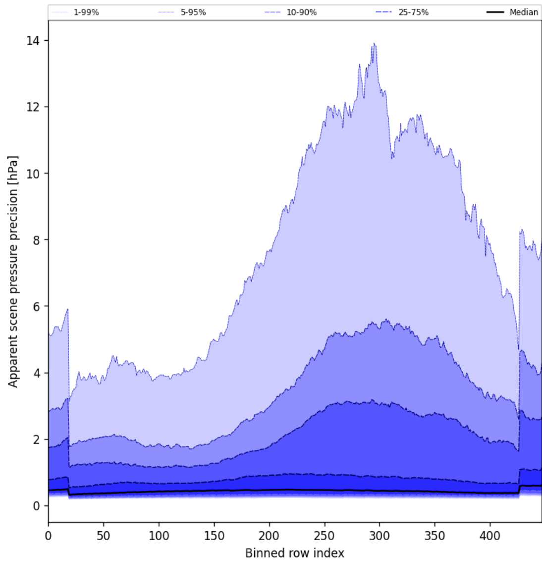
Figure 52: Along track statistics of “Apparent scene pressure precision” for 2025-10-29 to 2025-10-30
