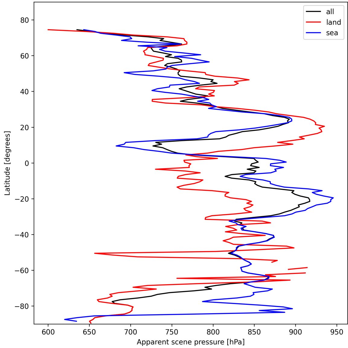
Figure 17: Zonal average of “Apparent scene pressure” for 2025-10-29 to 2025-10-30.
