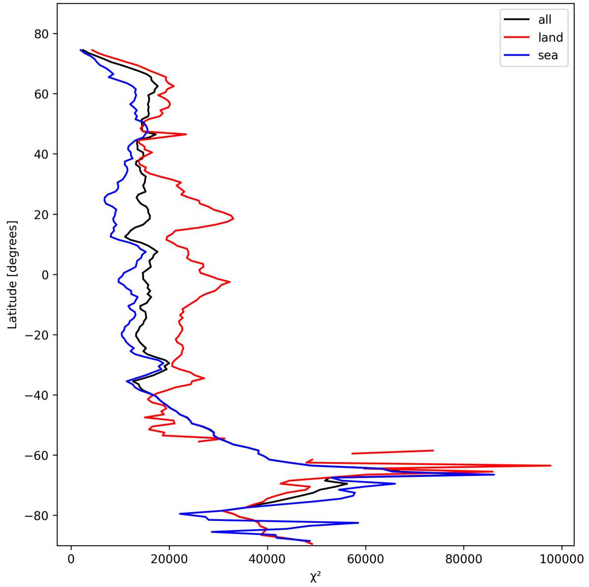
Figure 19: Zonal average of “ \chi^2 ” for 2025-10-29 to 2025-10-30.
