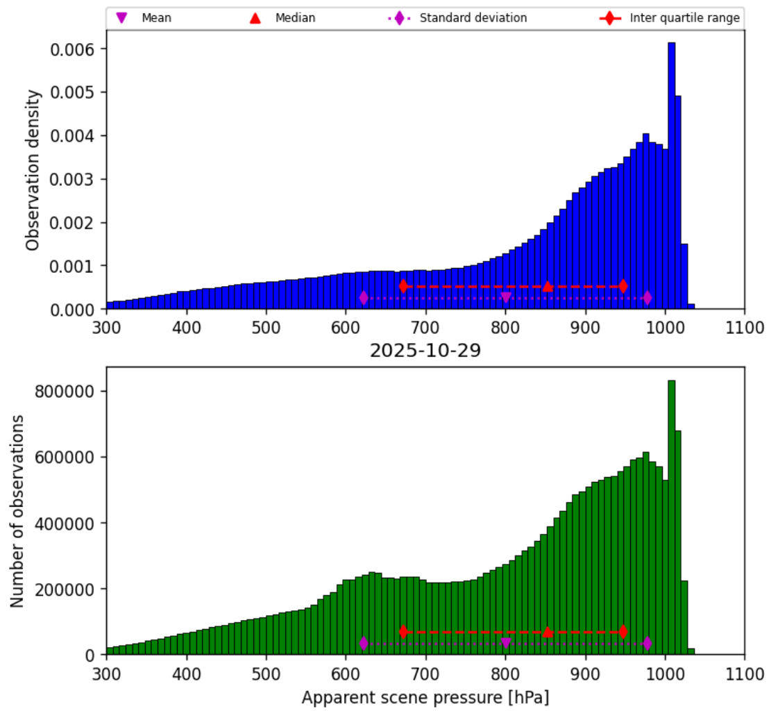
Figure 34: Histogram of “Apparent scene pressure” for 2025-10-29 to 2025-10-30
