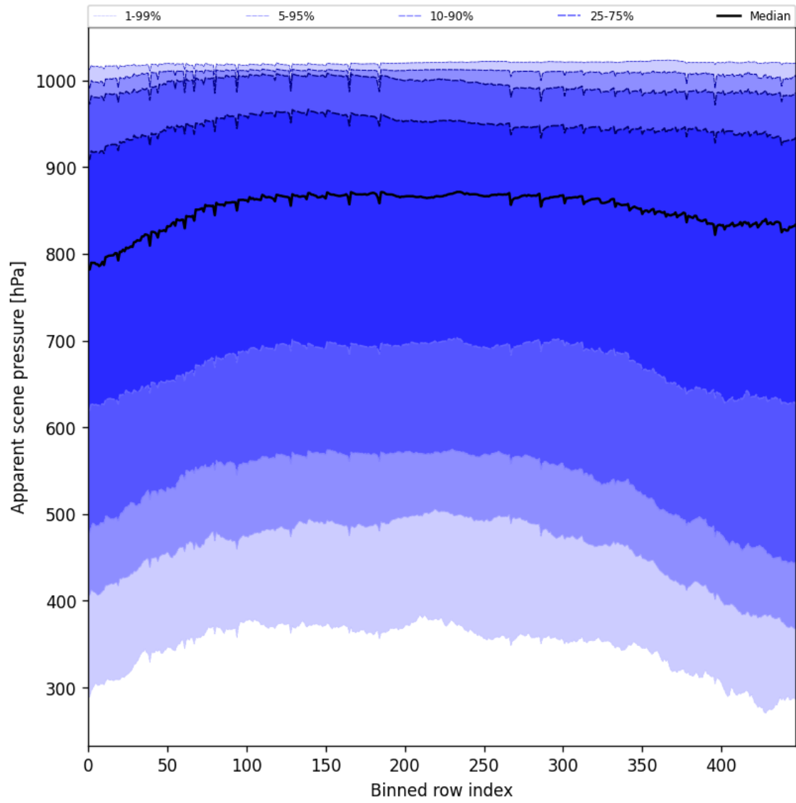
Figure 51: Along track statistics of “Apparent scene pressure” for 2025-10-29 to 2025-10-30
