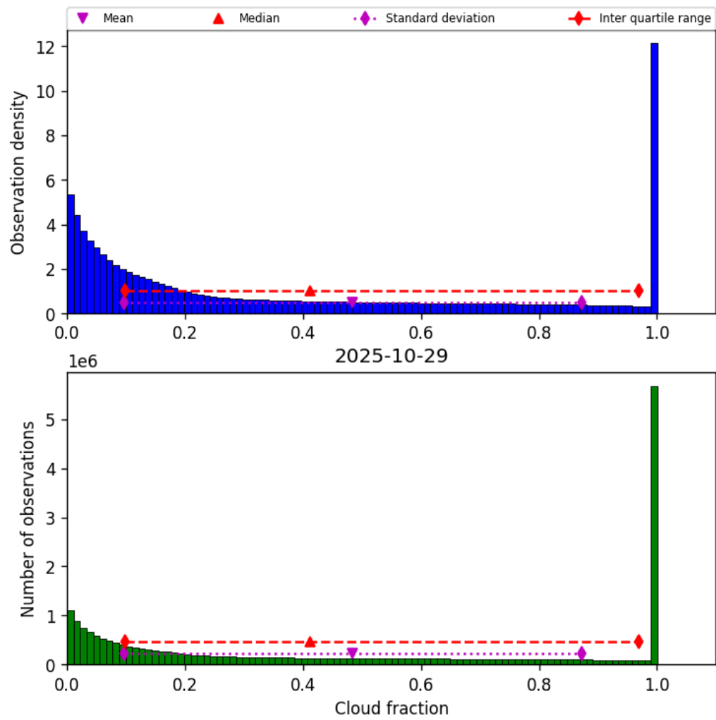
Figure 30: Histogram of “Cloud fraction” for 2025-10-29 to 2025-10-30
