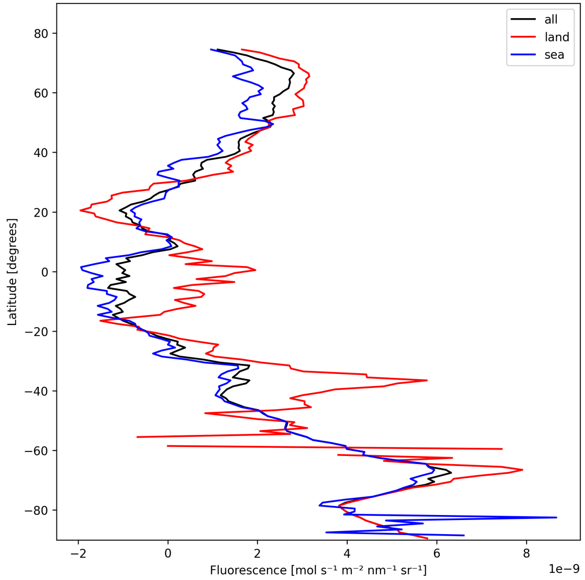
Figure 21: Zonal average of “Fluorescence” for 2025-10-29 to 2025-10-30.
