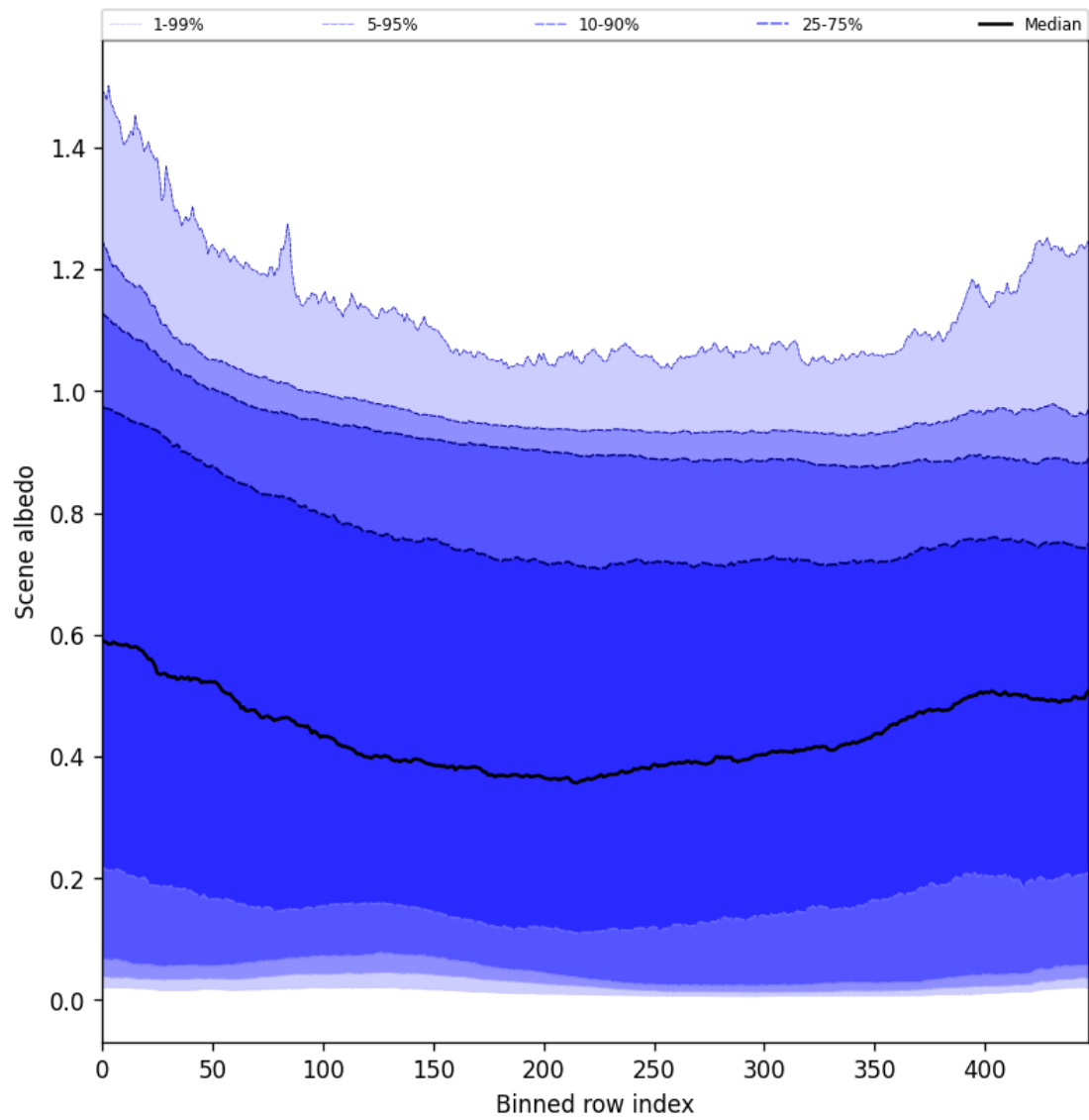
Figure 49: Along track statistics of “Scene albedo” for 2025-10-29 to 2025-10-30
