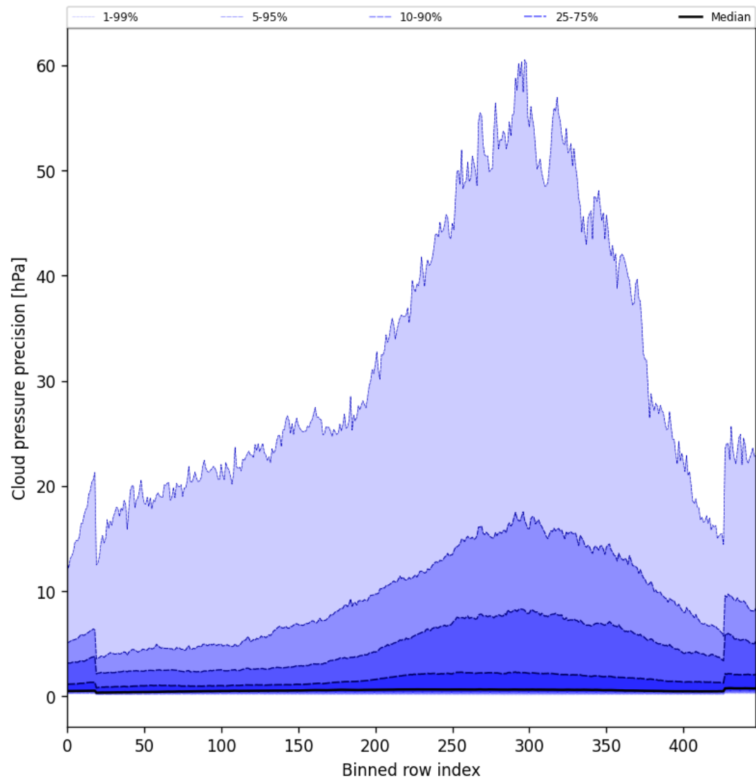
Figure 46: Along track statistics of “Cloud pressure precision” for 2025-10-29 to 2025-10-30
