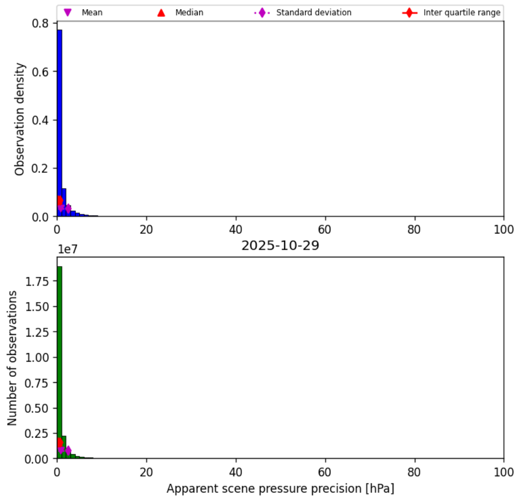
Figure 35: Histogram of “Apparent scene pressure precision” for 2025-10-29 to 2025-10-30
