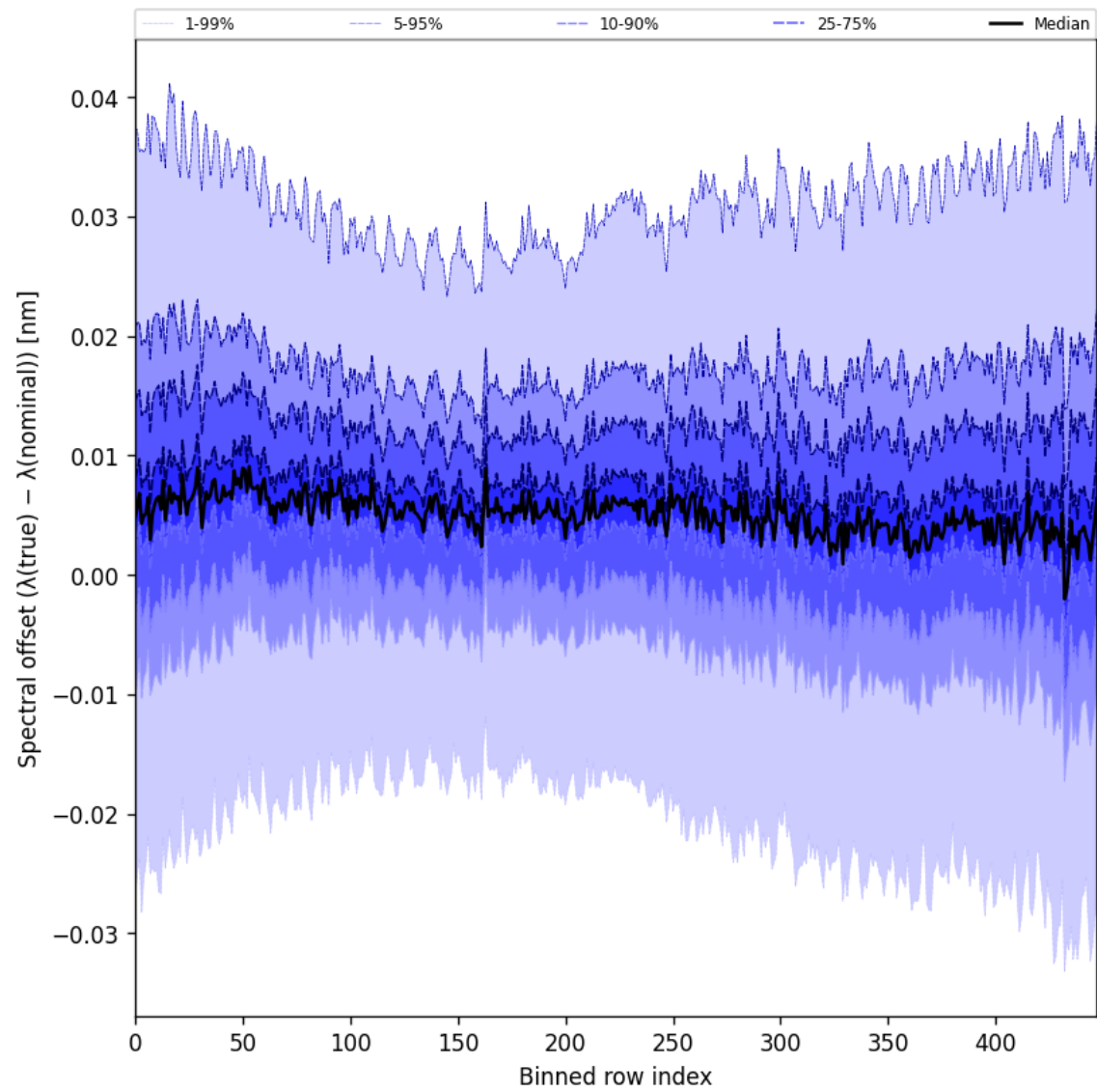
Figure 60: Along track statistics of “Spectral offset ( \lambda_{\text{true}} - \lambda_{\text{nominal}} )” for 2025-10-29 to 2025-10-30
