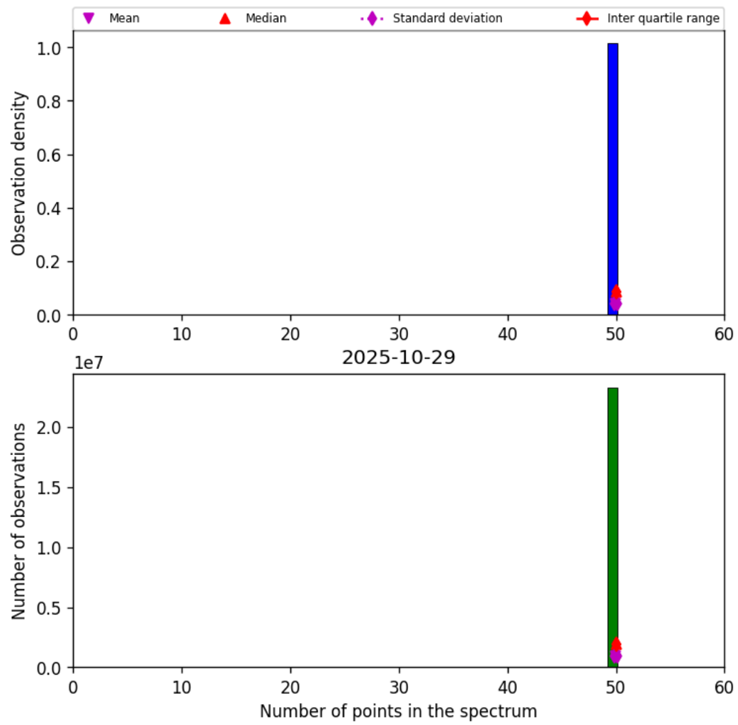
Figure 42: Histogram of “Number of points in the spectrum” for 2025-10-29 to 2025-10-30
