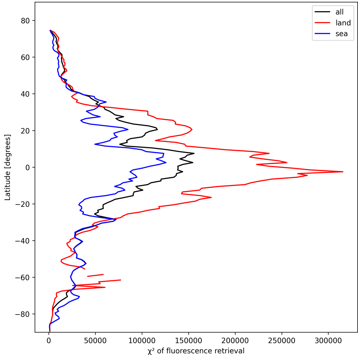
Figure 23: Zonal average of “ \chi^2 of fluorescence retrieval” for 2025-10-29 to 2025-10-30.
