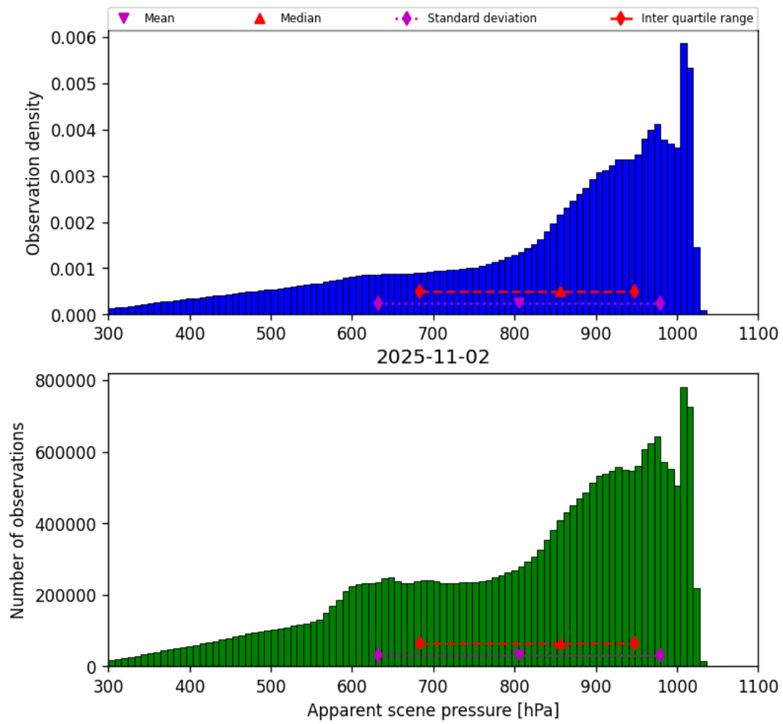
Figure 34: Histogram of “Apparent scene pressure” for 2025-11-02 to 2025-11-03
