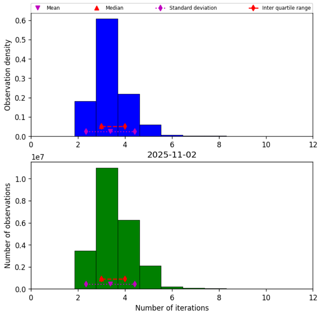
Figure 37: Histogram of “Number of iterations” for 2025-11-02 to 2025-11-03
