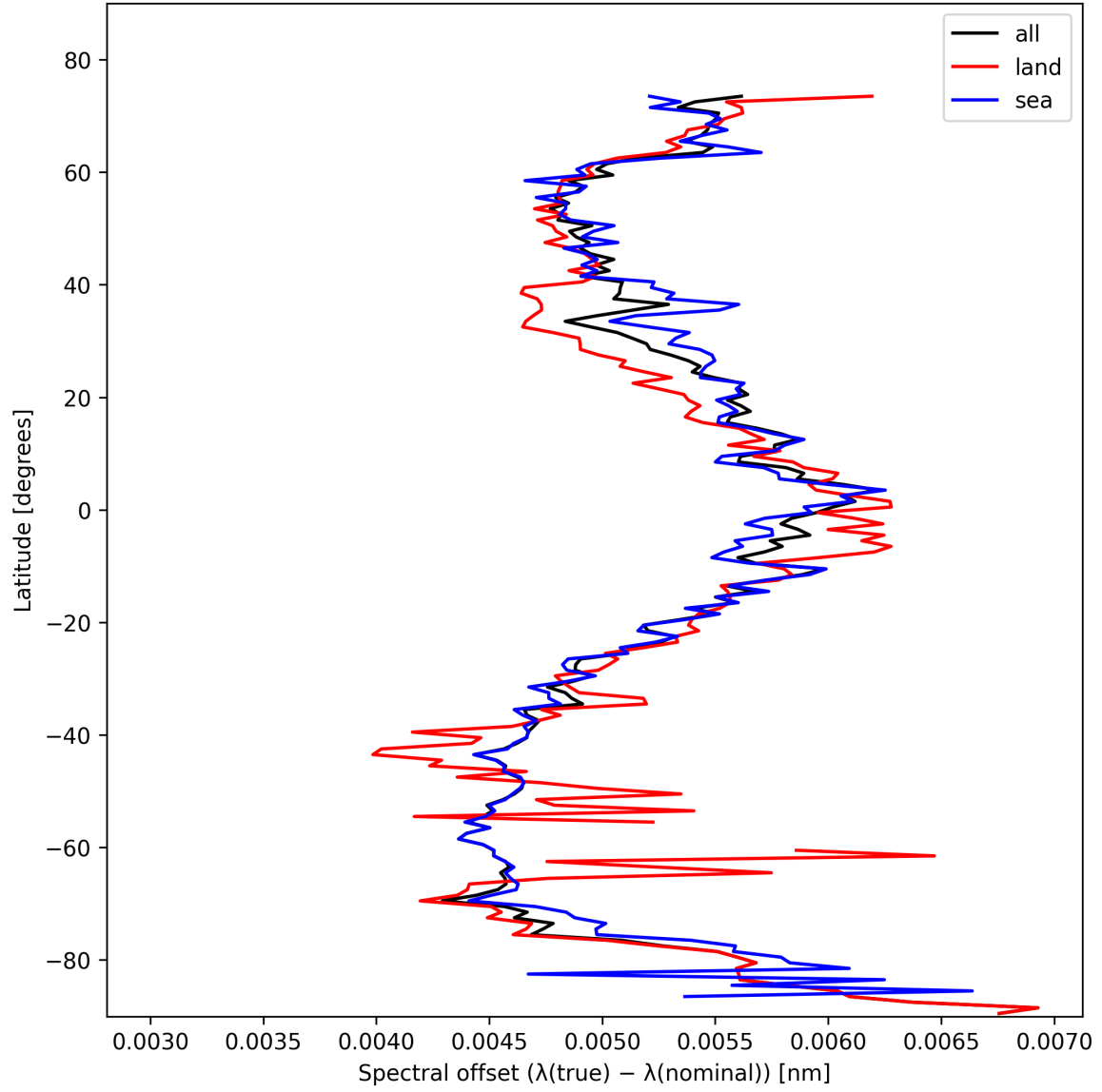
Figure 26: Zonal average of “Spectral offset ( \lambda_{\text{true}} - \lambda_{\text{nominal}} )” for 2025-11-02 to 2025-11-03.
