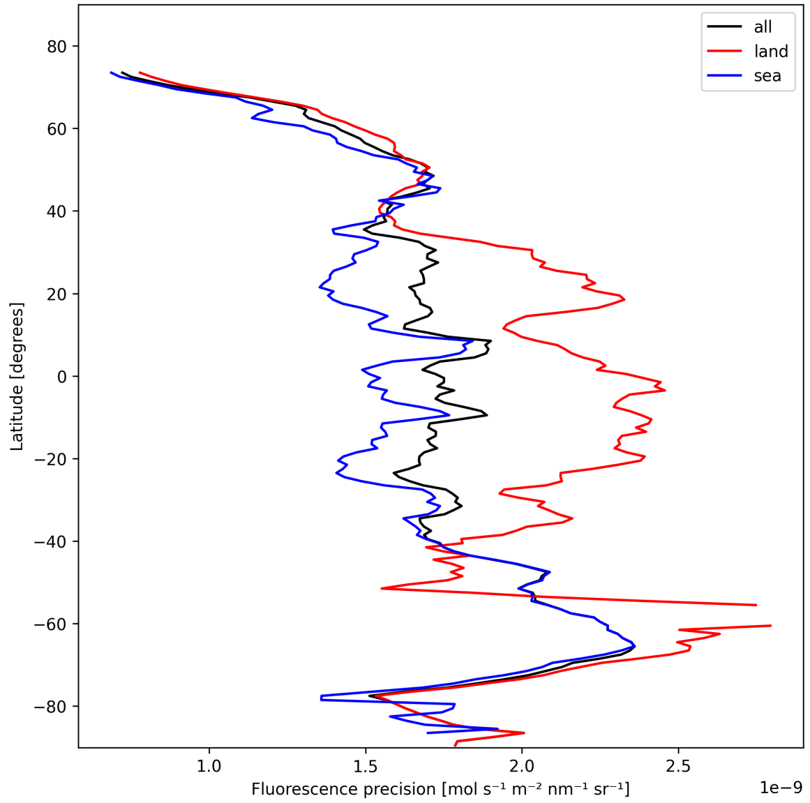
Figure 22: Zonal average of “Fluorescence precision” for 2025-11-02 to 2025-11-03.
