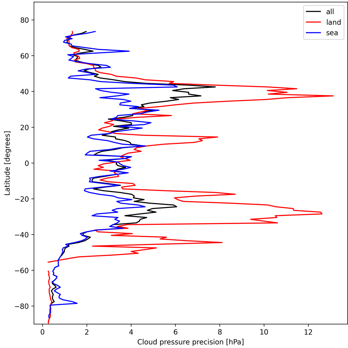
Figure 12: Zonal average of “Cloud pressure precision” for 2025-11-02 to 2025-11-03.
