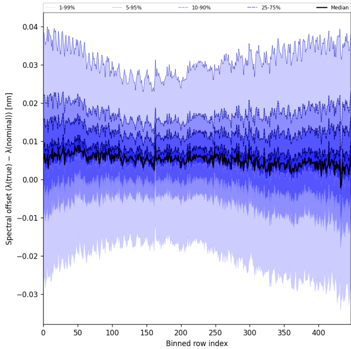
Figure 60: Along track statistics of “Spectral offset ( \lambda_{\text{true}} - \lambda_{\text{nominal}} )” for 2025-11-02 to 2025-11-03
