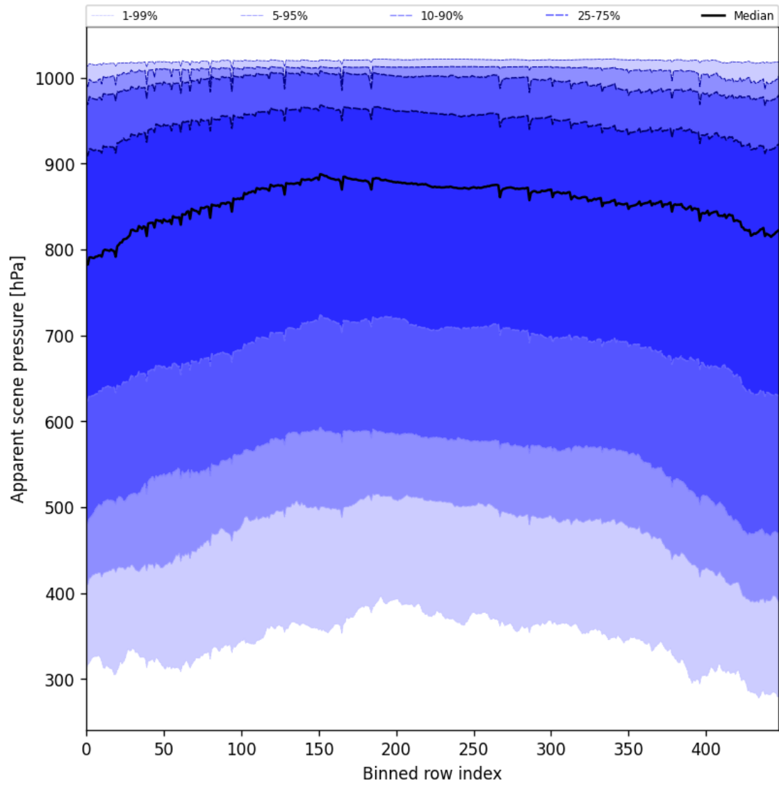
Figure 51: Along track statistics of “Apparent scene pressure” for 2025-11-02 to 2025-11-03
