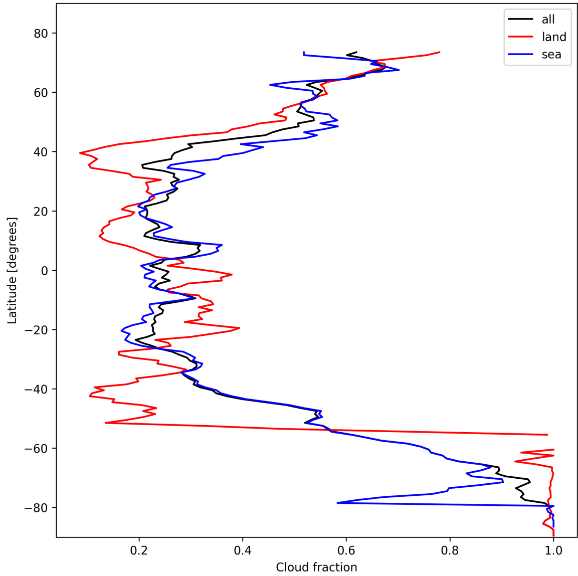
Figure 13: Zonal average of “Cloud fraction” for 2025-11-02 to 2025-11-03.
