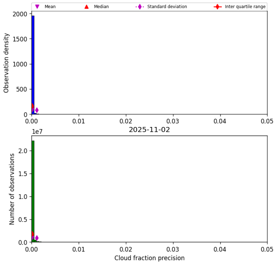
Figure 31: Histogram of “Cloud fraction precision” for 2025-11-02 to 2025-11-03
