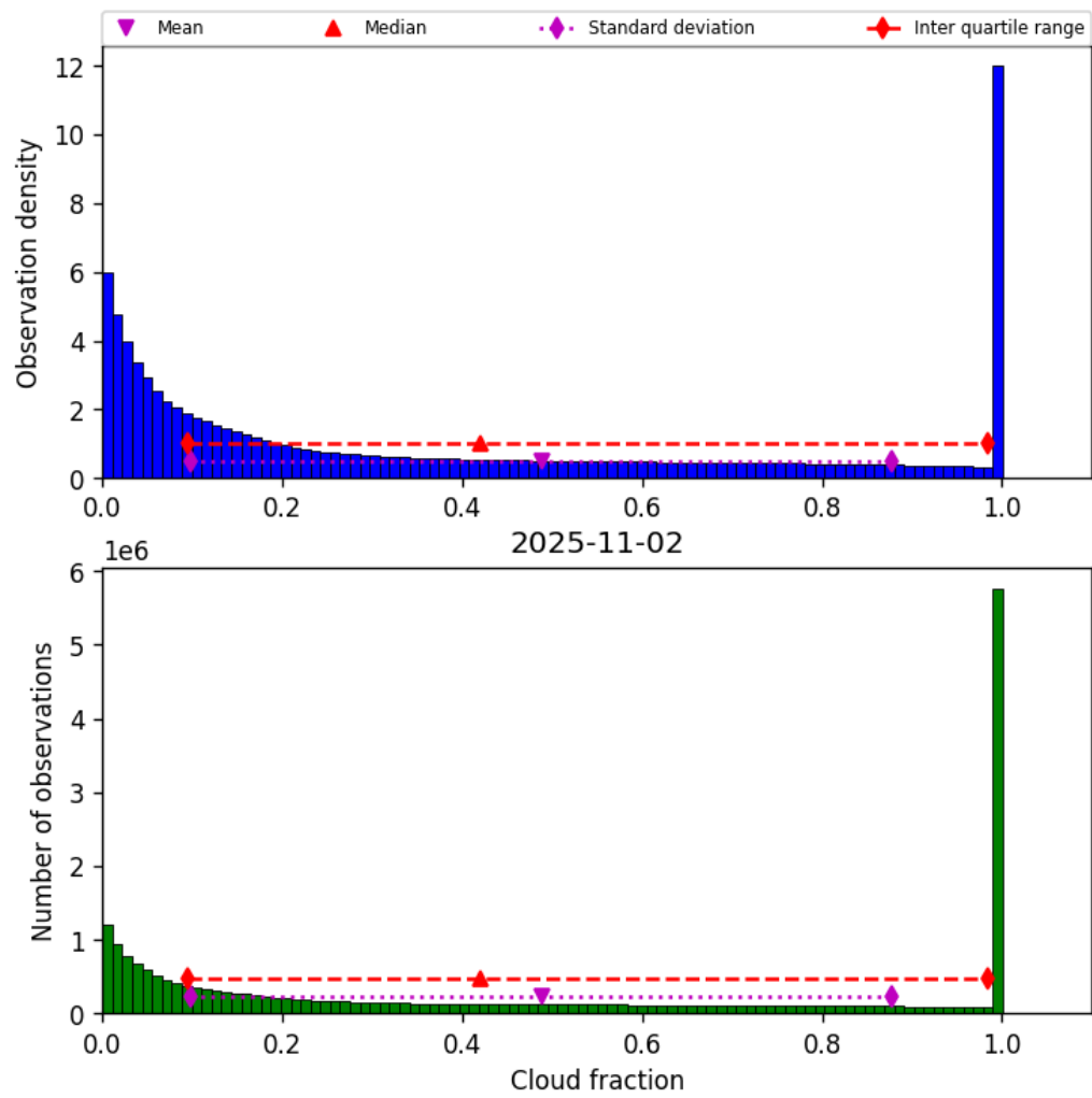
Figure 30: Histogram of “Cloud fraction” for 2025-11-02 to 2025-11-03
