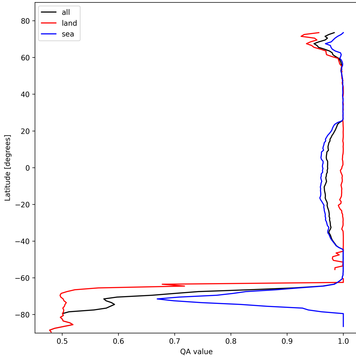
Figure 10: Zonal average of “QA value” for 2025-11-02 to 2025-11-03.
