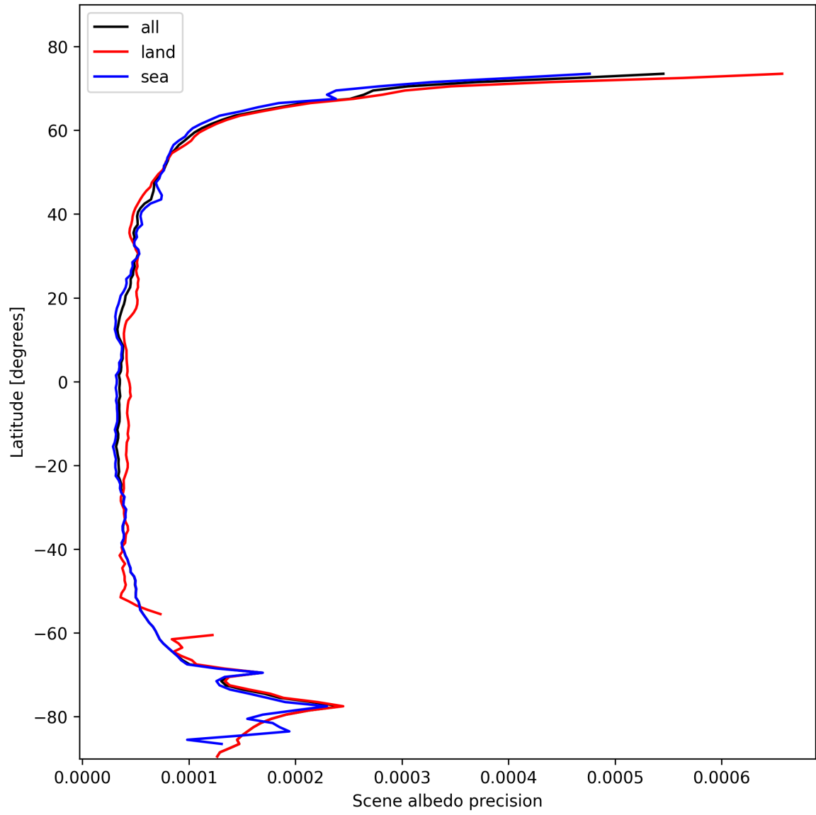
Figure 16: Zonal average of “Scene albedo precision” for 2025-11-02 to 2025-11-03.
