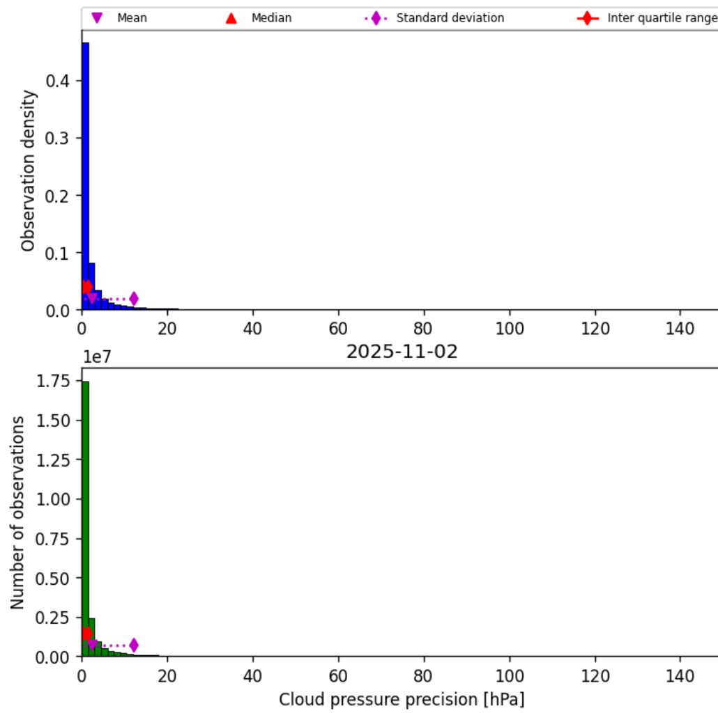
Figure 29: Histogram of “Cloud pressure precision” for 2025-11-02 to 2025-11-03
