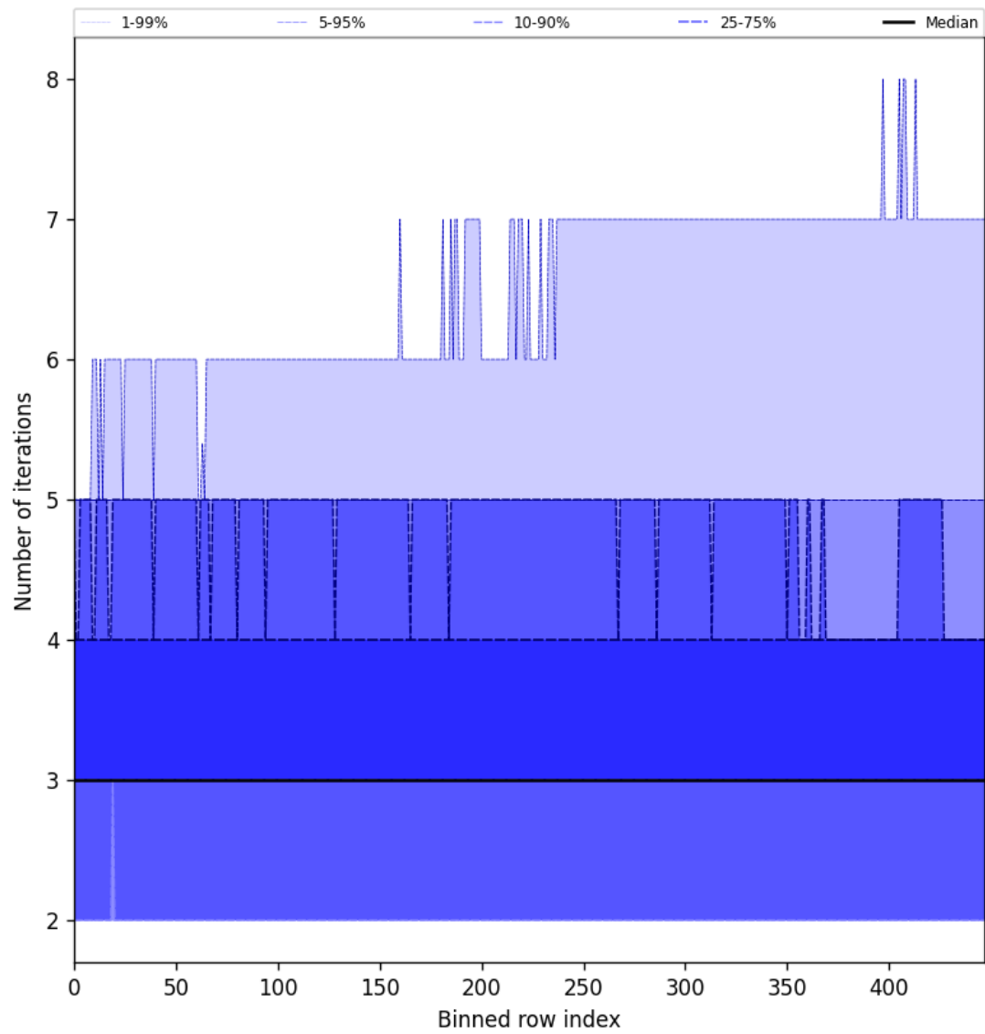
Figure 54: Along track statistics of “Number of iterations” for 2025-11-02 to 2025-11-03
