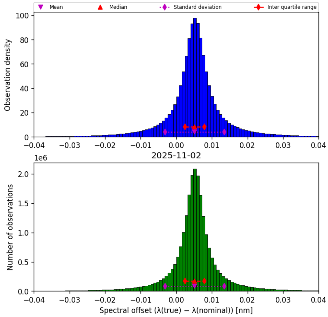
Figure 43: Histogram of “Spectral offset ( \lambda_{\text{true}} - \lambda_{\text{nominal}} )” for 2025-11-02 to 2025-11-03
