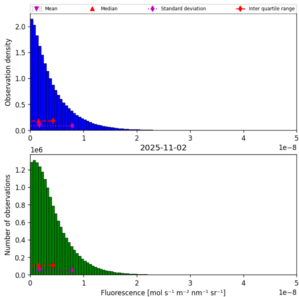
Figure 38: Histogram of “Fluorescence” for 2025-11-02 to 2025-11-03
