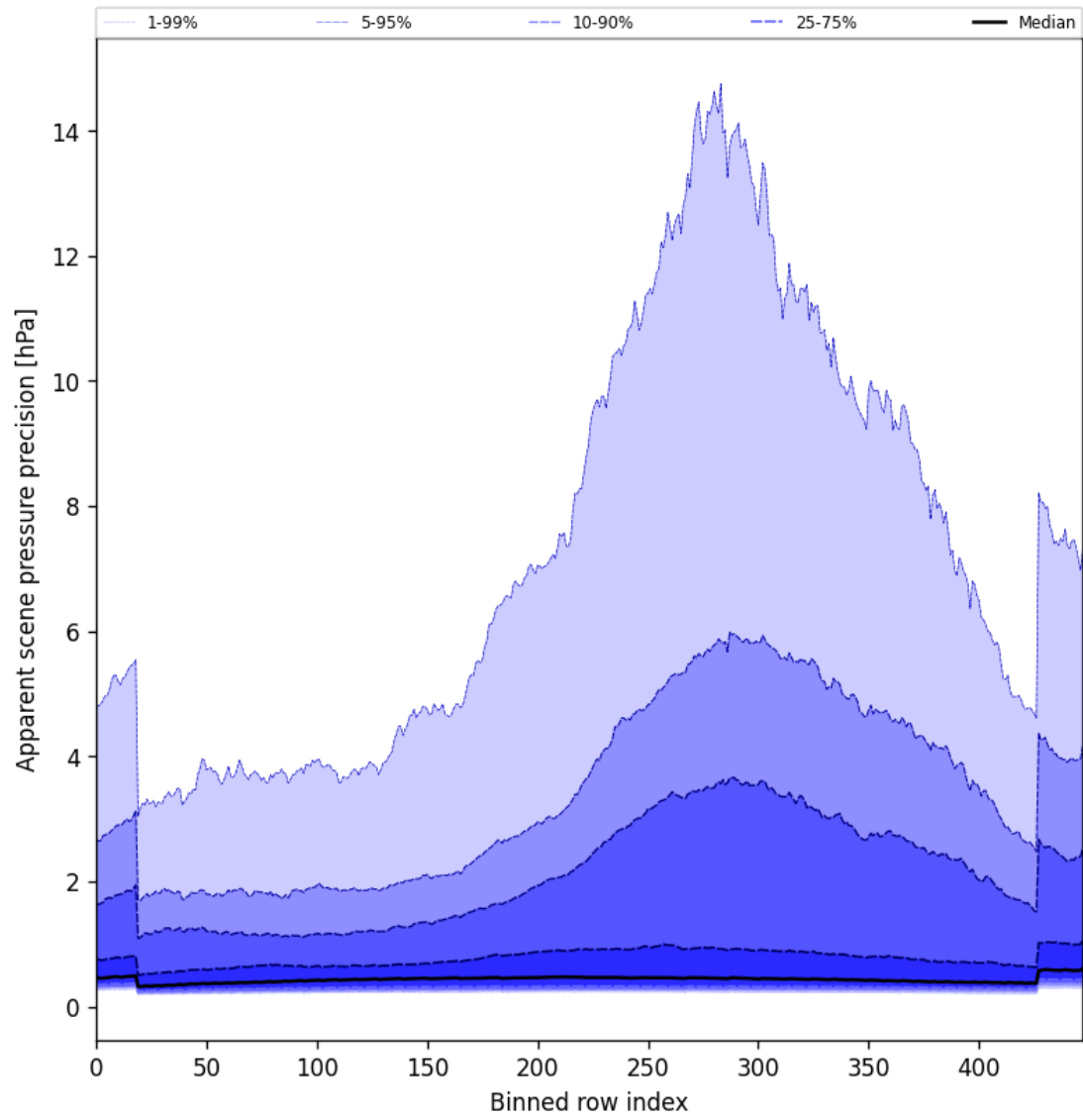
Figure 52: Along track statistics of “Apparent scene pressure precision” for 2025-11-02 to 2025-11-03
