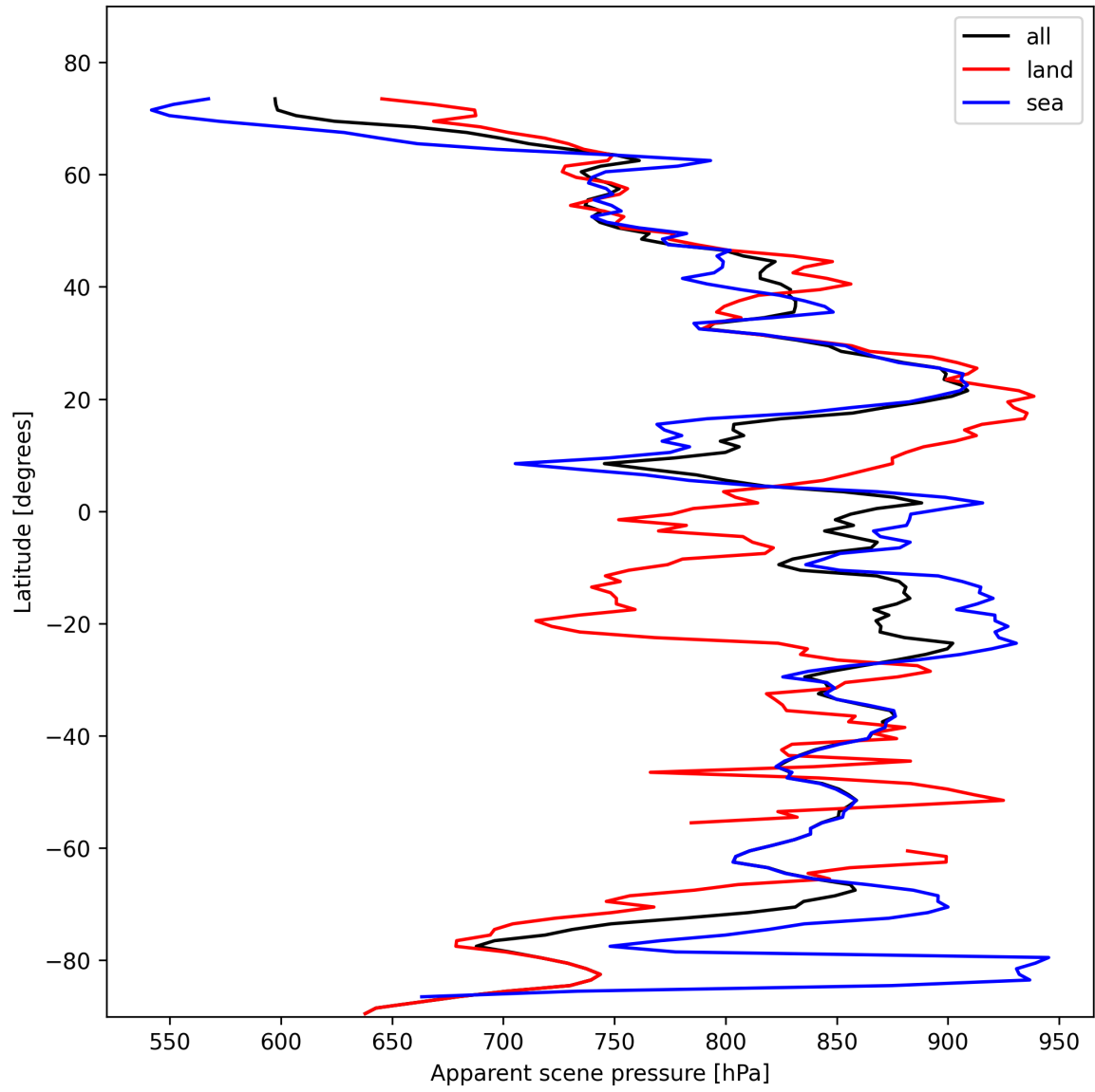
Figure 17: Zonal average of “Apparent scene pressure” for 2025-11-02 to 2025-11-03.
