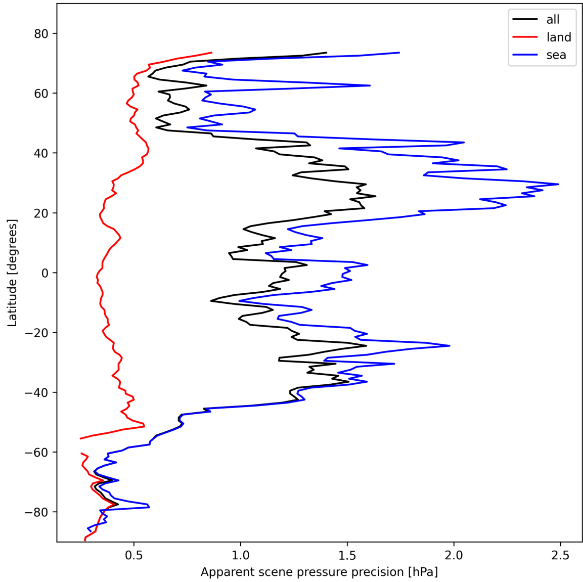
Figure 18: Zonal average of “Apparent scene pressure precision” for 2025-11-02 to 2025-11-03.
