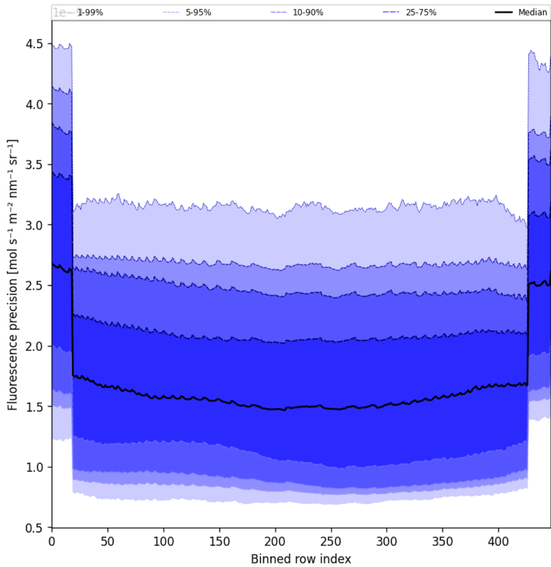
Figure 56: Along track statistics of “Fluorescence precision” for 2025-11-02 to 2025-11-03
