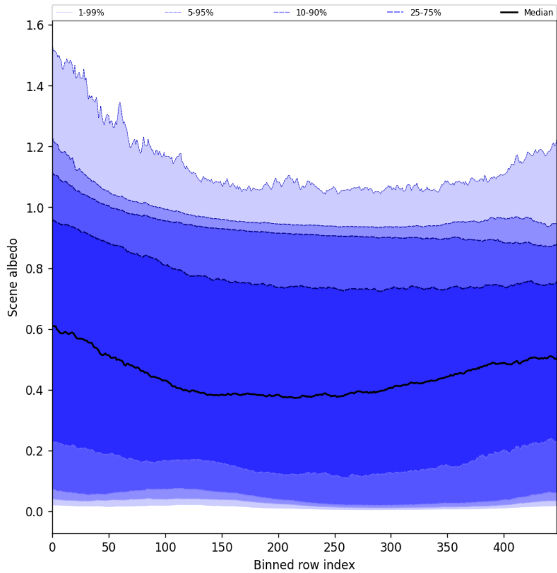
Figure 49: Along track statistics of “Scene albedo” for 2025-11-02 to 2025-11-03
