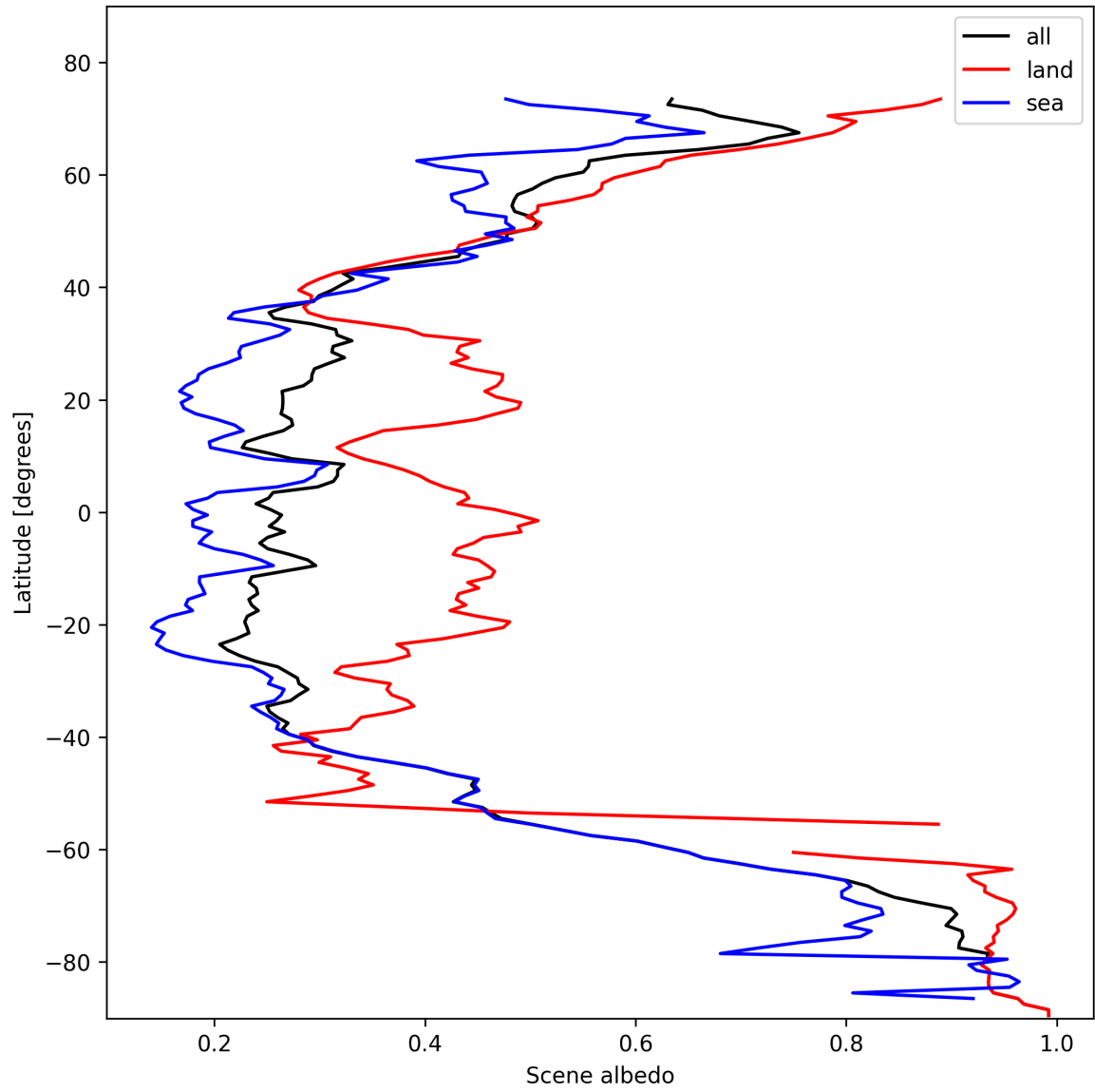
Figure 15: Zonal average of “Scene albedo” for 2025-11-02 to 2025-11-03.
