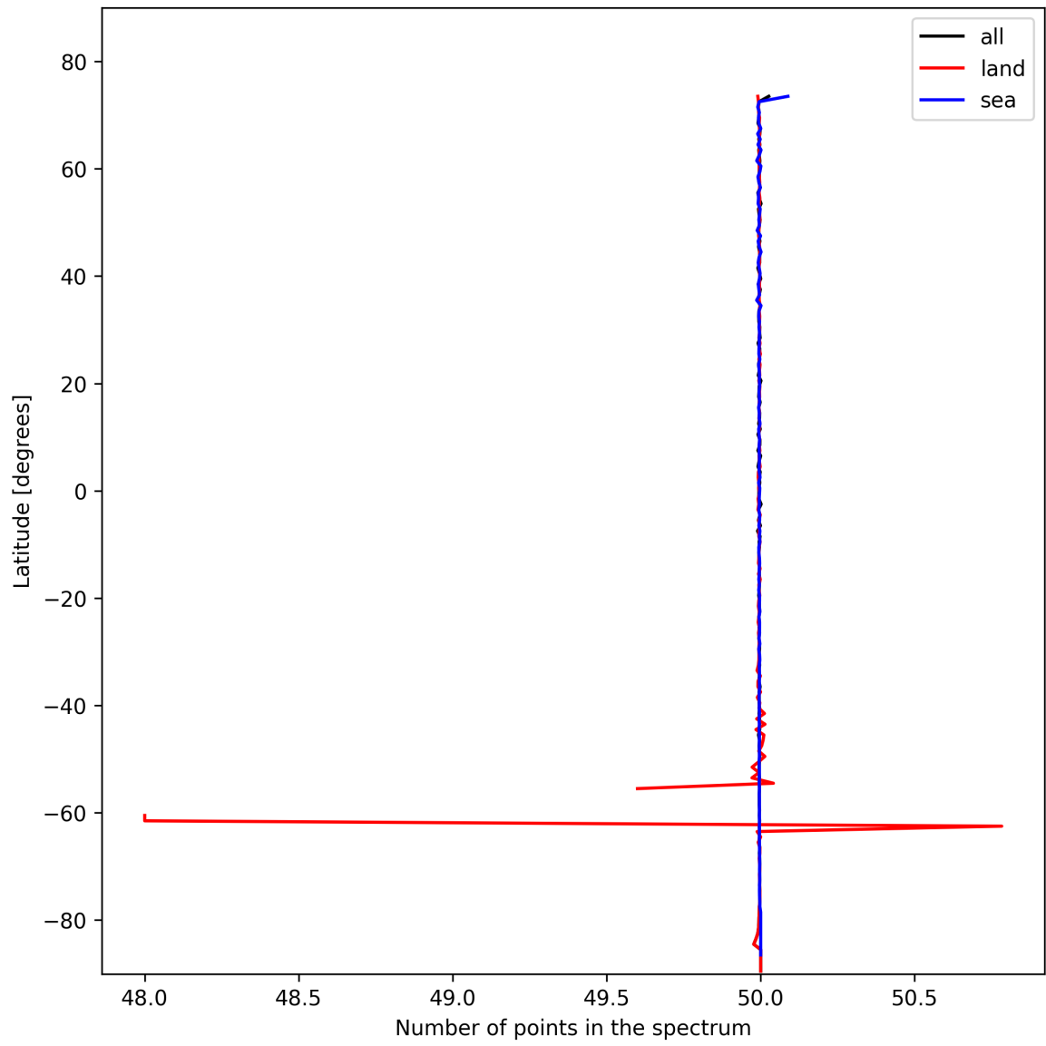
Figure 25: Zonal average of “Number of points in the spectrum” for 2025-11-02 to 2025-11-03.
