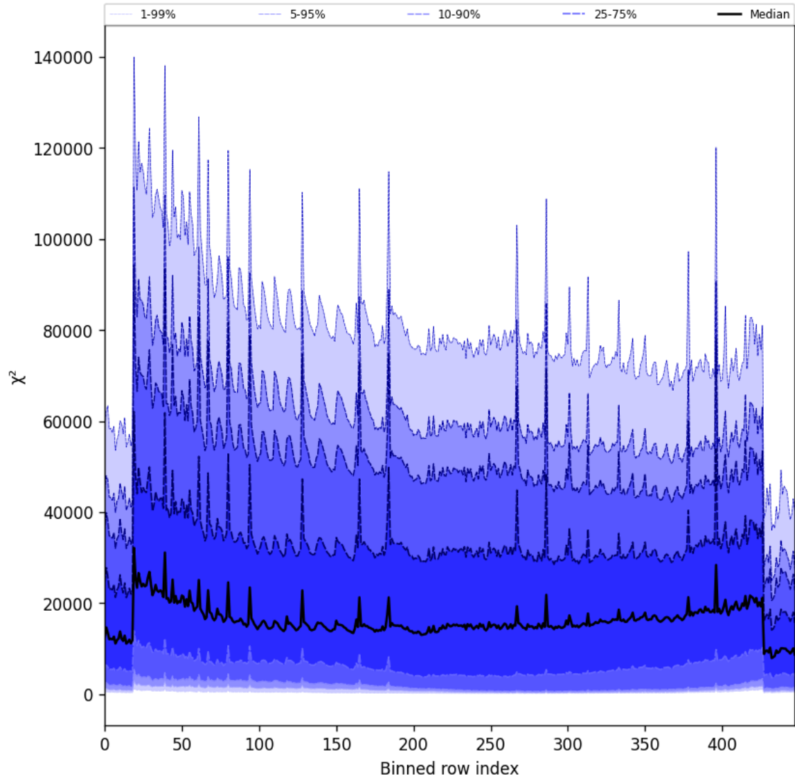
Figure 53: Along track statistics of “ \chi^2 ” for 2025-11-02 to 2025-11-03
