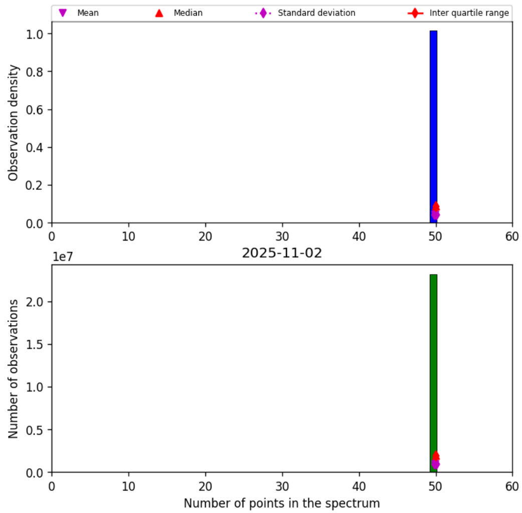
Figure 42: Histogram of “Number of points in the spectrum” for 2025-11-02 to 2025-11-03
