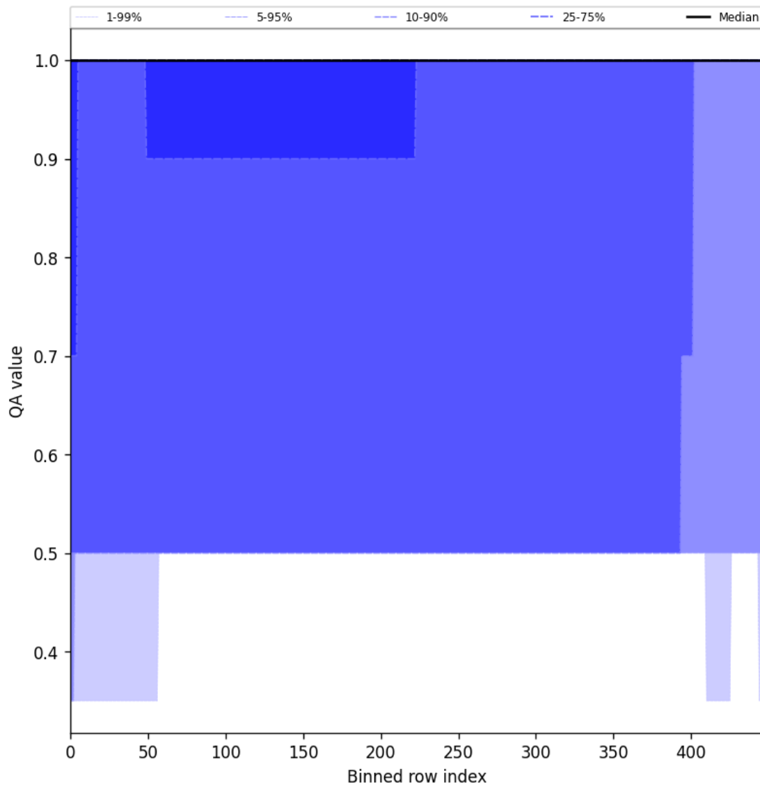
Figure 44: Along track statistics of “QA value” for 2025-11-02 to 2025-11-03
