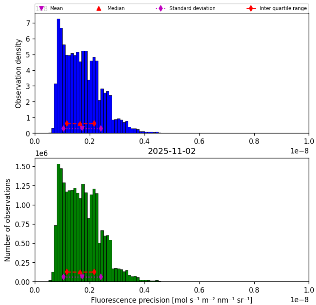
Figure 39: Histogram of “Fluorescence precision” for 2025-11-02 to 2025-11-03
