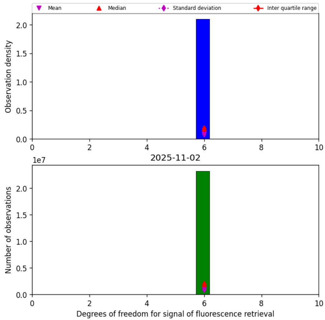
Figure 41: Histogram of “Degrees of freedom for signal of fluorescence retrieval” for 2025-11-02 to 2025-11-03
