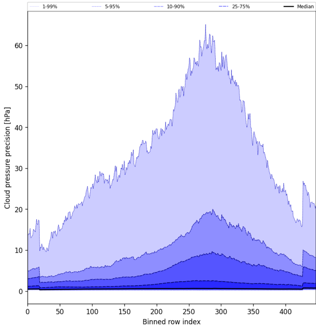
Figure 46: Along track statistics of “Cloud pressure precision” for 2025-11-02 to 2025-11-03
