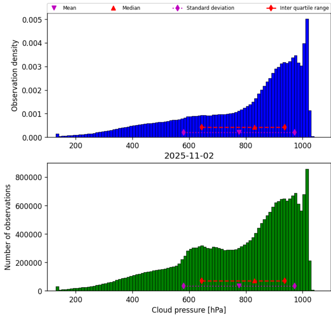
Figure 28: Histogram of “Cloud pressure” for 2025-11-02 to 2025-11-03
