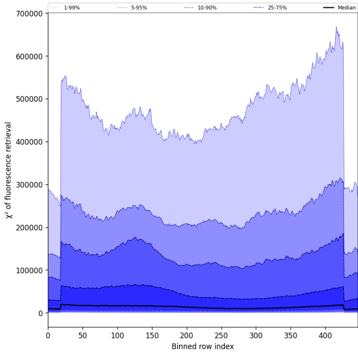
Figure 57: Along track statistics of “ \chi^2 of fluorescence retrieval” for 2025-11-02 to 2025-11-03
