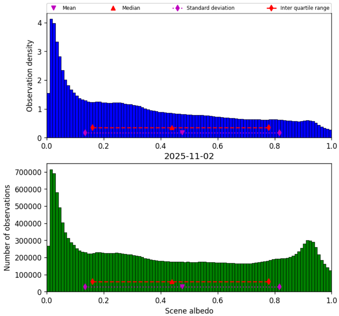
Figure 32: Histogram of “Scene albedo” for 2025-11-02 to 2025-11-03
