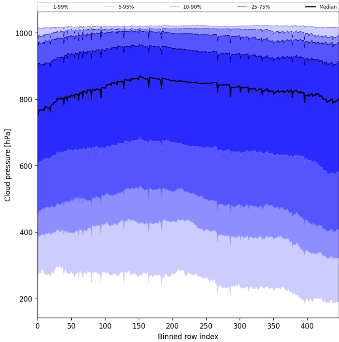
Figure 45: Along track statistics of “Cloud pressure” for 2025-11-02 to 2025-11-03
