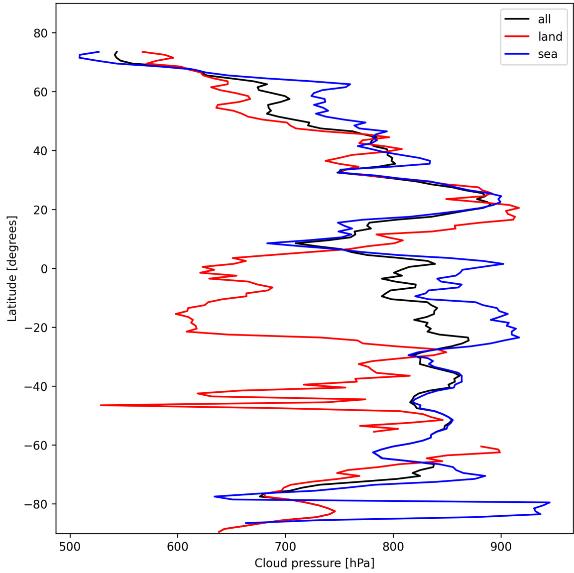
Figure 11: Zonal average of “Cloud pressure” for 2025-11-02 to 2025-11-03.
