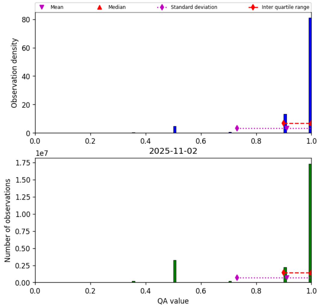
Figure 27: Histogram of “QA value” for 2025-11-02 to 2025-11-03
