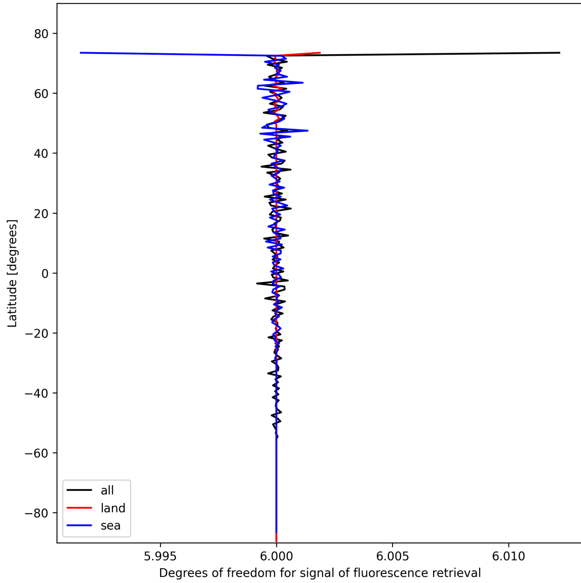
Figure 24: Zonal average of “Degrees of freedom for signal of fluorescence retrieval” for 2025-11-02 to 2025-11-03.
