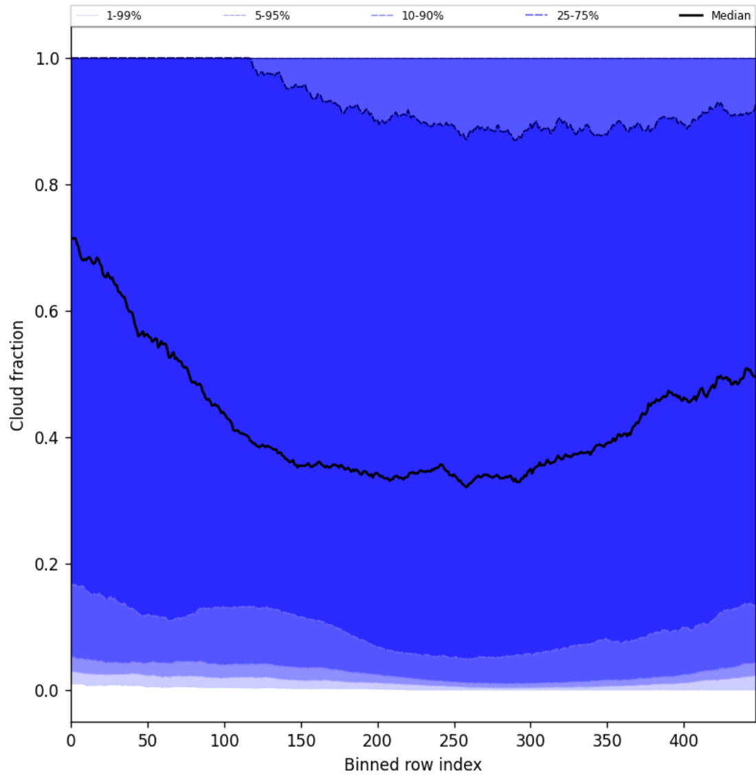
Figure 47: Along track statistics of “Cloud fraction” for 2025-11-02 to 2025-11-03
