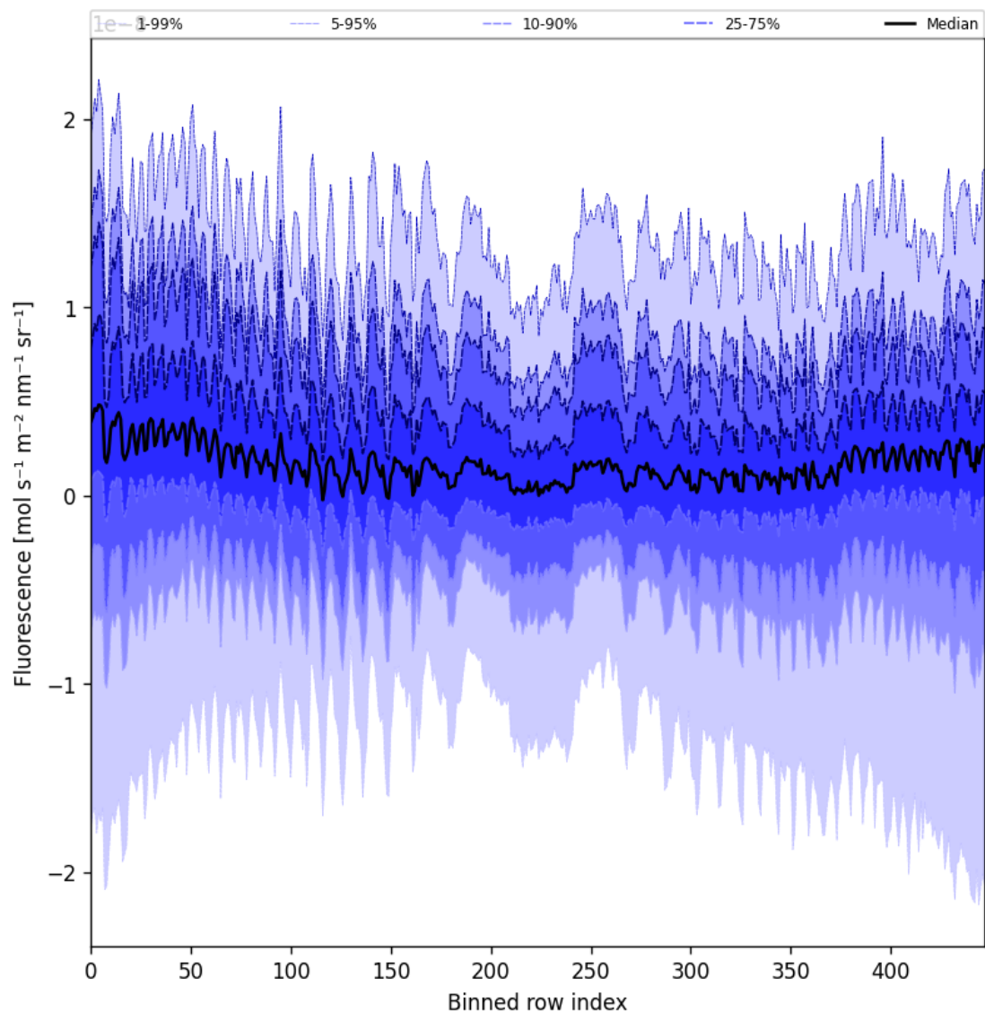
Figure 55: Along track statistics of “Fluorescence” for 2025-11-02 to 2025-11-03
