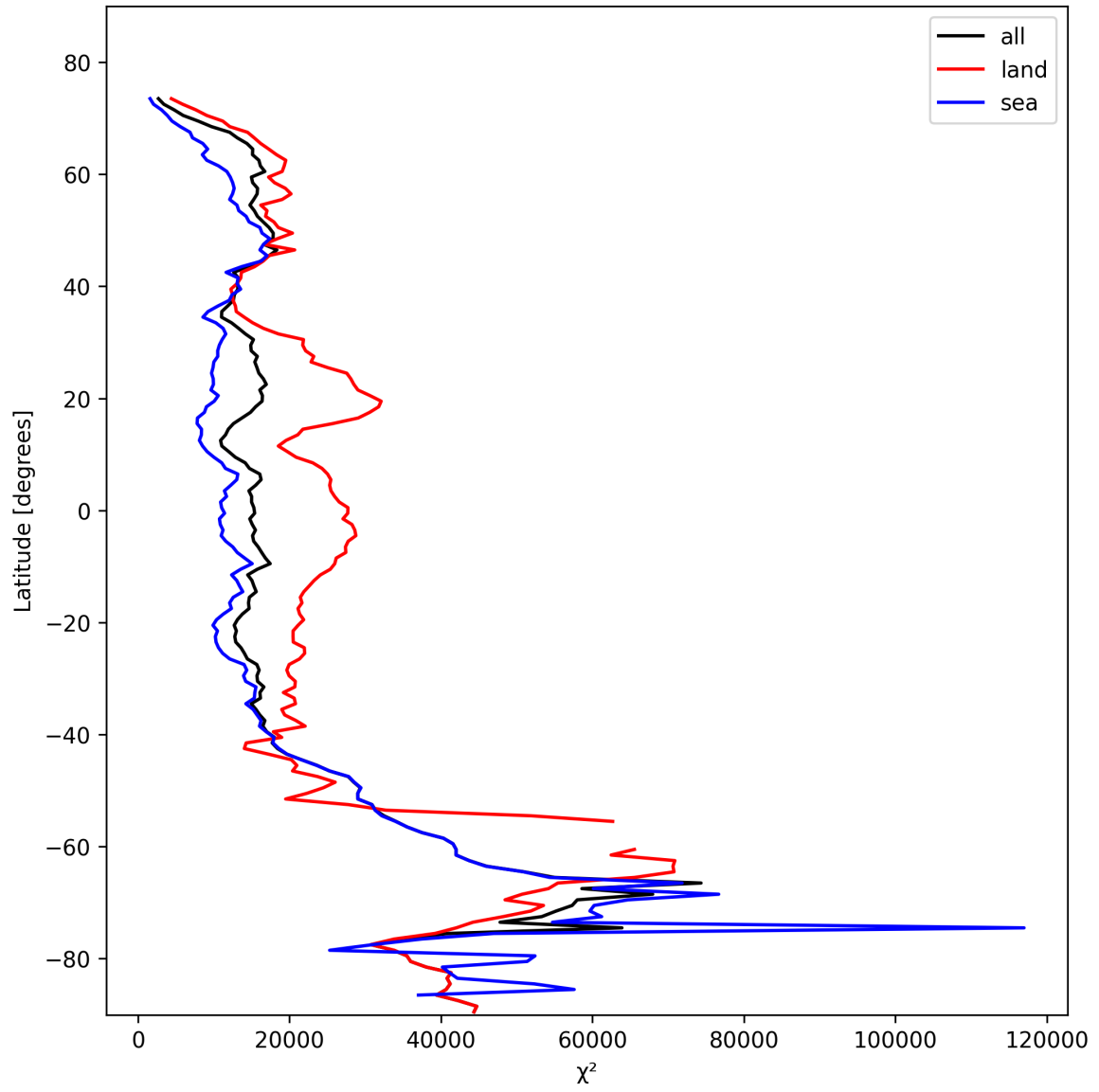
Figure 19: Zonal average of “ \chi^2 ” for 2025-11-02 to 2025-11-03.
