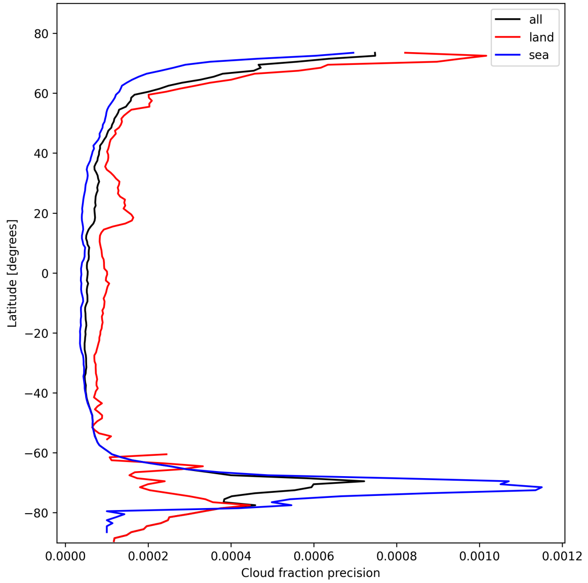
Figure 14: Zonal average of “Cloud fraction precision” for 2025-11-02 to 2025-11-03.
