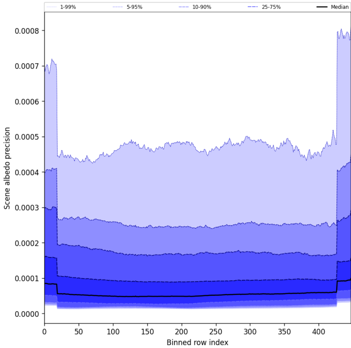
Figure 50: Along track statistics of “Scene albedo precision” for 2025-11-02 to 2025-11-03
