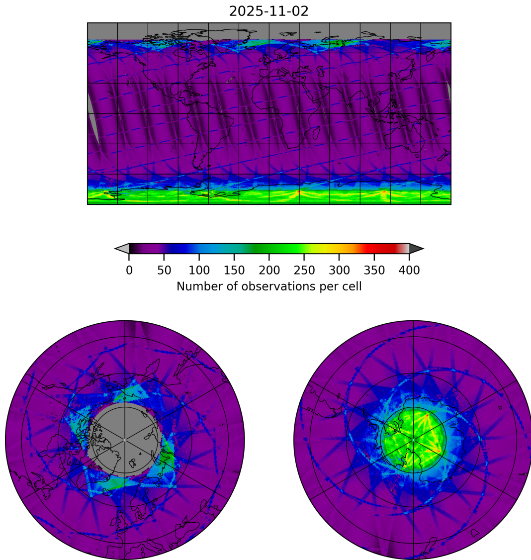
Figure 9: Map of the number of observations for 2025-11-02 to 2025-11-03
