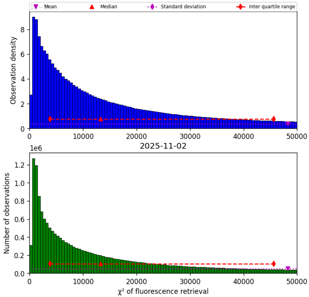
Figure 40: Histogram of “ \chi^2 of fluorescence retrieval” for 2025-11-02 to 2025-11-03
