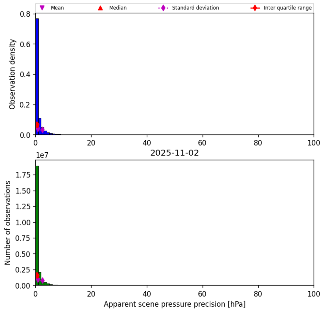
Figure 35: Histogram of “Apparent scene pressure precision” for 2025-11-02 to 2025-11-03
