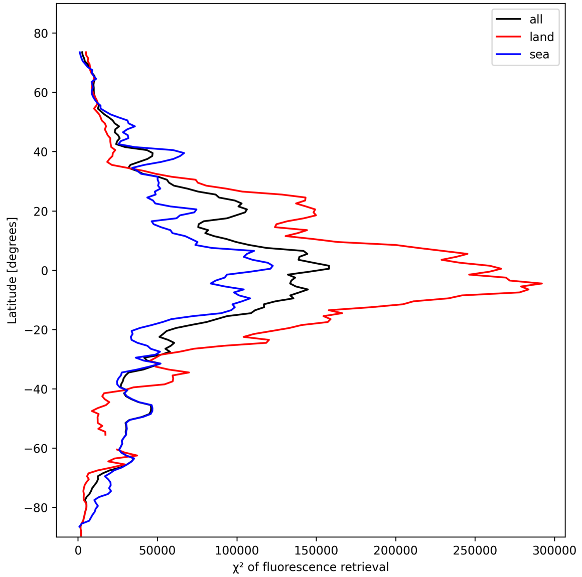
Figure 23: Zonal average of “ \chi^2 of fluorescence retrieval” for 2025-11-02 to 2025-11-03.
