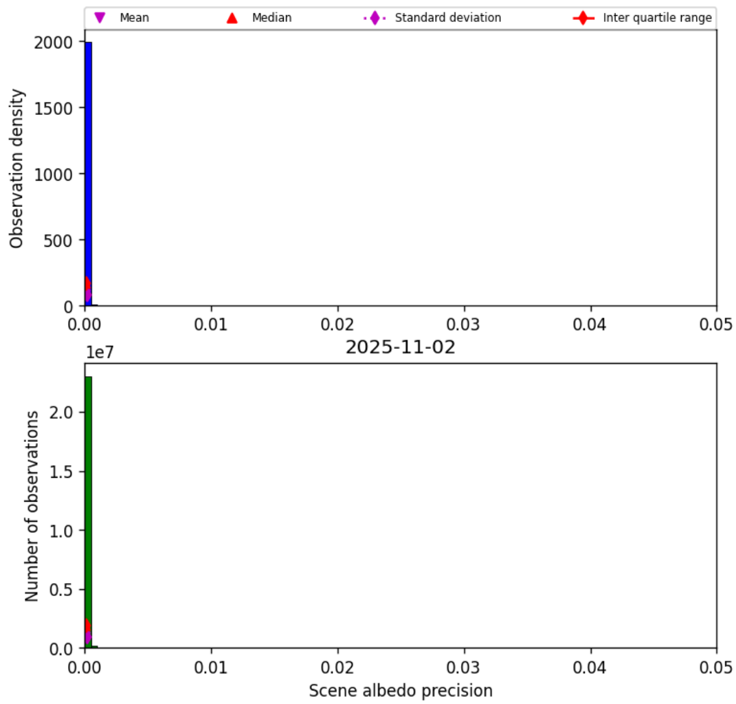
Figure 33: Histogram of “Scene albedo precision” for 2025-11-02 to 2025-11-03
