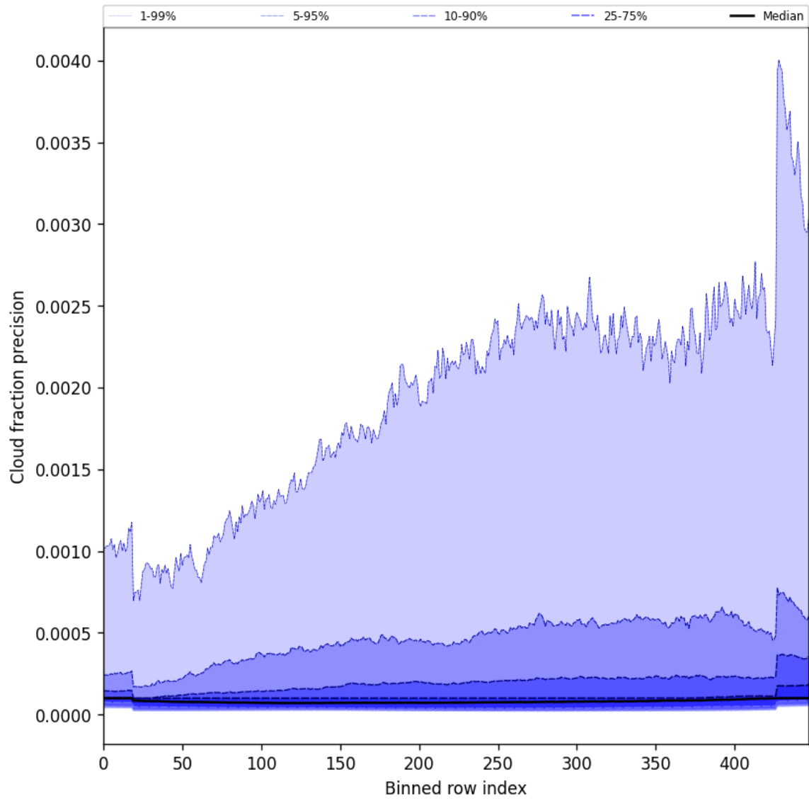
Figure 48: Along track statistics of “Cloud fraction precision” for 2025-11-02 to 2025-11-03
