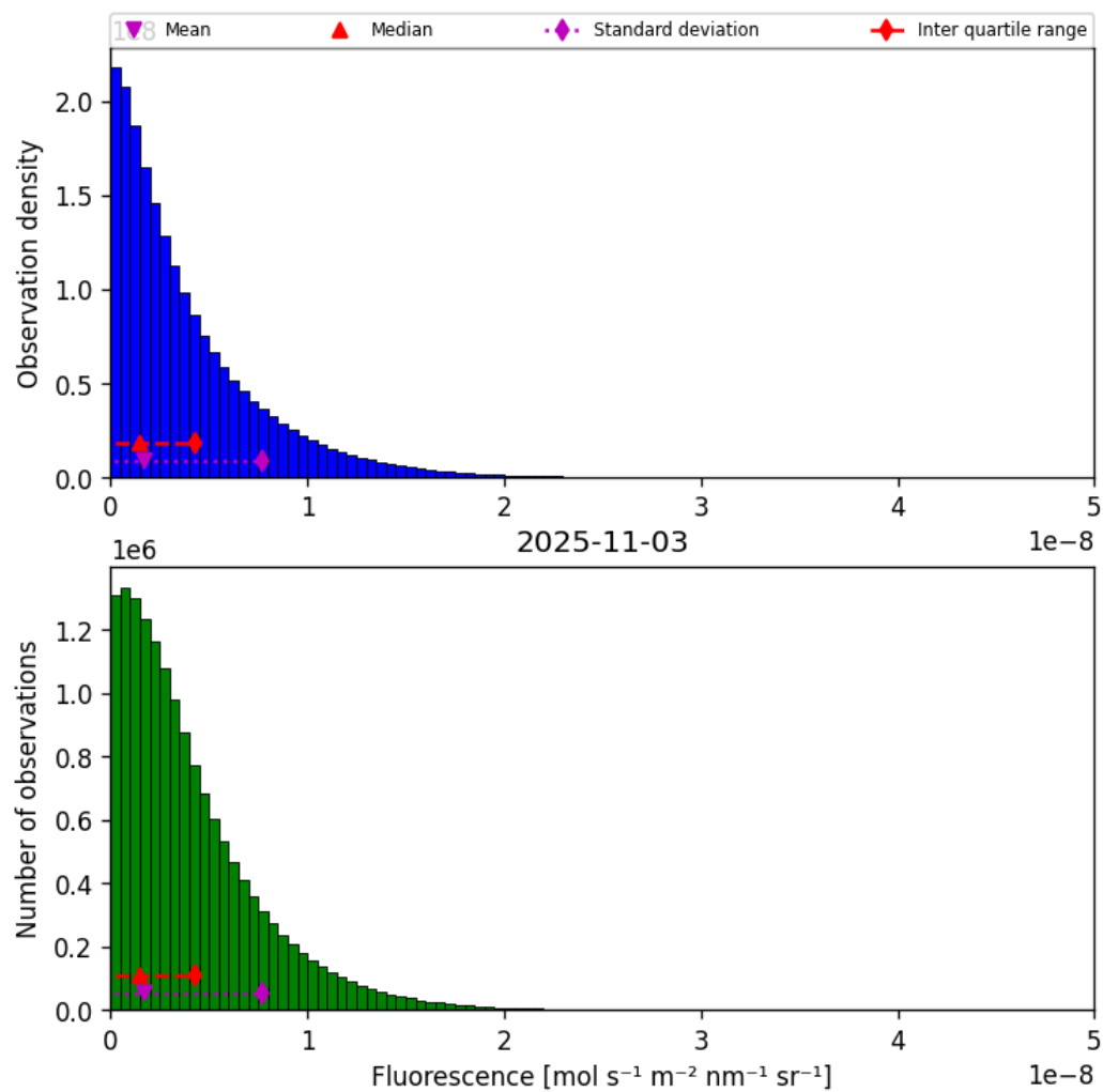
Figure 38: Histogram of “Fluorescence” for 2025-11-03 to 2025-11-04
