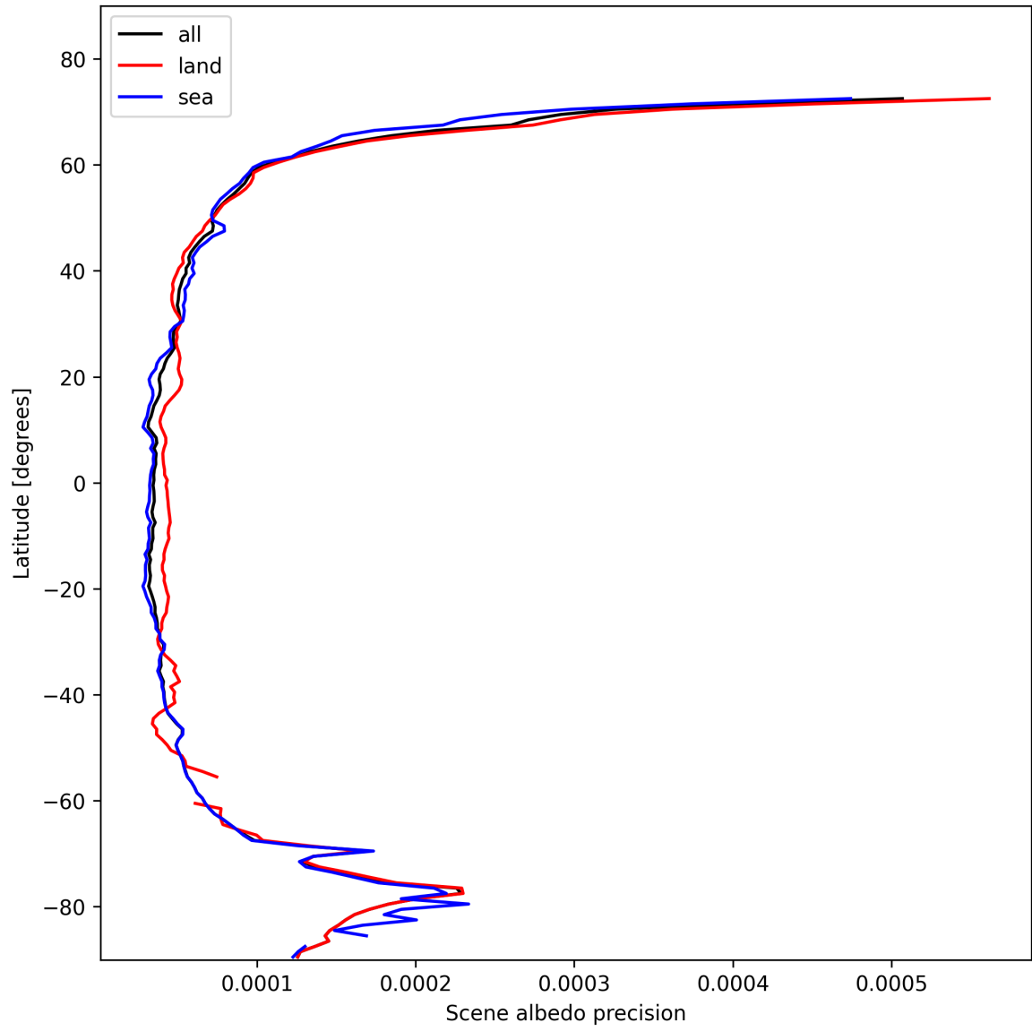
Figure 16: Zonal average of “Scene albedo precision” for 2025-11-03 to 2025-11-04.
