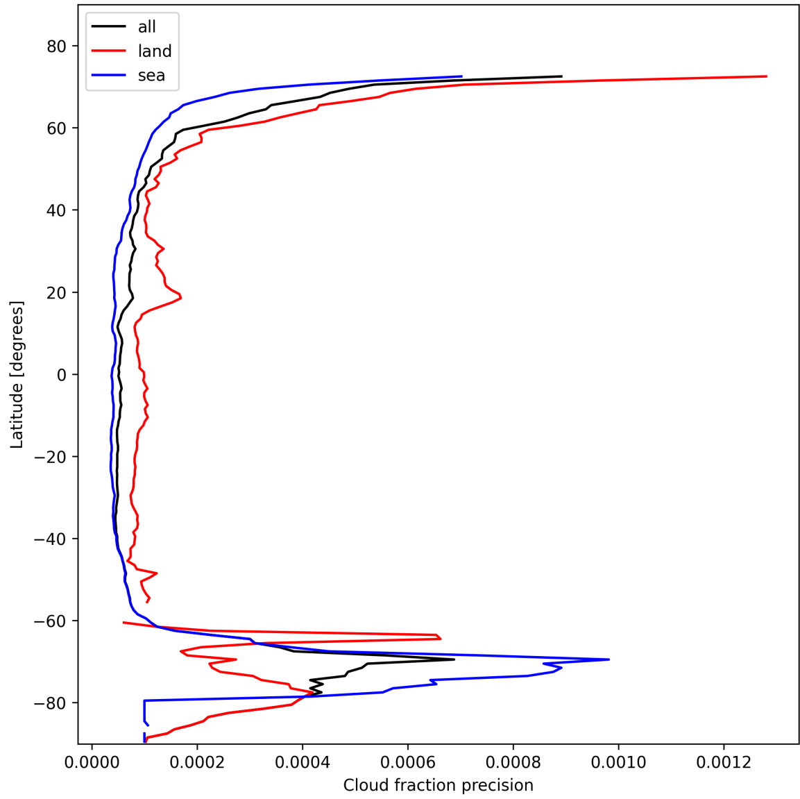
Figure 14: Zonal average of “Cloud fraction precision” for 2025-11-03 to 2025-11-04.
