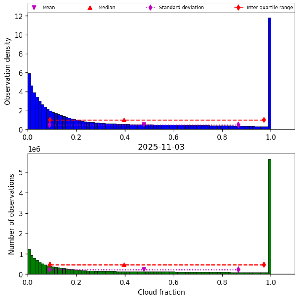
Figure 30: Histogram of “Cloud fraction” for 2025-11-03 to 2025-11-04
