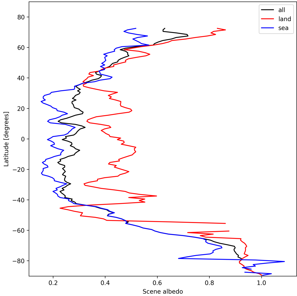
Figure 15: Zonal average of “Scene albedo” for 2025-11-03 to 2025-11-04.
