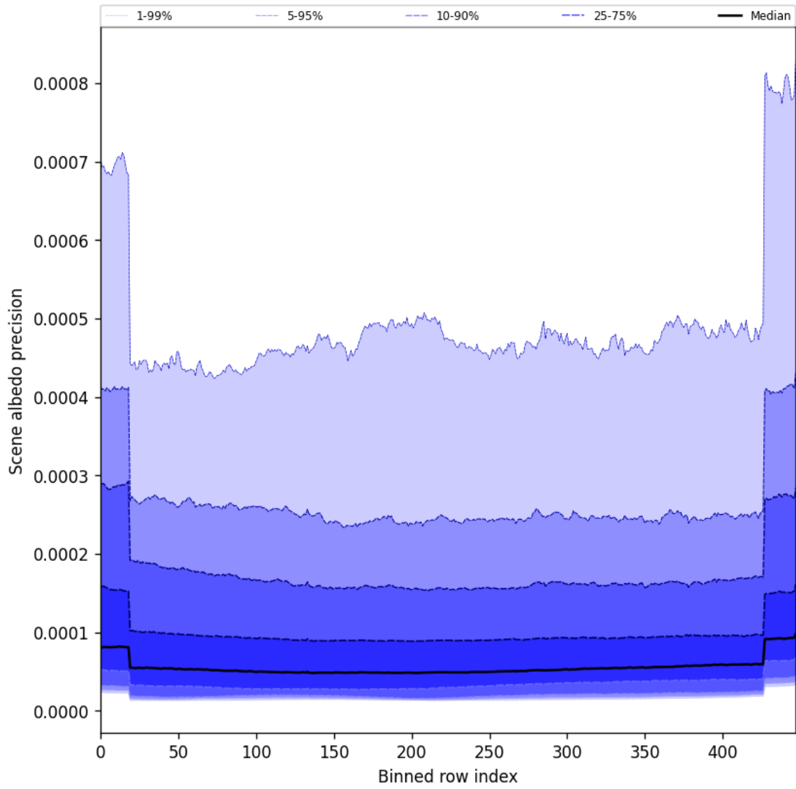
Figure 50: Along track statistics of “Scene albedo precision” for 2025-11-03 to 2025-11-04
