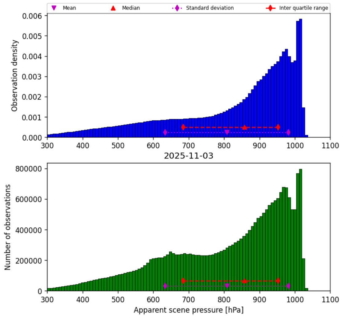
Figure 34: Histogram of “Apparent scene pressure” for 2025-11-03 to 2025-11-04
