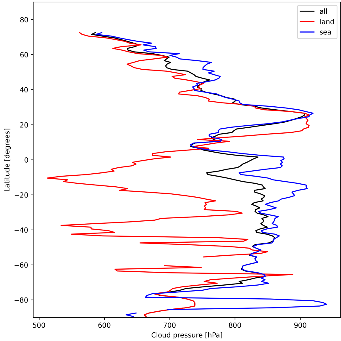
Figure 11: Zonal average of “Cloud pressure” for 2025-11-03 to 2025-11-04.
