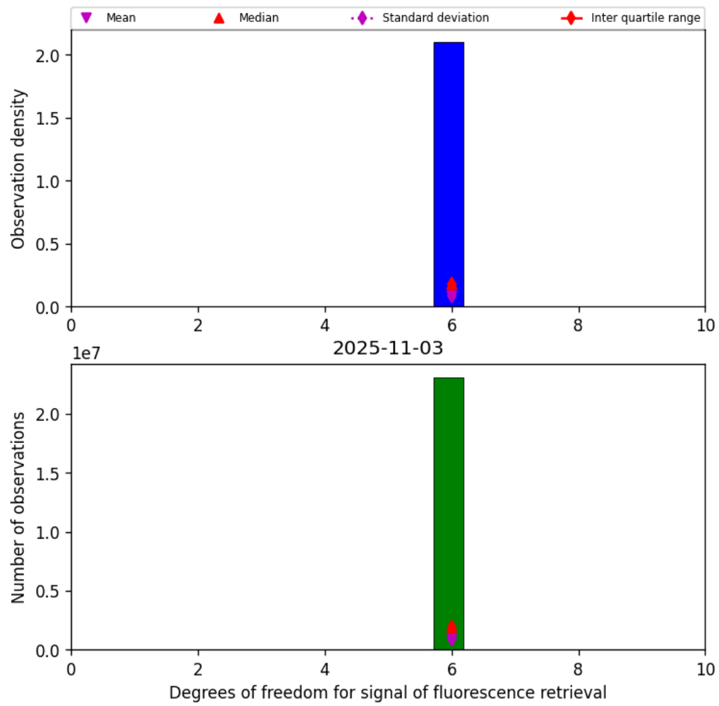
Figure 41: Histogram of “Degrees of freedom for signal of fluorescence retrieval” for 2025-11-03 to 2025-11-04
