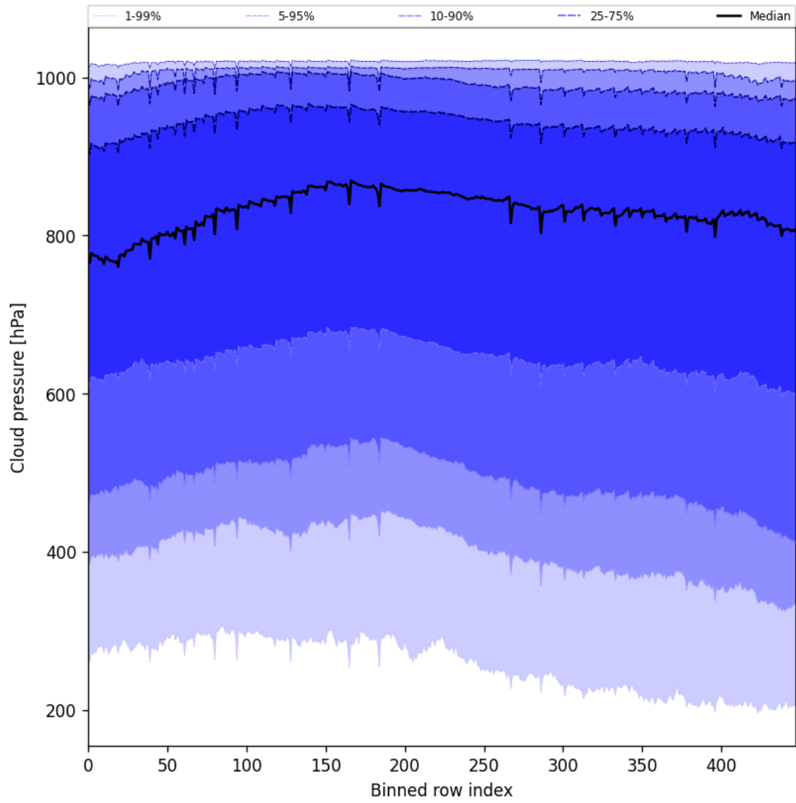
Figure 45: Along track statistics of “Cloud pressure” for 2025-11-03 to 2025-11-04
