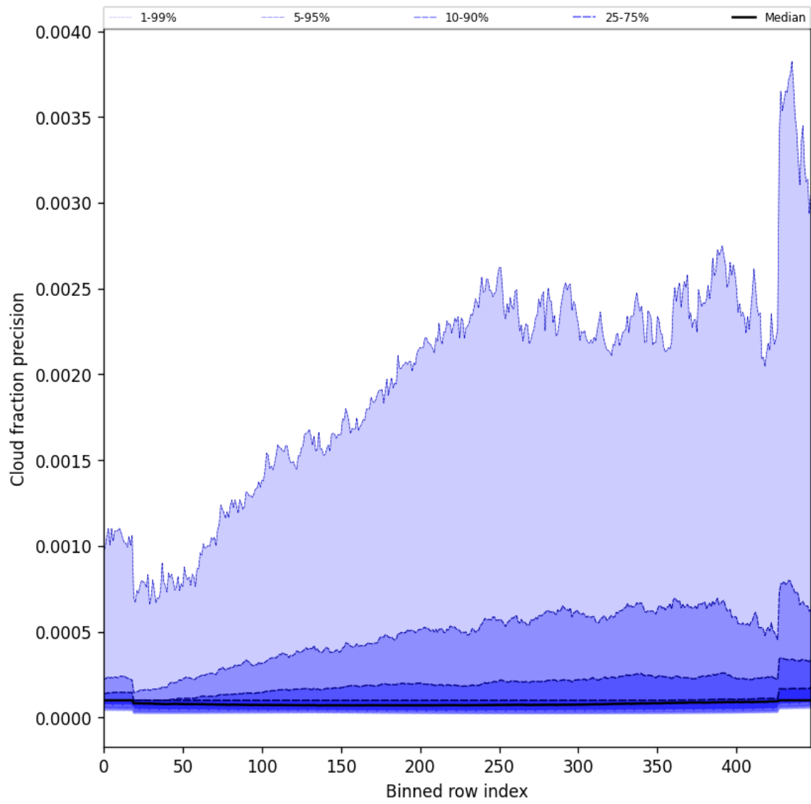
Figure 48: Along track statistics of “Cloud fraction precision” for 2025-11-03 to 2025-11-04
