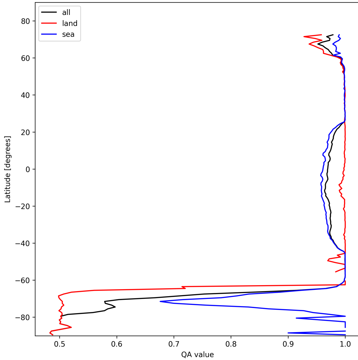
Figure 10: Zonal average of “QA value” for 2025-11-03 to 2025-11-04.
