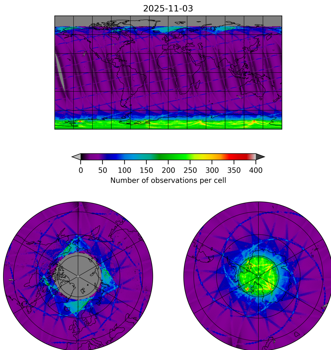
Figure 9: Map of the number of observations for 2025-11-03 to 2025-11-04
