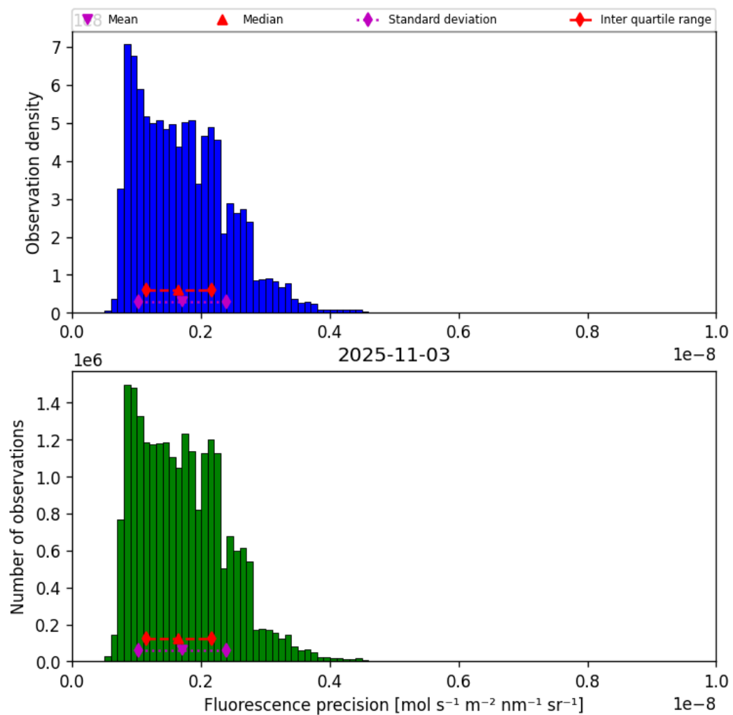
Figure 39: Histogram of “Fluorescence precision” for 2025-11-03 to 2025-11-04
