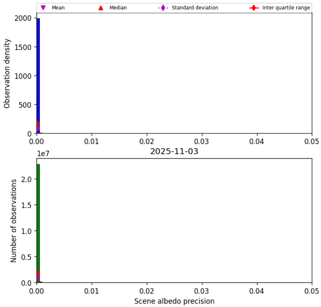
Figure 33: Histogram of “Scene albedo precision” for 2025-11-03 to 2025-11-04
