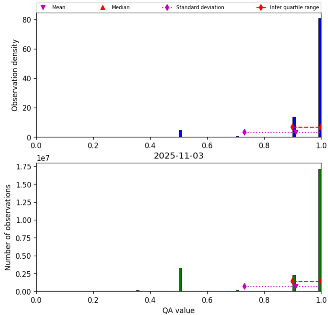
Figure 27: Histogram of “QA value” for 2025-11-03 to 2025-11-04
