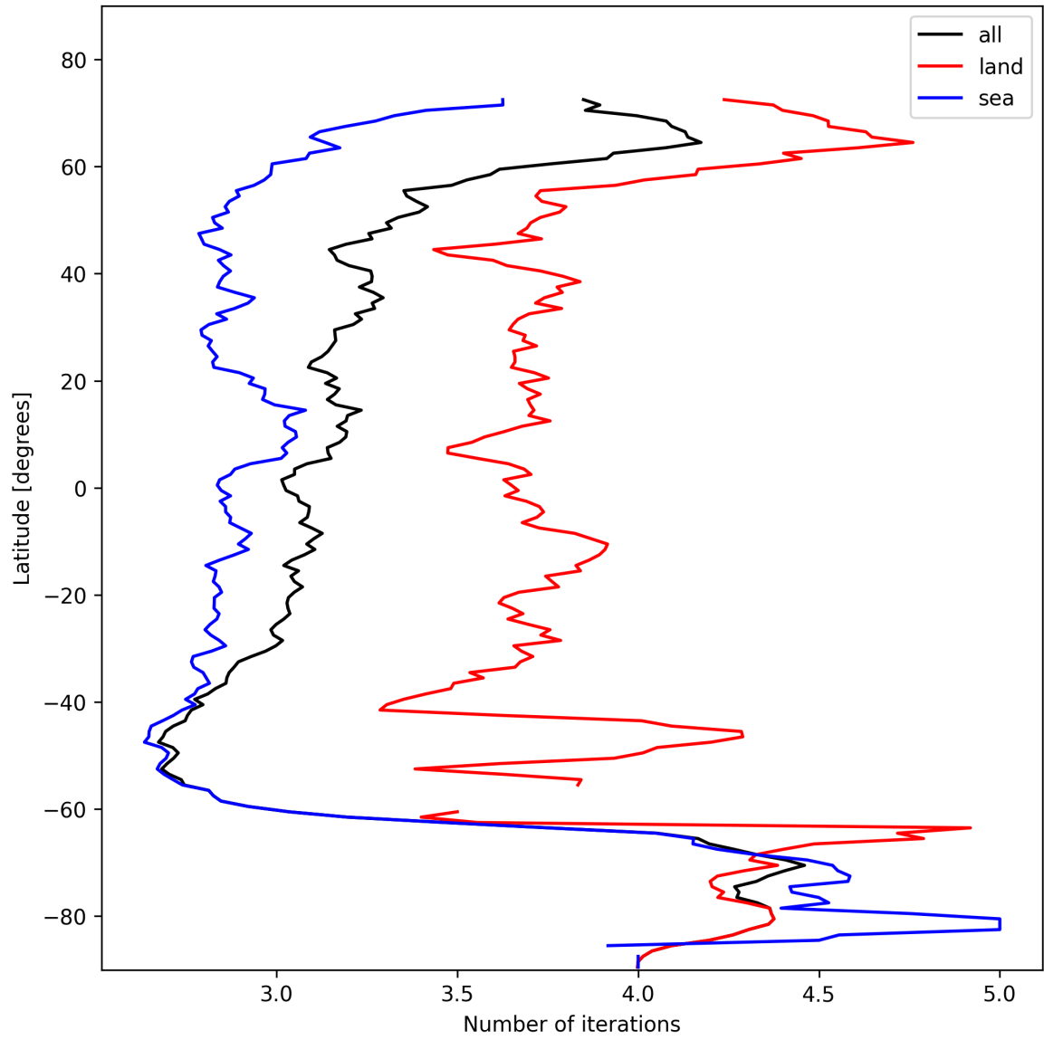
Figure 20: Zonal average of “Number of iterations” for 2025-11-03 to 2025-11-04.
