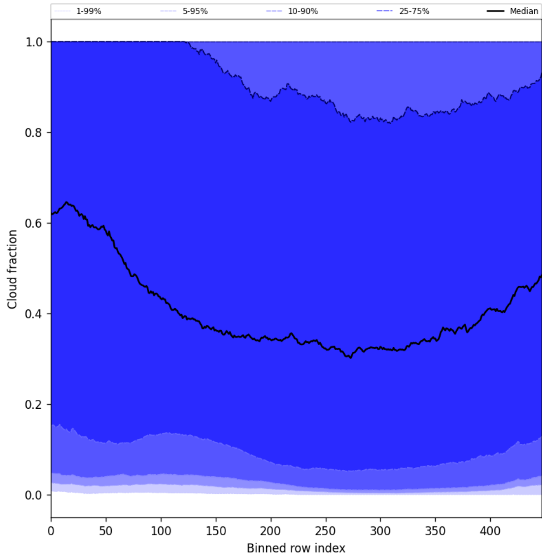
Figure 47: Along track statistics of “Cloud fraction” for 2025-11-03 to 2025-11-04
