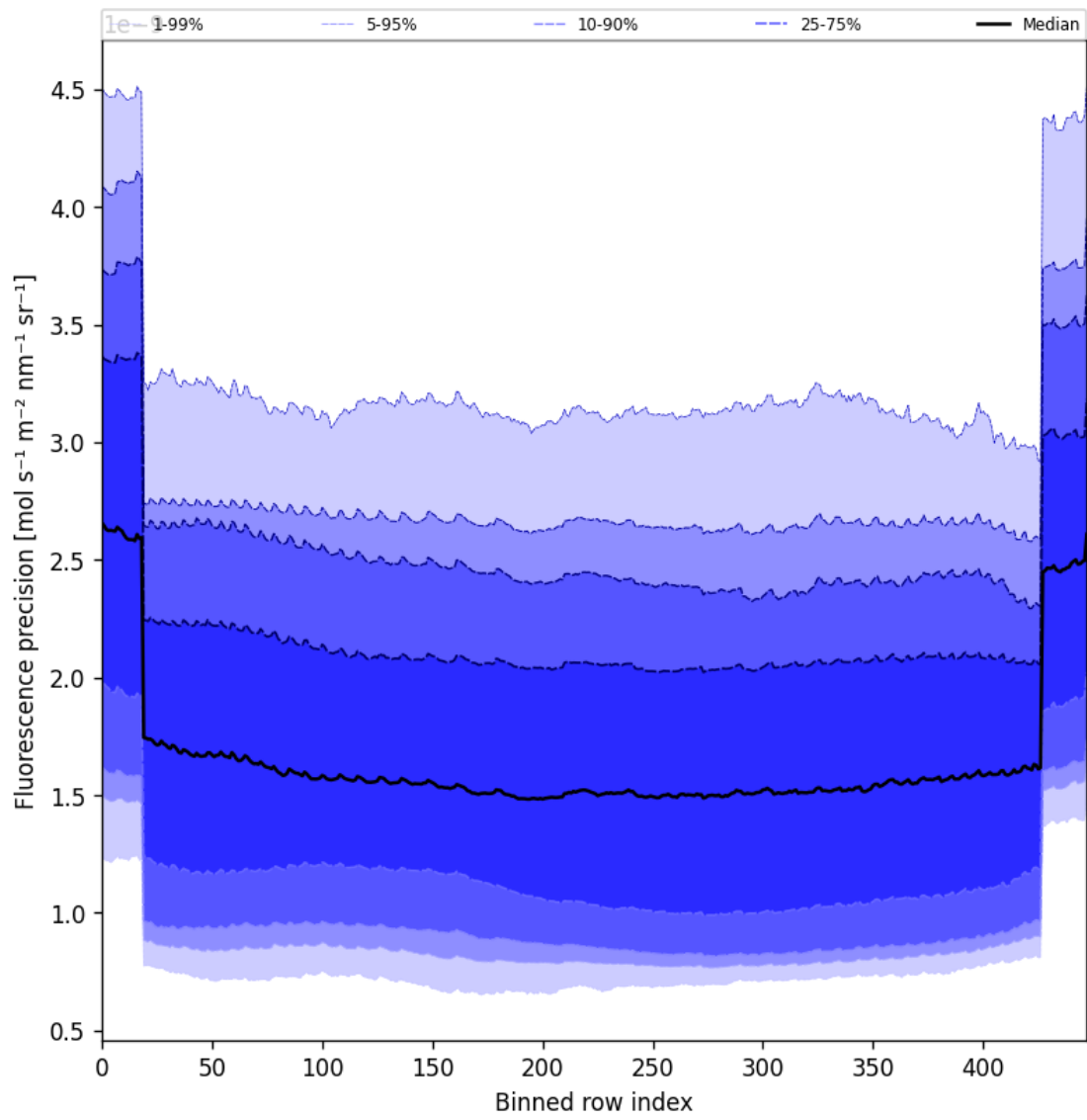
Figure 56: Along track statistics of “Fluorescence precision” for 2025-11-03 to 2025-11-04
