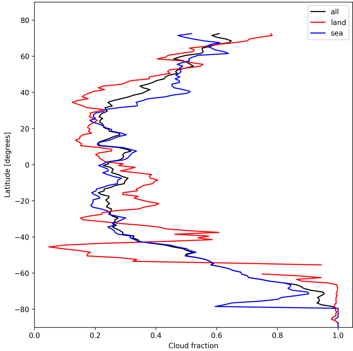
Figure 13: Zonal average of “Cloud fraction” for 2025-11-03 to 2025-11-04.
