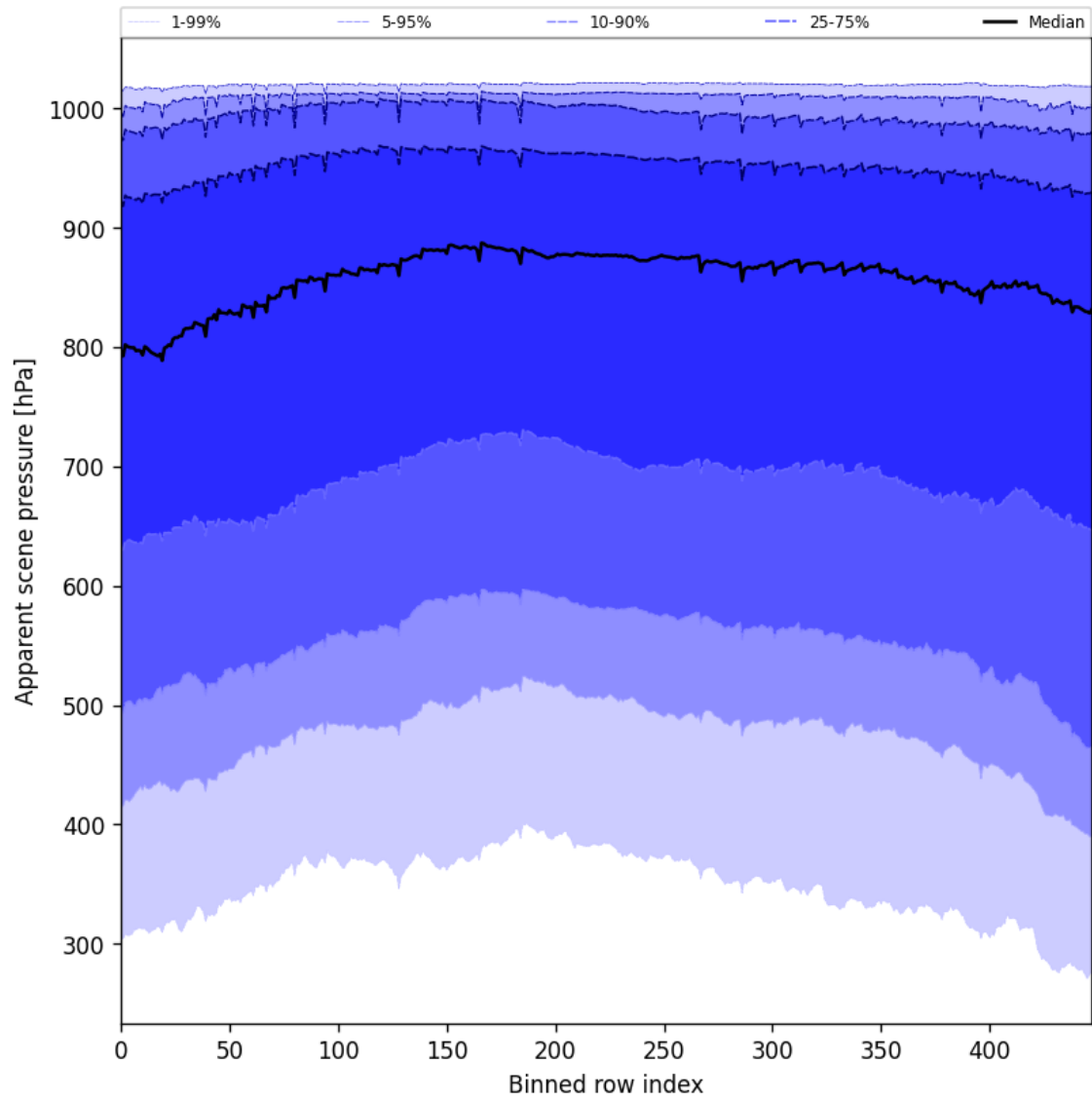
Figure 51: Along track statistics of “Apparent scene pressure” for 2025-11-03 to 2025-11-04
