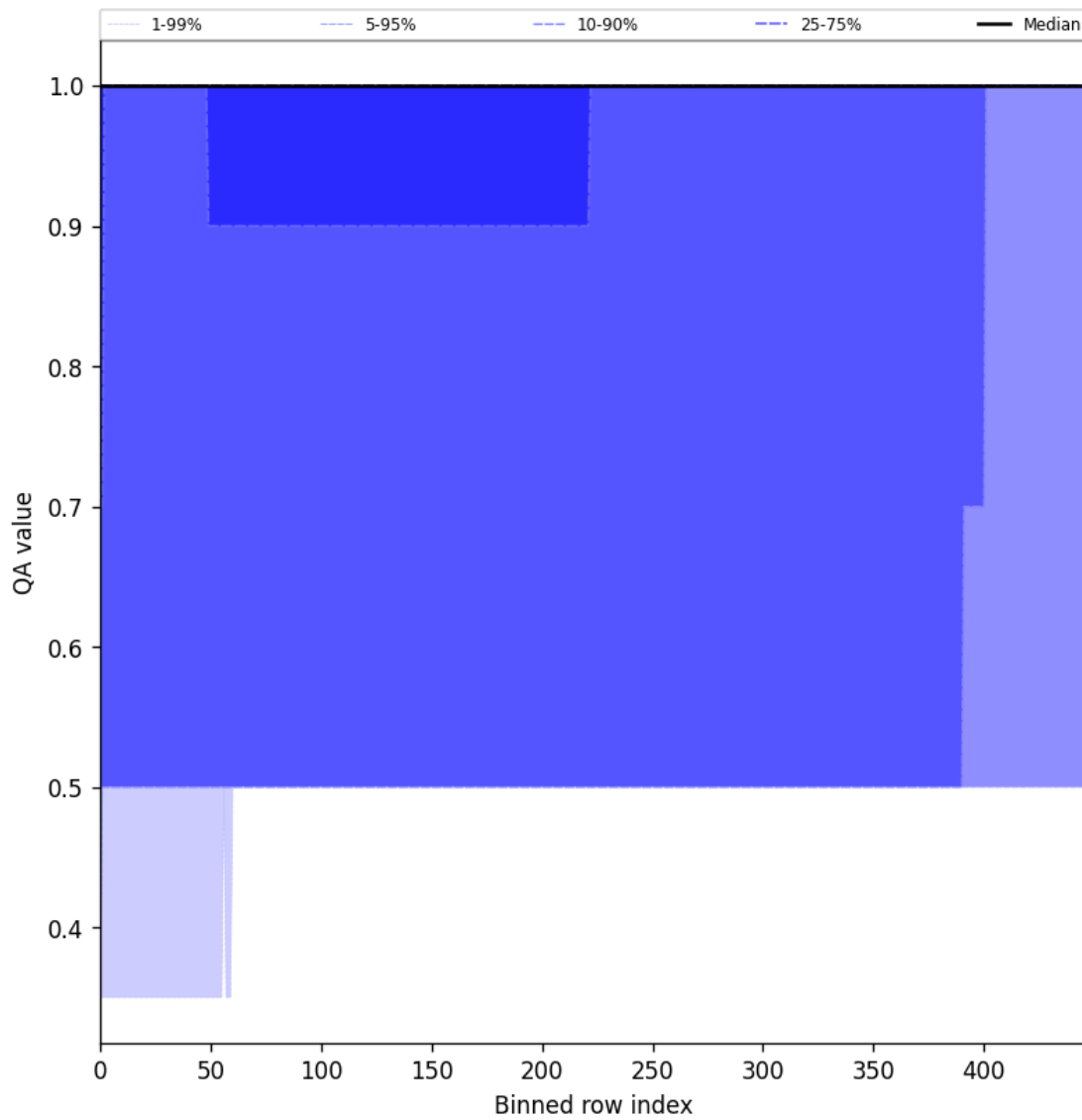
Figure 44: Along track statistics of “QA value” for 2025-11-03 to 2025-11-04
