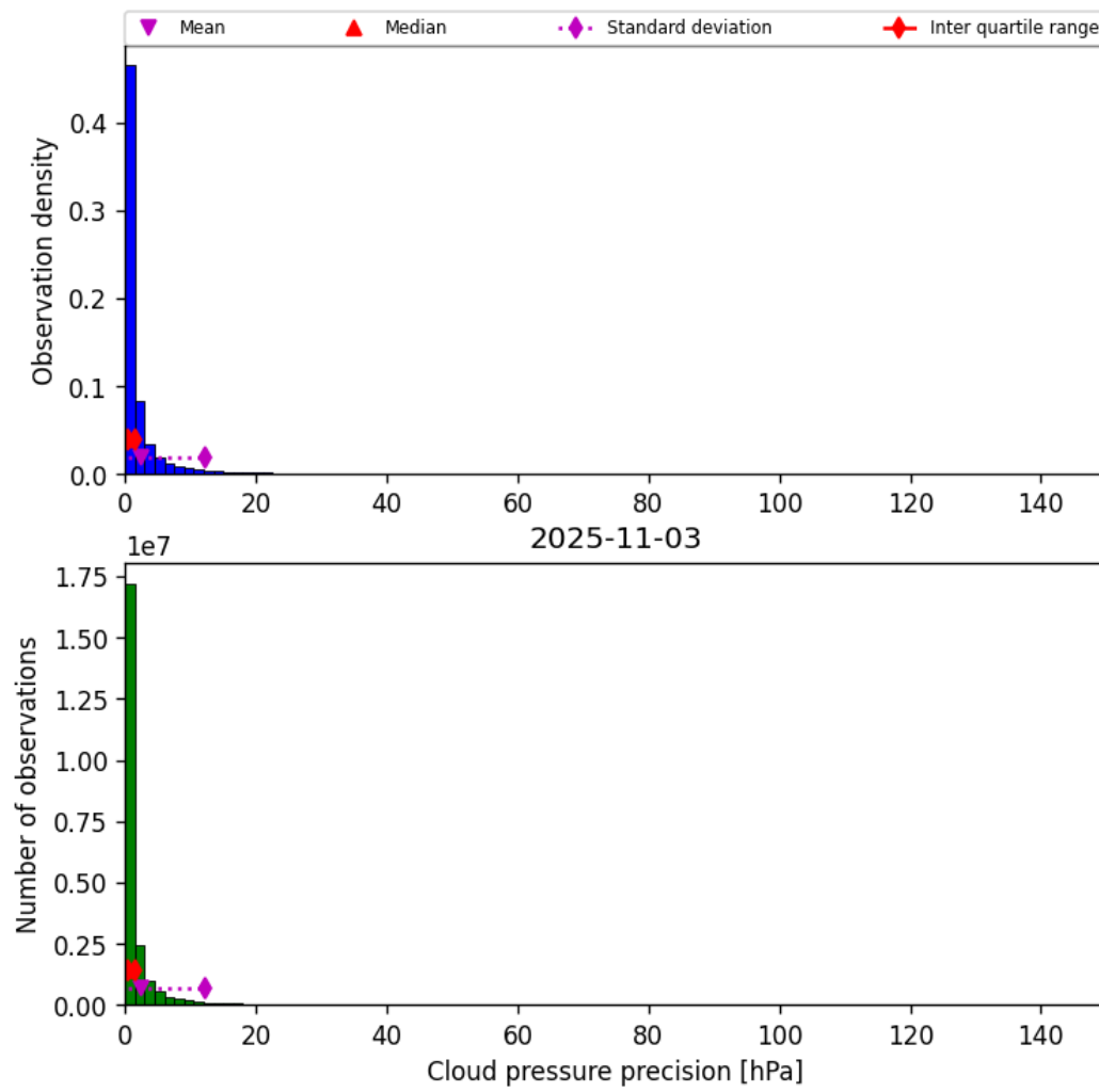
Figure 29: Histogram of “Cloud pressure precision” for 2025-11-03 to 2025-11-04
