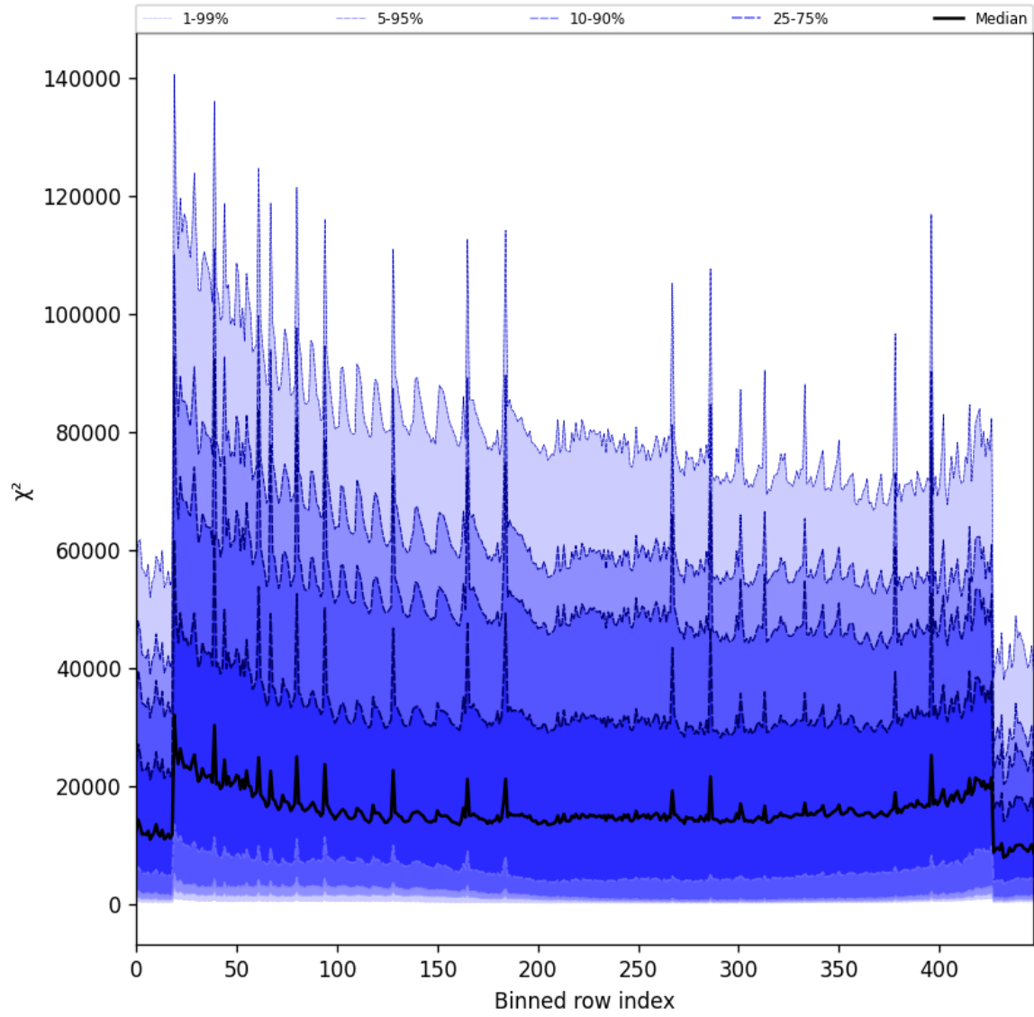
Figure 53: Along track statistics of “ \chi^2 ” for 2025-11-03 to 2025-11-04
