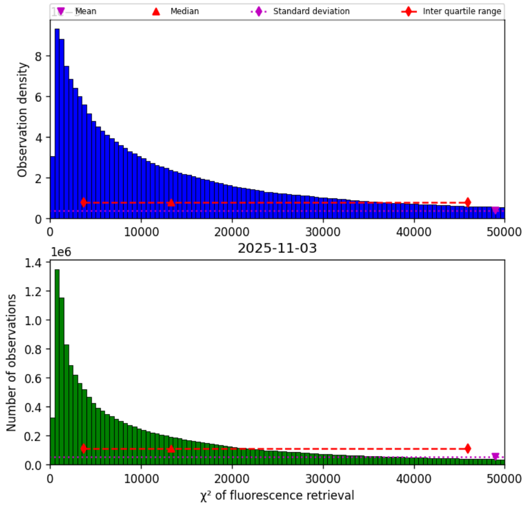
Figure 40: Histogram of “ \chi^2 of fluorescence retrieval” for 2025-11-03 to 2025-11-04
