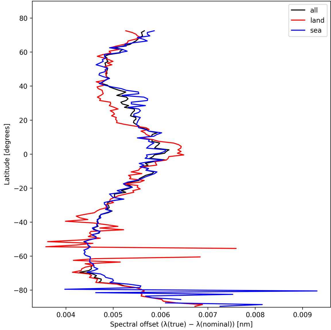
Figure 26: Zonal average of “Spectral offset ( \lambda_{\text{true}} - \lambda_{\text{nominal}} )” for 2025-11-03 to 2025-11-04.
