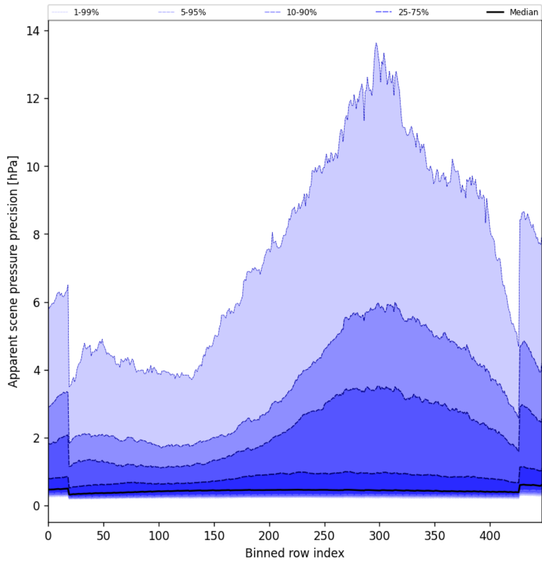
Figure 52: Along track statistics of “Apparent scene pressure precision” for 2025-11-03 to 2025-11-04
