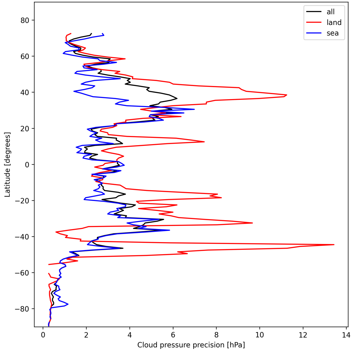
Figure 12: Zonal average of “Cloud pressure precision” for 2025-11-03 to 2025-11-04.
