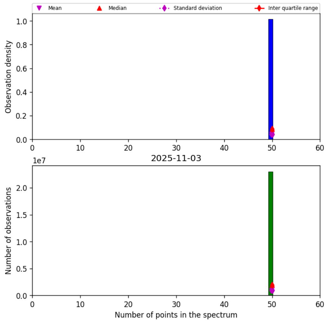
Figure 42: Histogram of “Number of points in the spectrum” for 2025-11-03 to 2025-11-04
