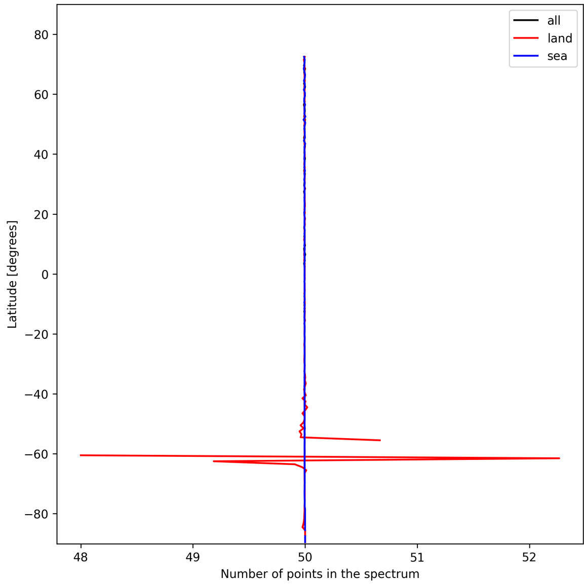
Figure 25: Zonal average of “Number of points in the spectrum” for 2025-11-03 to 2025-11-04.
