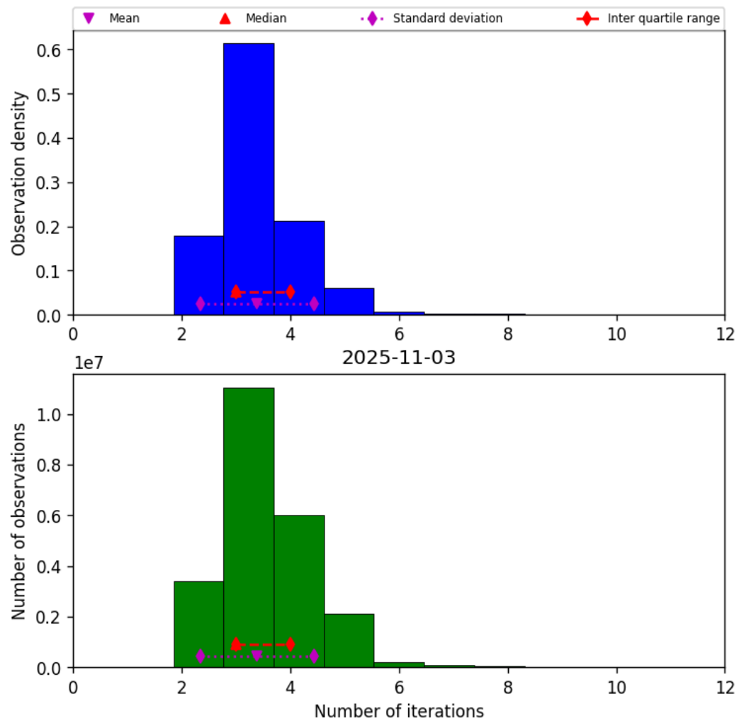
Figure 37: Histogram of “Number of iterations” for 2025-11-03 to 2025-11-04
