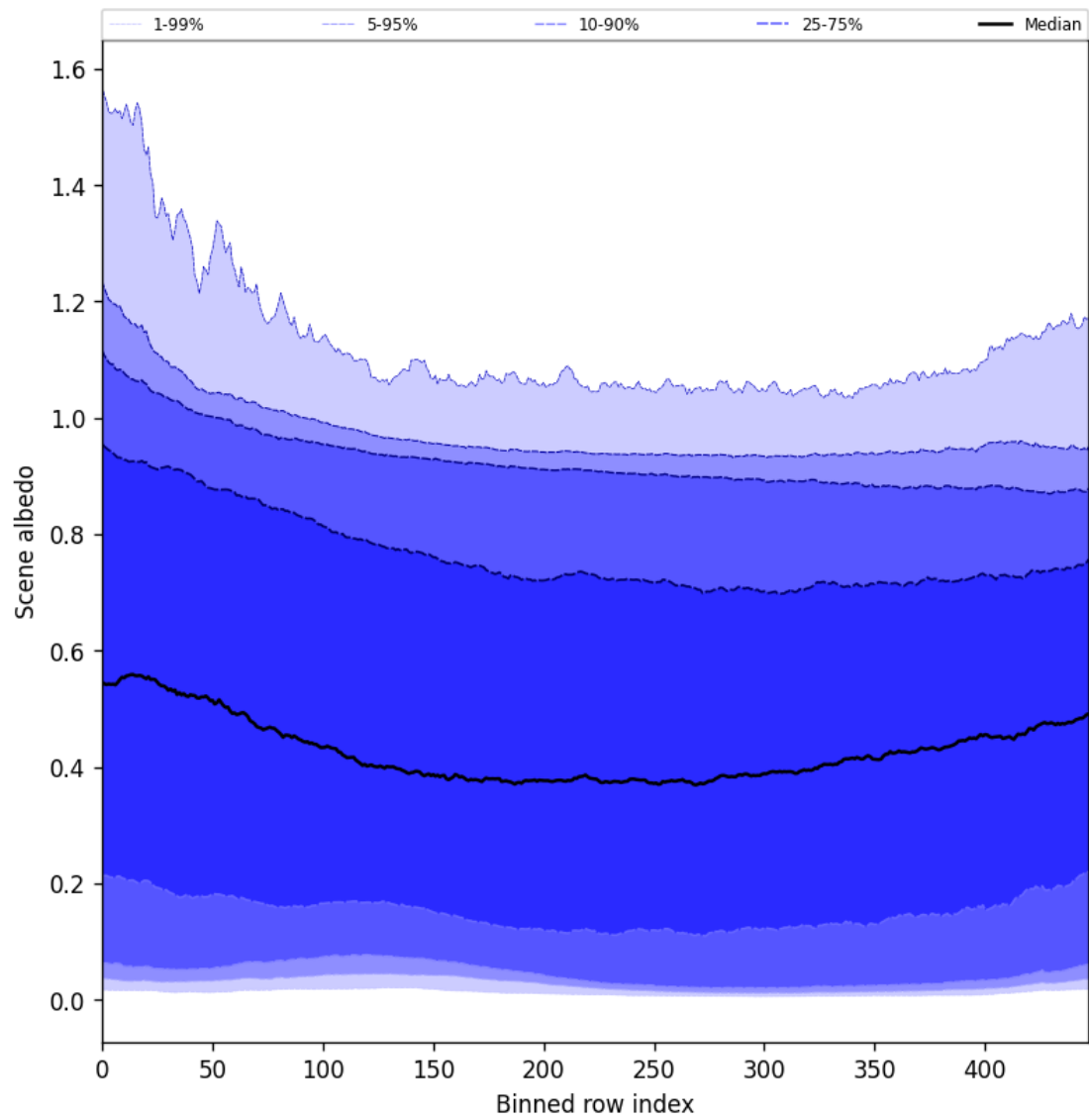
Figure 49: Along track statistics of “Scene albedo” for 2025-11-03 to 2025-11-04
