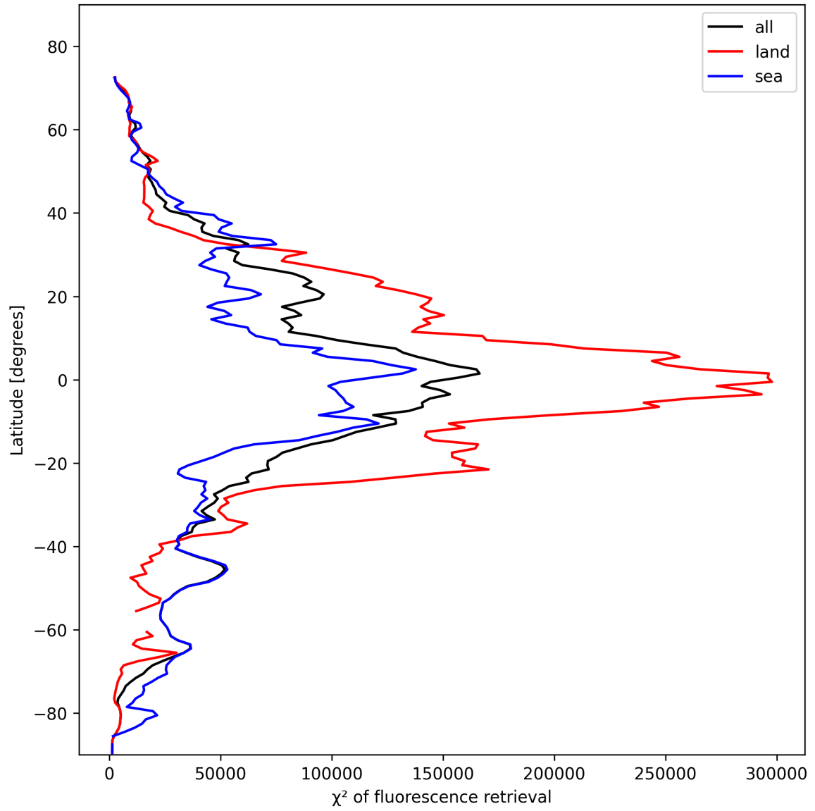
Figure 23: Zonal average of “ \chi^2 of fluorescence retrieval” for 2025-11-03 to 2025-11-04.
