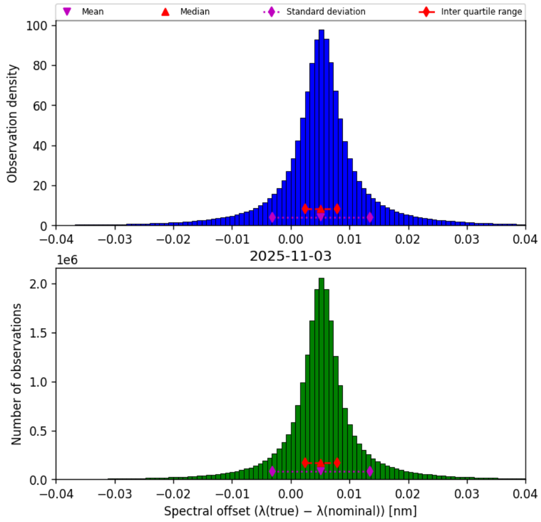
Figure 43: Histogram of “Spectral offset ( \lambda_{\text{true}} - \lambda_{\text{nominal}} )” for 2025-11-03 to 2025-11-04
