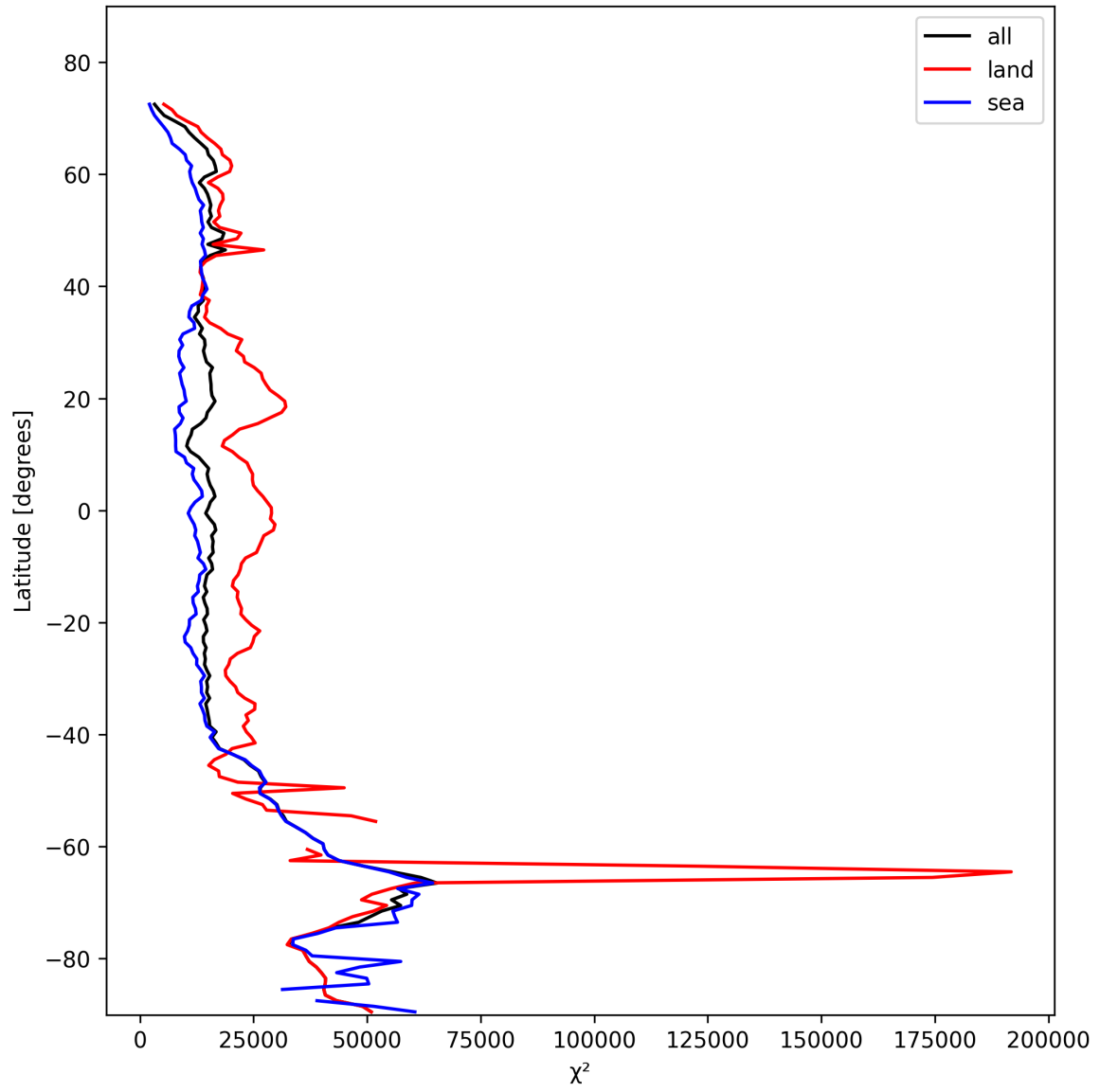
Figure 19: Zonal average of “ \chi^2 ” for 2025-11-03 to 2025-11-04.
