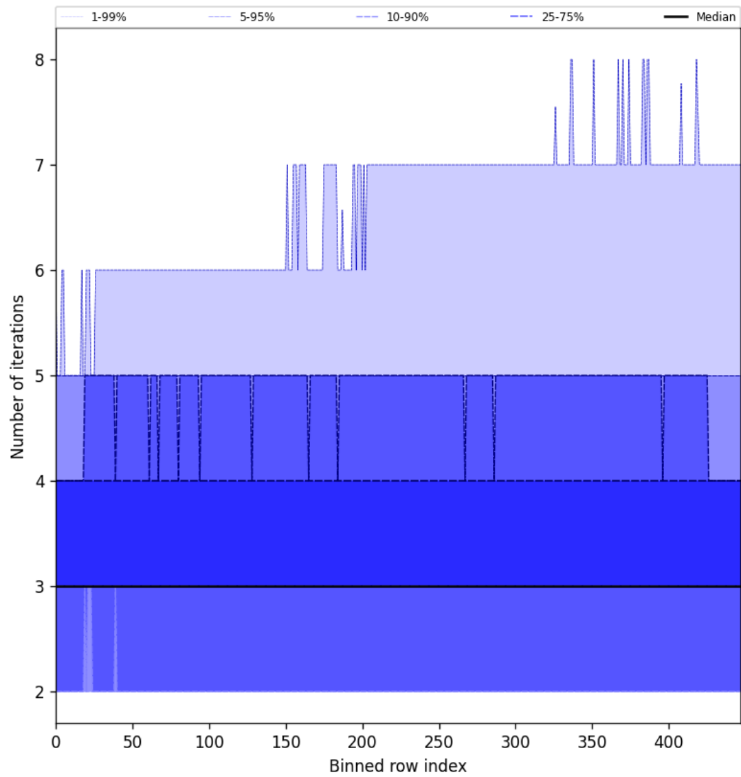
Figure 54: Along track statistics of “Number of iterations” for 2025-11-03 to 2025-11-04
