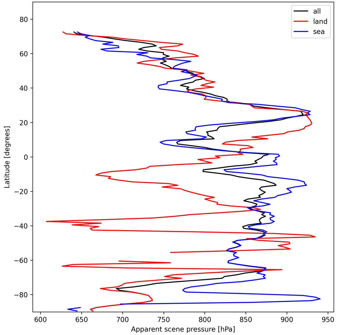
Figure 17: Zonal average of “Apparent scene pressure” for 2025-11-03 to 2025-11-04.
