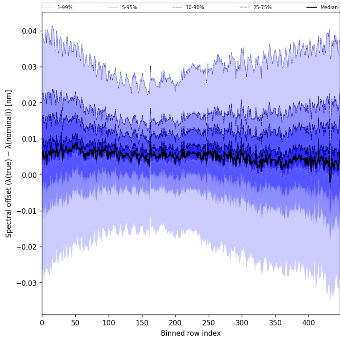
Figure 60: Along track statistics of “Spectral offset ( \lambda_{\text{true}} - \lambda_{\text{nominal}} )” for 2025-11-03 to 2025-11-04
