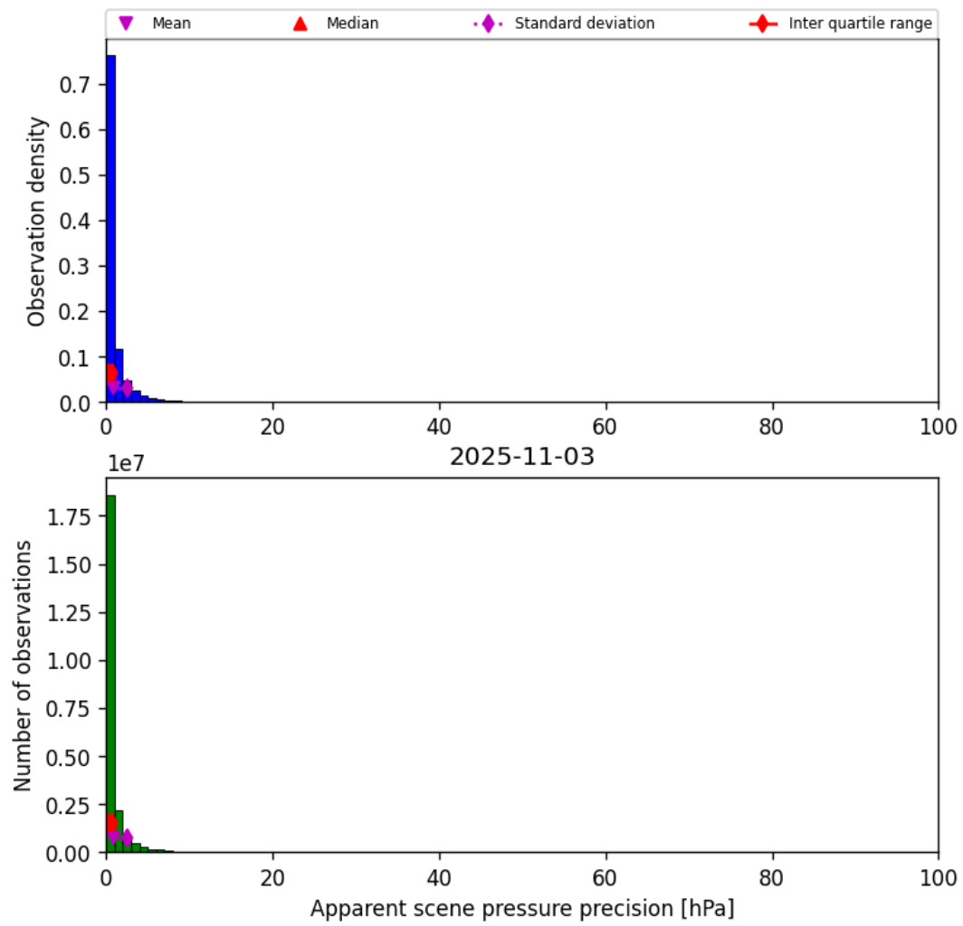
Figure 35: Histogram of “Apparent scene pressure precision” for 2025-11-03 to 2025-11-04
