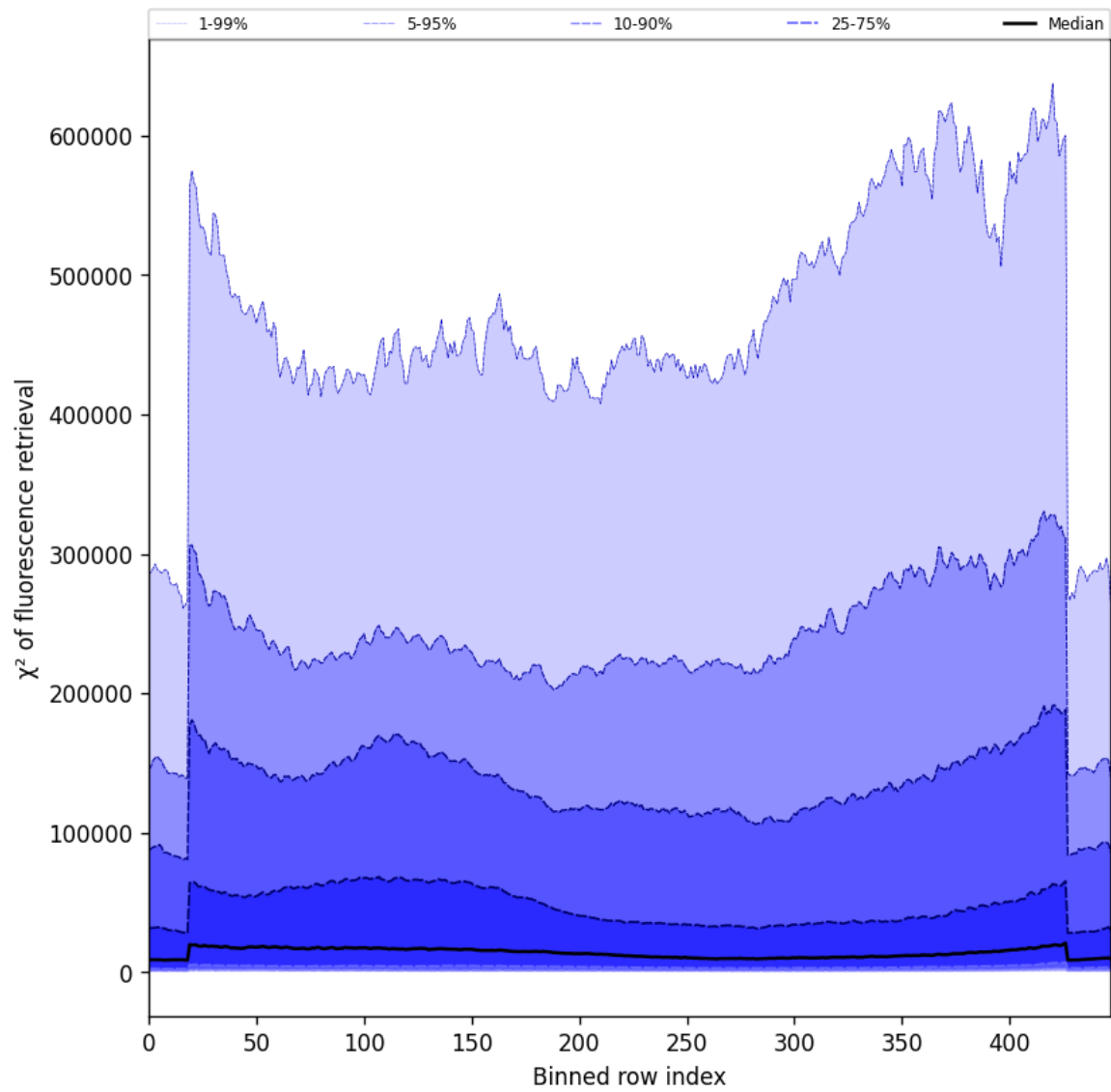
Figure 57: Along track statistics of “ \chi^2 of fluorescence retrieval” for 2025-11-03 to 2025-11-04
