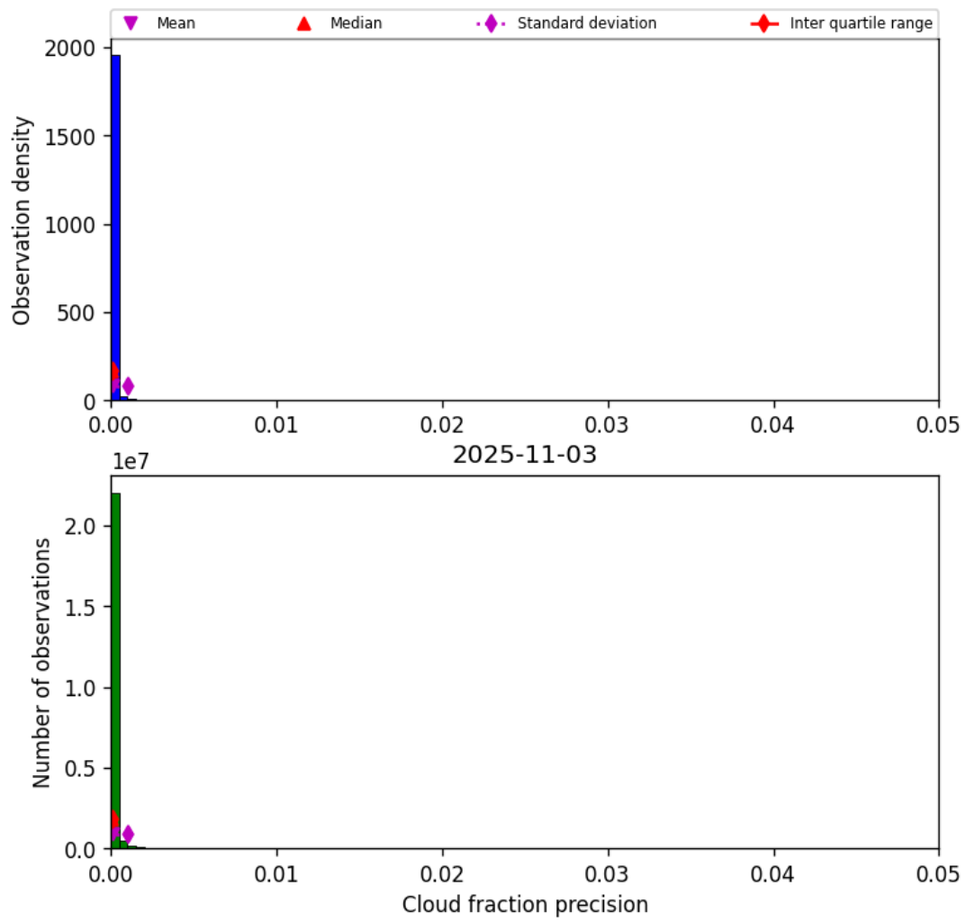
Figure 31: Histogram of “Cloud fraction precision” for 2025-11-03 to 2025-11-04
