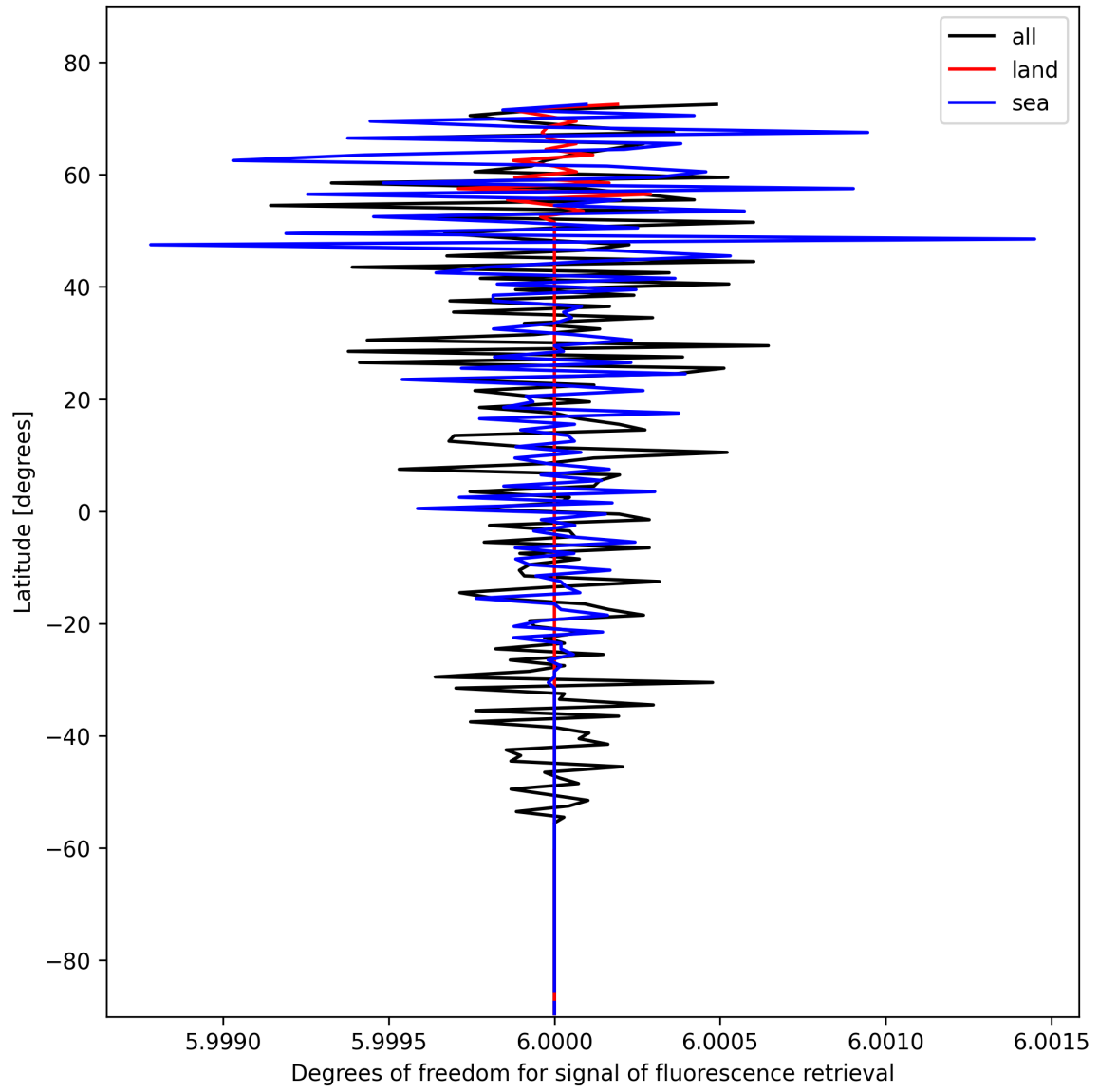
Figure 24: Zonal average of “Degrees of freedom for signal of fluorescence retrieval” for 2025-11-03 to 2025-11-04.
