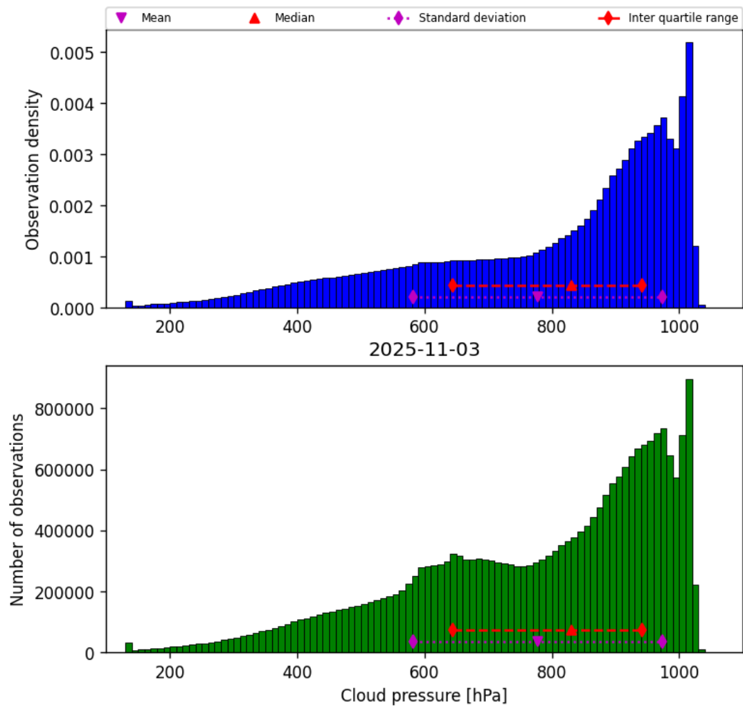
Figure 28: Histogram of “Cloud pressure” for 2025-11-03 to 2025-11-04
