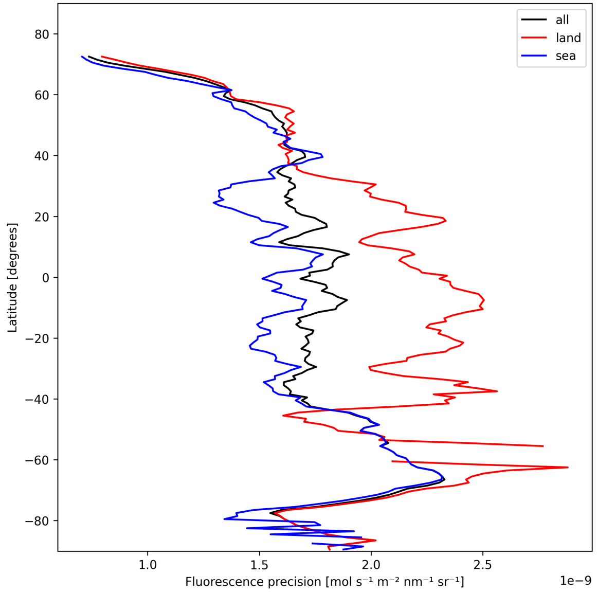
Figure 22: Zonal average of “Fluorescence precision” for 2025-11-03 to 2025-11-04.
