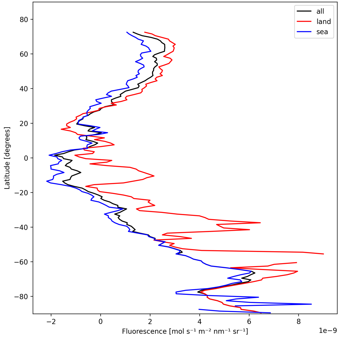
Figure 21: Zonal average of “Fluorescence” for 2025-11-03 to 2025-11-04.
