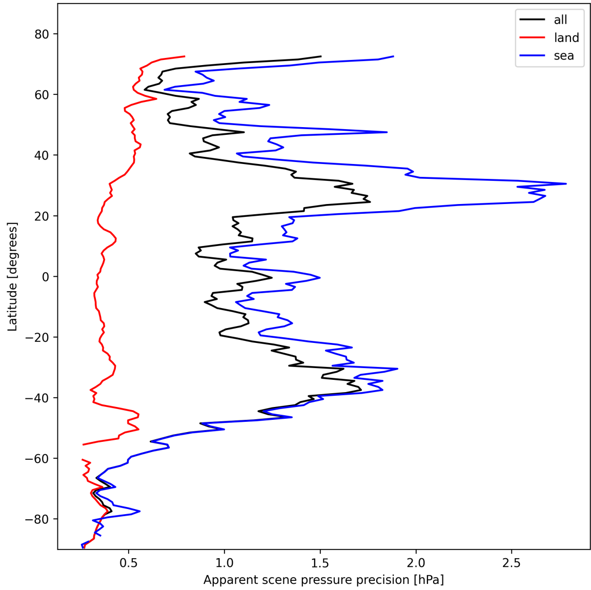
Figure 18: Zonal average of “Apparent scene pressure precision” for 2025-11-03 to 2025-11-04.
