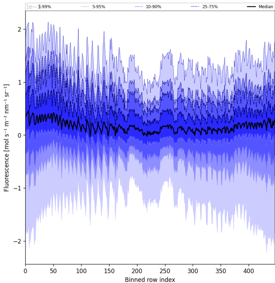
Figure 55: Along track statistics of “Fluorescence” for 2025-11-03 to 2025-11-04
