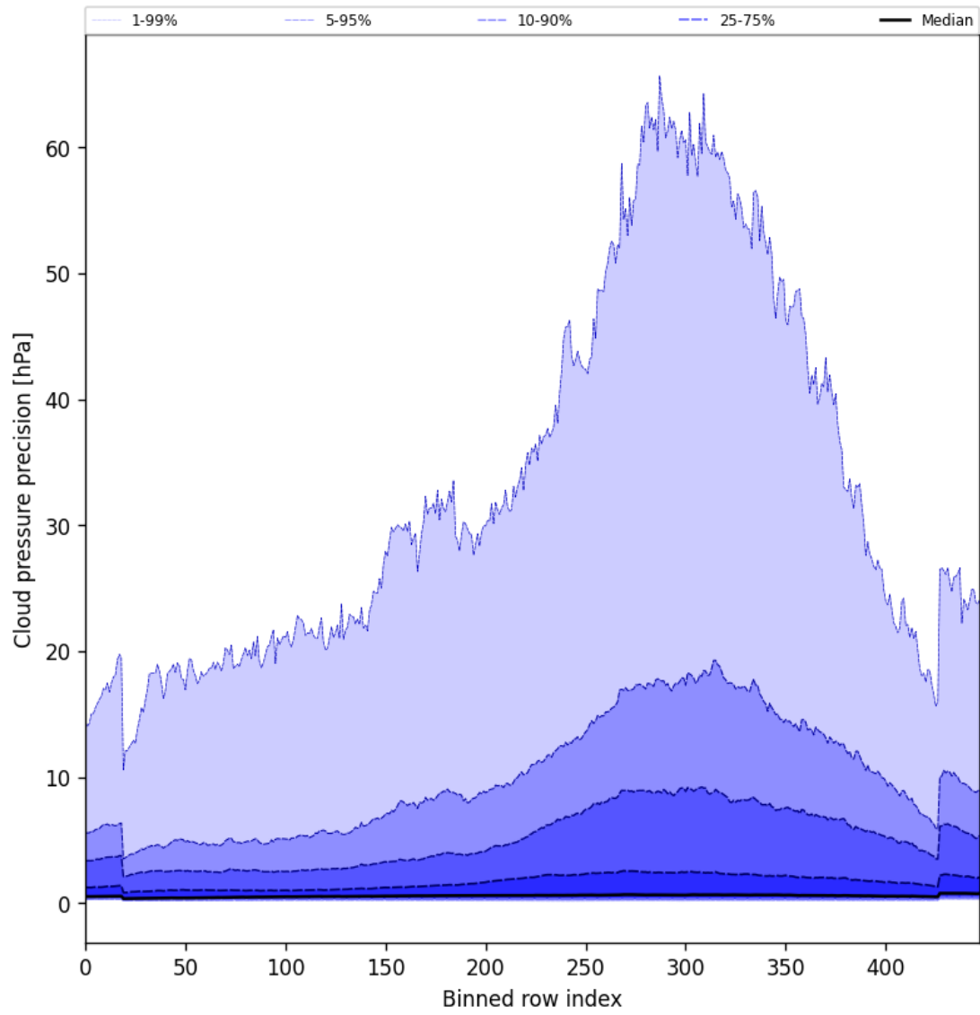
Figure 46: Along track statistics of “Cloud pressure precision” for 2025-11-03 to 2025-11-04
