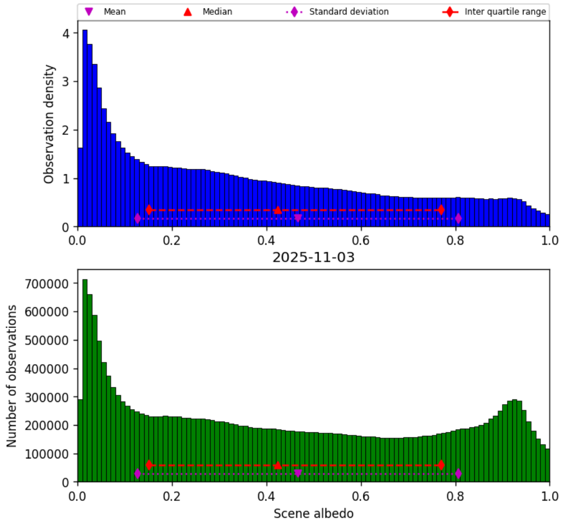
Figure 32: Histogram of “Scene albedo” for 2025-11-03 to 2025-11-04
