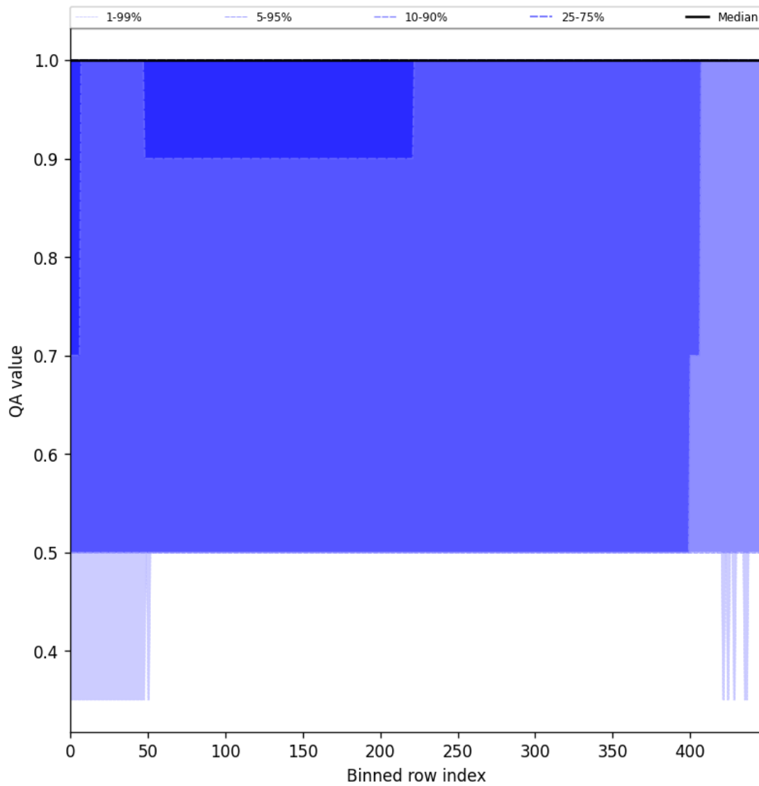
Figure 44: Along track statistics of “QA value” for 2025-11-04 to 2025-11-05
