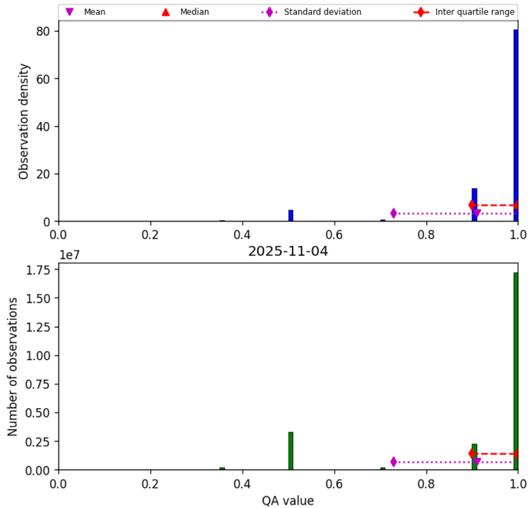
Figure 27: Histogram of “QA value” for 2025-11-04 to 2025-11-05
