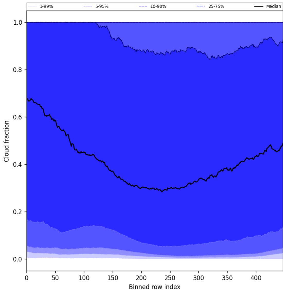
Figure 47: Along track statistics of “Cloud fraction” for 2025-11-04 to 2025-11-05
