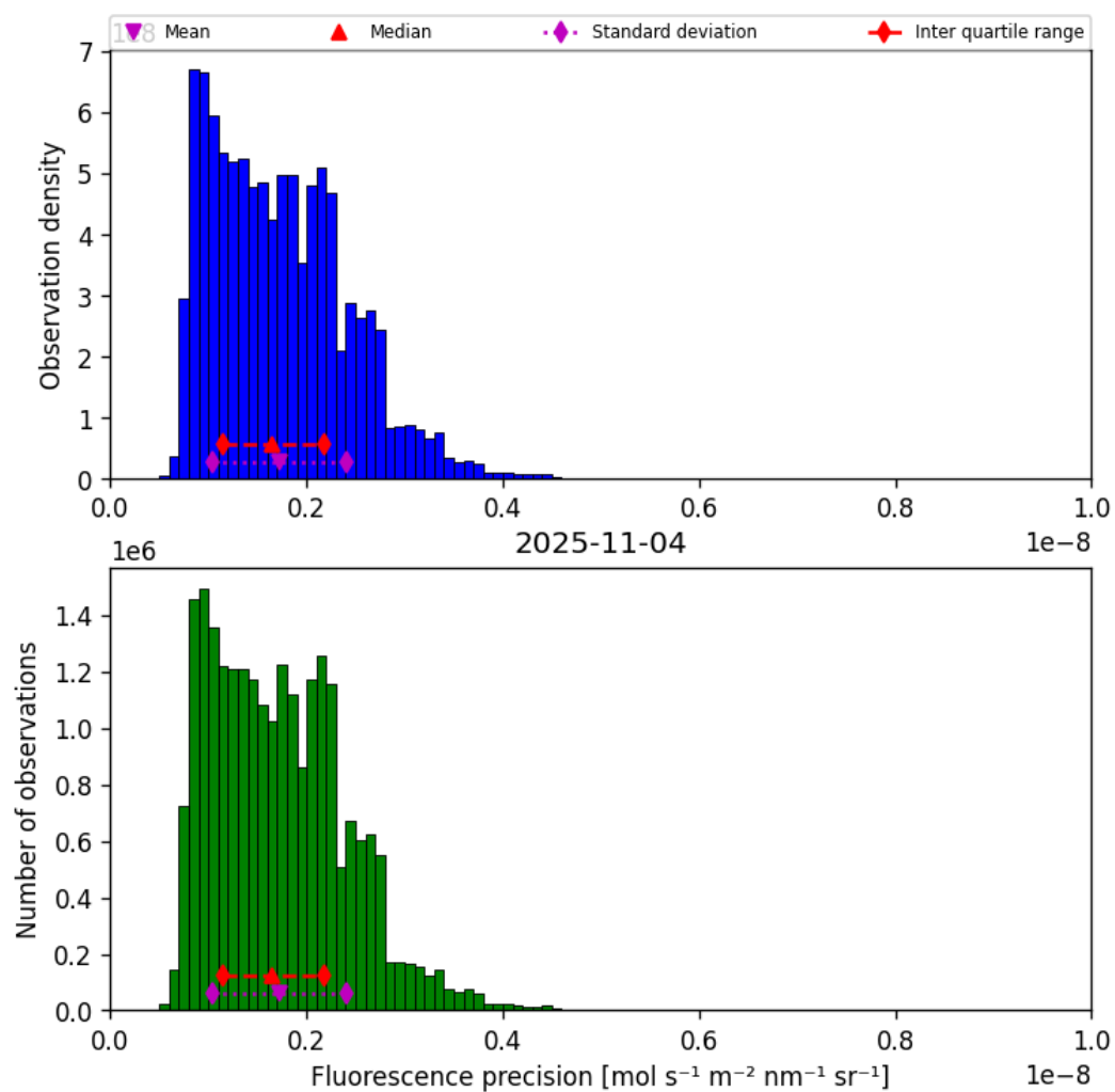
Figure 39: Histogram of “Fluorescence precision” for 2025-11-04 to 2025-11-05
