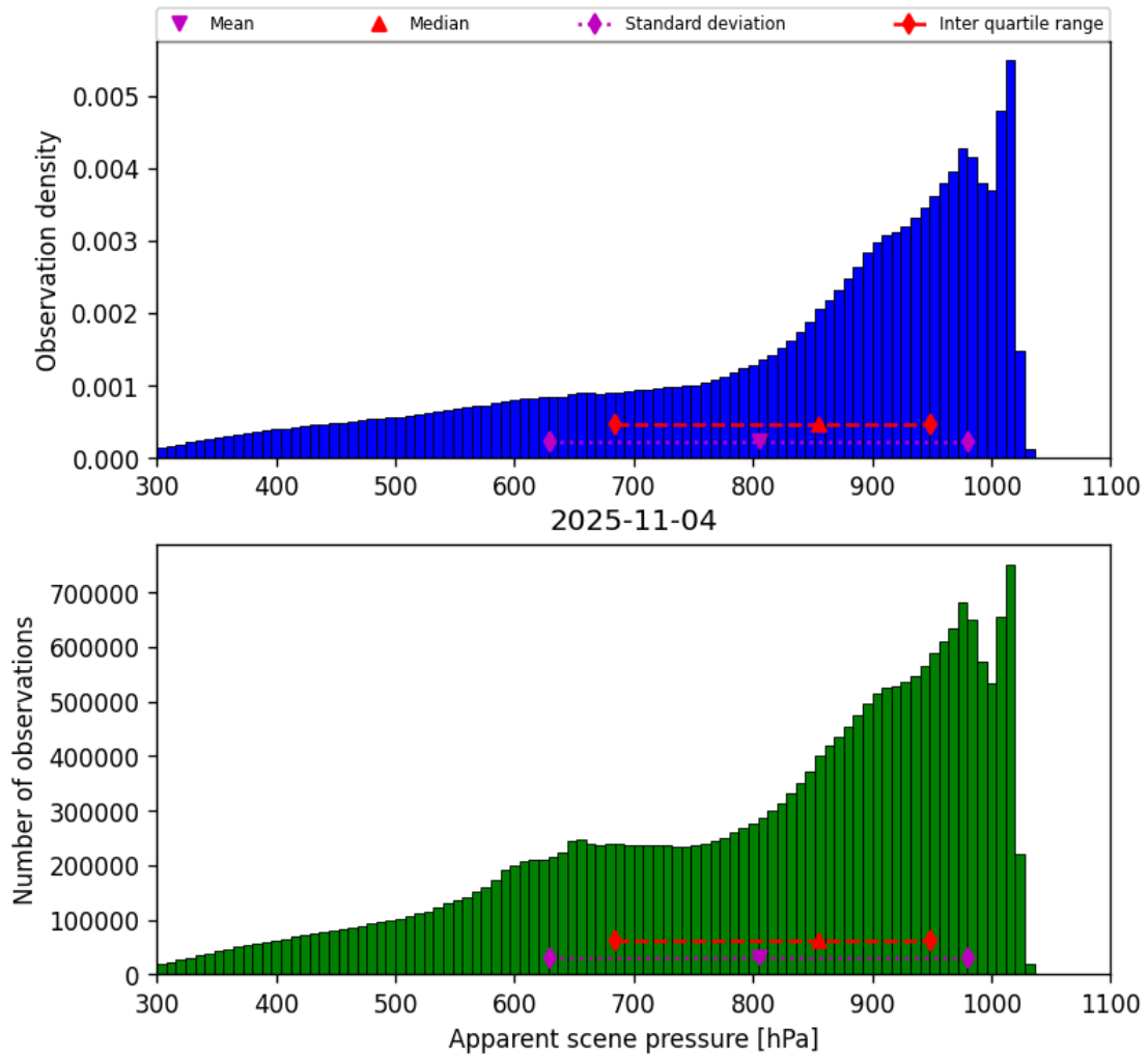
Figure 34: Histogram of “Apparent scene pressure” for 2025-11-04 to 2025-11-05
