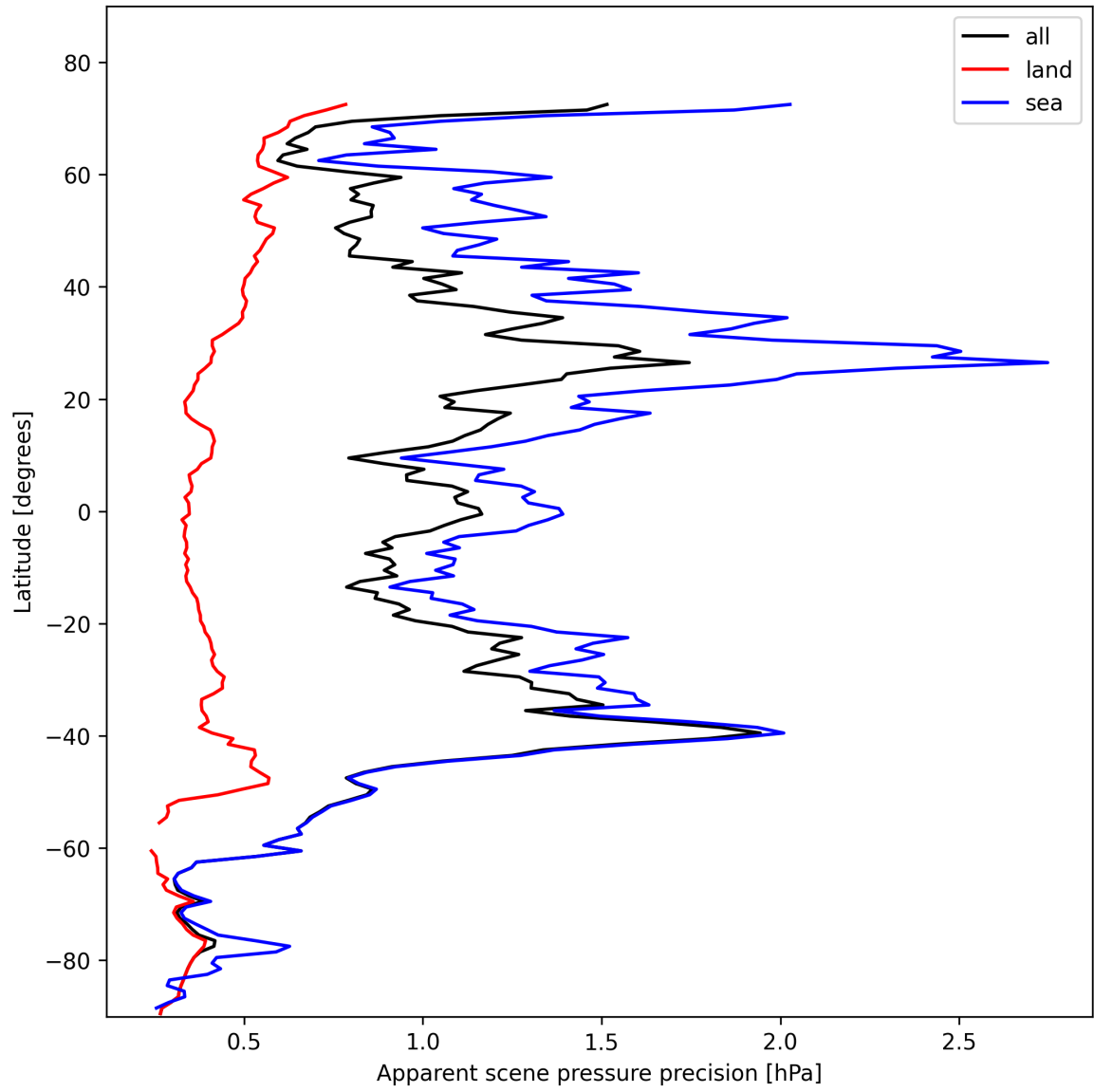
Figure 18: Zonal average of “Apparent scene pressure precision” for 2025-11-04 to 2025-11-05.
