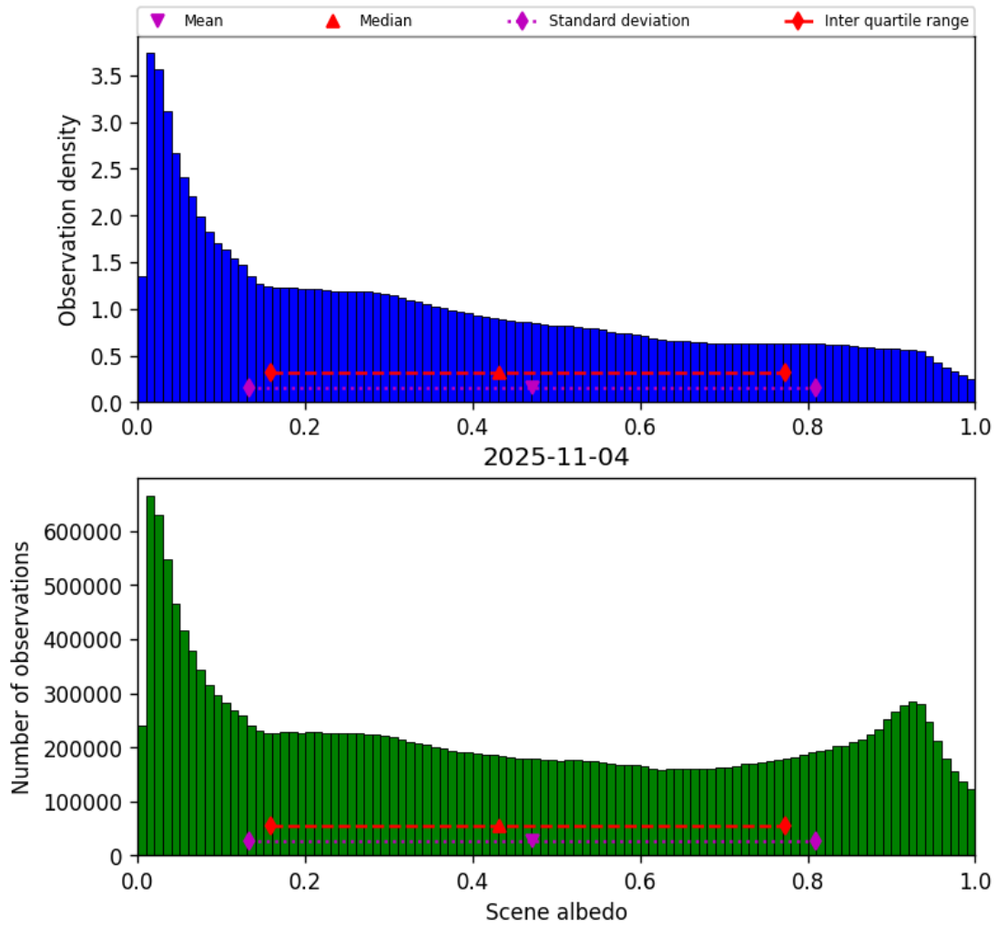
Figure 32: Histogram of “Scene albedo” for 2025-11-04 to 2025-11-05
