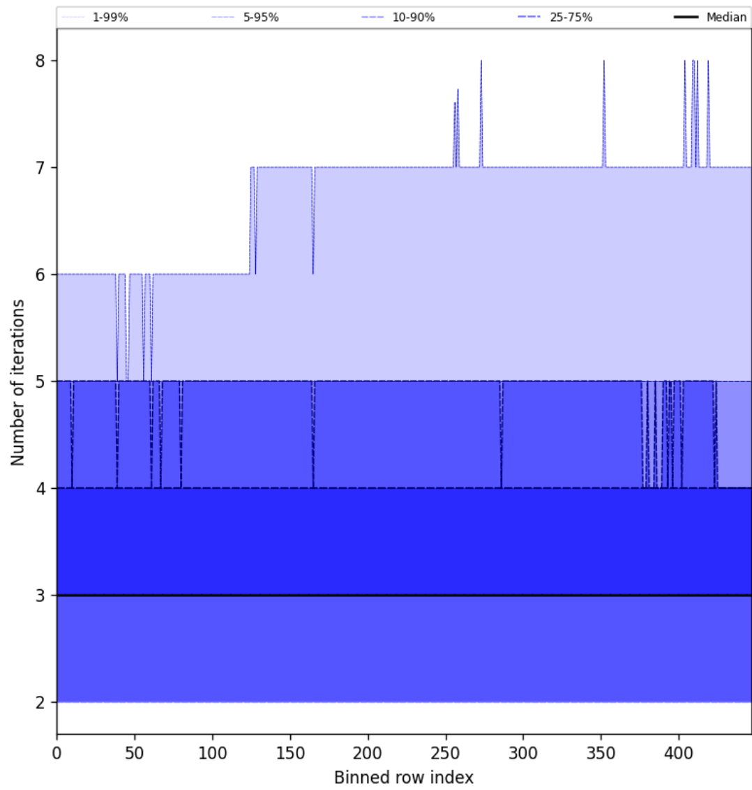
Figure 54: Along track statistics of “Number of iterations” for 2025-11-04 to 2025-11-05
