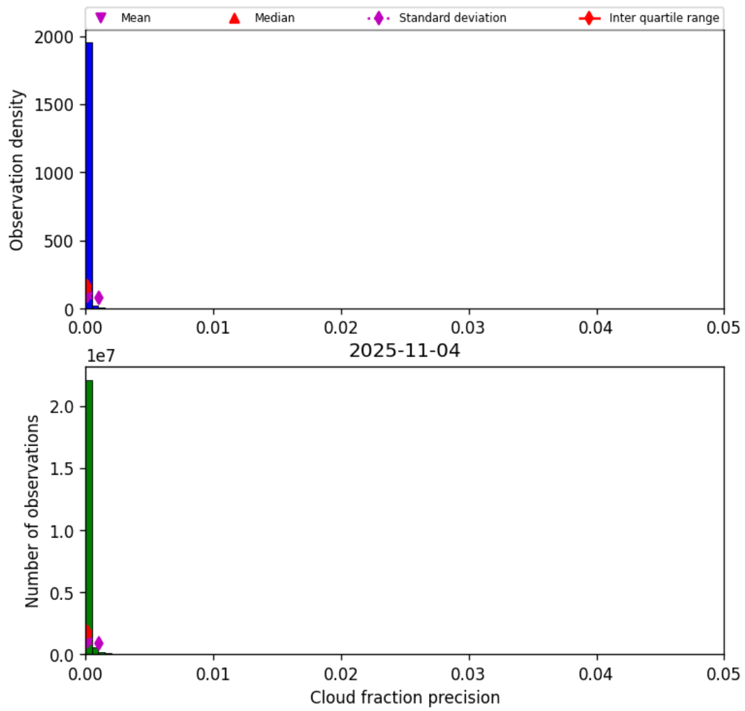
Figure 31: Histogram of “Cloud fraction precision” for 2025-11-04 to 2025-11-05
