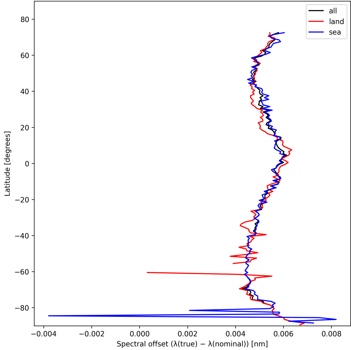
Figure 26: Zonal average of “Spectral offset ( \lambda_{\text{true}} - \lambda_{\text{nominal}} )” for 2025-11-04 to 2025-11-05.
